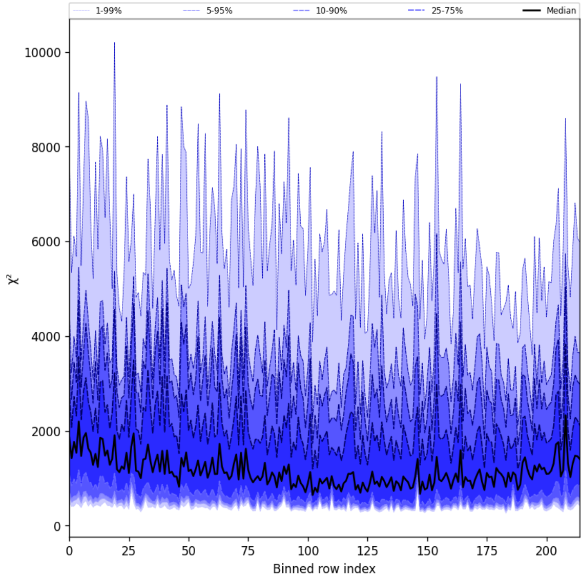
Figure 24: Along track statistics of “ \chi^2 ” for 2025-01-10 to 2025-01-10
