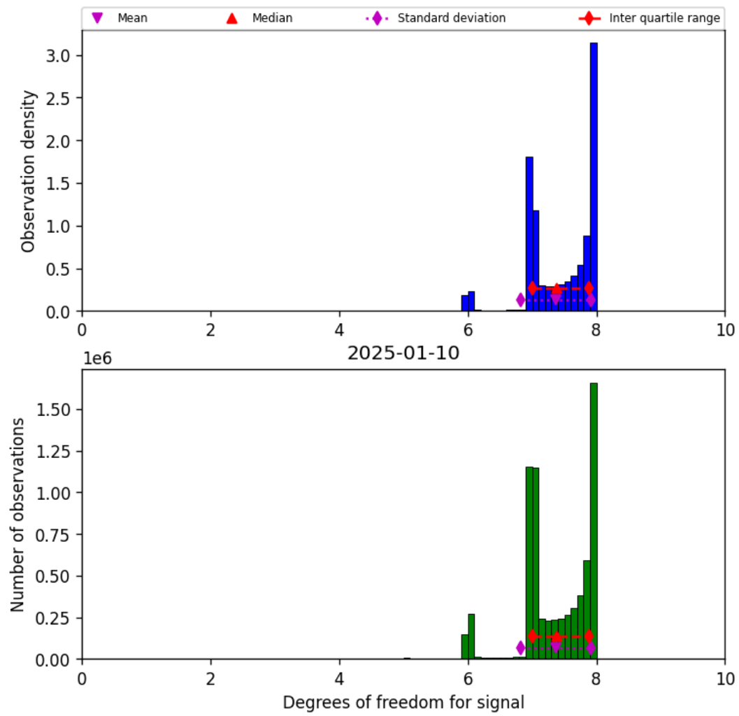
Figure 18: Histogram of “Degrees of freedom for signal” for 2025-01-10 to 2025-01-10
