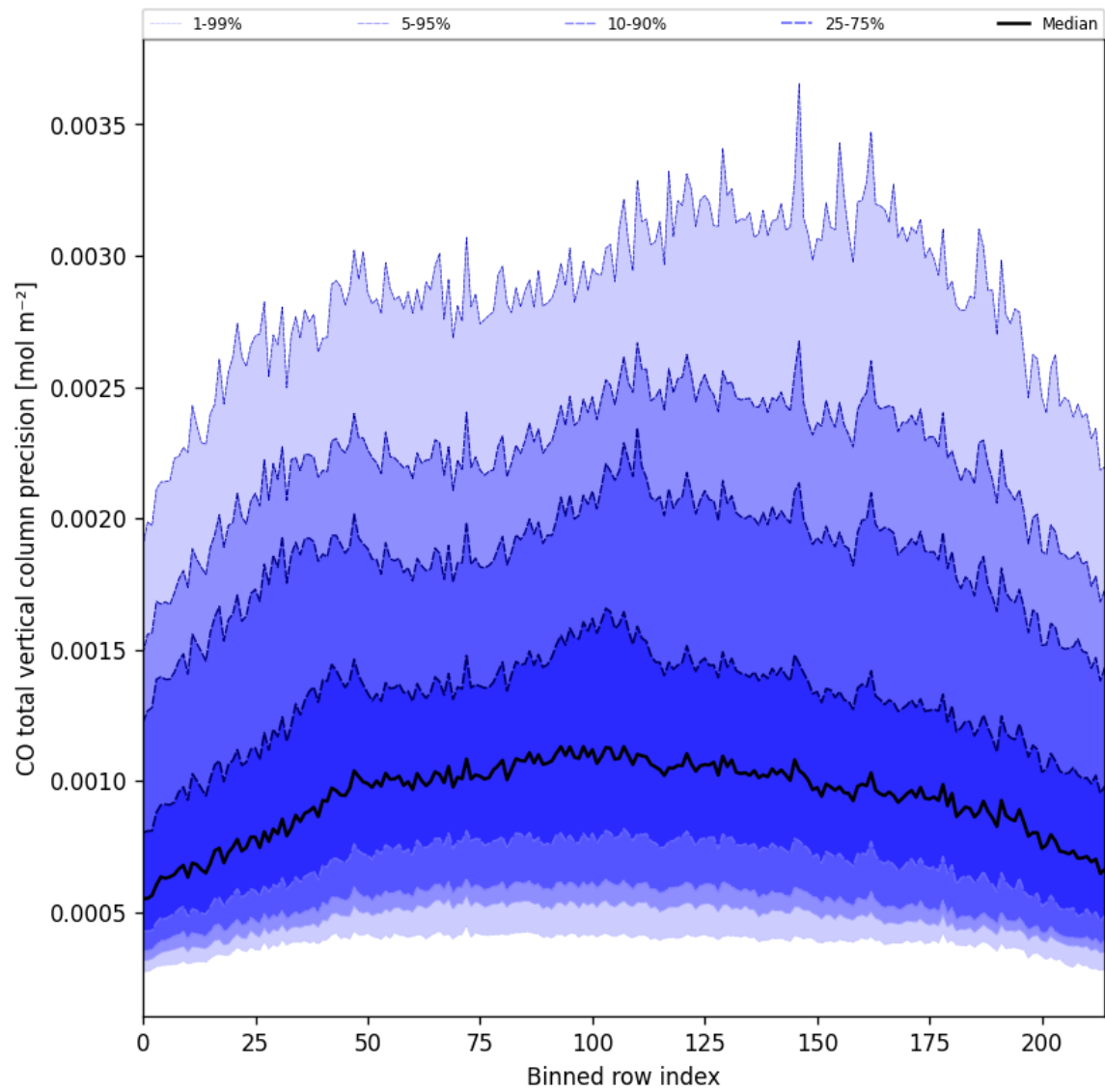
Figure 22: Along track statistics of “CO total vertical column precision” for 2025-01-10 to 2025-01-10
