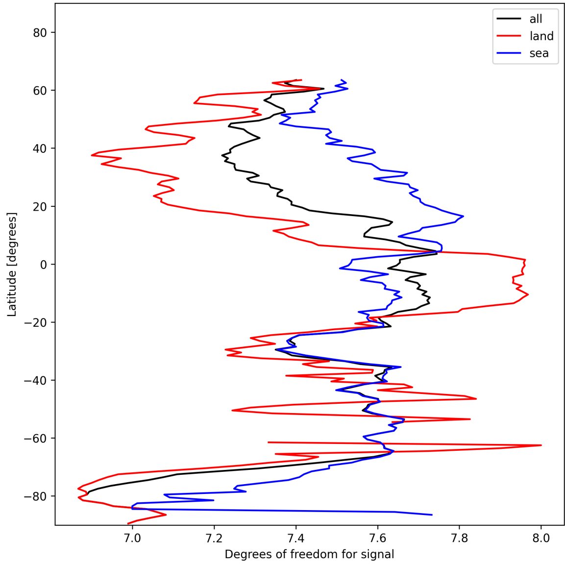
Figure 11: Zonal average of “Degrees of freedom for signal” for 2025-01-10 to 2025-01-10.
