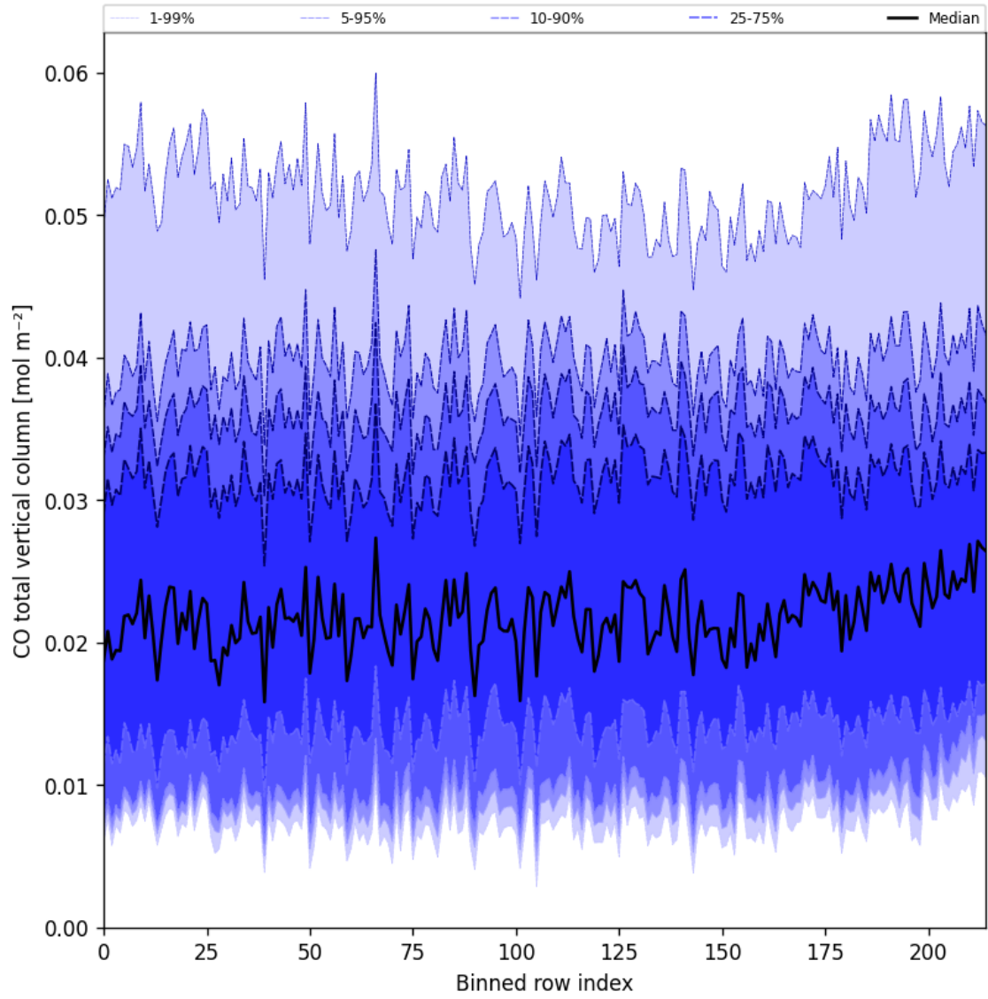
Figure 21: Along track statistics of “CO total vertical column” for 2025-01-10 to 2025-01-10
