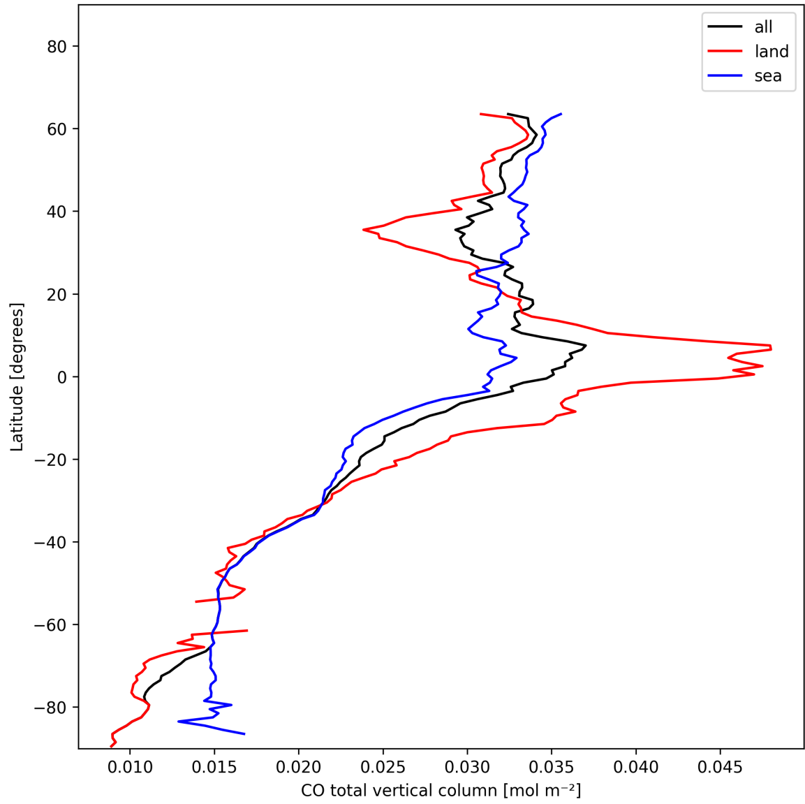
Figure 7: Zonal average of “CO total vertical column” for 2025-01-10 to 2025-01-10.
