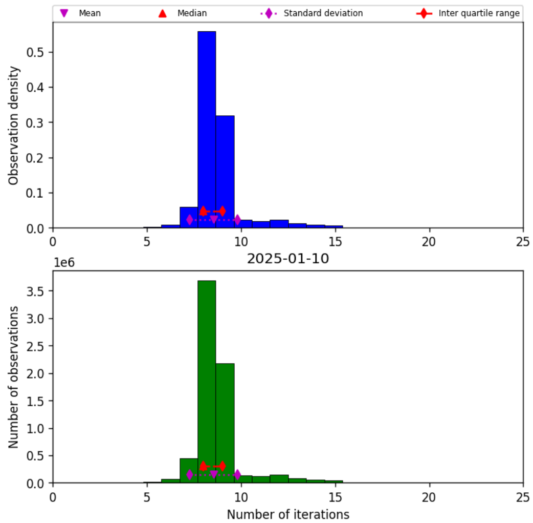
Figure 19: Histogram of “Number of iterations” for 2025-01-10 to 2025-01-10
