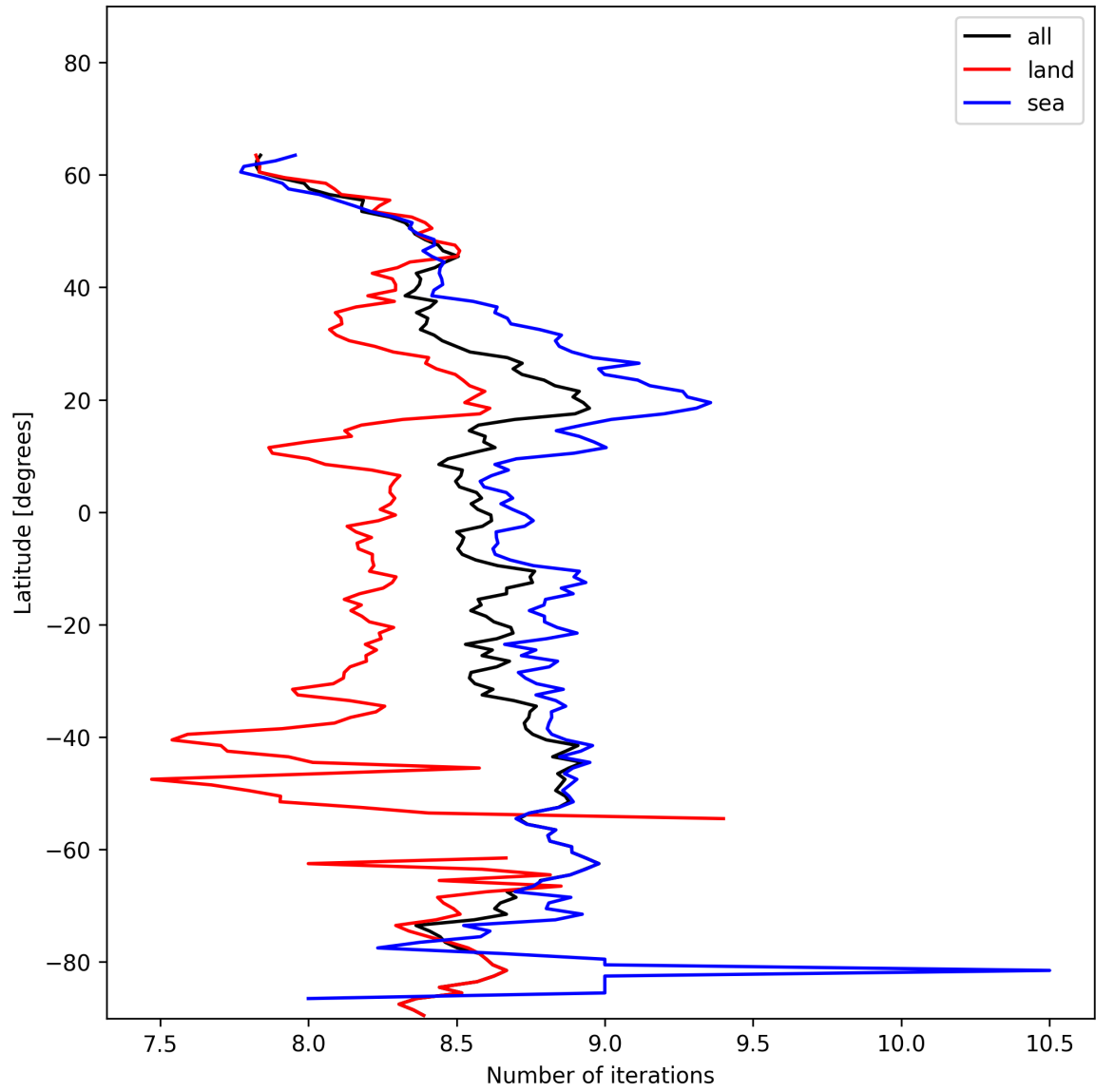
Figure 12: Zonal average of “Number of iterations” for 2025-01-10 to 2025-01-10.
