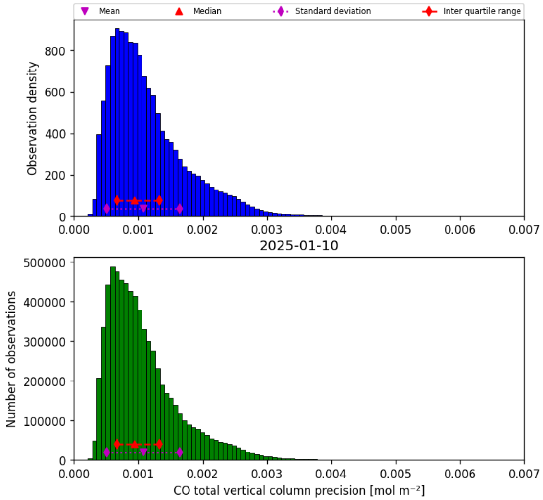
Figure 15: Histogram of “CO total vertical column precision” for 2025-01-10 to 2025-01-10
