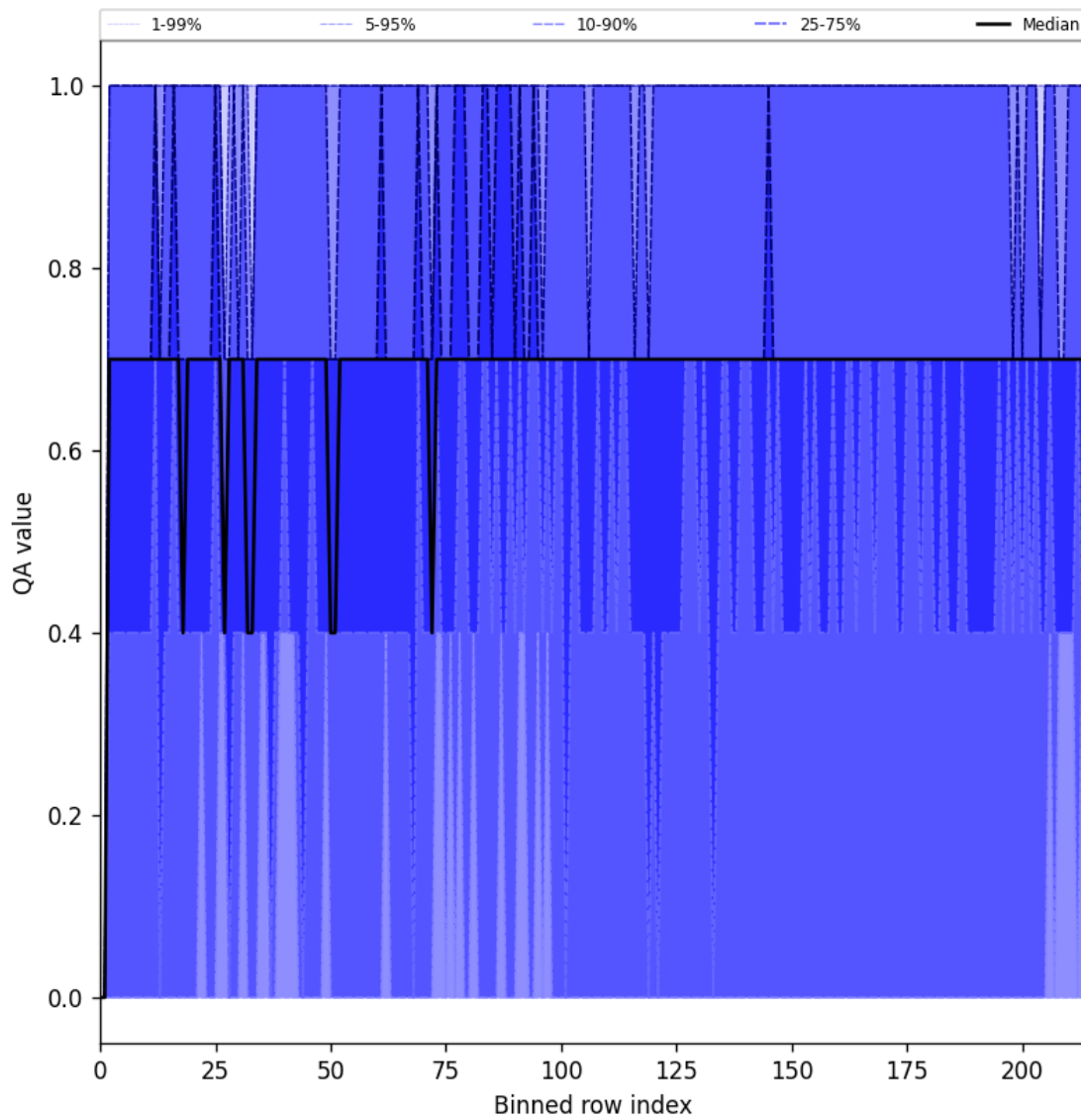
Figure 20: Along track statistics of “QA value” for 2025-01-10 to 2025-01-10
