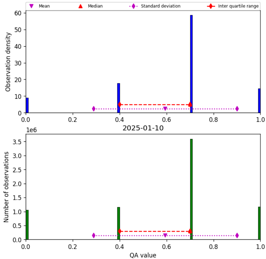
Figure 13: Histogram of “QA value” for 2025-01-10 to 2025-01-10
