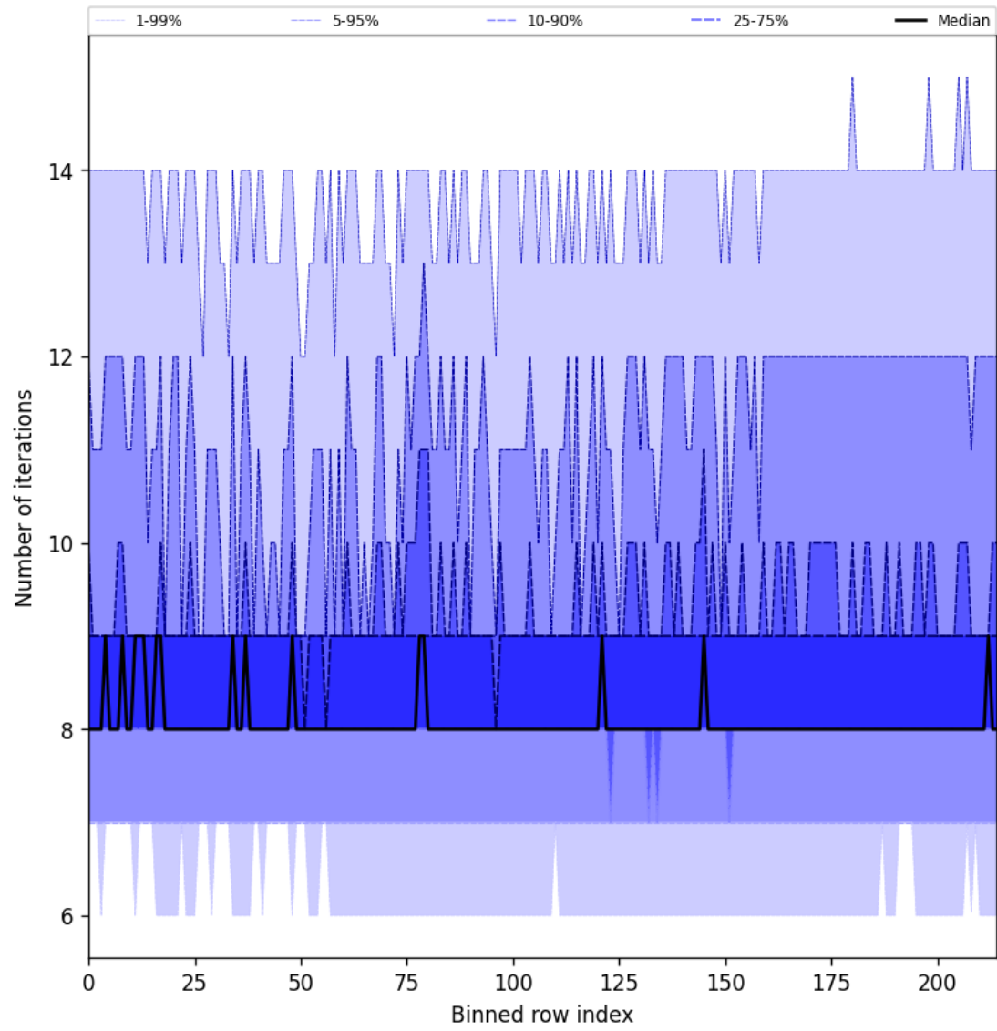
Figure 26: Along track statistics of “Number of iterations” for 2025-01-10 to 2025-01-10
