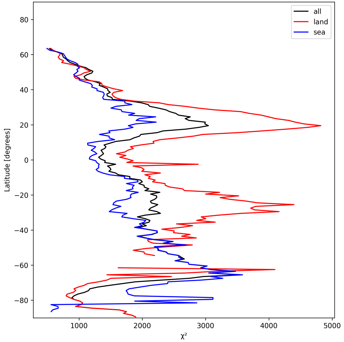
Figure 10: Zonal average of “ \chi^2 ” for 2025-01-10 to 2025-01-10.
