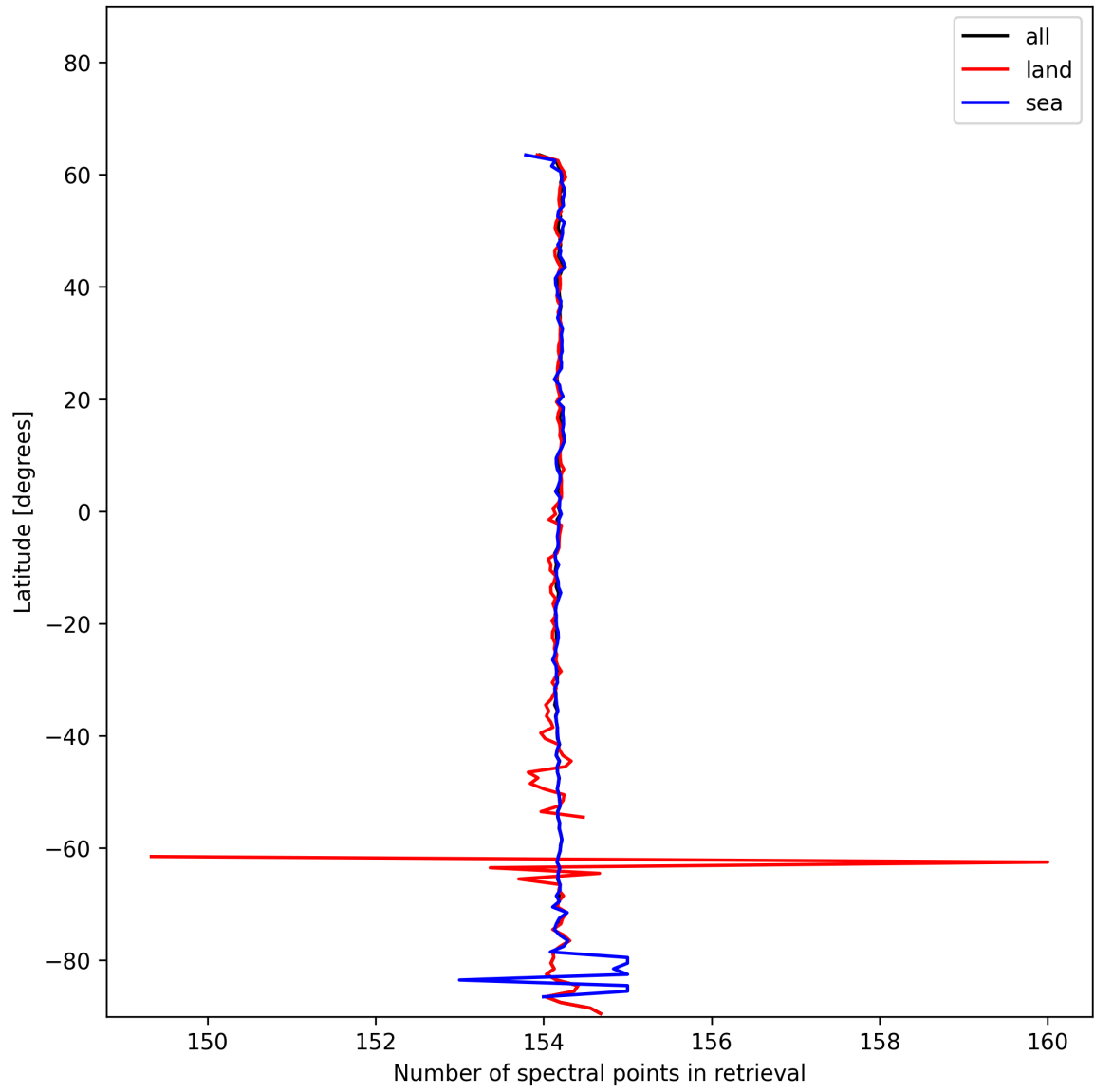
Figure 9: Zonal average of “Number of spectral points in retrieval” for 2025-01-10 to 2025-01-10.
