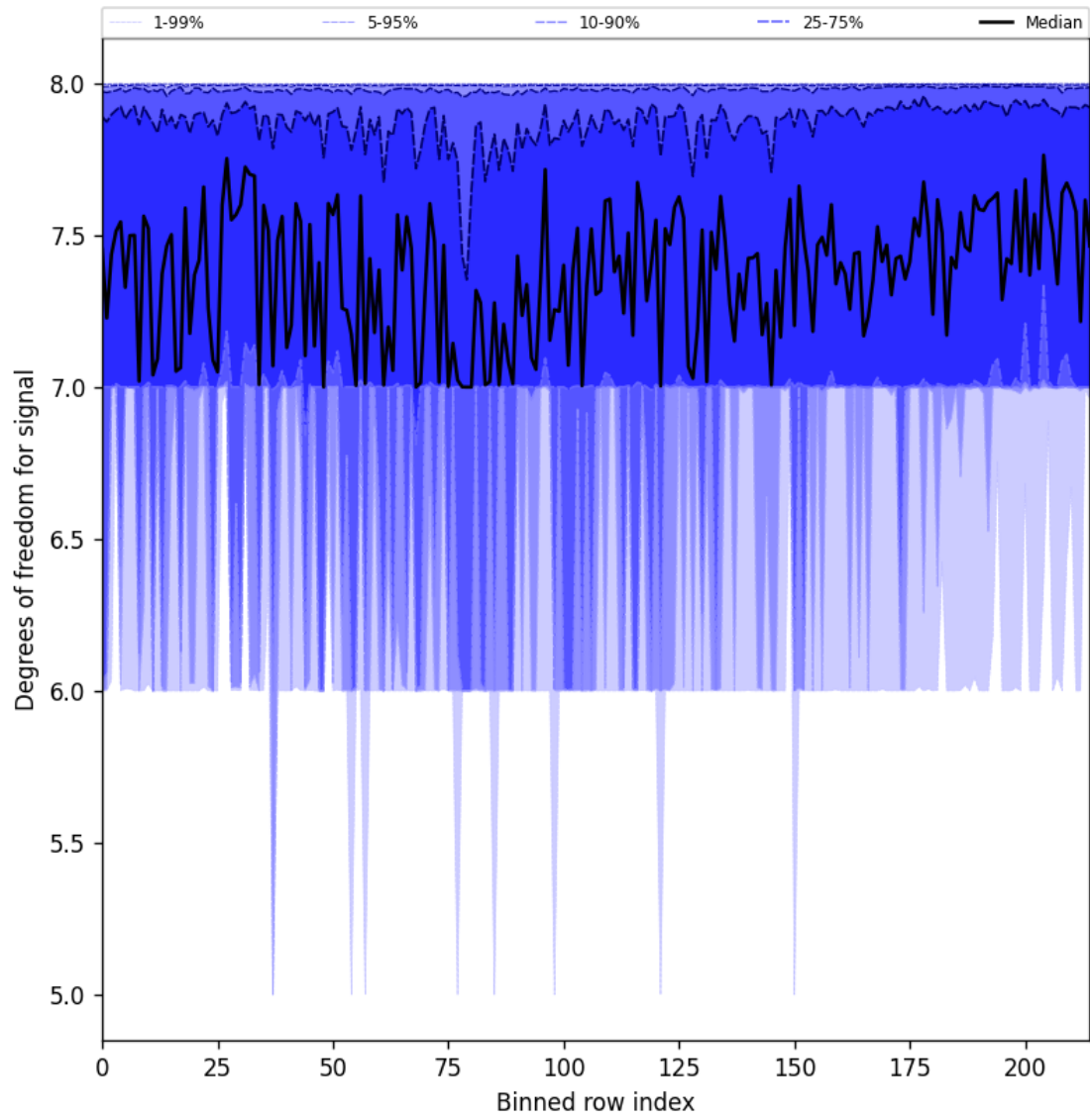
Figure 25: Along track statistics of “Degrees of freedom for signal” for 2025-01-10 to 2025-01-10
