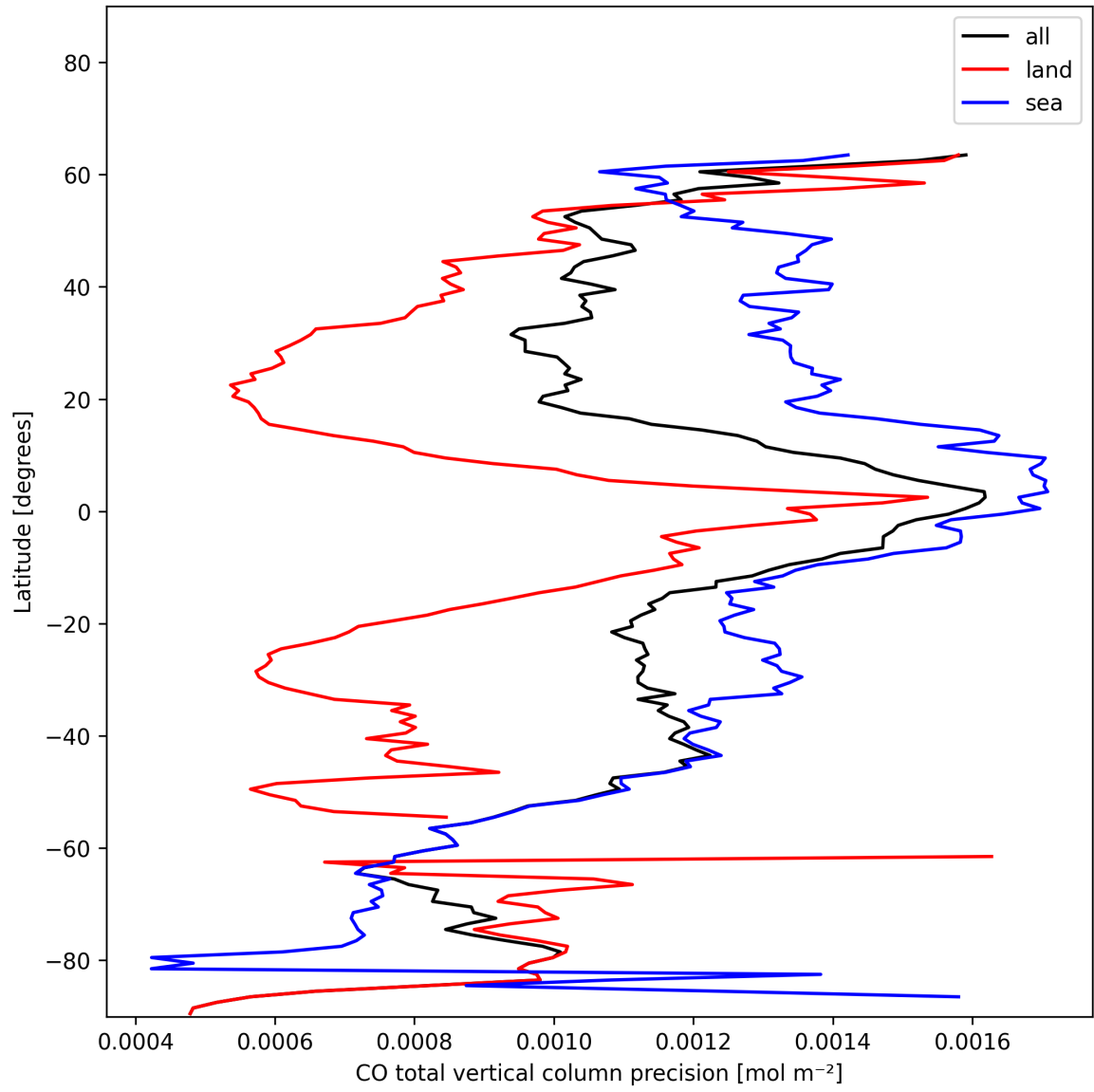
Figure 8: Zonal average of “CO total vertical column precision” for 2025-01-10 to 2025-01-10.
