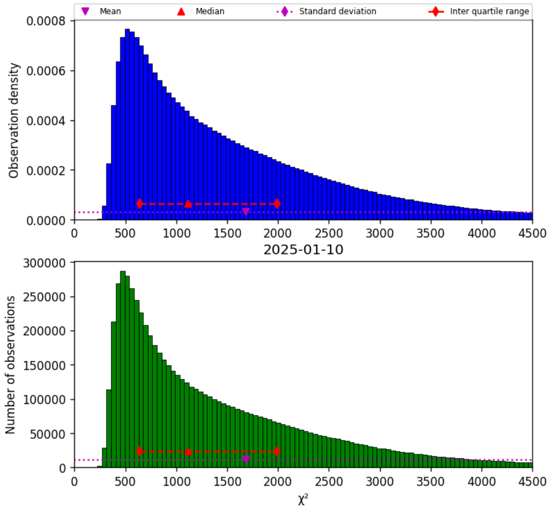
Figure 17: Histogram of " \chi^2 " for 2025-01-10 to 2025-01-10
