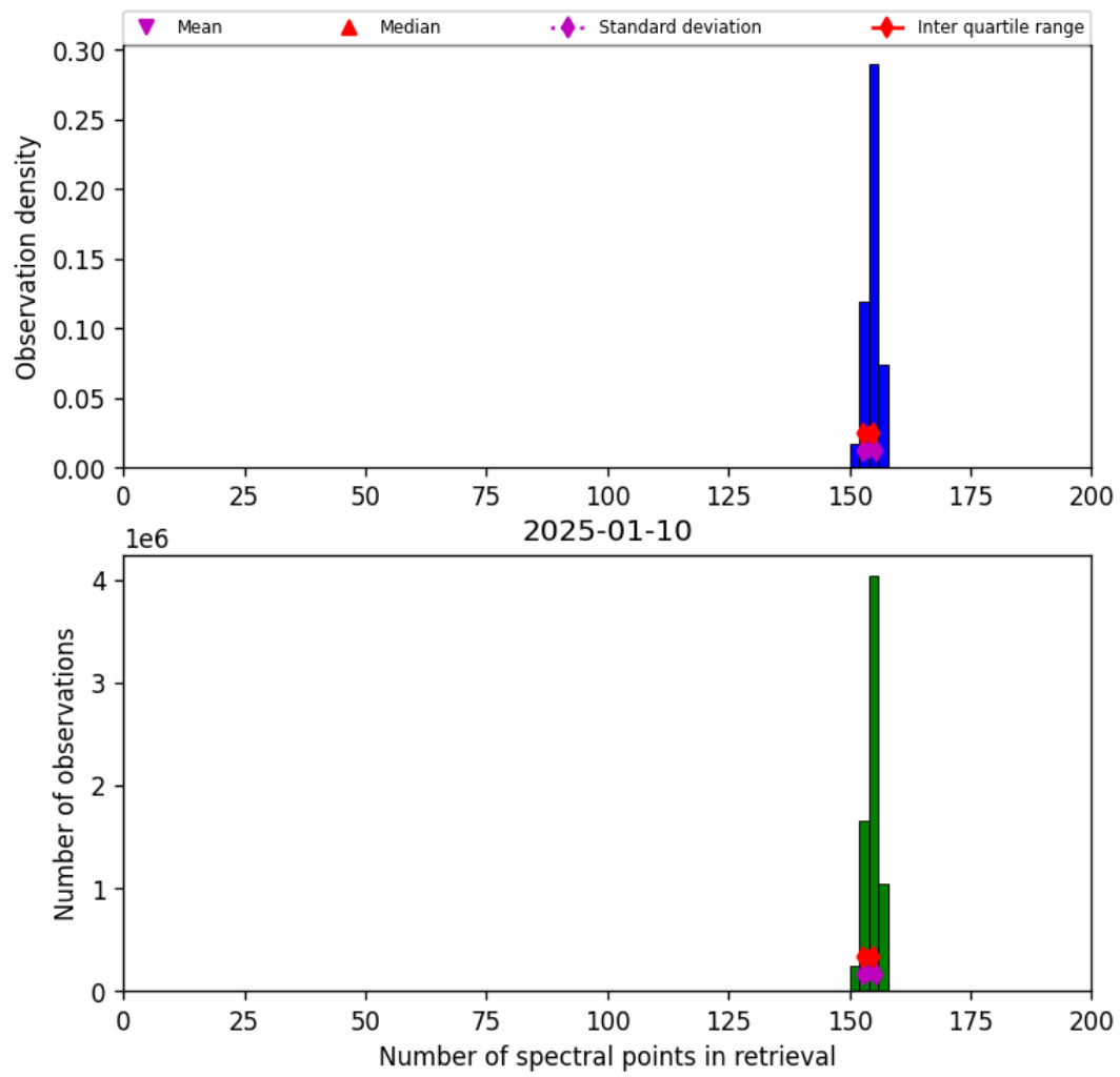
Figure 16: Histogram of “Number of spectral points in retrieval” for 2025-01-10 to 2025-01-10
