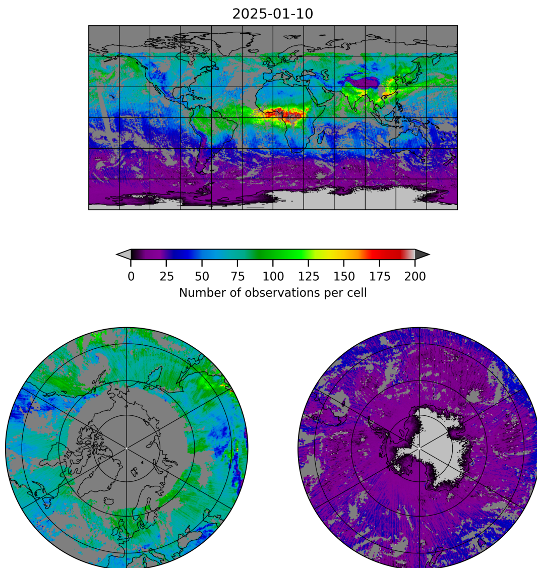
Figure 5: Map of the number of observations for 2025-01-10 to 2025-01-10
