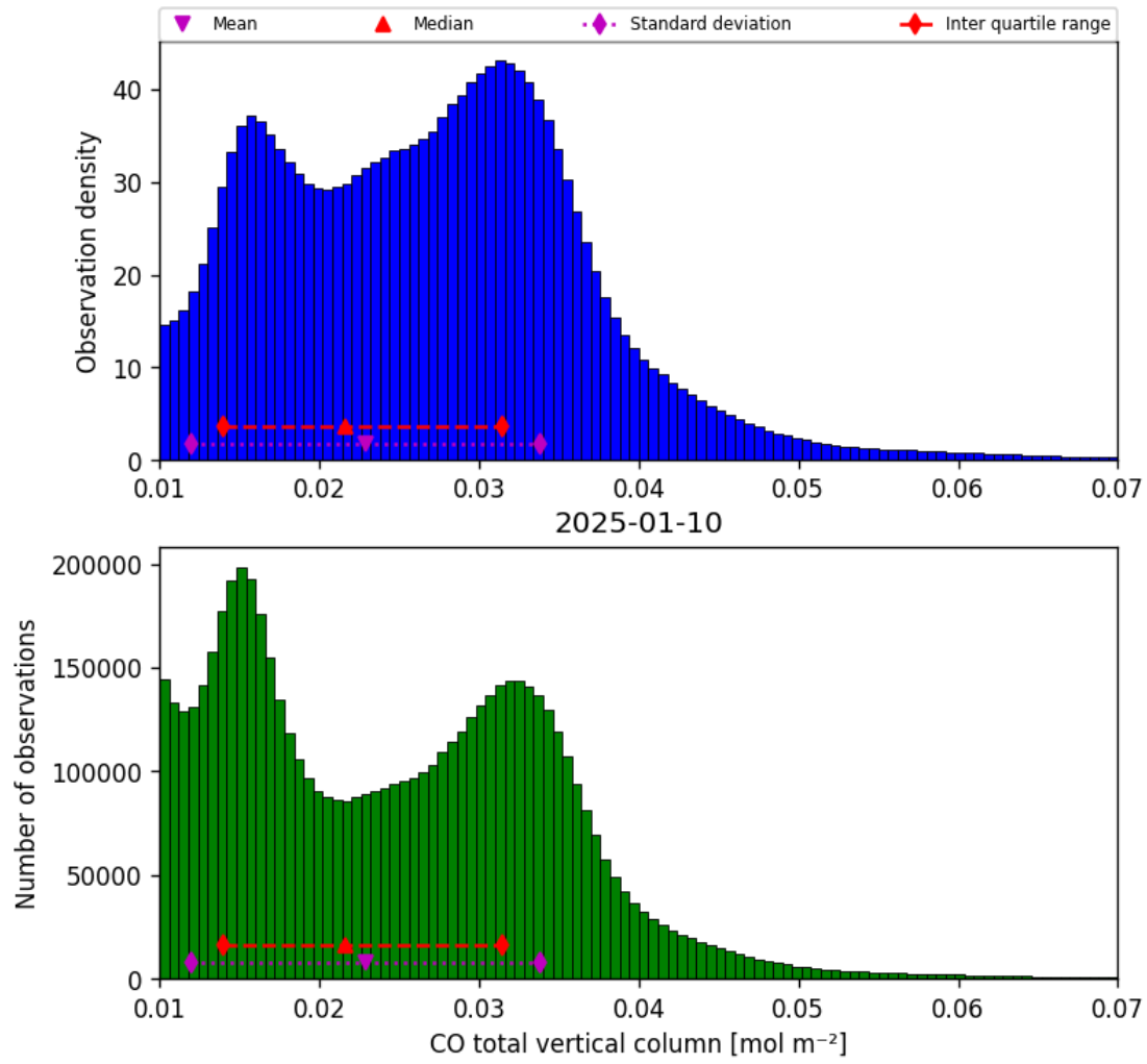
Figure 14: Histogram of “CO total vertical column” for 2025-01-10 to 2025-01-10
