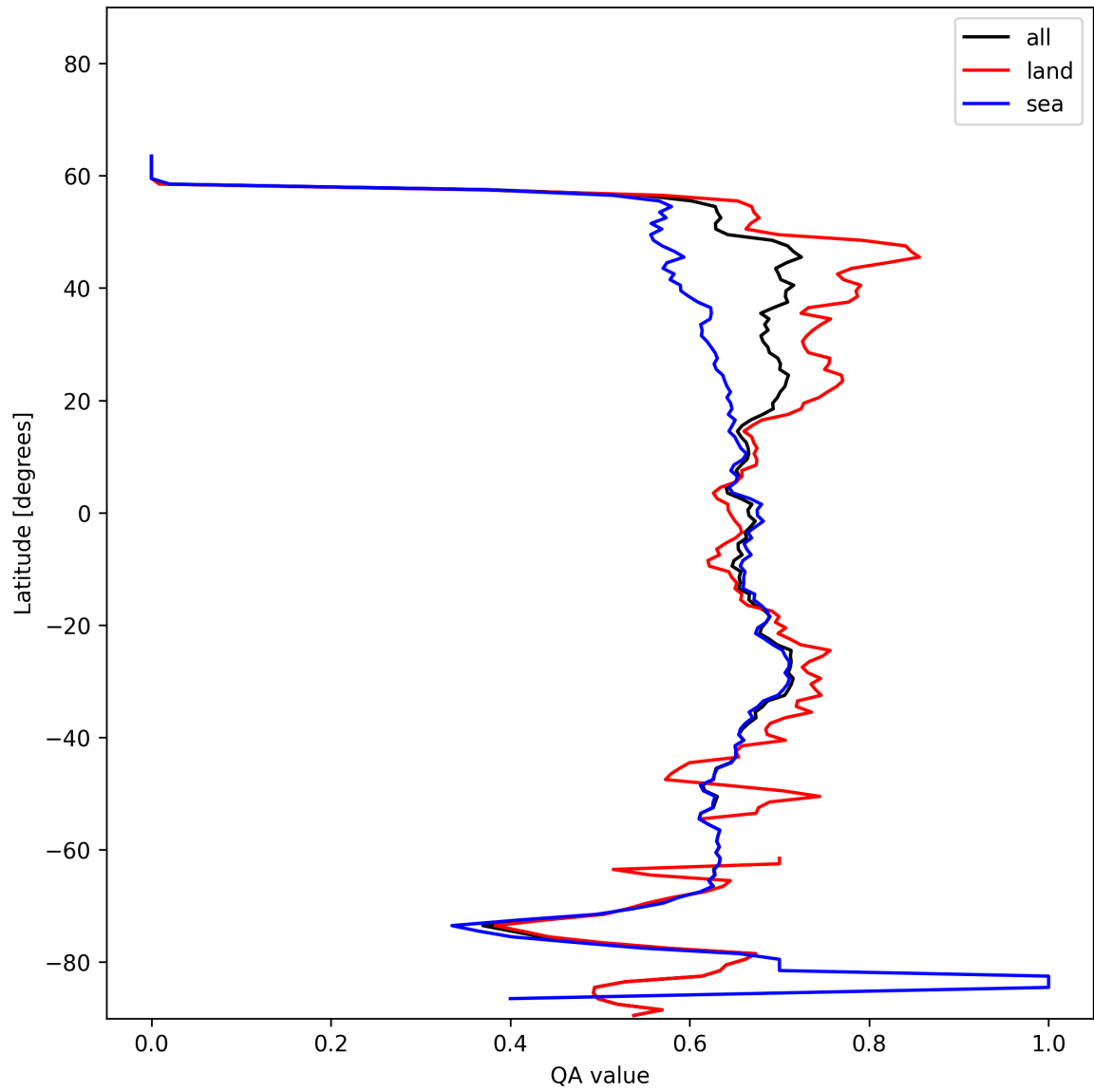
Figure 6: Zonal average of “QA value” for 2025-01-10 to 2025-01-10.
