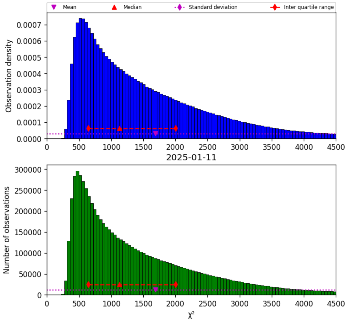
Figure 17: Histogram of “ \chi^2 ” for 2025-01-11 to 2025-01-12
