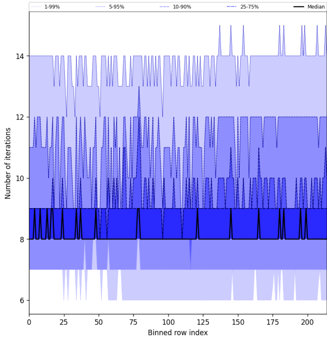
Figure 26: Along track statistics of “Number of iterations” for 2025-01-11 to 2025-01-12
