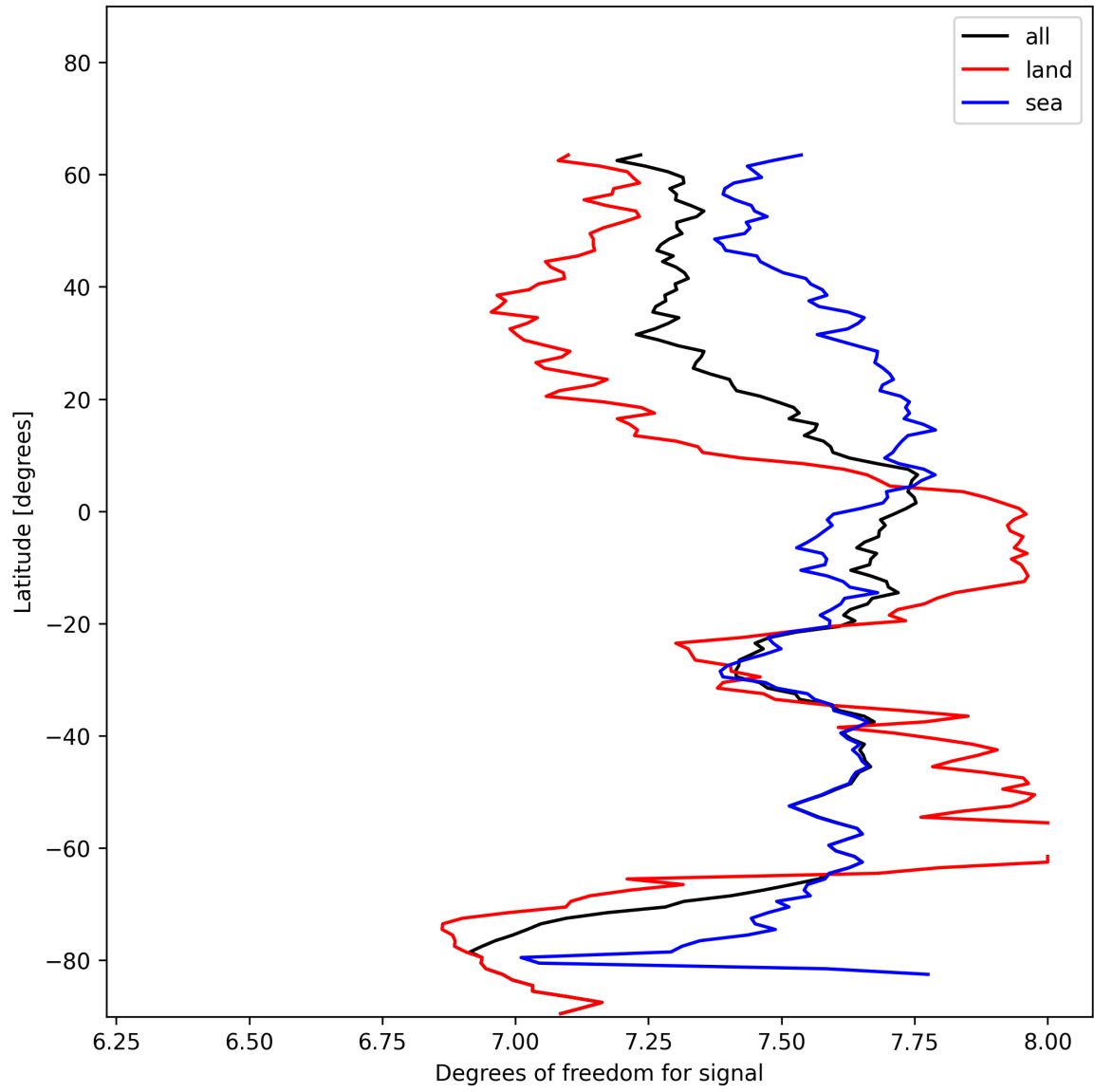
Figure 11: Zonal average of “Degrees of freedom for signal” for 2025-01-11 to 2025-01-12.
