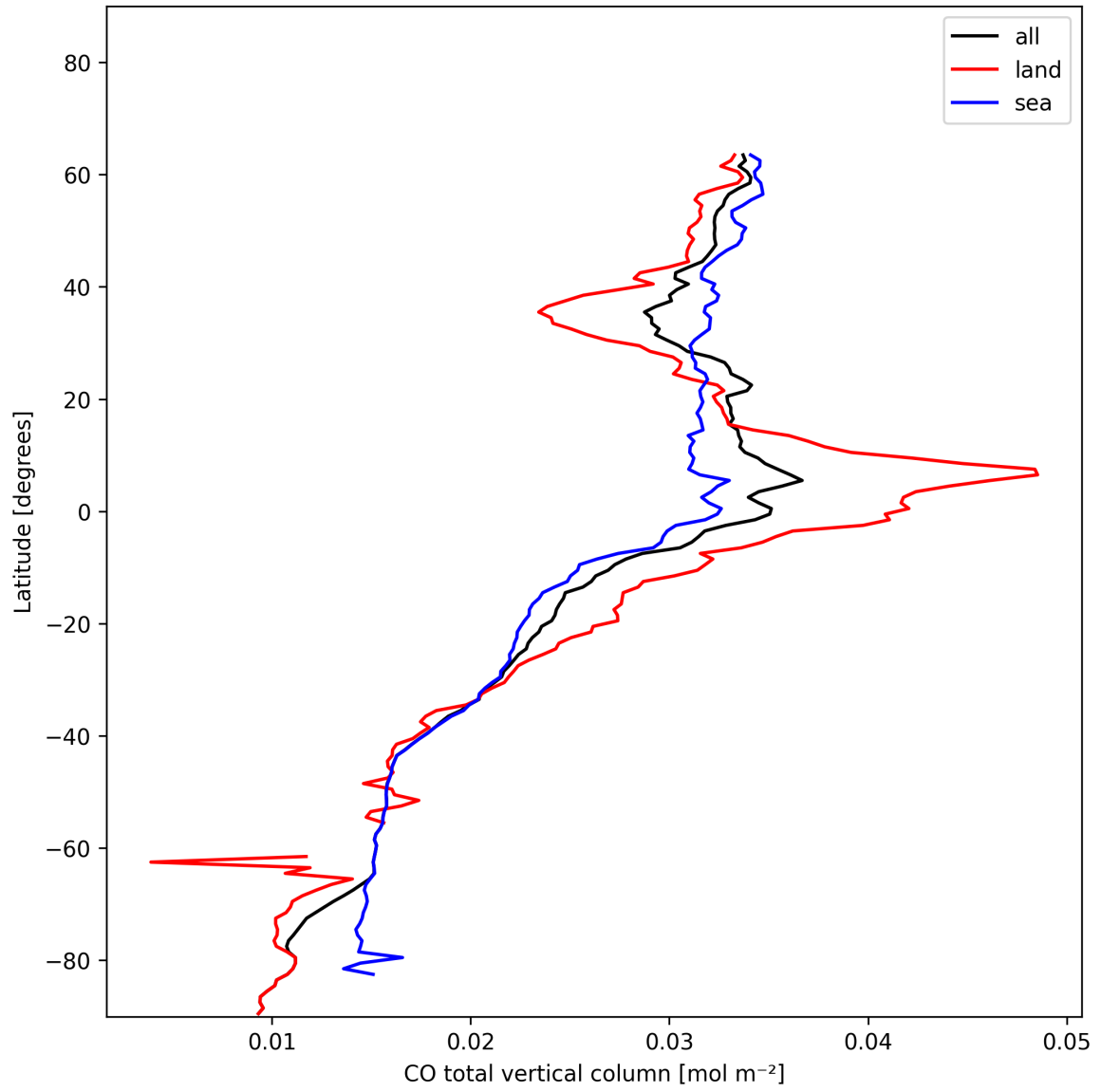
Figure 7: Zonal average of “CO total vertical column” for 2025-01-11 to 2025-01-12.
