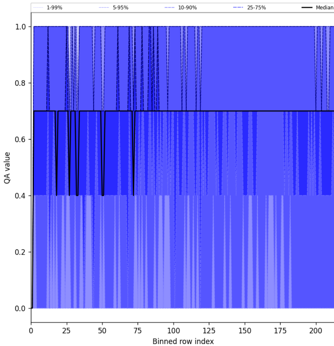
Figure 20: Along track statistics of “QA value” for 2025-01-11 to 2025-01-12
