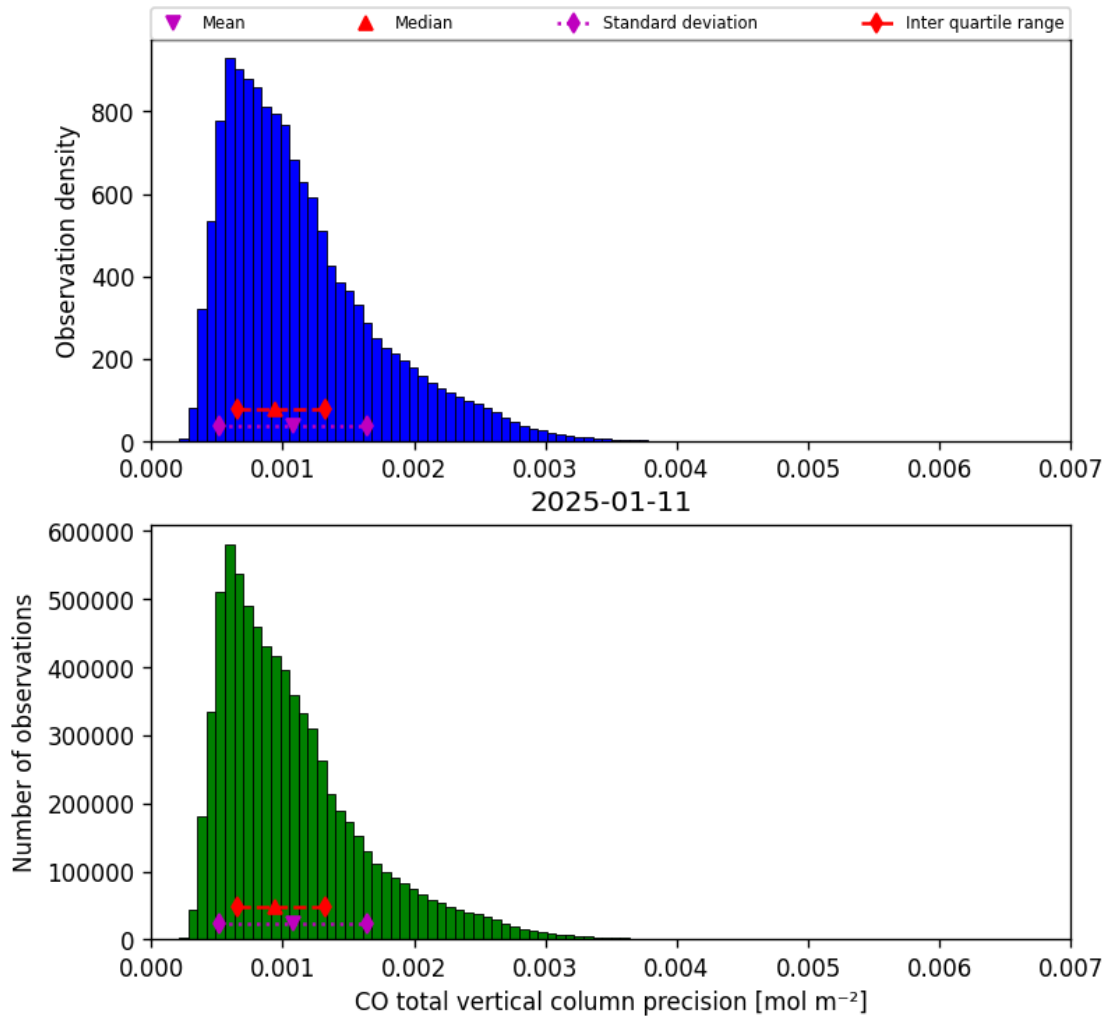
Figure 15: Histogram of “CO total vertical column precision” for 2025-01-11 to 2025-01-12
