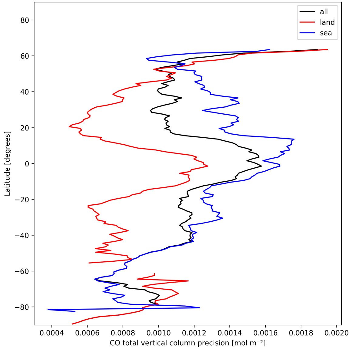
Figure 8: Zonal average of “CO total vertical column precision” for 2025-01-11 to 2025-01-12.
