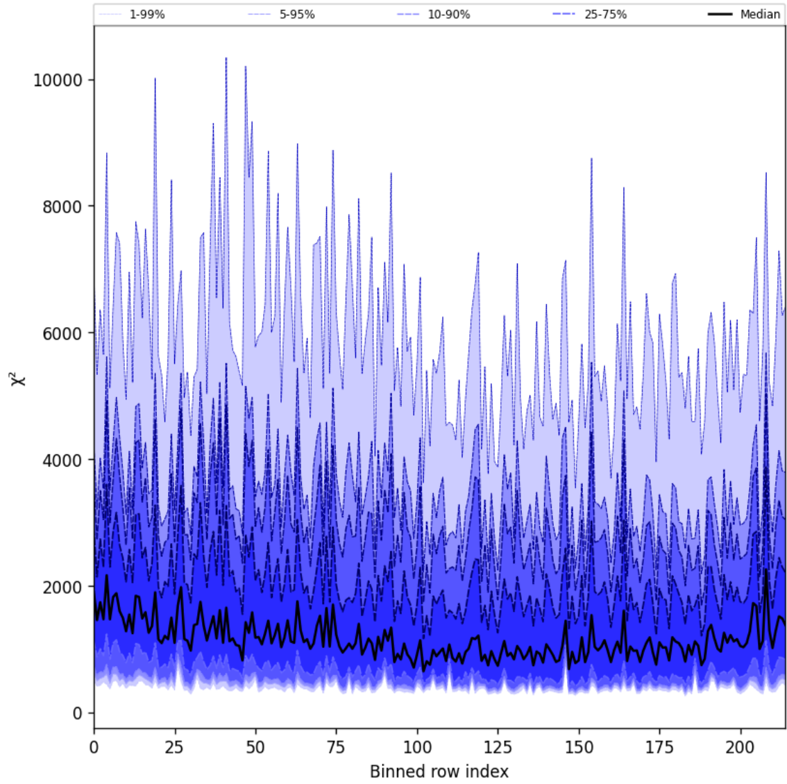
Figure 24: Along track statistics of “ \chi^2 ” for 2025-01-11 to 2025-01-12
