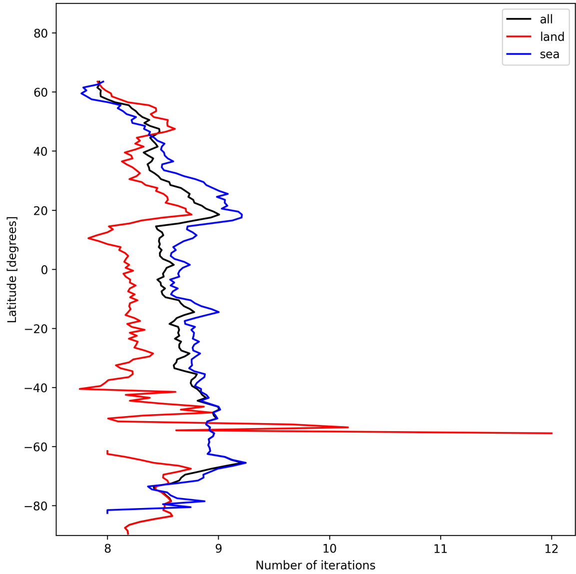
Figure 12: Zonal average of “Number of iterations” for 2025-01-11 to 2025-01-12.
