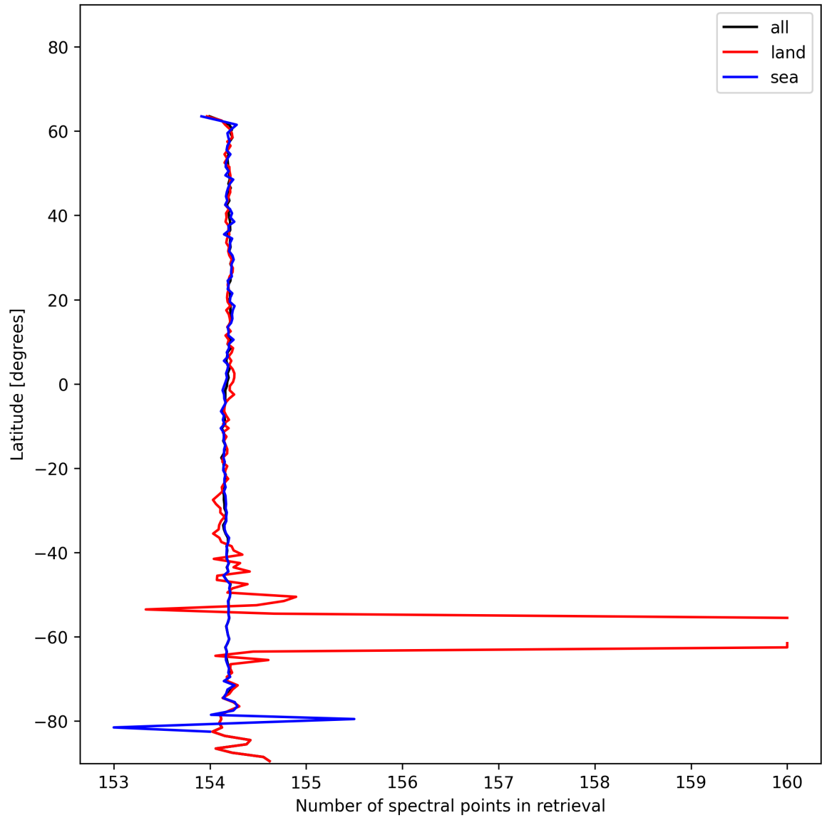
Figure 9: Zonal average of “Number of spectral points in retrieval” for 2025-01-11 to 2025-01-12.
