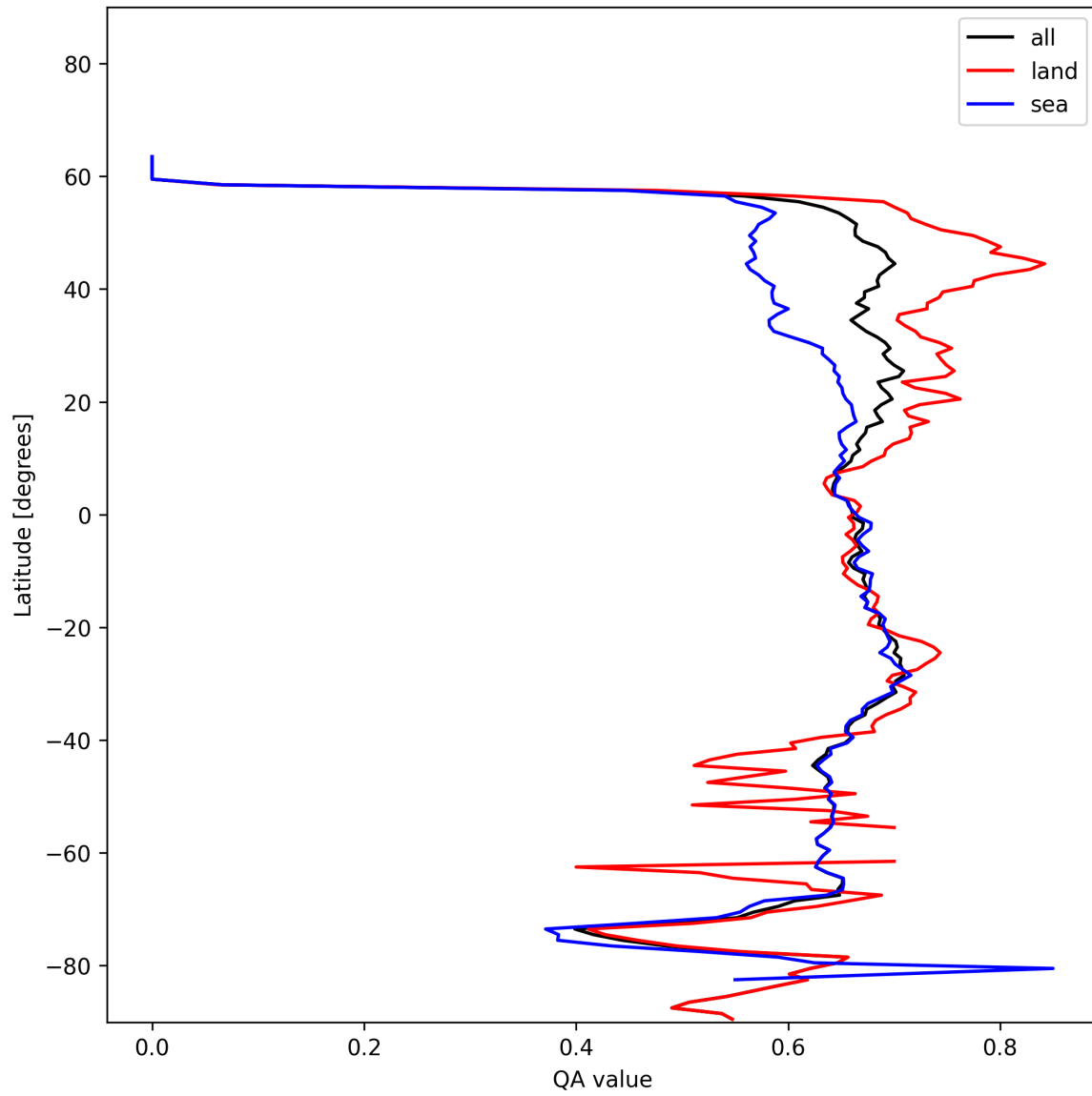
Figure 6: Zonal average of “QA value” for 2025-01-11 to 2025-01-12.
