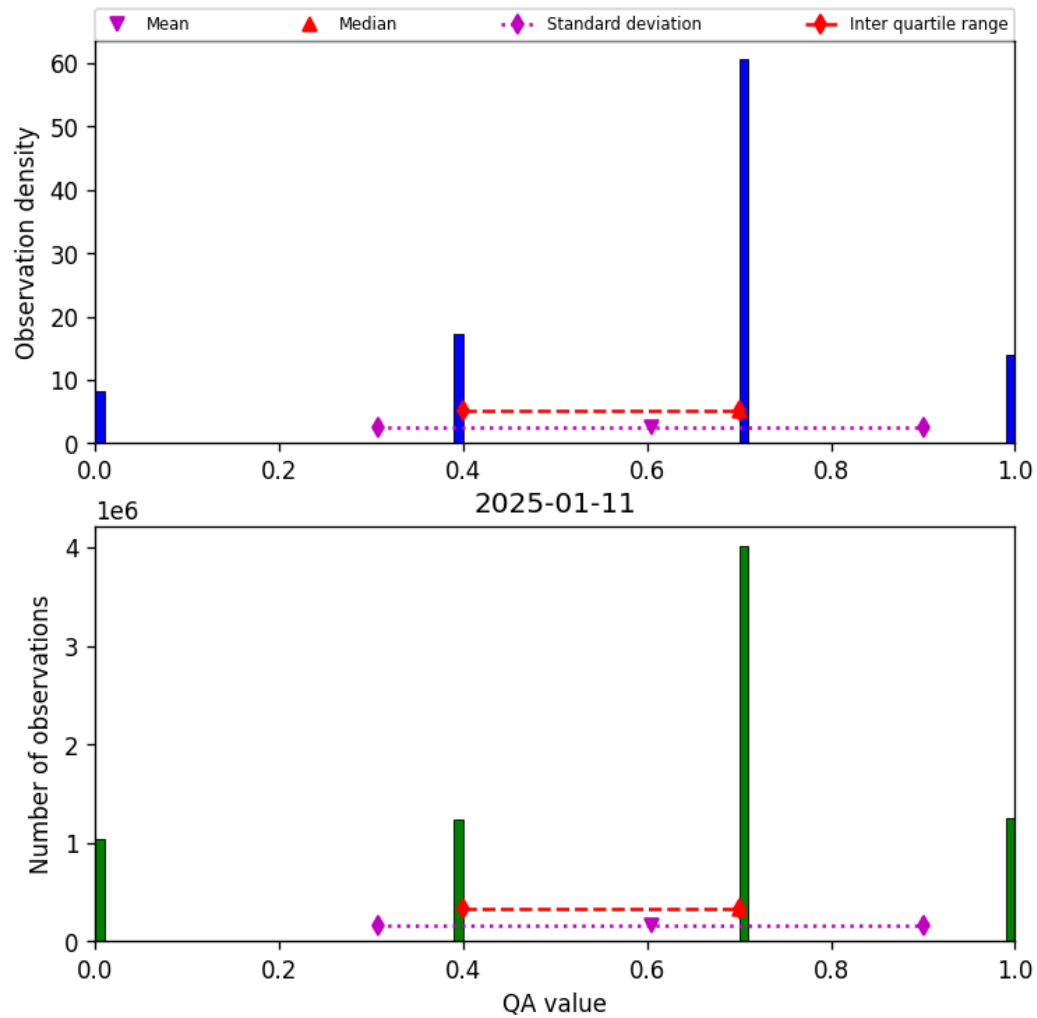
Figure 13: Histogram of “QA value” for 2025-01-11 to 2025-01-12
