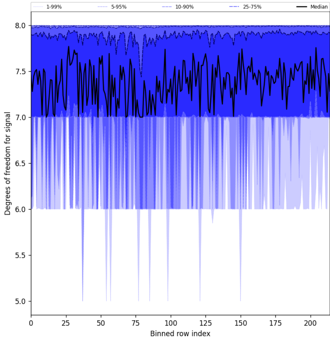
Figure 25: Along track statistics of “Degrees of freedom for signal” for 2025-01-11 to 2025-01-12
