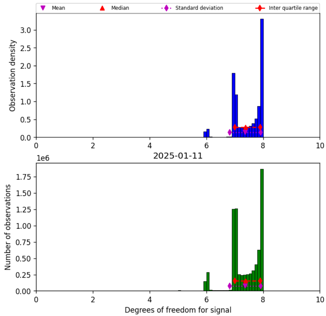
Figure 18: Histogram of “Degrees of freedom for signal” for 2025-01-11 to 2025-01-12
