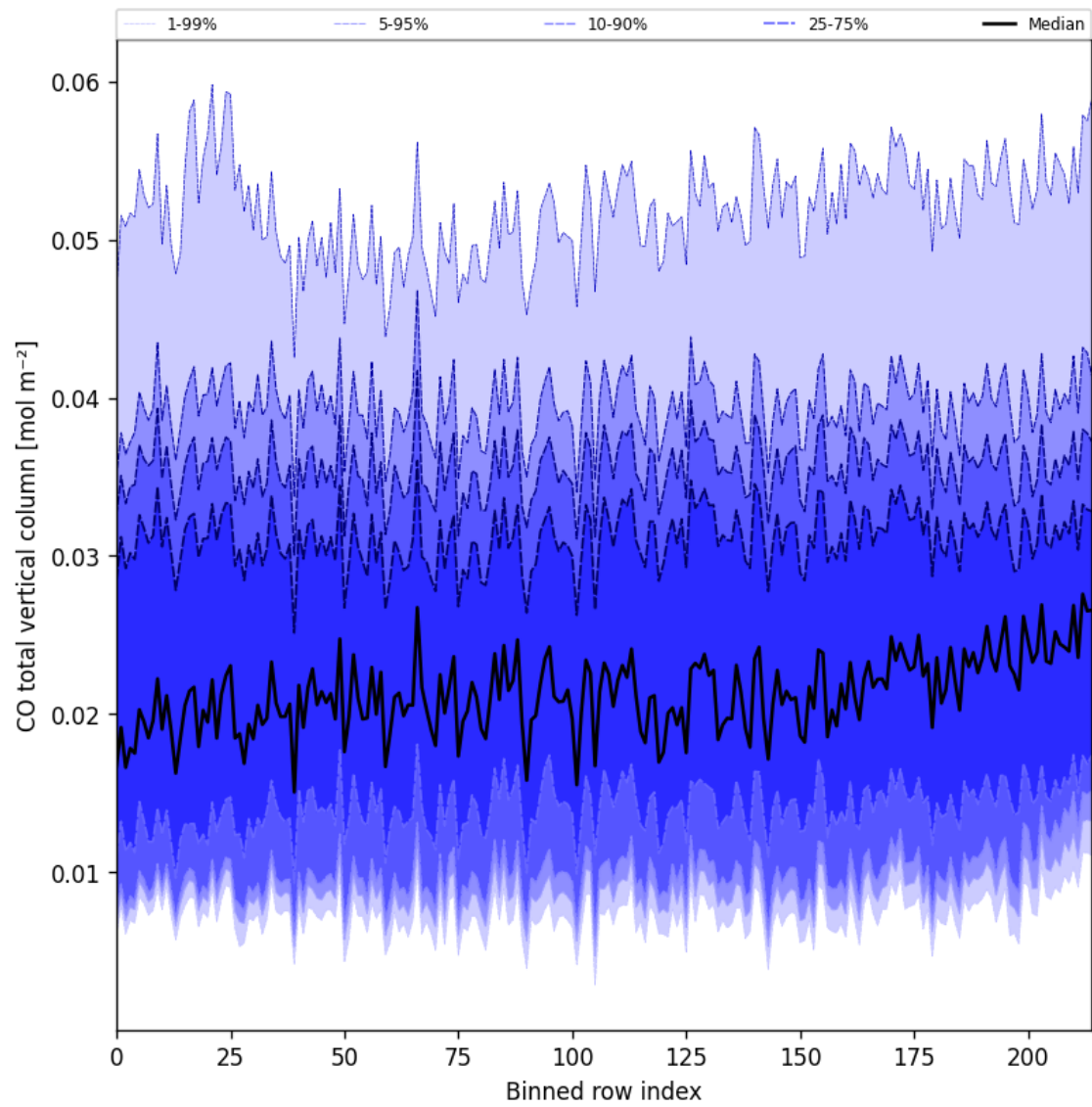
Figure 21: Along track statistics of “CO total vertical column” for 2025-01-11 to 2025-01-12
