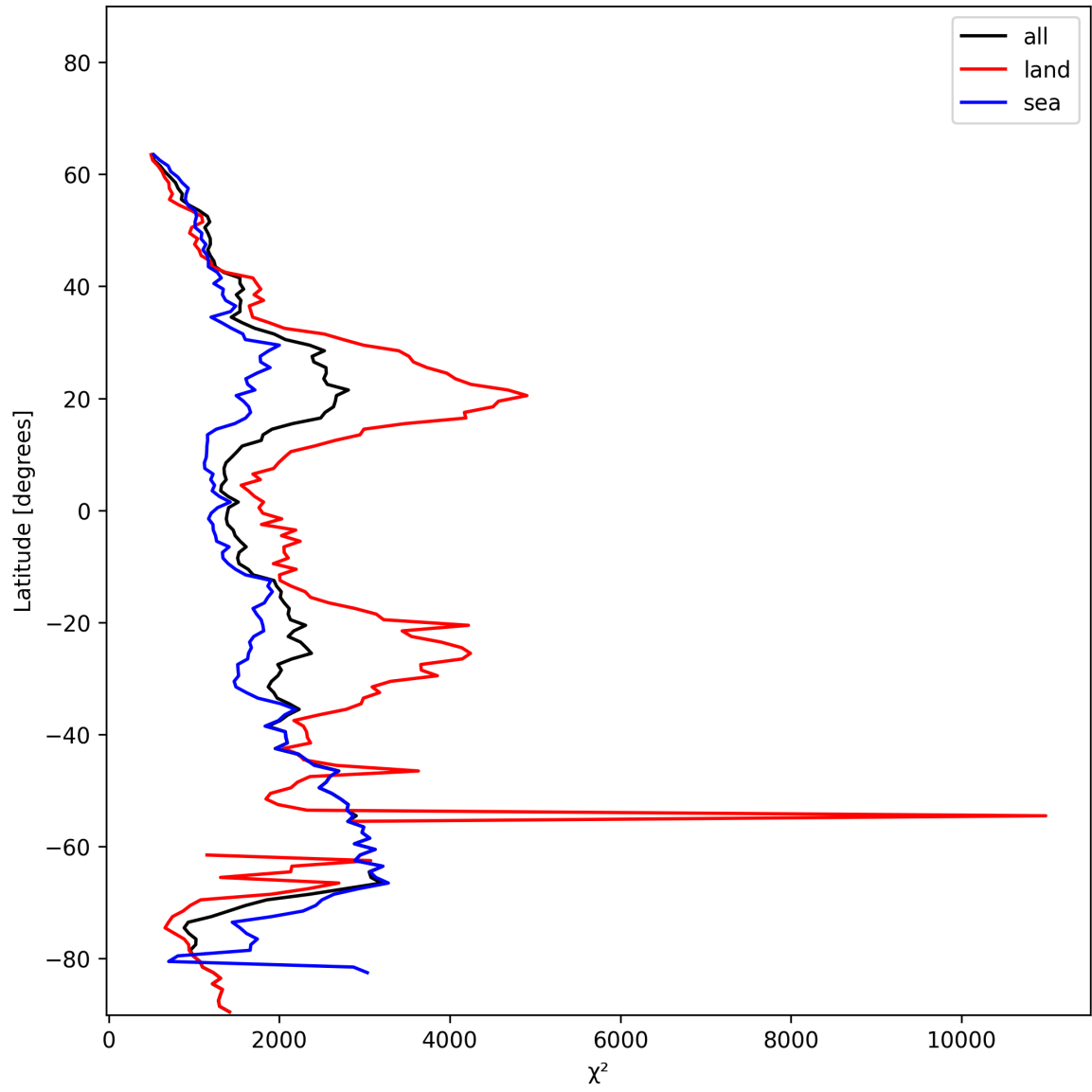
Figure 10: Zonal average of “ \chi^2 ” for 2025-01-11 to 2025-01-12.
