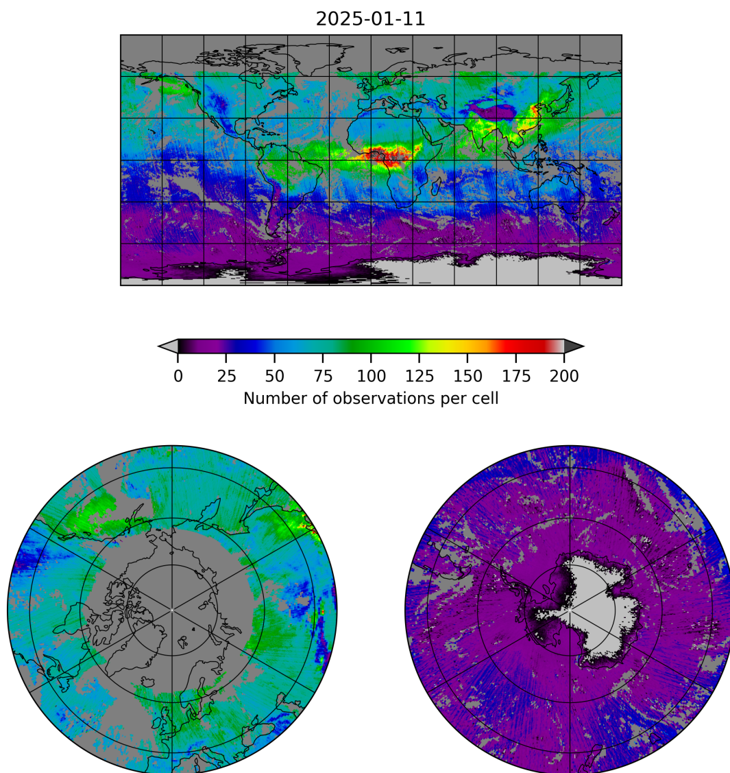
Figure 5: Map of the number of observations for 2025-01-11 to 2025-01-12
