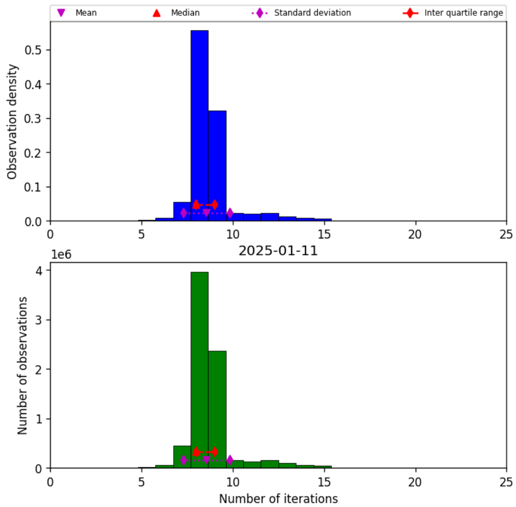
Figure 19: Histogram of “Number of iterations” for 2025-01-11 to 2025-01-12
