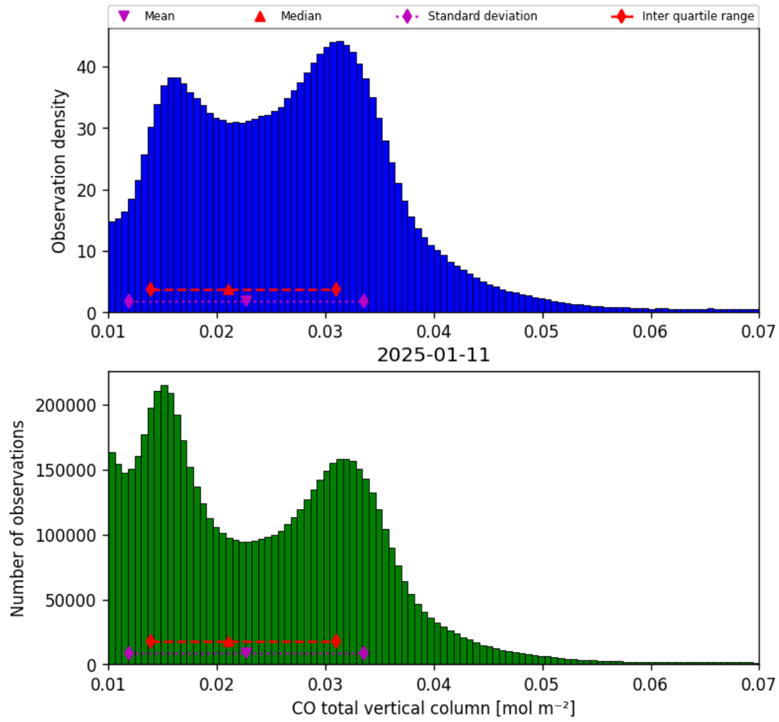
Figure 14: Histogram of “CO total vertical column” for 2025-01-11 to 2025-01-12
