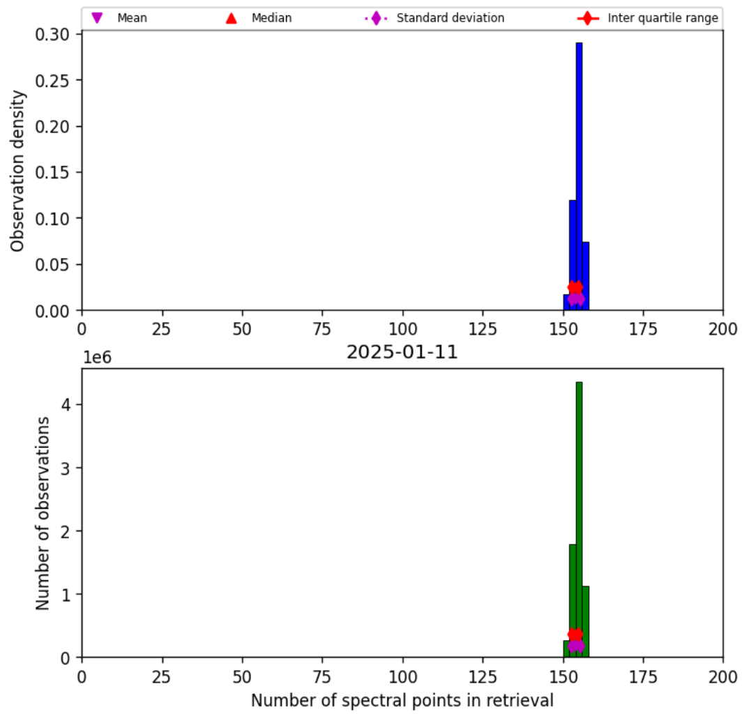
Figure 16: Histogram of “Number of spectral points in retrieval” for 2025-01-11 to 2025-01-12
