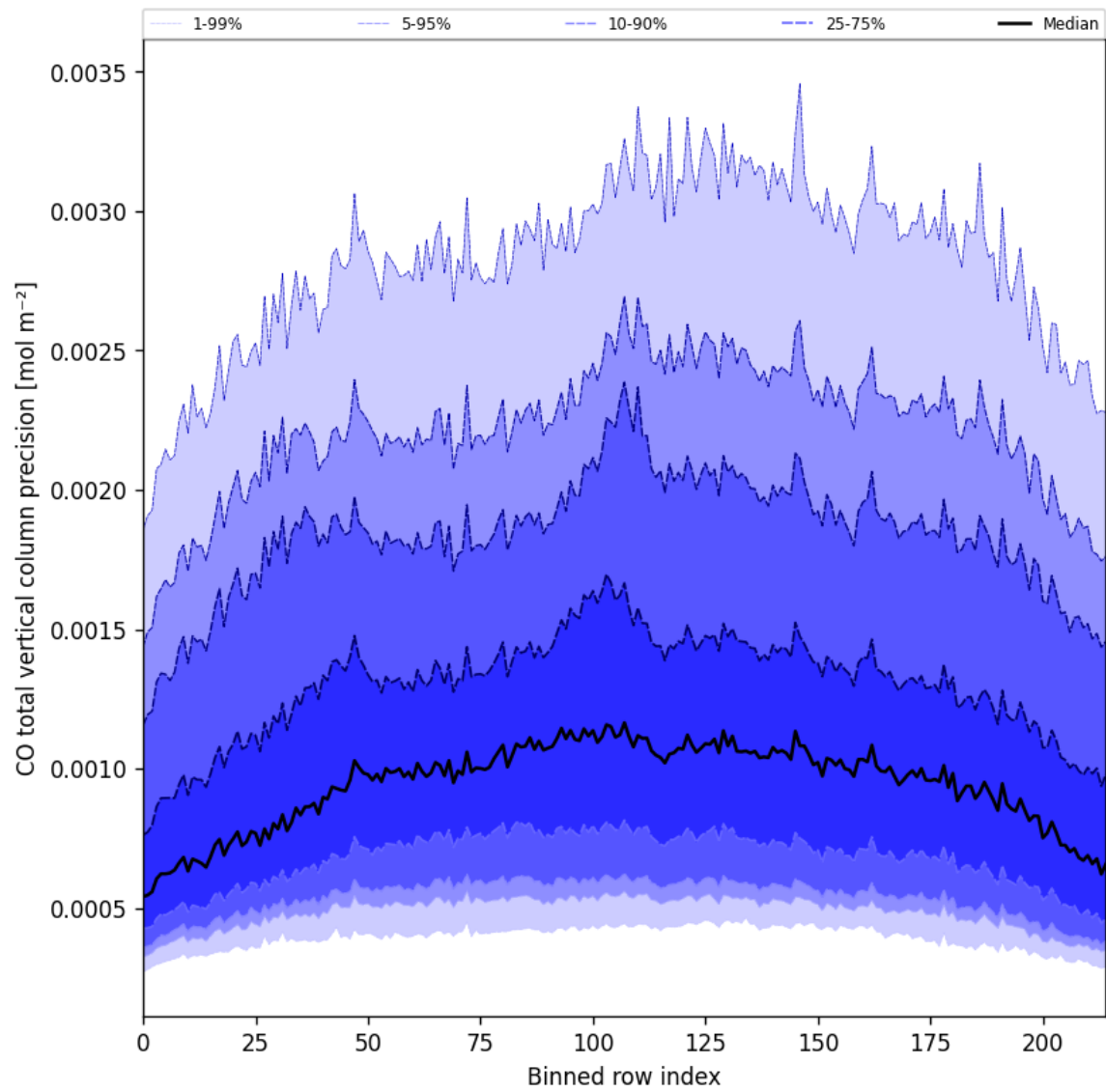
Figure 22: Along track statistics of “CO total vertical column precision” for 2025-01-11 to 2025-01-12
