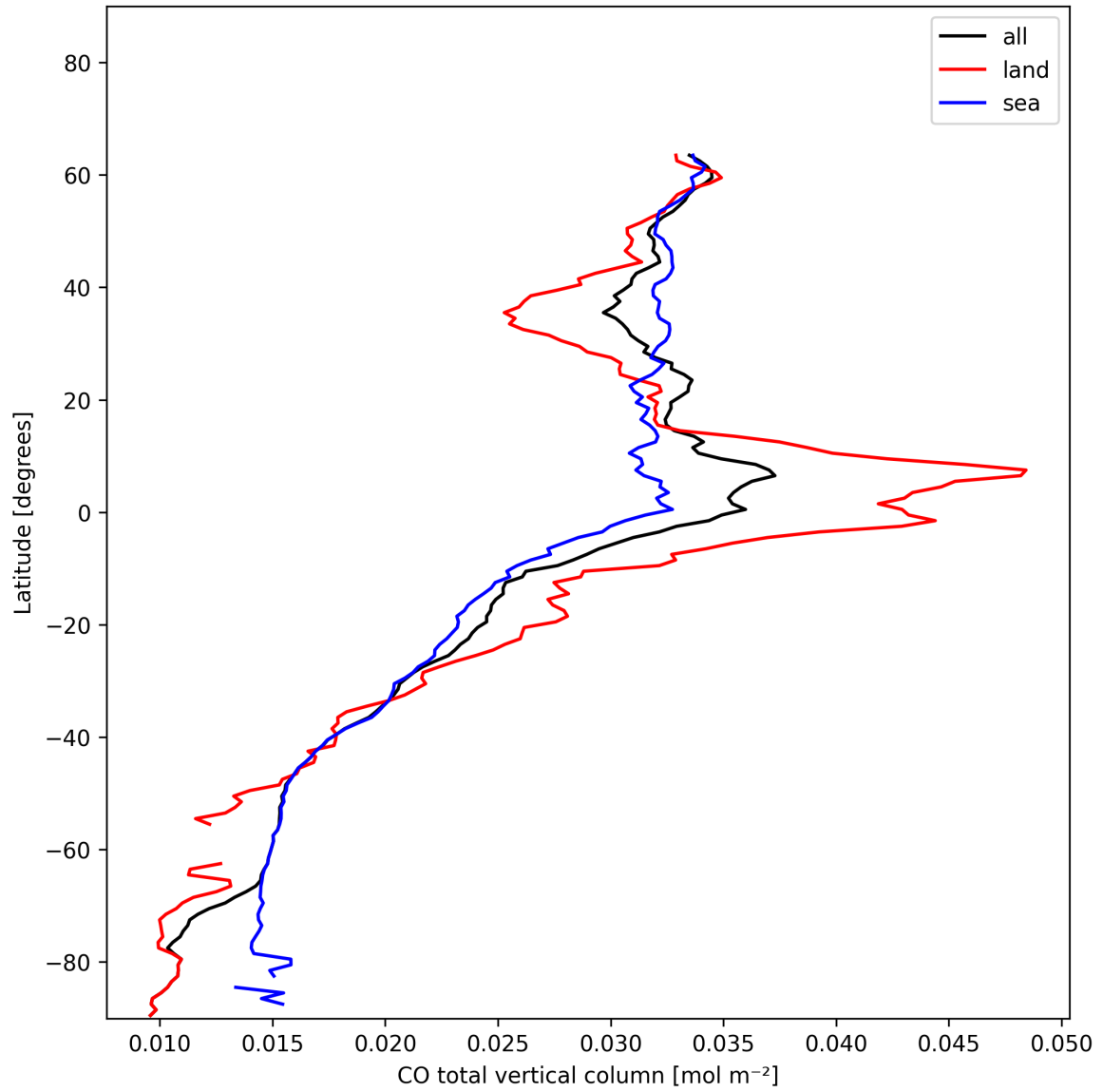
Figure 7: Zonal average of “CO total vertical column” for 2025-01-12 to 2025-01-13.
