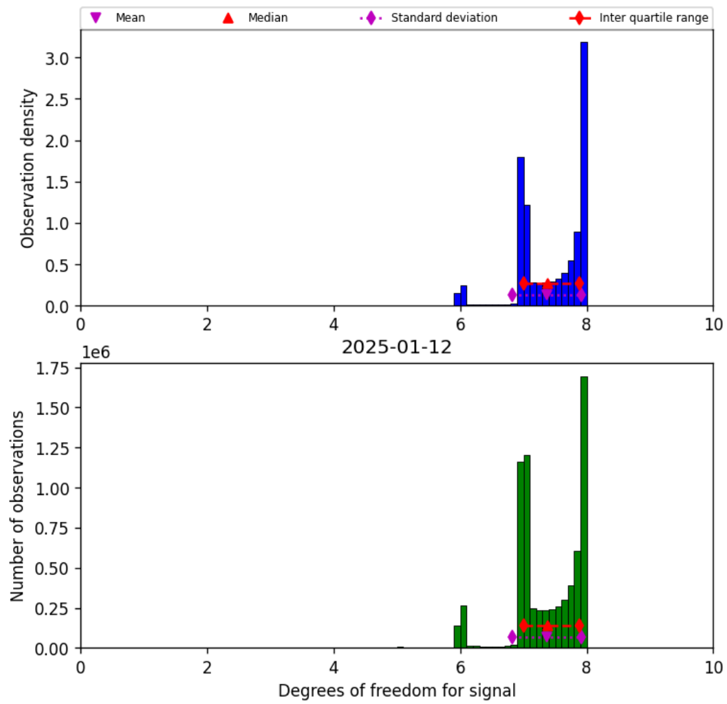
Figure 18: Histogram of “Degrees of freedom for signal” for 2025-01-12 to 2025-01-13
