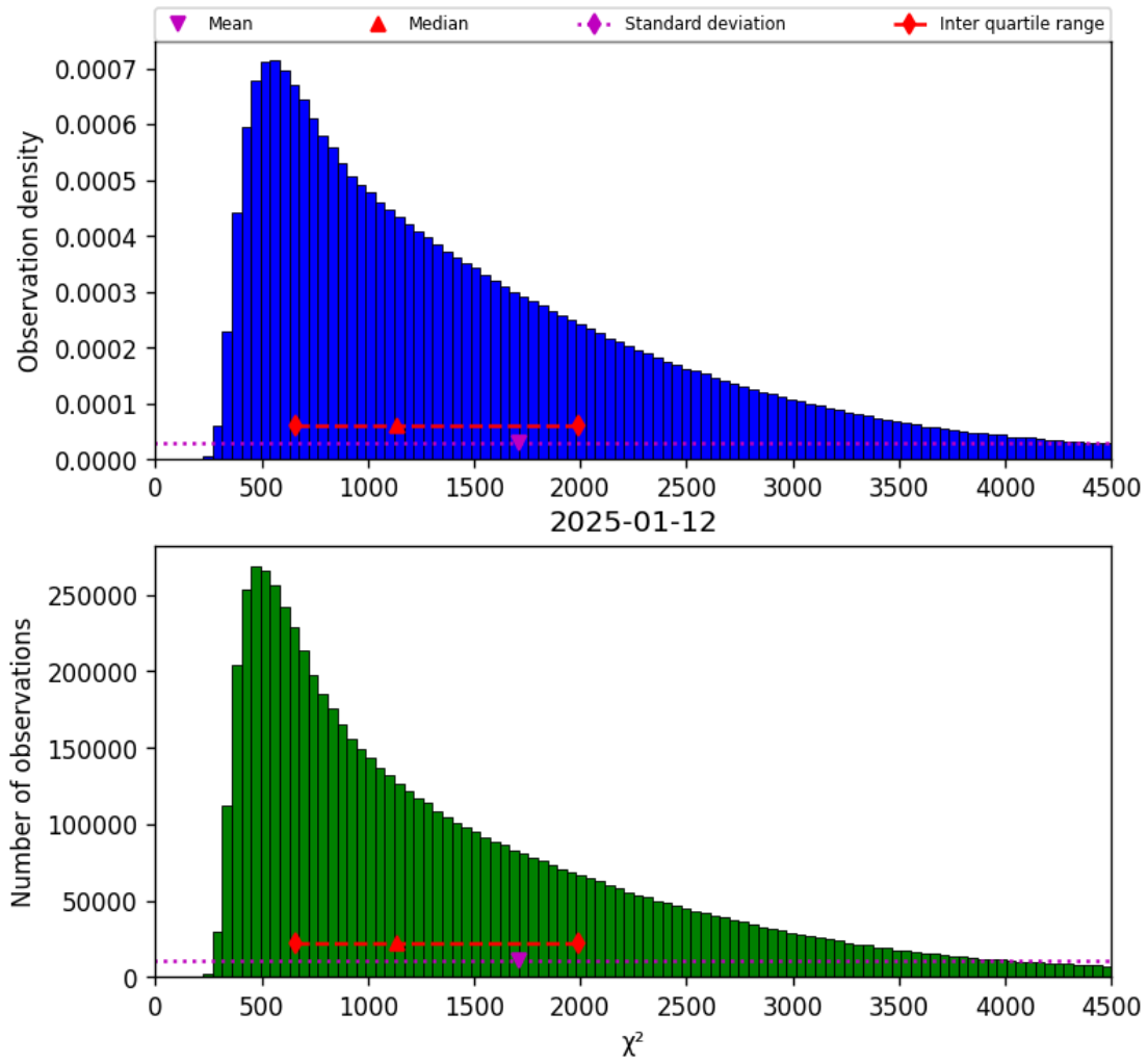
Figure 17: Histogram of “ \chi^2 ” for 2025-01-12 to 2025-01-13
