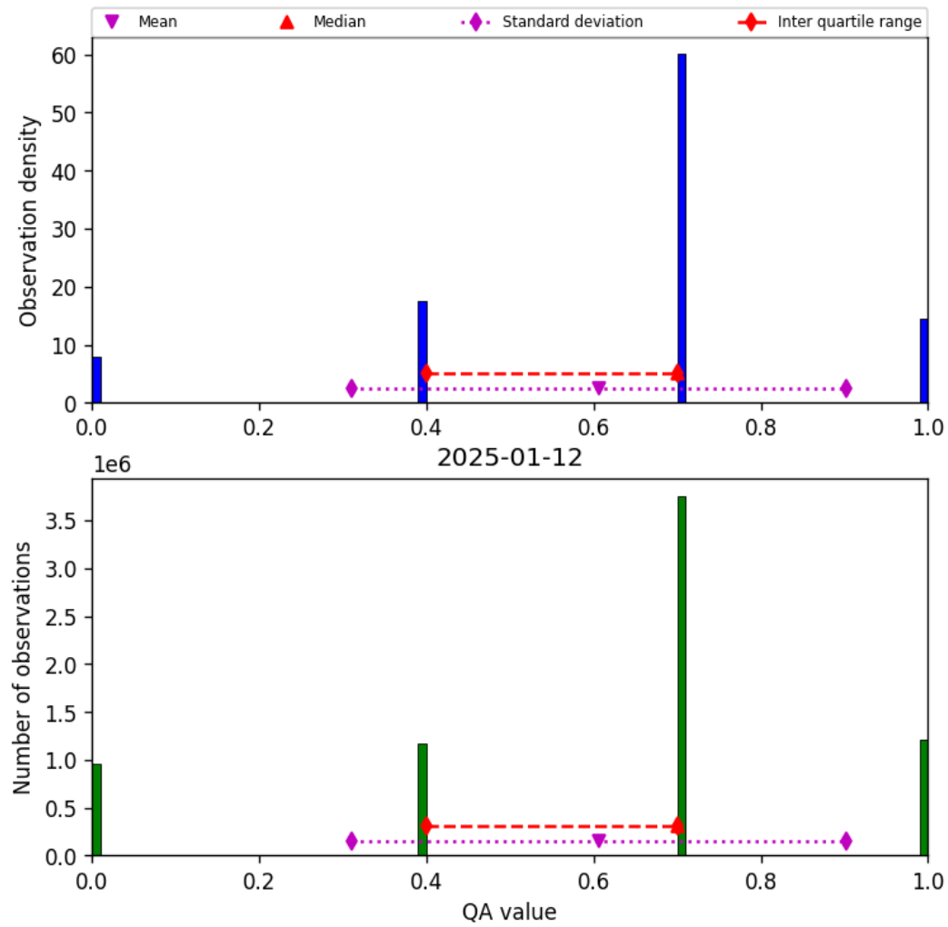
Figure 13: Histogram of “QA value” for 2025-01-12 to 2025-01-13
