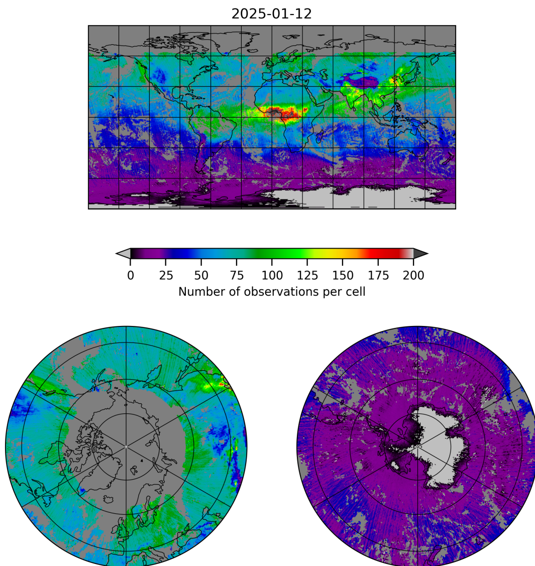
Figure 5: Map of the number of observations for 2025-01-12 to 2025-01-13
