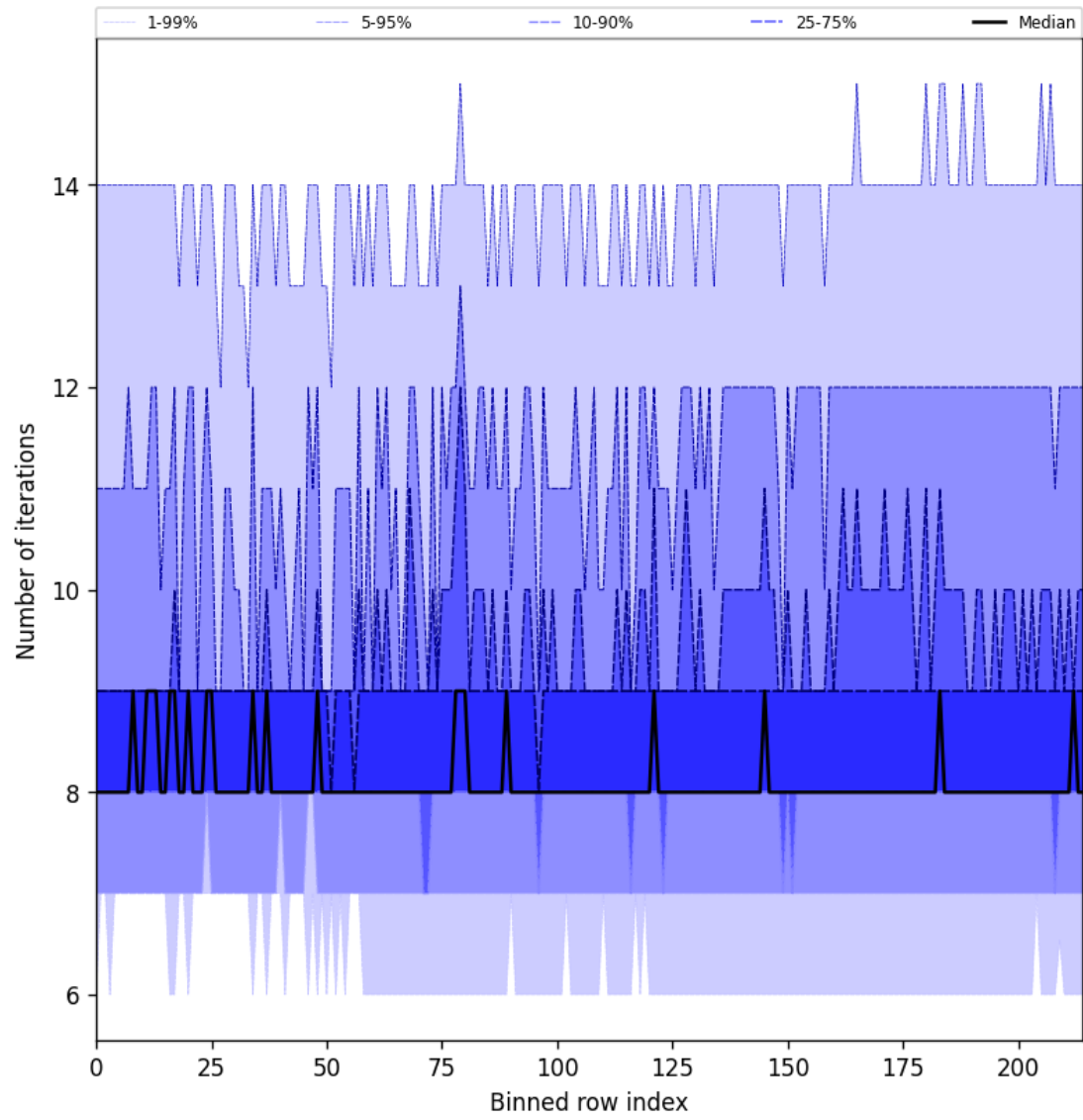
Figure 26: Along track statistics of “Number of iterations” for 2025-01-12 to 2025-01-13
