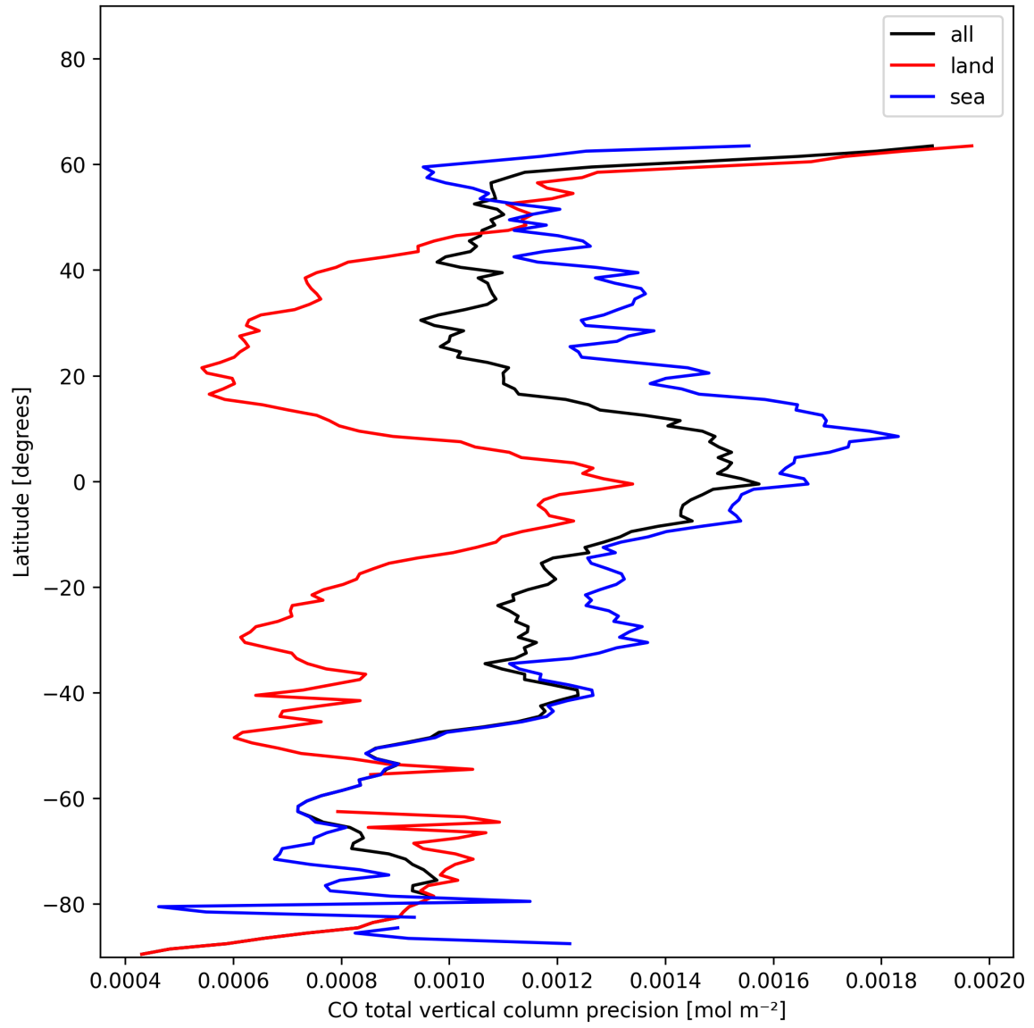
Figure 8: Zonal average of “CO total vertical column precision” for 2025-01-12 to 2025-01-13.
