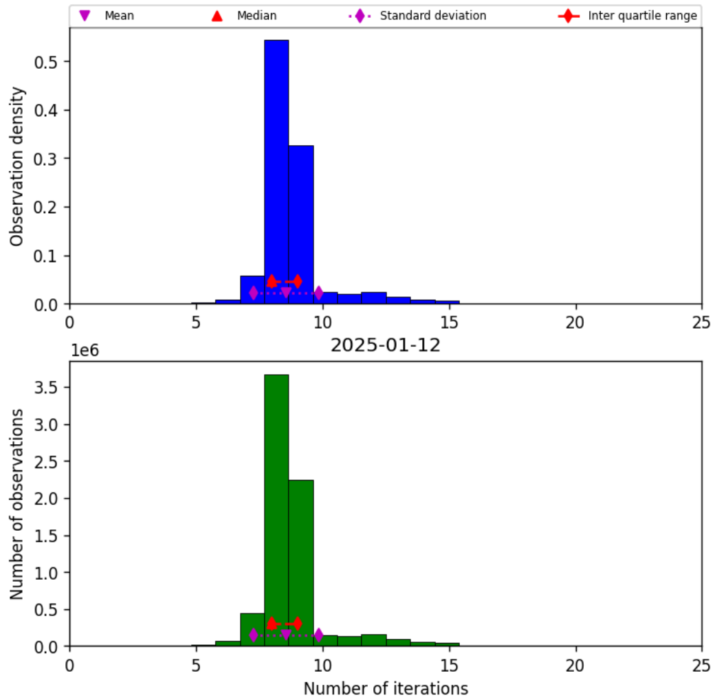
Figure 19: Histogram of “Number of iterations” for 2025-01-12 to 2025-01-13
