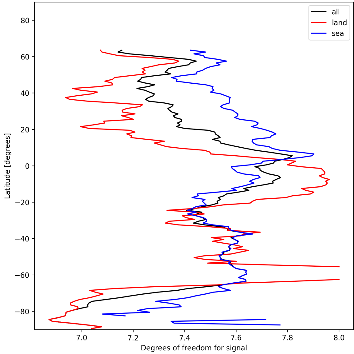
Figure 11: Zonal average of “Degrees of freedom for signal” for 2025-01-12 to 2025-01-13.
