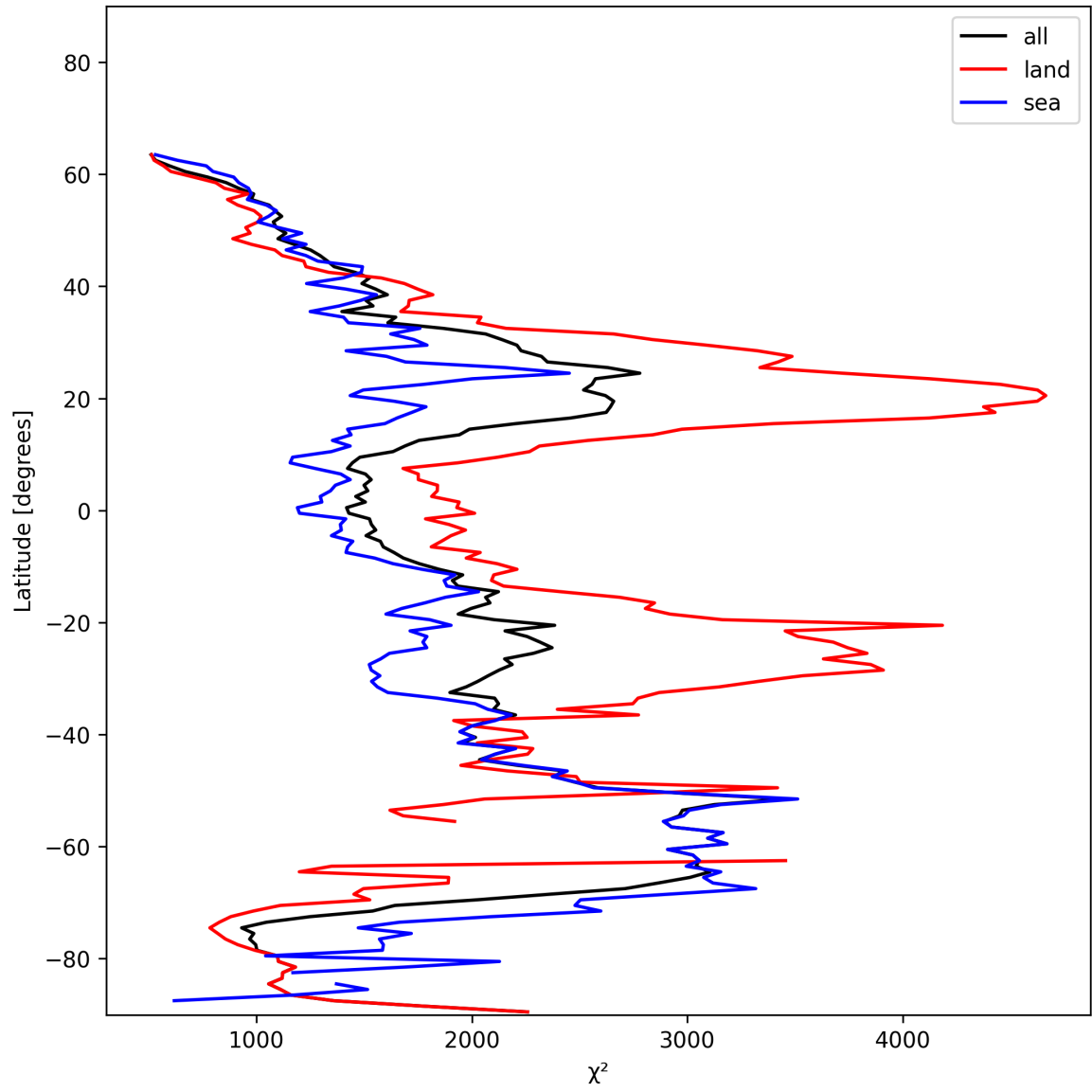
Figure 10: Zonal average of “ \chi^2 ” for 2025-01-12 to 2025-01-13.
