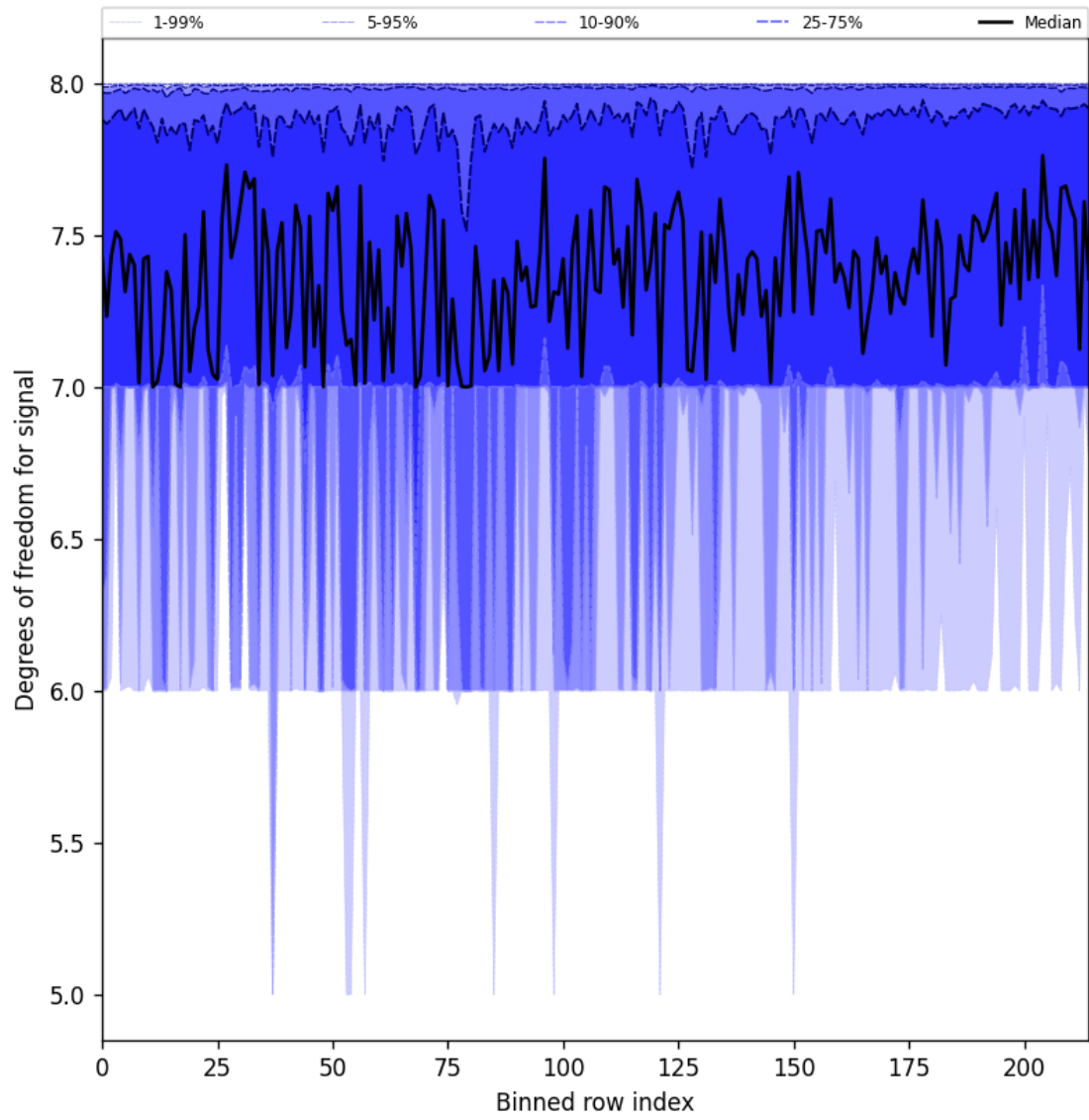
Figure 25: Along track statistics of “Degrees of freedom for signal” for 2025-01-12 to 2025-01-13
