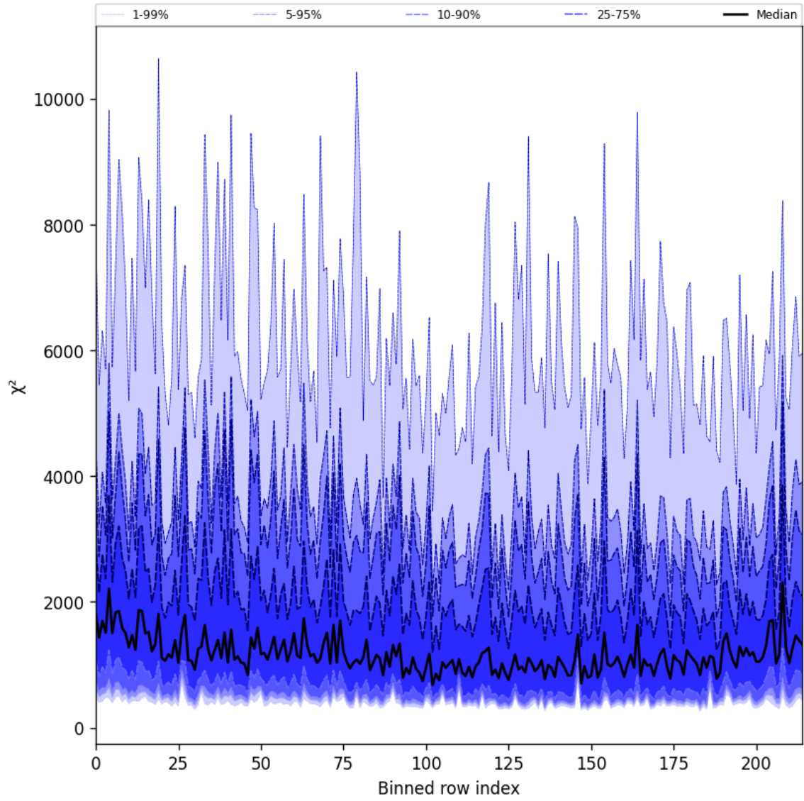
Figure 24: Along track statistics of “ \chi^2 ” for 2025-01-12 to 2025-01-13
