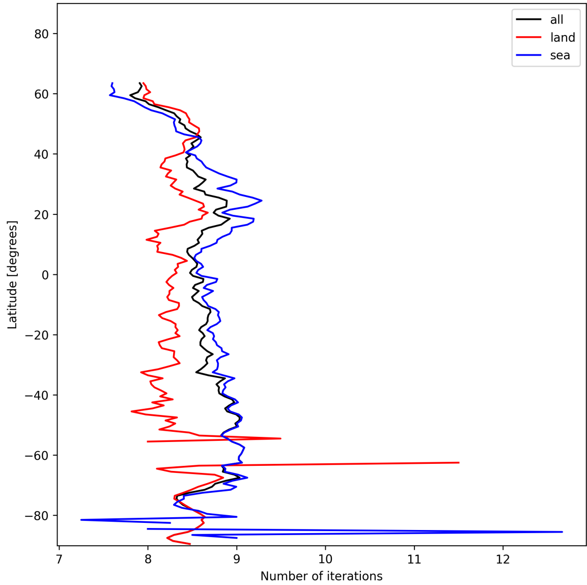
Figure 12: Zonal average of “Number of iterations” for 2025-01-12 to 2025-01-13.
