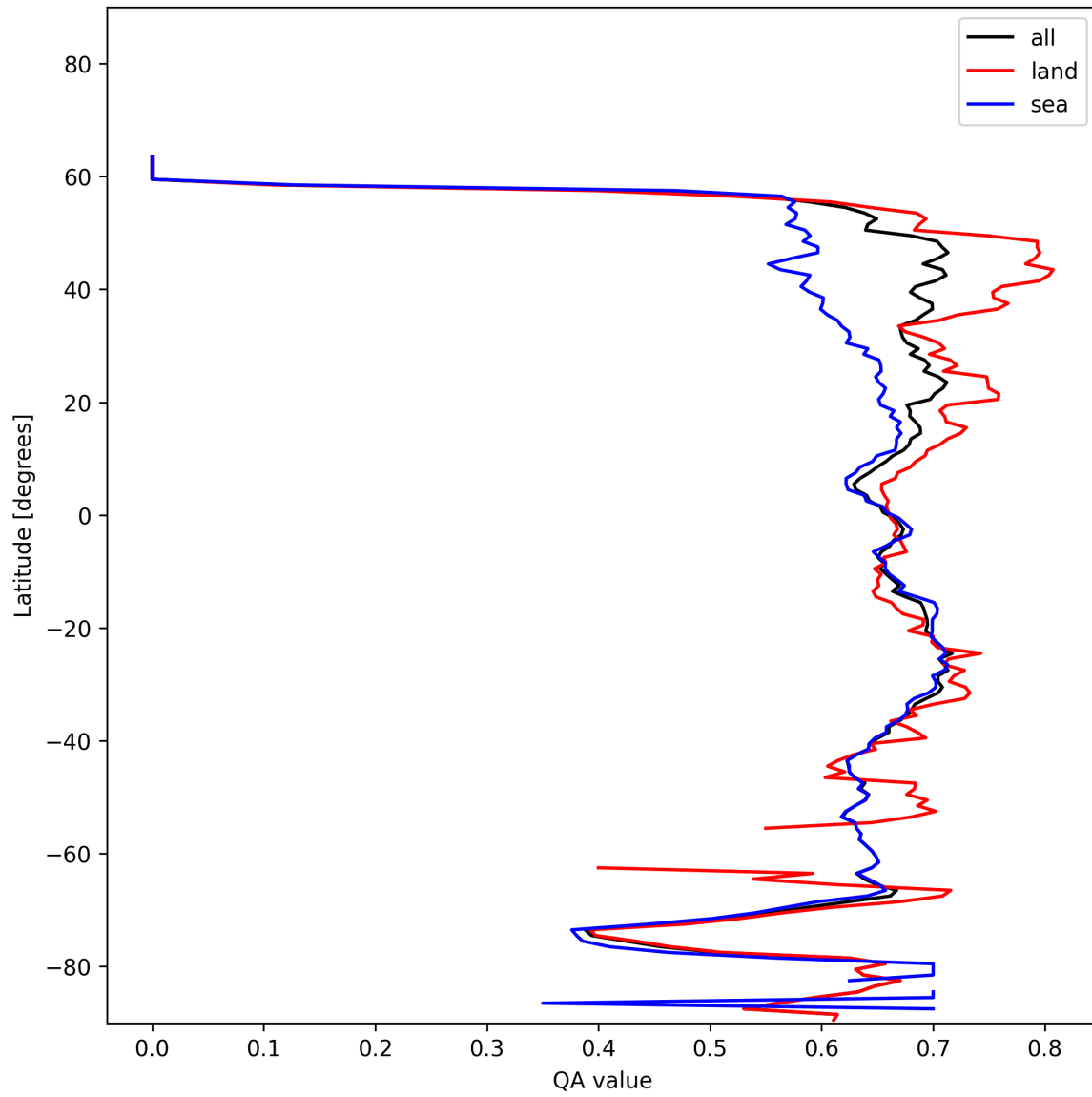
Figure 6: Zonal average of “QA value” for 2025-01-12 to 2025-01-13.
