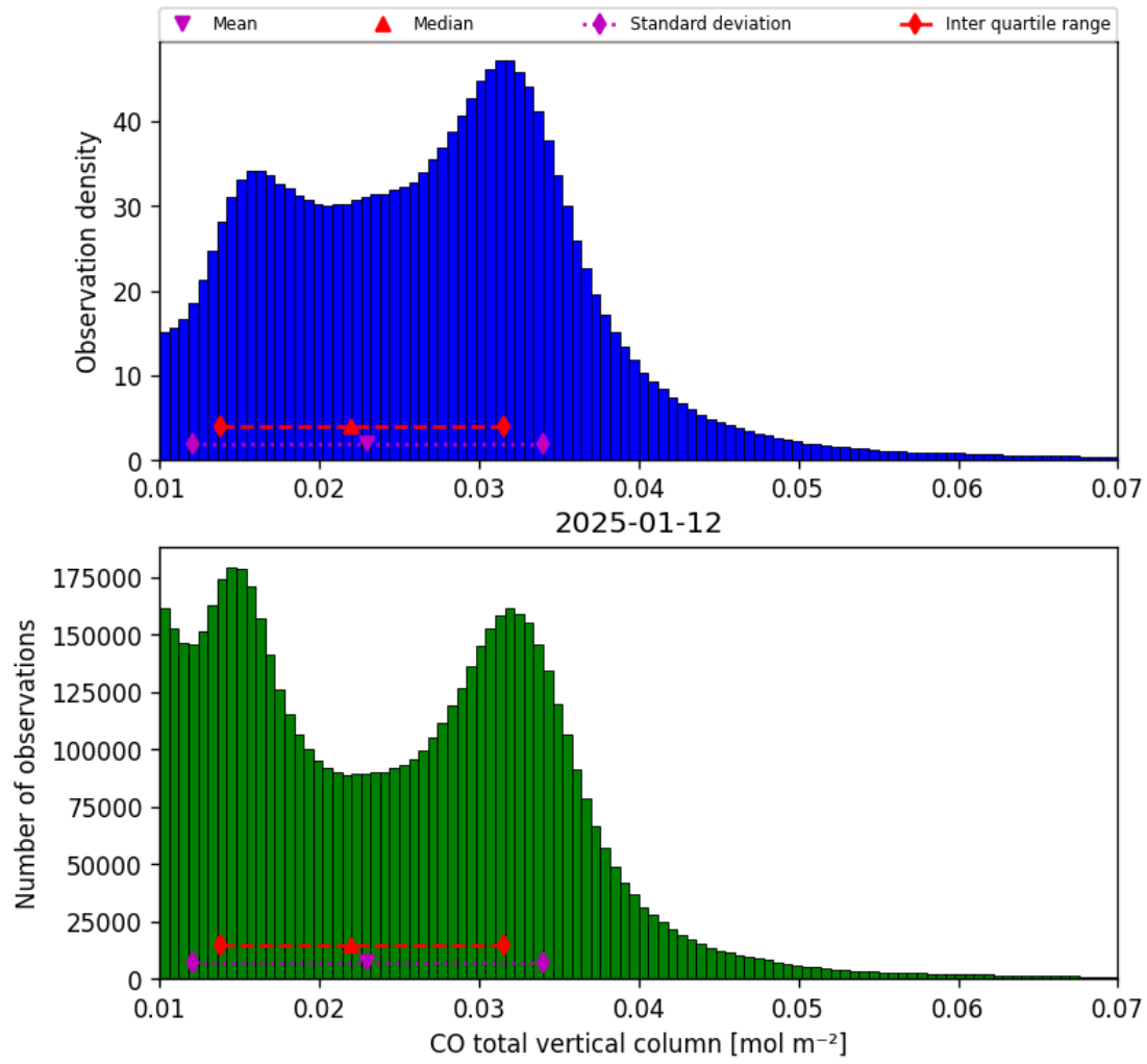
Figure 14: Histogram of “CO total vertical column” for 2025-01-12 to 2025-01-13
