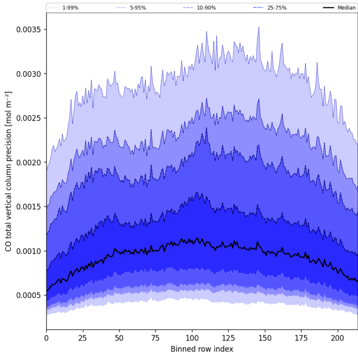
Figure 22: Along track statistics of “CO total vertical column precision” for 2025-01-12 to 2025-01-13
