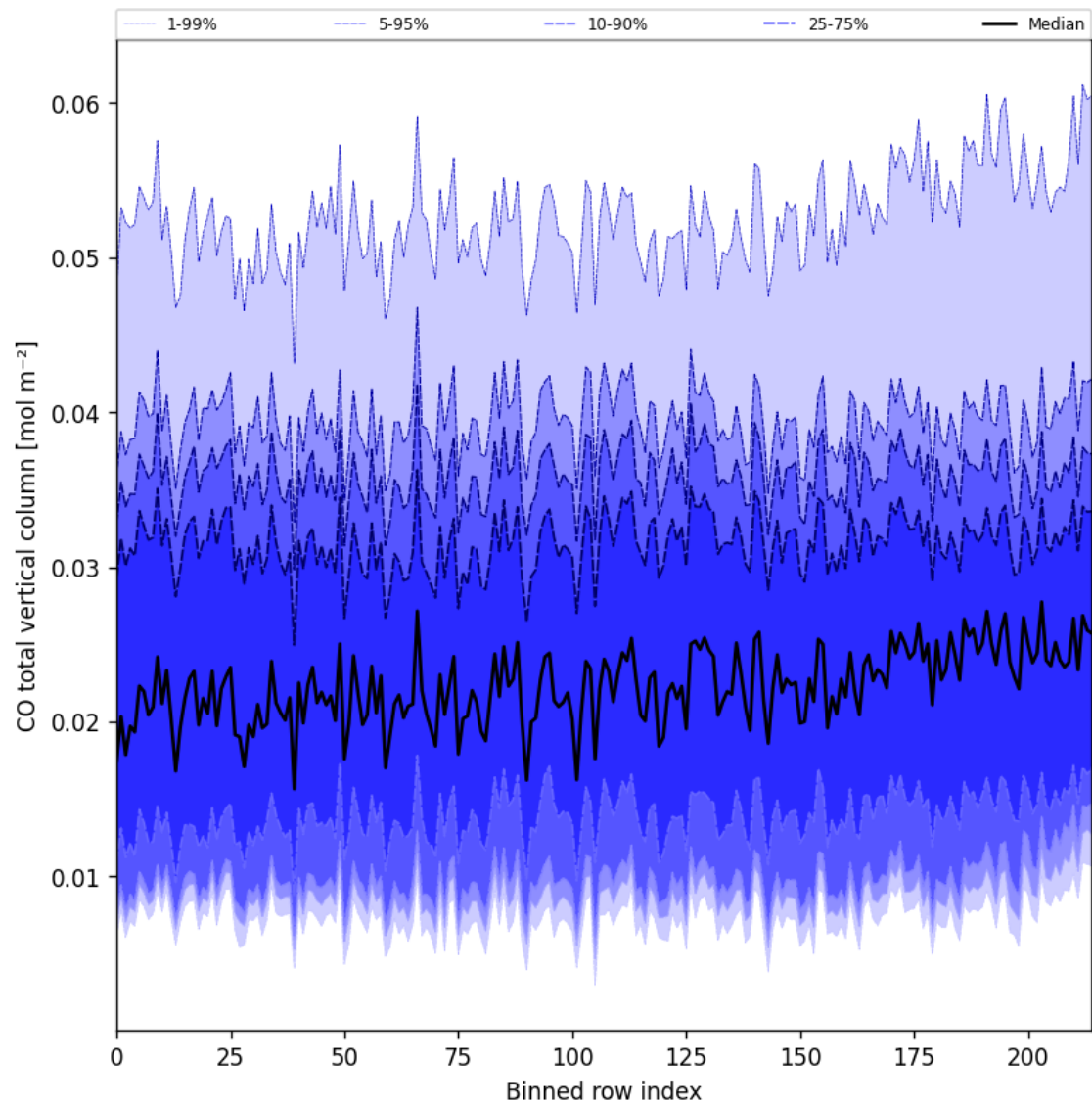
Figure 21: Along track statistics of “CO total vertical column” for 2025-01-12 to 2025-01-13
