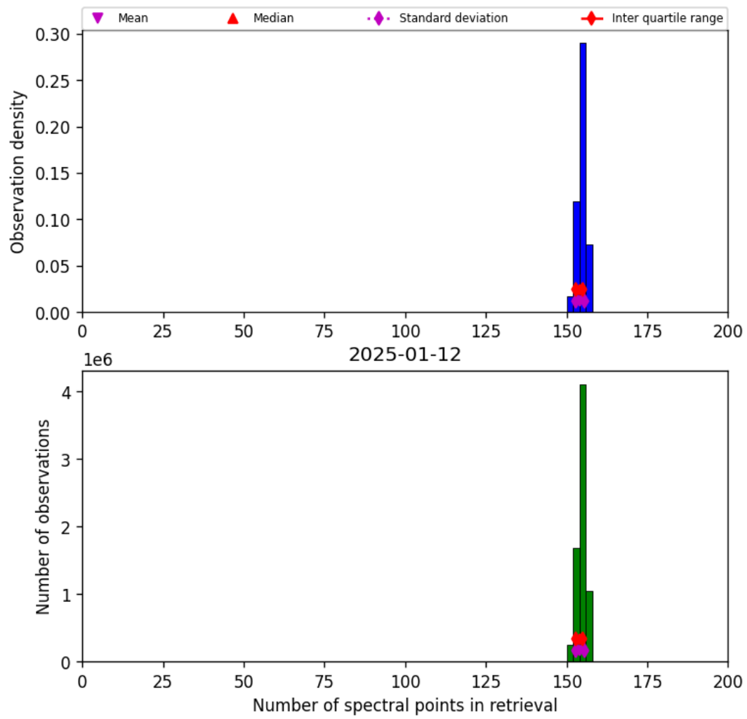
Figure 16: Histogram of “Number of spectral points in retrieval” for 2025-01-12 to 2025-01-13
