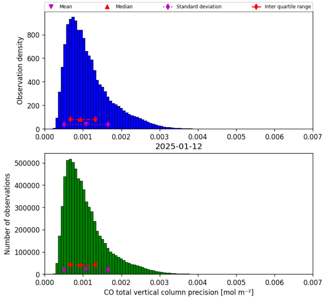
Figure 15: Histogram of “CO total vertical column precision” for 2025-01-12 to 2025-01-13
