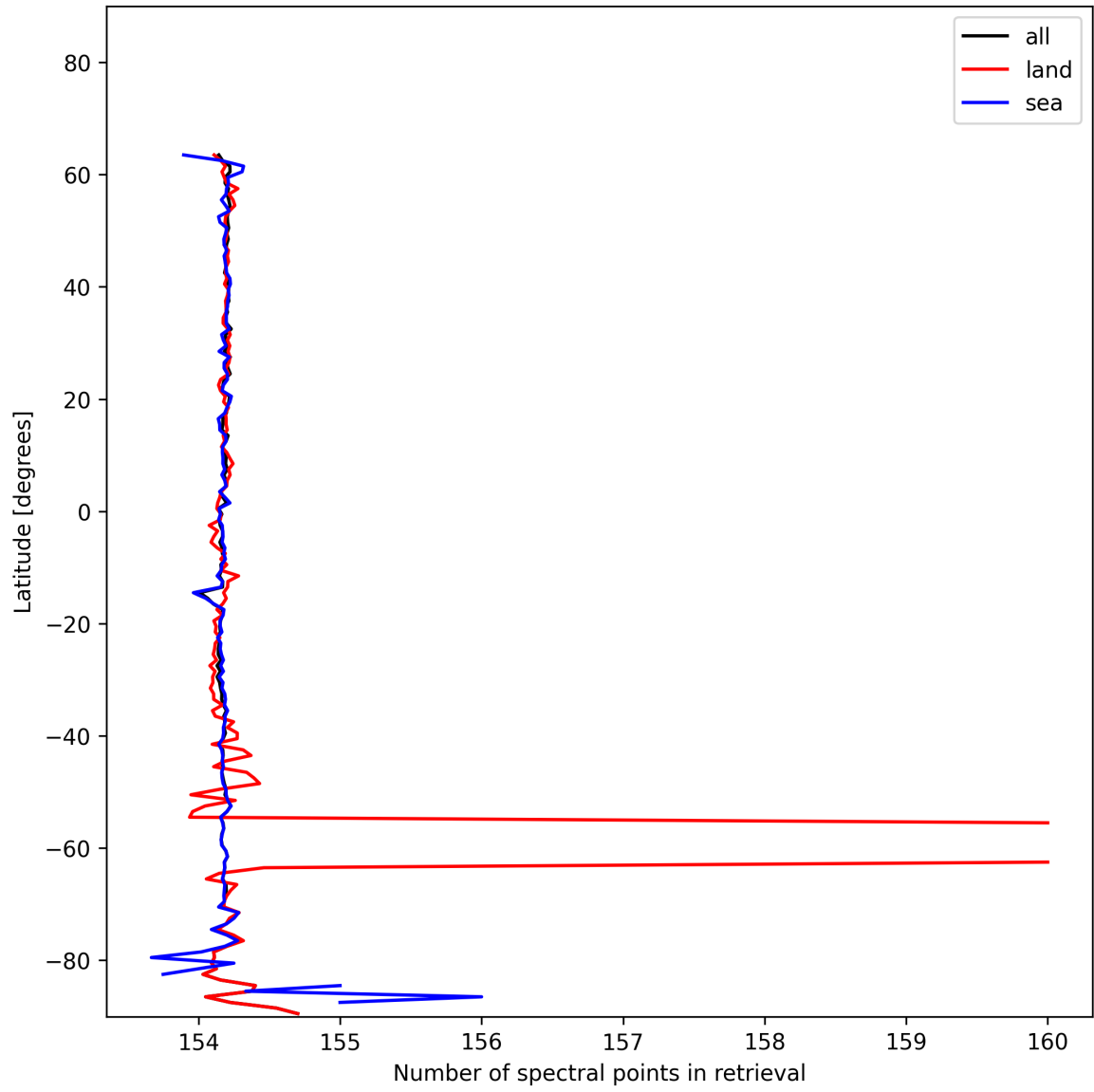
Figure 9: Zonal average of “Number of spectral points in retrieval” for 2025-01-12 to 2025-01-13.
