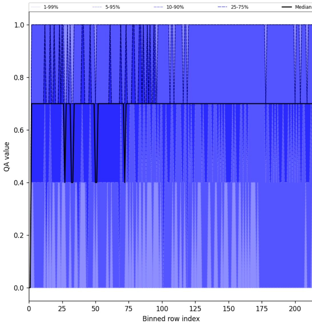
Figure 20: Along track statistics of “QA value” for 2025-01-12 to 2025-01-13
