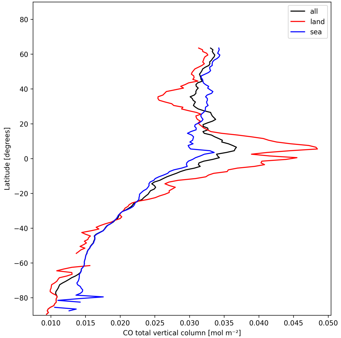
Figure 7: Zonal average of “CO total vertical column” for 2025-01-14 to 2025-01-15.
