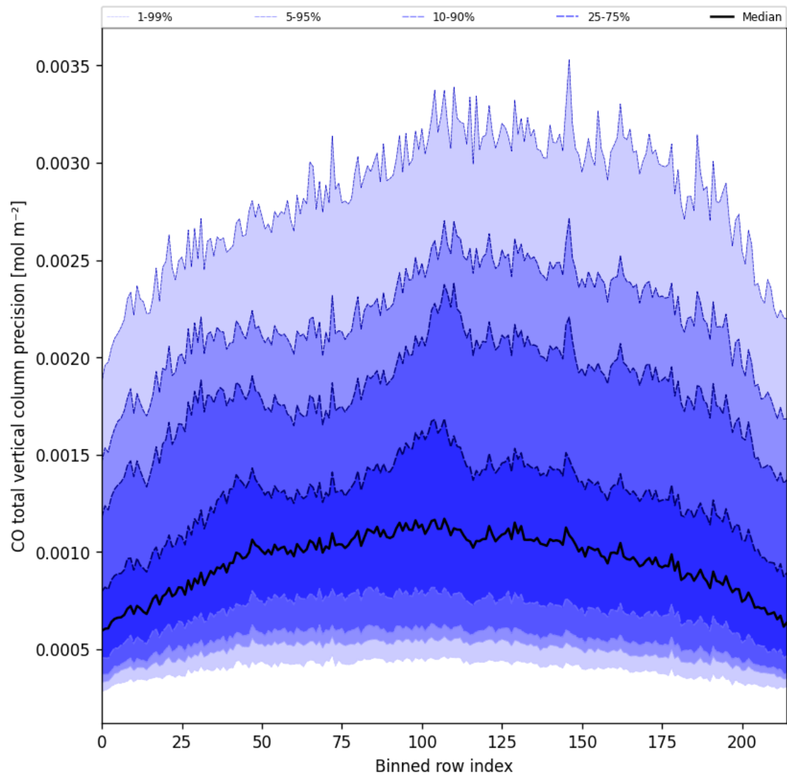
Figure 22: Along track statistics of “CO total vertical column precision” for 2025-01-14 to 2025-01-15
