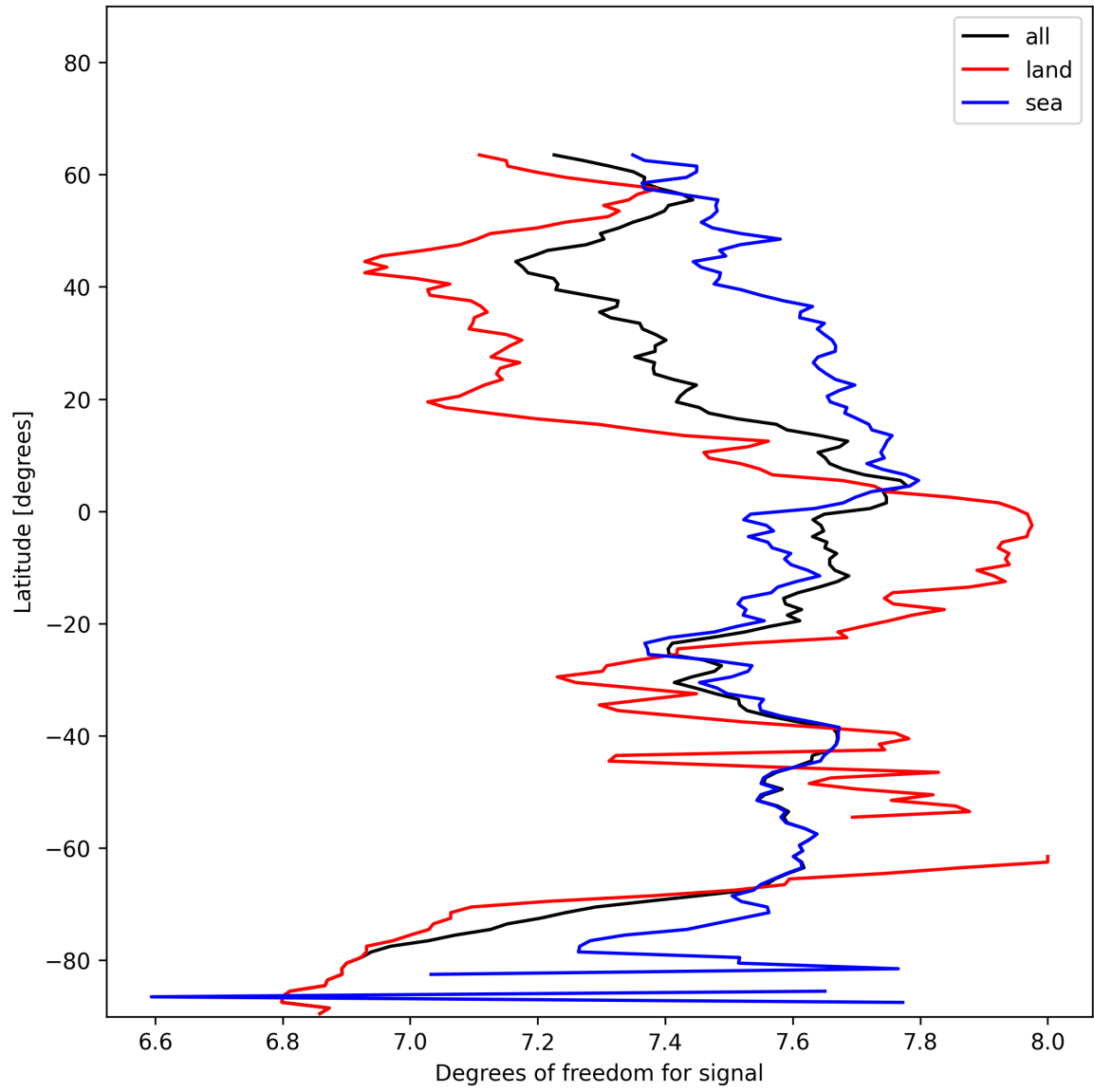
Figure 11: Zonal average of “Degrees of freedom for signal” for 2025-01-14 to 2025-01-15.
