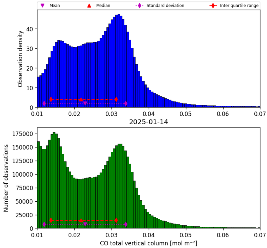
Figure 14: Histogram of “CO total vertical column” for 2025-01-14 to 2025-01-15
