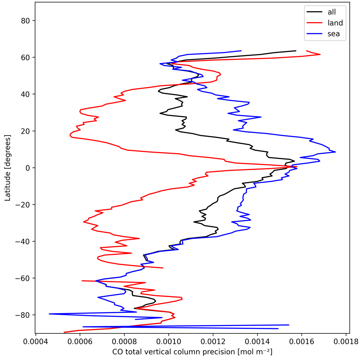
Figure 8: Zonal average of “CO total vertical column precision” for 2025-01-14 to 2025-01-15.
