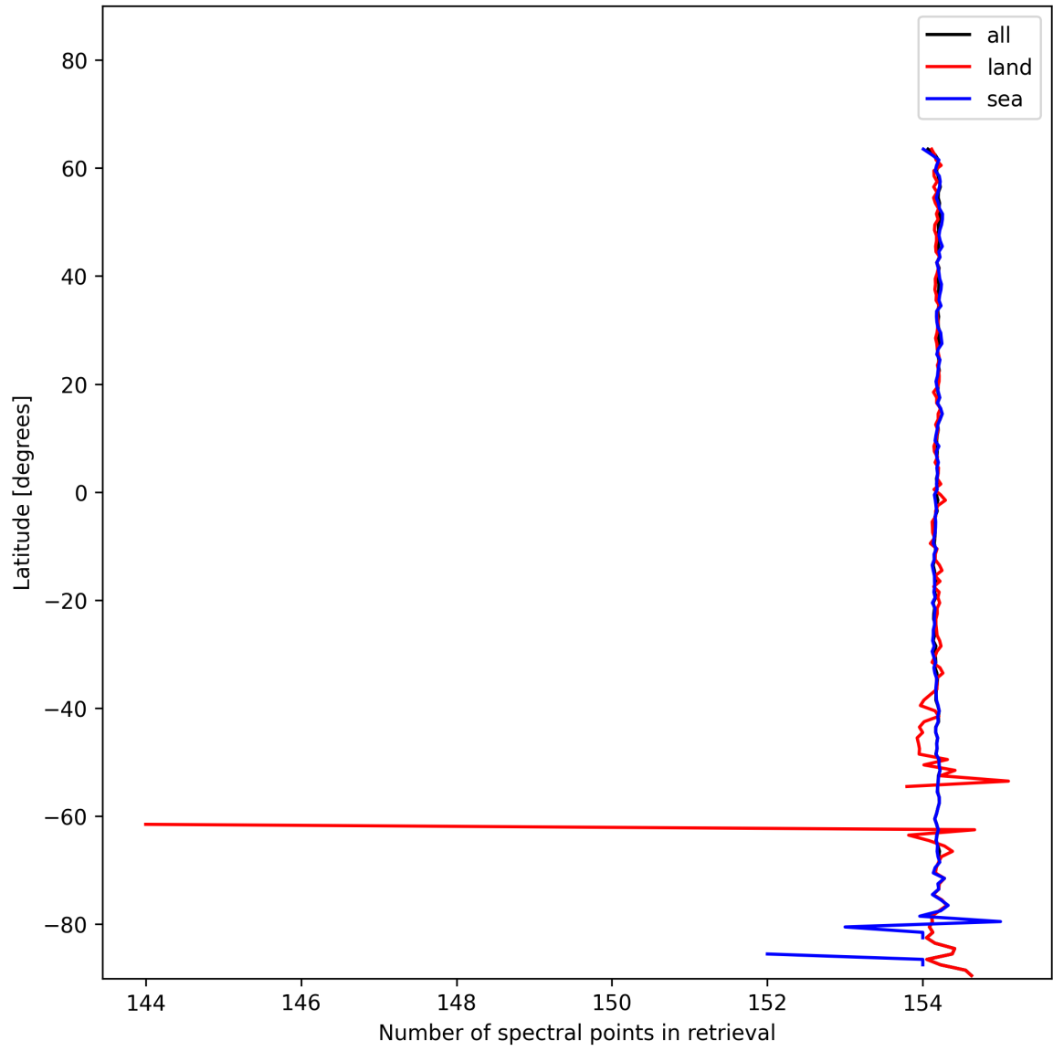
Figure 9: Zonal average of “Number of spectral points in retrieval” for 2025-01-14 to 2025-01-15.
