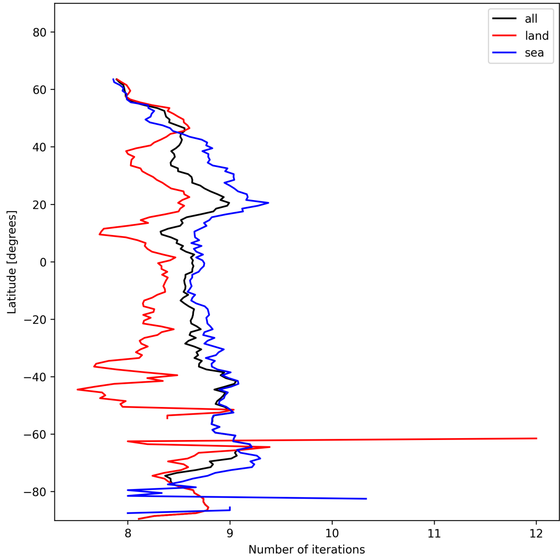
Figure 12: Zonal average of “Number of iterations” for 2025-01-14 to 2025-01-15.
