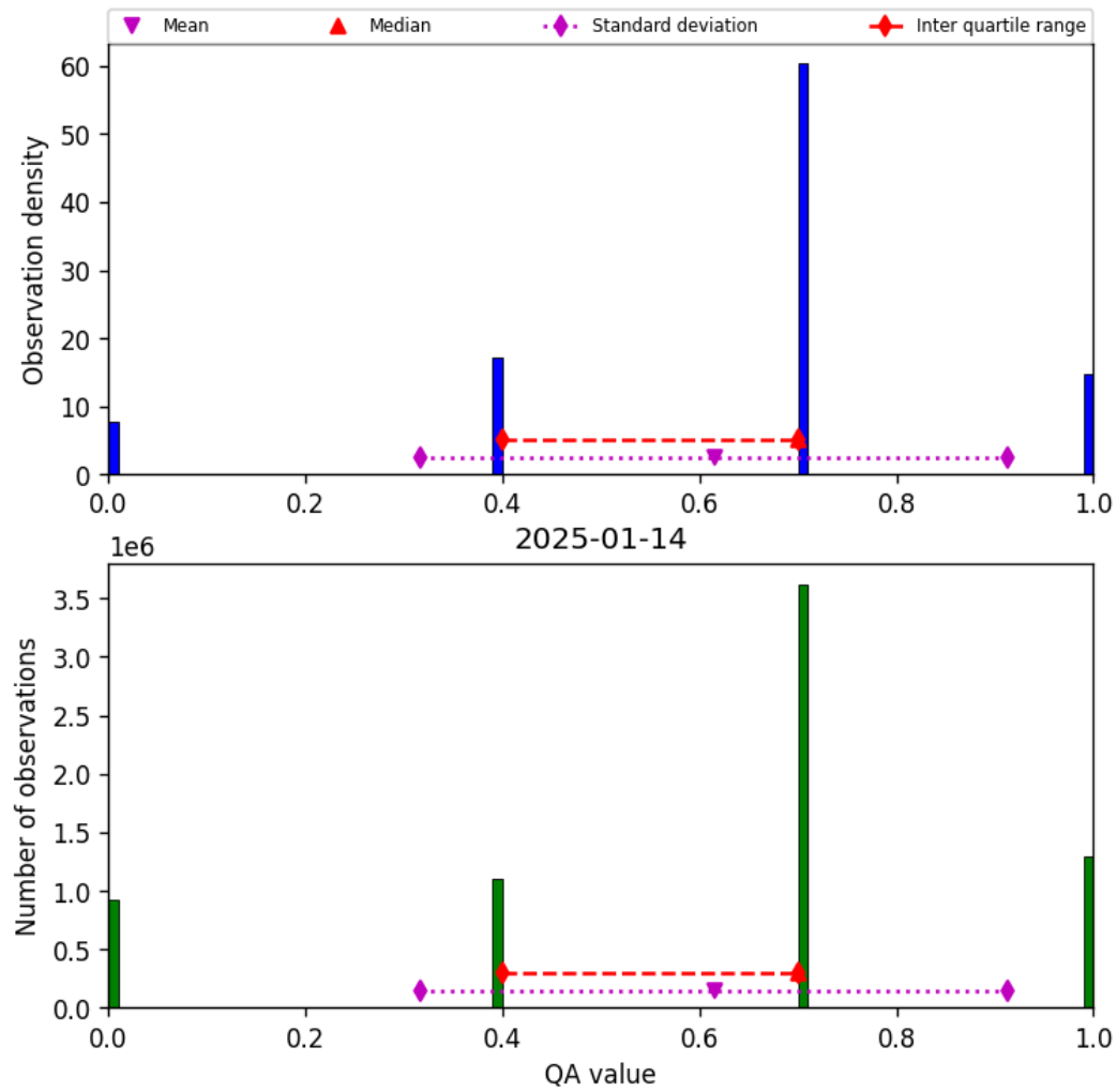
Figure 13: Histogram of “QA value” for 2025-01-14 to 2025-01-15
