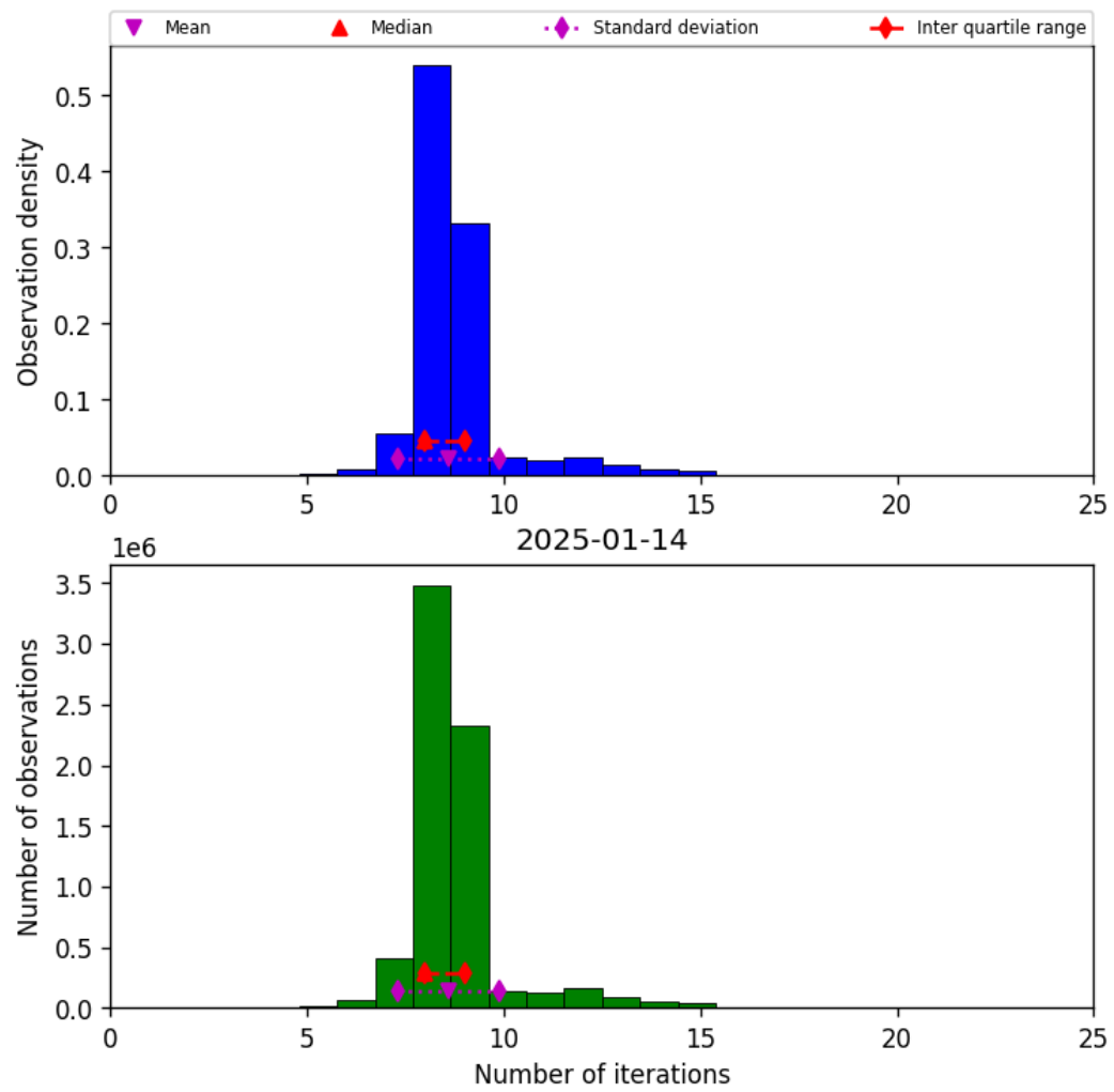
Figure 19: Histogram of “Number of iterations” for 2025-01-14 to 2025-01-15
