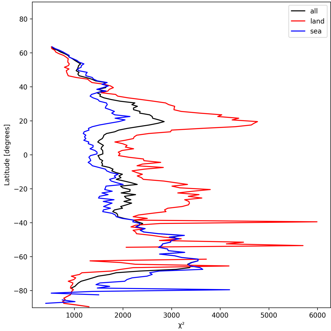
Figure 10: Zonal average of “ \chi^2 ” for 2025-01-14 to 2025-01-15.
