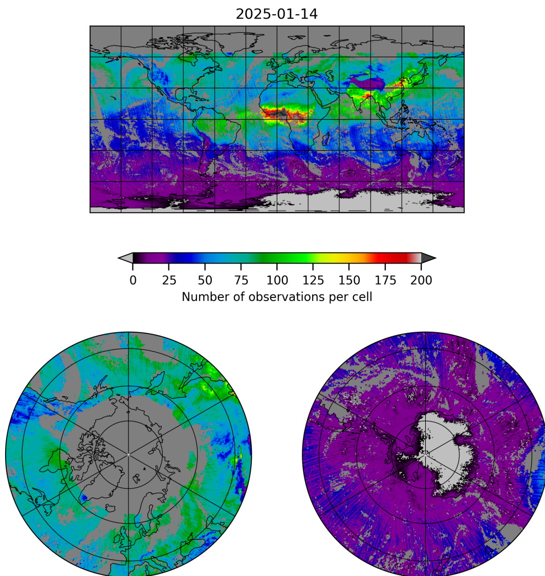
Figure 5: Map of the number of observations for 2025-01-14 to 2025-01-15
