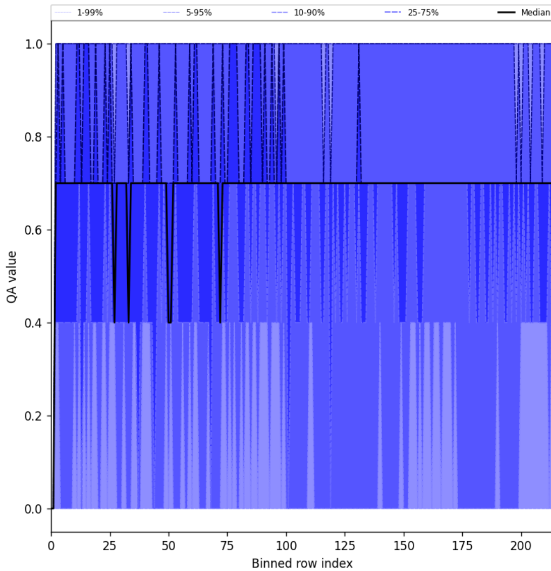
Figure 20: Along track statistics of “QA value” for 2025-01-14 to 2025-01-15
