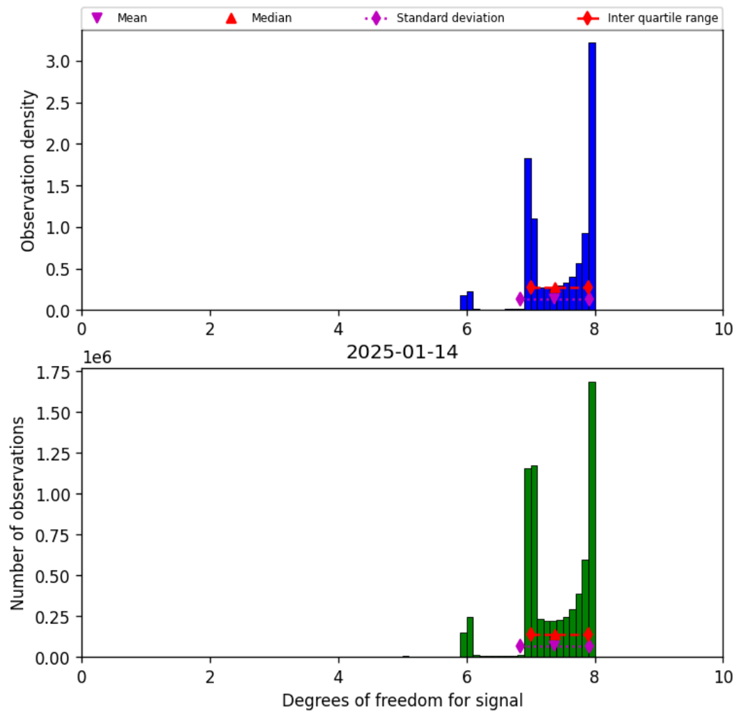
Figure 18: Histogram of “Degrees of freedom for signal” for 2025-01-14 to 2025-01-15
