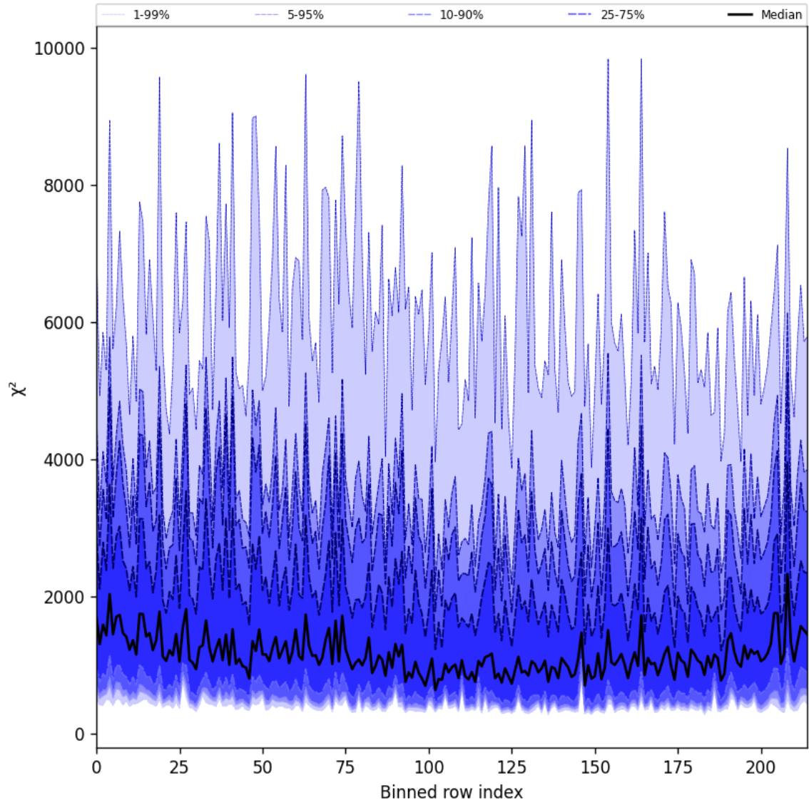
Figure 24: Along track statistics of “ \chi^2 ” for 2025-01-14 to 2025-01-15
