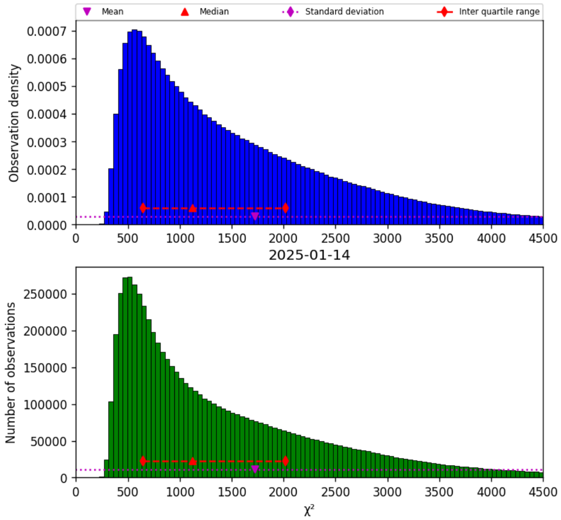
Figure 17: Histogram of “ \chi^2 ” for 2025-01-14 to 2025-01-15
