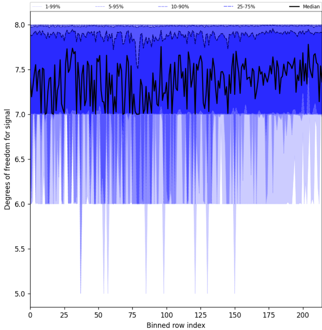
Figure 25: Along track statistics of “Degrees of freedom for signal” for 2025-01-14 to 2025-01-15
