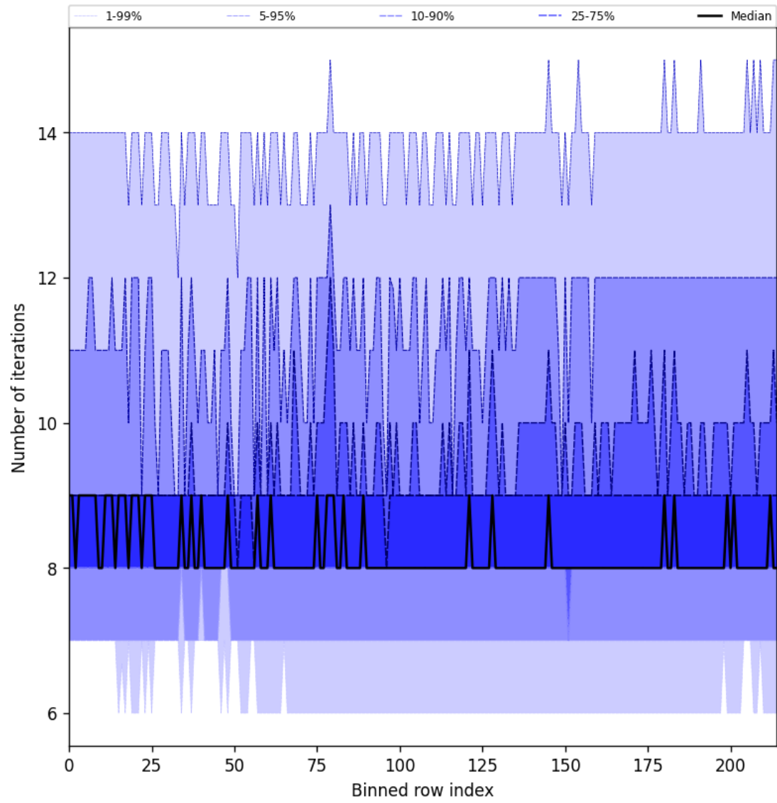
Figure 26: Along track statistics of “Number of iterations” for 2025-01-14 to 2025-01-15
