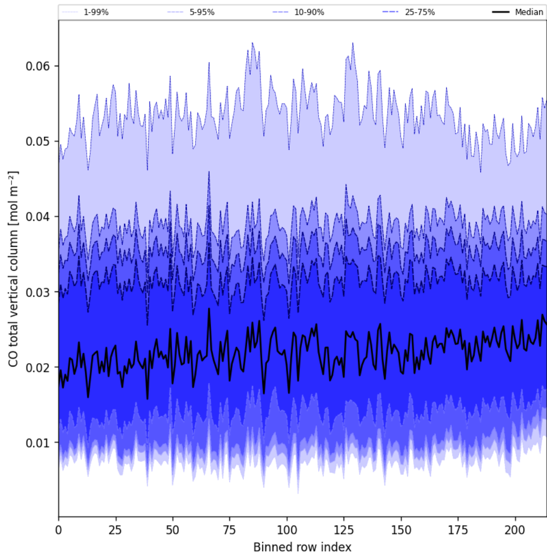
Figure 21: Along track statistics of “CO total vertical column” for 2025-01-14 to 2025-01-15
