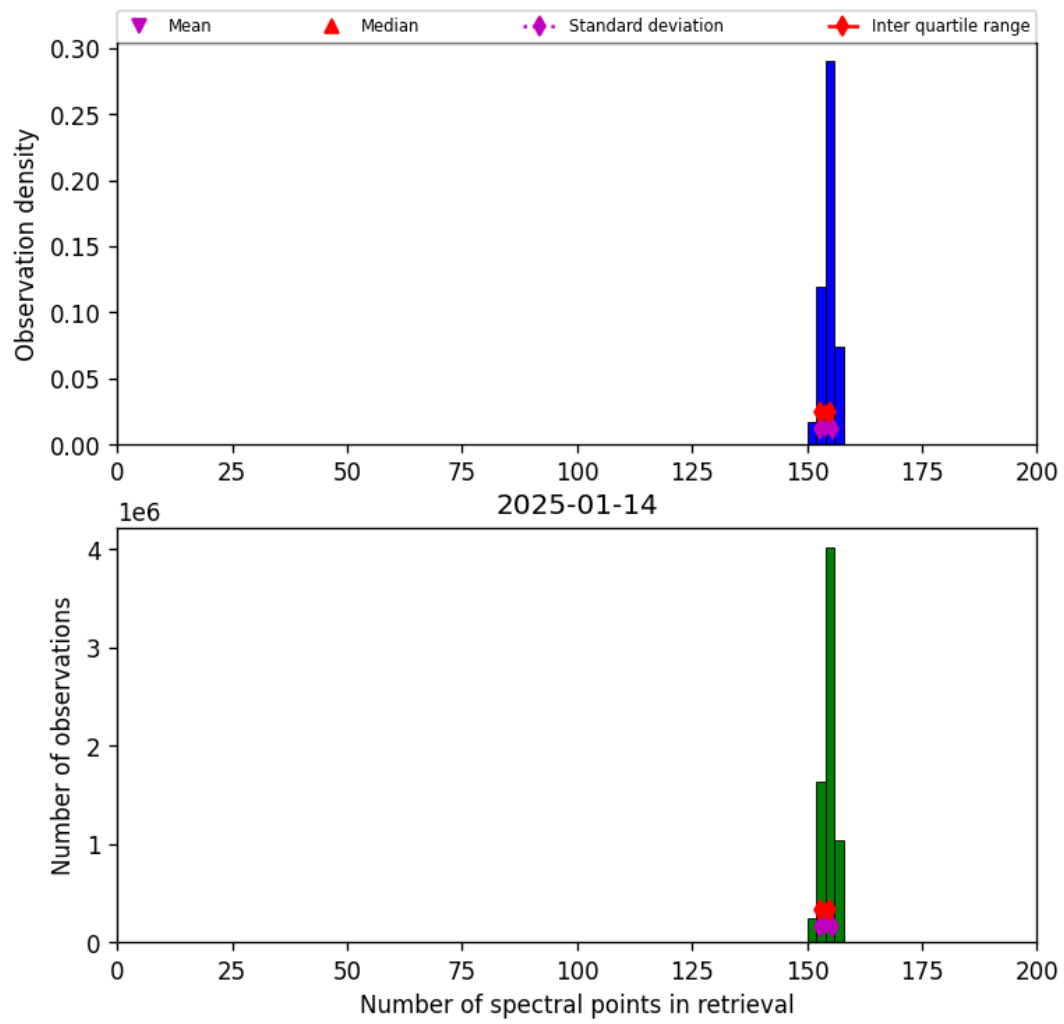
Figure 16: Histogram of “Number of spectral points in retrieval” for 2025-01-14 to 2025-01-15
