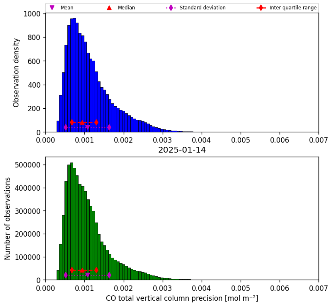
Figure 15: Histogram of “CO total vertical column precision” for 2025-01-14 to 2025-01-15
