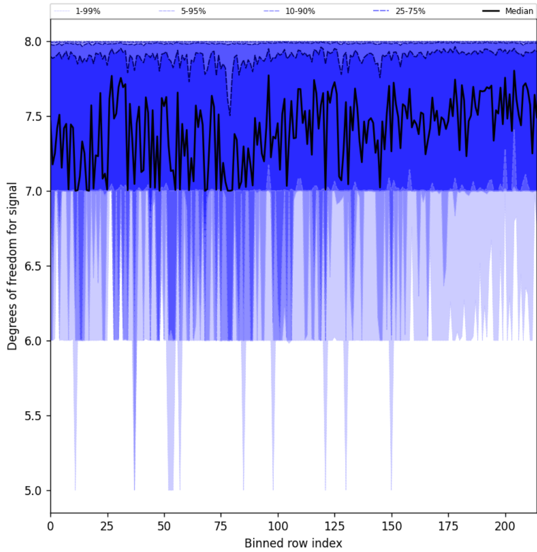
Figure 25: Along track statistics of “Degrees of freedom for signal” for 2025-01-16 to 2025-01-17
