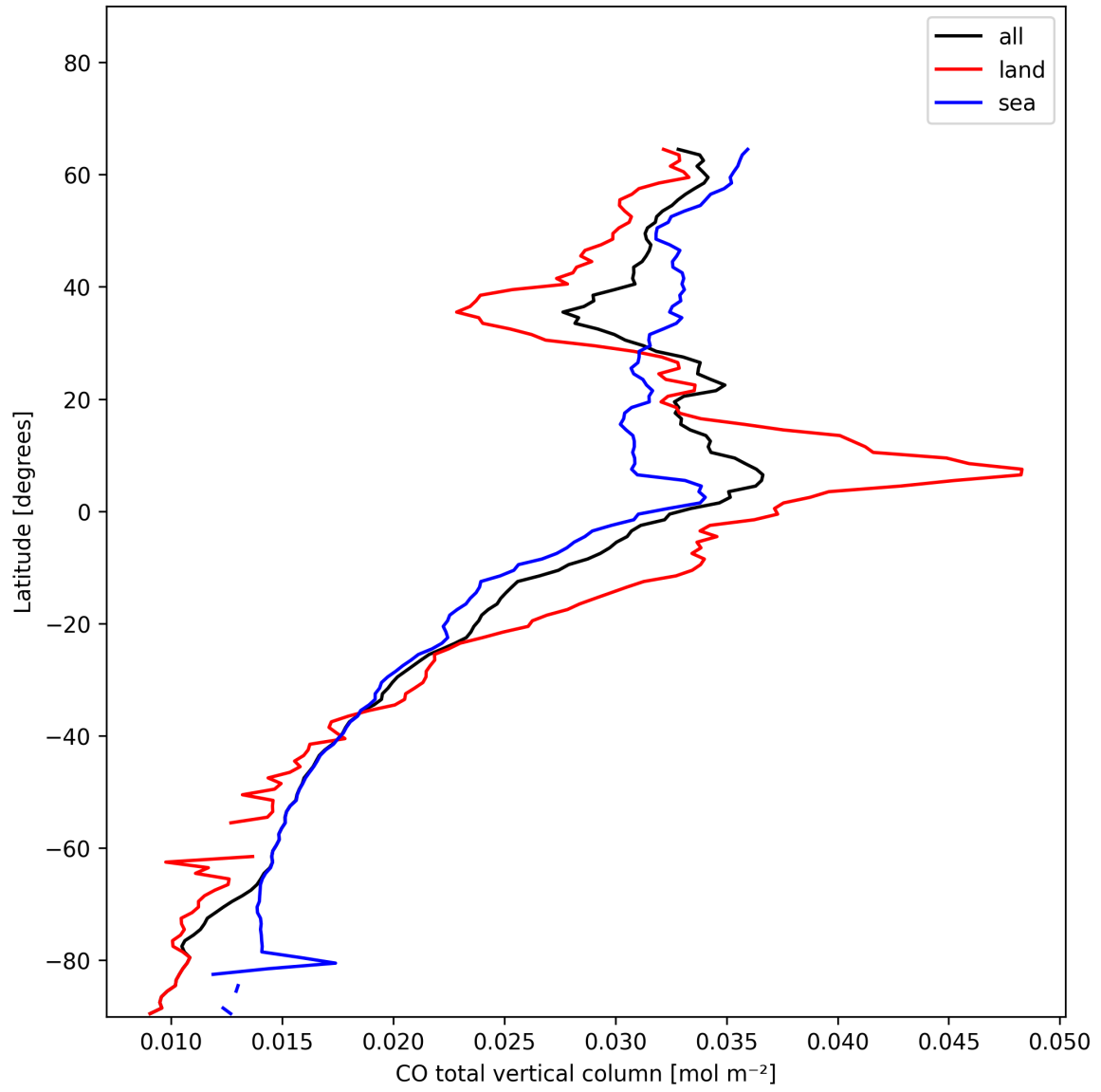
Figure 7: Zonal average of “CO total vertical column” for 2025-01-16 to 2025-01-17.
