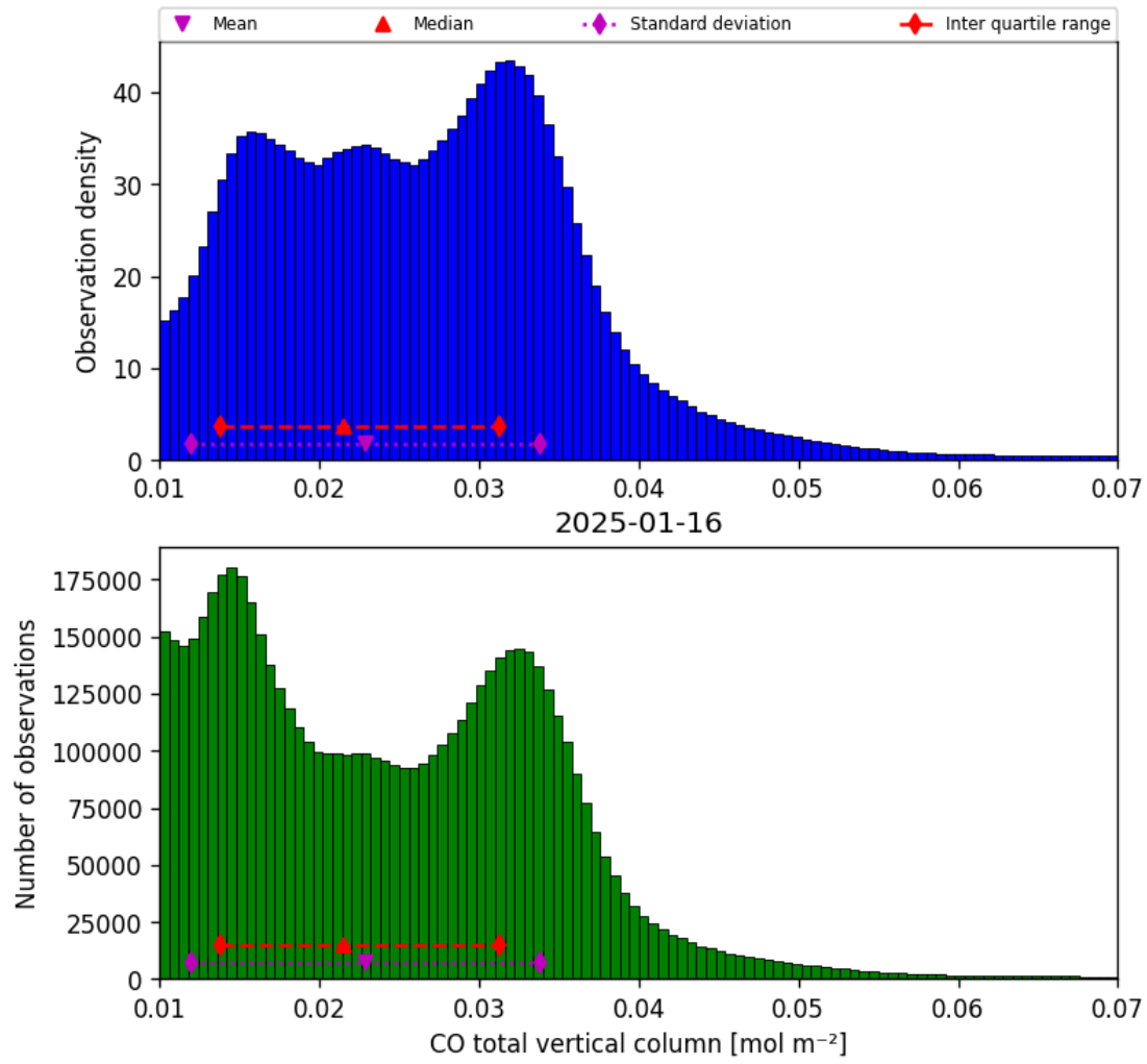
Figure 14: Histogram of “CO total vertical column” for 2025-01-16 to 2025-01-17
