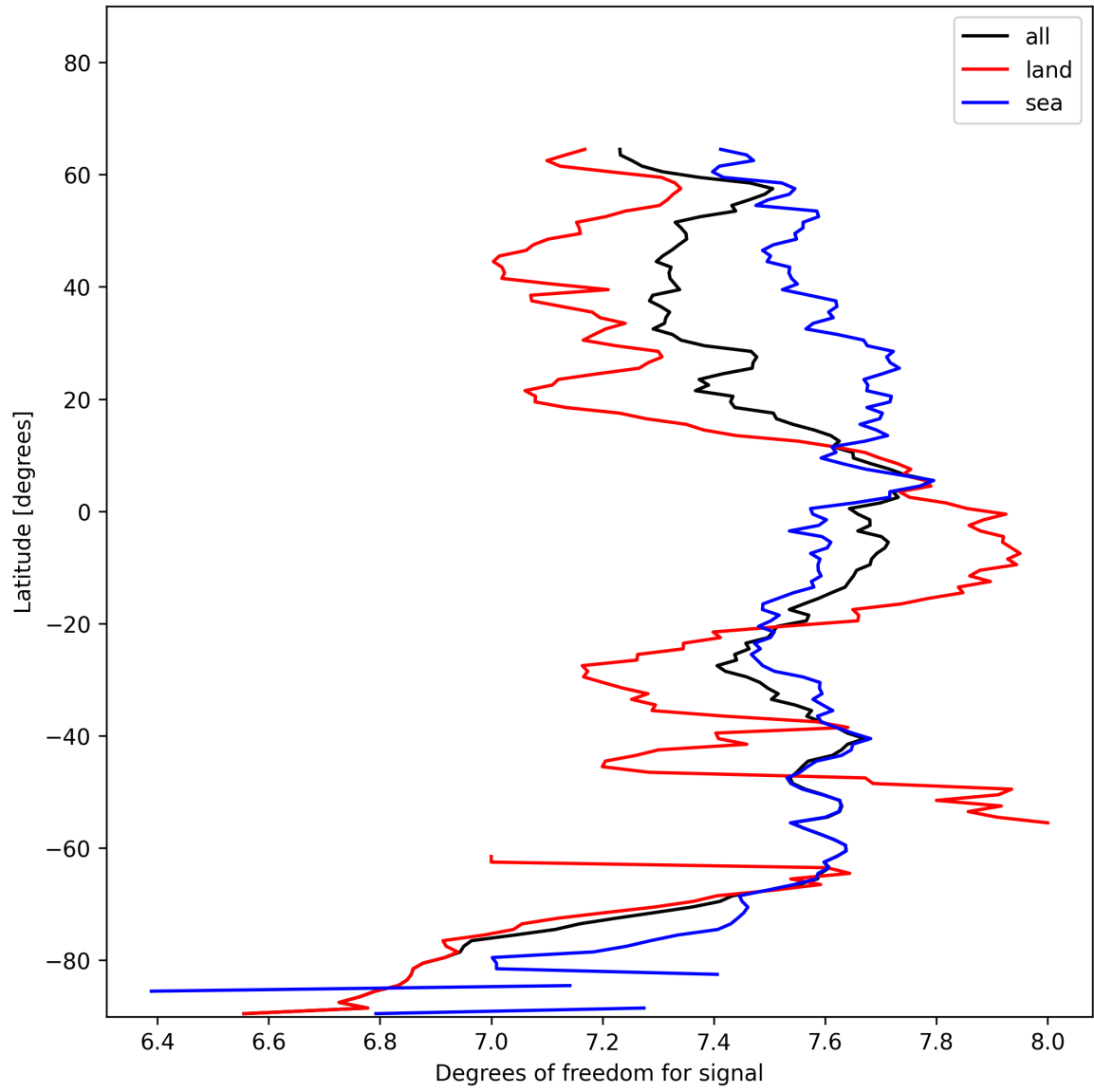
Figure 11: Zonal average of “Degrees of freedom for signal” for 2025-01-16 to 2025-01-17.
