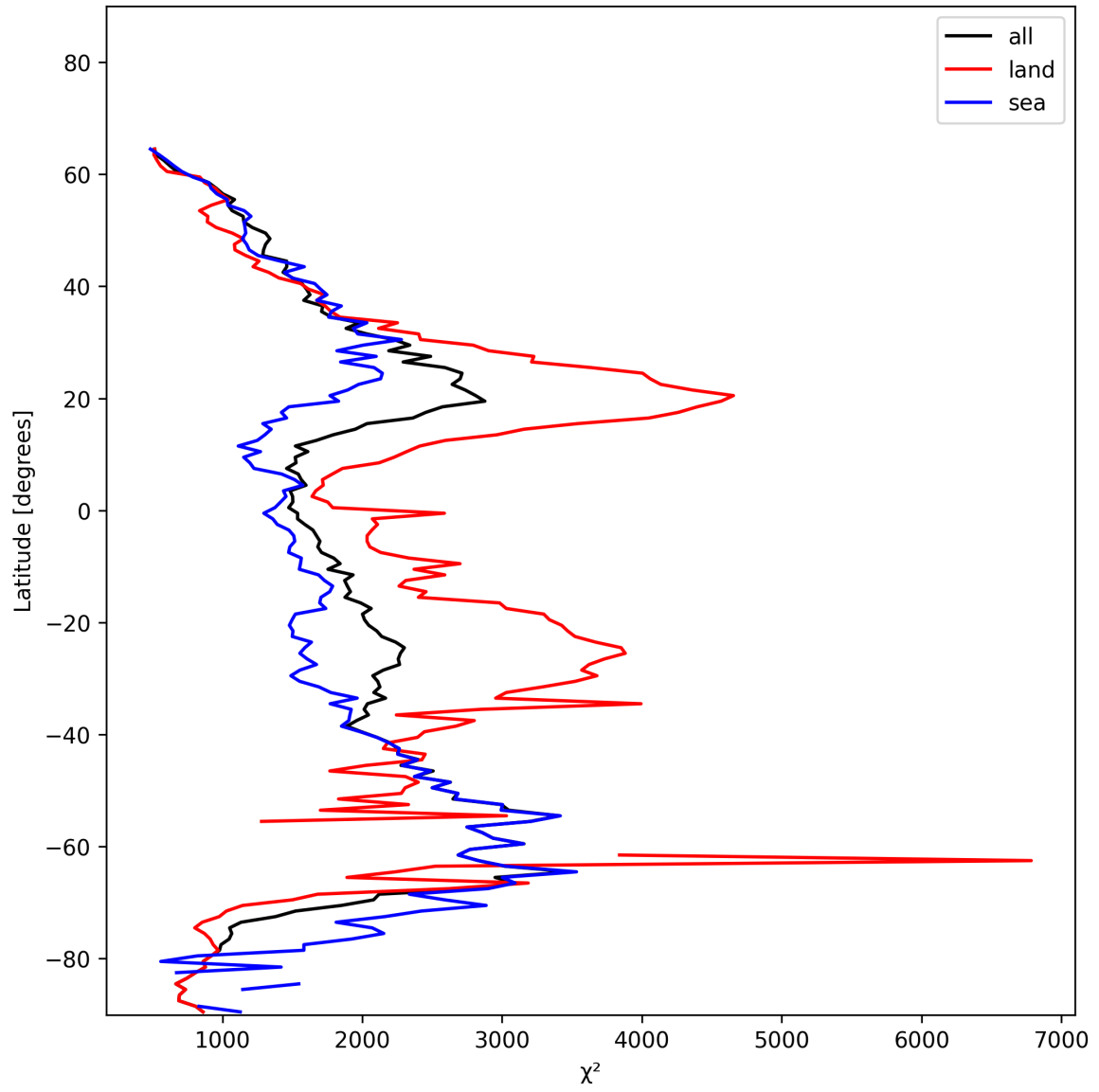
Figure 10: Zonal average of “ \chi^2 ” for 2025-01-16 to 2025-01-17.
