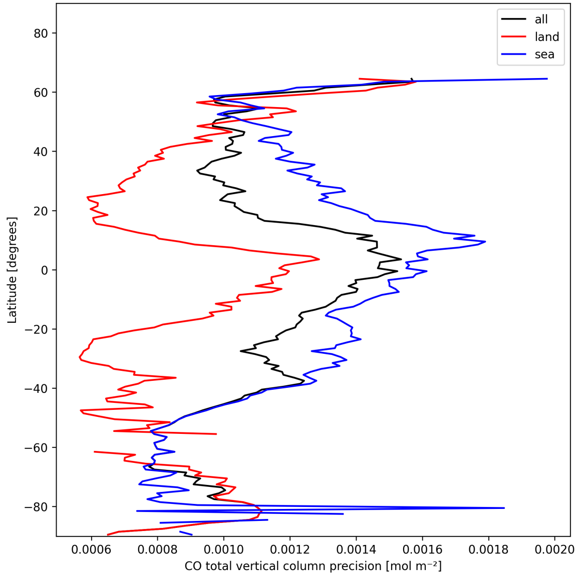
Figure 8: Zonal average of “CO total vertical column precision” for 2025-01-16 to 2025-01-17.
