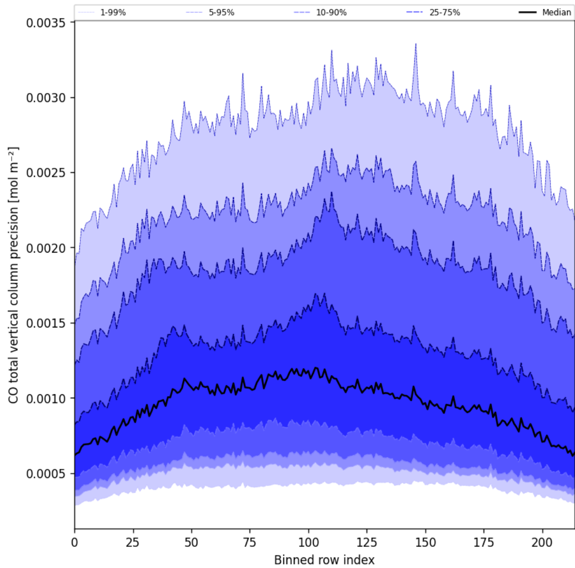
Figure 22: Along track statistics of “CO total vertical column precision” for 2025-01-16 to 2025-01-17
