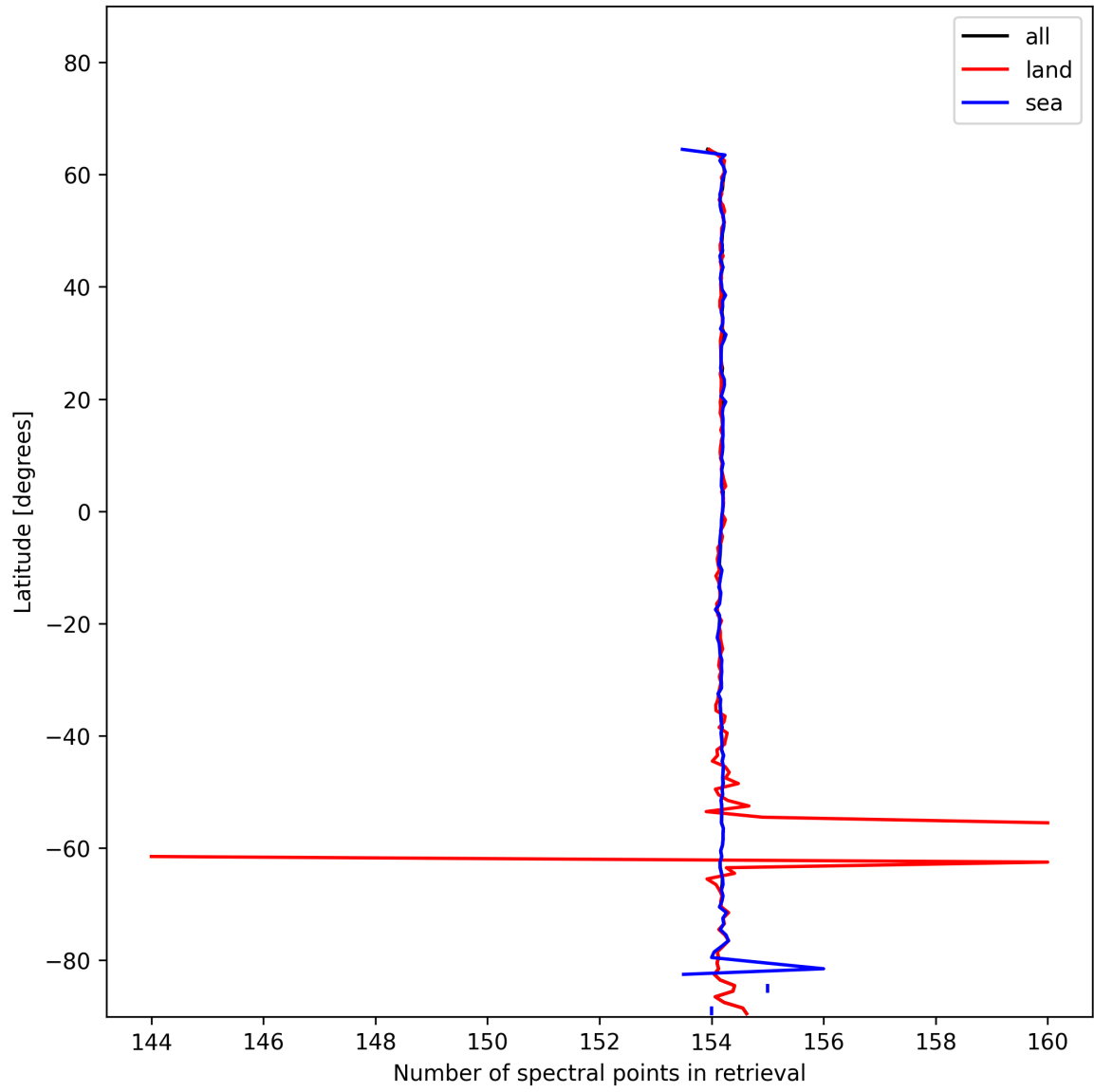
Figure 9: Zonal average of “Number of spectral points in retrieval” for 2025-01-16 to 2025-01-17.
