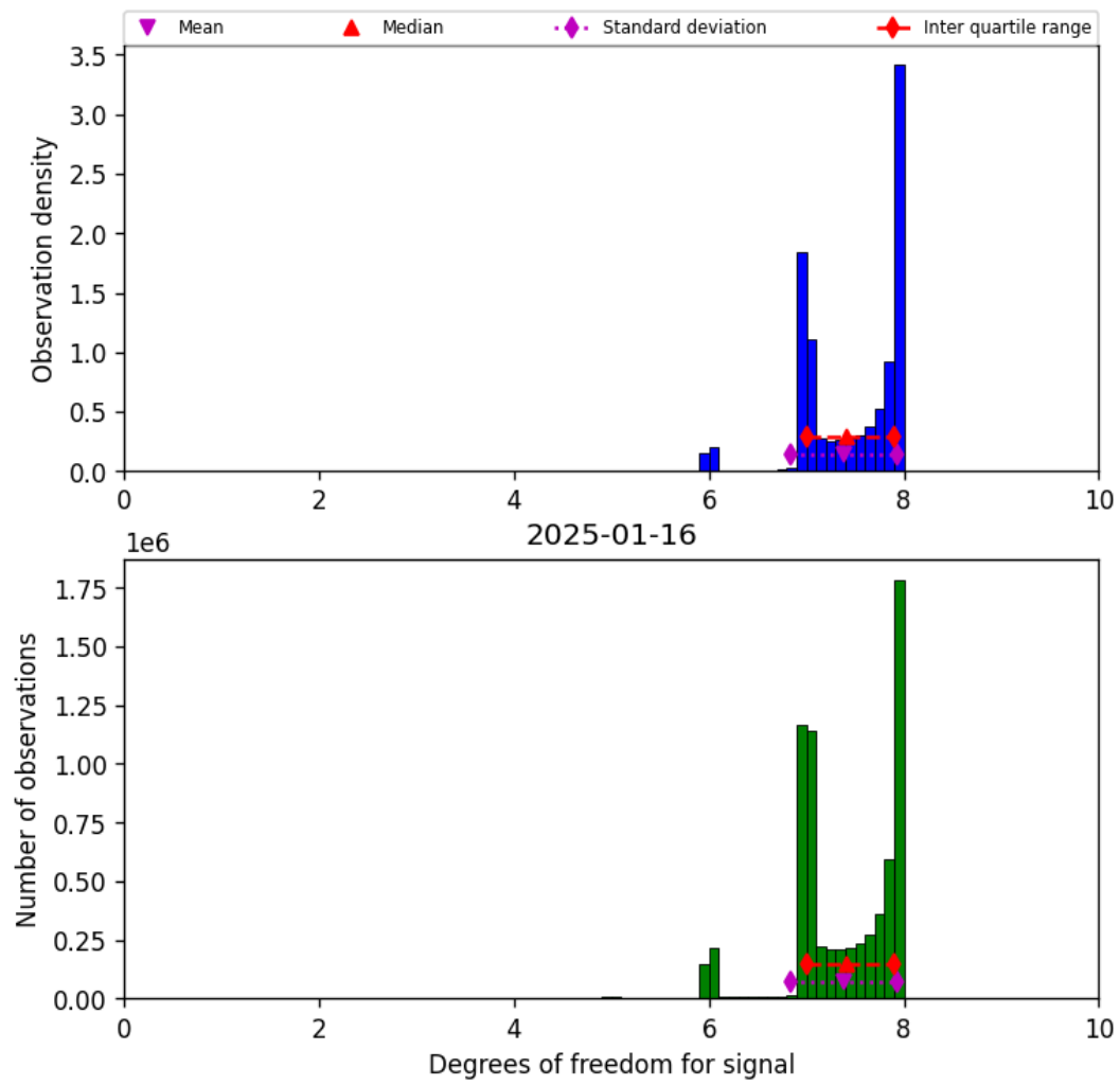
Figure 18: Histogram of “Degrees of freedom for signal” for 2025-01-16 to 2025-01-17
