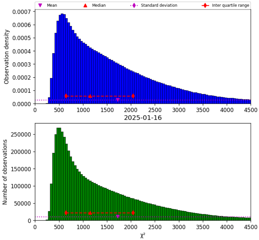
Figure 17: Histogram of “ \chi^2 ” for 2025-01-16 to 2025-01-17
