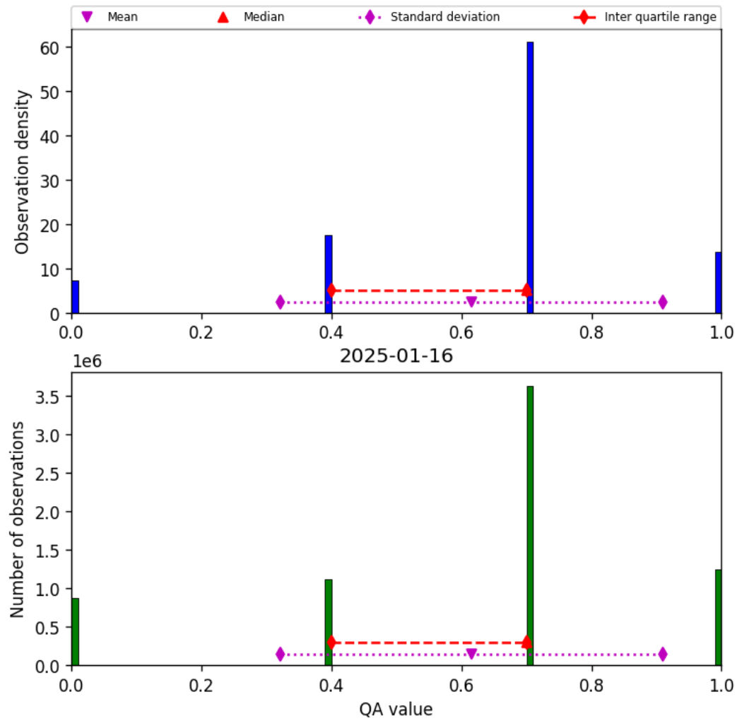
Figure 13: Histogram of “QA value” for 2025-01-16 to 2025-01-17
