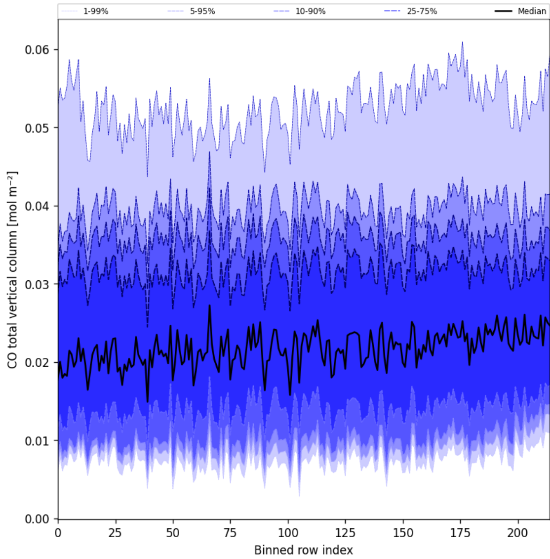
Figure 21: Along track statistics of “CO total vertical column” for 2025-01-16 to 2025-01-17
