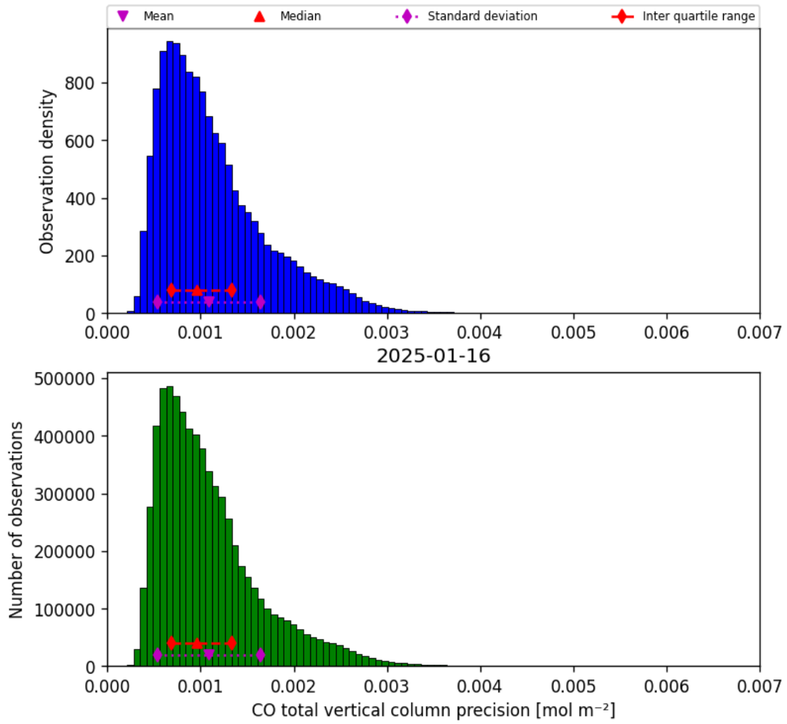
Figure 15: Histogram of “CO total vertical column precision” for 2025-01-16 to 2025-01-17
