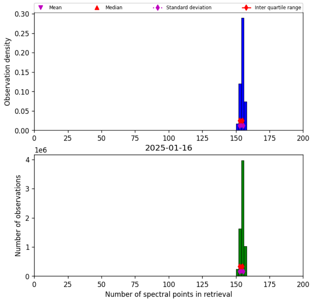
Figure 16: Histogram of “Number of spectral points in retrieval” for 2025-01-16 to 2025-01-17
