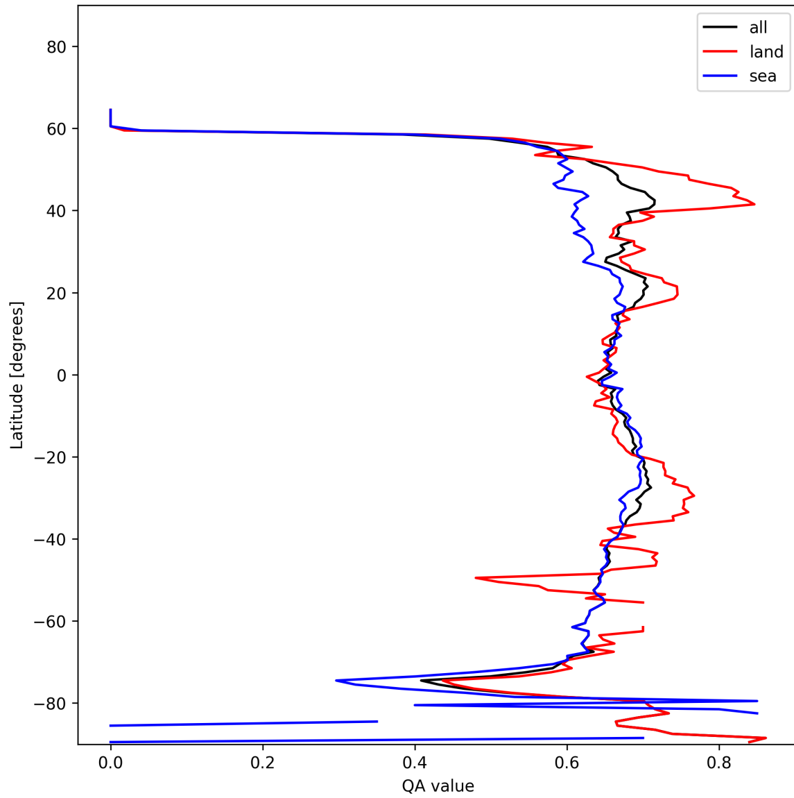
Figure 6: Zonal average of “QA value” for 2025-01-16 to 2025-01-17.
