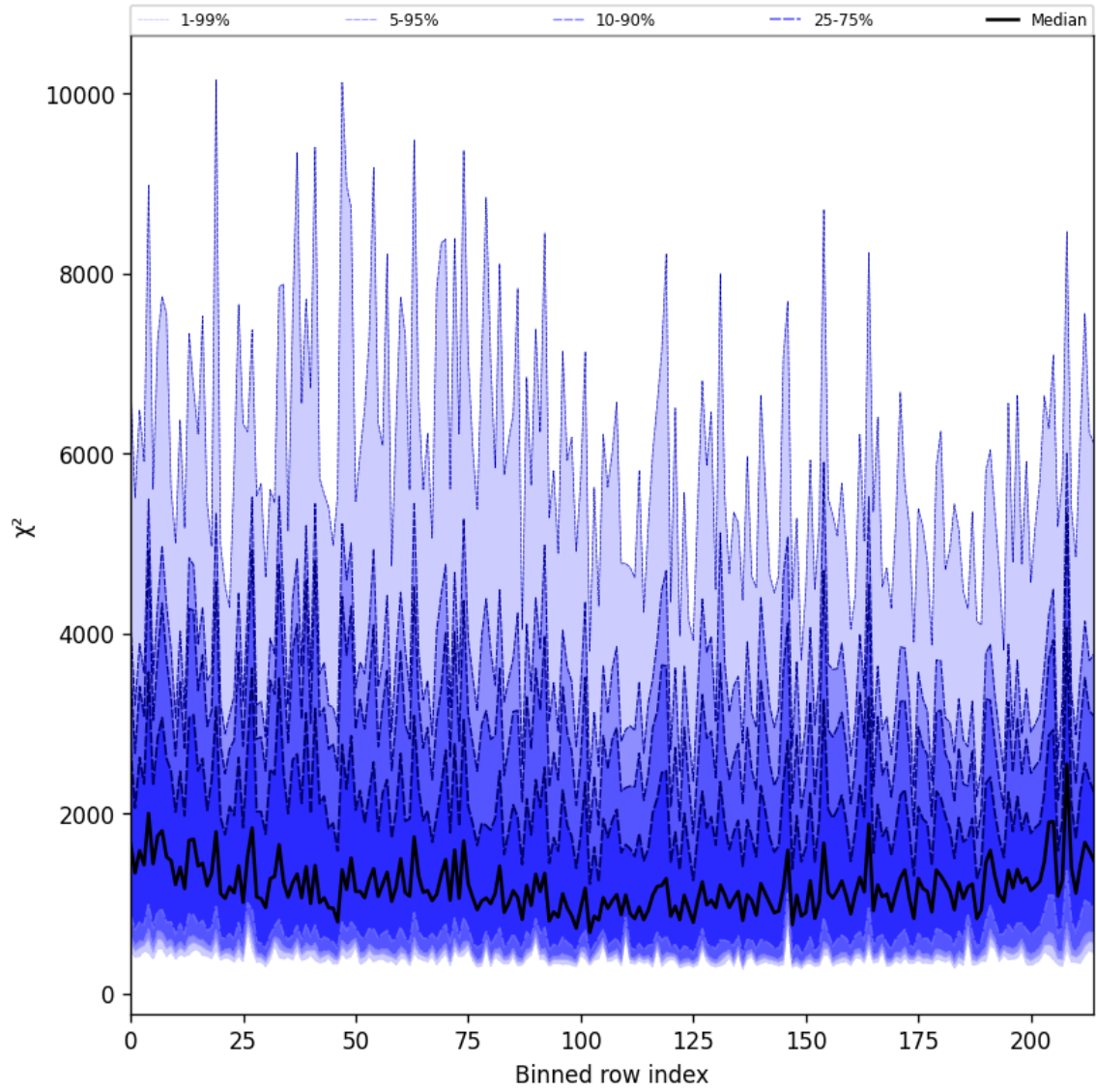
Figure 24: Along track statistics of “ \chi^2 ” for 2025-01-16 to 2025-01-17
