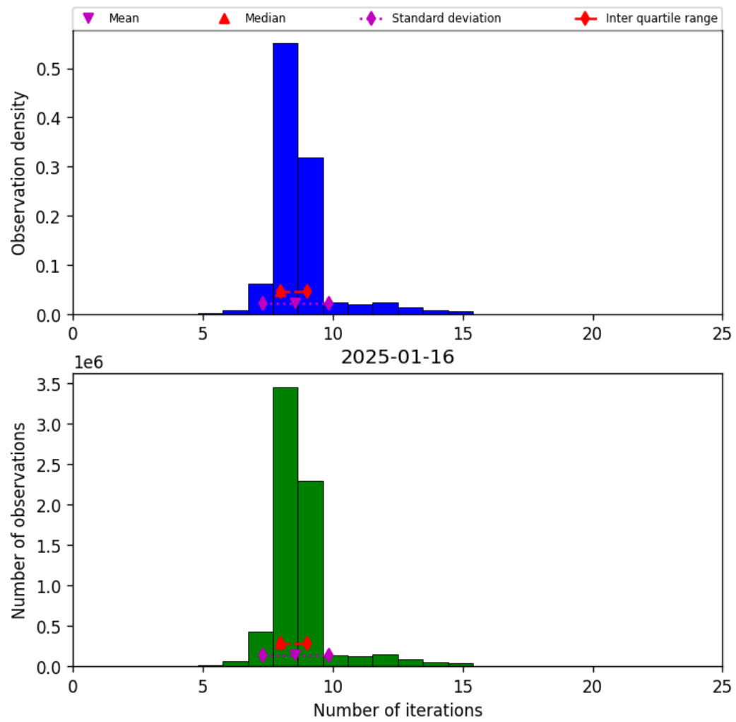
Figure 19: Histogram of “Number of iterations” for 2025-01-16 to 2025-01-17
