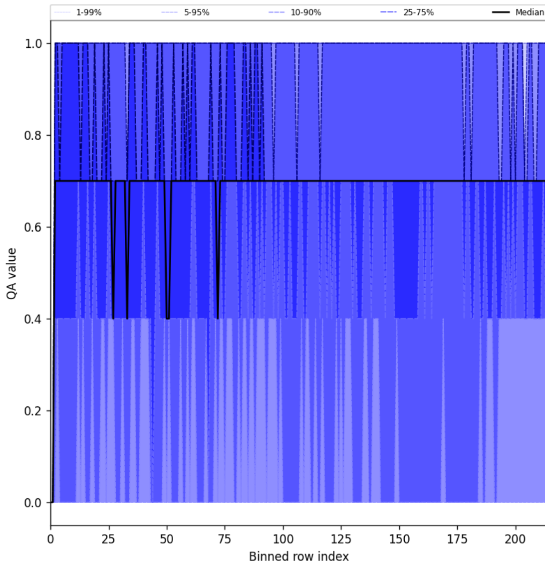
Figure 20: Along track statistics of “QA value” for 2025-01-16 to 2025-01-17
