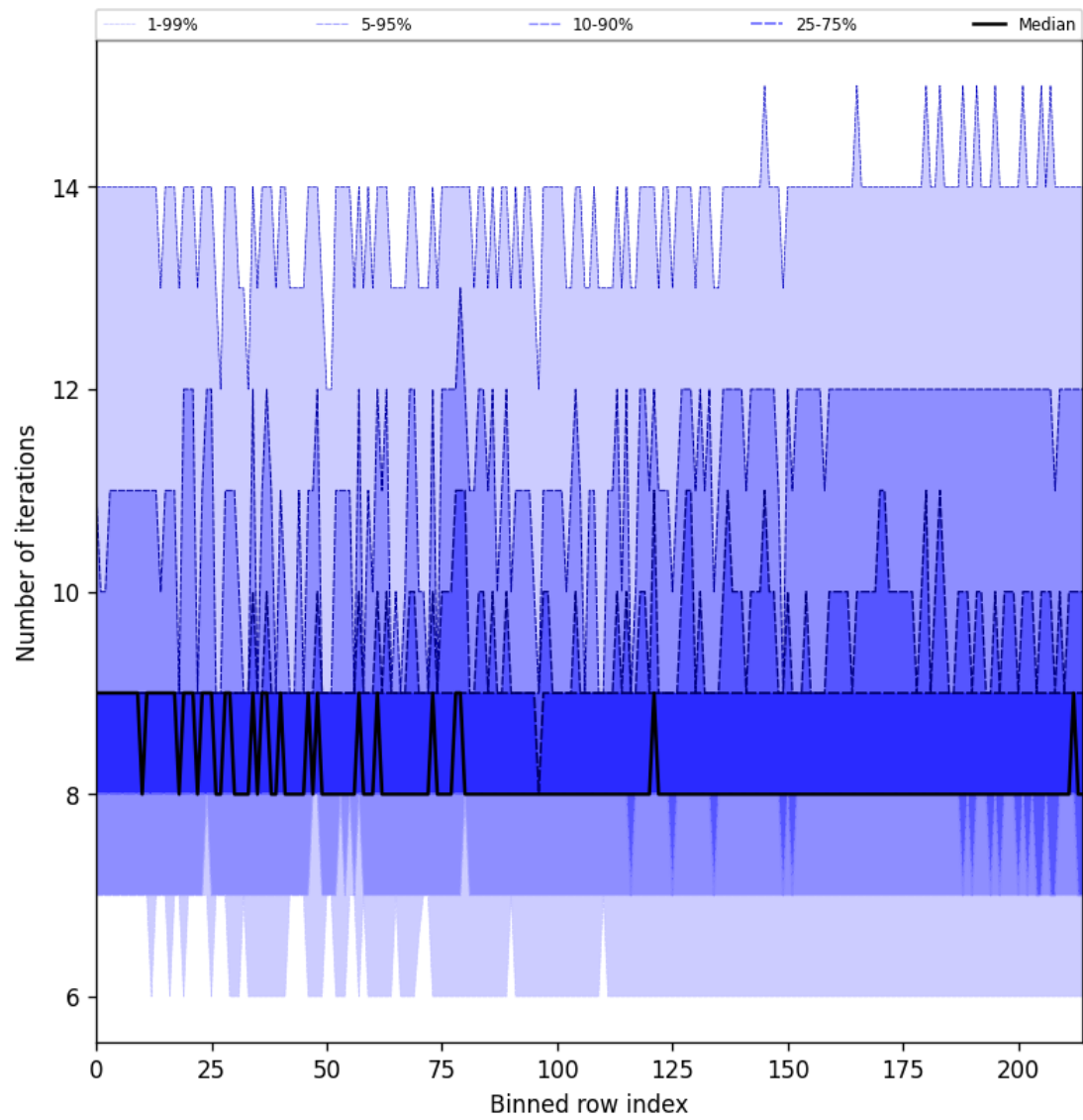
Figure 26: Along track statistics of “Number of iterations” for 2025-01-16 to 2025-01-17
