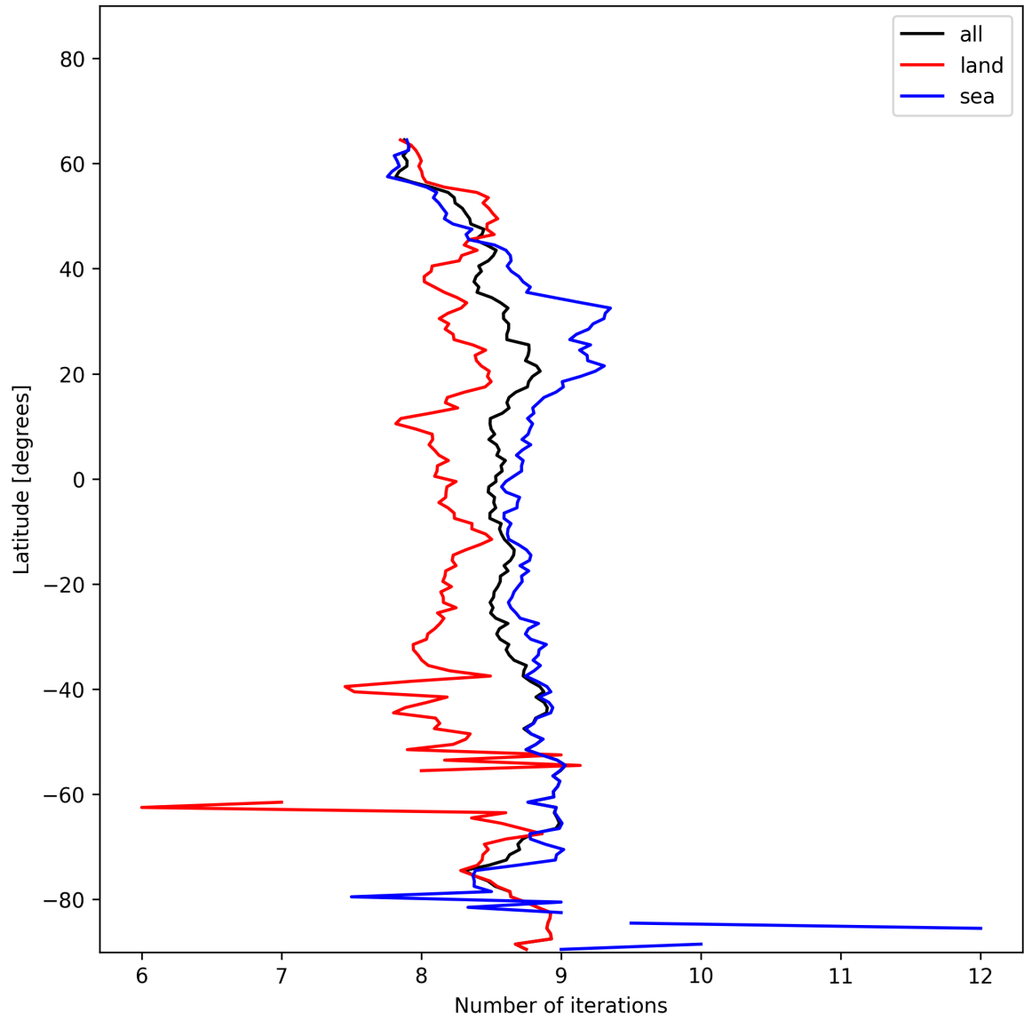
Figure 12: Zonal average of “Number of iterations” for 2025-01-16 to 2025-01-17.
