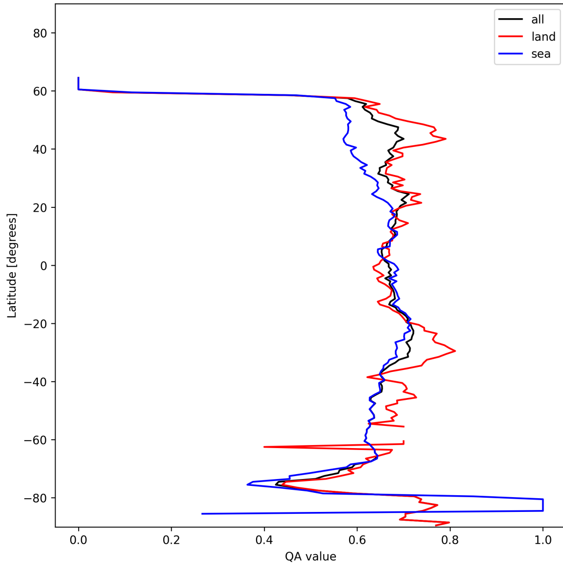
Figure 6: Zonal average of “QA value” for 2025-01-17 to 2025-01-18.
