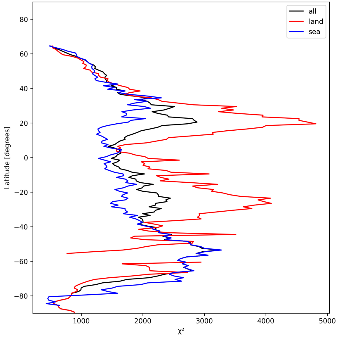
Figure 10: Zonal average of “ \chi^2 ” for 2025-01-17 to 2025-01-18.
