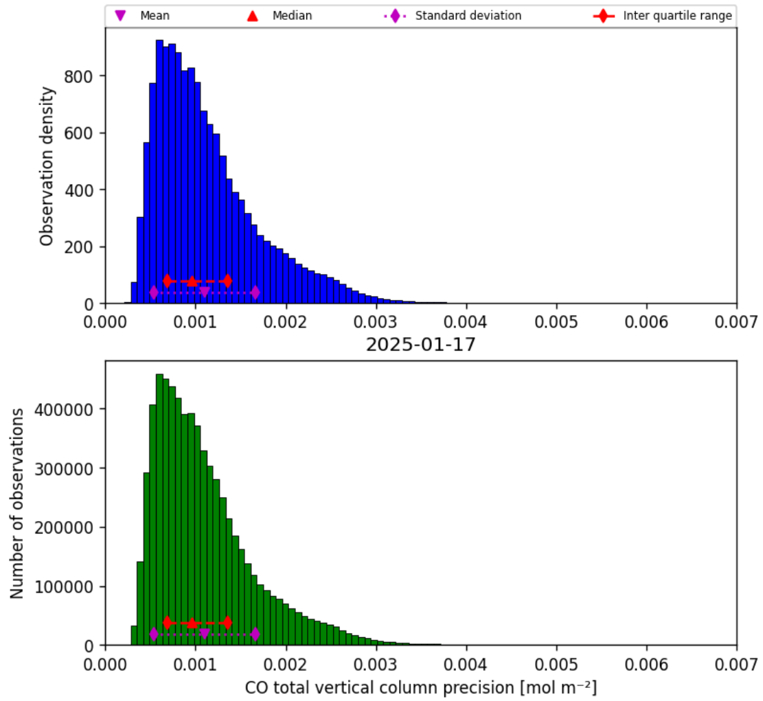
Figure 15: Histogram of “CO total vertical column precision” for 2025-01-17 to 2025-01-18
