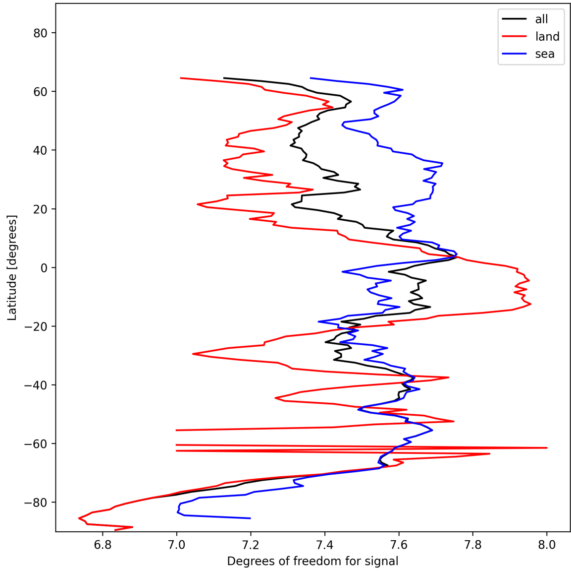
Figure 11: Zonal average of “Degrees of freedom for signal” for 2025-01-17 to 2025-01-18.
