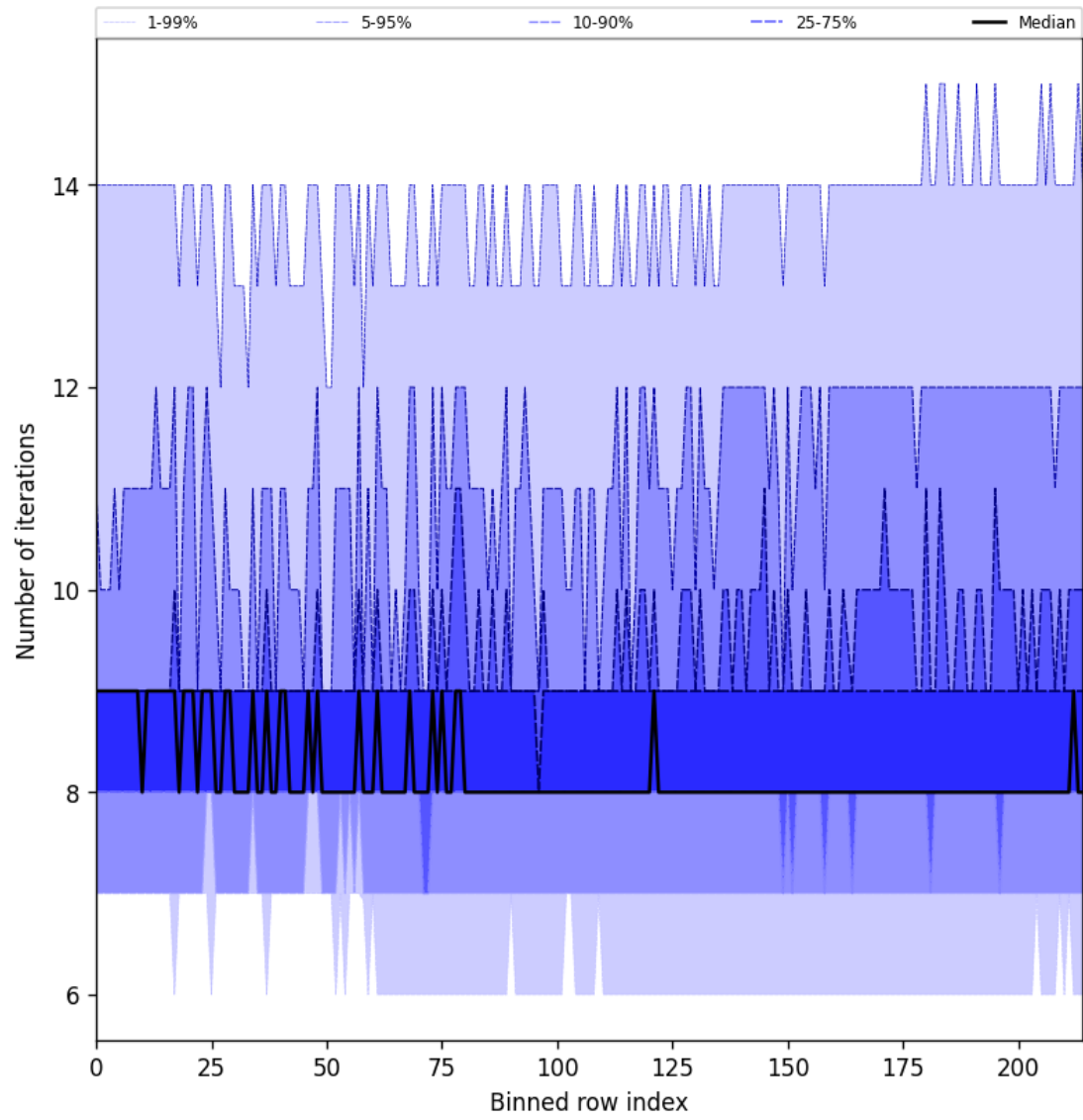
Figure 26: Along track statistics of “Number of iterations” for 2025-01-17 to 2025-01-18
