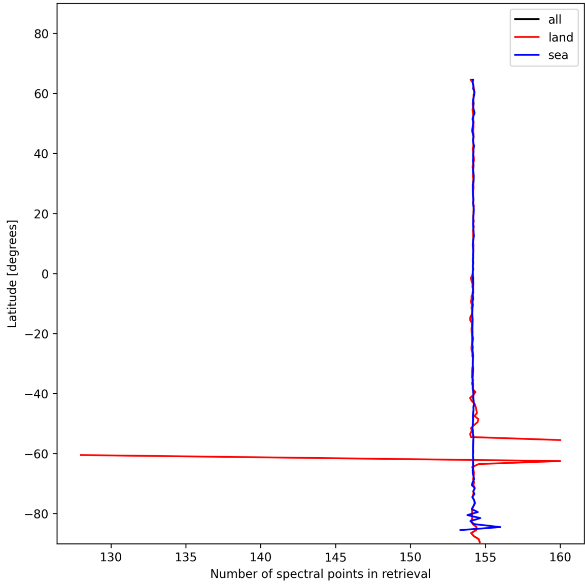
Figure 9: Zonal average of “Number of spectral points in retrieval” for 2025-01-17 to 2025-01-18.
