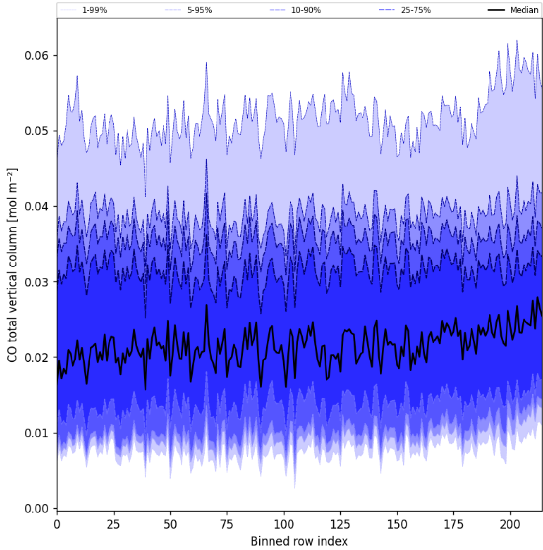
Figure 21: Along track statistics of “CO total vertical column” for 2025-01-17 to 2025-01-18
