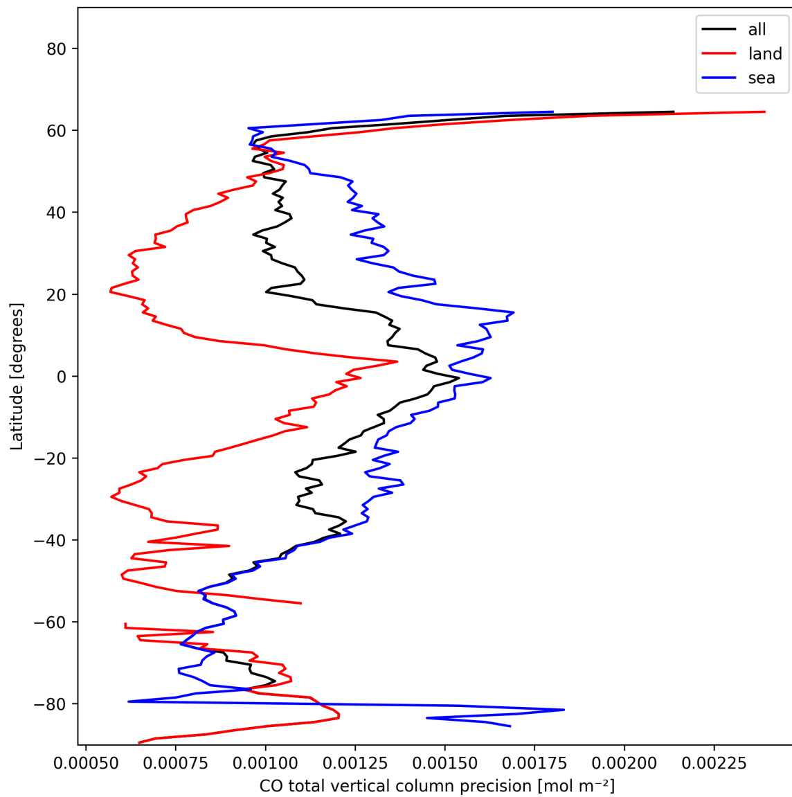
Figure 8: Zonal average of “CO total vertical column precision” for 2025-01-17 to 2025-01-18.
