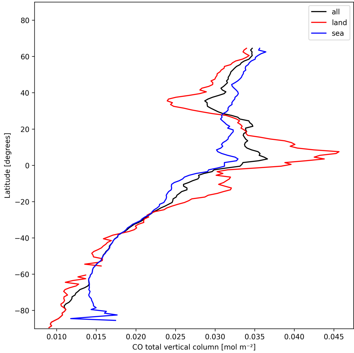
Figure 7: Zonal average of “CO total vertical column” for 2025-01-17 to 2025-01-18.
