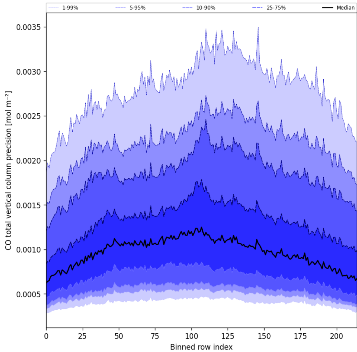
Figure 22: Along track statistics of “CO total vertical column precision” for 2025-01-17 to 2025-01-18
