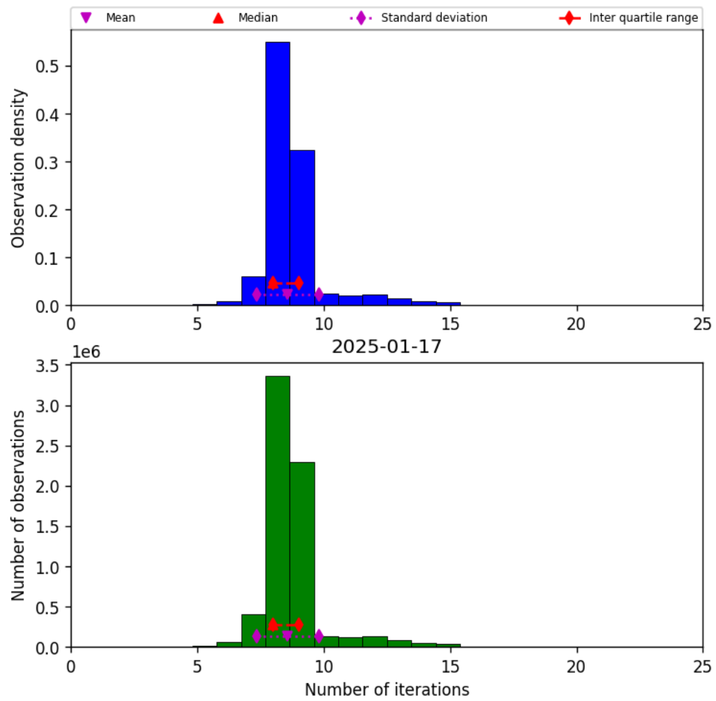
Figure 19: Histogram of “Number of iterations” for 2025-01-17 to 2025-01-18
