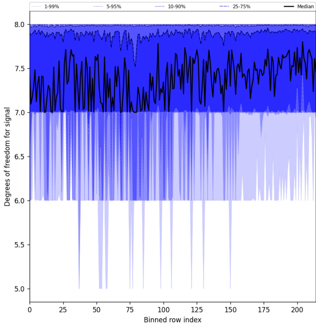
Figure 25: Along track statistics of “Degrees of freedom for signal” for 2025-01-17 to 2025-01-18
