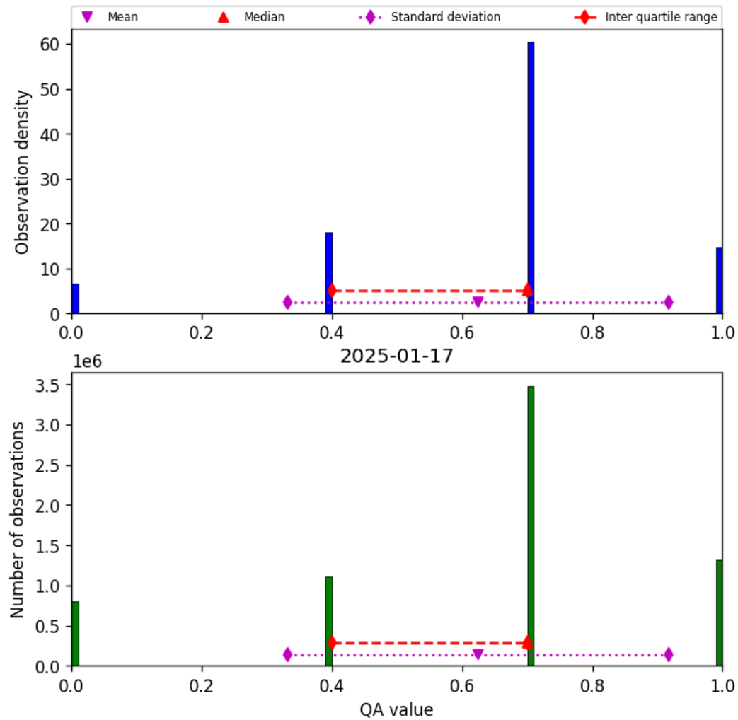
Figure 13: Histogram of “QA value” for 2025-01-17 to 2025-01-18
