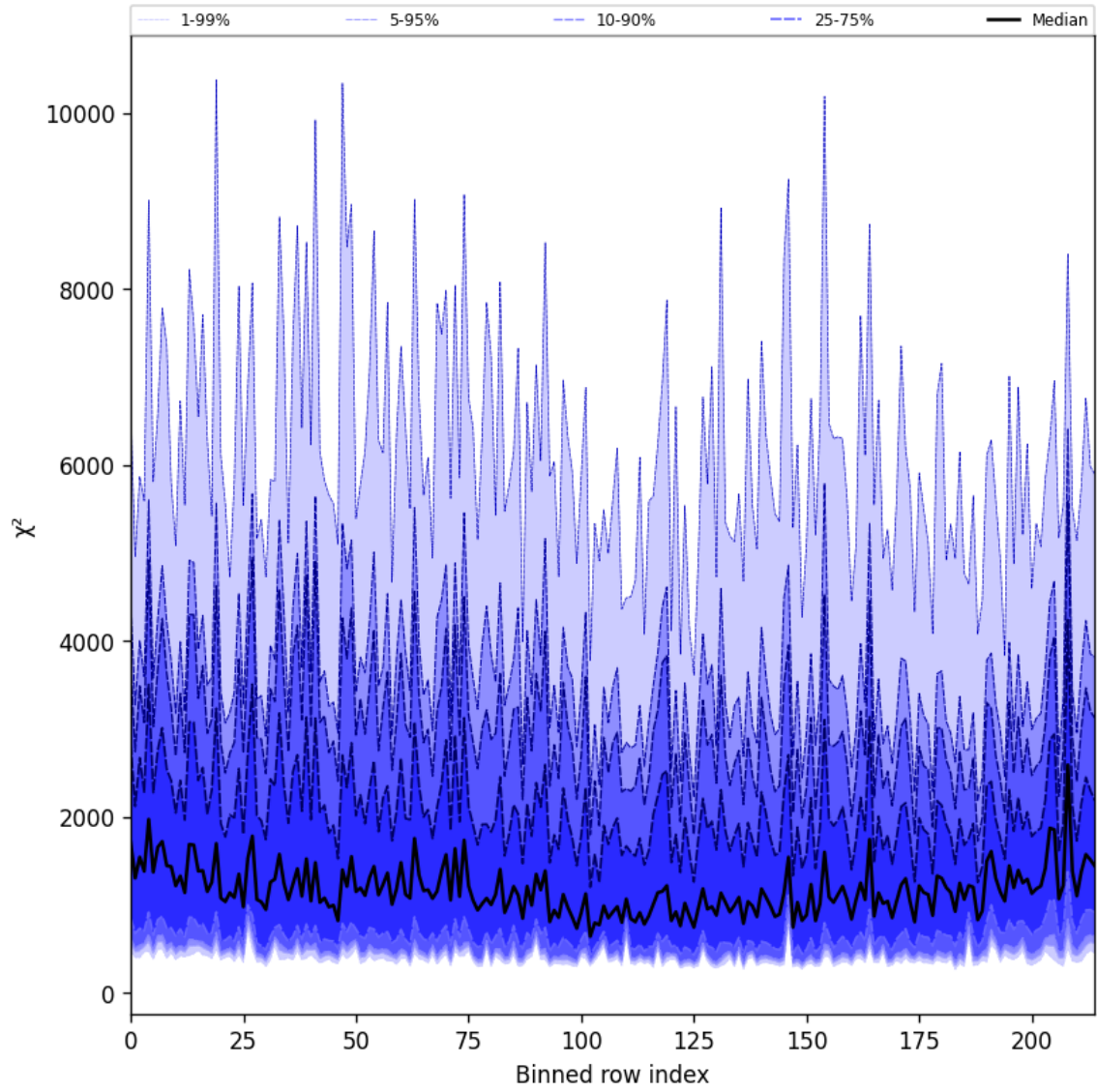
Figure 24: Along track statistics of “ \chi^2 ” for 2025-01-17 to 2025-01-18
