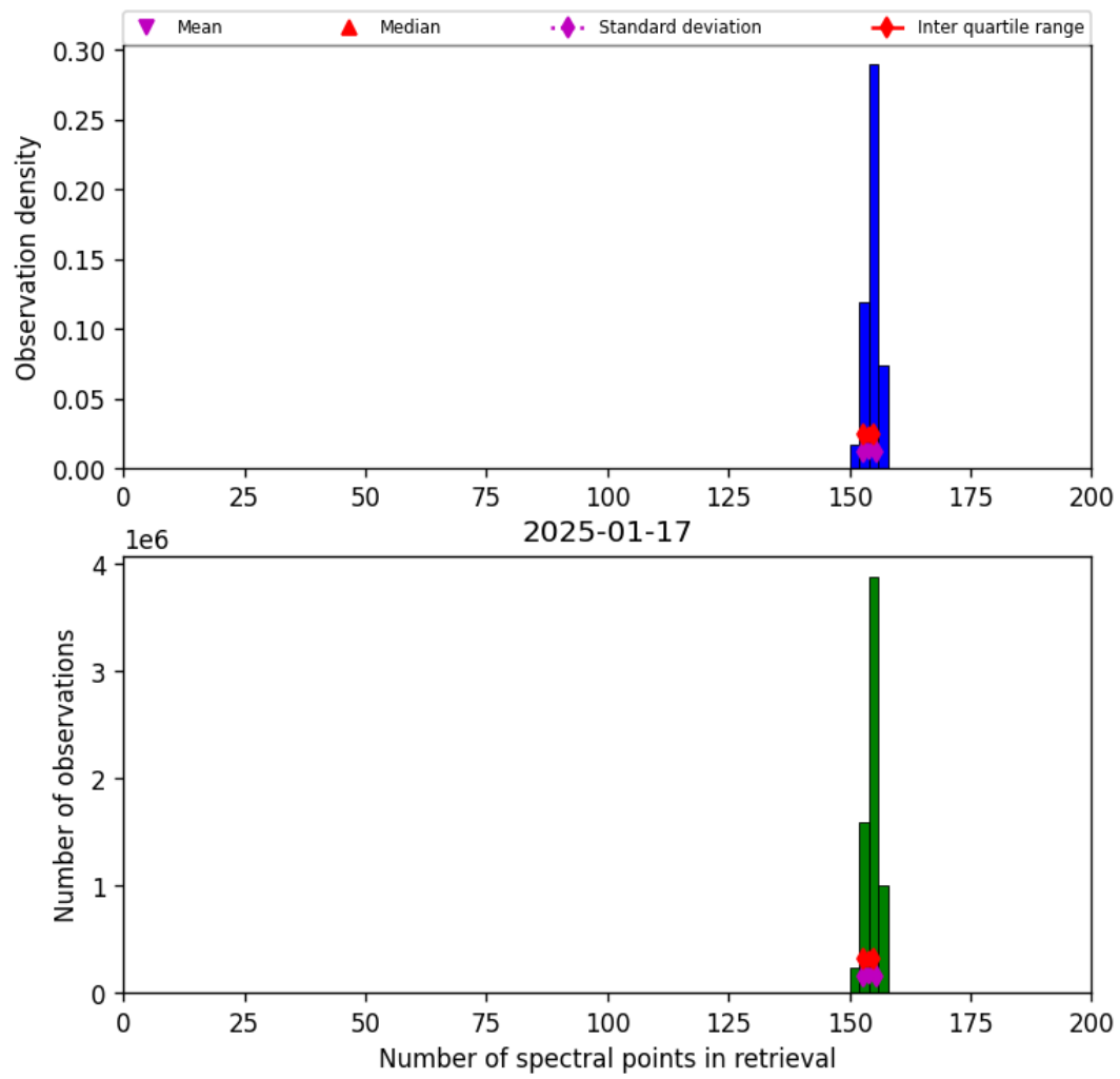
Figure 16: Histogram of “Number of spectral points in retrieval” for 2025-01-17 to 2025-01-18
