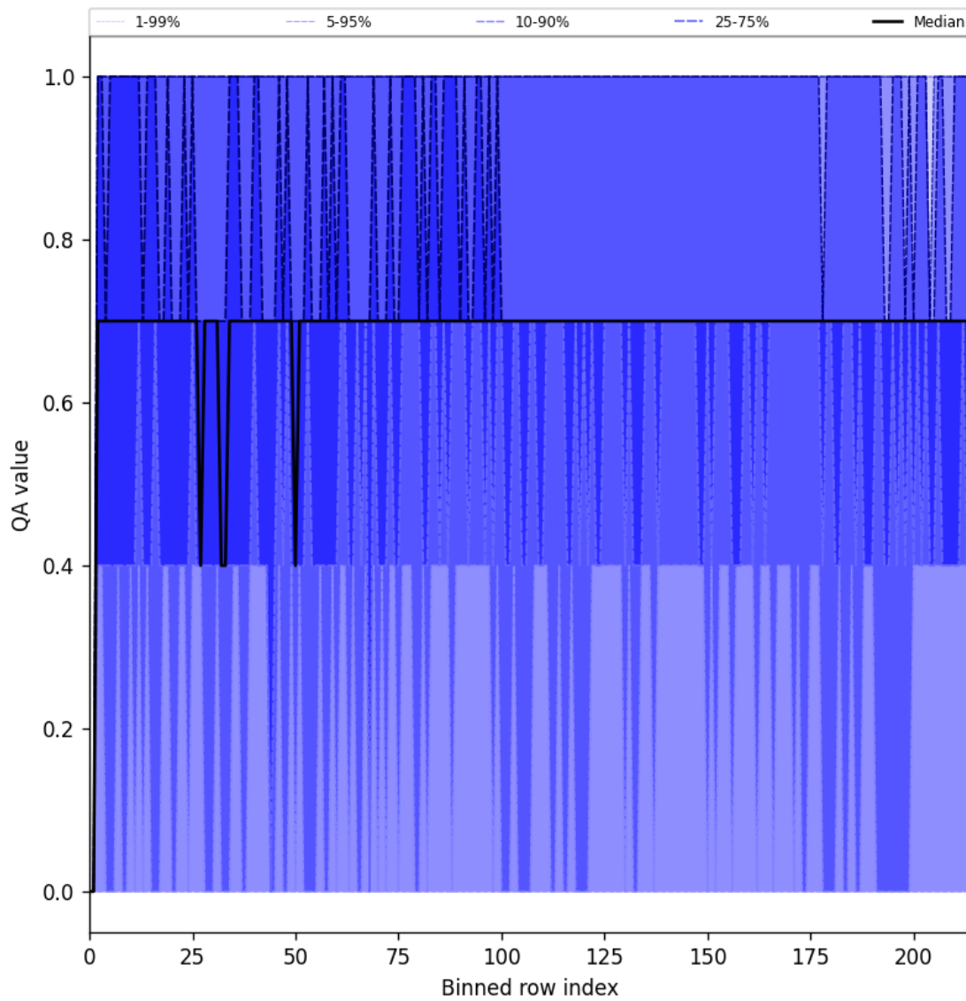
Figure 20: Along track statistics of “QA value” for 2025-01-17 to 2025-01-18
