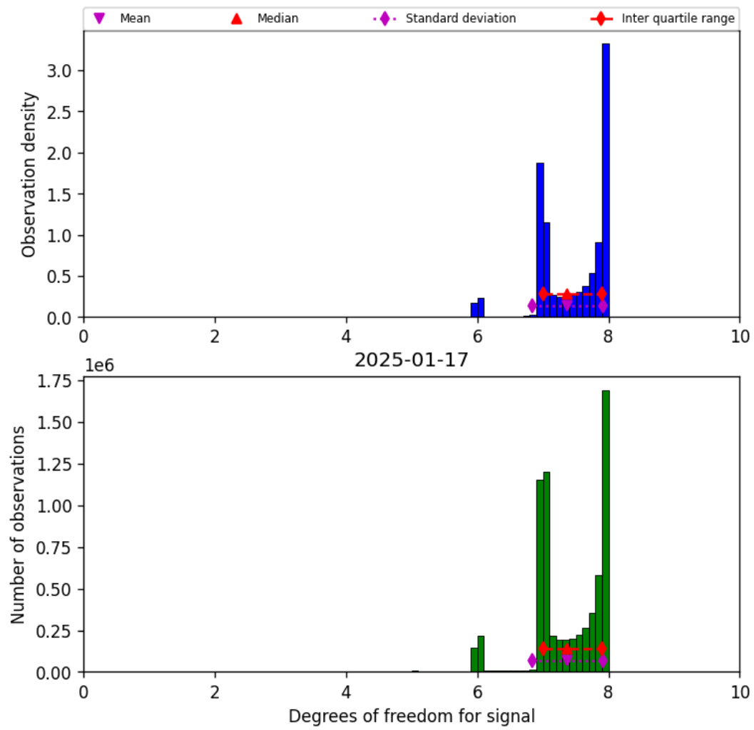
Figure 18: Histogram of “Degrees of freedom for signal” for 2025-01-17 to 2025-01-18
