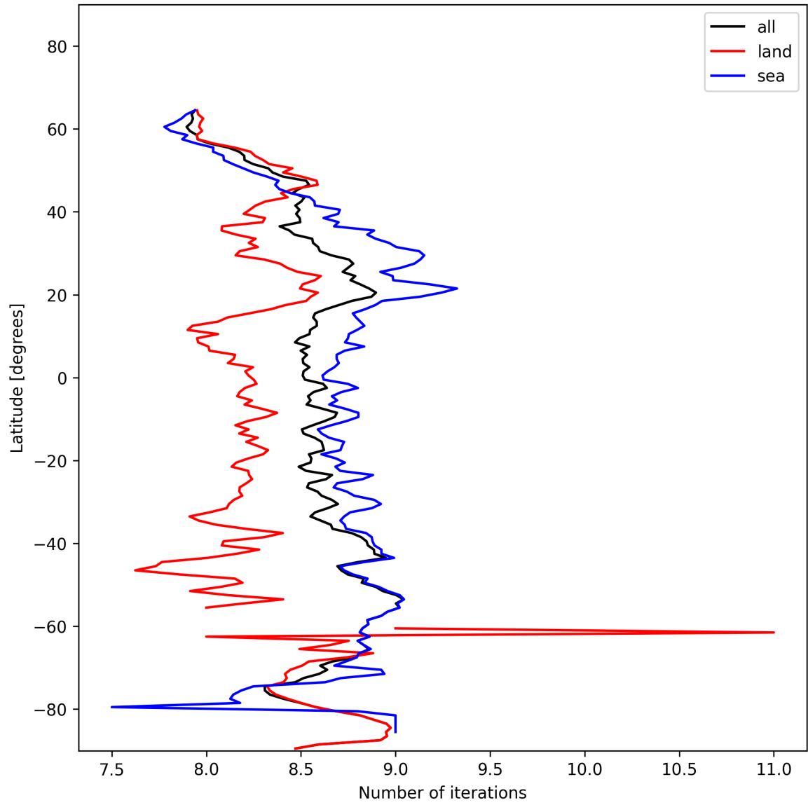
Figure 12: Zonal average of “Number of iterations” for 2025-01-17 to 2025-01-18.
