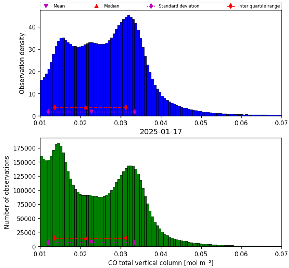
Figure 14: Histogram of “CO total vertical column” for 2025-01-17 to 2025-01-18
