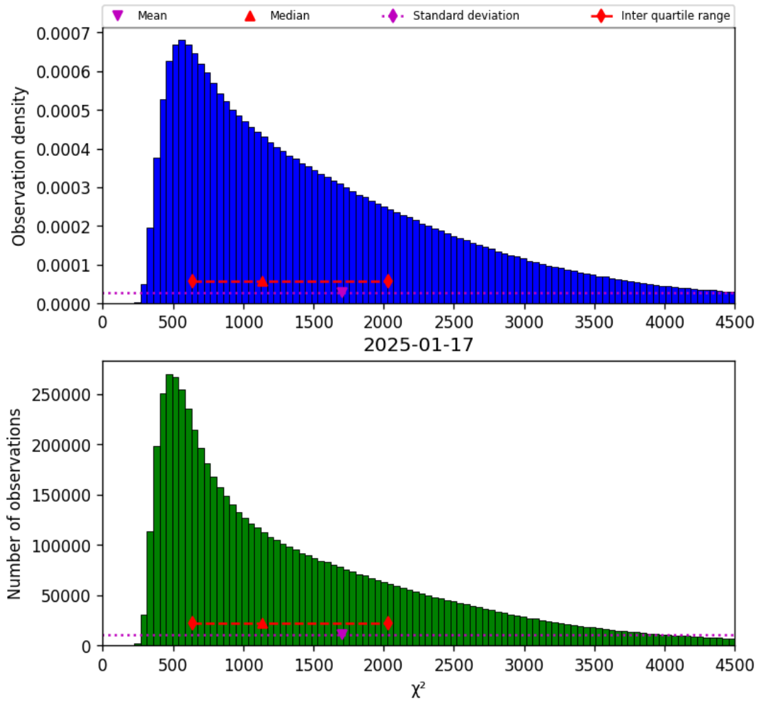
Figure 17: Histogram of “ \chi^2 ” for 2025-01-17 to 2025-01-18
