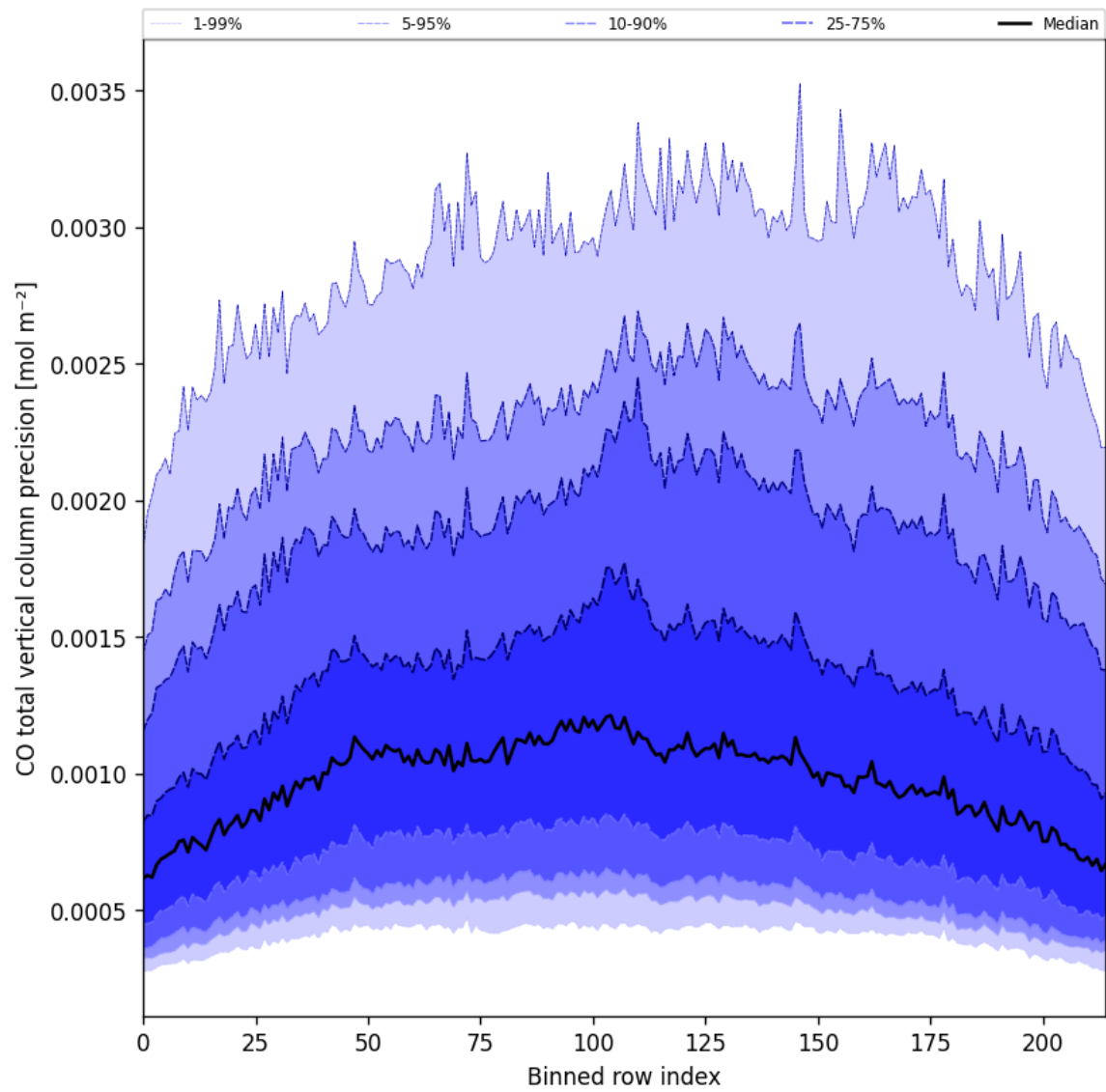
Figure 22: Along track statistics of “CO total vertical column precision” for 2025-01-18 to 2025-01-19
