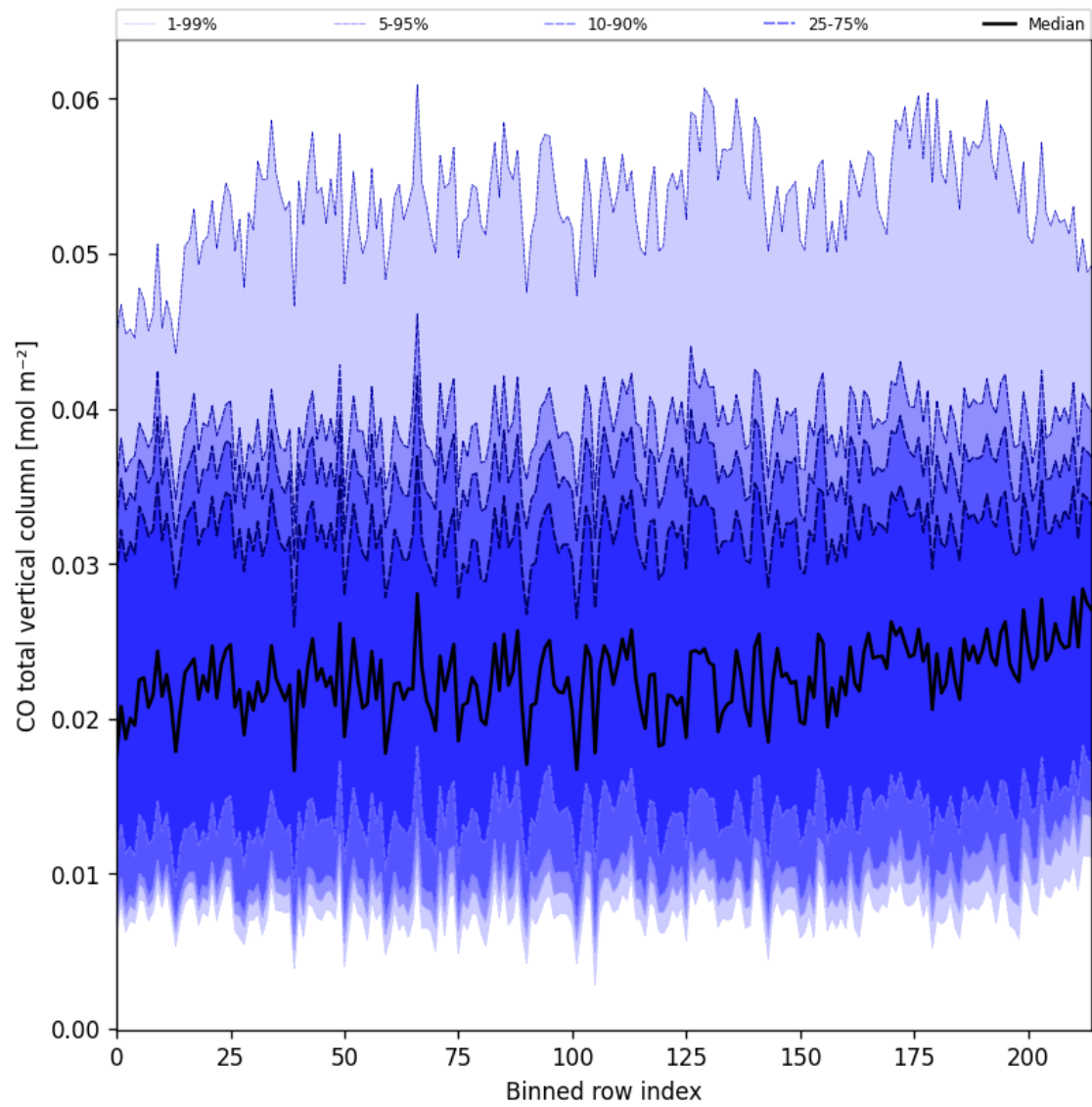
Figure 21: Along track statistics of “CO total vertical column” for 2025-01-18 to 2025-01-19
