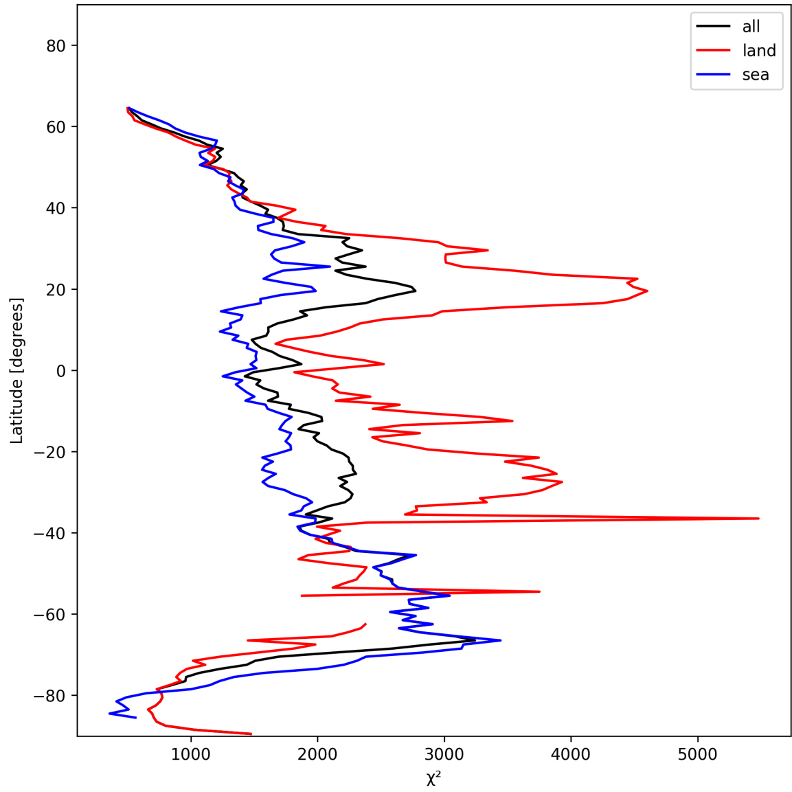
Figure 10: Zonal average of “ \chi^2 ” for 2025-01-18 to 2025-01-19.
