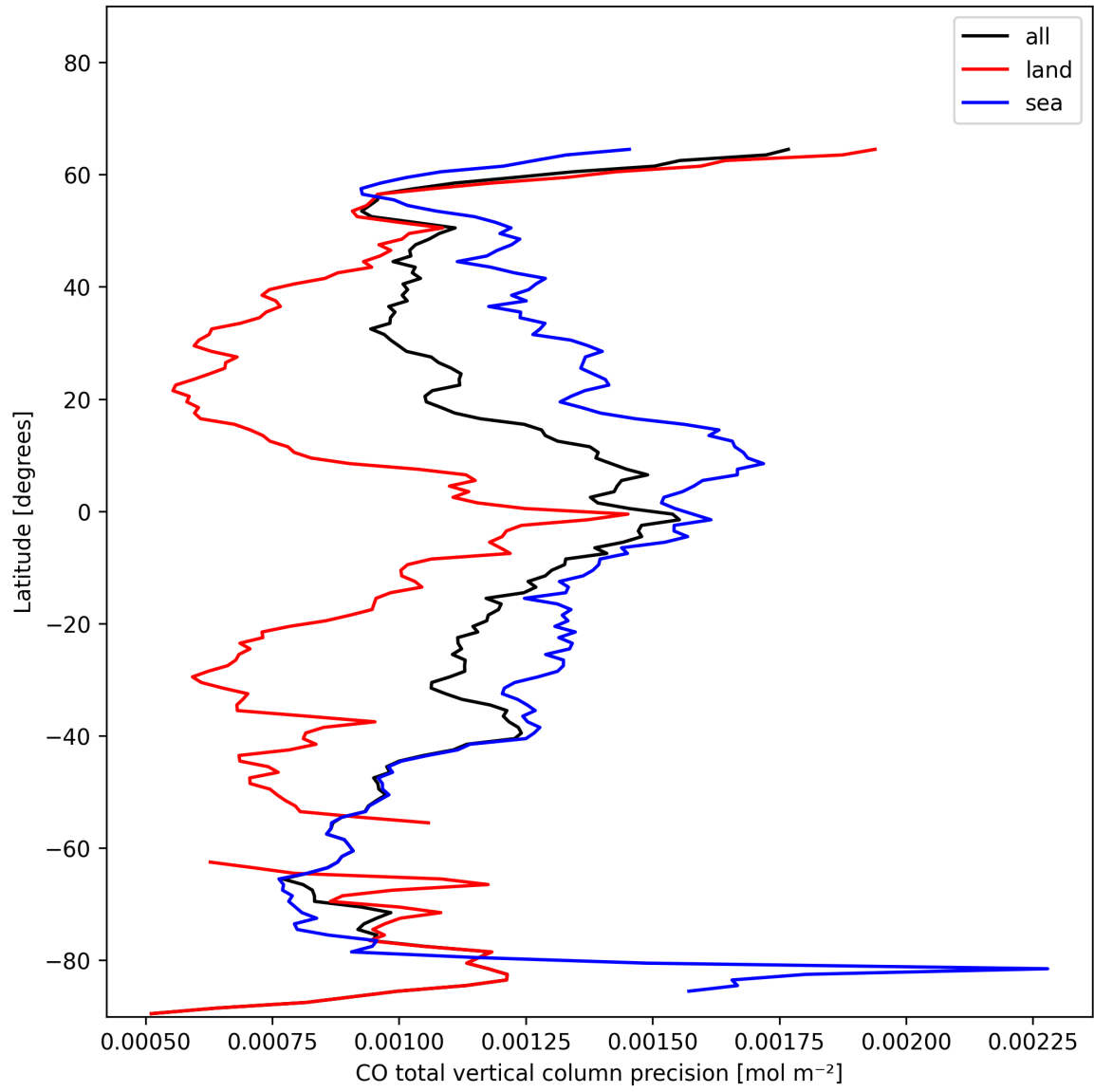
Figure 8: Zonal average of “CO total vertical column precision” for 2025-01-18 to 2025-01-19.
