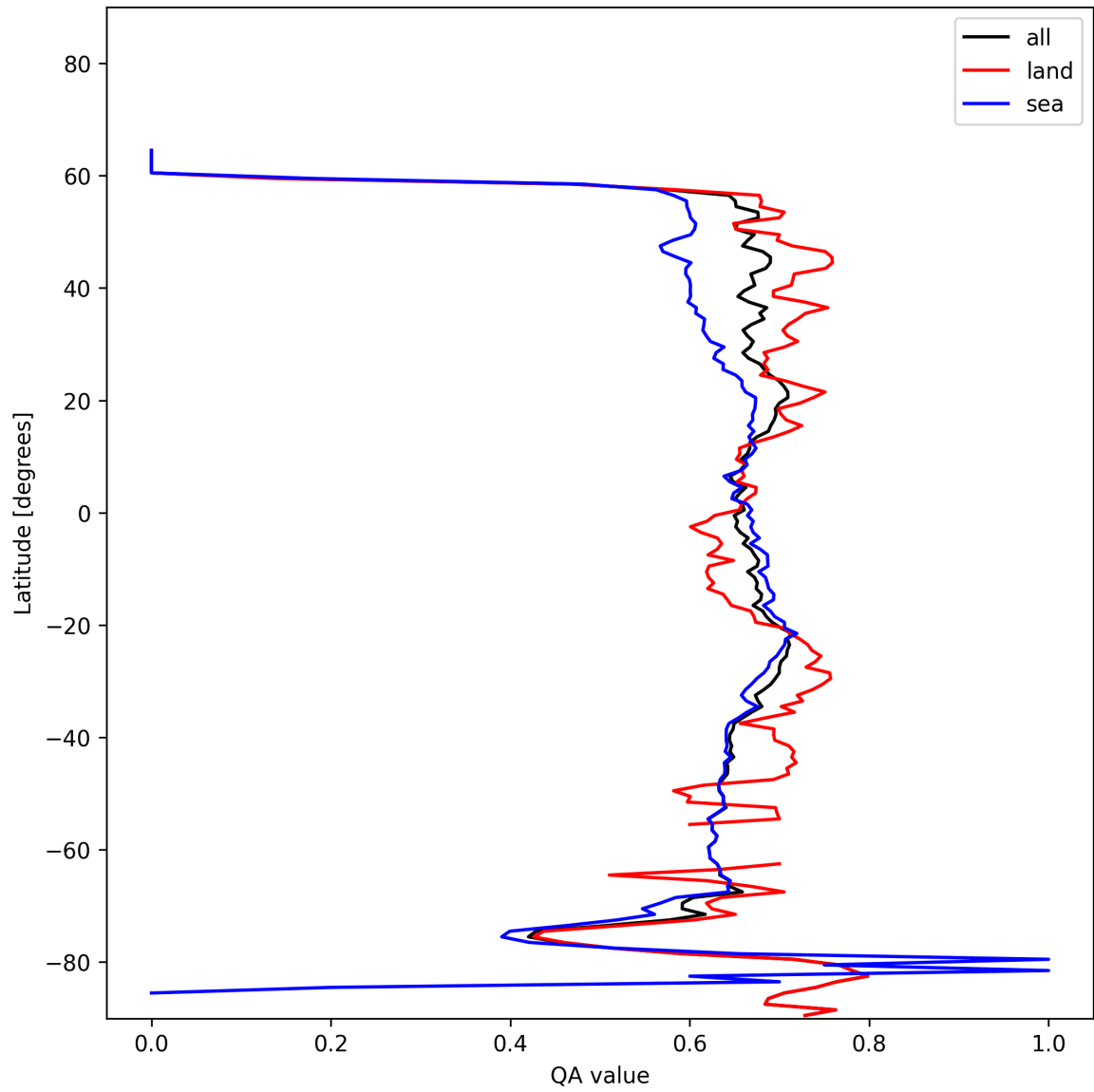
Figure 6: Zonal average of "QA value" for 2025-01-18 to 2025-01-19.
