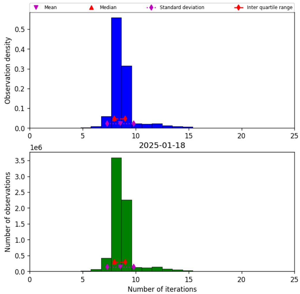
Figure 19: Histogram of “Number of iterations” for 2025-01-18 to 2025-01-19
