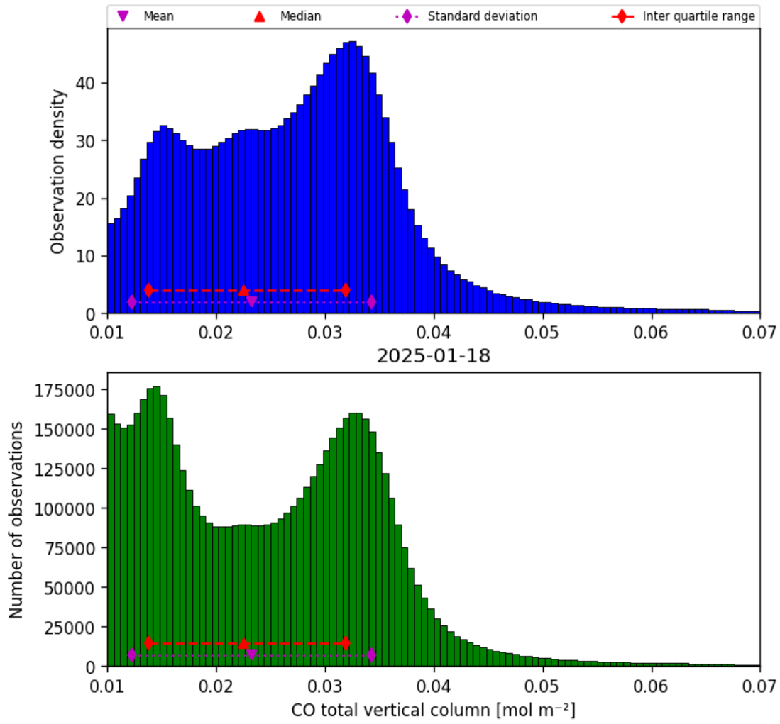
Figure 14: Histogram of “CO total vertical column” for 2025-01-18 to 2025-01-19
