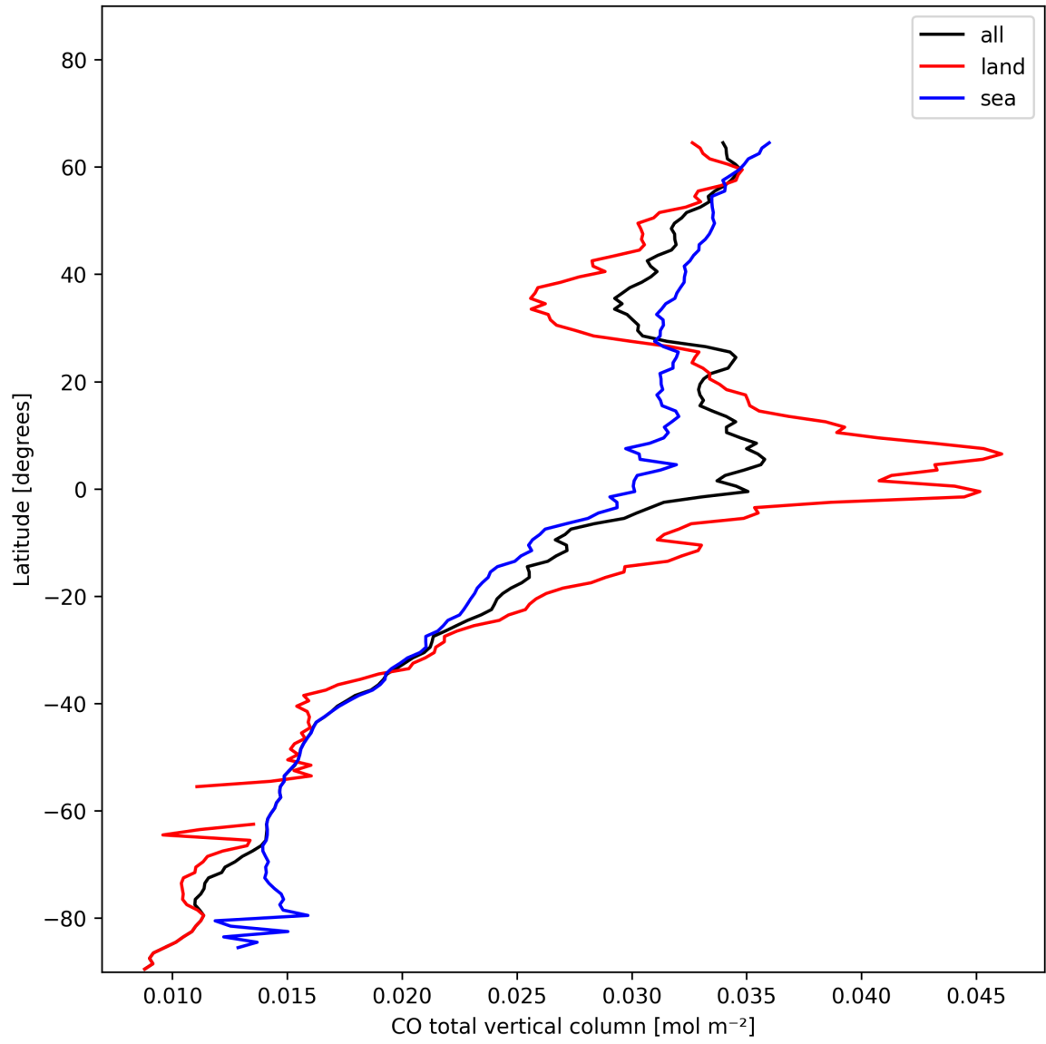
Figure 7: Zonal average of “CO total vertical column” for 2025-01-18 to 2025-01-19.
