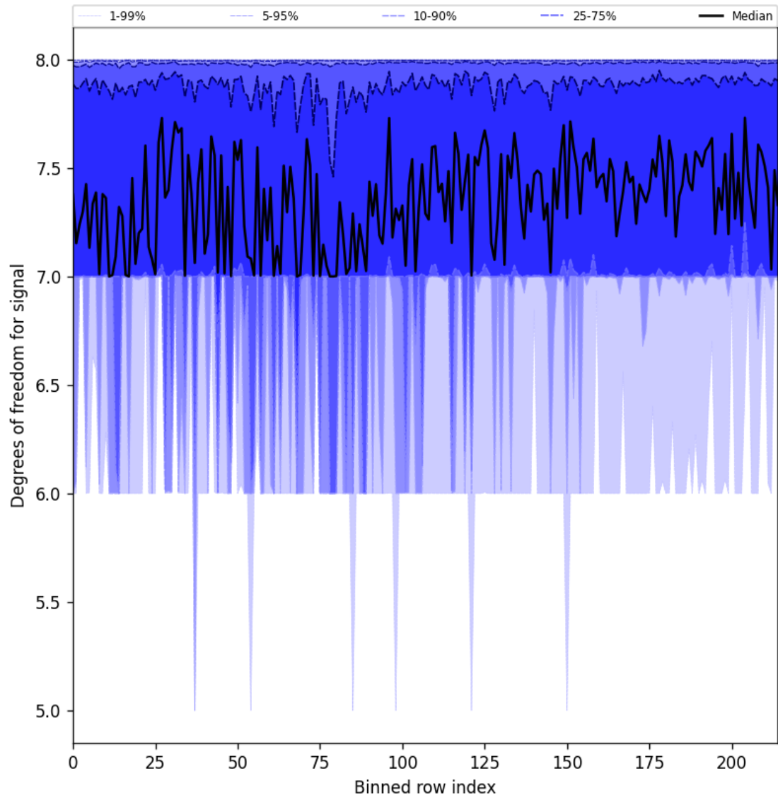
Figure 25: Along track statistics of “Degrees of freedom for signal” for 2025-01-18 to 2025-01-19
