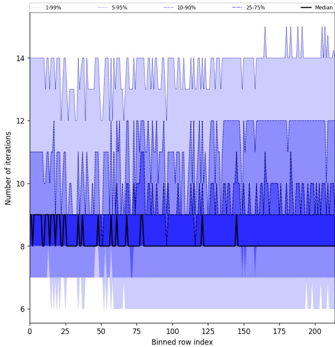
Figure 26: Along track statistics of “Number of iterations” for 2025-01-18 to 2025-01-19
