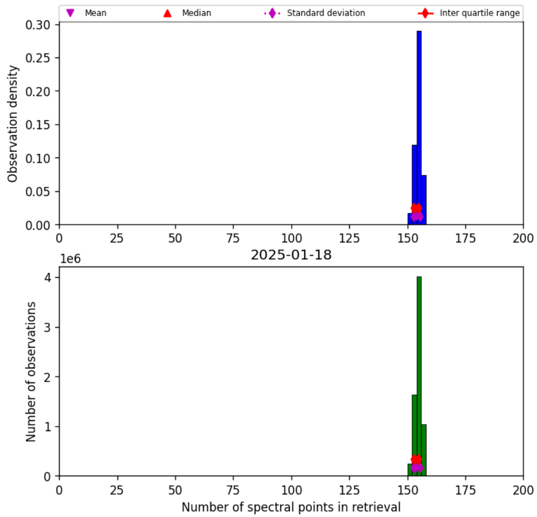
Figure 16: Histogram of “Number of spectral points in retrieval” for 2025-01-18 to 2025-01-19
