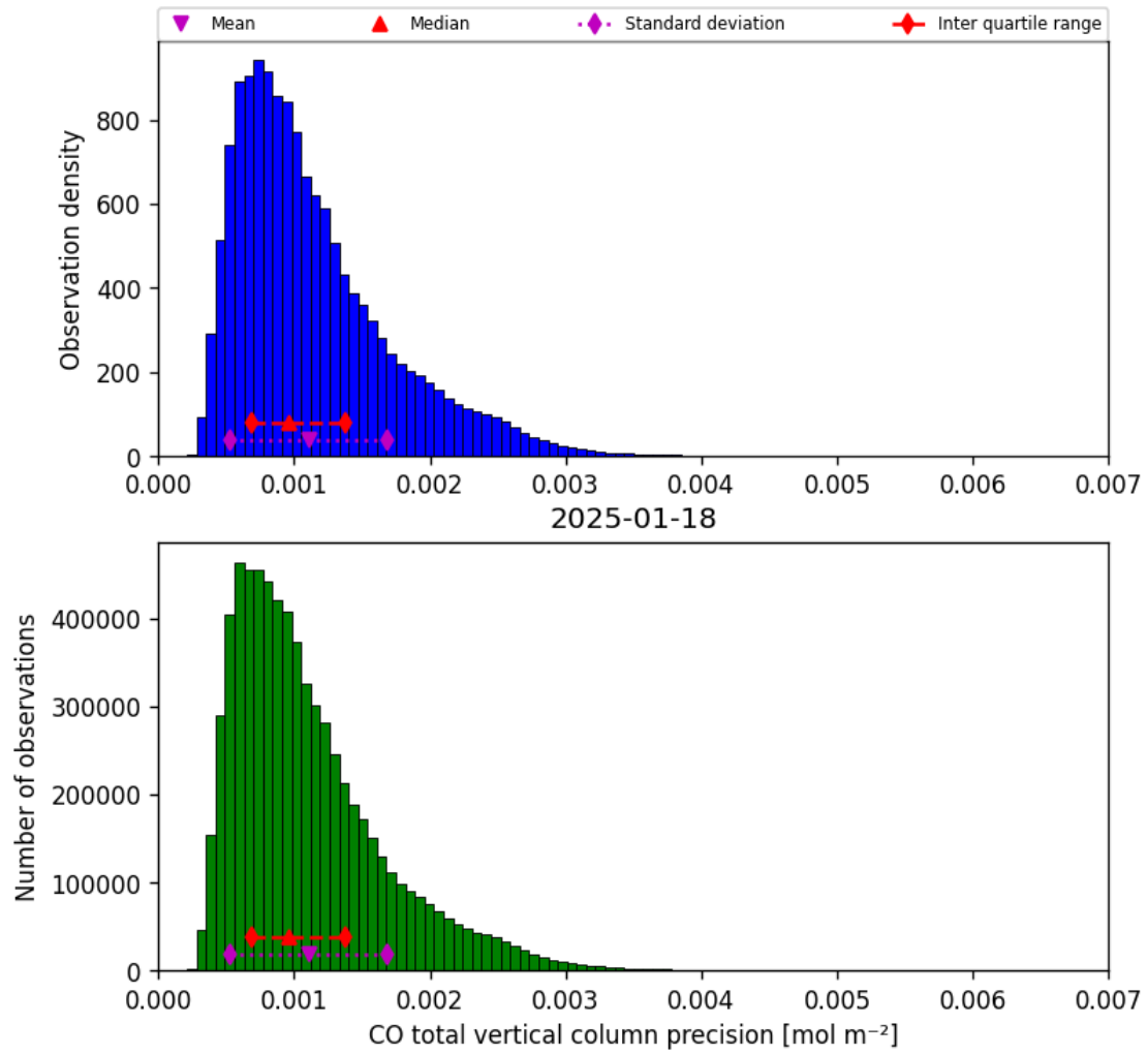
Figure 15: Histogram of “CO total vertical column precision” for 2025-01-18 to 2025-01-19
