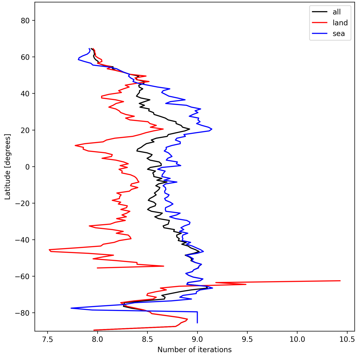
Figure 12: Zonal average of “Number of iterations” for 2025-01-18 to 2025-01-19.
