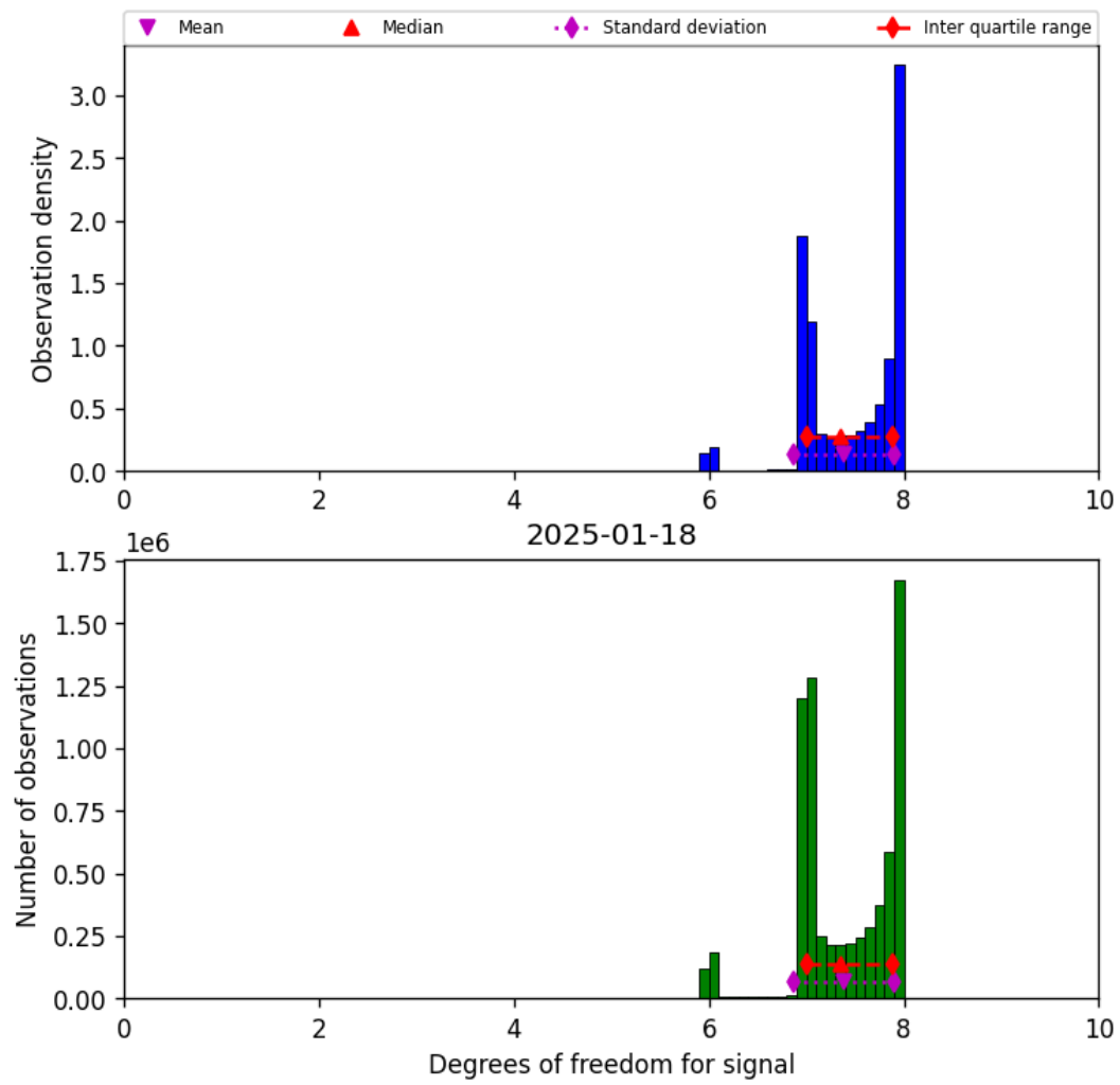
Figure 18: Histogram of “Degrees of freedom for signal” for 2025-01-18 to 2025-01-19
