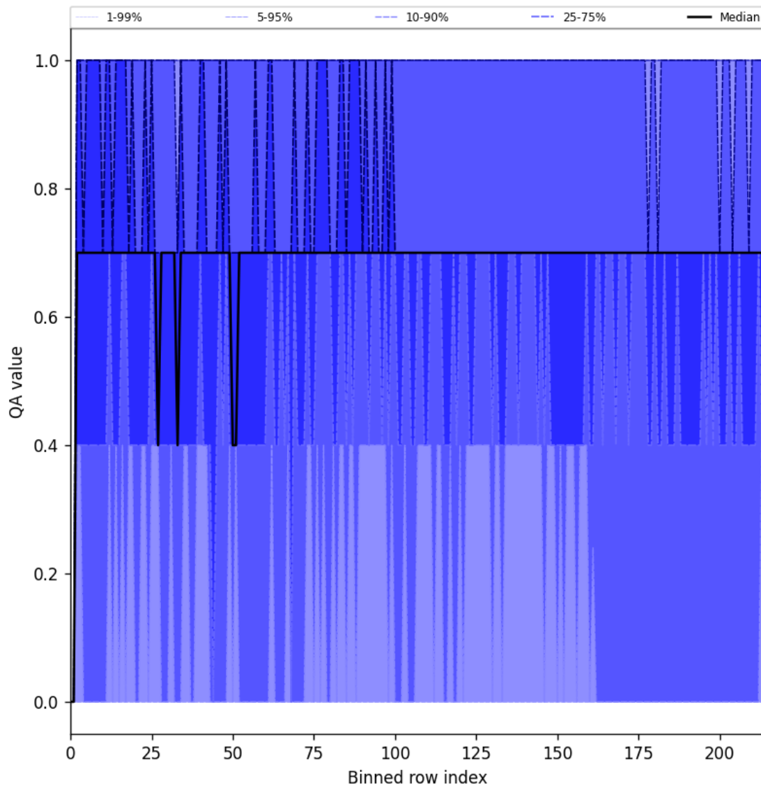
Figure 20: Along track statistics of “QA value” for 2025-01-18 to 2025-01-19
