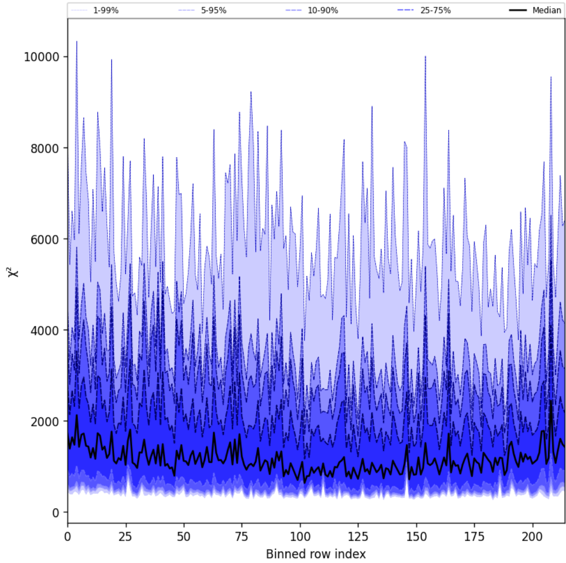
Figure 24: Along track statistics of “ \chi^2 ” for 2025-01-18 to 2025-01-19
