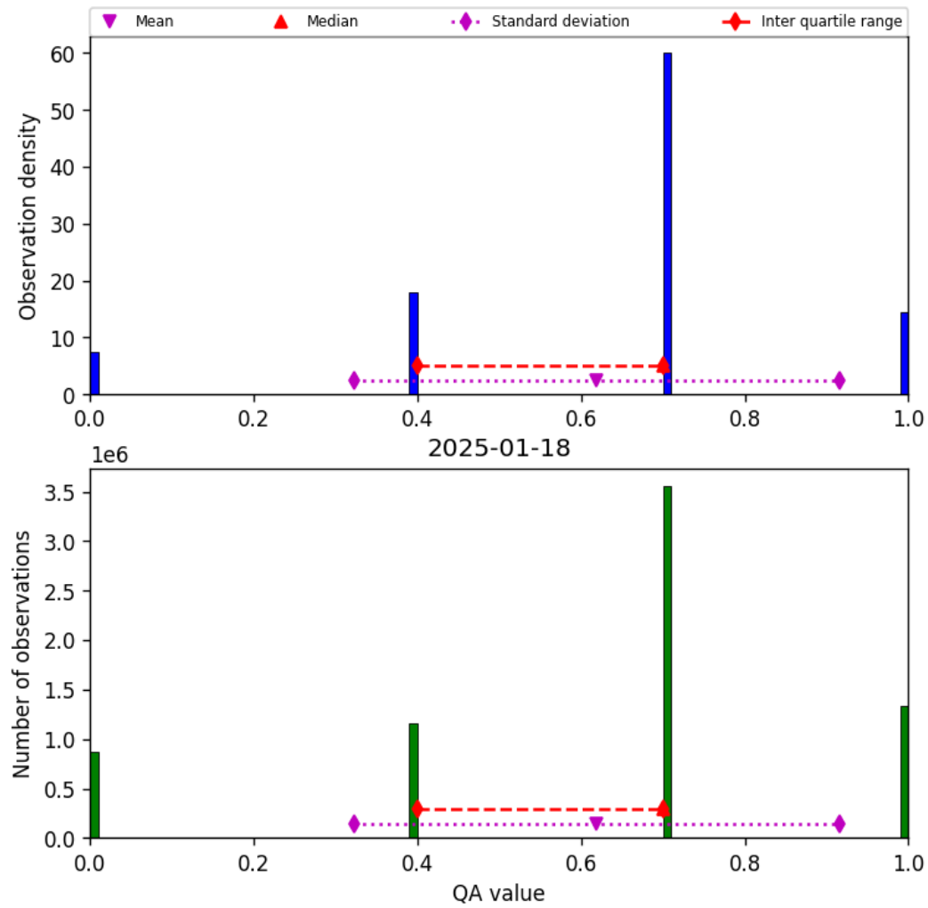
Figure 13: Histogram of “QA value” for 2025-01-18 to 2025-01-19
