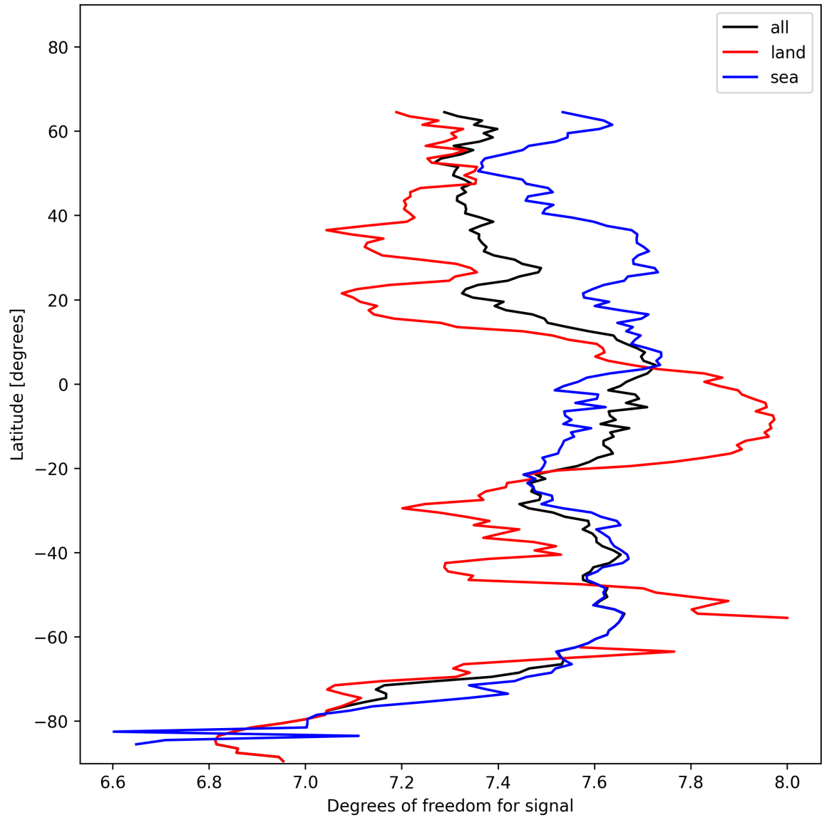
Figure 11: Zonal average of “Degrees of freedom for signal” for 2025-01-18 to 2025-01-19.
