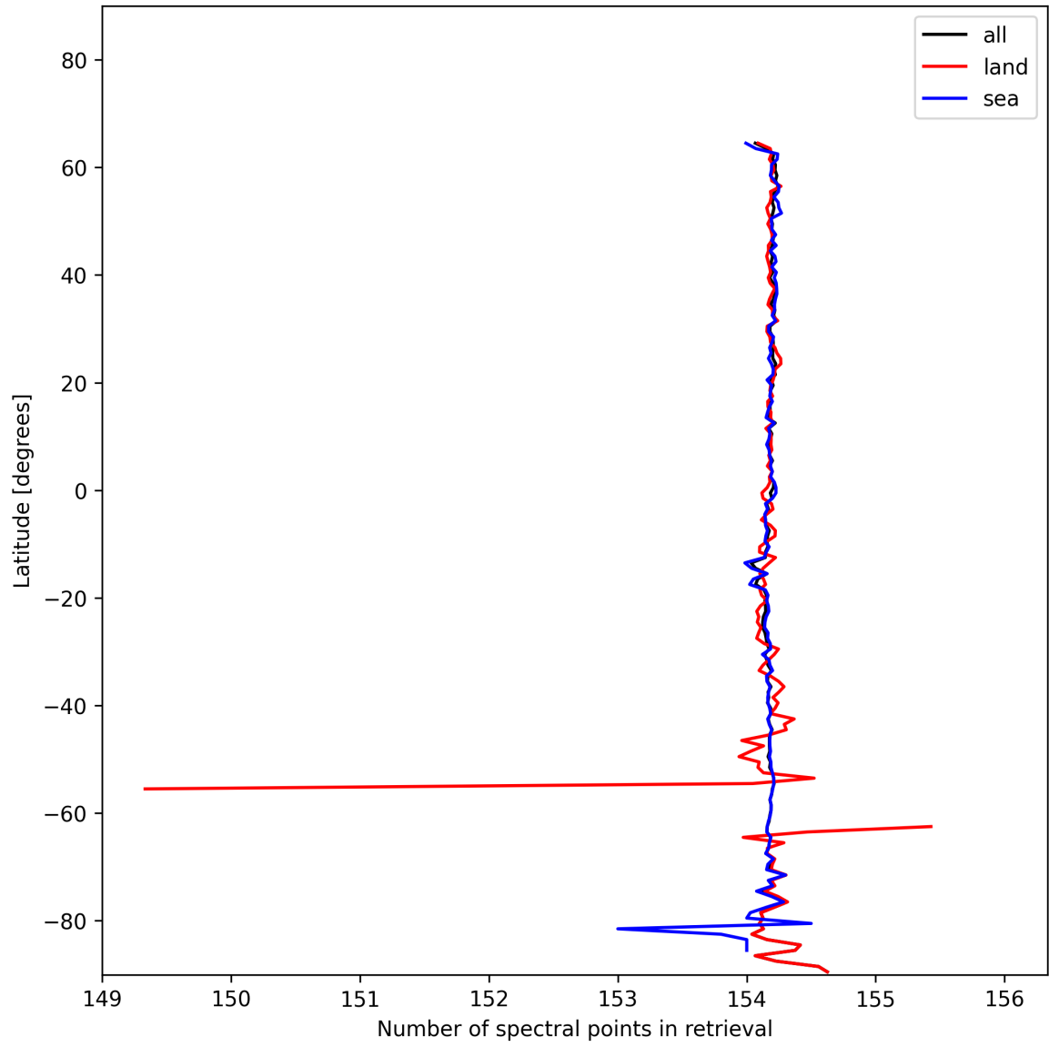
Figure 9: Zonal average of “Number of spectral points in retrieval” for 2025-01-18 to 2025-01-19.
