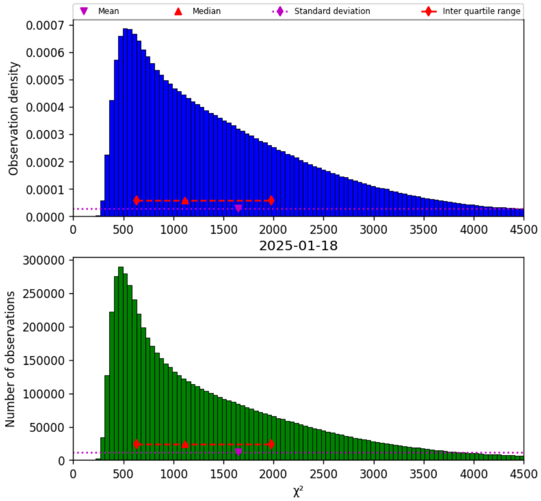
Figure 17: Histogram of “ \chi^2 ” for 2025-01-18 to 2025-01-19
