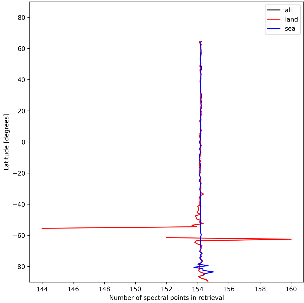
Figure 9: Zonal average of “Number of spectral points in retrieval” for 2025-01-19 to 2025-01-20.
