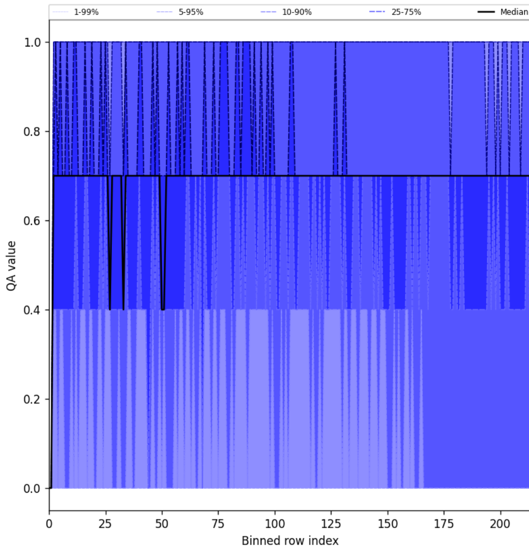
Figure 20: Along track statistics of “QA value” for 2025-01-19 to 2025-01-20
