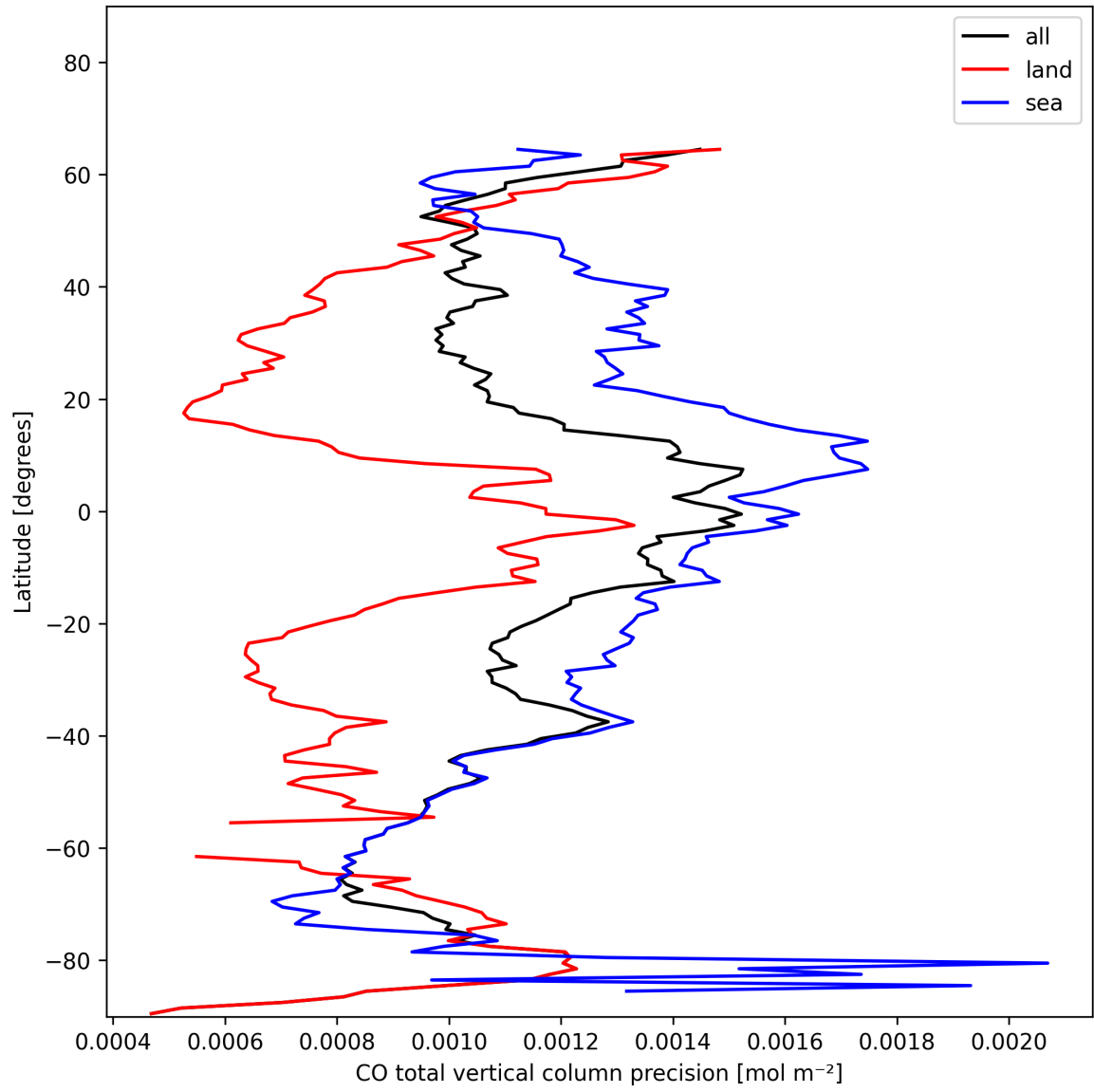
Figure 8: Zonal average of “CO total vertical column precision” for 2025-01-19 to 2025-01-20.
