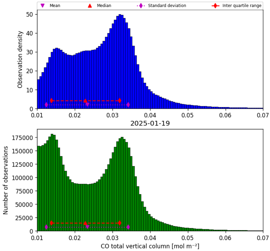
Figure 14: Histogram of “CO total vertical column” for 2025-01-19 to 2025-01-20
