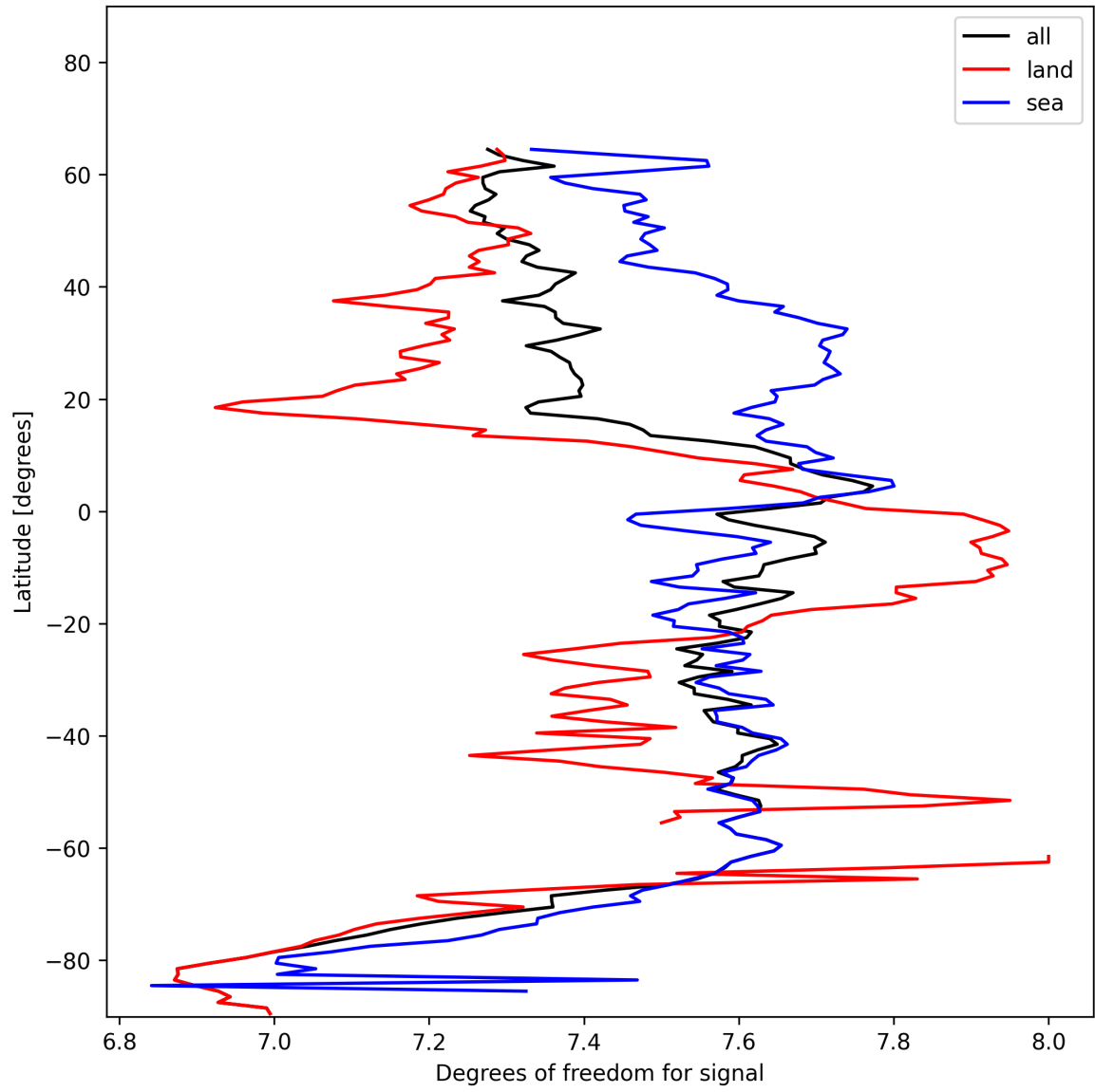
Figure 11: Zonal average of “Degrees of freedom for signal” for 2025-01-19 to 2025-01-20.
