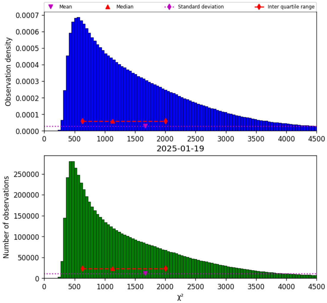
Figure 17: Histogram of “ \chi^2 ” for 2025-01-19 to 2025-01-20
