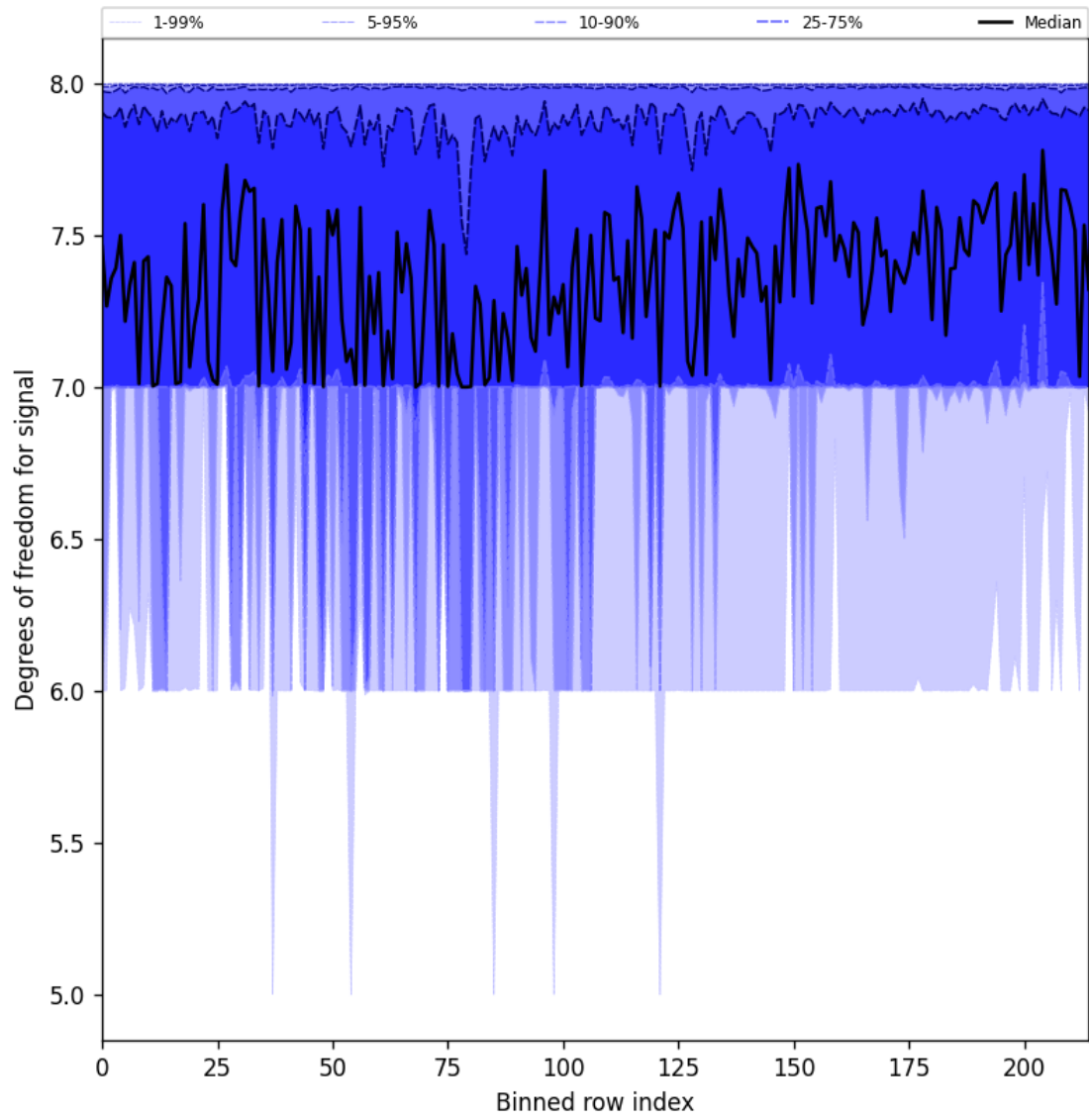
Figure 25: Along track statistics of “Degrees of freedom for signal” for 2025-01-19 to 2025-01-20
