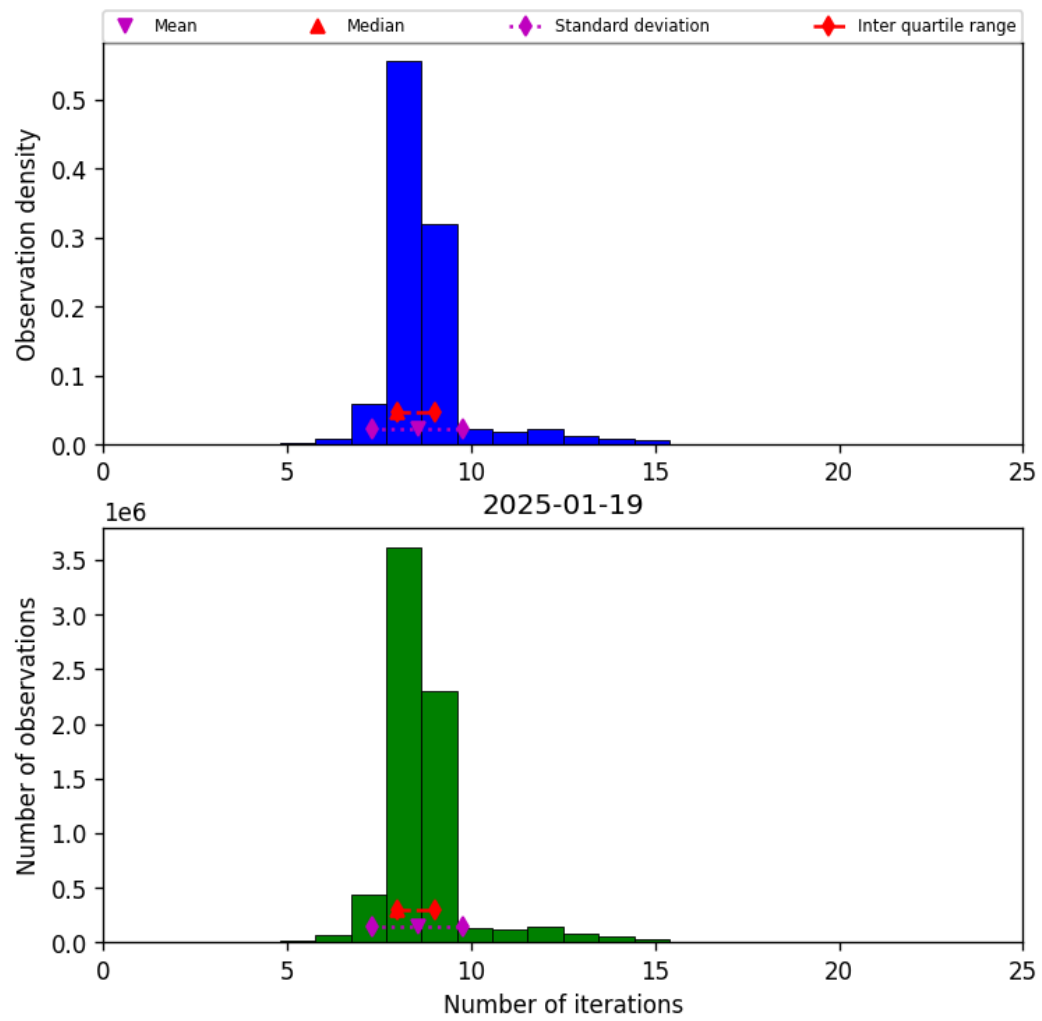
Figure 19: Histogram of “Number of iterations” for 2025-01-19 to 2025-01-20
