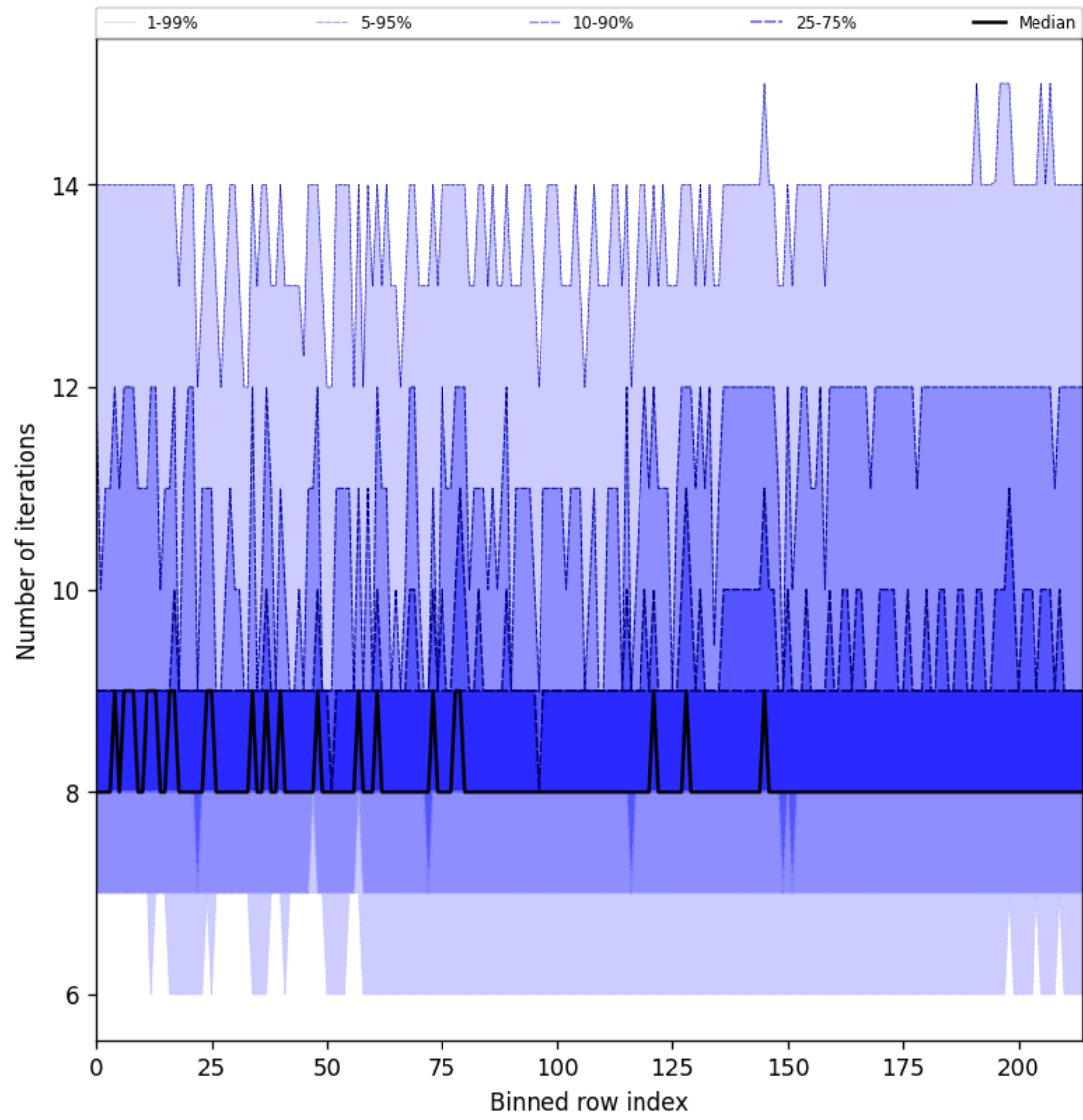
Figure 26: Along track statistics of “Number of iterations” for 2025-01-19 to 2025-01-20
