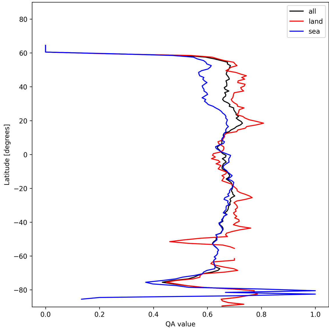
Figure 6: Zonal average of “QA value” for 2025-01-19 to 2025-01-20.
