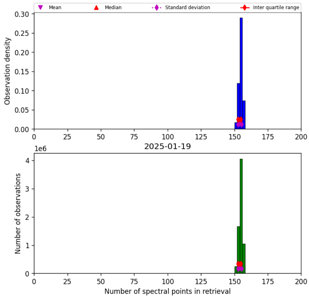
Figure 16: Histogram of “Number of spectral points in retrieval” for 2025-01-19 to 2025-01-20
