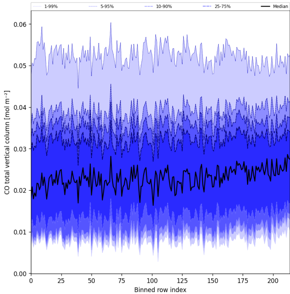
Figure 21: Along track statistics of “CO total vertical column” for 2025-01-19 to 2025-01-20
