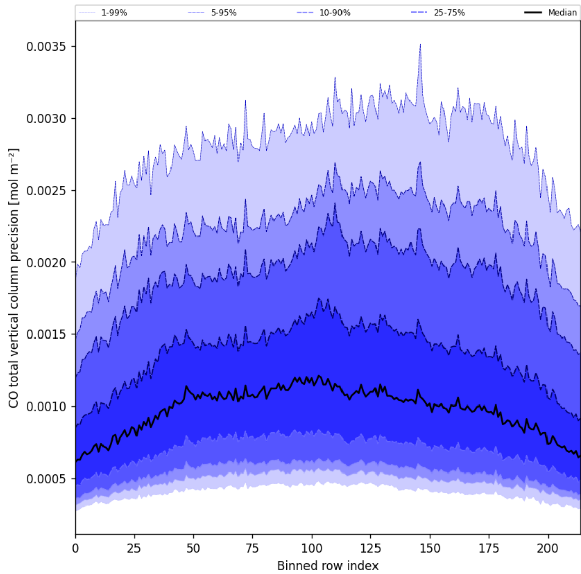
Figure 22: Along track statistics of “CO total vertical column precision” for 2025-01-19 to 2025-01-20
