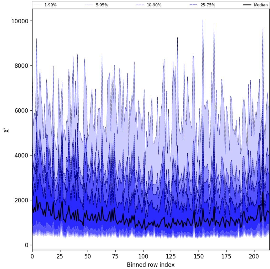
Figure 24: Along track statistics of “ \chi^2 ” for 2025-01-19 to 2025-01-20
