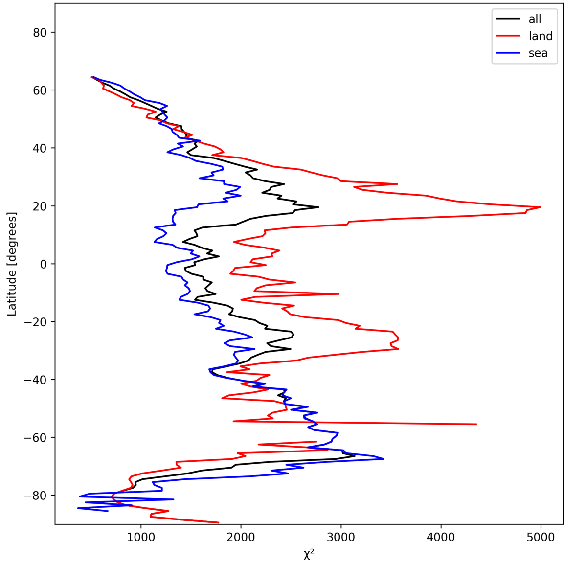
Figure 10: Zonal average of “ \chi^2 ” for 2025-01-19 to 2025-01-20.
