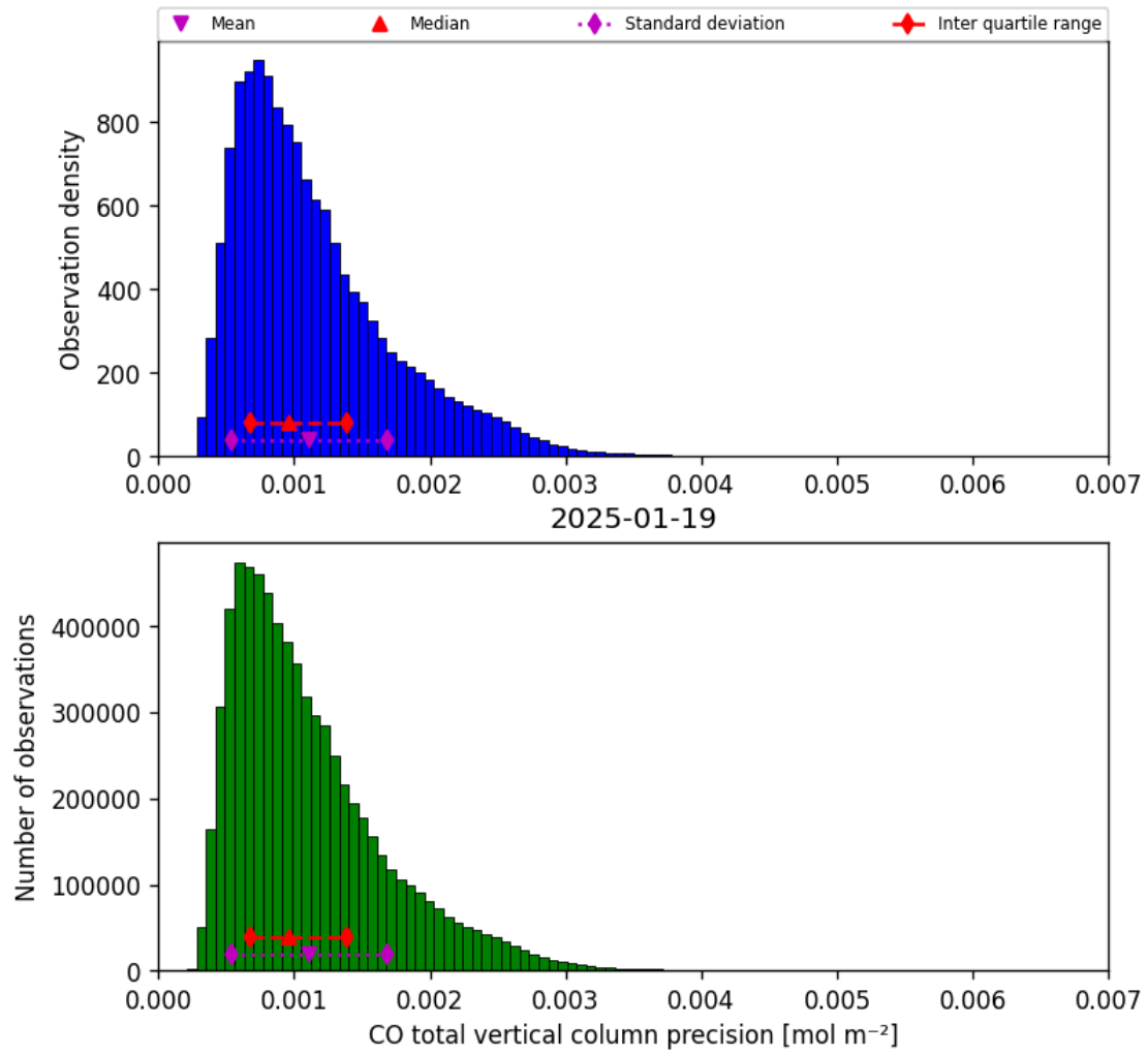
Figure 15: Histogram of “CO total vertical column precision” for 2025-01-19 to 2025-01-20
