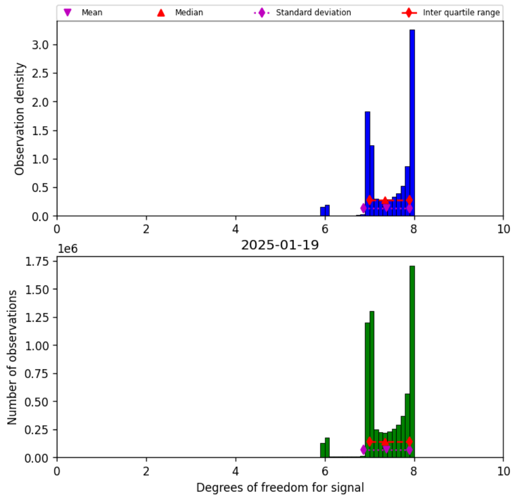
Figure 18: Histogram of “Degrees of freedom for signal” for 2025-01-19 to 2025-01-20
