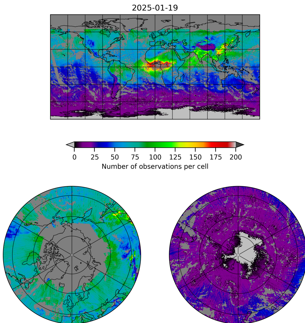
Figure 5: Map of the number of observations for 2025-01-19 to 2025-01-20
