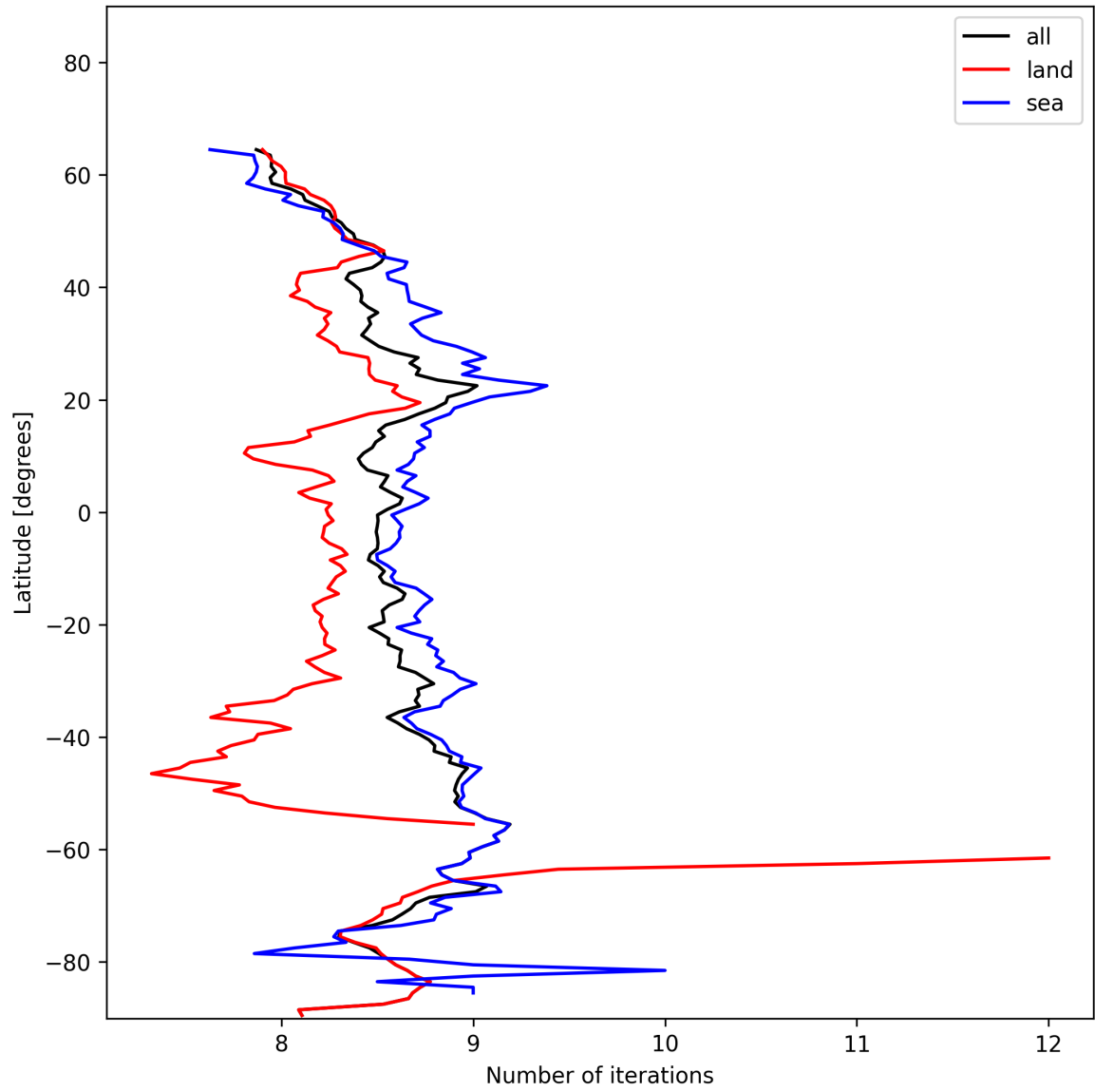
Figure 12: Zonal average of “Number of iterations” for 2025-01-19 to 2025-01-20.
