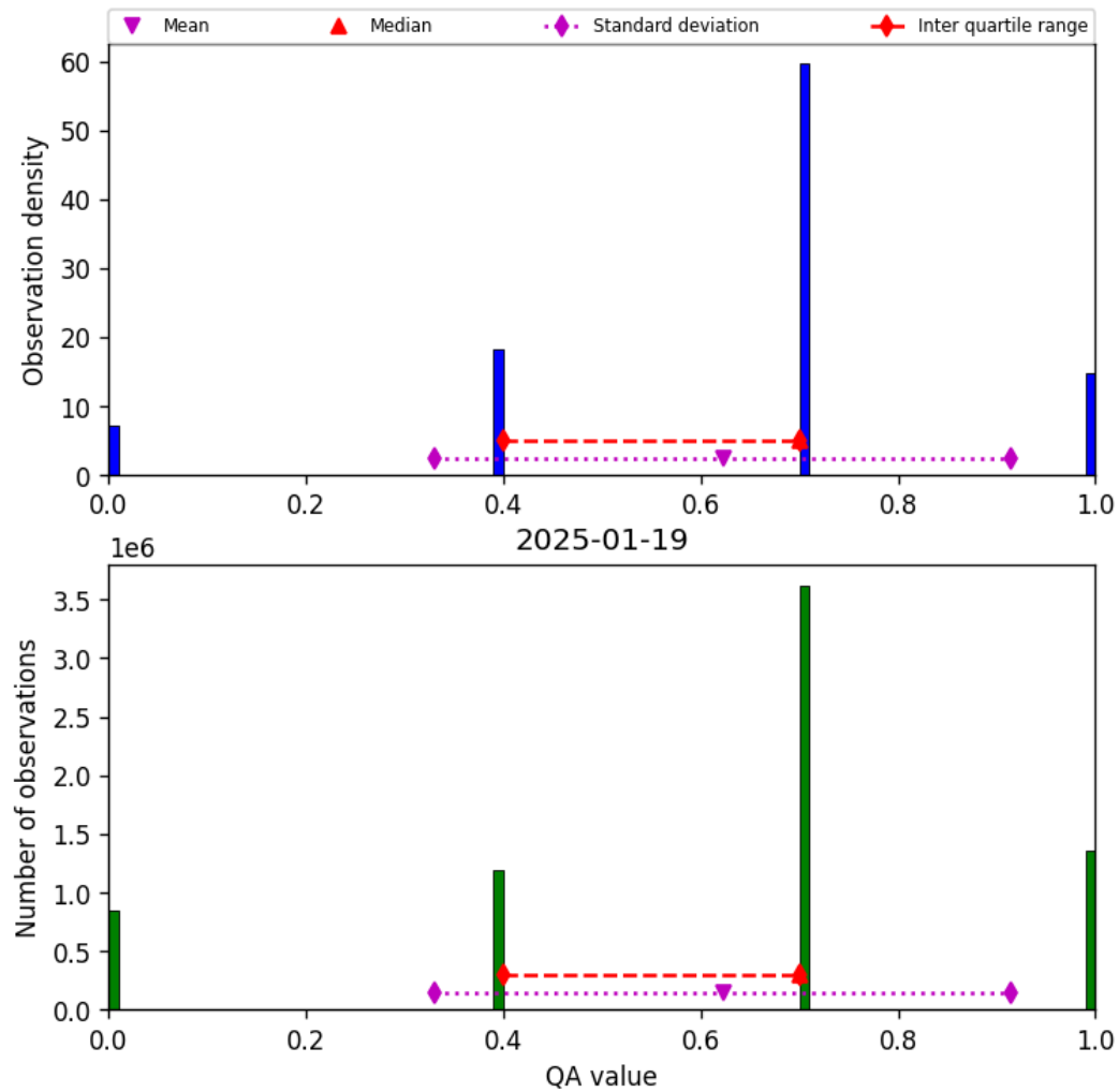
Figure 13: Histogram of “QA value” for 2025-01-19 to 2025-01-20
