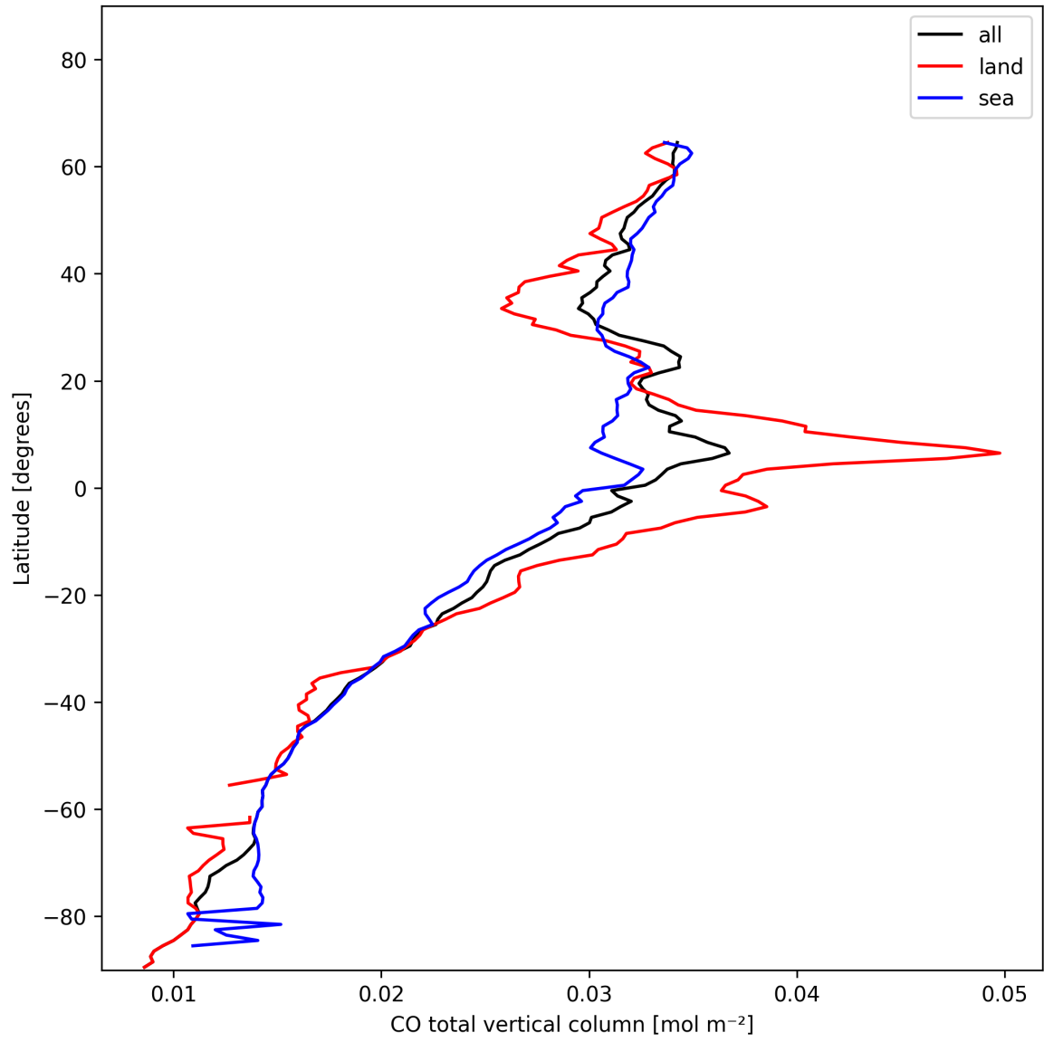
Figure 7: Zonal average of “CO total vertical column” for 2025-01-19 to 2025-01-20.
