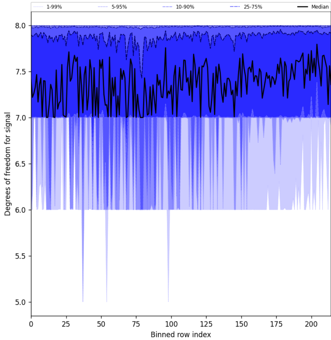
Figure 25: Along track statistics of “Degrees of freedom for signal” for 2025-01-20 to 2025-01-21
