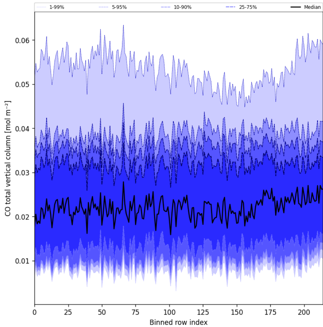
Figure 21: Along track statistics of “CO total vertical column” for 2025-01-20 to 2025-01-21
