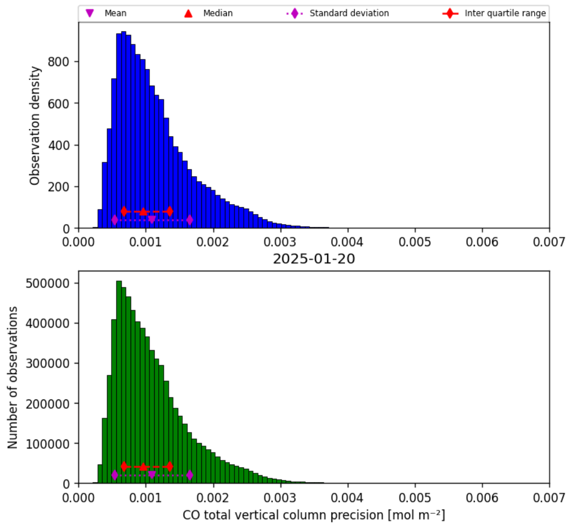
Figure 15: Histogram of “CO total vertical column precision” for 2025-01-20 to 2025-01-21
