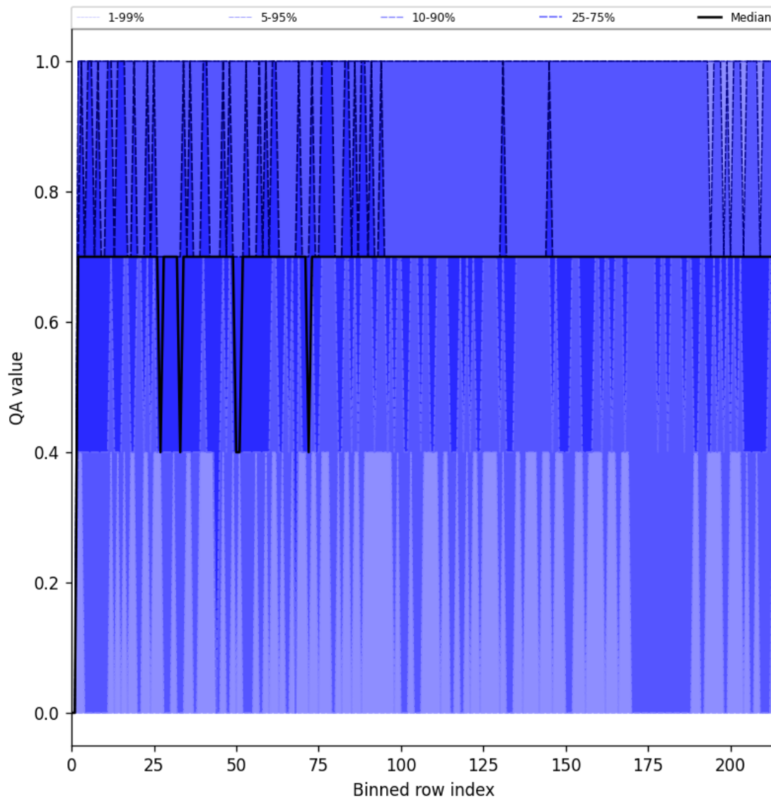
Figure 20: Along track statistics of “QA value” for 2025-01-20 to 2025-01-21
