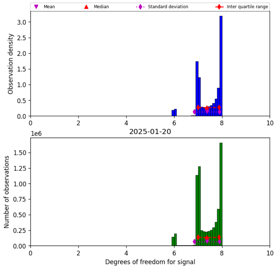
Figure 18: Histogram of “Degrees of freedom for signal” for 2025-01-20 to 2025-01-21
