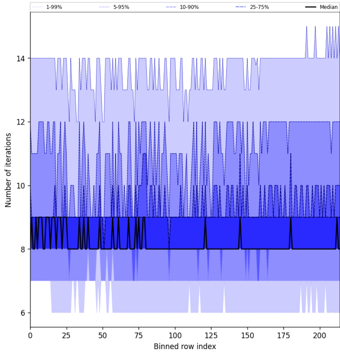
Figure 26: Along track statistics of “Number of iterations” for 2025-01-20 to 2025-01-21
