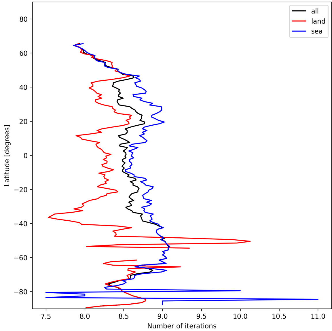
Figure 12: Zonal average of “Number of iterations” for 2025-01-20 to 2025-01-21.
