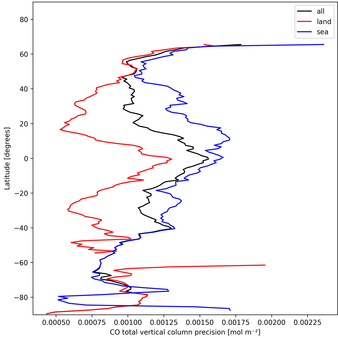
Figure 8: Zonal average of “CO total vertical column precision” for 2025-01-20 to 2025-01-21.
