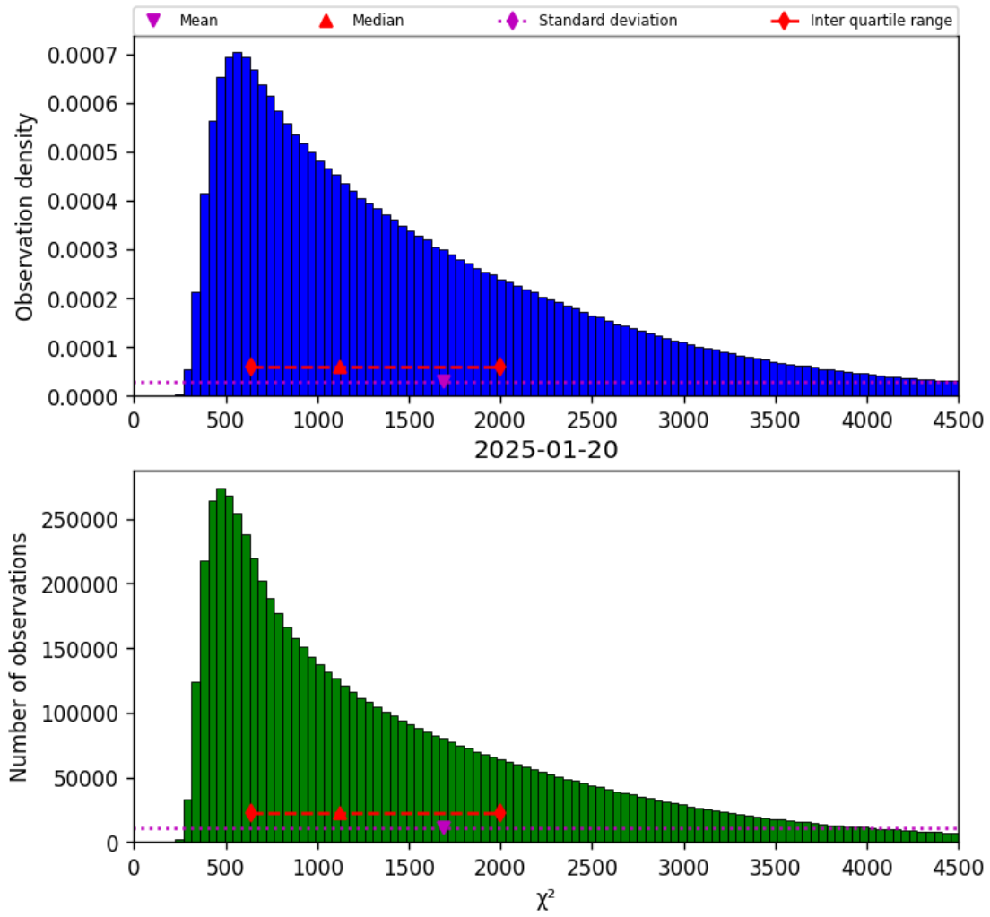
Figure 17: Histogram of “ \chi^2 ” for 2025-01-20 to 2025-01-21
