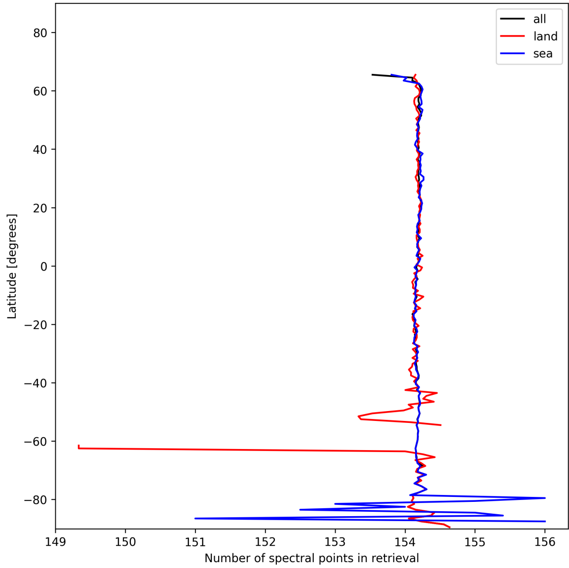
Figure 9: Zonal average of “Number of spectral points in retrieval” for 2025-01-20 to 2025-01-21.
