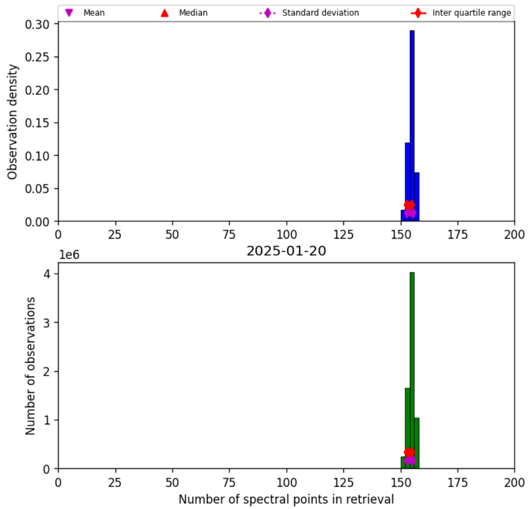
Figure 16: Histogram of “Number of spectral points in retrieval” for 2025-01-20 to 2025-01-21
