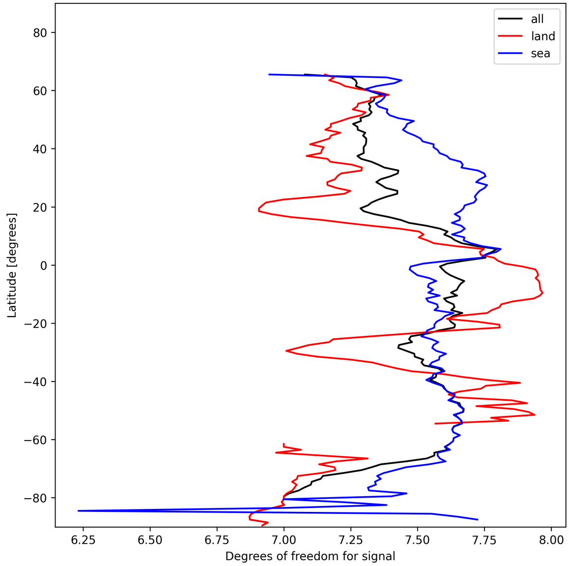
Figure 11: Zonal average of “Degrees of freedom for signal” for 2025-01-20 to 2025-01-21.
