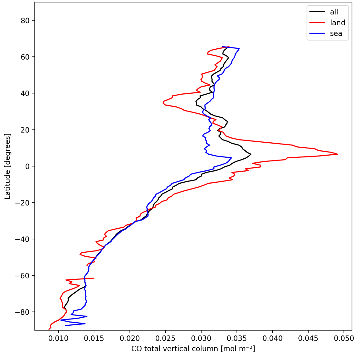
Figure 7: Zonal average of “CO total vertical column” for 2025-01-20 to 2025-01-21.
