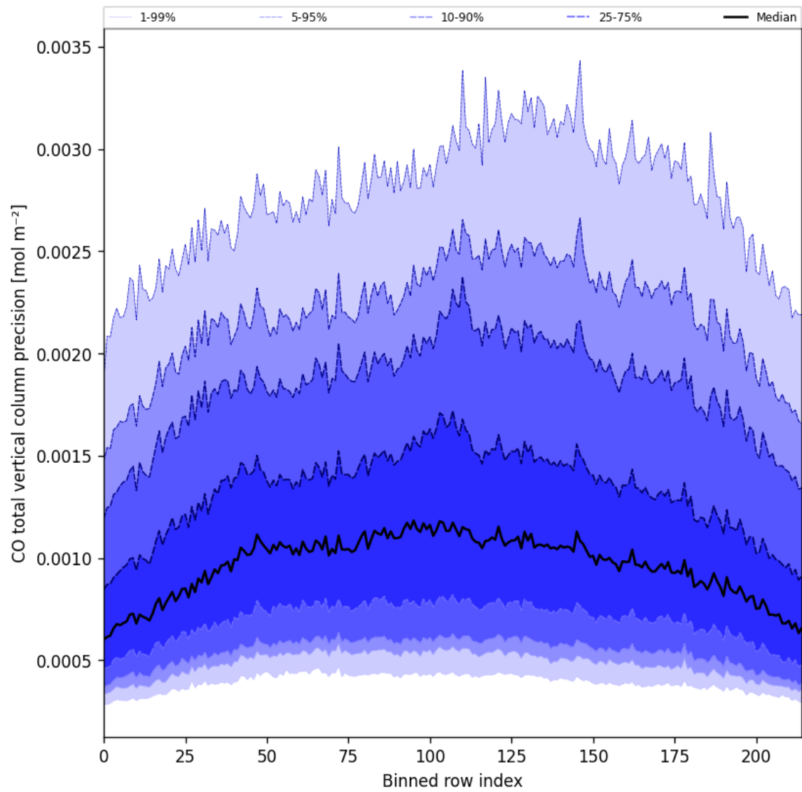
Figure 22: Along track statistics of “CO total vertical column precision” for 2025-01-20 to 2025-01-21
