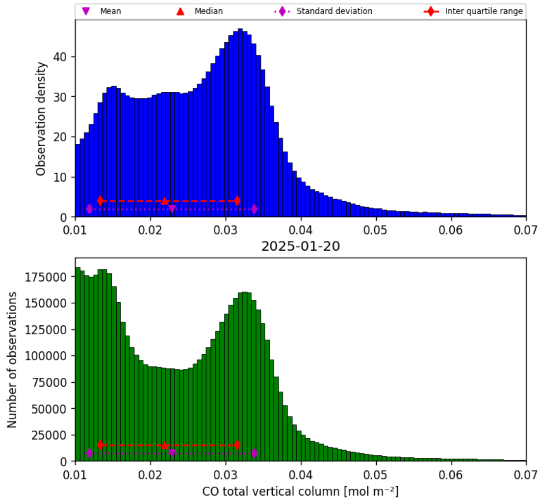
Figure 14: Histogram of “CO total vertical column” for 2025-01-20 to 2025-01-21
