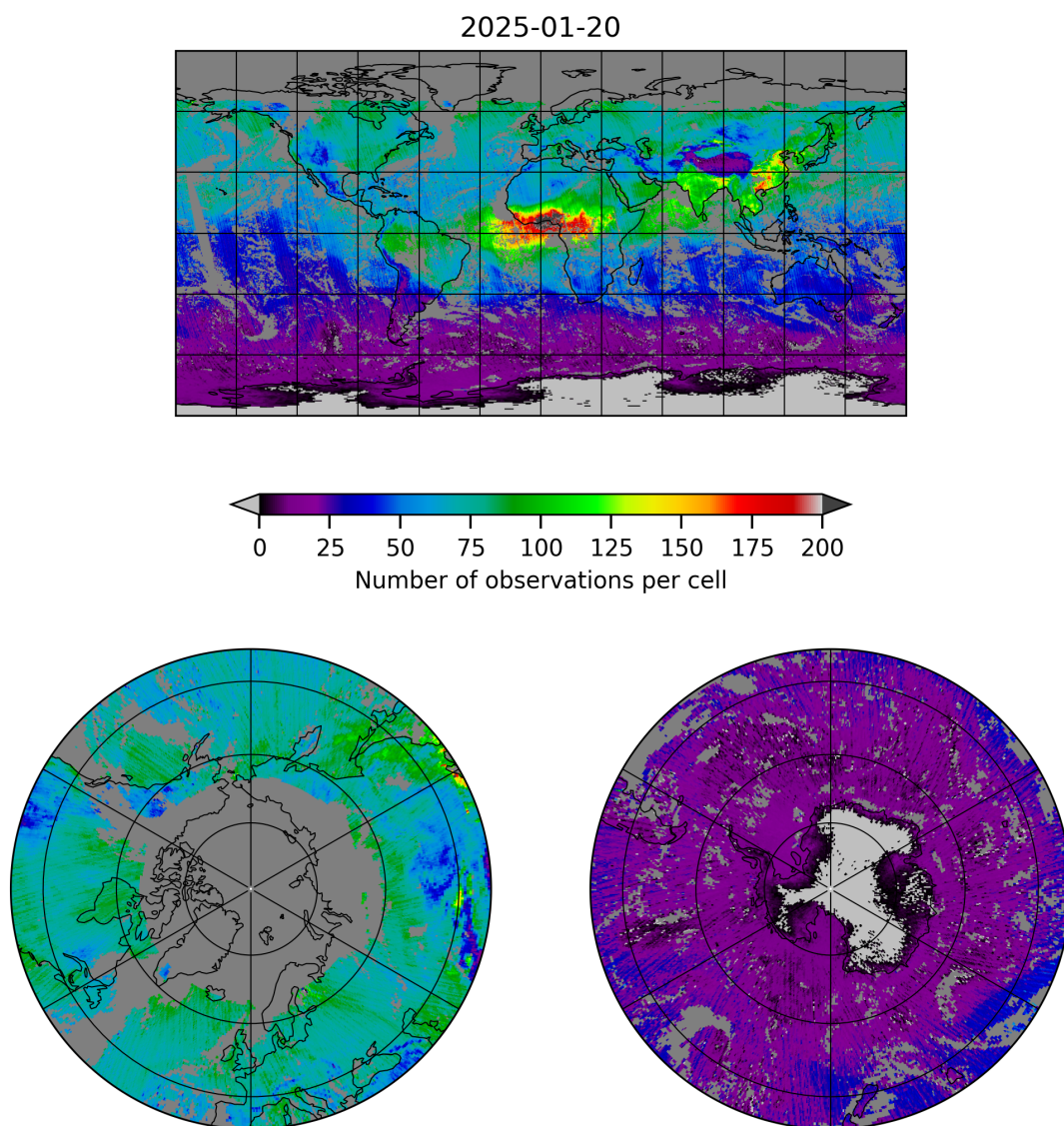
Figure 5: Map of the number of observations for 2025-01-20 to 2025-01-21
