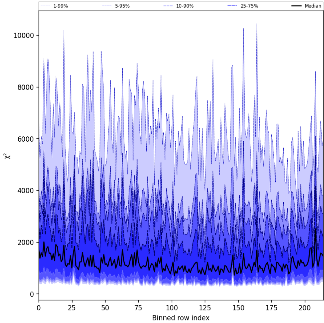
Figure 24: Along track statistics of “ \chi^2 ” for 2025-01-20 to 2025-01-21
