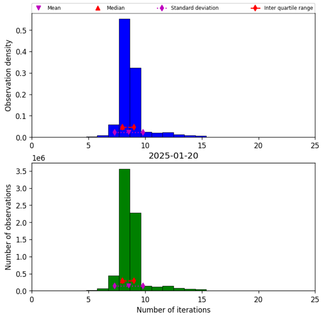
Figure 19: Histogram of “Number of iterations” for 2025-01-20 to 2025-01-21
