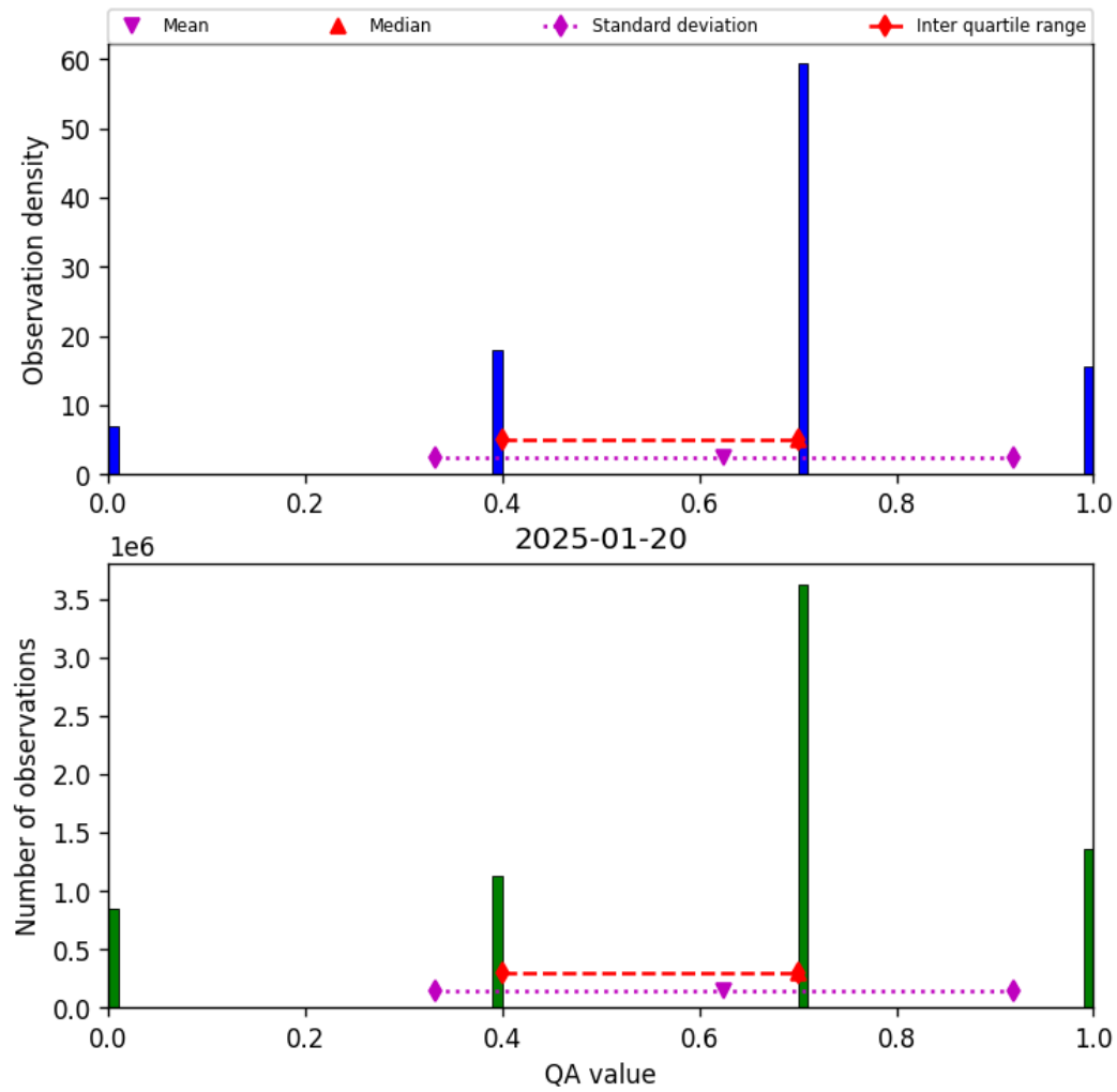
Figure 13: Histogram of “QA value” for 2025-01-20 to 2025-01-21
