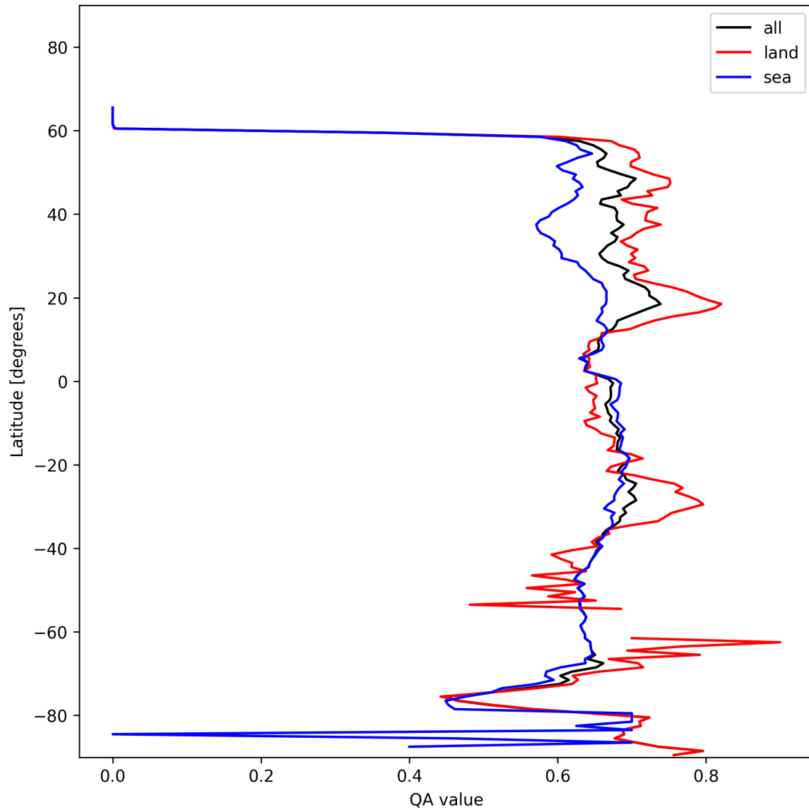
Figure 6: Zonal average of “QA value” for 2025-01-20 to 2025-01-21.
