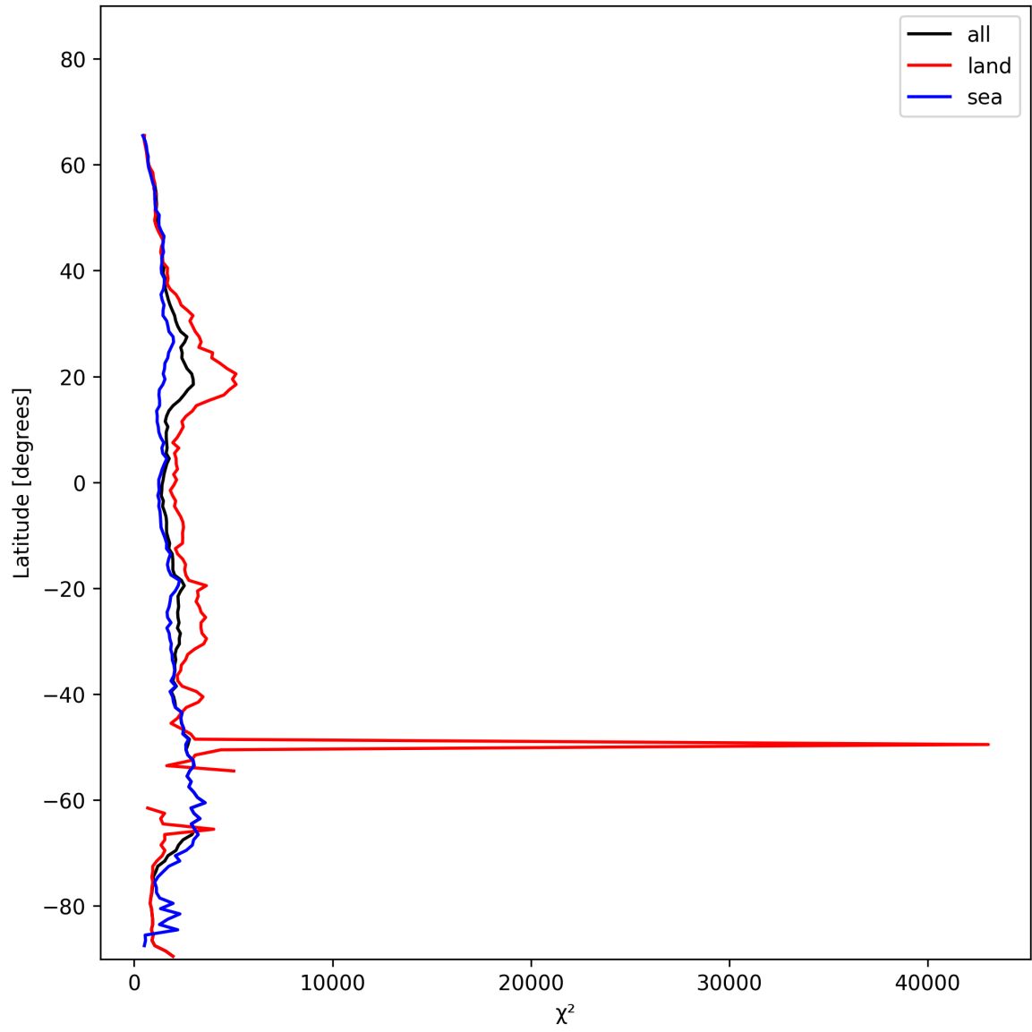
Figure 10: Zonal average of “ \chi^2 ” for 2025-01-20 to 2025-01-21.
