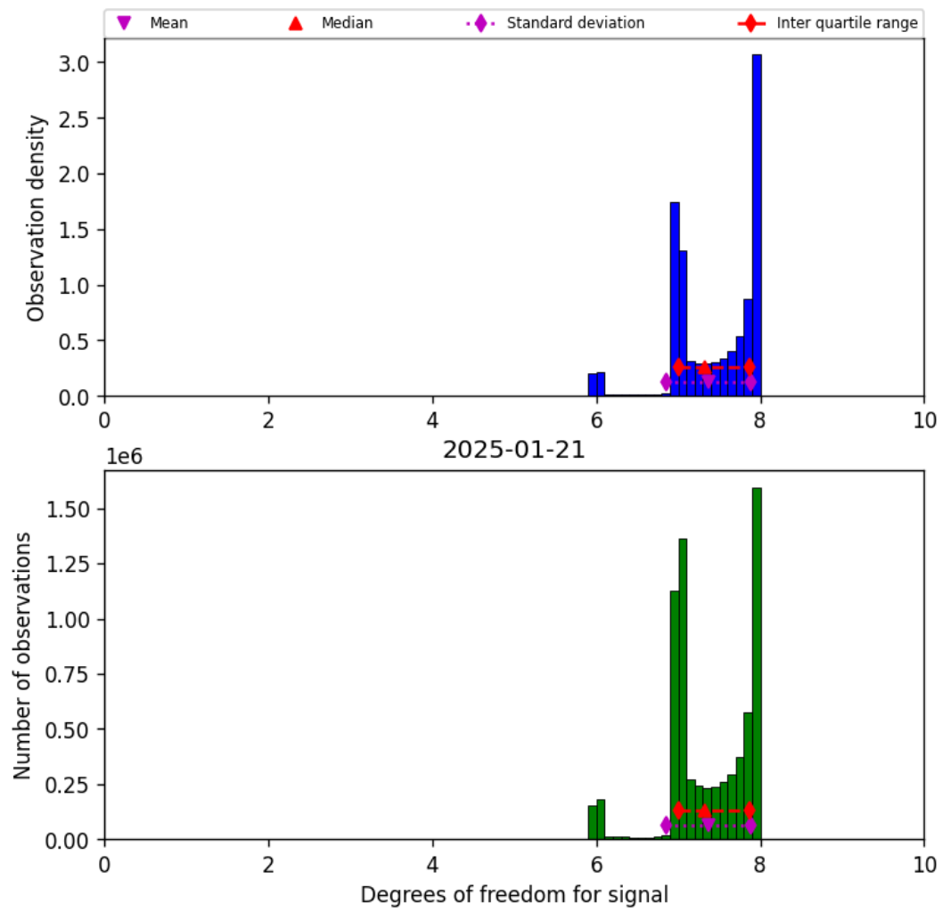
Figure 18: Histogram of “Degrees of freedom for signal” for 2025-01-21 to 2025-01-21
