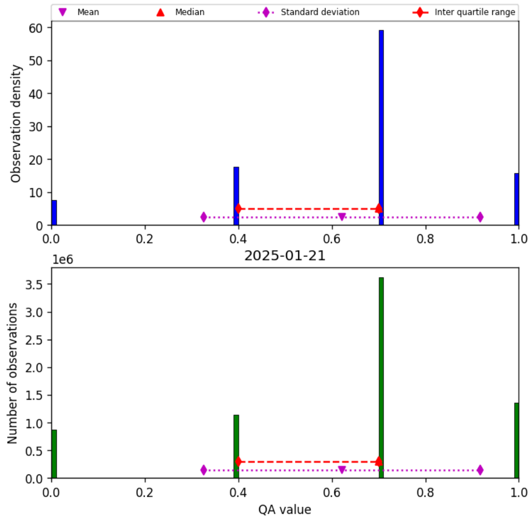
Figure 13: Histogram of “QA value” for 2025-01-21 to 2025-01-21
