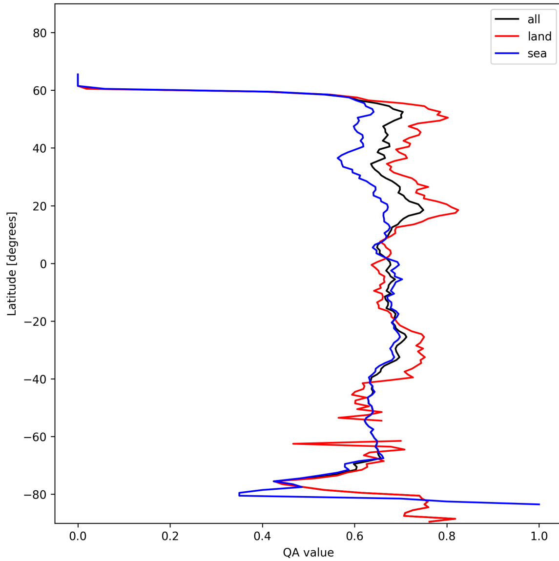
Figure 6: Zonal average of “QA value” for 2025-01-21 to 2025-01-21.
