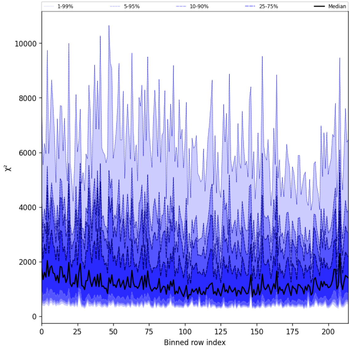
Figure 24: Along track statistics of “ \chi^2 ” for 2025-01-21 to 2025-01-21
