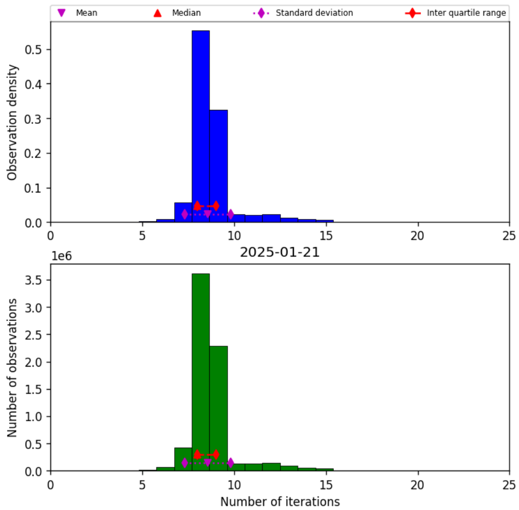
Figure 19: Histogram of “Number of iterations” for 2025-01-21 to 2025-01-21
