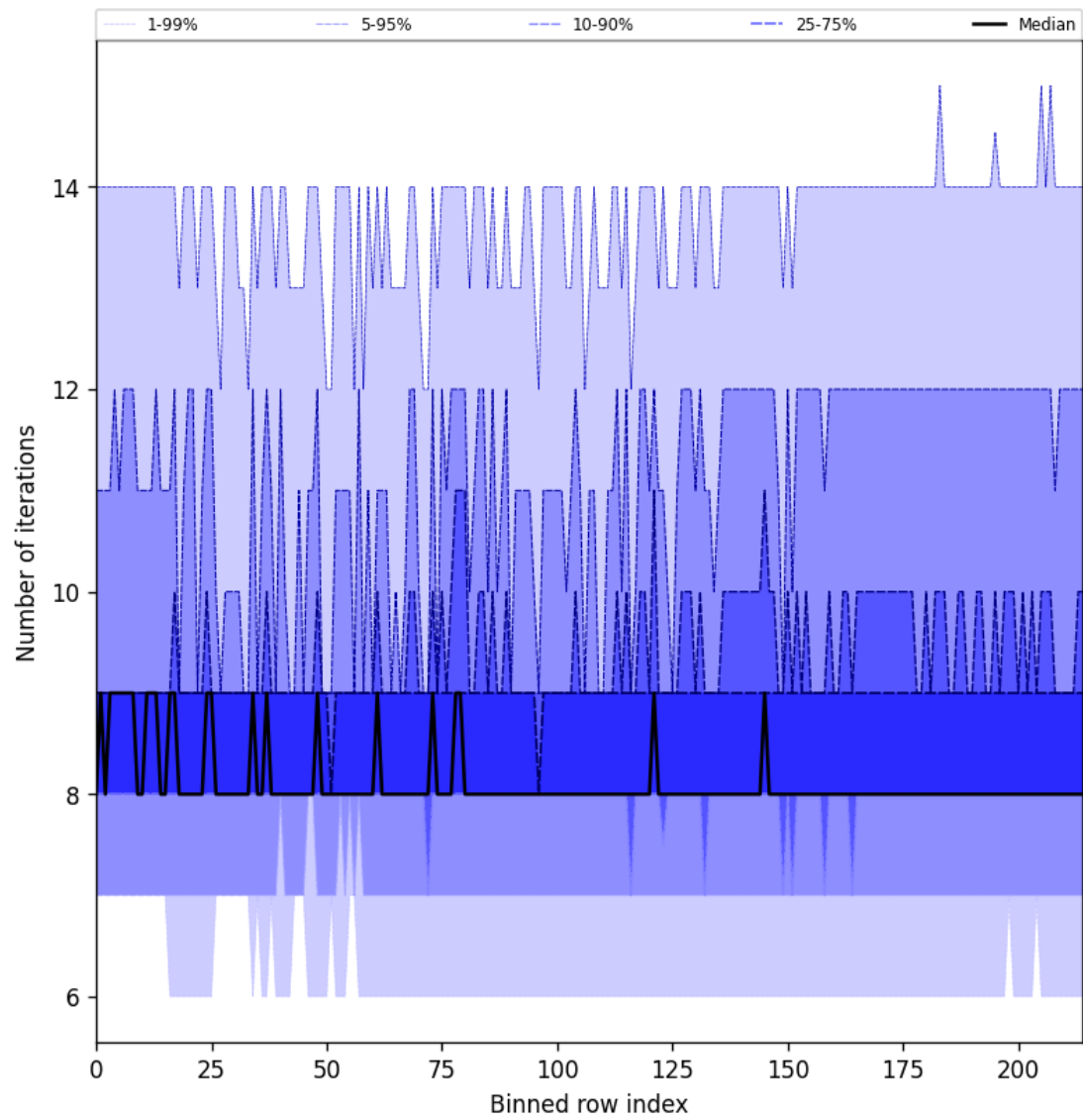
Figure 26: Along track statistics of “Number of iterations” for 2025-01-21 to 2025-01-21
