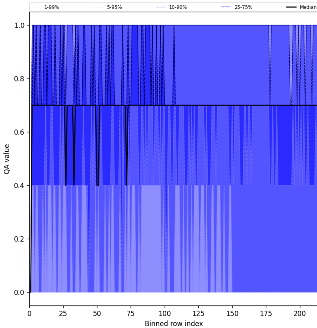
Figure 20: Along track statistics of “QA value” for 2025-01-21 to 2025-01-21
