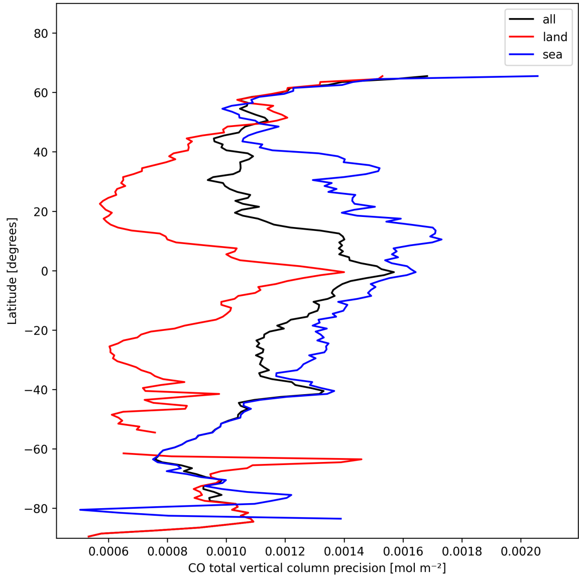
Figure 8: Zonal average of “CO total vertical column precision” for 2025-01-21 to 2025-01-21.
