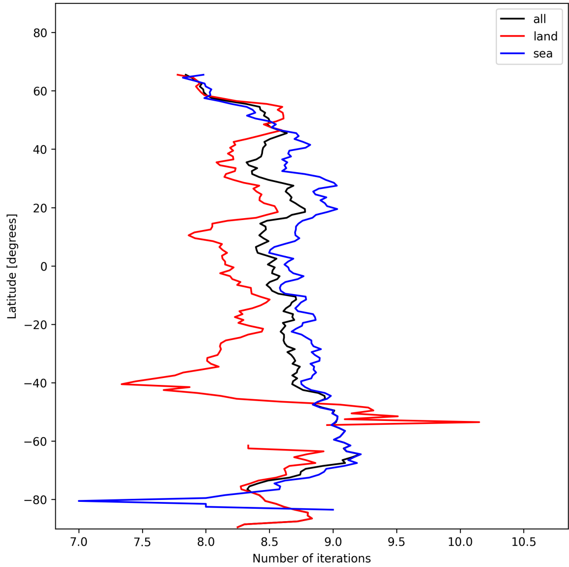
Figure 12: Zonal average of “Number of iterations” for 2025-01-21 to 2025-01-21.
