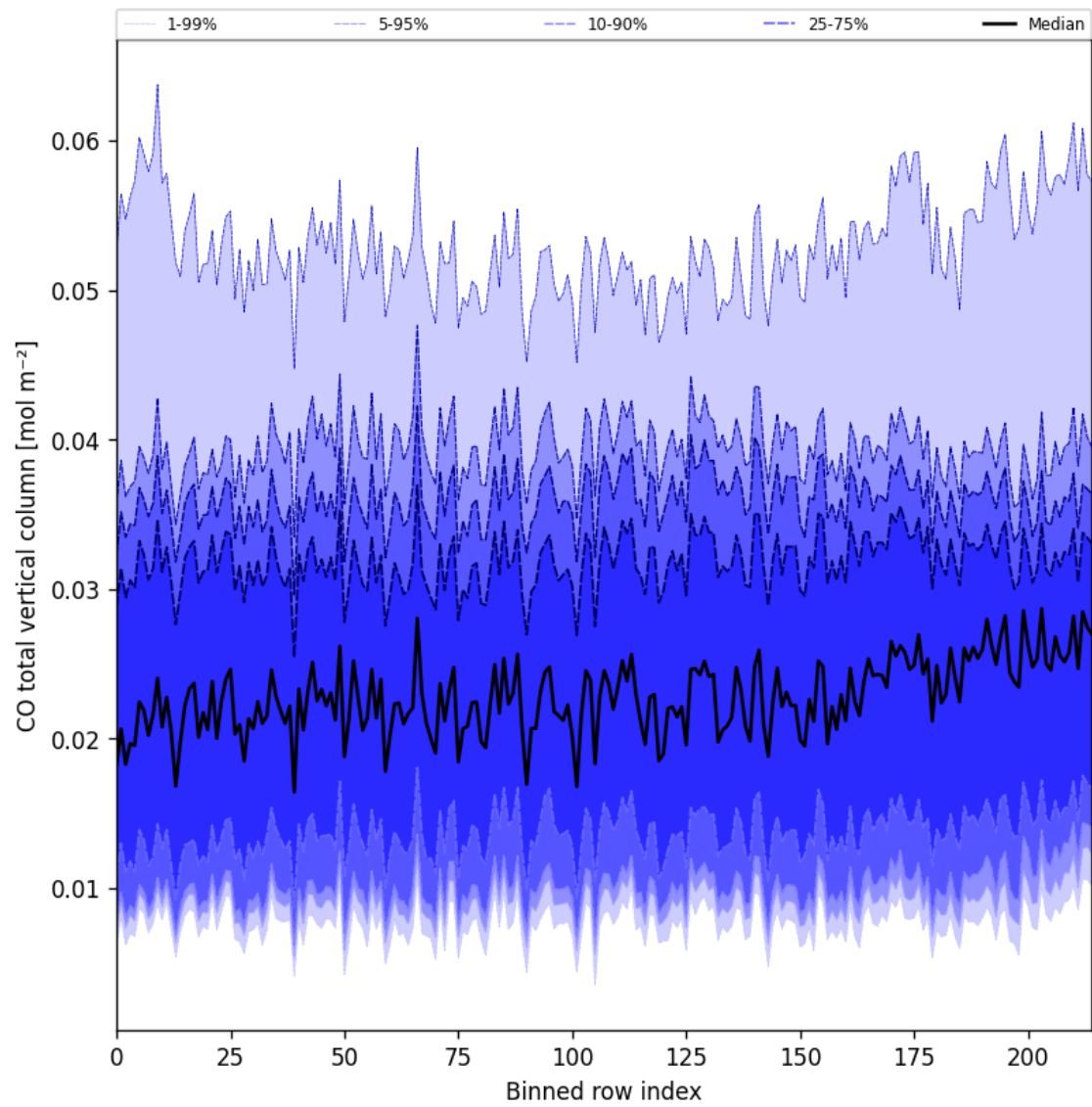
Figure 21: Along track statistics of “CO total vertical column” for 2025-01-21 to 2025-01-21
