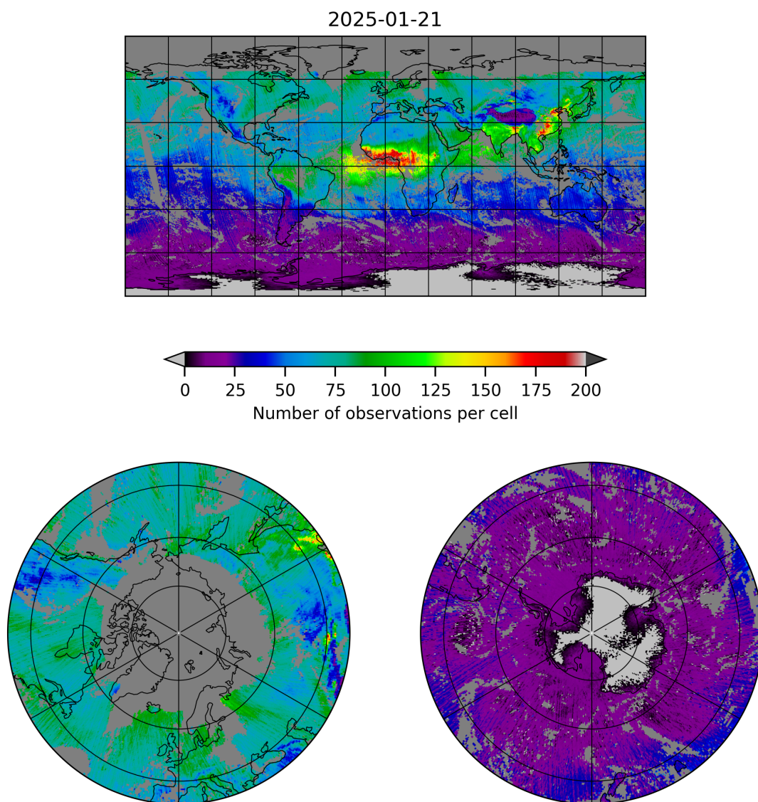
Figure 5: Map of the number of observations for 2025-01-21 to 2025-01-21
