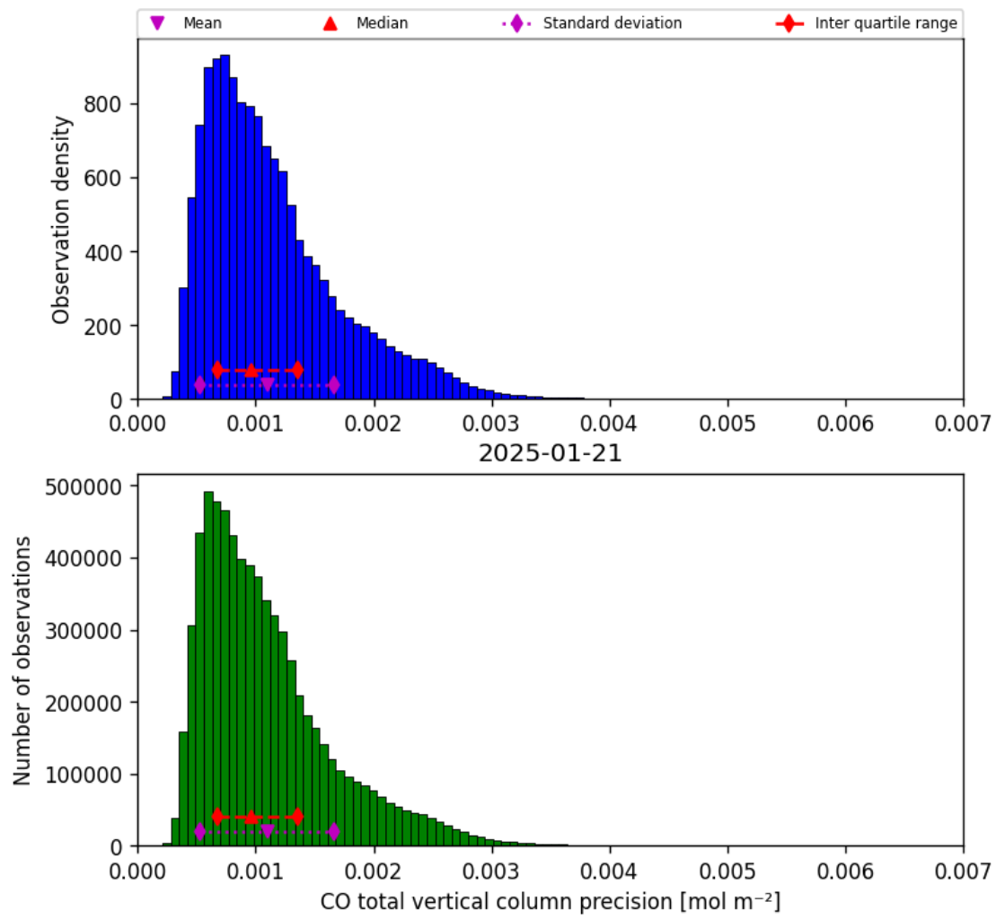
Figure 15: Histogram of “CO total vertical column precision” for 2025-01-21 to 2025-01-21
