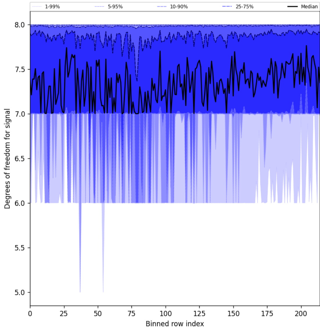
Figure 25: Along track statistics of “Degrees of freedom for signal” for 2025-01-21 to 2025-01-21
