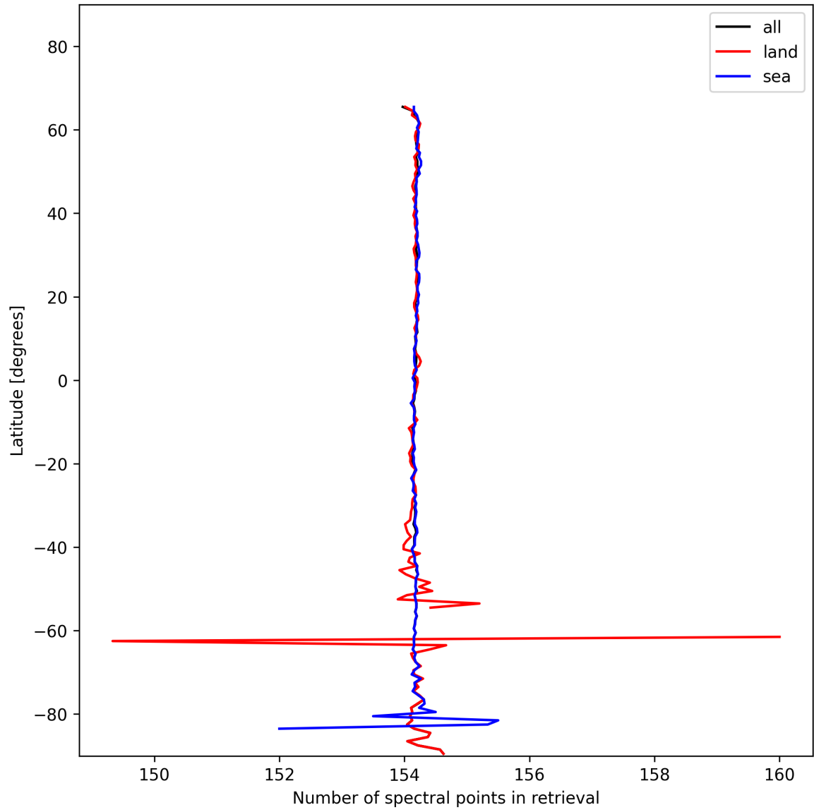
Figure 9: Zonal average of “Number of spectral points in retrieval” for 2025-01-21 to 2025-01-21.
