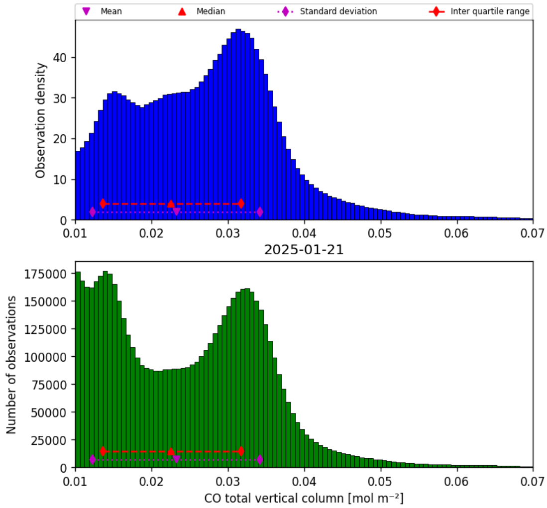
Figure 14: Histogram of “CO total vertical column” for 2025-01-21 to 2025-01-21
