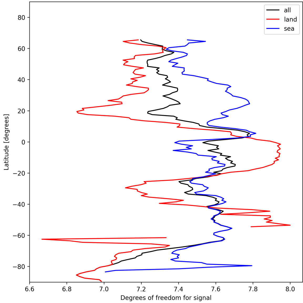
Figure 11: Zonal average of “Degrees of freedom for signal” for 2025-01-21 to 2025-01-21.
