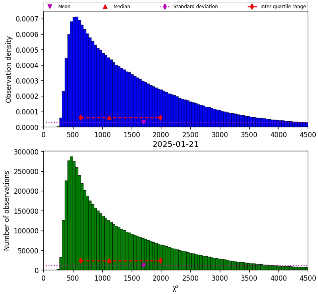
Figure 17: Histogram of " \chi^2 " for 2025-01-21 to 2025-01-21
