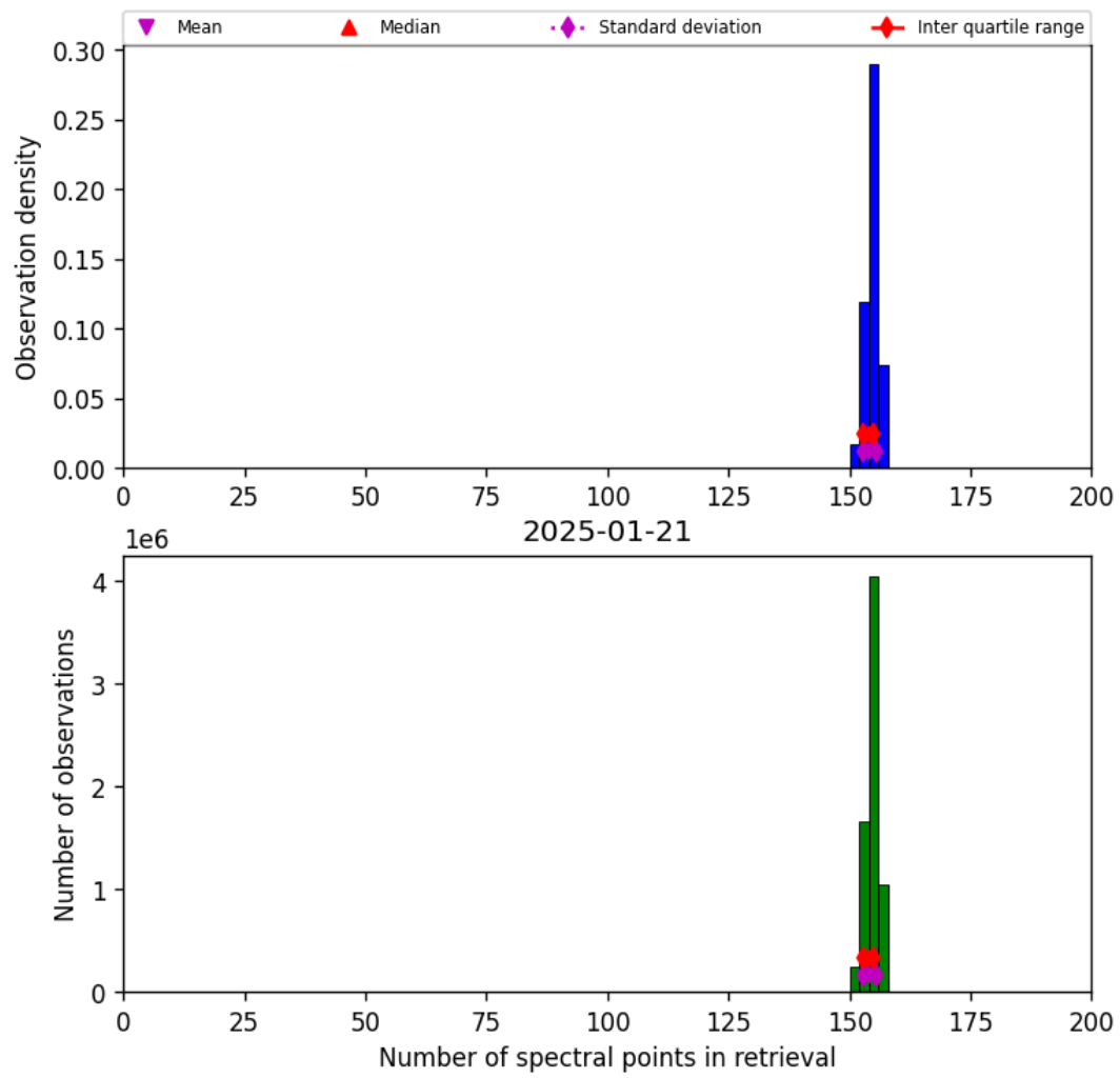
Figure 16: Histogram of “Number of spectral points in retrieval” for 2025-01-21 to 2025-01-21
