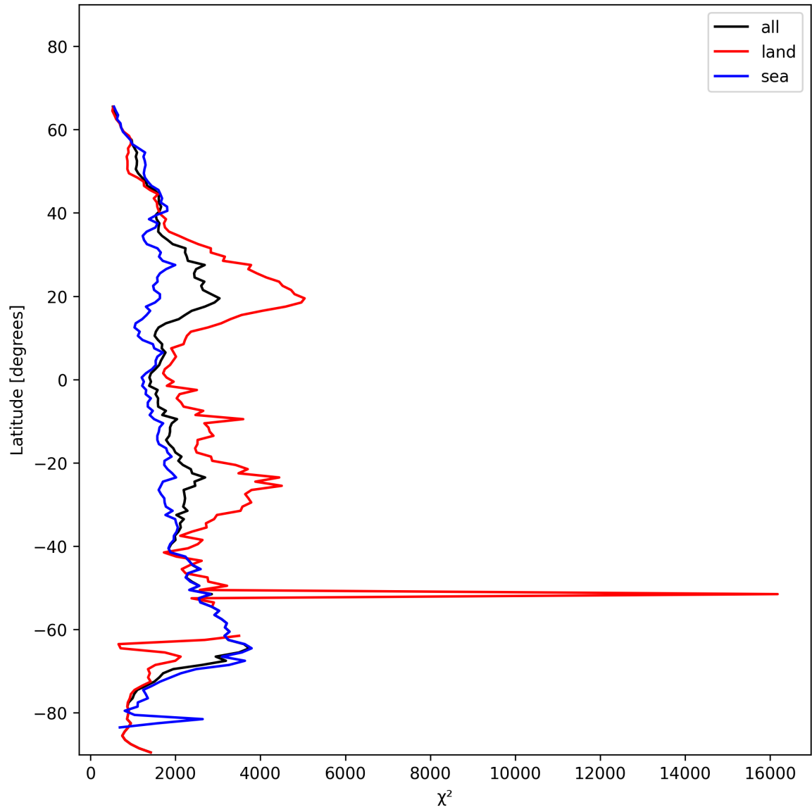
Figure 10: Zonal average of “ \chi^2 ” for 2025-01-21 to 2025-01-21.
