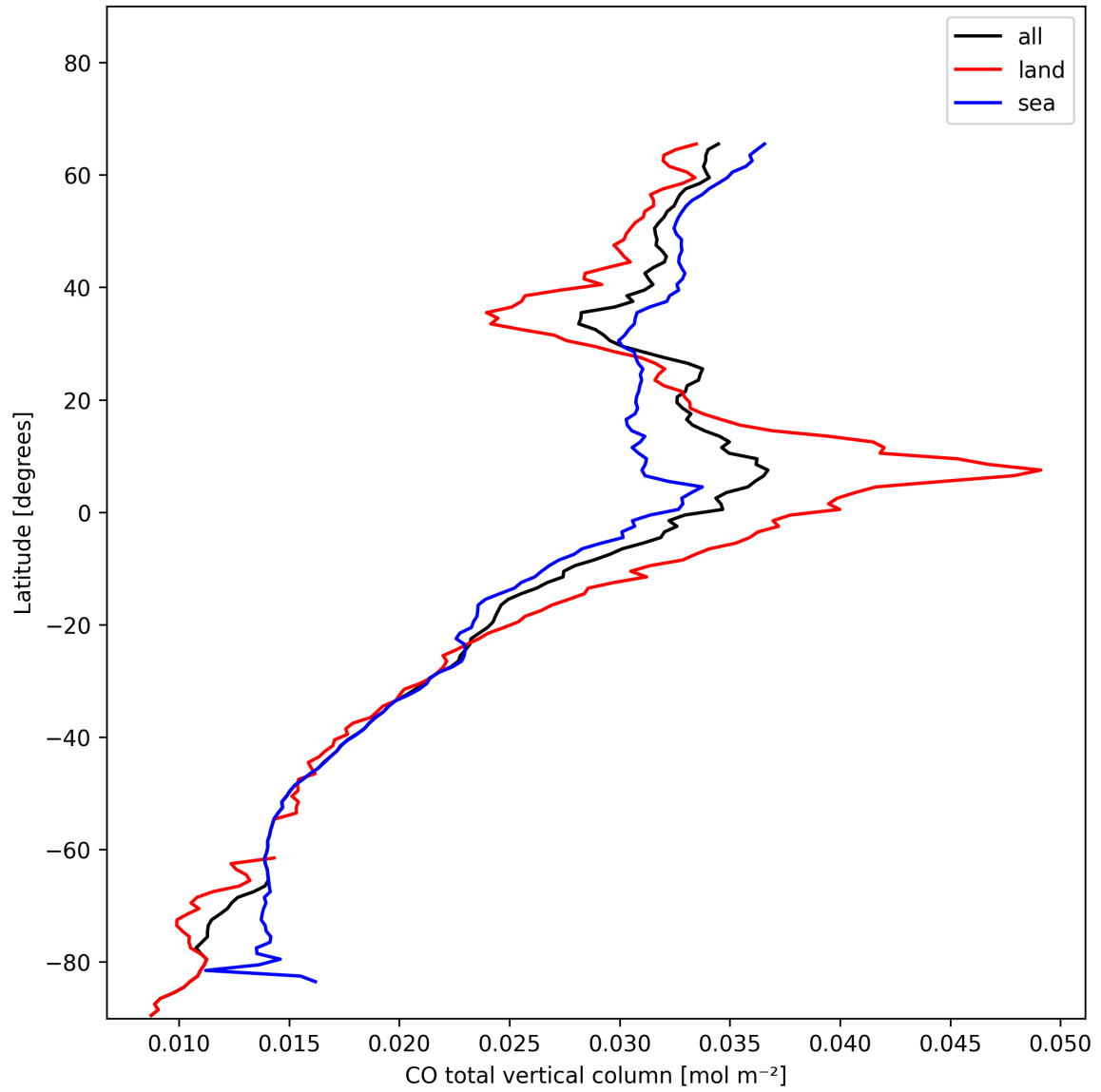
Figure 7: Zonal average of “CO total vertical column” for 2025-01-21 to 2025-01-21.
