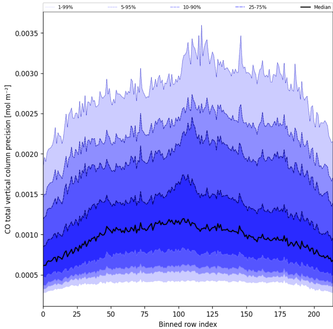
Figure 22: Along track statistics of “CO total vertical column precision” for 2025-01-21 to 2025-01-21
