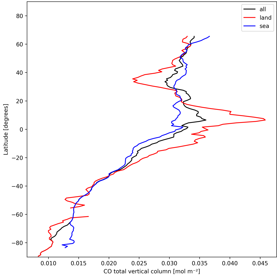
Figure 7: Zonal average of “CO total vertical column” for 2025-01-22 to 2025-01-23.
