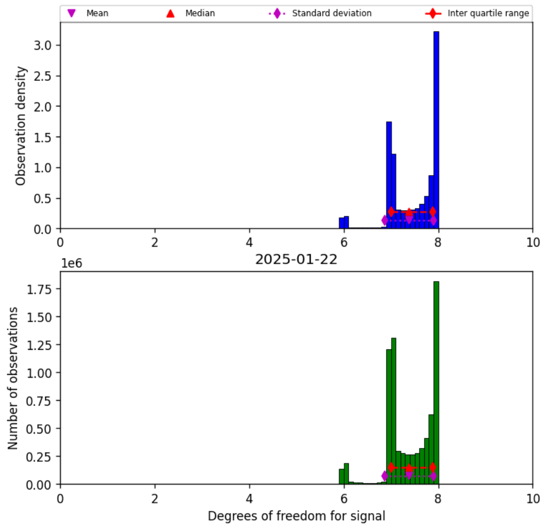
Figure 18: Histogram of “Degrees of freedom for signal” for 2025-01-22 to 2025-01-23
