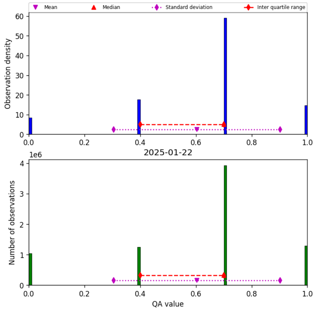
Figure 13: Histogram of “QA value” for 2025-01-22 to 2025-01-23
