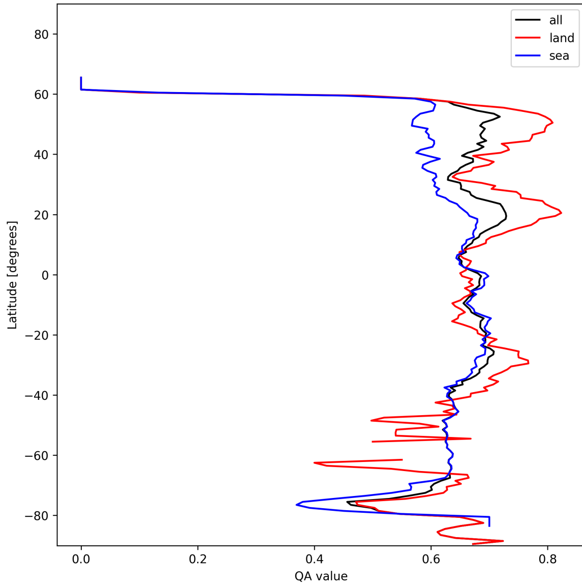
Figure 6: Zonal average of “QA value” for 2025-01-22 to 2025-01-23.
