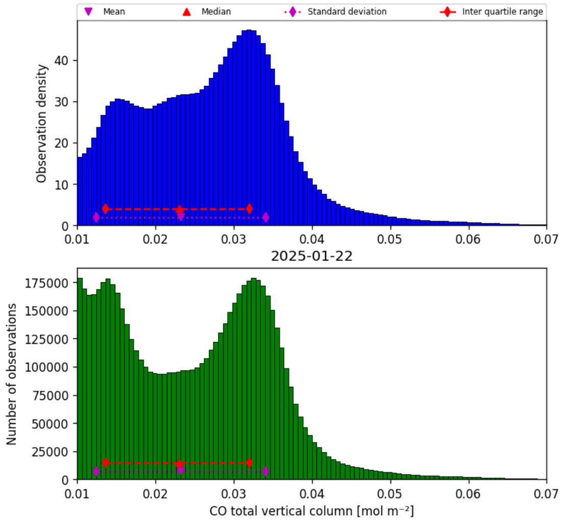
Figure 14: Histogram of “CO total vertical column” for 2025-01-22 to 2025-01-23
