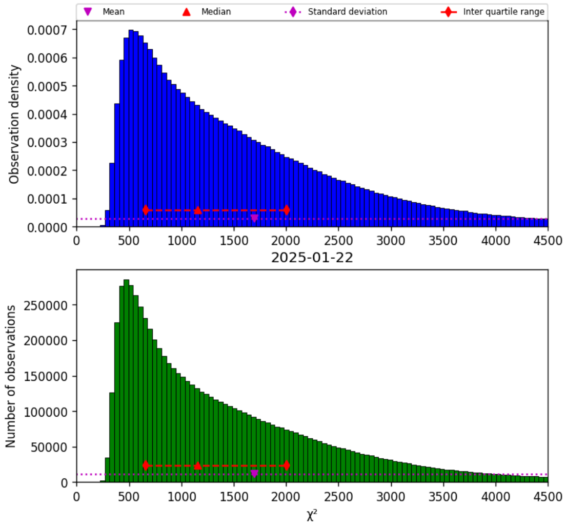
Figure 17: Histogram of “ \chi^2 ” for 2025-01-22 to 2025-01-23
