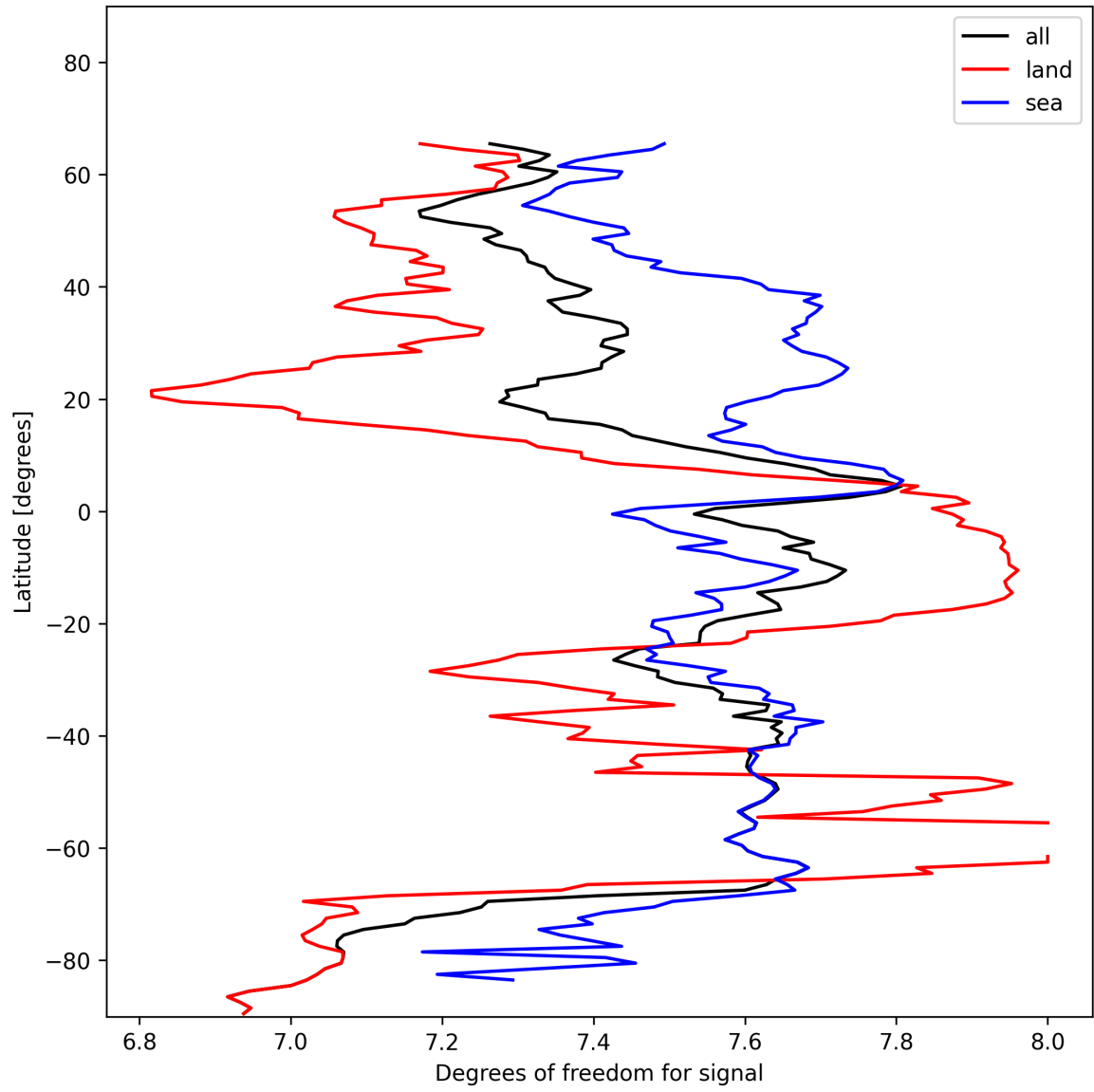
Figure 11: Zonal average of “Degrees of freedom for signal” for 2025-01-22 to 2025-01-23.
