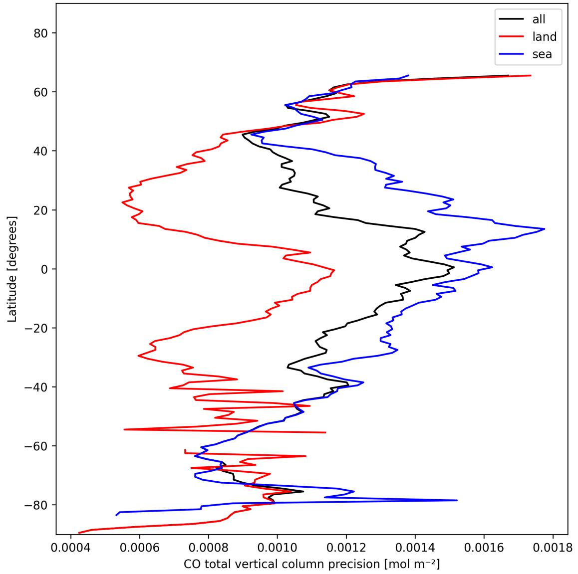
Figure 8: Zonal average of “CO total vertical column precision” for 2025-01-22 to 2025-01-23.
