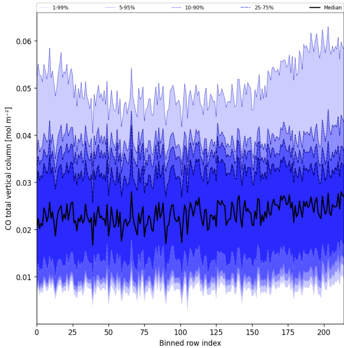
Figure 21: Along track statistics of “CO total vertical column” for 2025-01-22 to 2025-01-23
