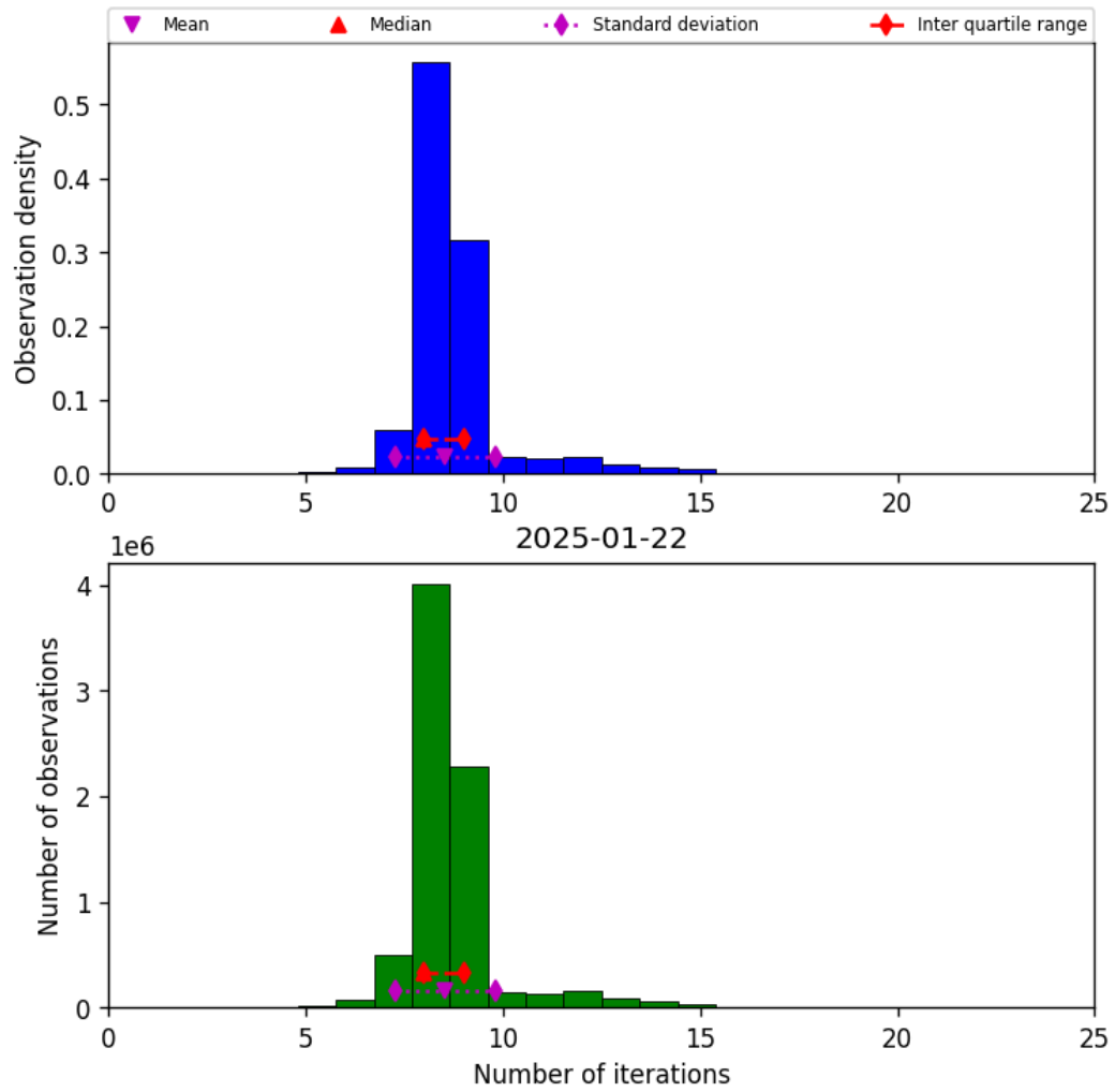
Figure 19: Histogram of “Number of iterations” for 2025-01-22 to 2025-01-23
