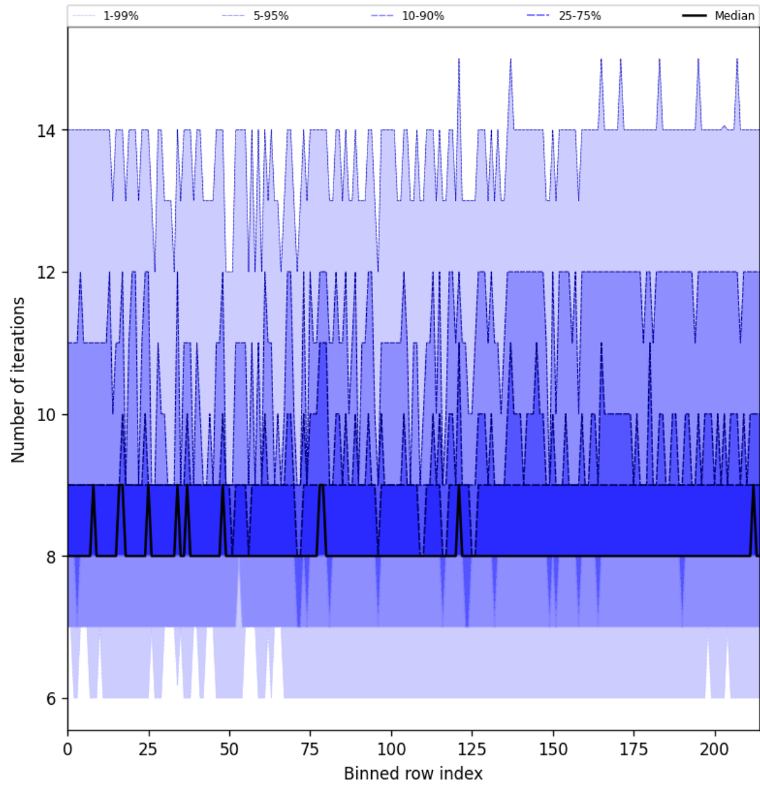
Figure 26: Along track statistics of “Number of iterations” for 2025-01-22 to 2025-01-23
