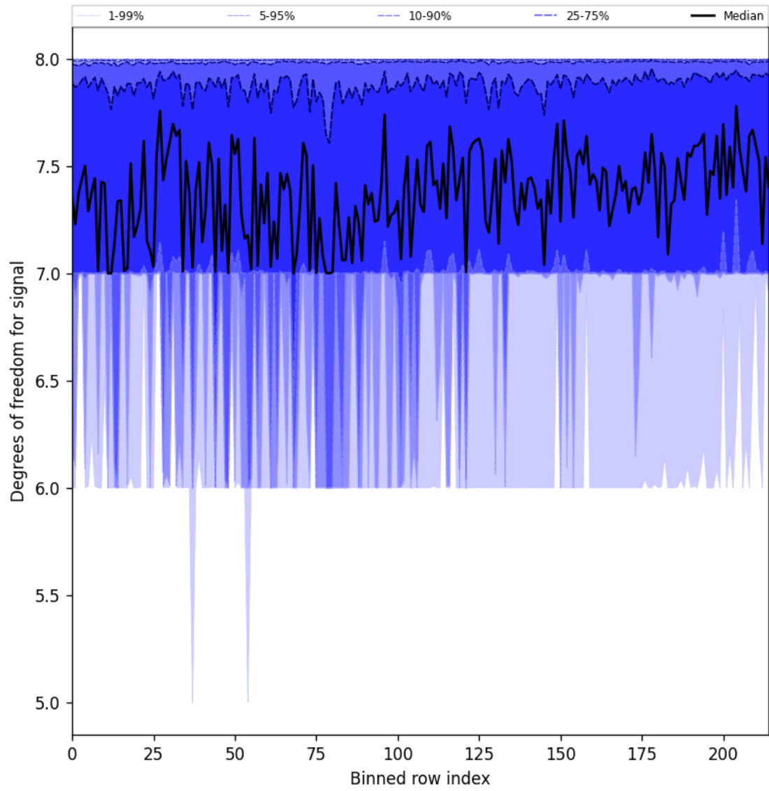
Figure 25: Along track statistics of “Degrees of freedom for signal” for 2025-01-22 to 2025-01-23
