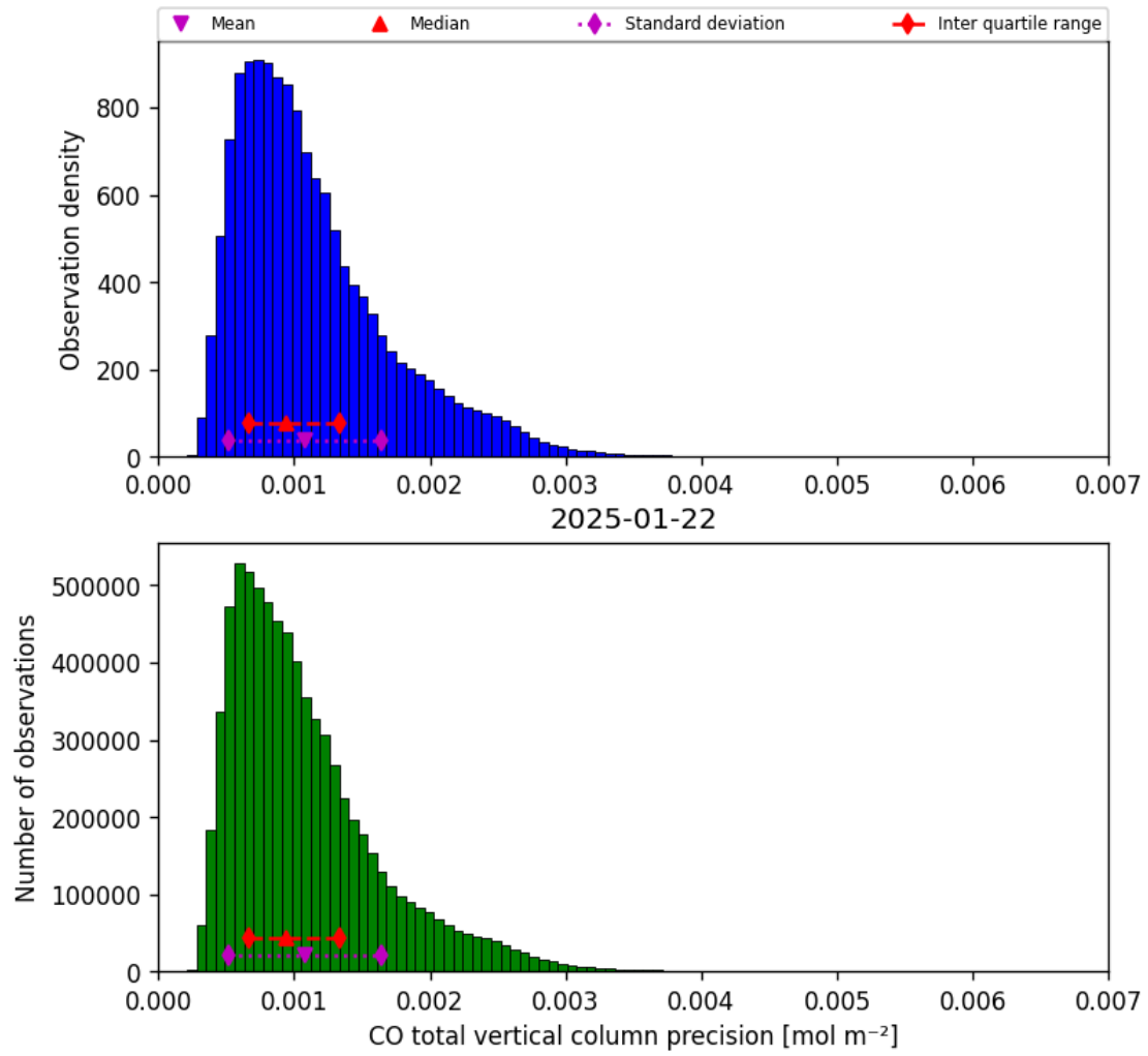
Figure 15: Histogram of “CO total vertical column precision” for 2025-01-22 to 2025-01-23
