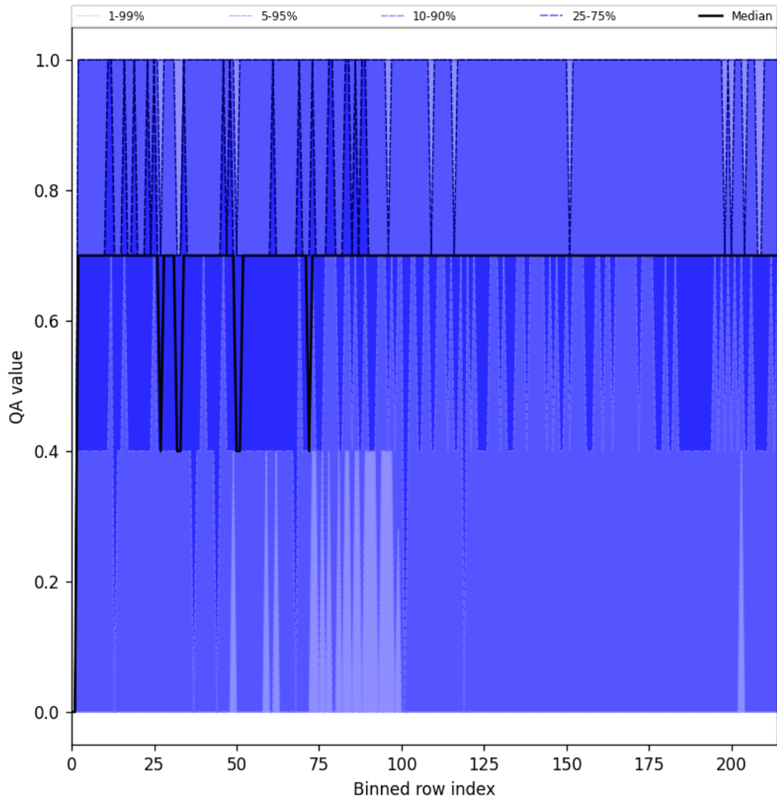
Figure 20: Along track statistics of “QA value” for 2025-01-22 to 2025-01-23
