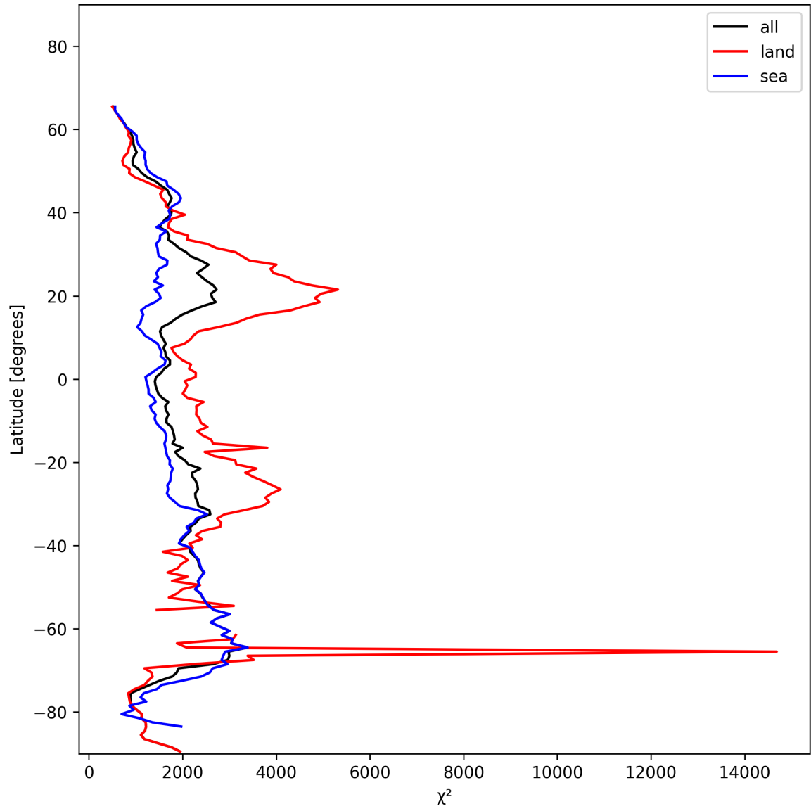
Figure 10: Zonal average of “ \chi^2 ” for 2025-01-22 to 2025-01-23.
