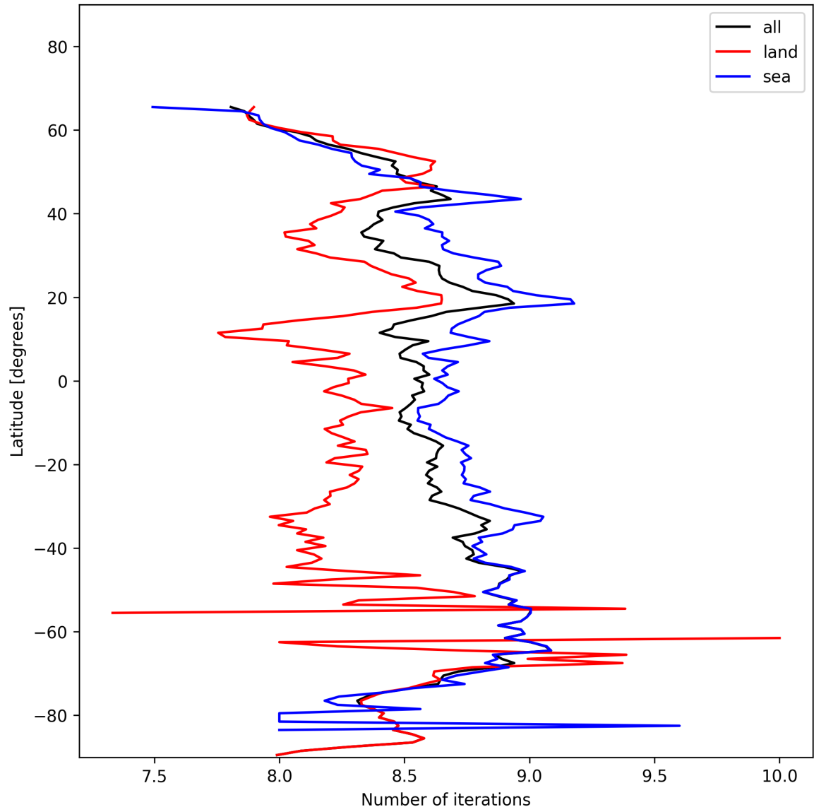
Figure 12: Zonal average of “Number of iterations” for 2025-01-22 to 2025-01-23.
