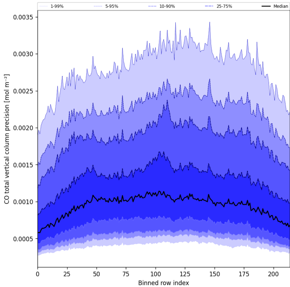
Figure 22: Along track statistics of “CO total vertical column precision” for 2025-01-22 to 2025-01-23
