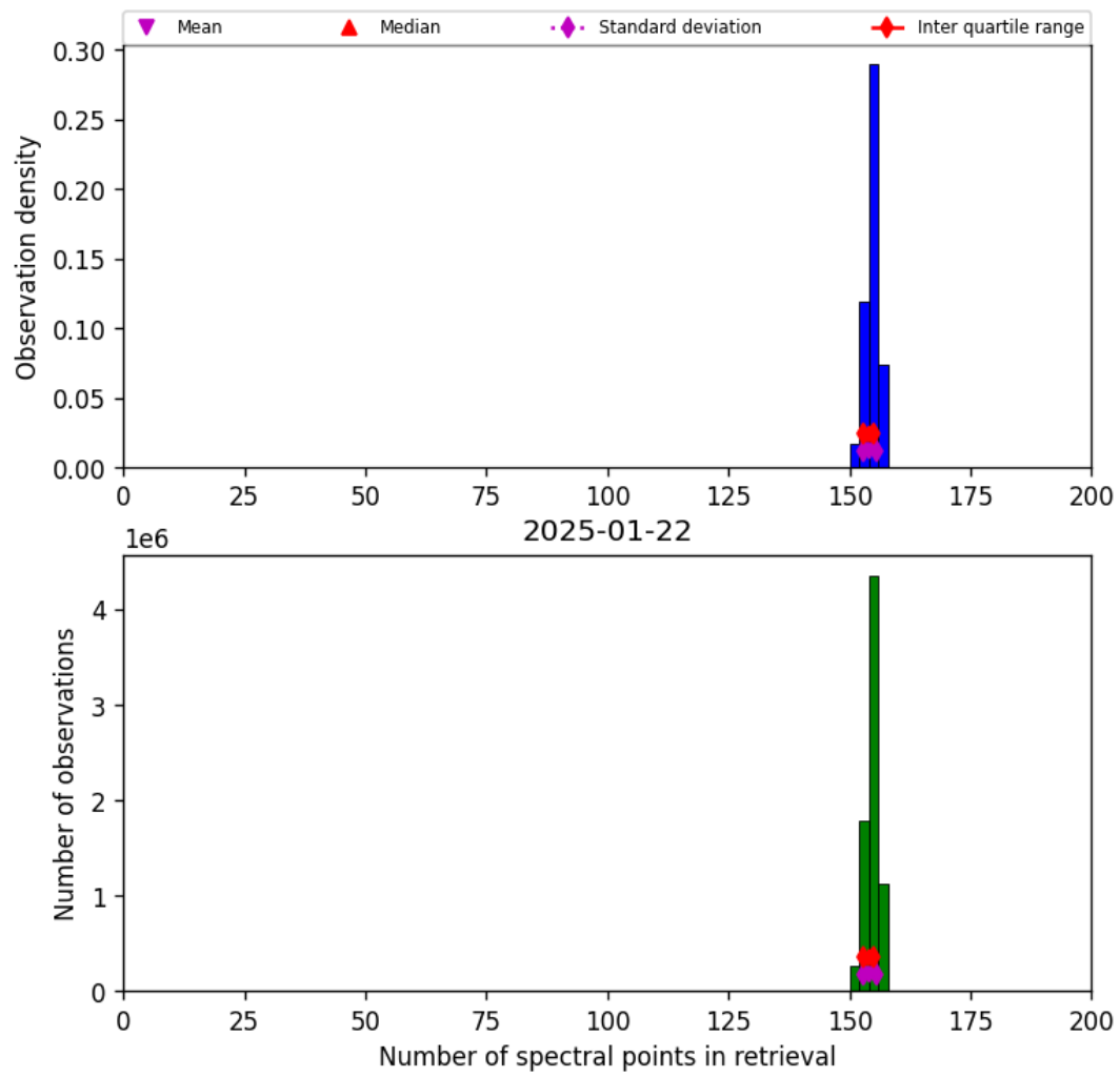
Figure 16: Histogram of “Number of spectral points in retrieval” for 2025-01-22 to 2025-01-23
