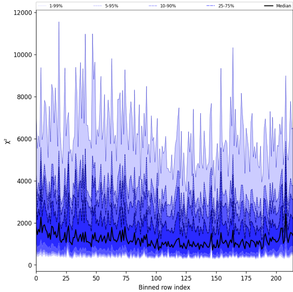
Figure 24: Along track statistics of “ \chi^2 ” for 2025-01-22 to 2025-01-23
