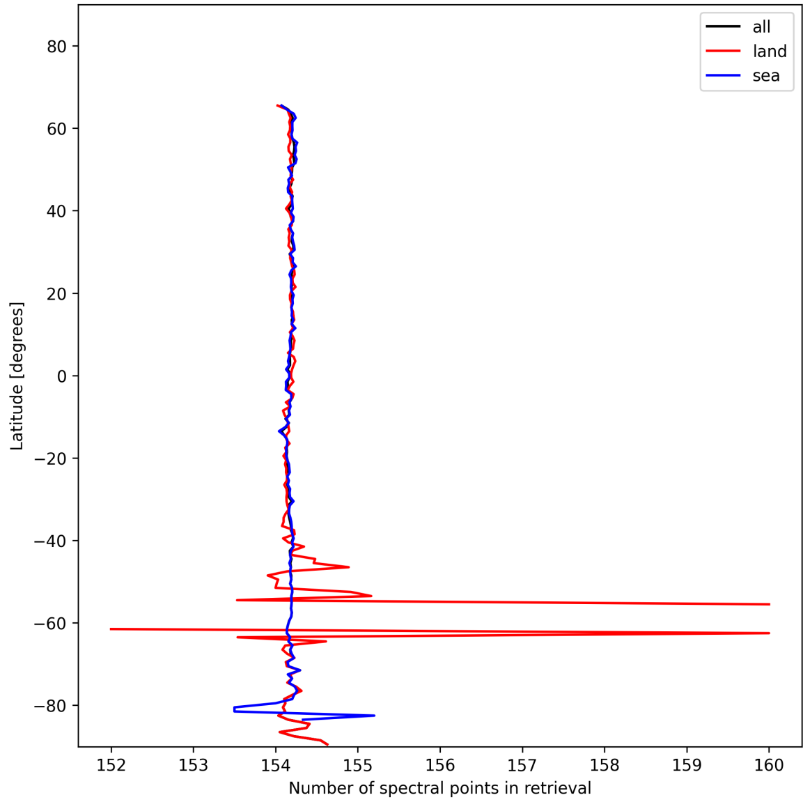
Figure 9: Zonal average of “Number of spectral points in retrieval” for 2025-01-22 to 2025-01-23.
