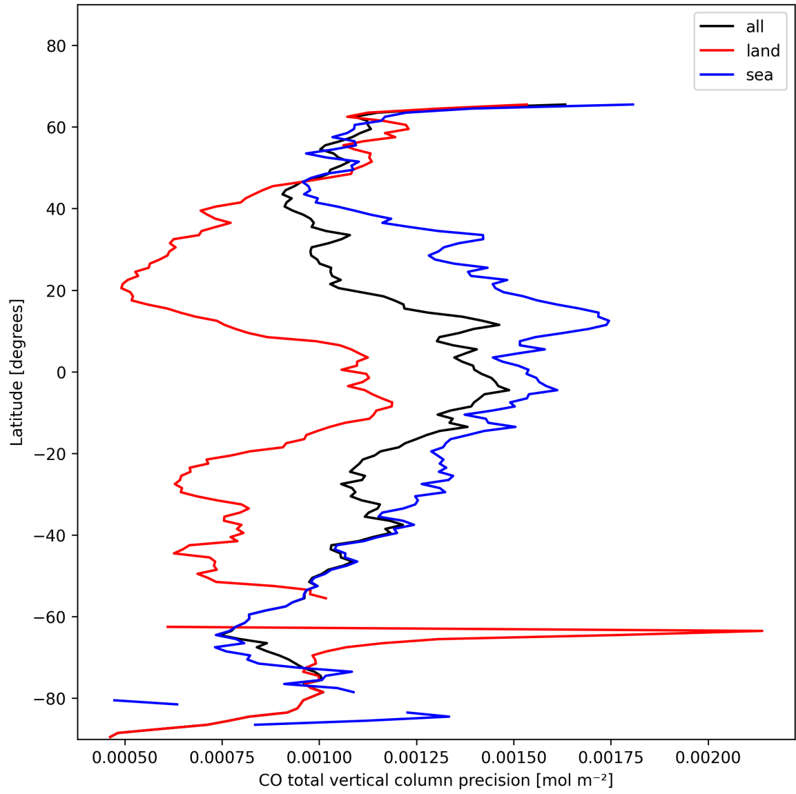
Figure 8: Zonal average of “CO total vertical column precision” for 2025-01-23 to 2025-01-24.
