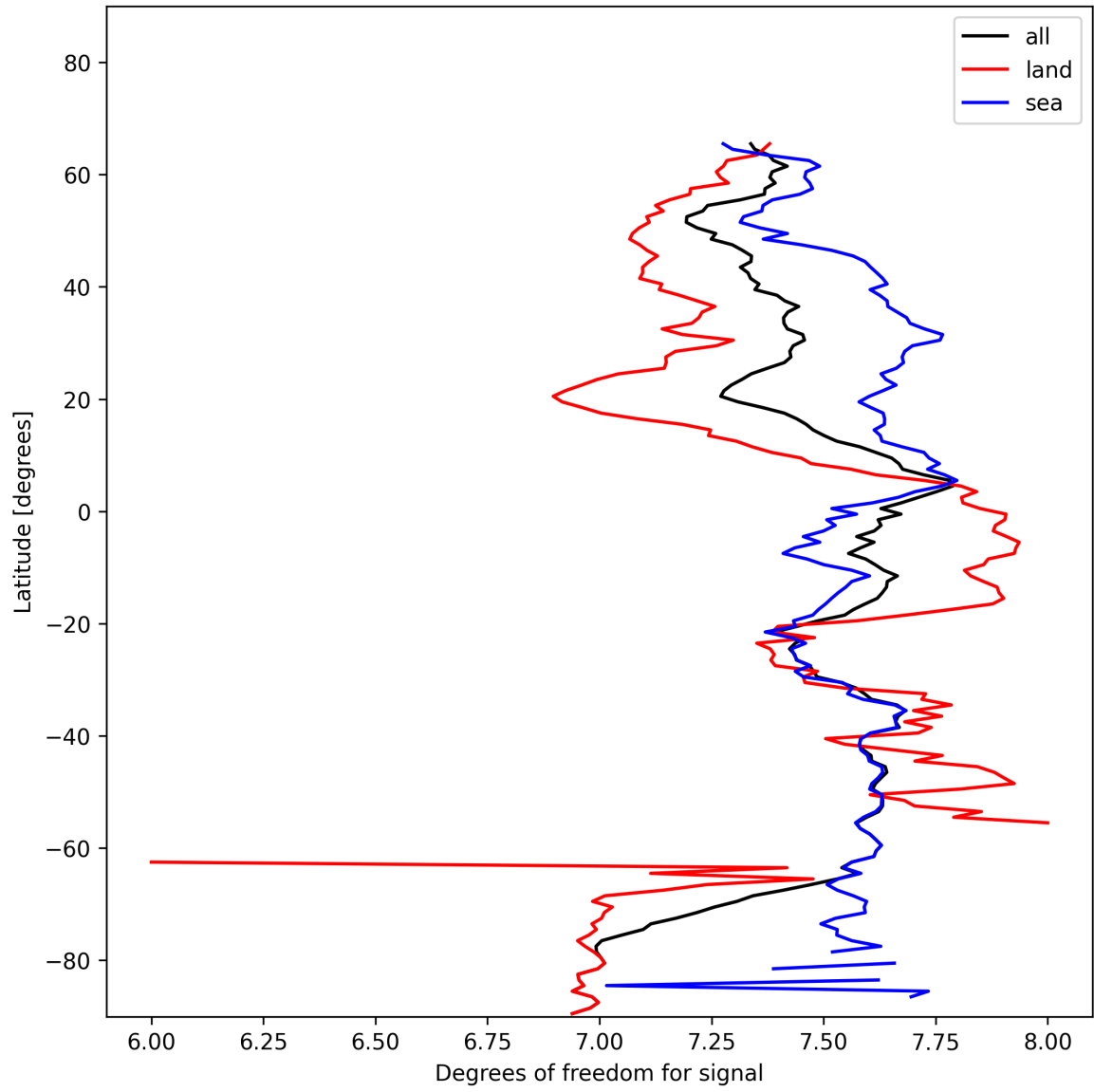
Figure 11: Zonal average of “Degrees of freedom for signal” for 2025-01-23 to 2025-01-24.
