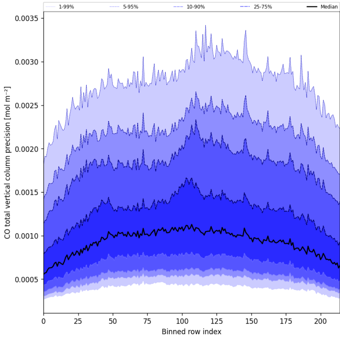
Figure 22: Along track statistics of “CO total vertical column precision” for 2025-01-23 to 2025-01-24
