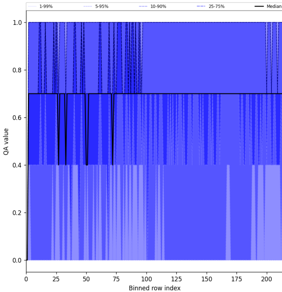
Figure 20: Along track statistics of “QA value” for 2025-01-23 to 2025-01-24
