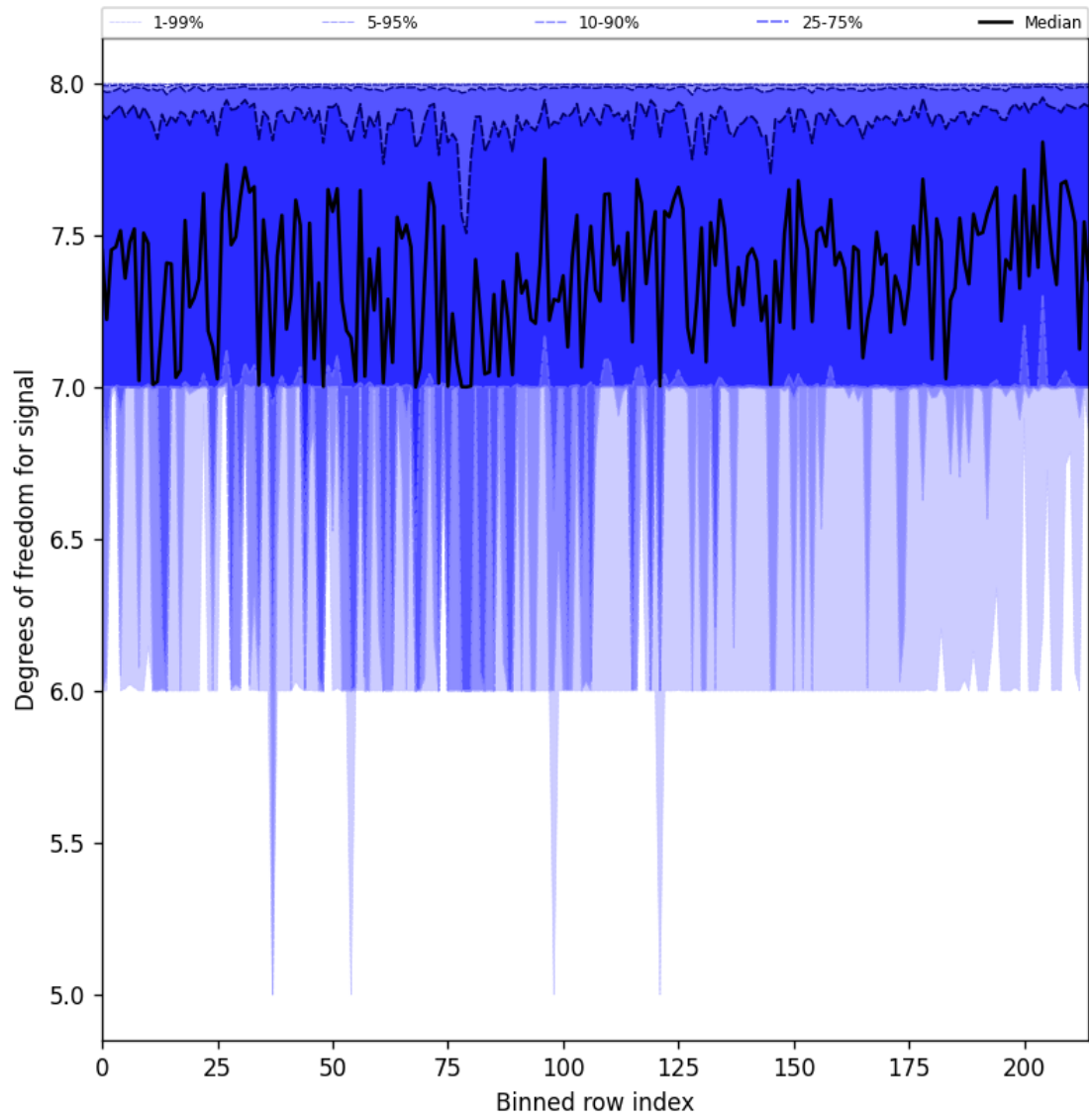
Figure 25: Along track statistics of “Degrees of freedom for signal” for 2025-01-23 to 2025-01-24
