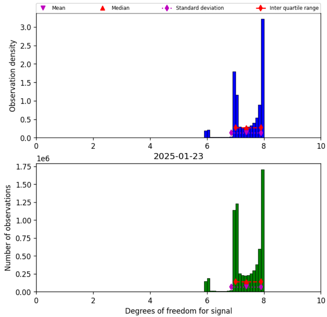
Figure 18: Histogram of “Degrees of freedom for signal” for 2025-01-23 to 2025-01-24
