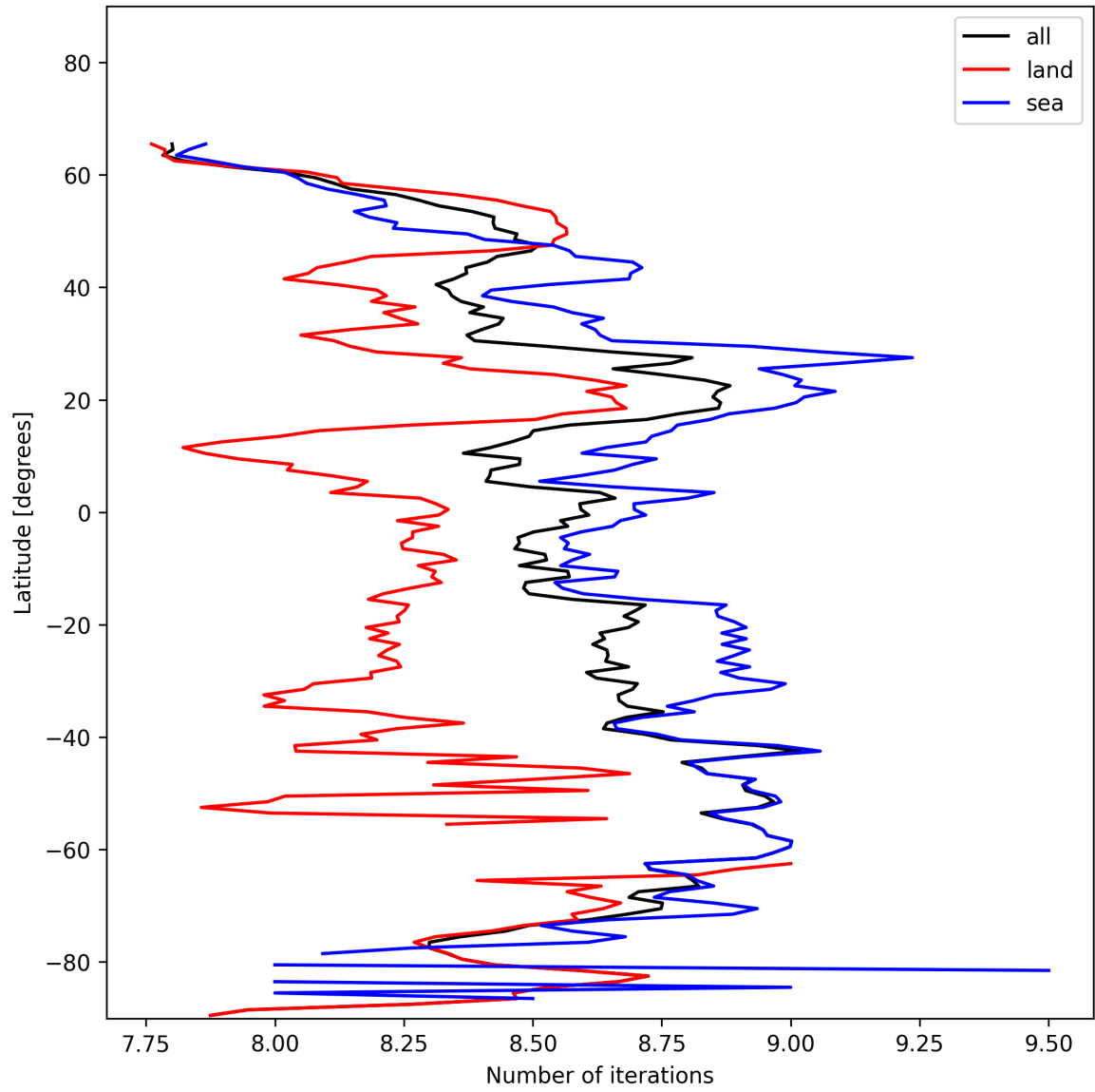
Figure 12: Zonal average of “Number of iterations” for 2025-01-23 to 2025-01-24.
