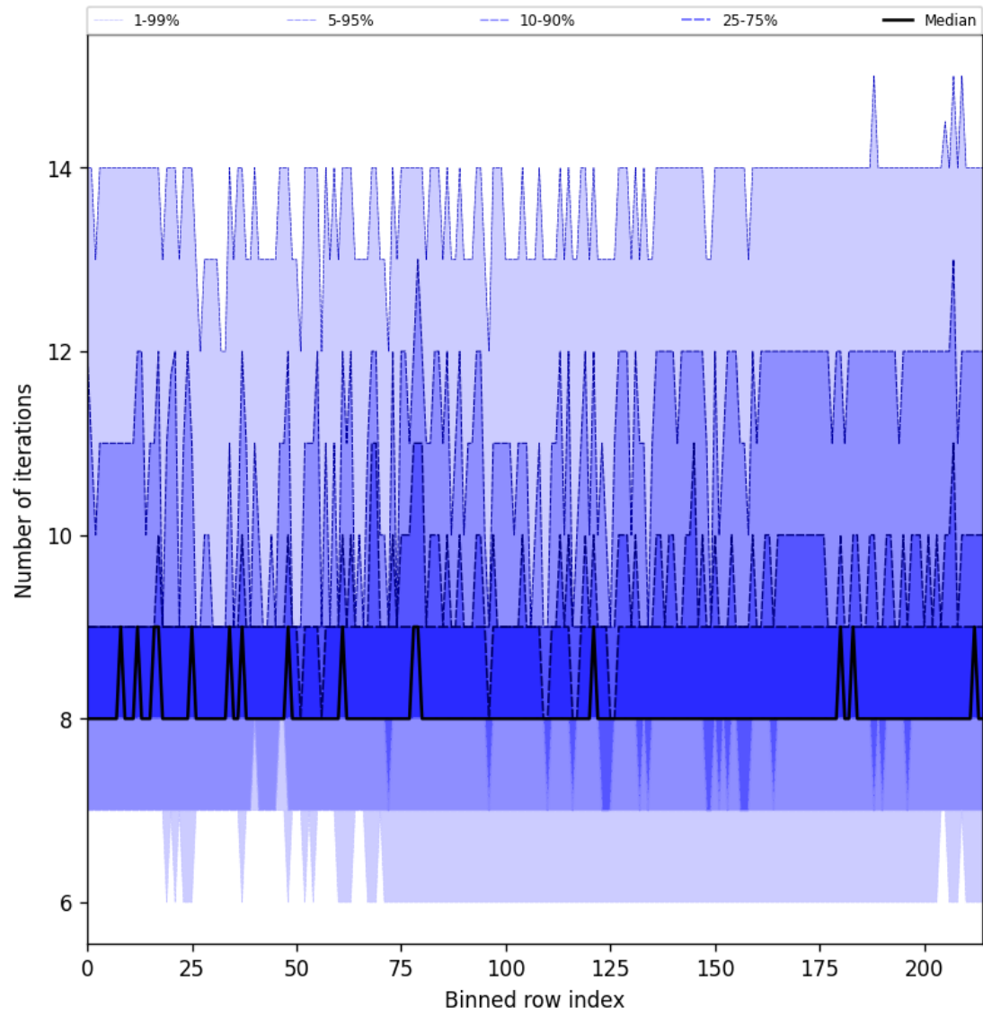
Figure 26: Along track statistics of “Number of iterations” for 2025-01-23 to 2025-01-24
