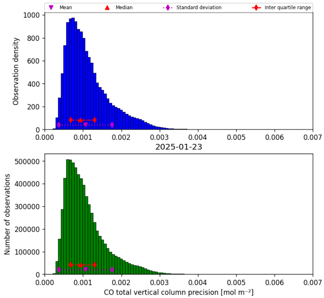
Figure 15: Histogram of “CO total vertical column precision” for 2025-01-23 to 2025-01-24
