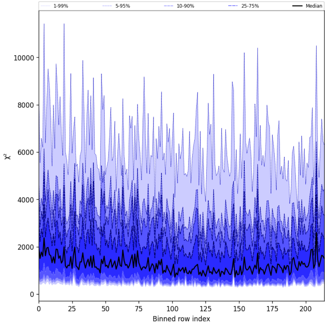
Figure 24: Along track statistics of “ \chi^2 ” for 2025-01-23 to 2025-01-24
