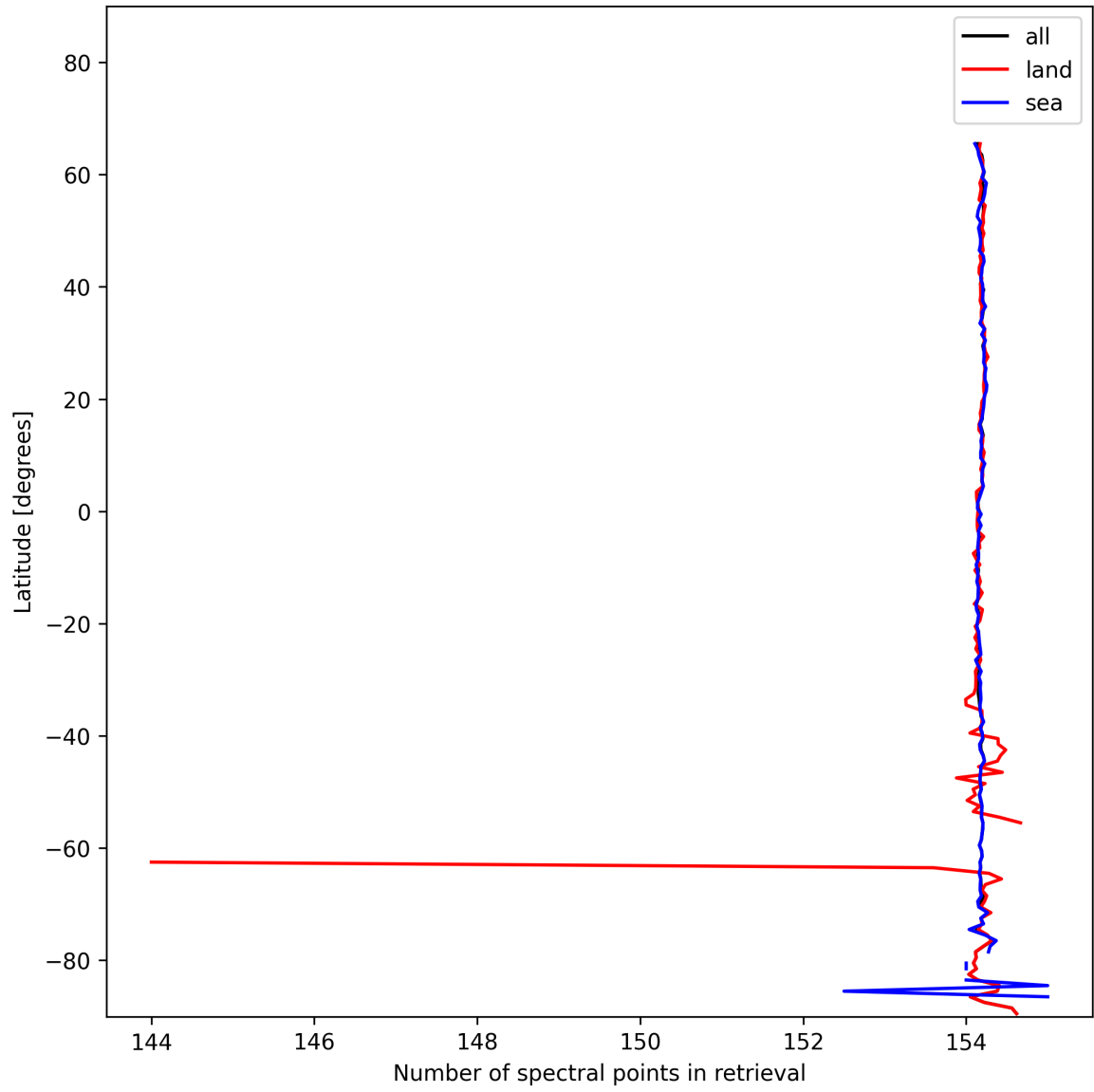
Figure 9: Zonal average of “Number of spectral points in retrieval” for 2025-01-23 to 2025-01-24.
