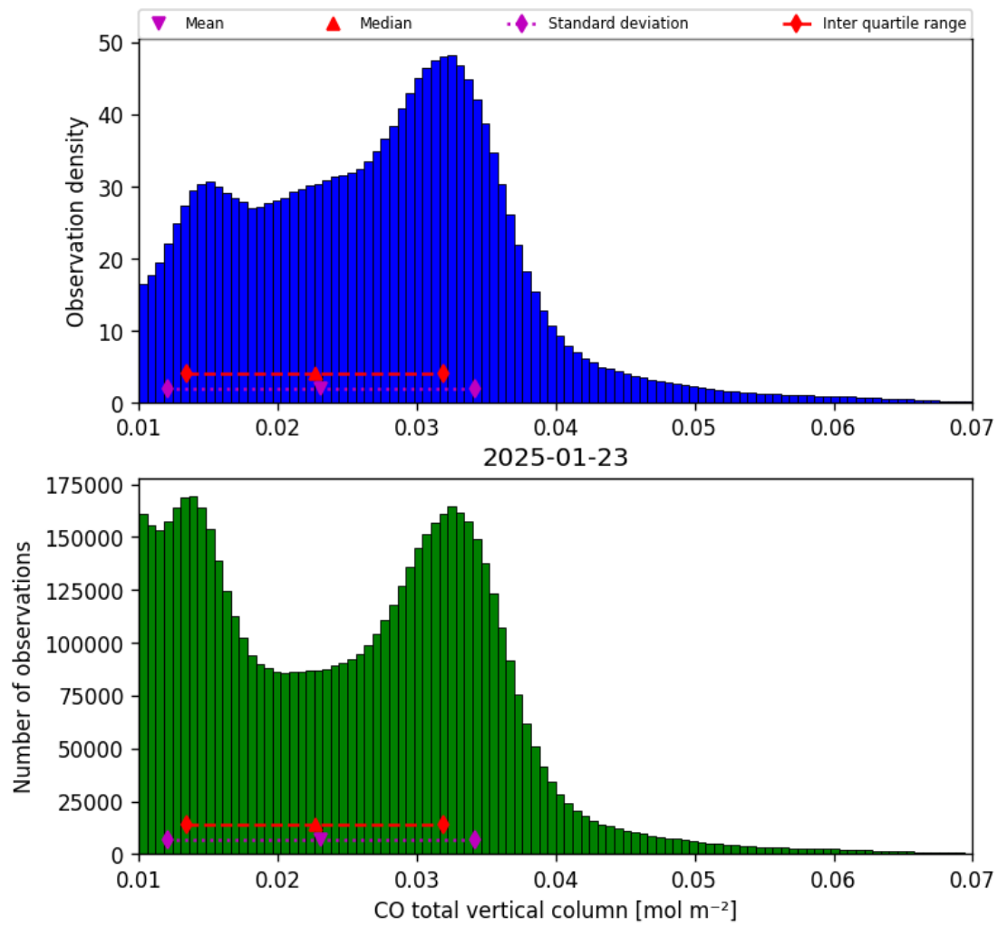
Figure 14: Histogram of “CO total vertical column” for 2025-01-23 to 2025-01-24
