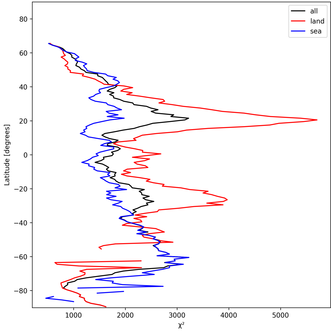
Figure 10: Zonal average of “ \chi^2 ” for 2025-01-23 to 2025-01-24.
