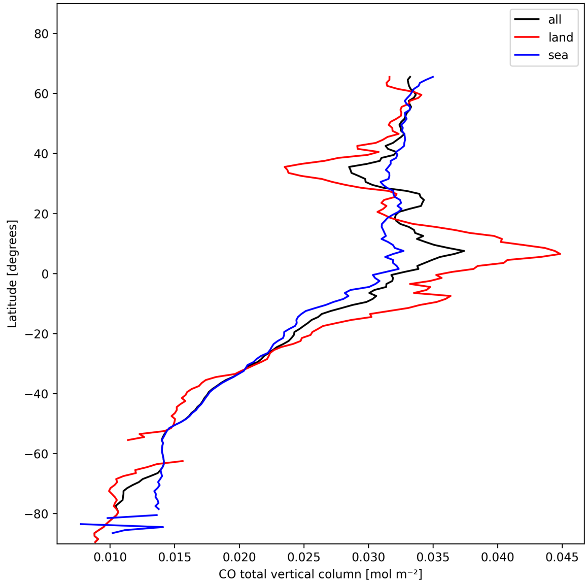
Figure 7: Zonal average of “CO total vertical column” for 2025-01-23 to 2025-01-24.
