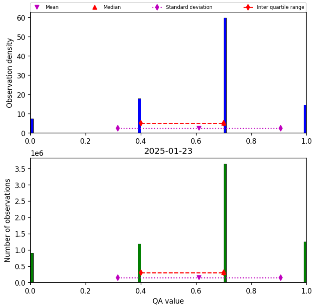
Figure 13: Histogram of “QA value” for 2025-01-23 to 2025-01-24
