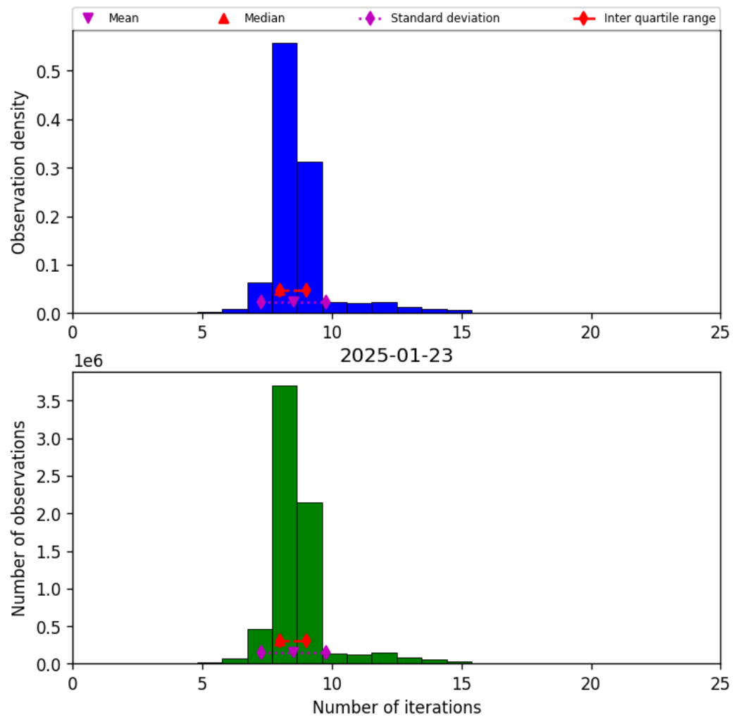
Figure 19: Histogram of “Number of iterations” for 2025-01-23 to 2025-01-24
