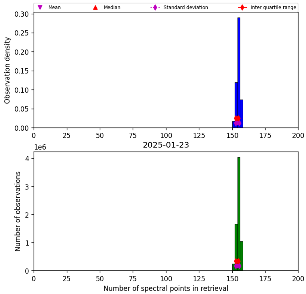
Figure 16: Histogram of “Number of spectral points in retrieval” for 2025-01-23 to 2025-01-24
