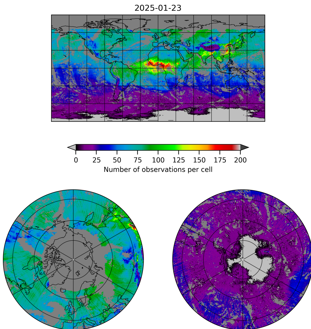
Figure 5: Map of the number of observations for 2025-01-23 to 2025-01-24
