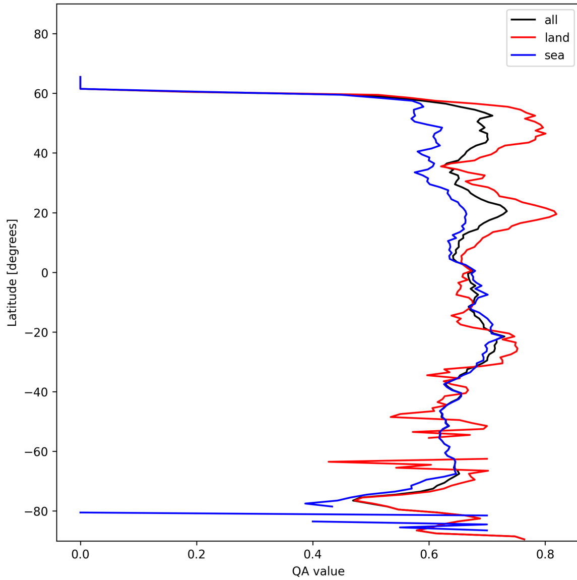
Figure 6: Zonal average of “QA value” for 2025-01-23 to 2025-01-24.
