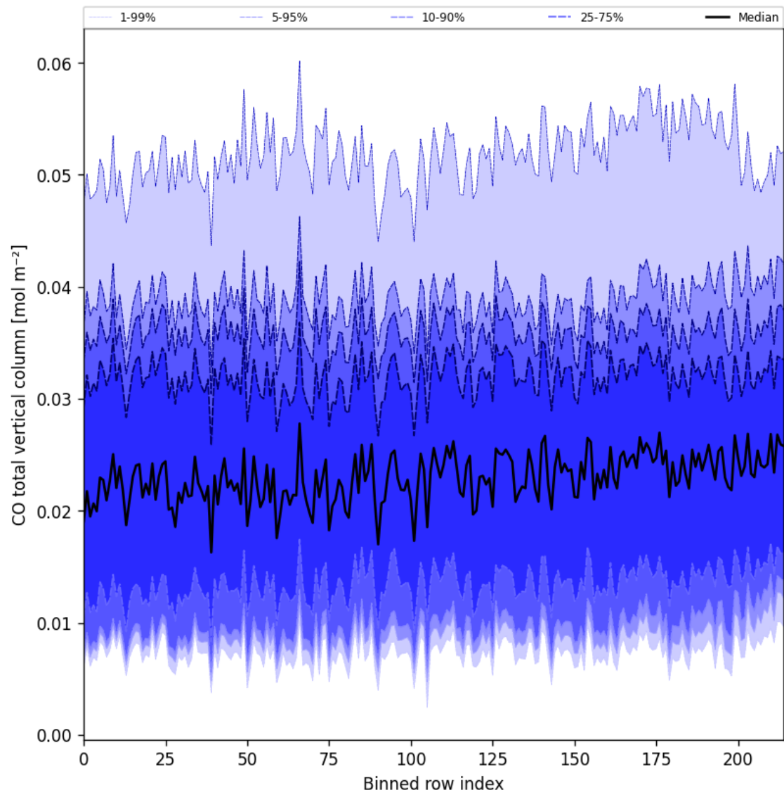
Figure 21: Along track statistics of “CO total vertical column” for 2025-01-23 to 2025-01-24
