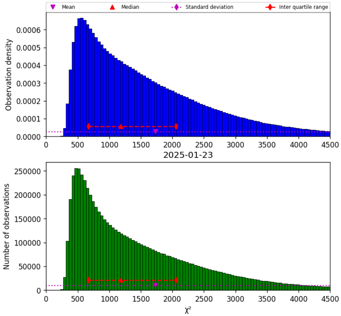
Figure 17: Histogram of “ \chi^2 ” for 2025-01-23 to 2025-01-24
