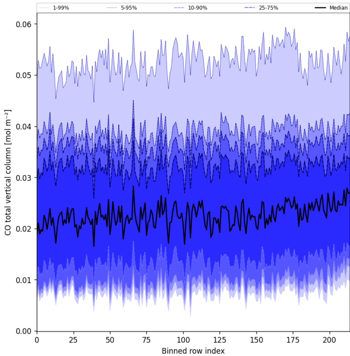
Figure 21: Along track statistics of “CO total vertical column” for 2025-01-24 to 2025-01-25
