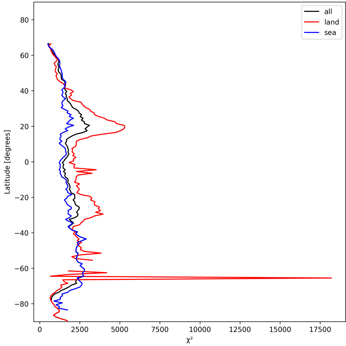
Figure 10: Zonal average of “ \chi^2 ” for 2025-01-24 to 2025-01-25.
