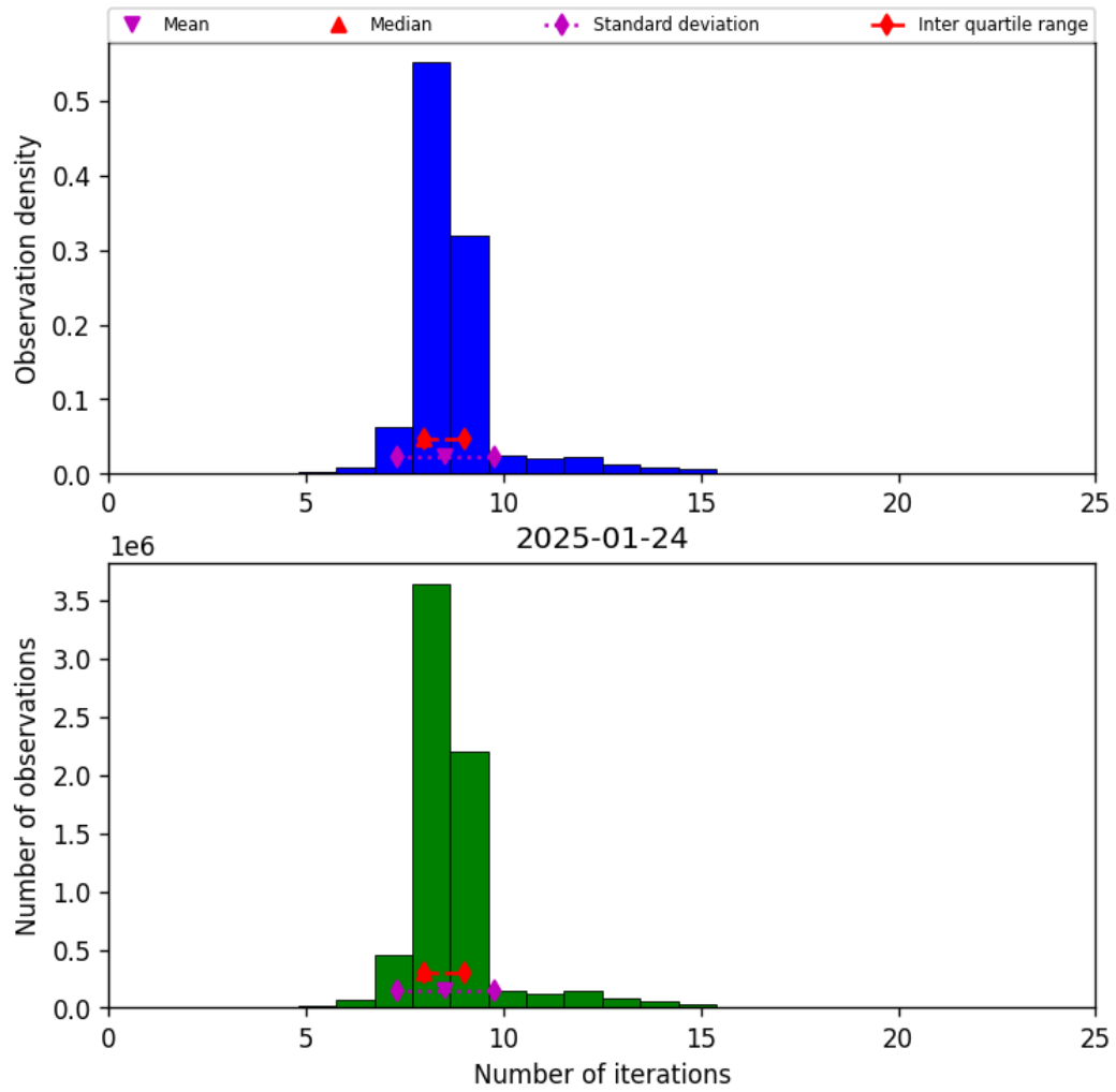
Figure 19: Histogram of “Number of iterations” for 2025-01-24 to 2025-01-25
