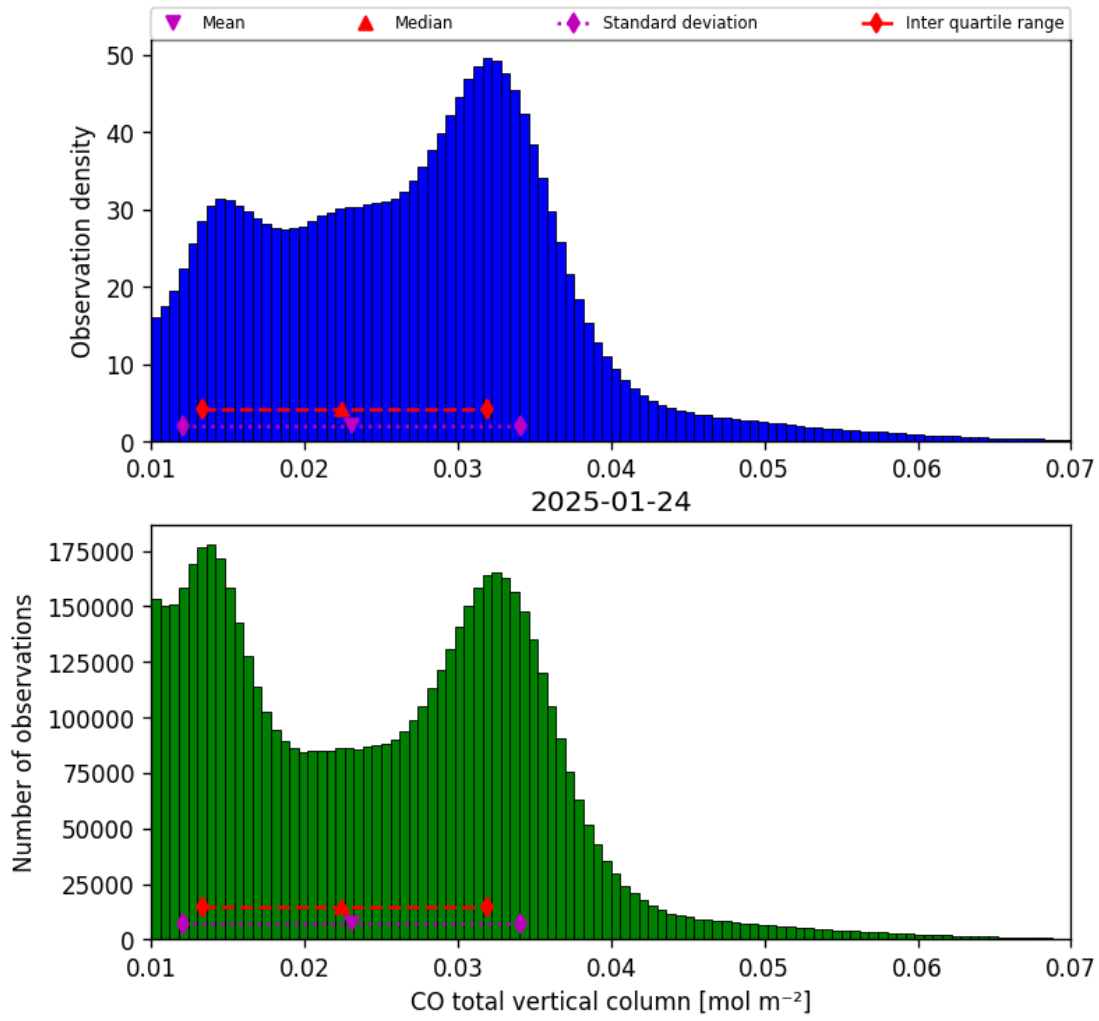
Figure 14: Histogram of “CO total vertical column” for 2025-01-24 to 2025-01-25
