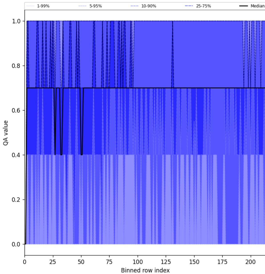
Figure 20: Along track statistics of “QA value” for 2025-01-24 to 2025-01-25
