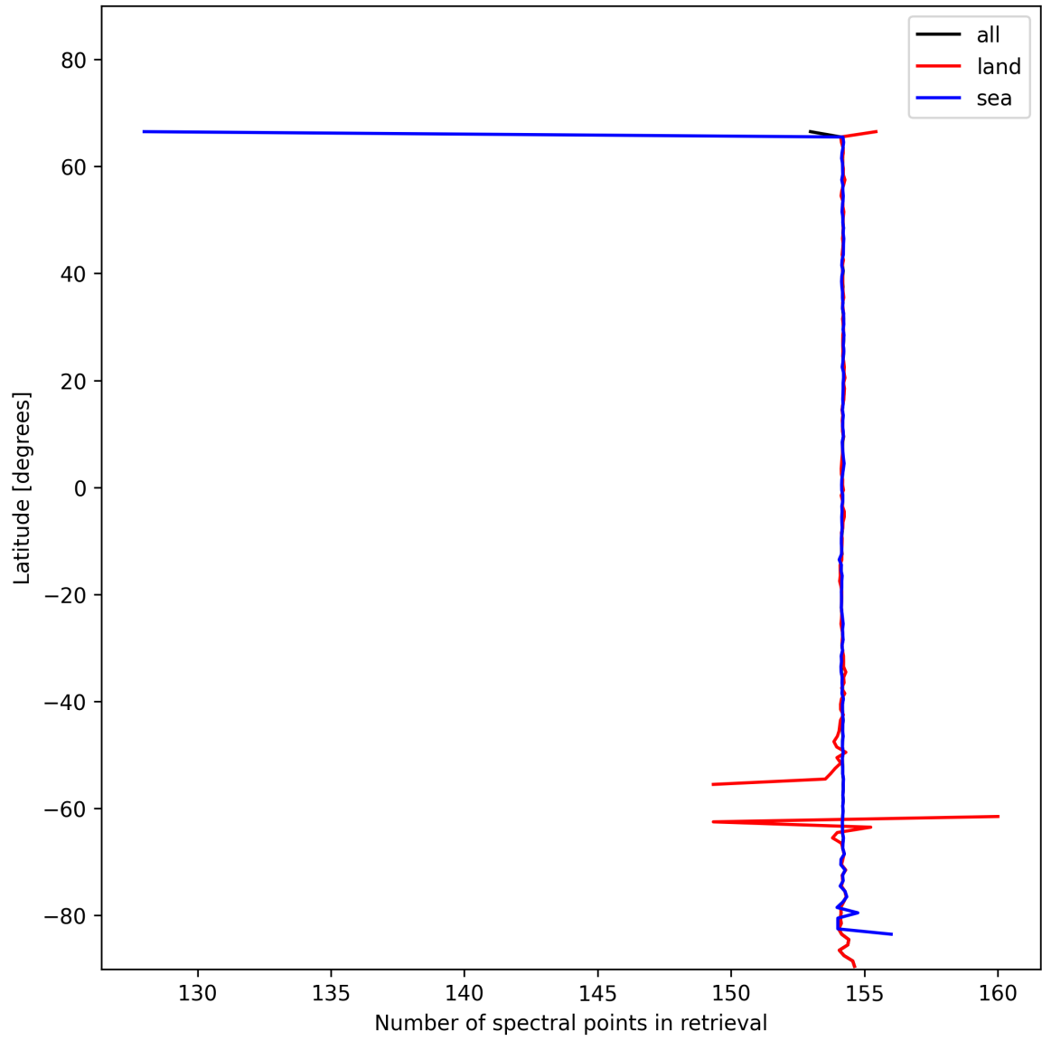
Figure 9: Zonal average of “Number of spectral points in retrieval” for 2025-01-24 to 2025-01-25.
