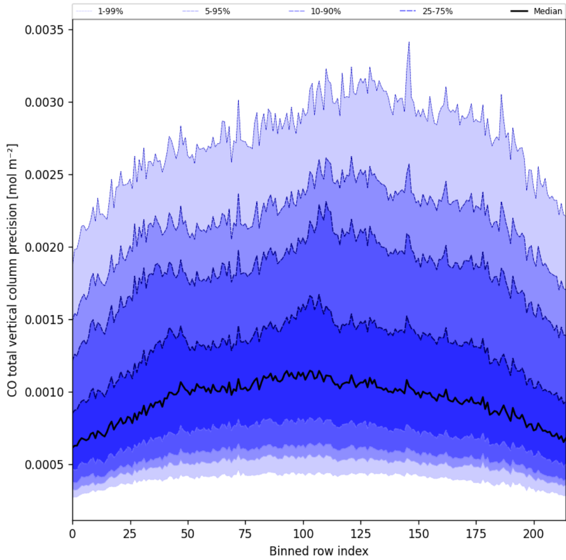
Figure 22: Along track statistics of “CO total vertical column precision” for 2025-01-24 to 2025-01-25
