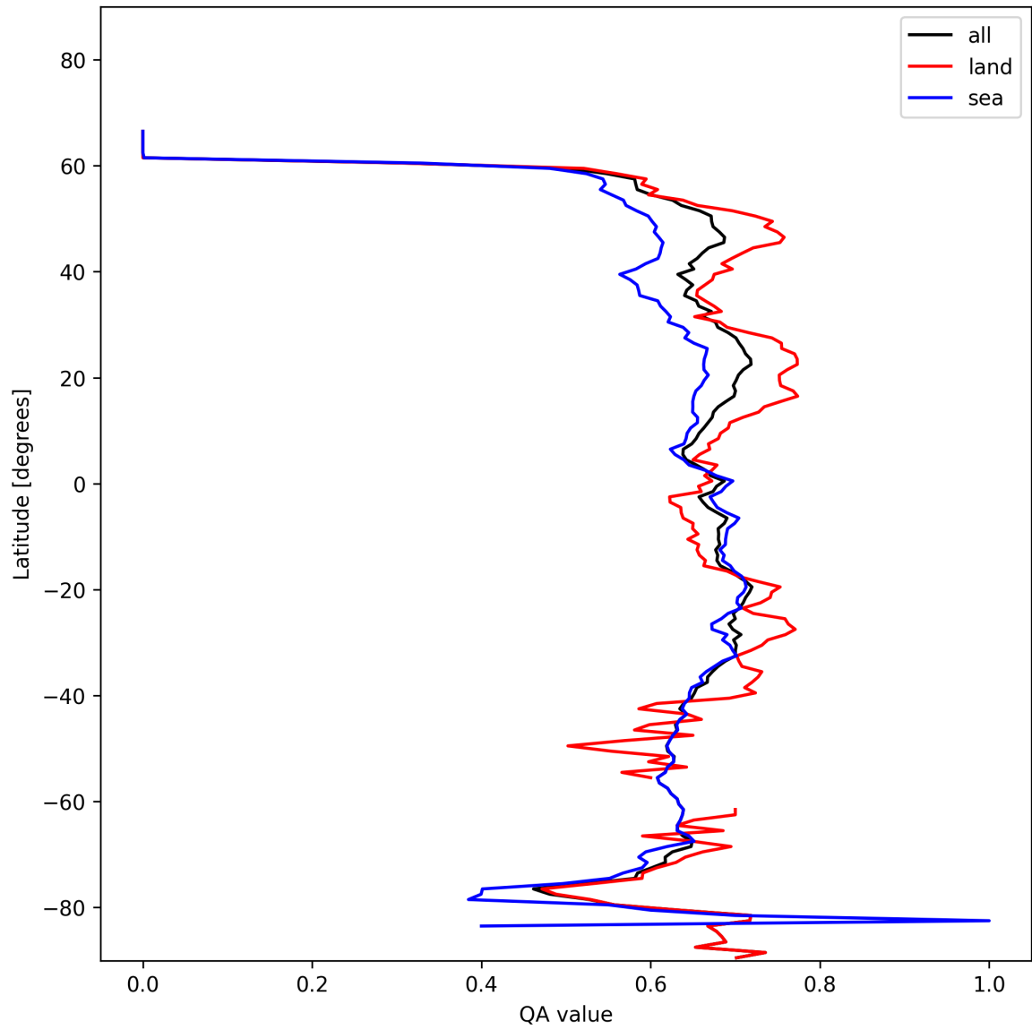
Figure 6: Zonal average of “QA value” for 2025-01-24 to 2025-01-25.
