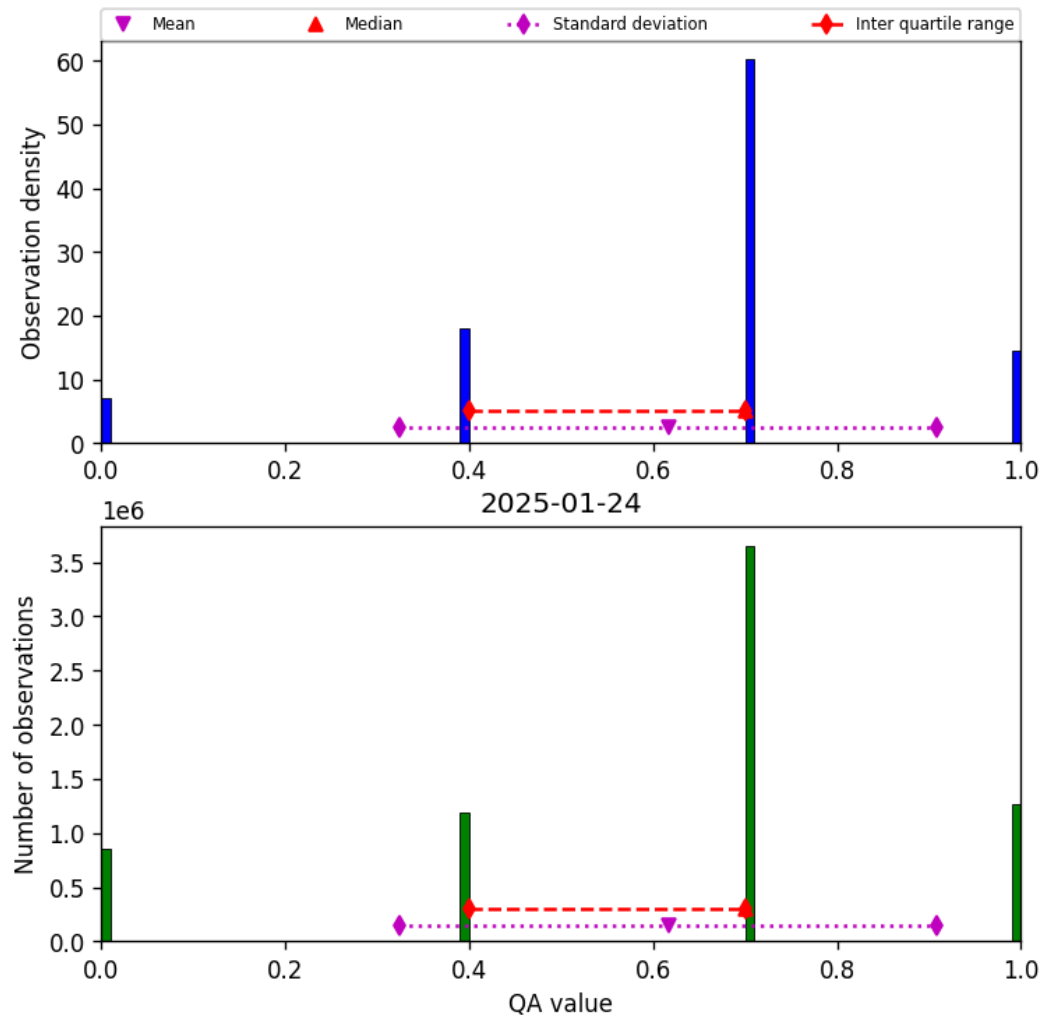
Figure 13: Histogram of “QA value” for 2025-01-24 to 2025-01-25
