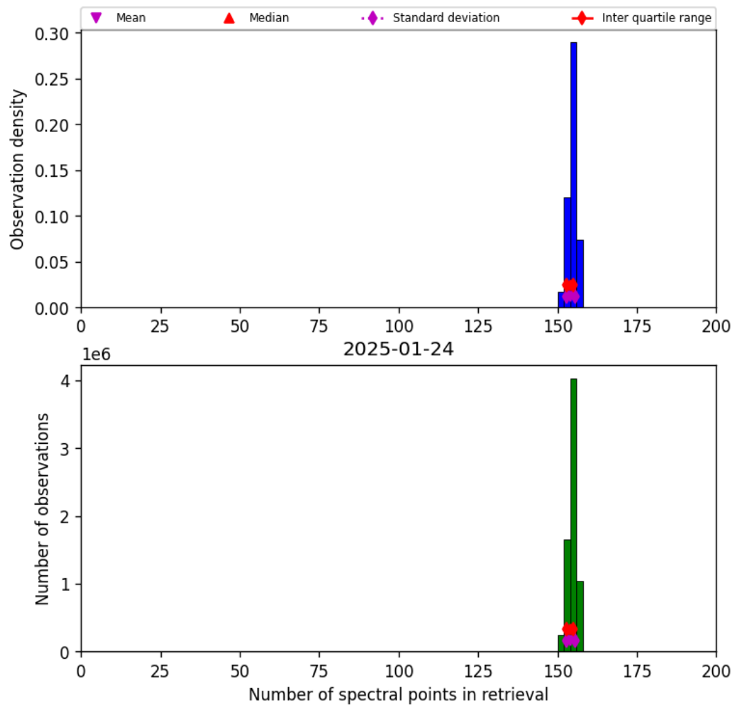
Figure 16: Histogram of “Number of spectral points in retrieval” for 2025-01-24 to 2025-01-25
