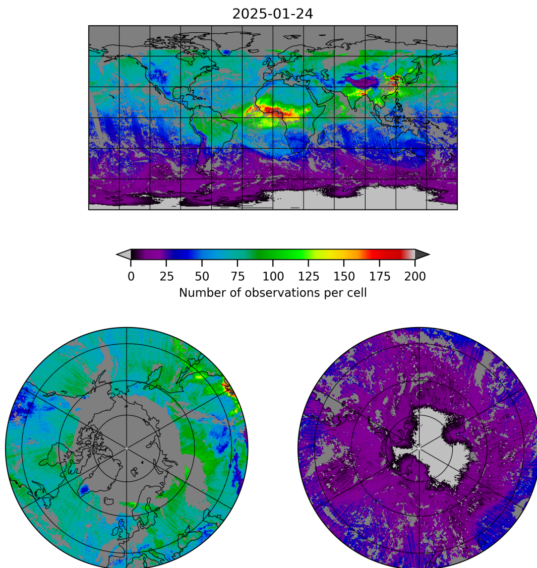
Figure 5: Map of the number of observations for 2025-01-24 to 2025-01-25
