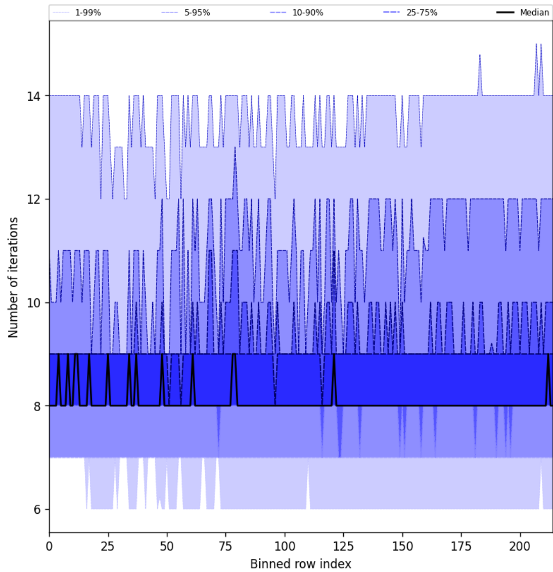
Figure 26: Along track statistics of “Number of iterations” for 2025-01-24 to 2025-01-25
