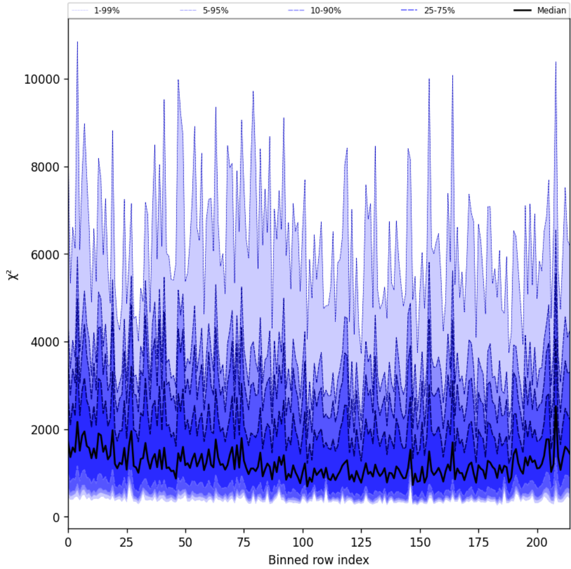
Figure 24: Along track statistics of “ \chi^2 ” for 2025-01-24 to 2025-01-25
