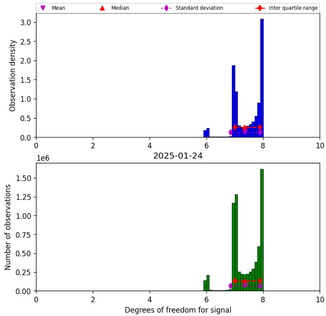
Figure 18: Histogram of “Degrees of freedom for signal” for 2025-01-24 to 2025-01-25
