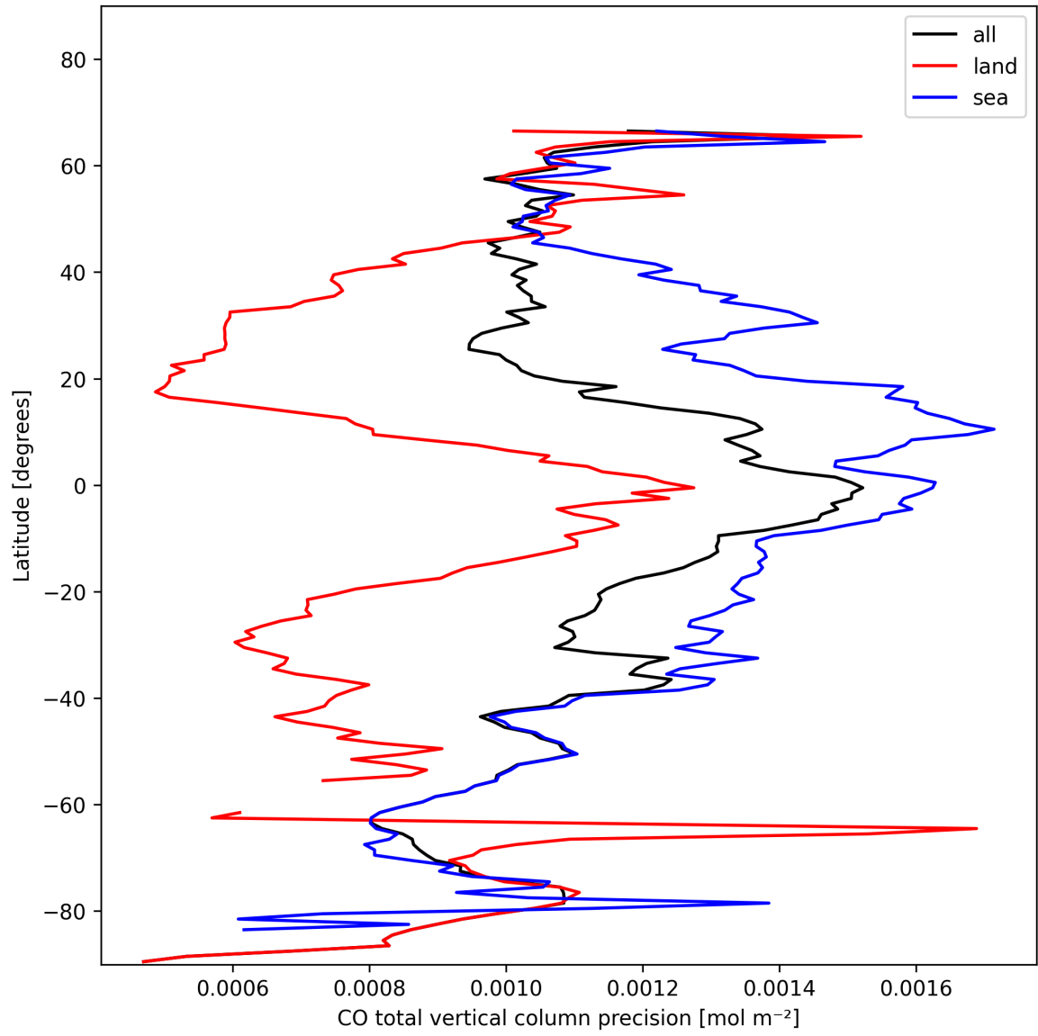
Figure 8: Zonal average of "CO total vertical column precision" for 2025-01-24 to 2025-01-25.
