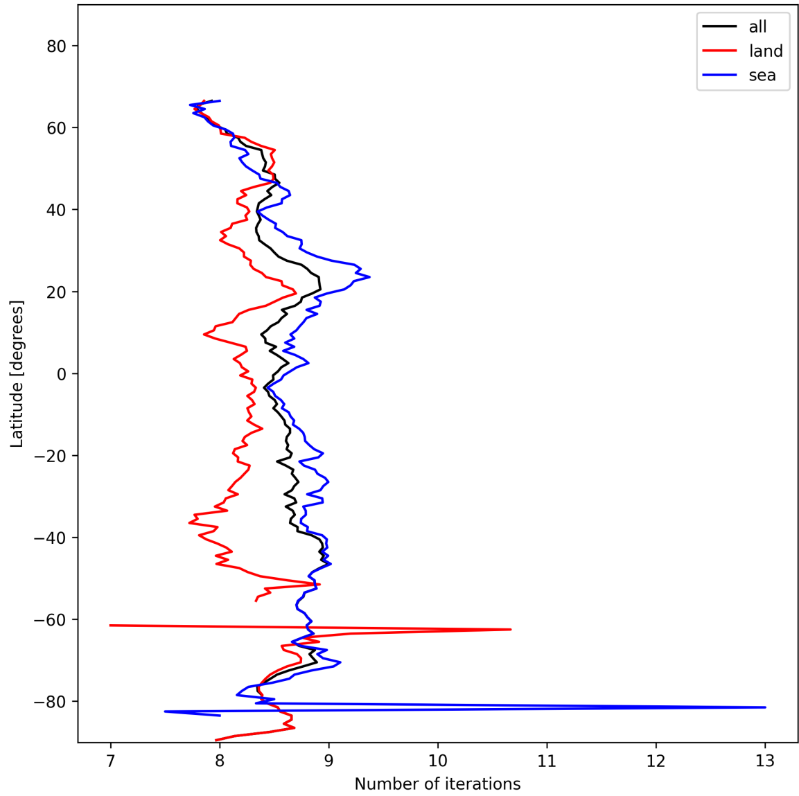
Figure 12: Zonal average of “Number of iterations” for 2025-01-24 to 2025-01-25.
