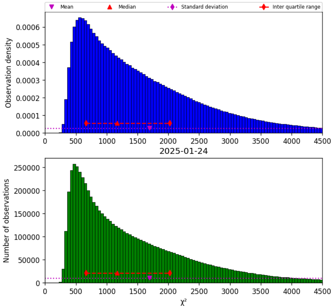
Figure 17: Histogram of “ \chi^2 ” for 2025-01-24 to 2025-01-25
