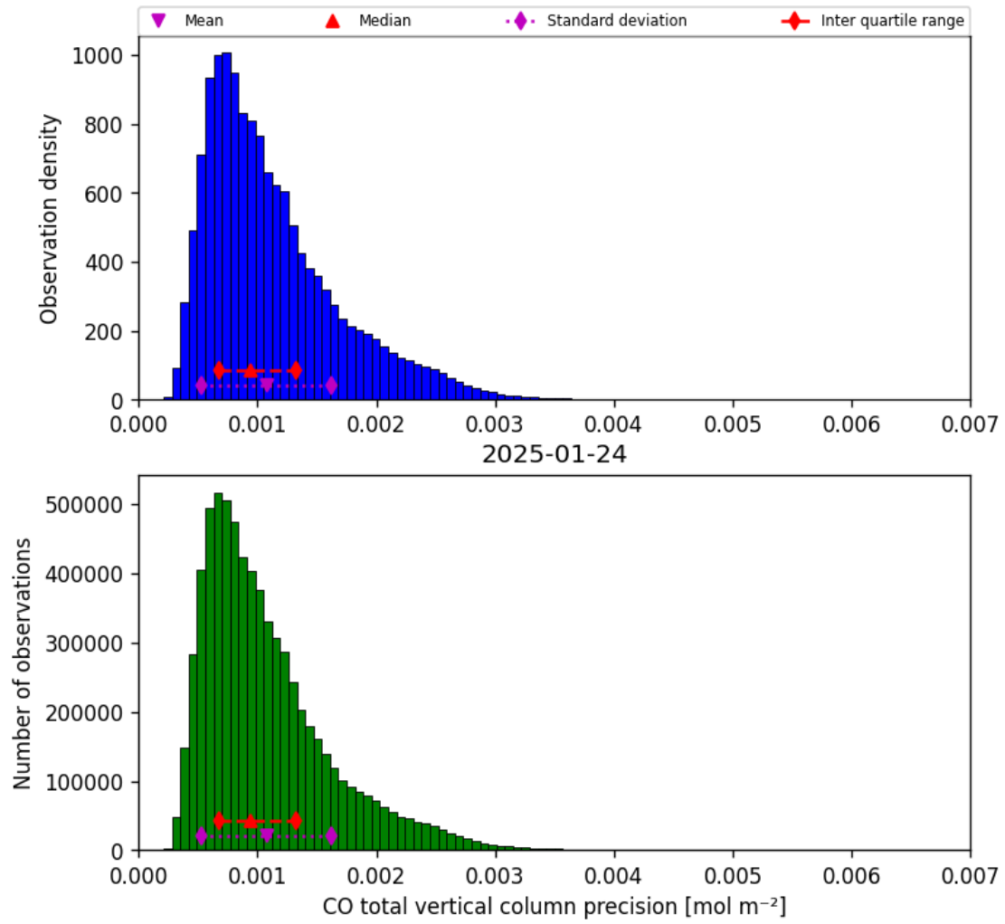
Figure 15: Histogram of “CO total vertical column precision” for 2025-01-24 to 2025-01-25
