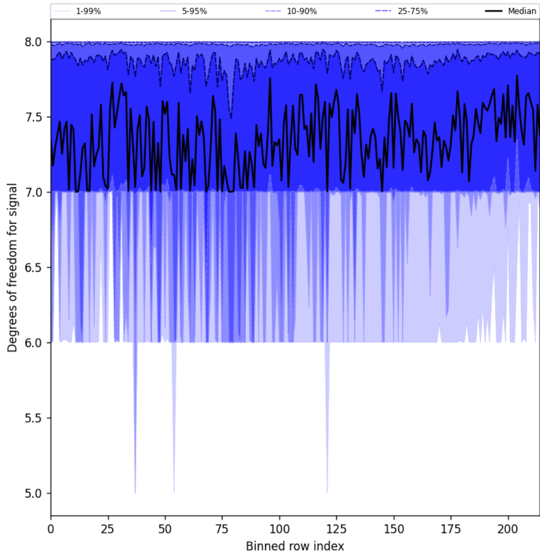
Figure 25: Along track statistics of “Degrees of freedom for signal” for 2025-01-24 to 2025-01-25
