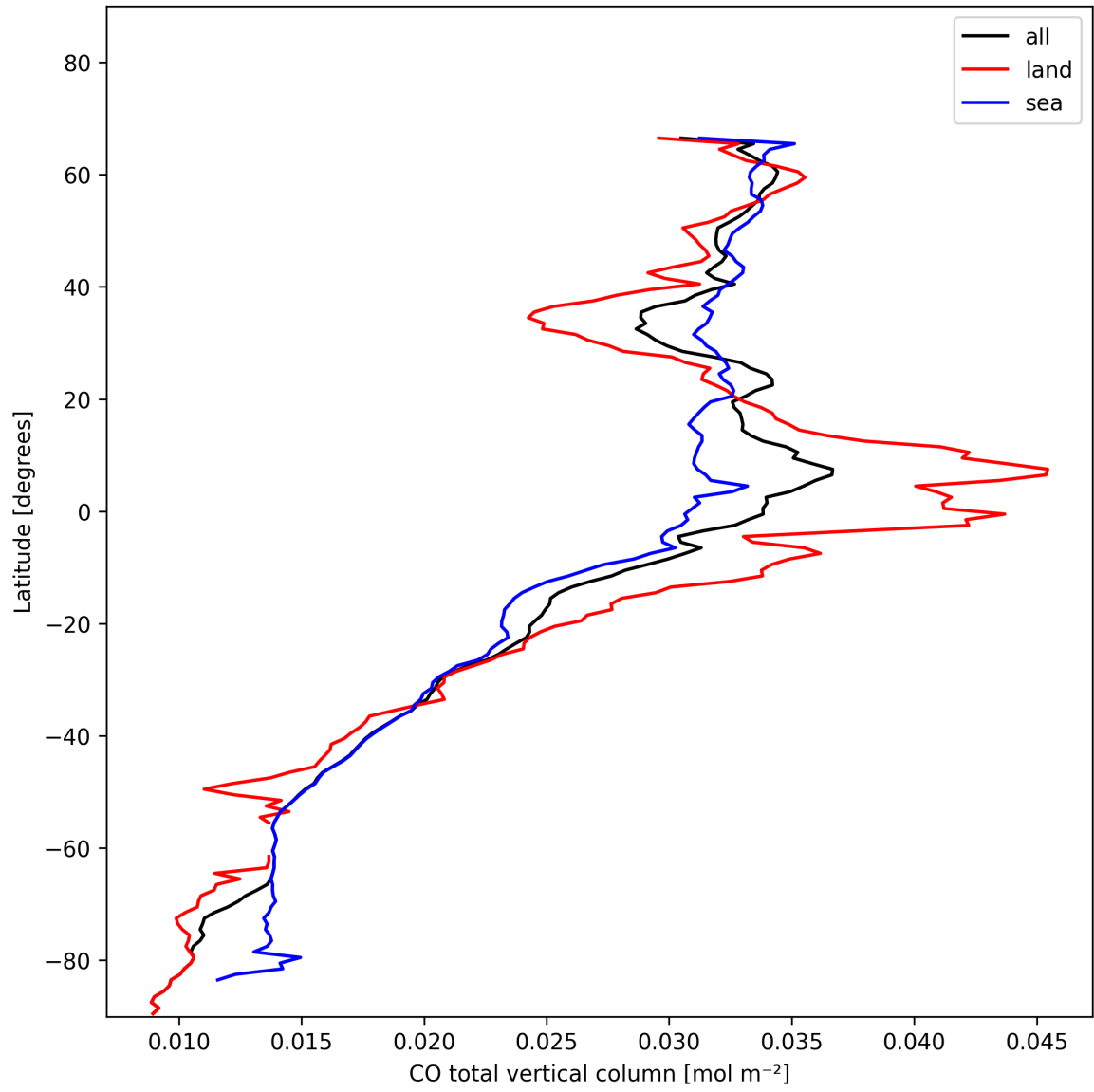
Figure 7: Zonal average of “CO total vertical column” for 2025-01-24 to 2025-01-25.
