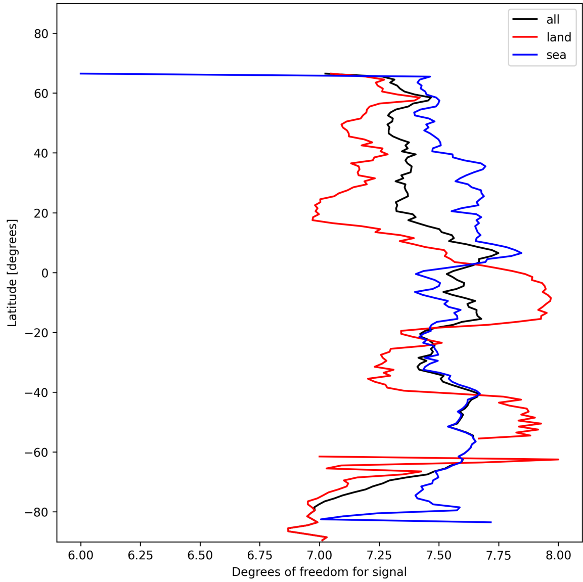
Figure 11: Zonal average of “Degrees of freedom for signal” for 2025-01-24 to 2025-01-25.
