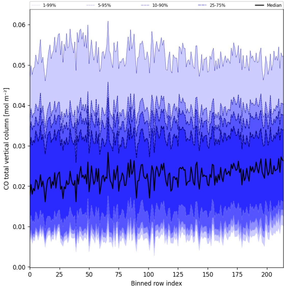
Figure 21: Along track statistics of “CO total vertical column” for 2025-01-25 to 2025-01-26
