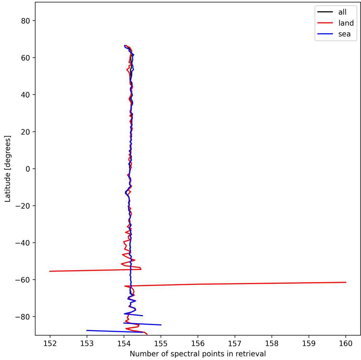
Figure 9: Zonal average of “Number of spectral points in retrieval” for 2025-01-25 to 2025-01-26.
