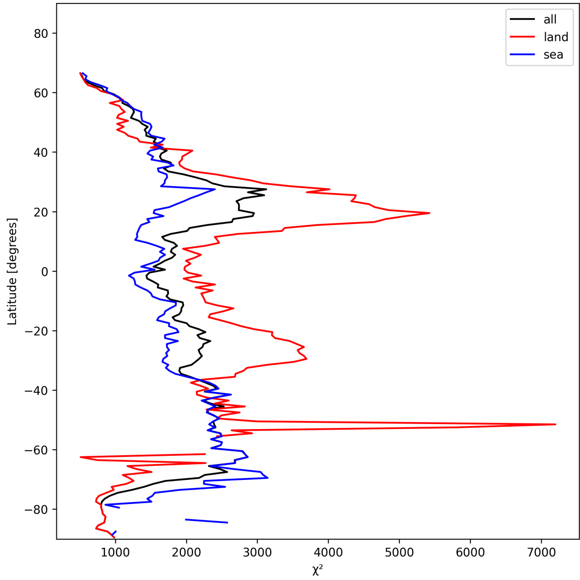
Figure 10: Zonal average of “ \chi^2 ” for 2025-01-25 to 2025-01-26.
