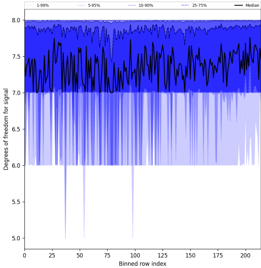
Figure 25: Along track statistics of “Degrees of freedom for signal” for 2025-01-25 to 2025-01-26
