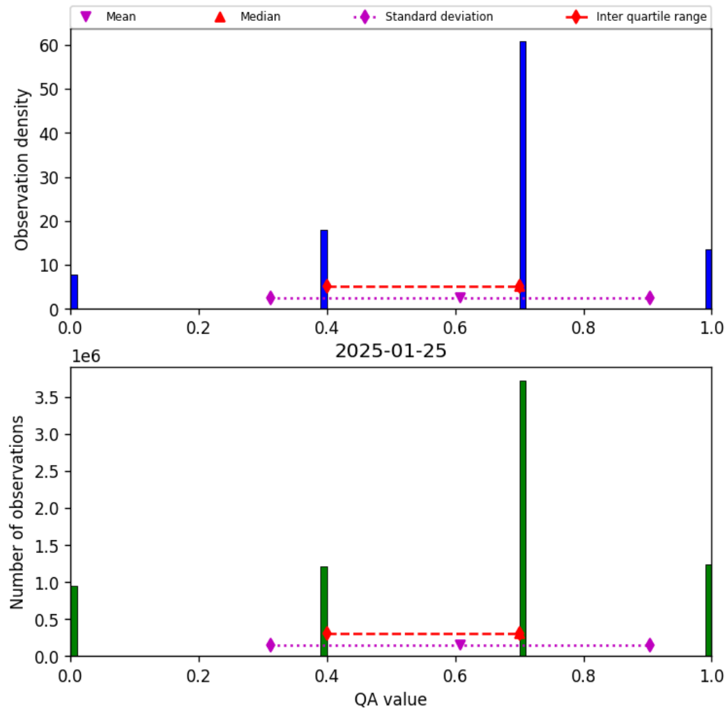
Figure 13: Histogram of “QA value” for 2025-01-25 to 2025-01-26
