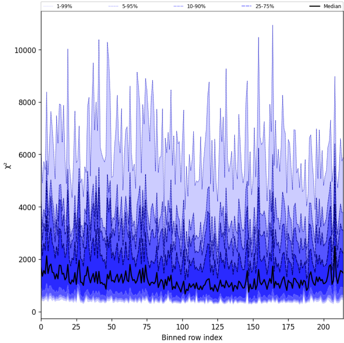
Figure 24: Along track statistics of “ \chi^2 ” for 2025-01-25 to 2025-01-26
