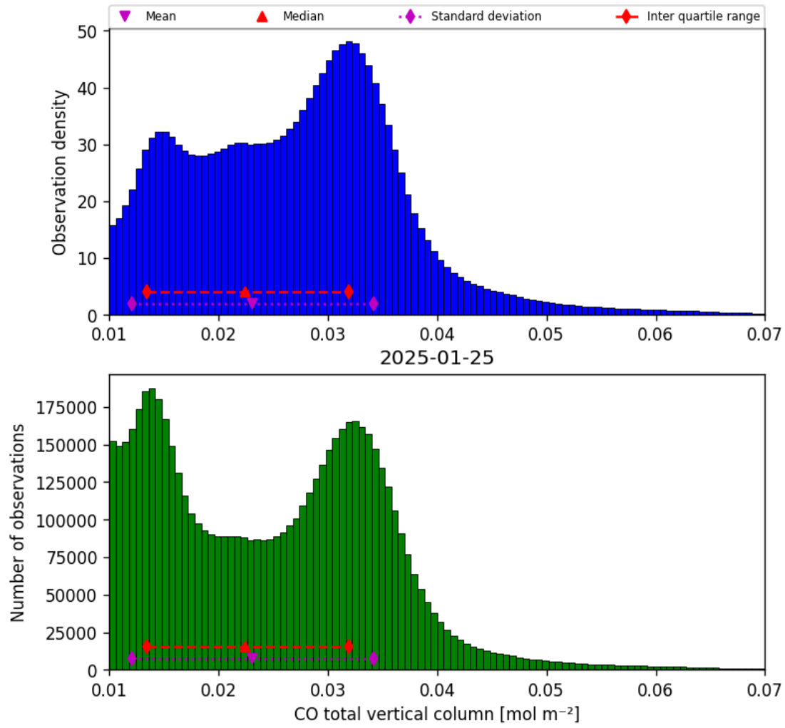
Figure 14: Histogram of “CO total vertical column” for 2025-01-25 to 2025-01-26
