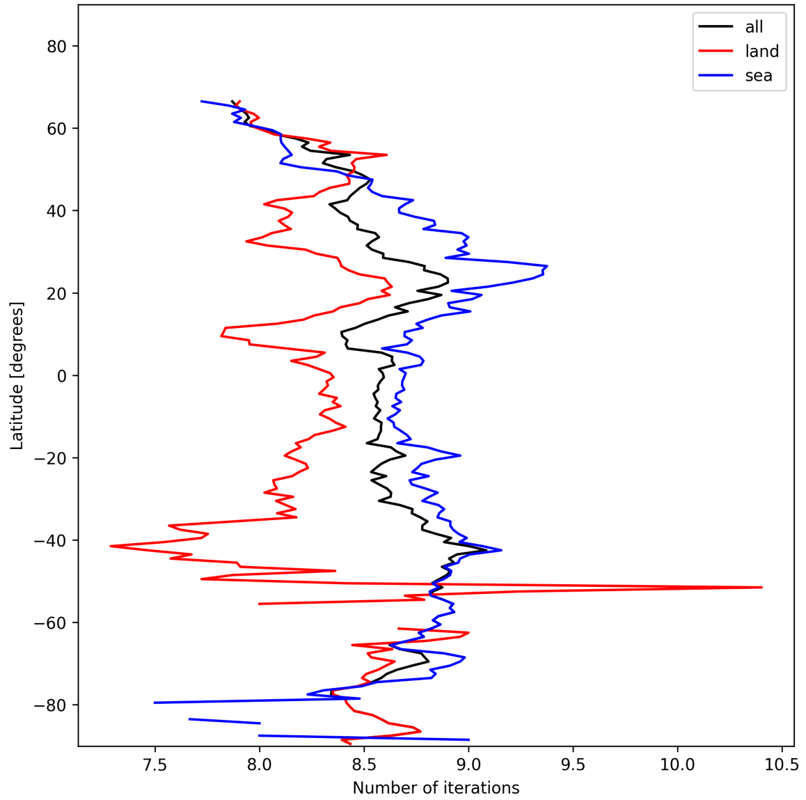
Figure 12: Zonal average of “Number of iterations” for 2025-01-25 to 2025-01-26.
