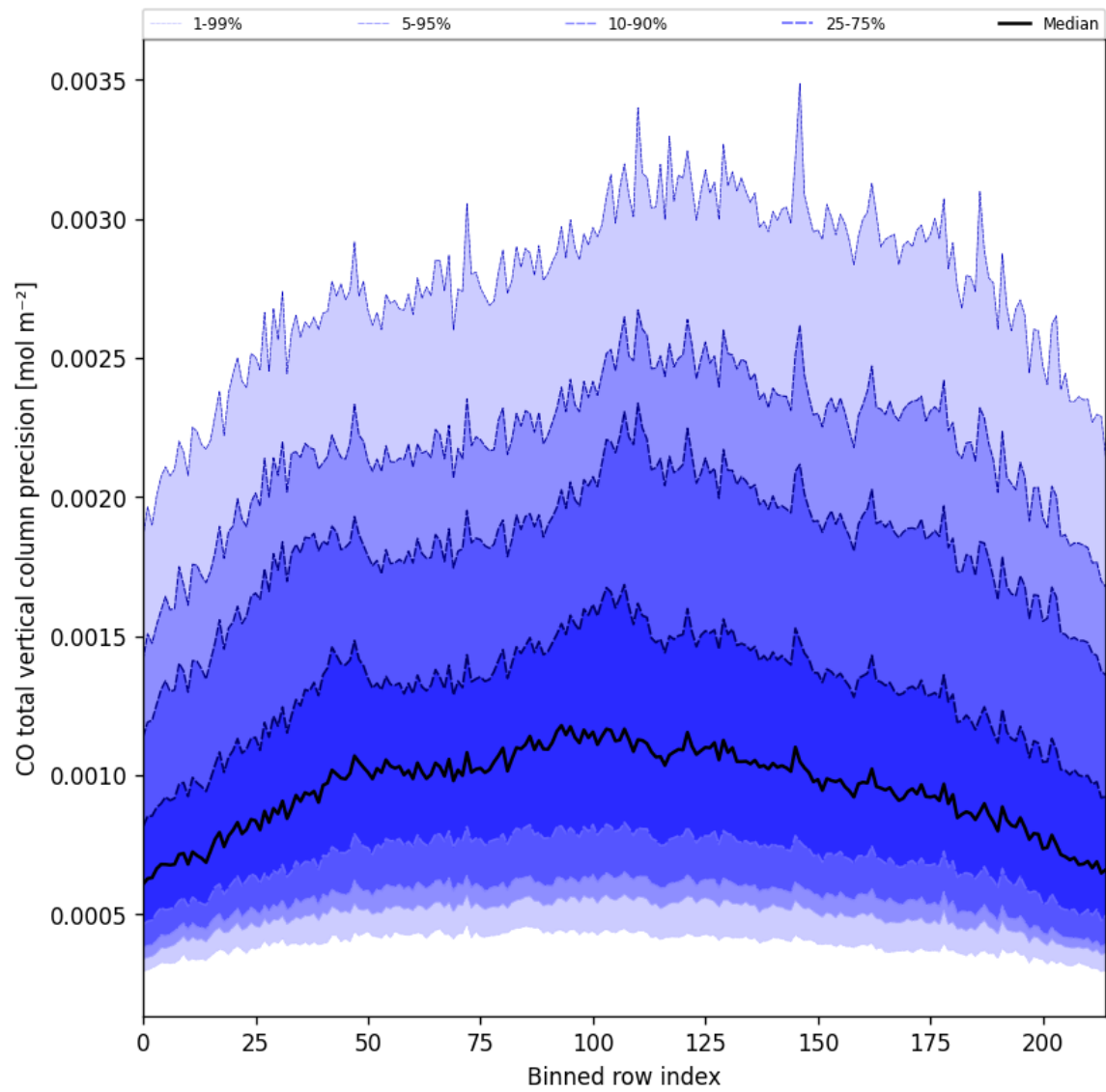
Figure 22: Along track statistics of “CO total vertical column precision” for 2025-01-25 to 2025-01-26
