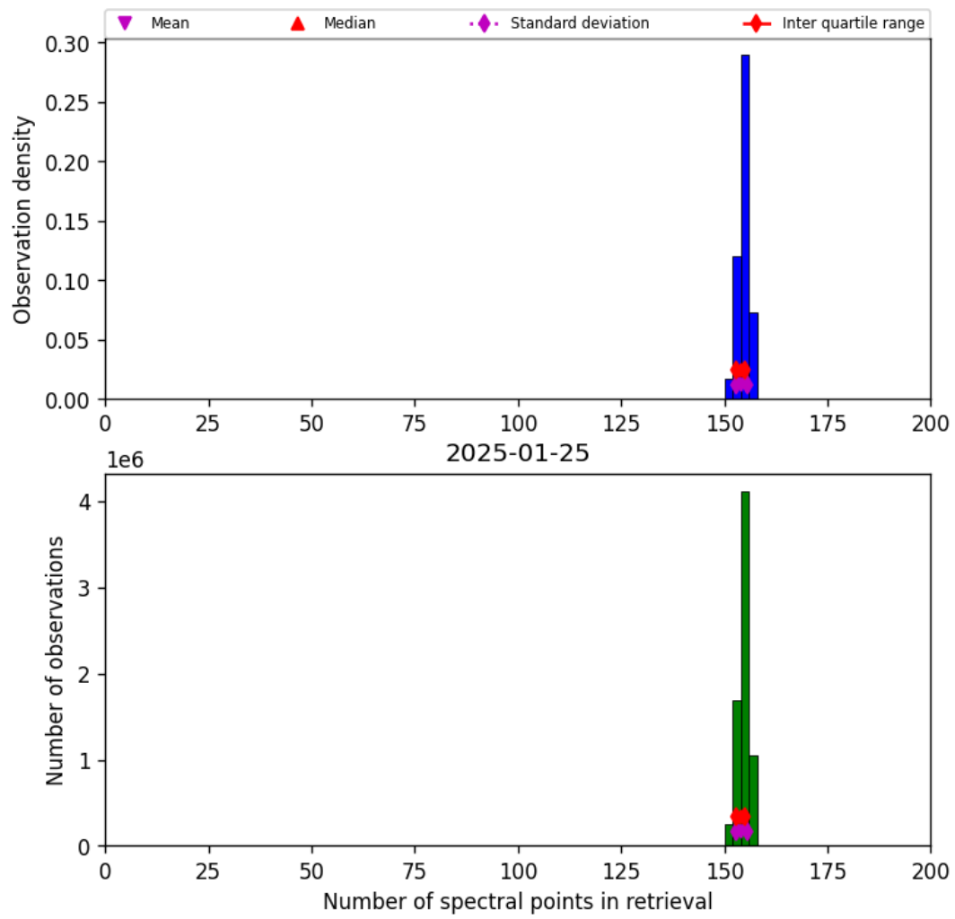
Figure 16: Histogram of “Number of spectral points in retrieval” for 2025-01-25 to 2025-01-26
