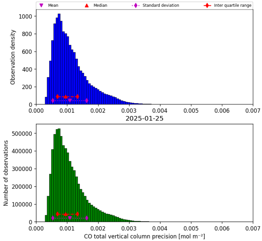
Figure 15: Histogram of “CO total vertical column precision” for 2025-01-25 to 2025-01-26
