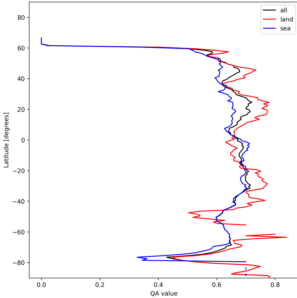
Figure 6: Zonal average of “QA value” for 2025-01-25 to 2025-01-26.
