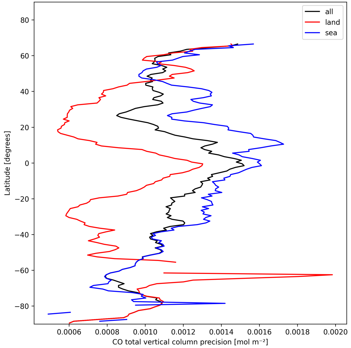
Figure 8: Zonal average of “CO total vertical column precision” for 2025-01-25 to 2025-01-26.
