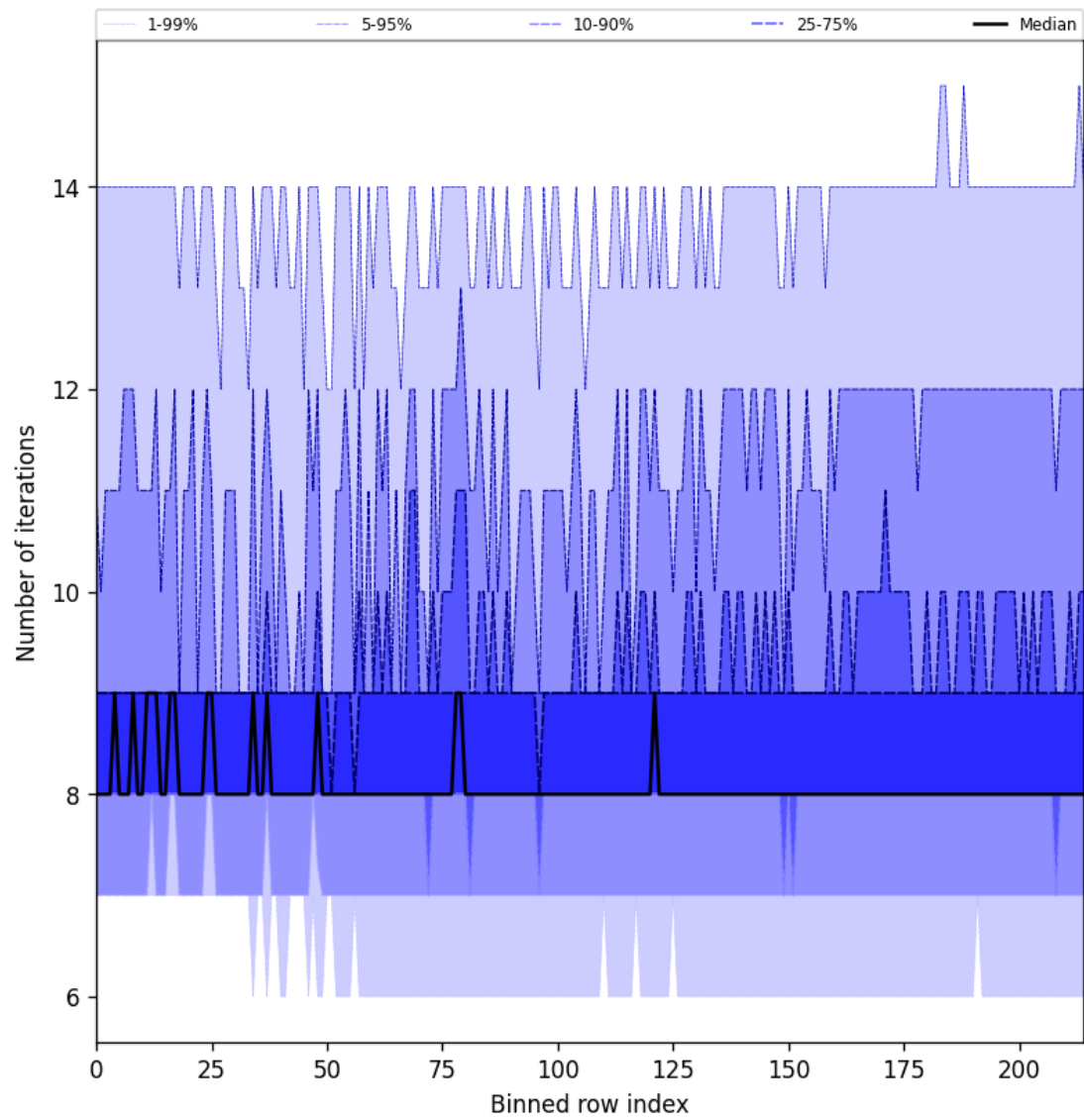
Figure 26: Along track statistics of “Number of iterations” for 2025-01-25 to 2025-01-26
