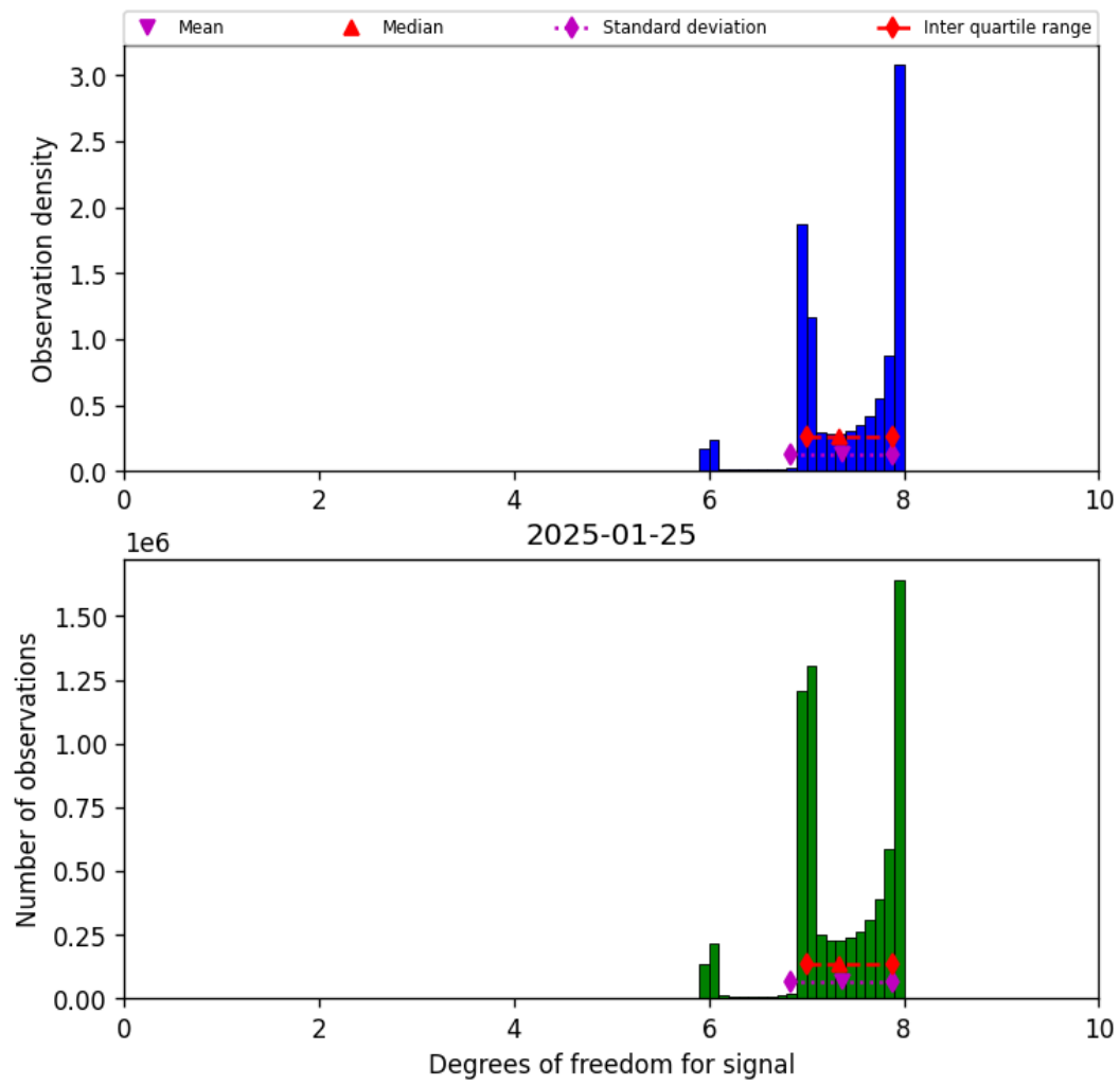
Figure 18: Histogram of “Degrees of freedom for signal” for 2025-01-25 to 2025-01-26
