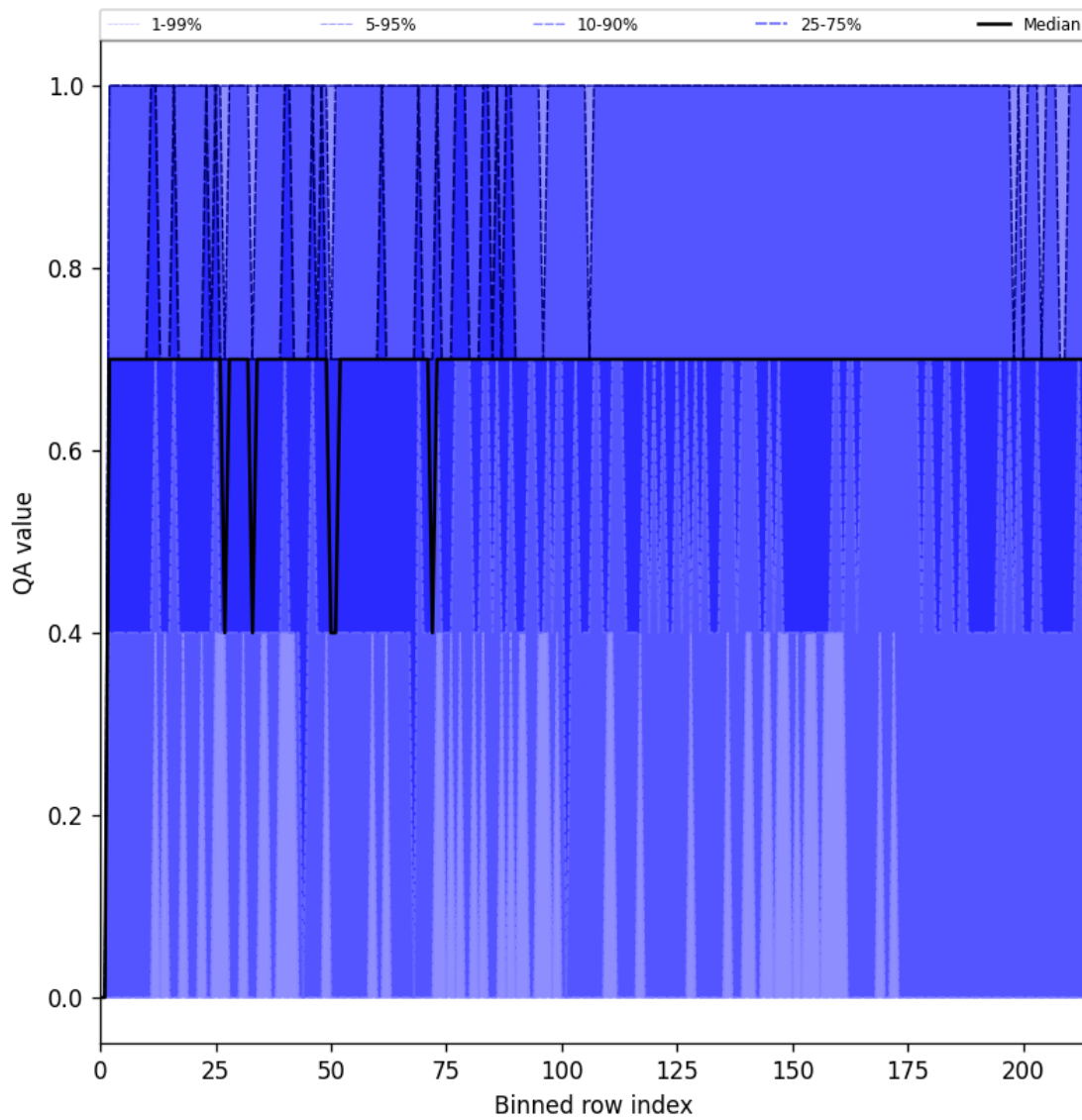
Figure 20: Along track statistics of “QA value” for 2025-01-25 to 2025-01-26
