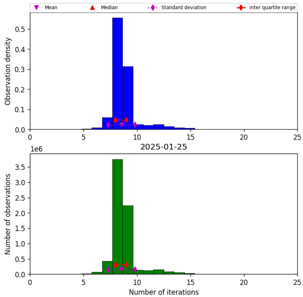
Figure 19: Histogram of “Number of iterations” for 2025-01-25 to 2025-01-26
