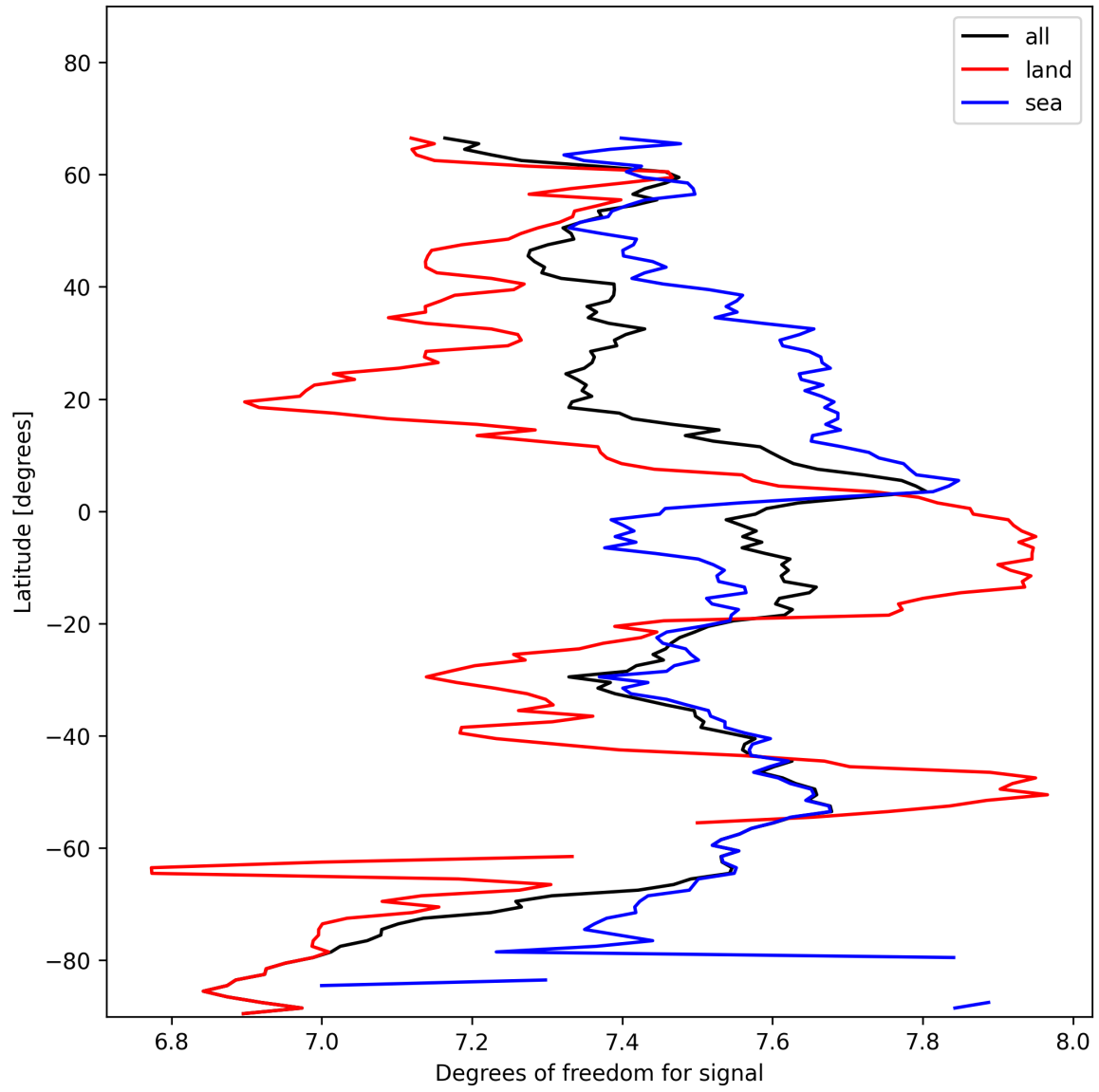
Figure 11: Zonal average of “Degrees of freedom for signal” for 2025-01-25 to 2025-01-26.
