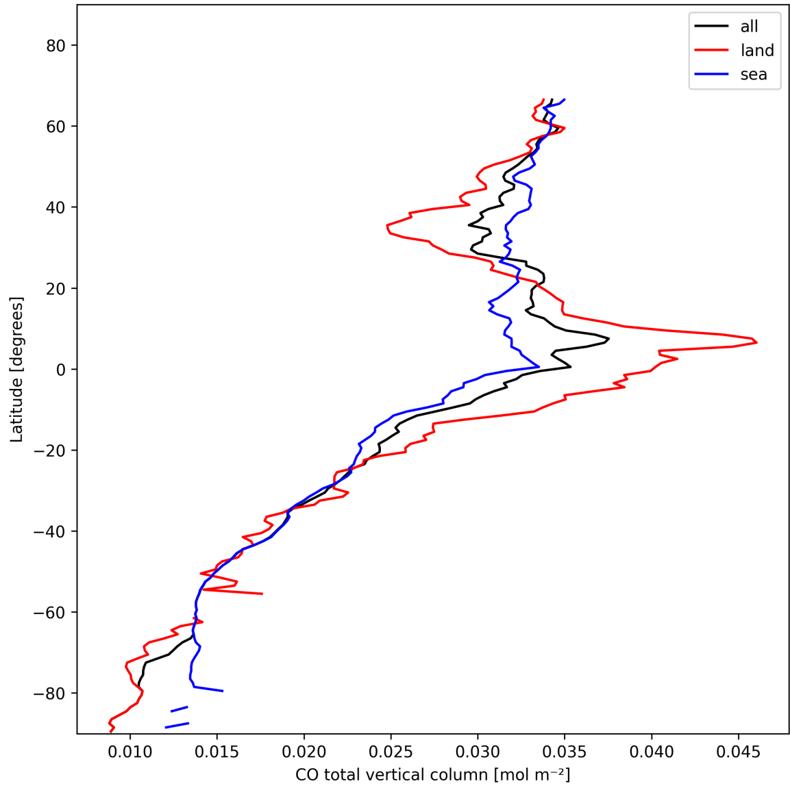
Figure 7: Zonal average of “CO total vertical column” for 2025-01-25 to 2025-01-26.
