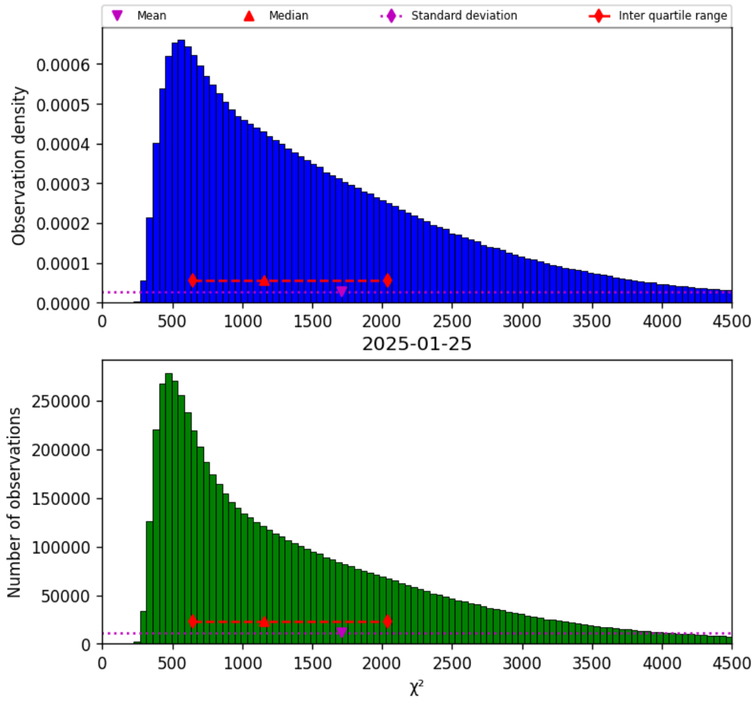
Figure 17: Histogram of “ \chi^2 ” for 2025-01-25 to 2025-01-26
