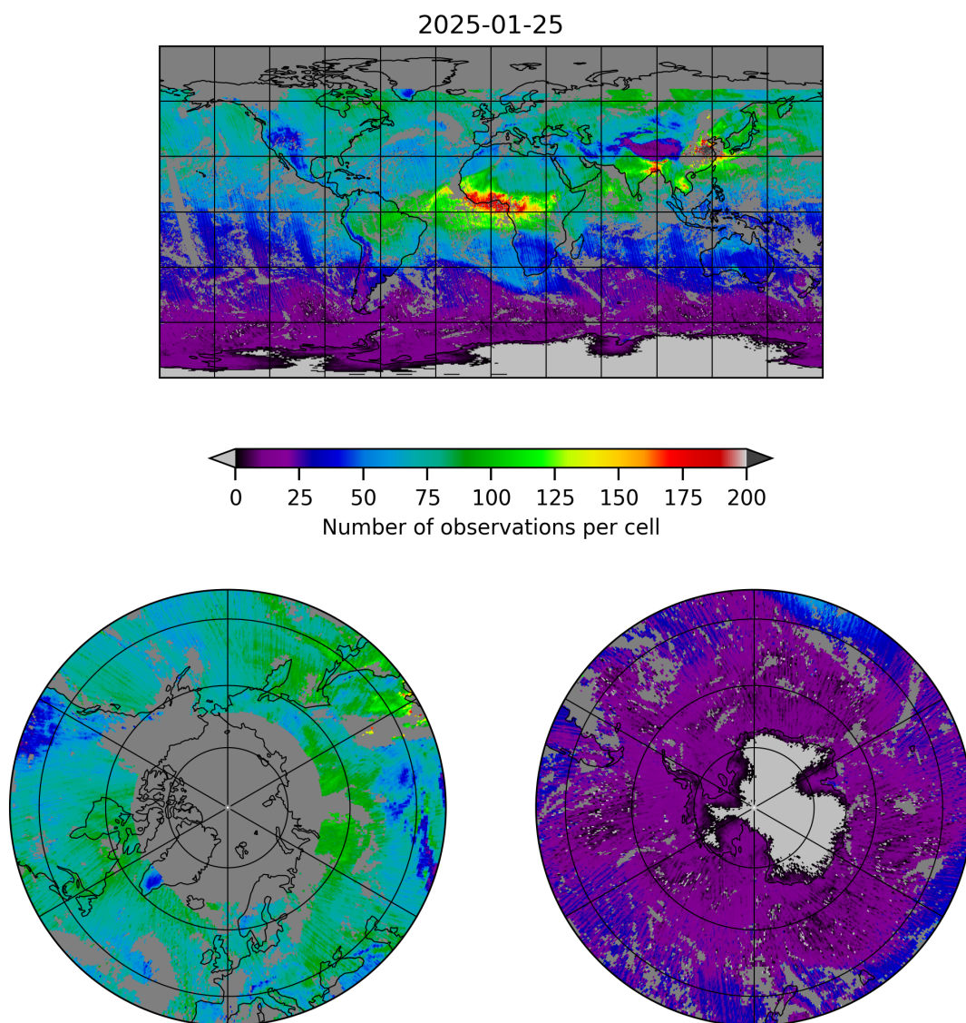
Figure 5: Map of the number of observations for 2025-01-25 to 2025-01-26
