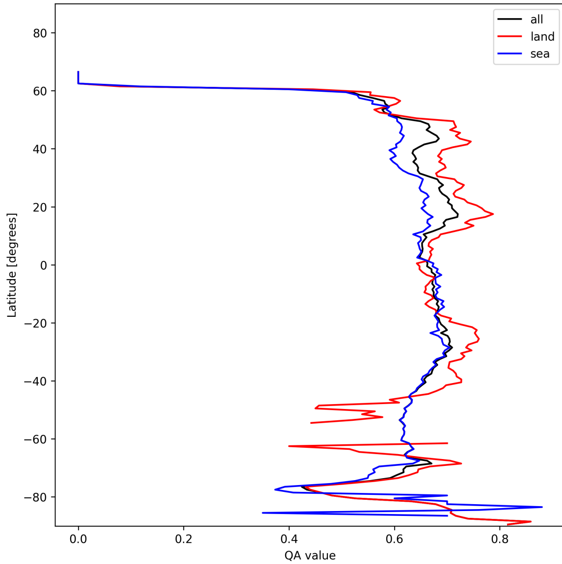
Figure 6: Zonal average of “QA value” for 2025-01-26 to 2025-01-26.
