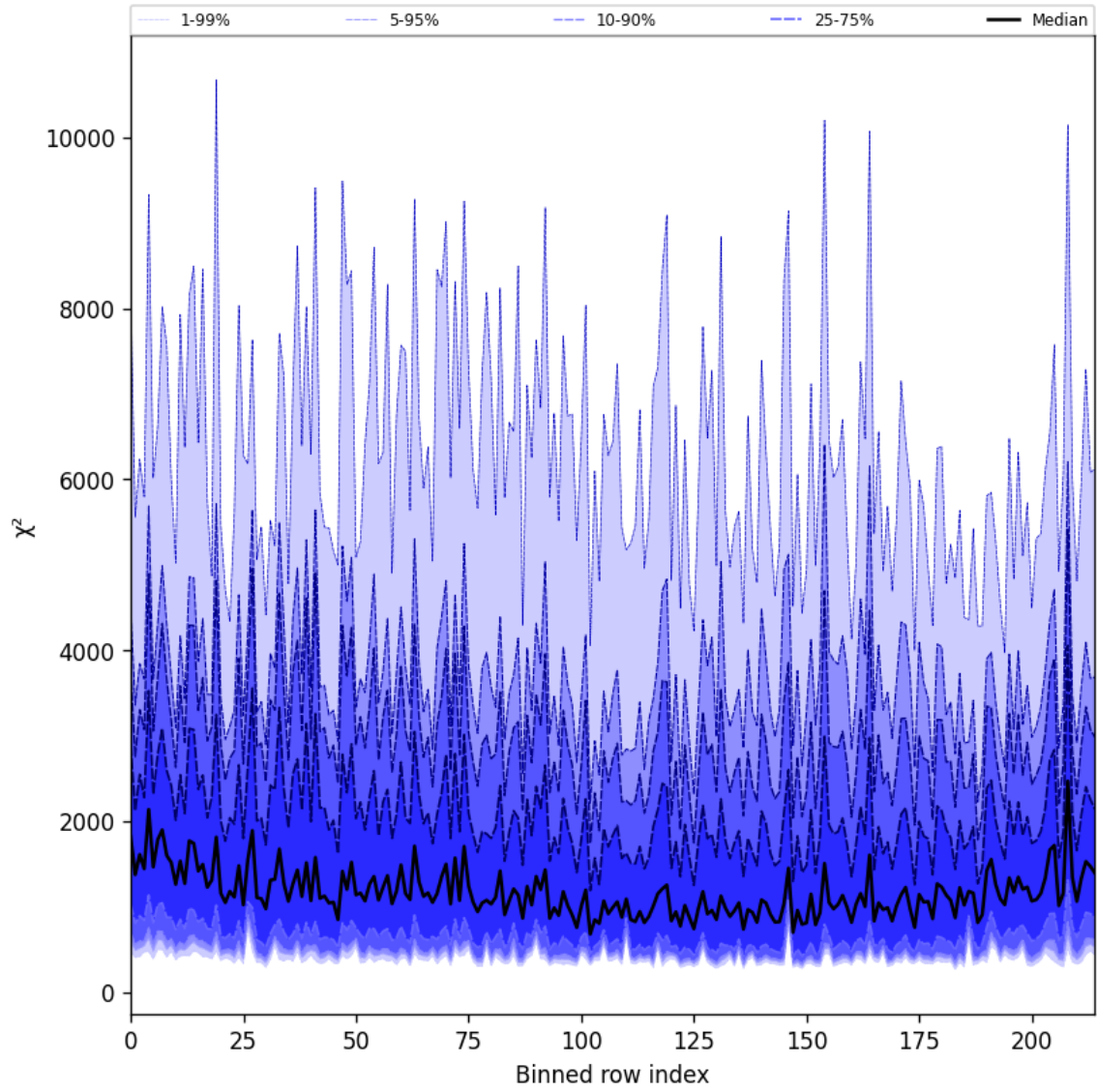
Figure 24: Along track statistics of “ \chi^2 ” for 2025-01-26 to 2025-01-26
