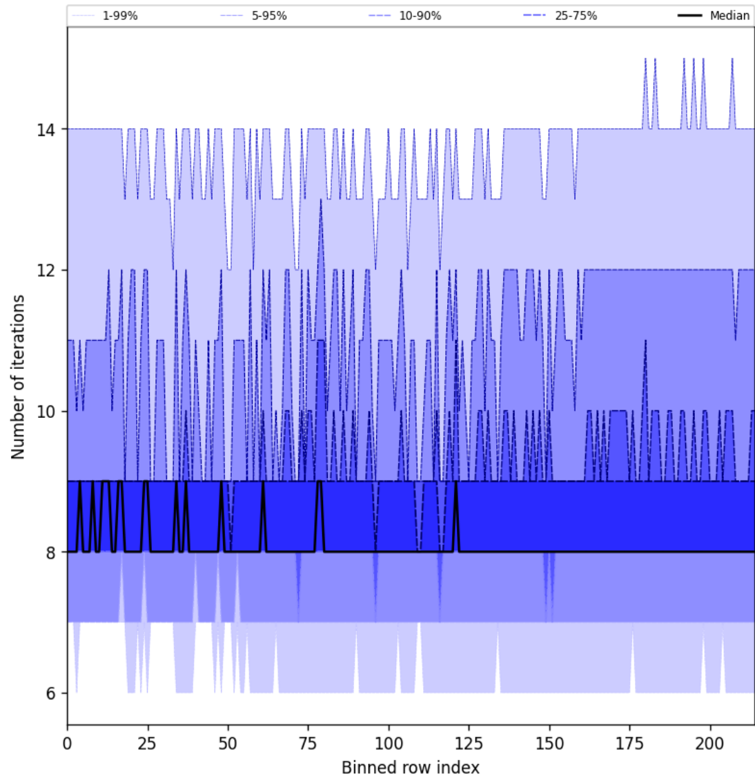
Figure 26: Along track statistics of “Number of iterations” for 2025-01-26 to 2025-01-26
