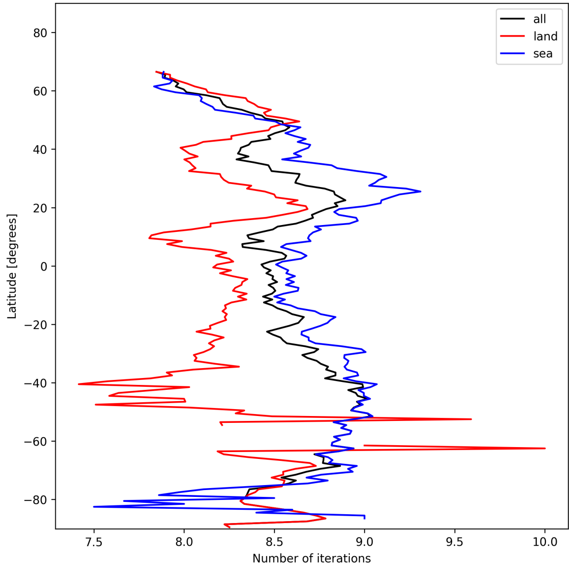
Figure 12: Zonal average of “Number of iterations” for 2025-01-26 to 2025-01-26.
