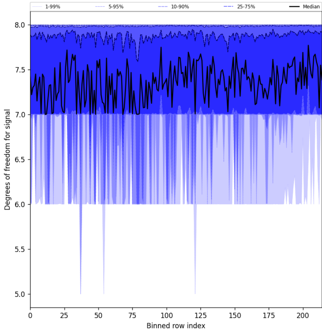
Figure 25: Along track statistics of “Degrees of freedom for signal” for 2025-01-26 to 2025-01-26
