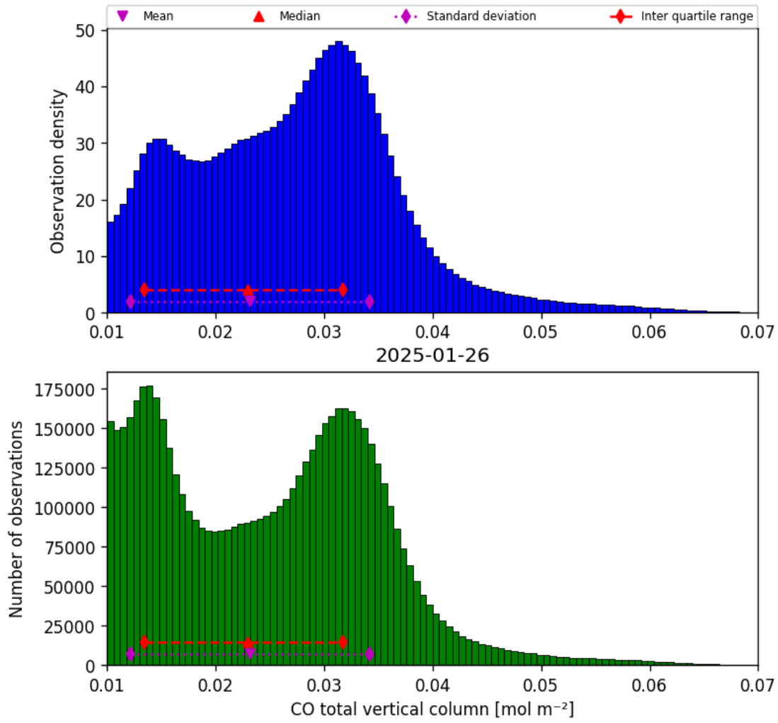
Figure 14: Histogram of “CO total vertical column” for 2025-01-26 to 2025-01-26
