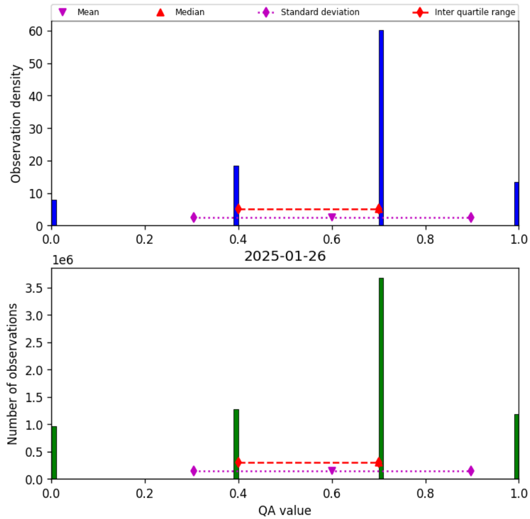
Figure 13: Histogram of “QA value” for 2025-01-26 to 2025-01-26
