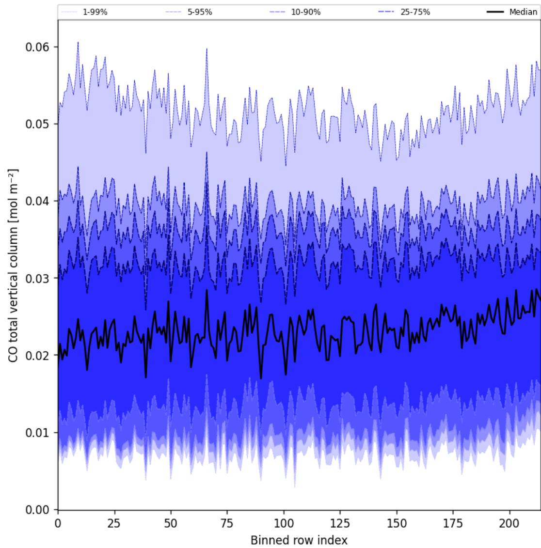
Figure 21: Along track statistics of “CO total vertical column” for 2025-01-26 to 2025-01-26
