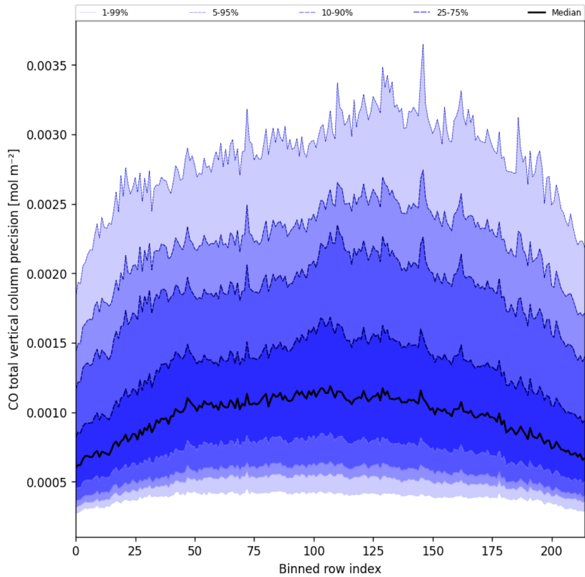
Figure 22: Along track statistics of “CO total vertical column precision” for 2025-01-26 to 2025-01-26
