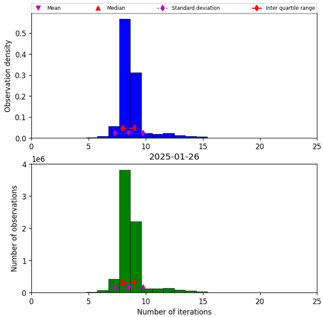
Figure 19: Histogram of “Number of iterations” for 2025-01-26 to 2025-01-26
