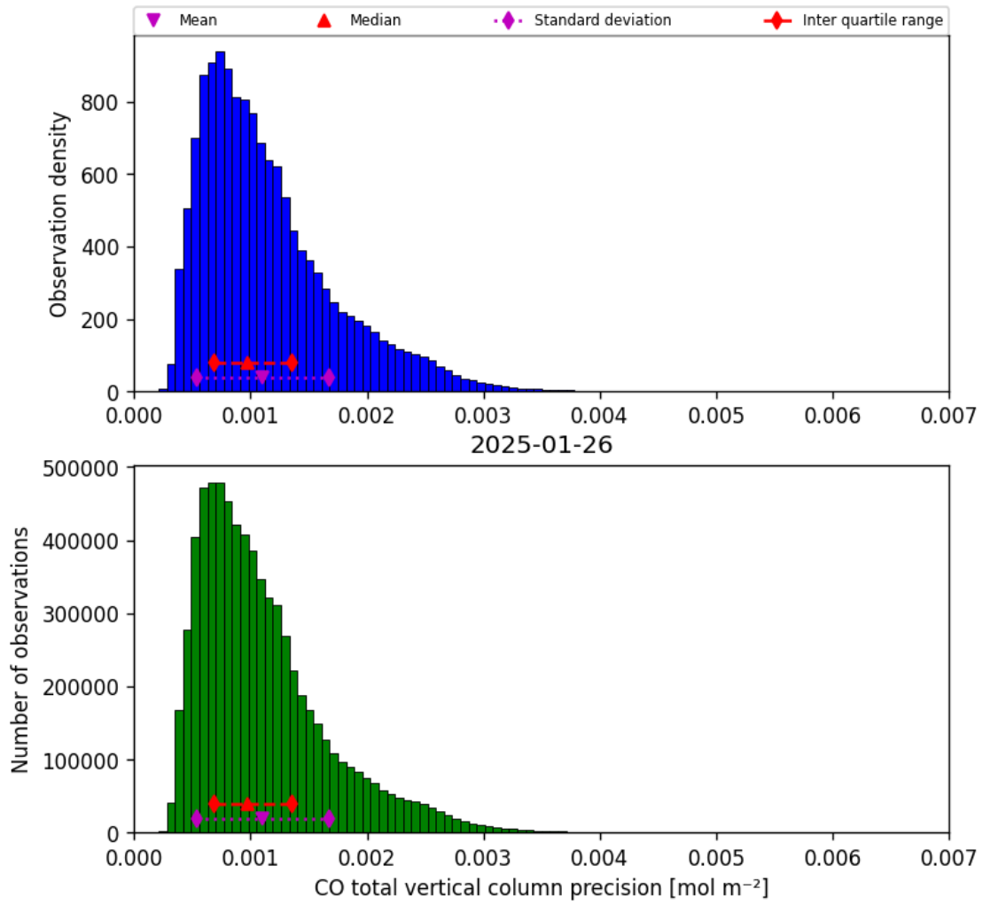
Figure 15: Histogram of “CO total vertical column precision” for 2025-01-26 to 2025-01-26
