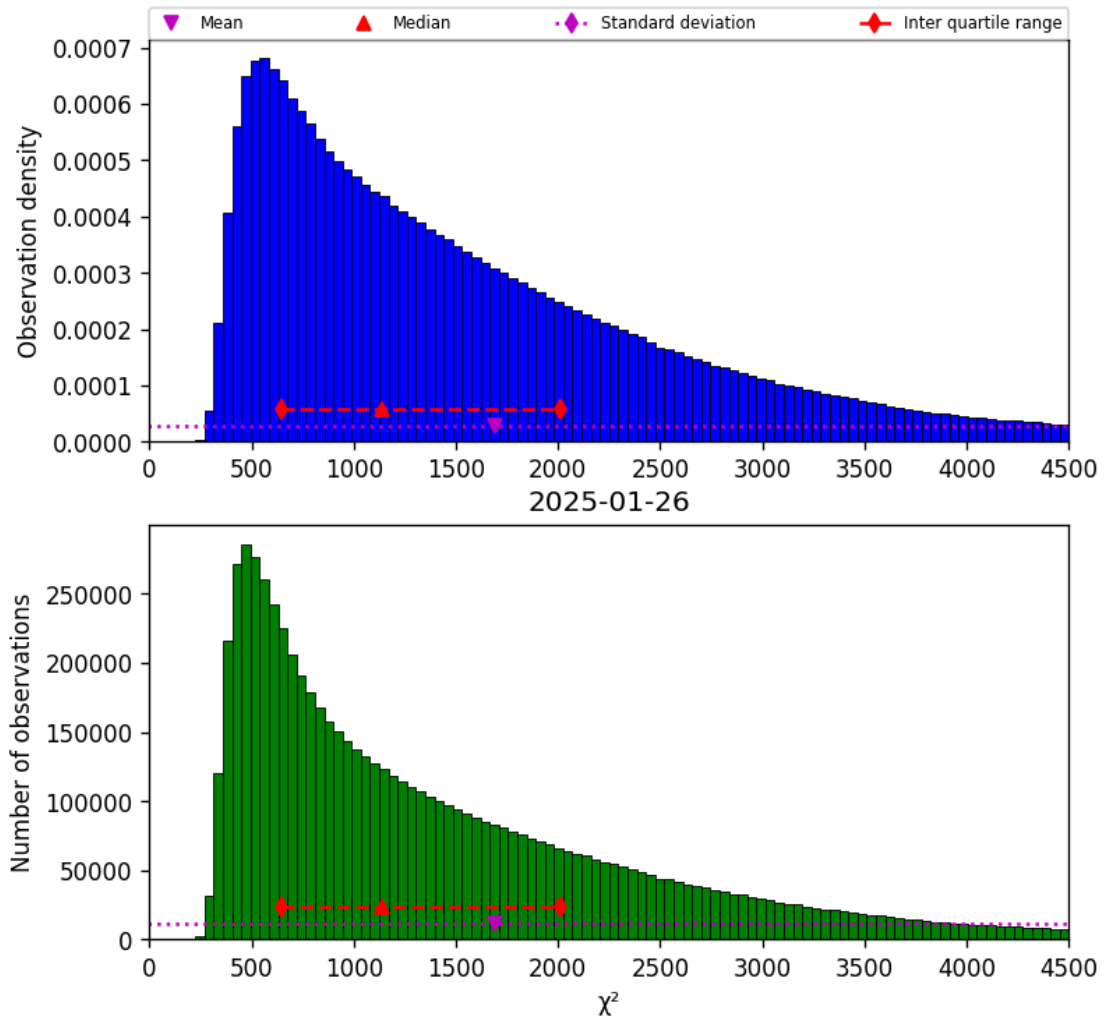
Figure 17: Histogram of " \chi^2 " for 2025-01-26 to 2025-01-26
