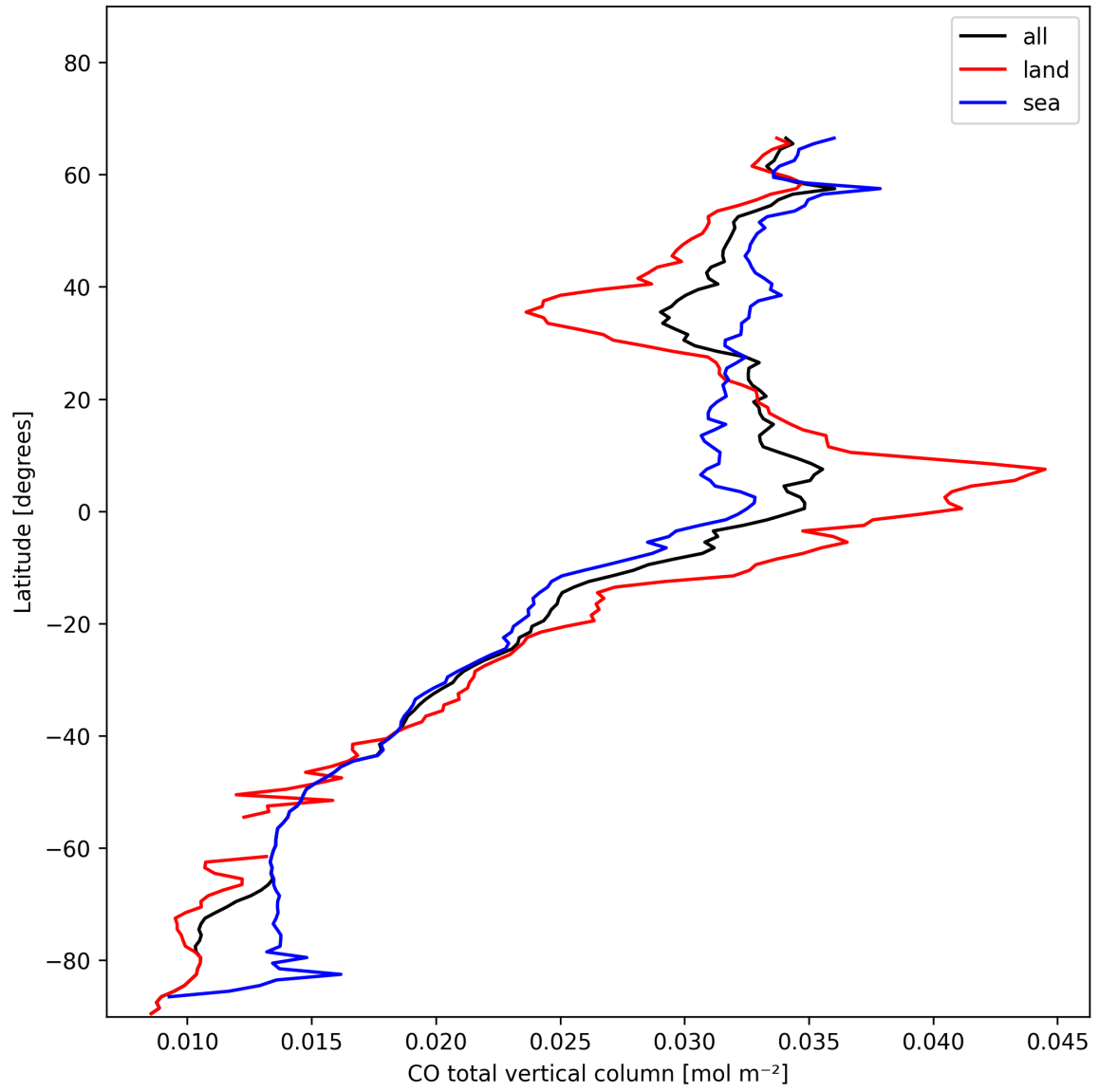
Figure 7: Zonal average of “CO total vertical column” for 2025-01-26 to 2025-01-26.
