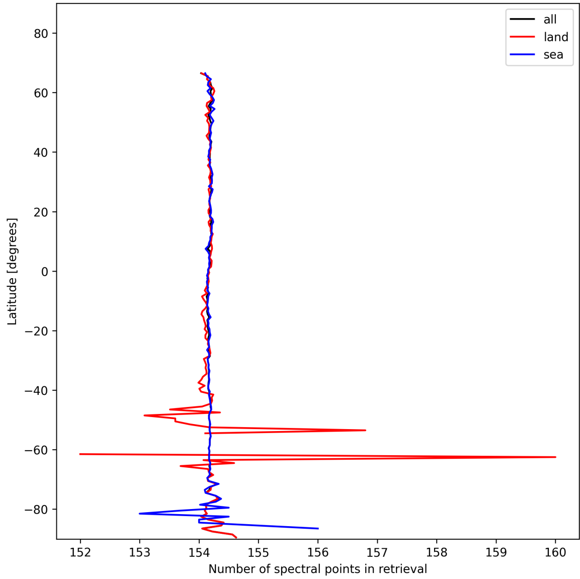
Figure 9: Zonal average of “Number of spectral points in retrieval” for 2025-01-26 to 2025-01-26.
