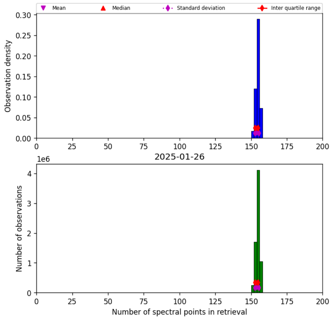
Figure 16: Histogram of “Number of spectral points in retrieval” for 2025-01-26 to 2025-01-26
