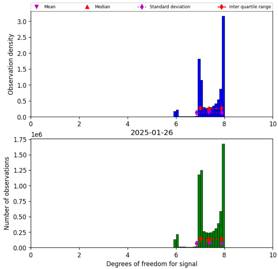
Figure 18: Histogram of “Degrees of freedom for signal” for 2025-01-26 to 2025-01-26
