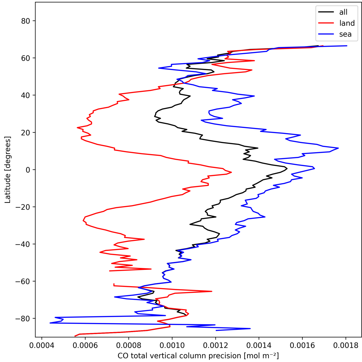
Figure 8: Zonal average of “CO total vertical column precision” for 2025-01-26 to 2025-01-26.
