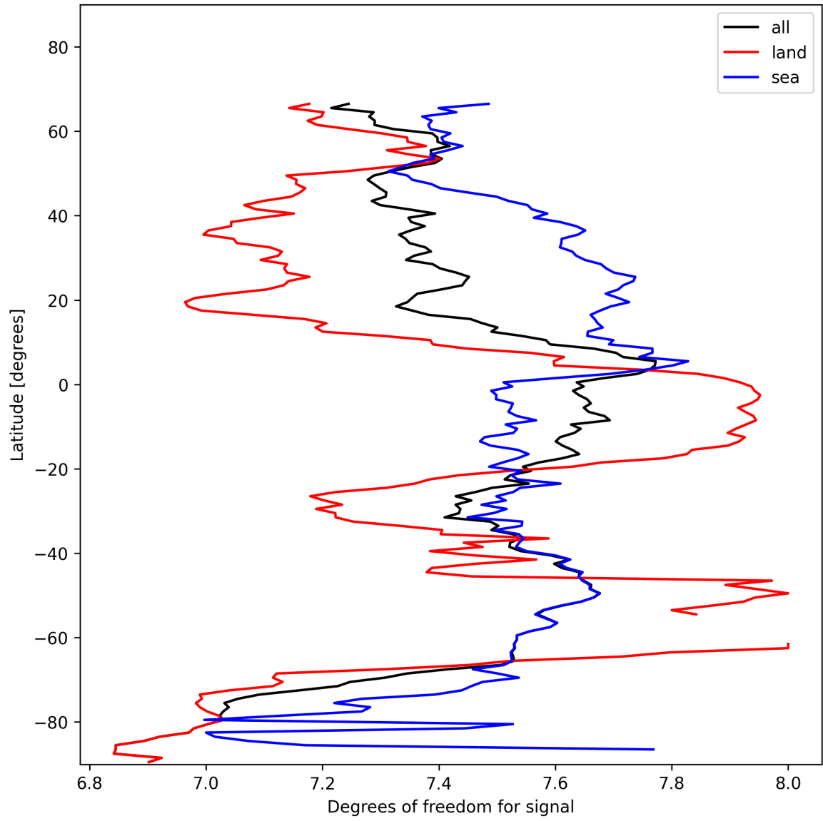
Figure 11: Zonal average of “Degrees of freedom for signal” for 2025-01-26 to 2025-01-26.
