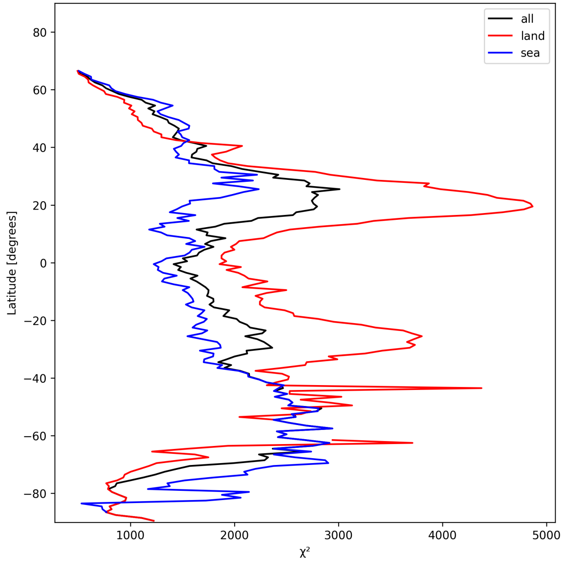
Figure 10: Zonal average of “ \chi^2 ” for 2025-01-26 to 2025-01-26.
