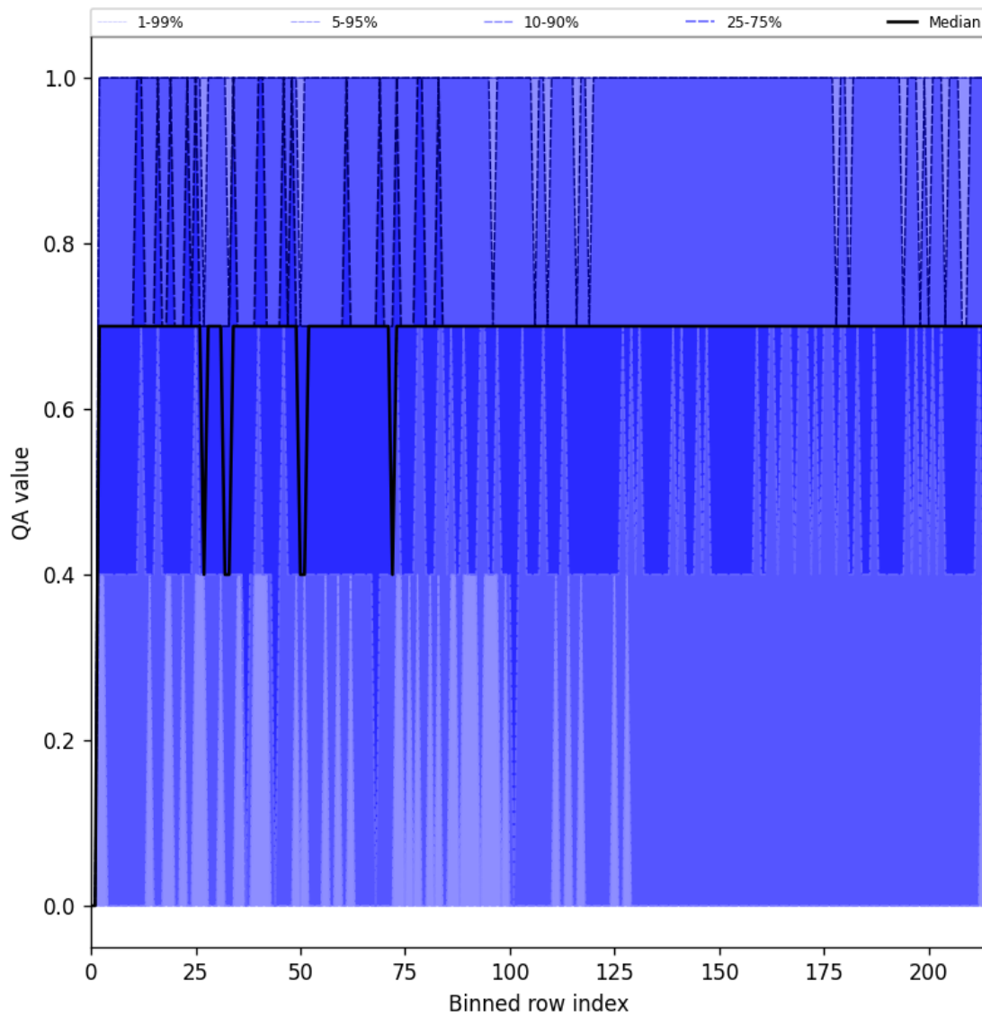
Figure 20: Along track statistics of “QA value” for 2025-01-26 to 2025-01-26
