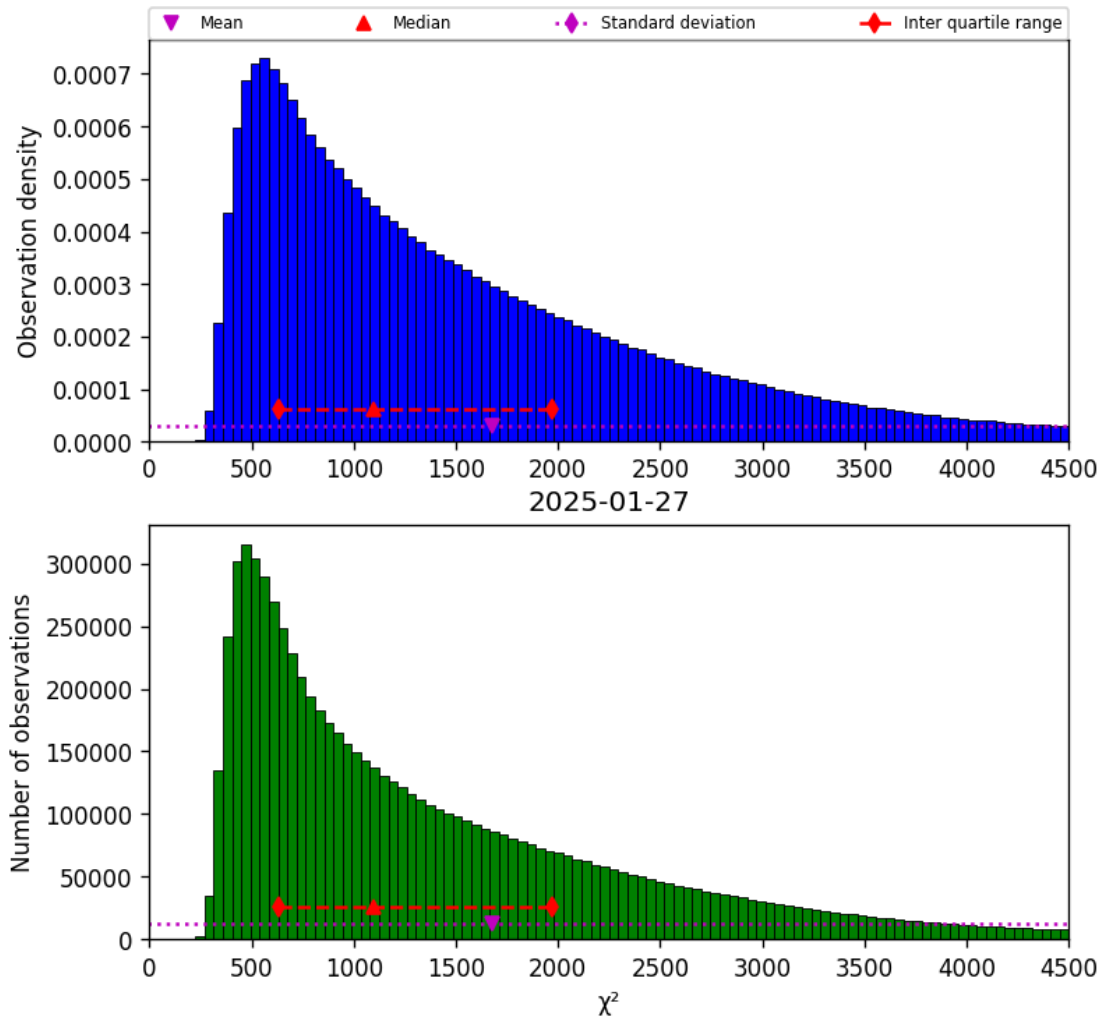
Figure 17: Histogram of “ \chi^2 ” for 2025-01-27 to 2025-01-28
