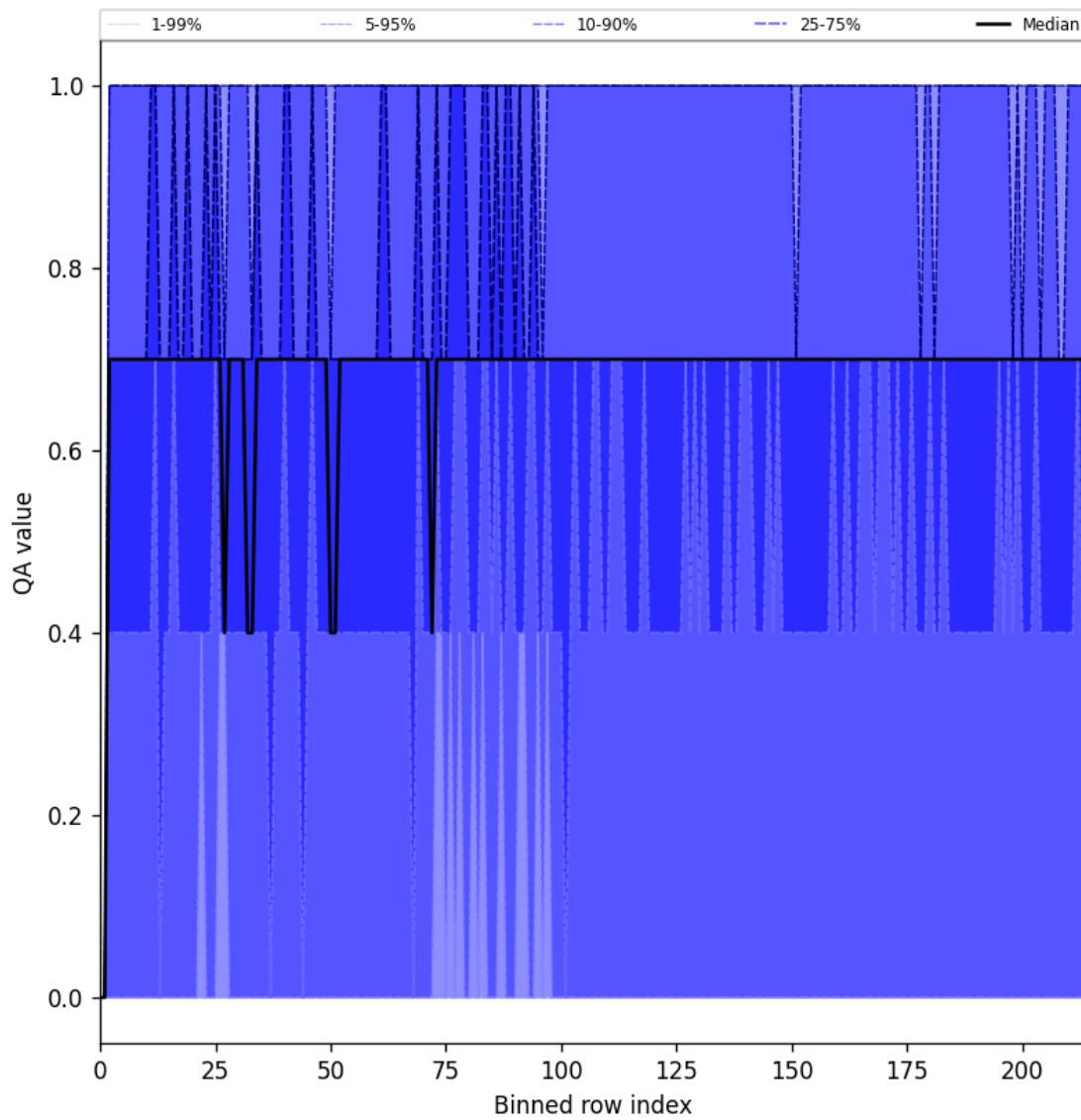
Figure 20: Along track statistics of “QA value” for 2025-01-27 to 2025-01-28
