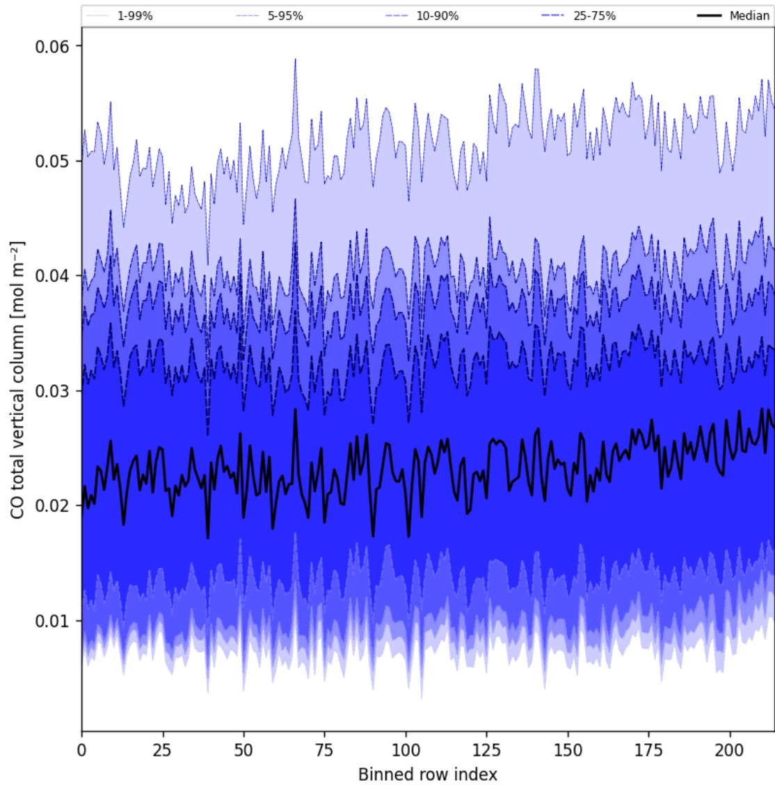
Figure 21: Along track statistics of “CO total vertical column” for 2025-01-27 to 2025-01-28
