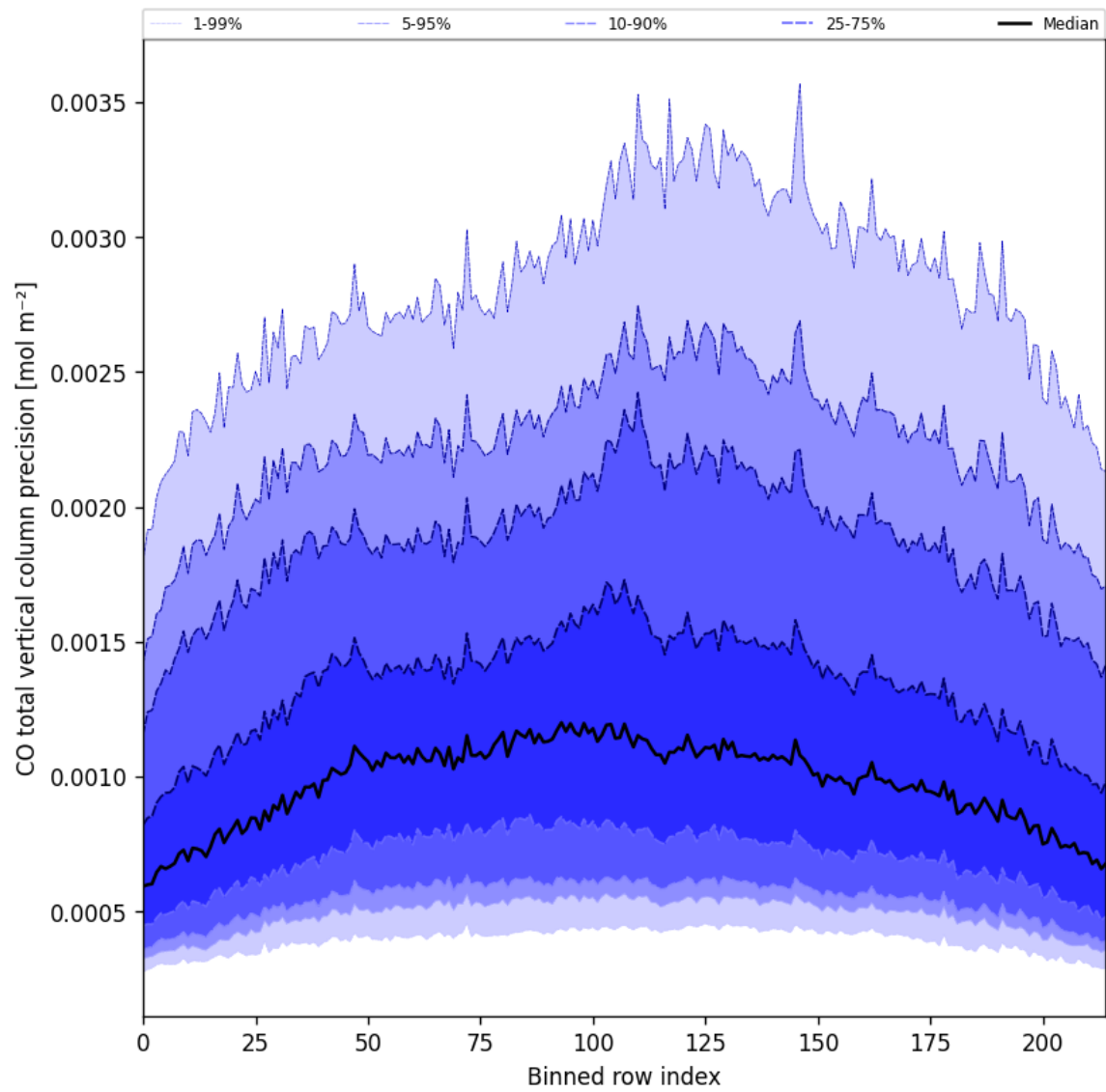
Figure 22: Along track statistics of “CO total vertical column precision” for 2025-01-27 to 2025-01-28
