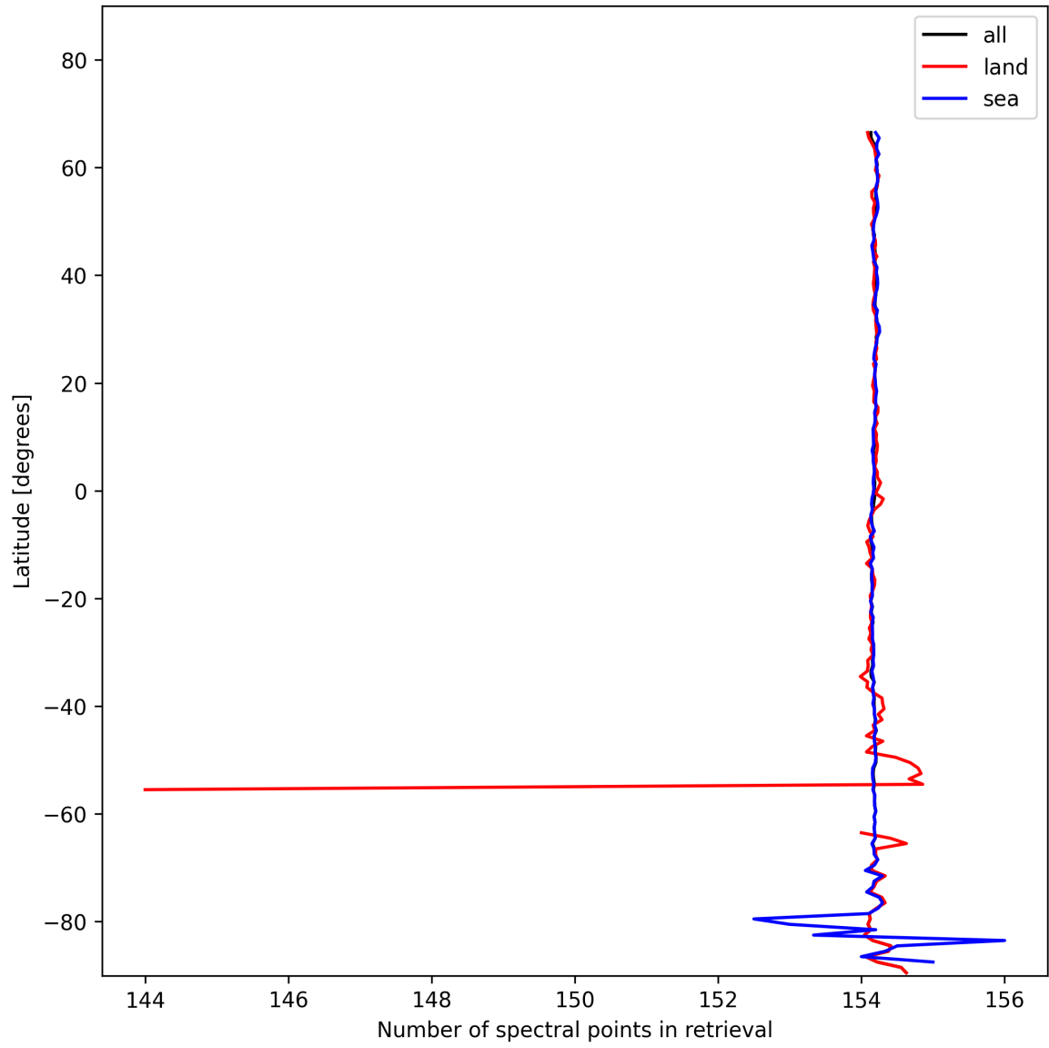
Figure 9: Zonal average of “Number of spectral points in retrieval” for 2025-01-27 to 2025-01-28.
