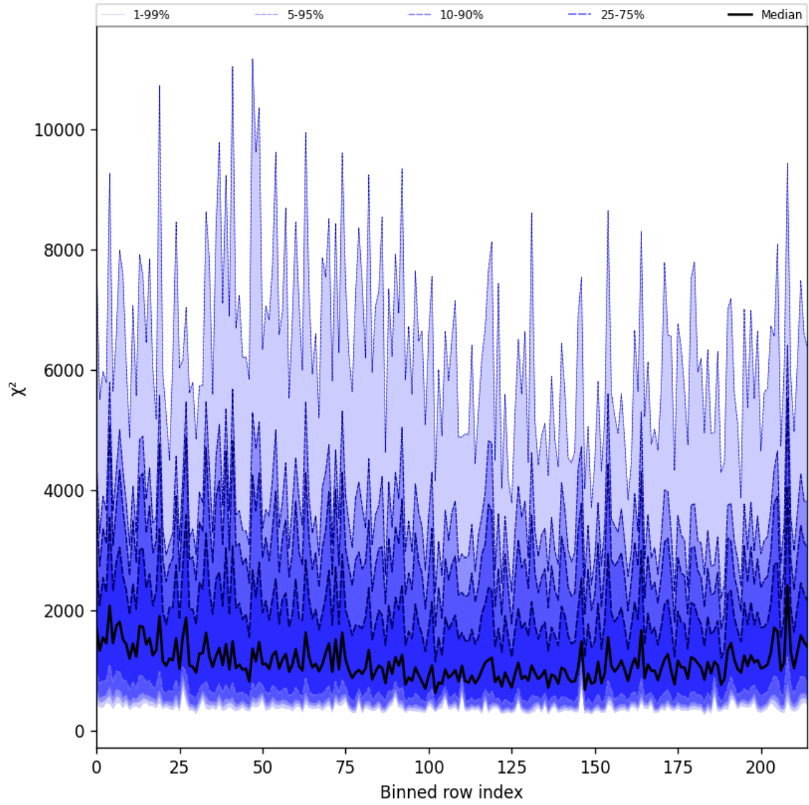
Figure 24: Along track statistics of “ \chi^2 ” for 2025-01-27 to 2025-01-28
