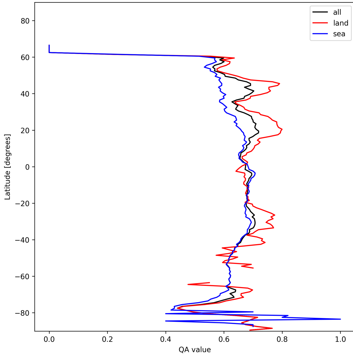
Figure 6: Zonal average of “QA value” for 2025-01-27 to 2025-01-28.
