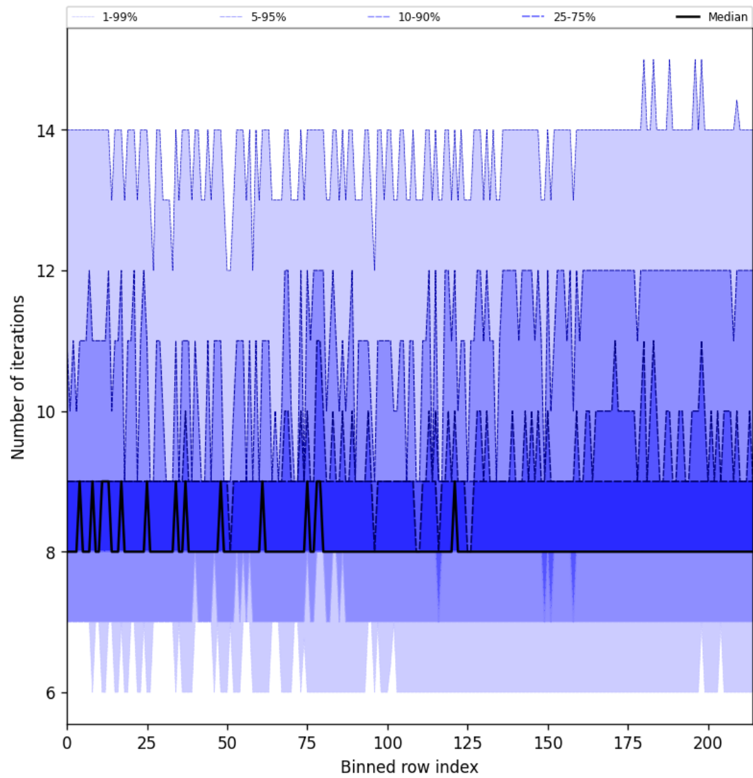
Figure 26: Along track statistics of “Number of iterations” for 2025-01-27 to 2025-01-28
