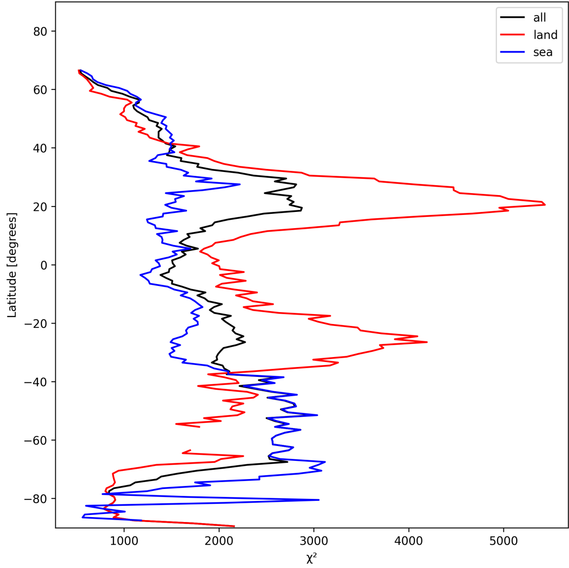
Figure 10: Zonal average of “ \chi^2 ” for 2025-01-27 to 2025-01-28.
