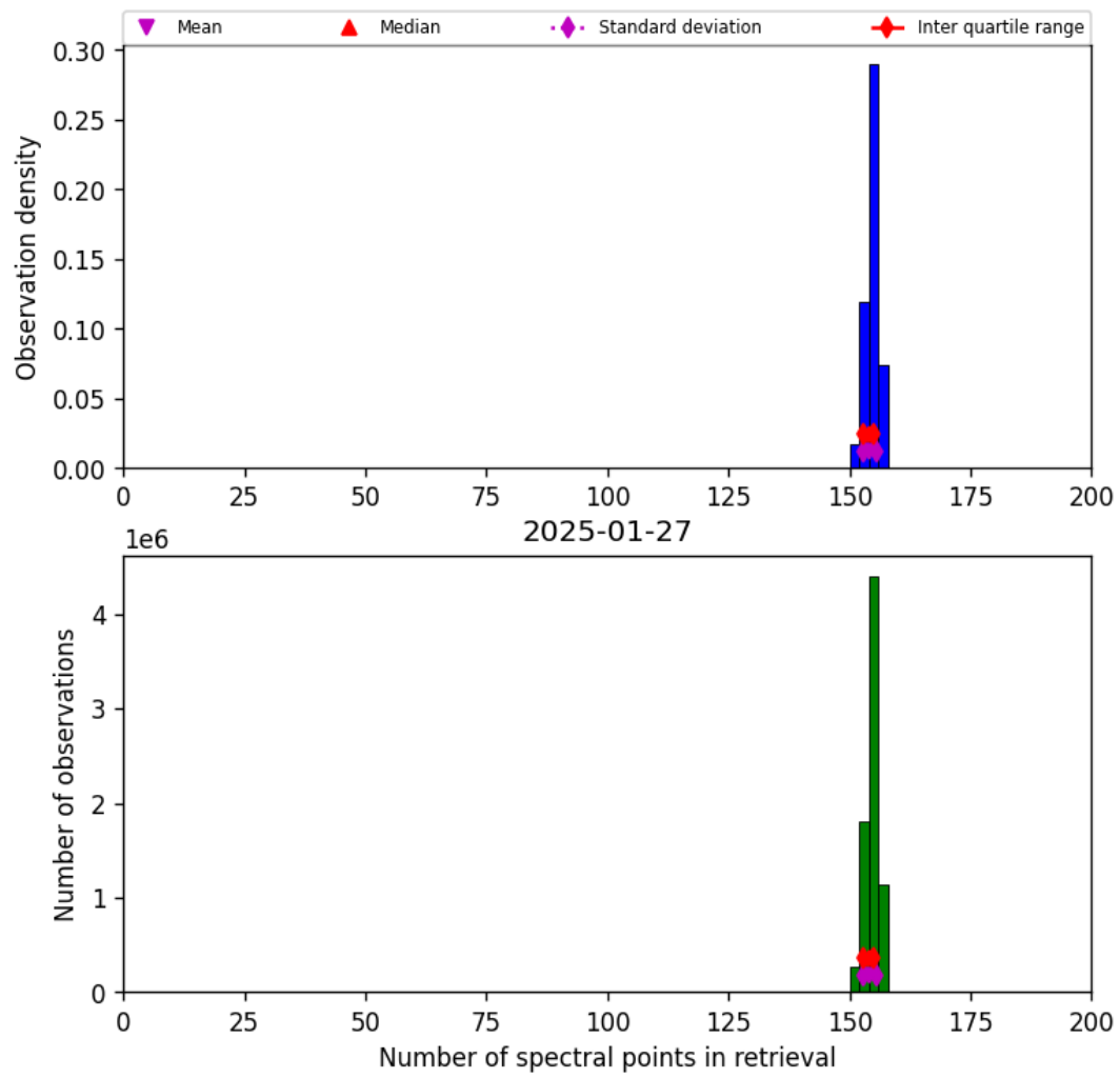
Figure 16: Histogram of “Number of spectral points in retrieval” for 2025-01-27 to 2025-01-28
