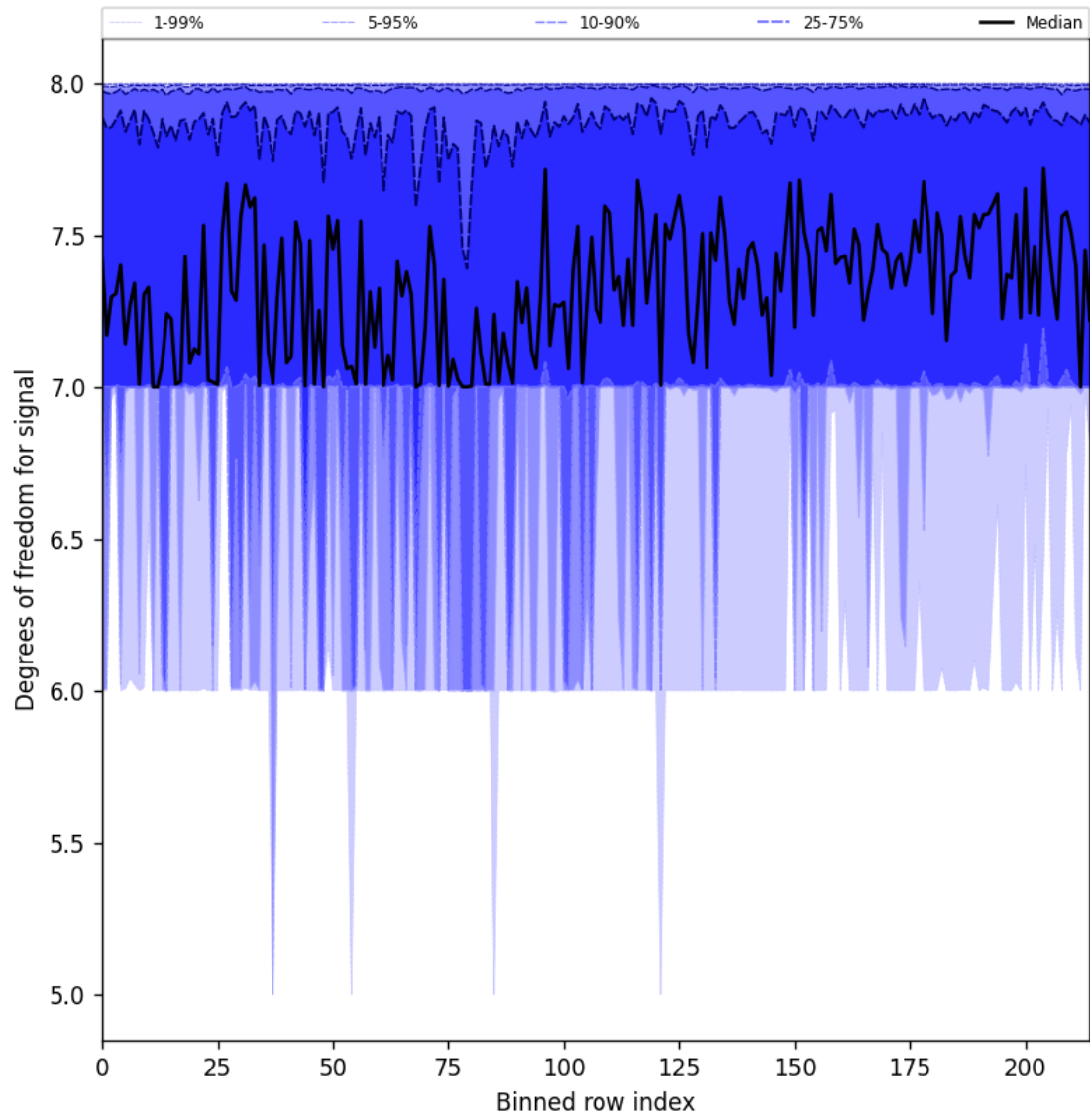
Figure 25: Along track statistics of “Degrees of freedom for signal” for 2025-01-27 to 2025-01-28
