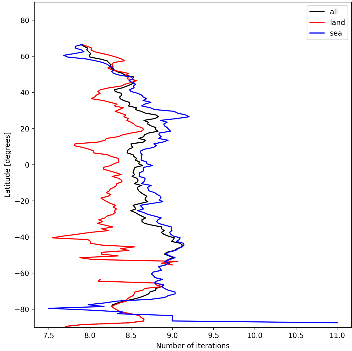
Figure 12: Zonal average of “Number of iterations” for 2025-01-27 to 2025-01-28.
