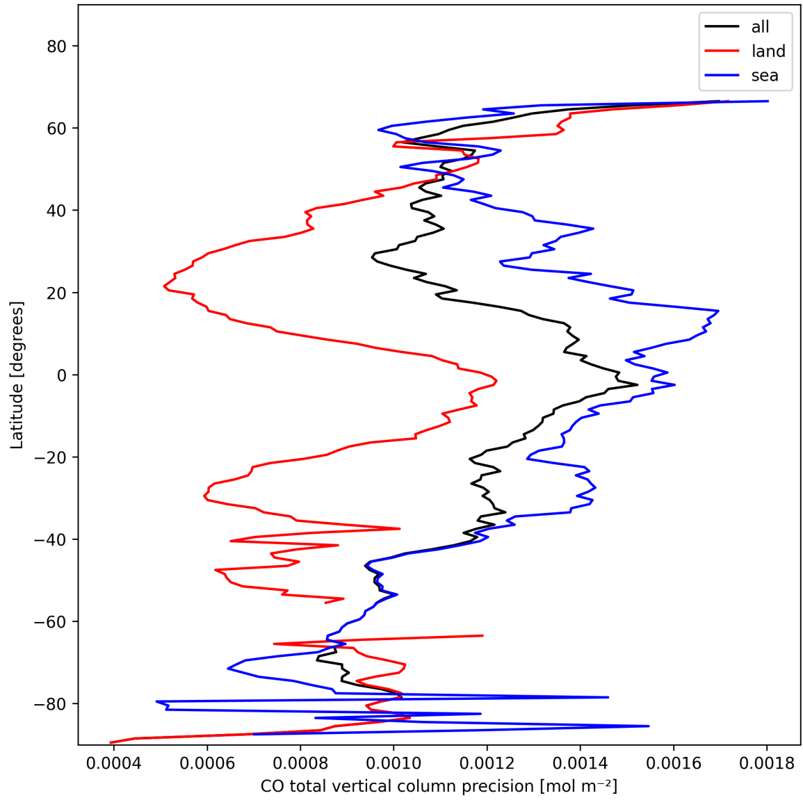
Figure 8: Zonal average of “CO total vertical column precision” for 2025-01-27 to 2025-01-28.
