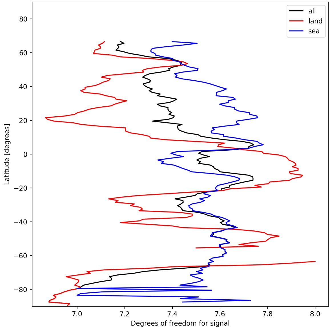
Figure 11: Zonal average of “Degrees of freedom for signal” for 2025-01-27 to 2025-01-28.
