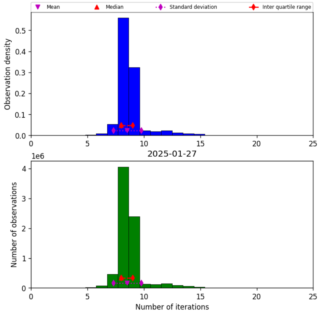
Figure 19: Histogram of “Number of iterations” for 2025-01-27 to 2025-01-28
