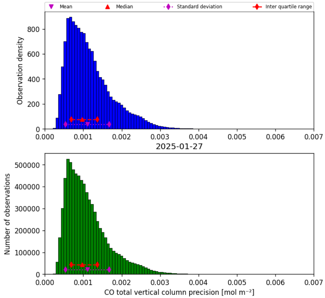
Figure 15: Histogram of “CO total vertical column precision” for 2025-01-27 to 2025-01-28
