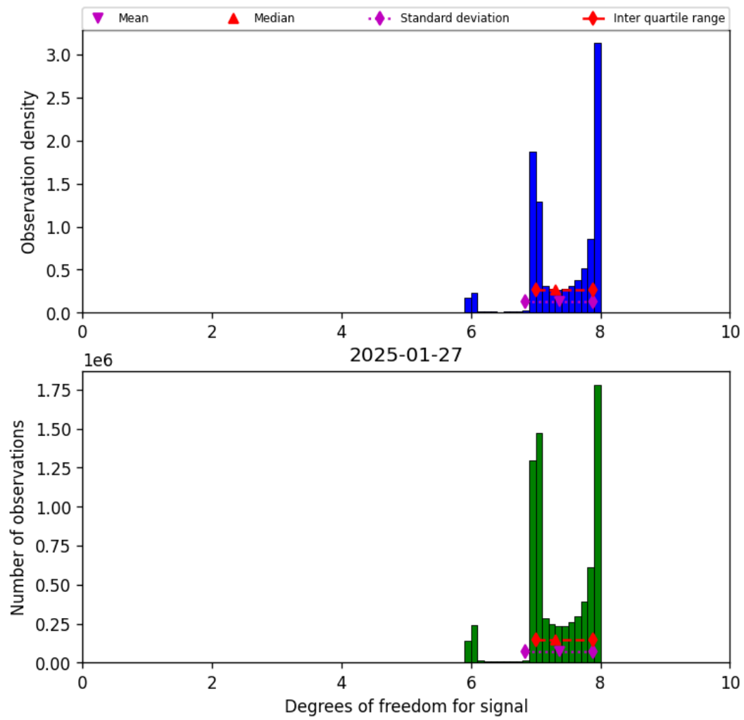
Figure 18: Histogram of “Degrees of freedom for signal” for 2025-01-27 to 2025-01-28
