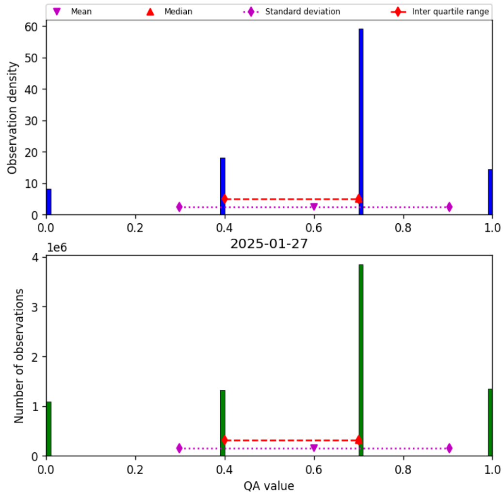
Figure 13: Histogram of “QA value” for 2025-01-27 to 2025-01-28
