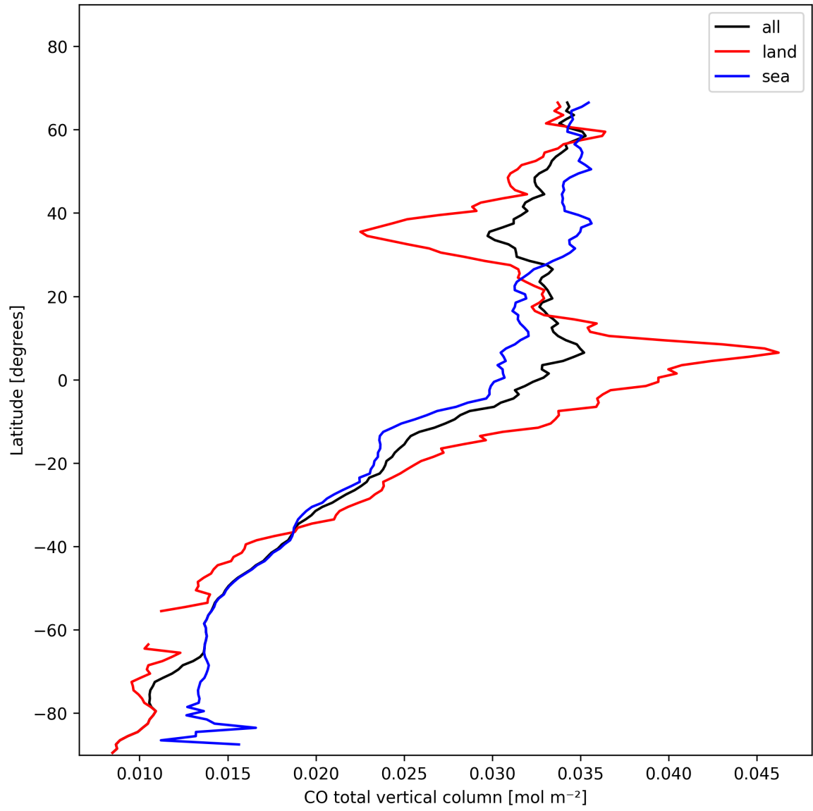
Figure 7: Zonal average of “CO total vertical column” for 2025-01-27 to 2025-01-28.
