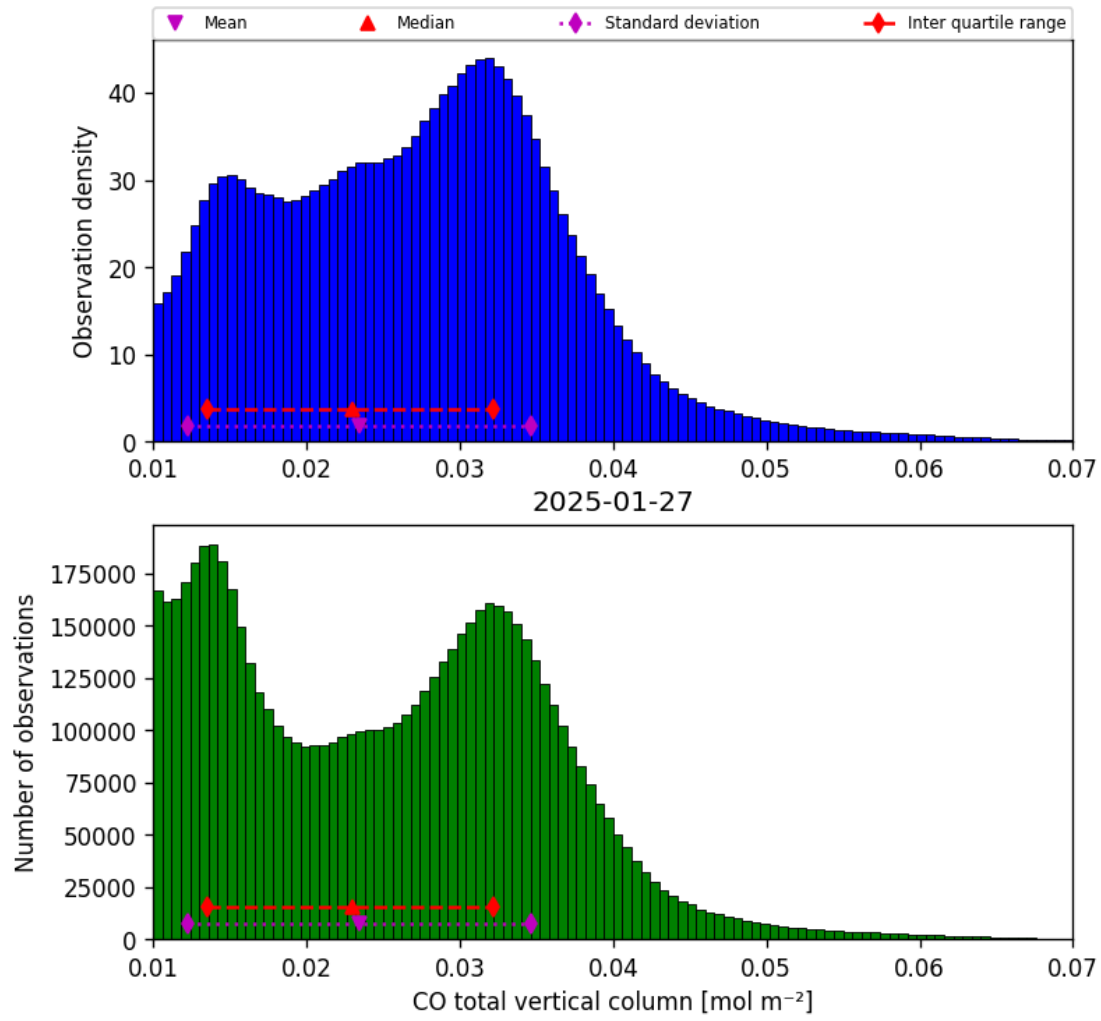
Figure 14: Histogram of “CO total vertical column” for 2025-01-27 to 2025-01-28
