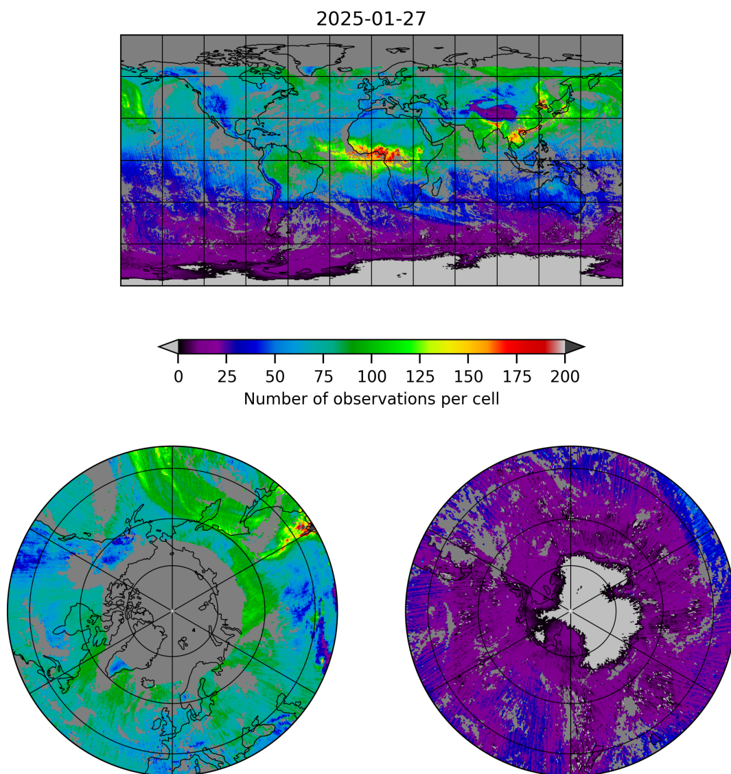
Figure 5: Map of the number of observations for 2025-01-27 to 2025-01-28
