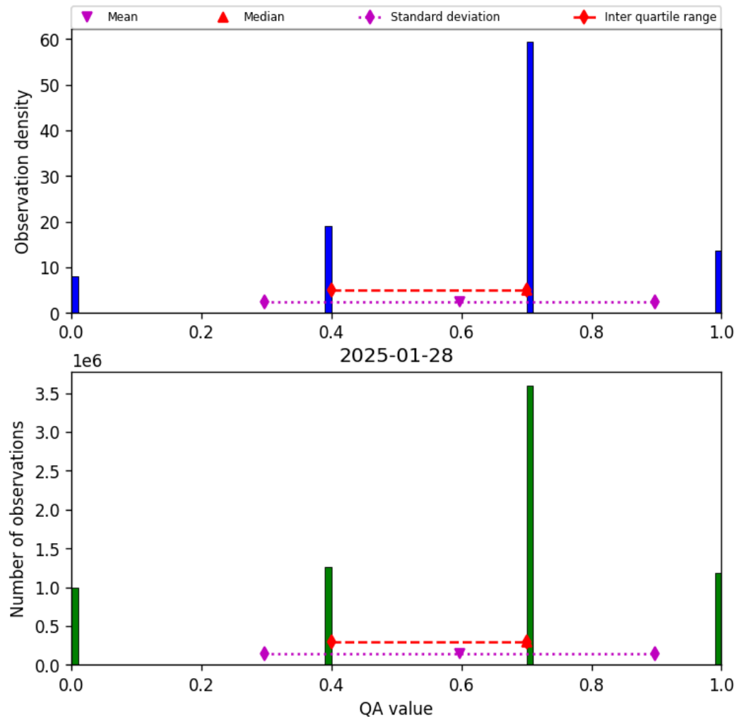
Figure 13: Histogram of “QA value” for 2025-01-28 to 2025-01-29
