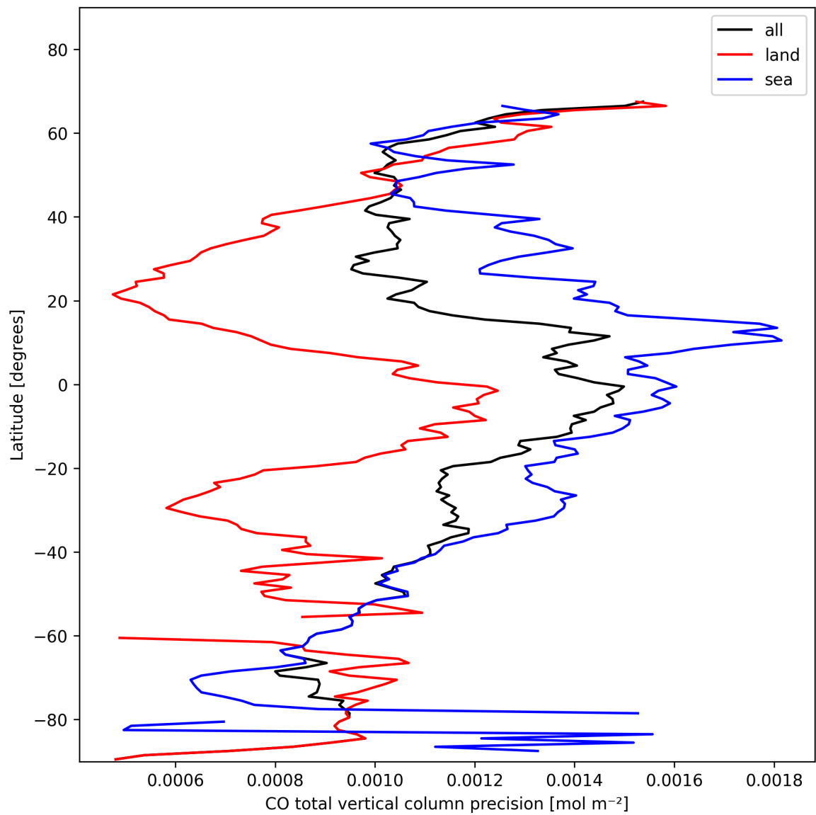
Figure 8: Zonal average of “CO total vertical column precision” for 2025-01-28 to 2025-01-29.
