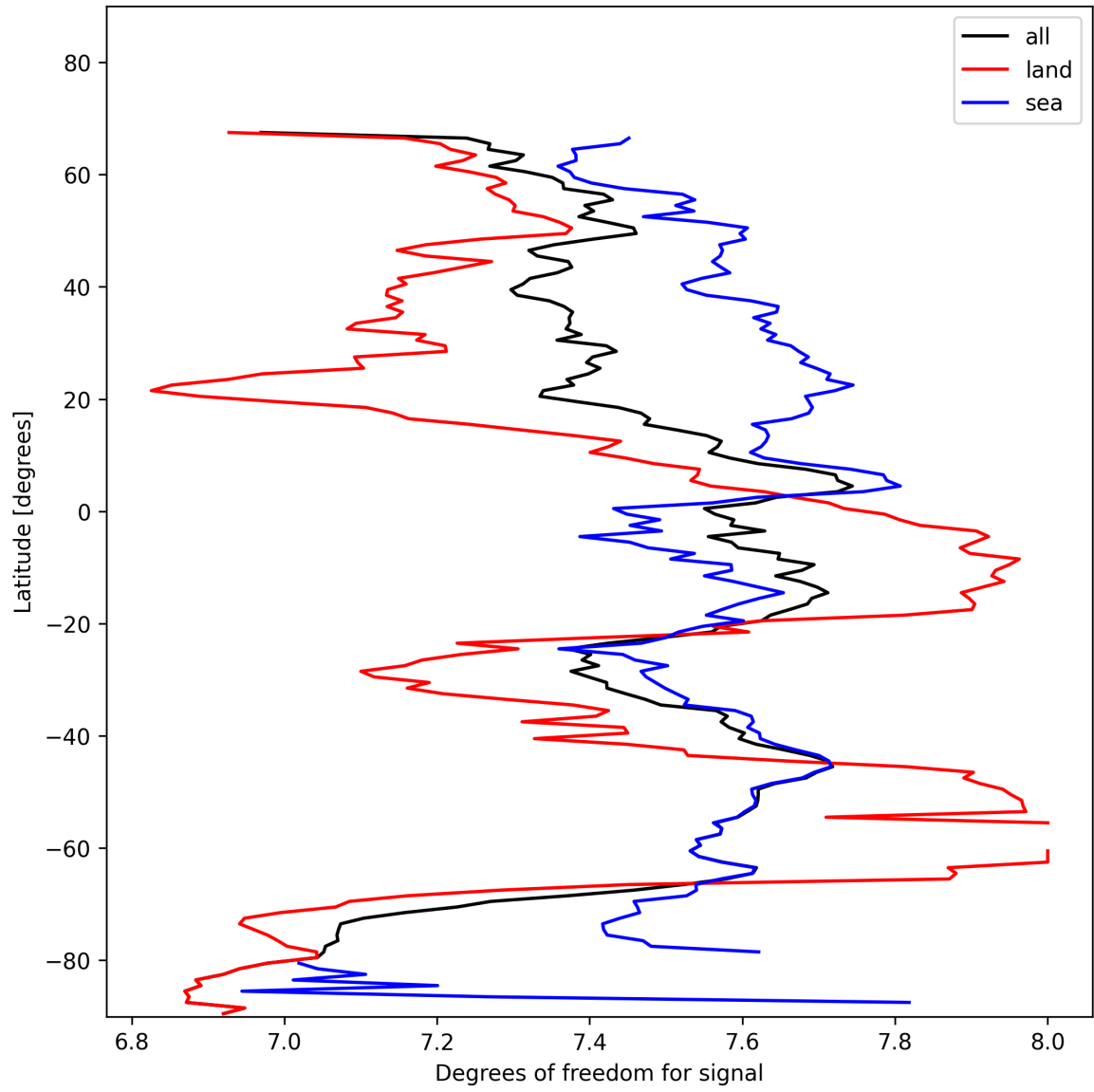
Figure 11: Zonal average of “Degrees of freedom for signal” for 2025-01-28 to 2025-01-29.
