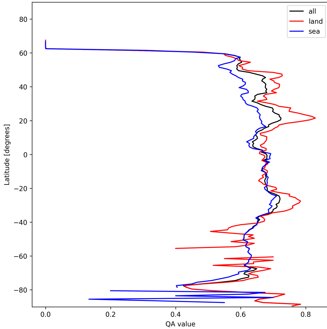
Figure 6: Zonal average of “QA value” for 2025-01-28 to 2025-01-29.
