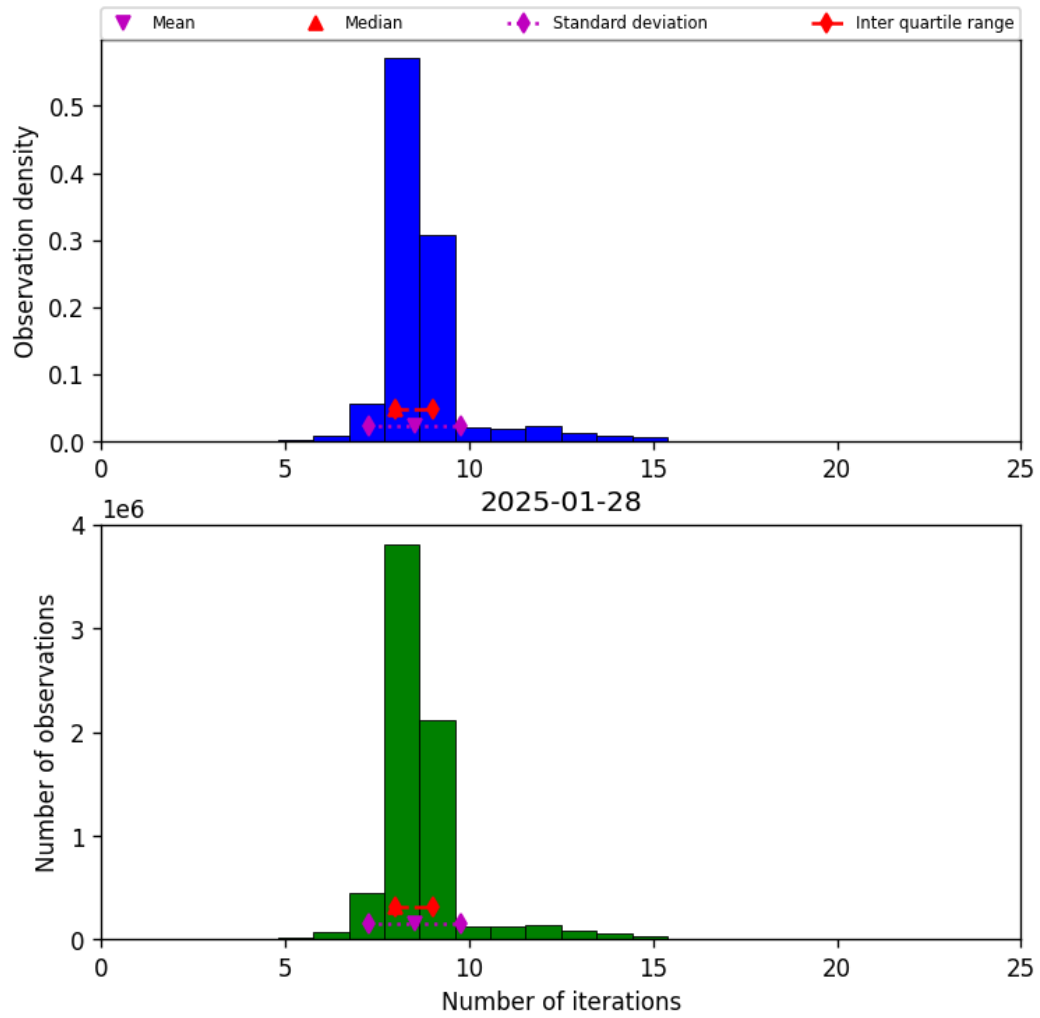
Figure 19: Histogram of “Number of iterations” for 2025-01-28 to 2025-01-29
