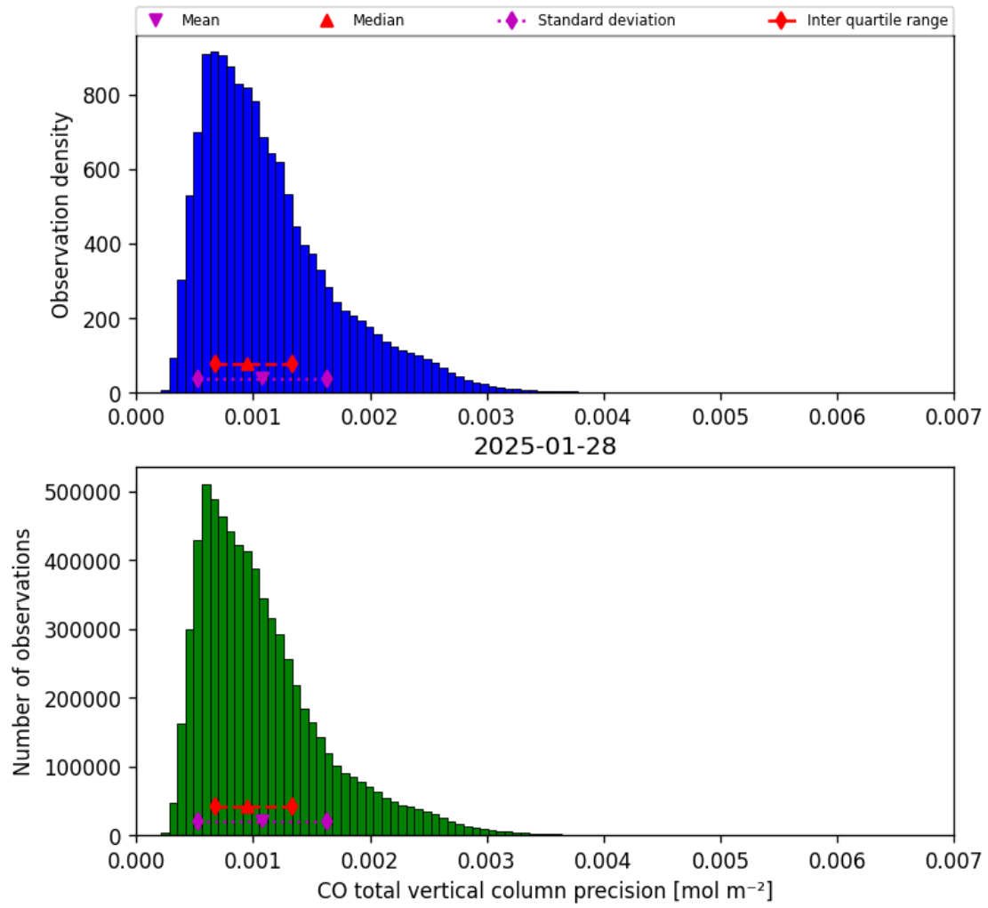
Figure 15: Histogram of “CO total vertical column precision” for 2025-01-28 to 2025-01-29
