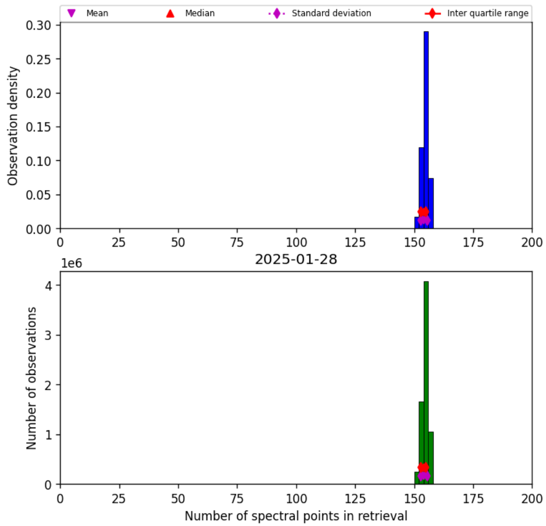
Figure 16: Histogram of “Number of spectral points in retrieval” for 2025-01-28 to 2025-01-29
