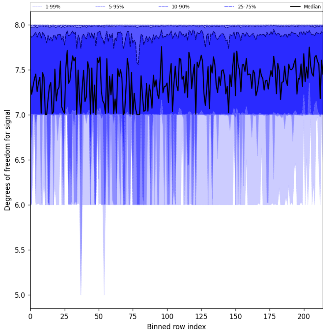
Figure 25: Along track statistics of “Degrees of freedom for signal” for 2025-01-28 to 2025-01-29
