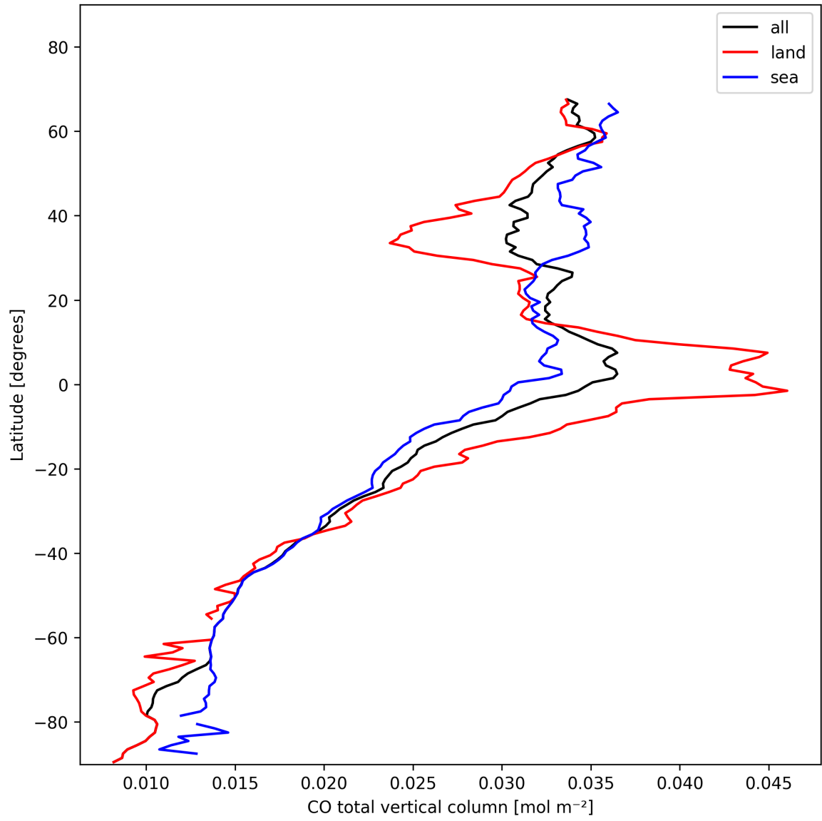
Figure 7: Zonal average of “CO total vertical column” for 2025-01-28 to 2025-01-29.
