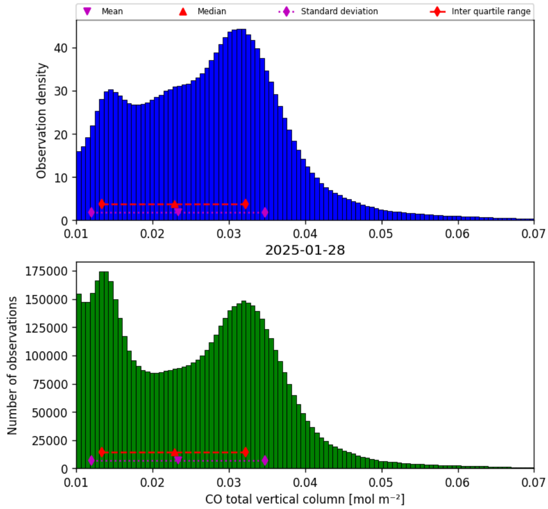
Figure 14: Histogram of “CO total vertical column” for 2025-01-28 to 2025-01-29
