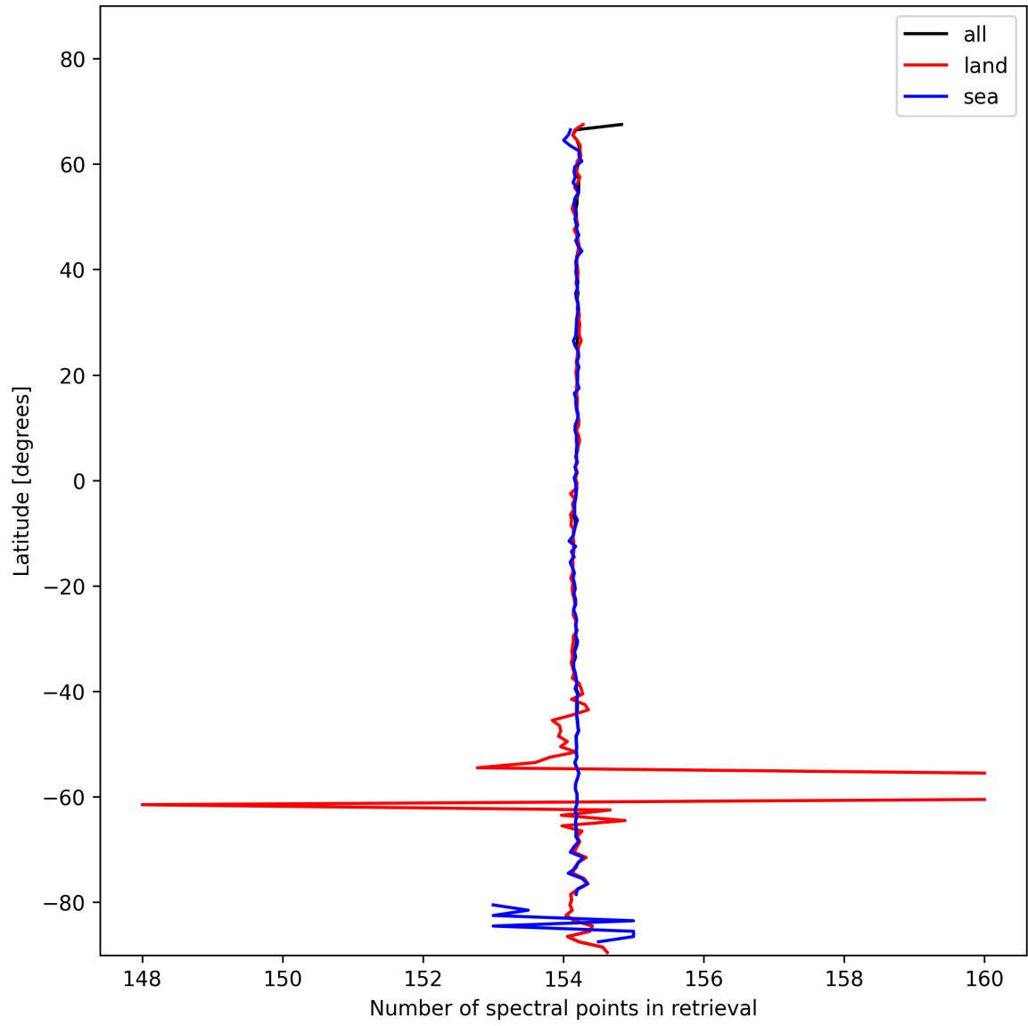
Figure 9: Zonal average of “Number of spectral points in retrieval” for 2025-01-28 to 2025-01-29.
