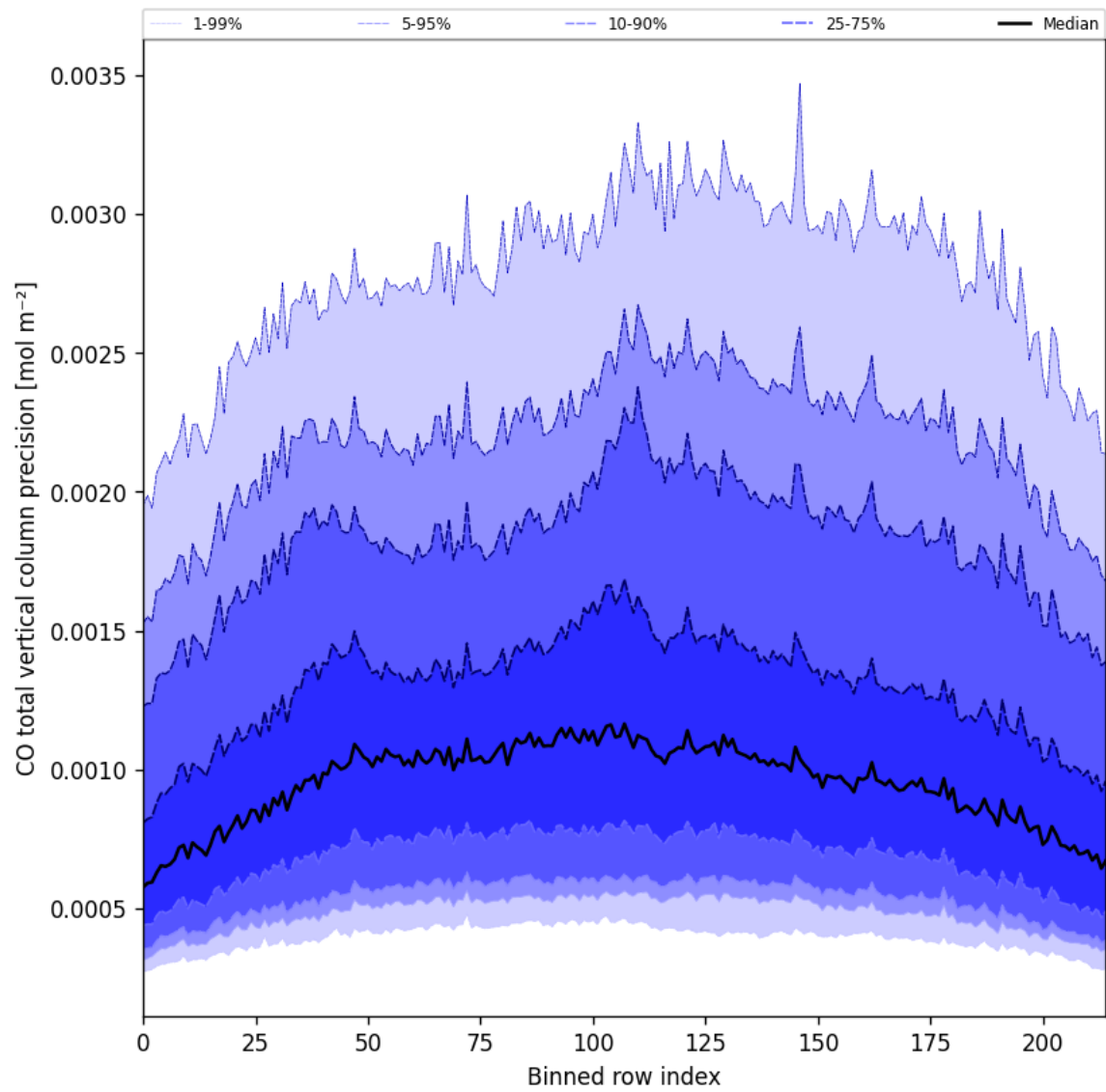
Figure 22: Along track statistics of “CO total vertical column precision” for 2025-01-28 to 2025-01-29
