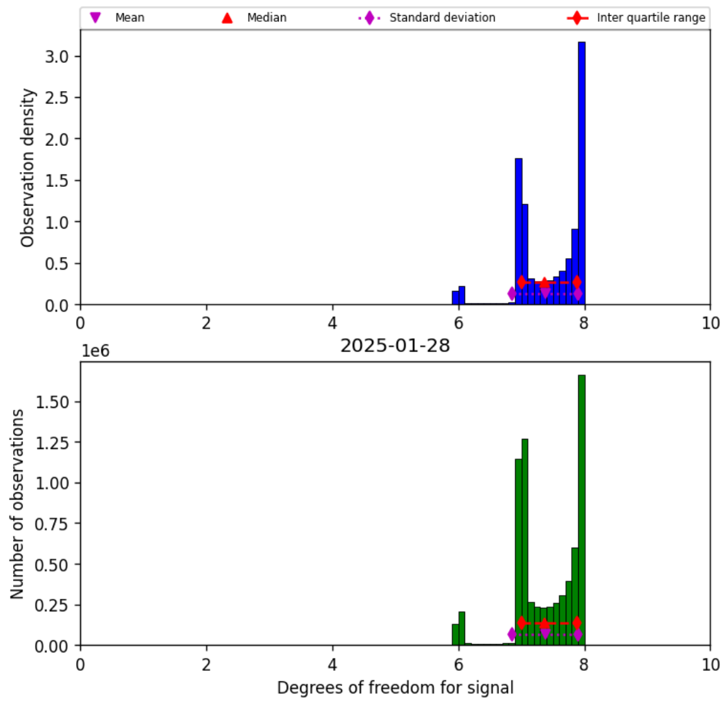
Figure 18: Histogram of “Degrees of freedom for signal” for 2025-01-28 to 2025-01-29
