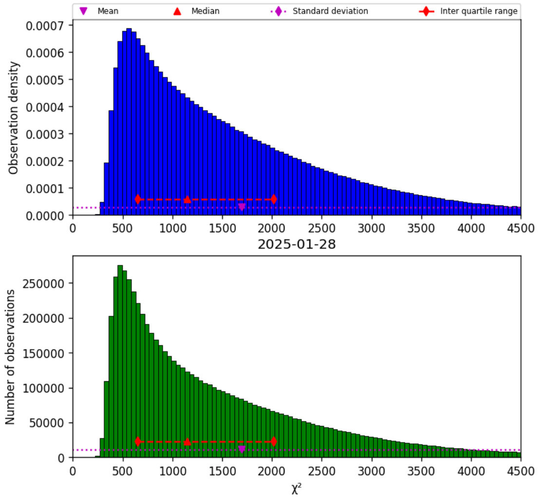
Figure 17: Histogram of “ \chi^2 ” for 2025-01-28 to 2025-01-29
