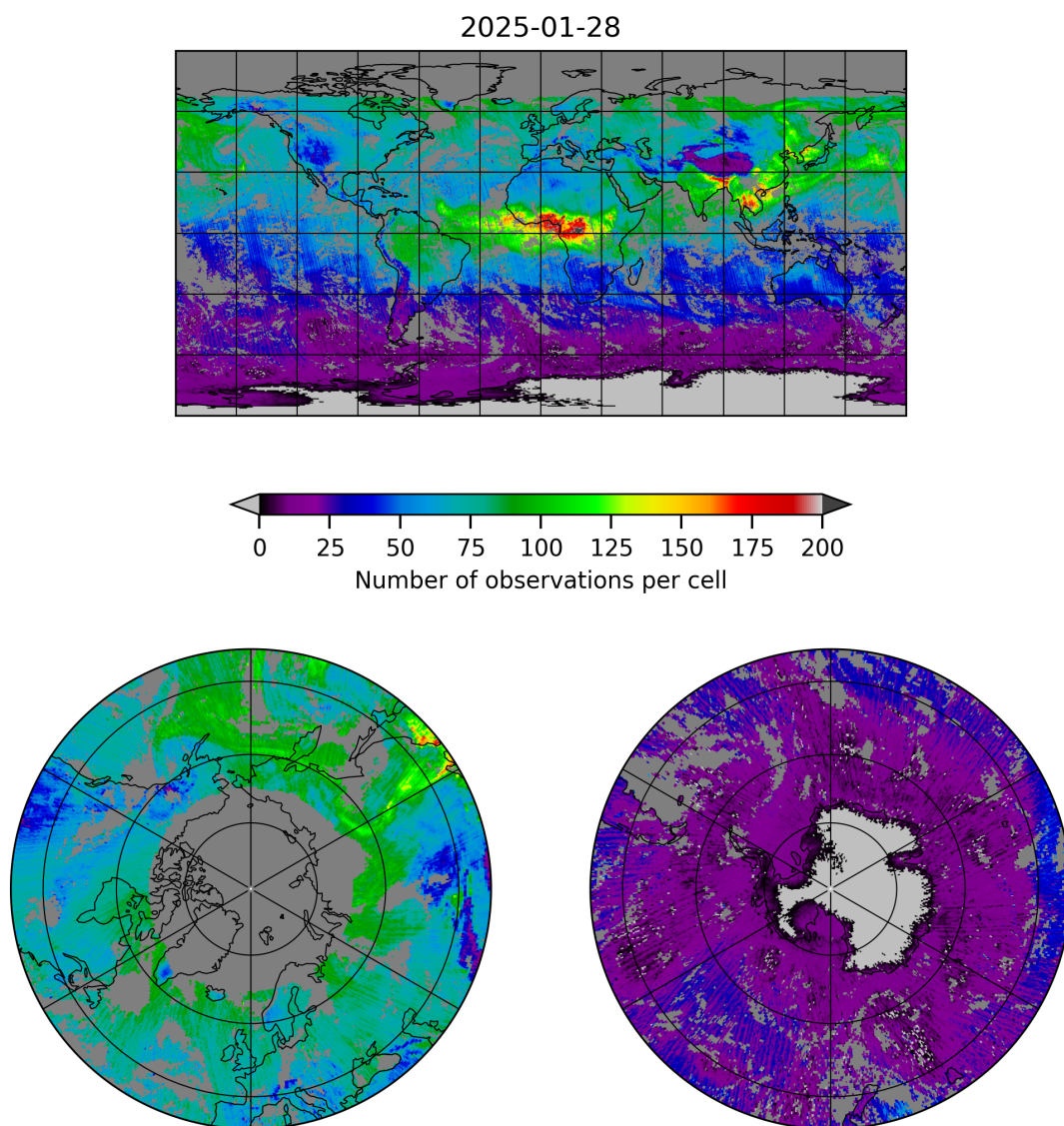
Figure 5: Map of the number of observations for 2025-01-28 to 2025-01-29
