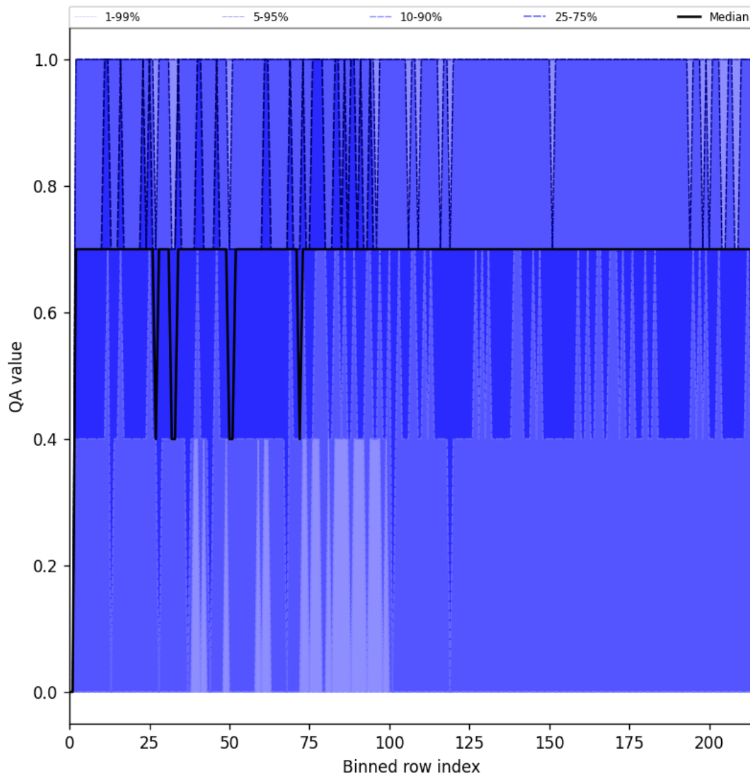
Figure 20: Along track statistics of “QA value” for 2025-01-28 to 2025-01-29
