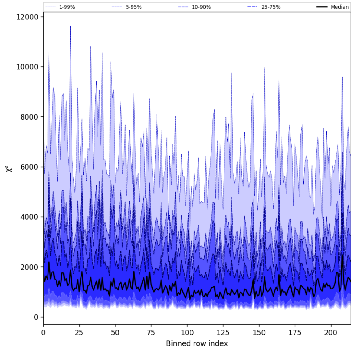
Figure 24: Along track statistics of “ \chi^2 ” for 2025-01-28 to 2025-01-29
