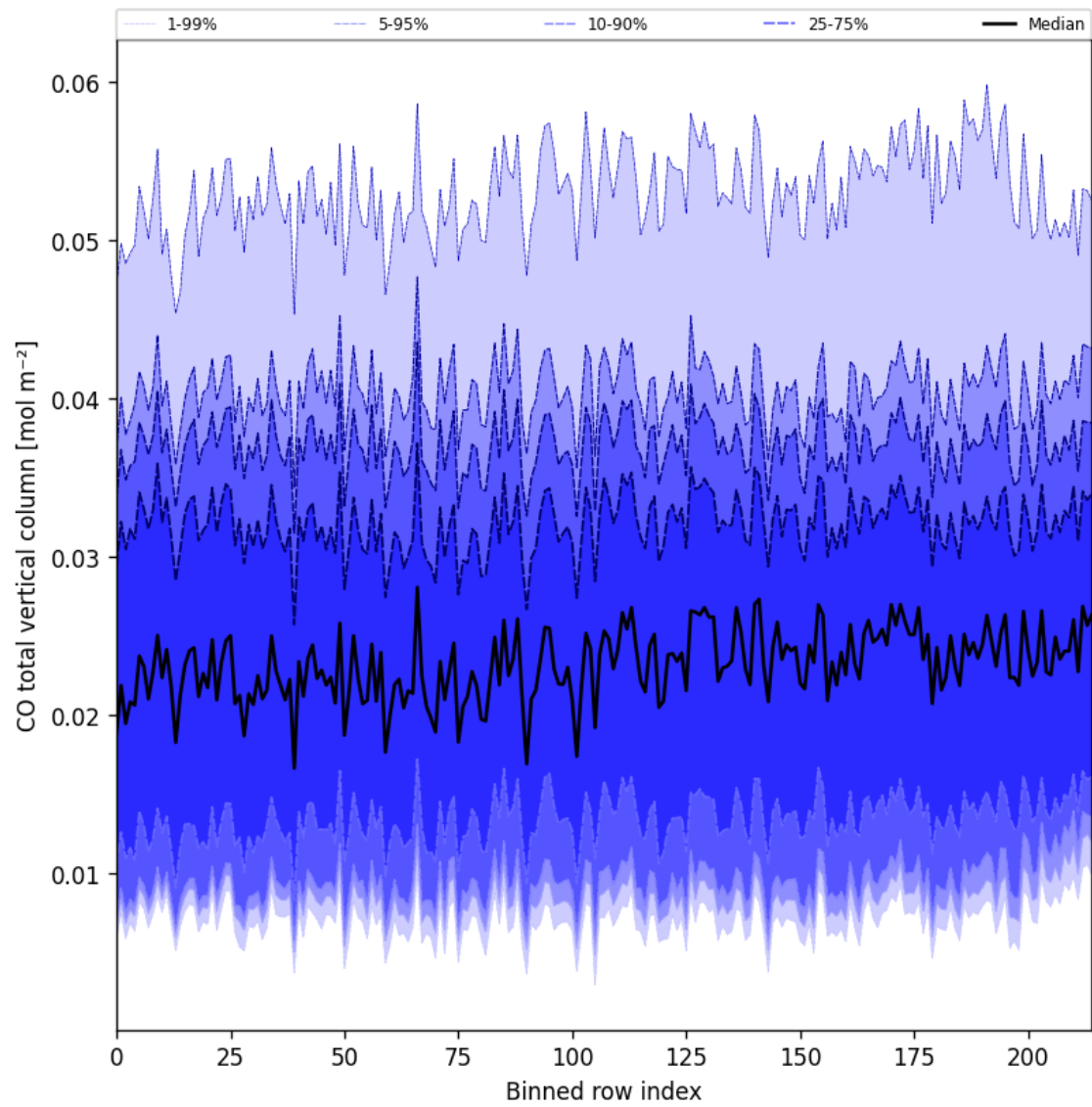
Figure 21: Along track statistics of “CO total vertical column” for 2025-01-28 to 2025-01-29
