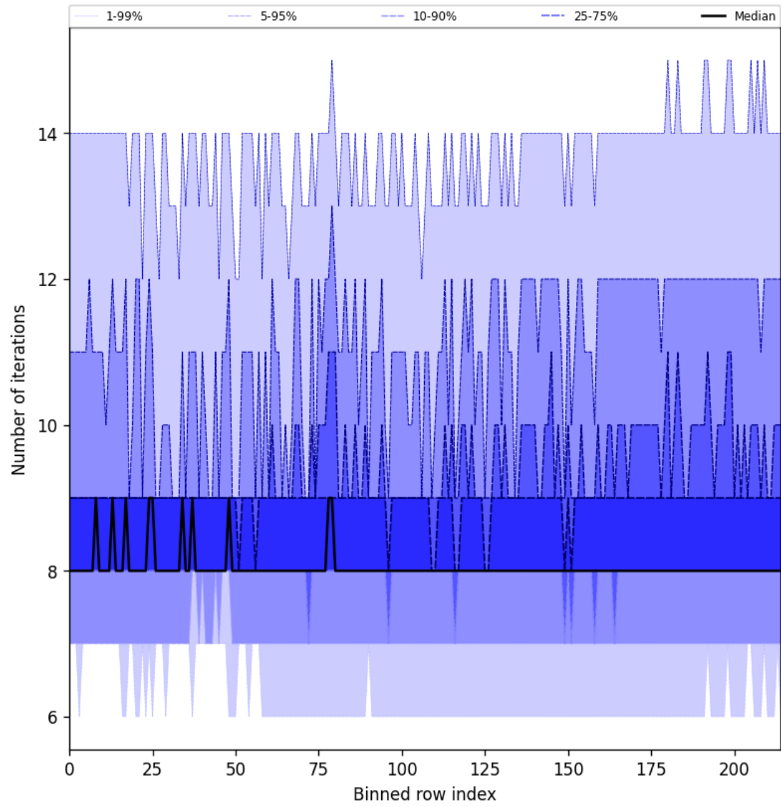
Figure 26: Along track statistics of “Number of iterations” for 2025-01-28 to 2025-01-29
