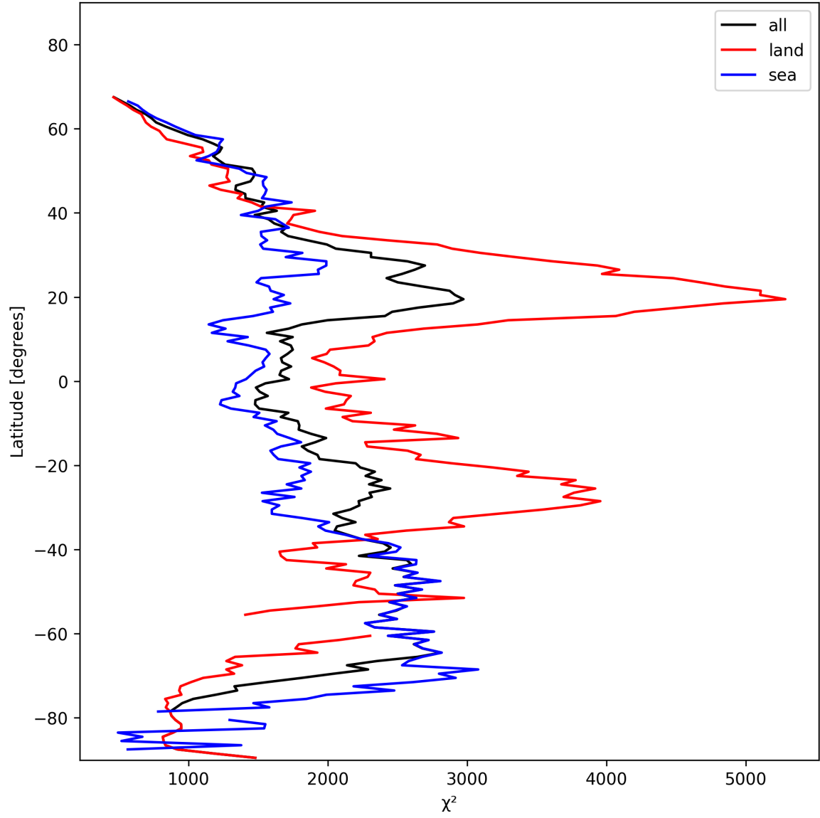
Figure 10: Zonal average of “ \chi^2 ” for 2025-01-28 to 2025-01-29.
