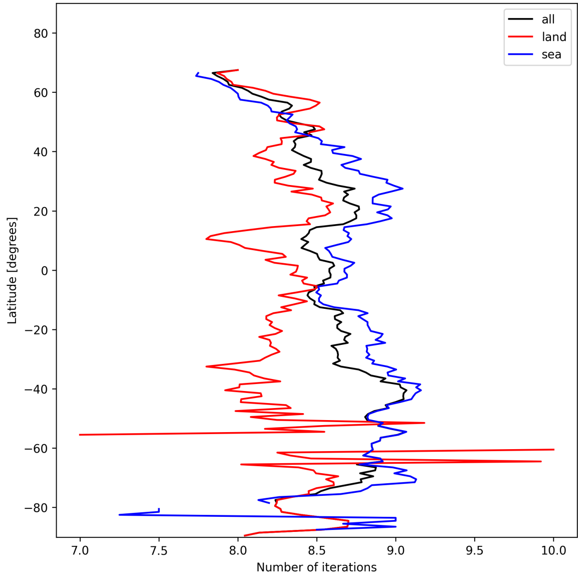
Figure 12: Zonal average of “Number of iterations” for 2025-01-28 to 2025-01-29.
