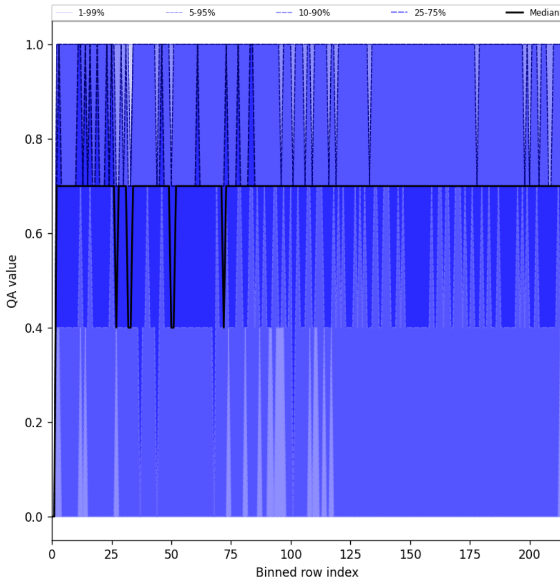
Figure 20: Along track statistics of “QA value” for 2025-01-29 to 2025-01-30
