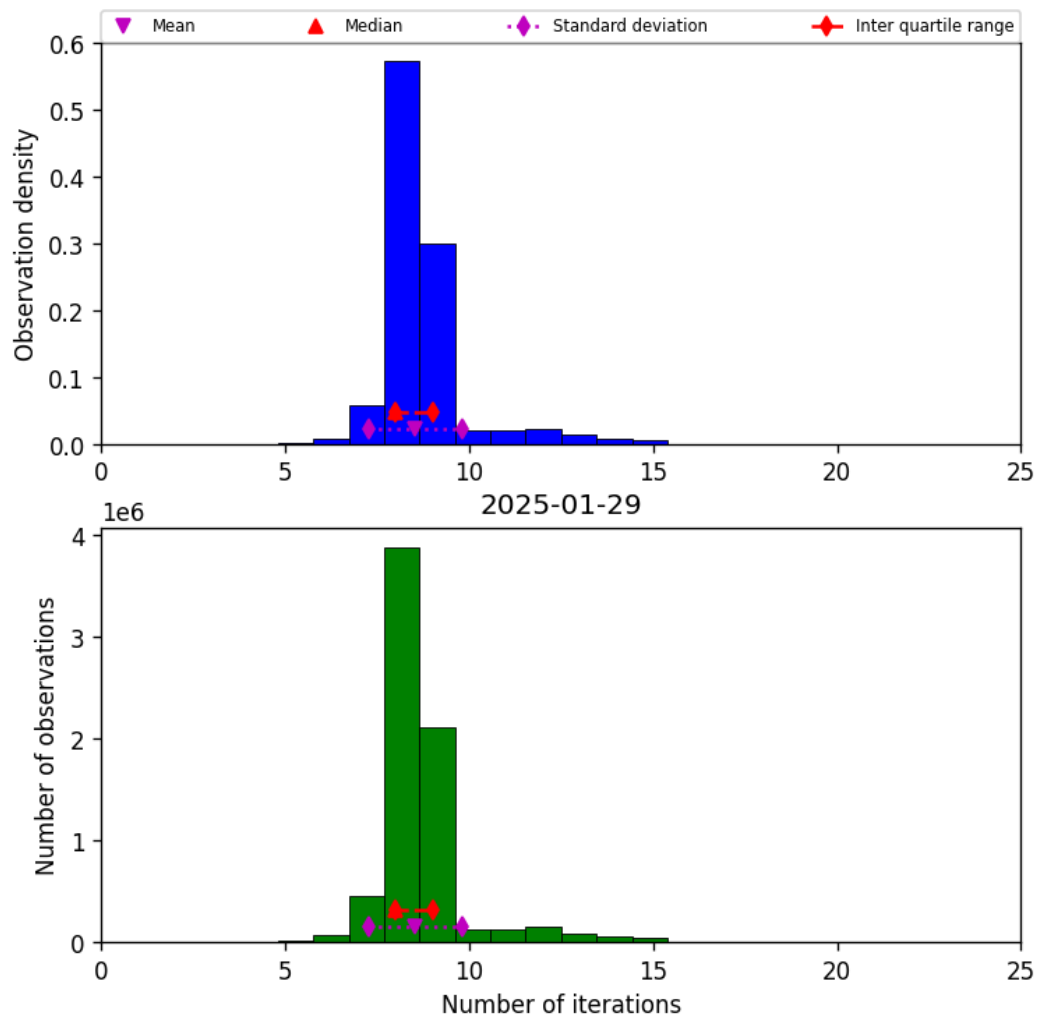
Figure 19: Histogram of “Number of iterations” for 2025-01-29 to 2025-01-30
