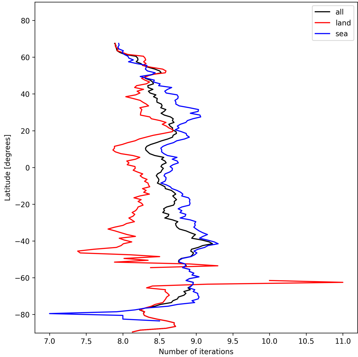
Figure 12: Zonal average of “Number of iterations” for 2025-01-29 to 2025-01-30.
