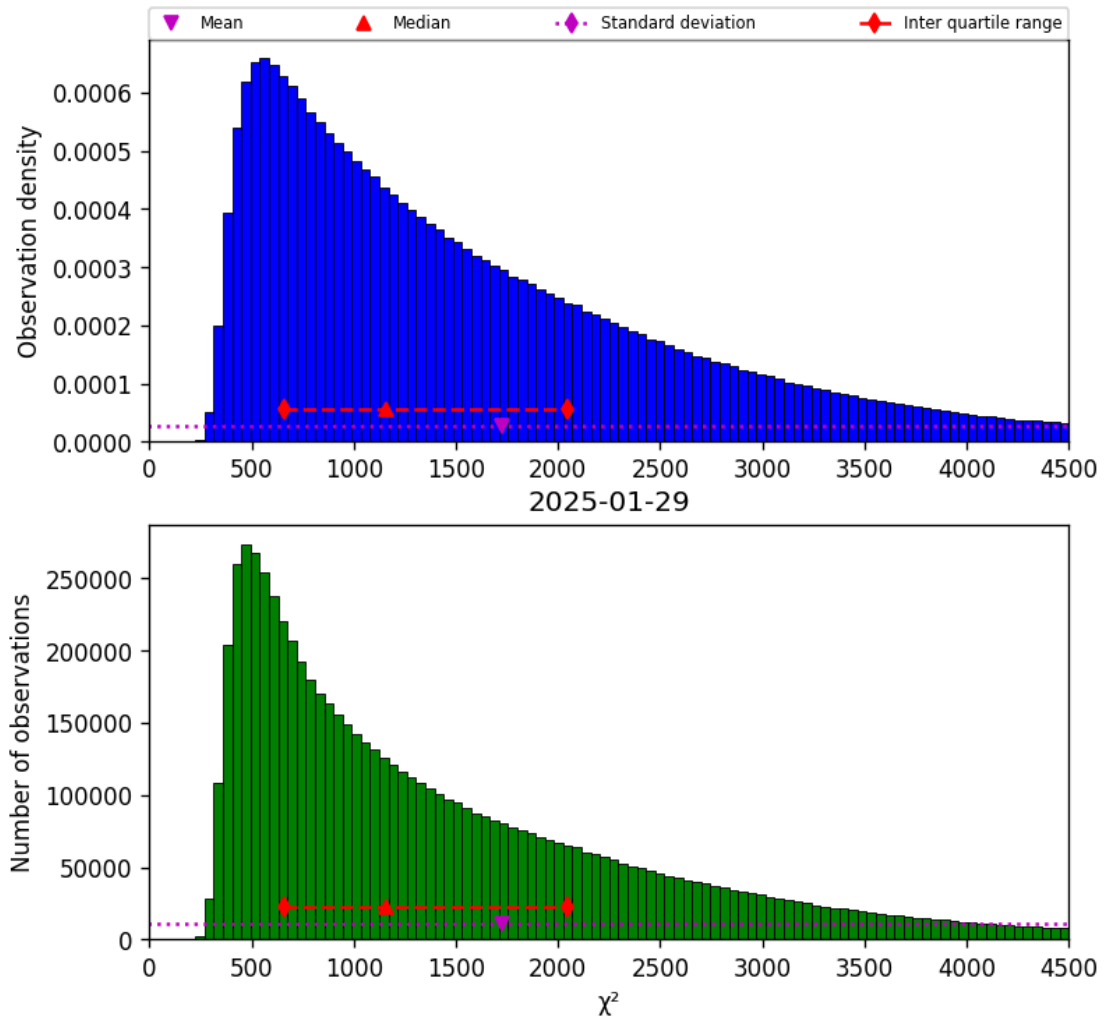
Figure 17: Histogram of “ \chi^2 ” for 2025-01-29 to 2025-01-30
