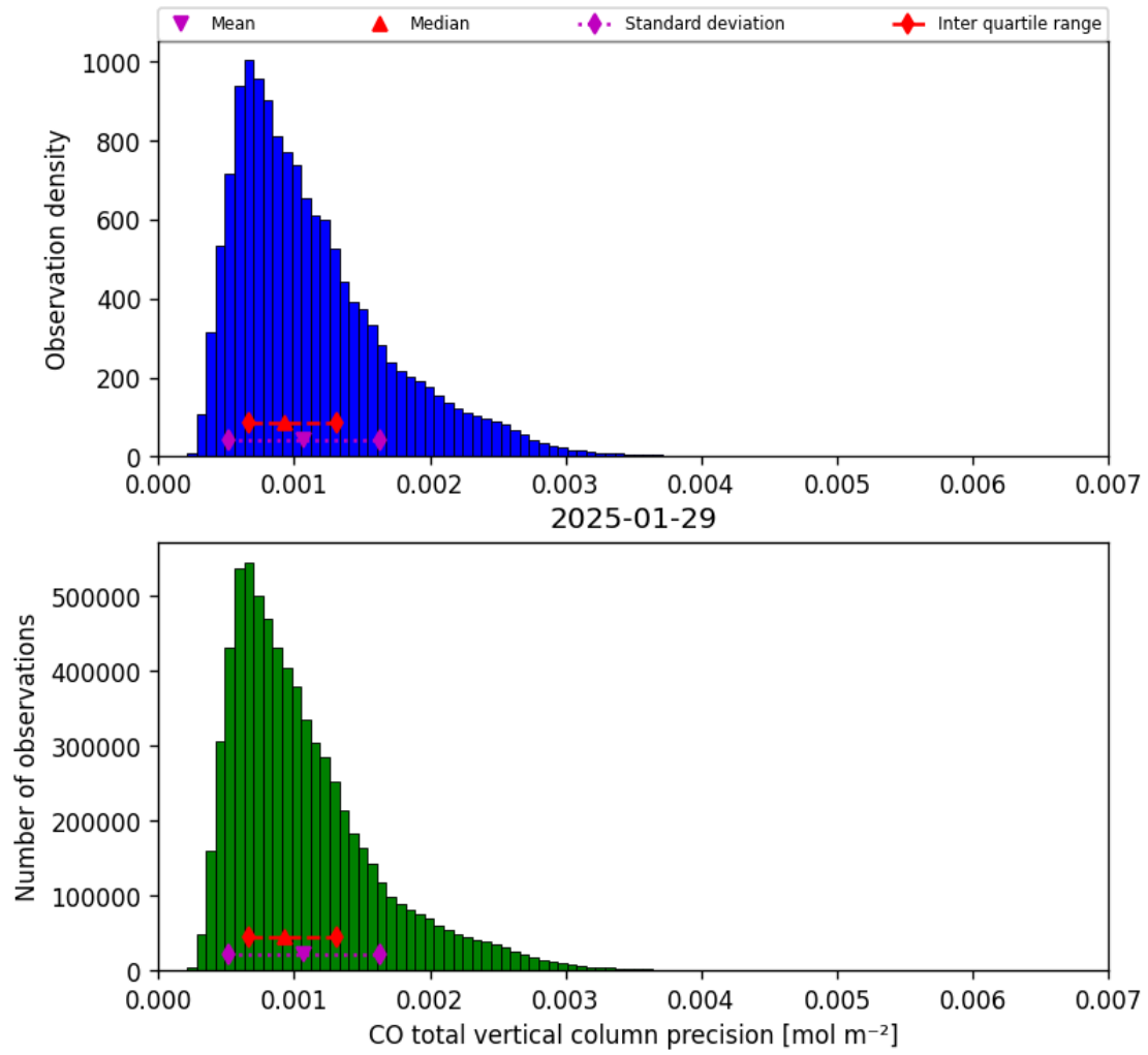
Figure 15: Histogram of “CO total vertical column precision” for 2025-01-29 to 2025-01-30
