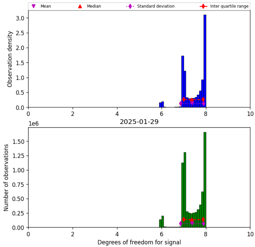
Figure 18: Histogram of “Degrees of freedom for signal” for 2025-01-29 to 2025-01-30
