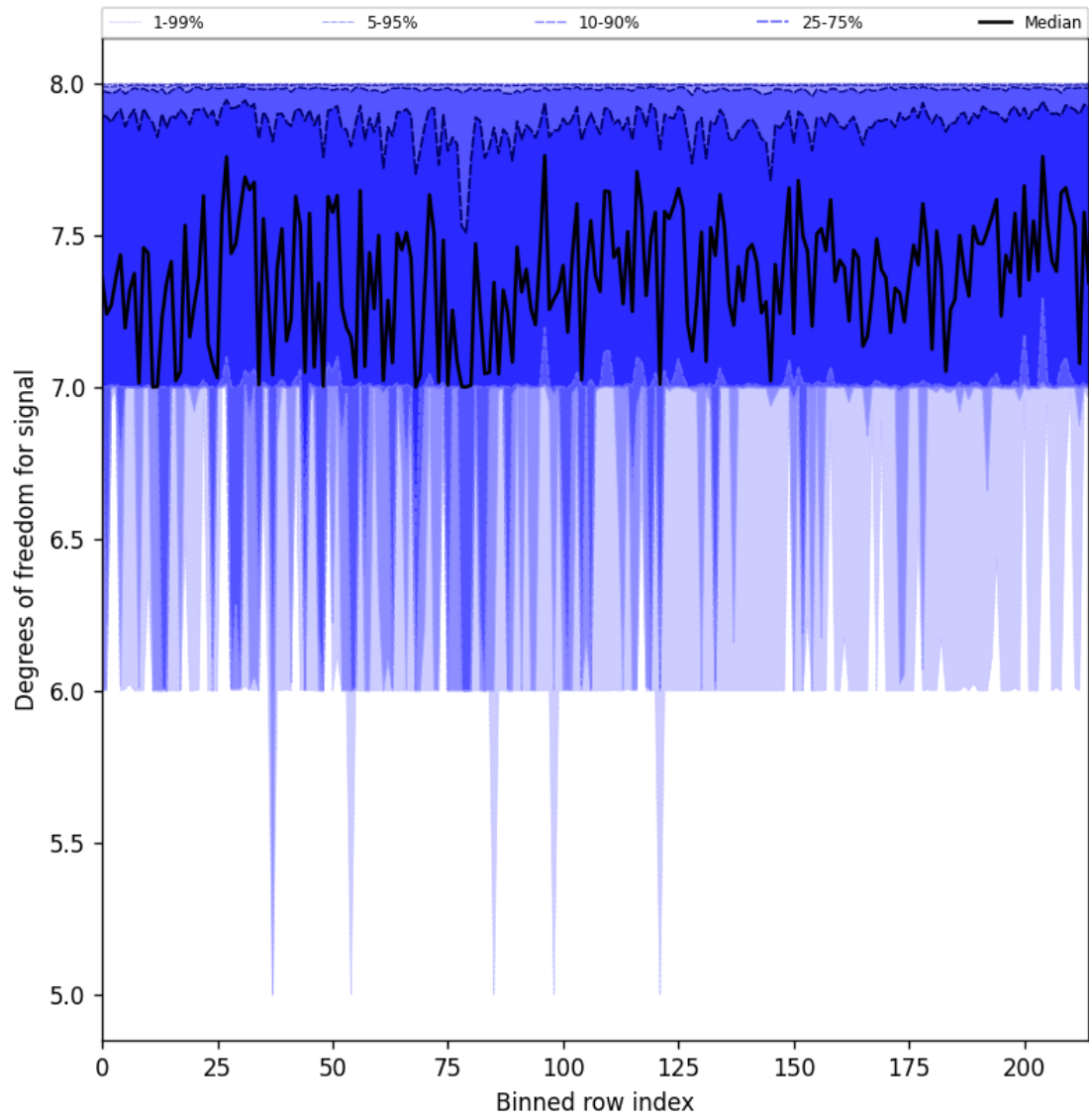
Figure 25: Along track statistics of “Degrees of freedom for signal” for 2025-01-29 to 2025-01-30
