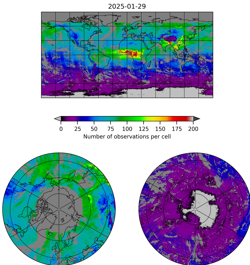
Figure 5: Map of the number of observations for 2025-01-29 to 2025-01-30
