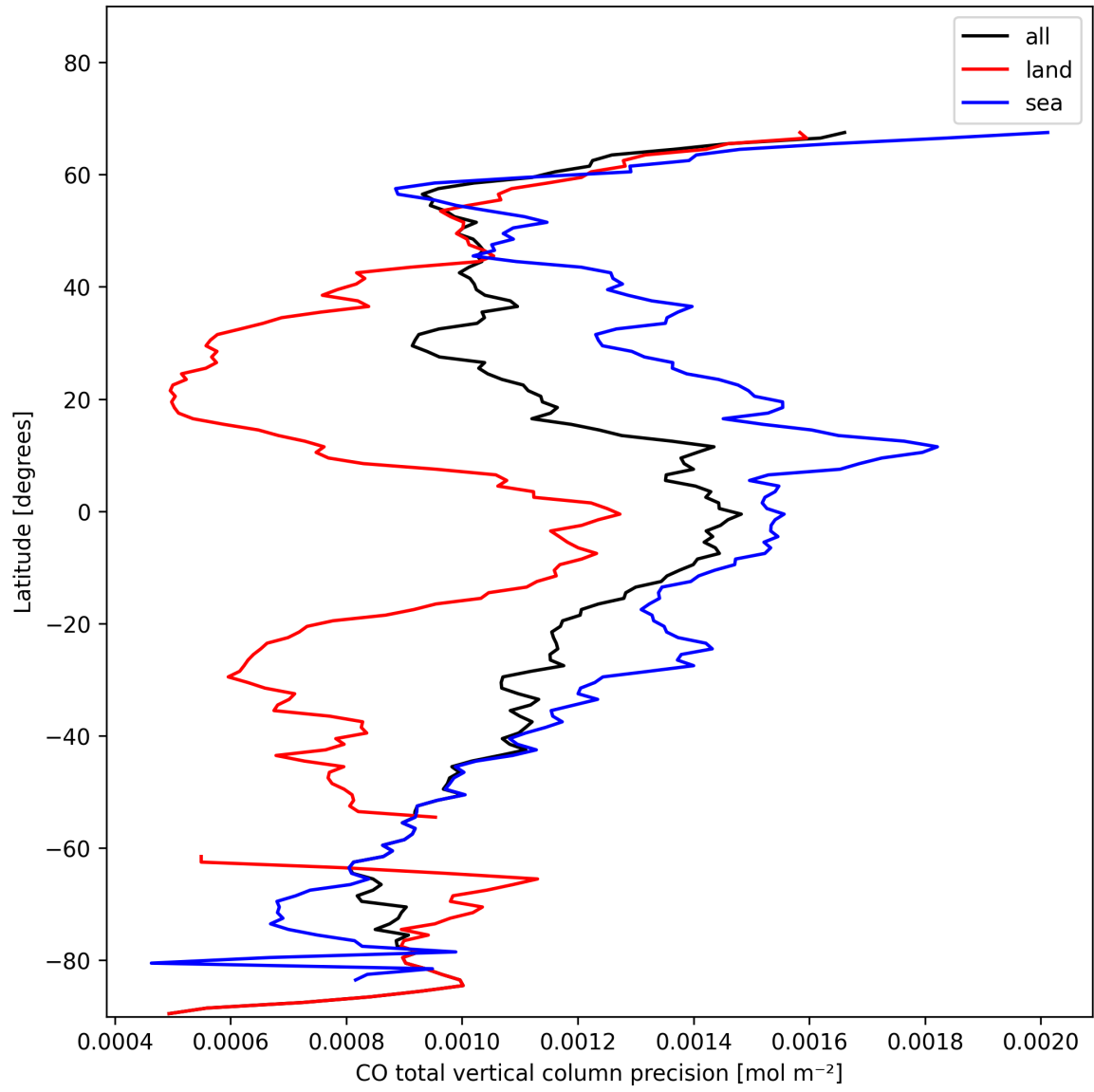
Figure 8: Zonal average of “CO total vertical column precision” for 2025-01-29 to 2025-01-30.
