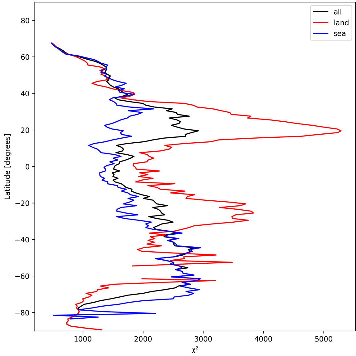
Figure 10: Zonal average of “ \chi^2 ” for 2025-01-29 to 2025-01-30.
