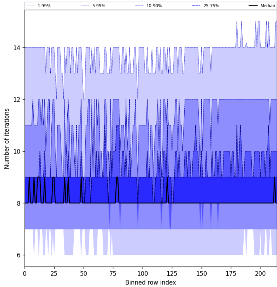
Figure 26: Along track statistics of “Number of iterations” for 2025-01-29 to 2025-01-30
