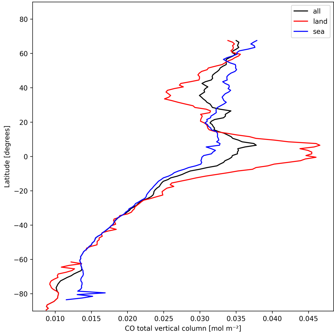
Figure 7: Zonal average of “CO total vertical column” for 2025-01-29 to 2025-01-30.
