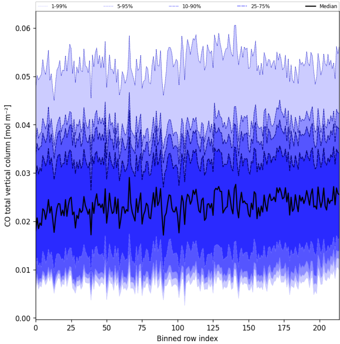
Figure 21: Along track statistics of “CO total vertical column” for 2025-01-29 to 2025-01-30
