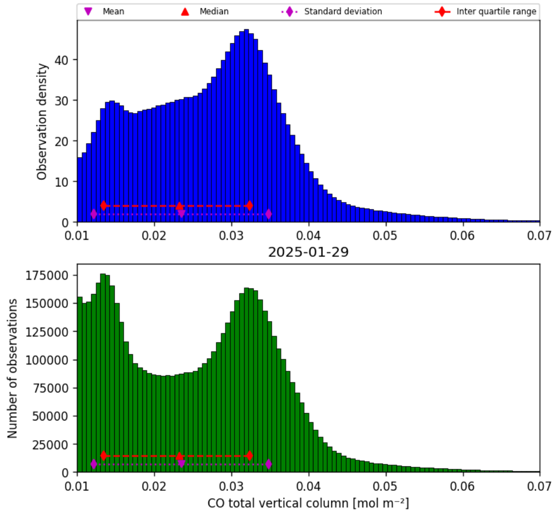
Figure 14: Histogram of “CO total vertical column” for 2025-01-29 to 2025-01-30
