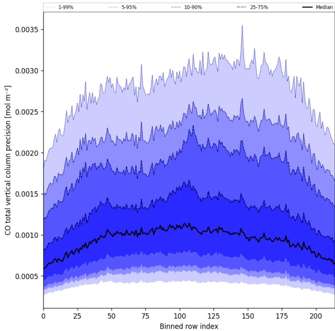
Figure 22: Along track statistics of “CO total vertical column precision” for 2025-01-29 to 2025-01-30
