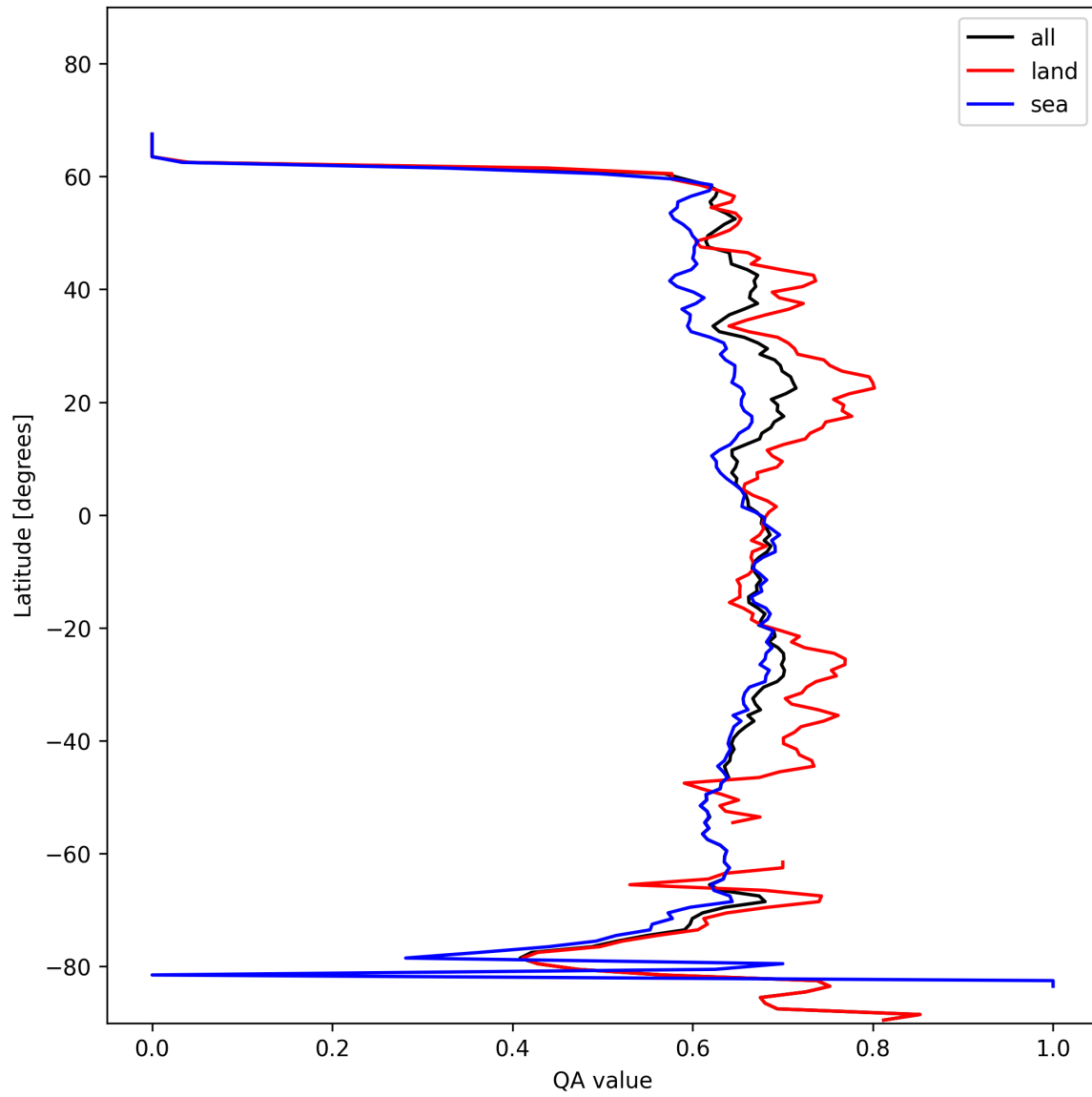
Figure 6: Zonal average of “QA value” for 2025-01-29 to 2025-01-30.
