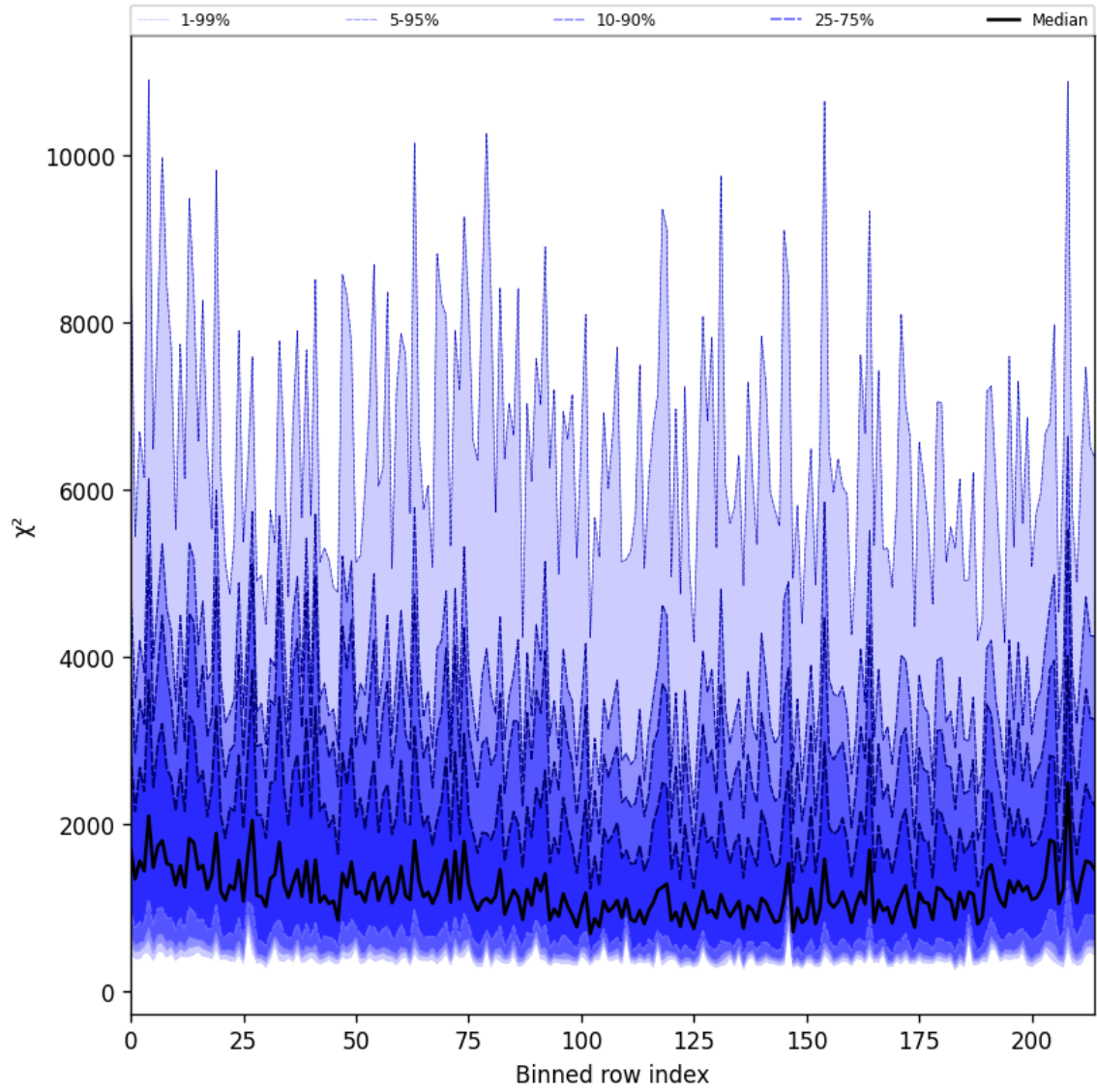
Figure 24: Along track statistics of “ \chi^2 ” for 2025-01-29 to 2025-01-30
