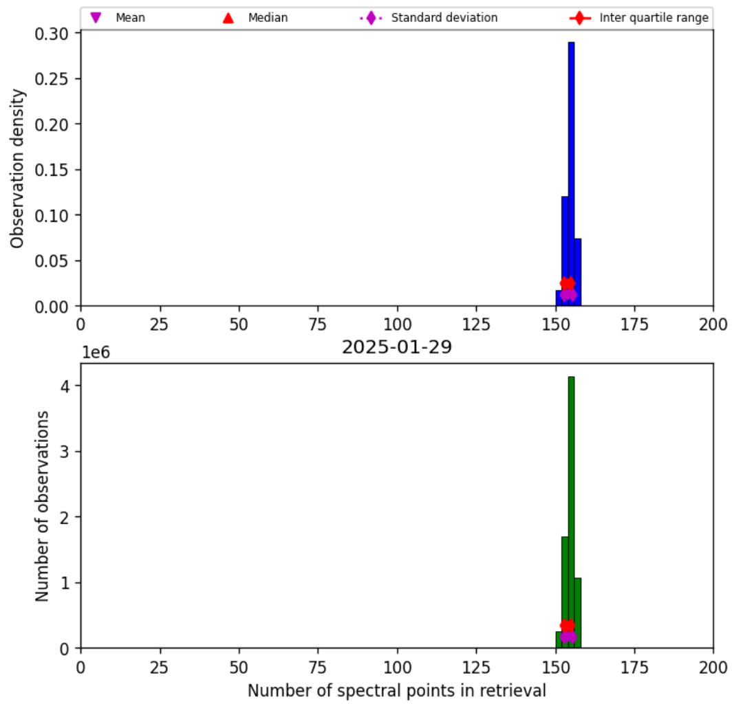
Figure 16: Histogram of “Number of spectral points in retrieval” for 2025-01-29 to 2025-01-30
