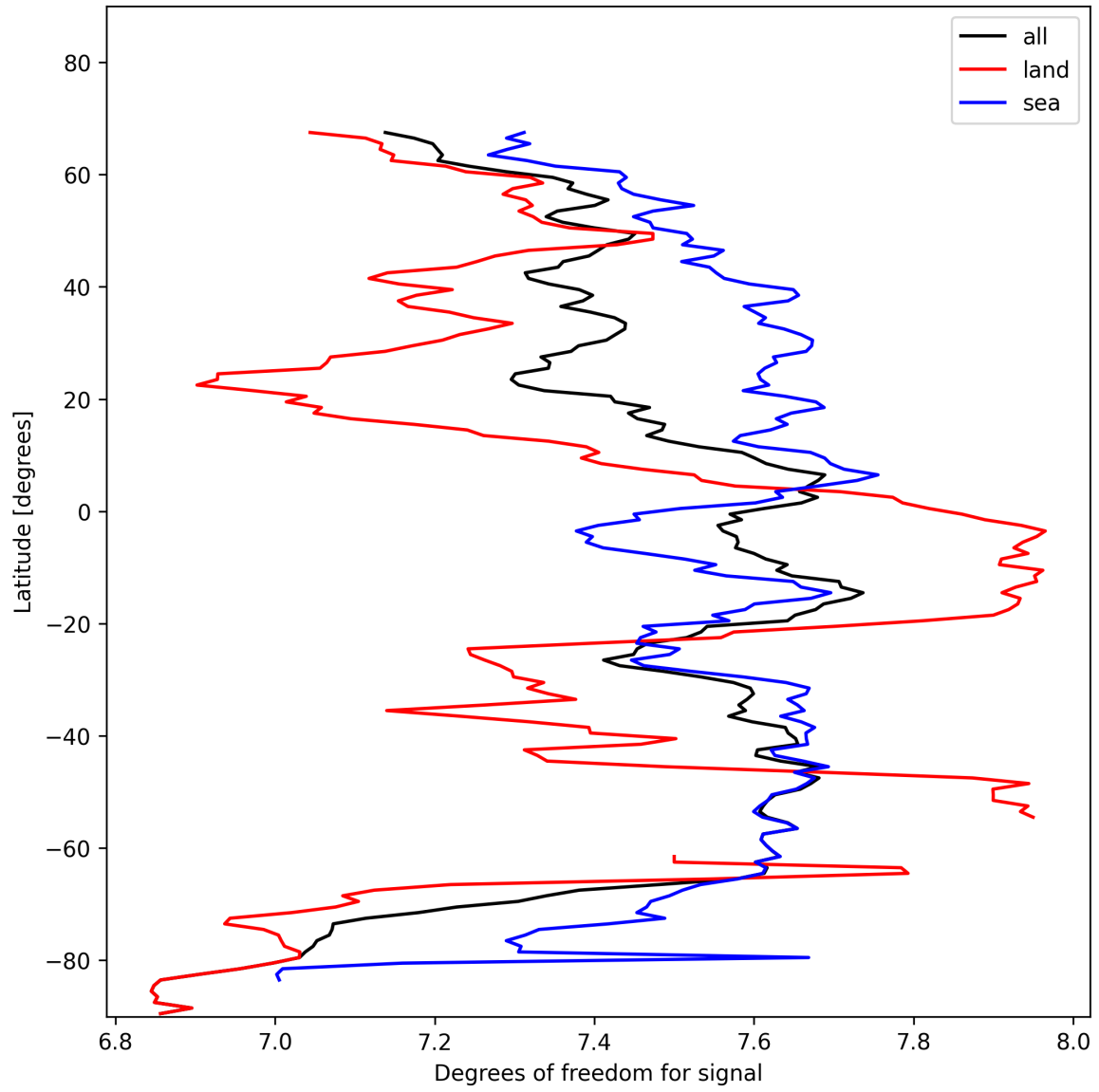
Figure 11: Zonal average of “Degrees of freedom for signal” for 2025-01-29 to 2025-01-30.
