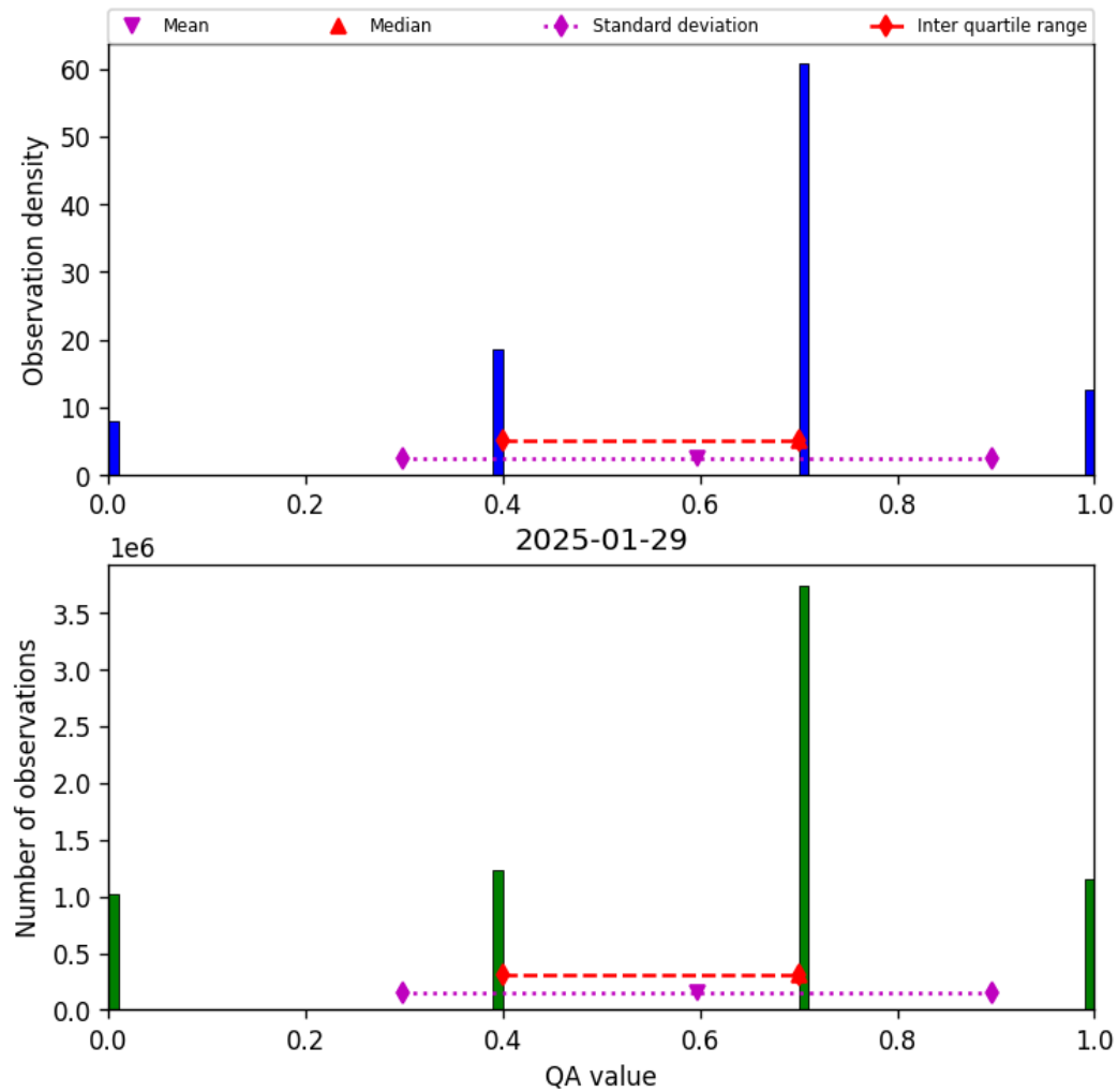
Figure 13: Histogram of “QA value” for 2025-01-29 to 2025-01-30
