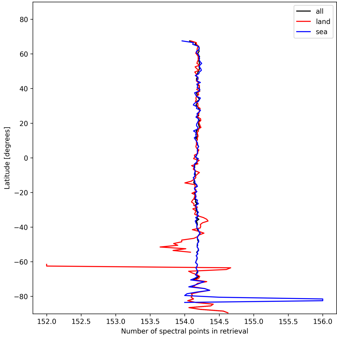
Figure 9: Zonal average of “Number of spectral points in retrieval” for 2025-01-29 to 2025-01-30.
