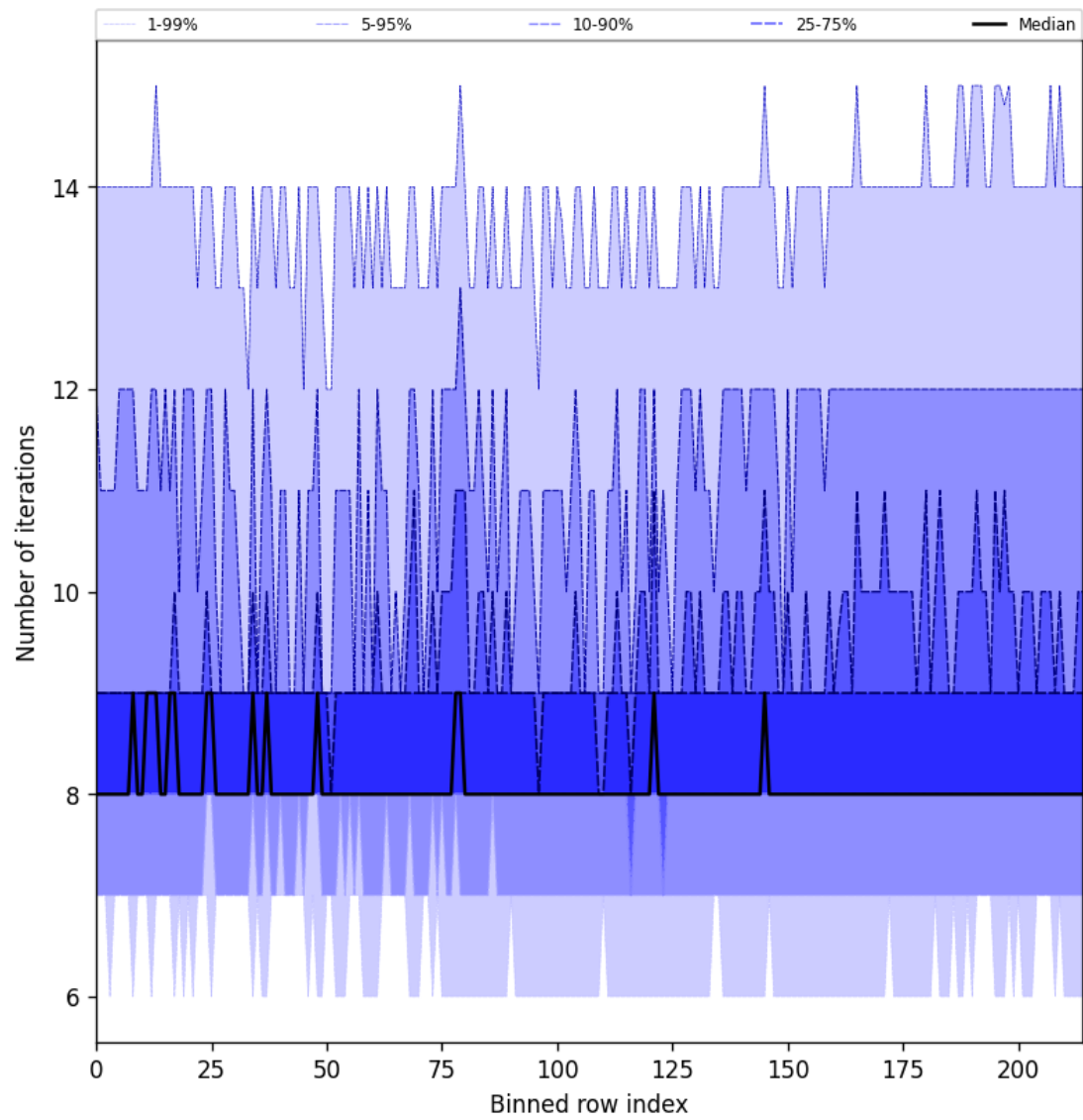
Figure 26: Along track statistics of “Number of iterations” for 2025-01-30 to 2025-01-31
