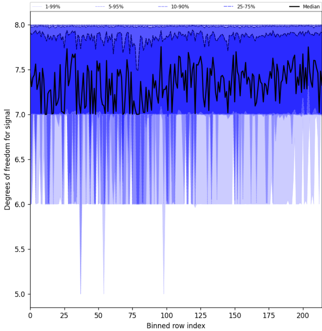
Figure 25: Along track statistics of “Degrees of freedom for signal” for 2025-01-30 to 2025-01-31
