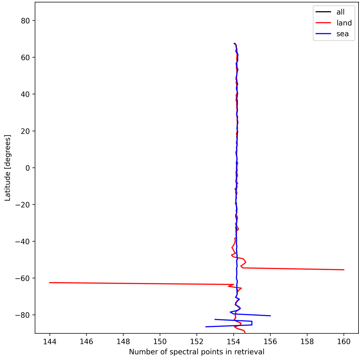
Figure 9: Zonal average of “Number of spectral points in retrieval” for 2025-01-30 to 2025-01-31.
