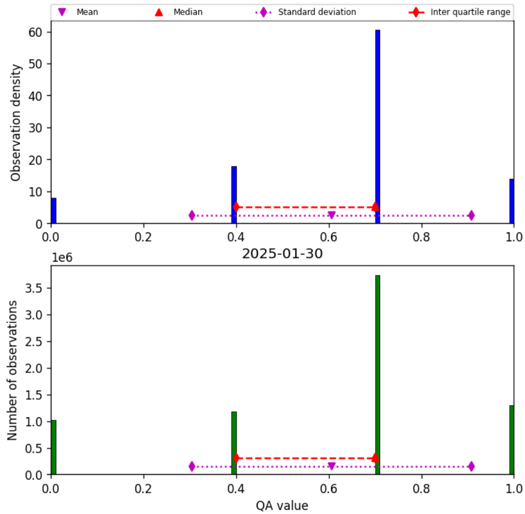
Figure 13: Histogram of “QA value” for 2025-01-30 to 2025-01-31
