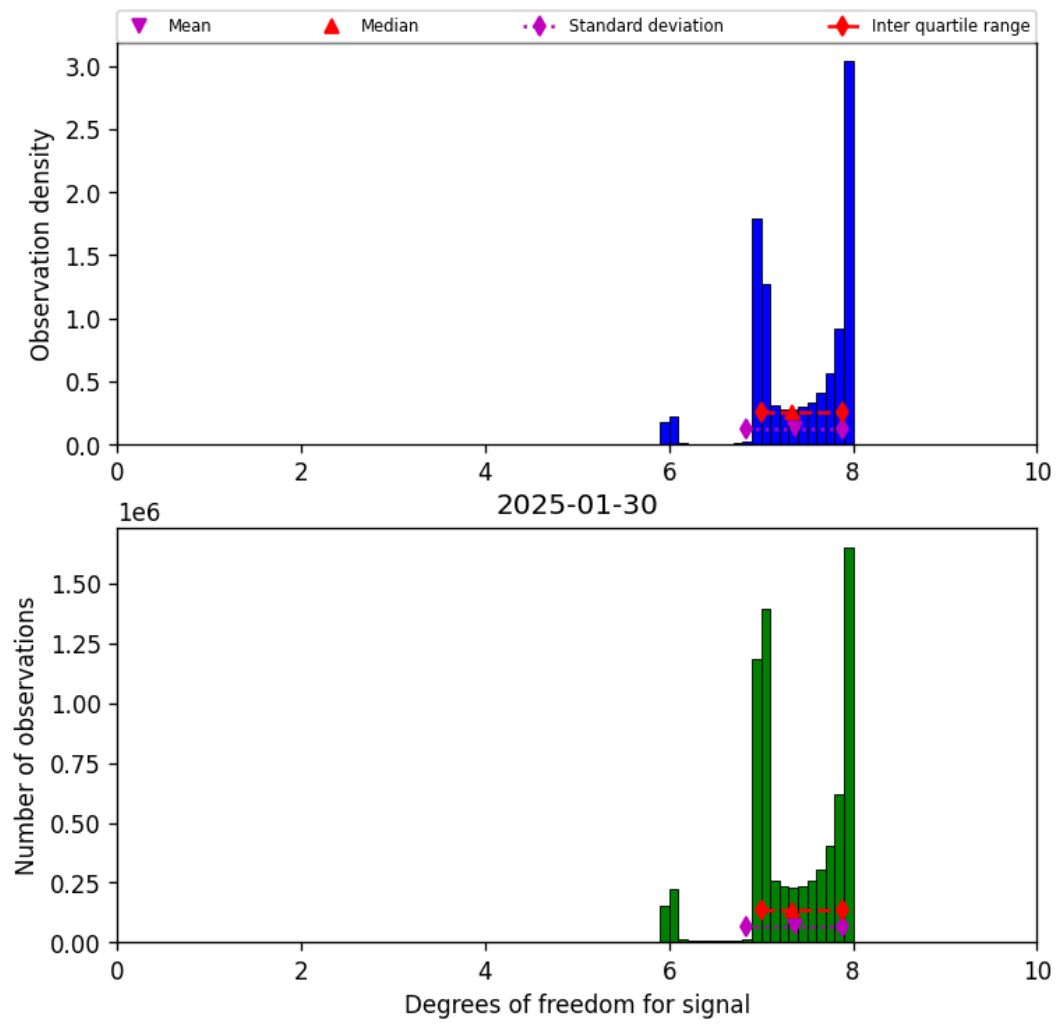
Figure 18: Histogram of “Degrees of freedom for signal” for 2025-01-30 to 2025-01-31
