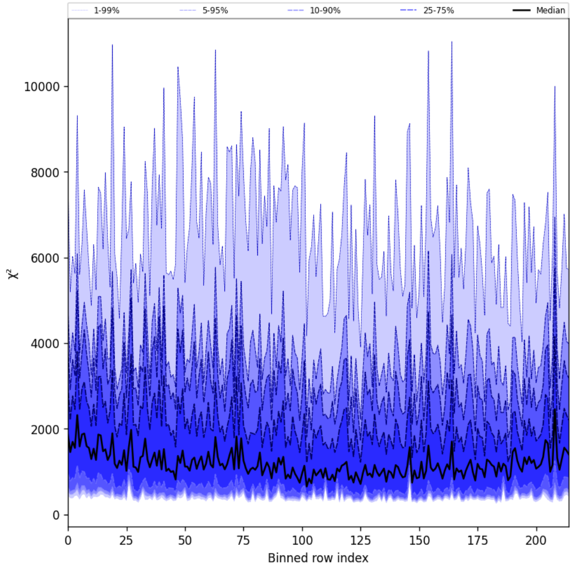
Figure 24: Along track statistics of “ \chi^2 ” for 2025-01-30 to 2025-01-31
