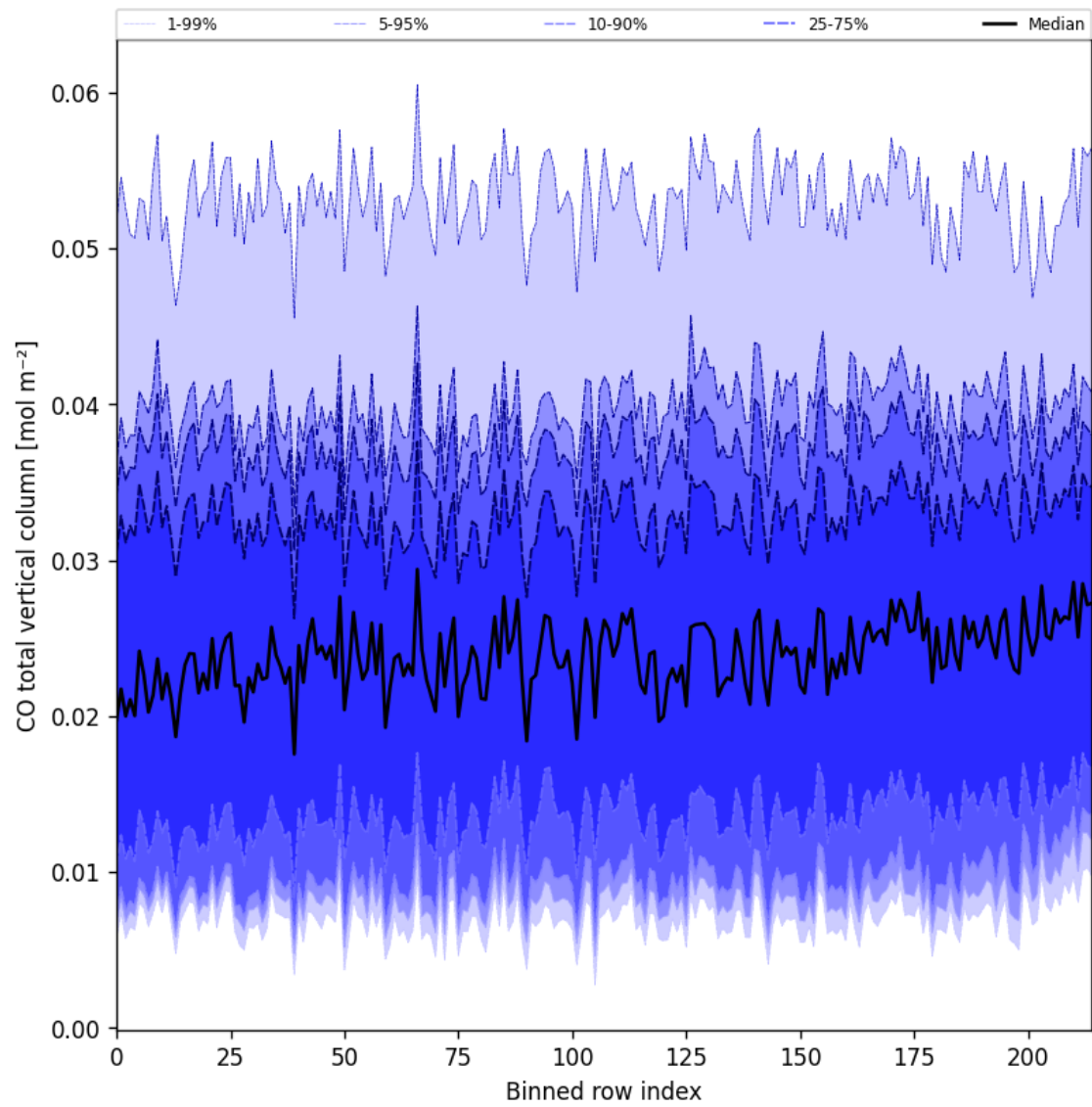
Figure 21: Along track statistics of “CO total vertical column” for 2025-01-30 to 2025-01-31
