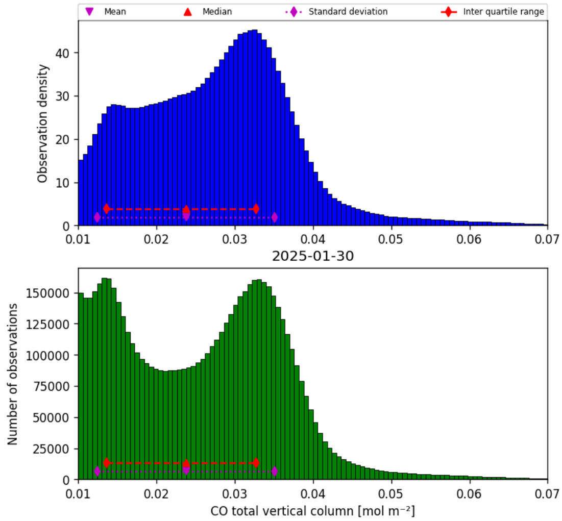
Figure 14: Histogram of “CO total vertical column” for 2025-01-30 to 2025-01-31
