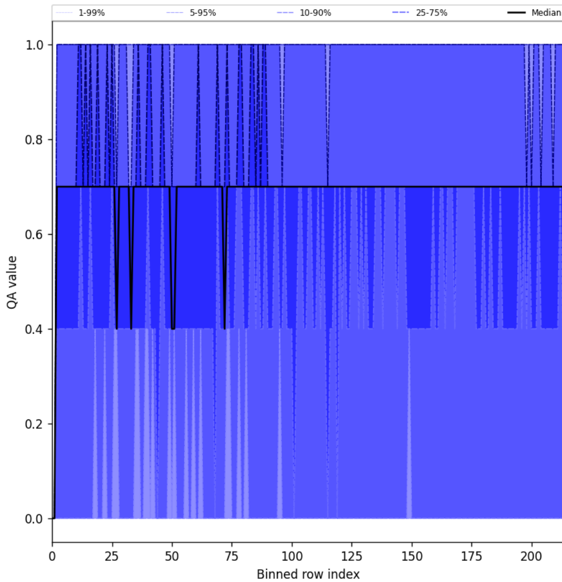
Figure 20: Along track statistics of “QA value” for 2025-01-30 to 2025-01-31
