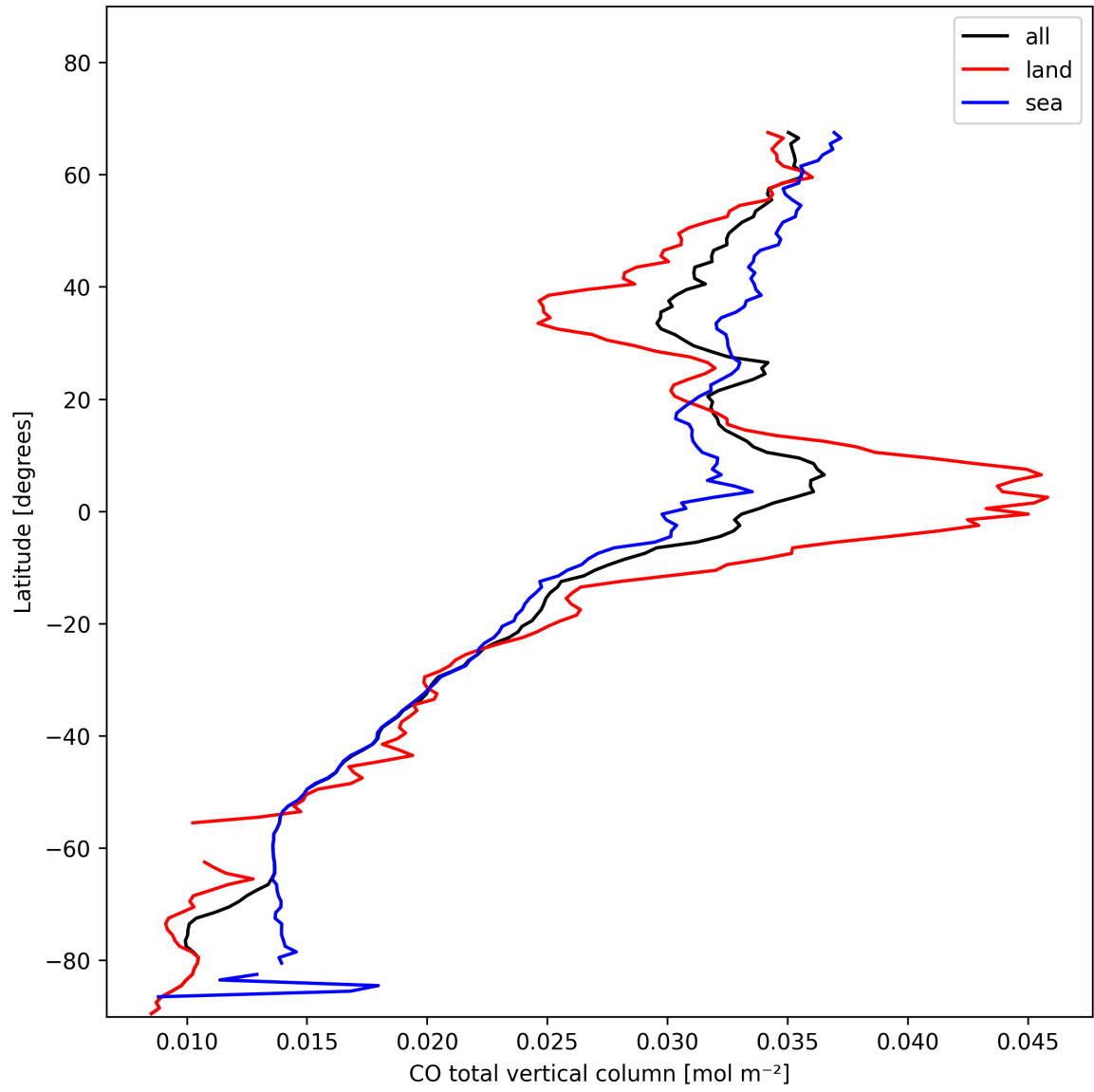
Figure 7: Zonal average of “CO total vertical column” for 2025-01-30 to 2025-01-31.
