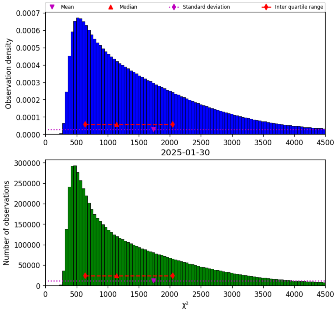
Figure 17: Histogram of " \chi^2 " for 2025-01-30 to 2025-01-31
