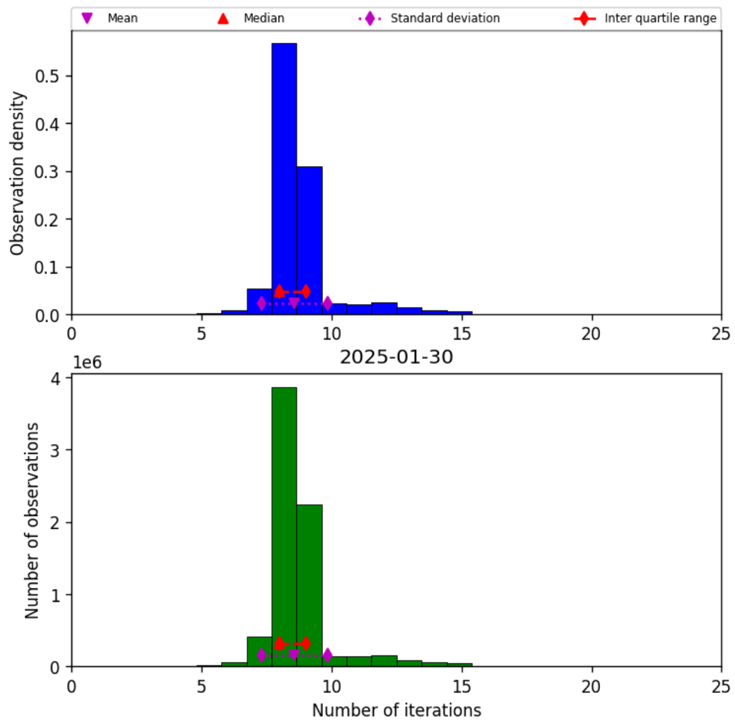
Figure 19: Histogram of “Number of iterations” for 2025-01-30 to 2025-01-31
