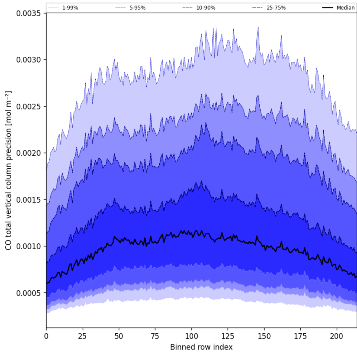
Figure 22: Along track statistics of “CO total vertical column precision” for 2025-01-30 to 2025-01-31
