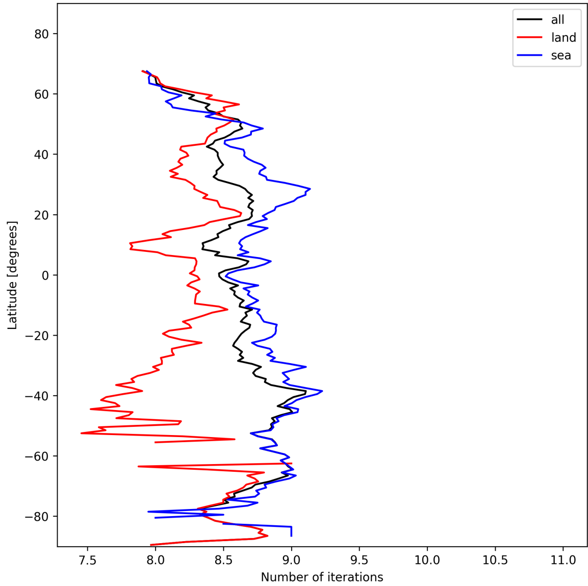
Figure 12: Zonal average of “Number of iterations” for 2025-01-30 to 2025-01-31.
