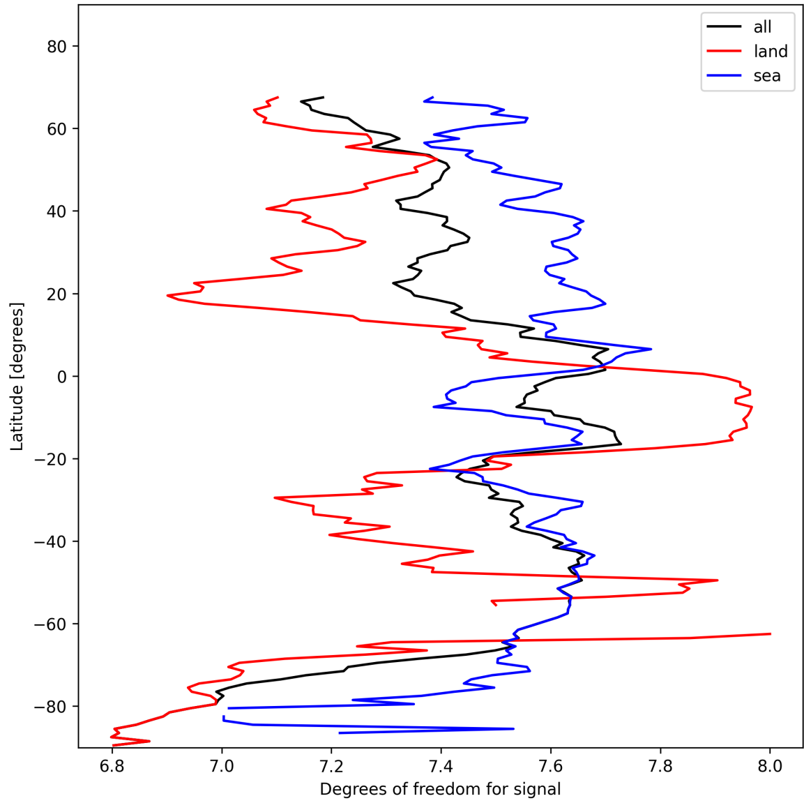
Figure 11: Zonal average of “Degrees of freedom for signal” for 2025-01-30 to 2025-01-31.
