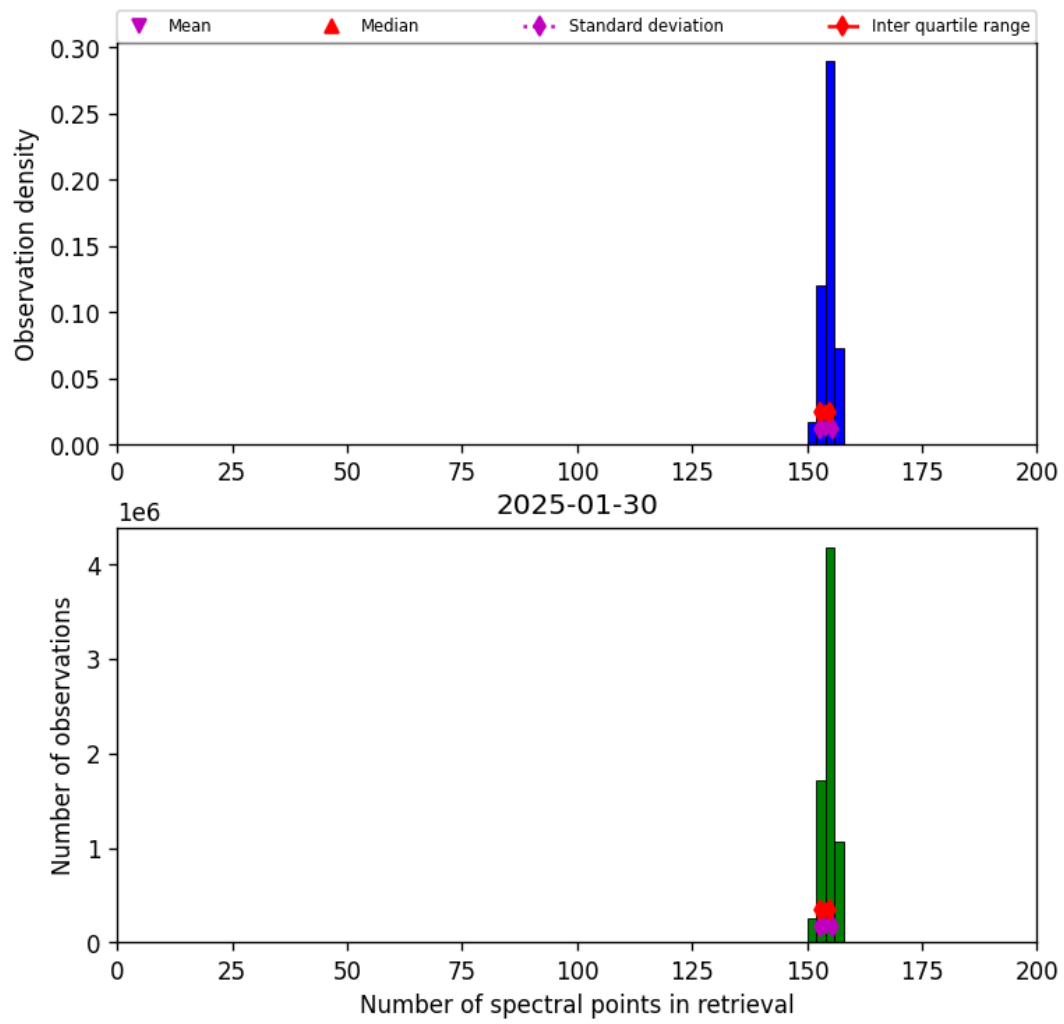
Figure 16: Histogram of “Number of spectral points in retrieval” for 2025-01-30 to 2025-01-31
