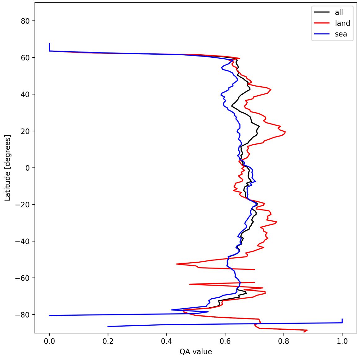
Figure 6: Zonal average of “QA value” for 2025-01-30 to 2025-01-31.
