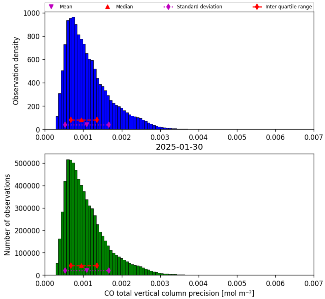
Figure 15: Histogram of “CO total vertical column precision” for 2025-01-30 to 2025-01-31
