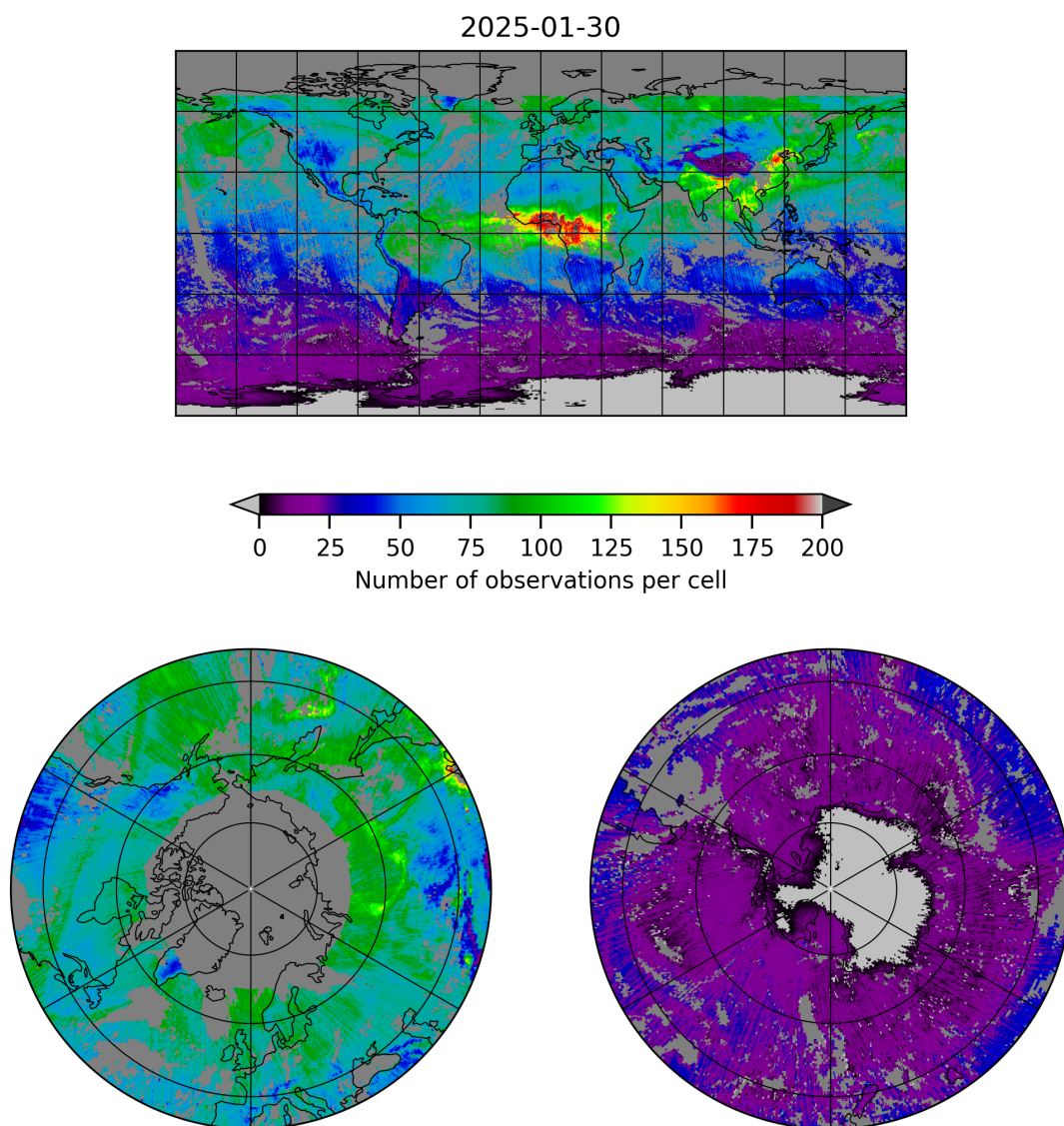
Figure 5: Map of the number of observations for 2025-01-30 to 2025-01-31
