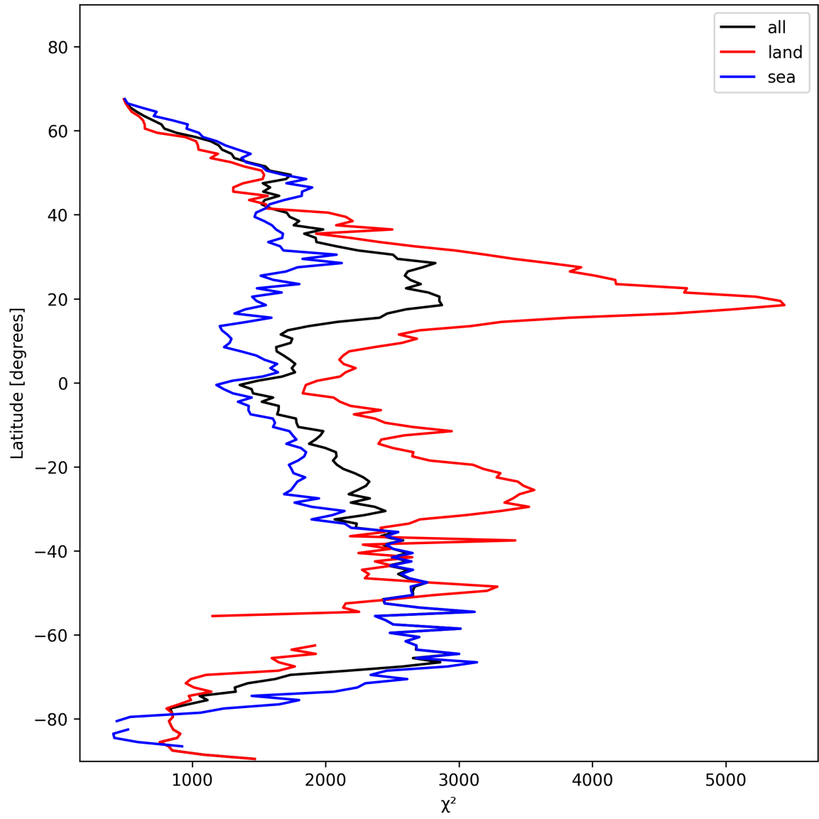
Figure 10: Zonal average of “ \chi^2 ” for 2025-01-30 to 2025-01-31.
