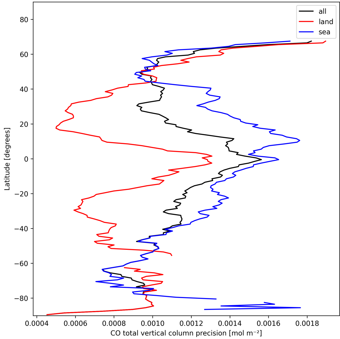
Figure 8: Zonal average of “CO total vertical column precision” for 2025-01-30 to 2025-01-31.
