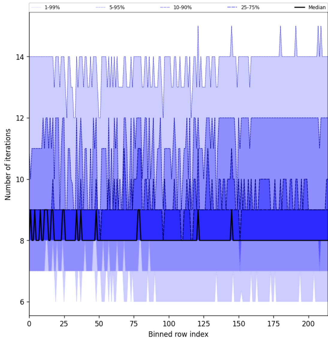
Figure 26: Along track statistics of “Number of iterations” for 2025-01-31 to 2025-01-31
