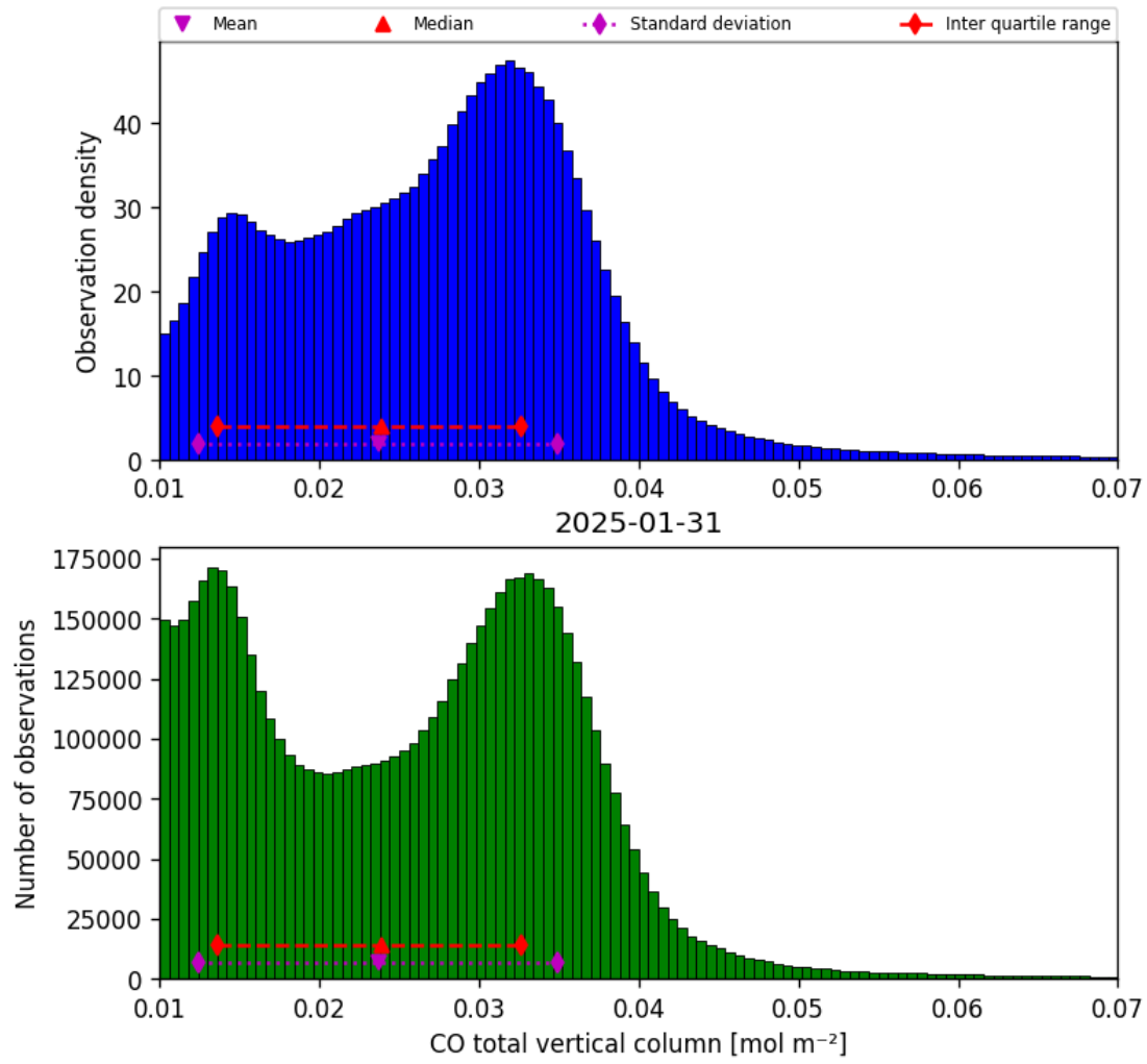
Figure 14: Histogram of “CO total vertical column” for 2025-01-31 to 2025-01-31
