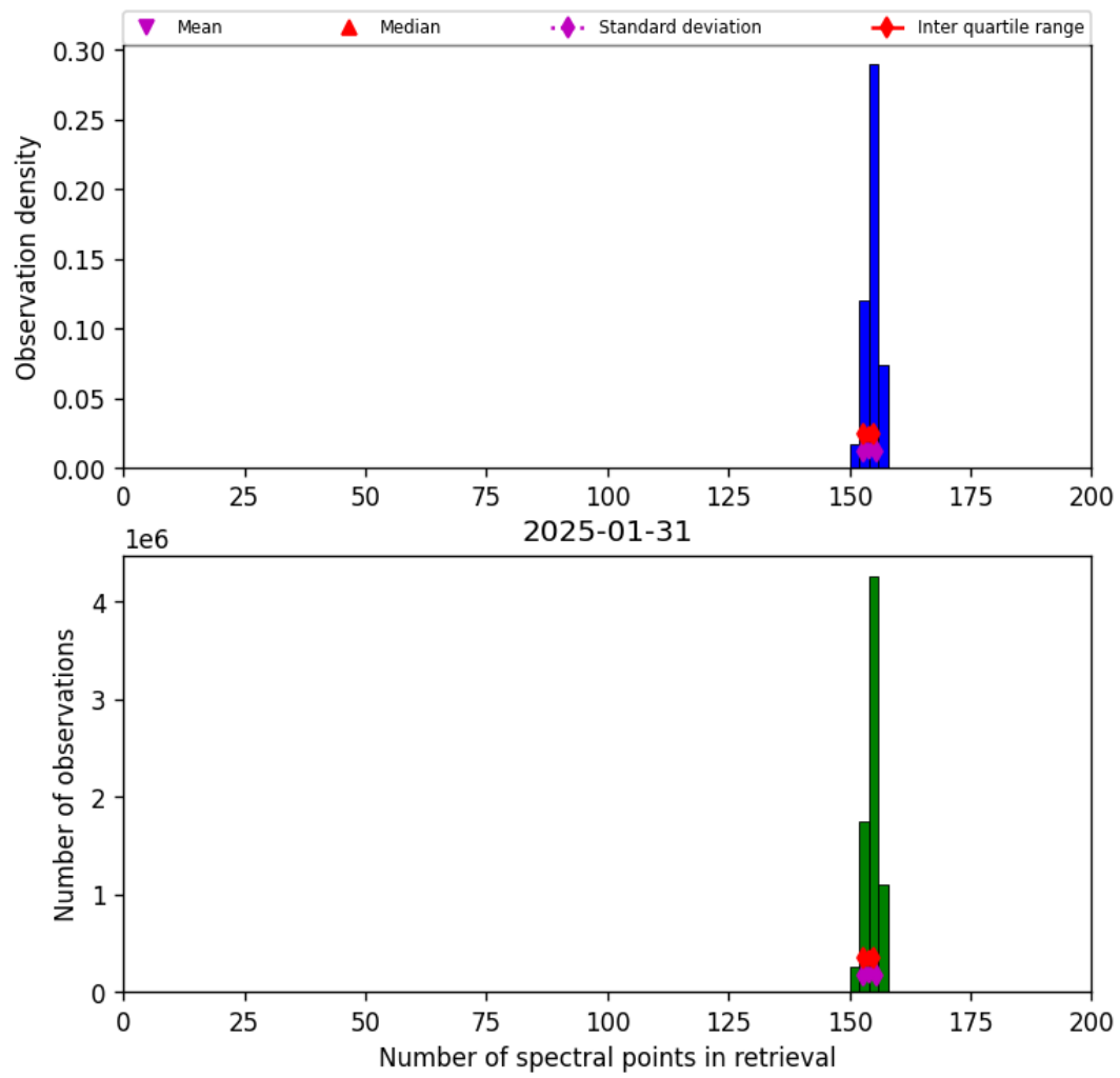
Figure 16: Histogram of “Number of spectral points in retrieval” for 2025-01-31 to 2025-01-31
