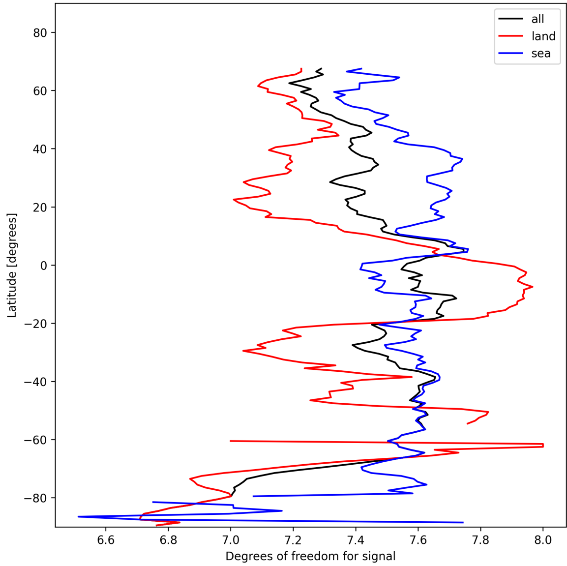
Figure 11: Zonal average of “Degrees of freedom for signal” for 2025-01-31 to 2025-01-31.
