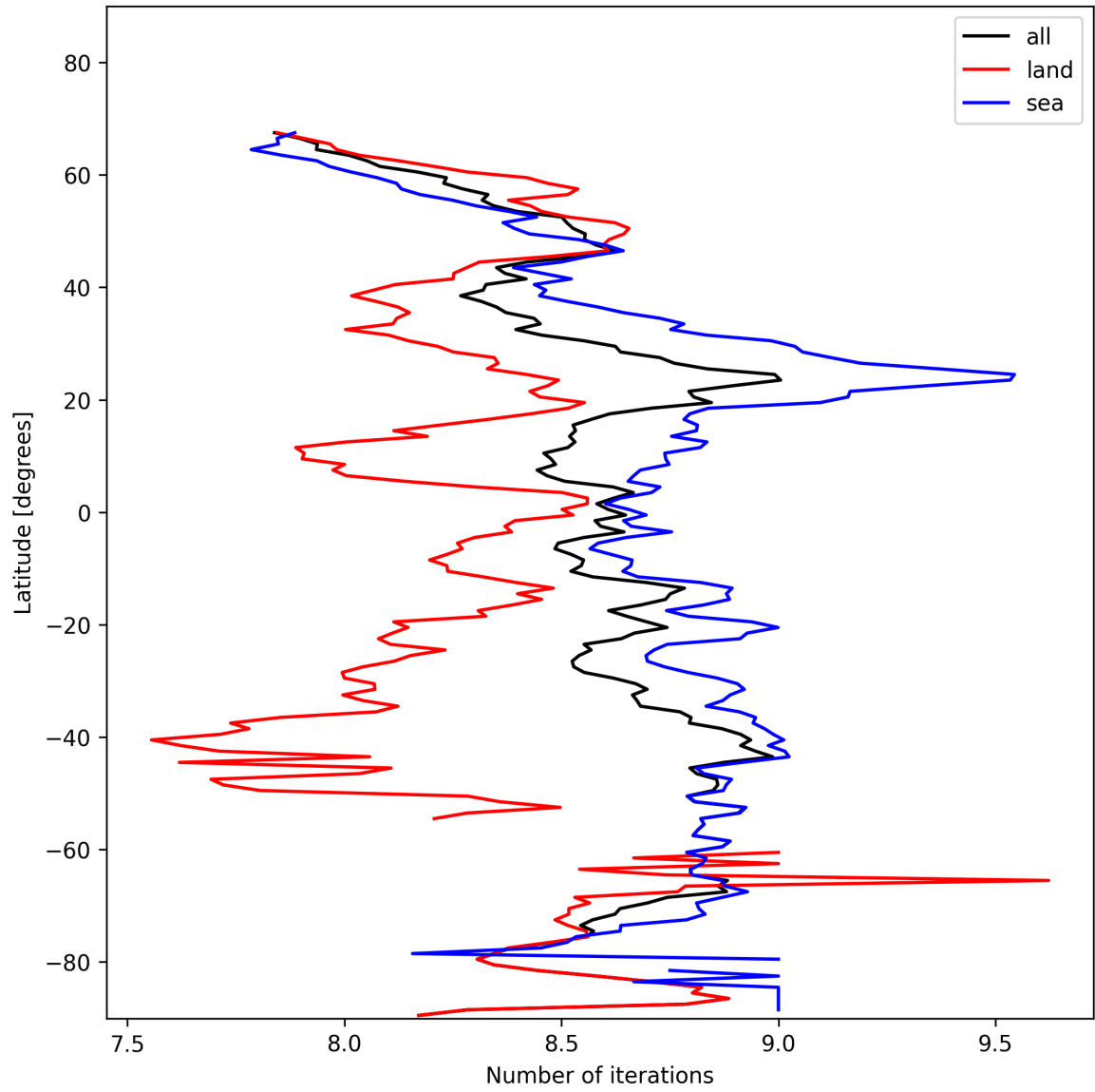
Figure 12: Zonal average of “Number of iterations” for 2025-01-31 to 2025-01-31.
