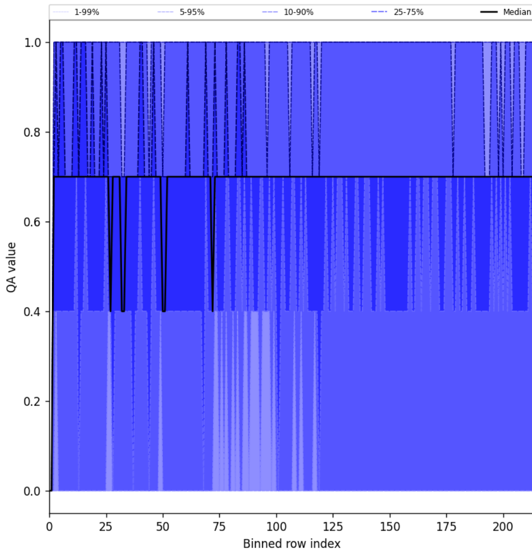
Figure 20: Along track statistics of “QA value” for 2025-01-31 to 2025-01-31
