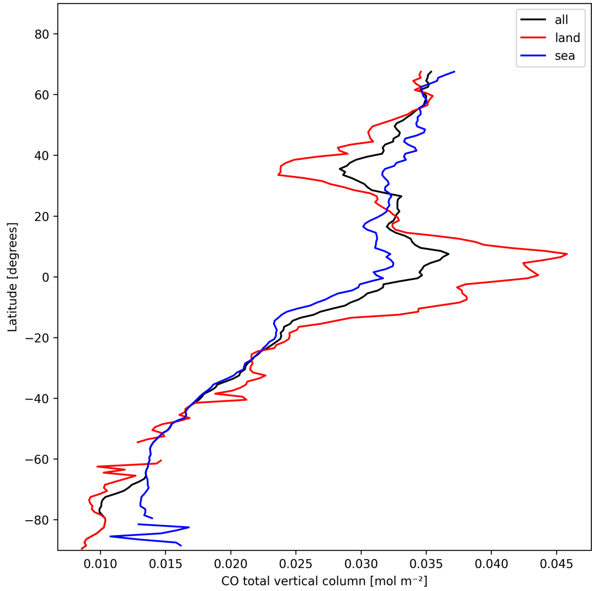
Figure 7: Zonal average of “CO total vertical column” for 2025-01-31 to 2025-01-31.
