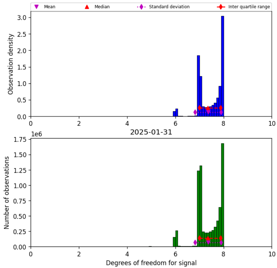
Figure 18: Histogram of “Degrees of freedom for signal” for 2025-01-31 to 2025-01-31
