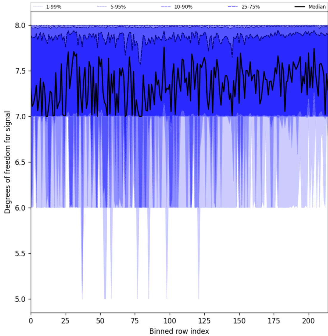
Figure 25: Along track statistics of “Degrees of freedom for signal” for 2025-01-31 to 2025-01-31
