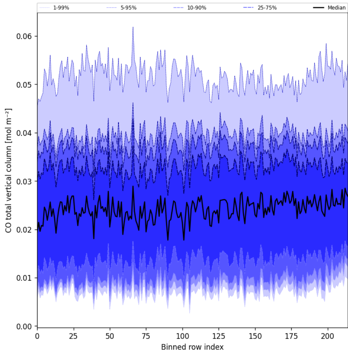
Figure 21: Along track statistics of “CO total vertical column” for 2025-01-31 to 2025-01-31
