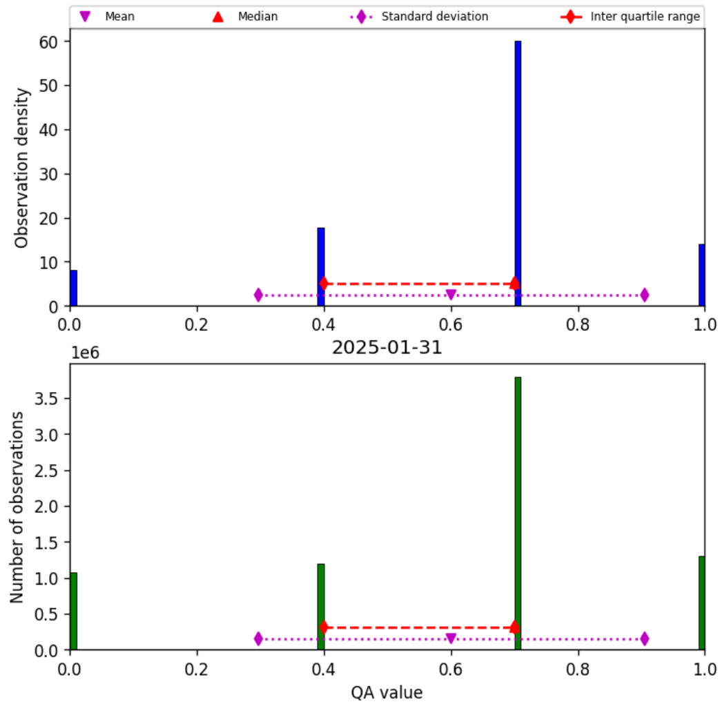
Figure 13: Histogram of “QA value” for 2025-01-31 to 2025-01-31
