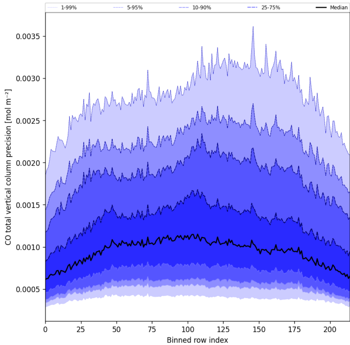
Figure 22: Along track statistics of “CO total vertical column precision” for 2025-01-31 to 2025-01-31
