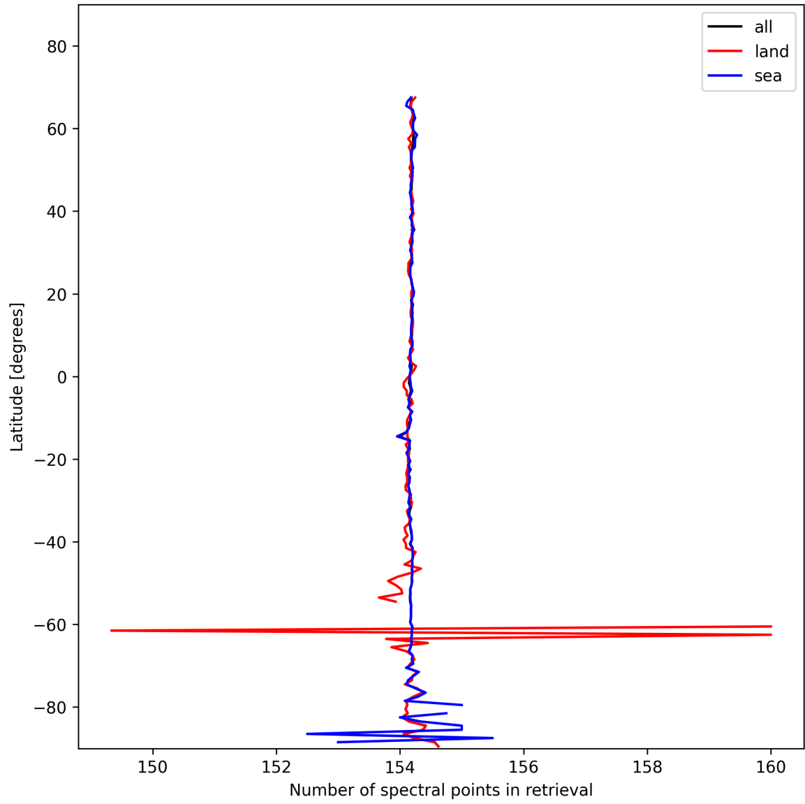
Figure 9: Zonal average of “Number of spectral points in retrieval” for 2025-01-31 to 2025-01-31.
