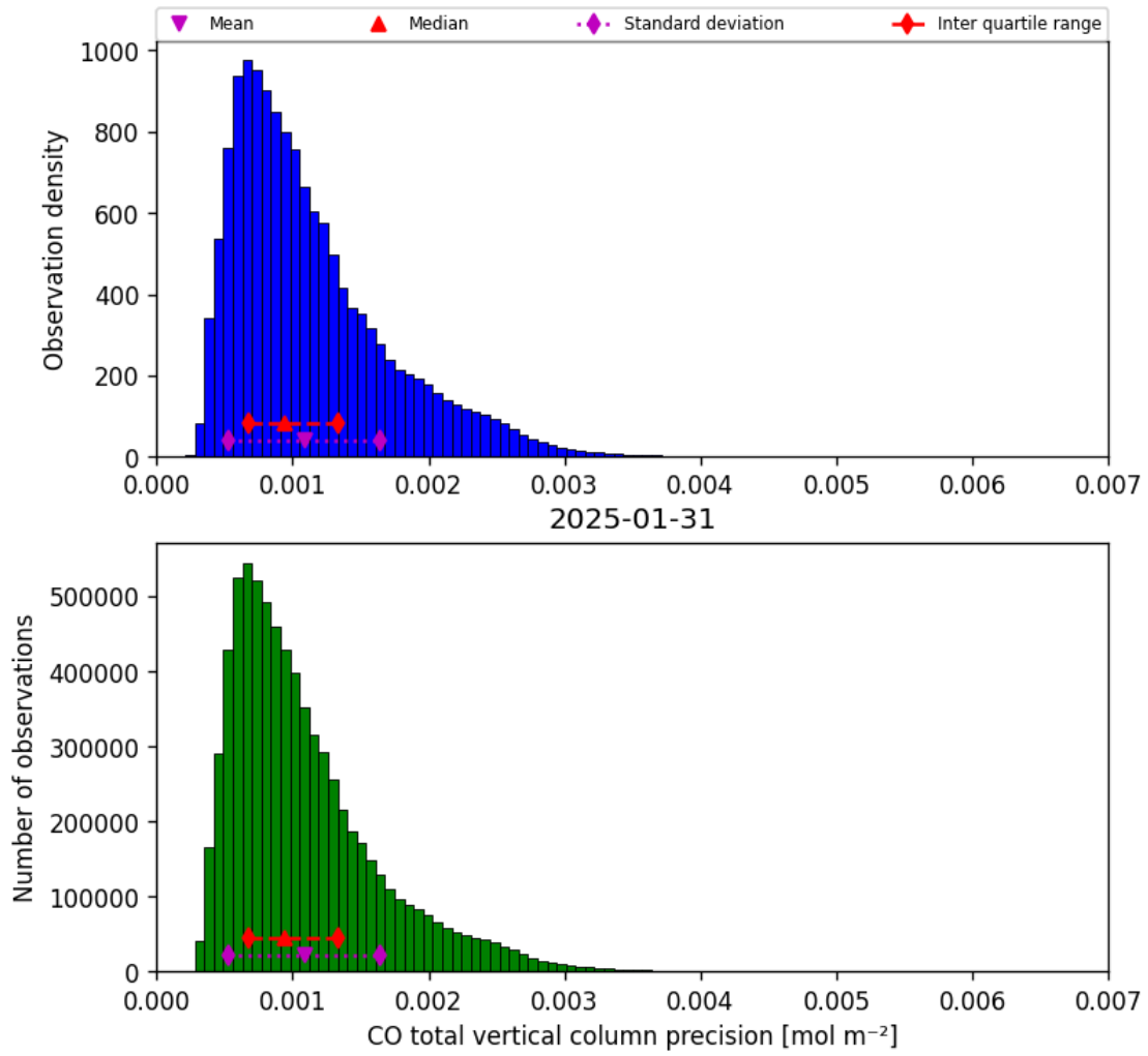
Figure 15: Histogram of “CO total vertical column precision” for 2025-01-31 to 2025-01-31
