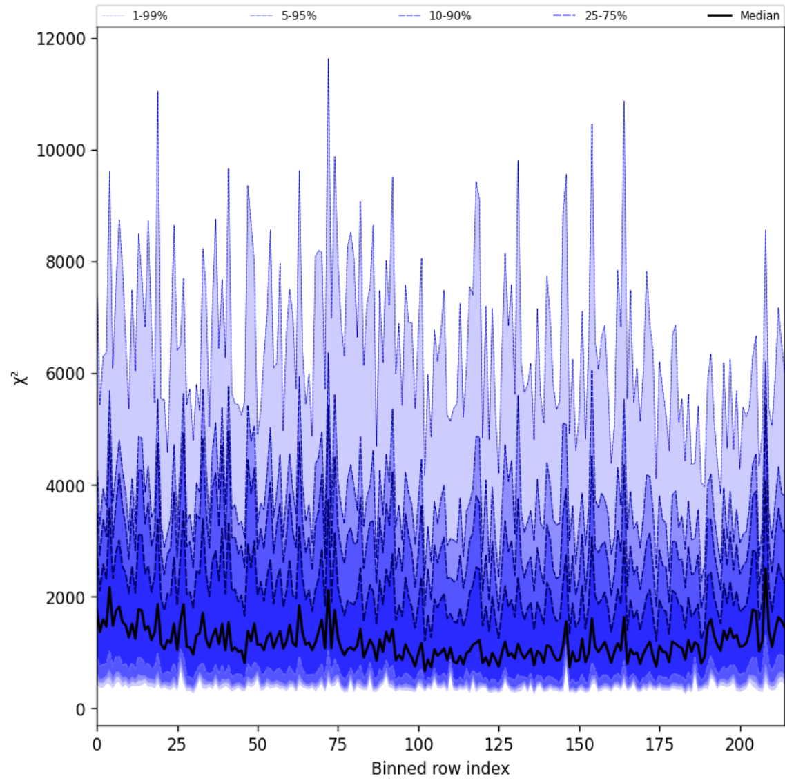
Figure 24: Along track statistics of “ \chi^2 ” for 2025-01-31 to 2025-01-31
