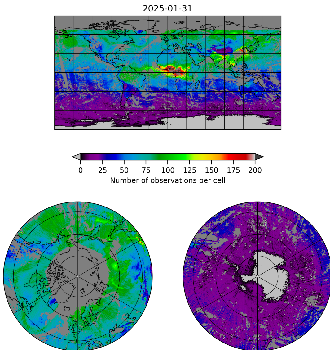
Figure 5: Map of the number of observations for 2025-01-31 to 2025-01-31
