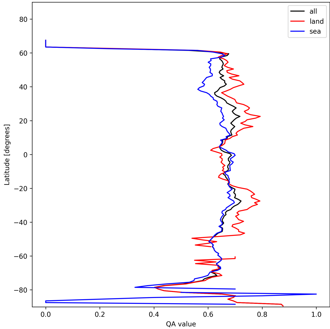
Figure 6: Zonal average of “QA value” for 2025-01-31 to 2025-01-31.
