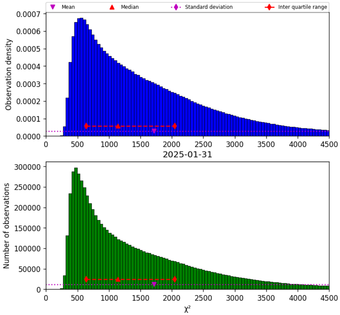
Figure 17: Histogram of “ \chi^2 ” for 2025-01-31 to 2025-01-31
