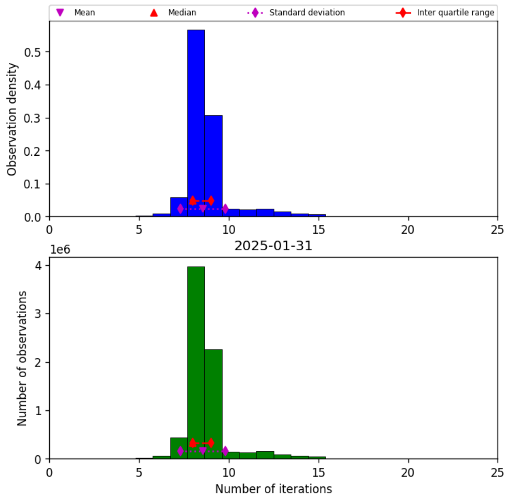
Figure 19: Histogram of “Number of iterations” for 2025-01-31 to 2025-01-31
