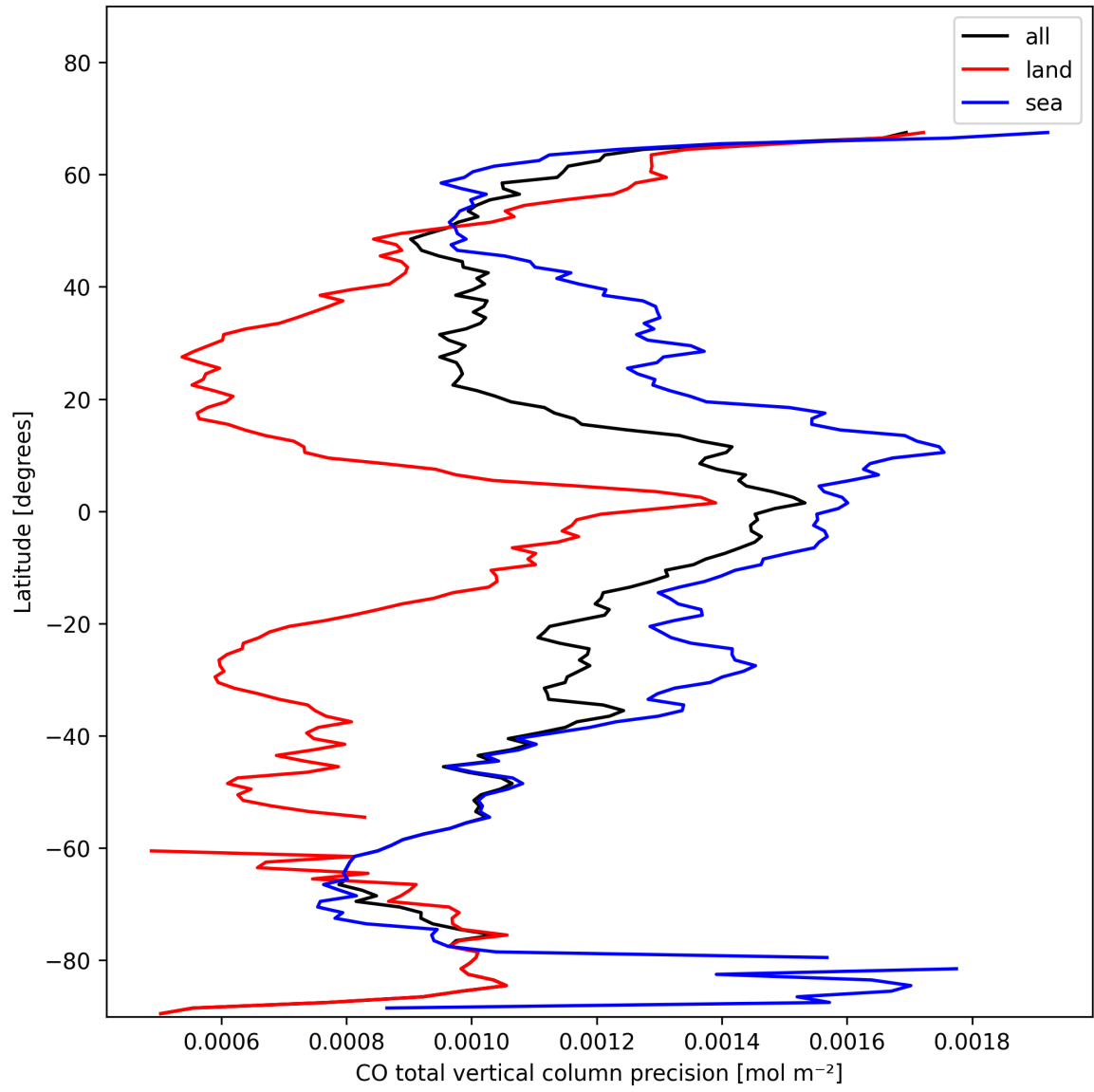
Figure 8: Zonal average of “CO total vertical column precision” for 2025-01-31 to 2025-01-31.
