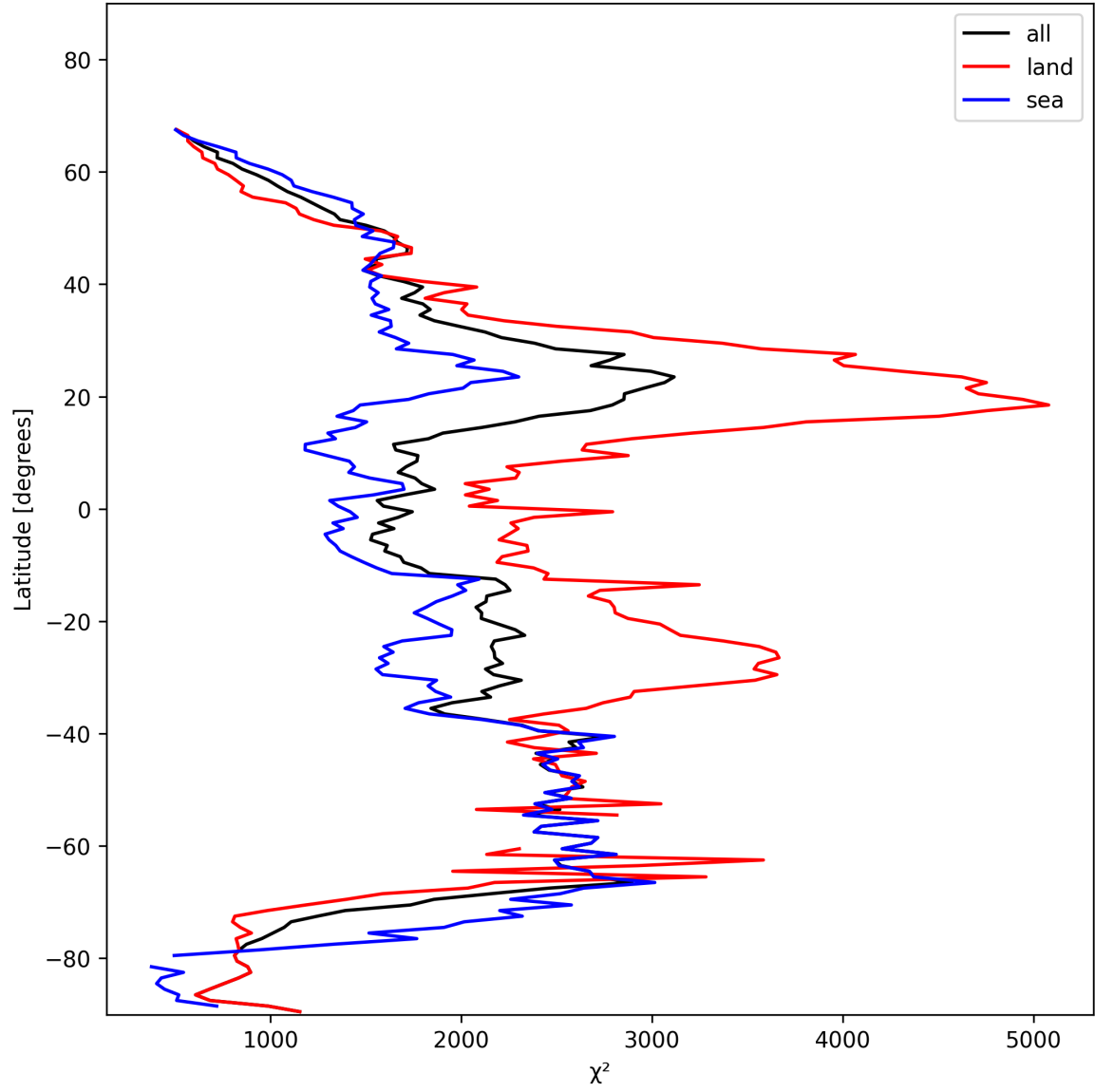
Figure 10: Zonal average of “ \chi^2 ” for 2025-01-31 to 2025-01-31.
