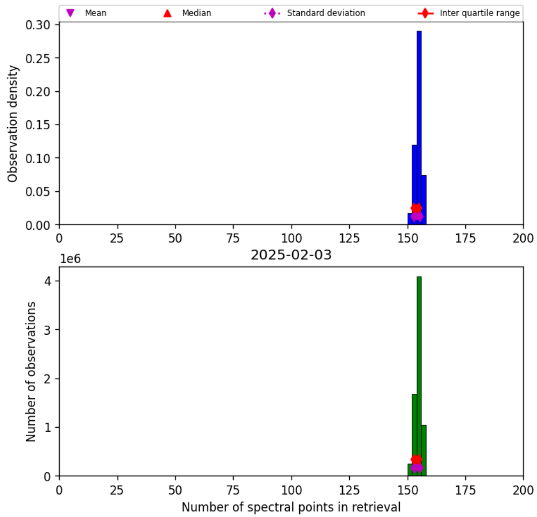
Figure 16: Histogram of “Number of spectral points in retrieval” for 2025-02-03 to 2025-02-04
