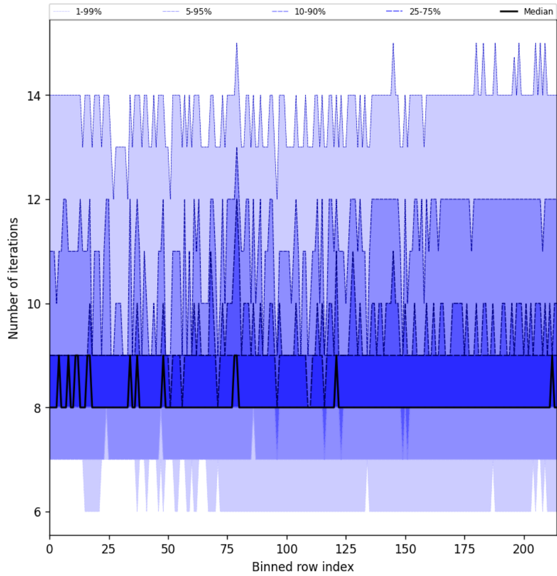
Figure 26: Along track statistics of “Number of iterations” for 2025-02-03 to 2025-02-04
