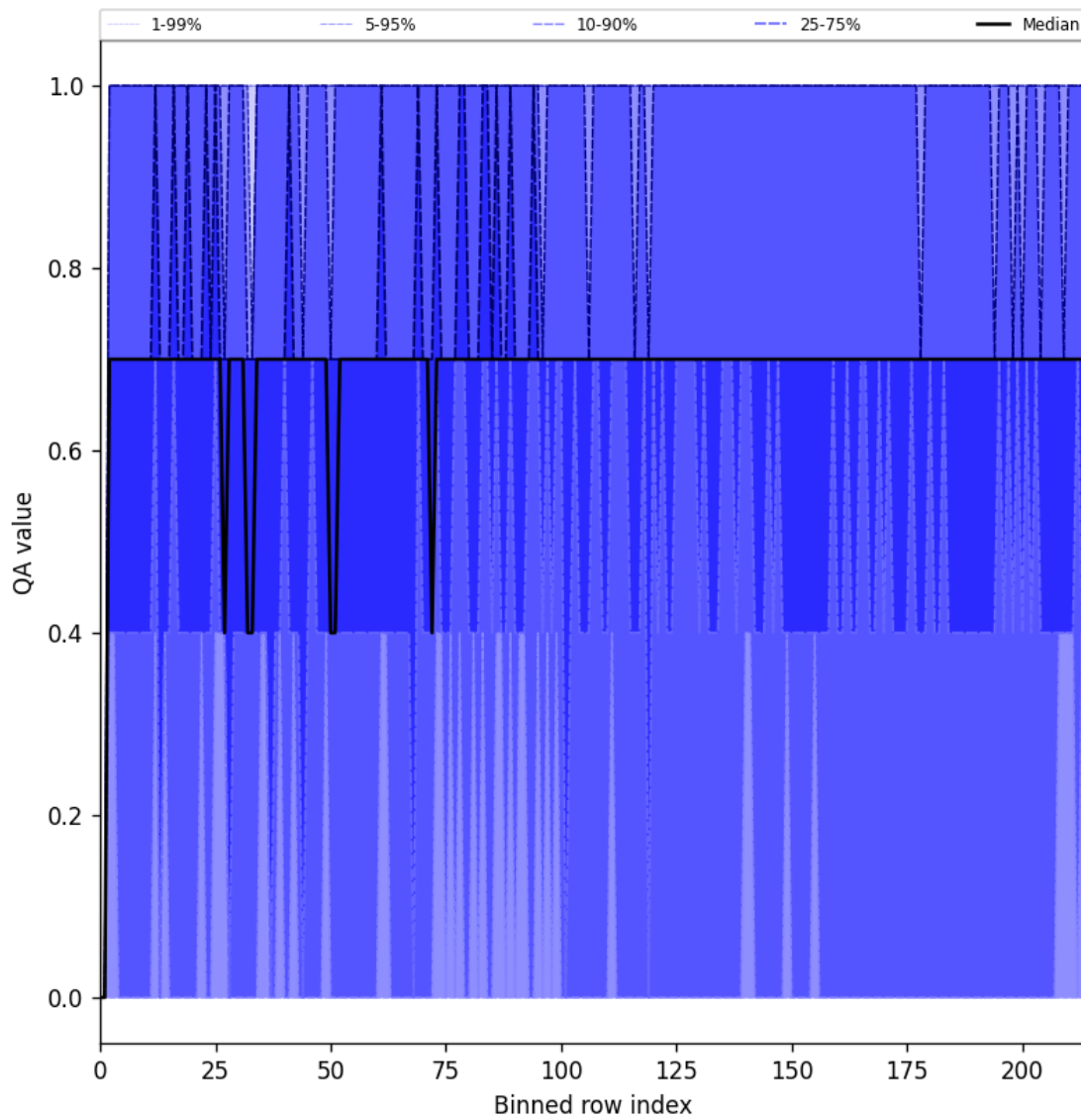
Figure 20: Along track statistics of “QA value” for 2025-02-03 to 2025-02-04
