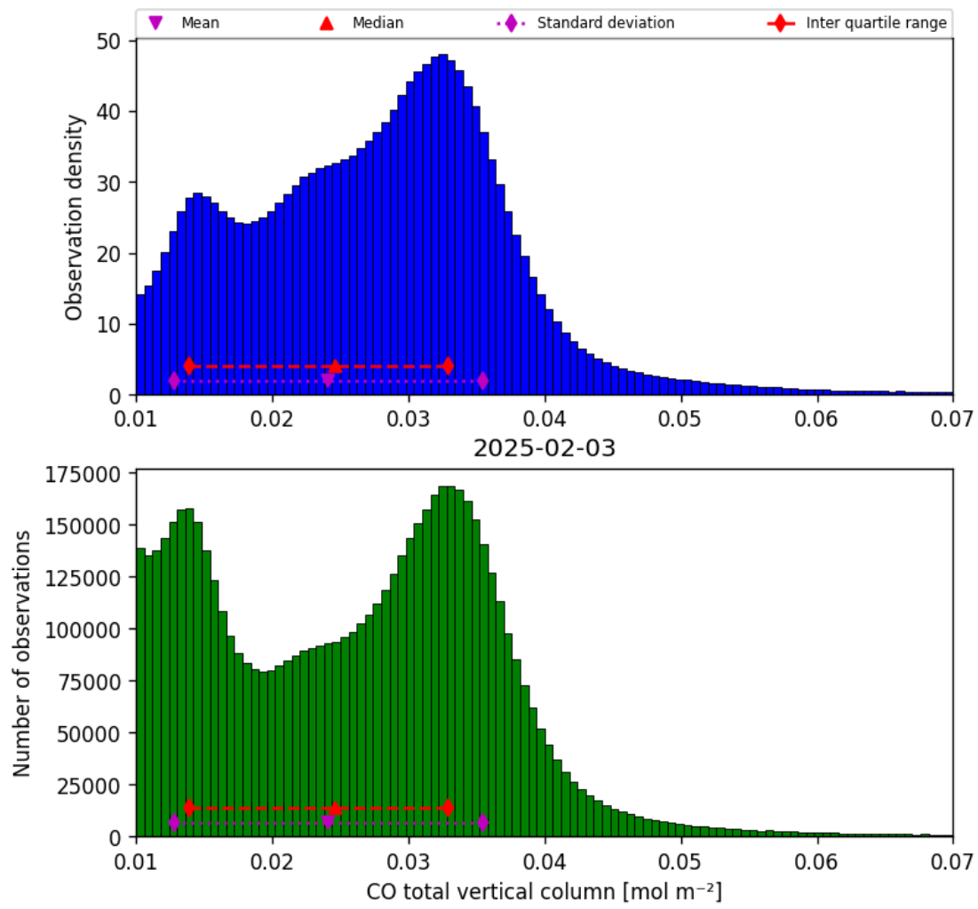
Figure 14: Histogram of “CO total vertical column” for 2025-02-03 to 2025-02-04
