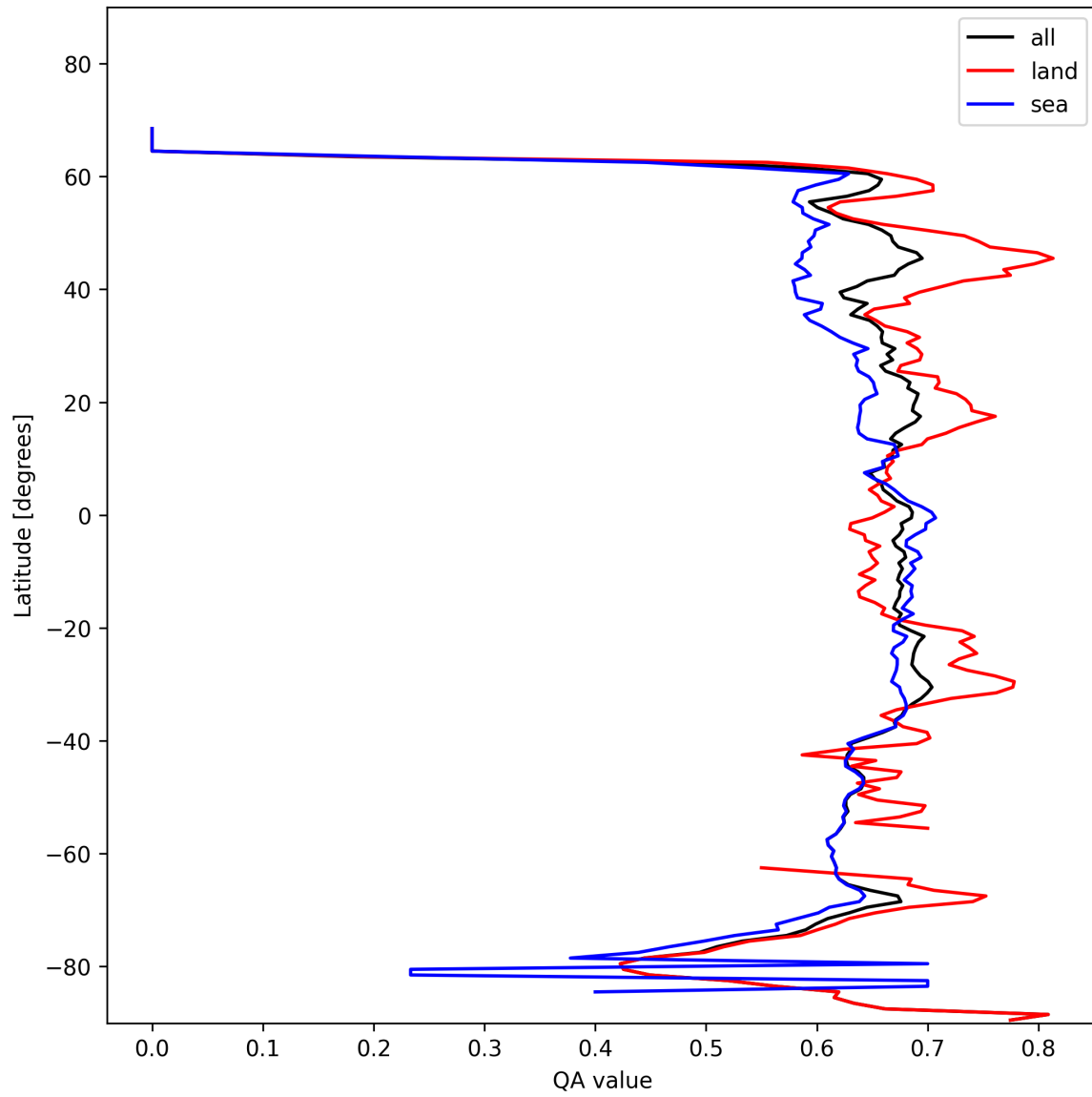
Figure 6: Zonal average of “QA value” for 2025-02-03 to 2025-02-04.
