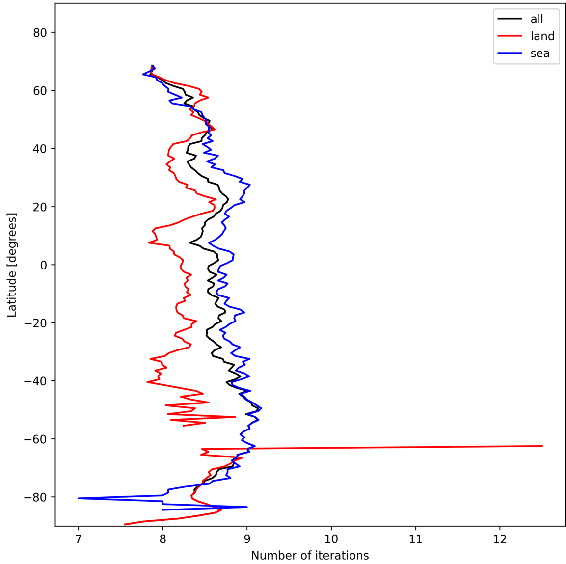
Figure 12: Zonal average of “Number of iterations” for 2025-02-03 to 2025-02-04.
