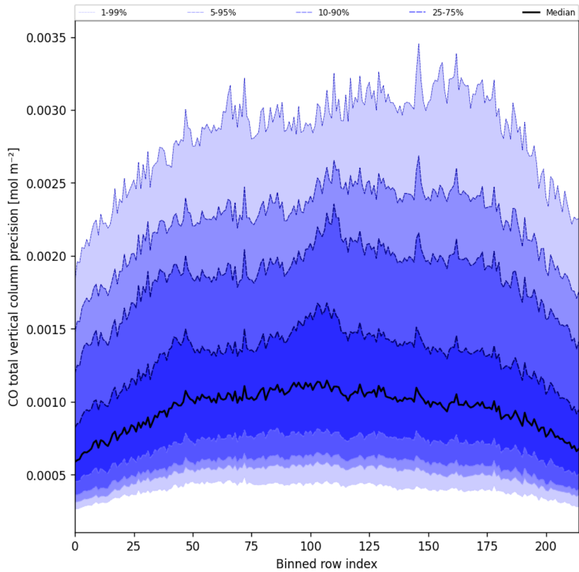
Figure 22: Along track statistics of “CO total vertical column precision” for 2025-02-03 to 2025-02-04
