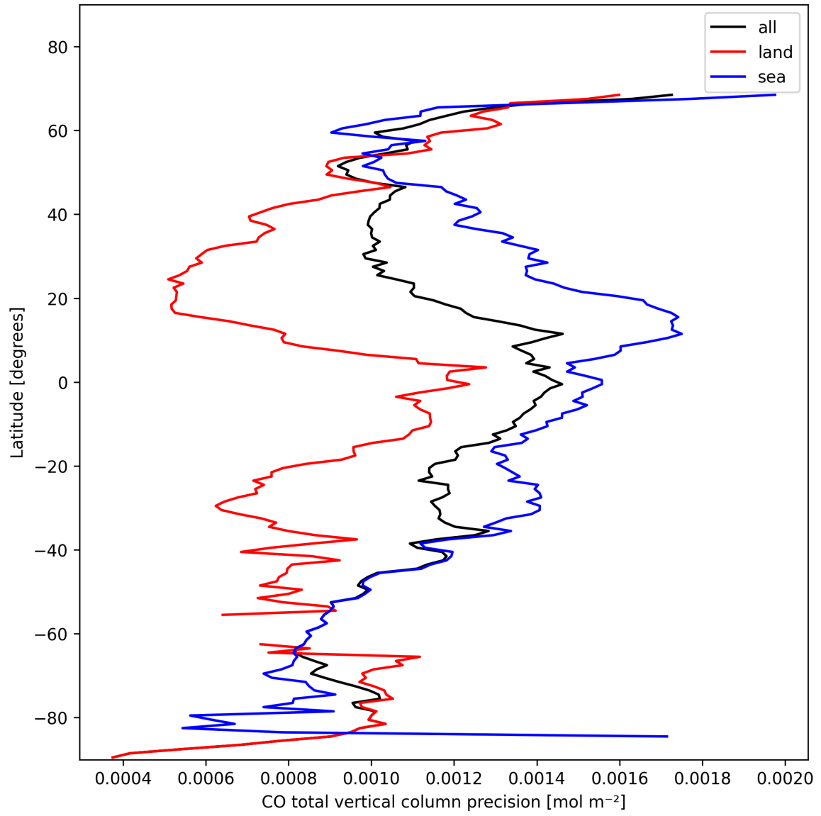
Figure 8: Zonal average of “CO total vertical column precision” for 2025-02-03 to 2025-02-04.
