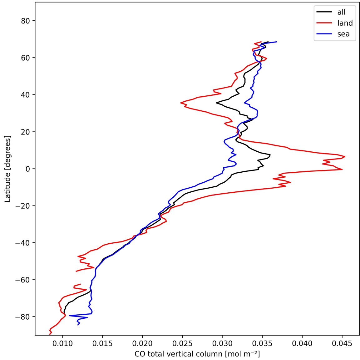
Figure 7: Zonal average of “CO total vertical column” for 2025-02-03 to 2025-02-04.
