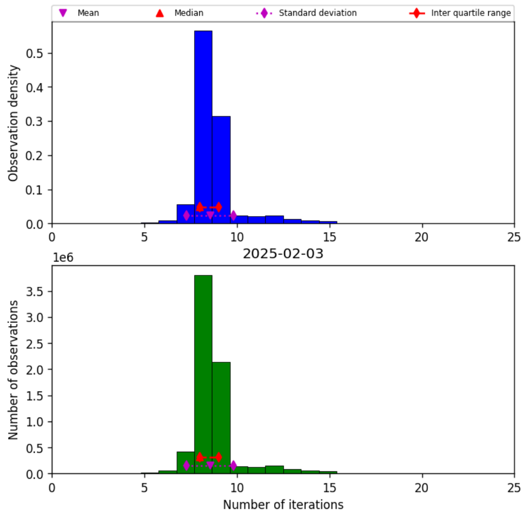
Figure 19: Histogram of “Number of iterations” for 2025-02-03 to 2025-02-04
