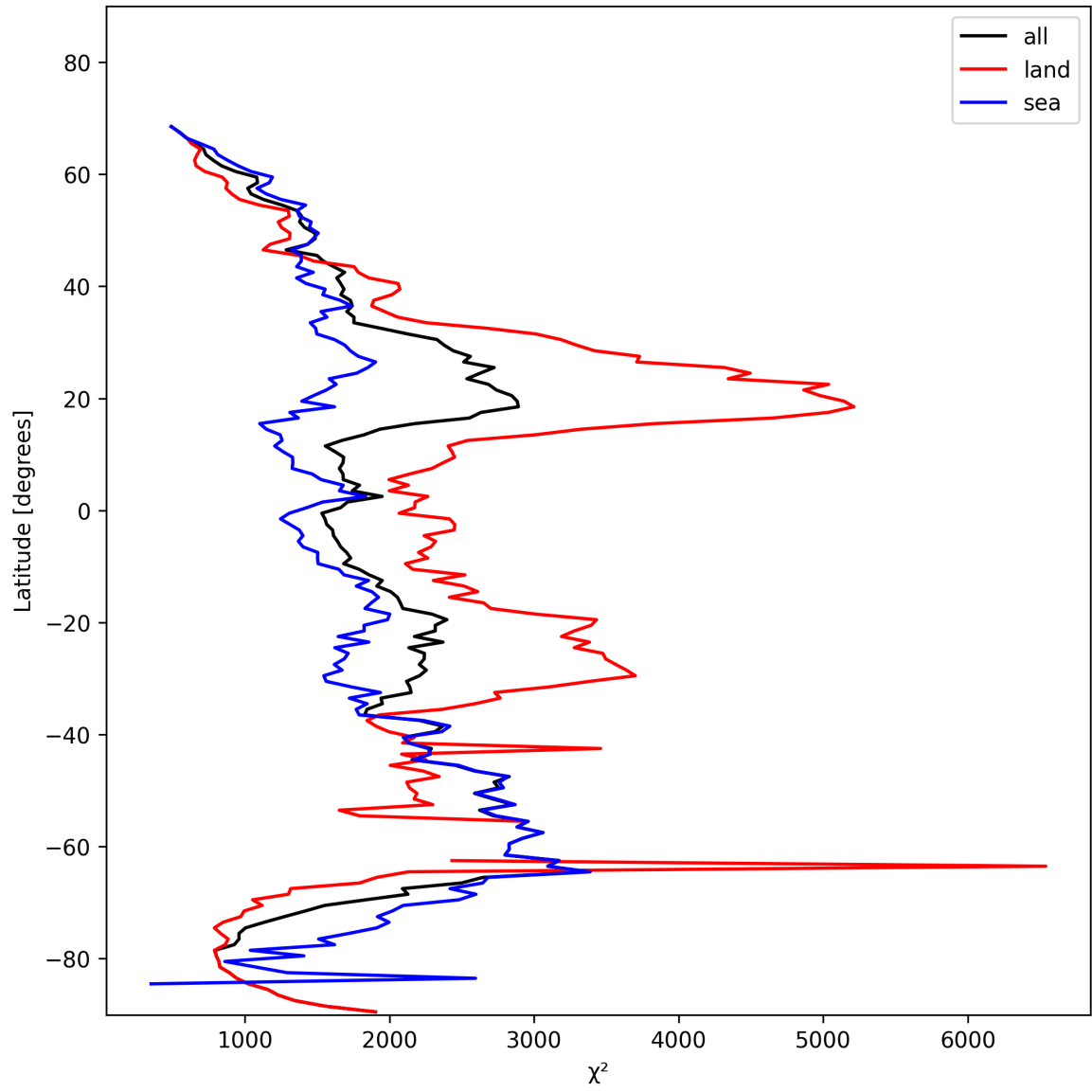
Figure 10: Zonal average of “ \chi^2 ” for 2025-02-03 to 2025-02-04.
