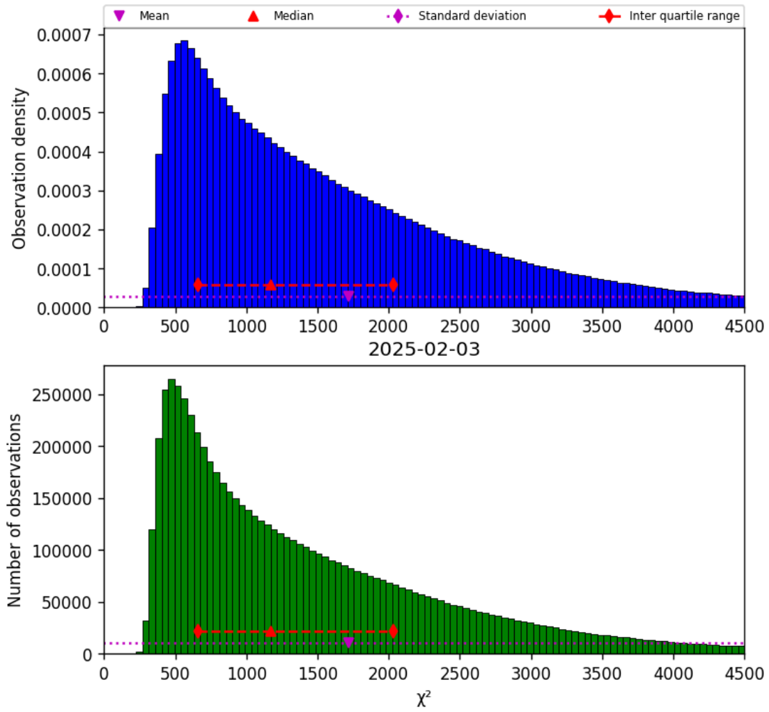
Figure 17: Histogram of “ \chi^2 ” for 2025-02-03 to 2025-02-04
