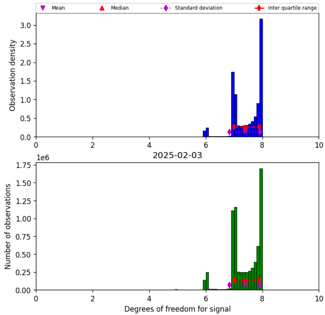
Figure 18: Histogram of “Degrees of freedom for signal” for 2025-02-03 to 2025-02-04
