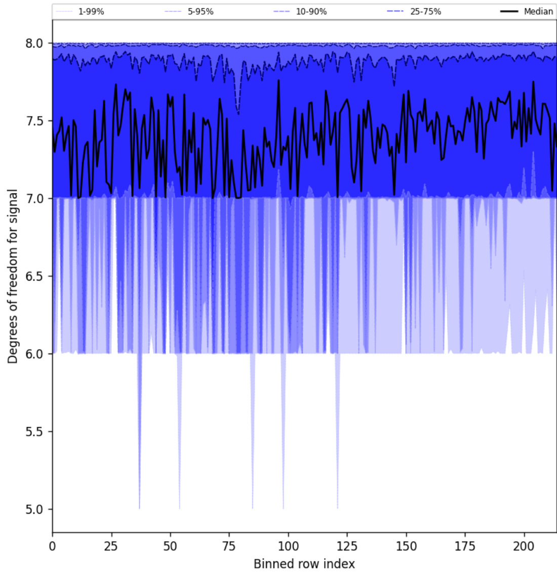
Figure 25: Along track statistics of “Degrees of freedom for signal” for 2025-02-03 to 2025-02-04
