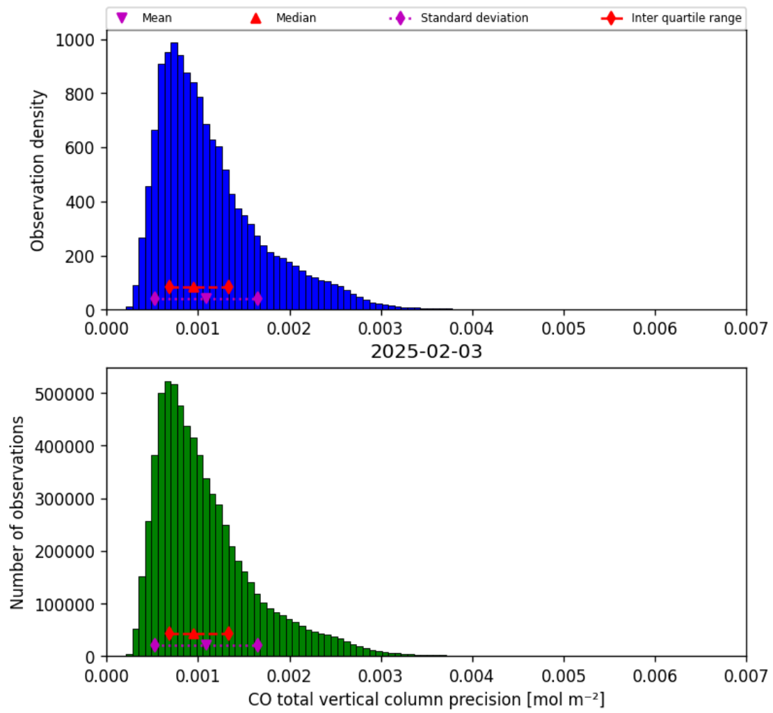
Figure 15: Histogram of “CO total vertical column precision” for 2025-02-03 to 2025-02-04
