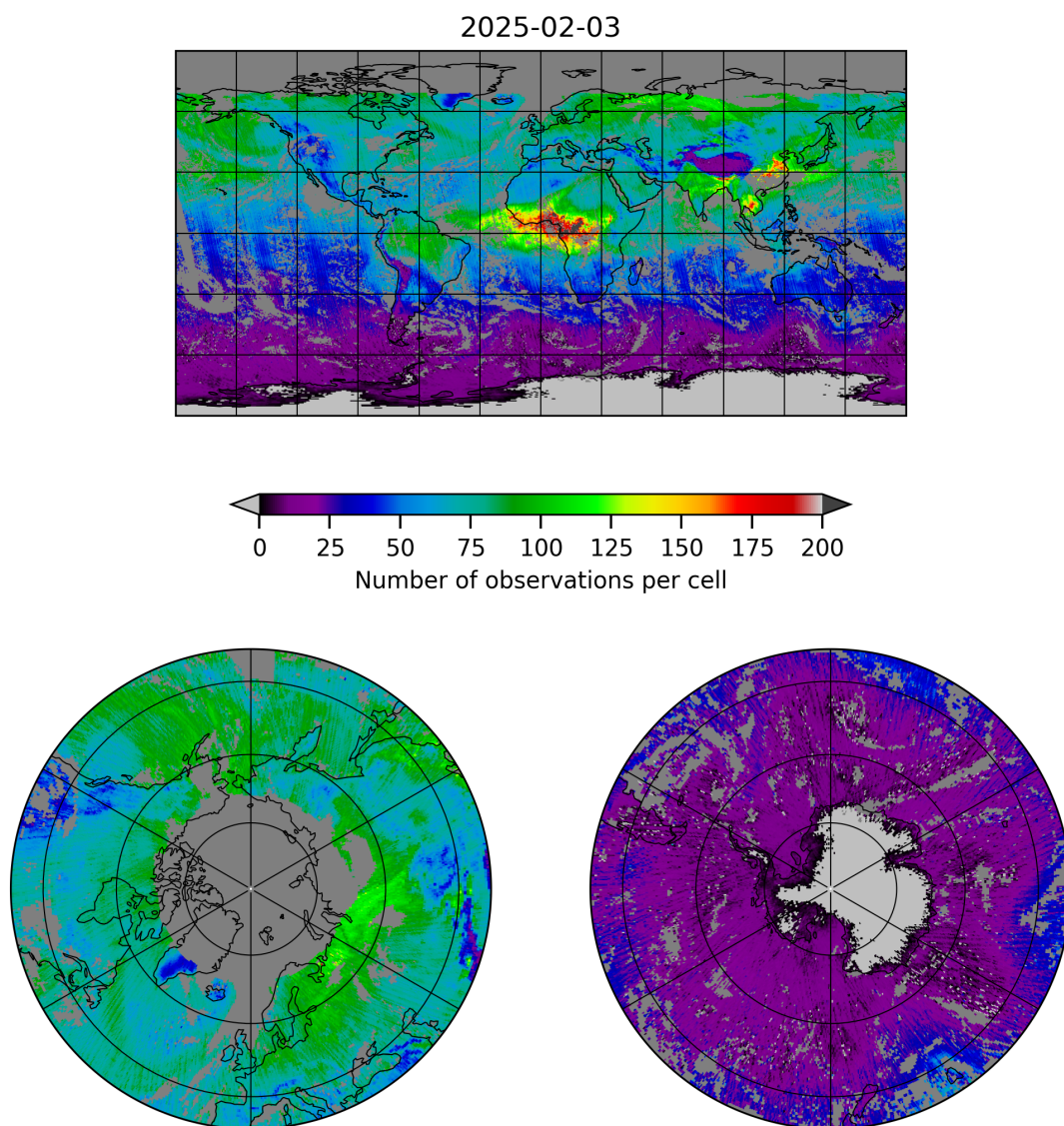
Figure 5: Map of the number of observations for 2025-02-03 to 2025-02-04
