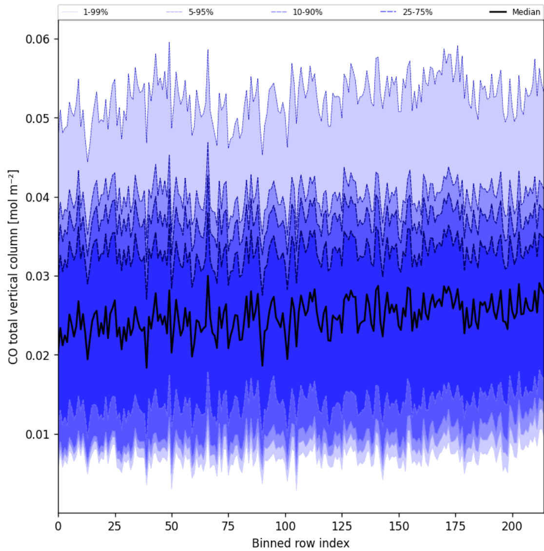
Figure 21: Along track statistics of “CO total vertical column” for 2025-02-03 to 2025-02-04
