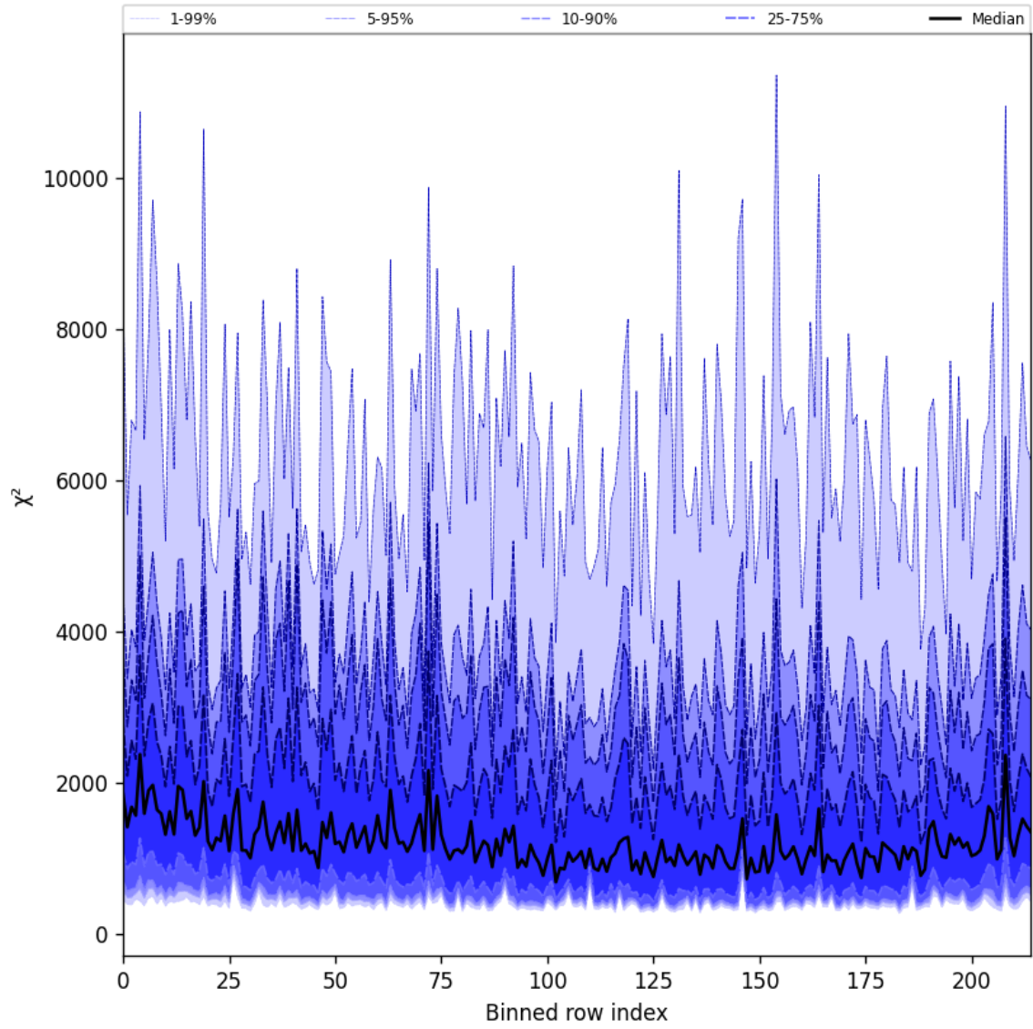
Figure 24: Along track statistics of “ \chi^2 ” for 2025-02-03 to 2025-02-04
