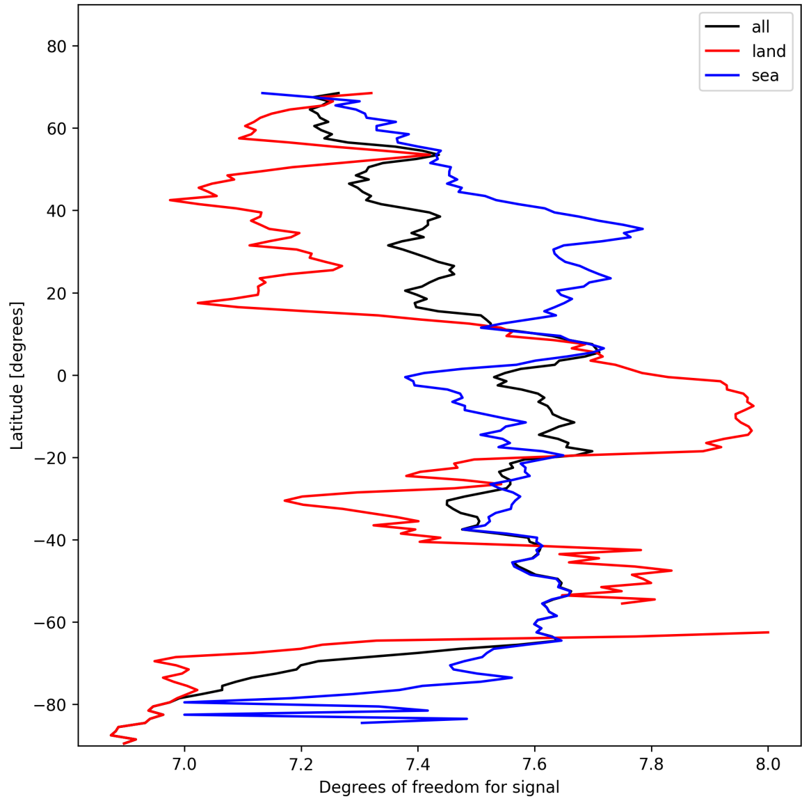
Figure 11: Zonal average of “Degrees of freedom for signal” for 2025-02-03 to 2025-02-04.
