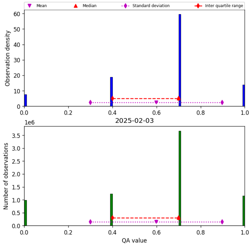
Figure 13: Histogram of “QA value” for 2025-02-03 to 2025-02-04
