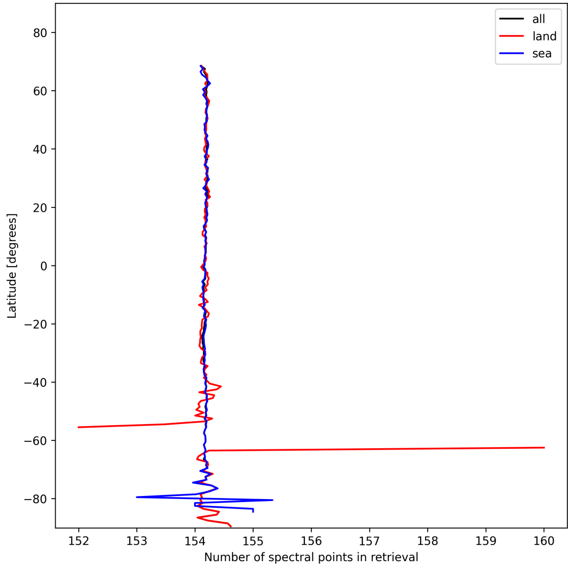
Figure 9: Zonal average of “Number of spectral points in retrieval” for 2025-02-03 to 2025-02-04.
