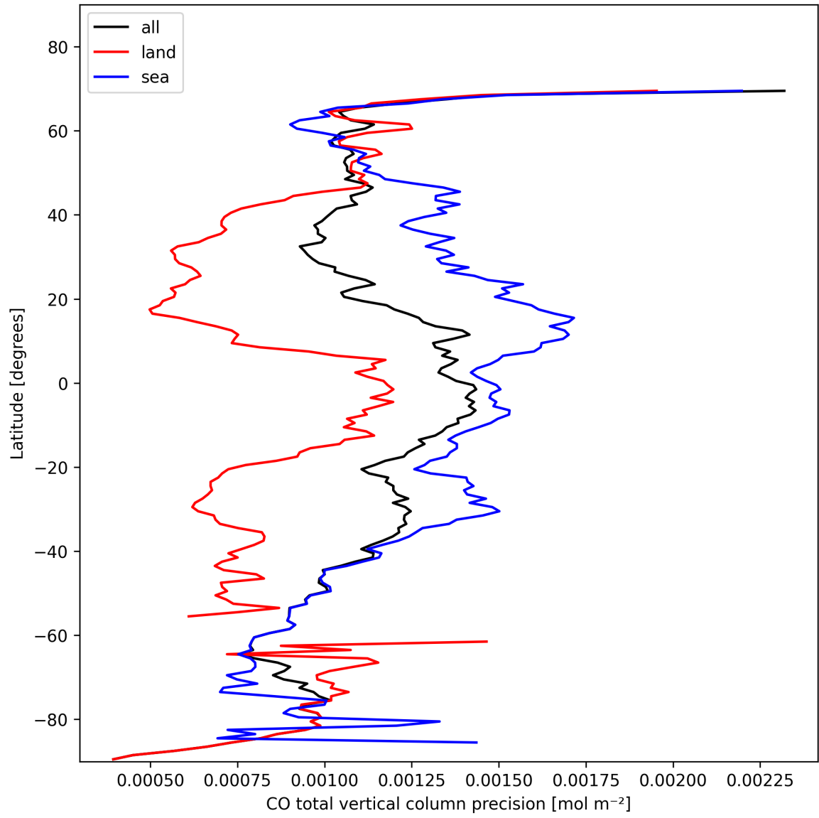
Figure 8: Zonal average of “CO total vertical column precision” for 2025-02-04 to 2025-02-05.
