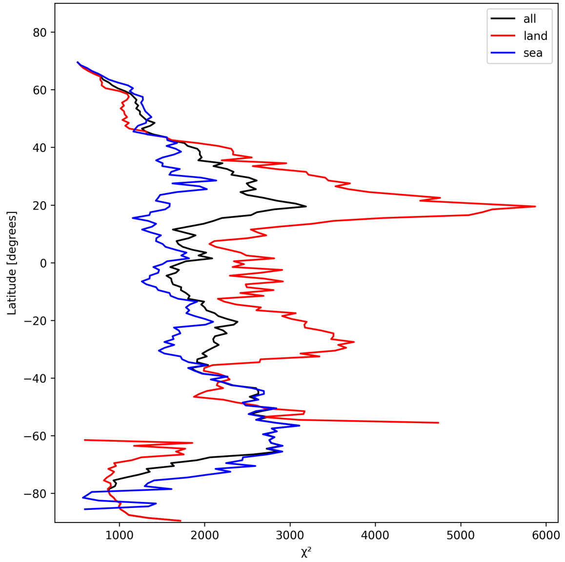
Figure 10: Zonal average of “ \chi^2 ” for 2025-02-04 to 2025-02-05.
