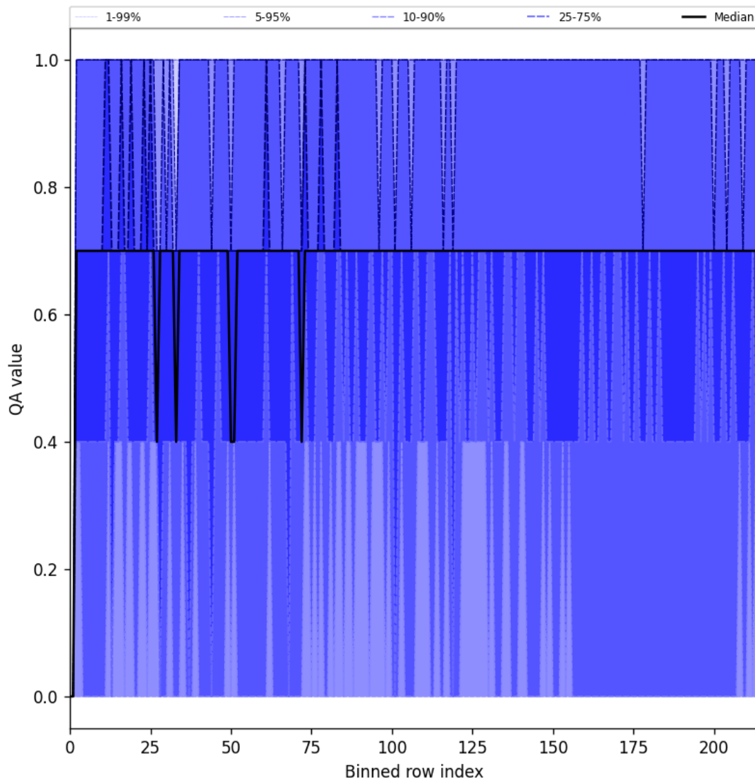
Figure 20: Along track statistics of “QA value” for 2025-02-04 to 2025-02-05
