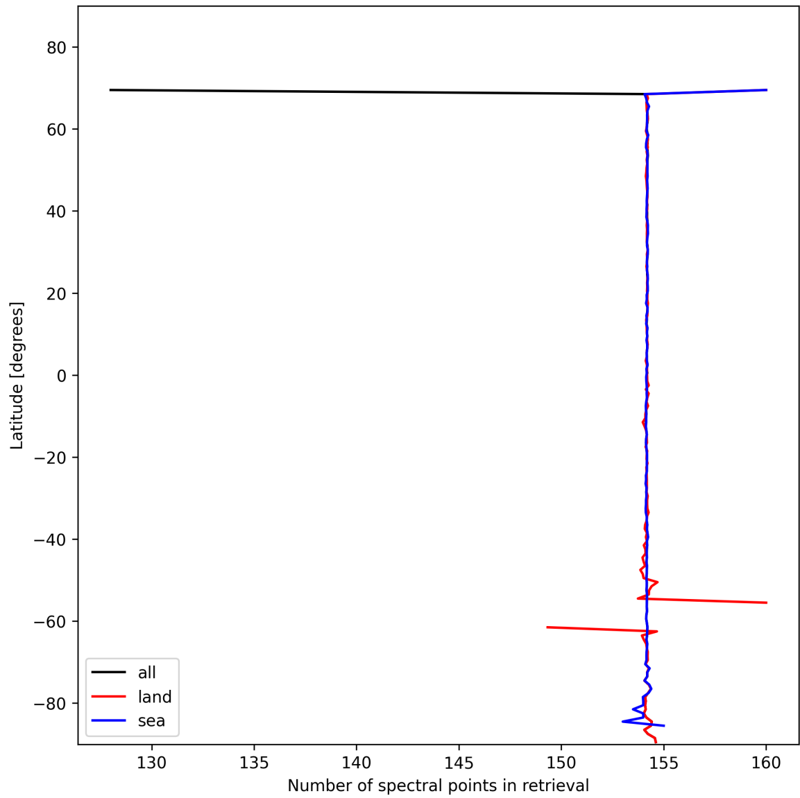
Figure 9: Zonal average of “Number of spectral points in retrieval” for 2025-02-04 to 2025-02-05.
