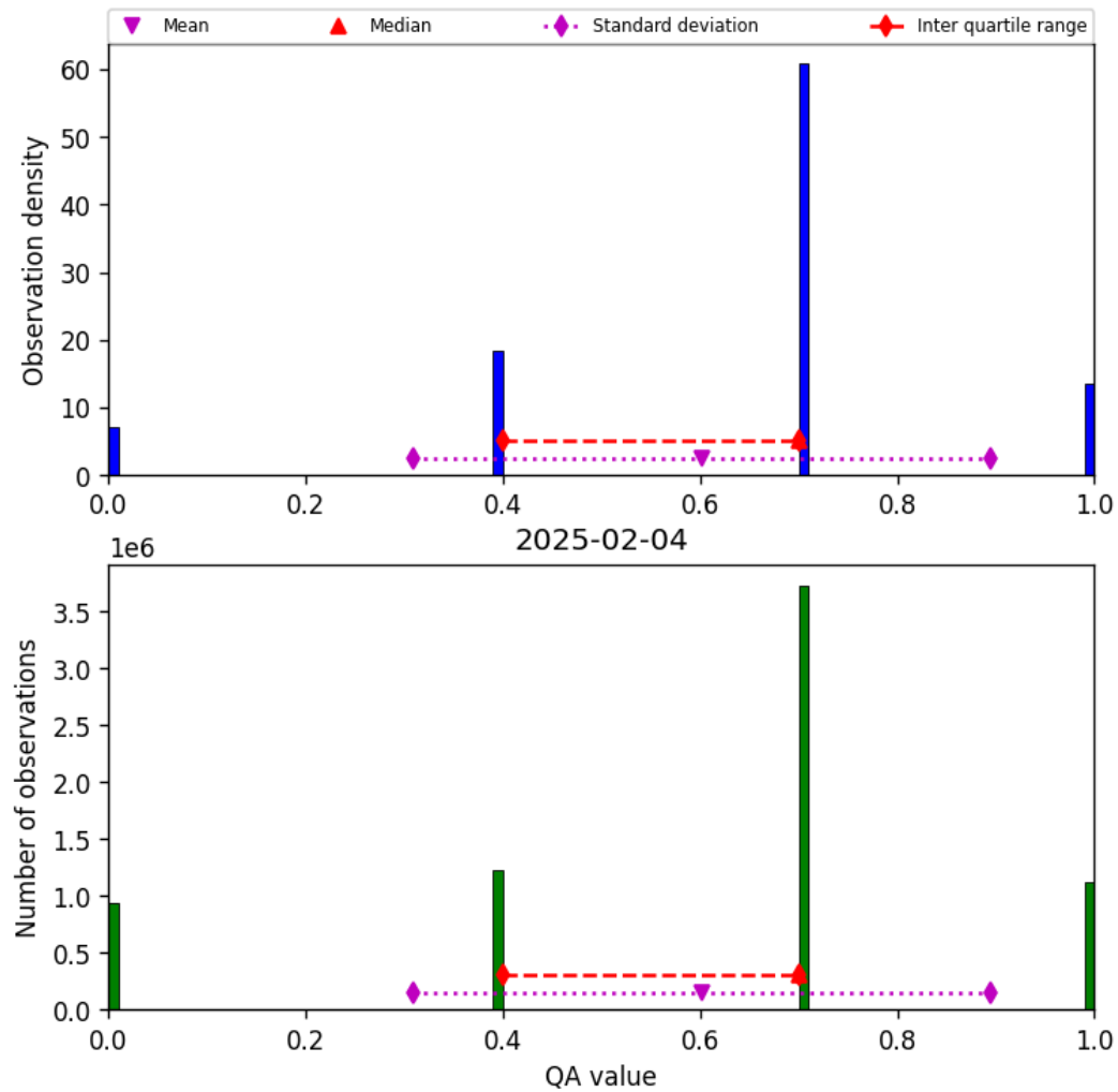
Figure 13: Histogram of “QA value” for 2025-02-04 to 2025-02-05
