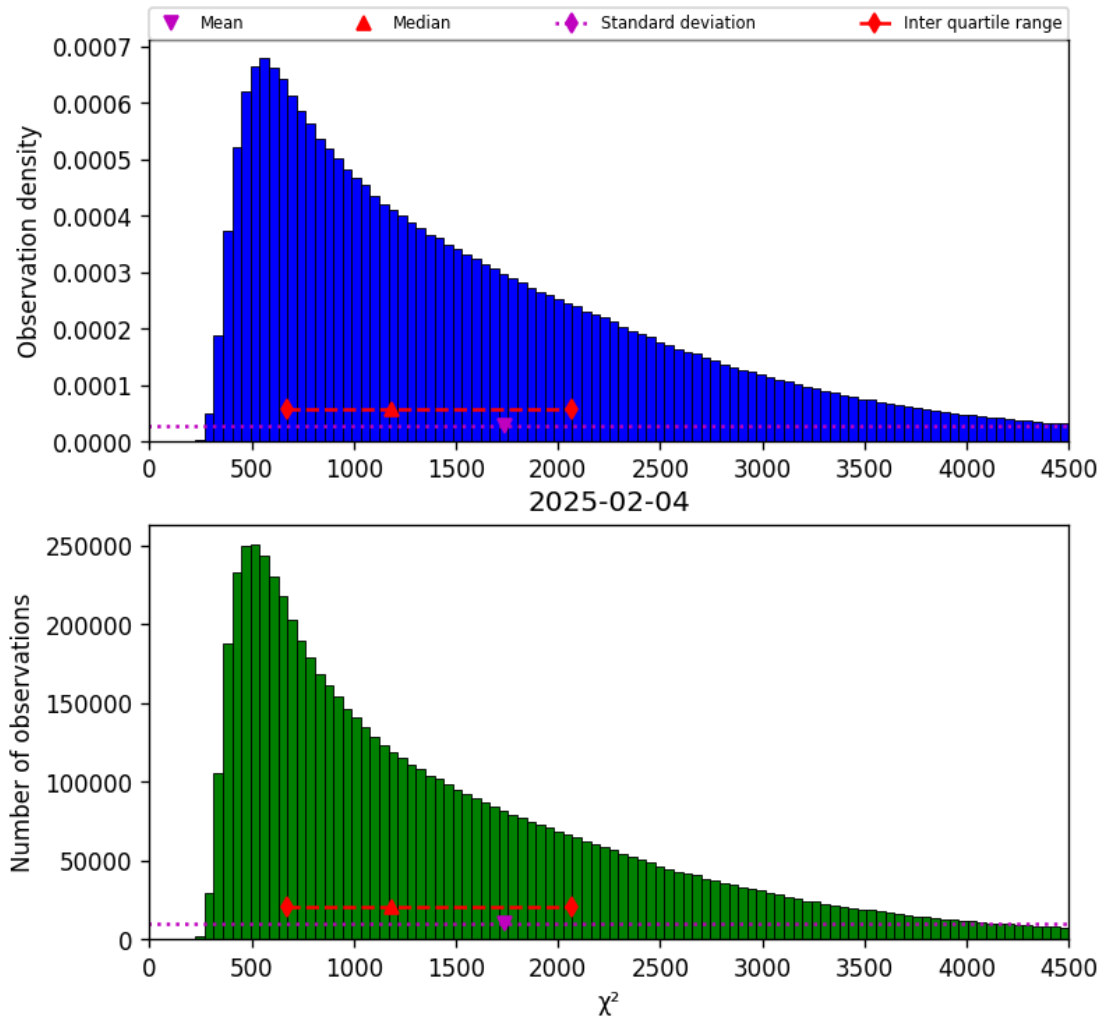
Figure 17: Histogram of " \chi^2 " for 2025-02-04 to 2025-02-05
