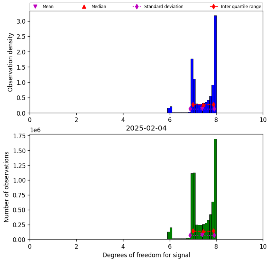
Figure 18: Histogram of “Degrees of freedom for signal” for 2025-02-04 to 2025-02-05
