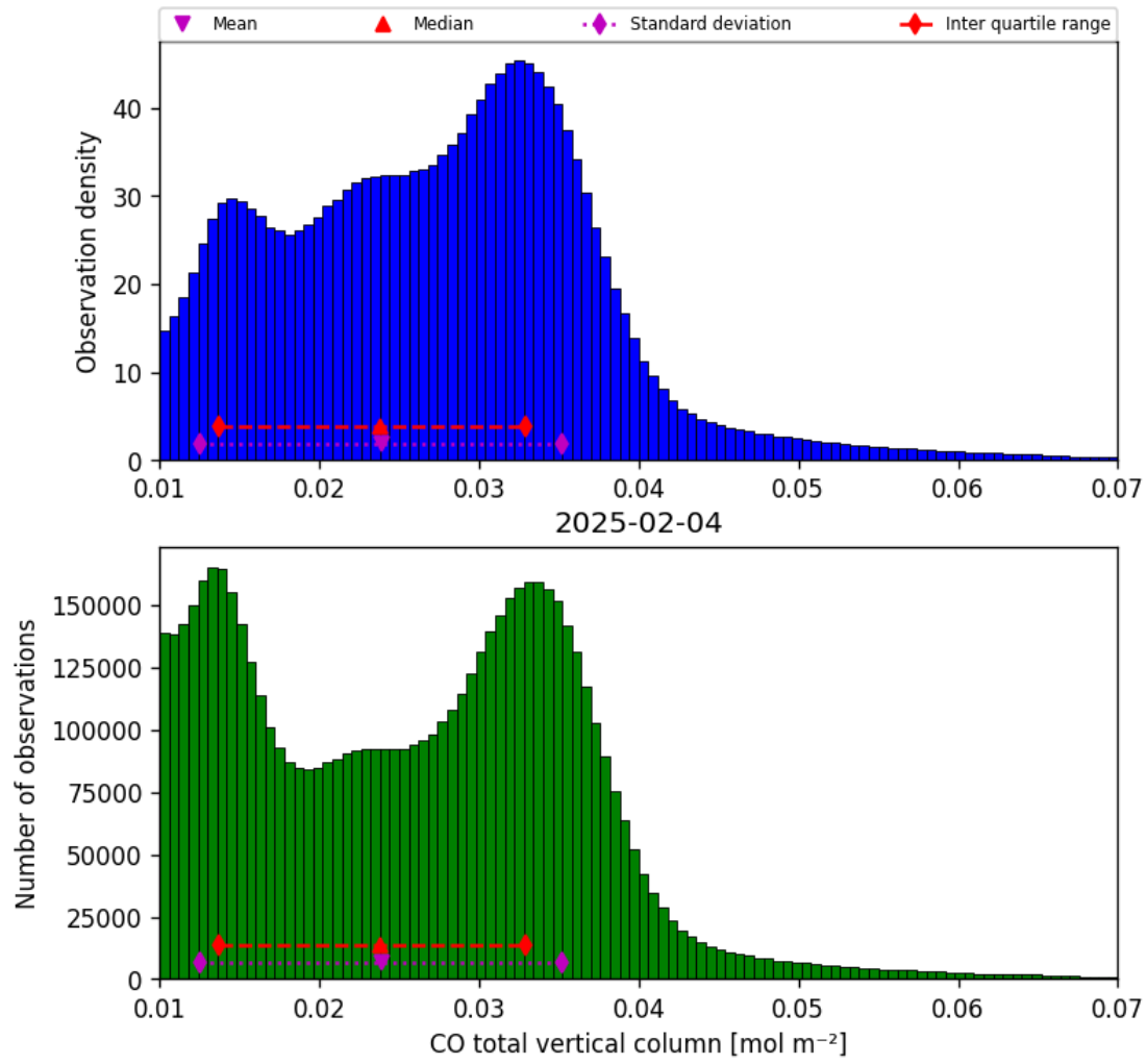
Figure 14: Histogram of “CO total vertical column” for 2025-02-04 to 2025-02-05
