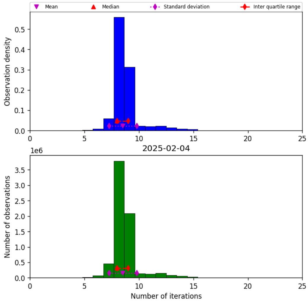
Figure 19: Histogram of “Number of iterations” for 2025-02-04 to 2025-02-05
