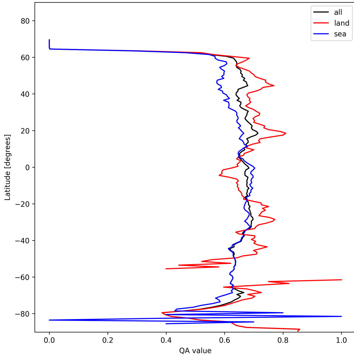
Figure 6: Zonal average of “QA value” for 2025-02-04 to 2025-02-05.
