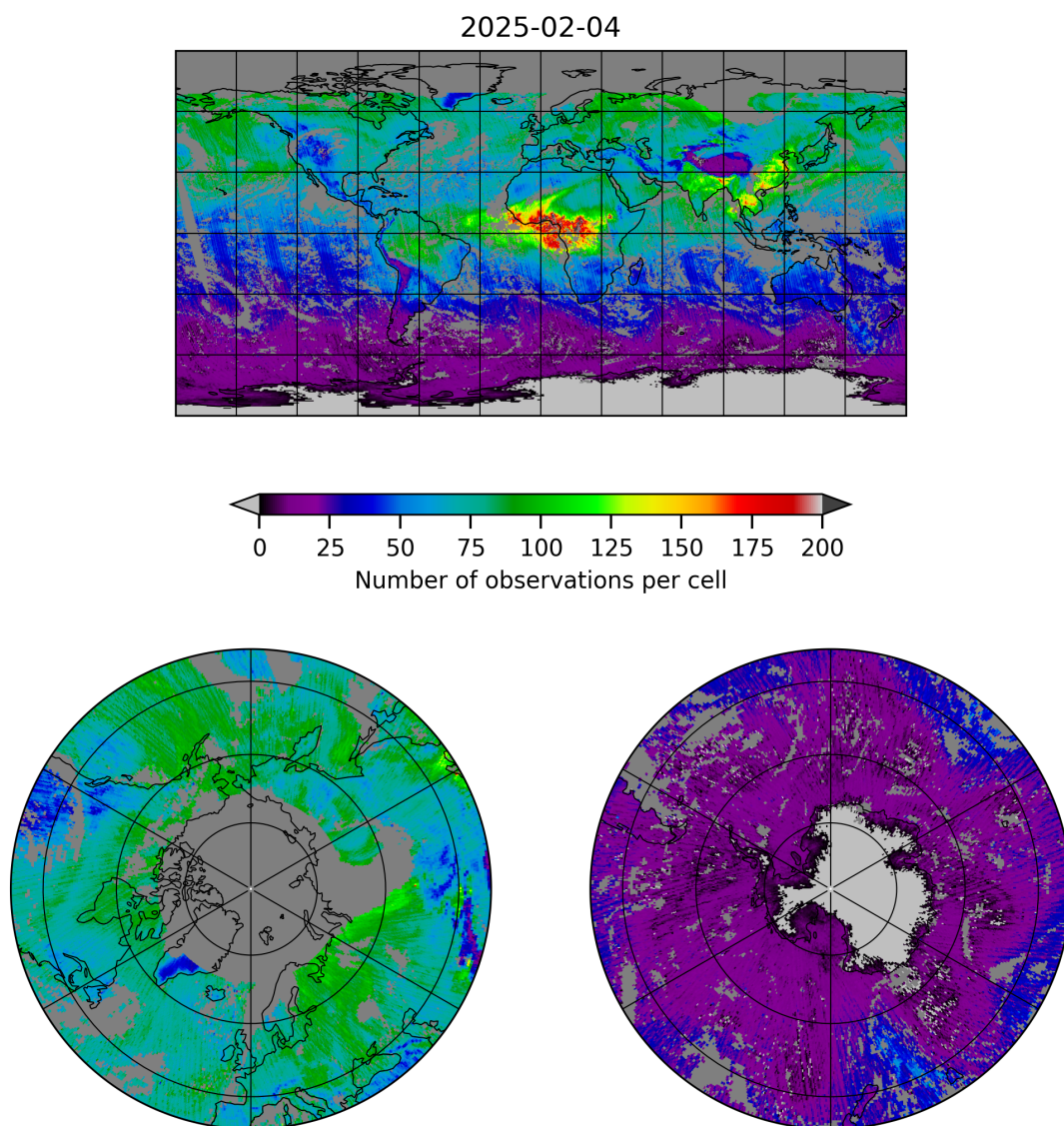
Figure 5: Map of the number of observations for 2025-02-04 to 2025-02-05
