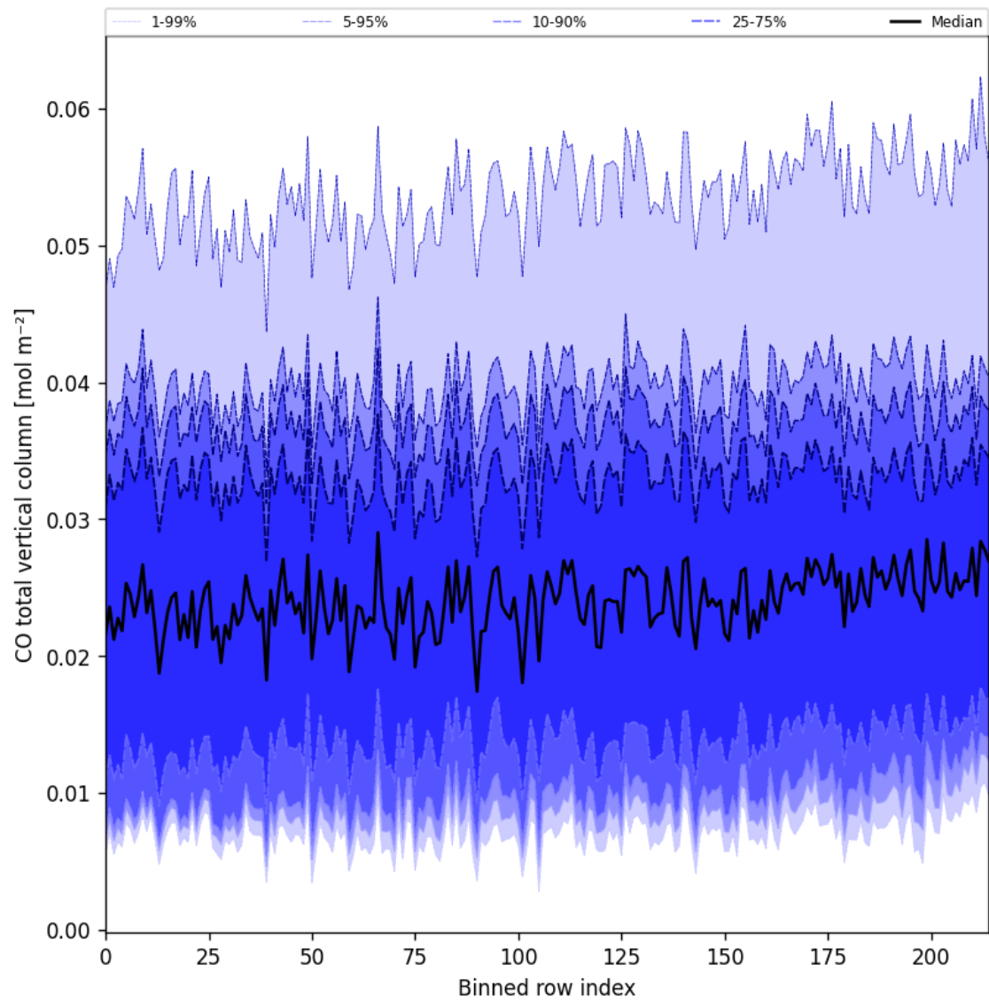
Figure 21: Along track statistics of “CO total vertical column” for 2025-02-04 to 2025-02-05
