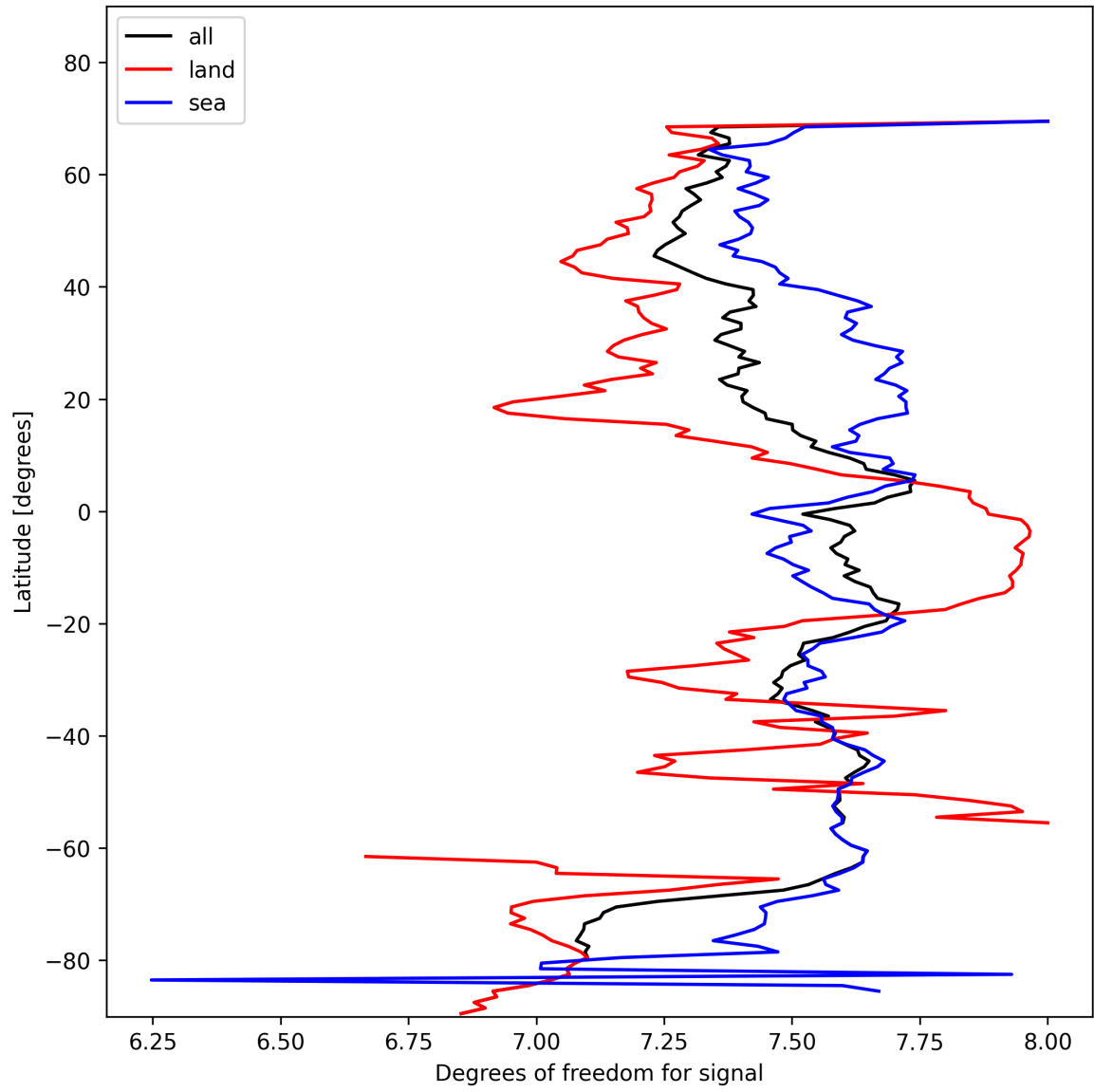
Figure 11: Zonal average of “Degrees of freedom for signal” for 2025-02-04 to 2025-02-05.
