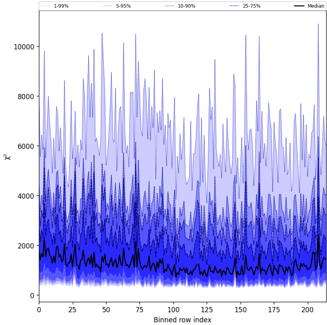
Figure 24: Along track statistics of “ \chi^2 ” for 2025-02-04 to 2025-02-05
