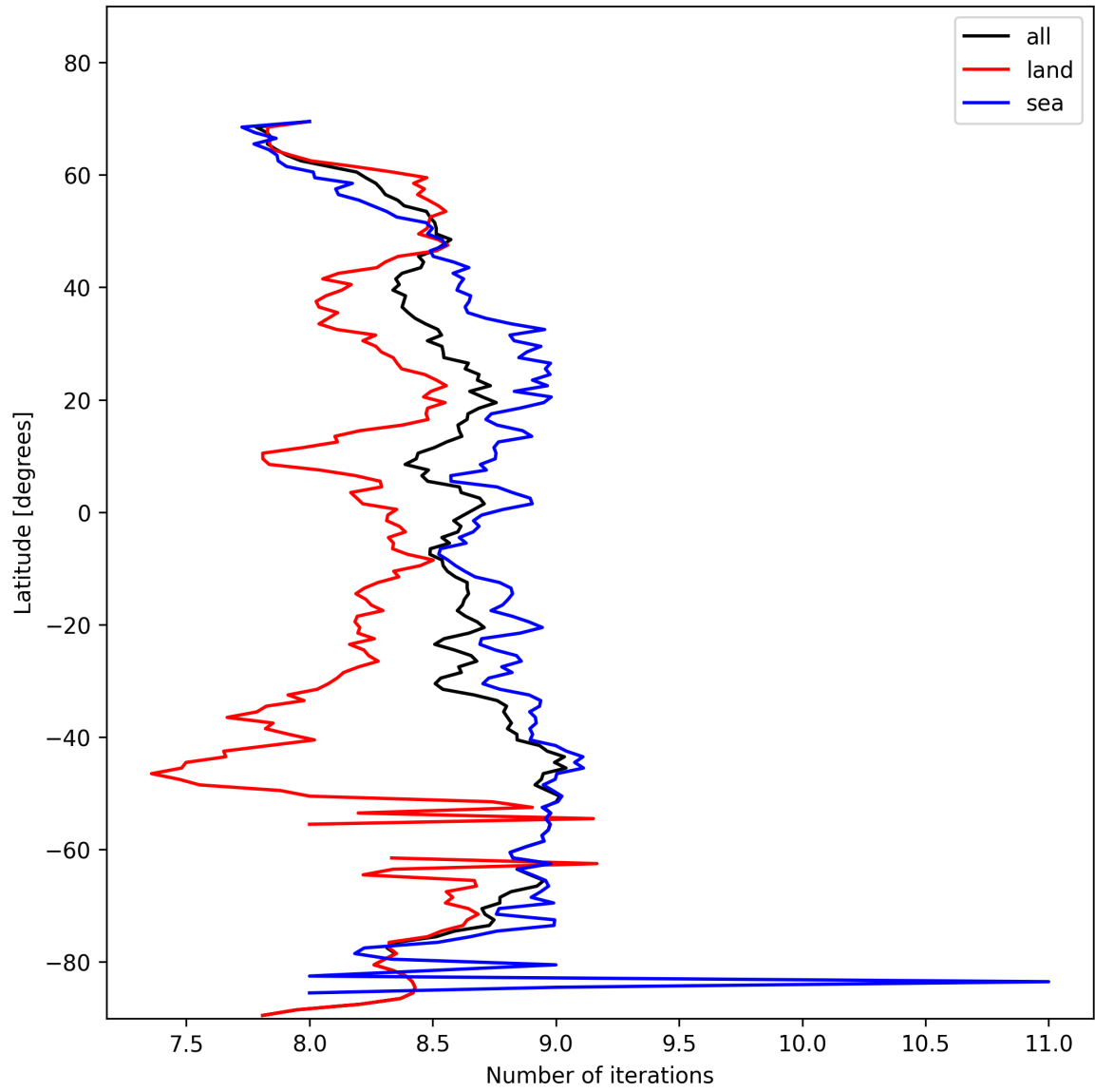
Figure 12: Zonal average of “Number of iterations” for 2025-02-04 to 2025-02-05.
