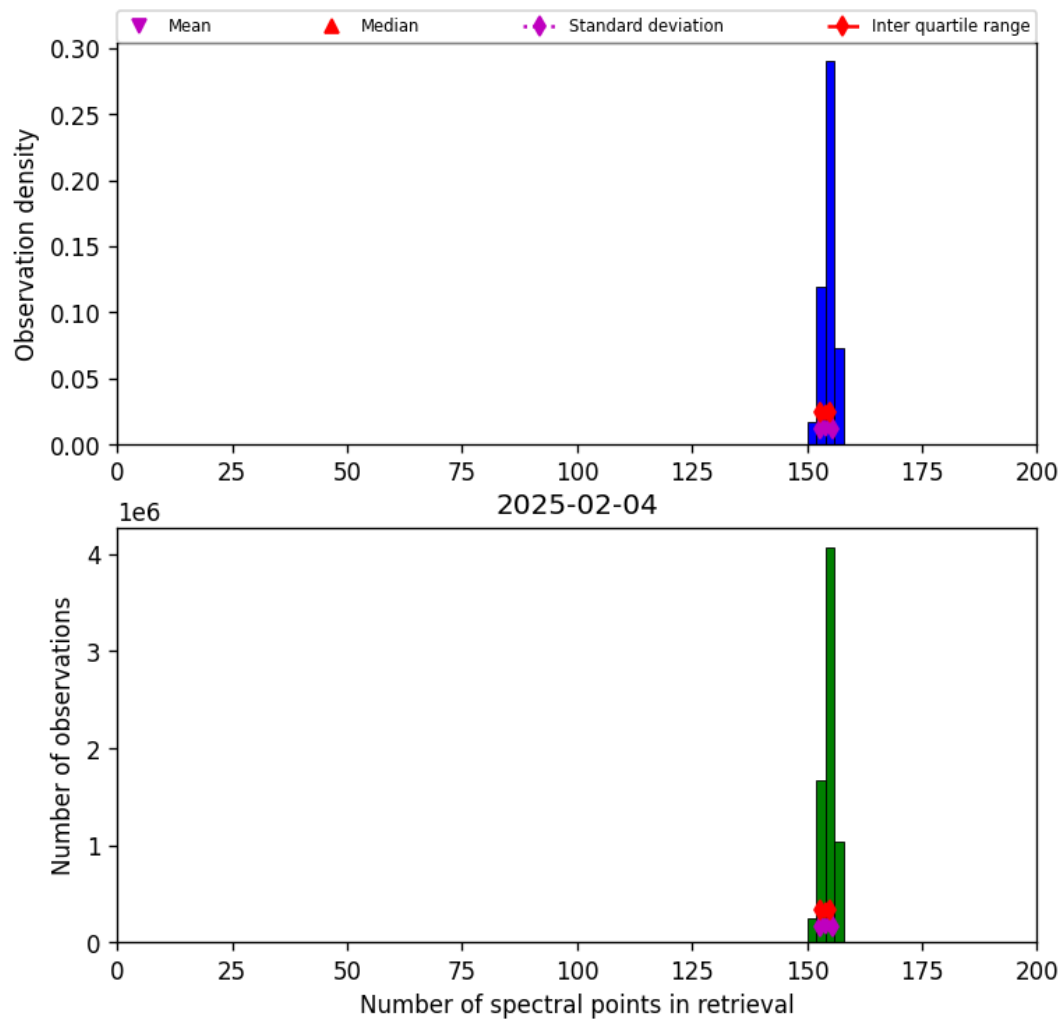
Figure 16: Histogram of “Number of spectral points in retrieval” for 2025-02-04 to 2025-02-05
