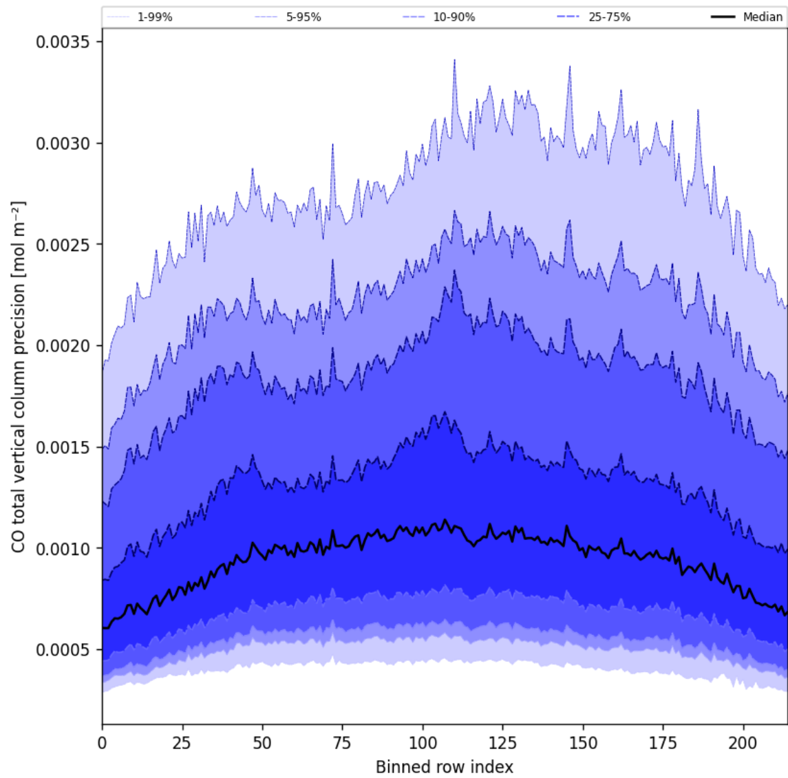
Figure 22: Along track statistics of “CO total vertical column precision” for 2025-02-04 to 2025-02-05
