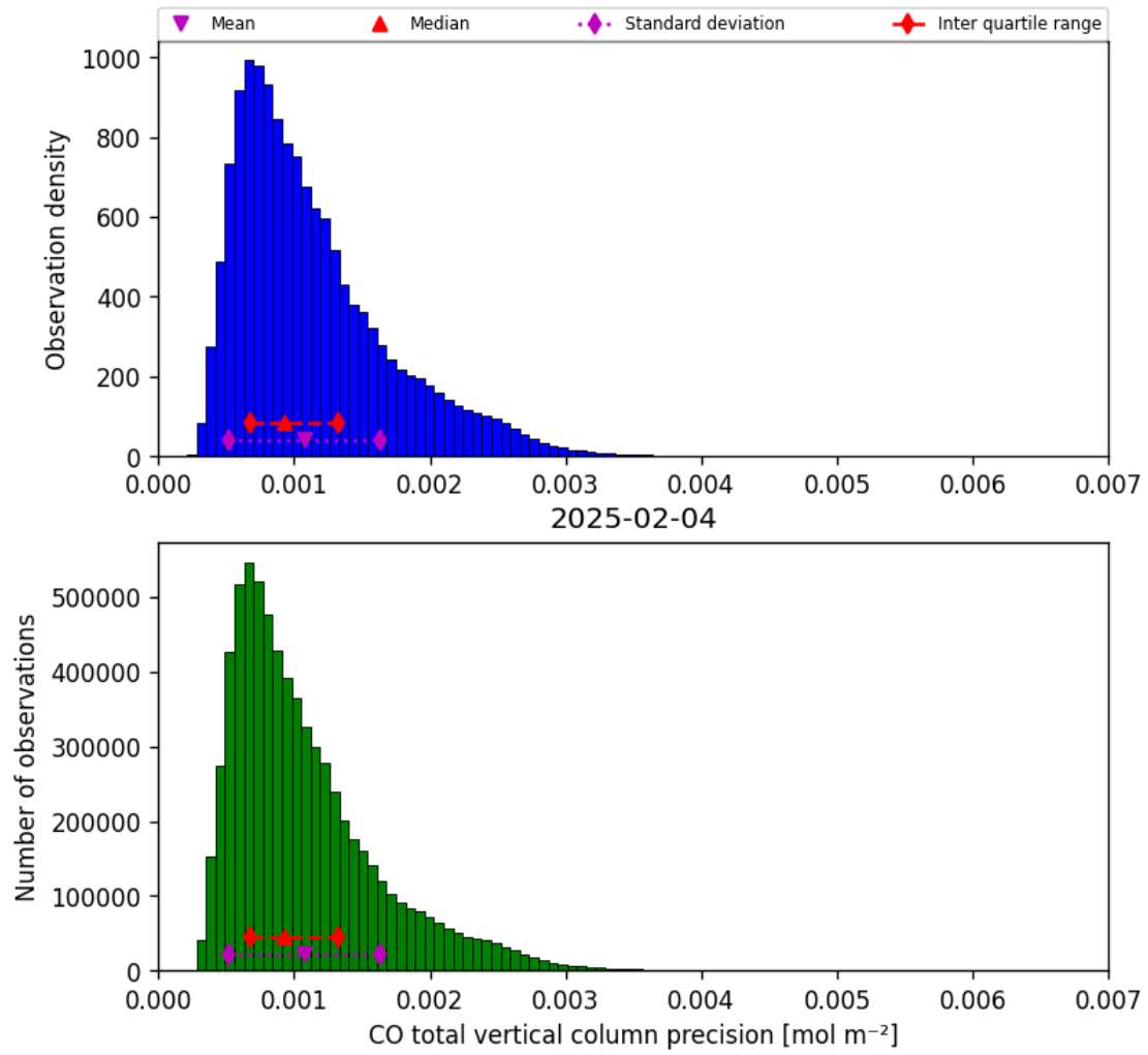
Figure 15: Histogram of “CO total vertical column precision” for 2025-02-04 to 2025-02-05
