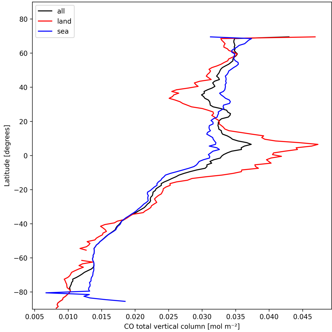
Figure 7: Zonal average of “CO total vertical column” for 2025-02-04 to 2025-02-05.
