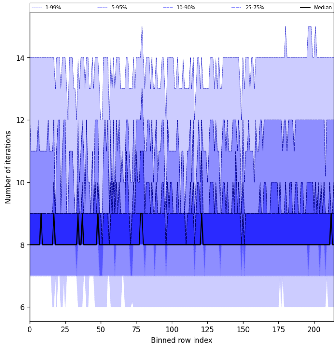
Figure 26: Along track statistics of “Number of iterations” for 2025-02-04 to 2025-02-05
