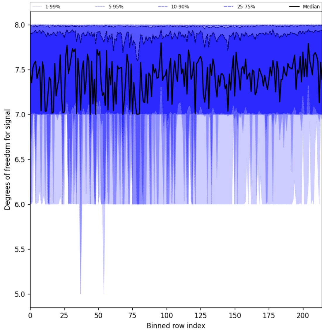
Figure 25: Along track statistics of “Degrees of freedom for signal” for 2025-02-04 to 2025-02-05
