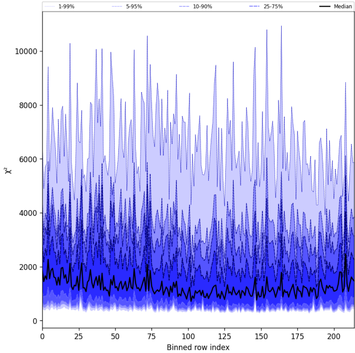
Figure 24: Along track statistics of “ \chi^2 ” for 2025-02-05 to 2025-02-06
