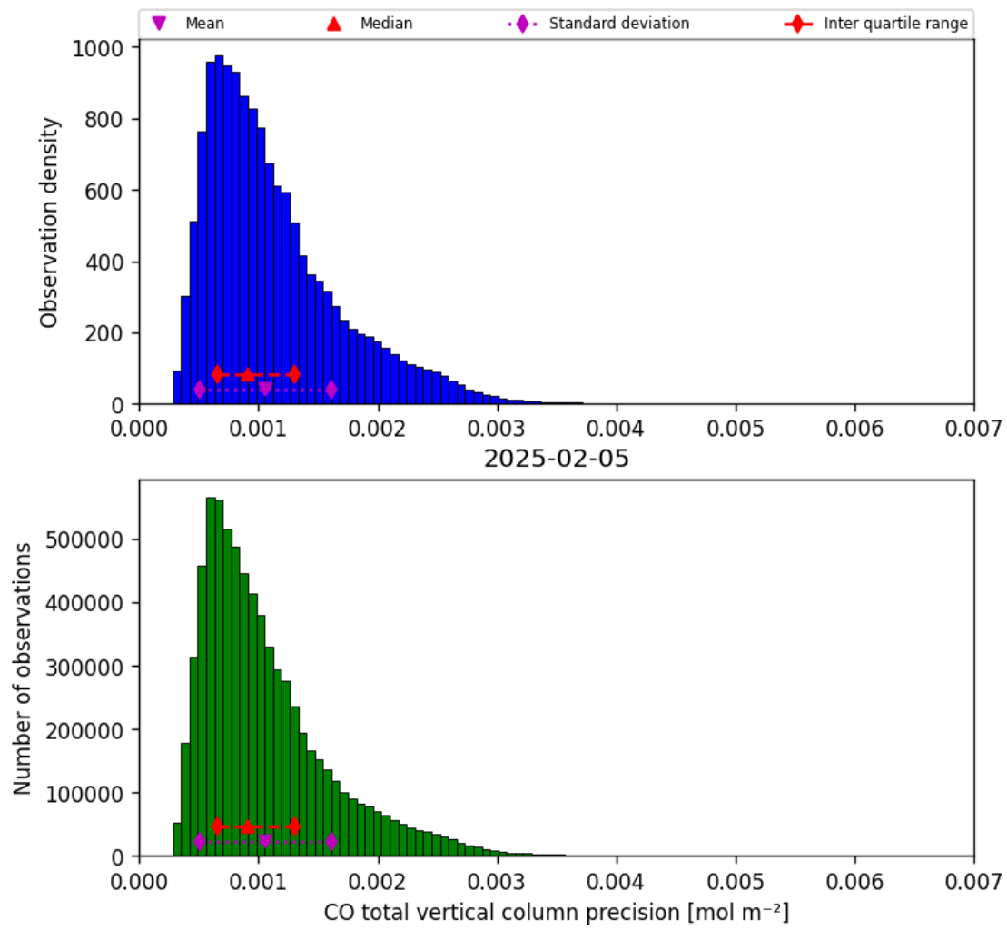
Figure 15: Histogram of “CO total vertical column precision” for 2025-02-05 to 2025-02-06
