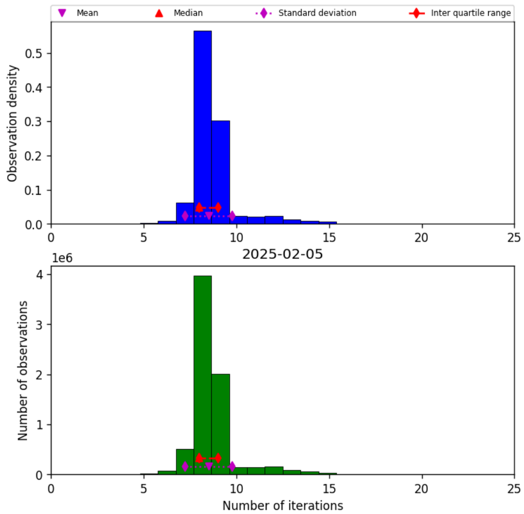
Figure 19: Histogram of “Number of iterations” for 2025-02-05 to 2025-02-06
