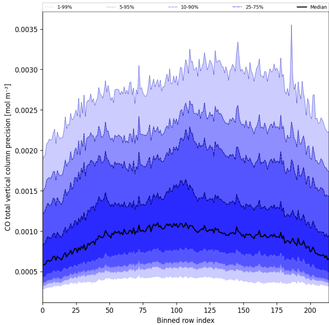
Figure 22: Along track statistics of “CO total vertical column precision” for 2025-02-05 to 2025-02-06
