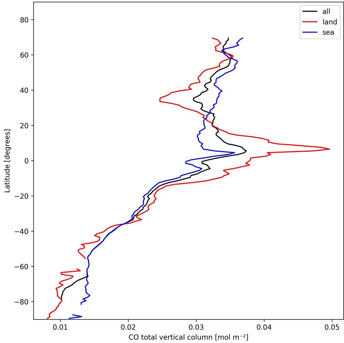
Figure 7: Zonal average of “CO total vertical column” for 2025-02-05 to 2025-02-06.
