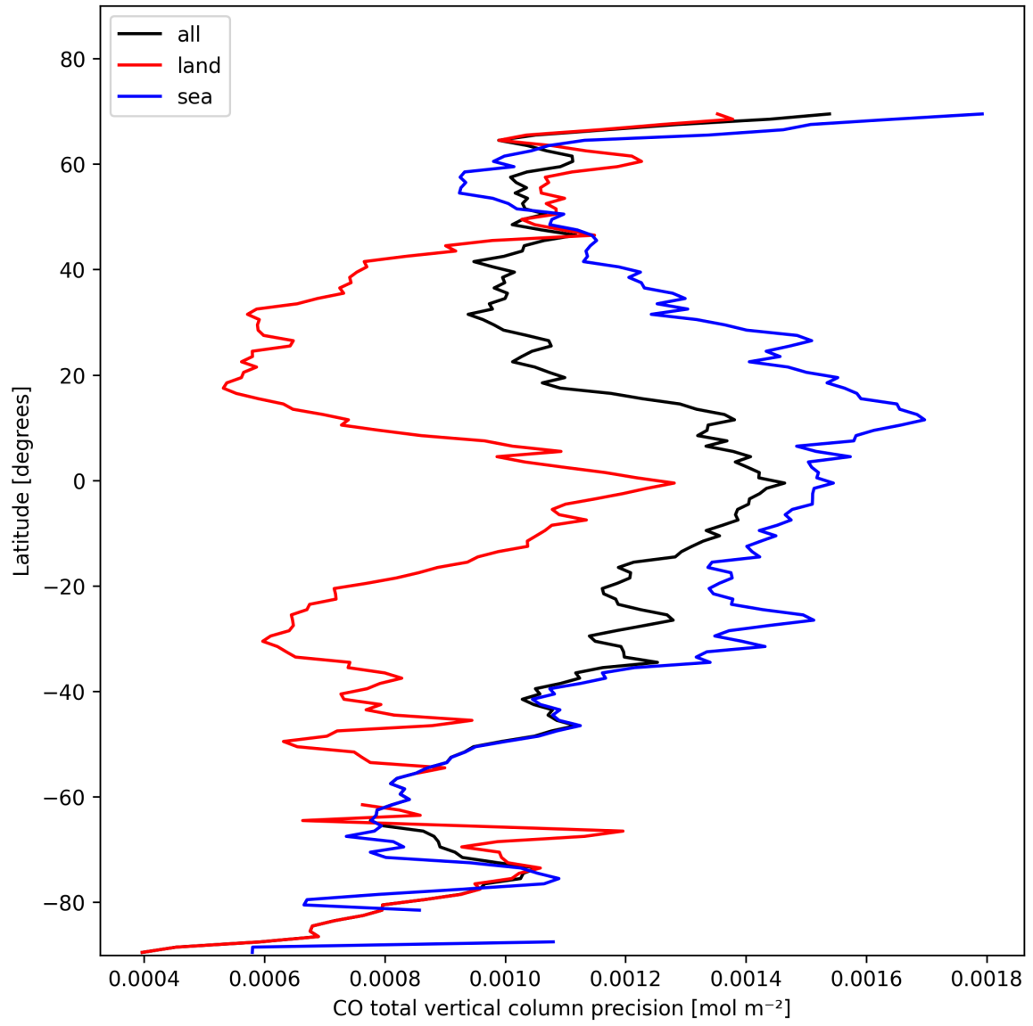
Figure 8: Zonal average of “CO total vertical column precision” for 2025-02-05 to 2025-02-06.
