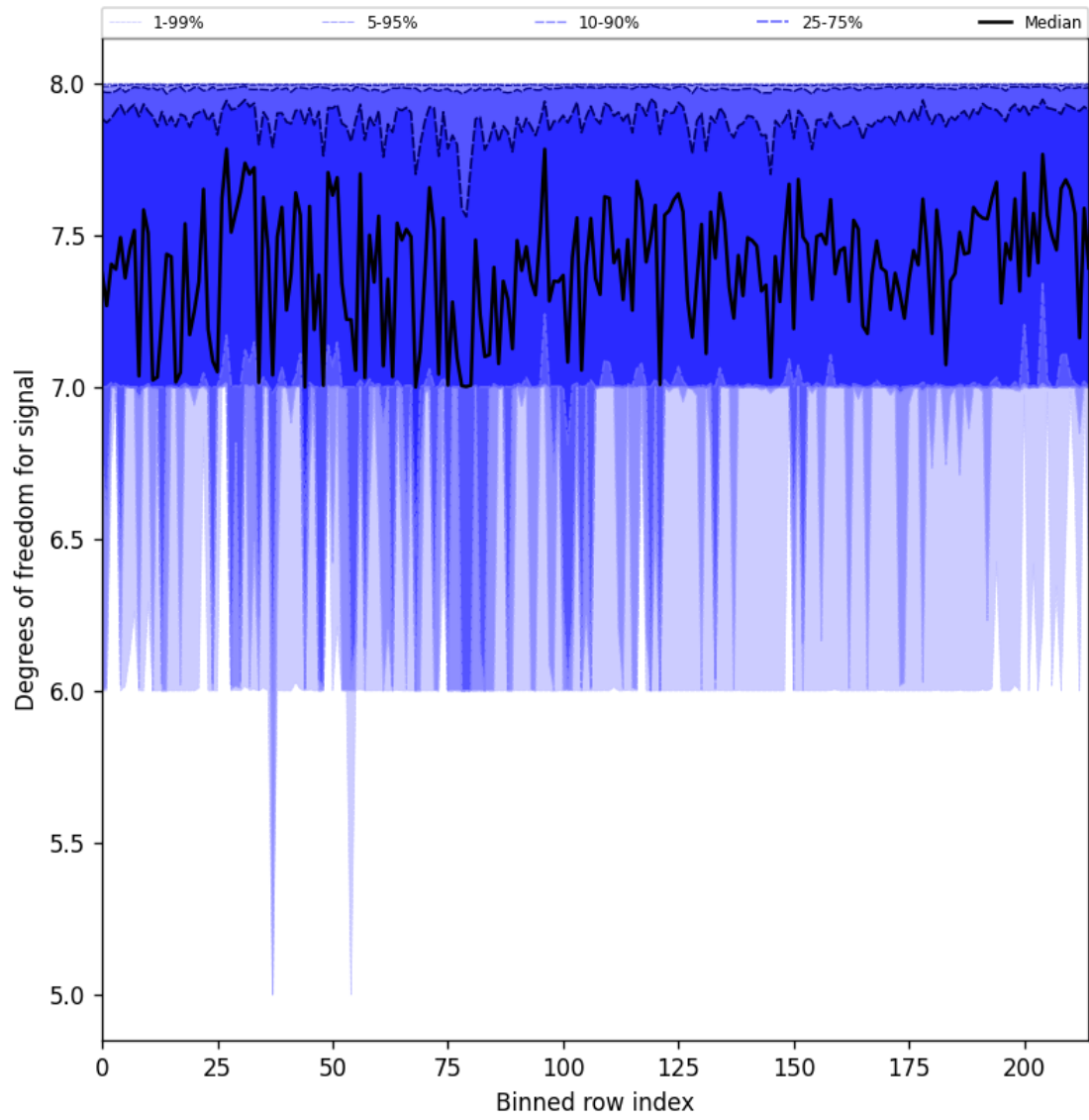
Figure 25: Along track statistics of “Degrees of freedom for signal” for 2025-02-05 to 2025-02-06
