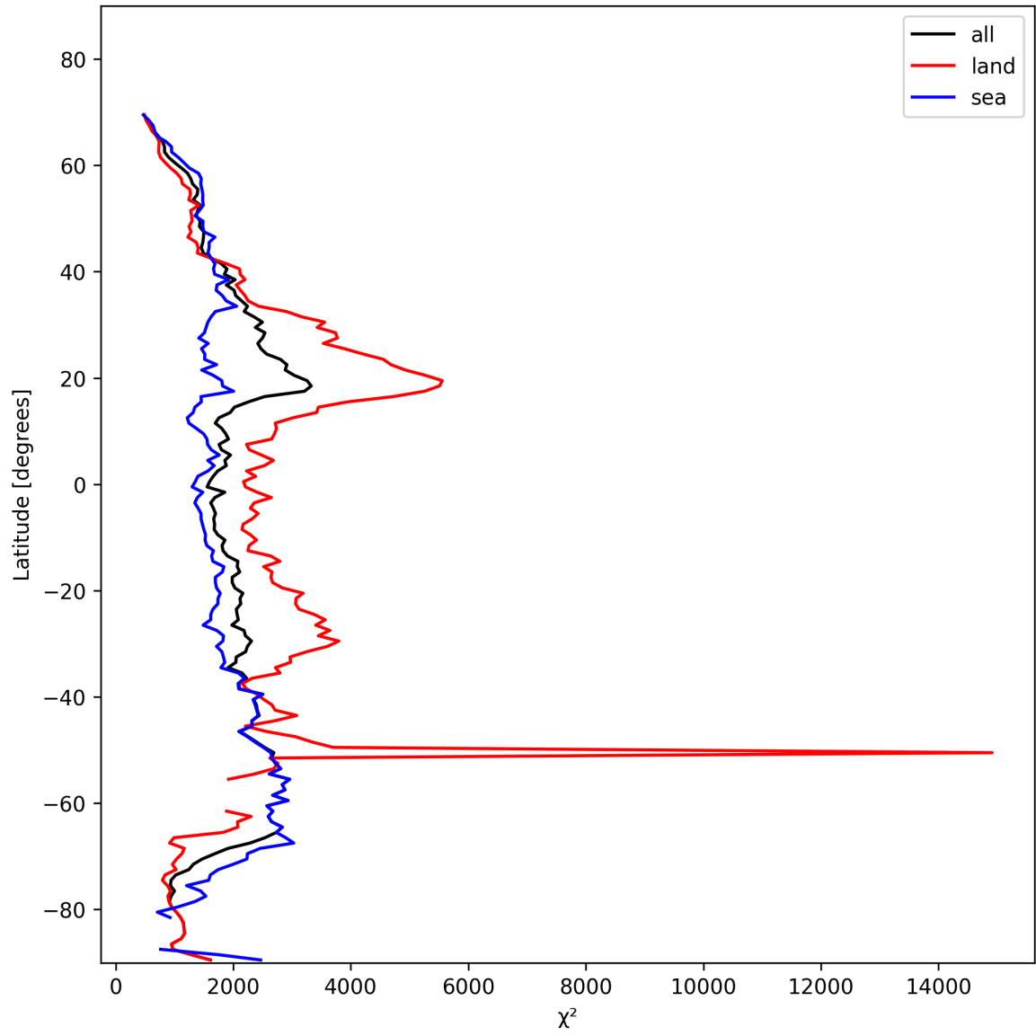
Figure 10: Zonal average of “ \chi^2 ” for 2025-02-05 to 2025-02-06.
