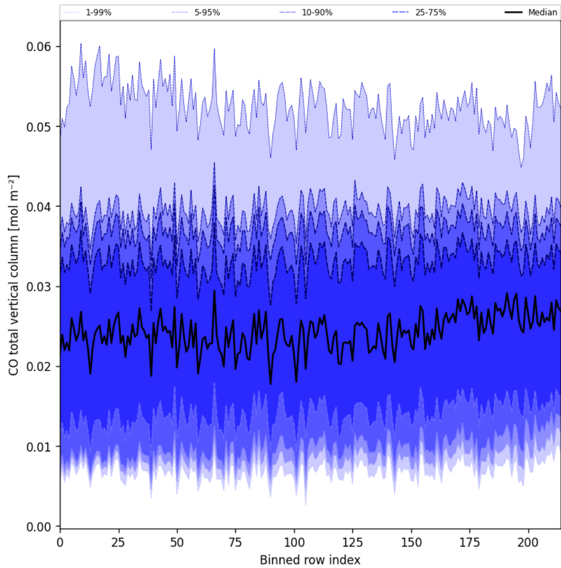
Figure 21: Along track statistics of “CO total vertical column” for 2025-02-05 to 2025-02-06
