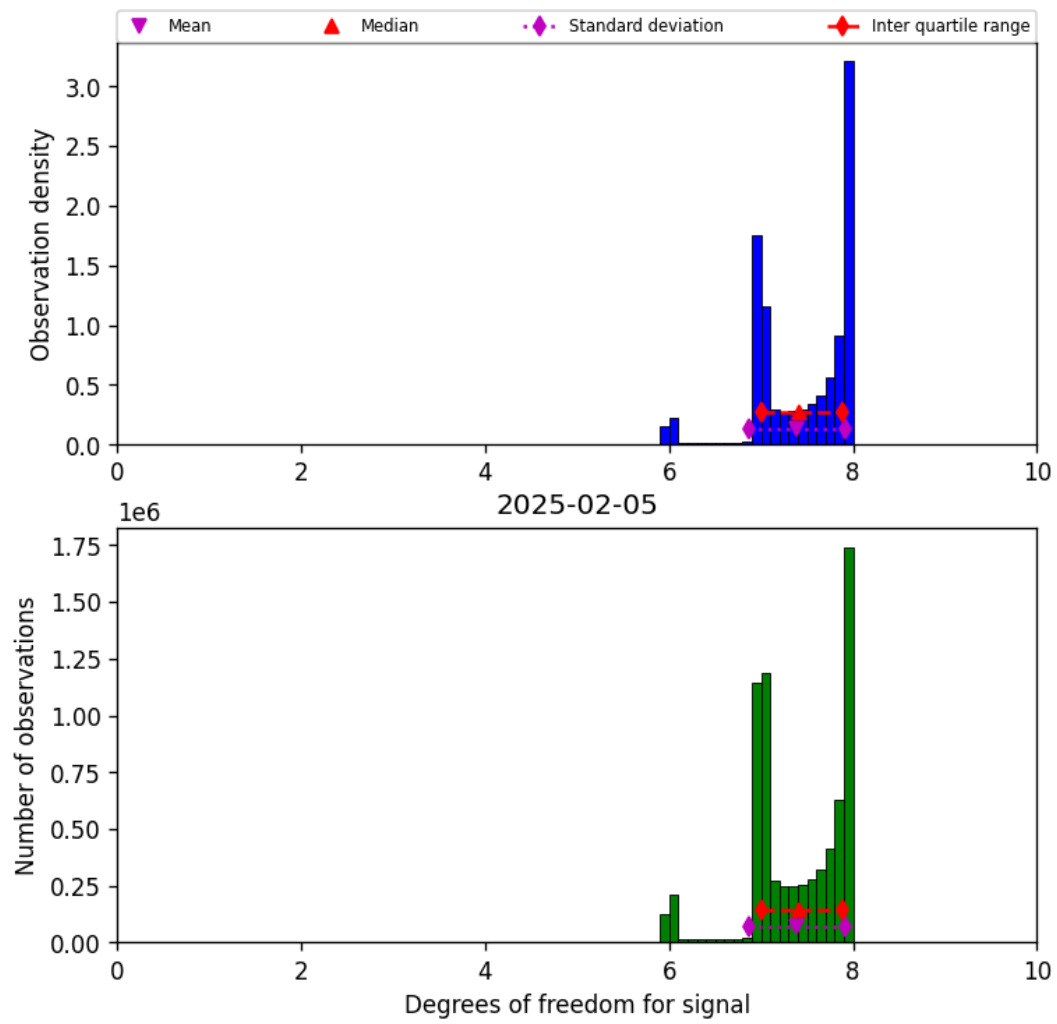
Figure 18: Histogram of “Degrees of freedom for signal” for 2025-02-05 to 2025-02-06
