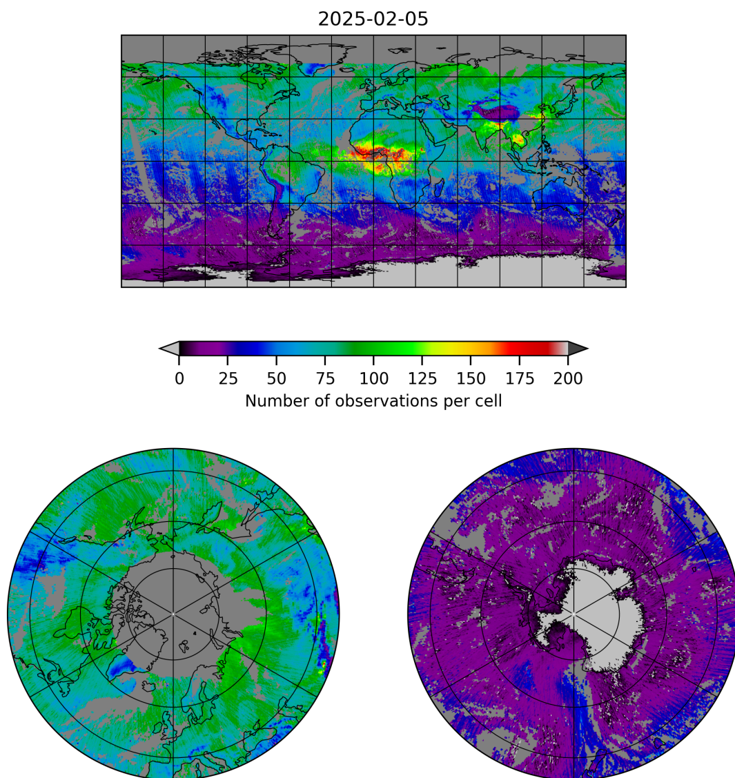
Figure 5: Map of the number of observations for 2025-02-05 to 2025-02-06
