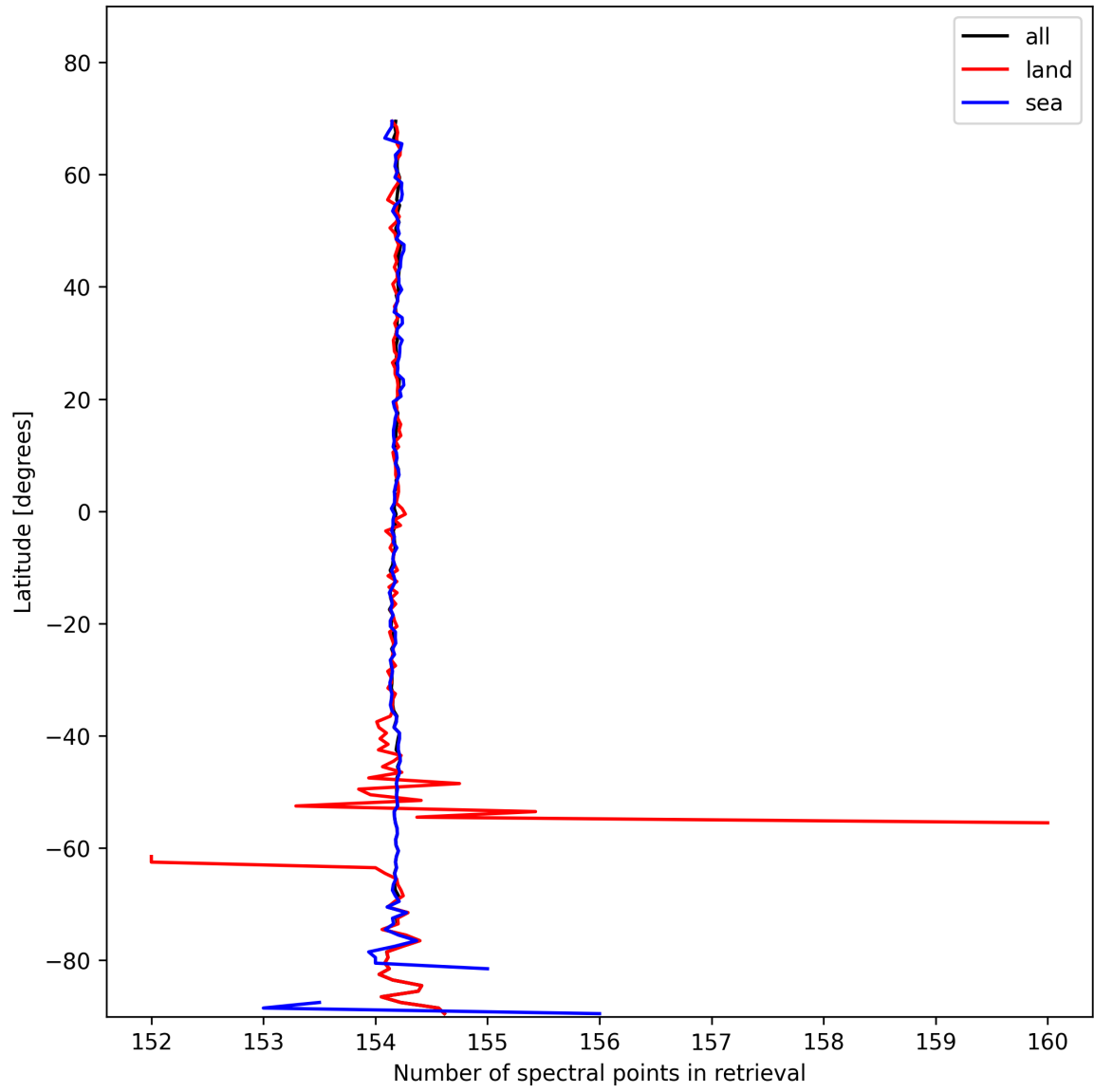
Figure 9: Zonal average of “Number of spectral points in retrieval” for 2025-02-05 to 2025-02-06.
