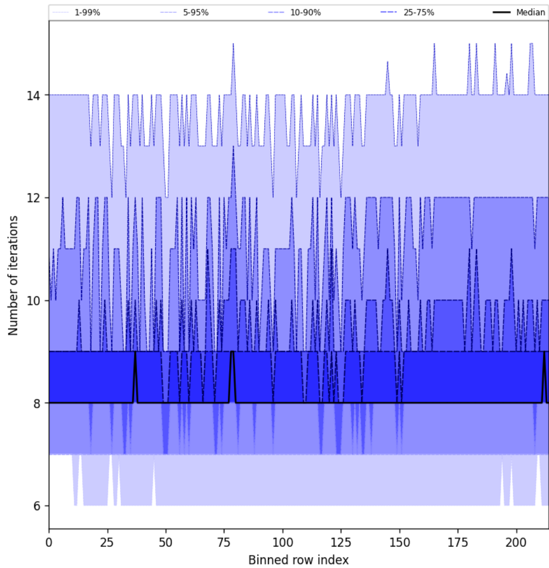
Figure 26: Along track statistics of “Number of iterations” for 2025-02-05 to 2025-02-06
