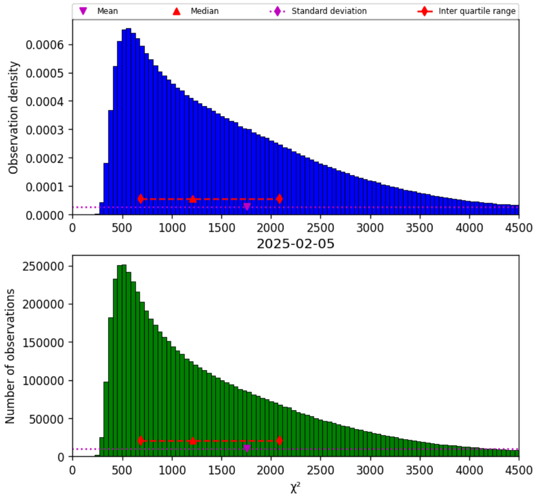
Figure 17: Histogram of “ \chi^2 ” for 2025-02-05 to 2025-02-06
