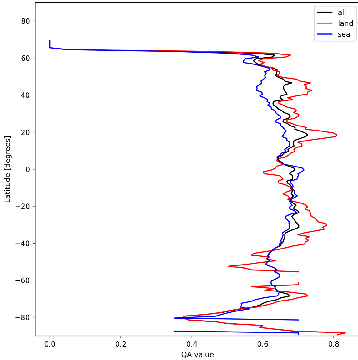
Figure 6: Zonal average of “QA value” for 2025-02-05 to 2025-02-06.
