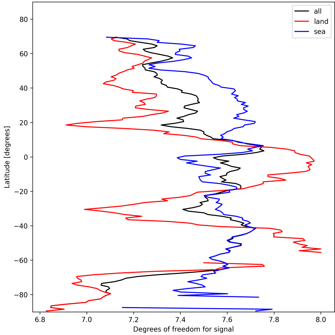
Figure 11: Zonal average of “Degrees of freedom for signal” for 2025-02-05 to 2025-02-06.
