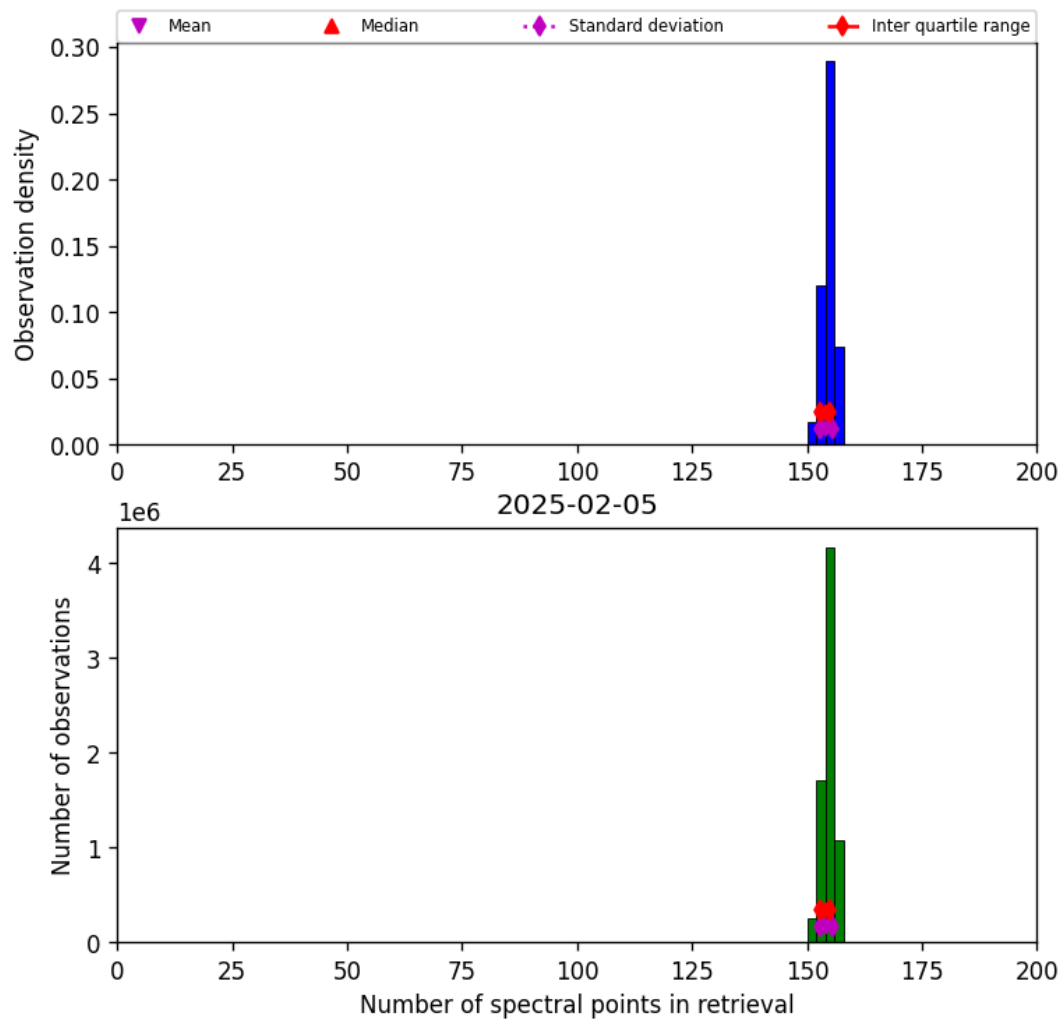
Figure 16: Histogram of “Number of spectral points in retrieval” for 2025-02-05 to 2025-02-06
