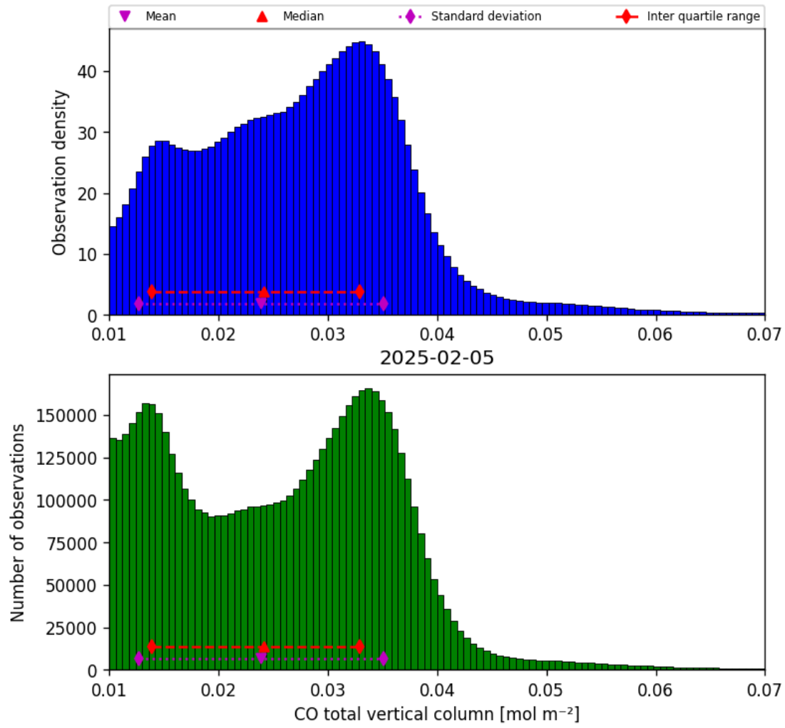
Figure 14: Histogram of “CO total vertical column” for 2025-02-05 to 2025-02-06
