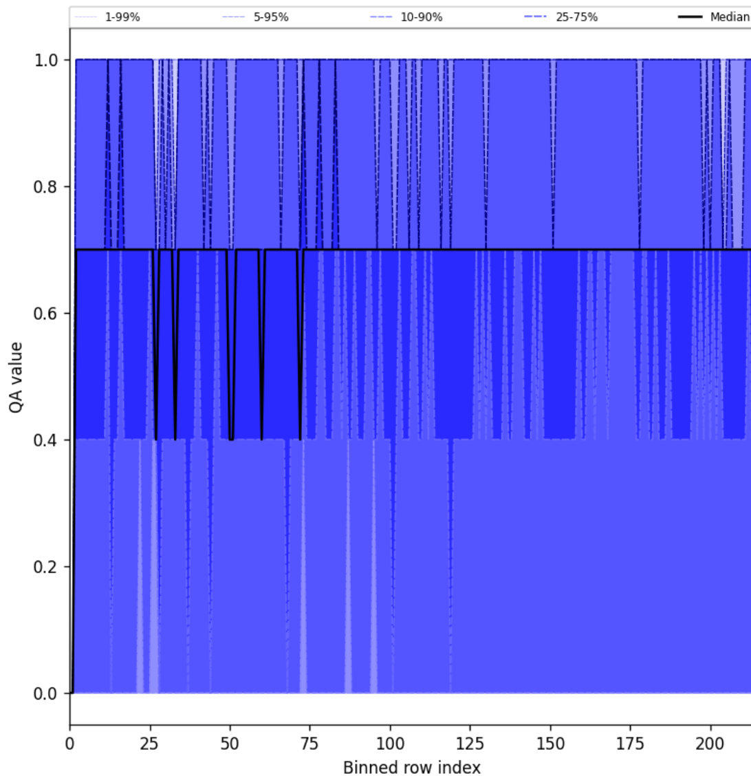
Figure 20: Along track statistics of “QA value” for 2025-02-05 to 2025-02-06
