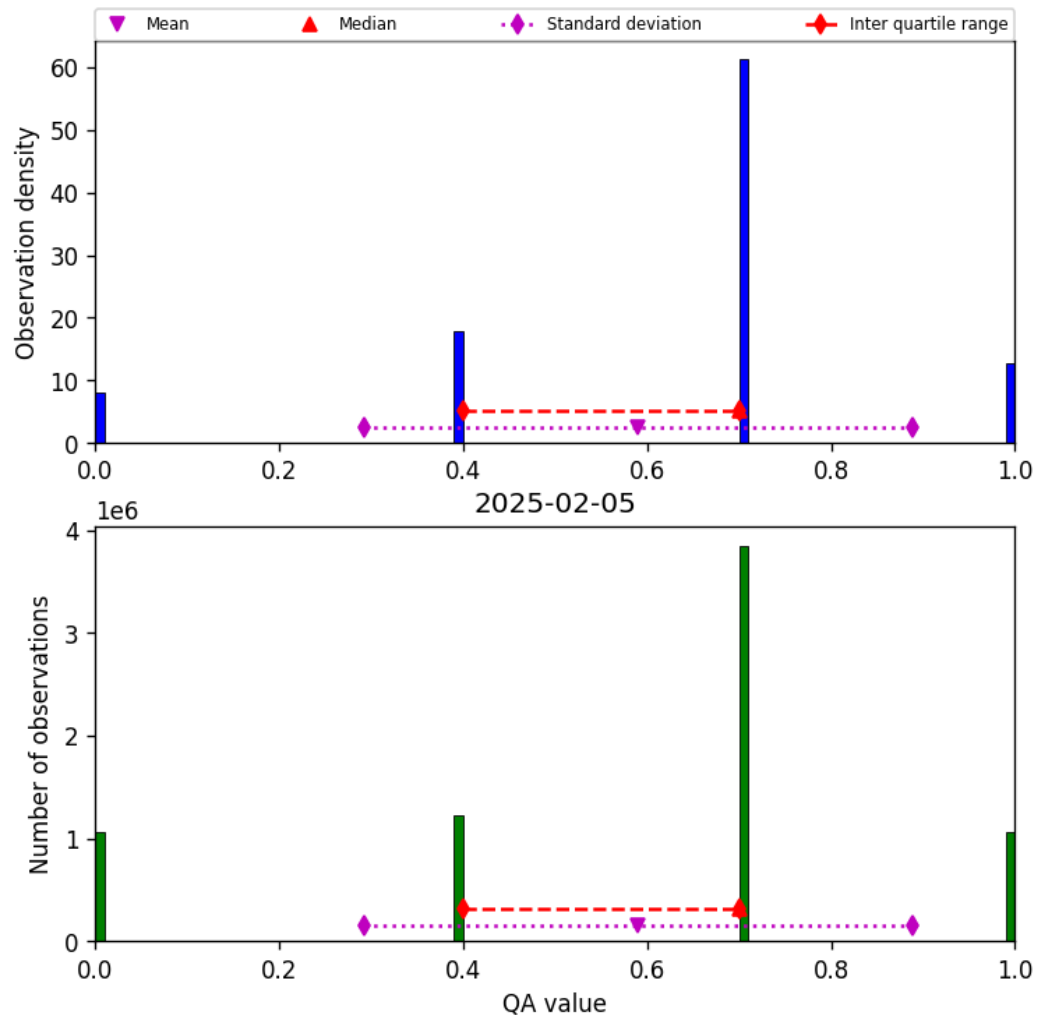
Figure 13: Histogram of “QA value” for 2025-02-05 to 2025-02-06
