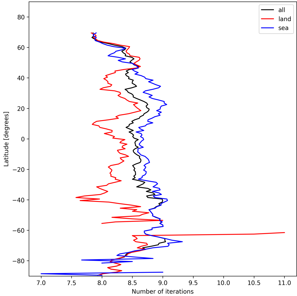
Figure 12: Zonal average of “Number of iterations” for 2025-02-05 to 2025-02-06.
