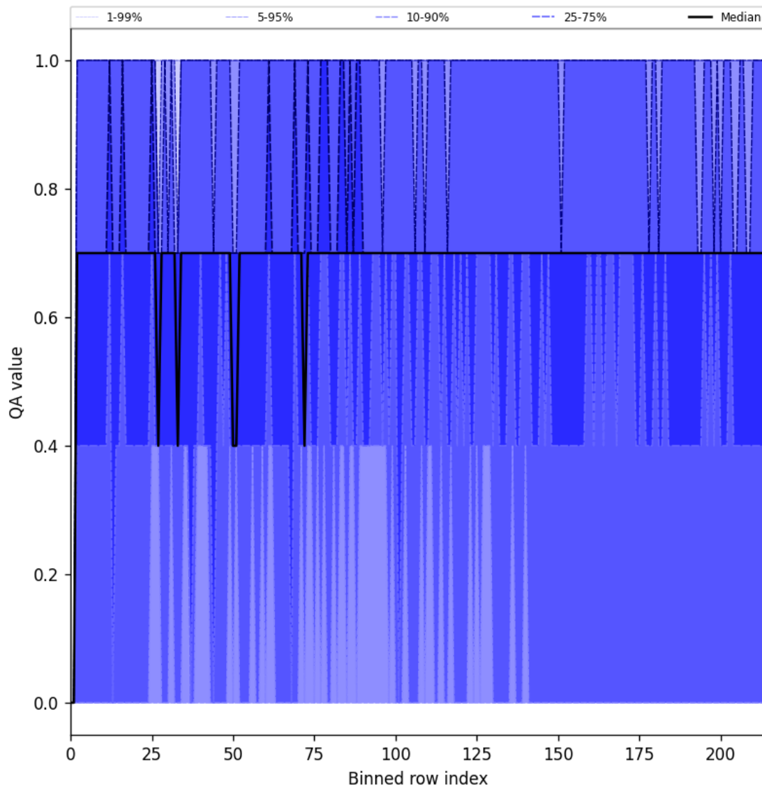
Figure 20: Along track statistics of “QA value” for 2025-02-06 to 2025-02-06
