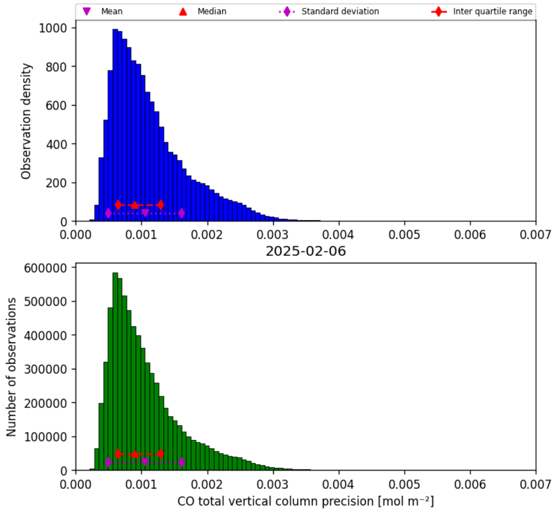
Figure 15: Histogram of “CO total vertical column precision” for 2025-02-06 to 2025-02-06
