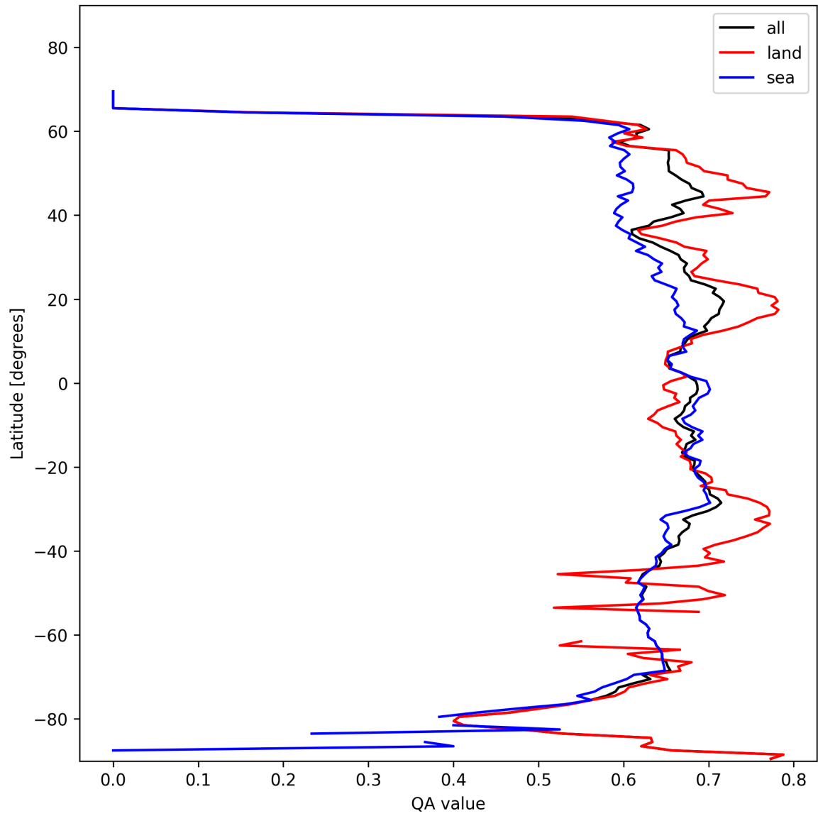
Figure 6: Zonal average of “QA value” for 2025-02-06 to 2025-02-06.
