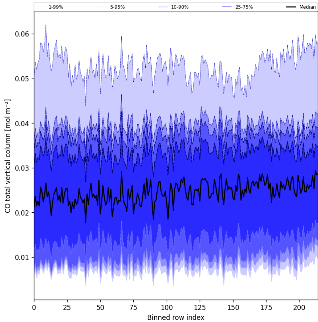
Figure 21: Along track statistics of “CO total vertical column” for 2025-02-06 to 2025-02-06
