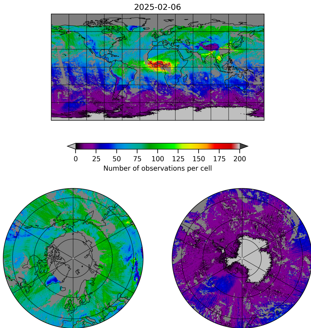
Figure 5: Map of the number of observations for 2025-02-06 to 2025-02-06
