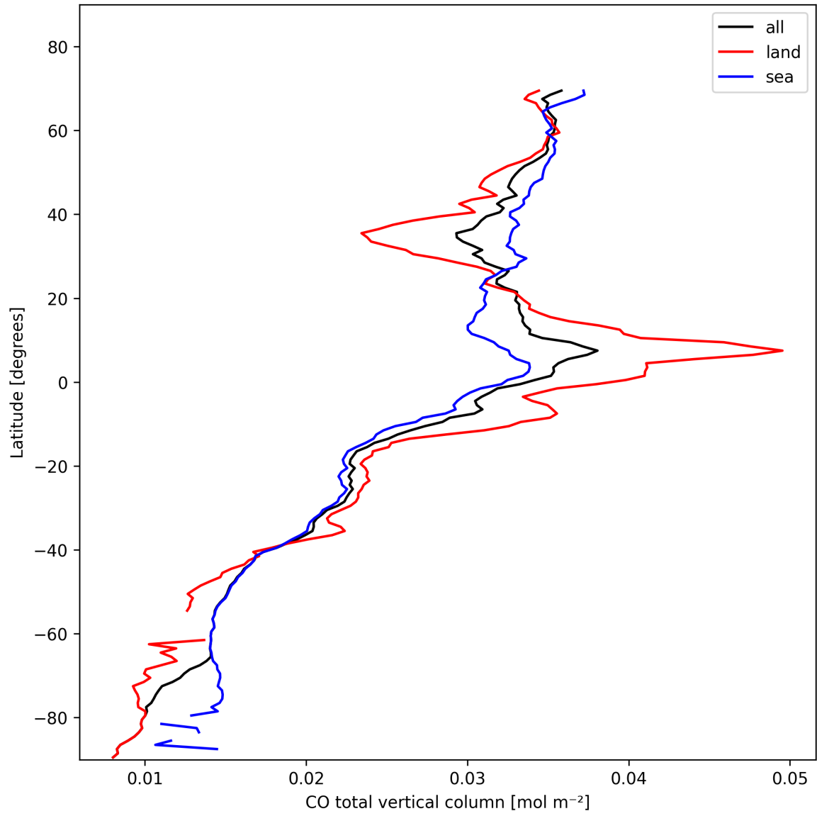
Figure 7: Zonal average of “CO total vertical column” for 2025-02-06 to 2025-02-06.
