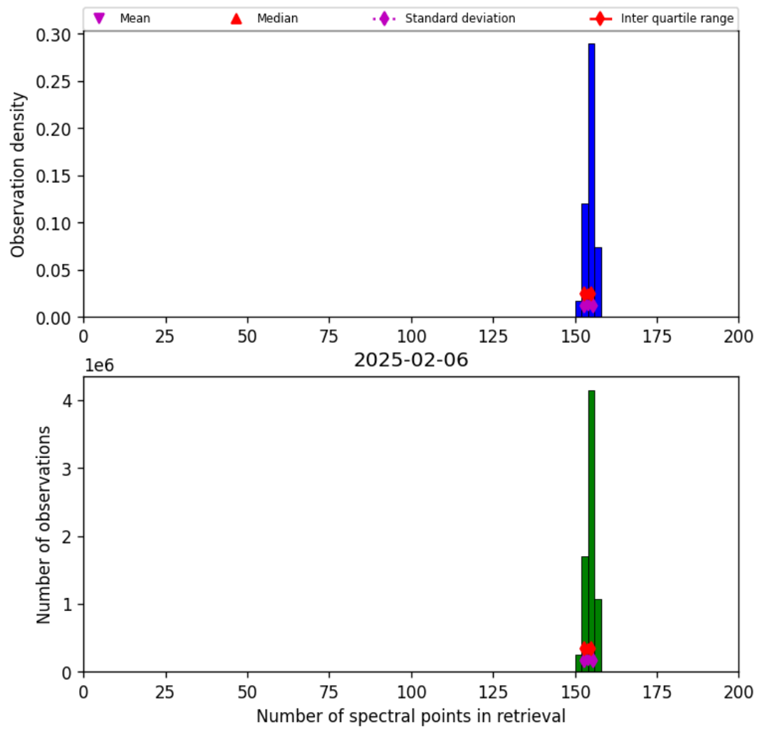
Figure 16: Histogram of “Number of spectral points in retrieval” for 2025-02-06 to 2025-02-06
