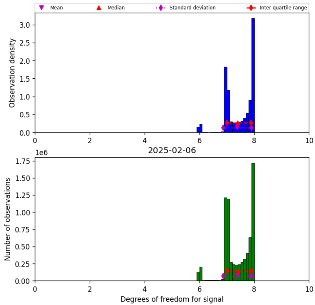
Figure 18: Histogram of “Degrees of freedom for signal” for 2025-02-06 to 2025-02-06
