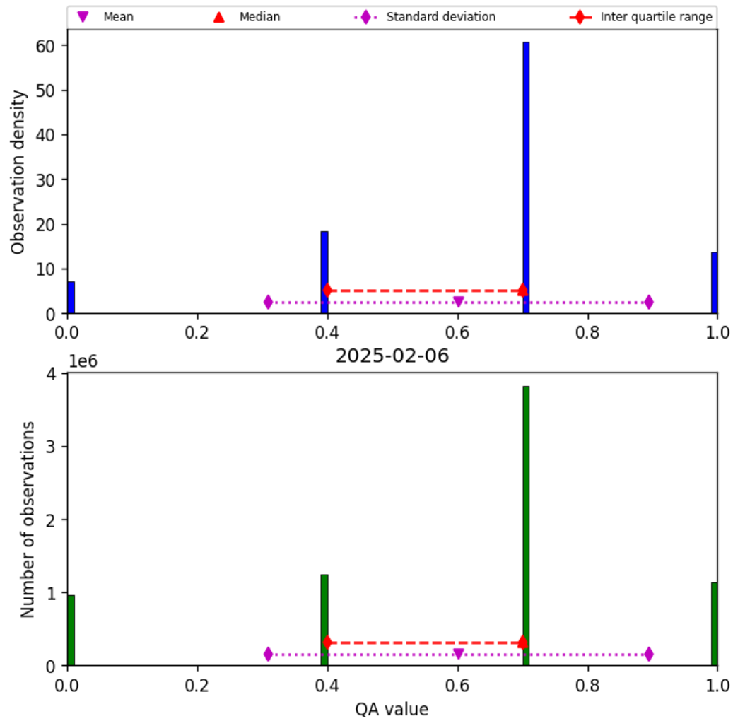
Figure 13: Histogram of “QA value” for 2025-02-06 to 2025-02-06
