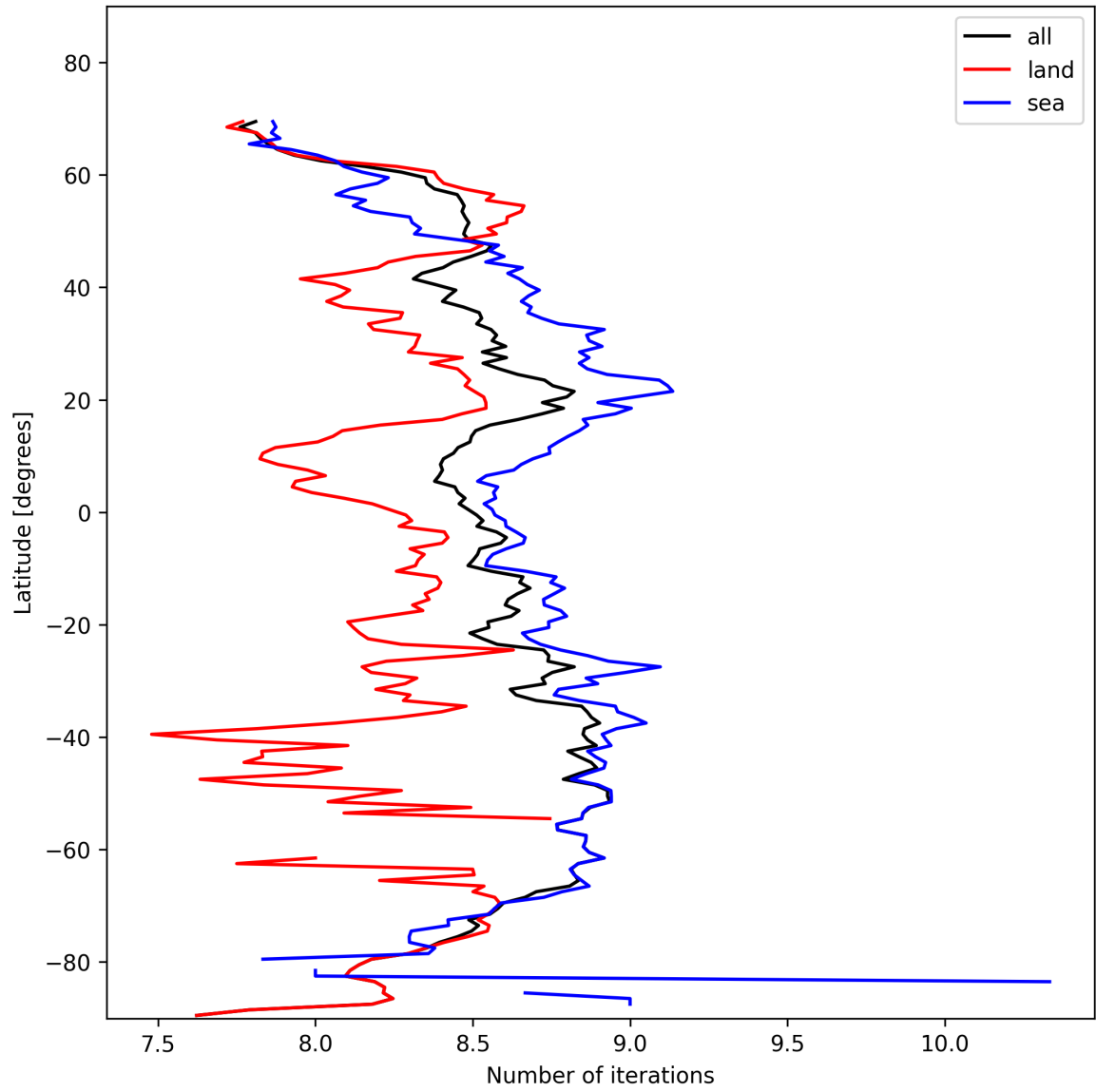
Figure 12: Zonal average of “Number of iterations” for 2025-02-06 to 2025-02-06.
