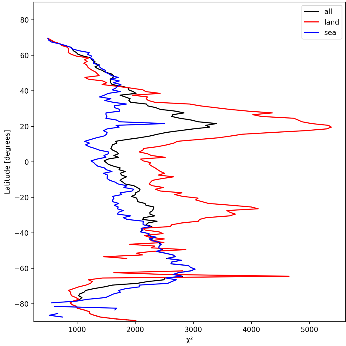
Figure 10: Zonal average of “ \chi^2 ” for 2025-02-06 to 2025-02-06.
