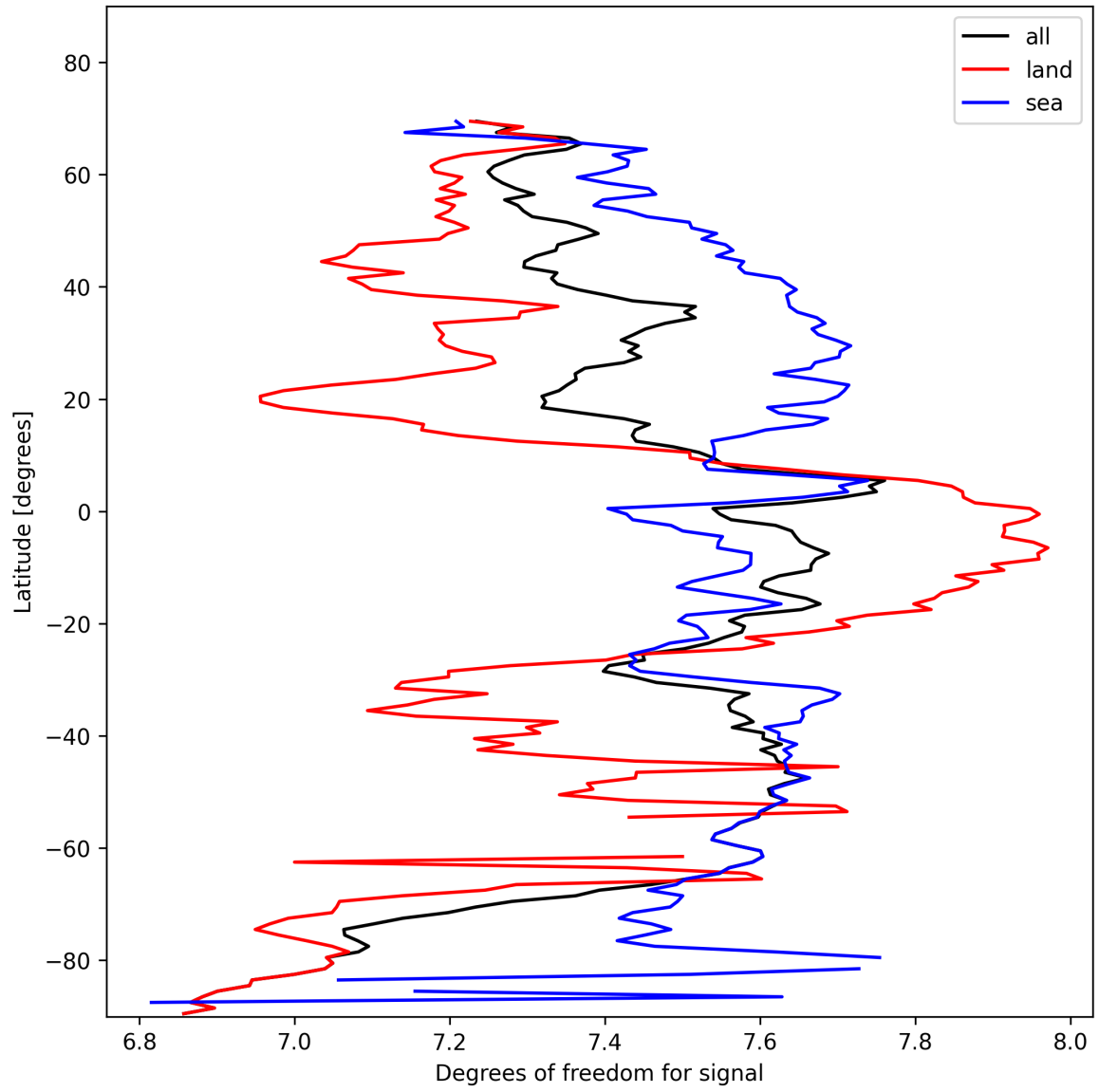
Figure 11: Zonal average of “Degrees of freedom for signal” for 2025-02-06 to 2025-02-06.
