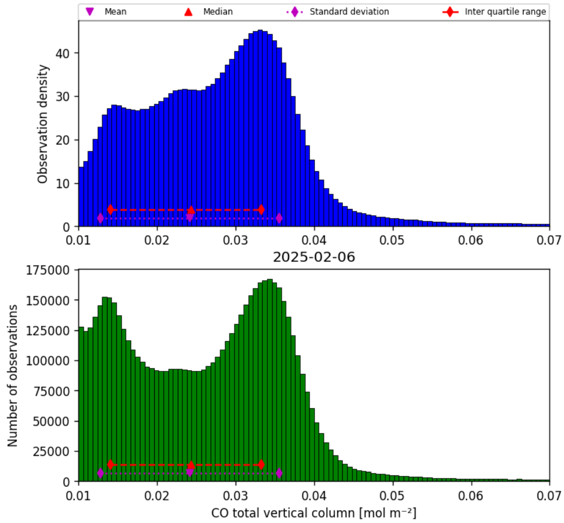
Figure 14: Histogram of “CO total vertical column” for 2025-02-06 to 2025-02-06
