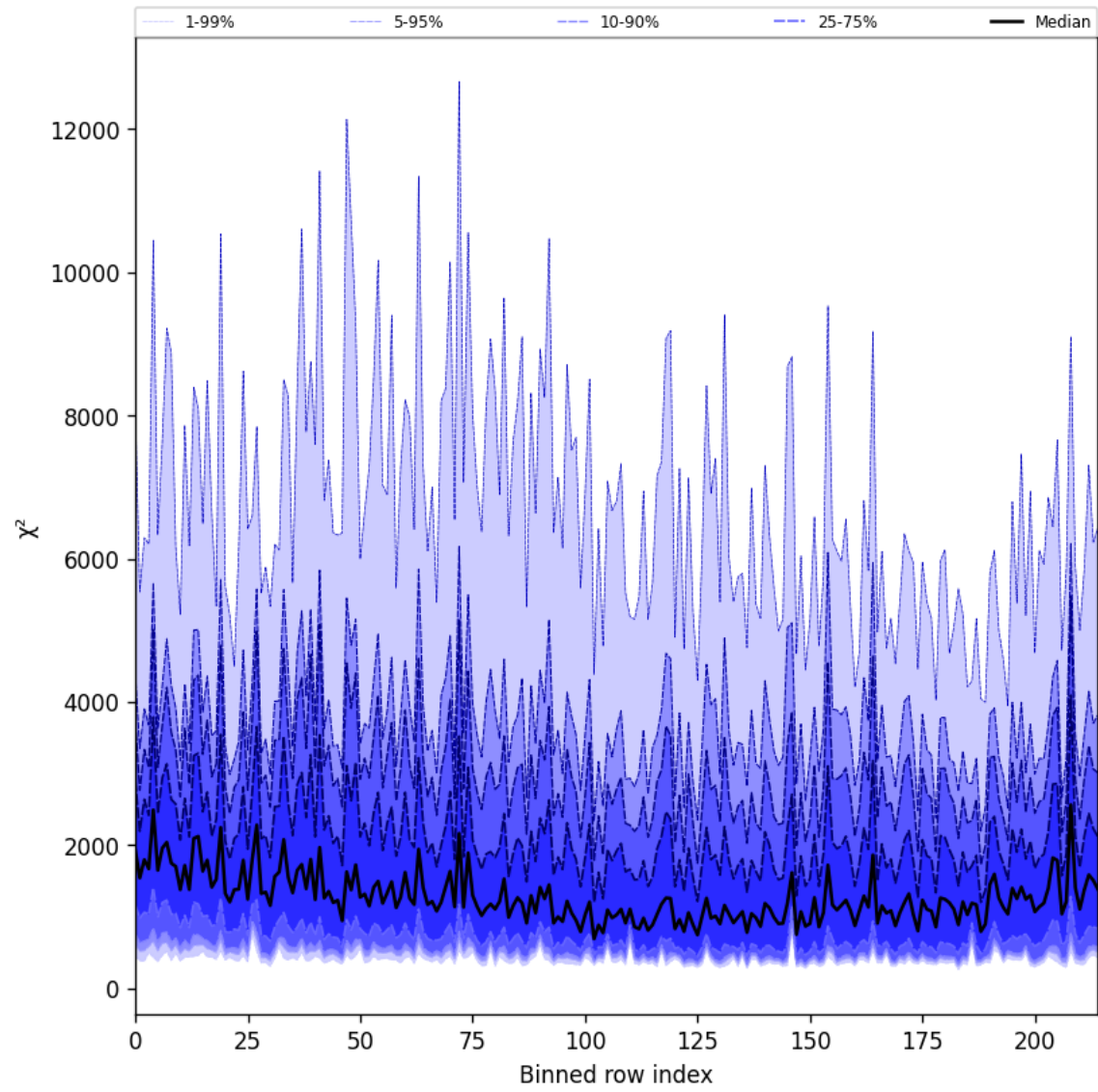
Figure 24: Along track statistics of “ \chi^2 ” for 2025-02-06 to 2025-02-06
