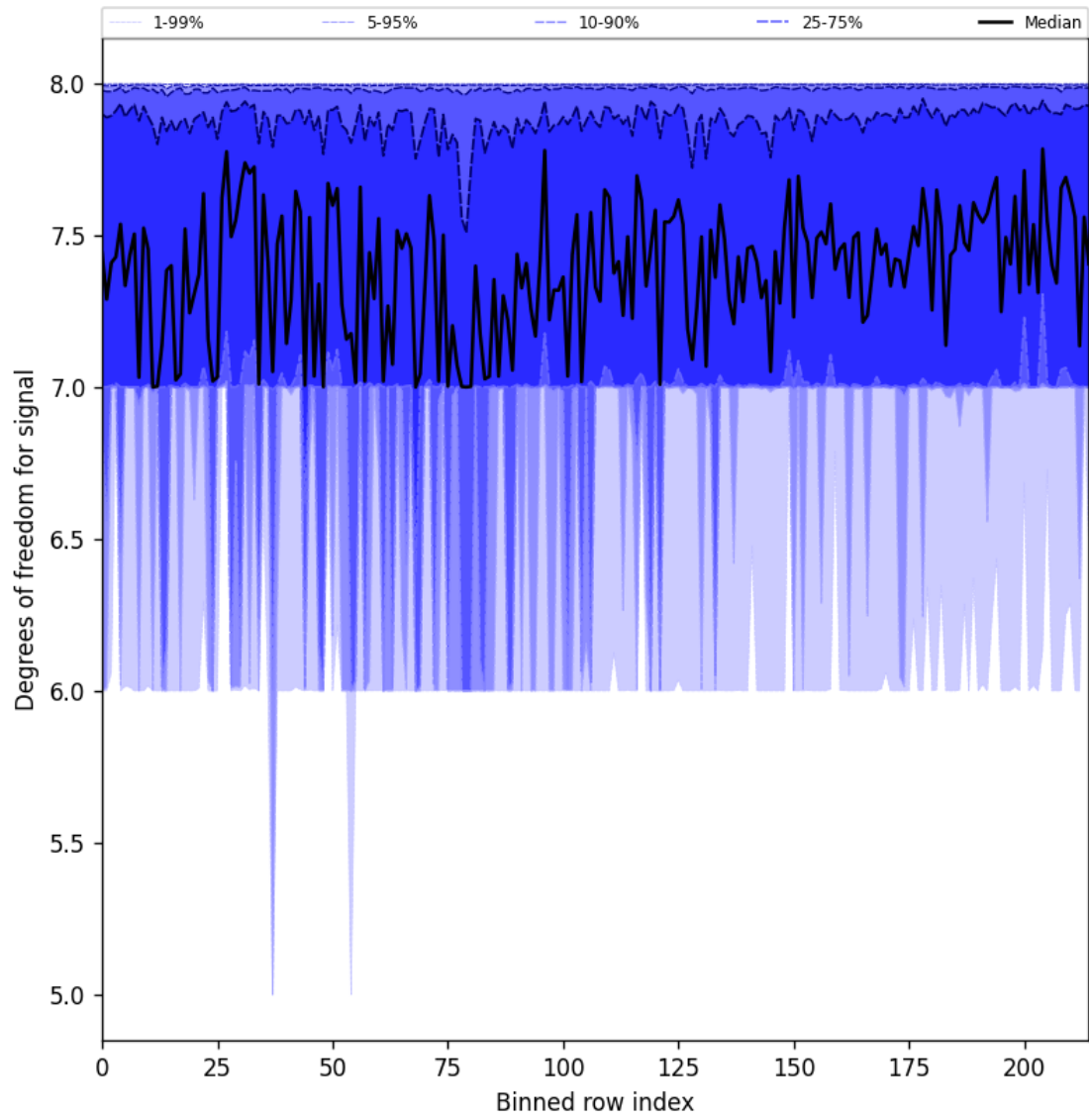
Figure 25: Along track statistics of “Degrees of freedom for signal” for 2025-02-06 to 2025-02-06
