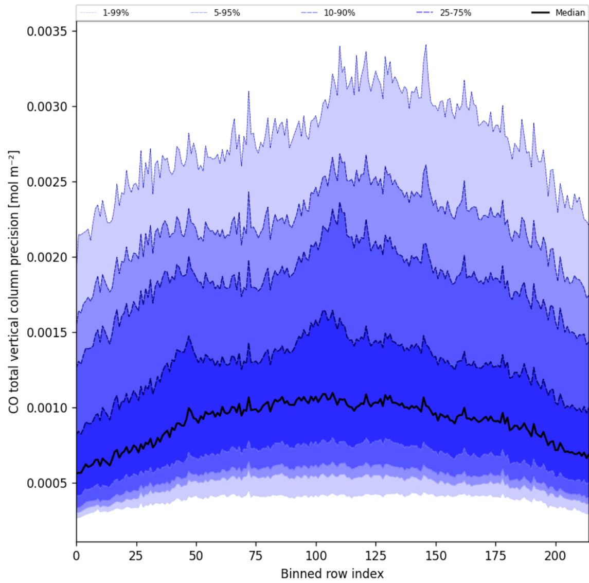
Figure 22: Along track statistics of “CO total vertical column precision” for 2025-02-06 to 2025-02-06
