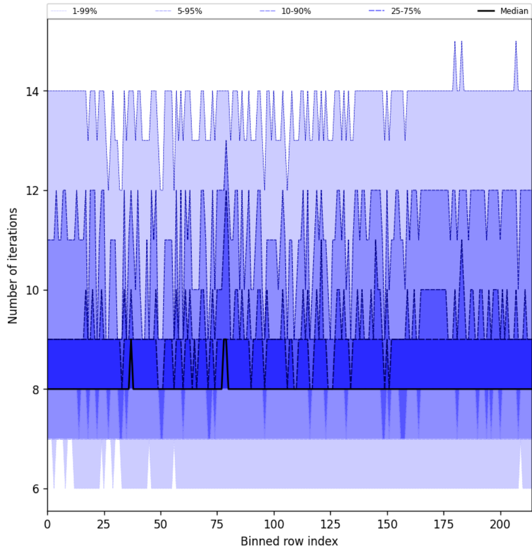
Figure 26: Along track statistics of “Number of iterations” for 2025-02-06 to 2025-02-06
