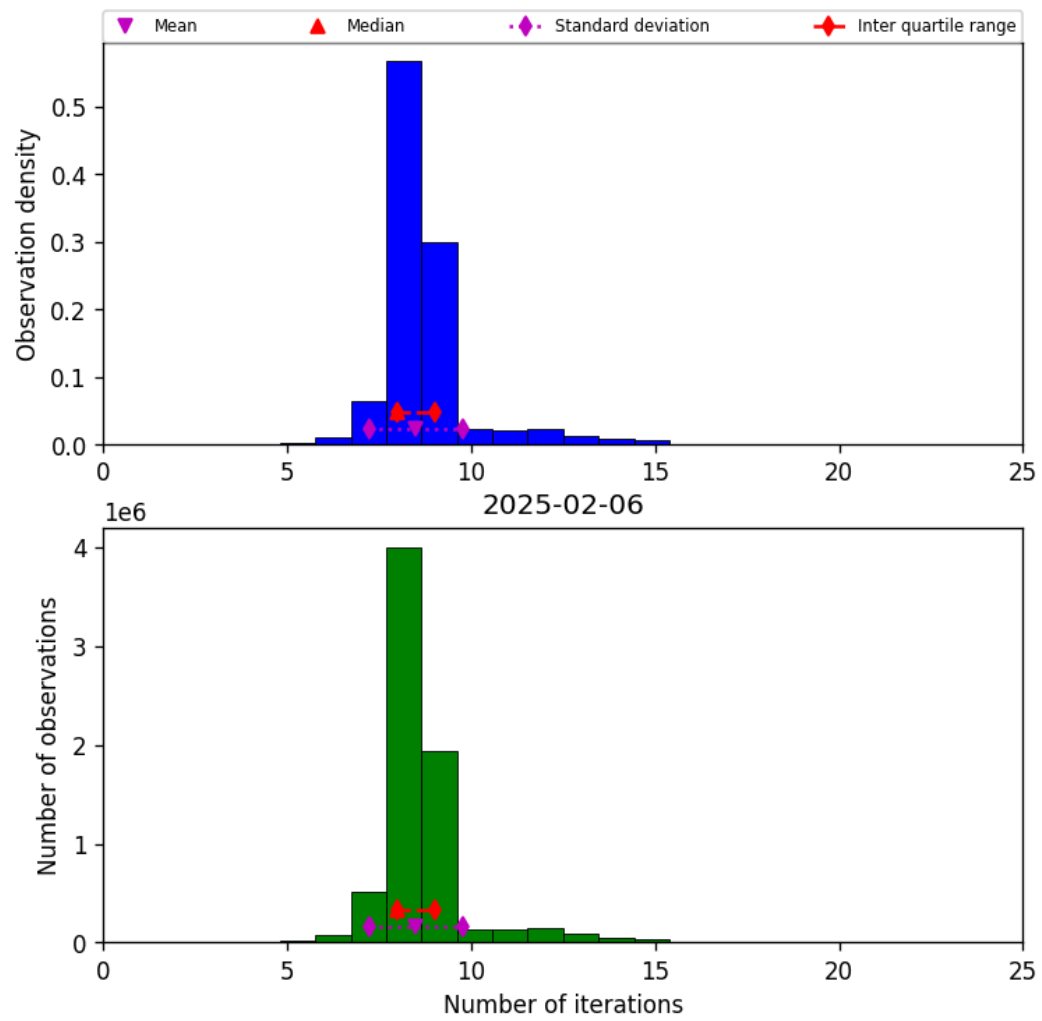
Figure 19: Histogram of “Number of iterations” for 2025-02-06 to 2025-02-06
