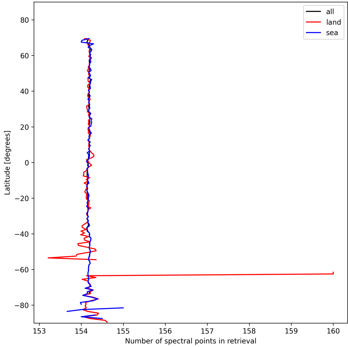
Figure 9: Zonal average of “Number of spectral points in retrieval” for 2025-02-06 to 2025-02-06.
