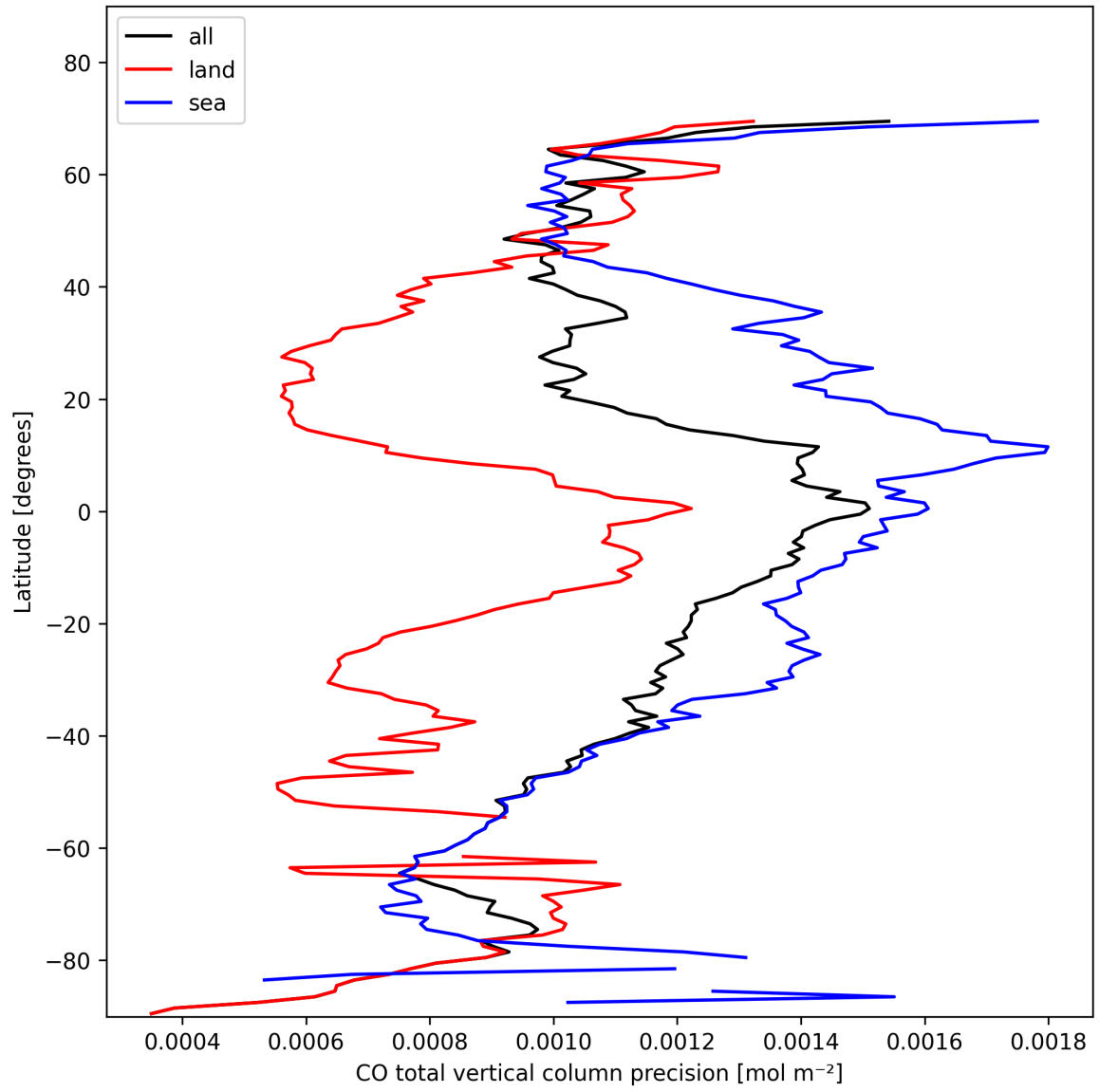
Figure 8: Zonal average of “CO total vertical column precision” for 2025-02-06 to 2025-02-06.
