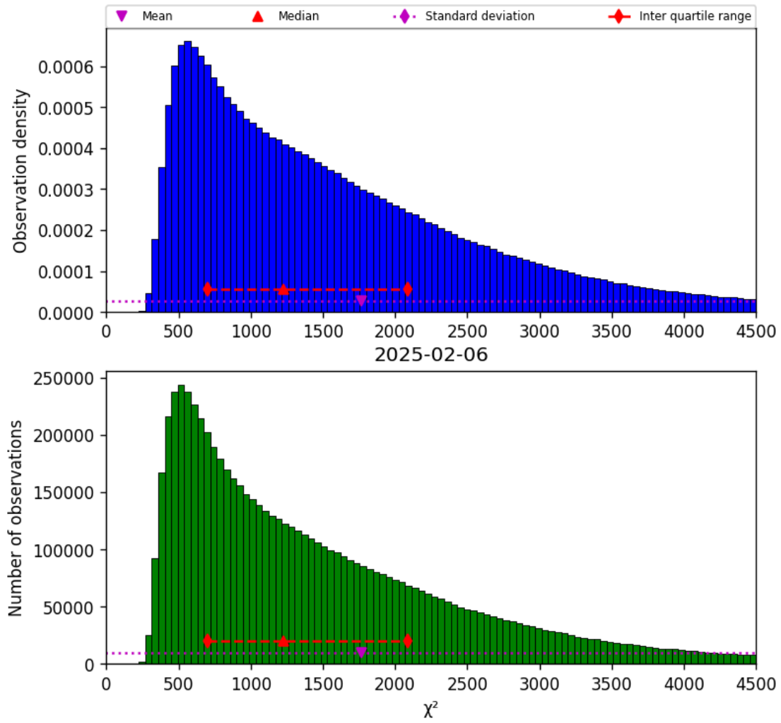
Figure 17: Histogram of “ \chi^2 ” for 2025-02-06 to 2025-02-06
