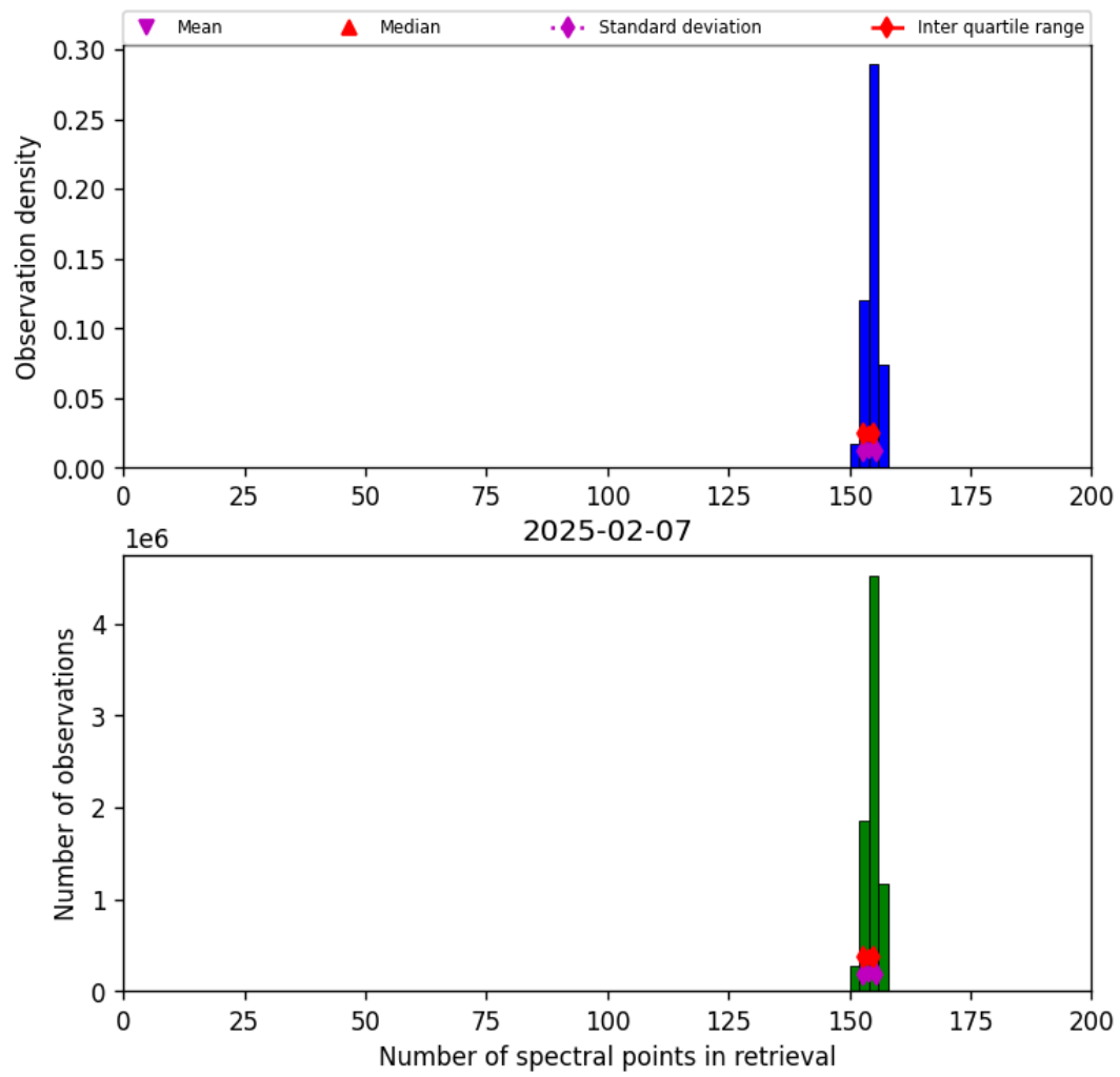
Figure 16: Histogram of “Number of spectral points in retrieval” for 2025-02-07 to 2025-02-08
