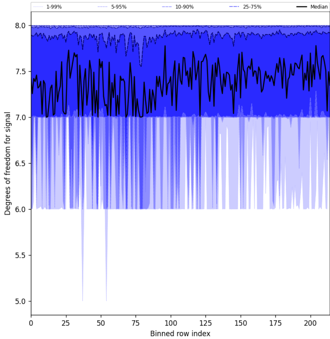
Figure 25: Along track statistics of “Degrees of freedom for signal” for 2025-02-07 to 2025-02-08
