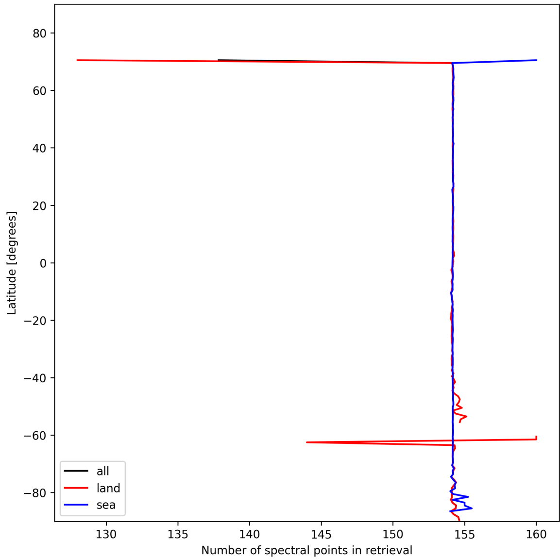
Figure 9: Zonal average of “Number of spectral points in retrieval” for 2025-02-07 to 2025-02-08.
