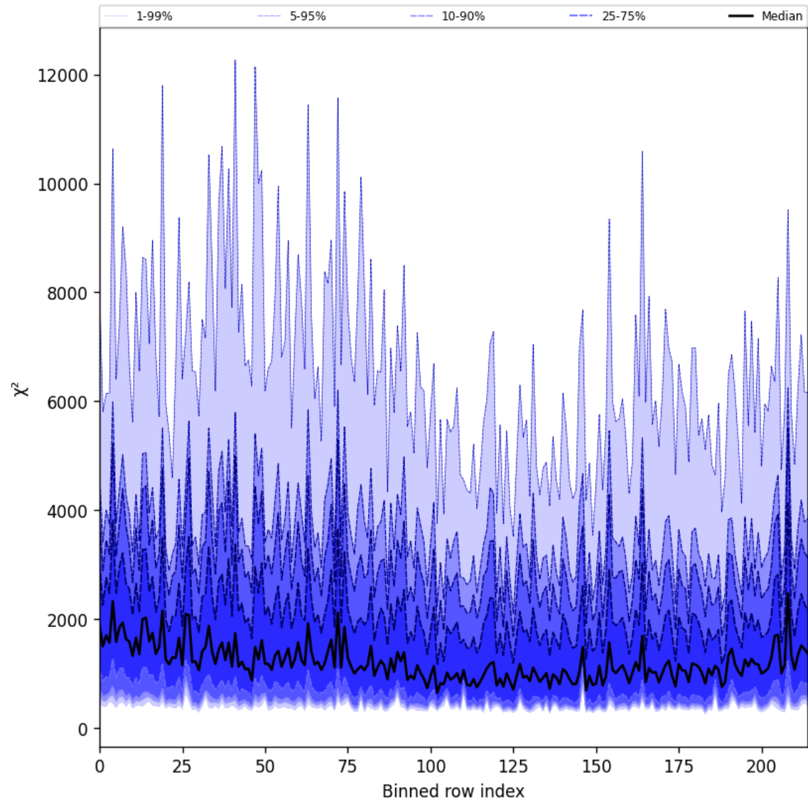
Figure 24: Along track statistics of “ \chi^2 ” for 2025-02-07 to 2025-02-08
