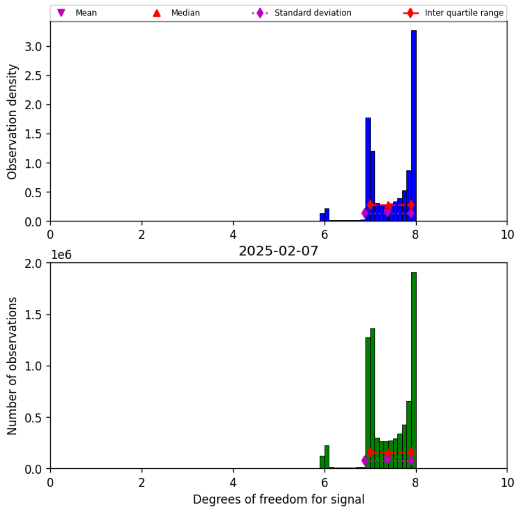
Figure 18: Histogram of “Degrees of freedom for signal” for 2025-02-07 to 2025-02-08
