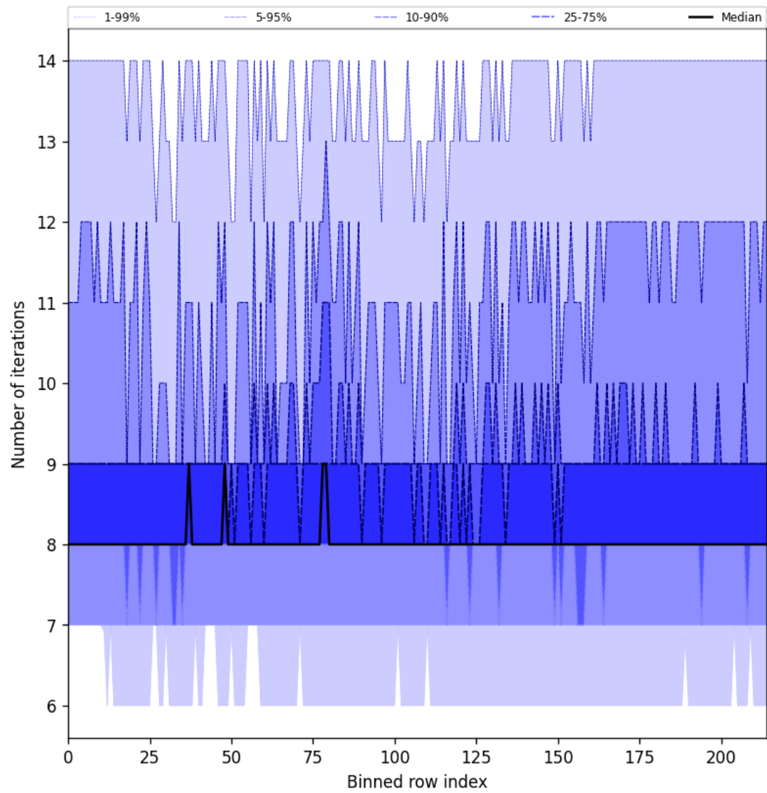
Figure 26: Along track statistics of “Number of iterations” for 2025-02-07 to 2025-02-08
