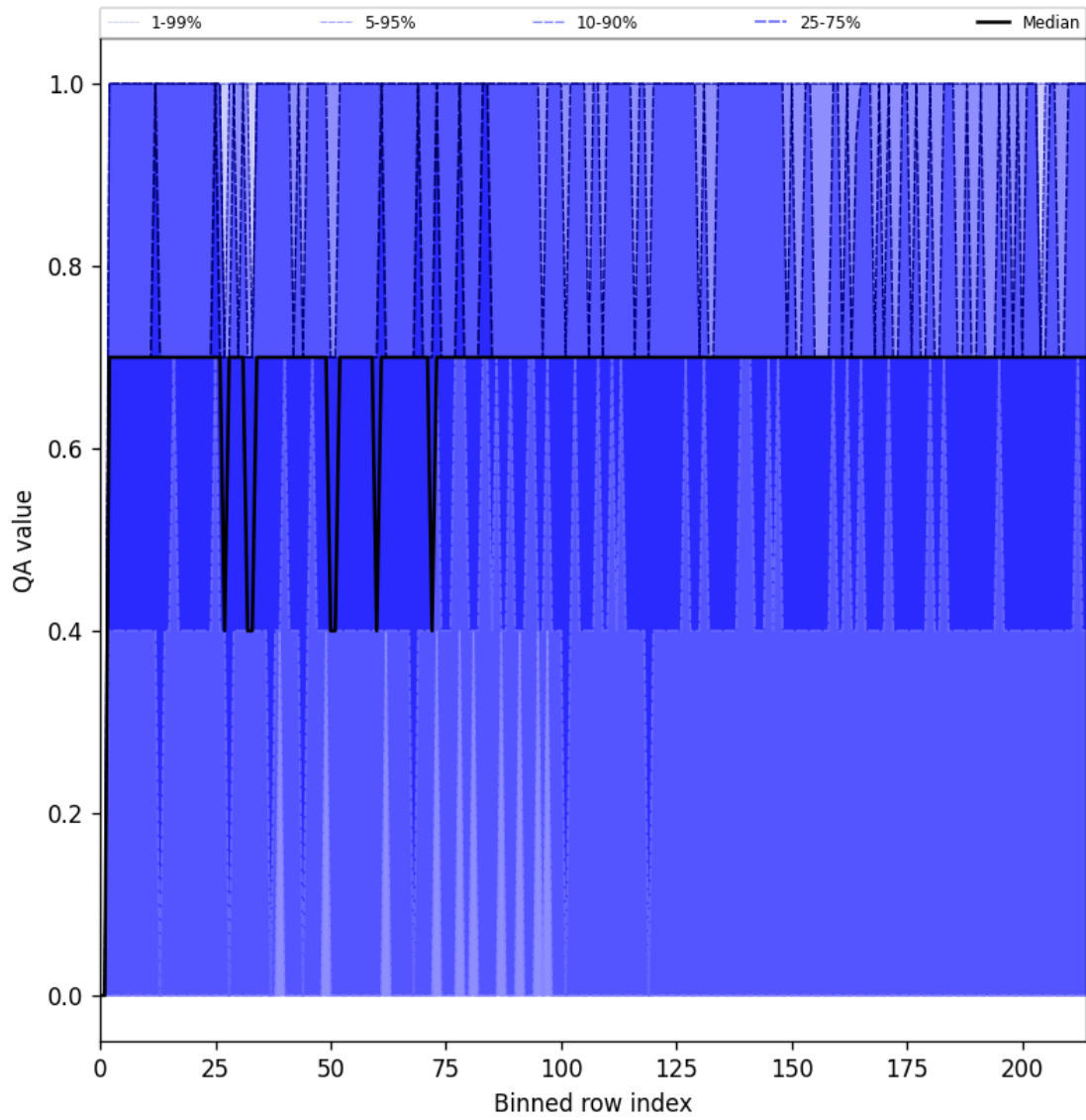
Figure 20: Along track statistics of “QA value” for 2025-02-07 to 2025-02-08
