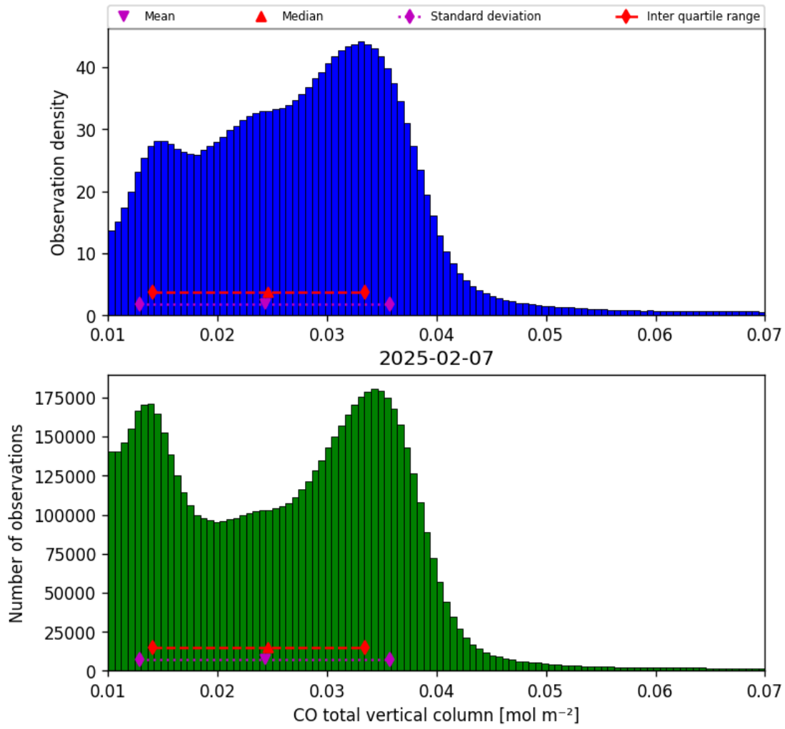
Figure 14: Histogram of “CO total vertical column” for 2025-02-07 to 2025-02-08
