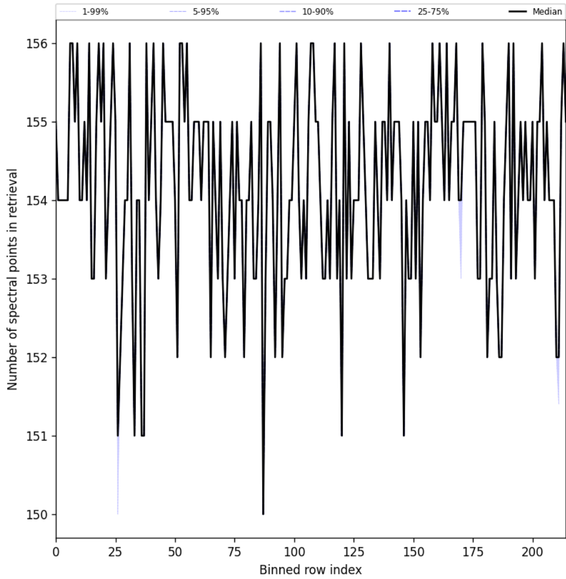
Figure 23: Along track statistics of “Number of spectral points in retrieval” for 2025-02-07 to 2025-02-08
