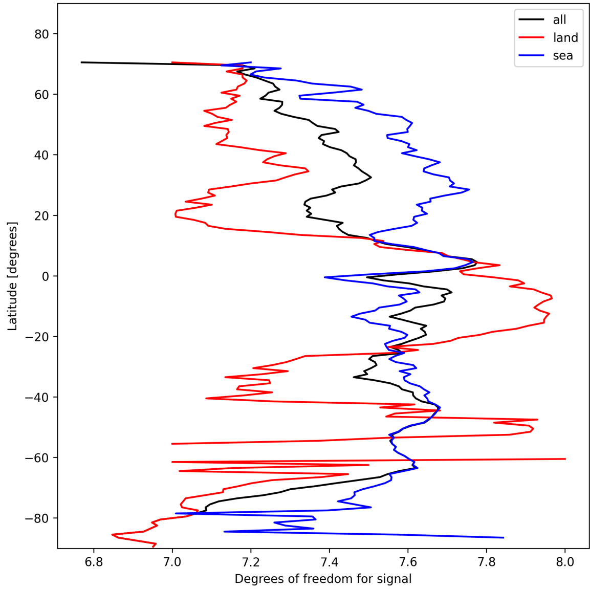
Figure 11: Zonal average of “Degrees of freedom for signal” for 2025-02-07 to 2025-02-08.
