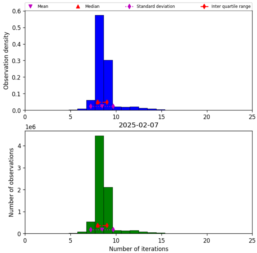
Figure 19: Histogram of “Number of iterations” for 2025-02-07 to 2025-02-08
