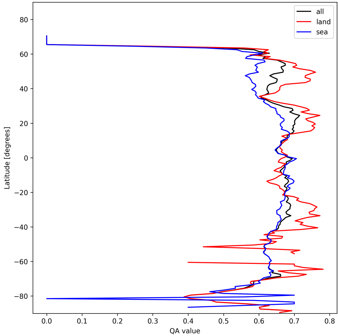
Figure 6: Zonal average of “QA value” for 2025-02-07 to 2025-02-08.
