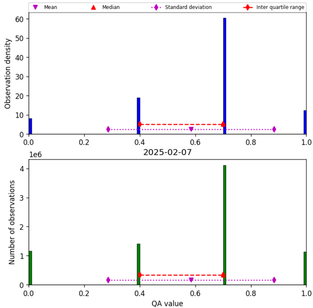
Figure 13: Histogram of “QA value” for 2025-02-07 to 2025-02-08
