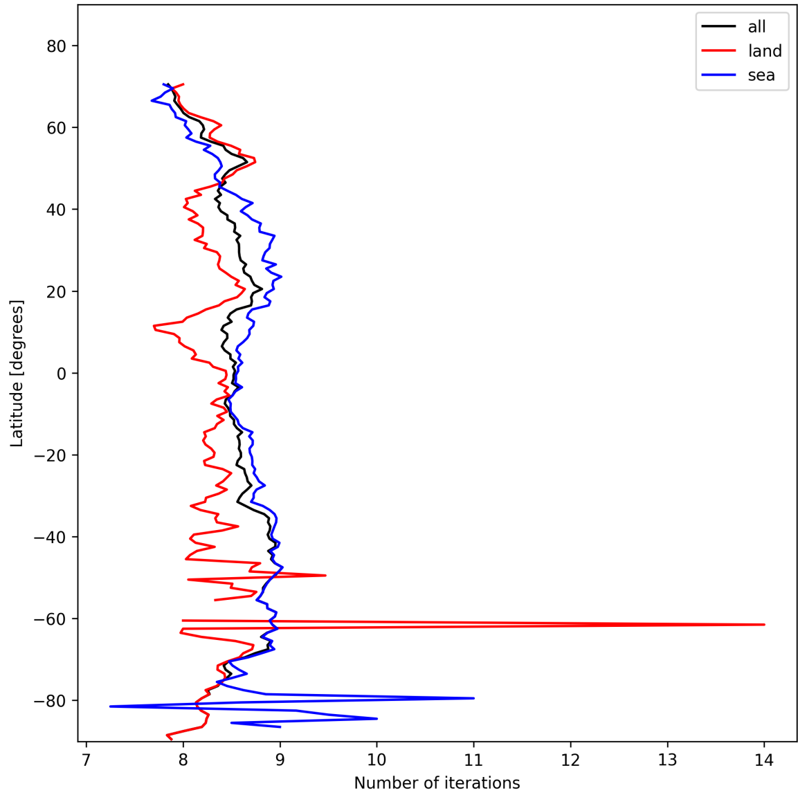
Figure 12: Zonal average of “Number of iterations” for 2025-02-07 to 2025-02-08.
