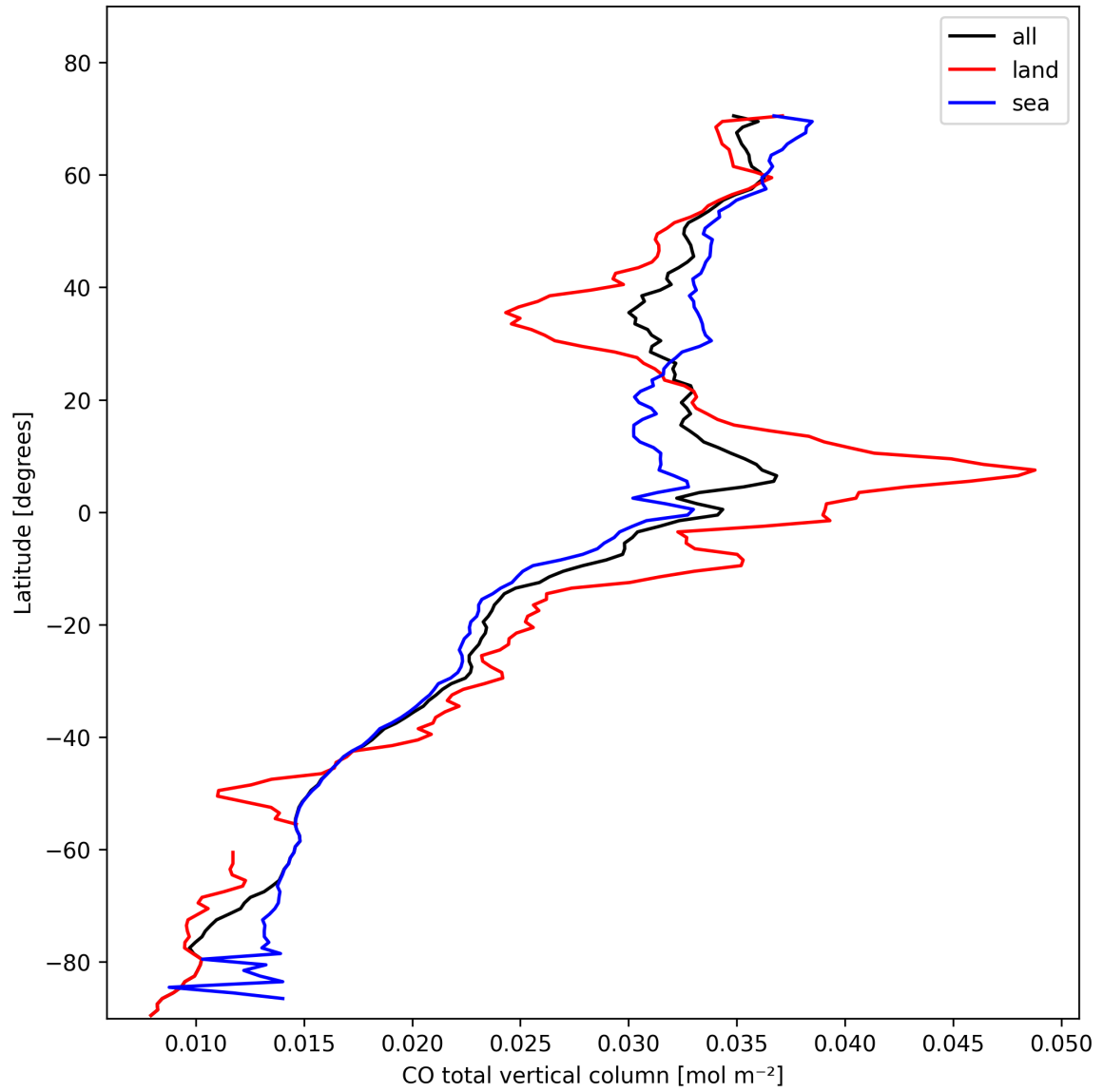
Figure 7: Zonal average of “CO total vertical column” for 2025-02-07 to 2025-02-08.
