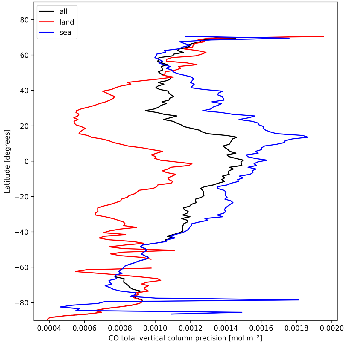
Figure 8: Zonal average of “CO total vertical column precision” for 2025-02-07 to 2025-02-08.
