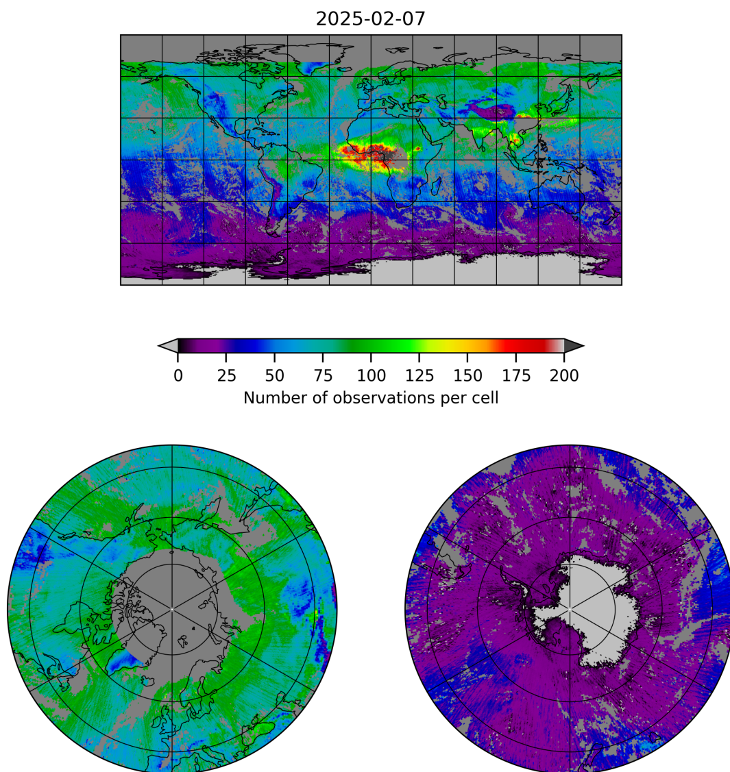
Figure 5: Map of the number of observations for 2025-02-07 to 2025-02-08
