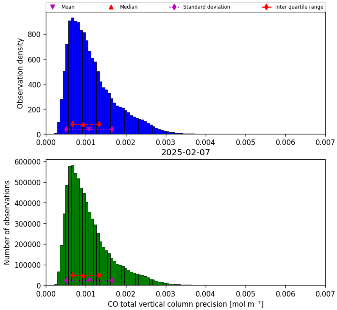
Figure 15: Histogram of “CO total vertical column precision” for 2025-02-07 to 2025-02-08
