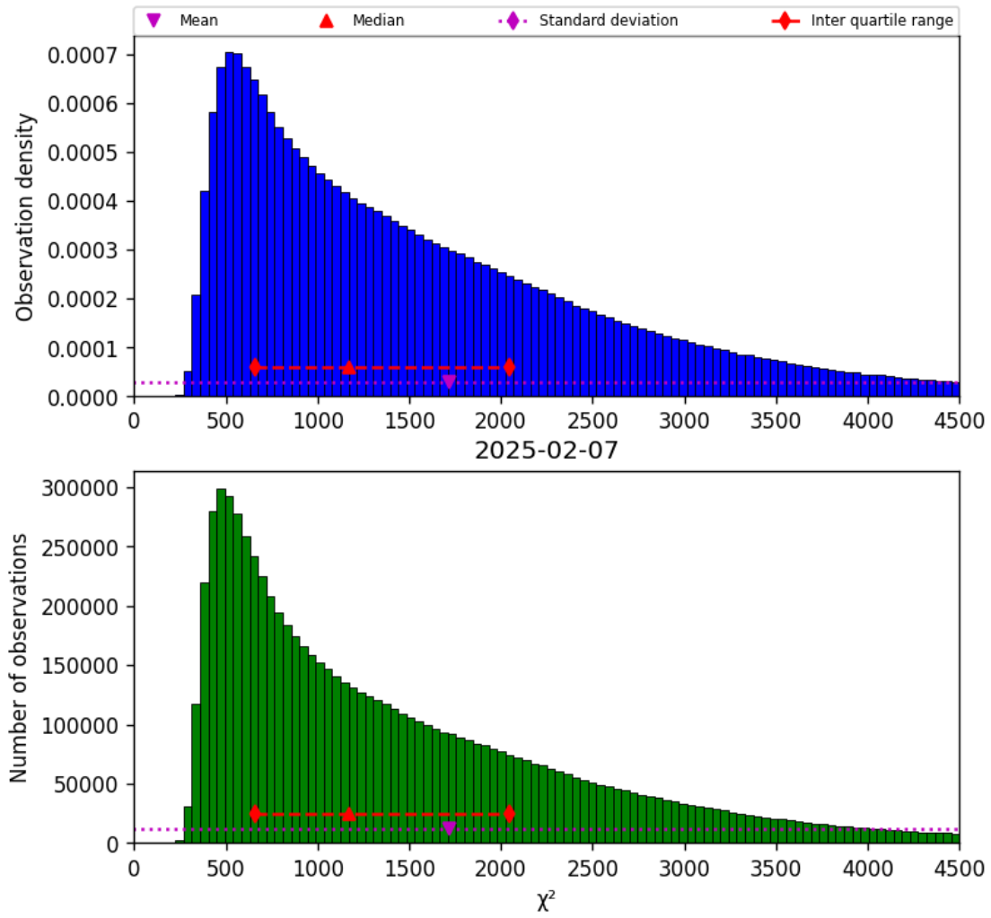
Figure 17: Histogram of " \chi^2 " for 2025-02-07 to 2025-02-08
