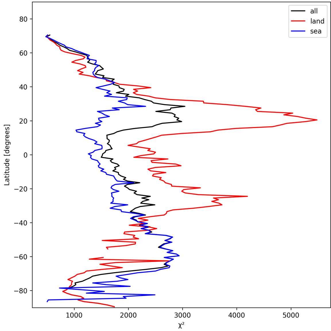
Figure 10: Zonal average of “ \chi^2 ” for 2025-02-07 to 2025-02-08.
