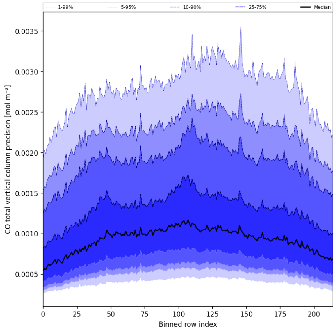
Figure 22: Along track statistics of “CO total vertical column precision” for 2025-02-07 to 2025-02-08
