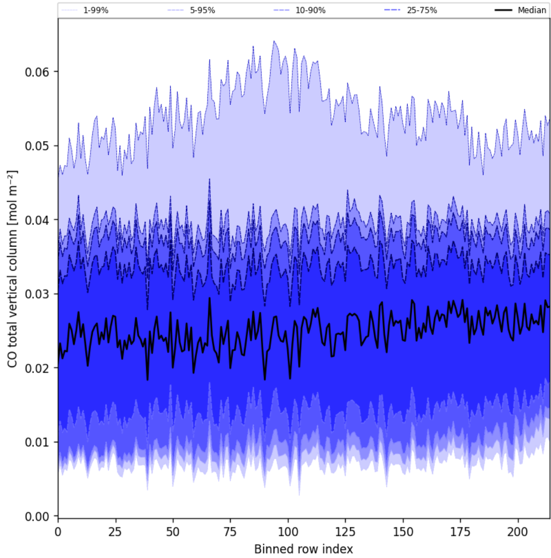
Figure 21: Along track statistics of “CO total vertical column” for 2025-02-07 to 2025-02-08
