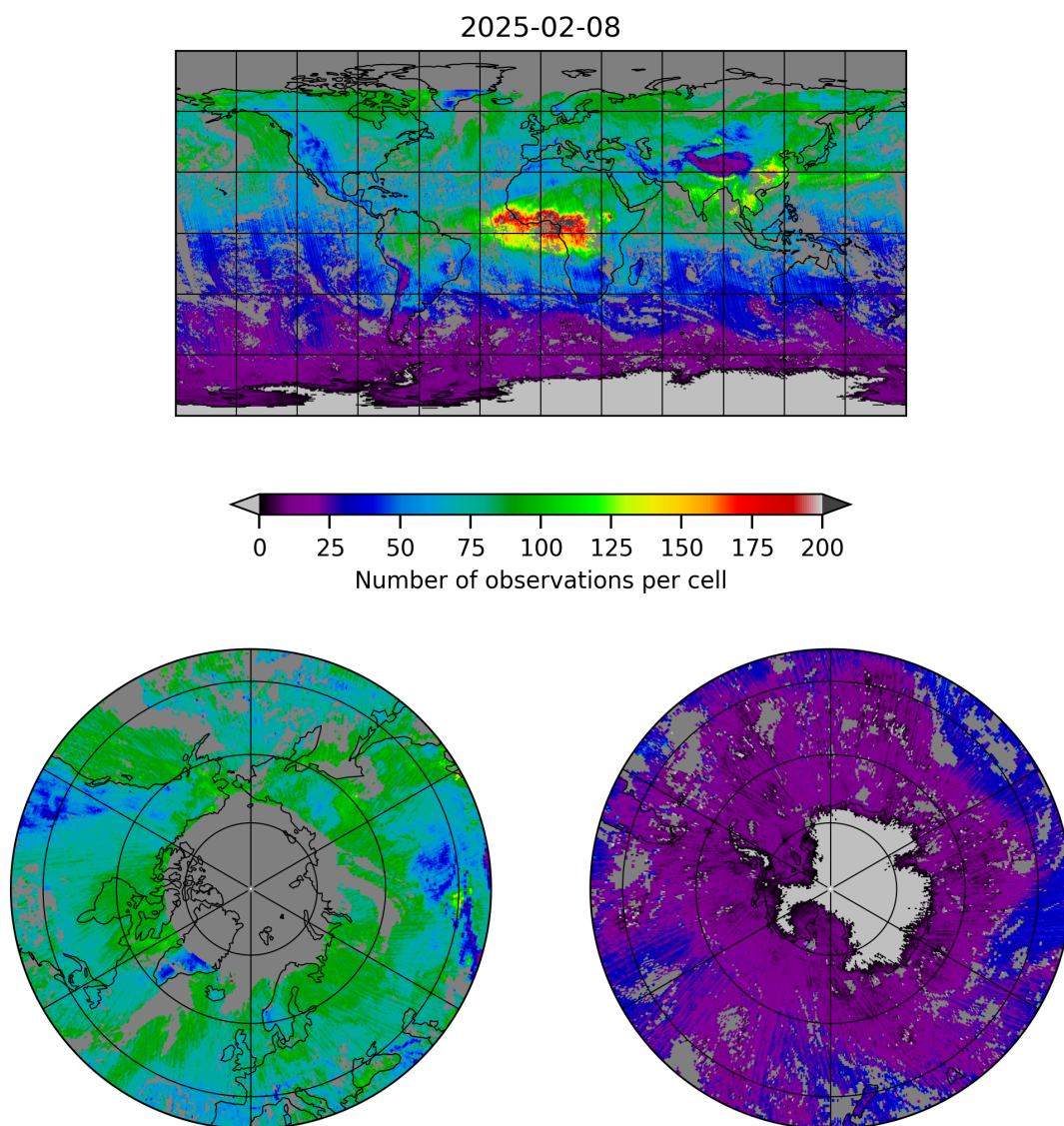
Figure 5: Map of the number of observations for 2025-02-08 to 2025-02-09
