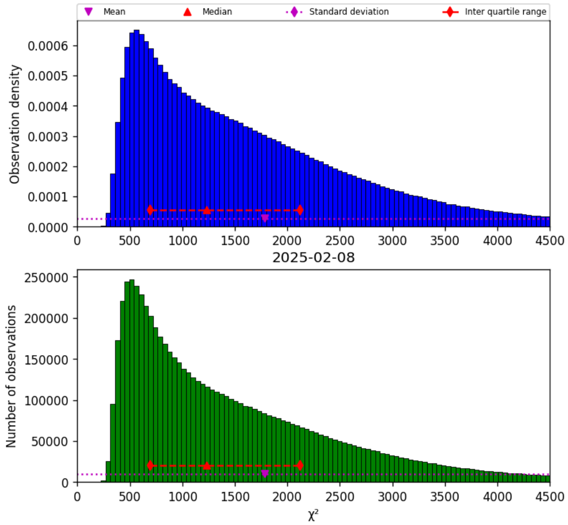
Figure 17: Histogram of “ \chi^2 ” for 2025-02-08 to 2025-02-09
