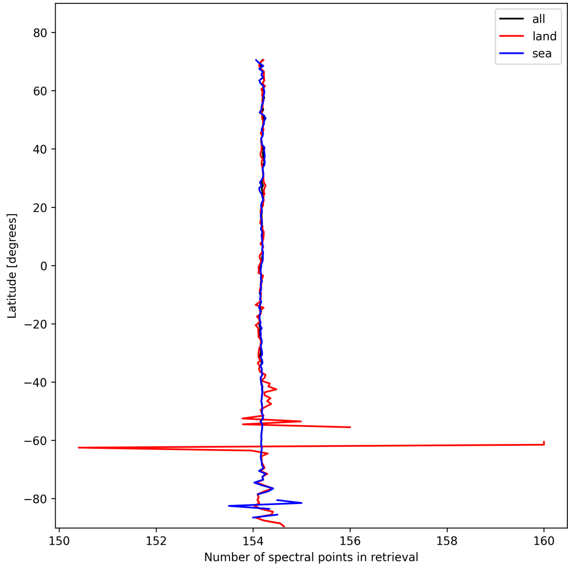
Figure 9: Zonal average of “Number of spectral points in retrieval” for 2025-02-08 to 2025-02-09.
