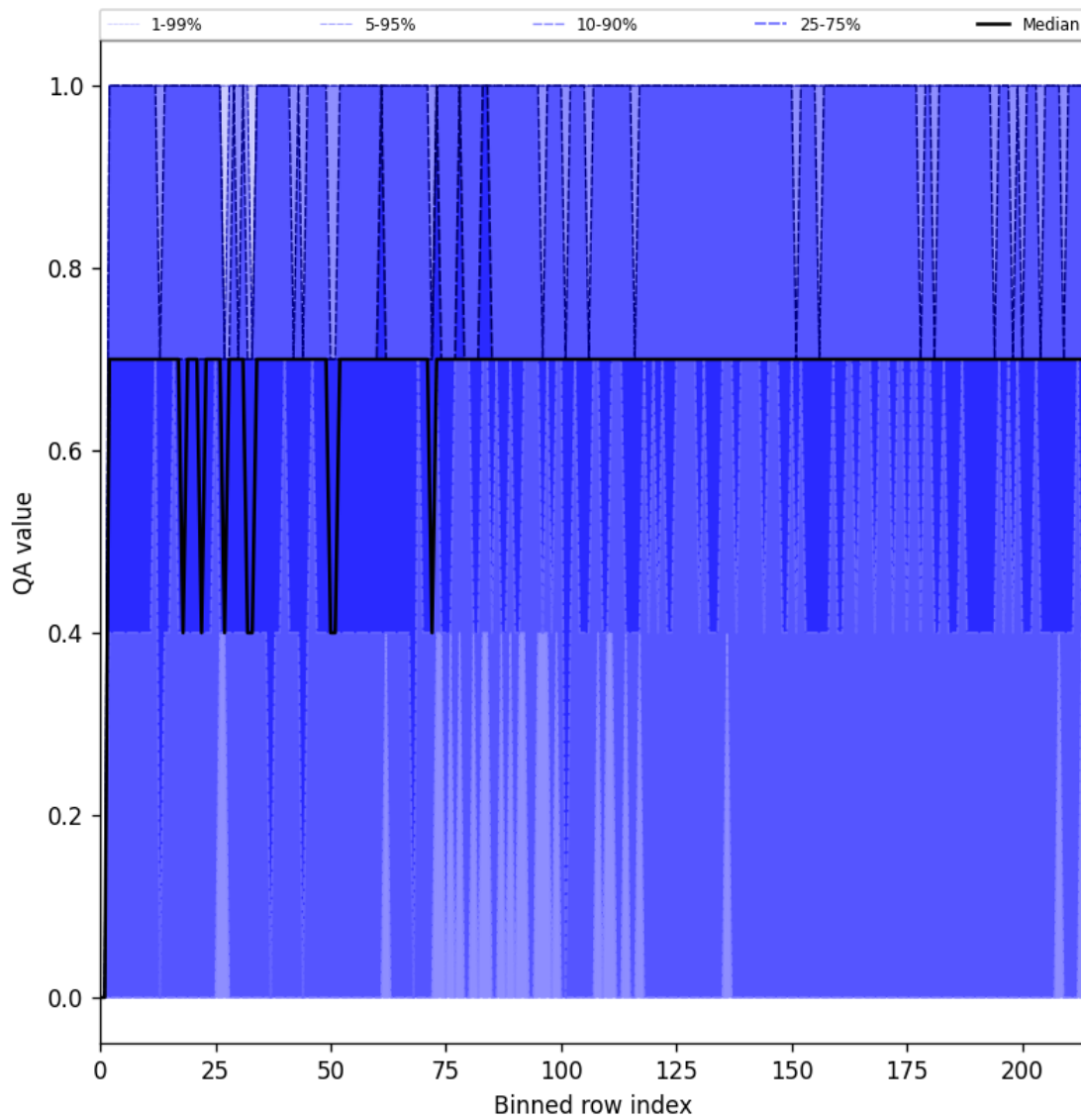
Figure 20: Along track statistics of “QA value” for 2025-02-08 to 2025-02-09
