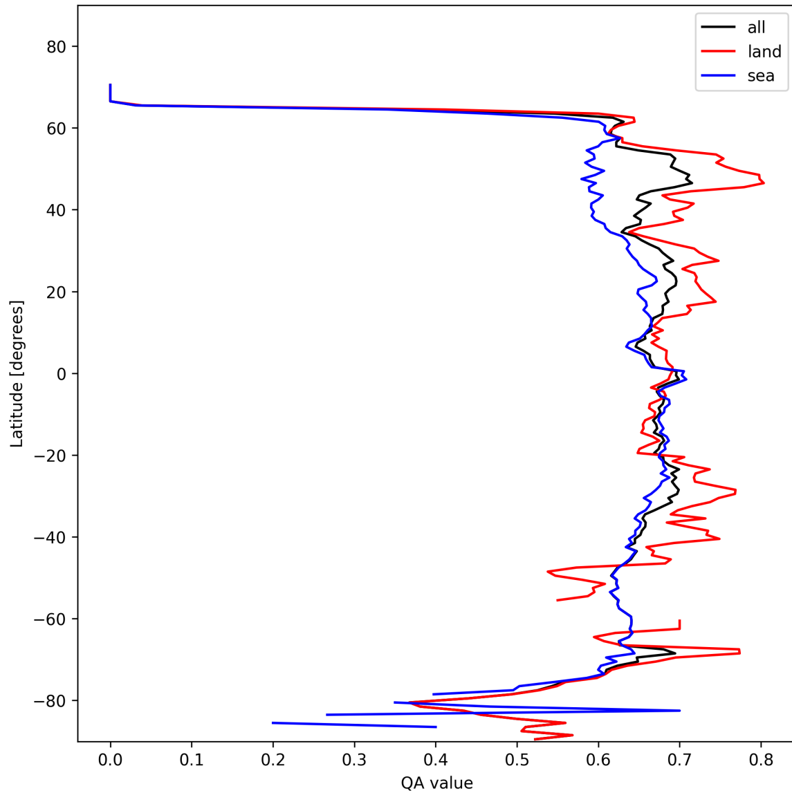
Figure 6: Zonal average of “QA value” for 2025-02-08 to 2025-02-09.
