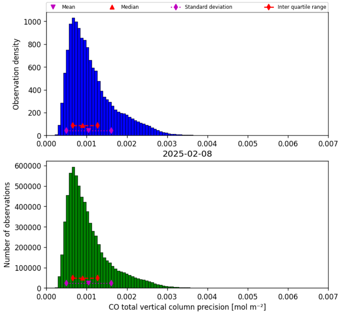
Figure 15: Histogram of “CO total vertical column precision” for 2025-02-08 to 2025-02-09
