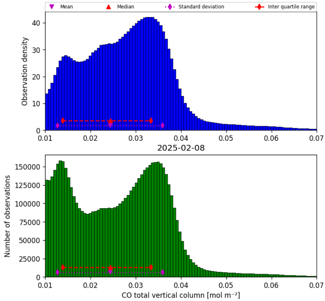
Figure 14: Histogram of “CO total vertical column” for 2025-02-08 to 2025-02-09
