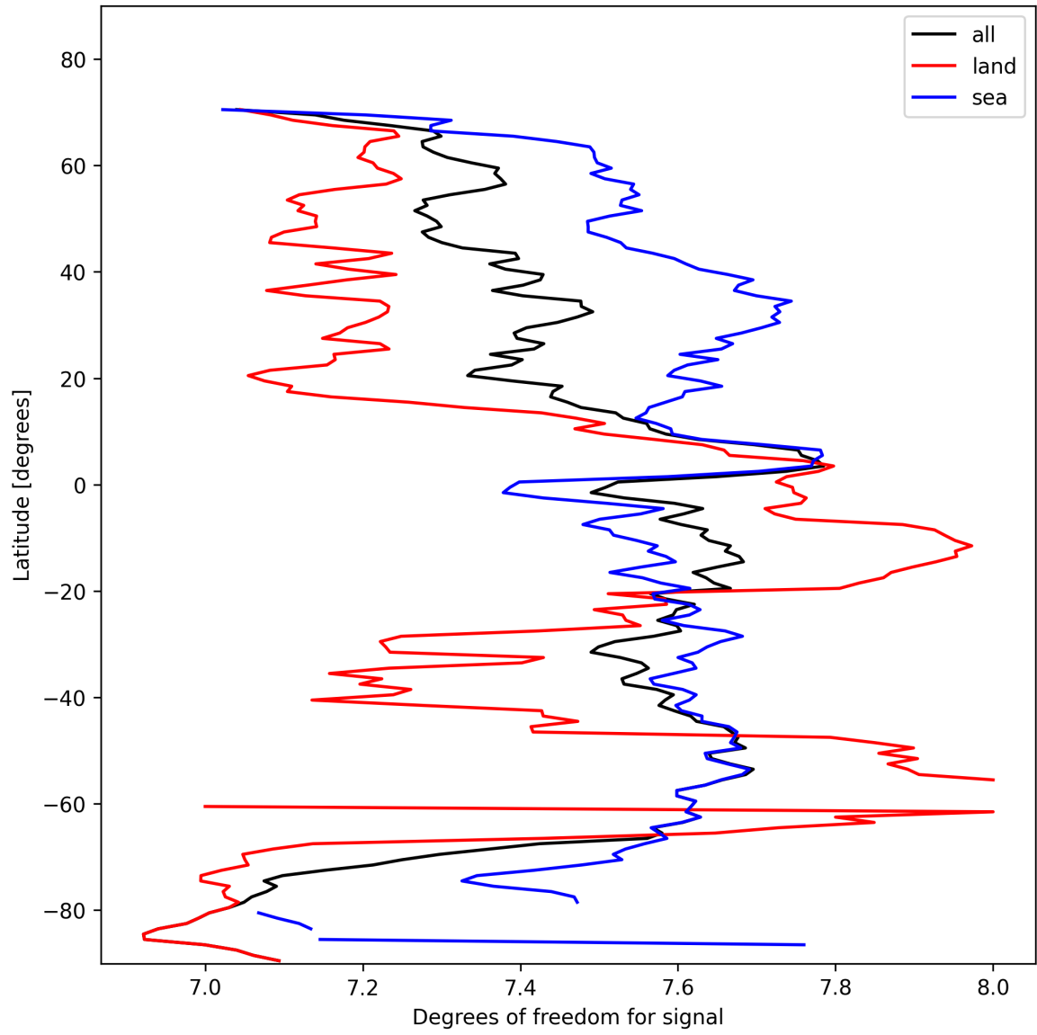
Figure 11: Zonal average of “Degrees of freedom for signal” for 2025-02-08 to 2025-02-09.
