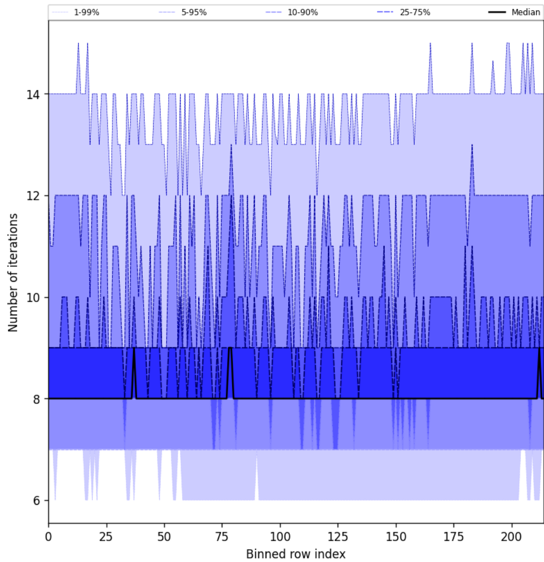
Figure 26: Along track statistics of “Number of iterations” for 2025-02-08 to 2025-02-09
