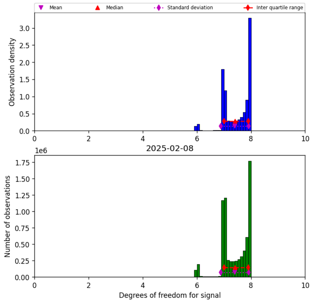
Figure 18: Histogram of “Degrees of freedom for signal” for 2025-02-08 to 2025-02-09
