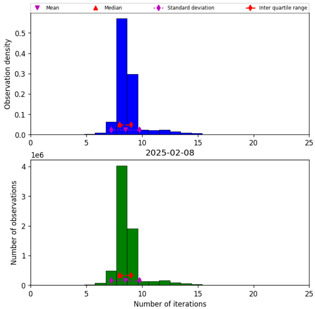
Figure 19: Histogram of “Number of iterations” for 2025-02-08 to 2025-02-09
