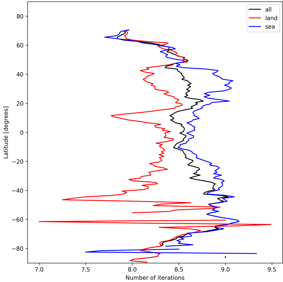
Figure 12: Zonal average of “Number of iterations” for 2025-02-08 to 2025-02-09.
