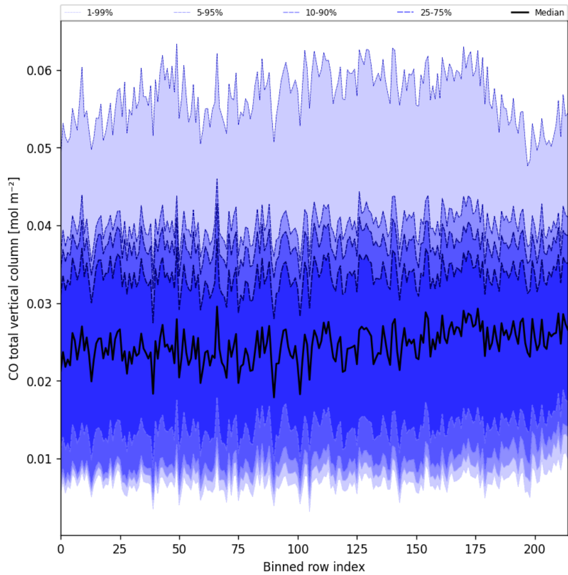
Figure 21: Along track statistics of “CO total vertical column” for 2025-02-08 to 2025-02-09
