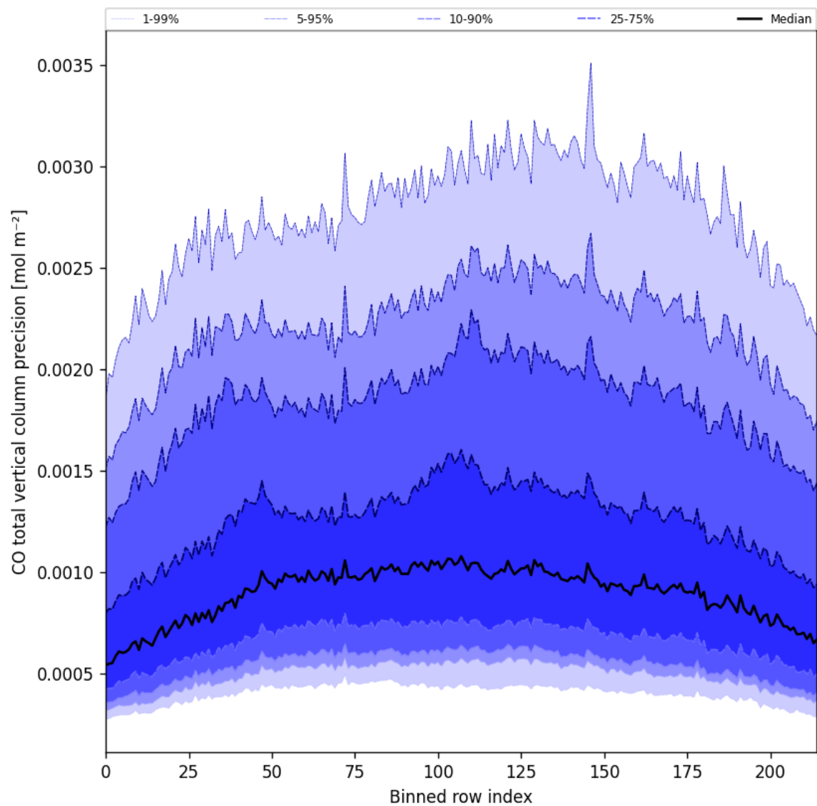
Figure 22: Along track statistics of “CO total vertical column precision” for 2025-02-08 to 2025-02-09
