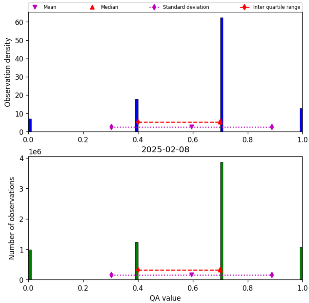
Figure 13: Histogram of “QA value” for 2025-02-08 to 2025-02-09
