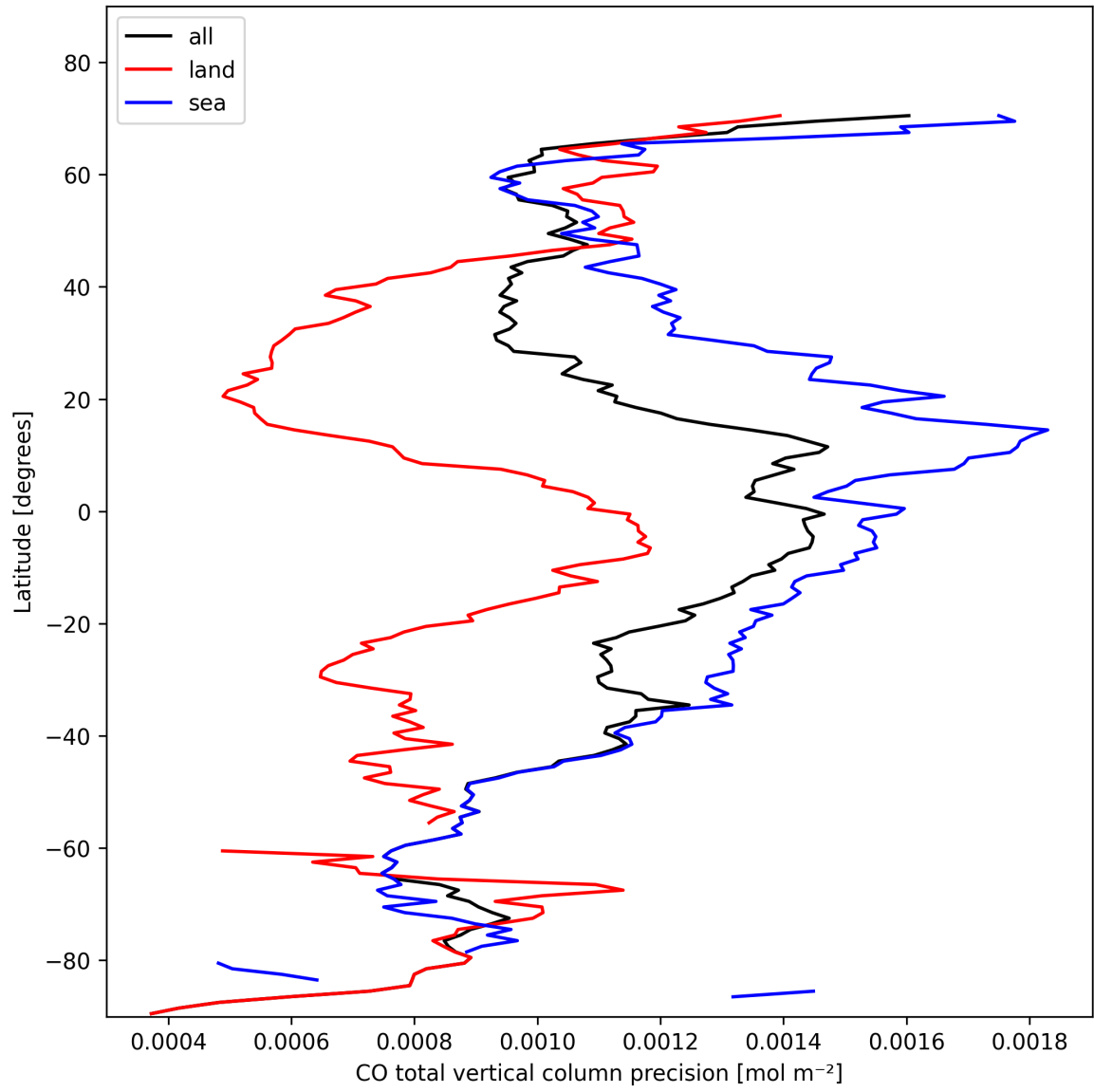
Figure 8: Zonal average of “CO total vertical column precision” for 2025-02-08 to 2025-02-09.
