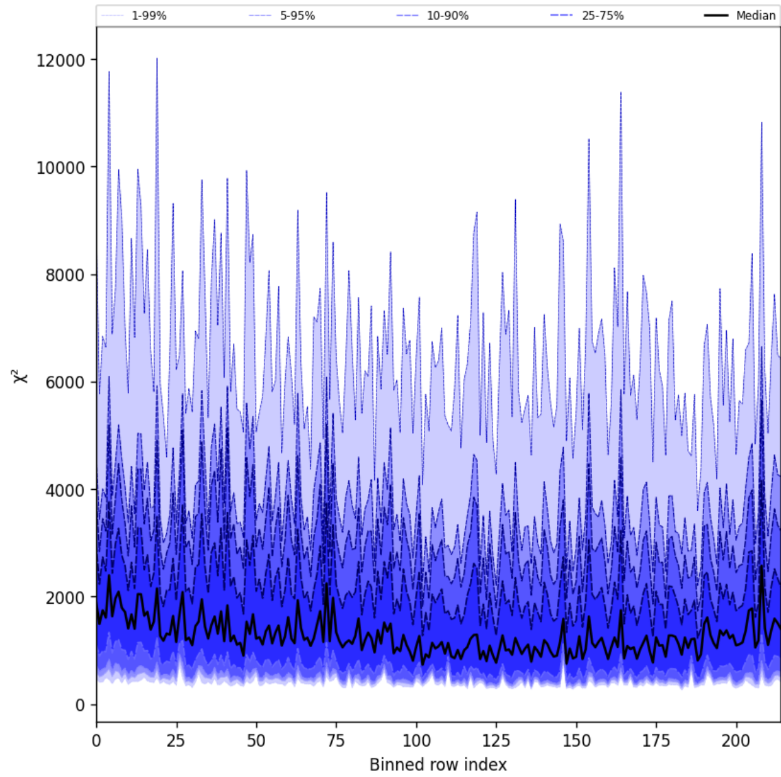
Figure 24: Along track statistics of “ \chi^2 ” for 2025-02-08 to 2025-02-09
