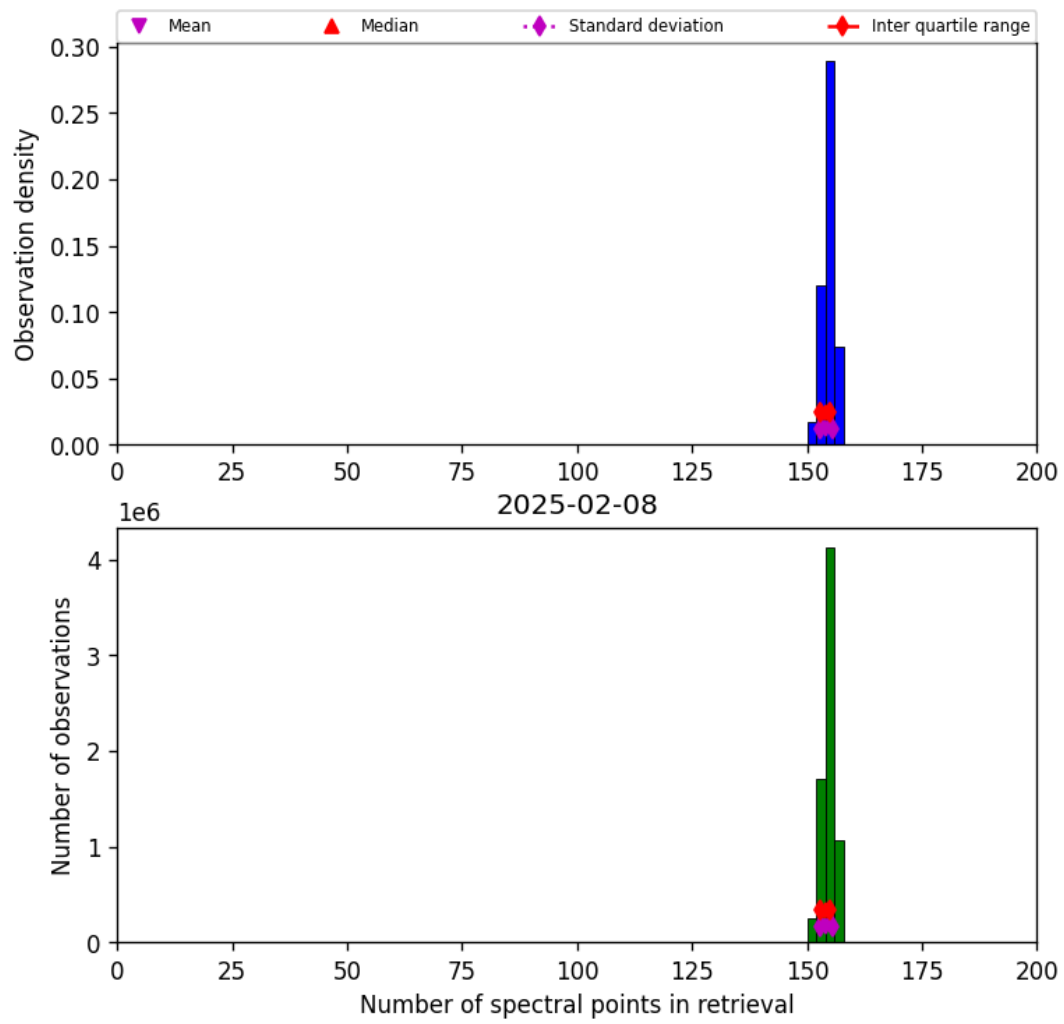
Figure 16: Histogram of “Number of spectral points in retrieval” for 2025-02-08 to 2025-02-09
