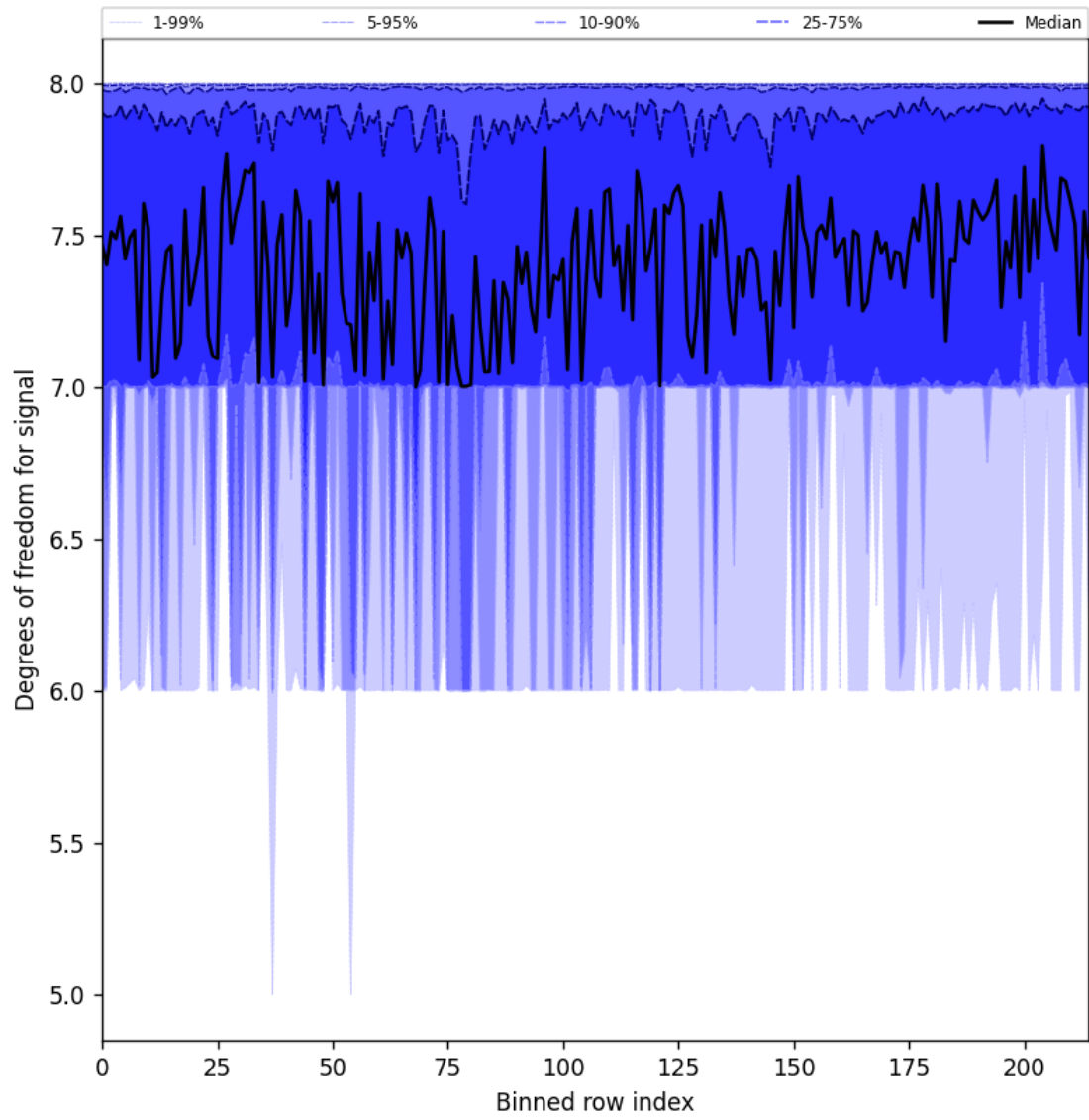
Figure 25: Along track statistics of “Degrees of freedom for signal” for 2025-02-08 to 2025-02-09
