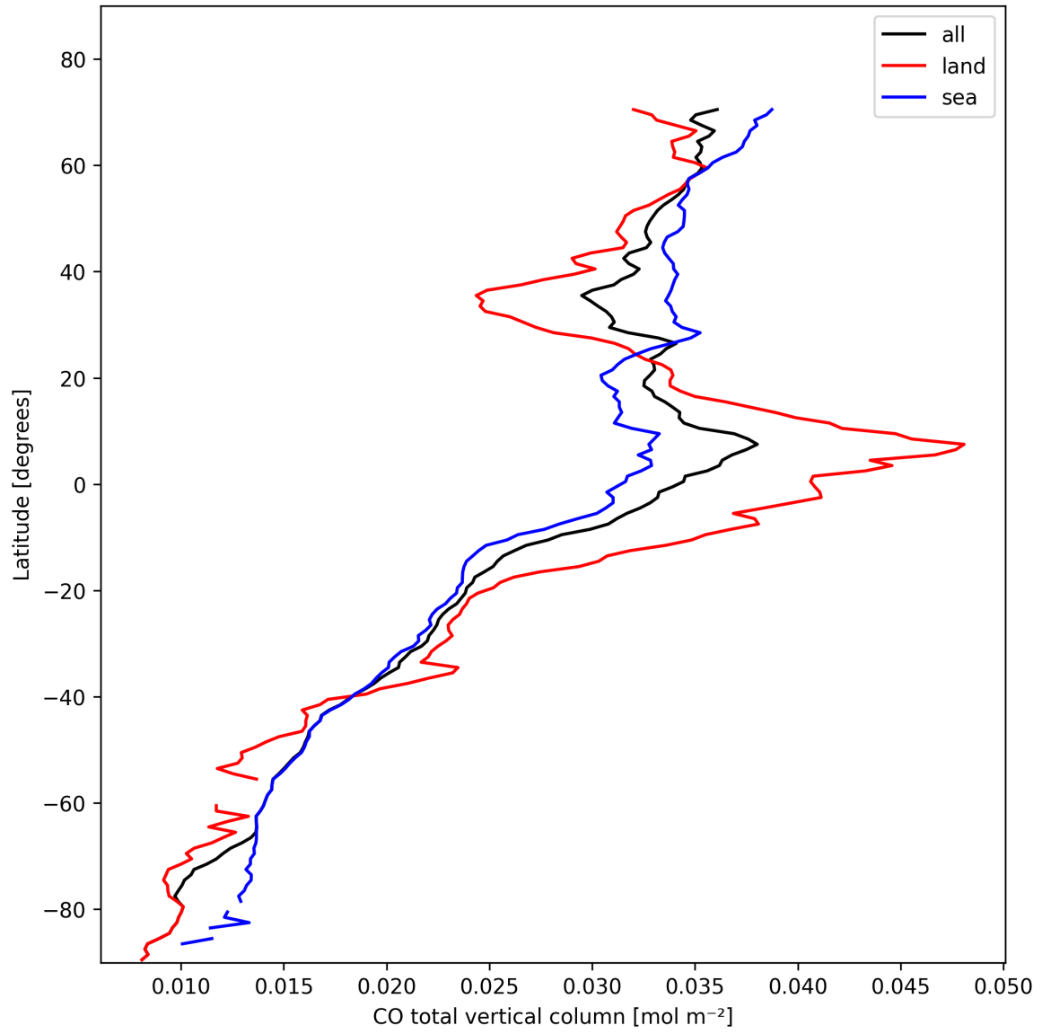
Figure 7: Zonal average of “CO total vertical column” for 2025-02-08 to 2025-02-09.
