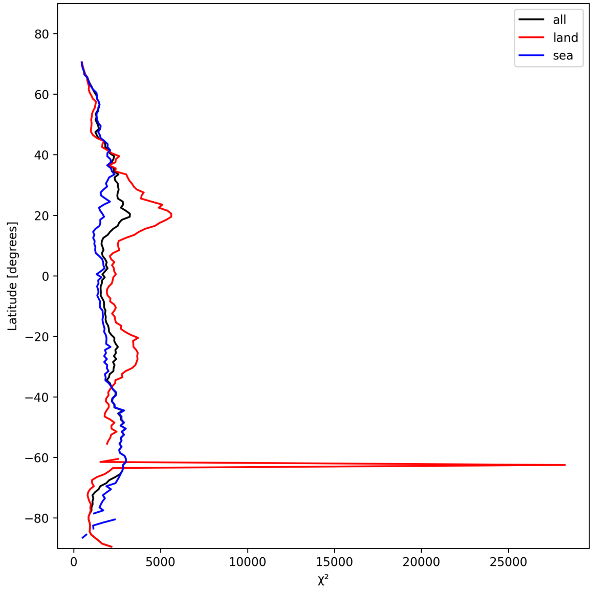
Figure 10: Zonal average of “ \chi^2 ” for 2025-02-08 to 2025-02-09.
