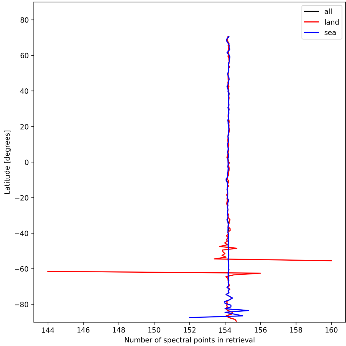
Figure 9: Zonal average of “Number of spectral points in retrieval” for 2025-02-09 to 2025-02-10.
