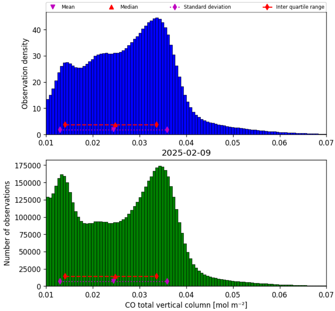
Figure 14: Histogram of “CO total vertical column” for 2025-02-09 to 2025-02-10
