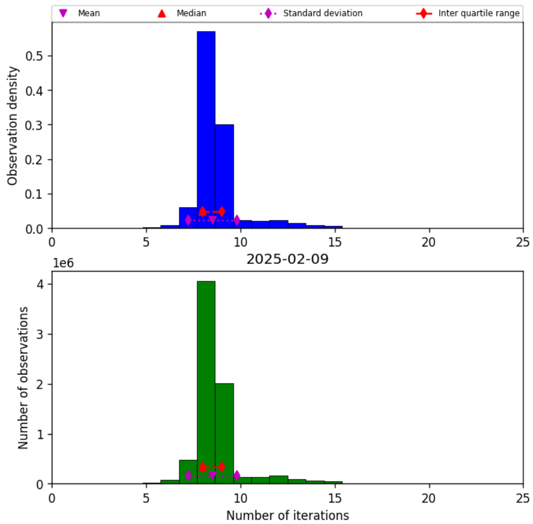
Figure 19: Histogram of “Number of iterations” for 2025-02-09 to 2025-02-10
