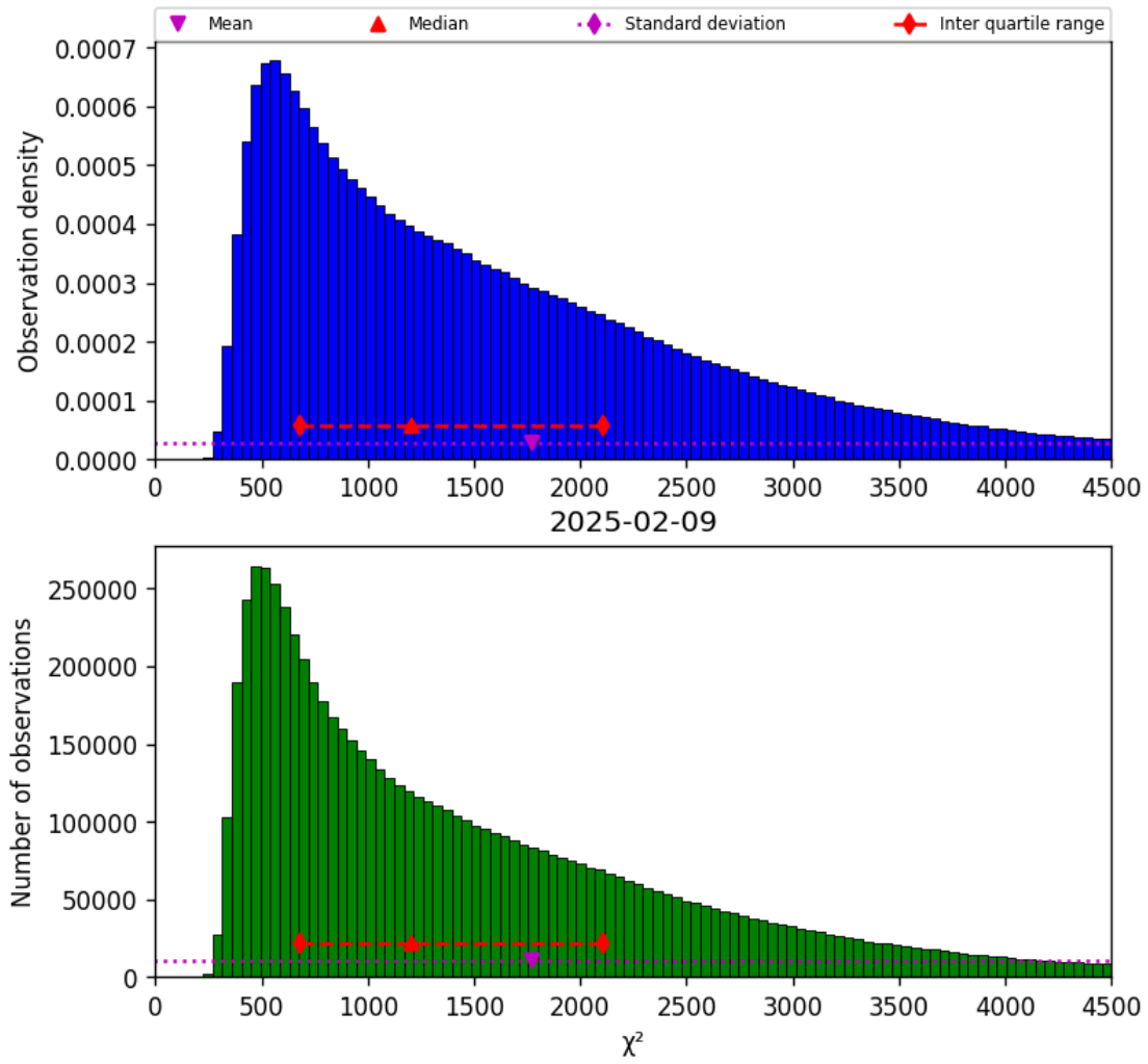
Figure 17: Histogram of " \chi^2 " for 2025-02-09 to 2025-02-10
