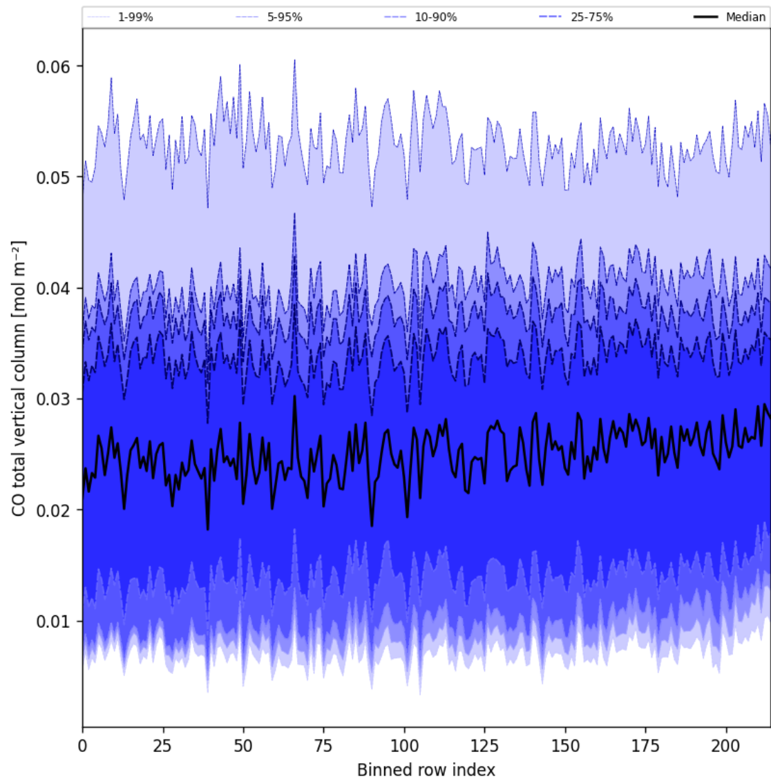
Figure 21: Along track statistics of “CO total vertical column” for 2025-02-09 to 2025-02-10
