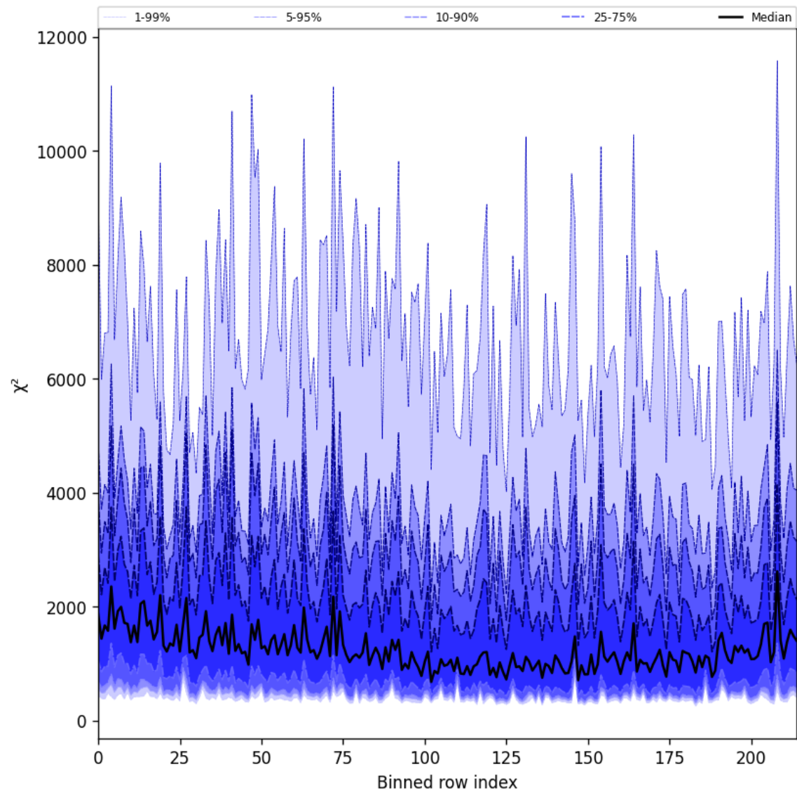
Figure 24: Along track statistics of “ \chi^2 ” for 2025-02-09 to 2025-02-10
