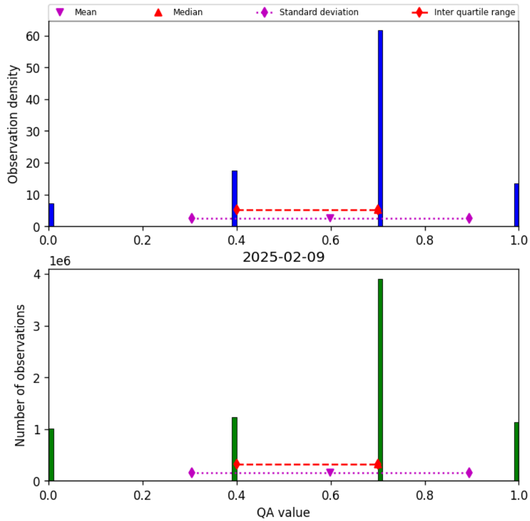
Figure 13: Histogram of “QA value” for 2025-02-09 to 2025-02-10
