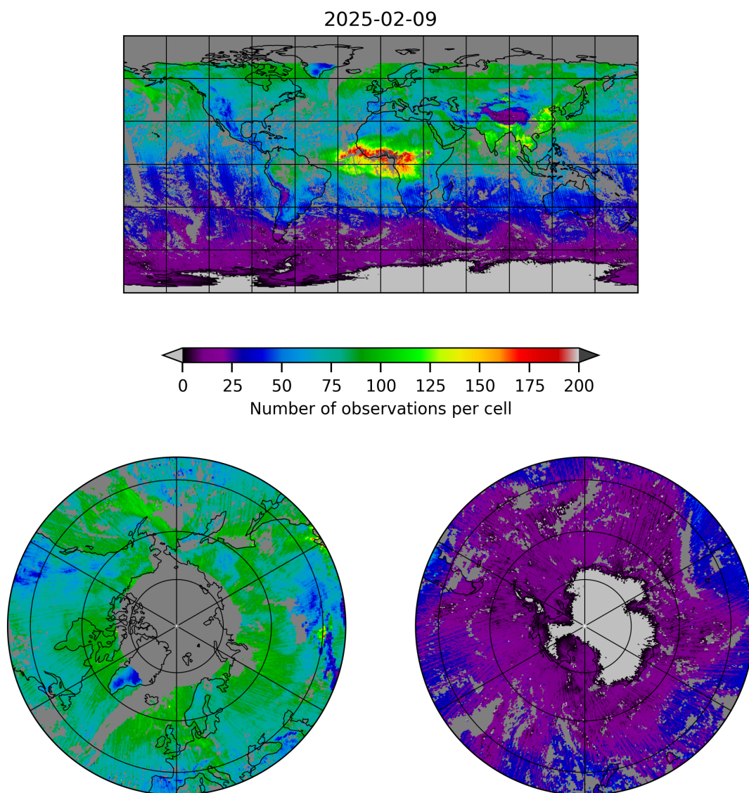
Figure 5: Map of the number of observations for 2025-02-09 to 2025-02-10
