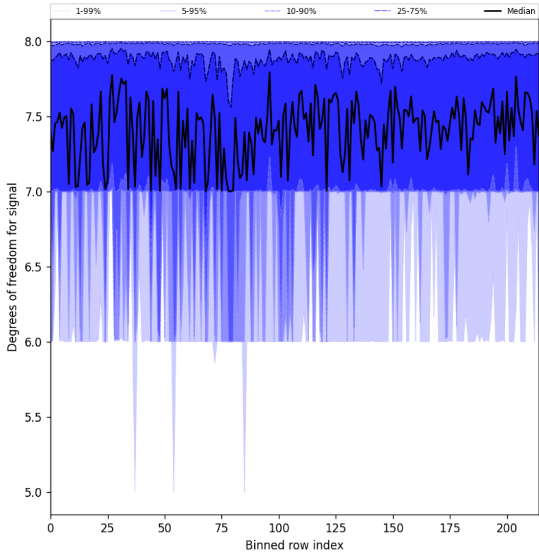
Figure 25: Along track statistics of “Degrees of freedom for signal” for 2025-02-09 to 2025-02-10
