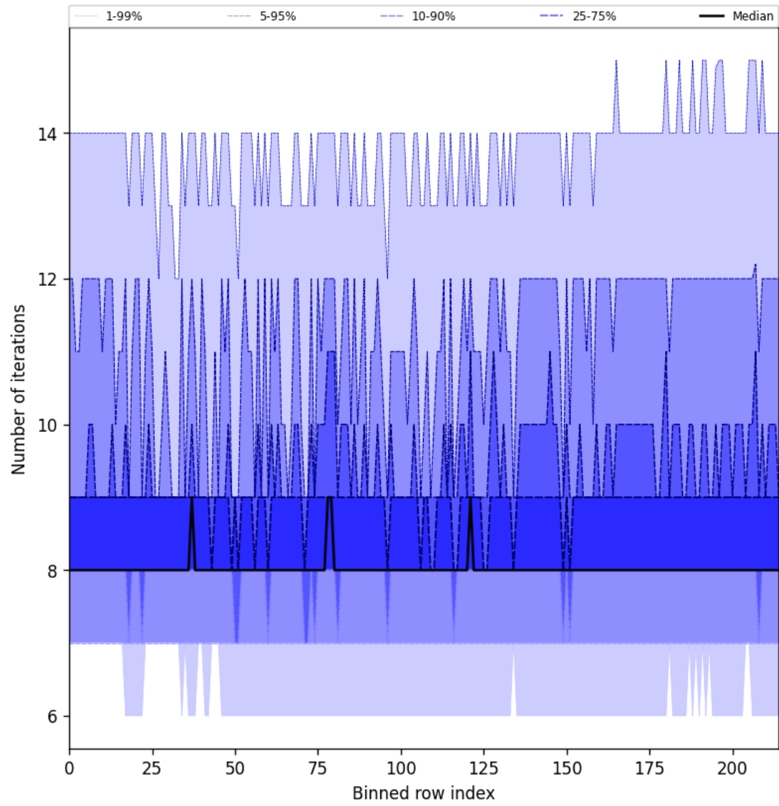
Figure 26: Along track statistics of “Number of iterations” for 2025-02-09 to 2025-02-10
