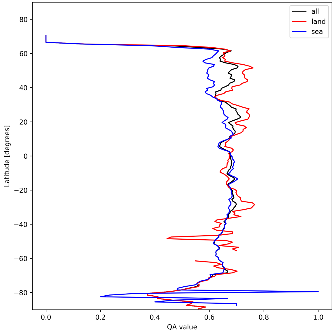
Figure 6: Zonal average of "QA value" for 2025-02-09 to 2025-02-10.
