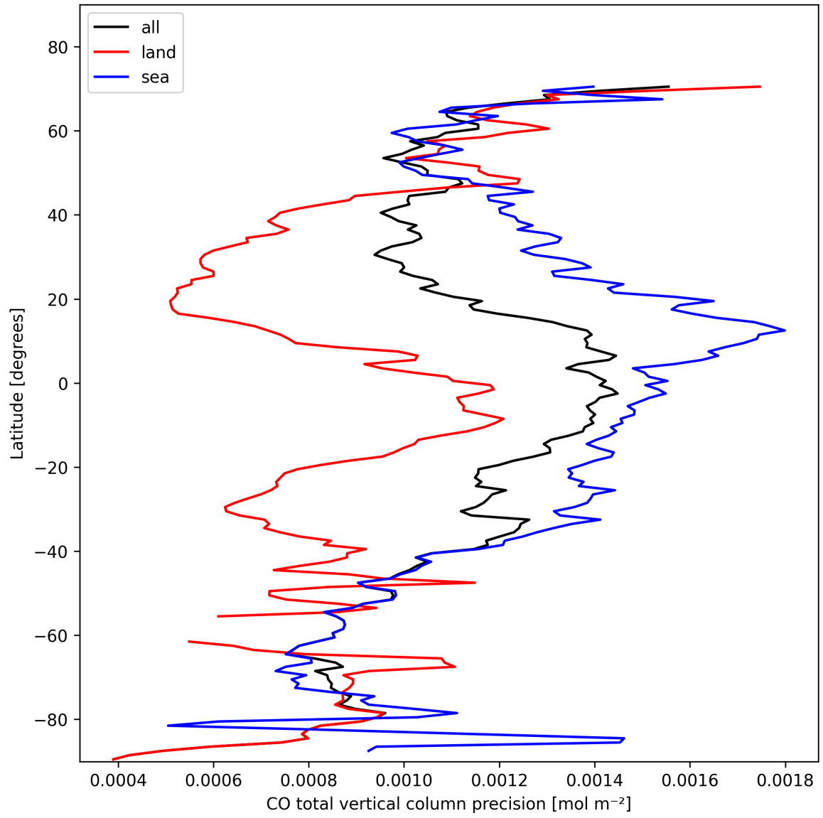
Figure 8: Zonal average of “CO total vertical column precision” for 2025-02-09 to 2025-02-10.
