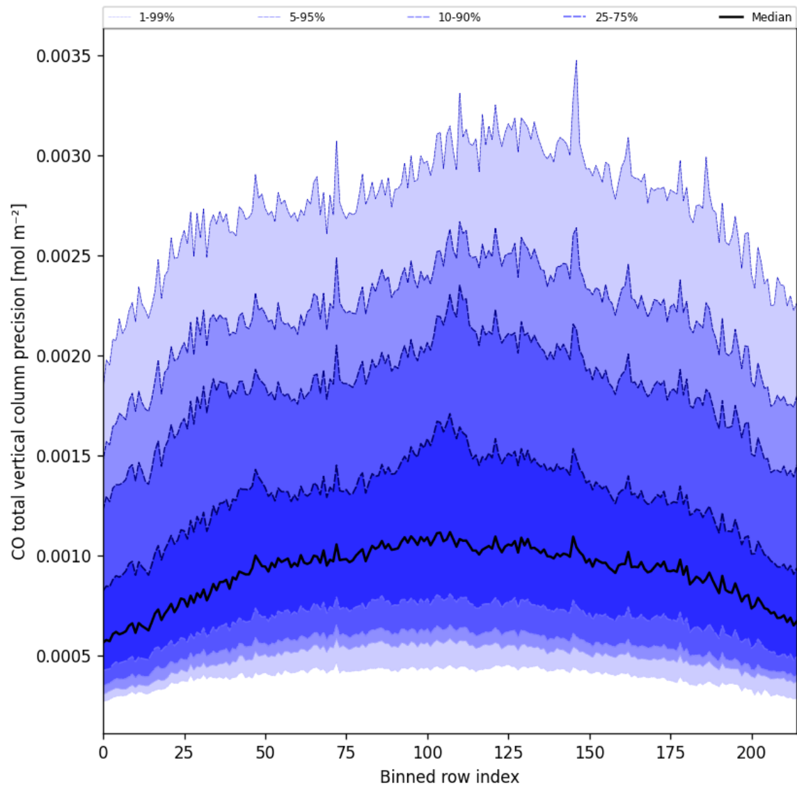
Figure 22: Along track statistics of “CO total vertical column precision” for 2025-02-09 to 2025-02-10
