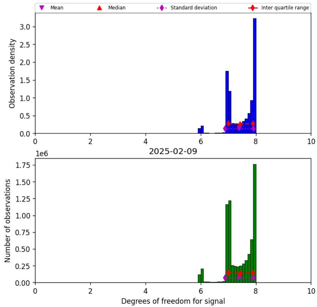
Figure 18: Histogram of “Degrees of freedom for signal” for 2025-02-09 to 2025-02-10
