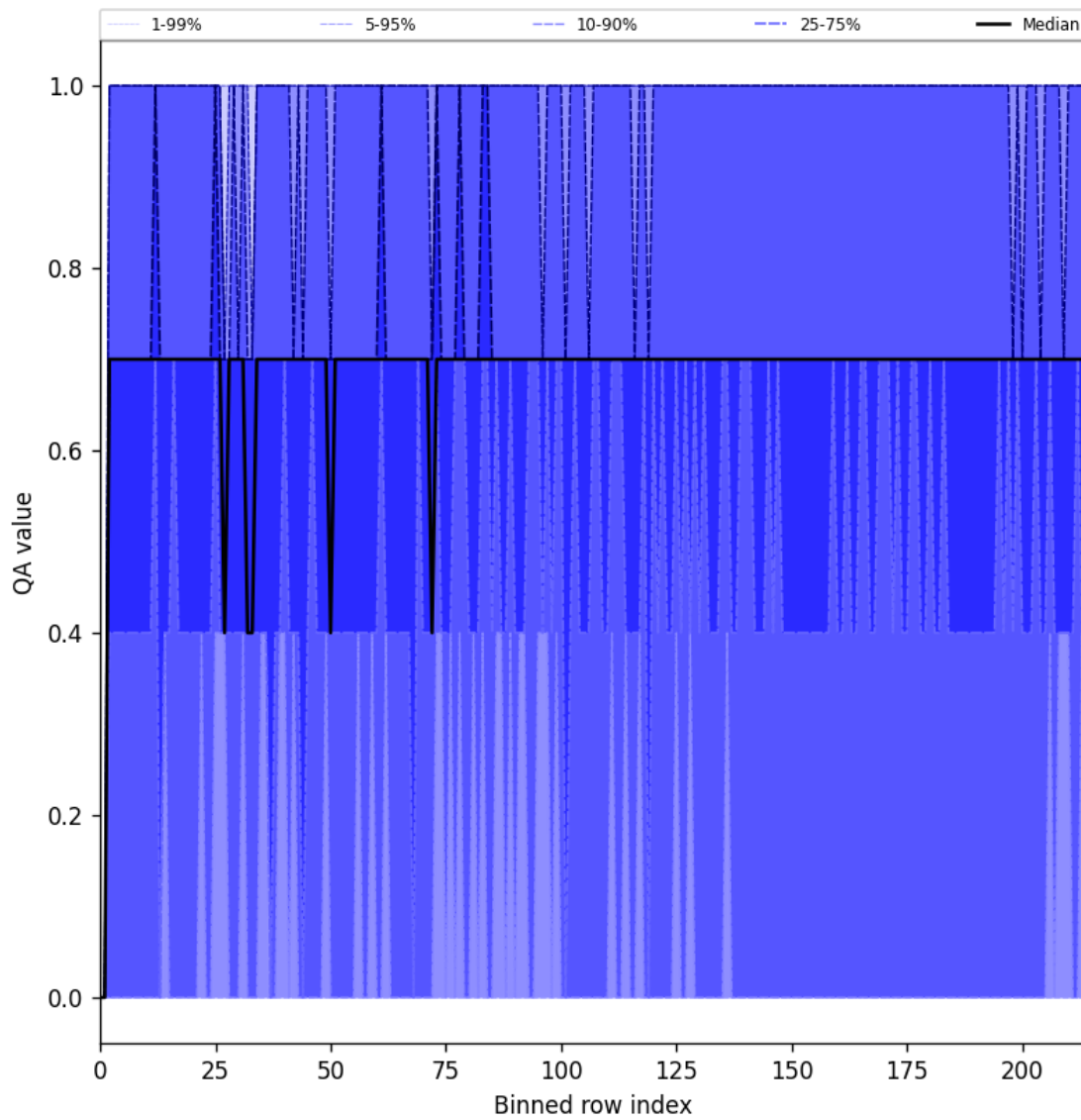
Figure 20: Along track statistics of “QA value” for 2025-02-09 to 2025-02-10
