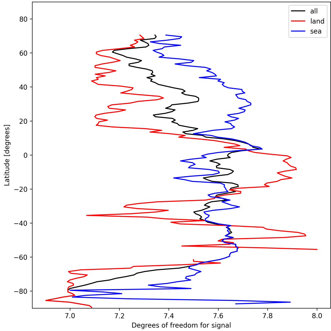
Figure 11: Zonal average of “Degrees of freedom for signal” for 2025-02-09 to 2025-02-10.
