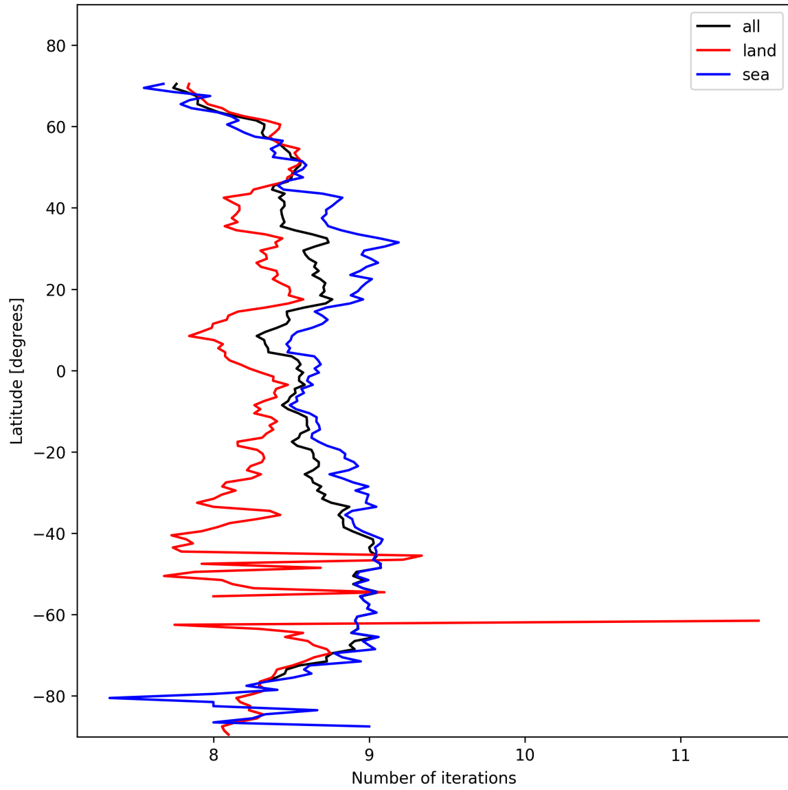
Figure 12: Zonal average of “Number of iterations” for 2025-02-09 to 2025-02-10.
