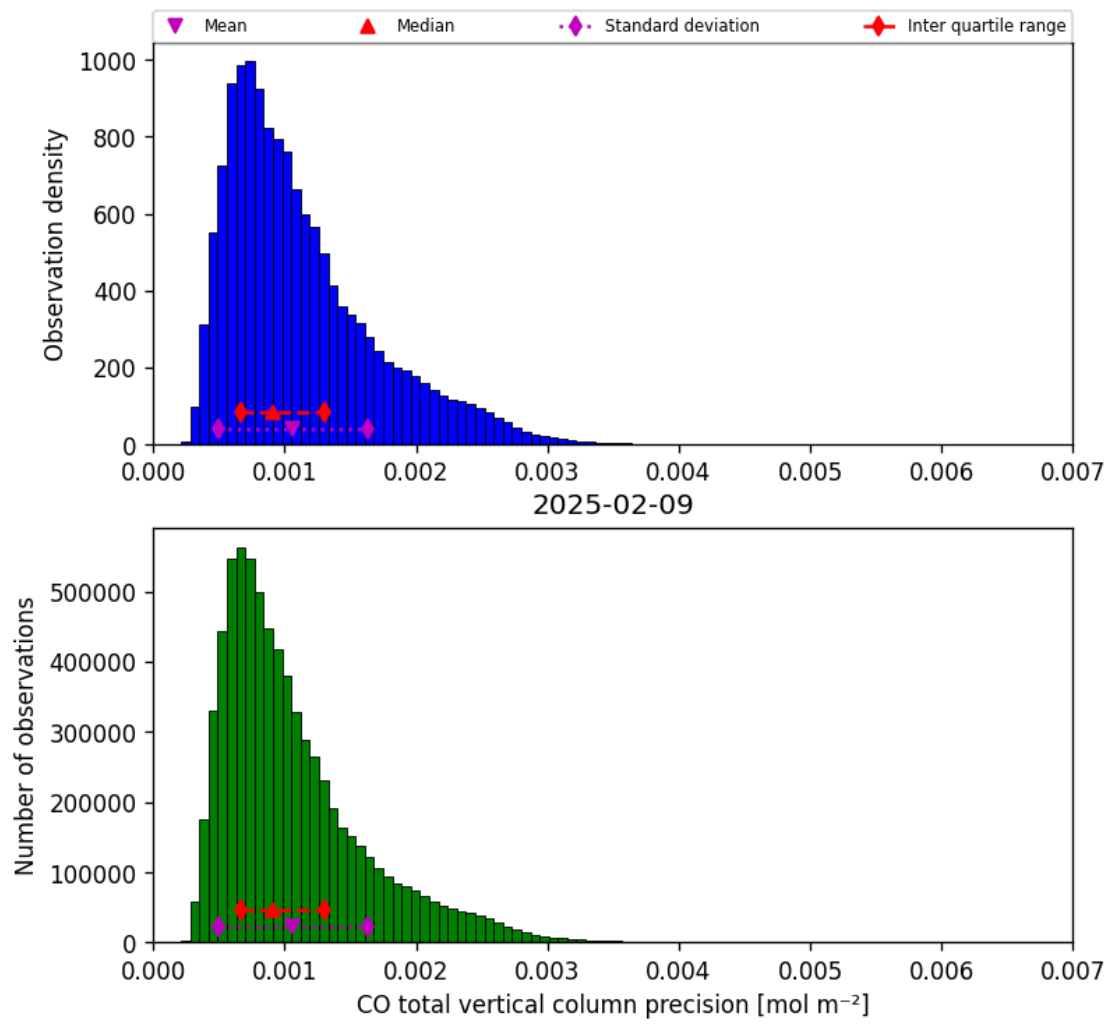
Figure 15: Histogram of “CO total vertical column precision” for 2025-02-09 to 2025-02-10
