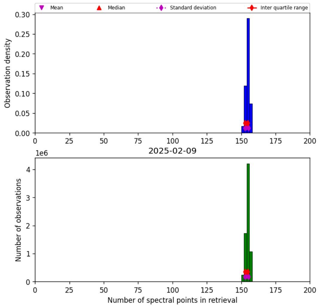
Figure 16: Histogram of “Number of spectral points in retrieval” for 2025-02-09 to 2025-02-10
