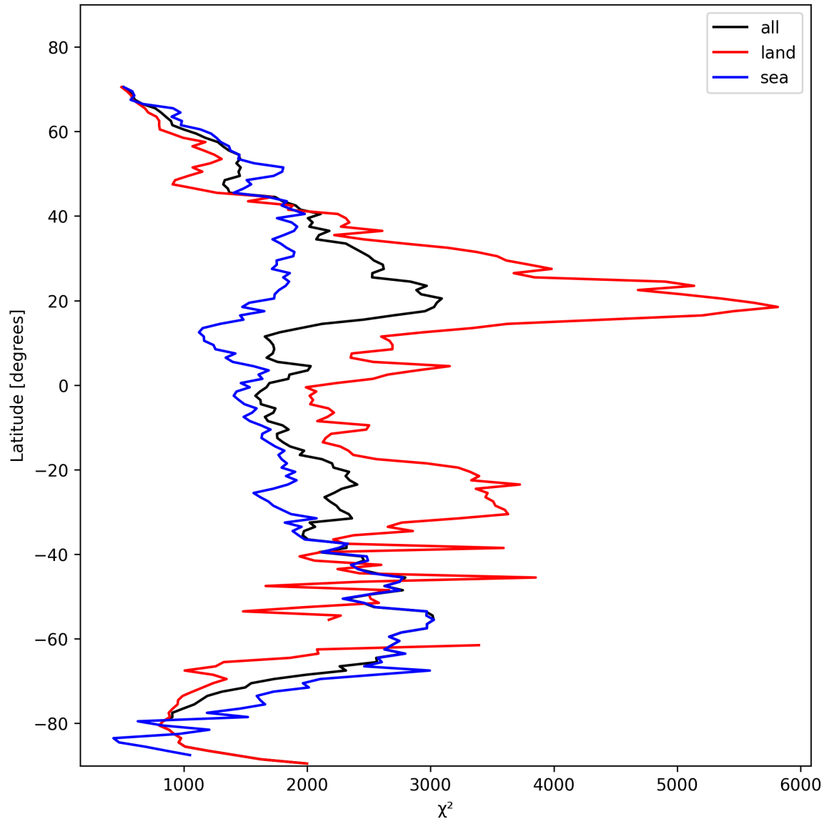
Figure 10: Zonal average of “ \chi^2 ” for 2025-02-09 to 2025-02-10.
