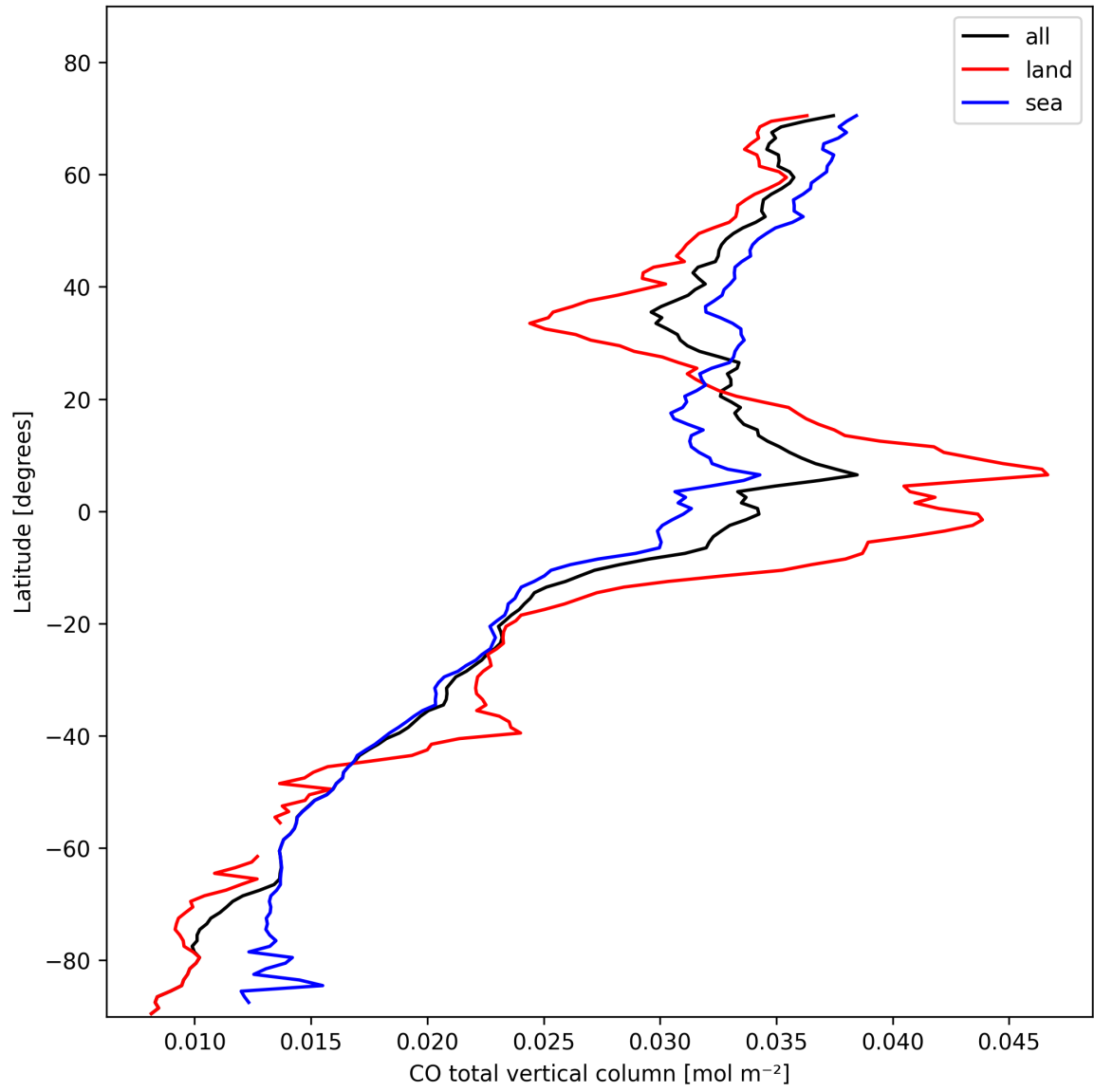
Figure 7: Zonal average of “CO total vertical column” for 2025-02-09 to 2025-02-10.
