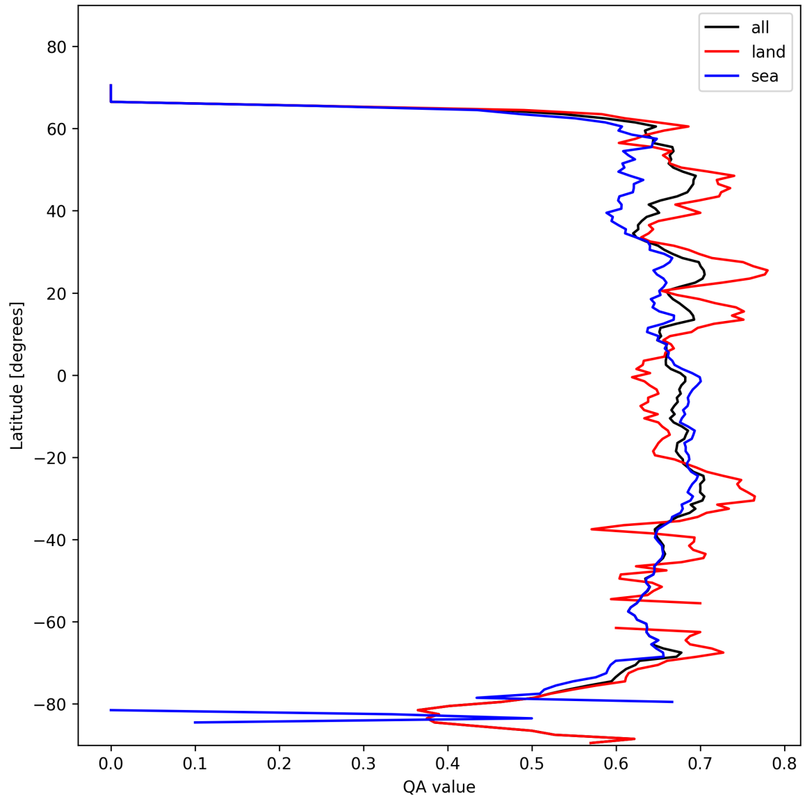
Figure 6: Zonal average of “QA value” for 2025-02-10 to 2025-02-11.
