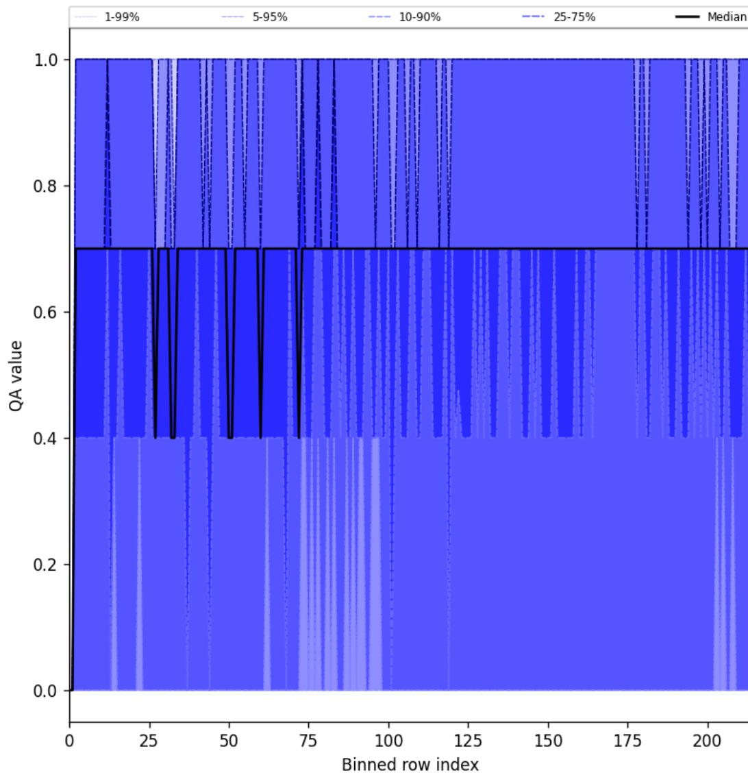
Figure 20: Along track statistics of “QA value” for 2025-02-10 to 2025-02-11
