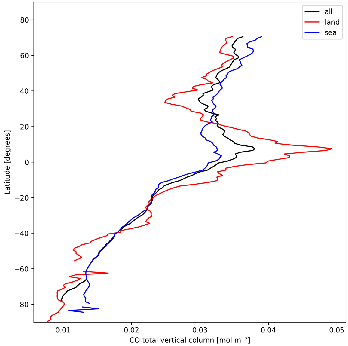
Figure 7: Zonal average of “CO total vertical column” for 2025-02-10 to 2025-02-11.
