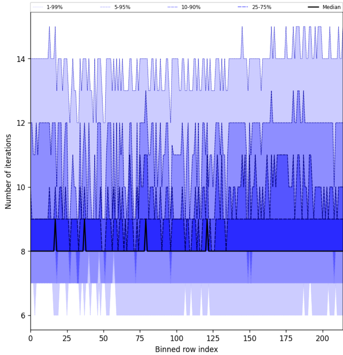
Figure 26: Along track statistics of “Number of iterations” for 2025-02-10 to 2025-02-11
