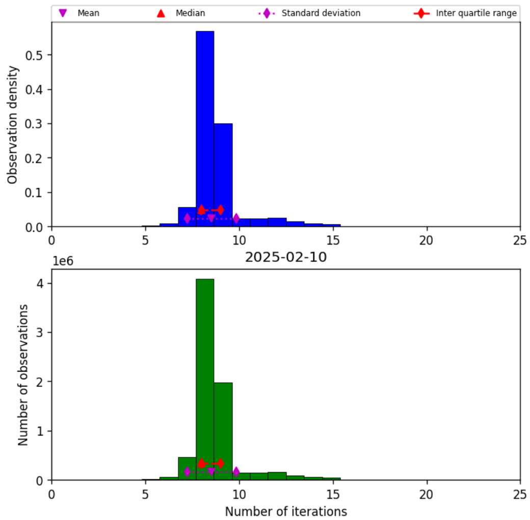
Figure 19: Histogram of “Number of iterations” for 2025-02-10 to 2025-02-11
