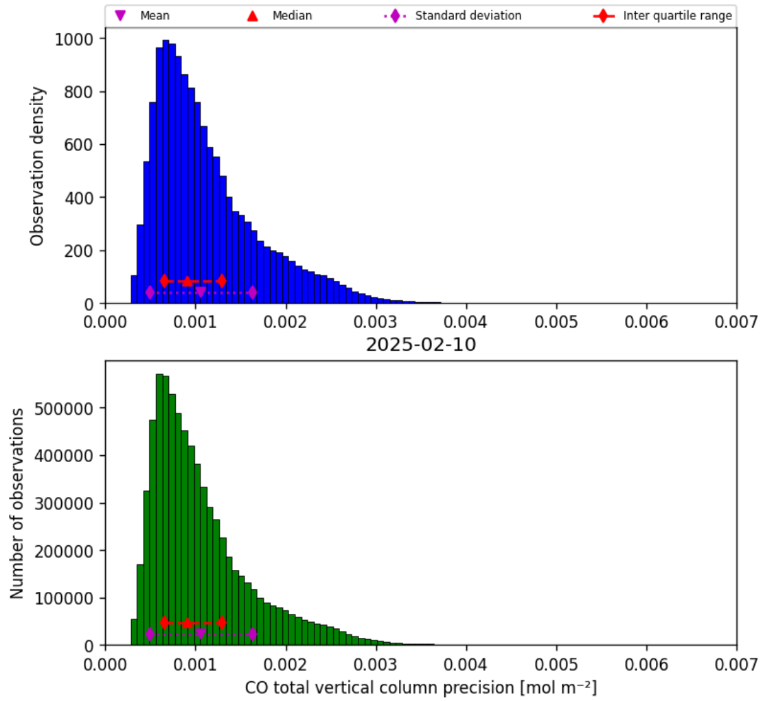
Figure 15: Histogram of “CO total vertical column precision” for 2025-02-10 to 2025-02-11
