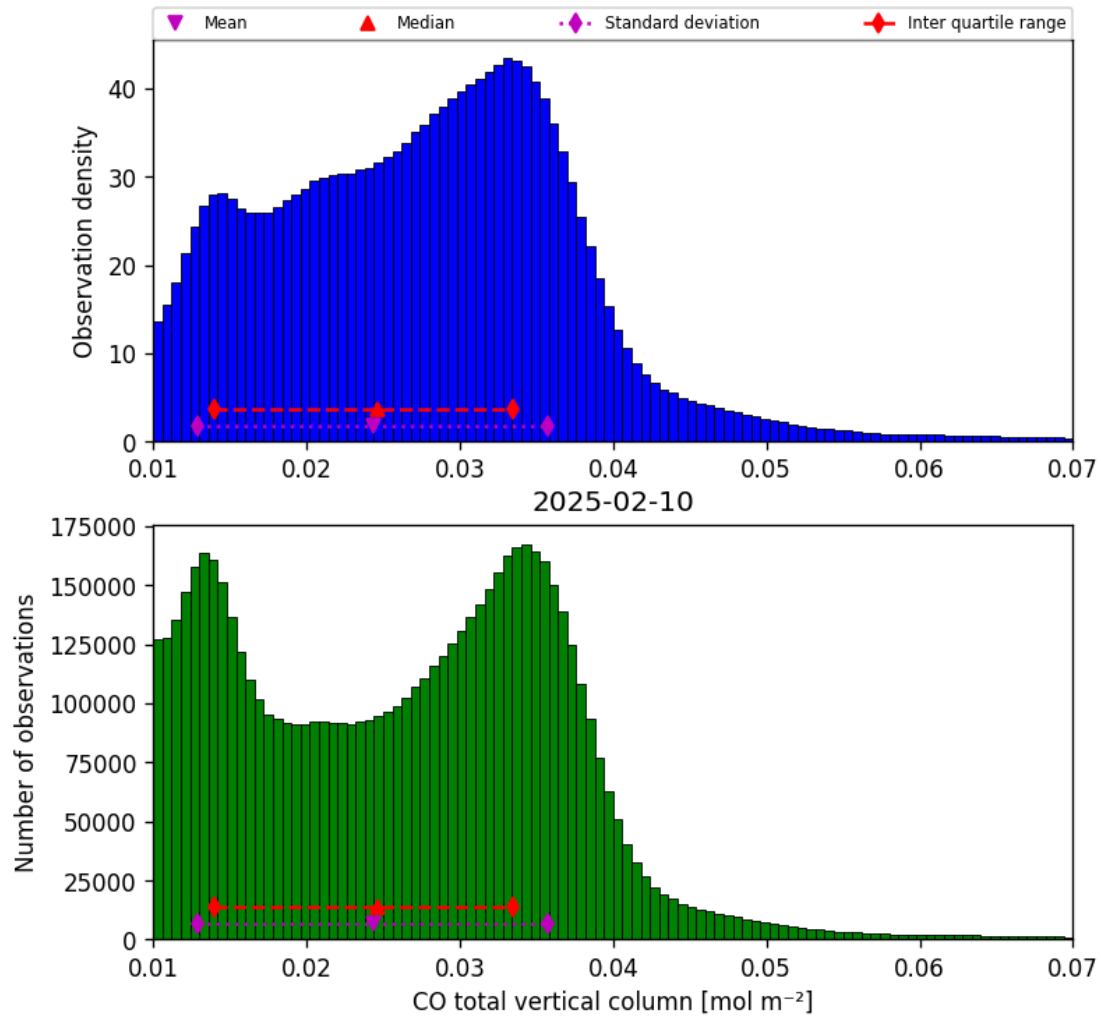
Figure 14: Histogram of “CO total vertical column” for 2025-02-10 to 2025-02-11
