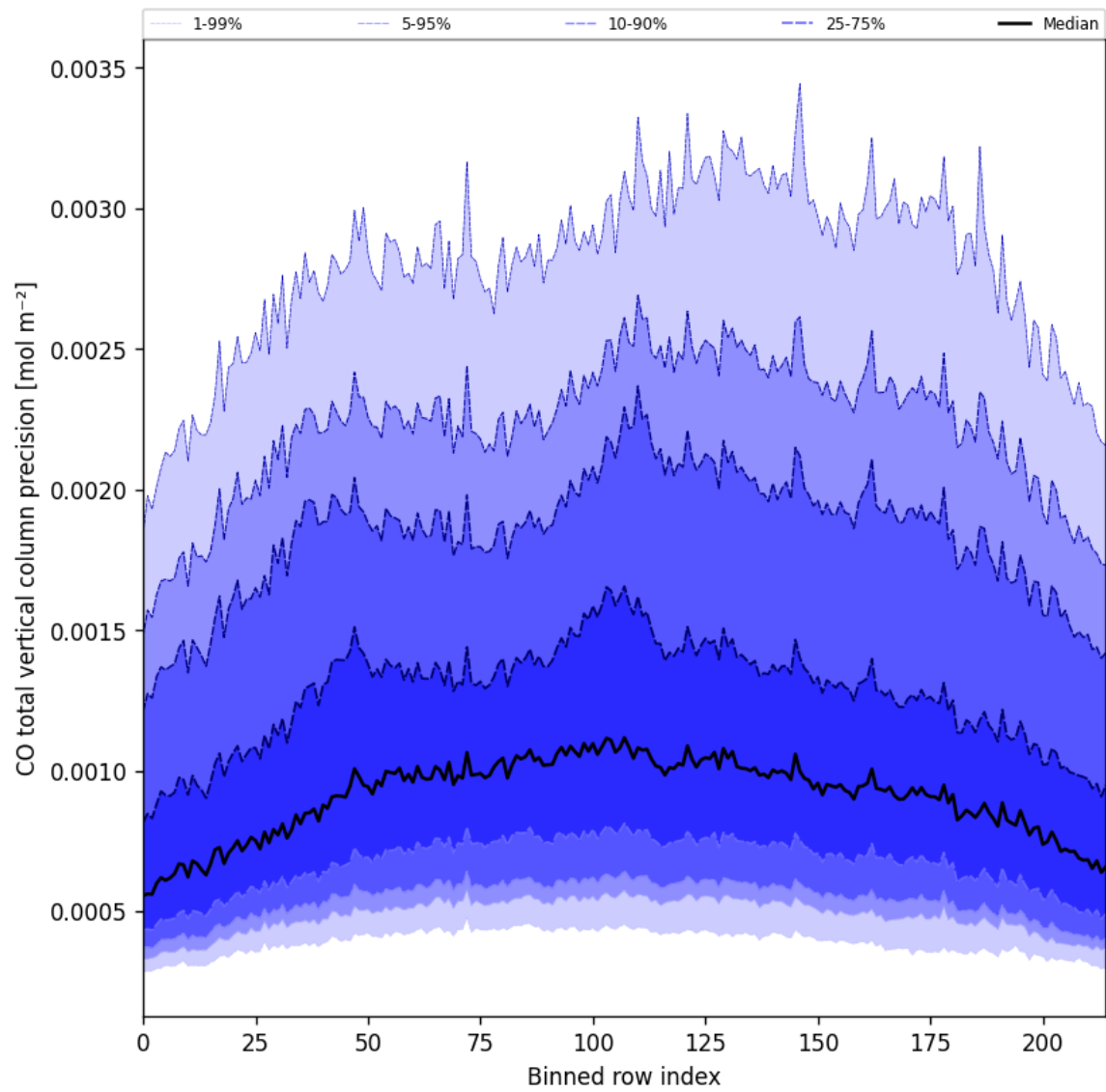
Figure 22: Along track statistics of “CO total vertical column precision” for 2025-02-10 to 2025-02-11
