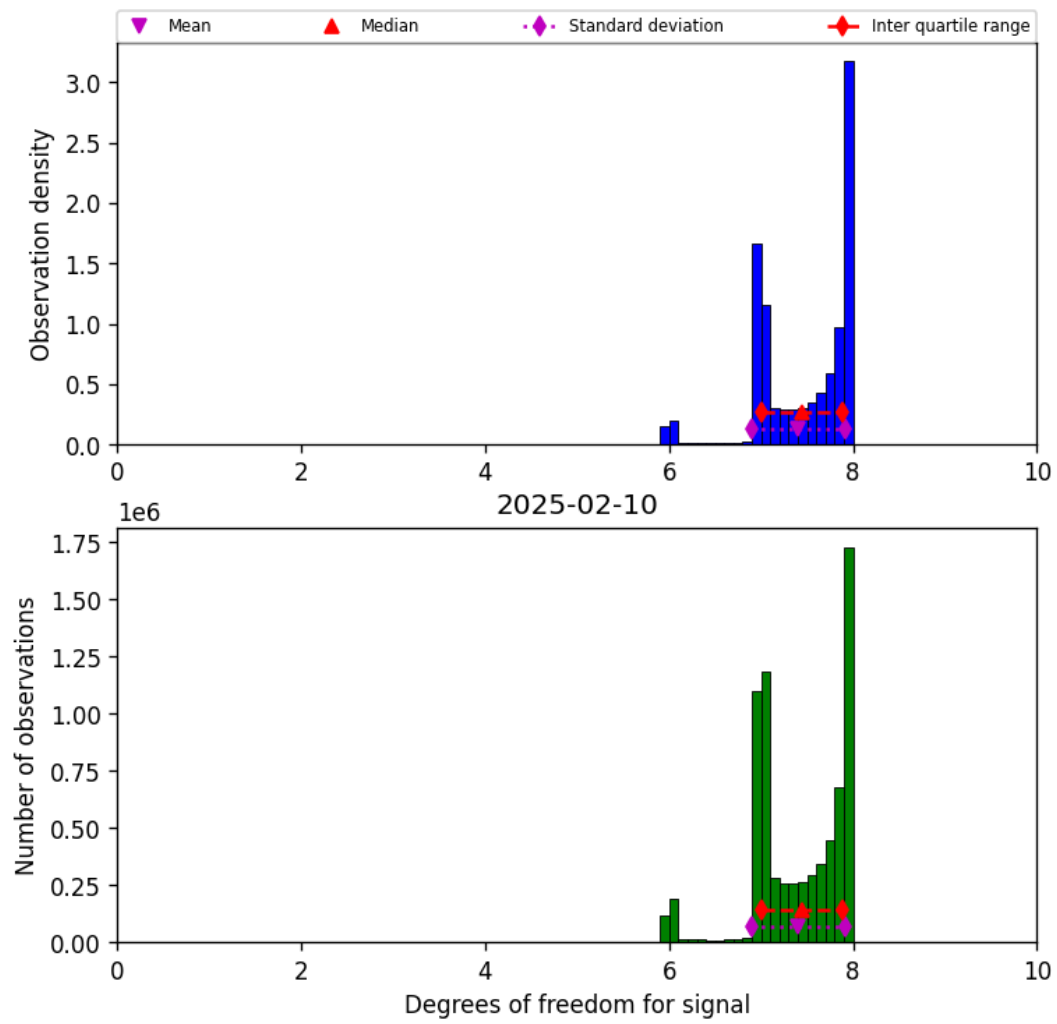
Figure 18: Histogram of “Degrees of freedom for signal” for 2025-02-10 to 2025-02-11
