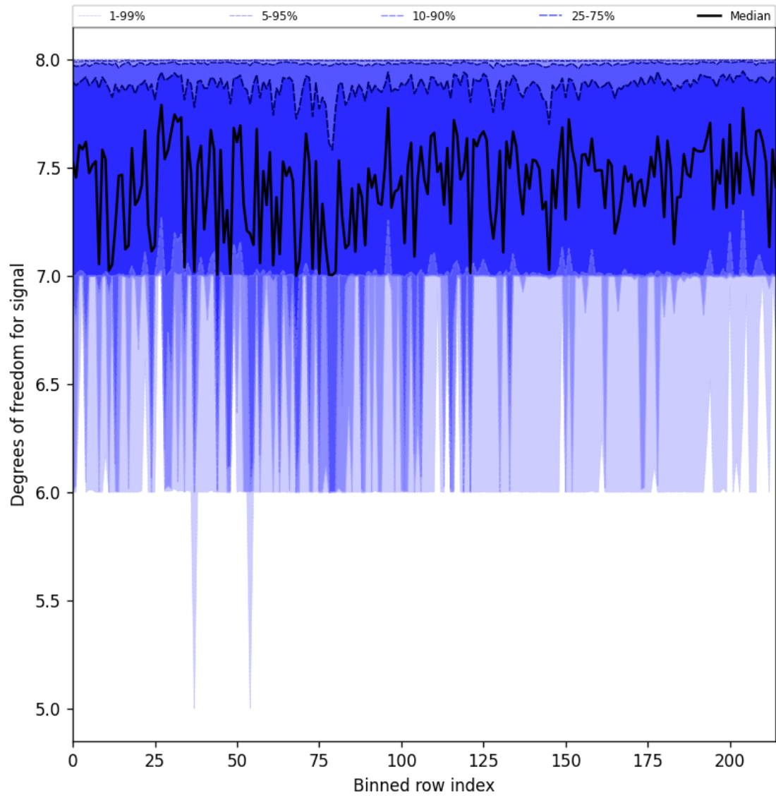
Figure 25: Along track statistics of “Degrees of freedom for signal” for 2025-02-10 to 2025-02-11
