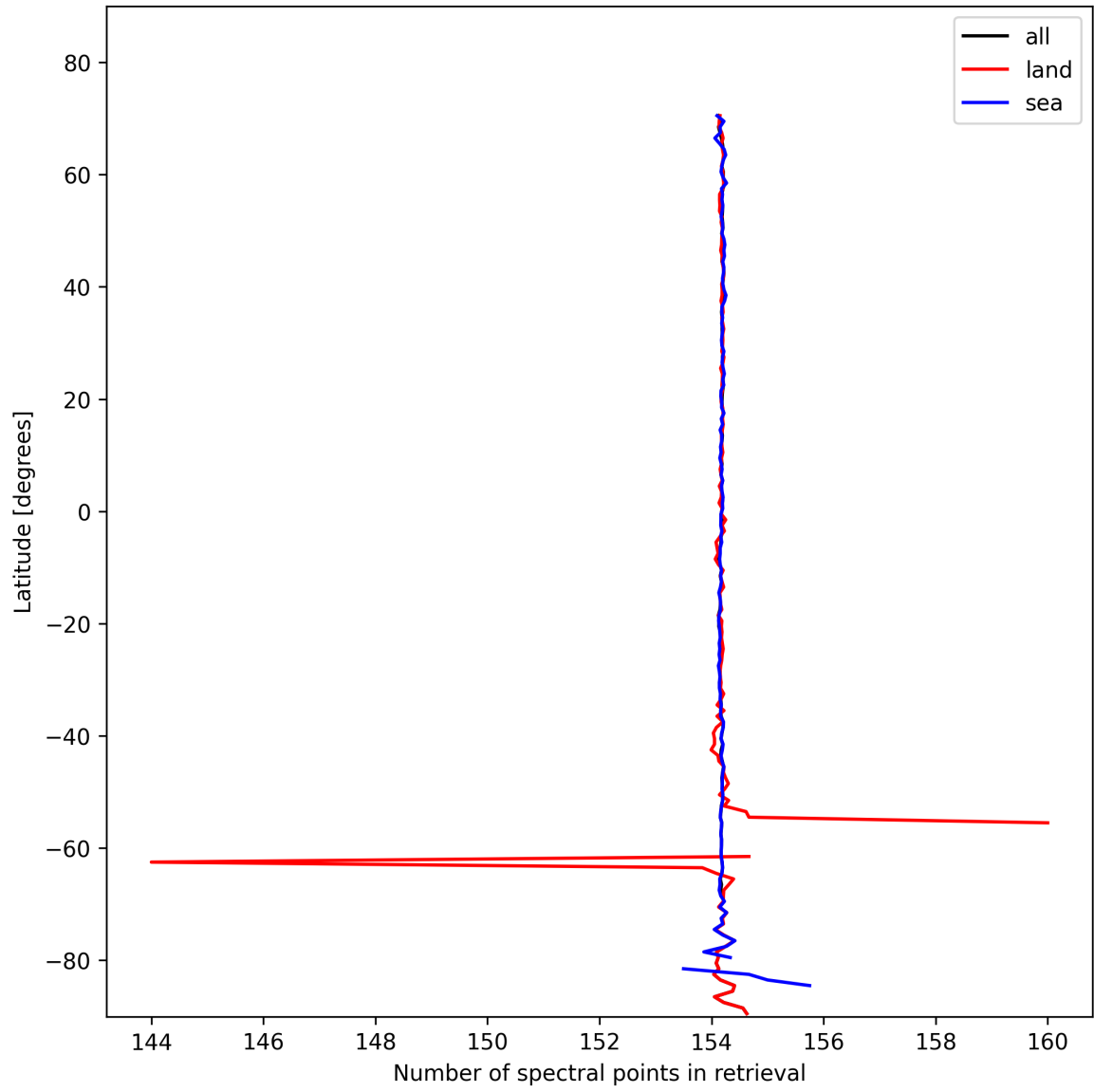
Figure 9: Zonal average of “Number of spectral points in retrieval” for 2025-02-10 to 2025-02-11.
