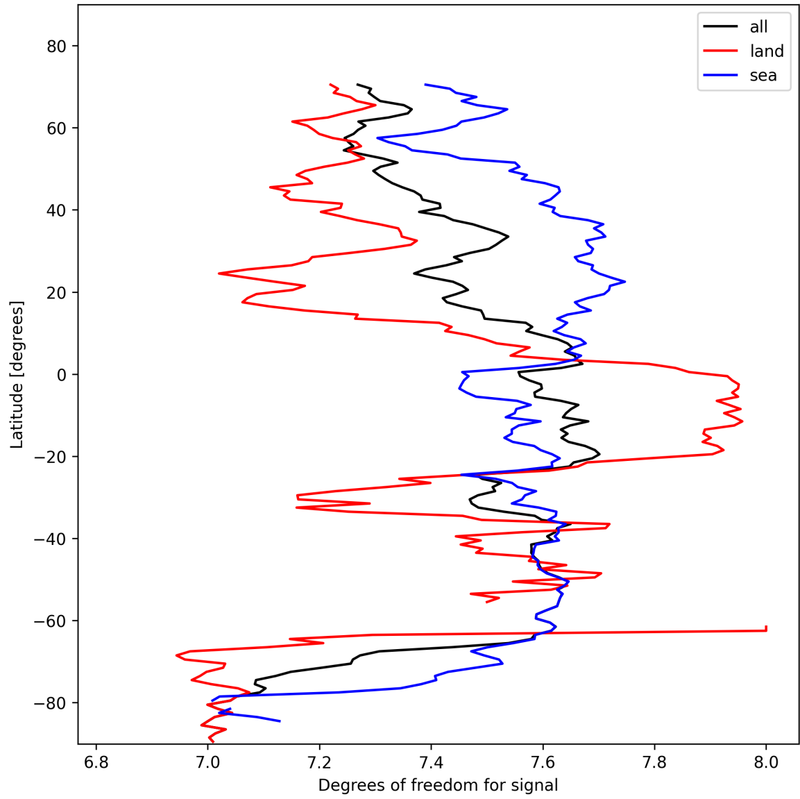
Figure 11: Zonal average of “Degrees of freedom for signal” for 2025-02-10 to 2025-02-11.
