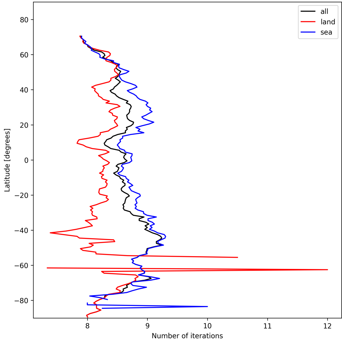
Figure 12: Zonal average of “Number of iterations” for 2025-02-10 to 2025-02-11.
