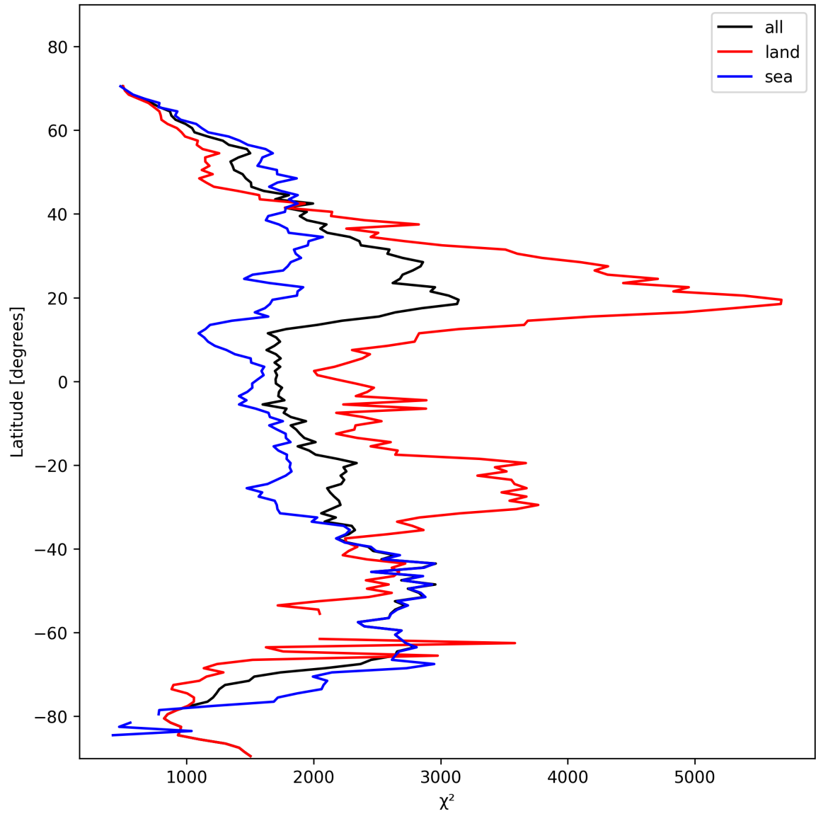
Figure 10: Zonal average of “ \chi^2 ” for 2025-02-10 to 2025-02-11.
