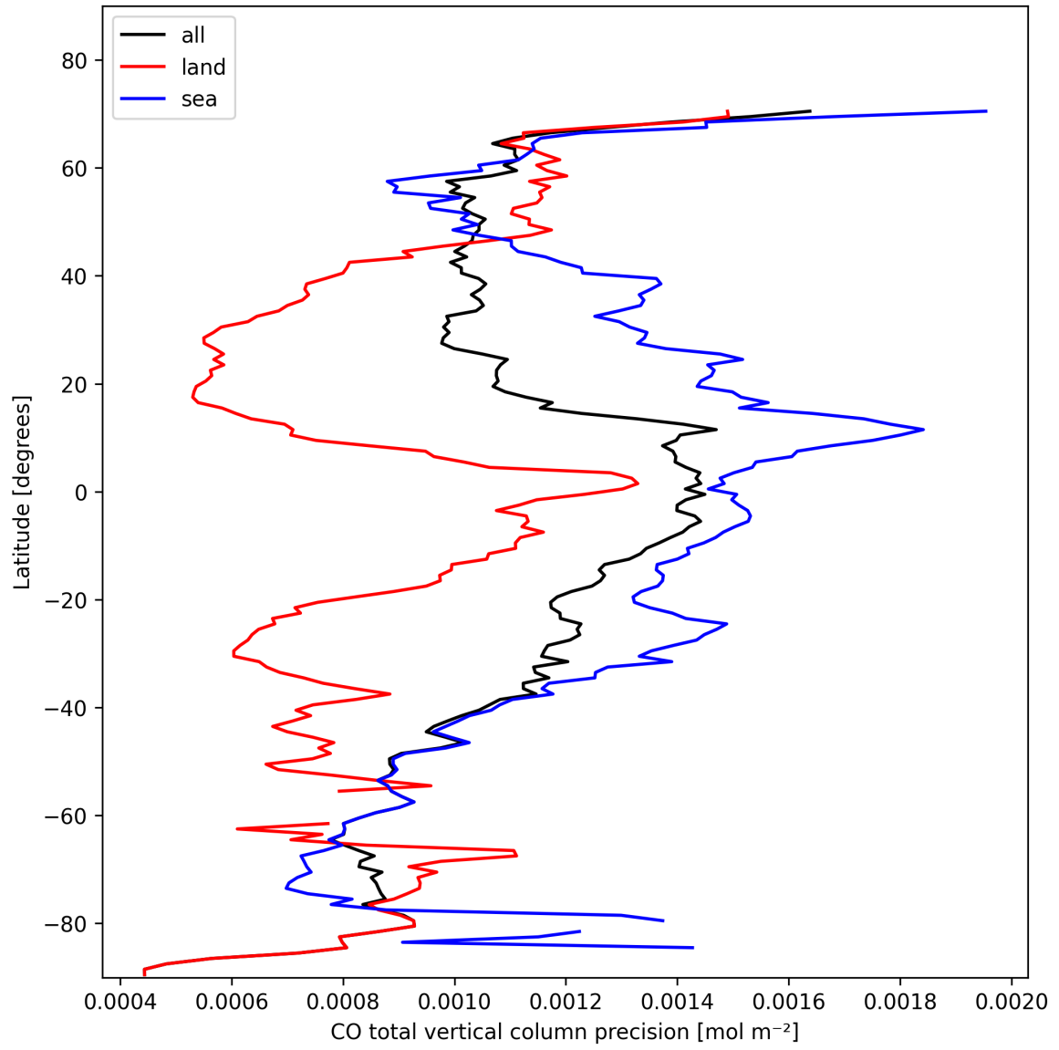
Figure 8: Zonal average of “CO total vertical column precision” for 2025-02-10 to 2025-02-11.
