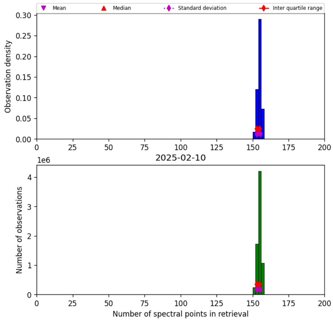
Figure 16: Histogram of “Number of spectral points in retrieval” for 2025-02-10 to 2025-02-11
