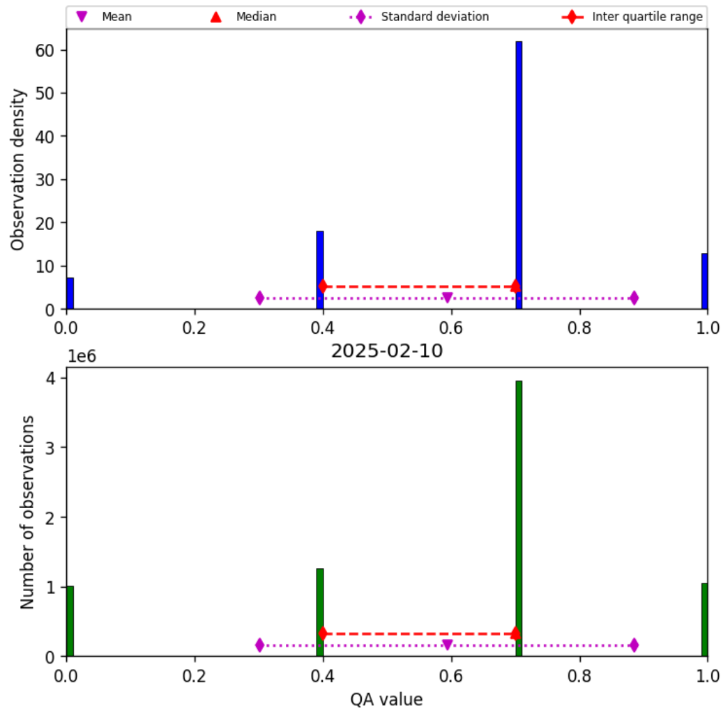
Figure 13: Histogram of “QA value” for 2025-02-10 to 2025-02-11
