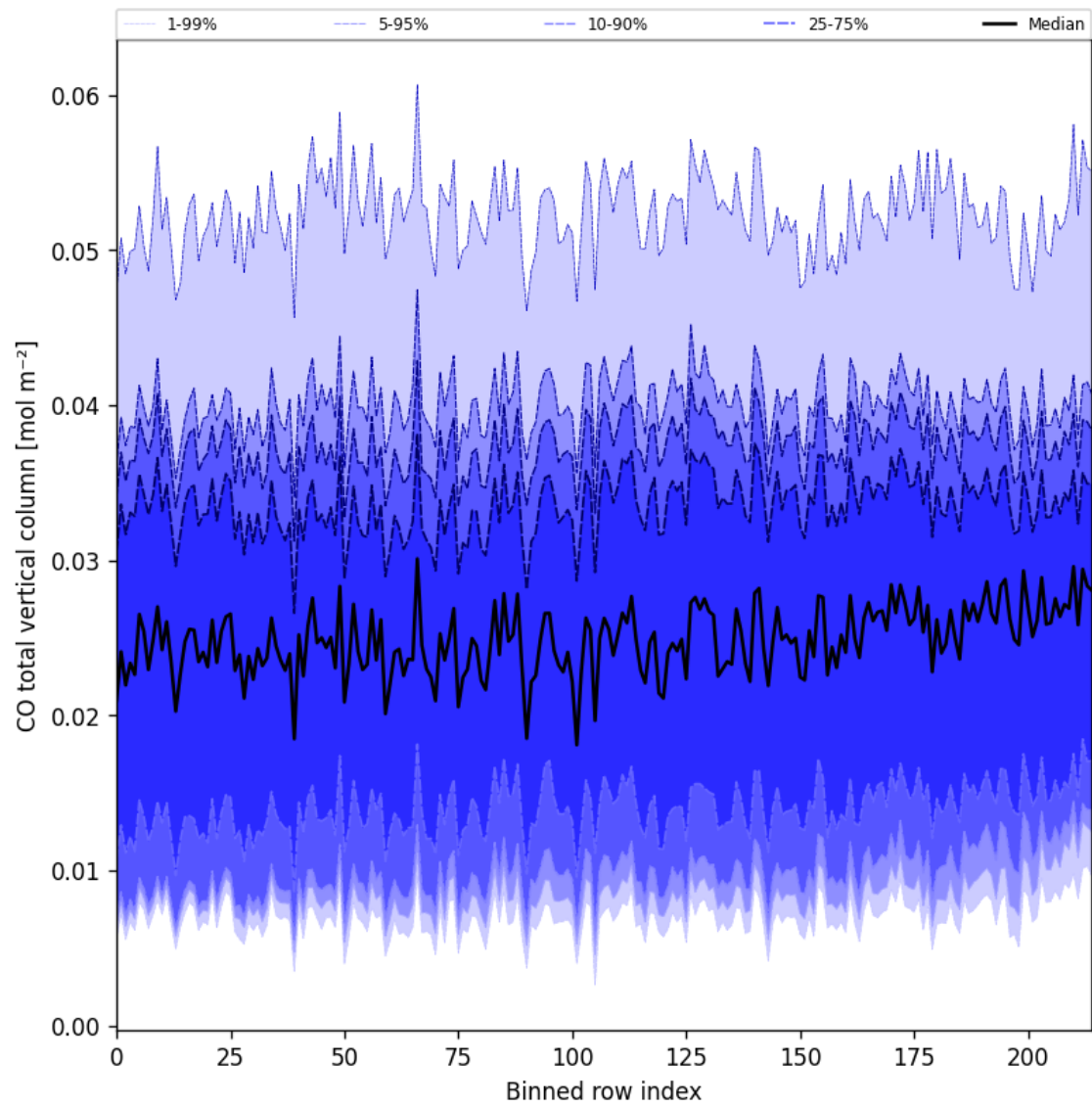
Figure 21: Along track statistics of “CO total vertical column” for 2025-02-10 to 2025-02-11
