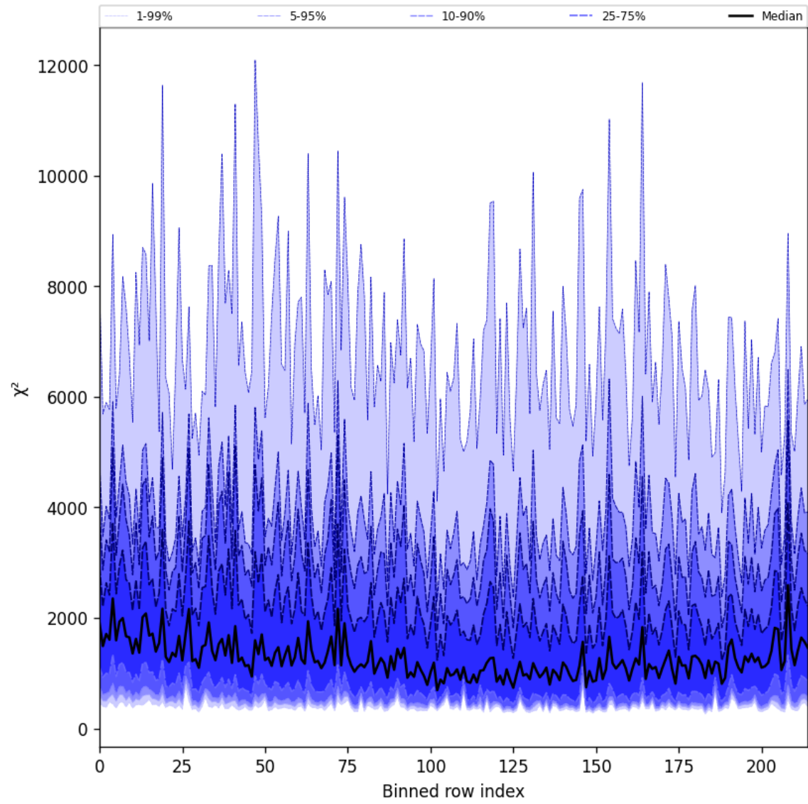
Figure 24: Along track statistics of “ \chi^2 ” for 2025-02-10 to 2025-02-11
