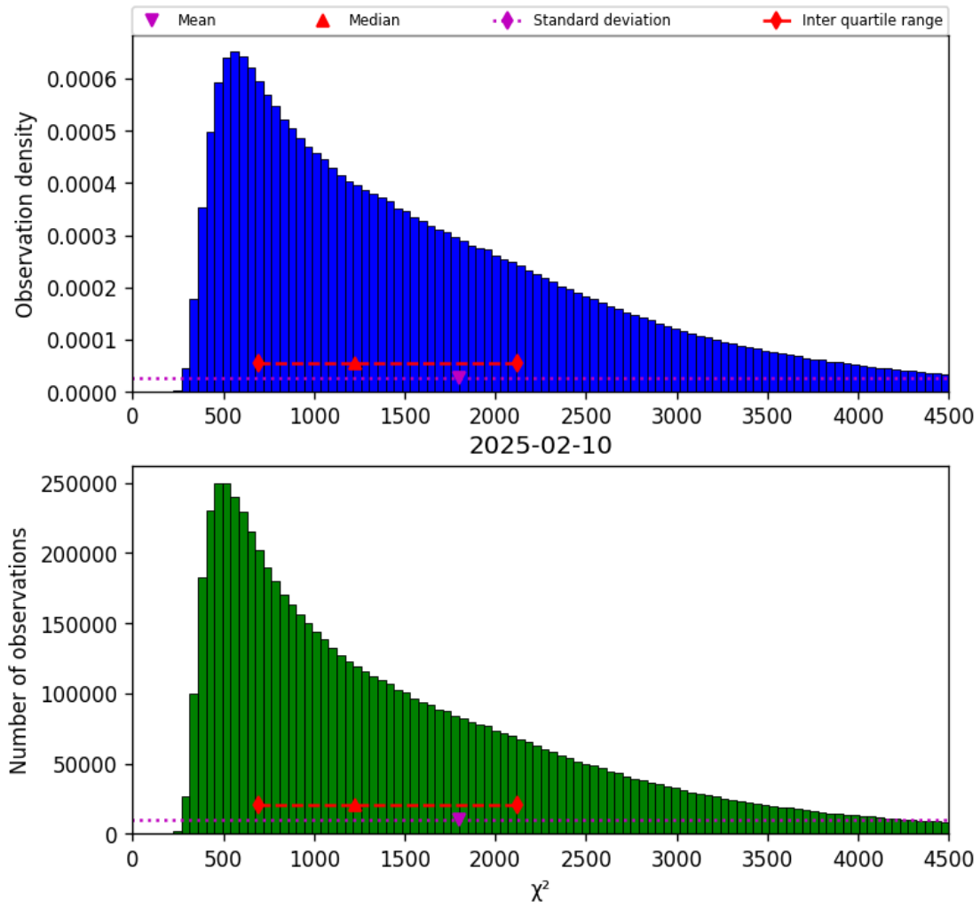
Figure 17: Histogram of “ \chi^2 ” for 2025-02-10 to 2025-02-11
