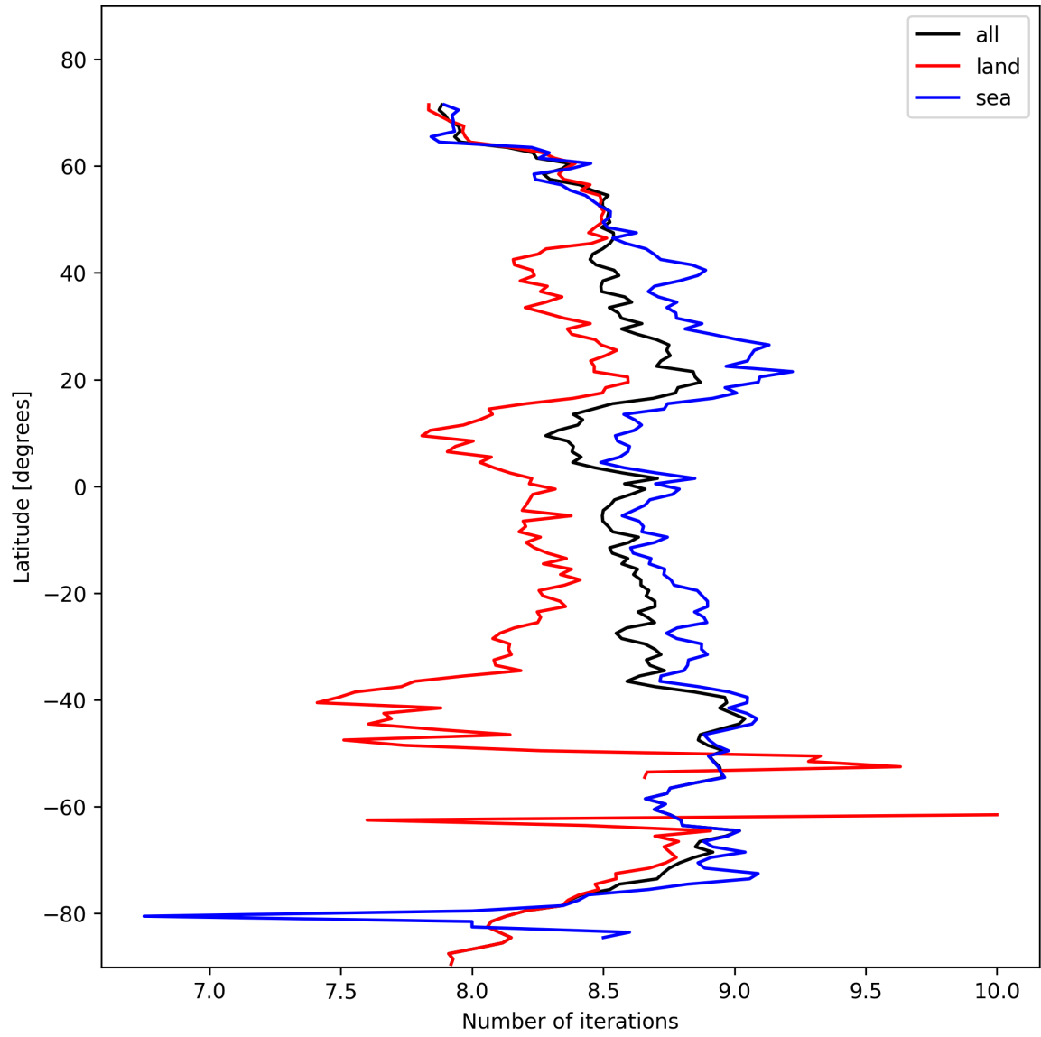
Figure 12: Zonal average of “Number of iterations” for 2025-02-11 to 2025-02-11.
