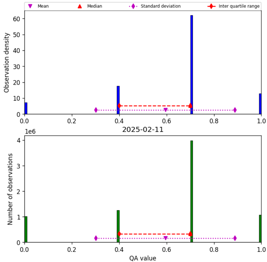
Figure 13: Histogram of "QA value" for 2025-02-11 to 2025-02-11
