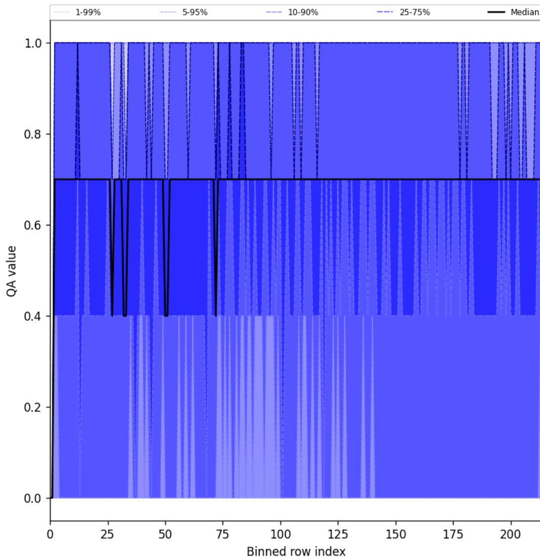
Figure 20: Along track statistics of “QA value” for 2025-02-11 to 2025-02-11
