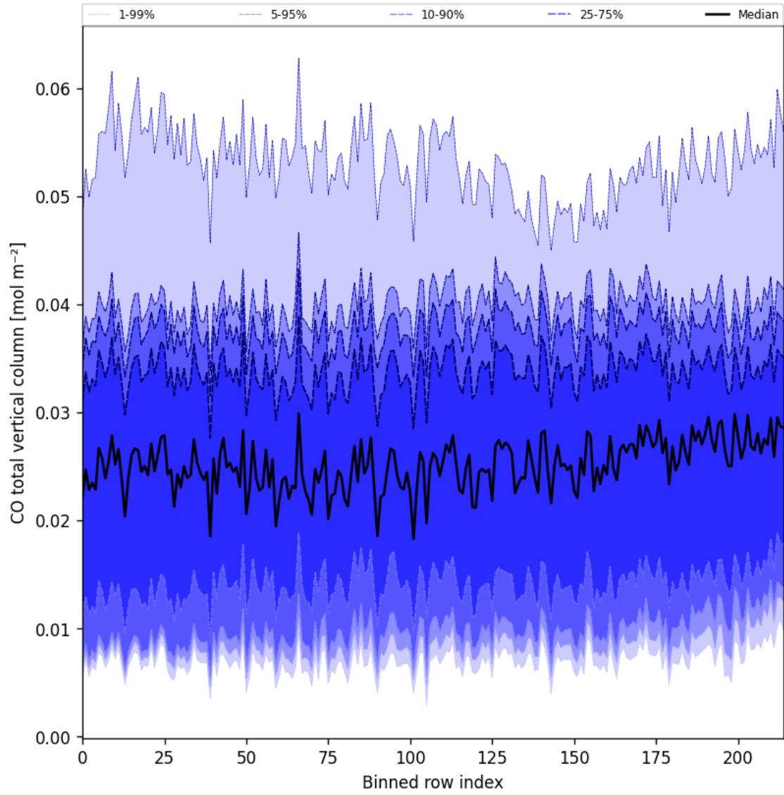
Figure 21: Along track statistics of “CO total vertical column” for 2025-02-11 to 2025-02-11
