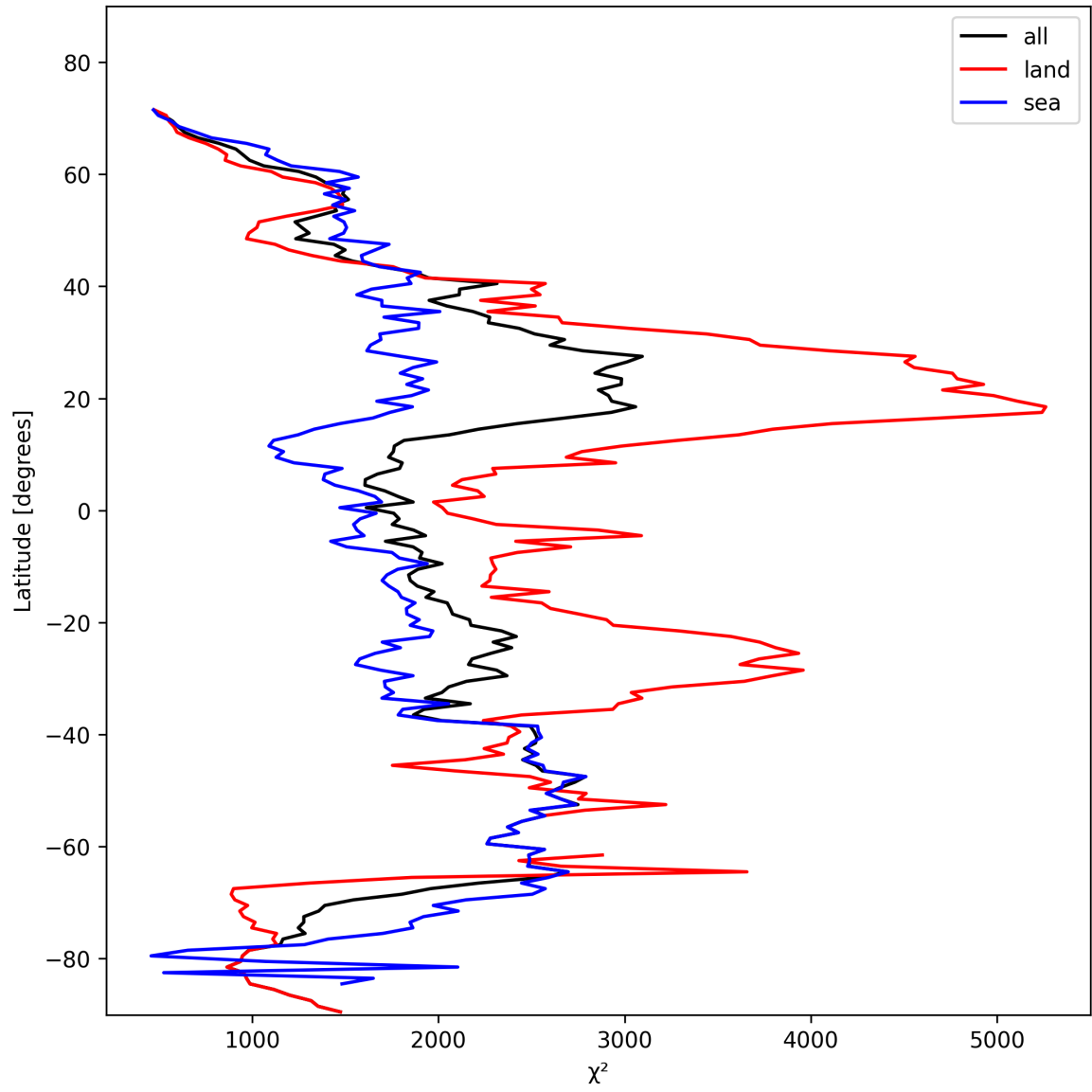
Figure 10: Zonal average of “ \chi^2 ” for 2025-02-11 to 2025-02-11.
