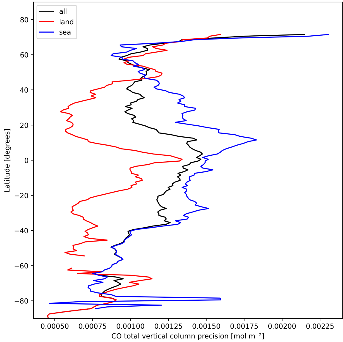
Figure 8: Zonal average of “CO total vertical column precision” for 2025-02-11 to 2025-02-11.
