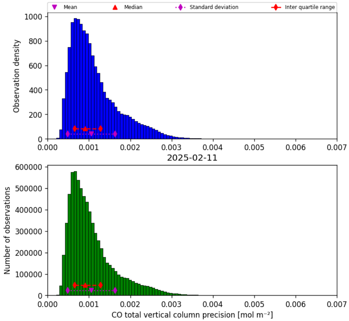
Figure 15: Histogram of “CO total vertical column precision” for 2025-02-11 to 2025-02-11
