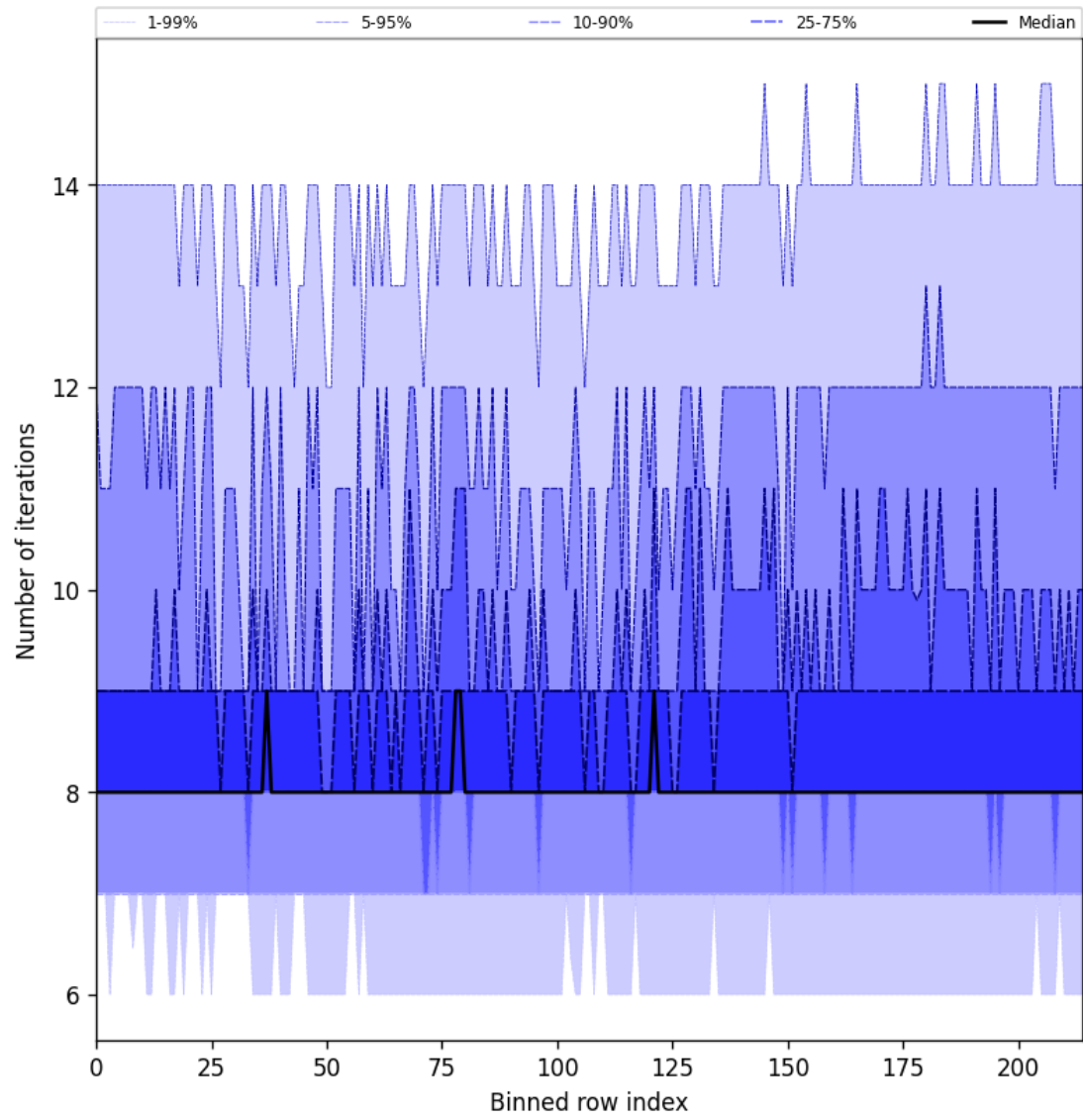
Figure 26: Along track statistics of “Number of iterations” for 2025-02-11 to 2025-02-11
