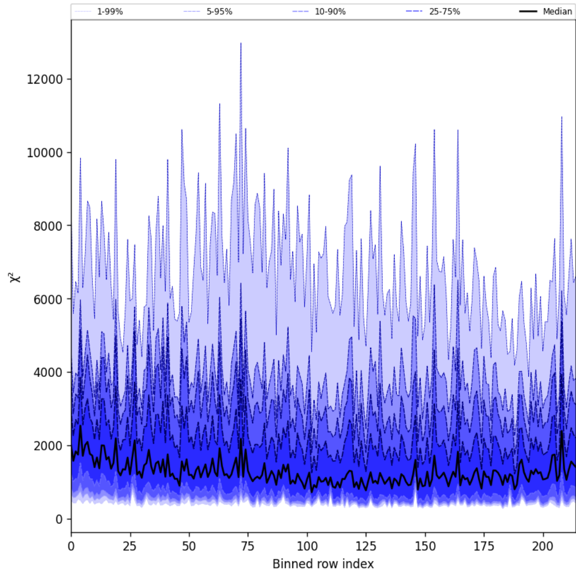
Figure 24: Along track statistics of “ \chi^2 ” for 2025-02-11 to 2025-02-11
