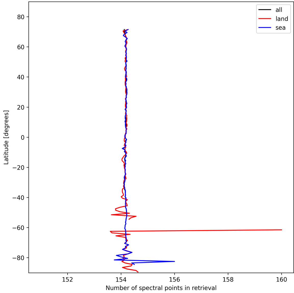
Figure 9: Zonal average of “Number of spectral points in retrieval” for 2025-02-11 to 2025-02-11.
