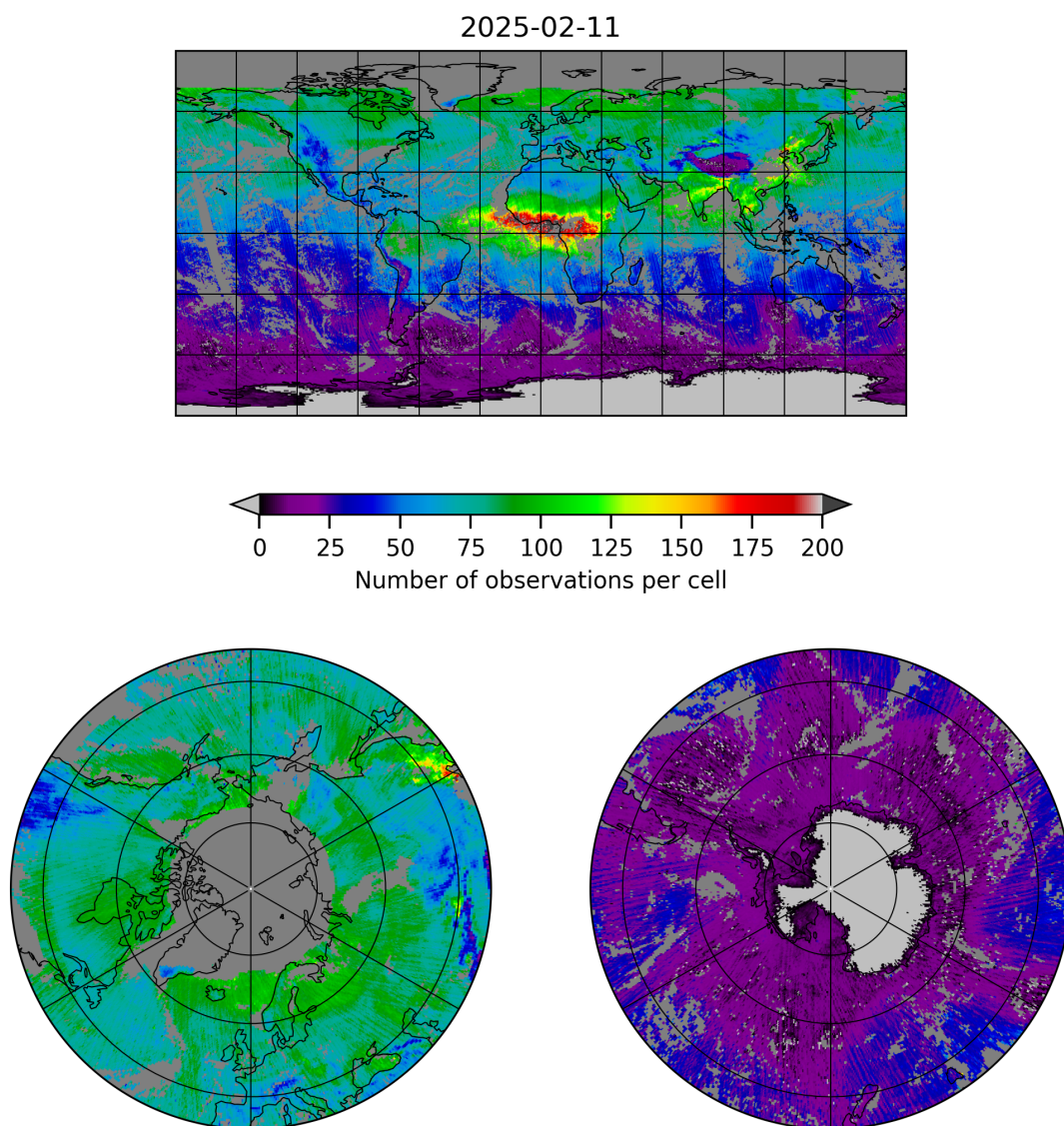
Figure 5: Map of the number of observations for 2025-02-11 to 2025-02-11
