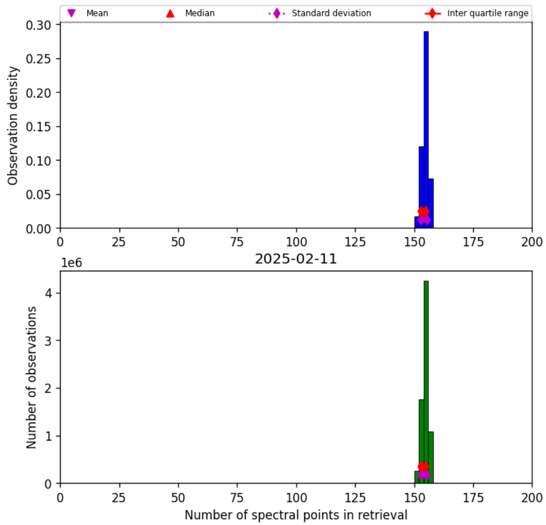
Figure 16: Histogram of “Number of spectral points in retrieval” for 2025-02-11 to 2025-02-11
