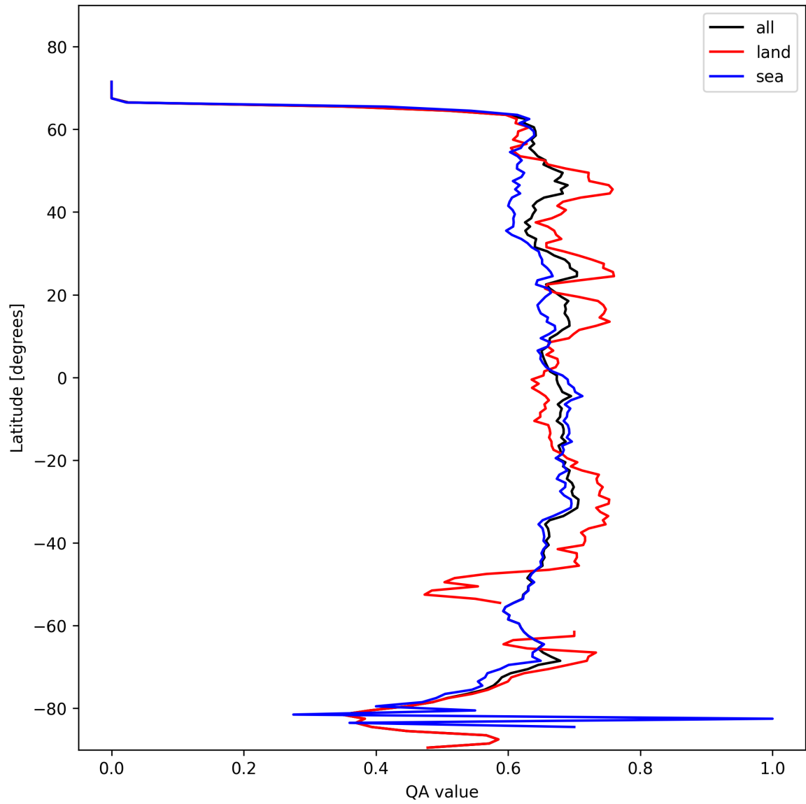
Figure 6: Zonal average of “QA value” for 2025-02-11 to 2025-02-11.
