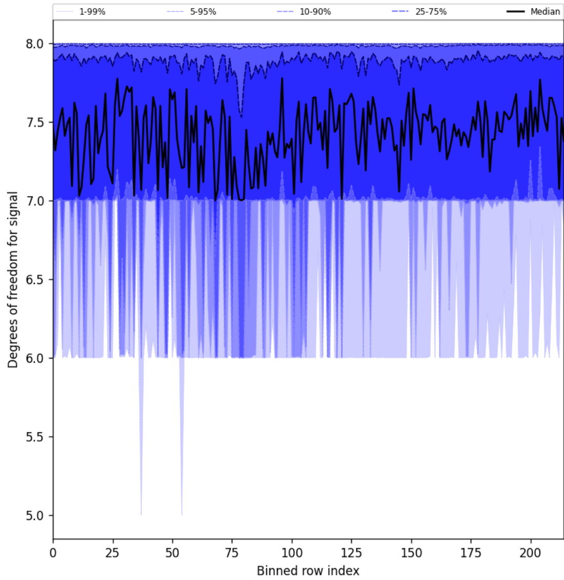
Figure 25: Along track statistics of “Degrees of freedom for signal” for 2025-02-11 to 2025-02-11
