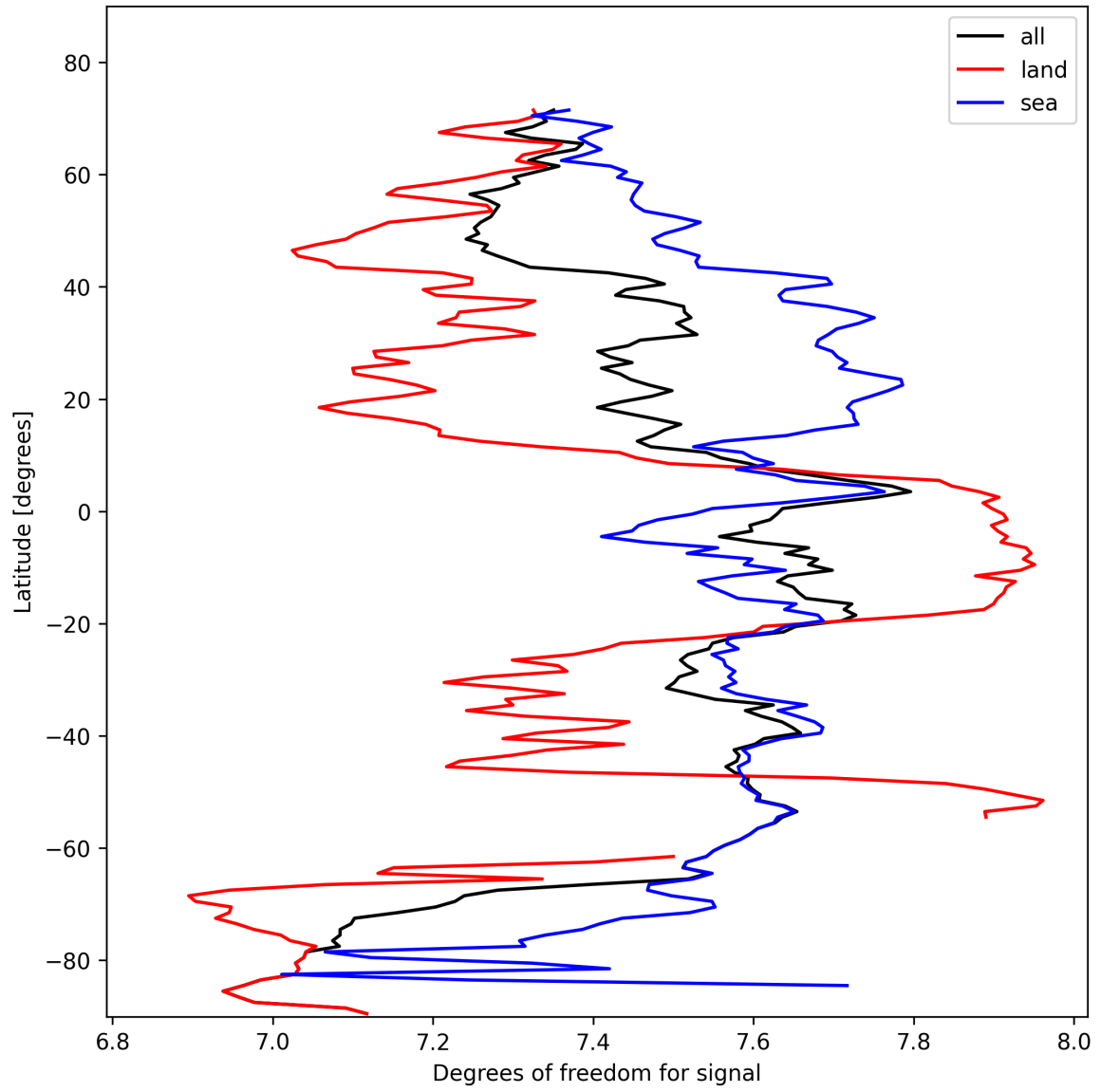
Figure 11: Zonal average of “Degrees of freedom for signal” for 2025-02-11 to 2025-02-11.
