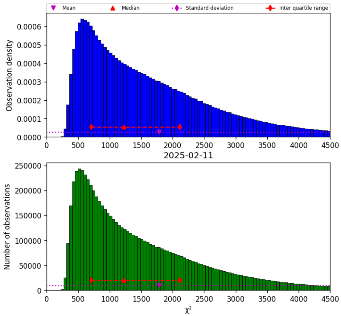
Figure 17: Histogram of “ \chi^2 ” for 2025-02-11 to 2025-02-11
