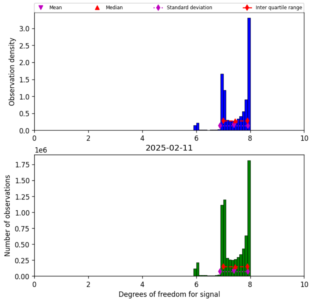
Figure 18: Histogram of “Degrees of freedom for signal” for 2025-02-11 to 2025-02-11
