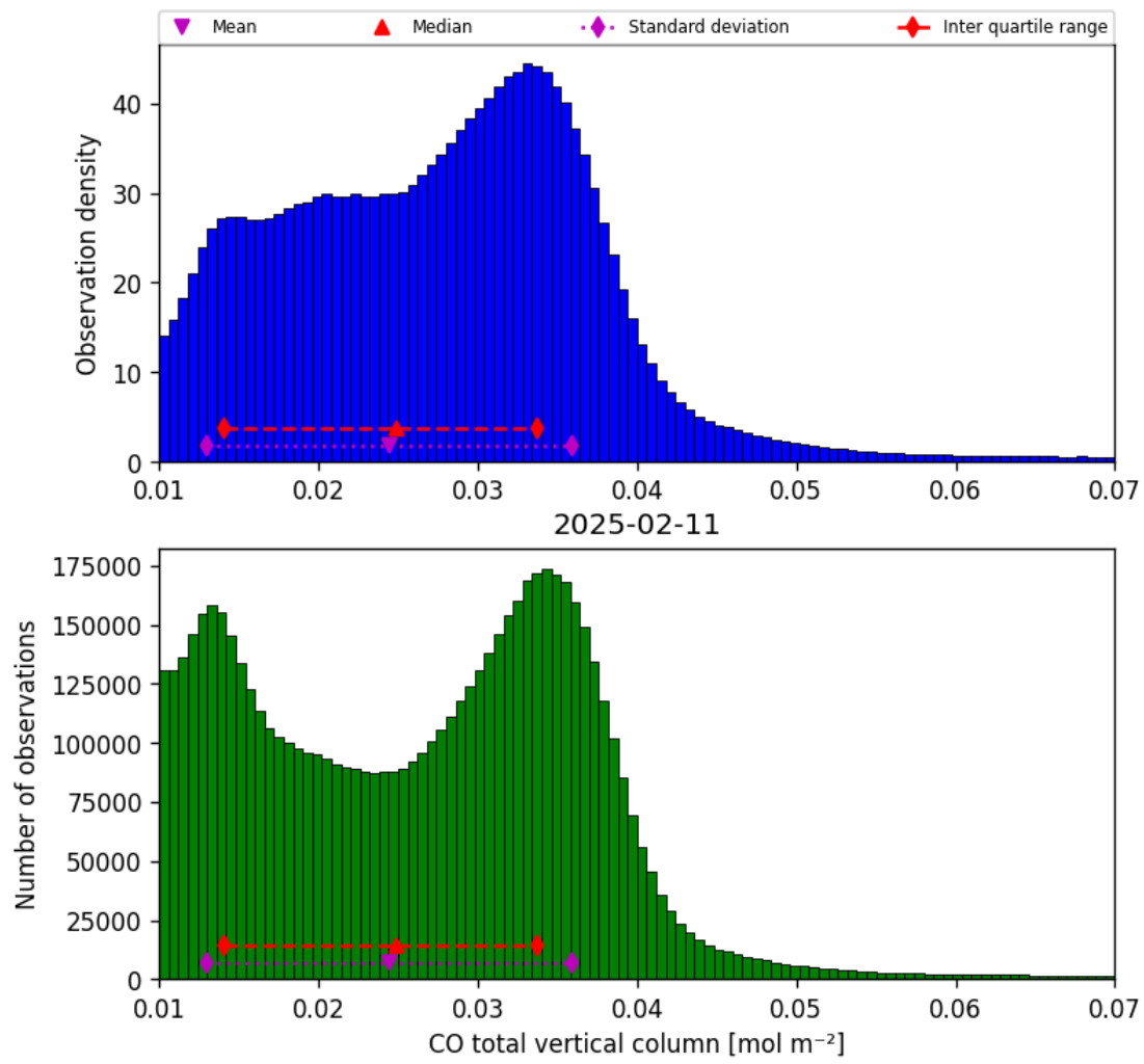
Figure 14: Histogram of “CO total vertical column” for 2025-02-11 to 2025-02-11
