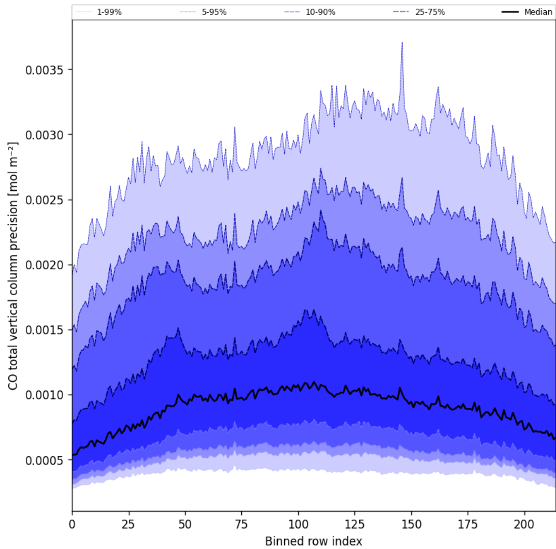
Figure 22: Along track statistics of “CO total vertical column precision” for 2025-02-11 to 2025-02-11
