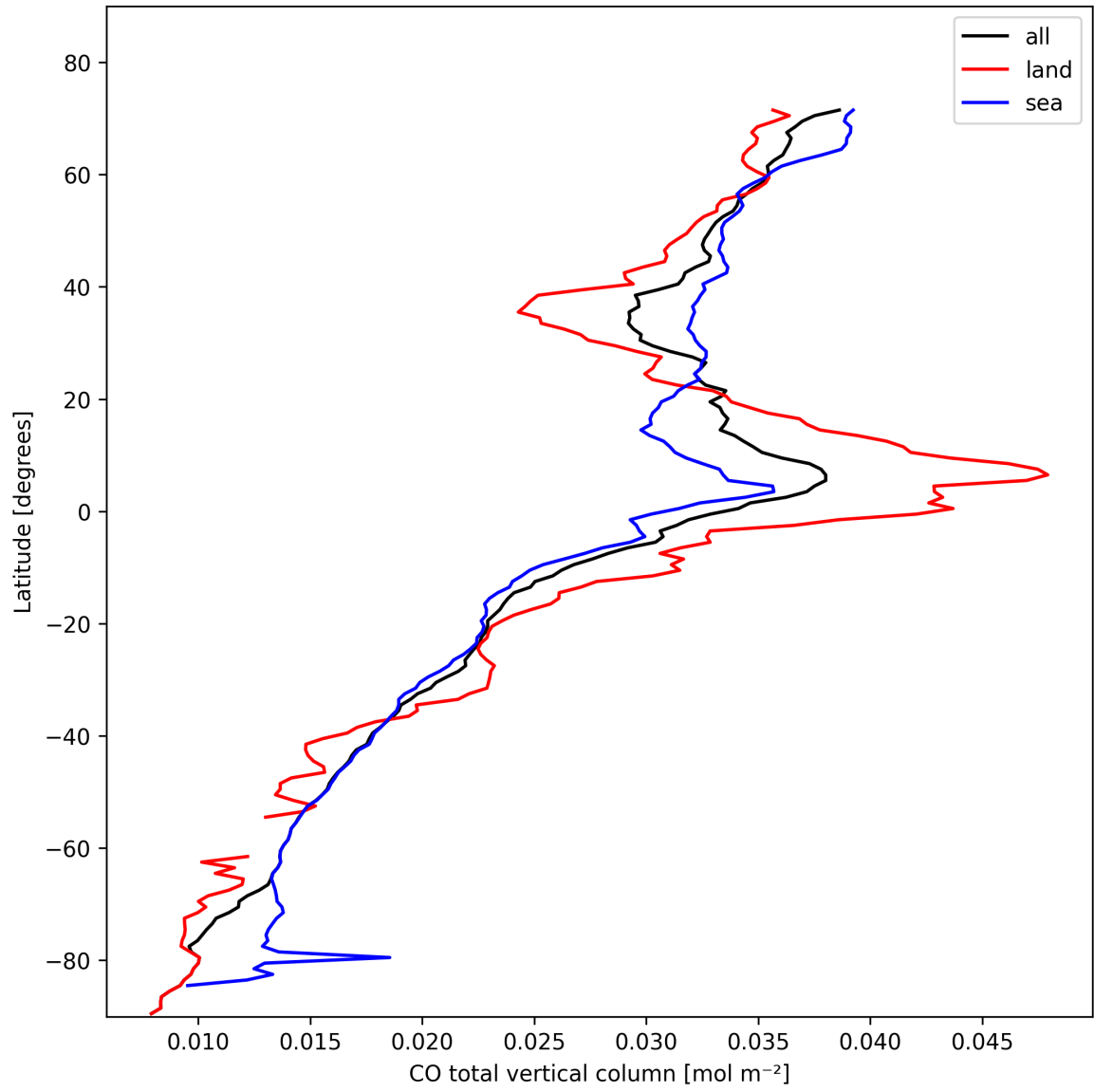
Figure 7: Zonal average of “CO total vertical column” for 2025-02-11 to 2025-02-11.
