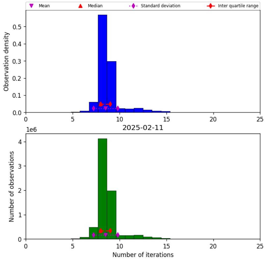
Figure 19: Histogram of “Number of iterations” for 2025-02-11 to 2025-02-11
