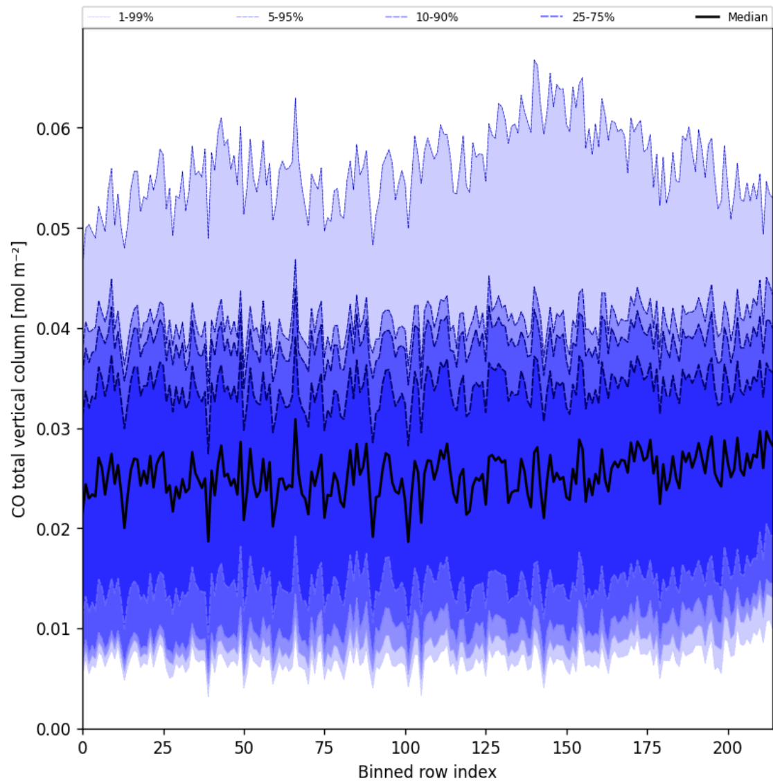
Figure 21: Along track statistics of “CO total vertical column” for 2025-02-14 to 2025-02-15
