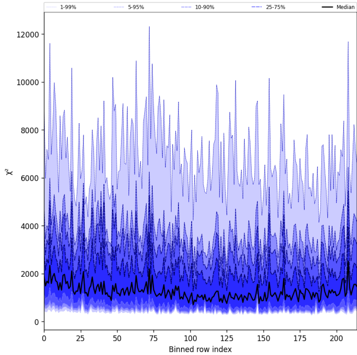
Figure 24: Along track statistics of “ \chi^2 ” for 2025-02-14 to 2025-02-15
