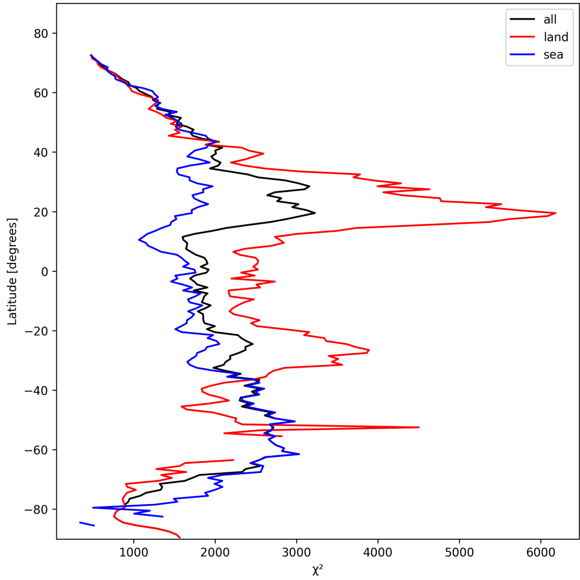
Figure 10: Zonal average of “ \chi^2 ” for 2025-02-14 to 2025-02-15.
