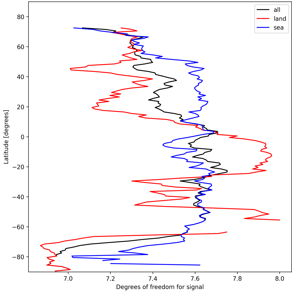
Figure 11: Zonal average of “Degrees of freedom for signal” for 2025-02-14 to 2025-02-15.
