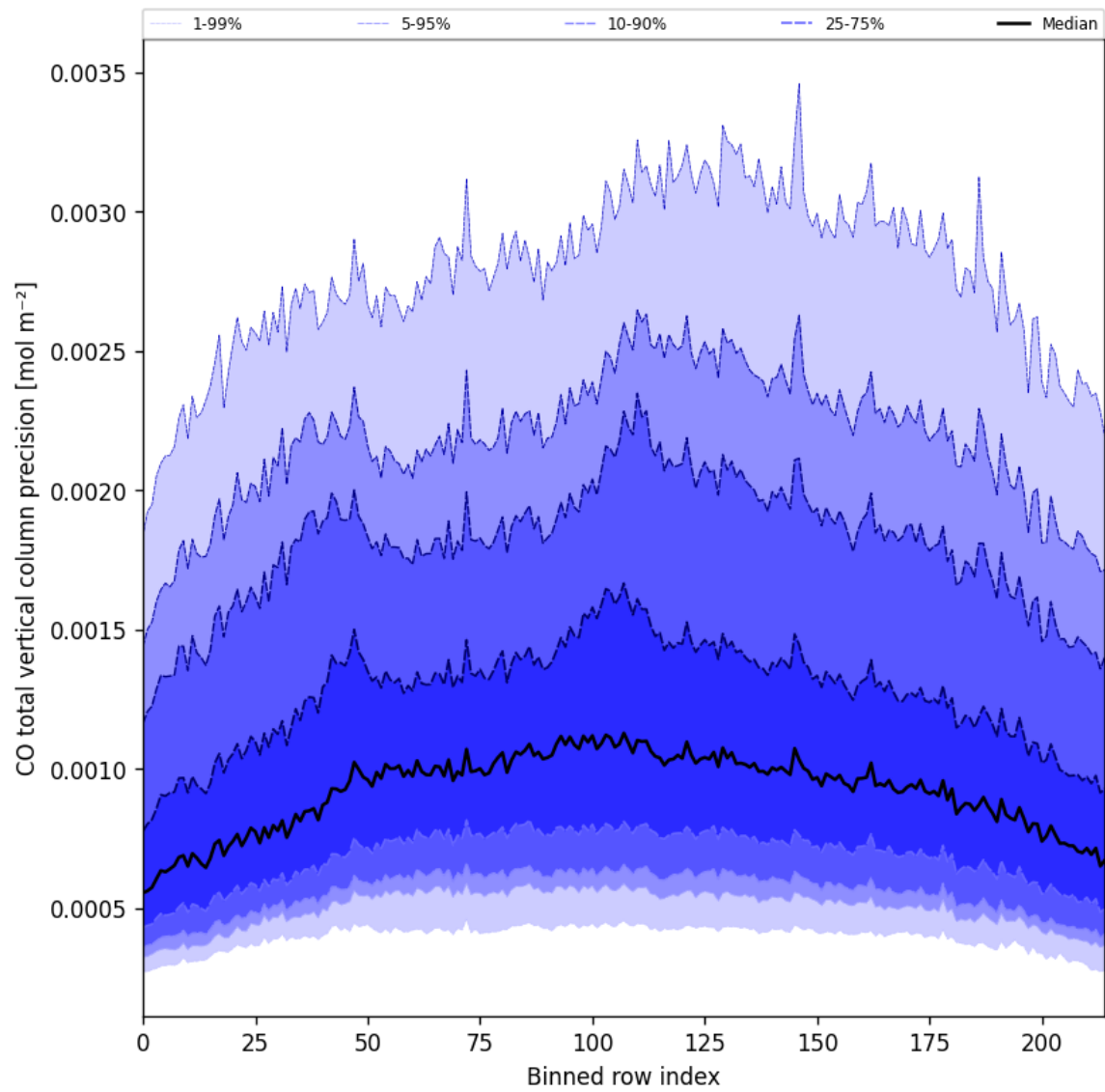
Figure 22: Along track statistics of “CO total vertical column precision” for 2025-02-14 to 2025-02-15
