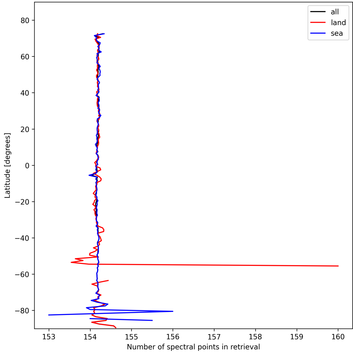
Figure 9: Zonal average of “Number of spectral points in retrieval” for 2025-02-14 to 2025-02-15.
