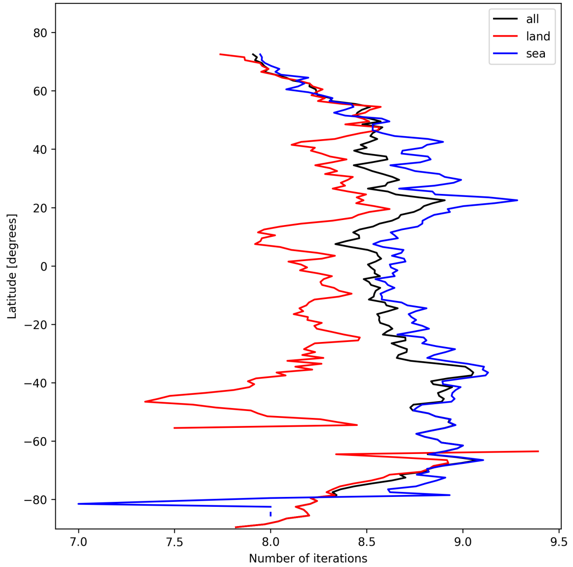
Figure 12: Zonal average of “Number of iterations” for 2025-02-14 to 2025-02-15.
