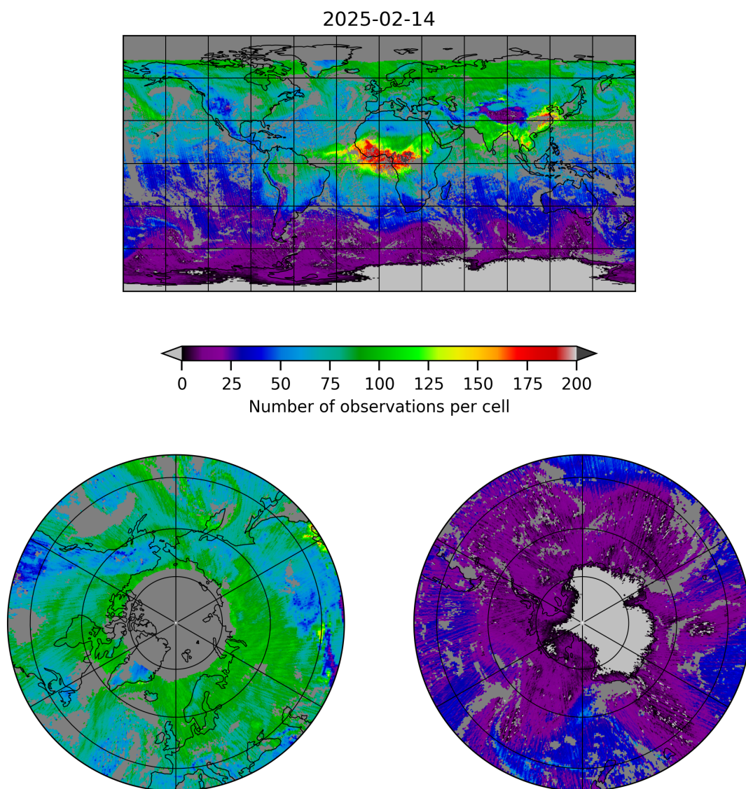
Figure 5: Map of the number of observations for 2025-02-14 to 2025-02-15
