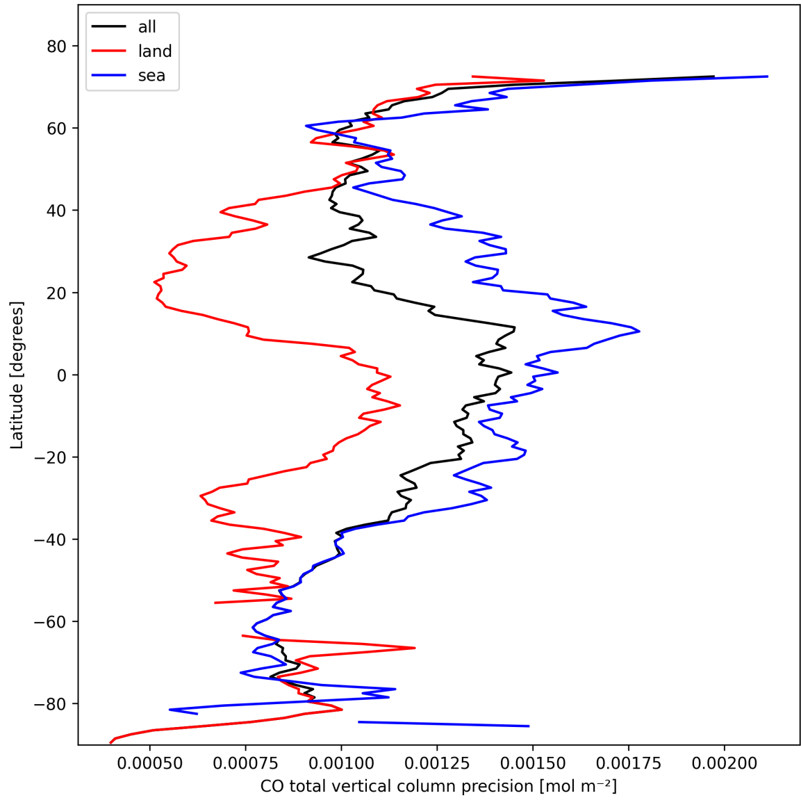
Figure 8: Zonal average of “CO total vertical column precision” for 2025-02-14 to 2025-02-15.
