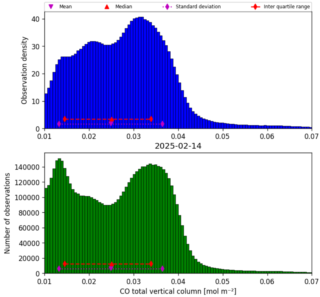
Figure 14: Histogram of “CO total vertical column” for 2025-02-14 to 2025-02-15
