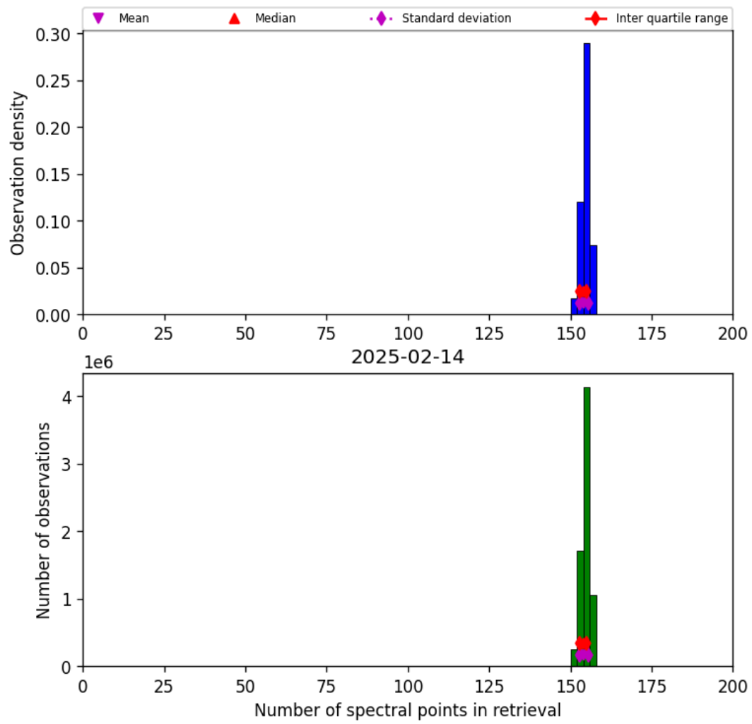
Figure 16: Histogram of “Number of spectral points in retrieval” for 2025-02-14 to 2025-02-15
