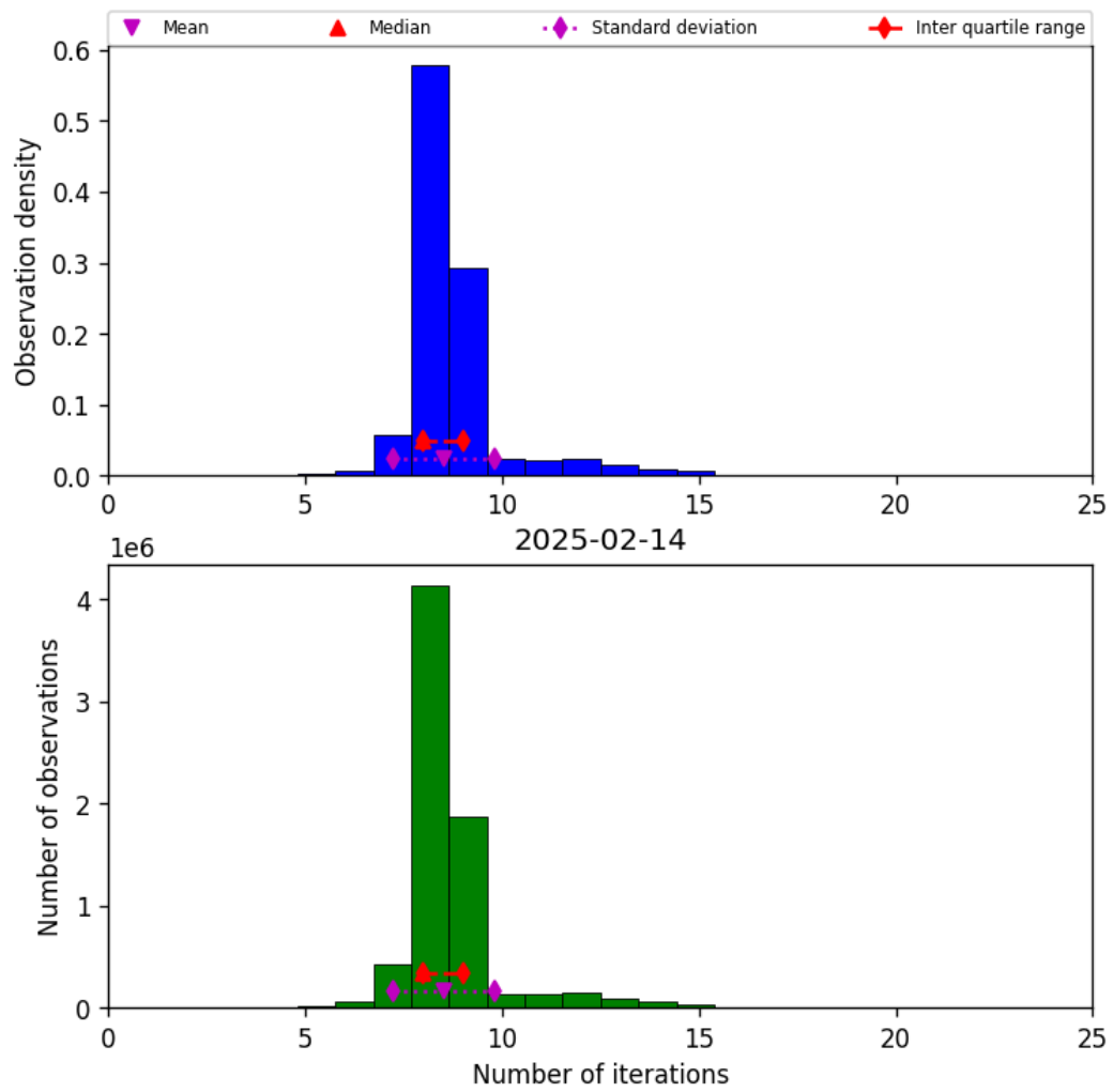
Figure 19: Histogram of “Number of iterations” for 2025-02-14 to 2025-02-15
