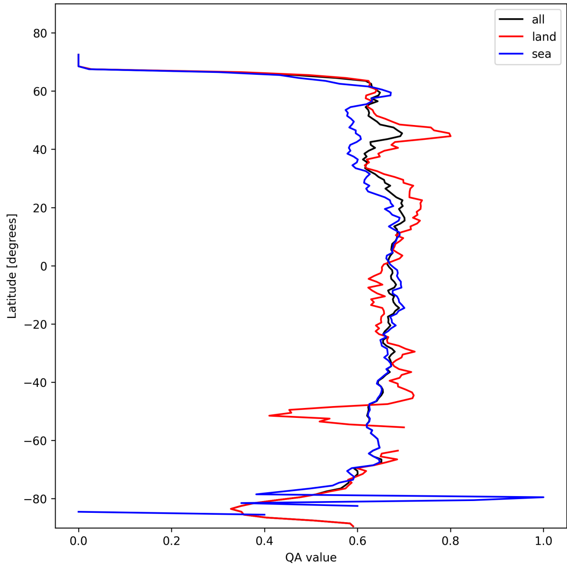
Figure 6: Zonal average of “QA value” for 2025-02-14 to 2025-02-15.
