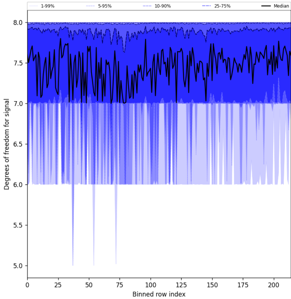
Figure 25: Along track statistics of “Degrees of freedom for signal” for 2025-02-14 to 2025-02-15
