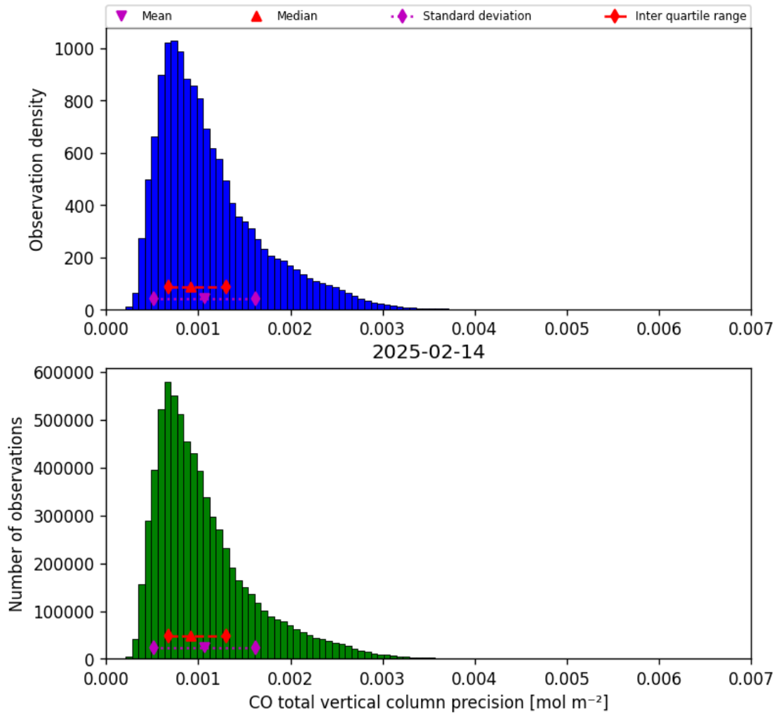
Figure 15: Histogram of “CO total vertical column precision” for 2025-02-14 to 2025-02-15
