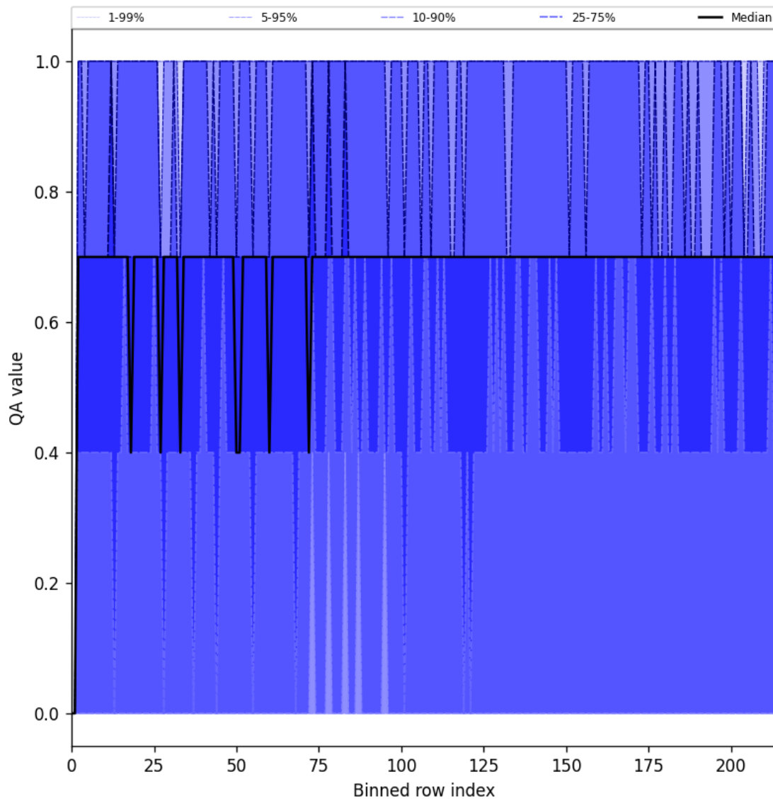
Figure 20: Along track statistics of “QA value” for 2025-02-14 to 2025-02-15
