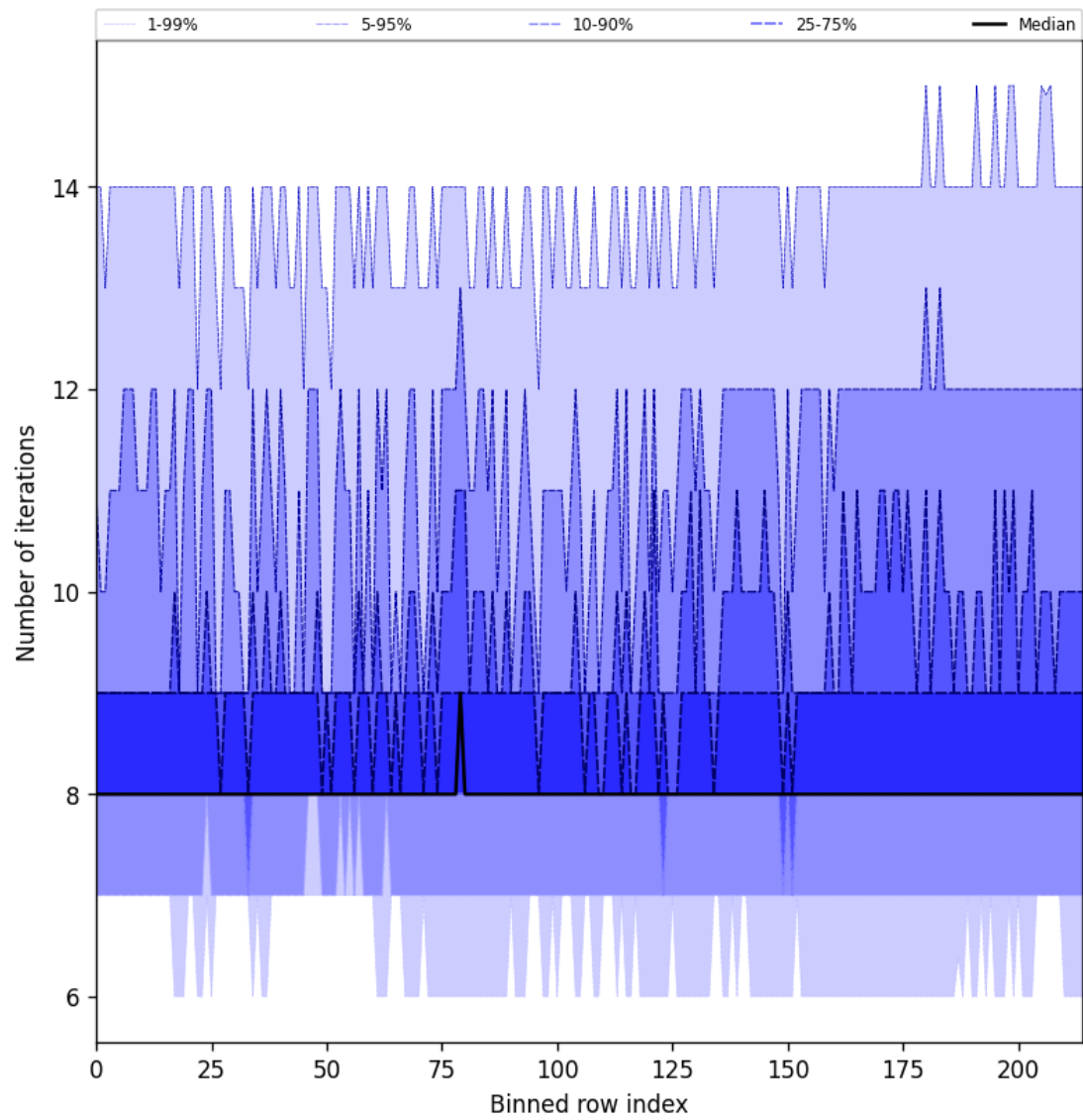
Figure 26: Along track statistics of “Number of iterations” for 2025-02-14 to 2025-02-15
