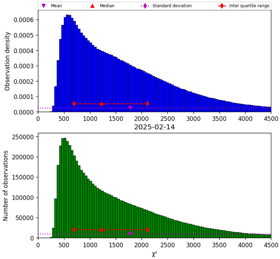
Figure 17: Histogram of “ \chi^2 ” for 2025-02-14 to 2025-02-15
