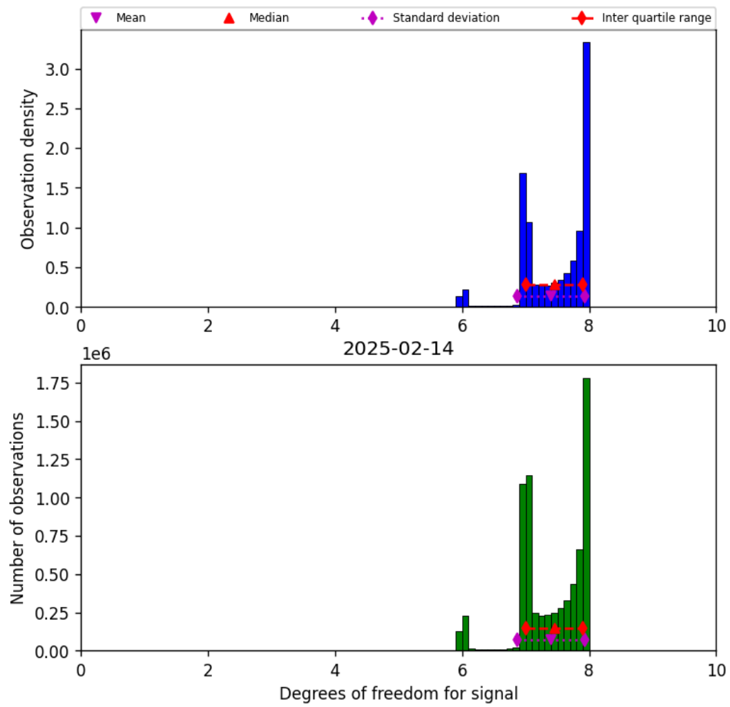
Figure 18: Histogram of “Degrees of freedom for signal” for 2025-02-14 to 2025-02-15
