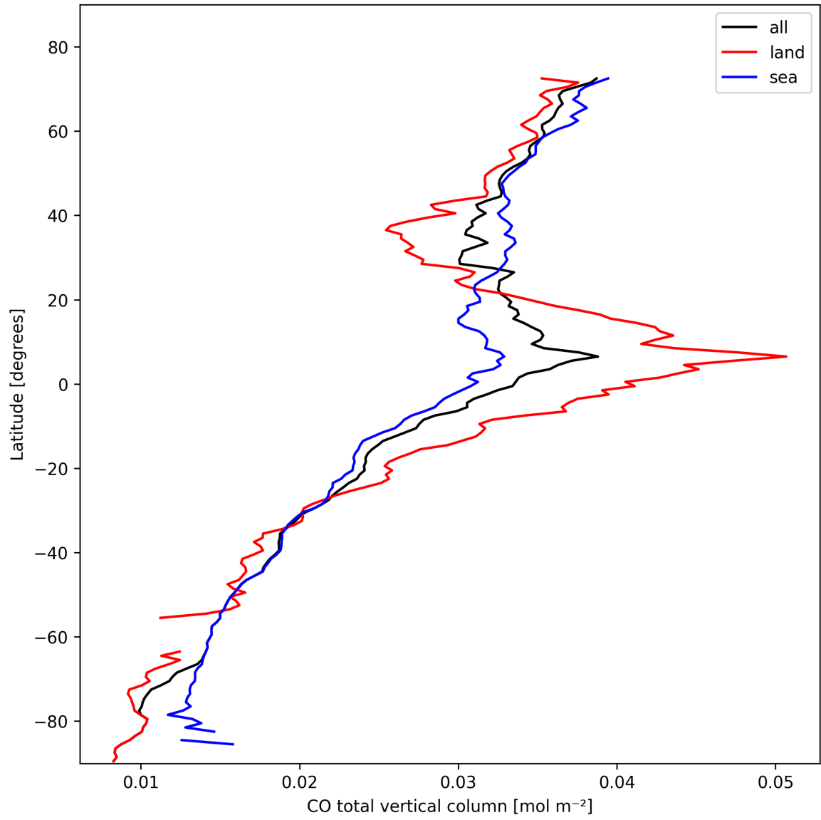
Figure 7: Zonal average of “CO total vertical column” for 2025-02-14 to 2025-02-15.
