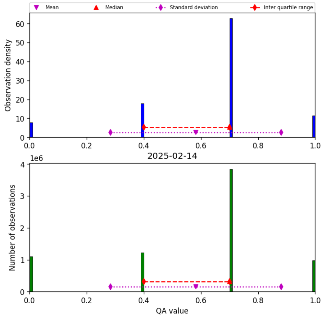
Figure 13: Histogram of “QA value” for 2025-02-14 to 2025-02-15
