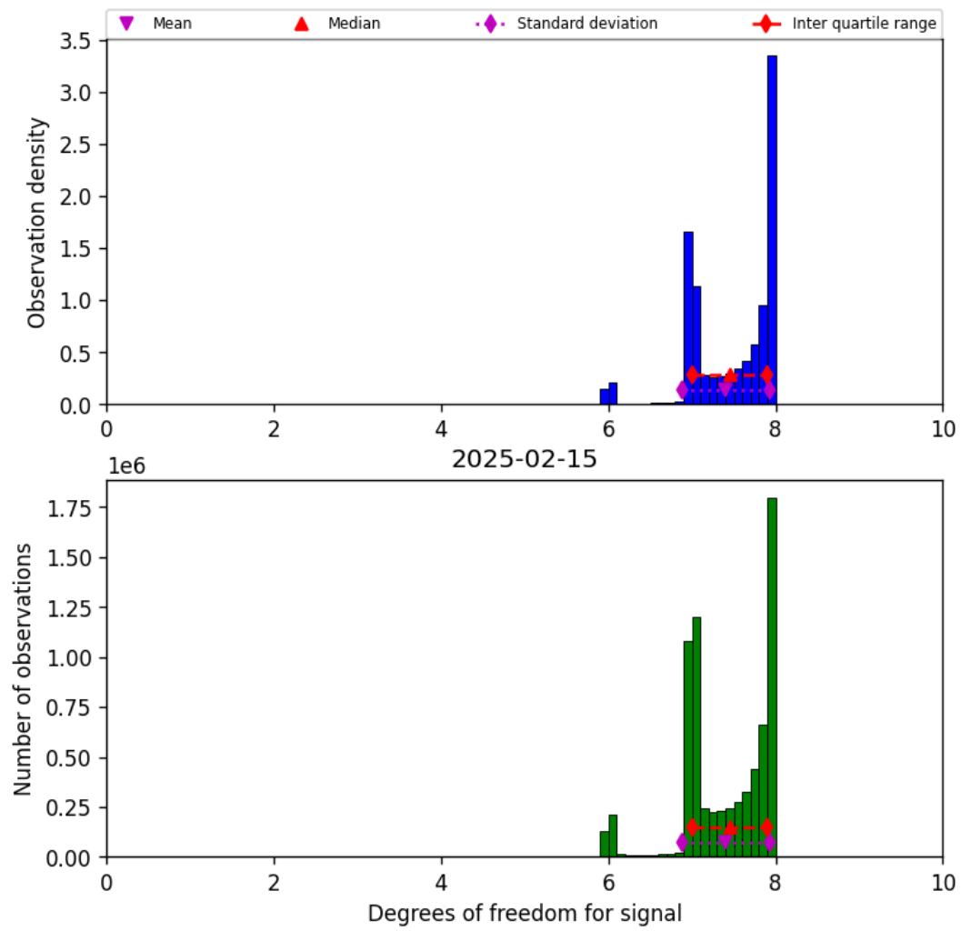
Figure 18: Histogram of “Degrees of freedom for signal” for 2025-02-15 to 2025-02-16
