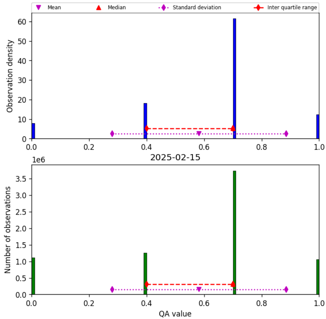
Figure 13: Histogram of “QA value” for 2025-02-15 to 2025-02-16
