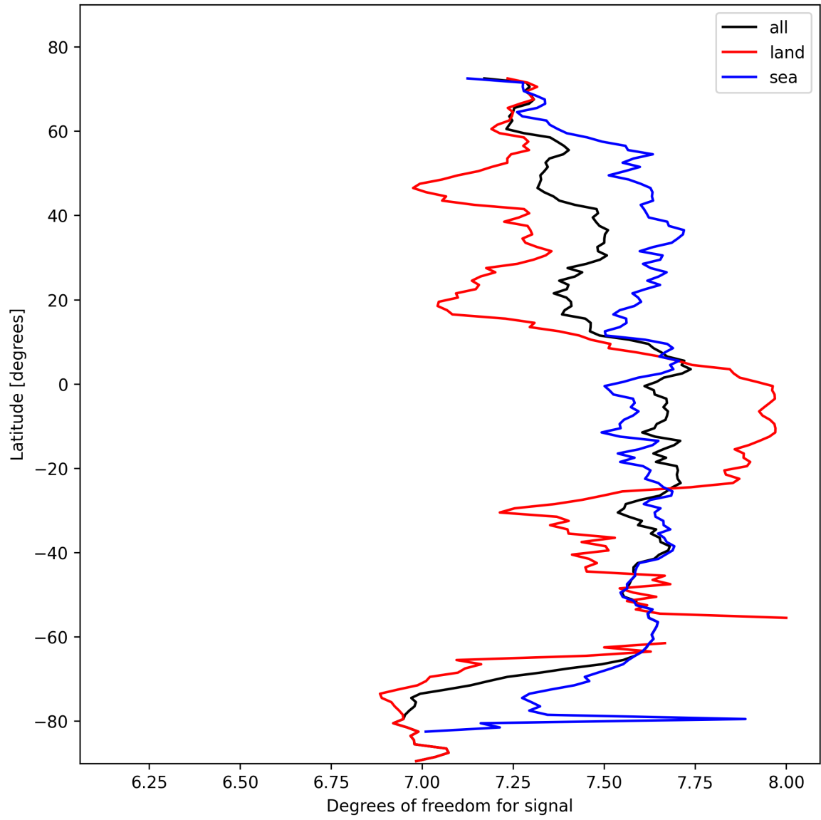
Figure 11: Zonal average of “Degrees of freedom for signal” for 2025-02-15 to 2025-02-16.
