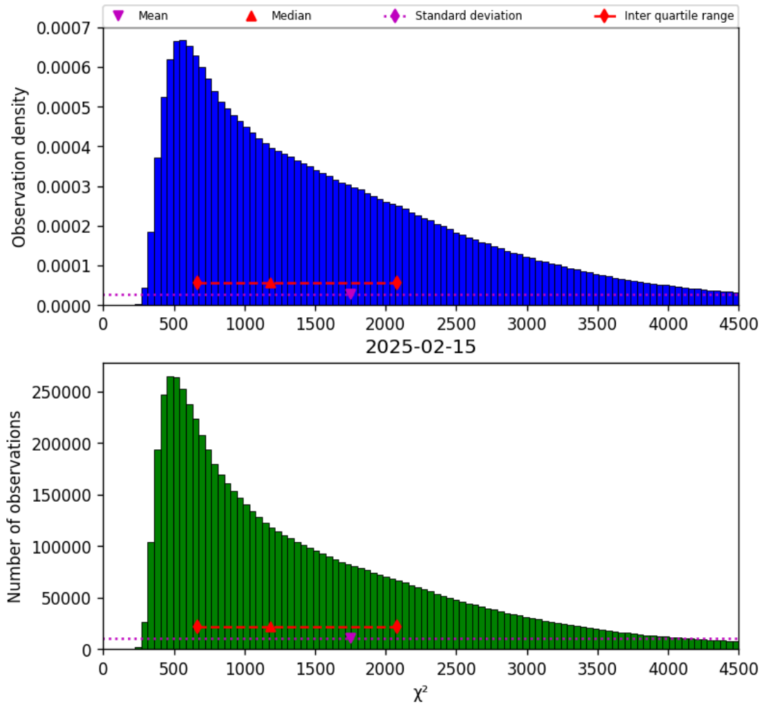
Figure 17: Histogram of “ \chi^2 ” for 2025-02-15 to 2025-02-16
