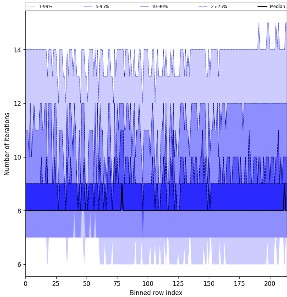
Figure 26: Along track statistics of “Number of iterations” for 2025-02-15 to 2025-02-16
