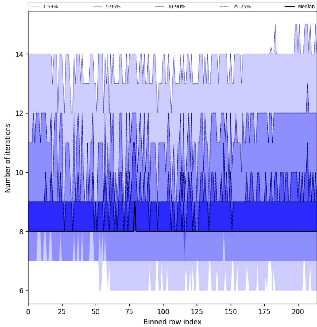
Figure 26: Along track statistics of “Number of iterations” for 2025-02-16 to 2025-02-16
