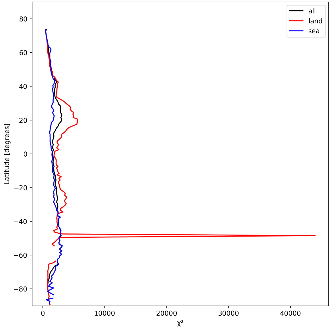
Figure 10: Zonal average of “ \chi^2 ” for 2025-02-16 to 2025-02-16.
