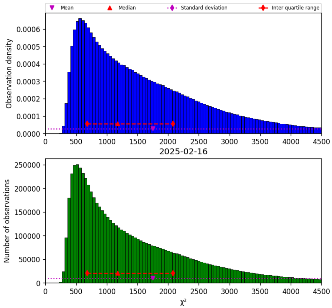
Figure 17: Histogram of " \chi^2 " for 2025-02-16 to 2025-02-16
