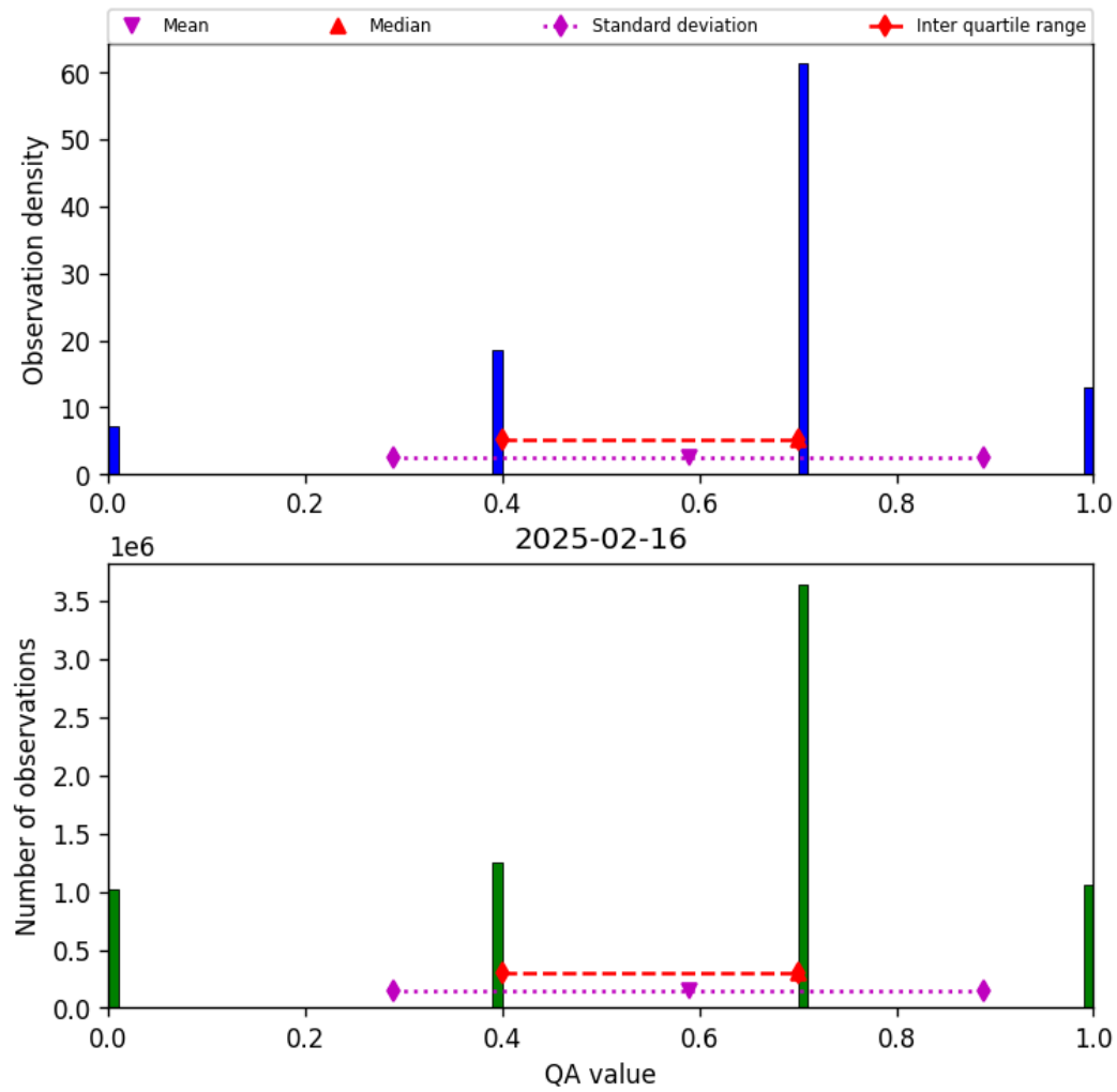
Figure 13: Histogram of “QA value” for 2025-02-16 to 2025-02-16
