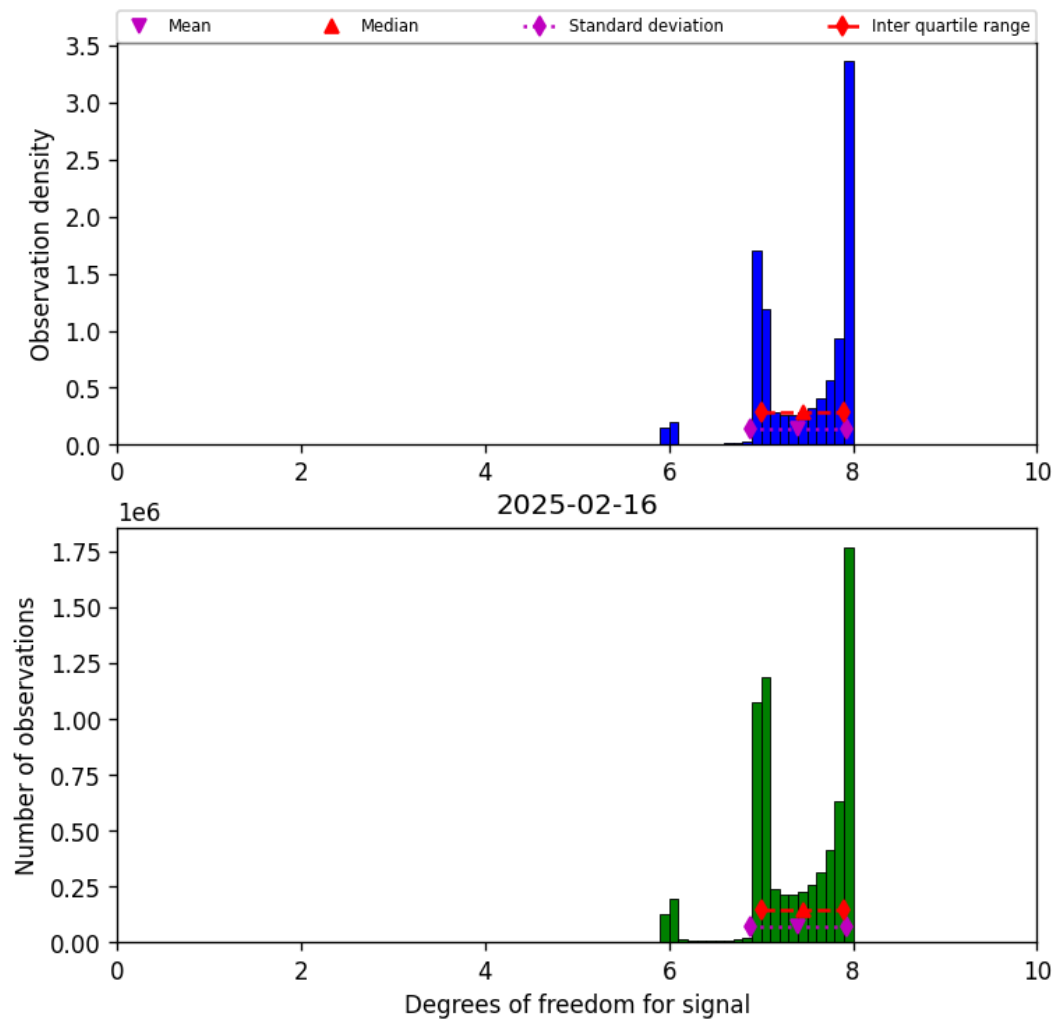
Figure 18: Histogram of “Degrees of freedom for signal” for 2025-02-16 to 2025-02-16
