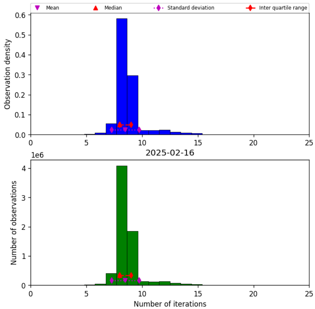
Figure 19: Histogram of “Number of iterations” for 2025-02-16 to 2025-02-16
