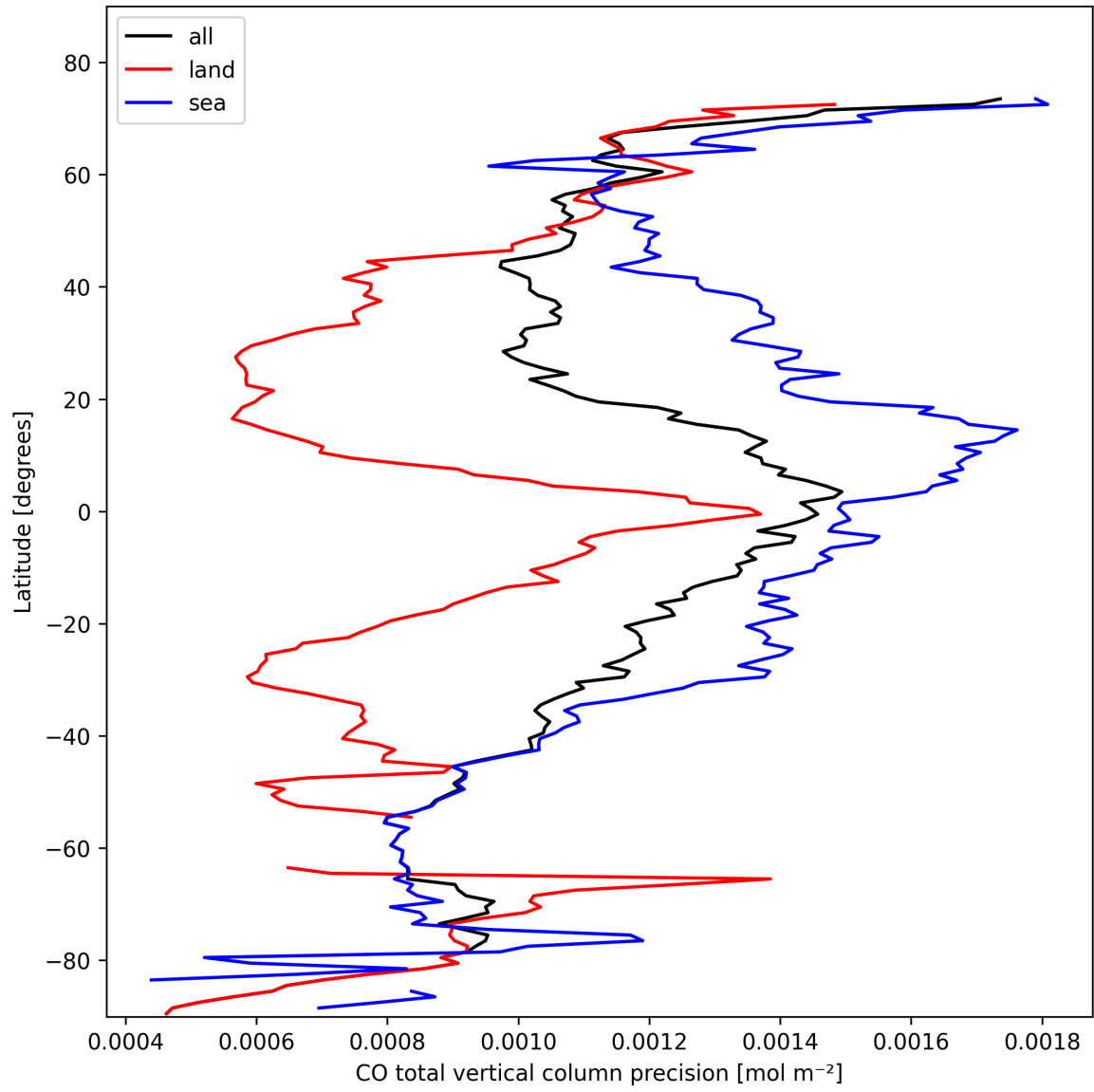
Figure 8: Zonal average of “CO total vertical column precision” for 2025-02-16 to 2025-02-16.
