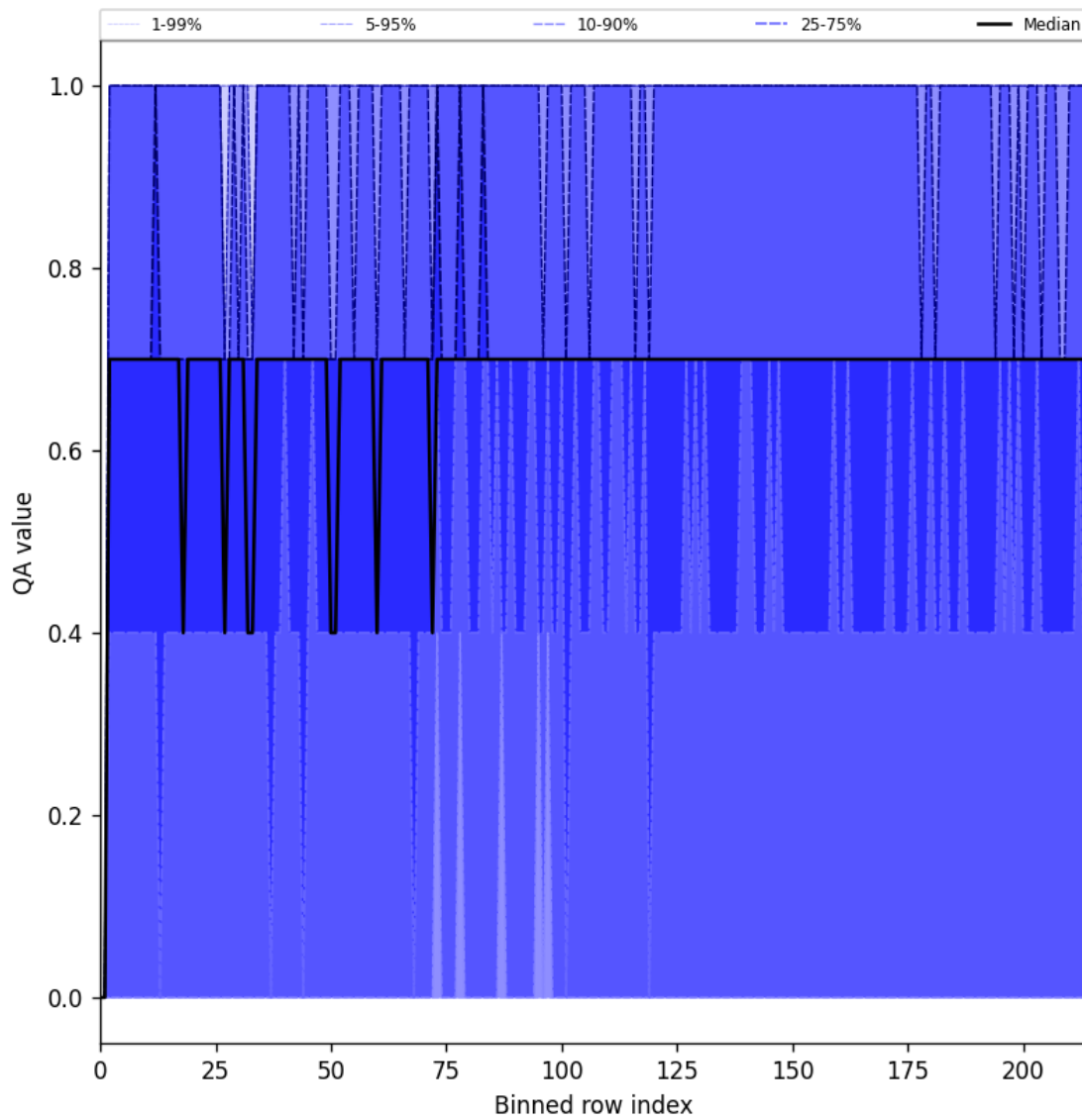
Figure 20: Along track statistics of “QA value” for 2025-02-16 to 2025-02-16
