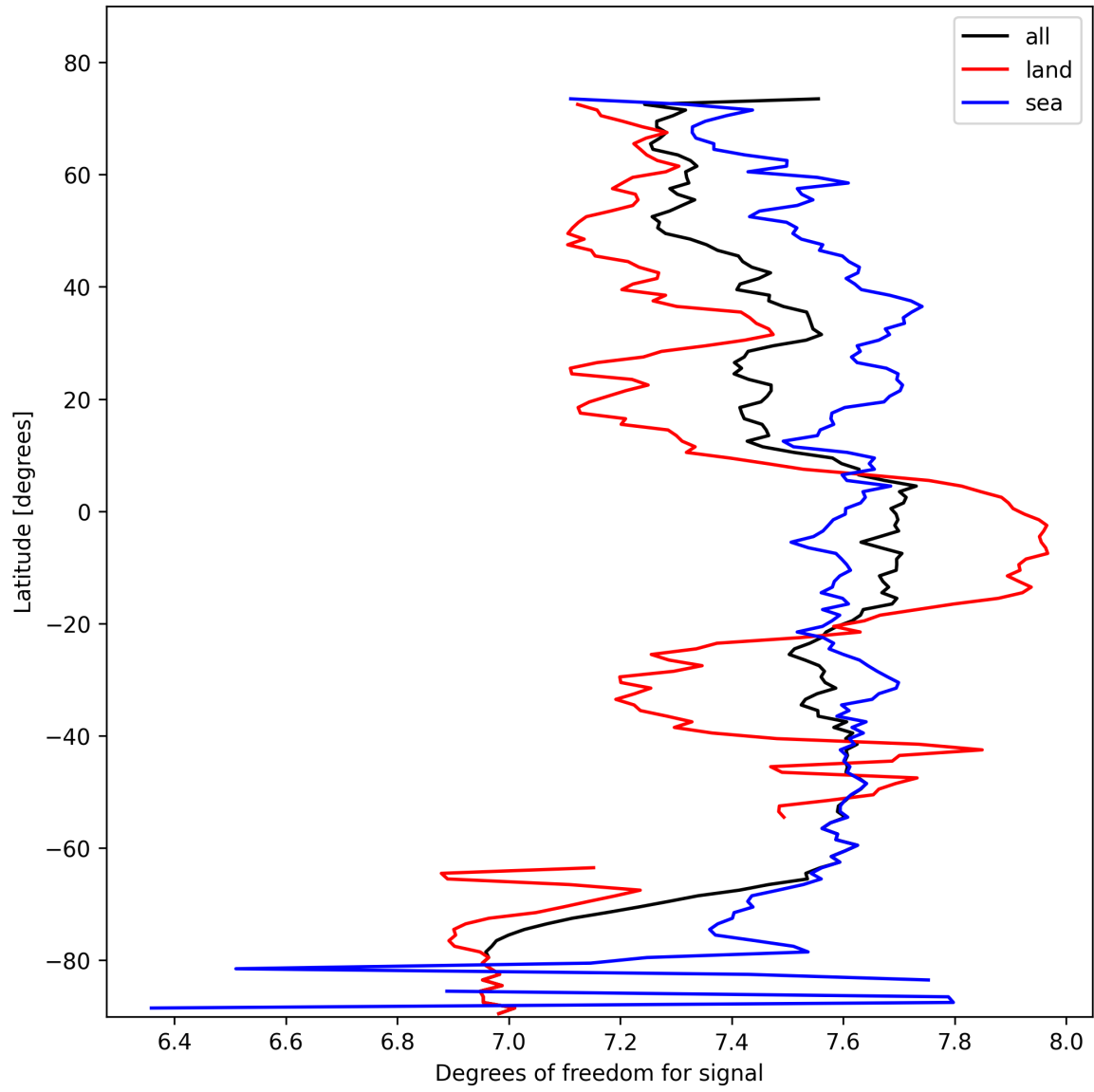
Figure 11: Zonal average of “Degrees of freedom for signal” for 2025-02-16 to 2025-02-16.
