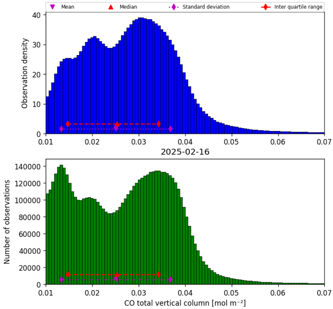
Figure 14: Histogram of “CO total vertical column” for 2025-02-16 to 2025-02-16
