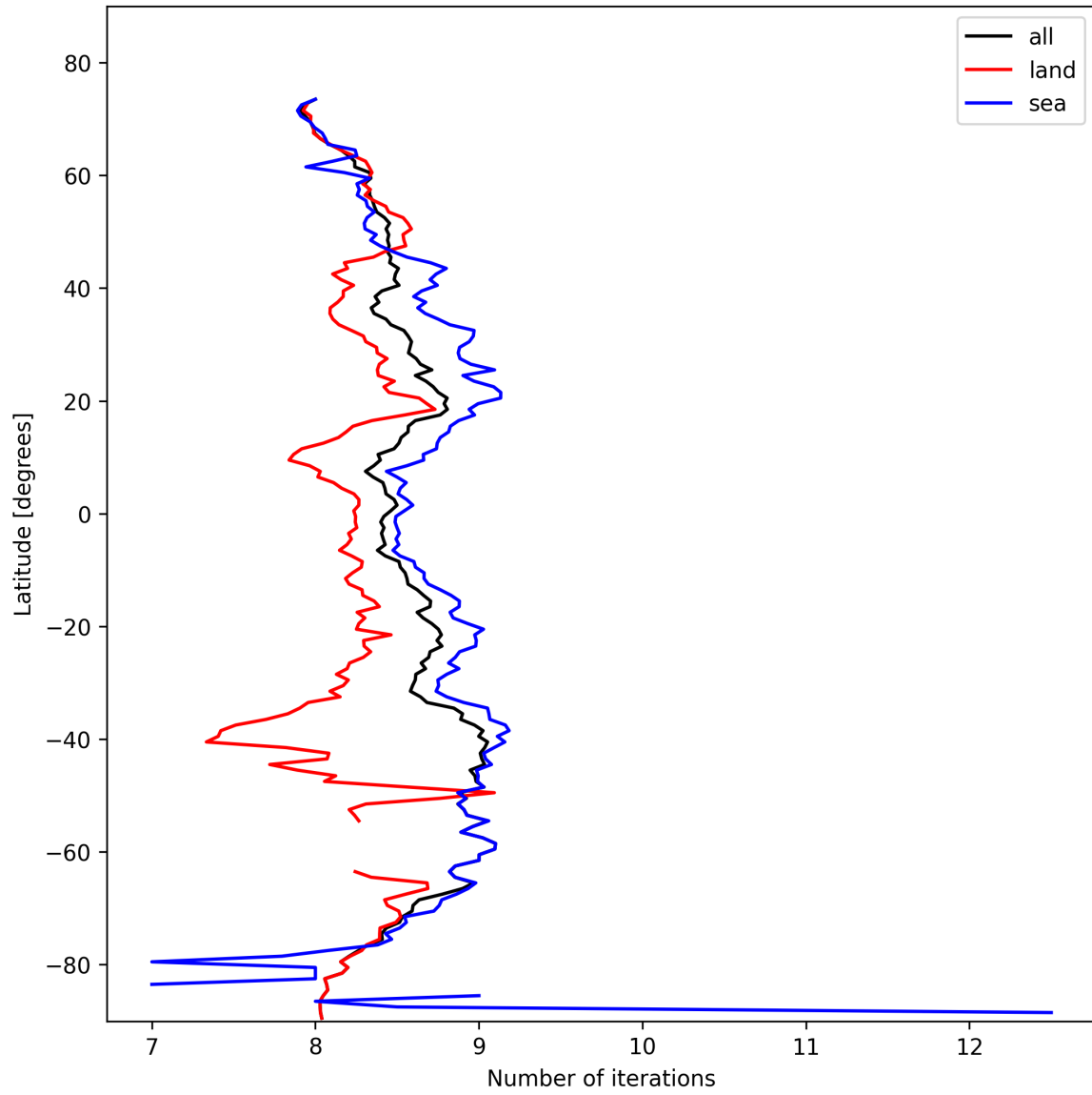
Figure 12: Zonal average of “Number of iterations” for 2025-02-16 to 2025-02-16.
