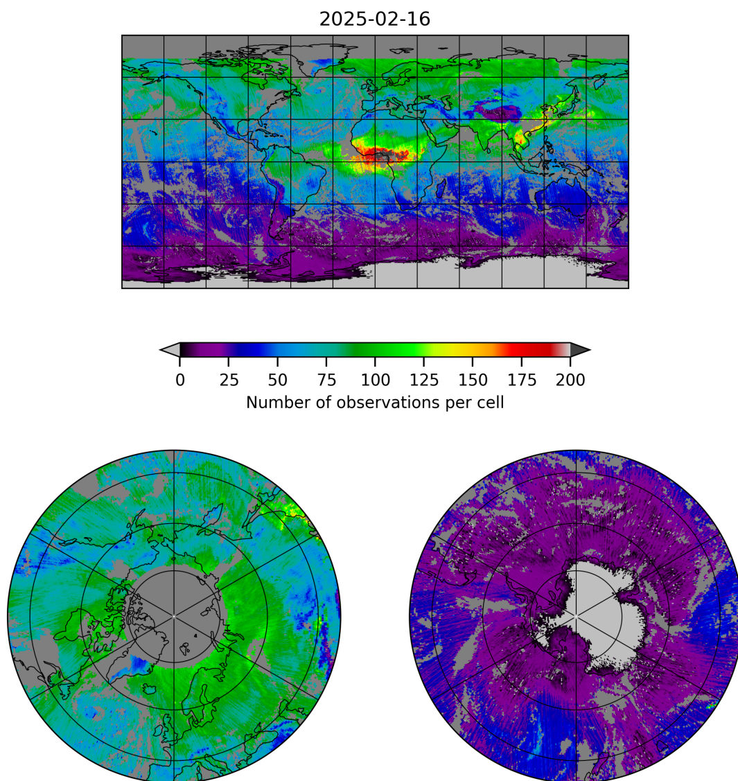
Figure 5: Map of the number of observations for 2025-02-16 to 2025-02-16
