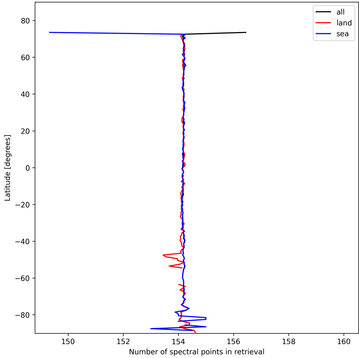
Figure 9: Zonal average of “Number of spectral points in retrieval” for 2025-02-16 to 2025-02-16.
