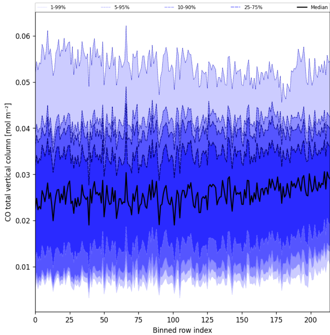
Figure 21: Along track statistics of “CO total vertical column” for 2025-02-16 to 2025-02-16
