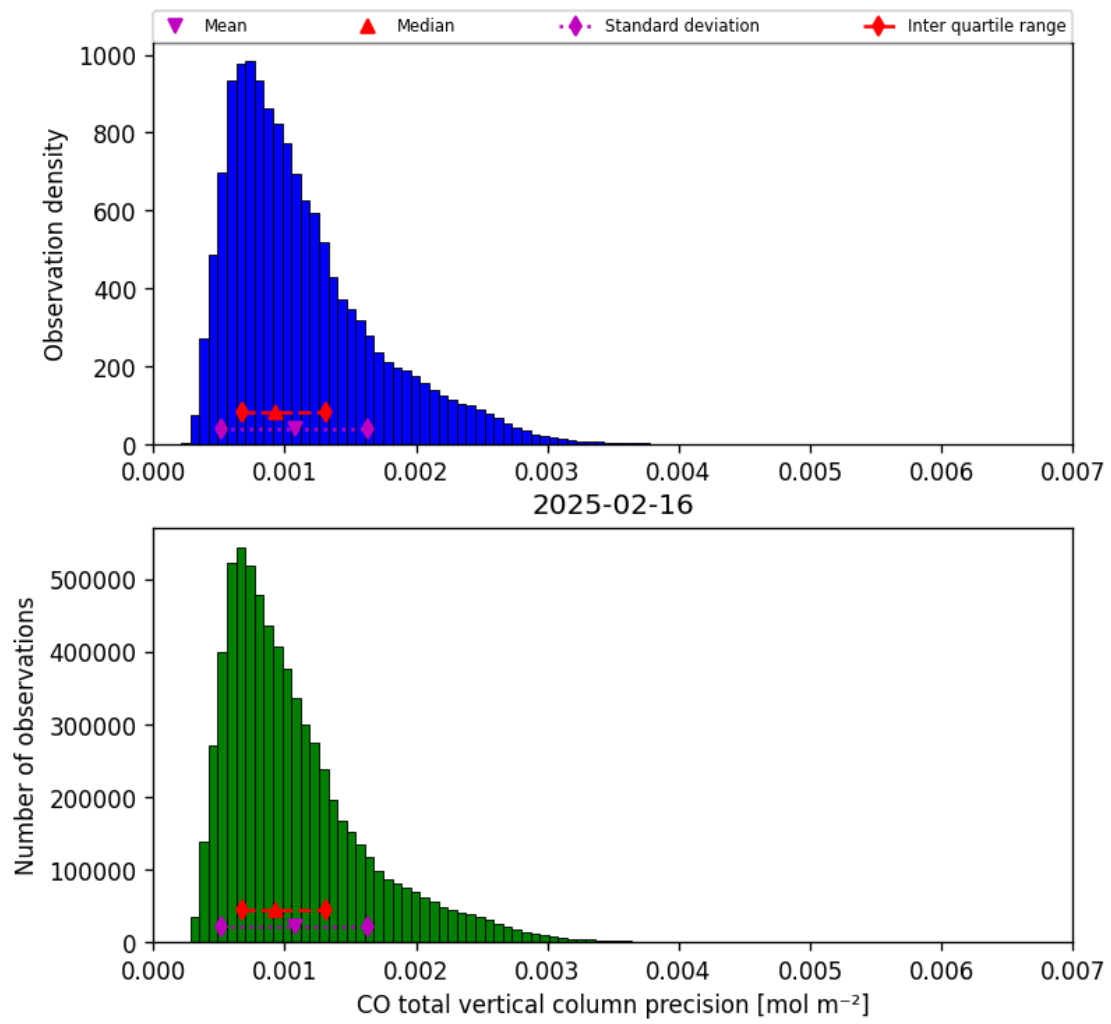
Figure 15: Histogram of “CO total vertical column precision” for 2025-02-16 to 2025-02-16
