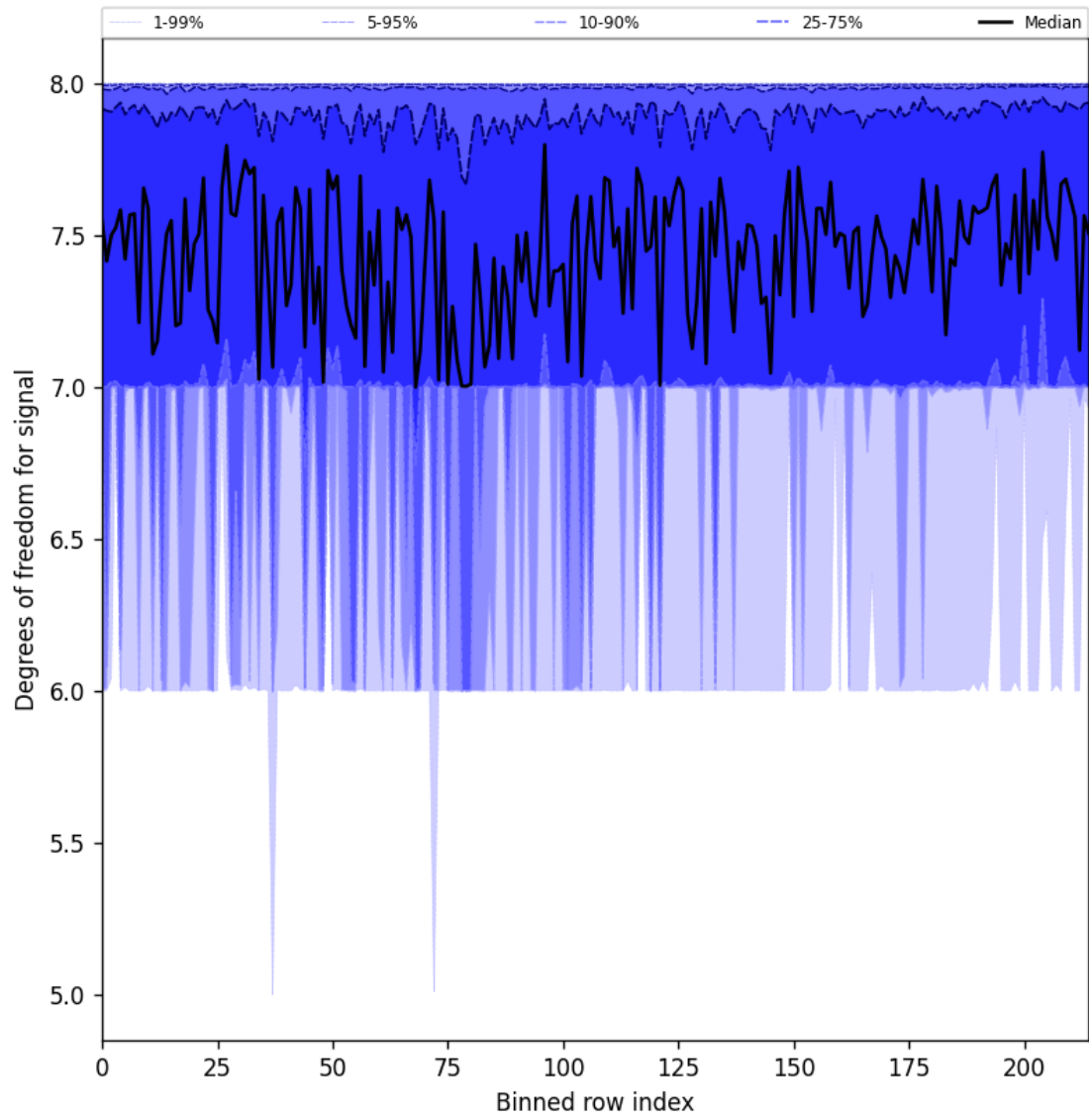
Figure 25: Along track statistics of “Degrees of freedom for signal” for 2025-02-16 to 2025-02-16
