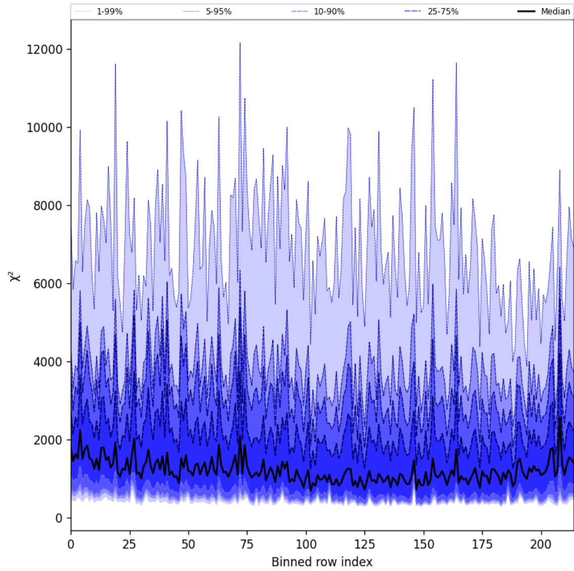
Figure 24: Along track statistics of “ \chi^2 ” for 2025-02-16 to 2025-02-16
