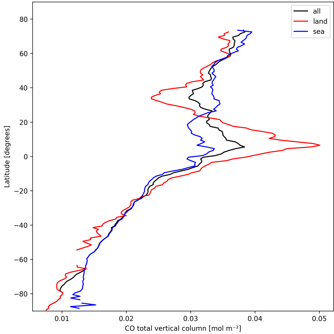
Figure 7: Zonal average of “CO total vertical column” for 2025-02-16 to 2025-02-16.
