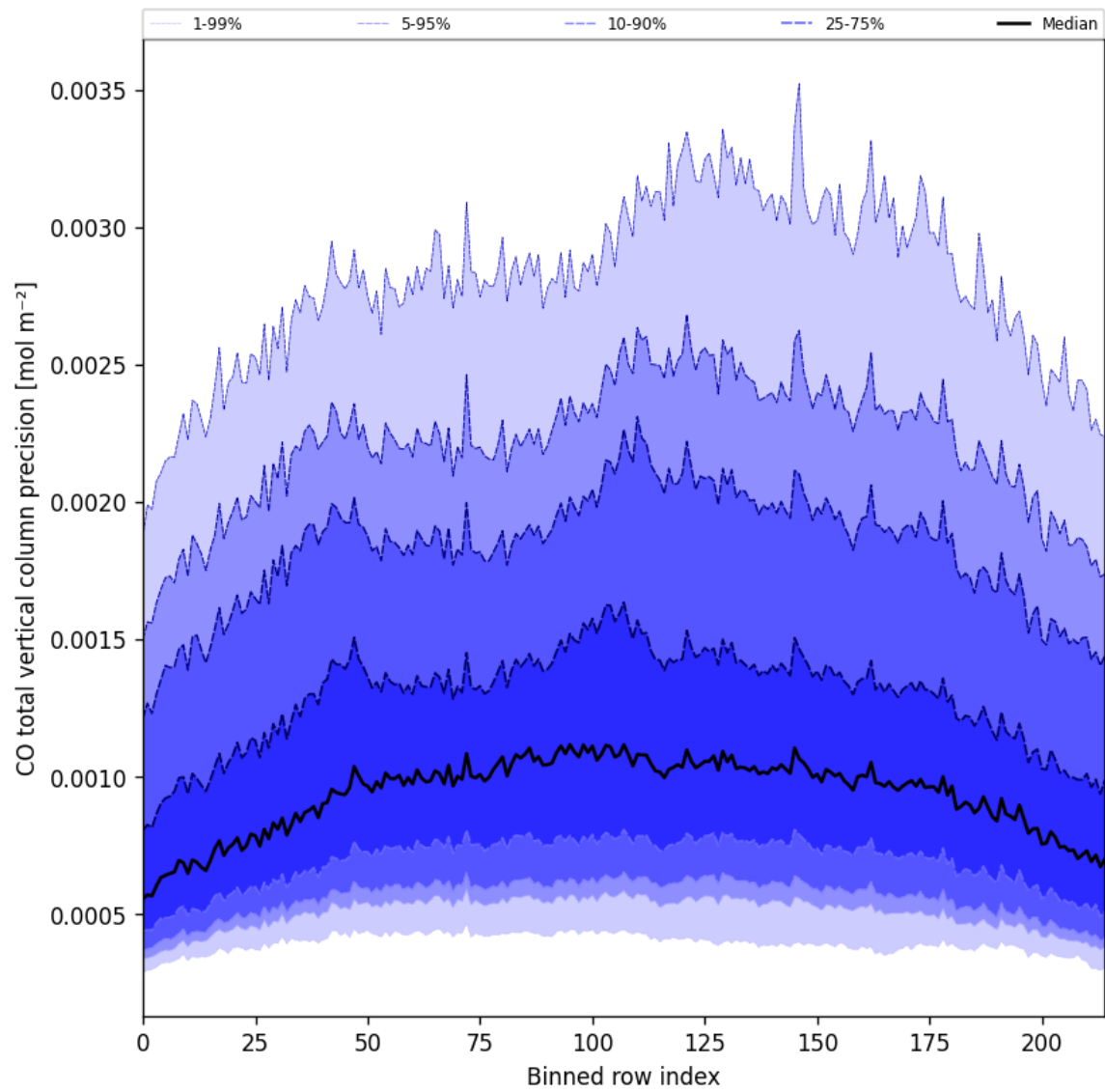
Figure 22: Along track statistics of “CO total vertical column precision” for 2025-02-16 to 2025-02-16
