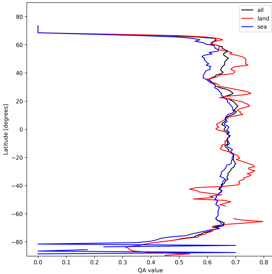
Figure 6: Zonal average of “QA value” for 2025-02-16 to 2025-02-16.
