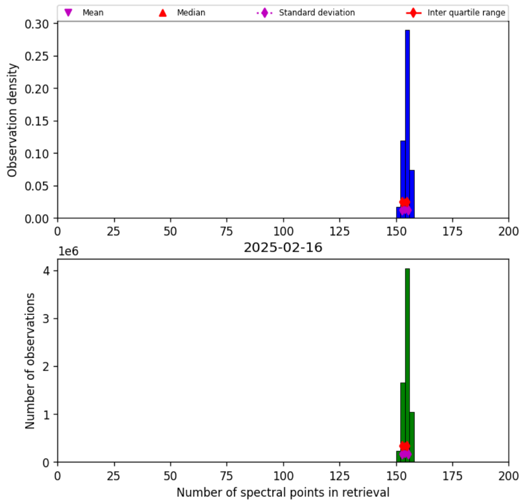
Figure 16: Histogram of “Number of spectral points in retrieval” for 2025-02-16 to 2025-02-16
