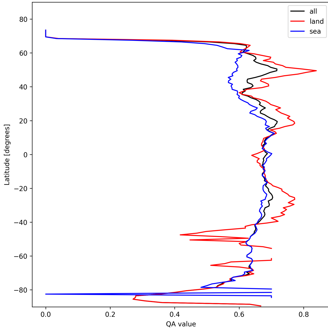
Figure 6: Zonal average of “QA value” for 2025-02-17 to 2025-02-18.
