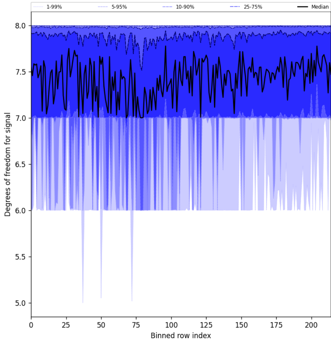
Figure 25: Along track statistics of “Degrees of freedom for signal” for 2025-02-17 to 2025-02-18
