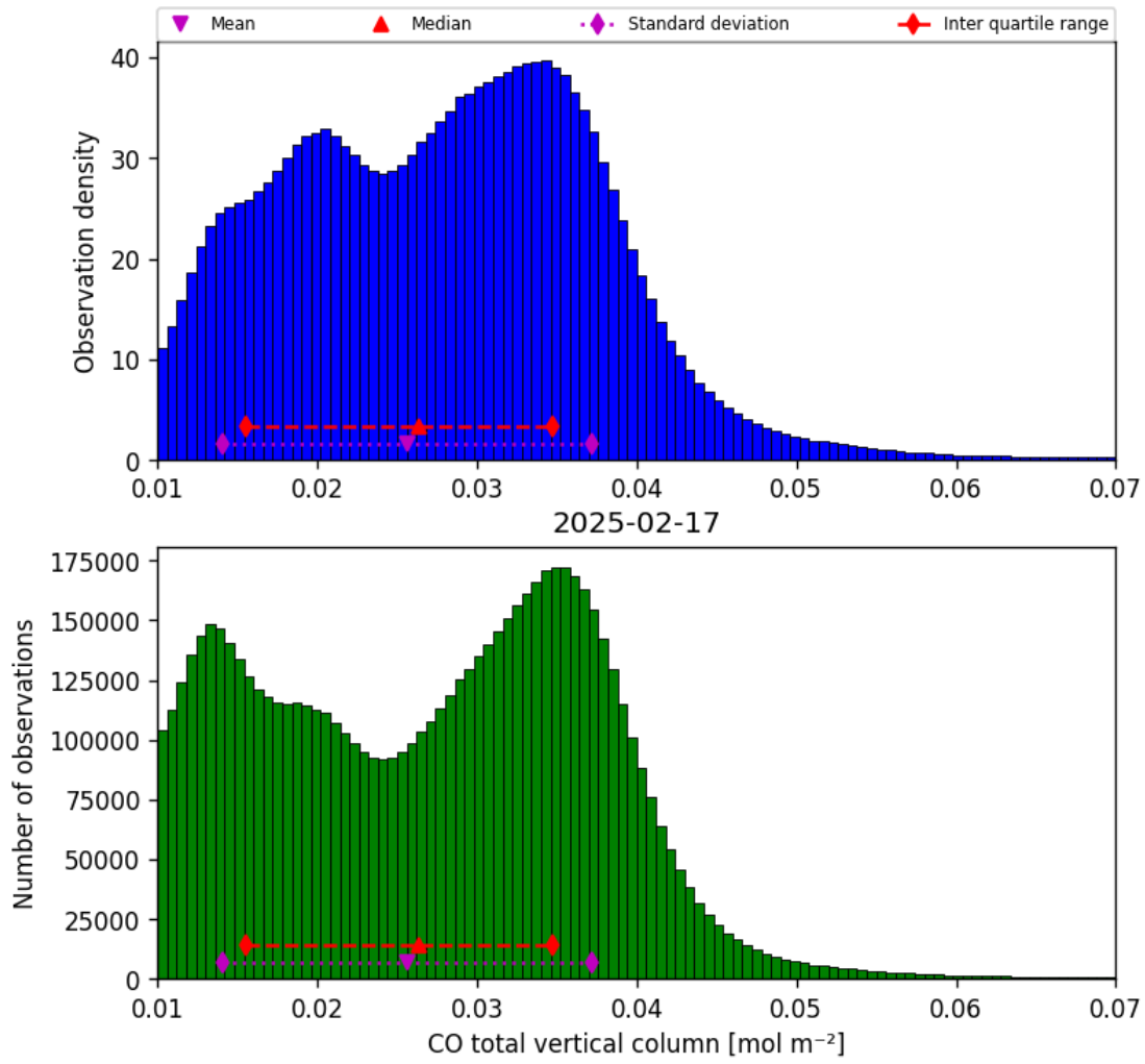
Figure 14: Histogram of “CO total vertical column” for 2025-02-17 to 2025-02-18
