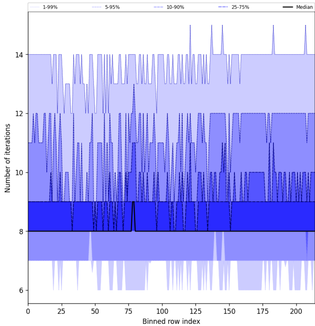
Figure 26: Along track statistics of “Number of iterations” for 2025-02-17 to 2025-02-18
