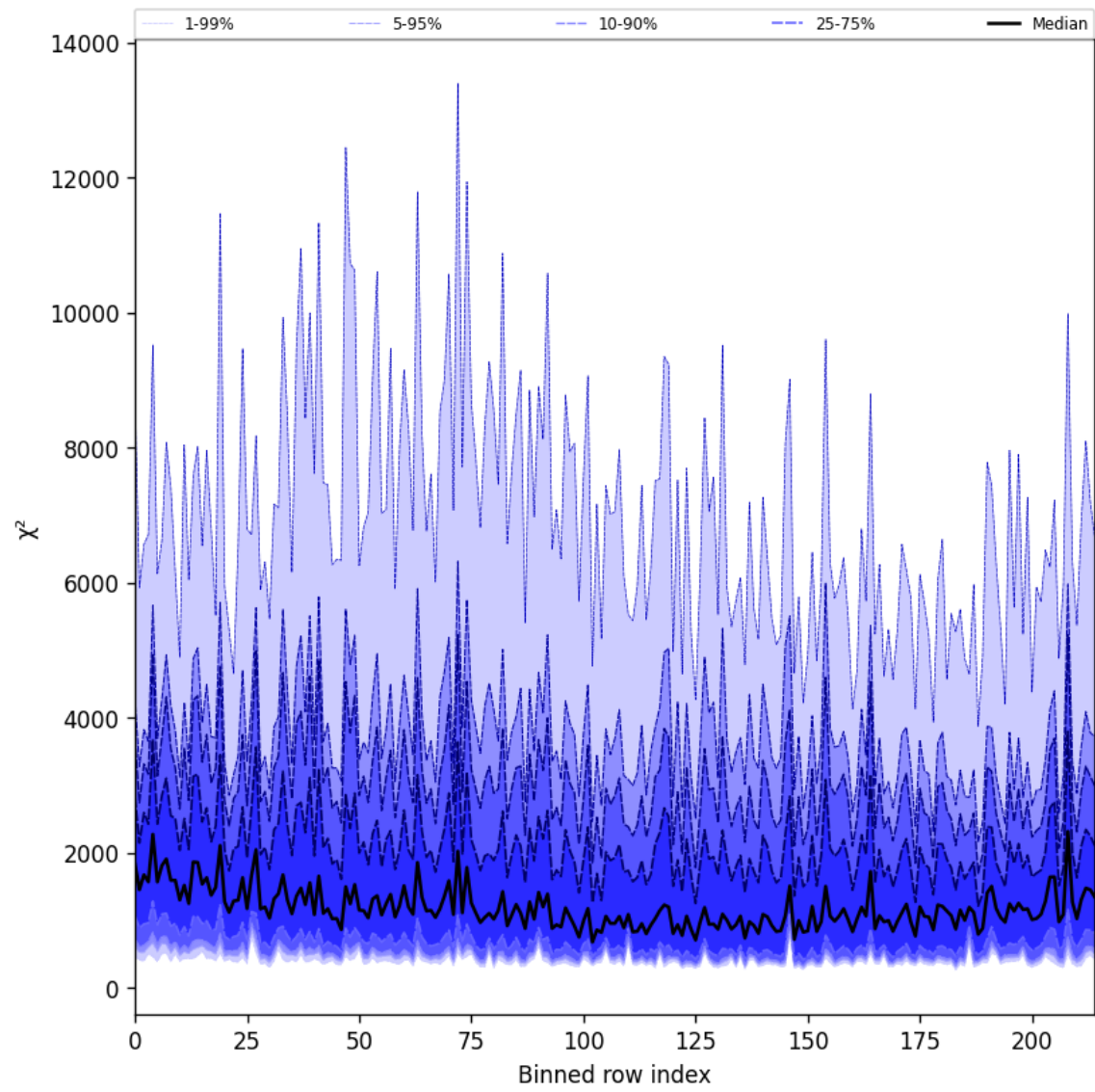
Figure 24: Along track statistics of “ \chi^2 ” for 2025-02-17 to 2025-02-18
