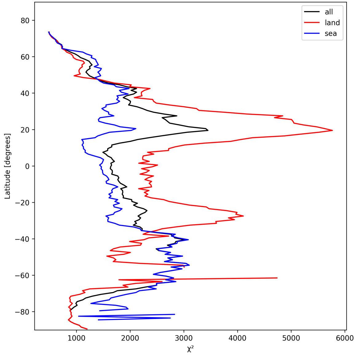
Figure 10: Zonal average of “ \chi^2 ” for 2025-02-17 to 2025-02-18.
