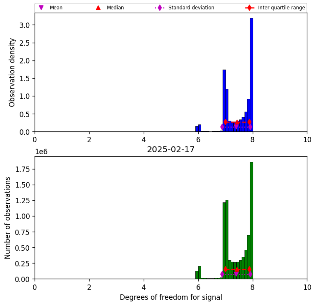
Figure 18: Histogram of “Degrees of freedom for signal” for 2025-02-17 to 2025-02-18
