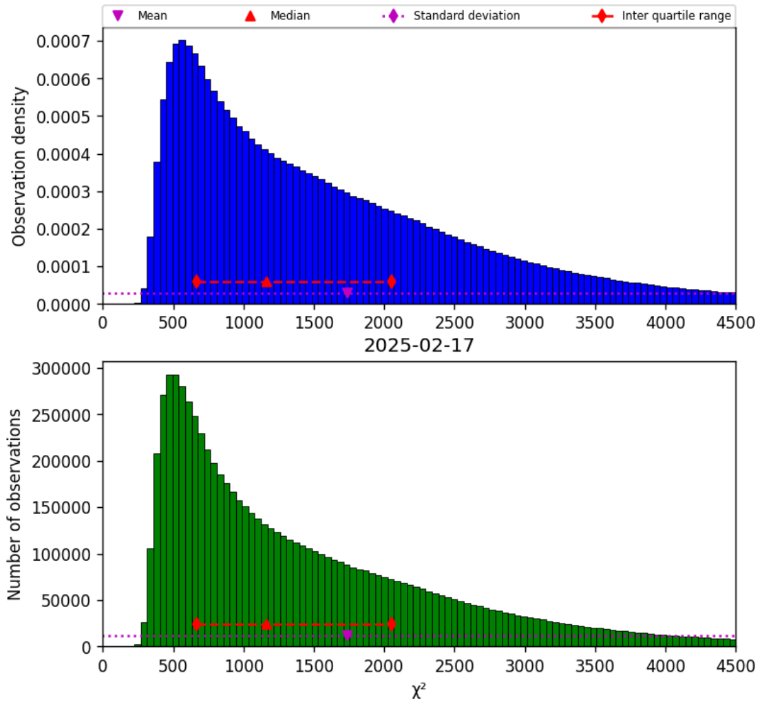
Figure 17: Histogram of “ \chi^2 ” for 2025-02-17 to 2025-02-18
