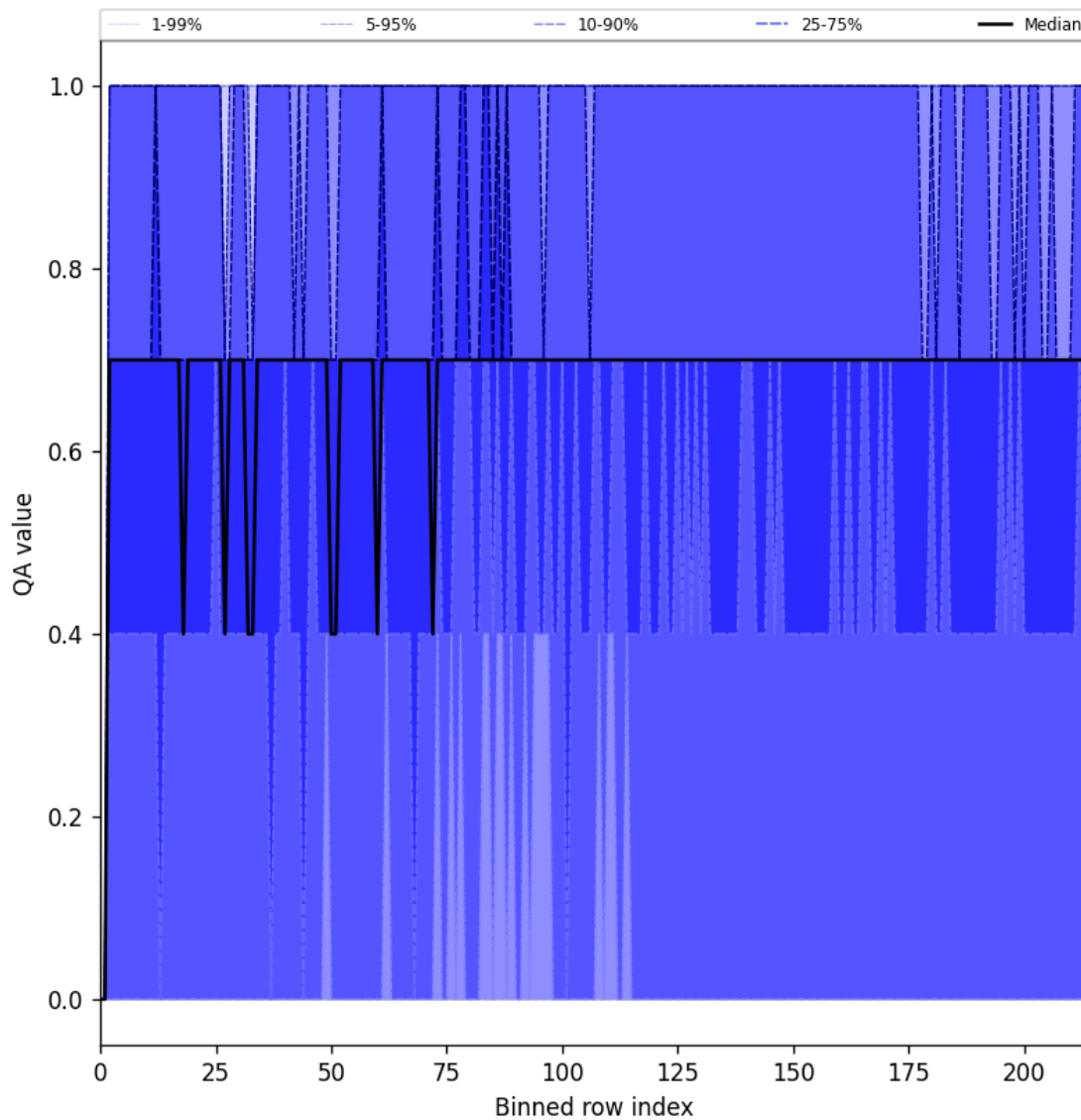
Figure 20: Along track statistics of “QA value” for 2025-02-17 to 2025-02-18
