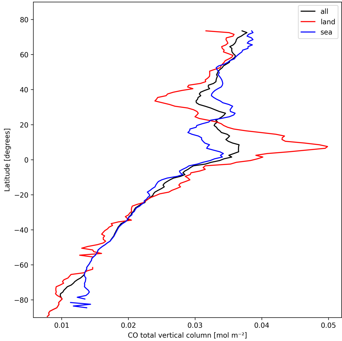
Figure 7: Zonal average of “CO total vertical column” for 2025-02-17 to 2025-02-18.
