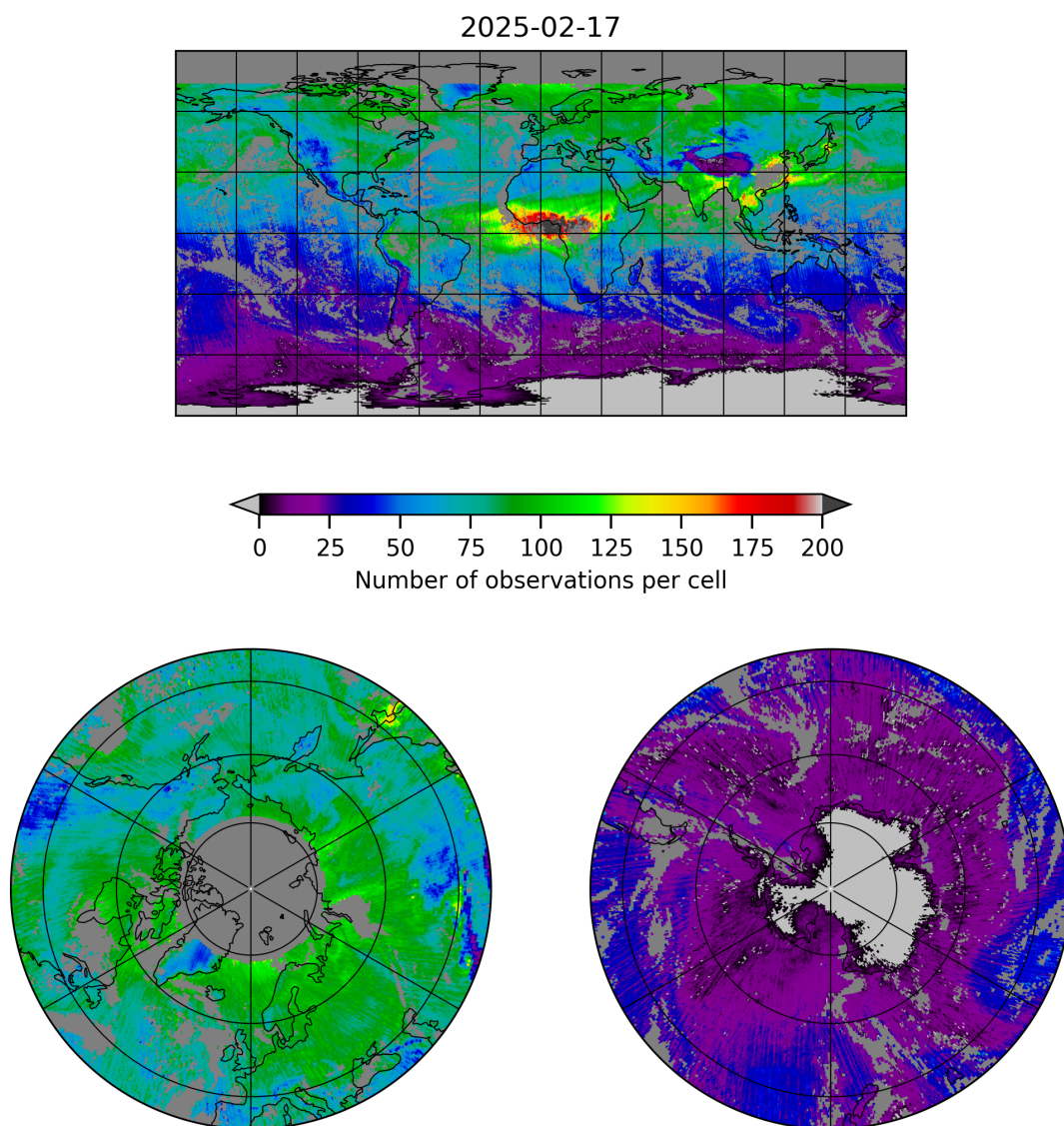
Figure 5: Map of the number of observations for 2025-02-17 to 2025-02-18
