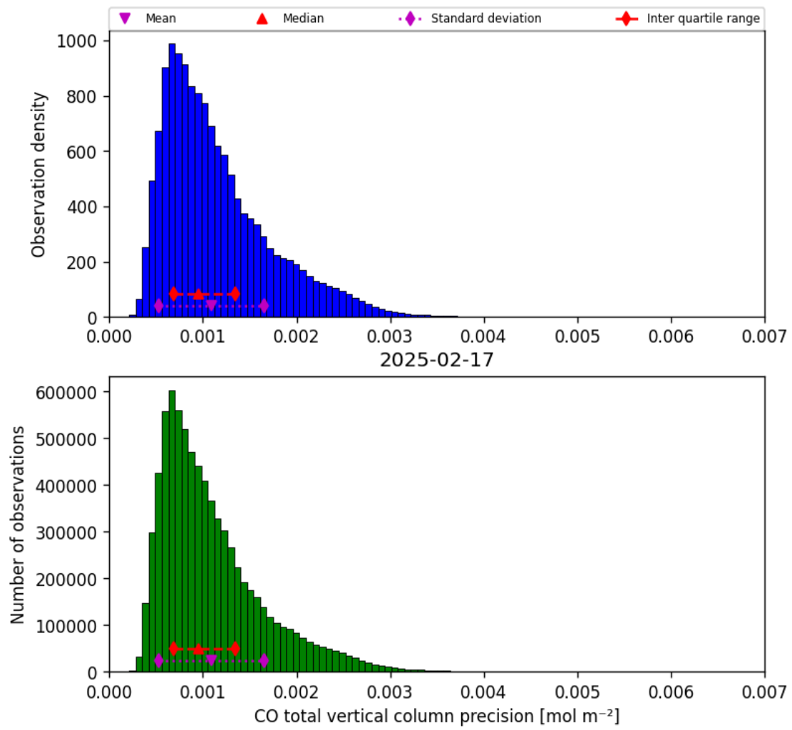
Figure 15: Histogram of “CO total vertical column precision” for 2025-02-17 to 2025-02-18
