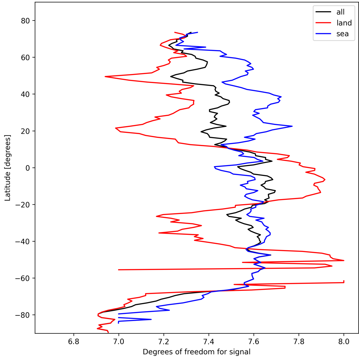
Figure 11: Zonal average of “Degrees of freedom for signal” for 2025-02-17 to 2025-02-18.
