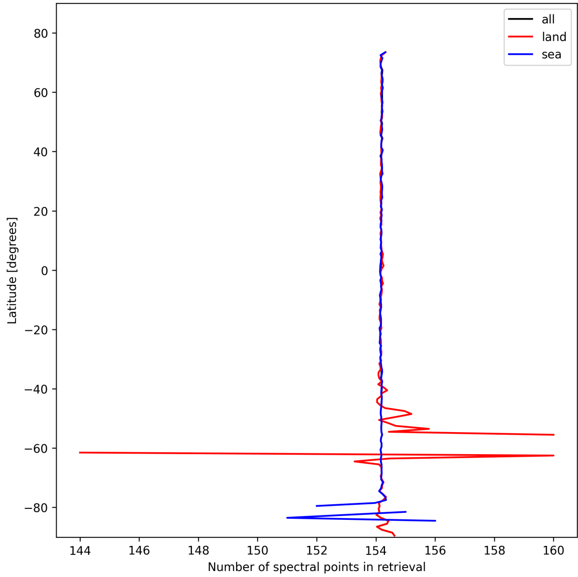
Figure 9: Zonal average of “Number of spectral points in retrieval” for 2025-02-17 to 2025-02-18.
