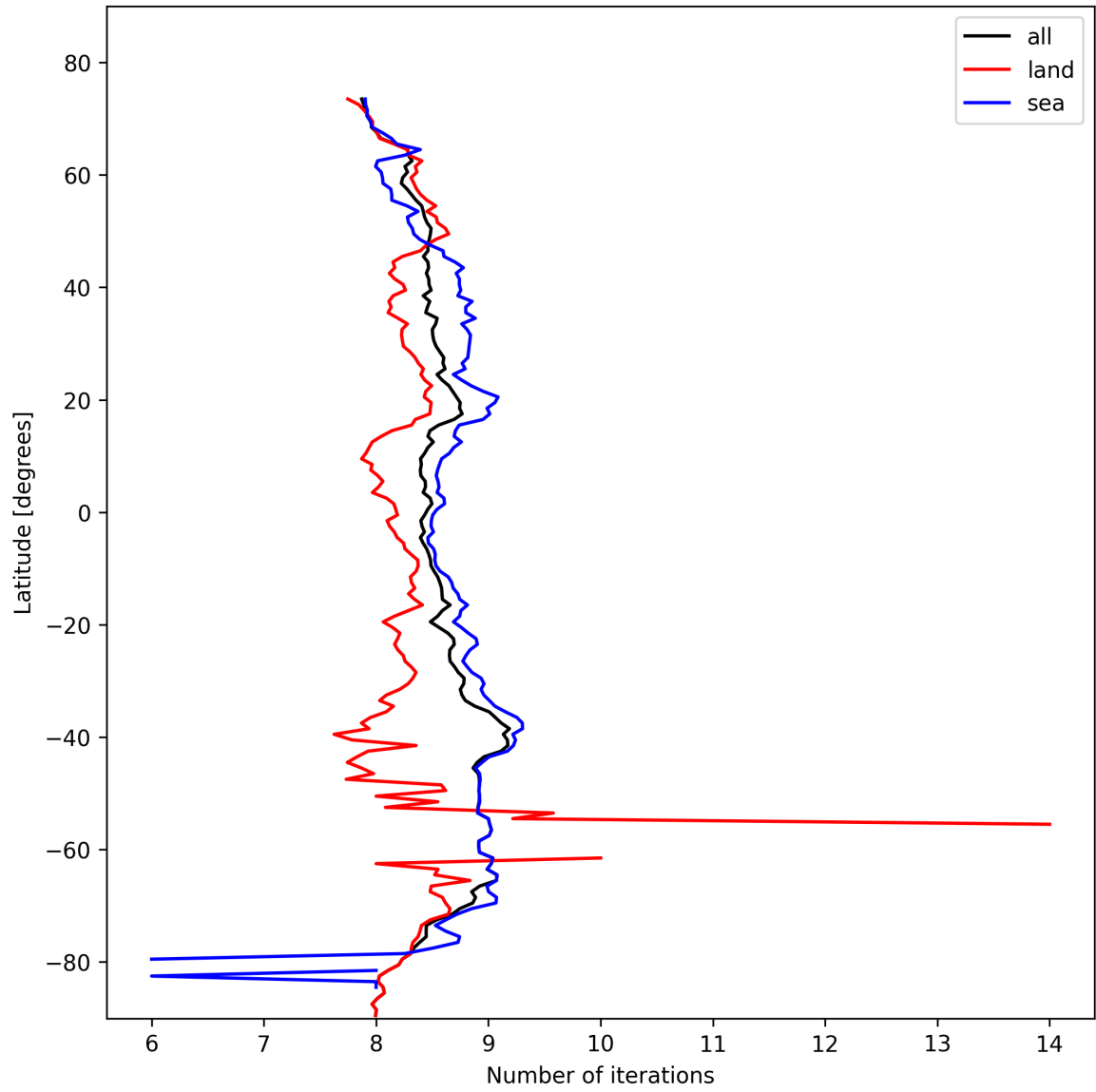
Figure 12: Zonal average of “Number of iterations” for 2025-02-17 to 2025-02-18.
