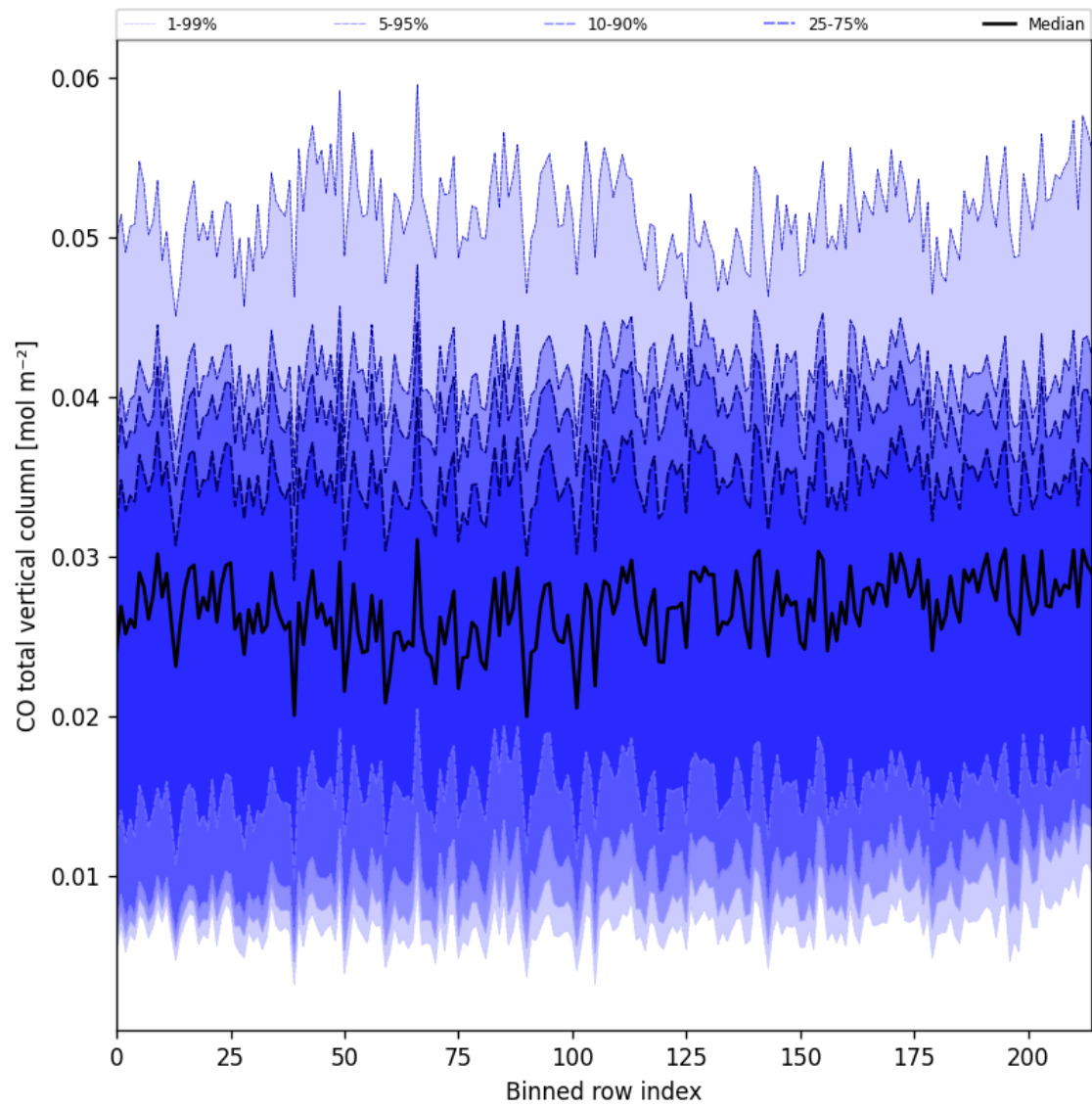
Figure 21: Along track statistics of "CO total vertical column" for 2025-02-17 to 2025-02-18
