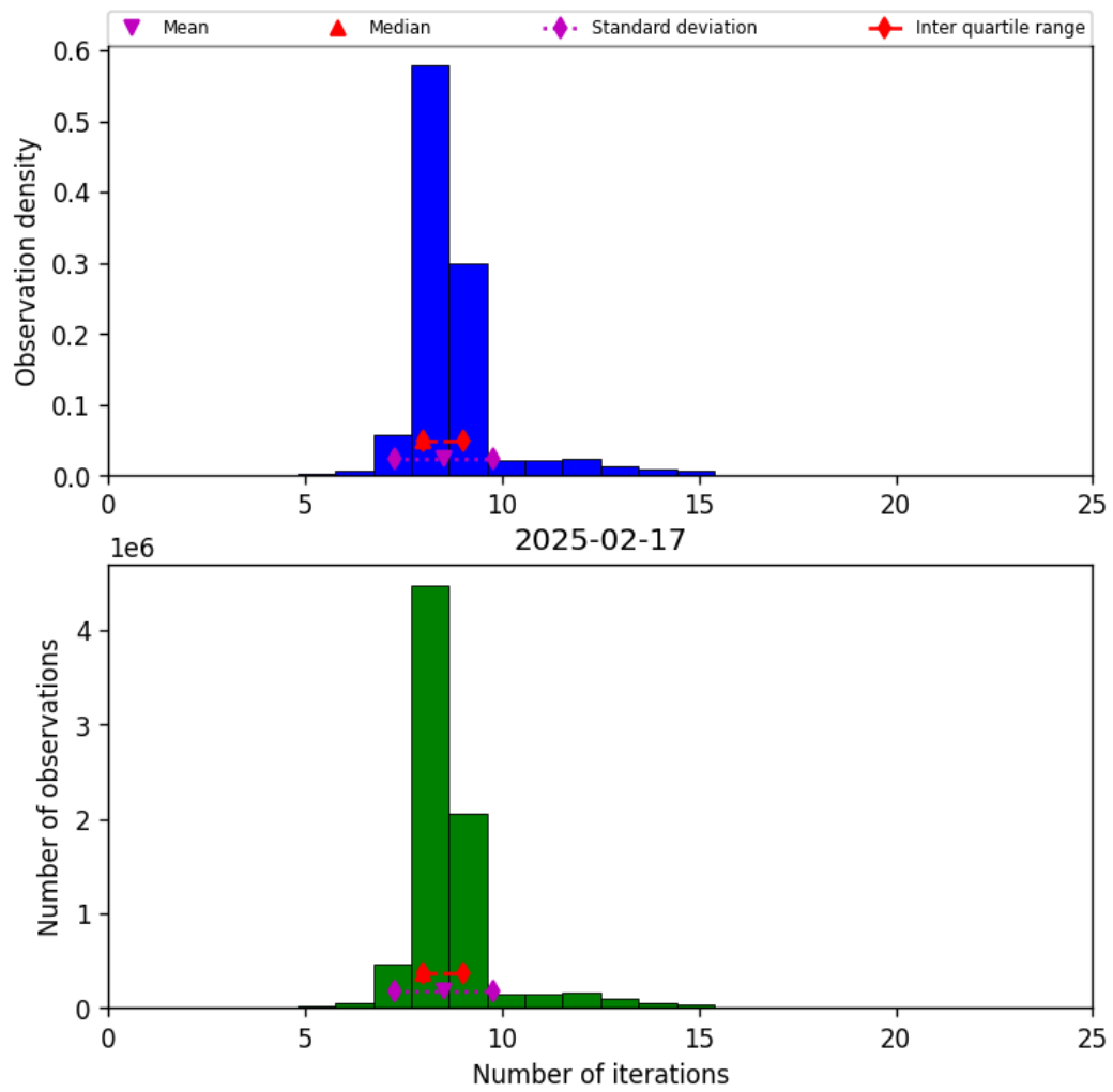
Figure 19: Histogram of “Number of iterations” for 2025-02-17 to 2025-02-18
