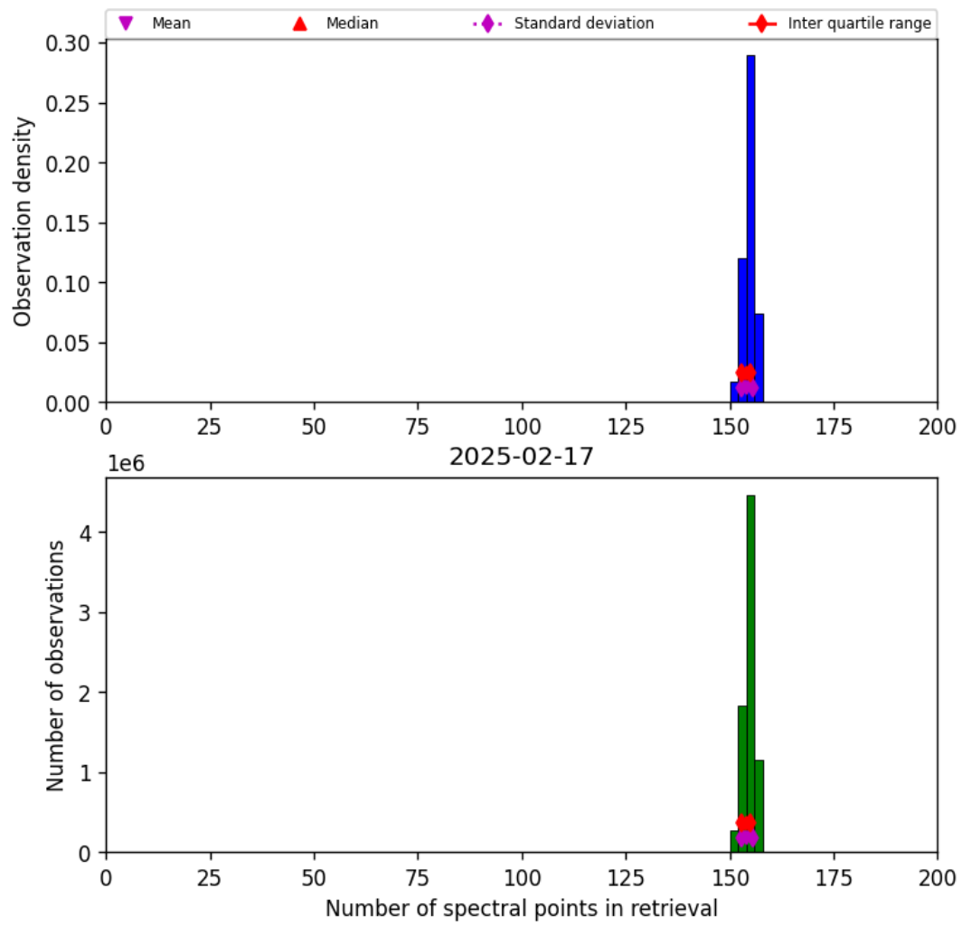
Figure 16: Histogram of “Number of spectral points in retrieval” for 2025-02-17 to 2025-02-18
