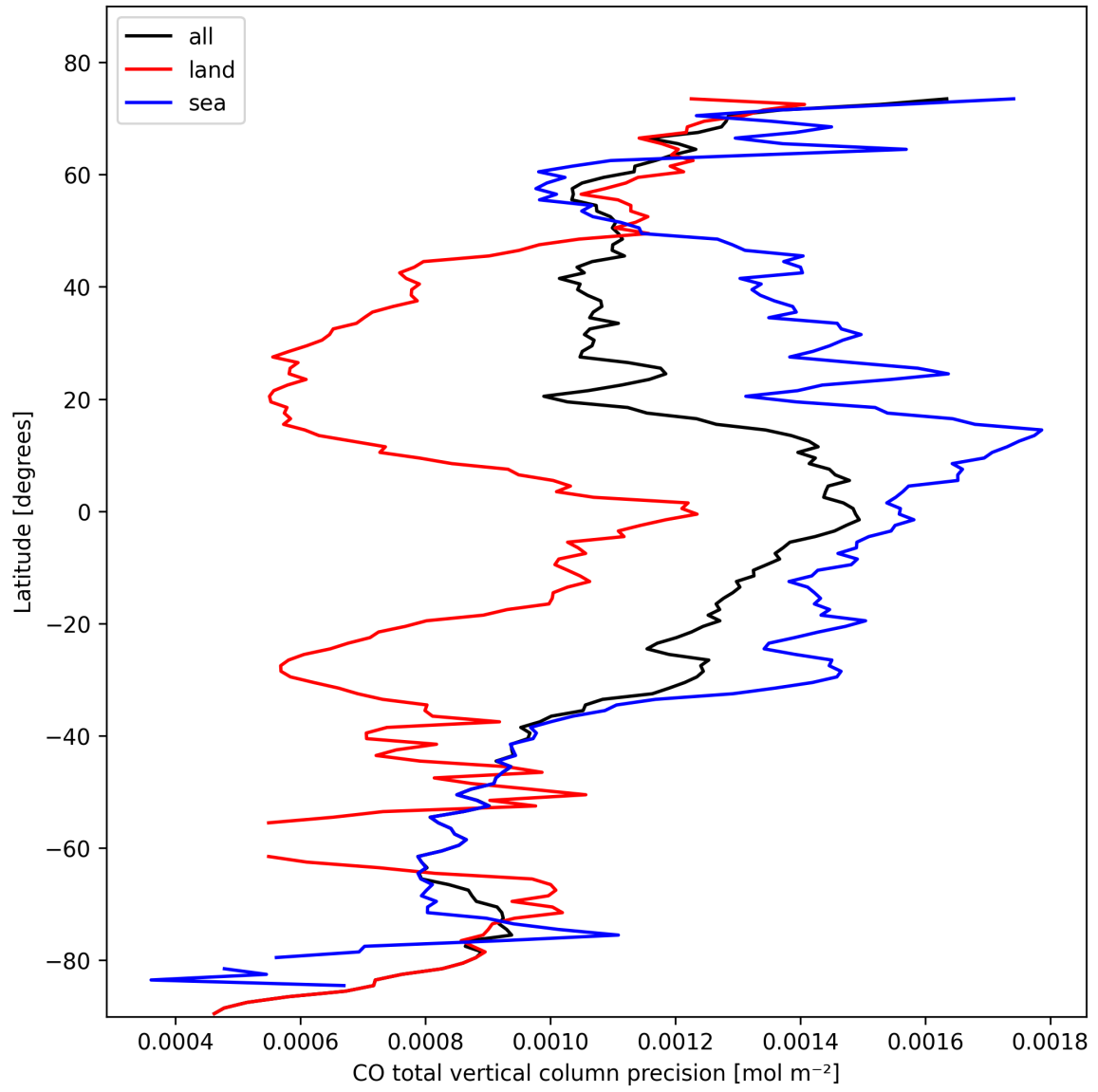
Figure 8: Zonal average of “CO total vertical column precision” for 2025-02-17 to 2025-02-18.
