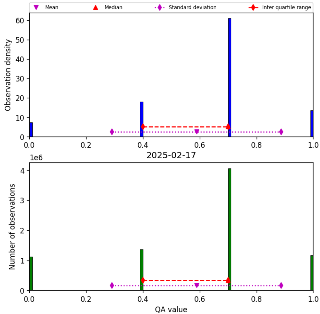
Figure 13: Histogram of “QA value” for 2025-02-17 to 2025-02-18
