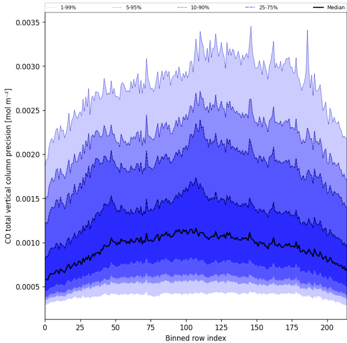
Figure 22: Along track statistics of “CO total vertical column precision” for 2025-02-17 to 2025-02-18
