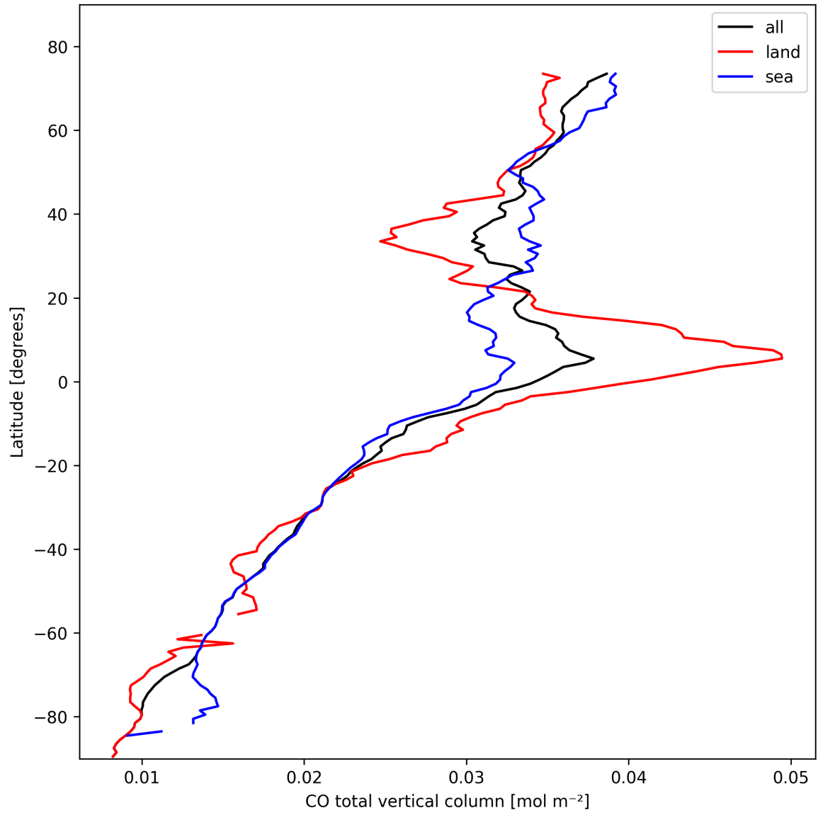
Figure 7: Zonal average of “CO total vertical column” for 2025-02-18 to 2025-02-19.
