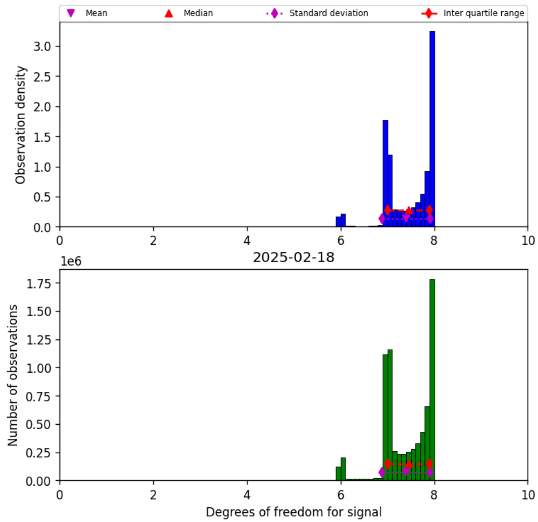
Figure 18: Histogram of “Degrees of freedom for signal” for 2025-02-18 to 2025-02-19
