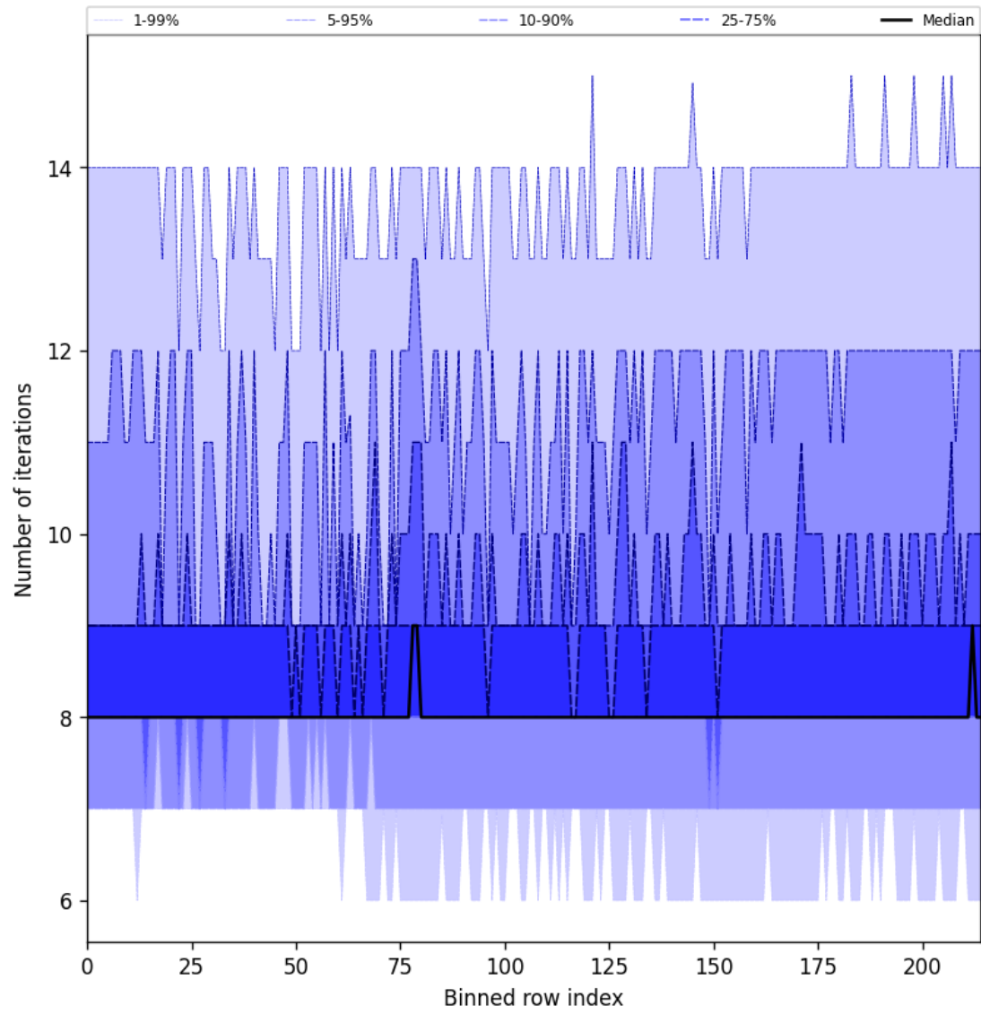
Figure 26: Along track statistics of “Number of iterations” for 2025-02-18 to 2025-02-19
