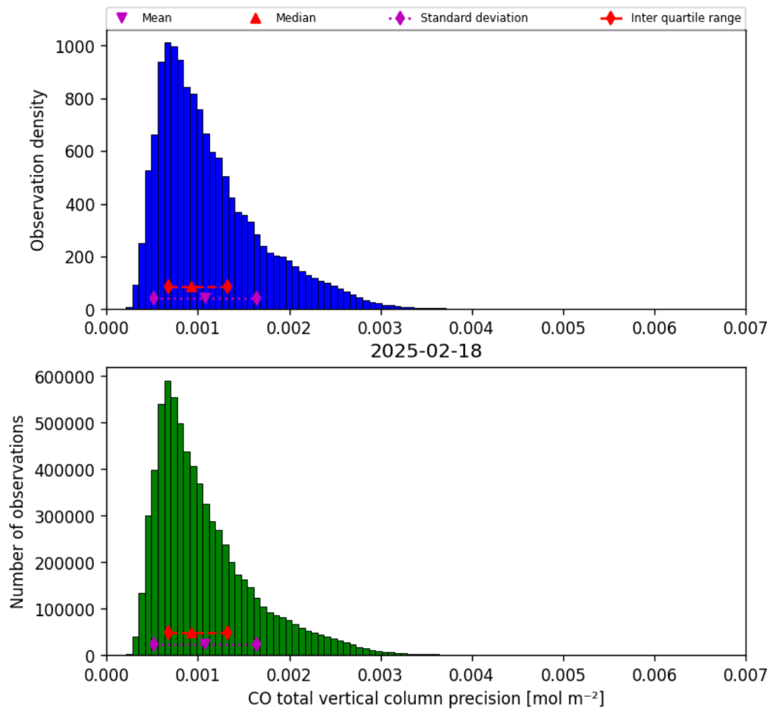
Figure 15: Histogram of “CO total vertical column precision” for 2025-02-18 to 2025-02-19
