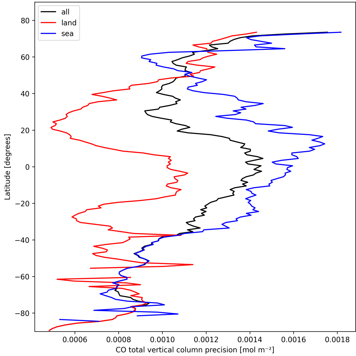
Figure 8: Zonal average of “CO total vertical column precision” for 2025-02-18 to 2025-02-19.
