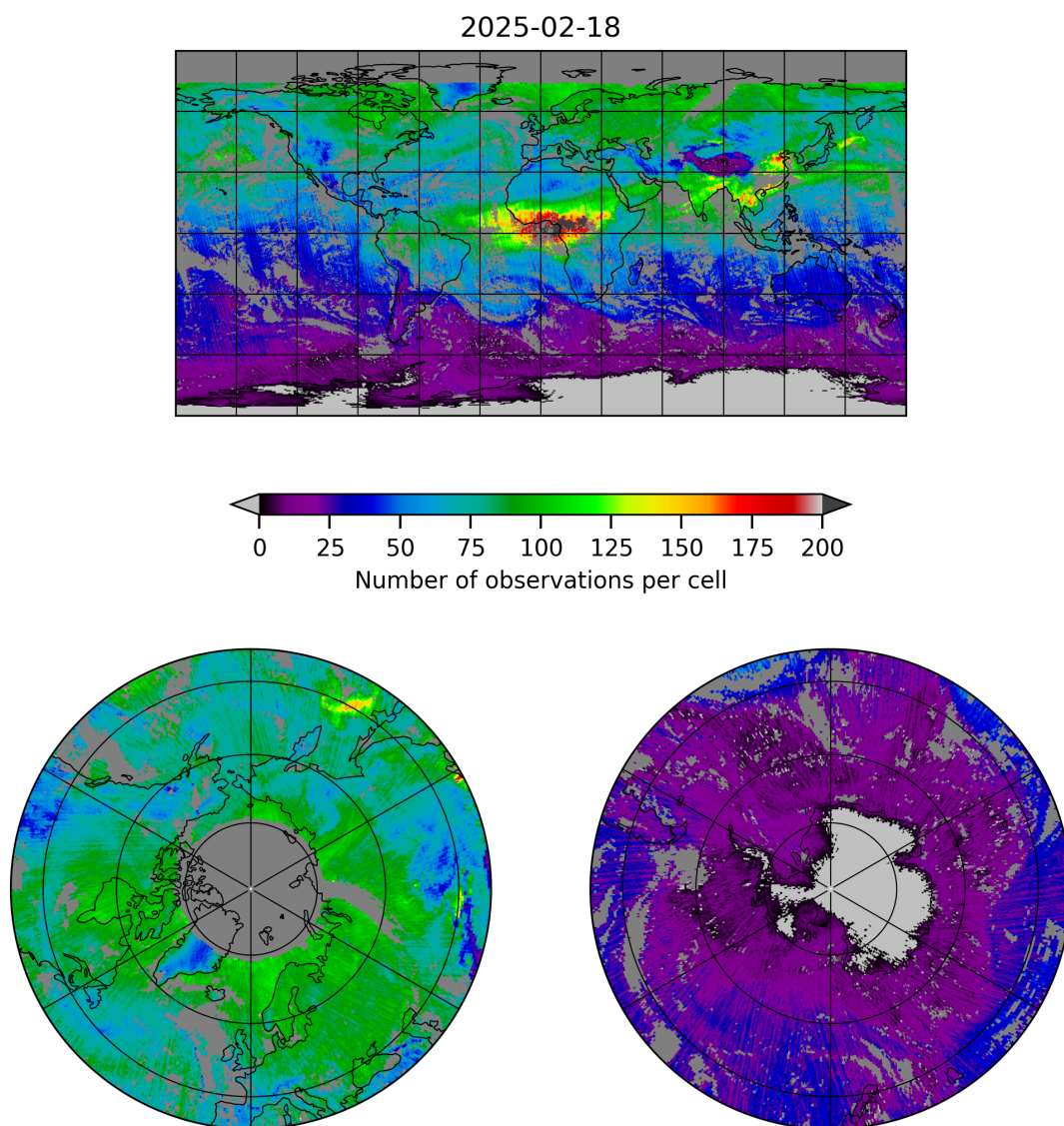
Figure 5: Map of the number of observations for 2025-02-18 to 2025-02-19
