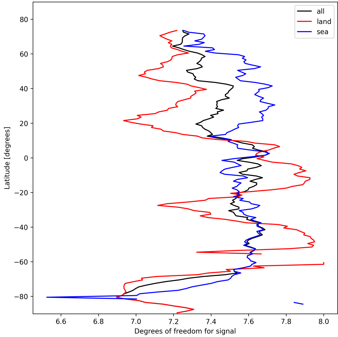
Figure 11: Zonal average of “Degrees of freedom for signal” for 2025-02-18 to 2025-02-19.
