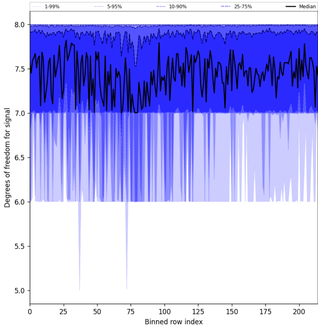
Figure 25: Along track statistics of “Degrees of freedom for signal” for 2025-02-18 to 2025-02-19
