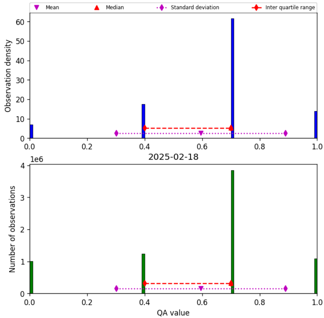
Figure 13: Histogram of “QA value” for 2025-02-18 to 2025-02-19
