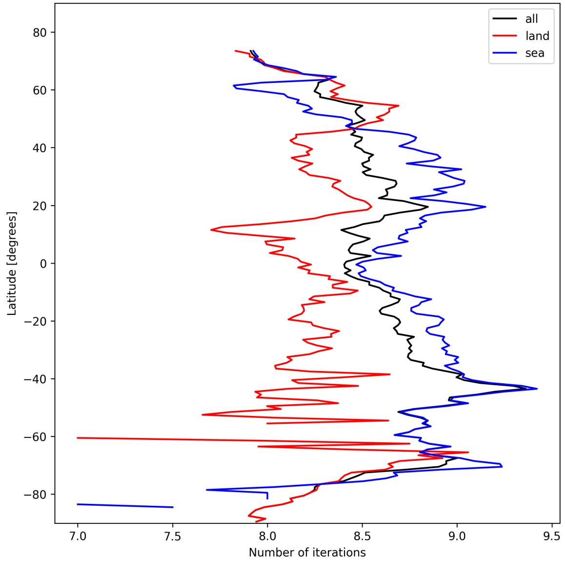
Figure 12: Zonal average of “Number of iterations” for 2025-02-18 to 2025-02-19.
