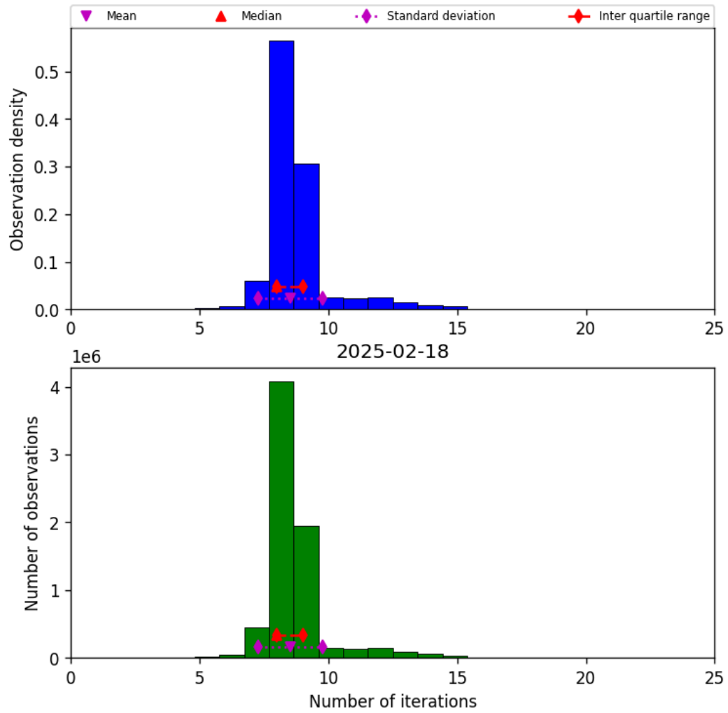
Figure 19: Histogram of “Number of iterations” for 2025-02-18 to 2025-02-19
