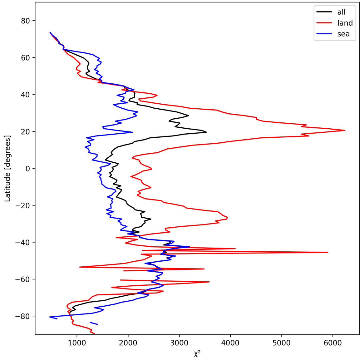
Figure 10: Zonal average of “ \chi^2 ” for 2025-02-18 to 2025-02-19.
