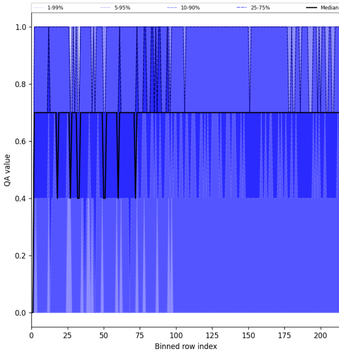
Figure 20: Along track statistics of “QA value” for 2025-02-18 to 2025-02-19
