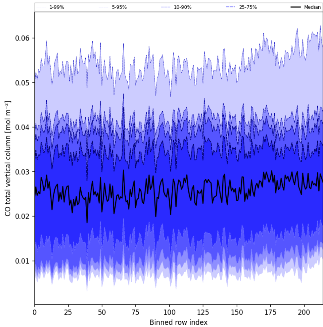
Figure 21: Along track statistics of “CO total vertical column” for 2025-02-18 to 2025-02-19
