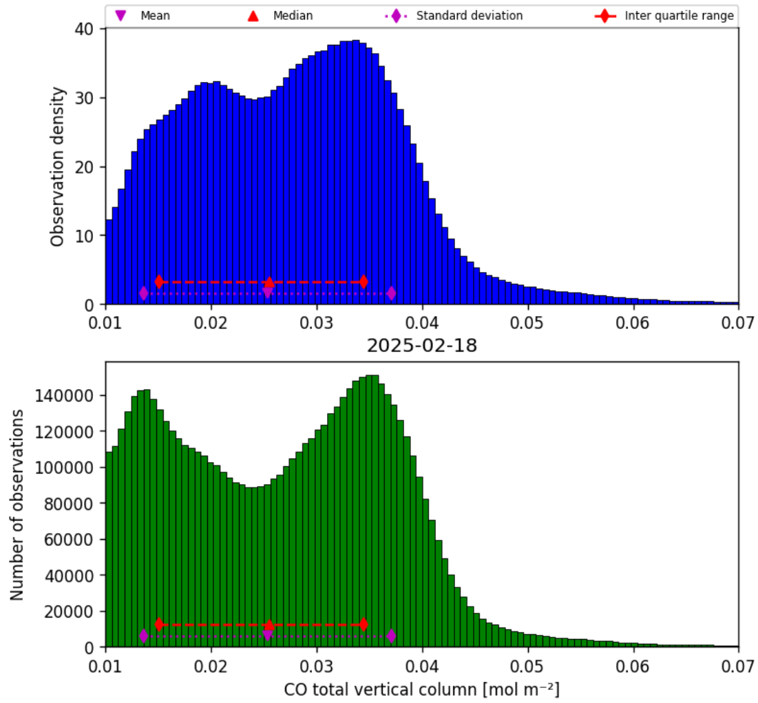
Figure 14: Histogram of “CO total vertical column” for 2025-02-18 to 2025-02-19
