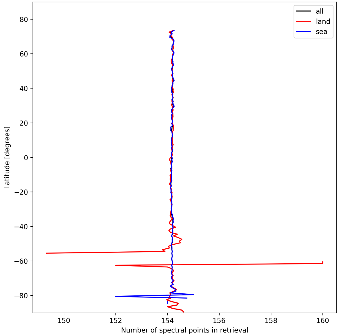
Figure 9: Zonal average of “Number of spectral points in retrieval” for 2025-02-18 to 2025-02-19.
