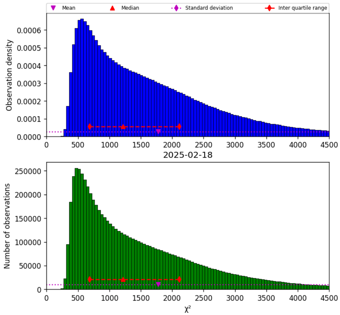
Figure 17: Histogram of “ \chi^2 ” for 2025-02-18 to 2025-02-19
