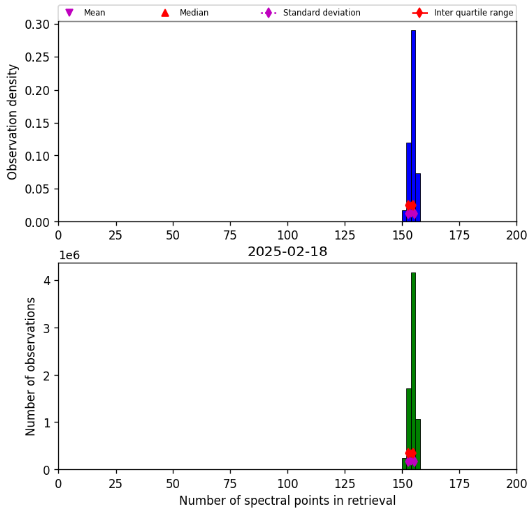
Figure 16: Histogram of “Number of spectral points in retrieval” for 2025-02-18 to 2025-02-19
