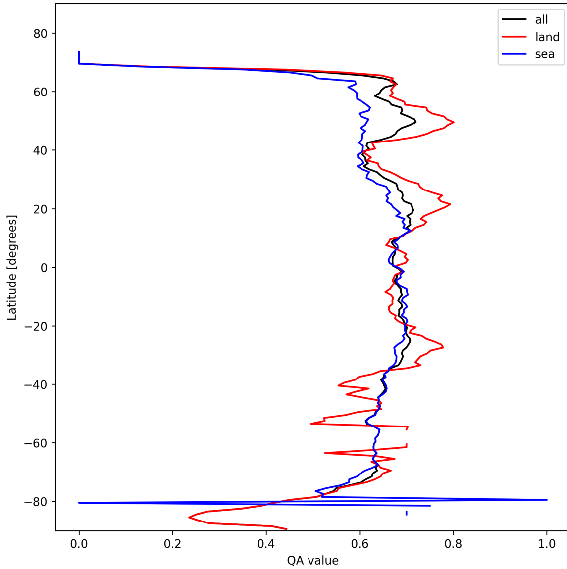
Figure 6: Zonal average of “QA value” for 2025-02-18 to 2025-02-19.
