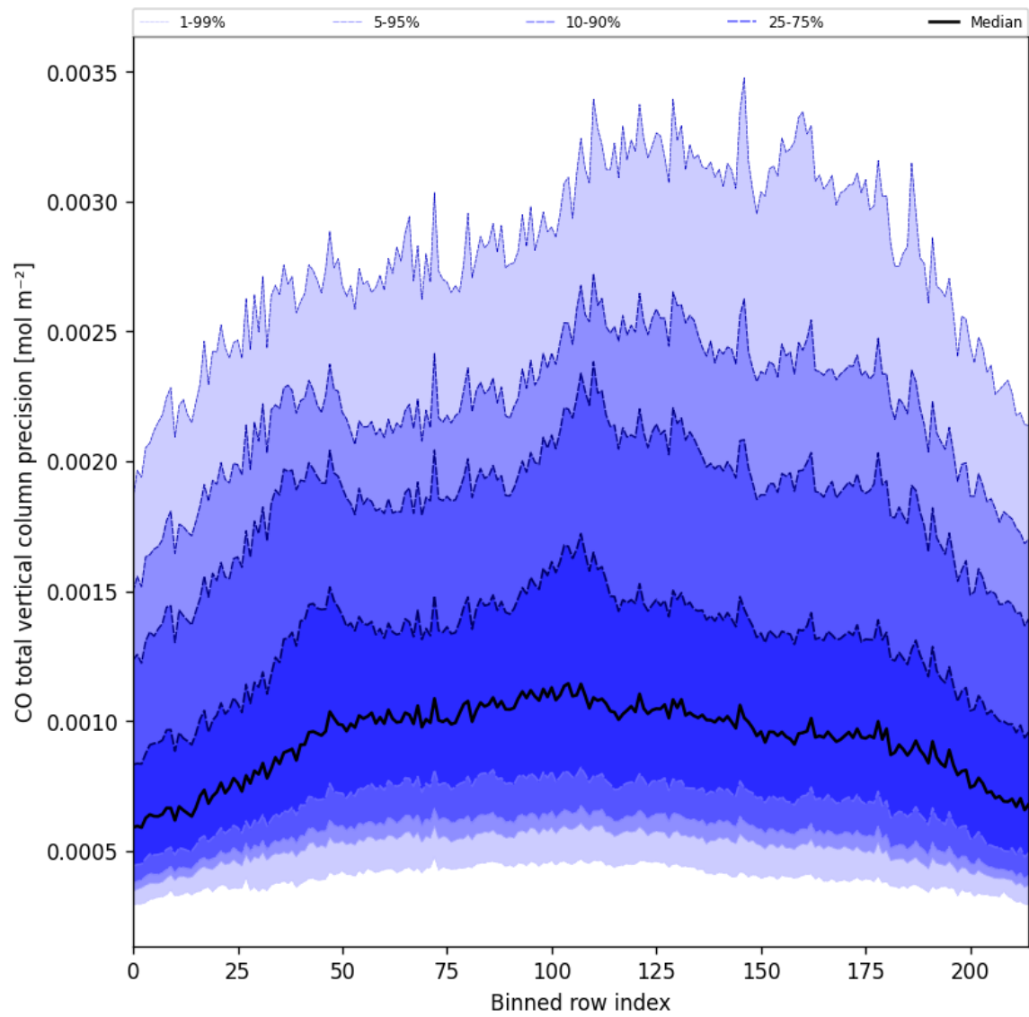
Figure 22: Along track statistics of “CO total vertical column precision” for 2025-02-18 to 2025-02-19
