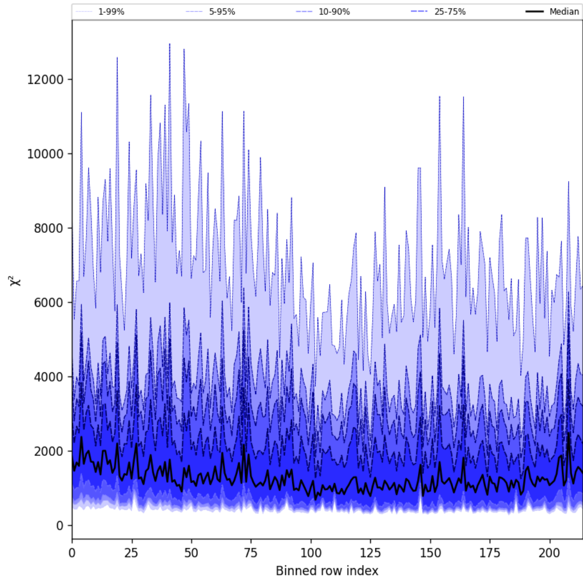
Figure 24: Along track statistics of “ \chi^2 ” for 2025-02-18 to 2025-02-19
