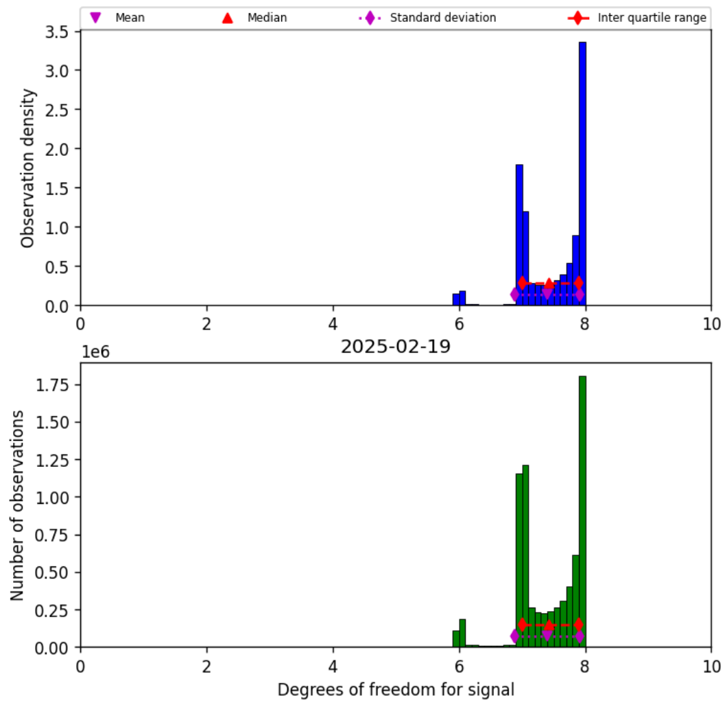
Figure 18: Histogram of “Degrees of freedom for signal” for 2025-02-19 to 2025-02-20
