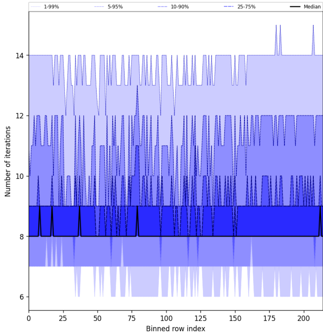
Figure 26: Along track statistics of “Number of iterations” for 2025-02-19 to 2025-02-20
