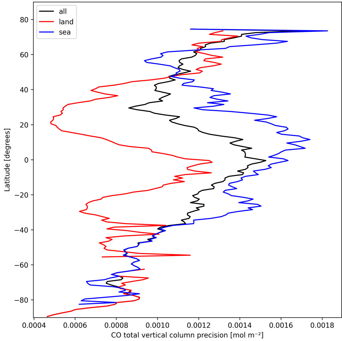
Figure 8: Zonal average of “CO total vertical column precision” for 2025-02-19 to 2025-02-20.
