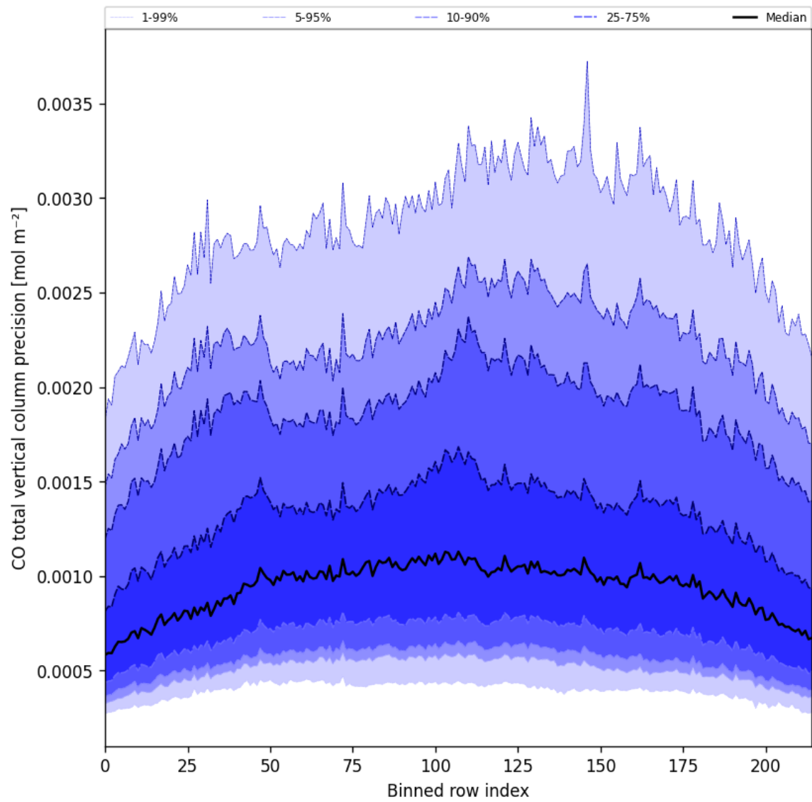
Figure 22: Along track statistics of “CO total vertical column precision” for 2025-02-19 to 2025-02-20
