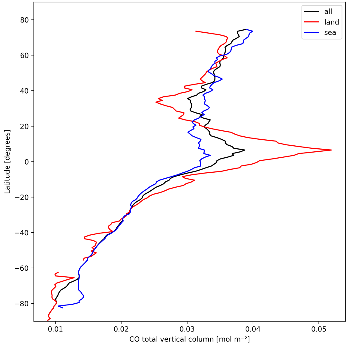
Figure 7: Zonal average of “CO total vertical column” for 2025-02-19 to 2025-02-20.
