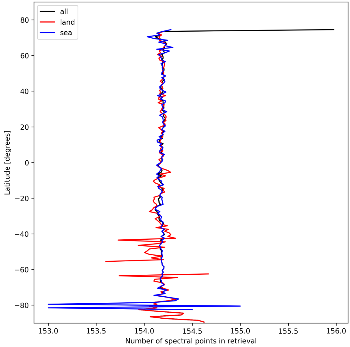
Figure 9: Zonal average of “Number of spectral points in retrieval” for 2025-02-19 to 2025-02-20.
