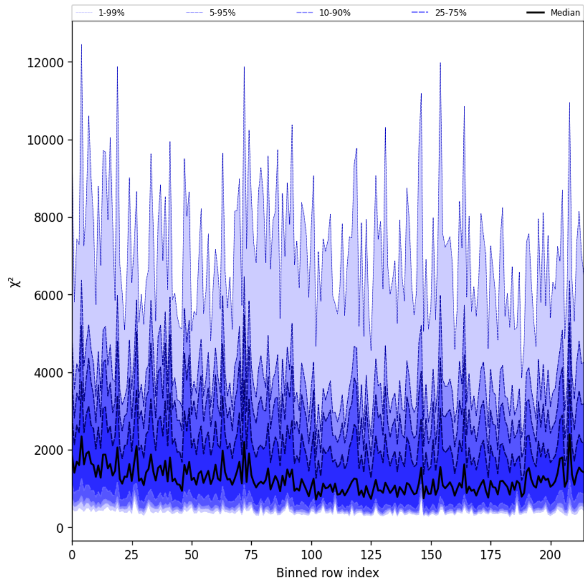
Figure 24: Along track statistics of “ \chi^2 ” for 2025-02-19 to 2025-02-20
