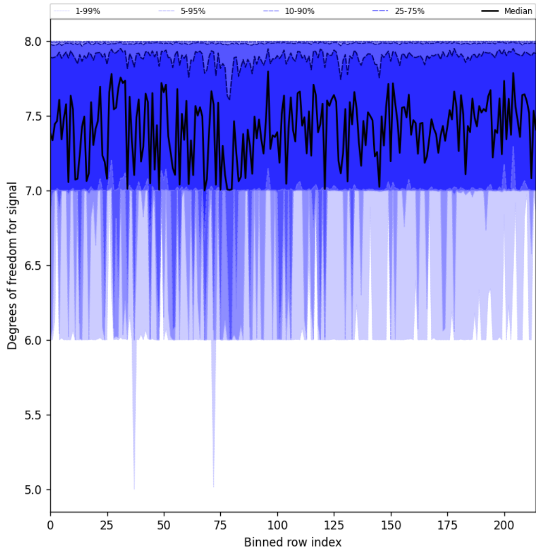
Figure 25: Along track statistics of “Degrees of freedom for signal” for 2025-02-19 to 2025-02-20
