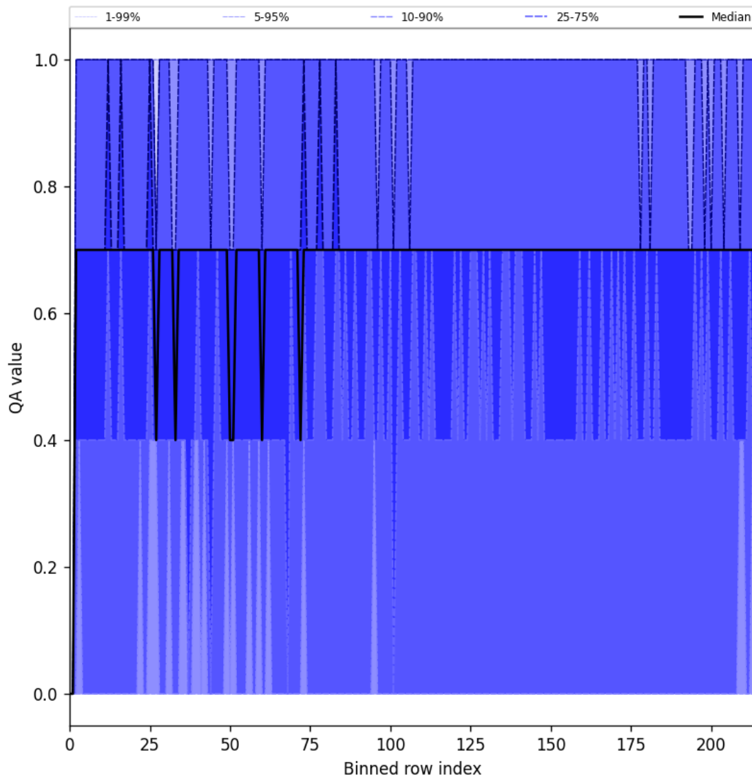
Figure 20: Along track statistics of “QA value” for 2025-02-19 to 2025-02-20
