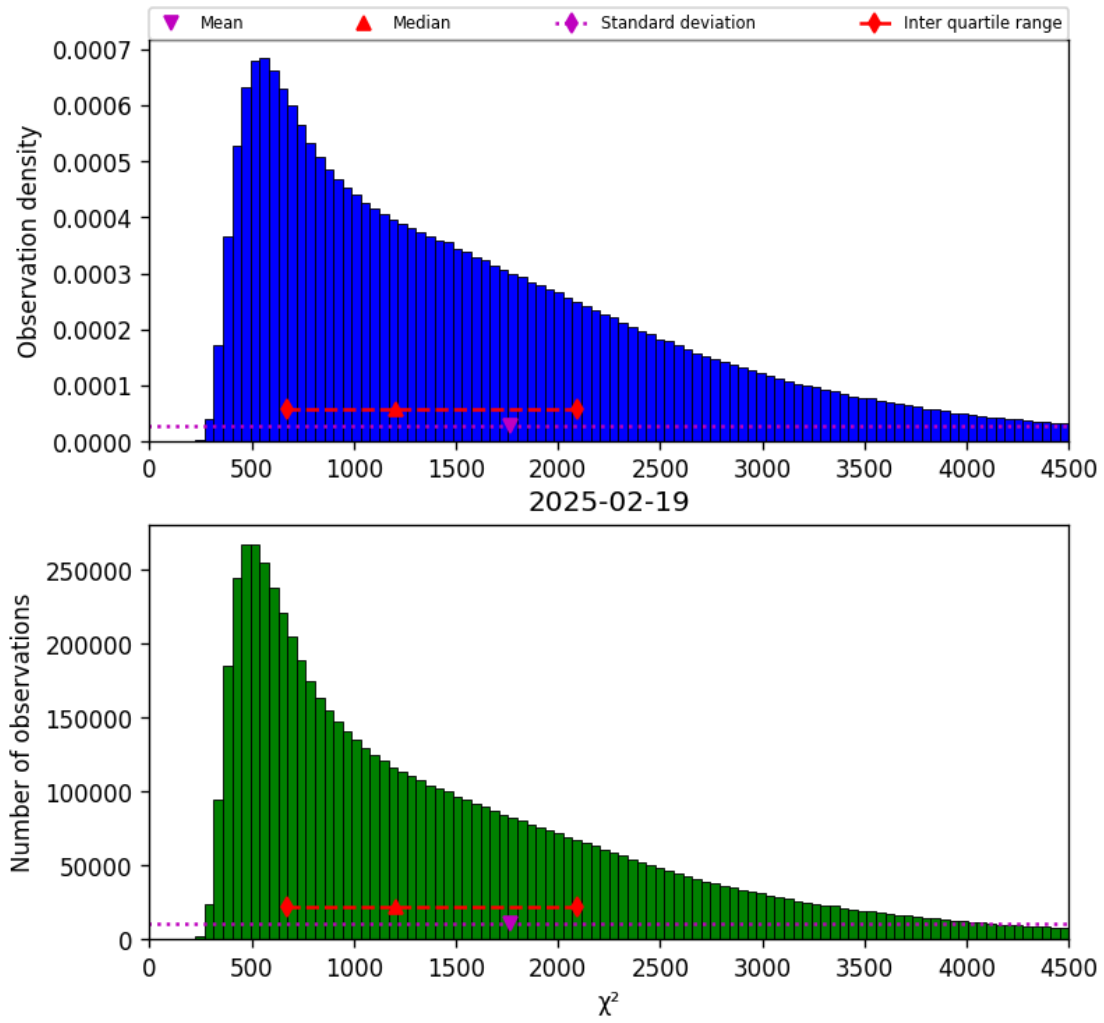
Figure 17: Histogram of “ \chi^2 ” for 2025-02-19 to 2025-02-20
