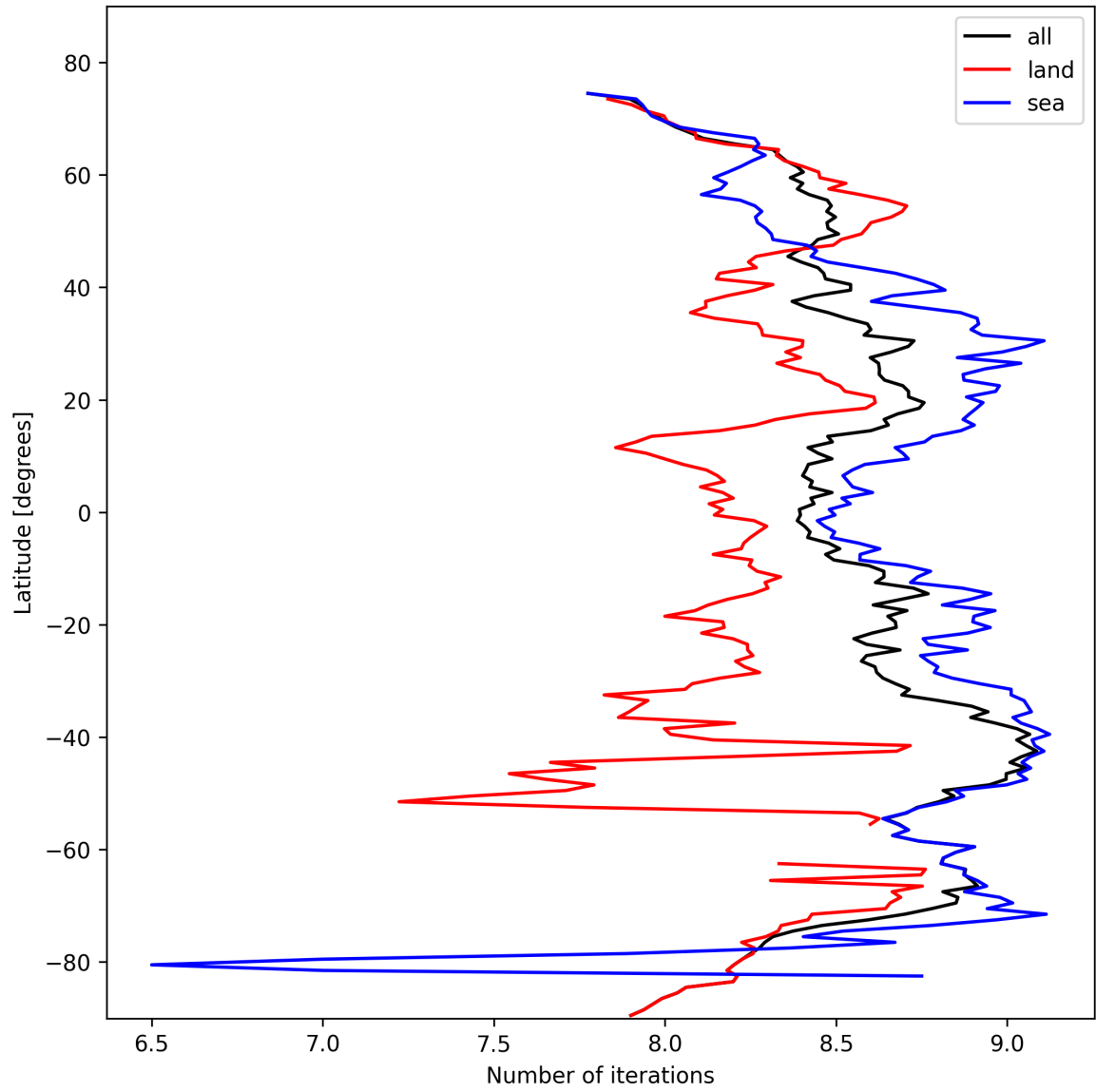
Figure 12: Zonal average of “Number of iterations” for 2025-02-19 to 2025-02-20.
