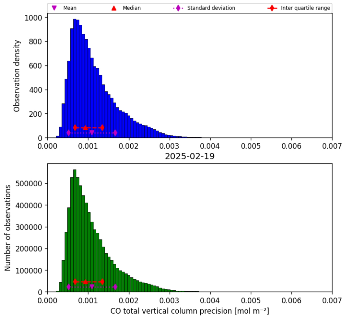
Figure 15: Histogram of “CO total vertical column precision” for 2025-02-19 to 2025-02-20
