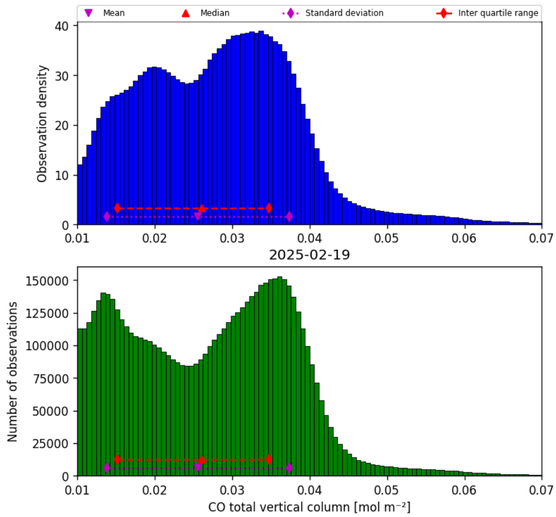
Figure 14: Histogram of “CO total vertical column” for 2025-02-19 to 2025-02-20
