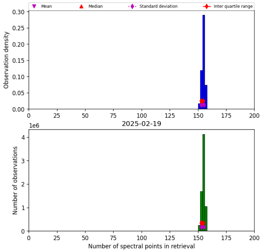
Figure 16: Histogram of “Number of spectral points in retrieval” for 2025-02-19 to 2025-02-20
