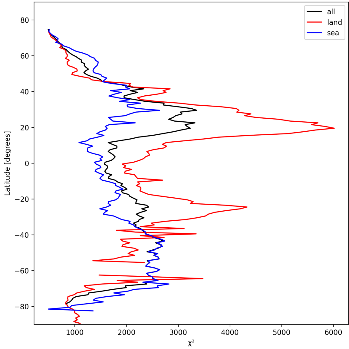
Figure 10: Zonal average of “ \chi^2 ” for 2025-02-19 to 2025-02-20.
