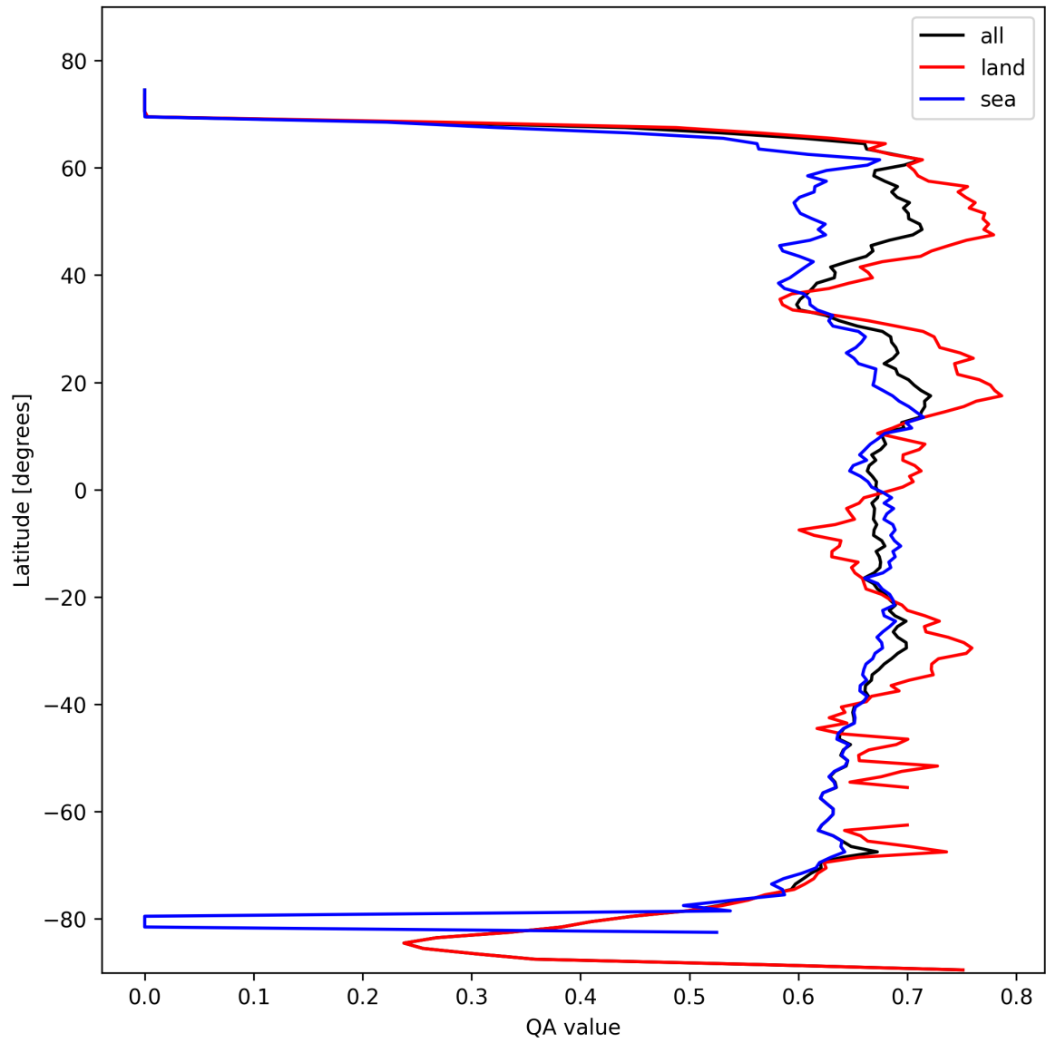
Figure 6: Zonal average of “QA value” for 2025-02-19 to 2025-02-20.
