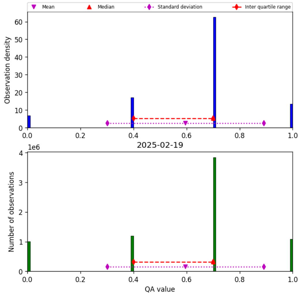
Figure 13: Histogram of “QA value” for 2025-02-19 to 2025-02-20
