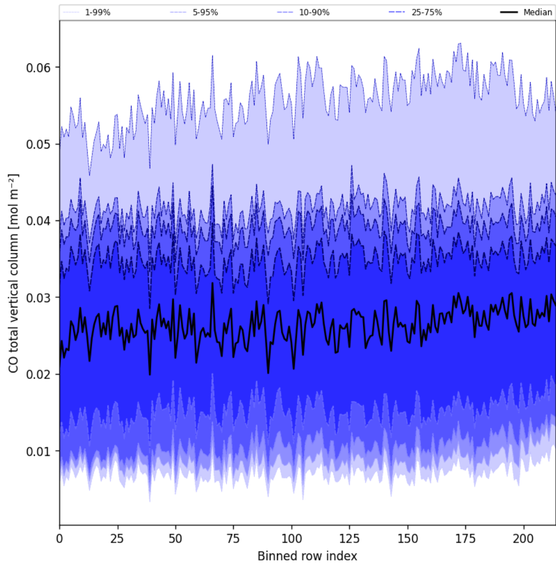
Figure 21: Along track statistics of “CO total vertical column” for 2025-02-19 to 2025-02-20
