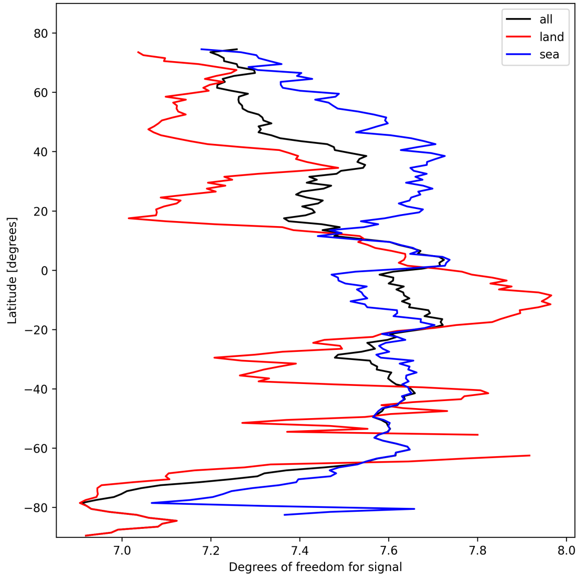
Figure 11: Zonal average of “Degrees of freedom for signal” for 2025-02-19 to 2025-02-20.
