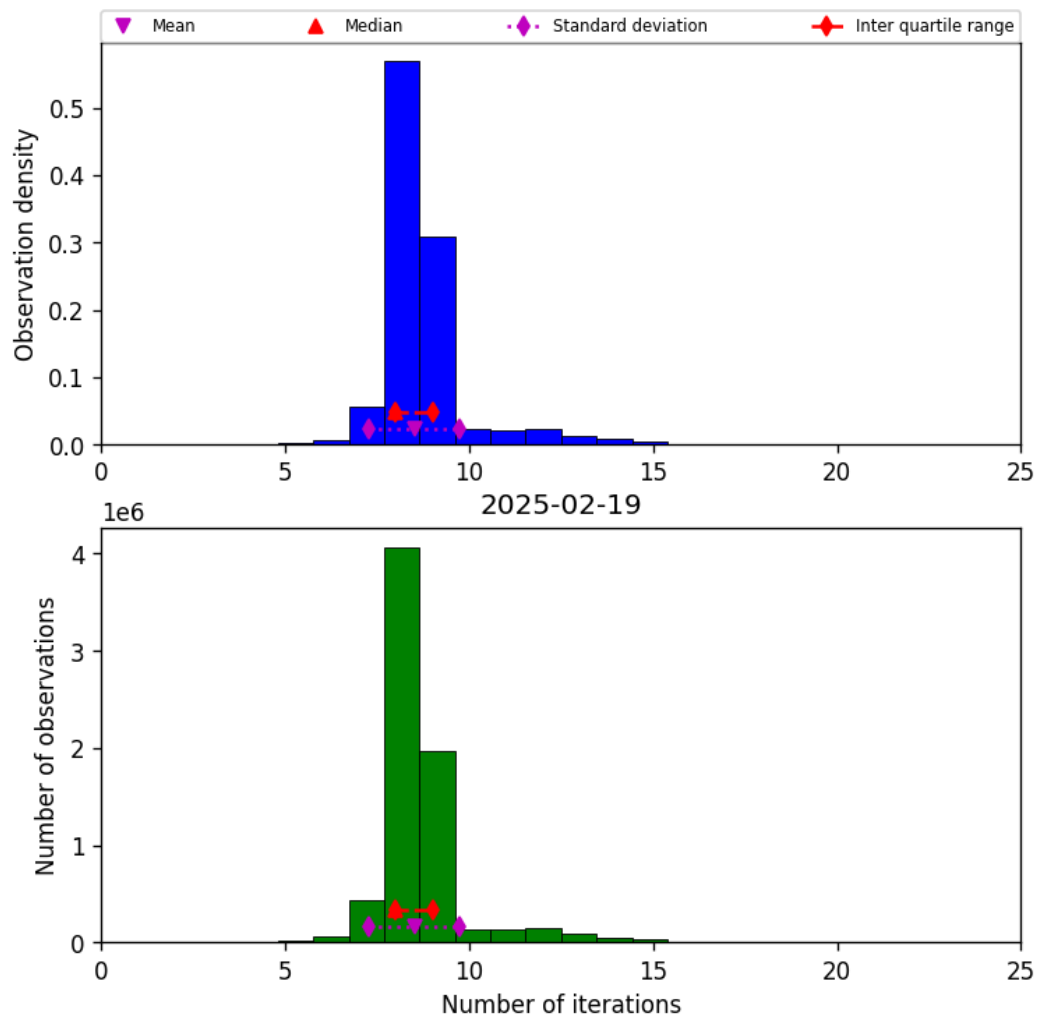
Figure 19: Histogram of “Number of iterations” for 2025-02-19 to 2025-02-20
