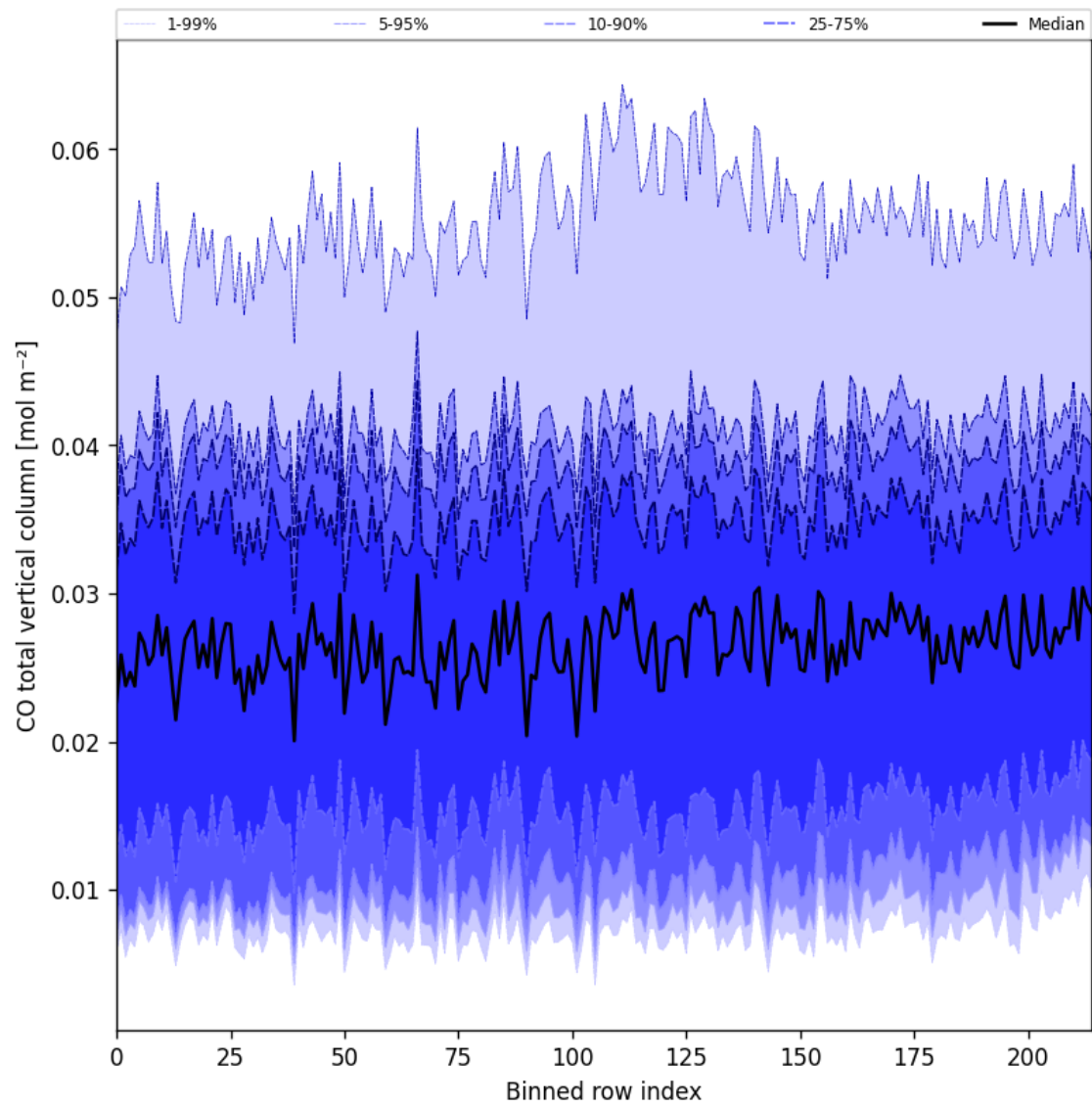
Figure 21: Along track statistics of “CO total vertical column” for 2025-02-20 to 2025-02-21
