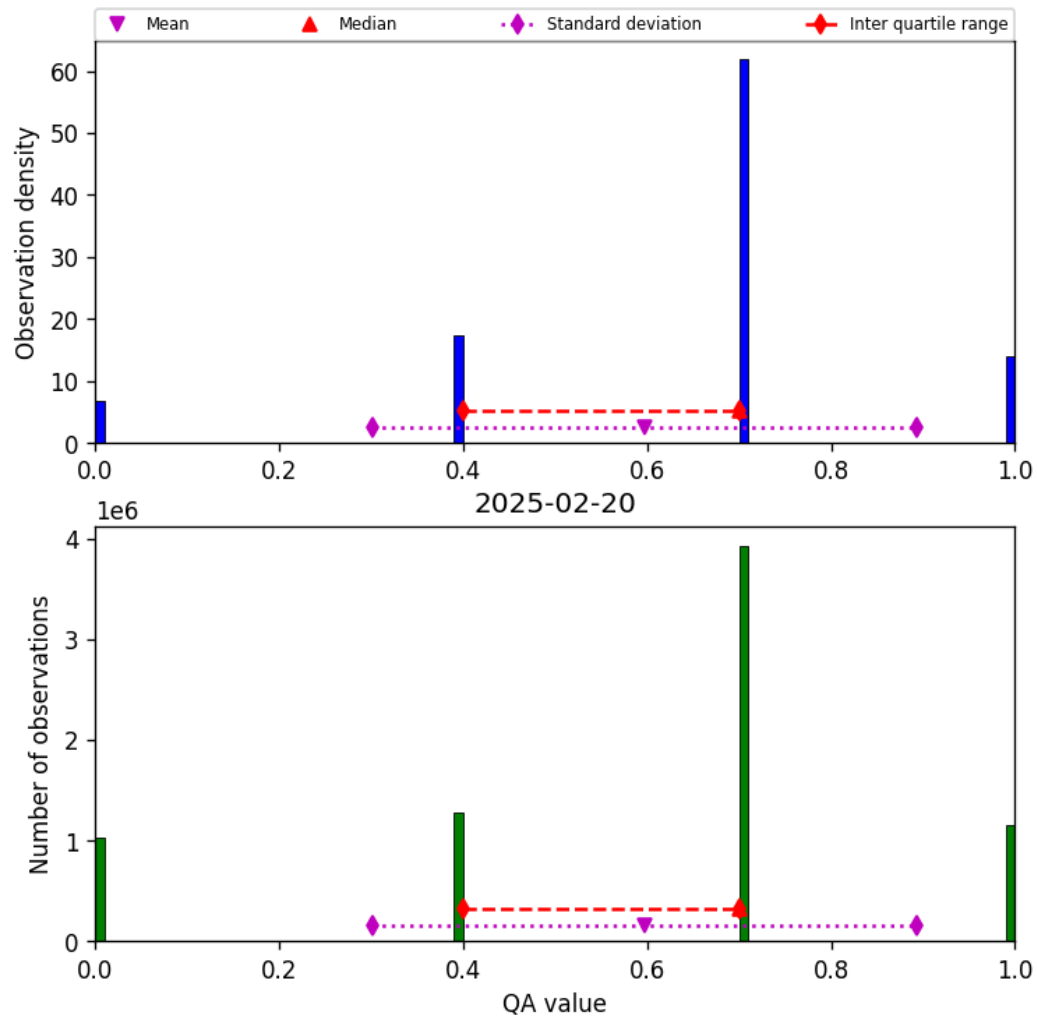
Figure 13: Histogram of “QA value” for 2025-02-20 to 2025-02-21
