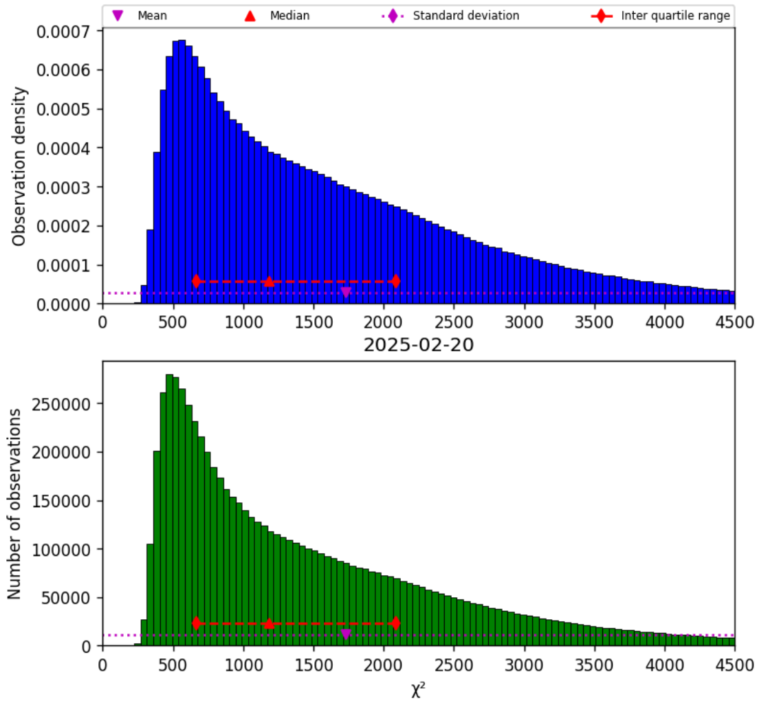
Figure 17: Histogram of " \chi^2 " for 2025-02-20 to 2025-02-21
