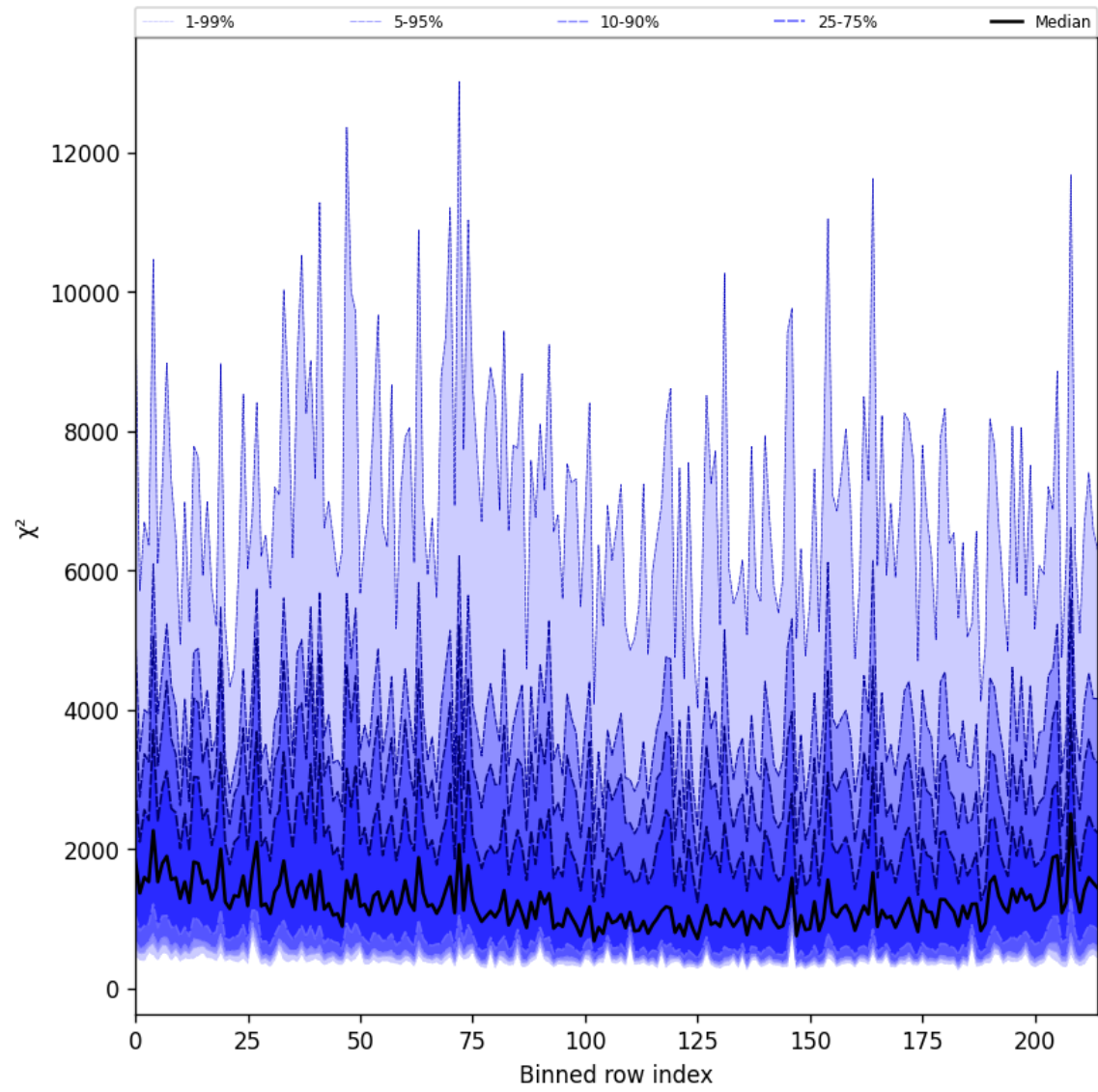
Figure 24: Along track statistics of “ \chi^2 ” for 2025-02-20 to 2025-02-21
