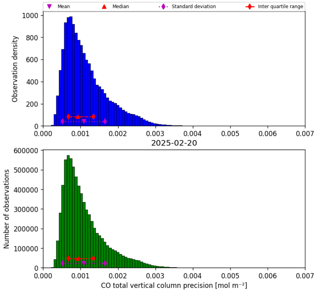
Figure 15: Histogram of “CO total vertical column precision” for 2025-02-20 to 2025-02-21
