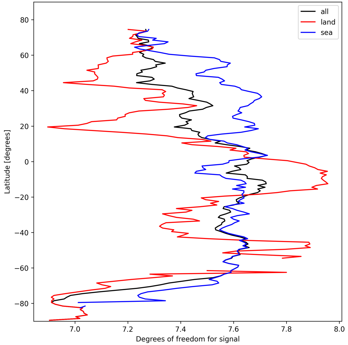
Figure 11: Zonal average of “Degrees of freedom for signal” for 2025-02-20 to 2025-02-21.
