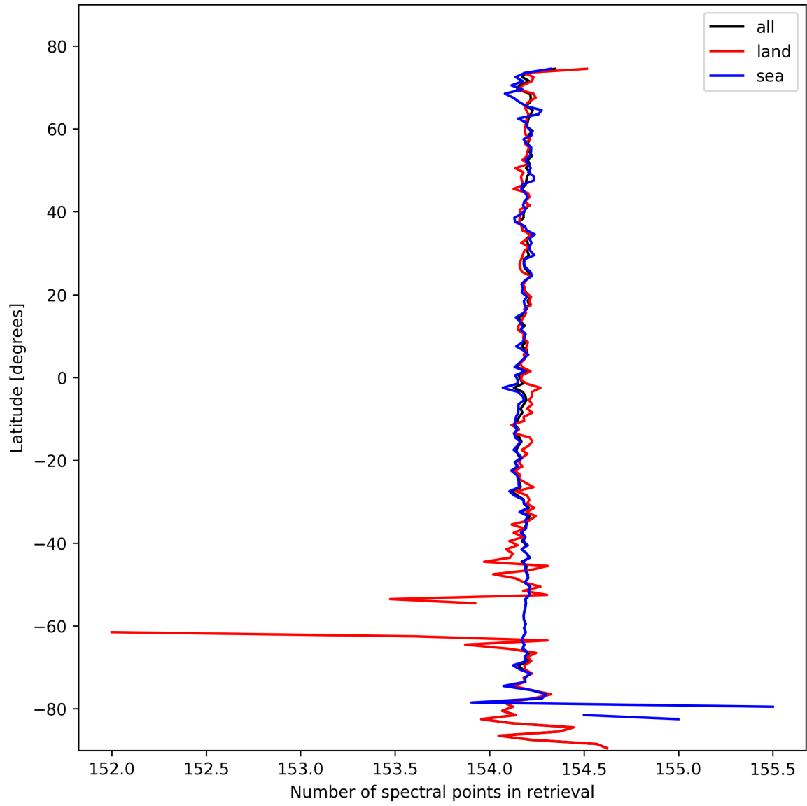
Figure 9: Zonal average of “Number of spectral points in retrieval” for 2025-02-20 to 2025-02-21.
