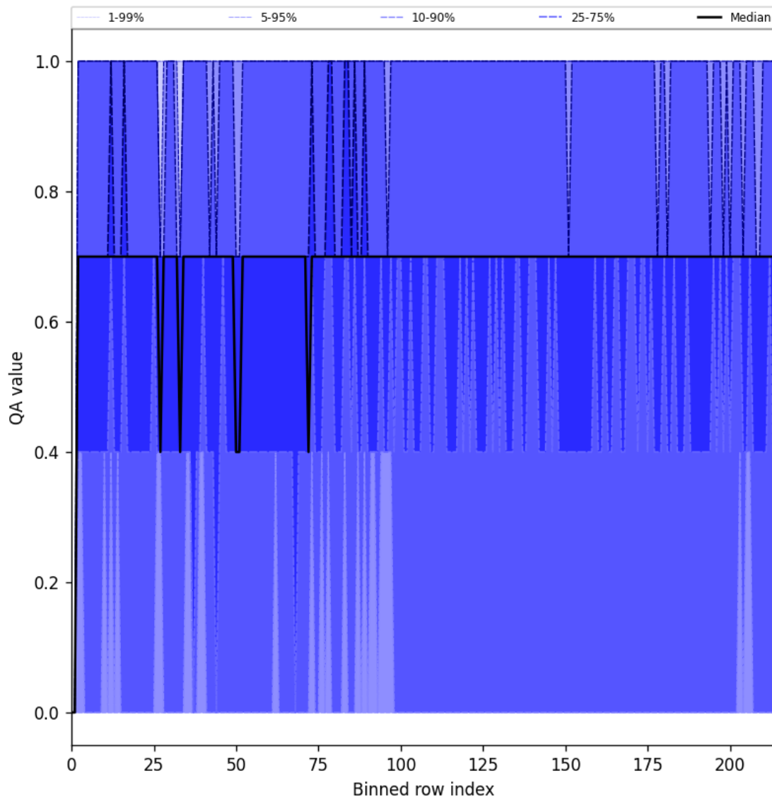
Figure 20: Along track statistics of “QA value” for 2025-02-20 to 2025-02-21
