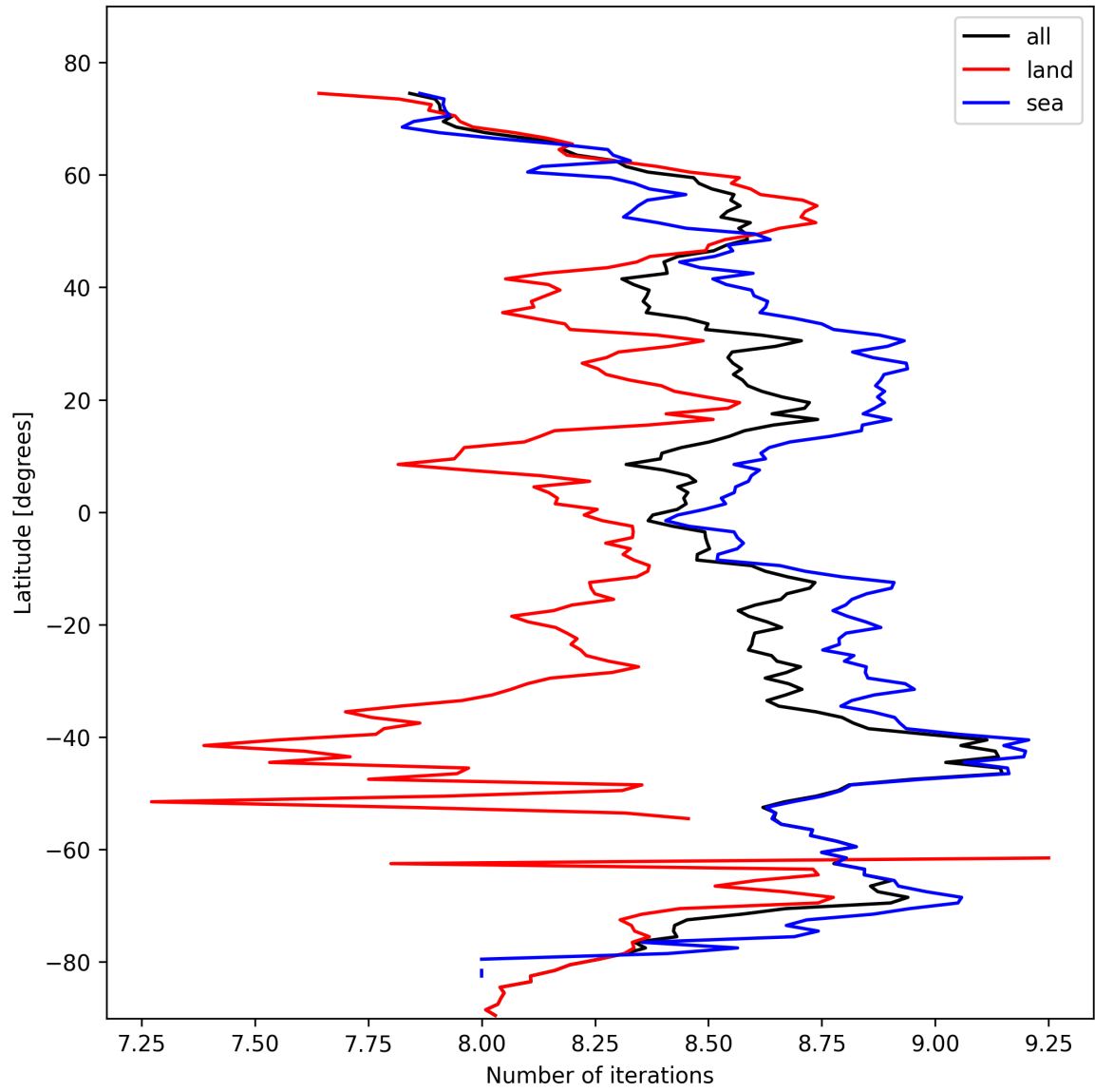
Figure 12: Zonal average of “Number of iterations” for 2025-02-20 to 2025-02-21.
