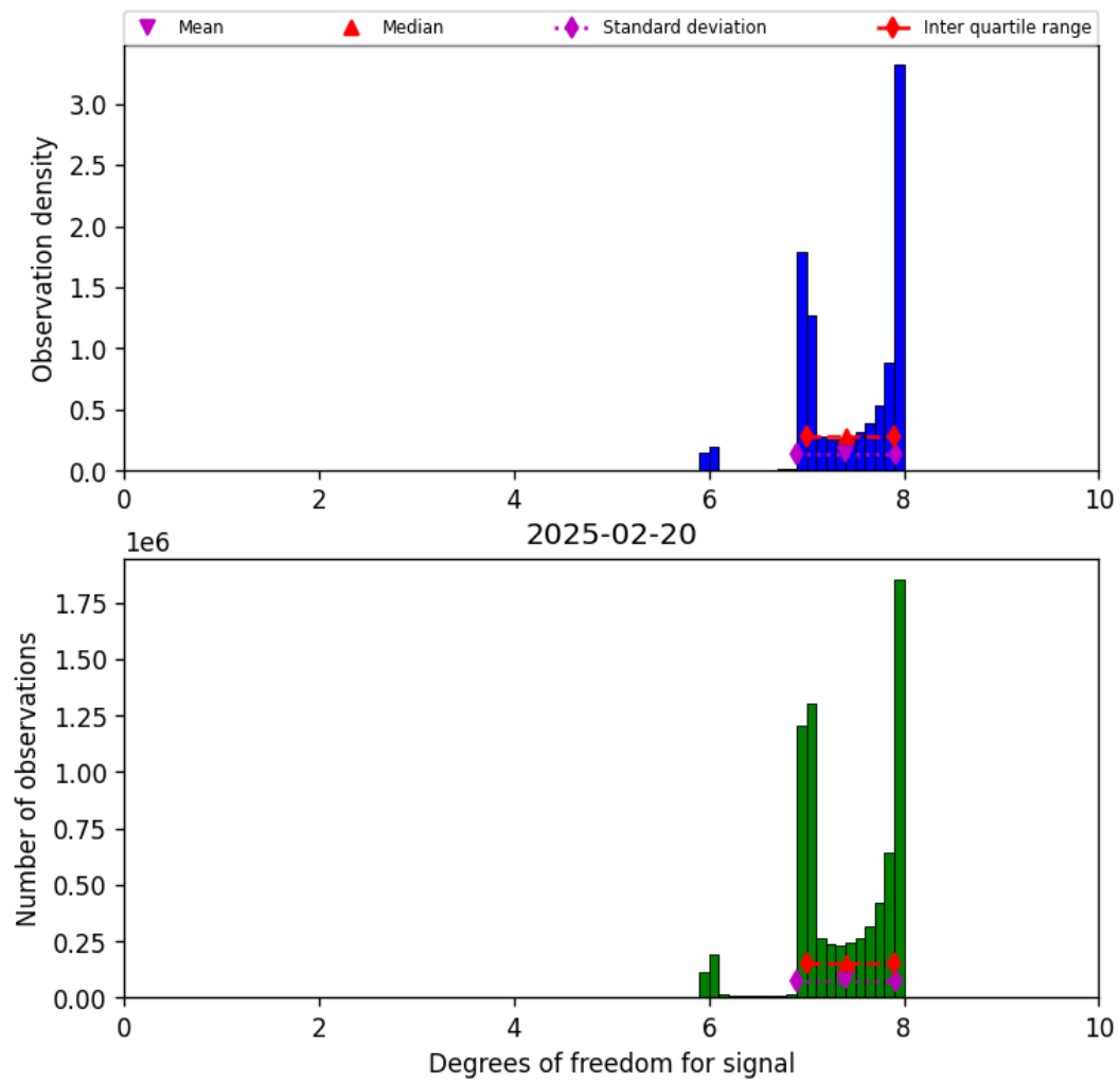
Figure 18: Histogram of “Degrees of freedom for signal” for 2025-02-20 to 2025-02-21
