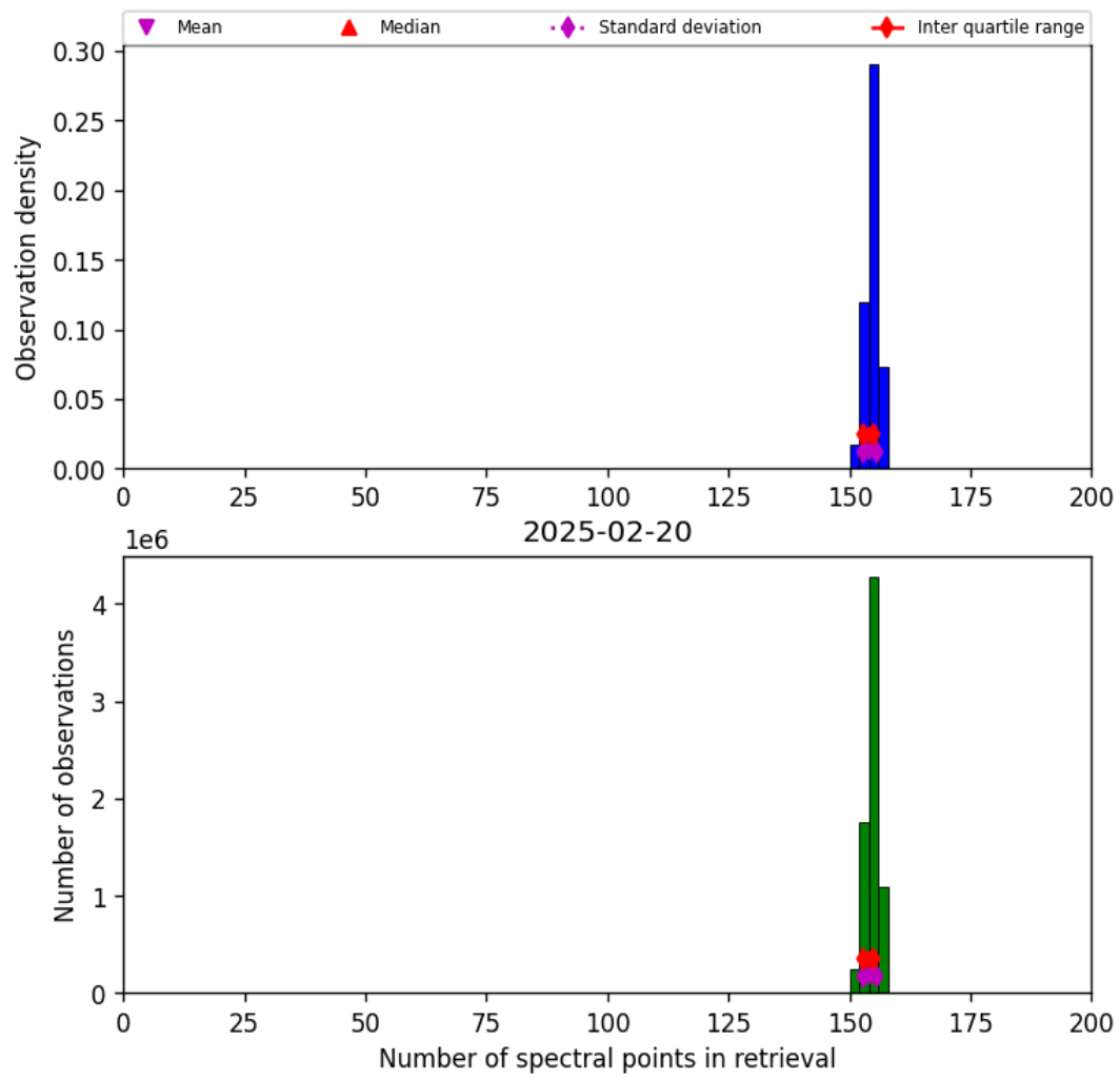
Figure 16: Histogram of “Number of spectral points in retrieval” for 2025-02-20 to 2025-02-21
