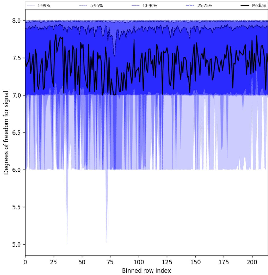
Figure 25: Along track statistics of “Degrees of freedom for signal” for 2025-02-20 to 2025-02-21
