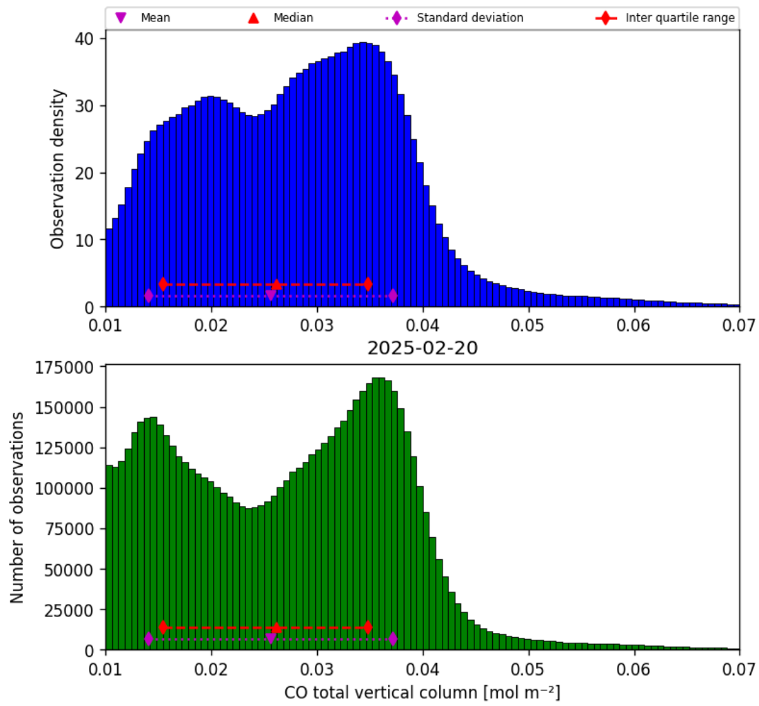
Figure 14: Histogram of “CO total vertical column” for 2025-02-20 to 2025-02-21
