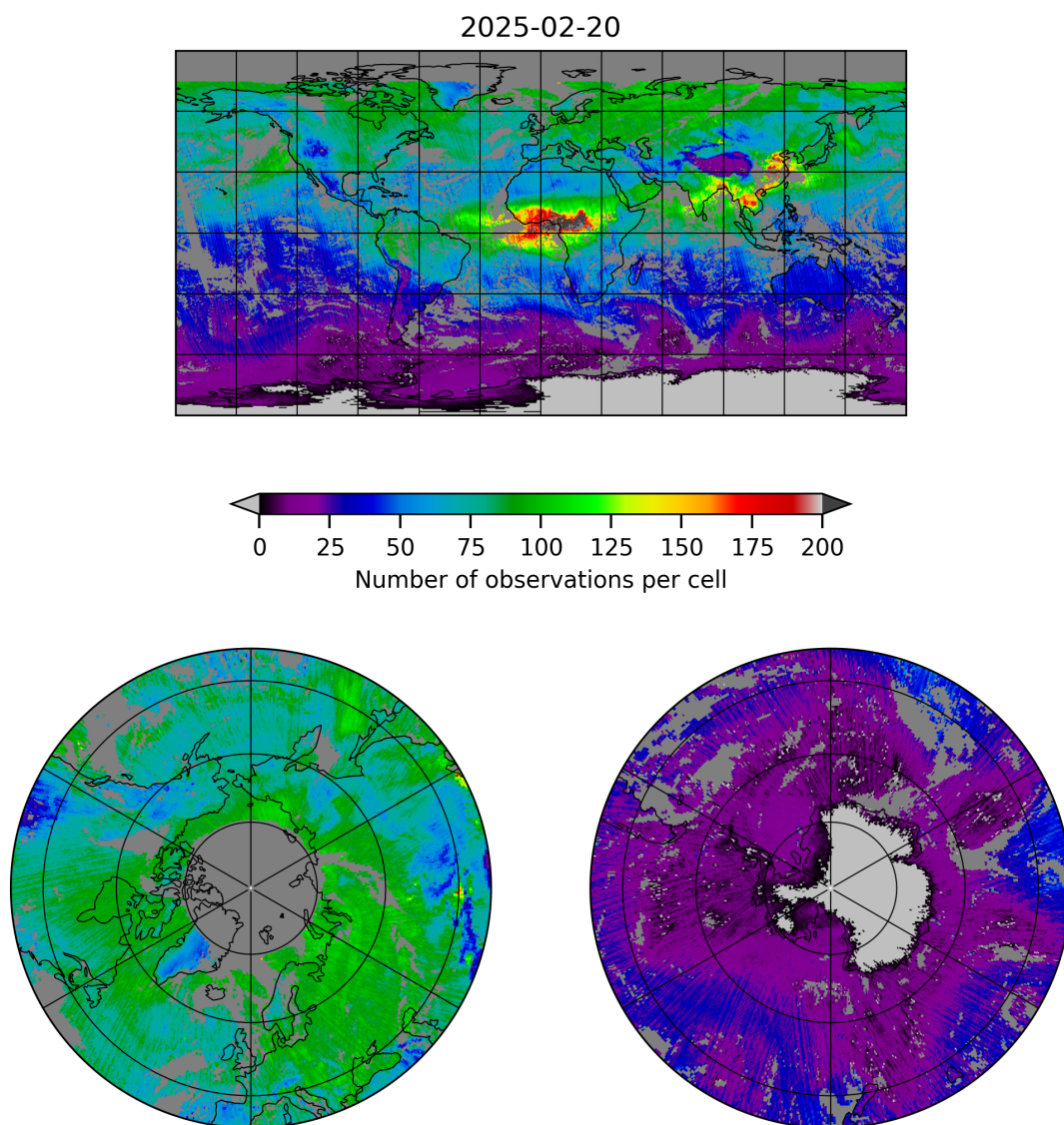
Figure 5: Map of the number of observations for 2025-02-20 to 2025-02-21
