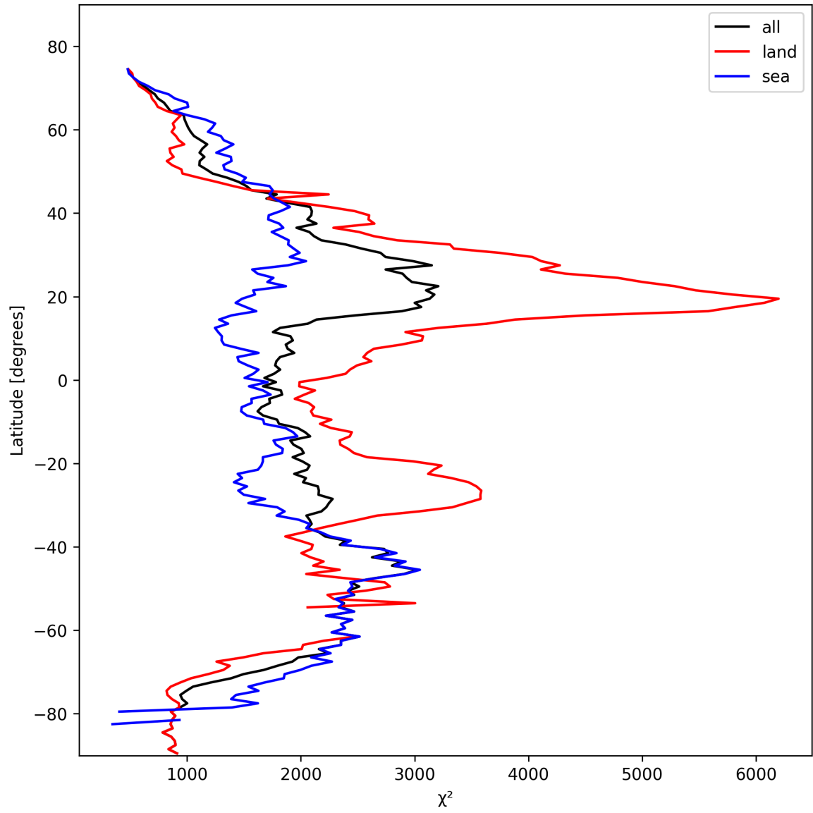
Figure 10: Zonal average of “ \chi^2 ” for 2025-02-20 to 2025-02-21.
