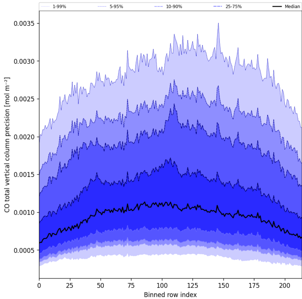
Figure 22: Along track statistics of “CO total vertical column precision” for 2025-02-20 to 2025-02-21
