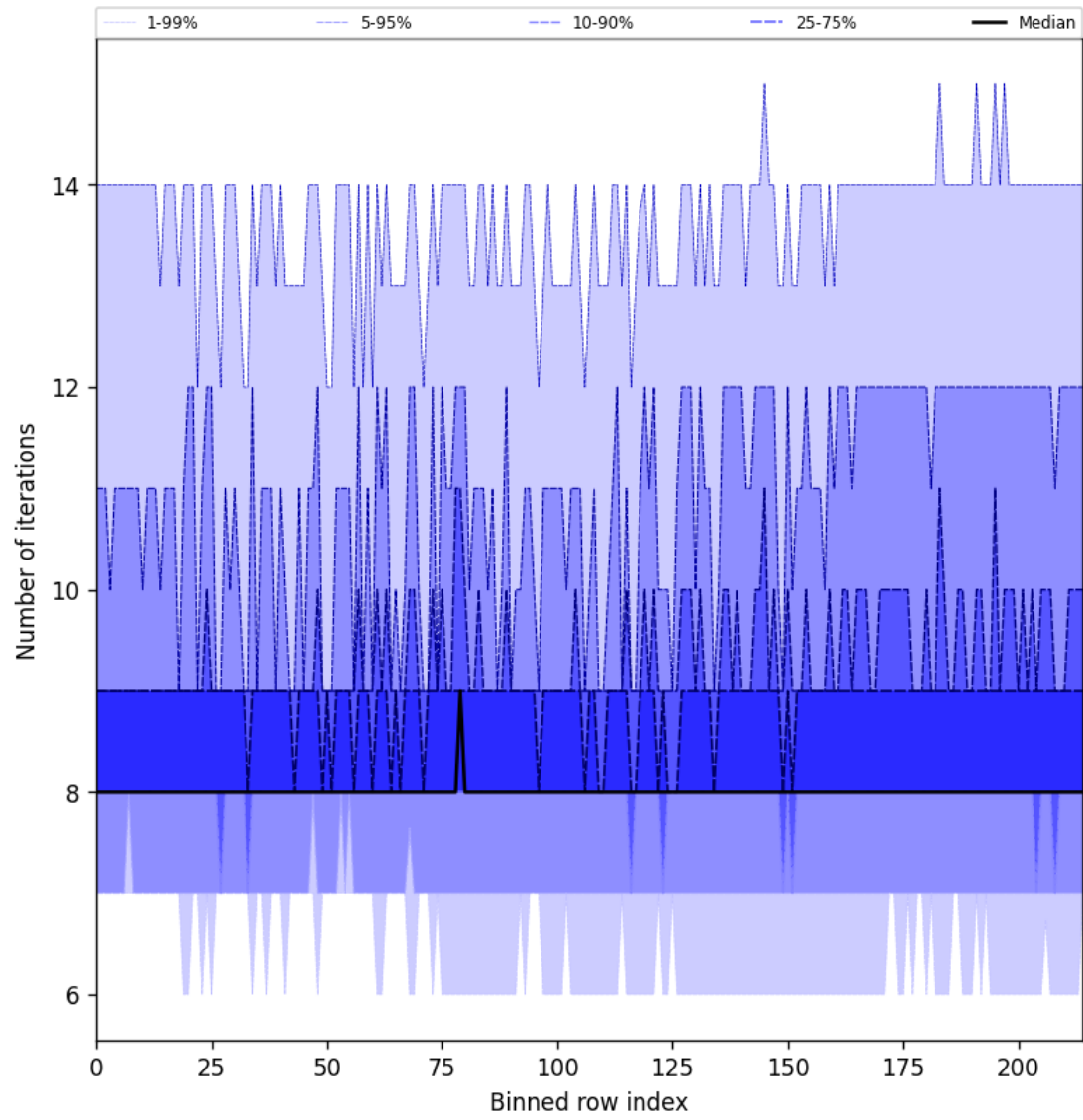
Figure 26: Along track statistics of “Number of iterations” for 2025-02-20 to 2025-02-21
