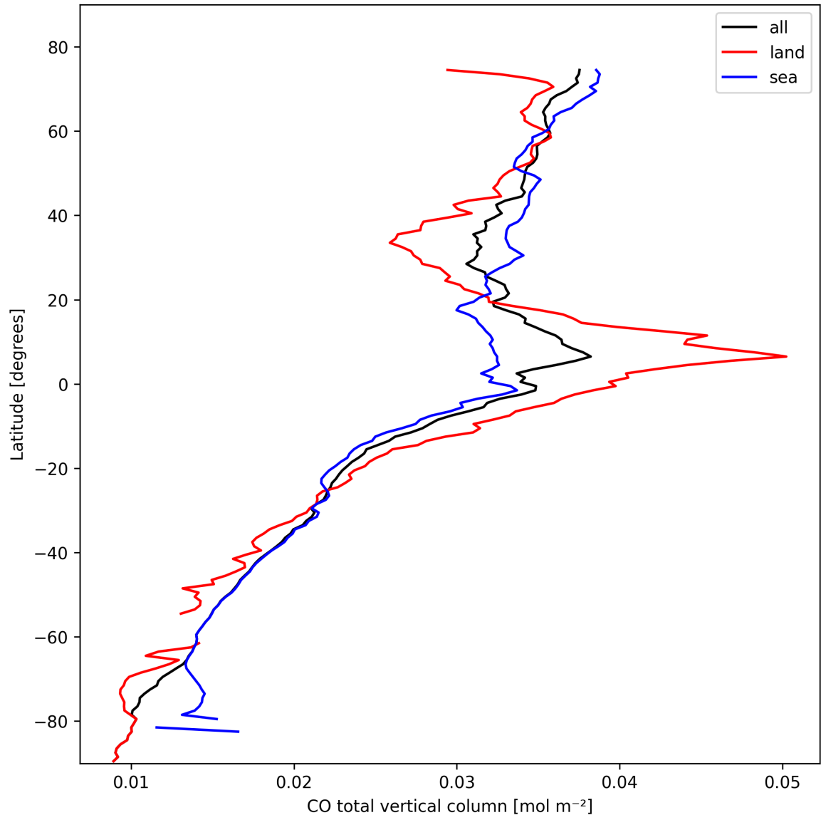
Figure 7: Zonal average of “CO total vertical column” for 2025-02-20 to 2025-02-21.
