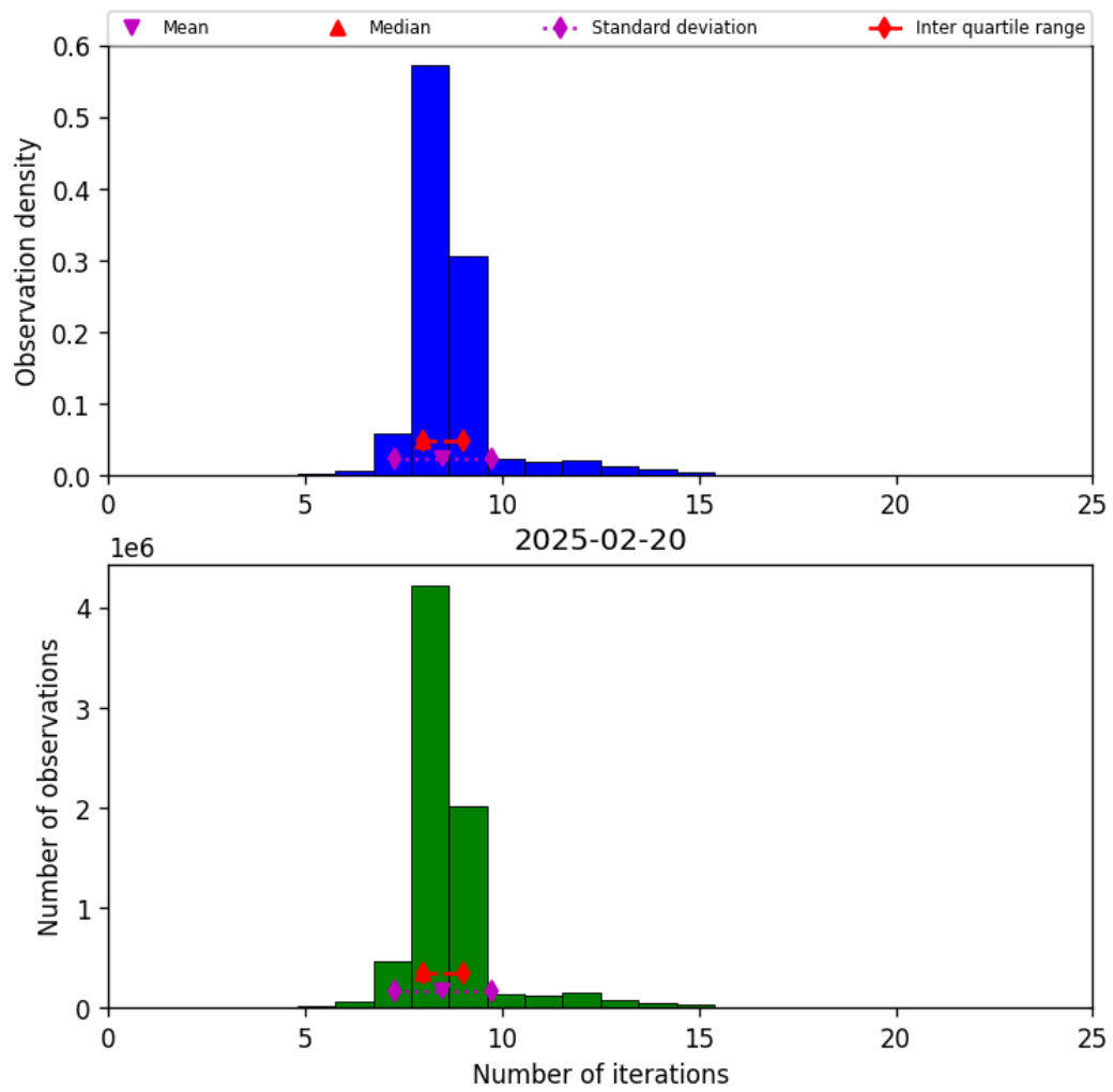
Figure 19: Histogram of “Number of iterations” for 2025-02-20 to 2025-02-21
