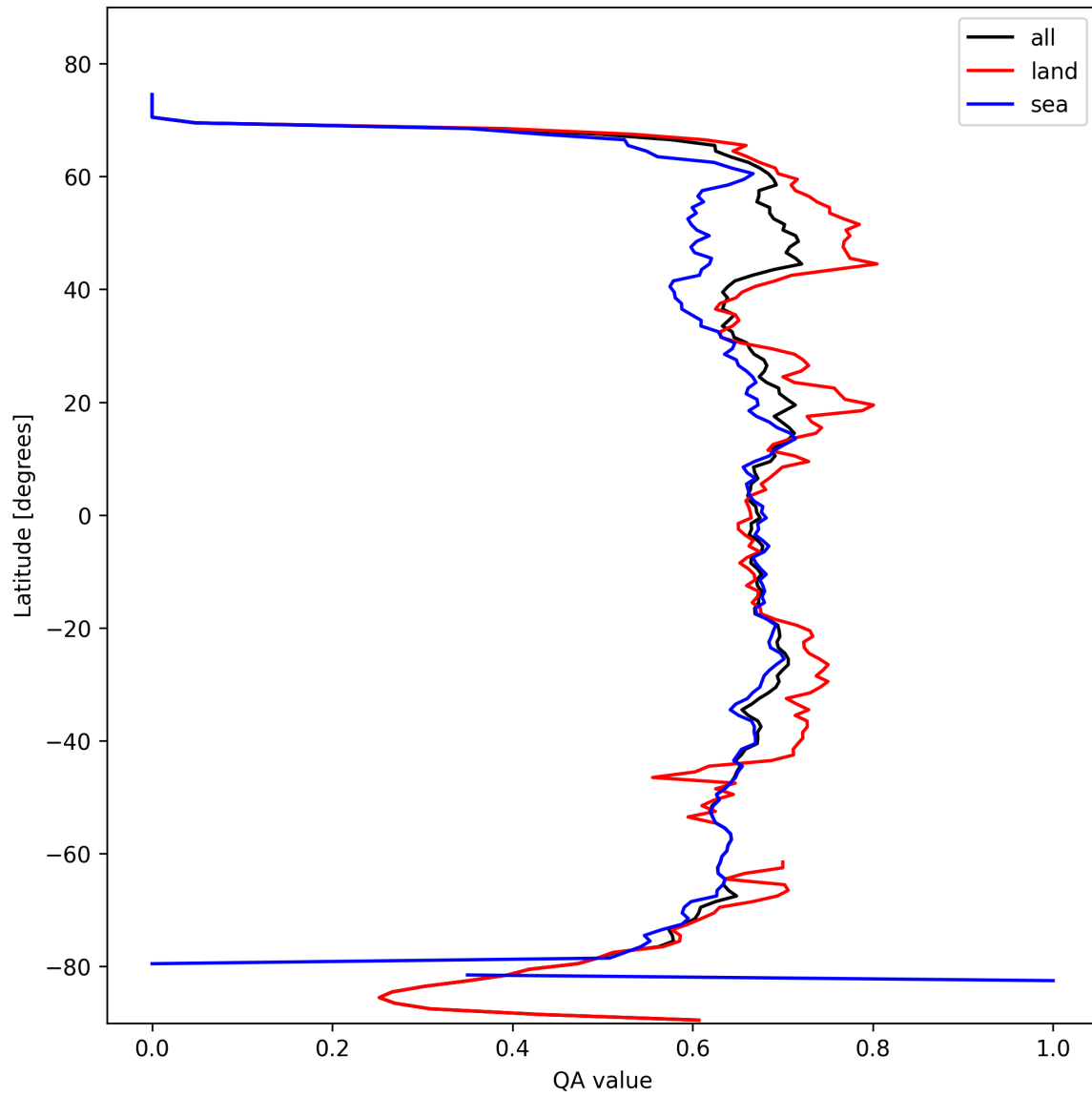
Figure 6: Zonal average of “QA value” for 2025-02-20 to 2025-02-21.
