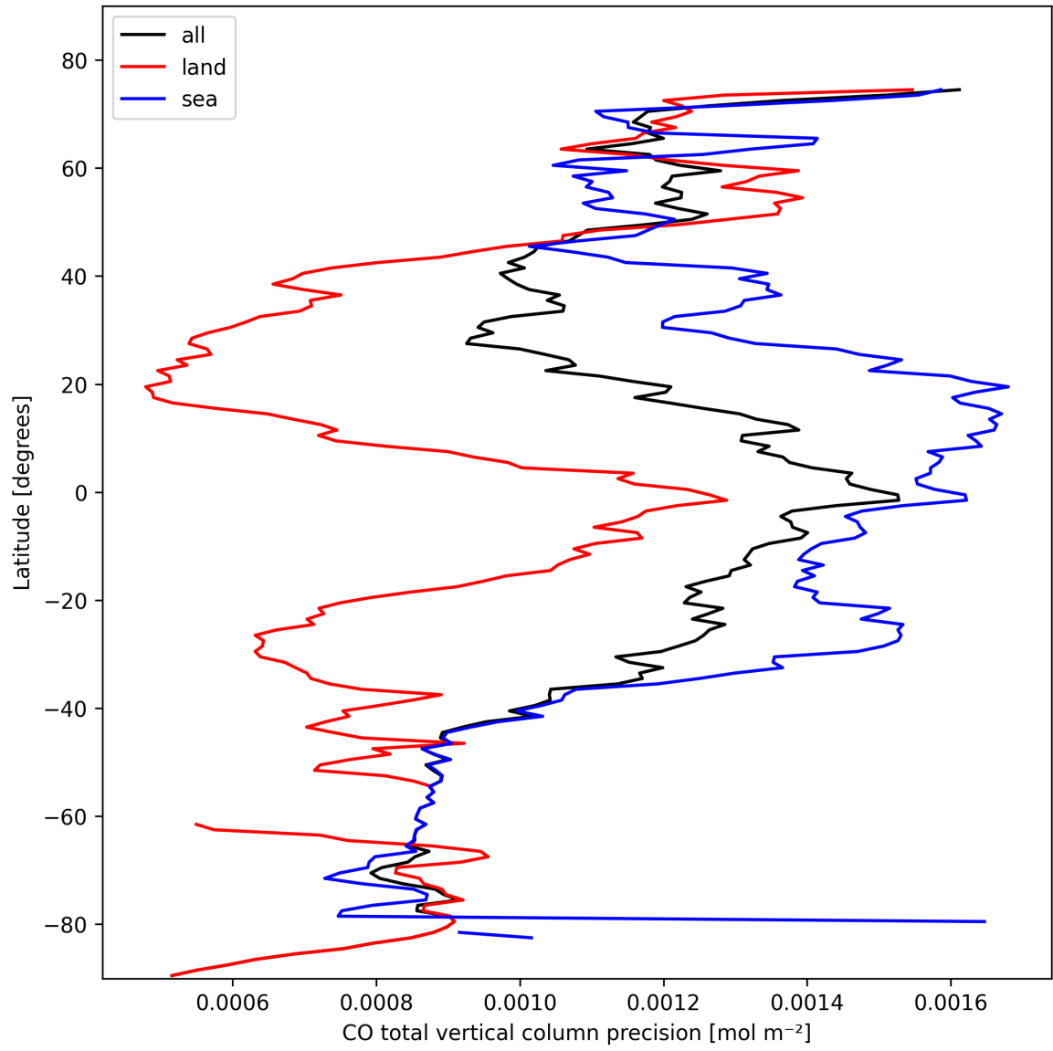
Figure 8: Zonal average of “CO total vertical column precision” for 2025-02-20 to 2025-02-21.
