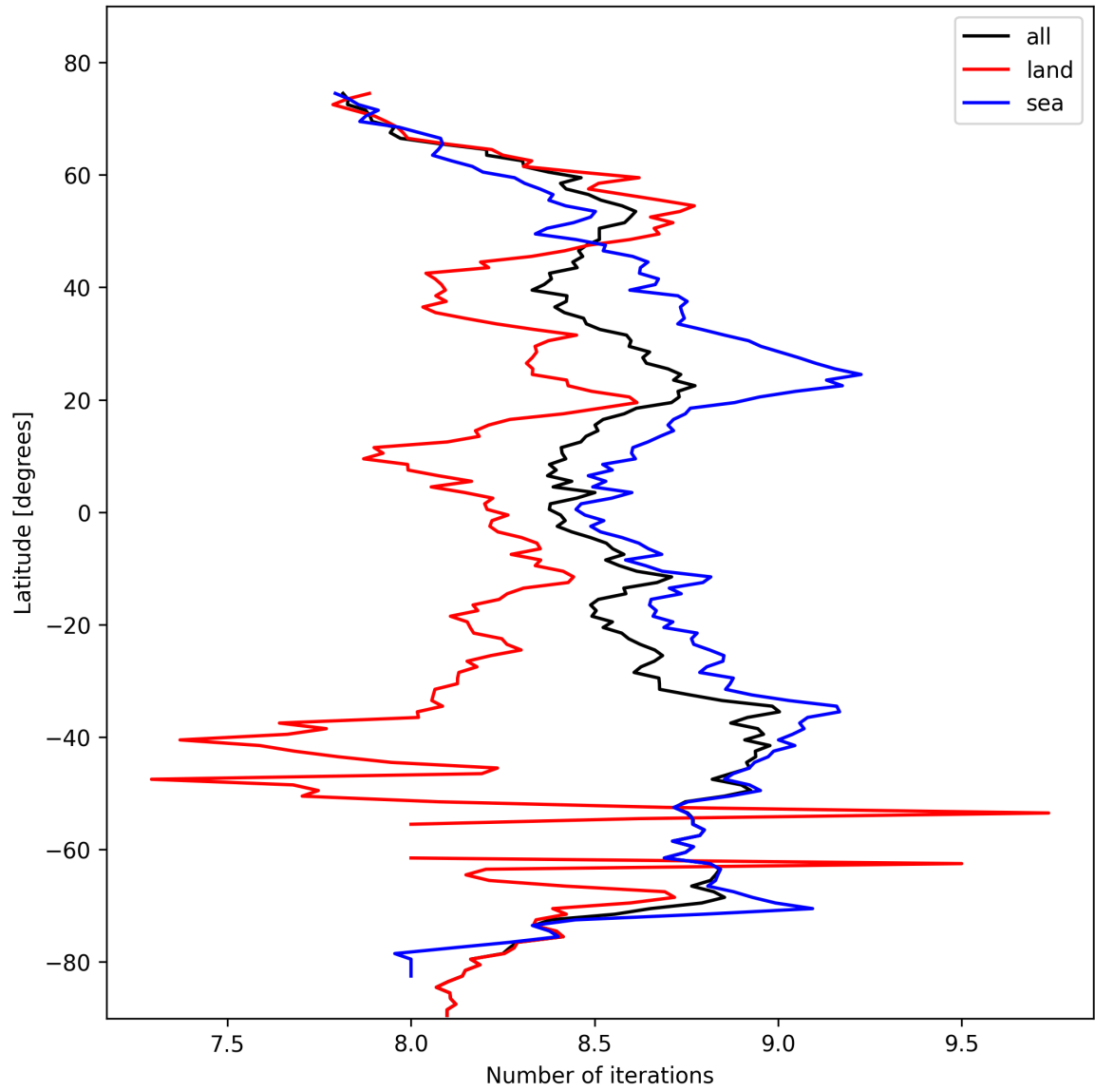
Figure 12: Zonal average of “Number of iterations” for 2025-02-21 to 2025-02-22.
