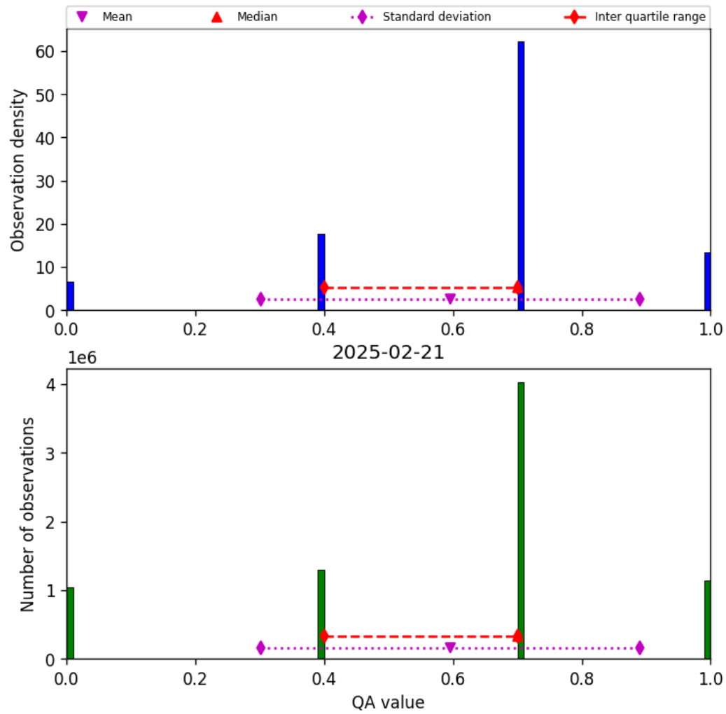
Figure 13: Histogram of “QA value” for 2025-02-21 to 2025-02-22
