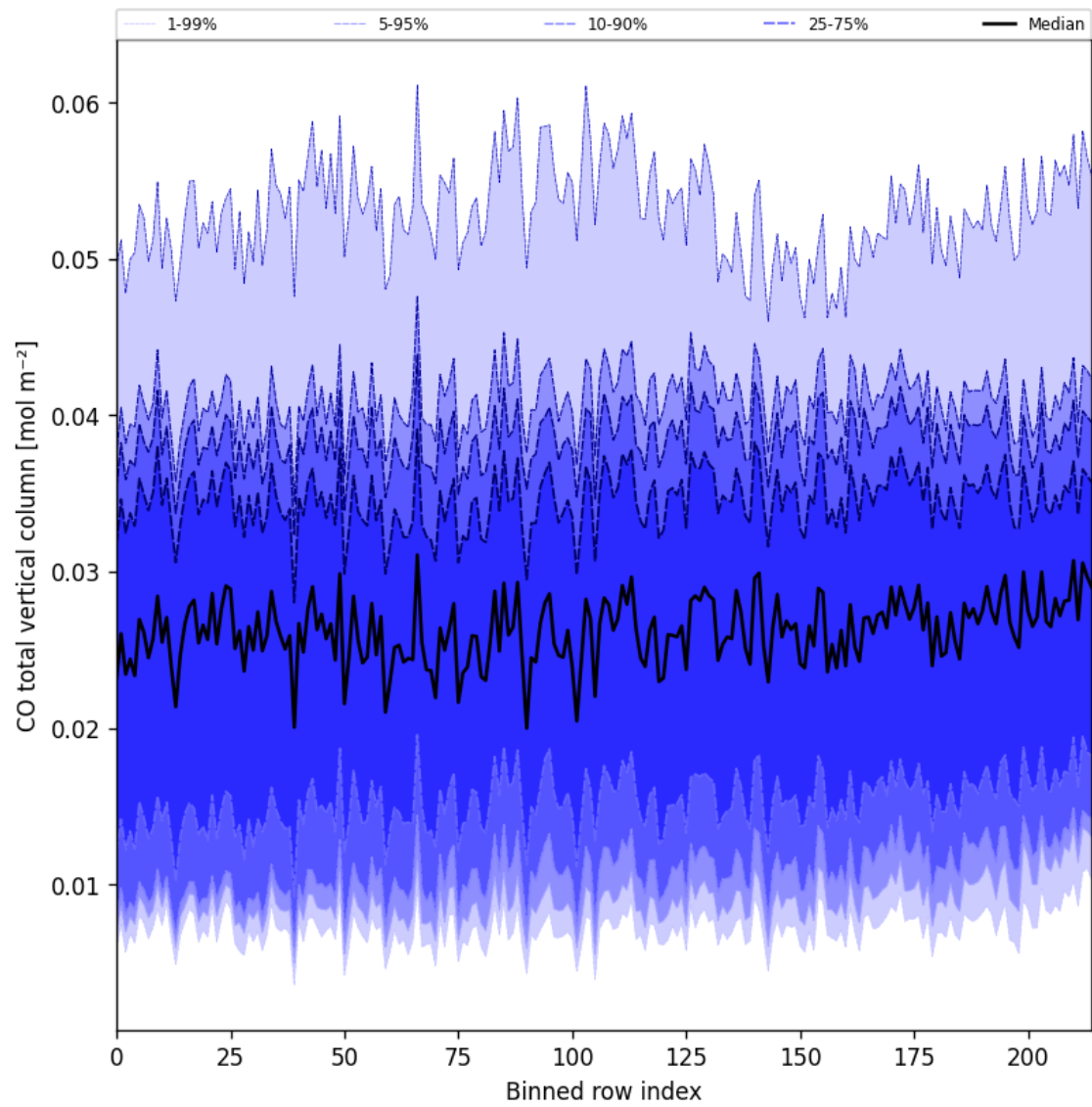
Figure 21: Along track statistics of “CO total vertical column” for 2025-02-21 to 2025-02-22
