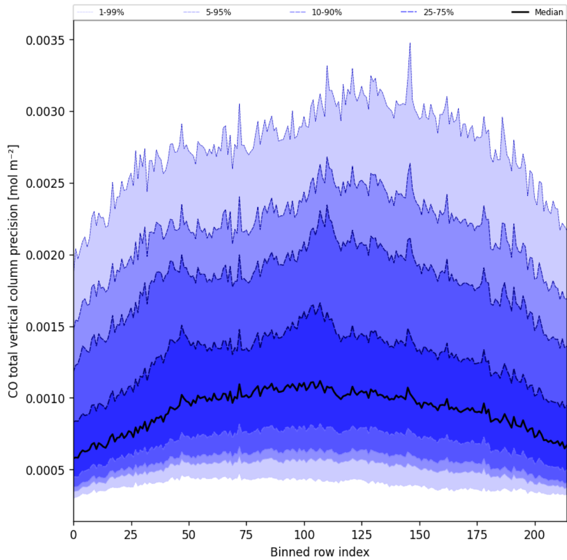
Figure 22: Along track statistics of “CO total vertical column precision” for 2025-02-21 to 2025-02-22
