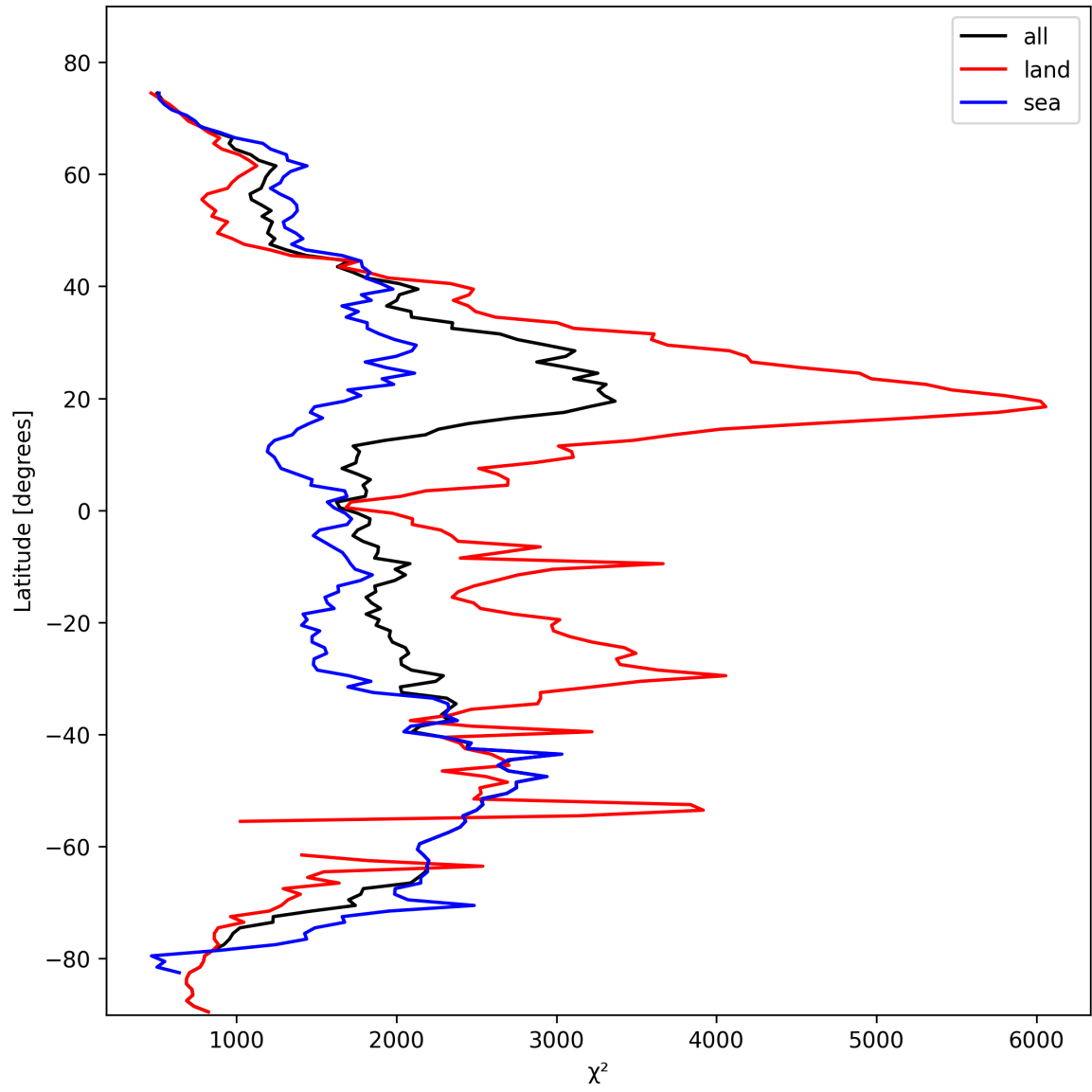
Figure 10: Zonal average of “ \chi^2 ” for 2025-02-21 to 2025-02-22.
