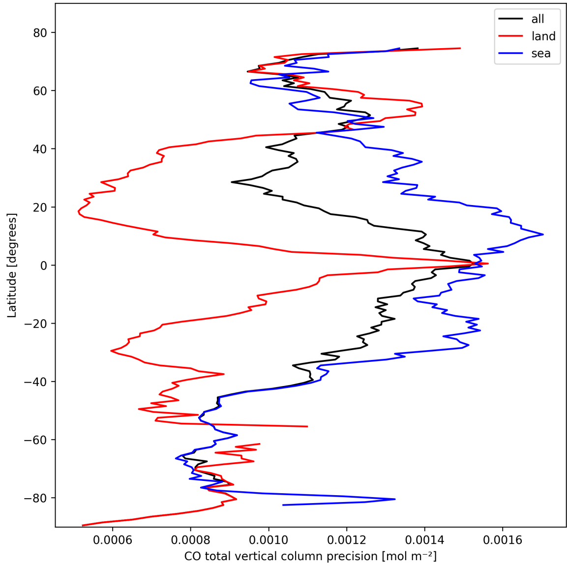
Figure 8: Zonal average of "CO total vertical column precision" for 2025-02-21 to 2025-02-22.
