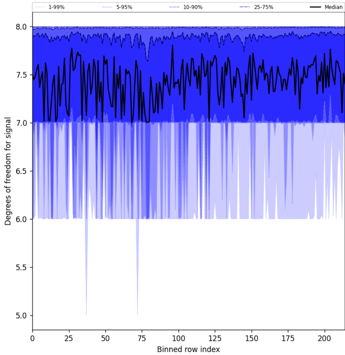
Figure 25: Along track statistics of “Degrees of freedom for signal” for 2025-02-21 to 2025-02-22
