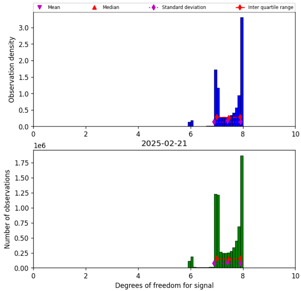
Figure 18: Histogram of “Degrees of freedom for signal” for 2025-02-21 to 2025-02-22
