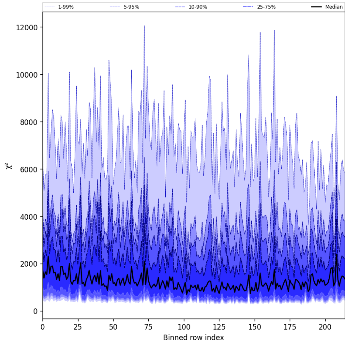
Figure 24: Along track statistics of “ \chi^2 ” for 2025-02-21 to 2025-02-22
