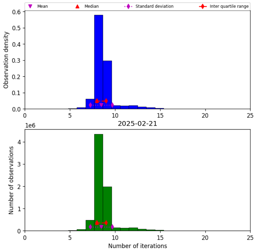
Figure 19: Histogram of “Number of iterations” for 2025-02-21 to 2025-02-22
