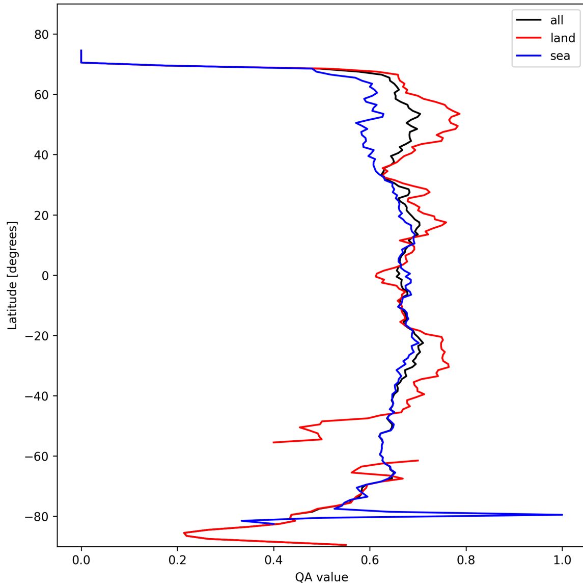
Figure 6: Zonal average of “QA value” for 2025-02-21 to 2025-02-22.
