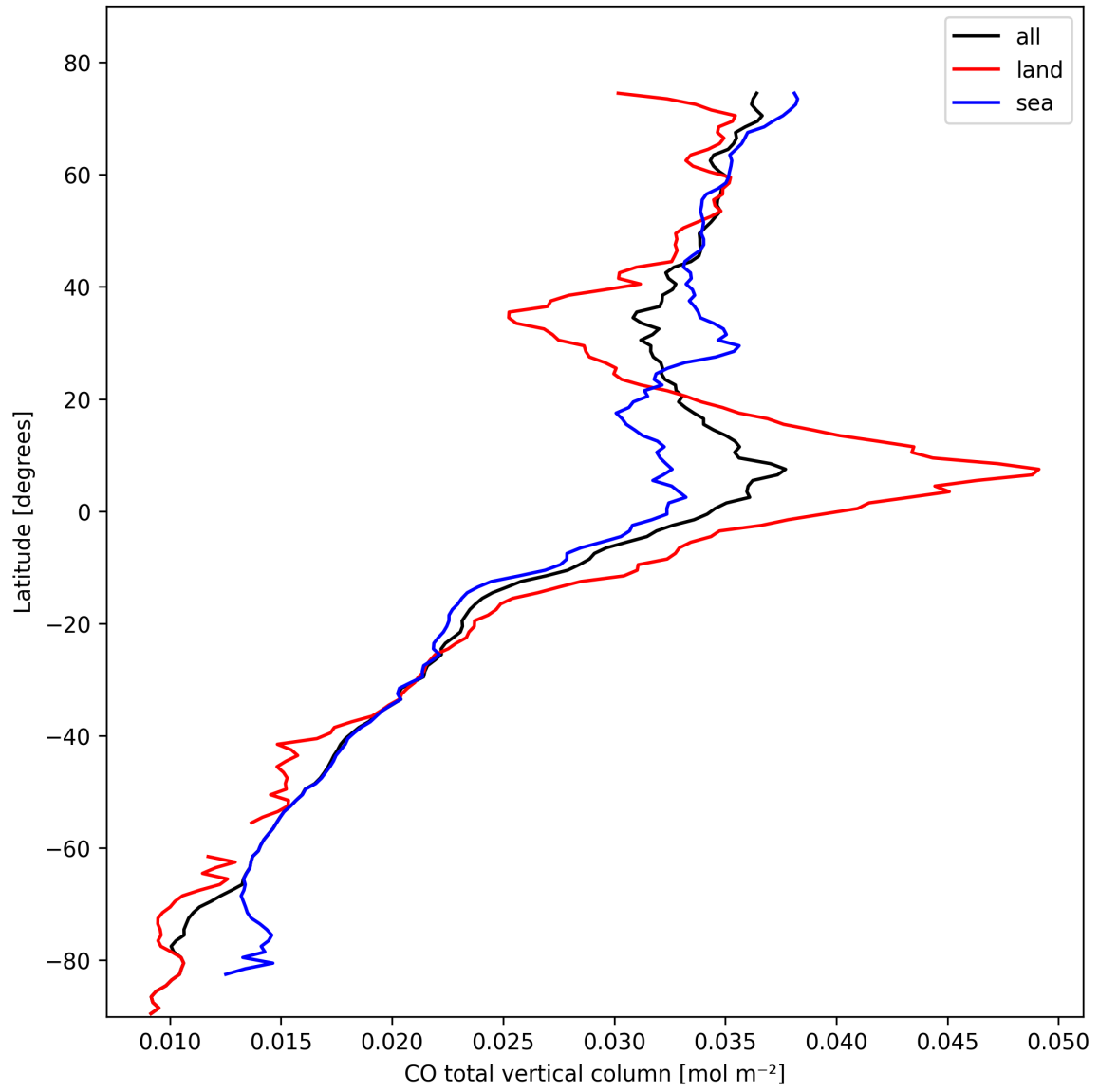
Figure 7: Zonal average of “CO total vertical column” for 2025-02-21 to 2025-02-22.
