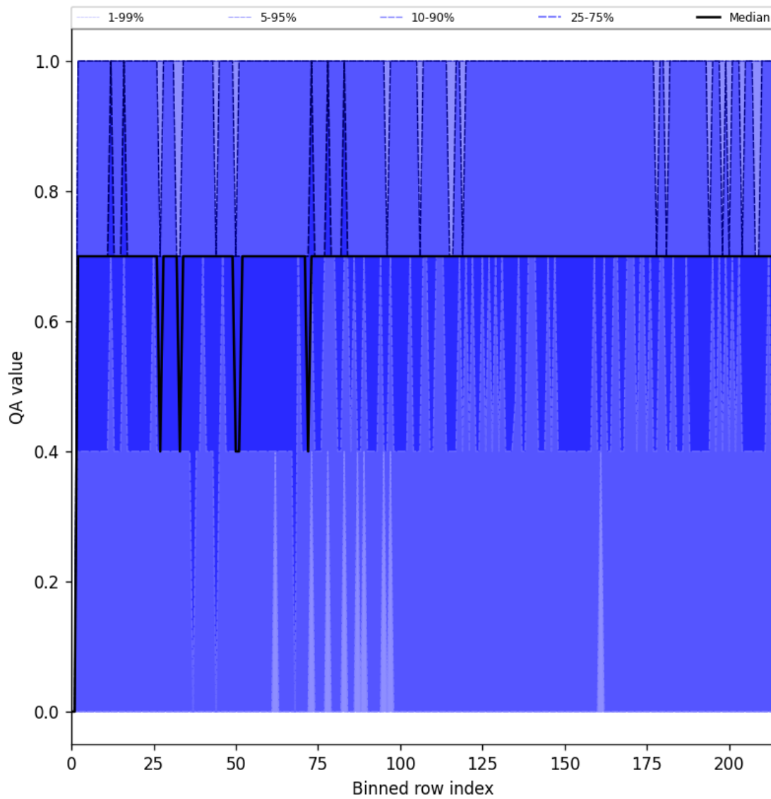
Figure 20: Along track statistics of “QA value” for 2025-02-21 to 2025-02-22
