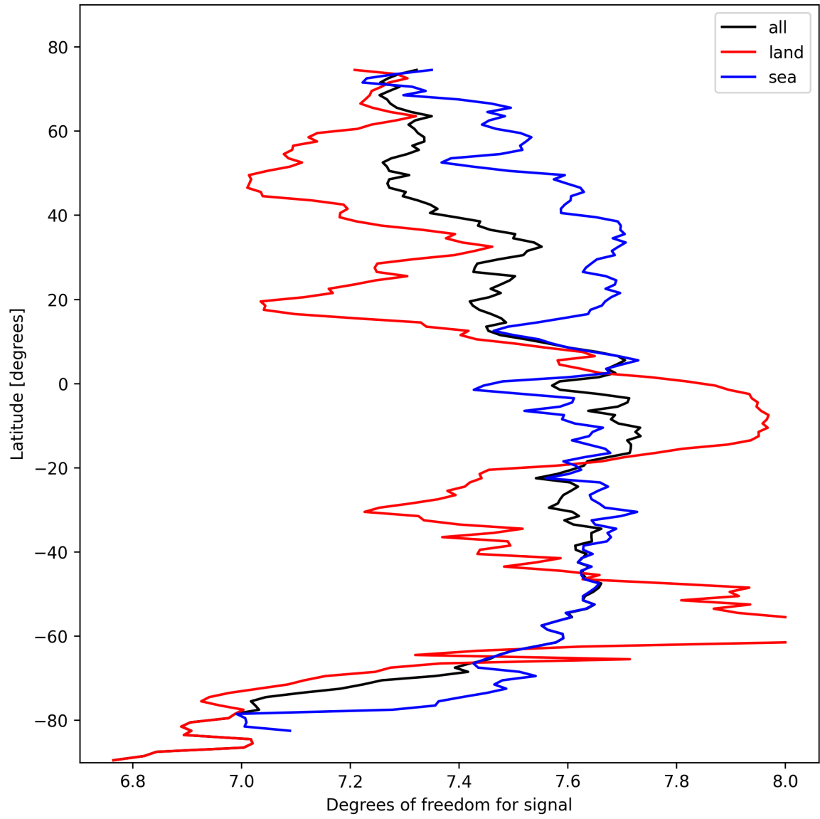
Figure 11: Zonal average of “Degrees of freedom for signal” for 2025-02-21 to 2025-02-22.
