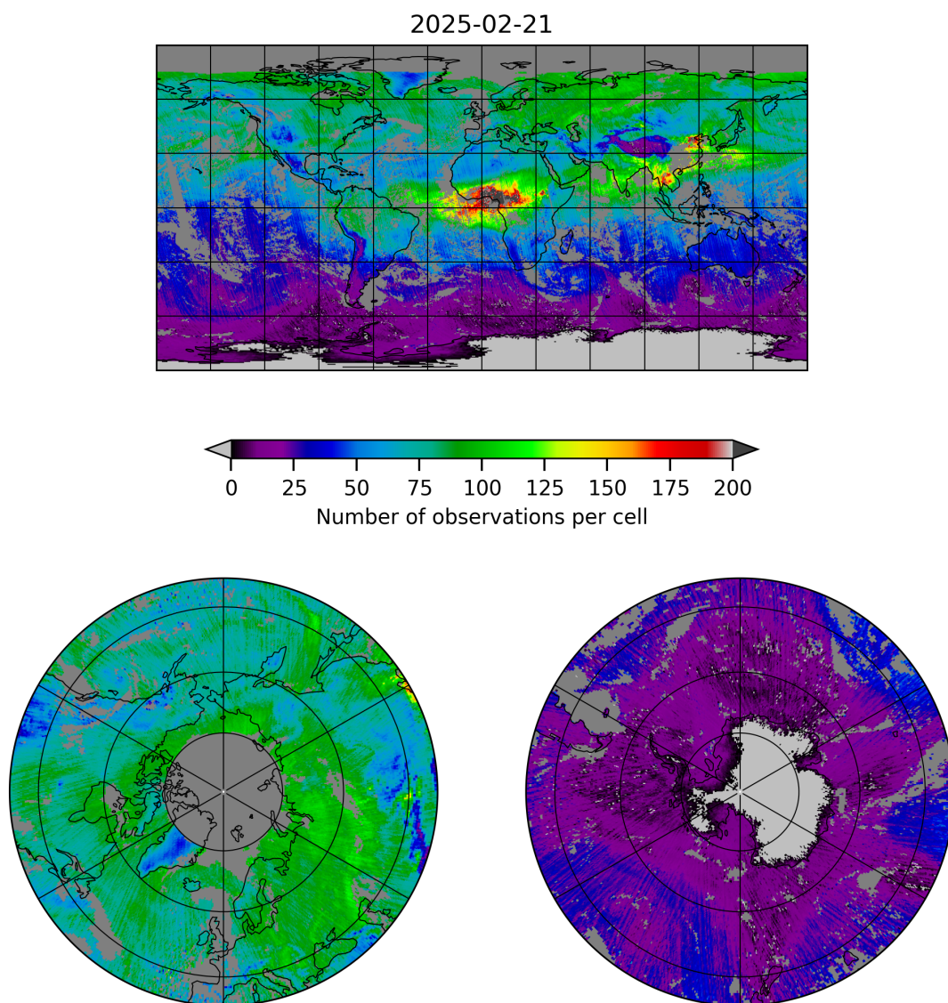
Figure 5: Map of the number of observations for 2025-02-21 to 2025-02-22
