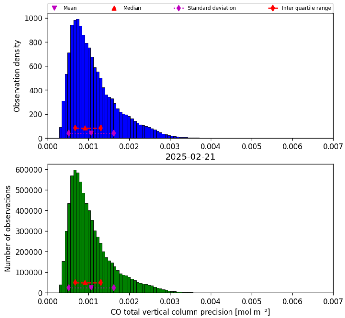
Figure 15: Histogram of “CO total vertical column precision” for 2025-02-21 to 2025-02-22
