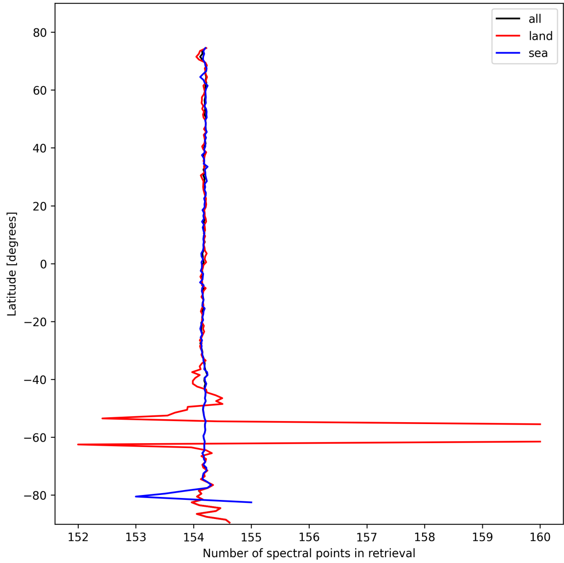
Figure 9: Zonal average of “Number of spectral points in retrieval” for 2025-02-21 to 2025-02-22.
