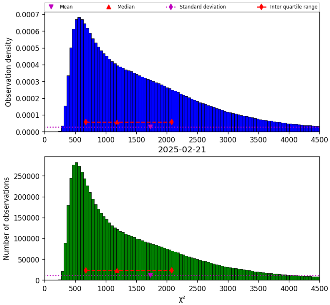
Figure 17: Histogram of “ \chi^2 ” for 2025-02-21 to 2025-02-22
