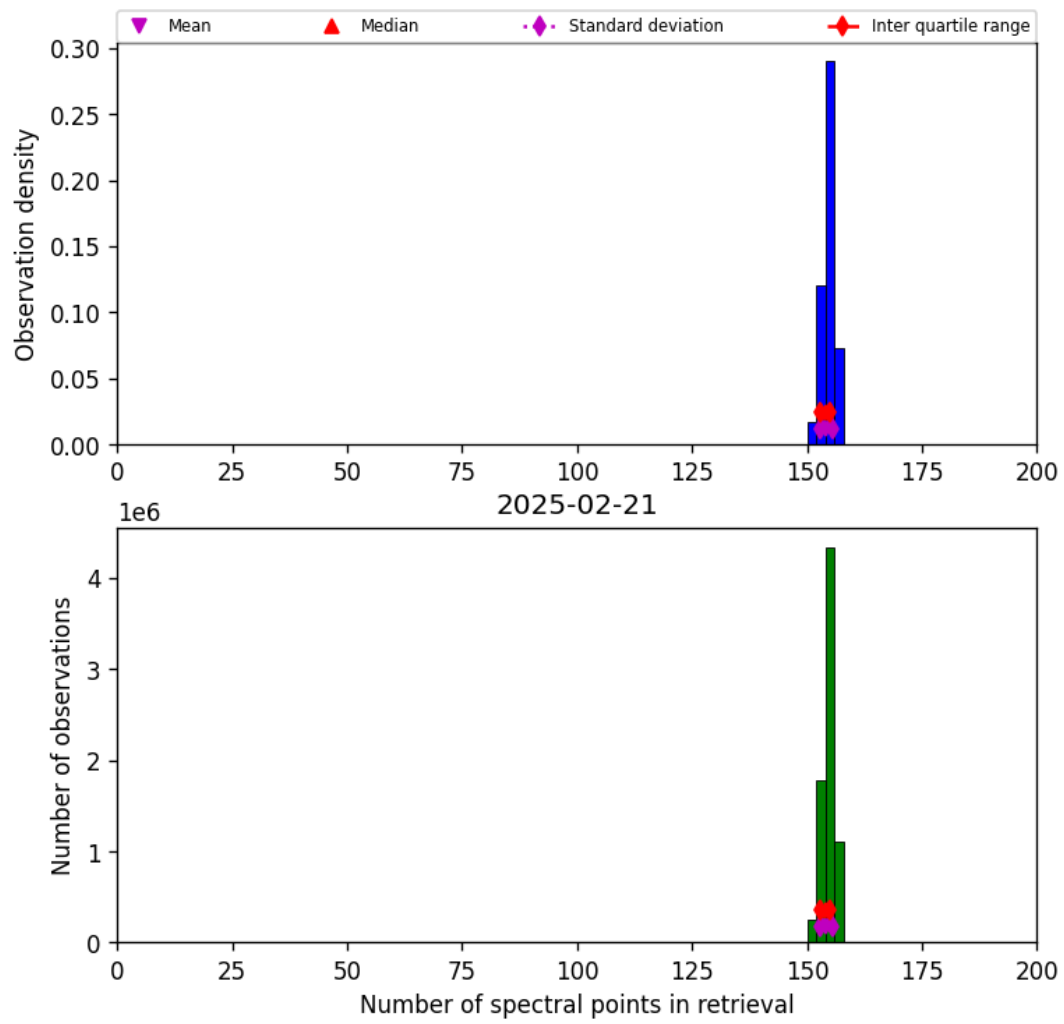
Figure 16: Histogram of “Number of spectral points in retrieval” for 2025-02-21 to 2025-02-22
