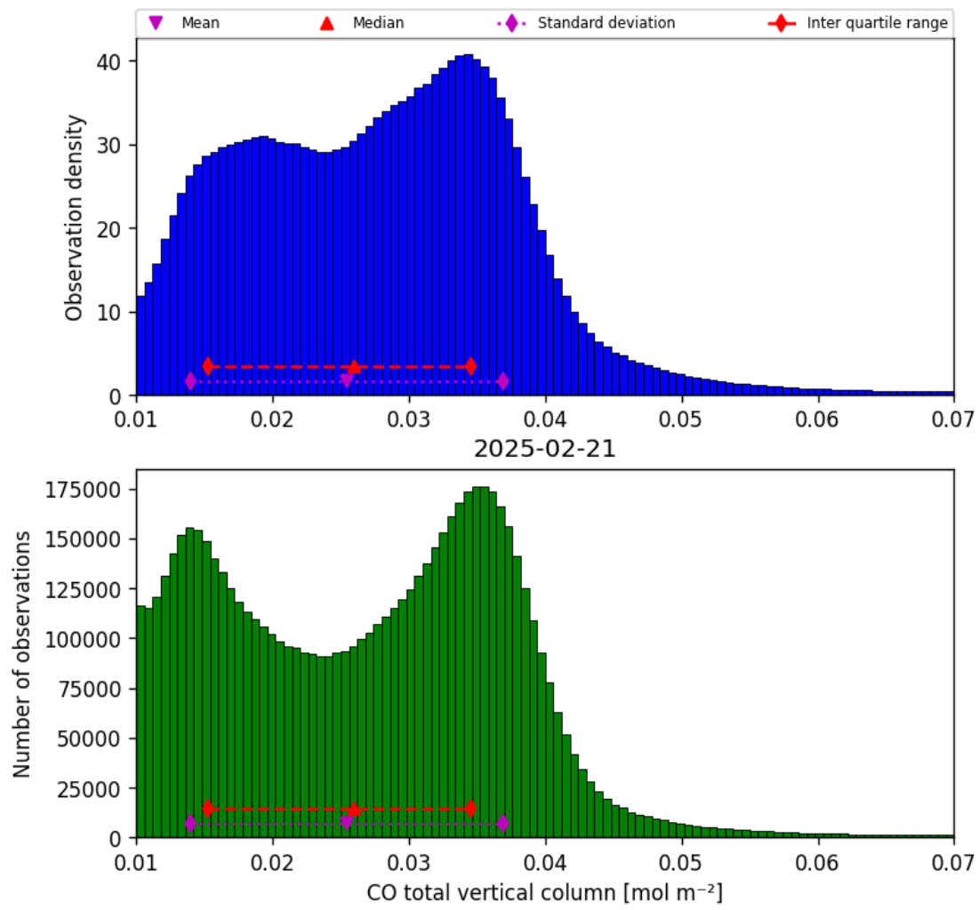
Figure 14: Histogram of “CO total vertical column” for 2025-02-21 to 2025-02-22
