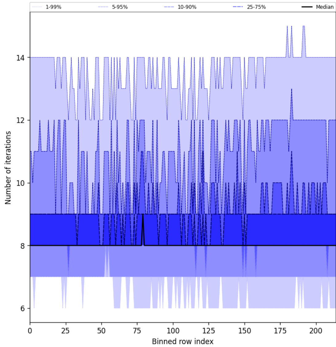
Figure 26: Along track statistics of “Number of iterations” for 2025-02-21 to 2025-02-22
