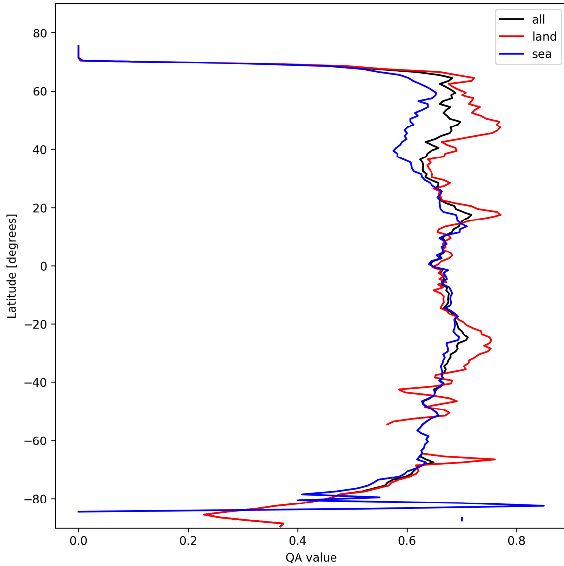
Figure 6: Zonal average of “QA value” for 2025-02-22 to 2025-02-22.
