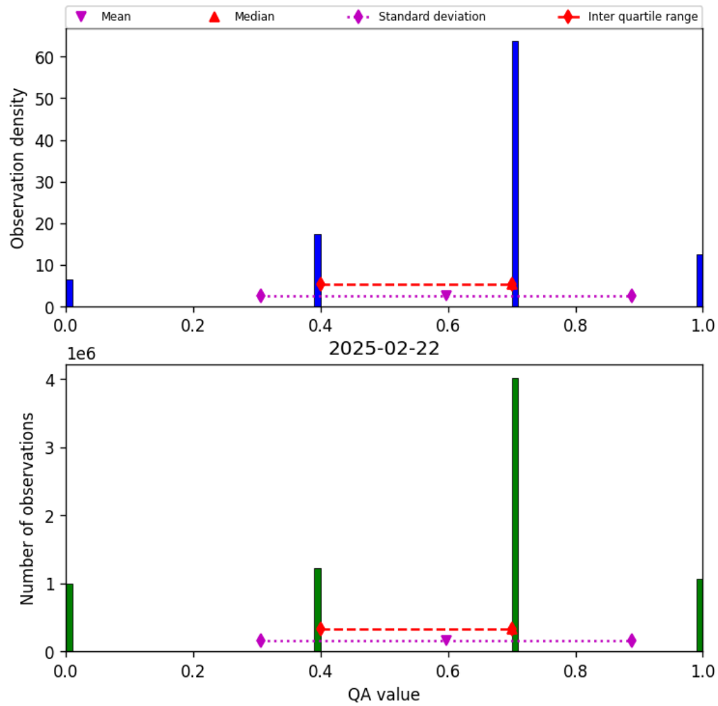
Figure 13: Histogram of “QA value” for 2025-02-22 to 2025-02-22
