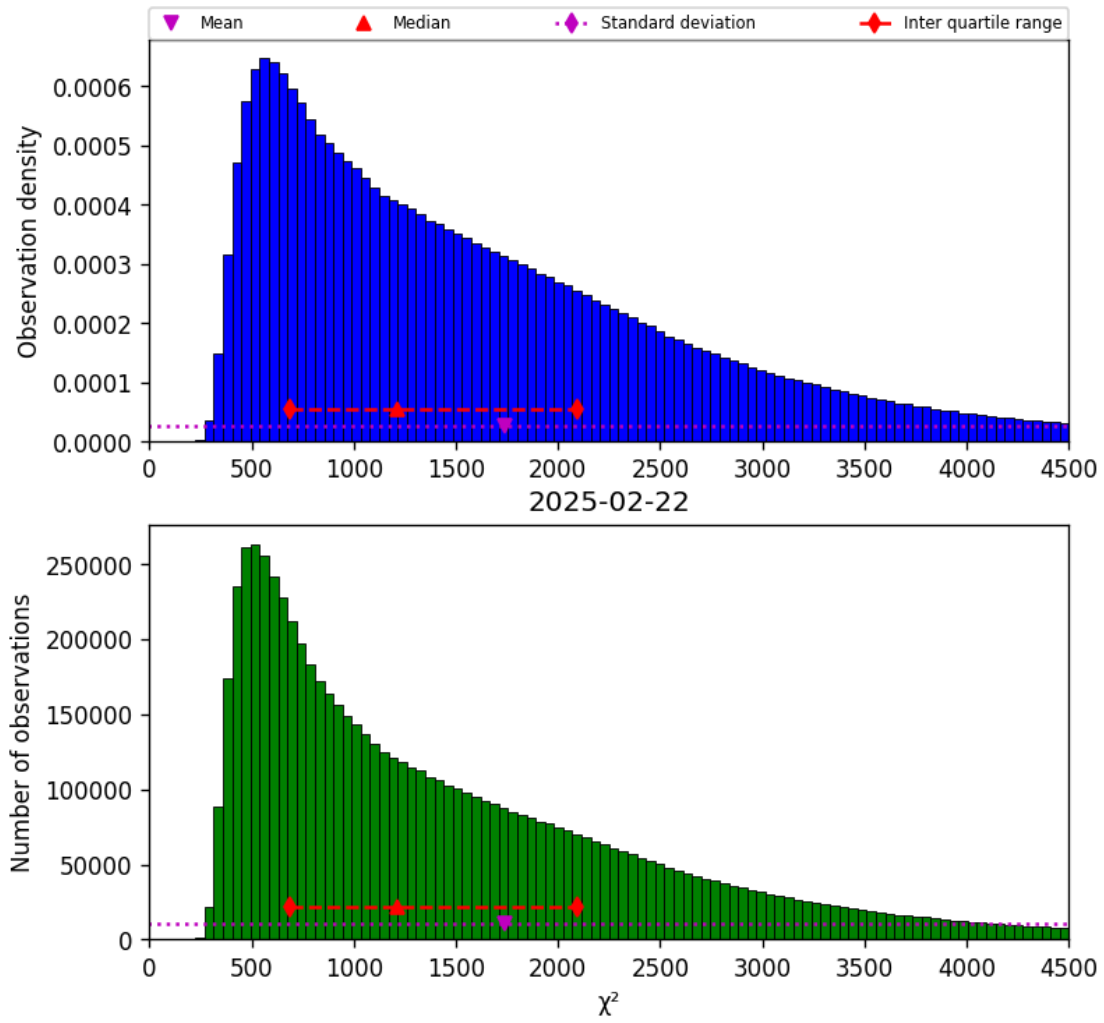
Figure 17: Histogram of “ \chi^2 ” for 2025-02-22 to 2025-02-22
