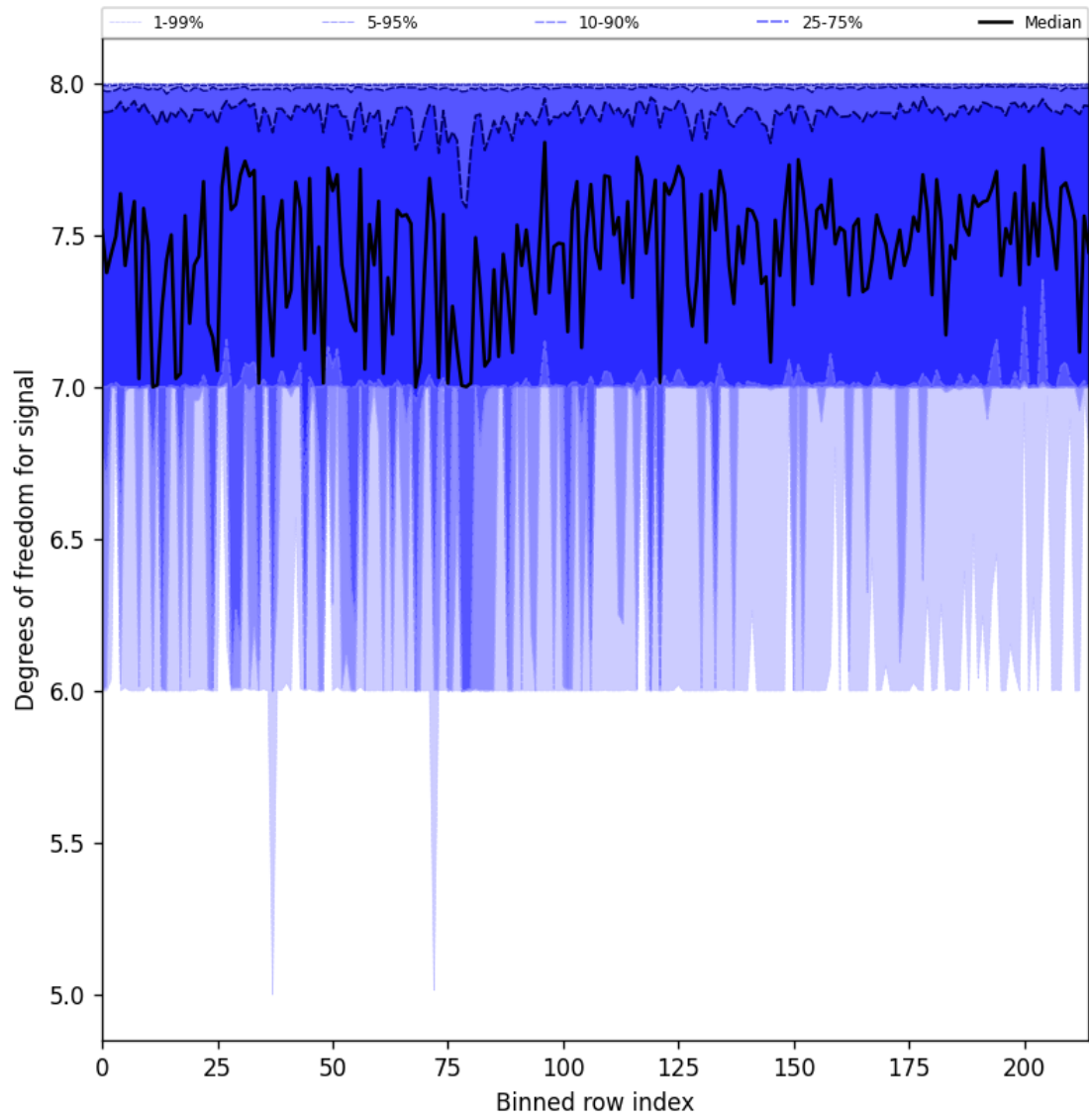
Figure 25: Along track statistics of “Degrees of freedom for signal” for 2025-02-22 to 2025-02-22
