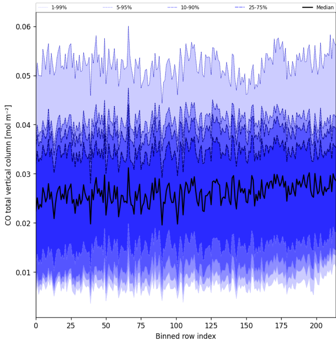
Figure 21: Along track statistics of “CO total vertical column” for 2025-02-22 to 2025-02-22
