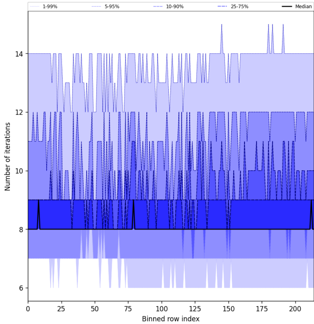
Figure 26: Along track statistics of “Number of iterations” for 2025-02-22 to 2025-02-22
