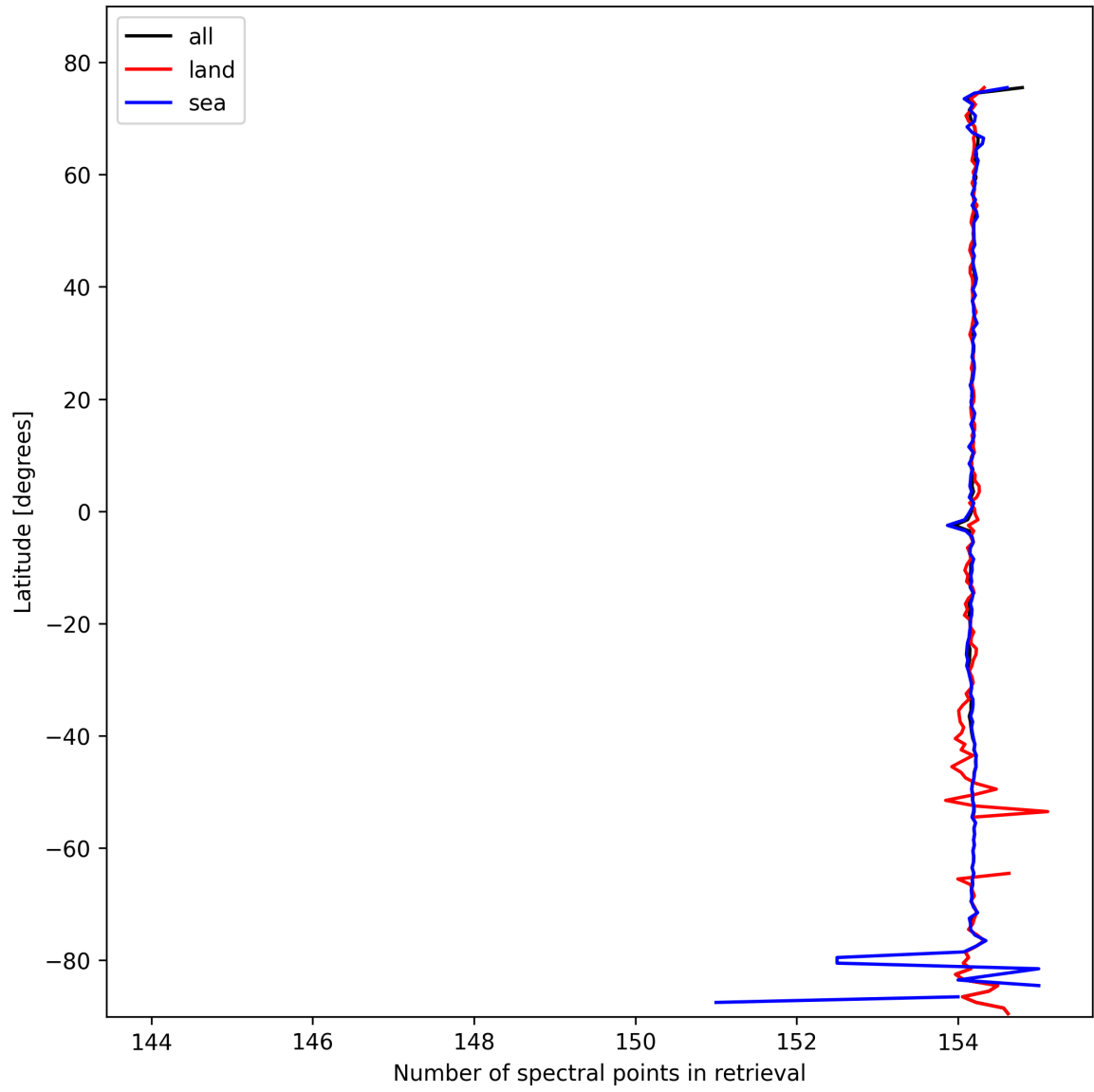
Figure 9: Zonal average of “Number of spectral points in retrieval” for 2025-02-22 to 2025-02-22.
