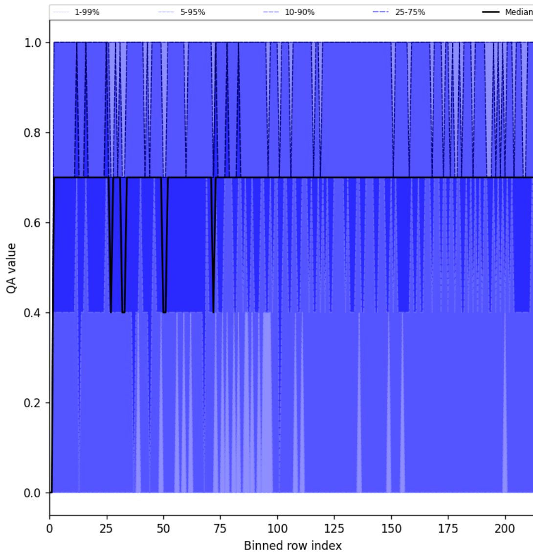
Figure 20: Along track statistics of “QA value” for 2025-02-22 to 2025-02-22
