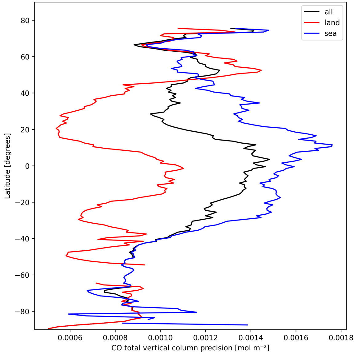
Figure 8: Zonal average of “CO total vertical column precision” for 2025-02-22 to 2025-02-22.
