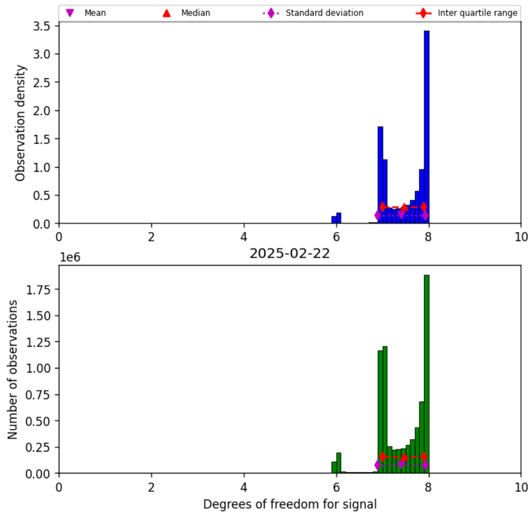
Figure 18: Histogram of “Degrees of freedom for signal” for 2025-02-22 to 2025-02-22
