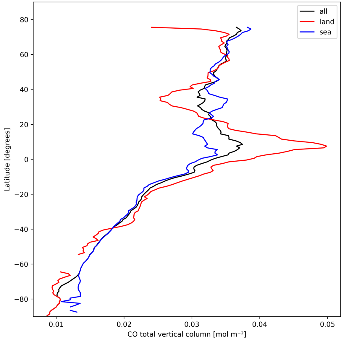
Figure 7: Zonal average of “CO total vertical column” for 2025-02-22 to 2025-02-22.
