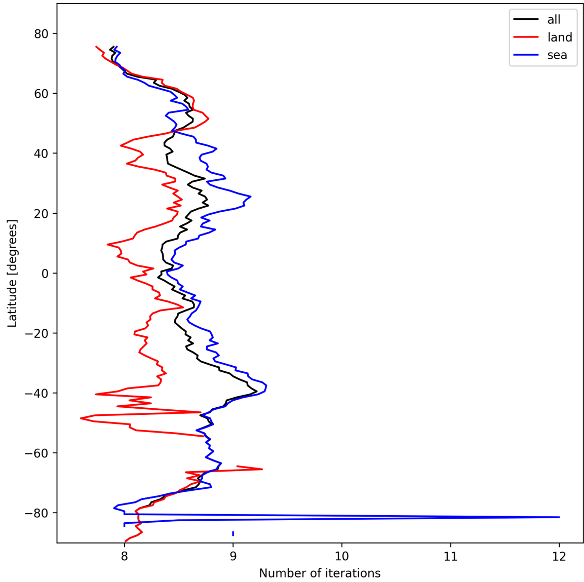
Figure 12: Zonal average of “Number of iterations” for 2025-02-22 to 2025-02-22.
