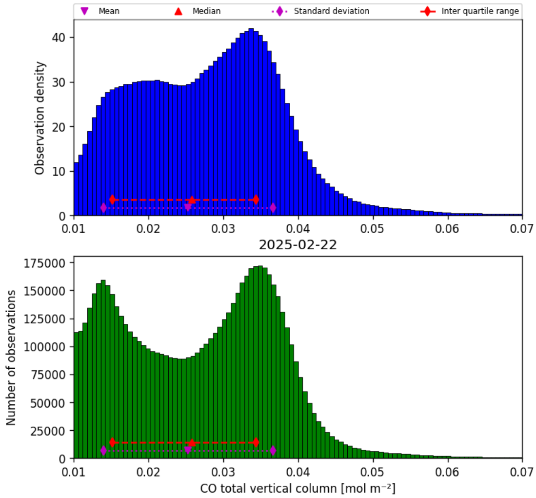
Figure 14: Histogram of “CO total vertical column” for 2025-02-22 to 2025-02-22
