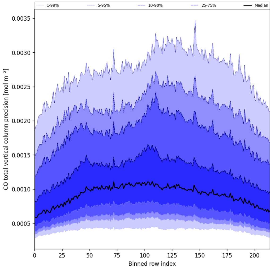
Figure 22: Along track statistics of “CO total vertical column precision” for 2025-02-22 to 2025-02-22
