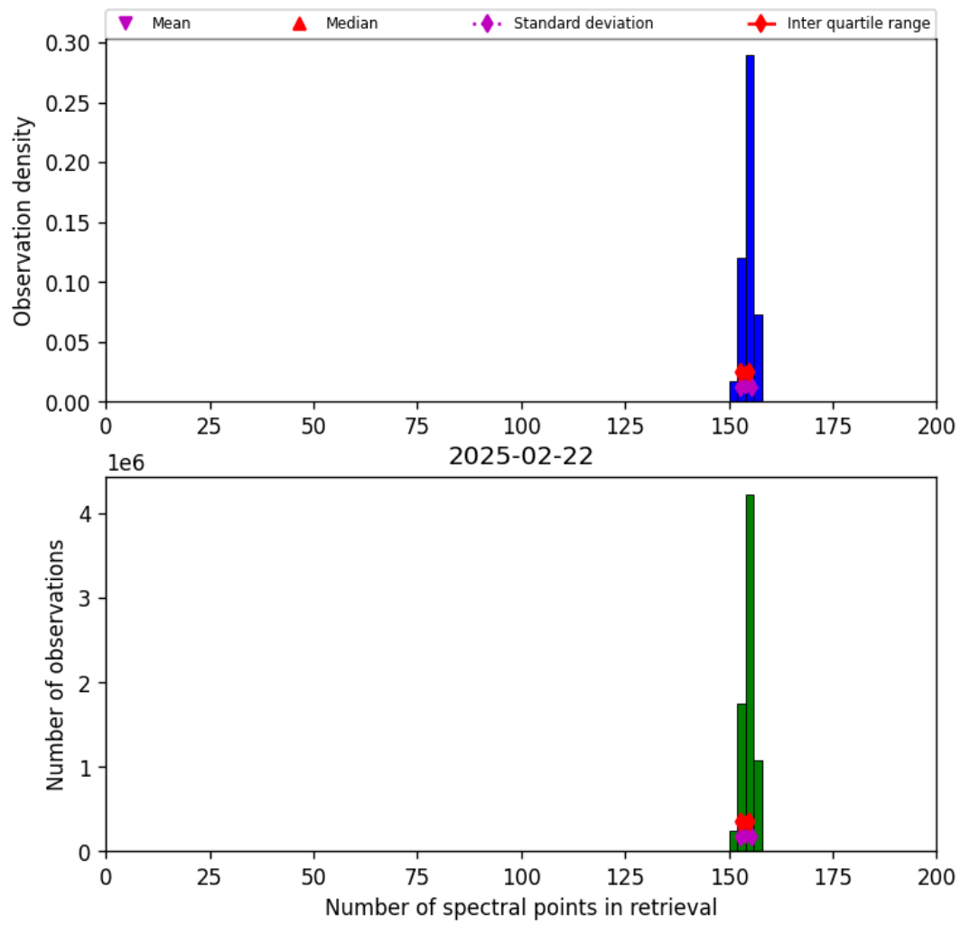
Figure 16: Histogram of “Number of spectral points in retrieval” for 2025-02-22 to 2025-02-22
