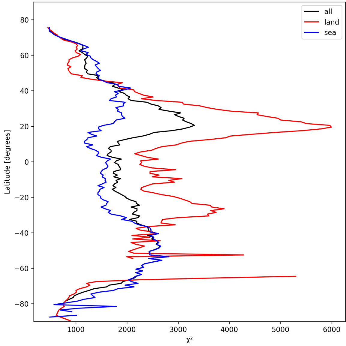
Figure 10: Zonal average of “ \chi^2 ” for 2025-02-22 to 2025-02-22.
