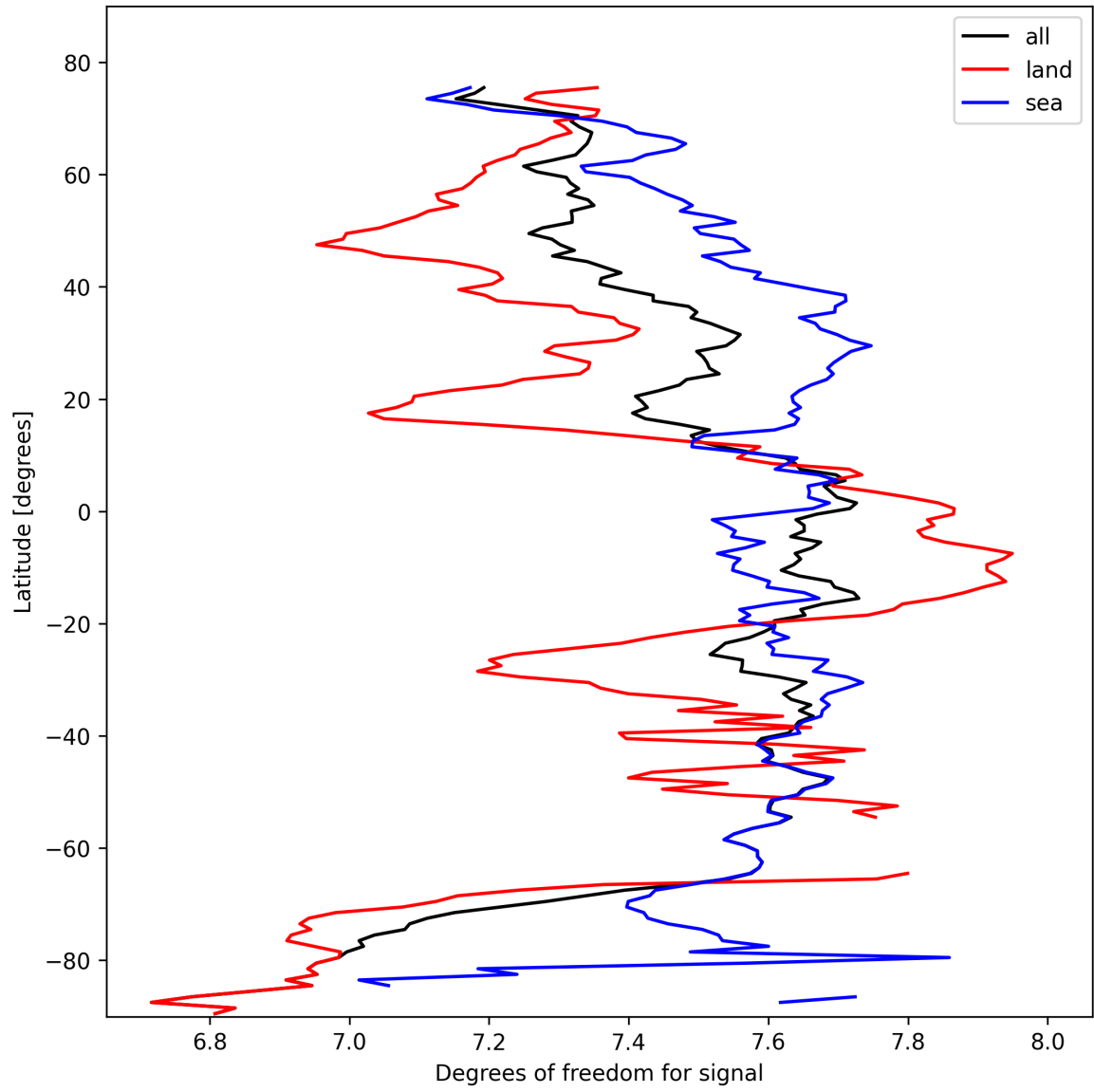
Figure 11: Zonal average of “Degrees of freedom for signal” for 2025-02-22 to 2025-02-22.
