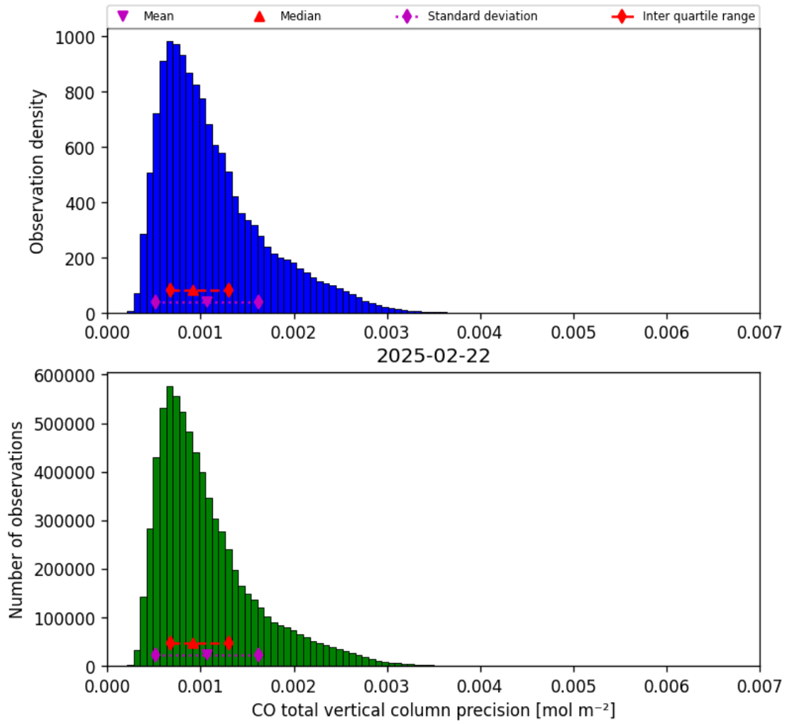
Figure 15: Histogram of “CO total vertical column precision” for 2025-02-22 to 2025-02-22
