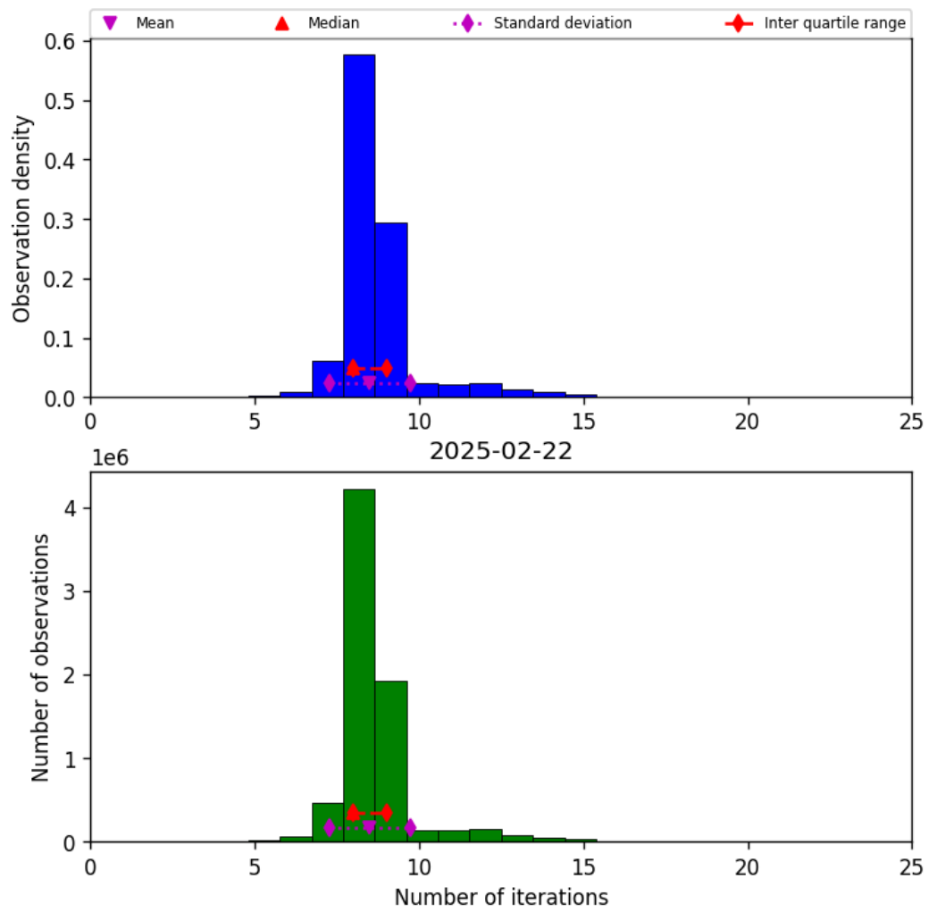
Figure 19: Histogram of “Number of iterations” for 2025-02-22 to 2025-02-22
