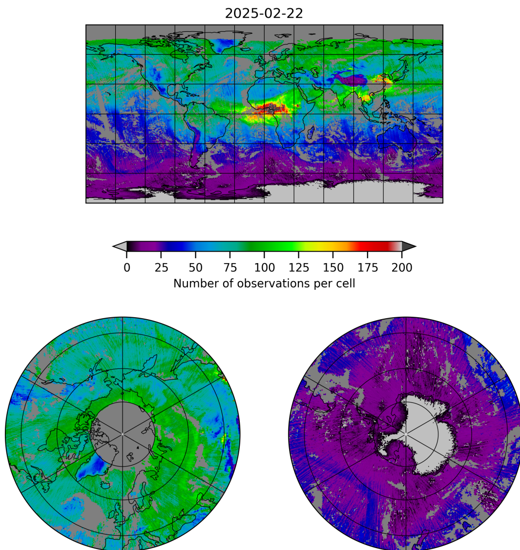
Figure 5: Map of the number of observations for 2025-02-22 to 2025-02-22
