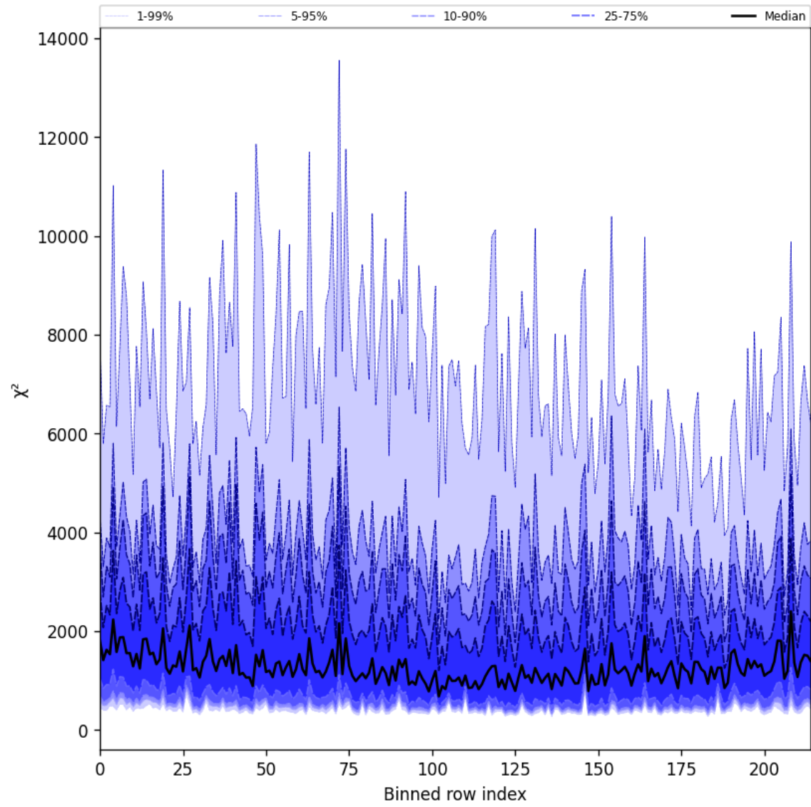
Figure 24: Along track statistics of “ \chi^2 ” for 2025-02-22 to 2025-02-22
