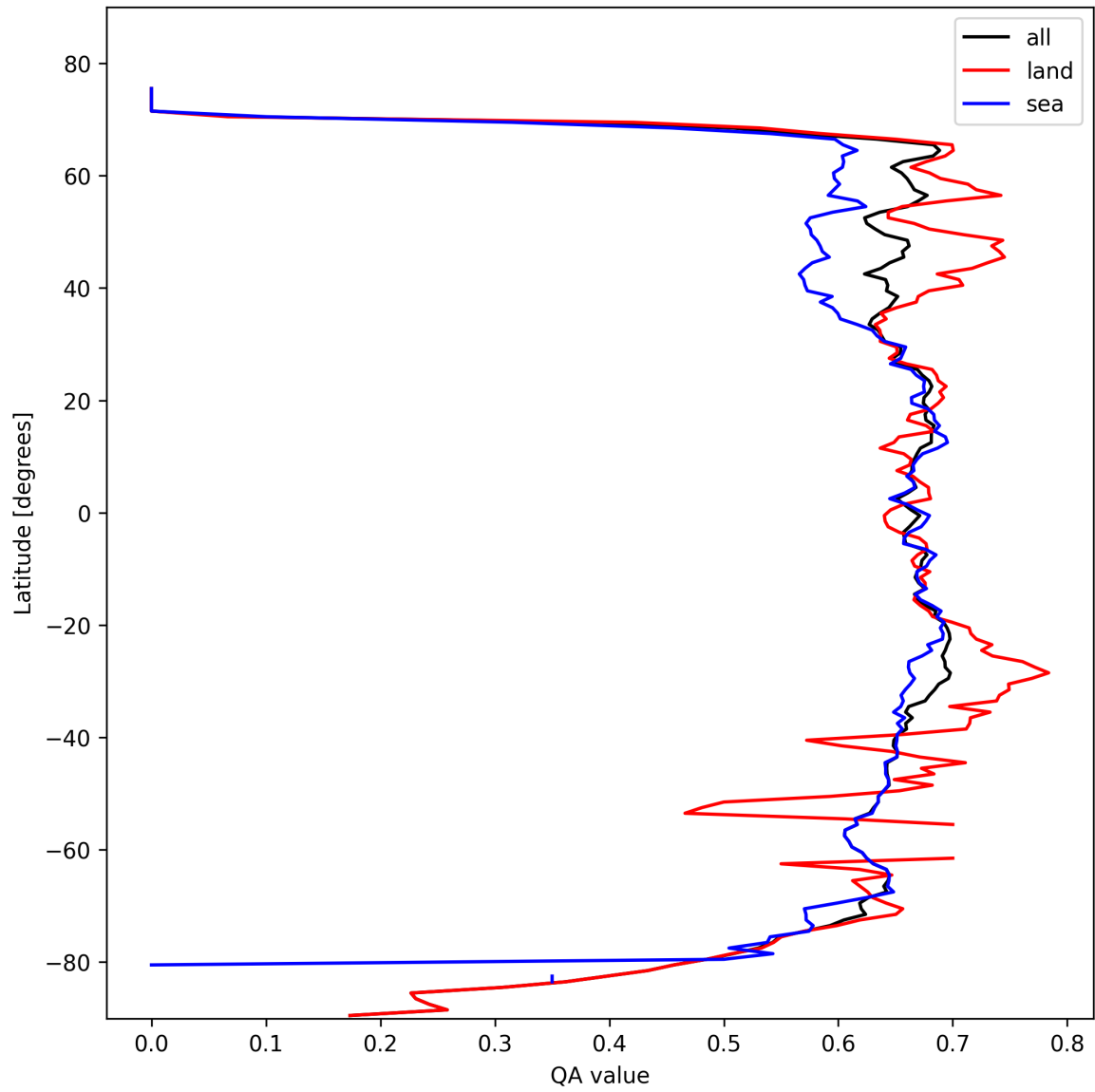
Figure 6: Zonal average of “QA value” for 2025-02-23 to 2025-02-24.
