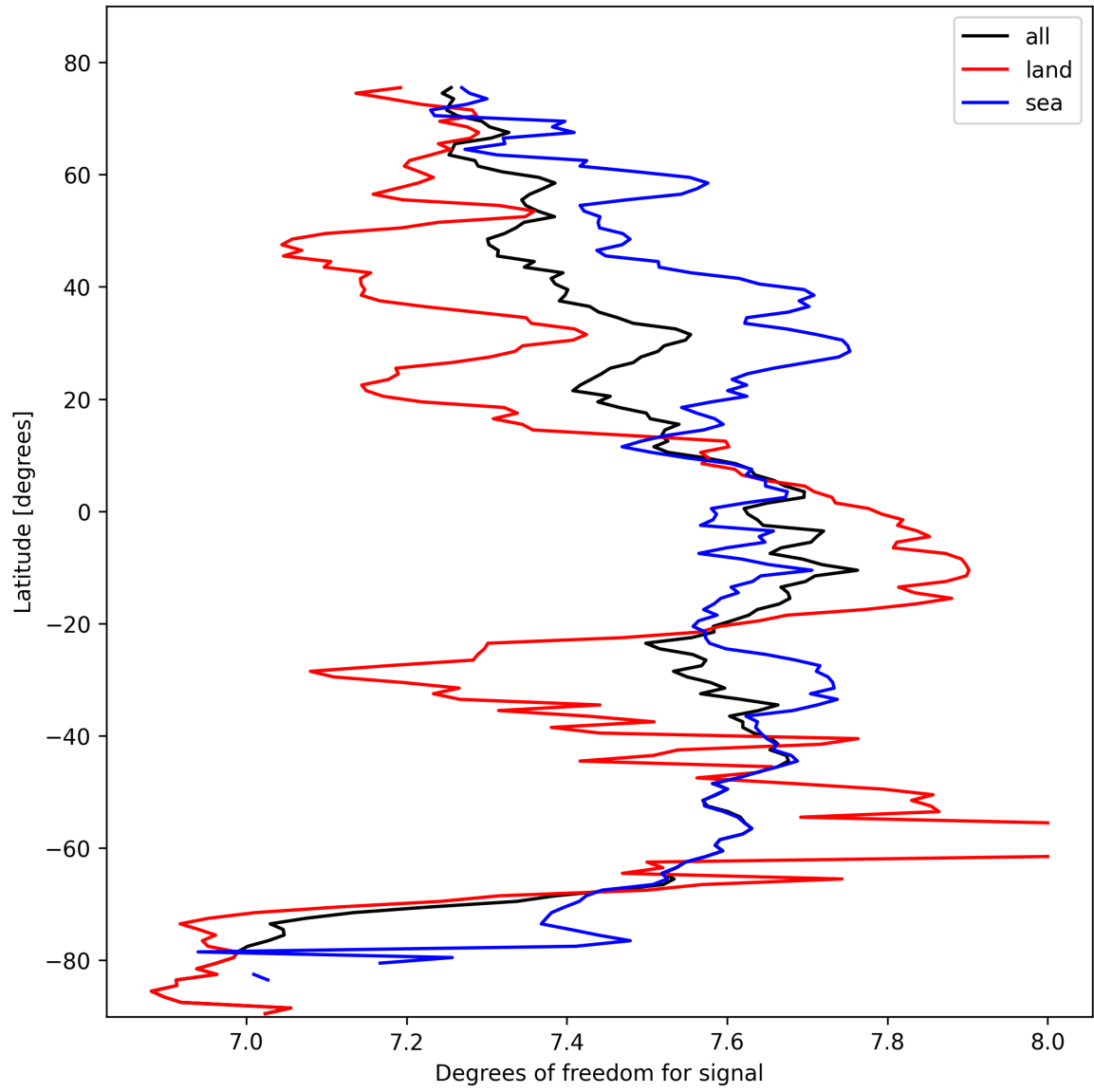
Figure 11: Zonal average of “Degrees of freedom for signal” for 2025-02-23 to 2025-02-24.
