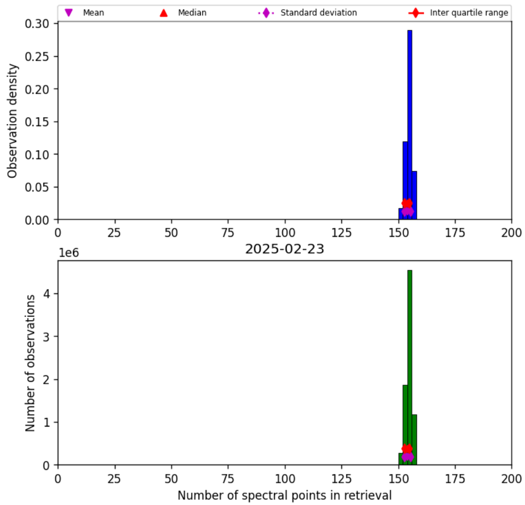
Figure 16: Histogram of “Number of spectral points in retrieval” for 2025-02-23 to 2025-02-24
