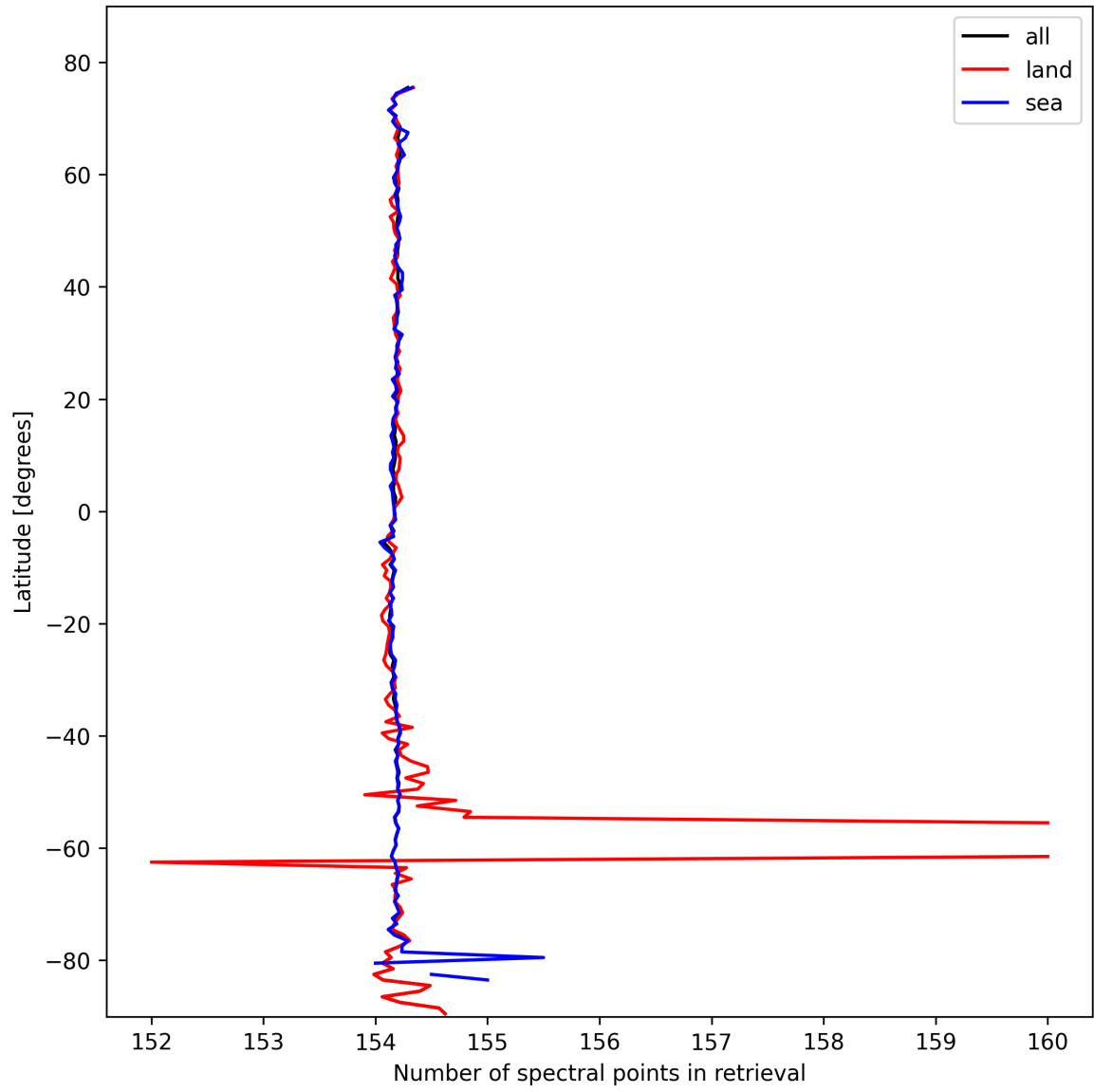
Figure 9: Zonal average of “Number of spectral points in retrieval” for 2025-02-23 to 2025-02-24.
