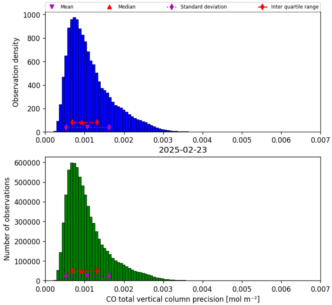
Figure 15: Histogram of “CO total vertical column precision” for 2025-02-23 to 2025-02-24
