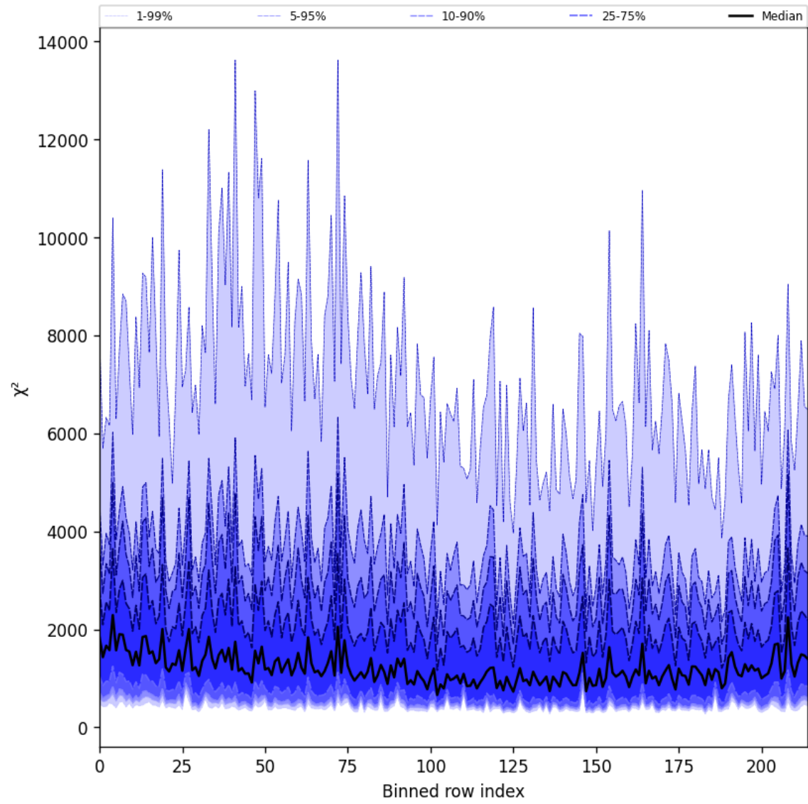
Figure 24: Along track statistics of “ \chi^2 ” for 2025-02-23 to 2025-02-24
