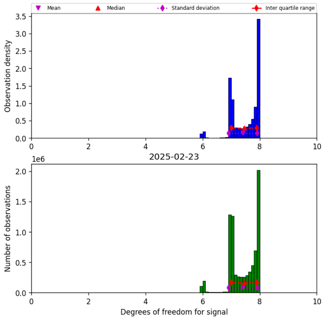
Figure 18: Histogram of “Degrees of freedom for signal” for 2025-02-23 to 2025-02-24
