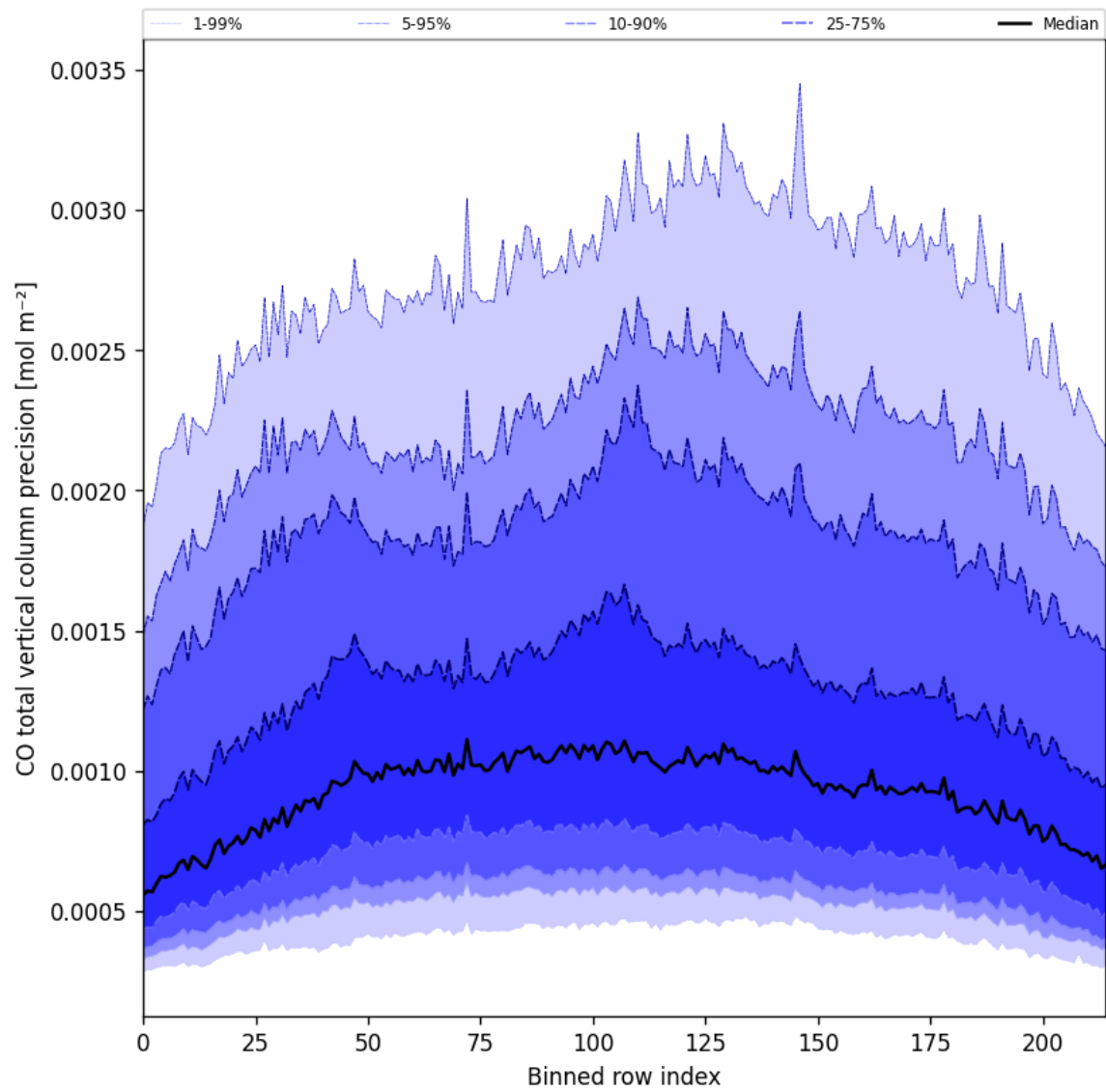
Figure 22: Along track statistics of “CO total vertical column precision” for 2025-02-23 to 2025-02-24
