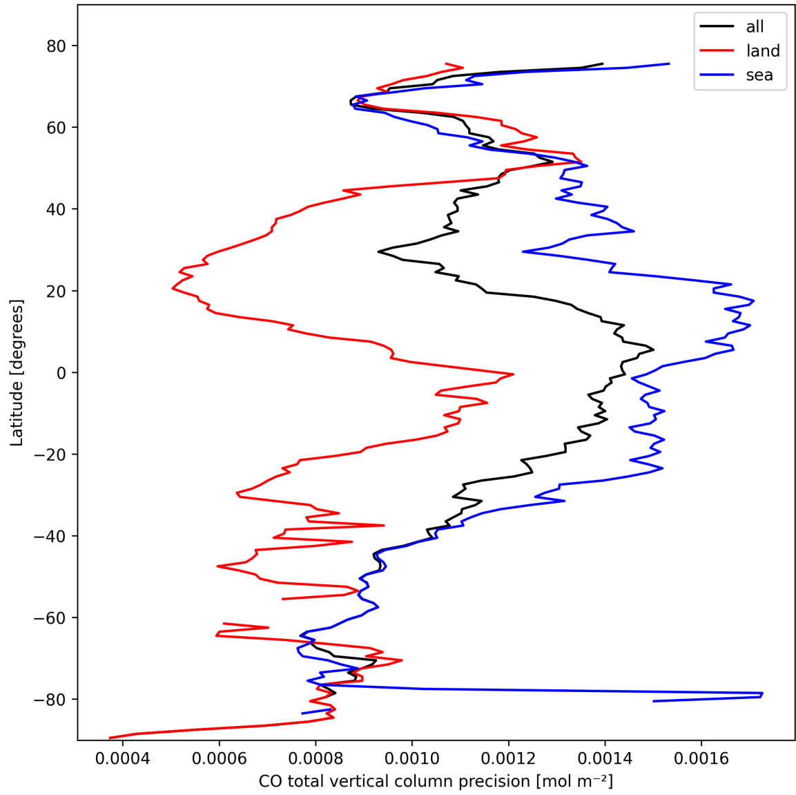
Figure 8: Zonal average of “CO total vertical column precision” for 2025-02-23 to 2025-02-24.
