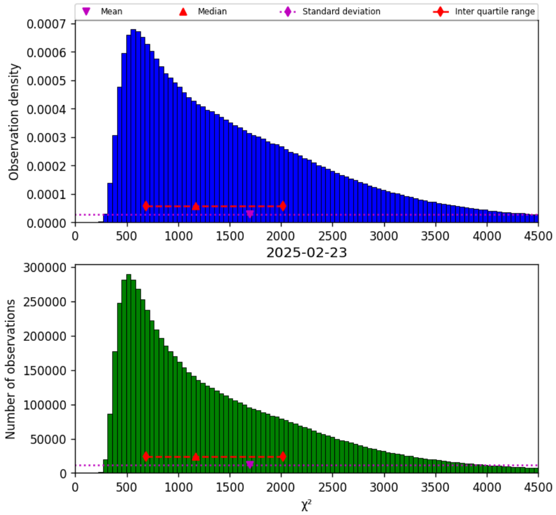
Figure 17: Histogram of “ \chi^2 ” for 2025-02-23 to 2025-02-24
