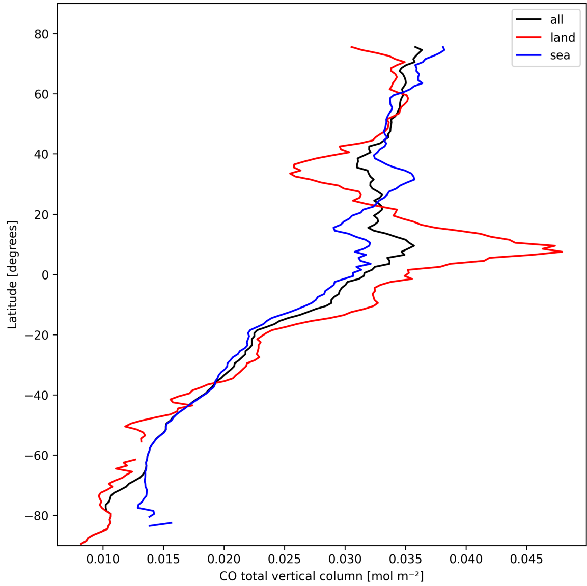
Figure 7: Zonal average of “CO total vertical column” for 2025-02-23 to 2025-02-24.
