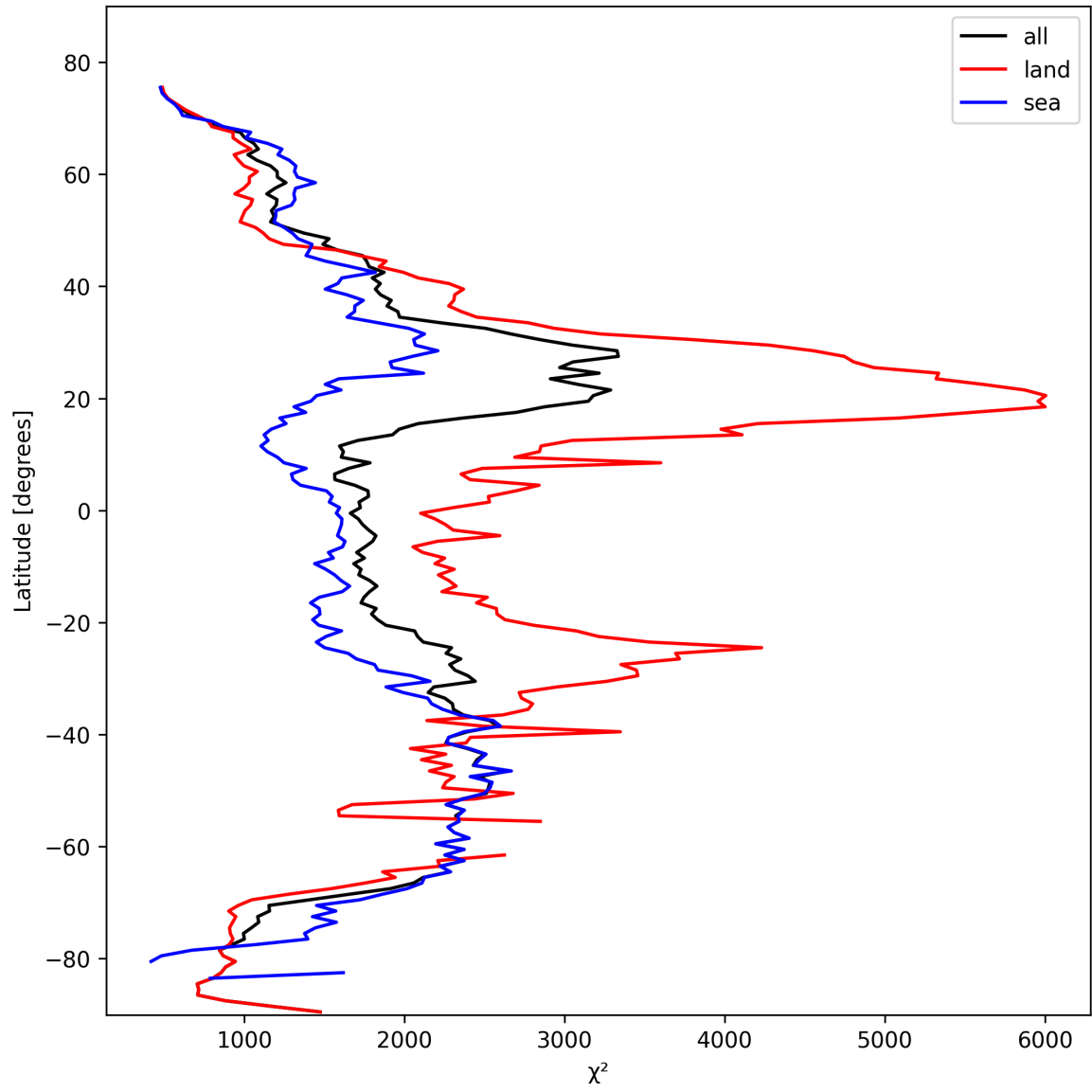
Figure 10: Zonal average of “ \chi^2 ” for 2025-02-23 to 2025-02-24.
