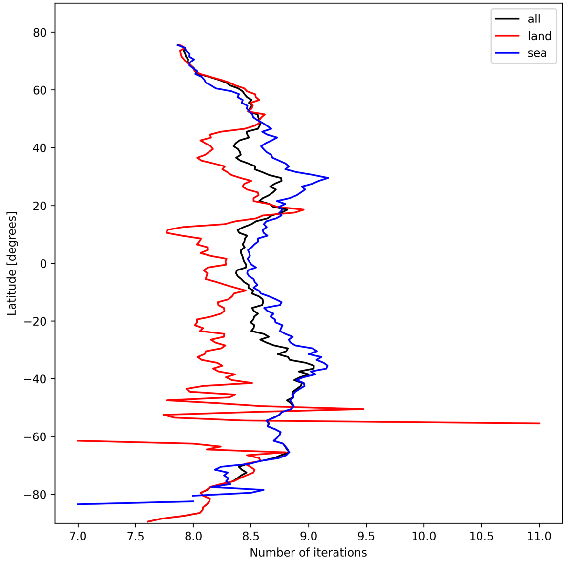
Figure 12: Zonal average of “Number of iterations” for 2025-02-23 to 2025-02-24.
