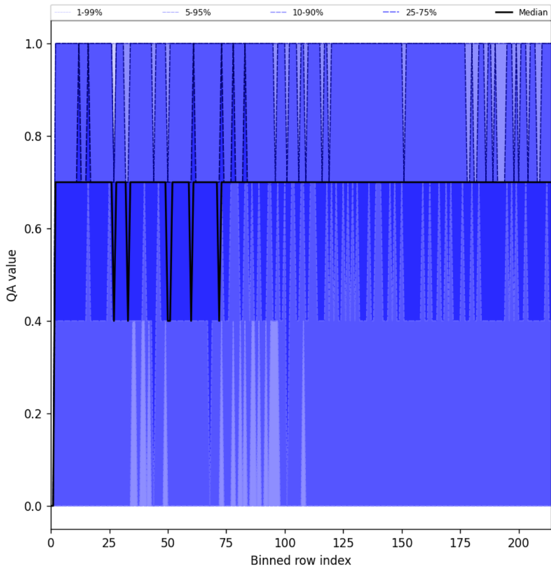
Figure 20: Along track statistics of “QA value” for 2025-02-23 to 2025-02-24
