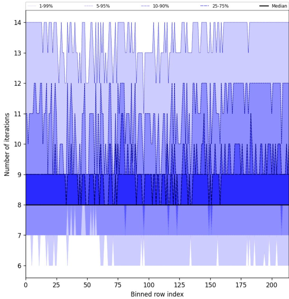
Figure 26: Along track statistics of “Number of iterations” for 2025-02-23 to 2025-02-24
