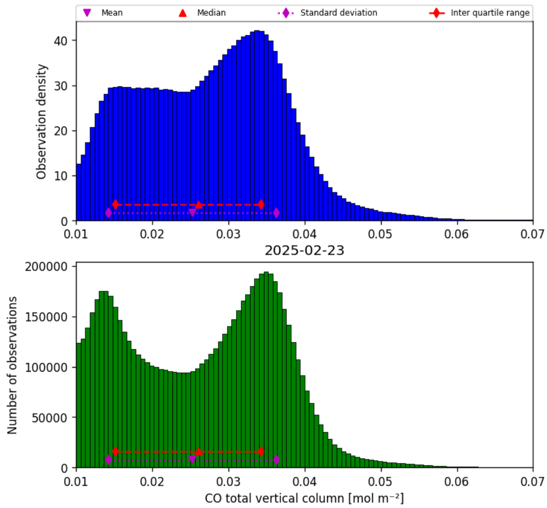
Figure 14: Histogram of “CO total vertical column” for 2025-02-23 to 2025-02-24
