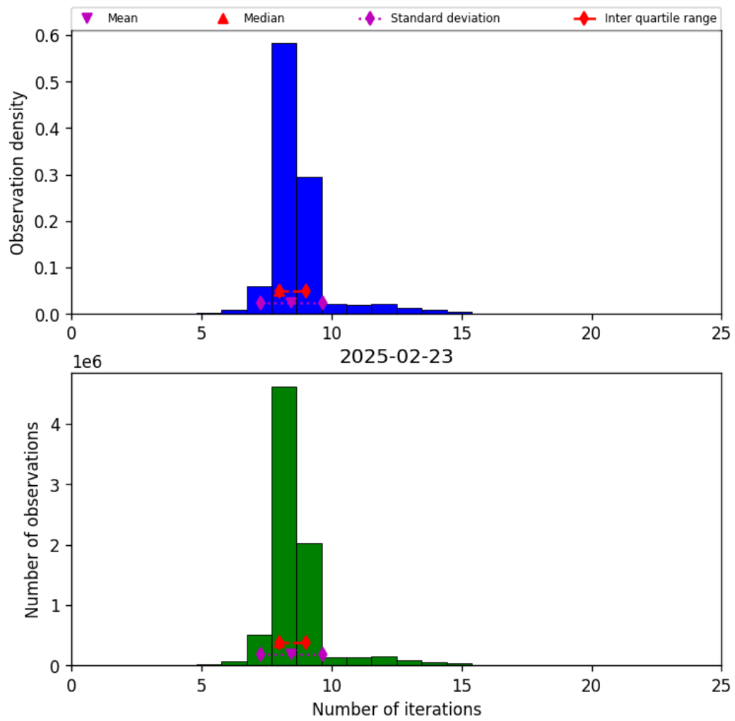
Figure 19: Histogram of “Number of iterations” for 2025-02-23 to 2025-02-24
