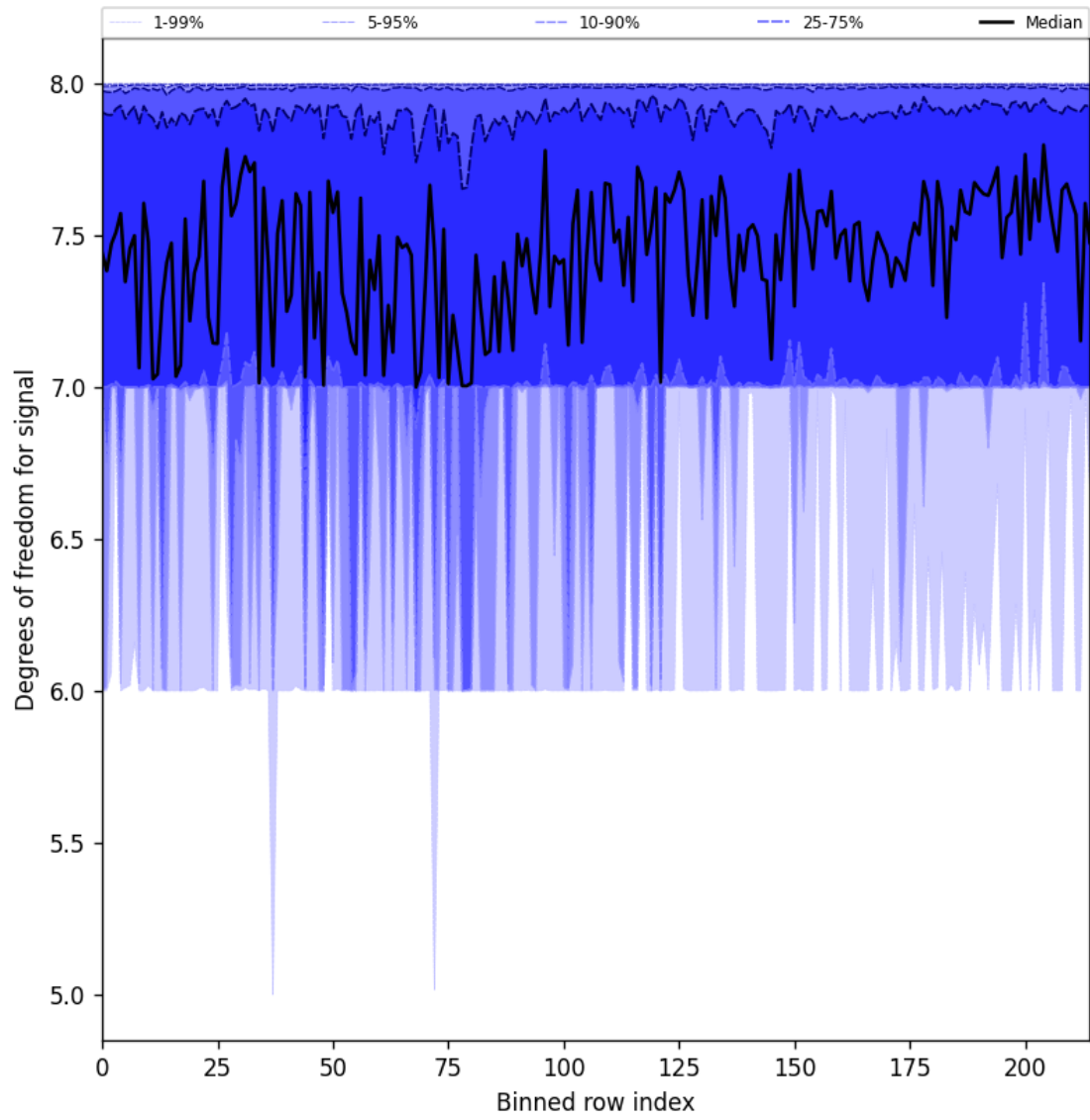
Figure 25: Along track statistics of “Degrees of freedom for signal” for 2025-02-23 to 2025-02-24
