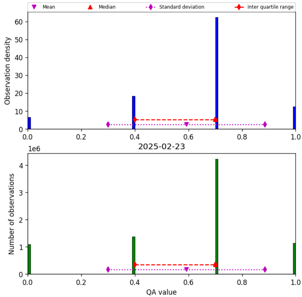
Figure 13: Histogram of “QA value” for 2025-02-23 to 2025-02-24
