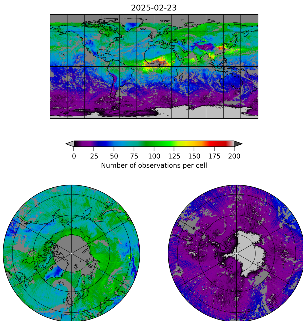
Figure 5: Map of the number of observations for 2025-02-23 to 2025-02-24
