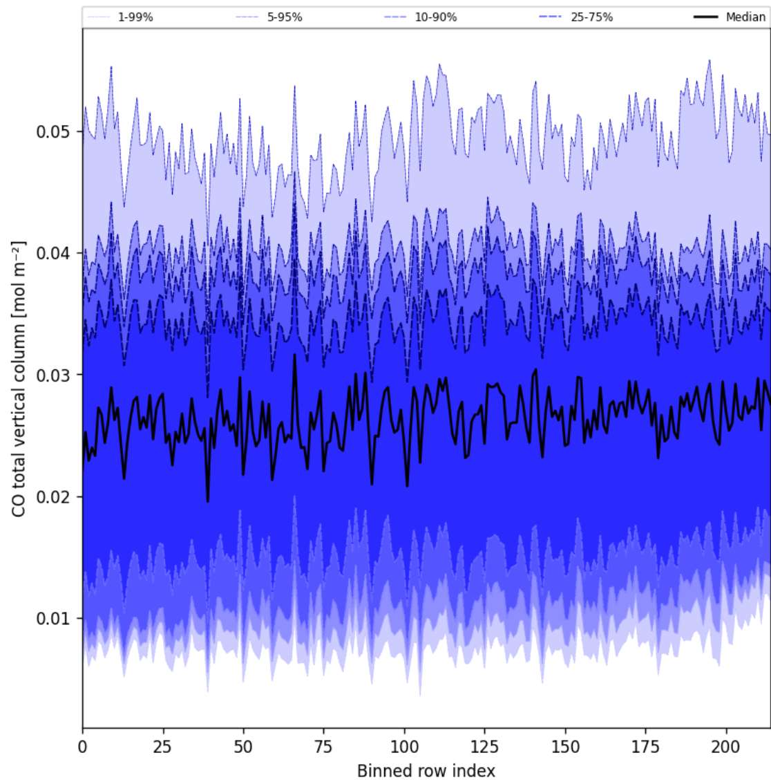
Figure 21: Along track statistics of “CO total vertical column” for 2025-02-23 to 2025-02-24
