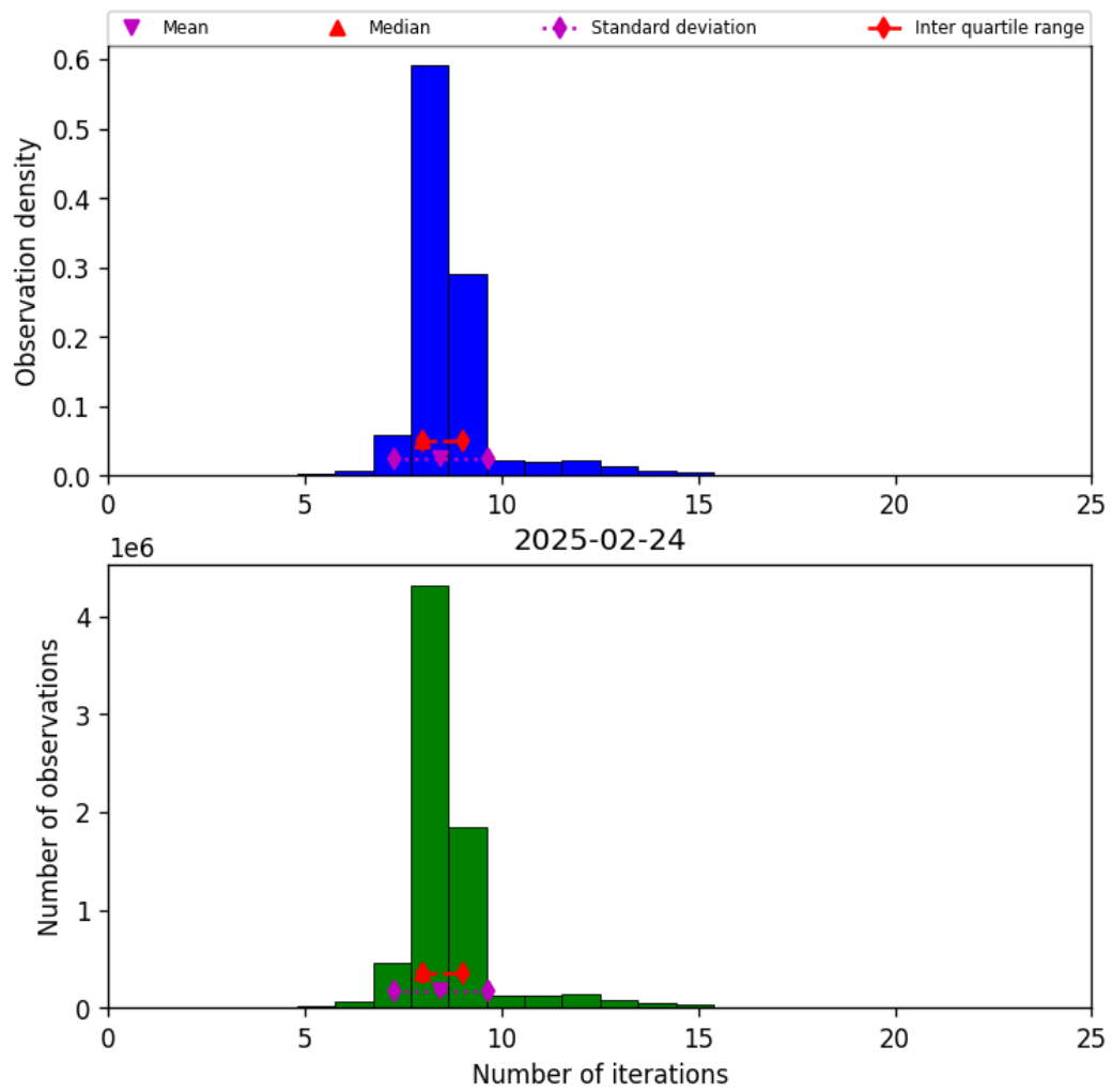
Figure 19: Histogram of “Number of iterations” for 2025-02-24 to 2025-02-25
