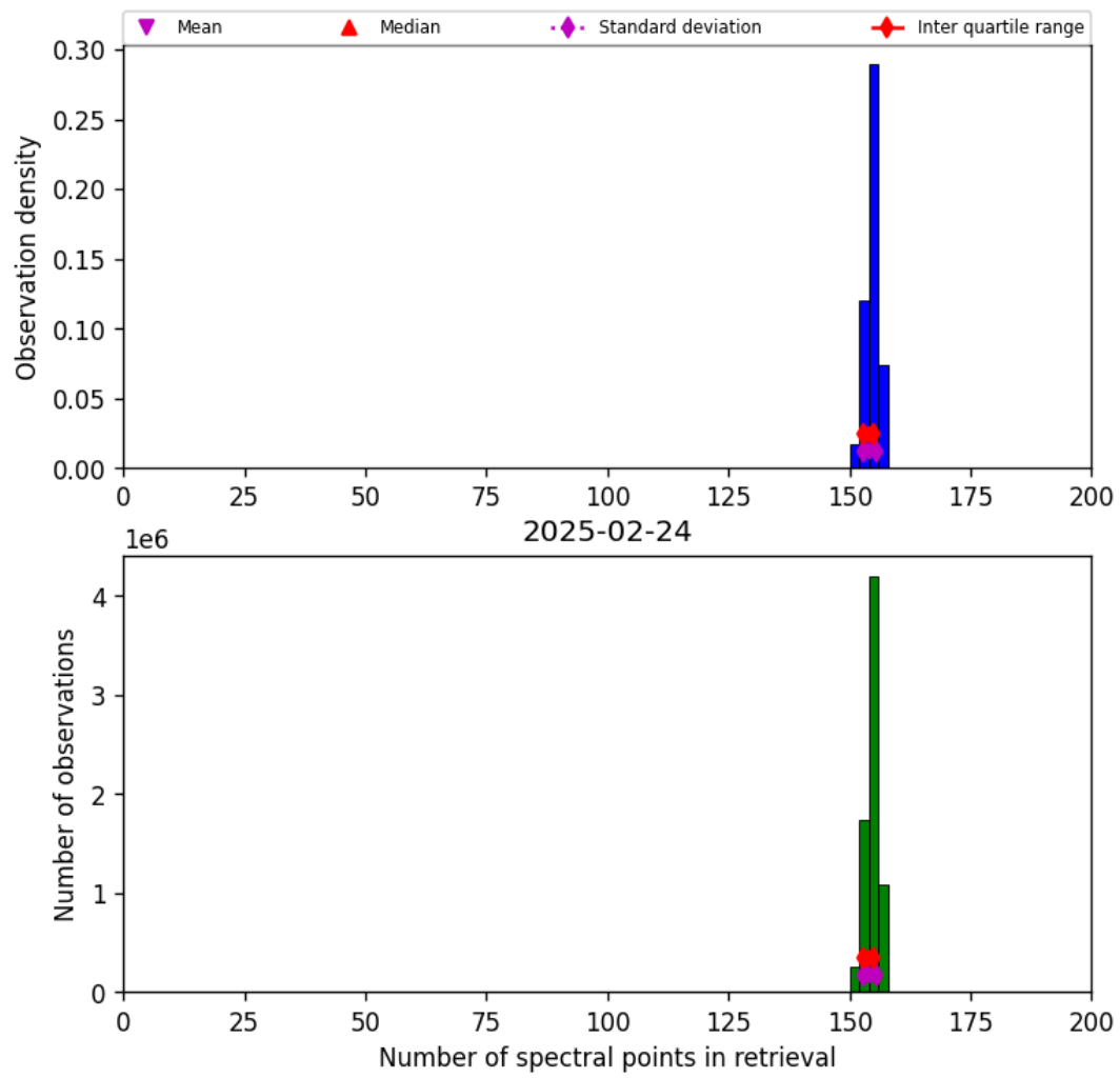
Figure 16: Histogram of “Number of spectral points in retrieval” for 2025-02-24 to 2025-02-25
