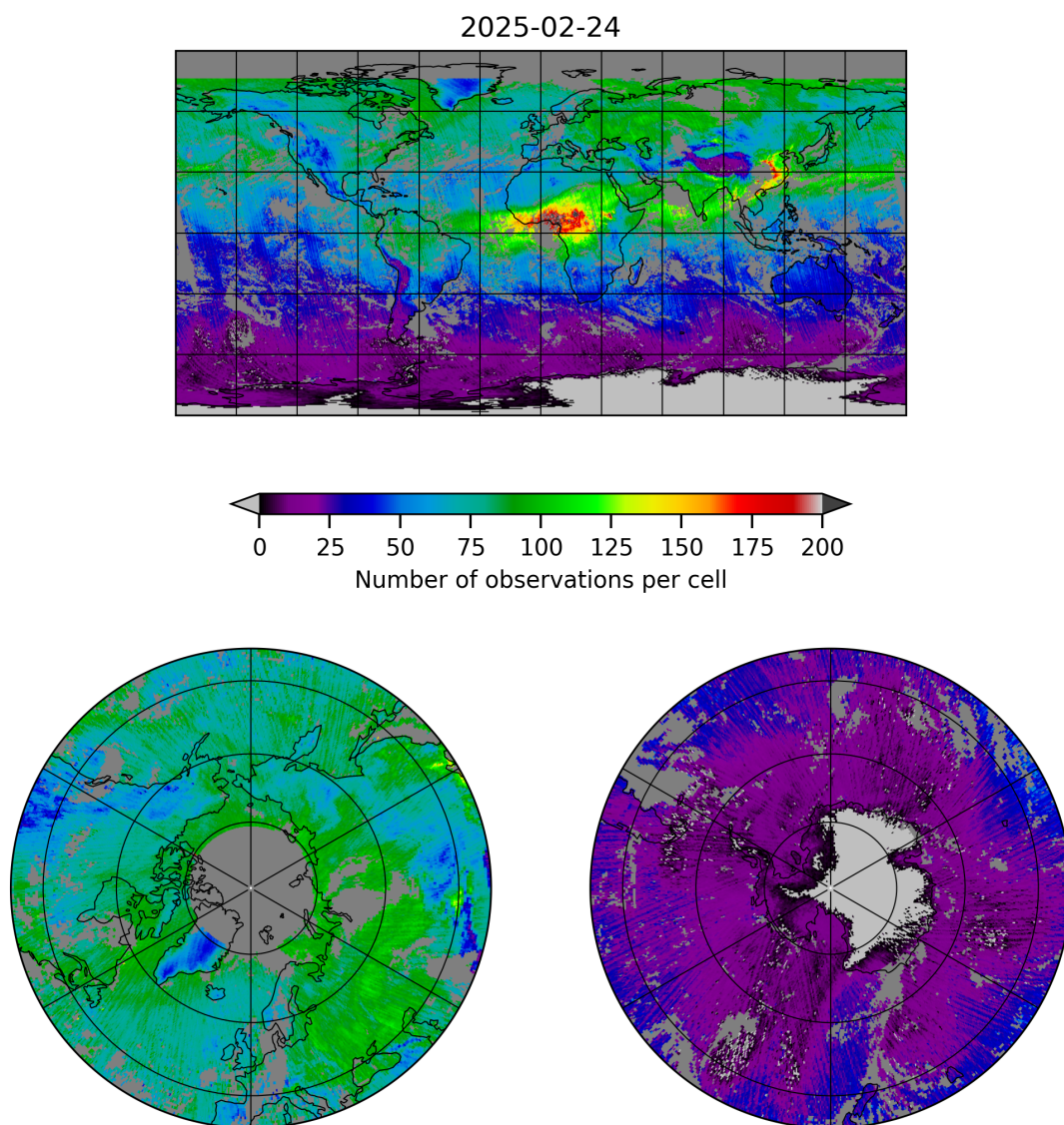
Figure 5: Map of the number of observations for 2025-02-24 to 2025-02-25
