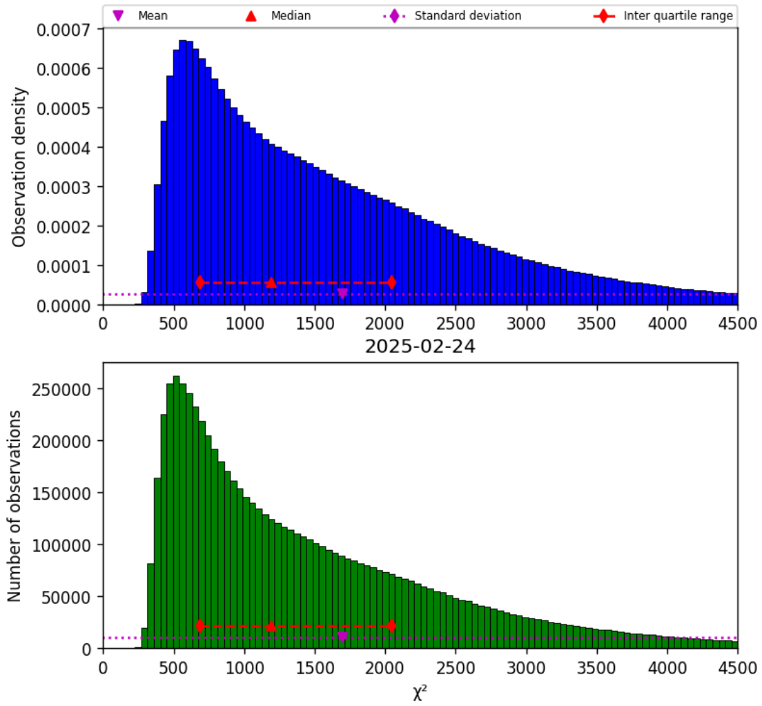
Figure 17: Histogram of “ \chi^2 ” for 2025-02-24 to 2025-02-25
