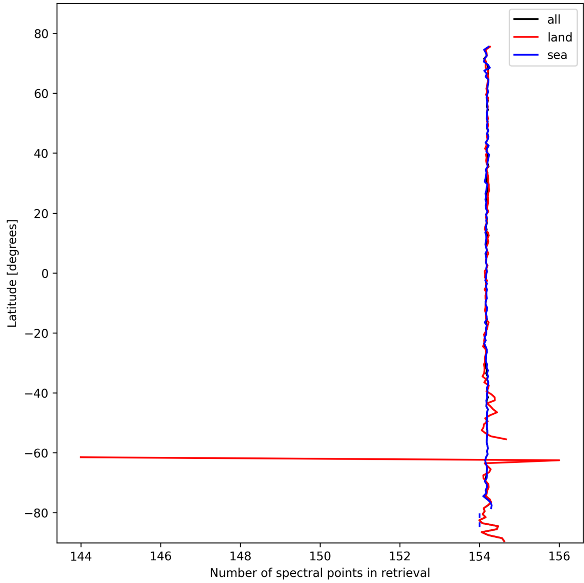
Figure 9: Zonal average of “Number of spectral points in retrieval” for 2025-02-24 to 2025-02-25.
