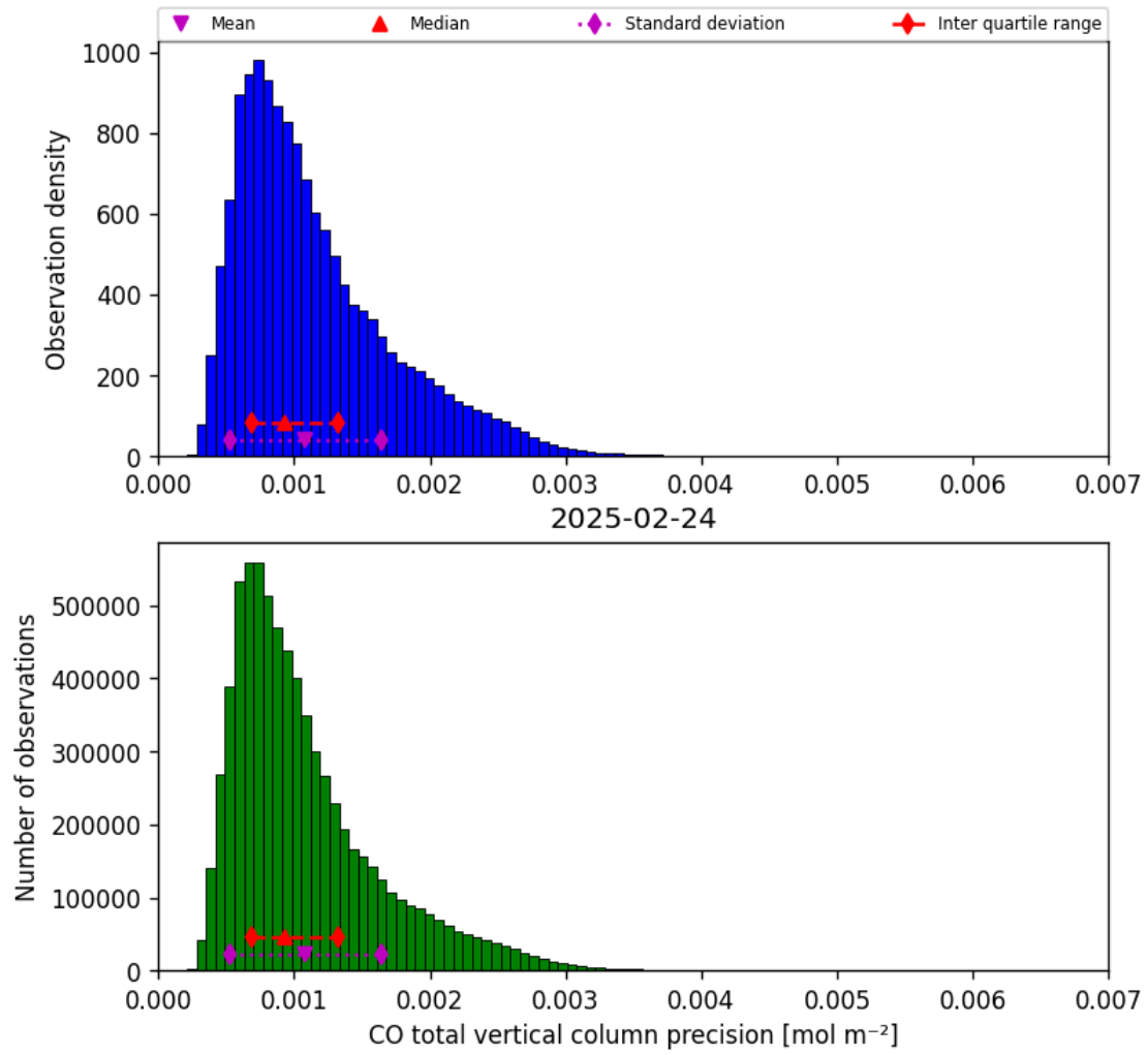
Figure 15: Histogram of “CO total vertical column precision” for 2025-02-24 to 2025-02-25
