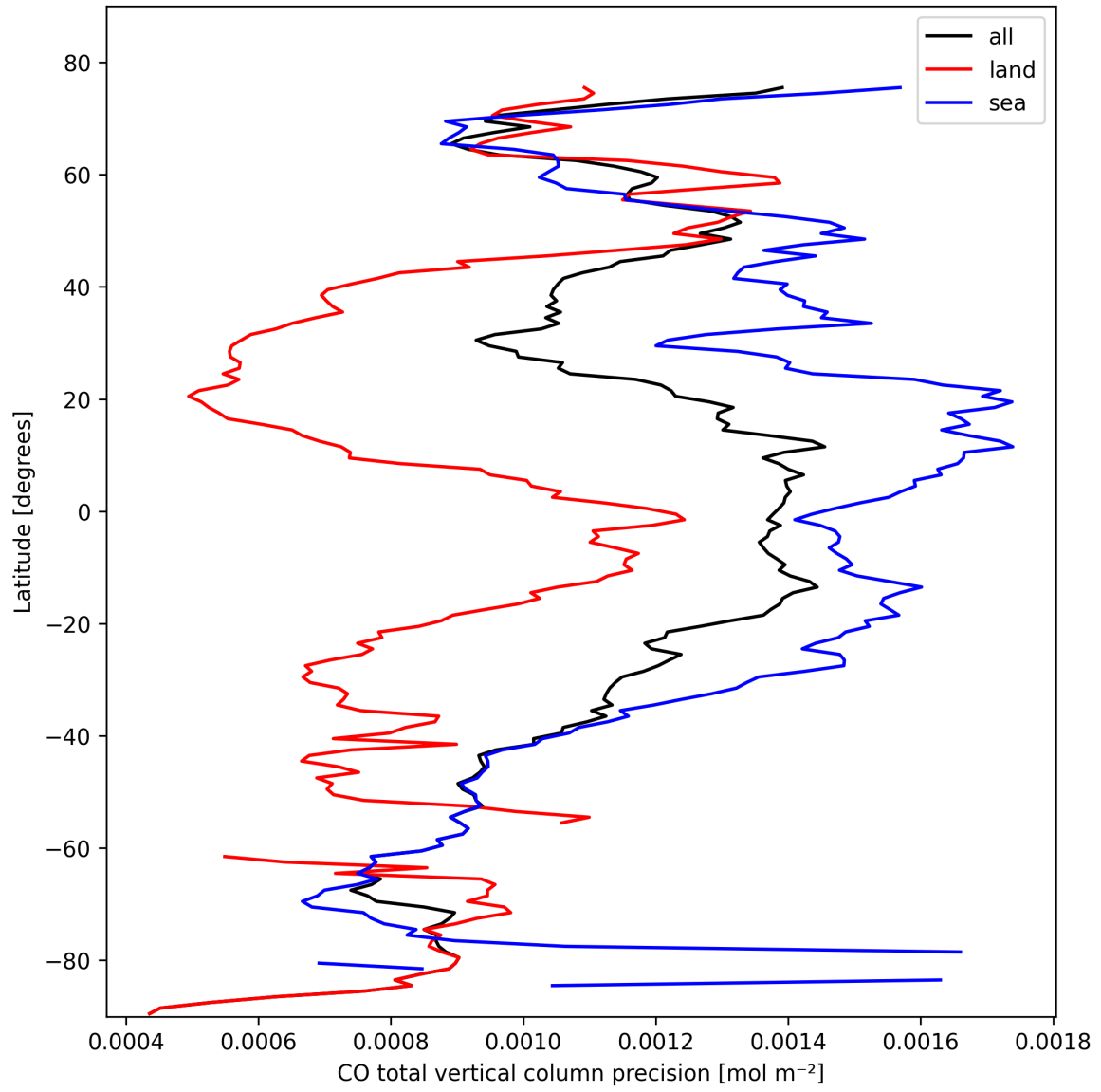
Figure 8: Zonal average of “CO total vertical column precision” for 2025-02-24 to 2025-02-25.
