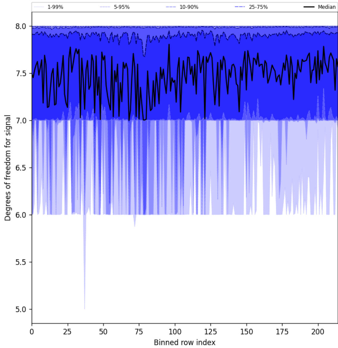
Figure 25: Along track statistics of “Degrees of freedom for signal” for 2025-02-24 to 2025-02-25
