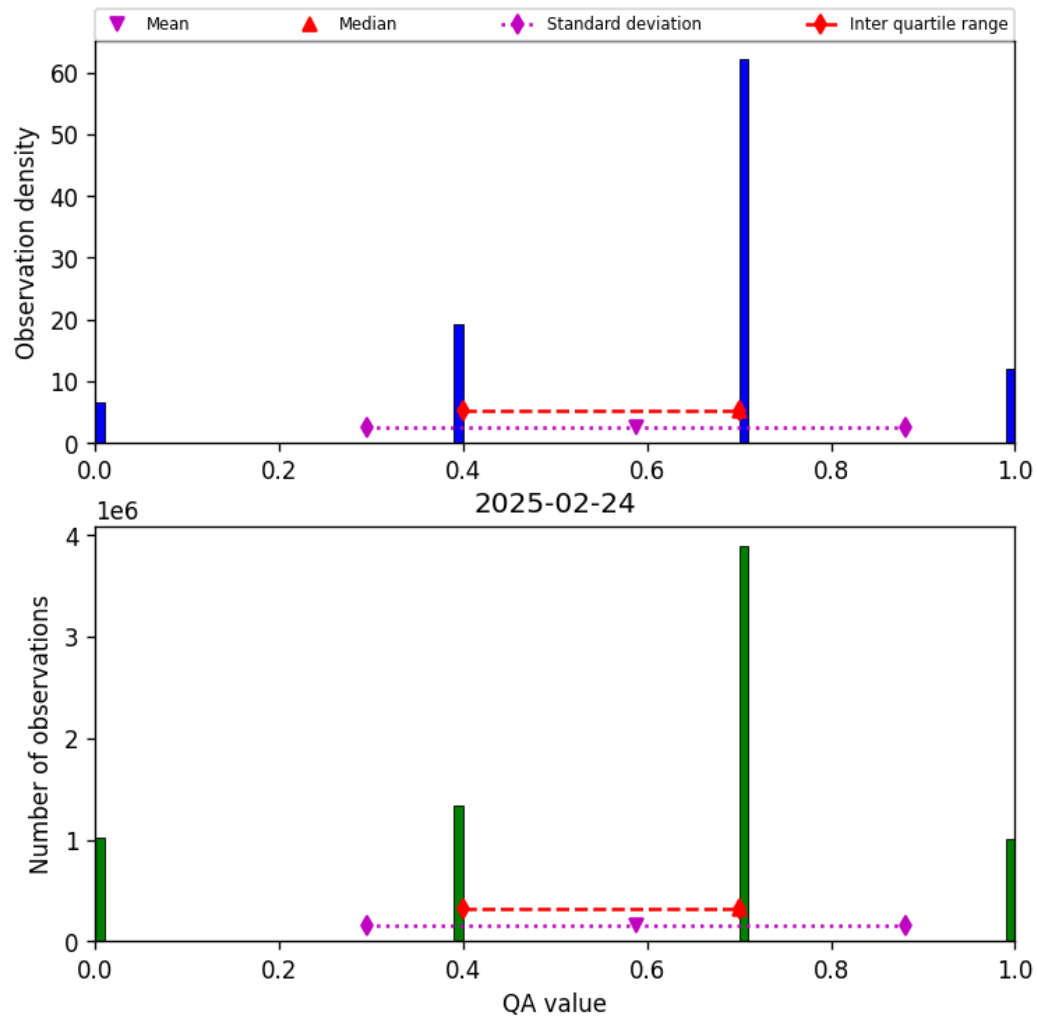
Figure 13: Histogram of “QA value” for 2025-02-24 to 2025-02-25
