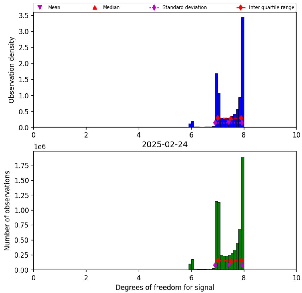
Figure 18: Histogram of “Degrees of freedom for signal” for 2025-02-24 to 2025-02-25
