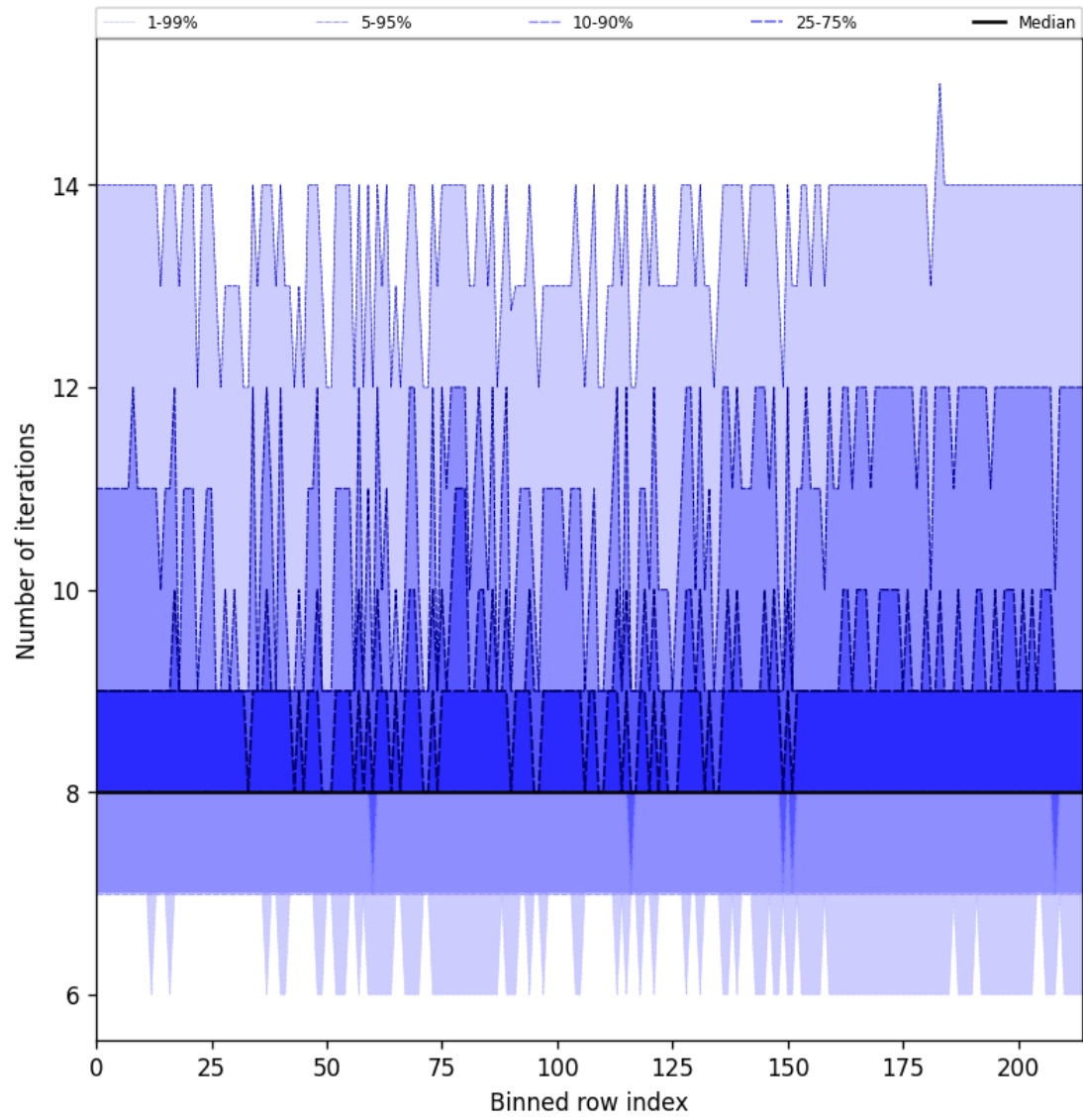
Figure 26: Along track statistics of “Number of iterations” for 2025-02-24 to 2025-02-25
