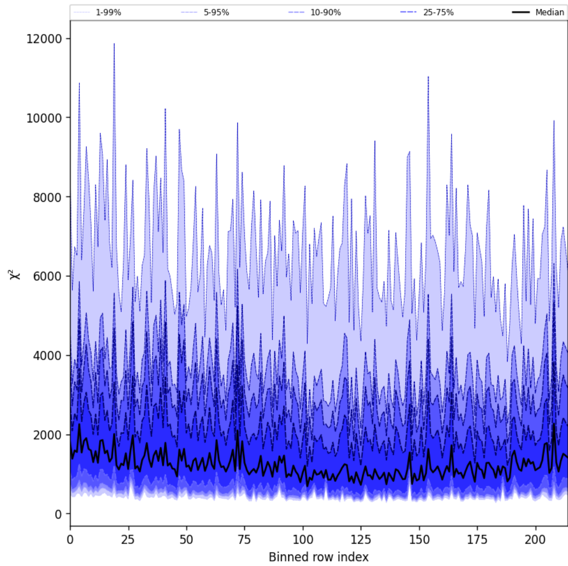
Figure 24: Along track statistics of “ \chi^2 ” for 2025-02-24 to 2025-02-25
