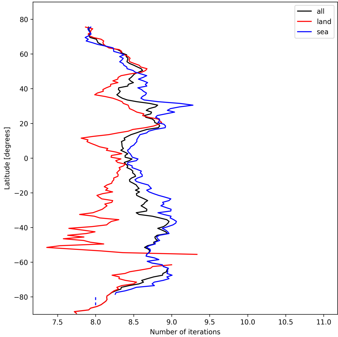
Figure 12: Zonal average of “Number of iterations” for 2025-02-24 to 2025-02-25.
