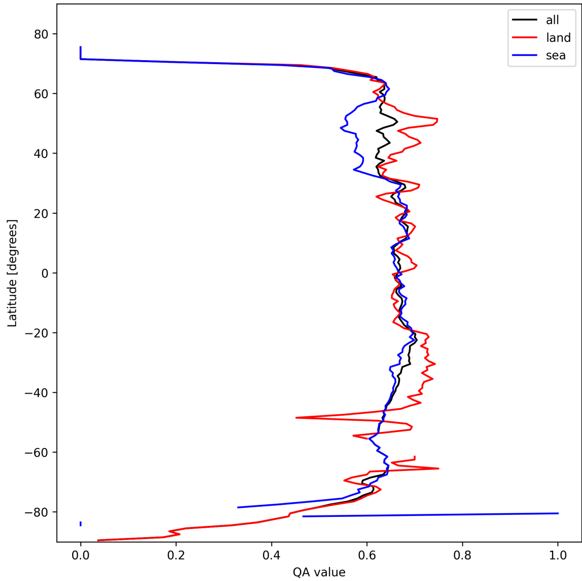
Figure 6: Zonal average of “QA value” for 2025-02-24 to 2025-02-25.
