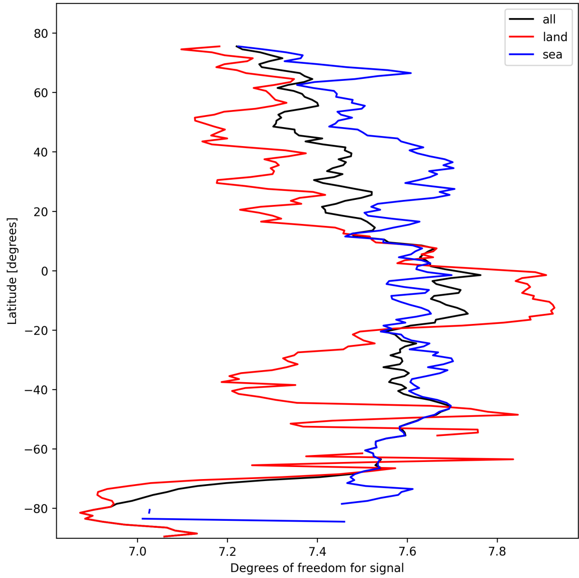
Figure 11: Zonal average of “Degrees of freedom for signal” for 2025-02-24 to 2025-02-25.
