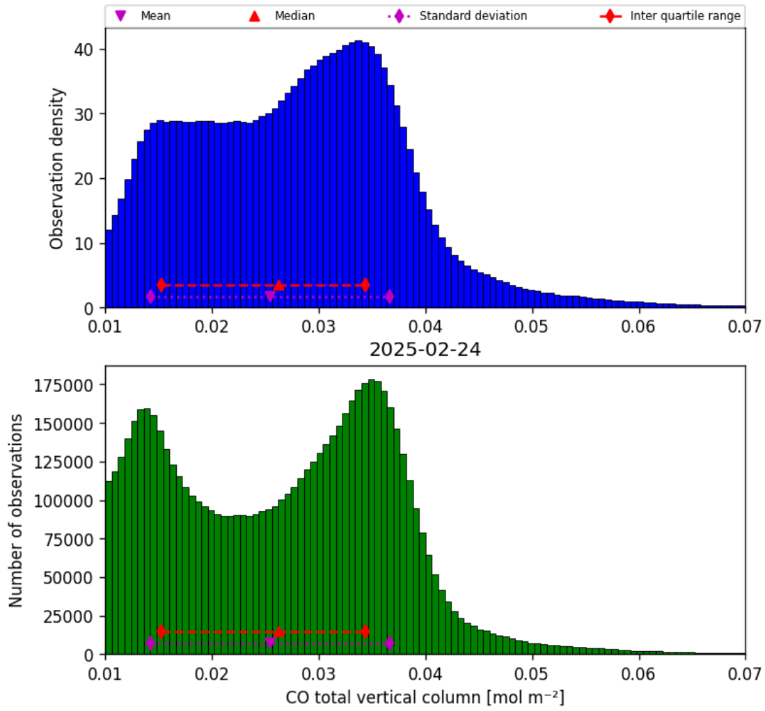
Figure 14: Histogram of “CO total vertical column” for 2025-02-24 to 2025-02-25
