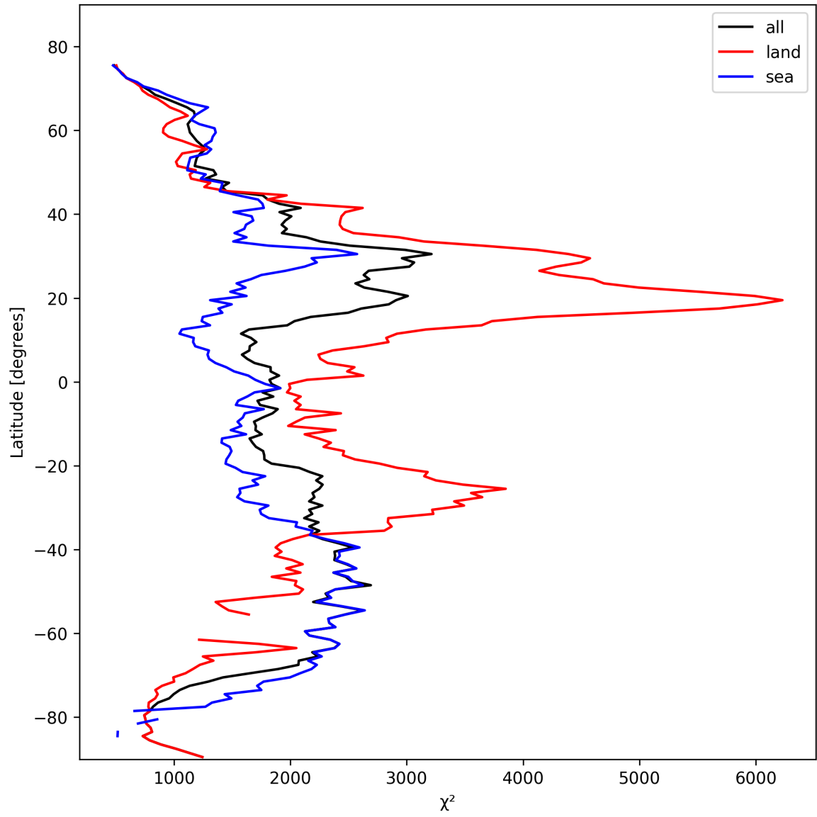
Figure 10: Zonal average of “ \chi^2 ” for 2025-02-24 to 2025-02-25.
