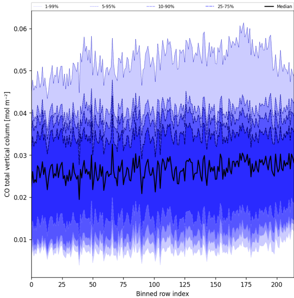
Figure 21: Along track statistics of “CO total vertical column” for 2025-02-24 to 2025-02-25
