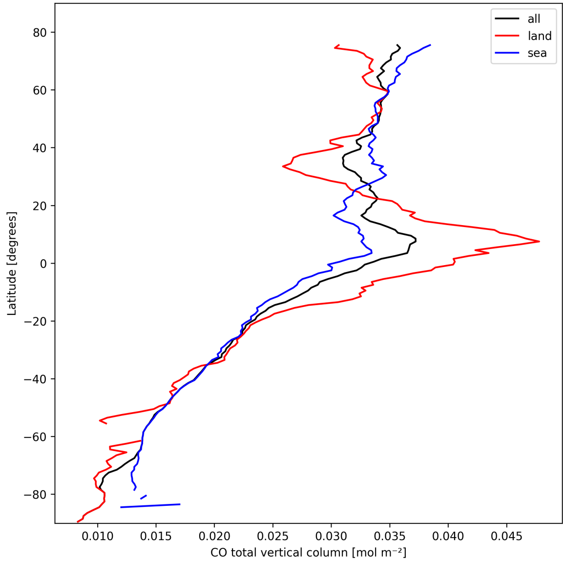
Figure 7: Zonal average of “CO total vertical column” for 2025-02-24 to 2025-02-25.
