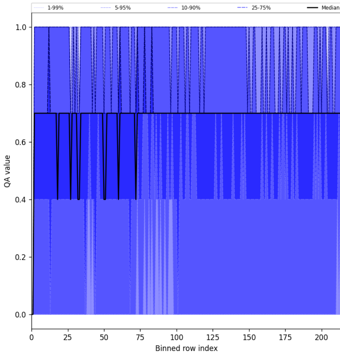
Figure 20: Along track statistics of “QA value” for 2025-02-24 to 2025-02-25
