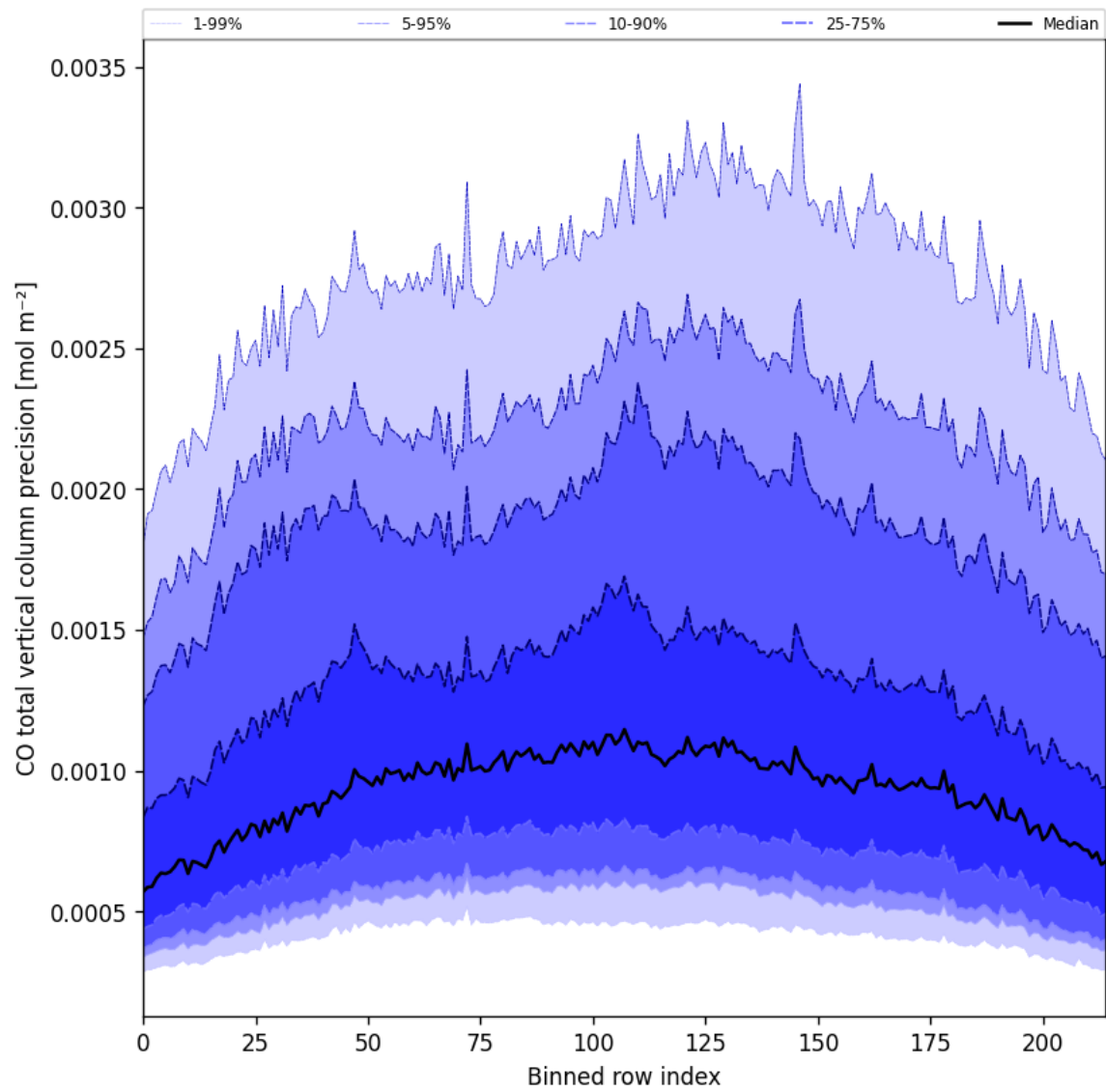
Figure 22: Along track statistics of “CO total vertical column precision” for 2025-02-24 to 2025-02-25
