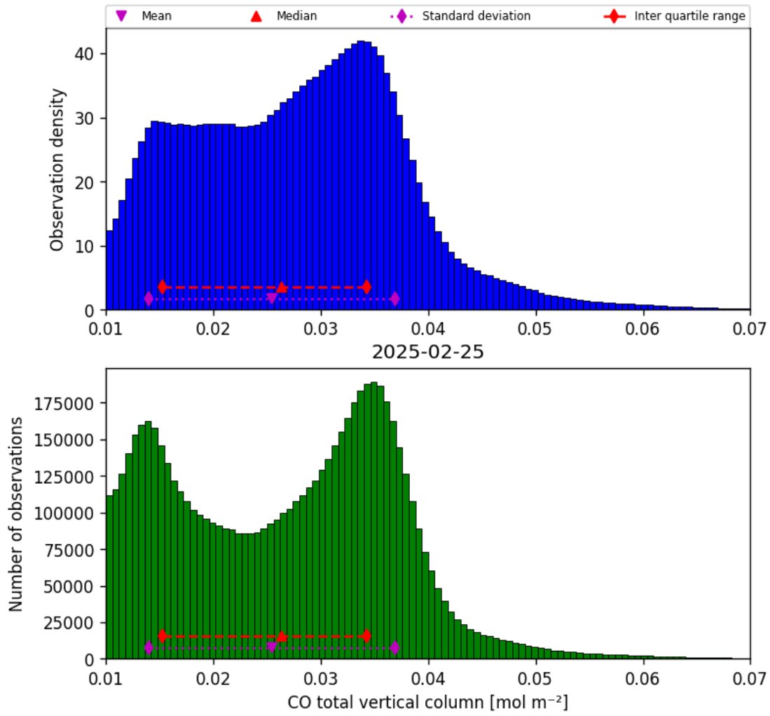
Figure 14: Histogram of “CO total vertical column” for 2025-02-25 to 2025-02-26
