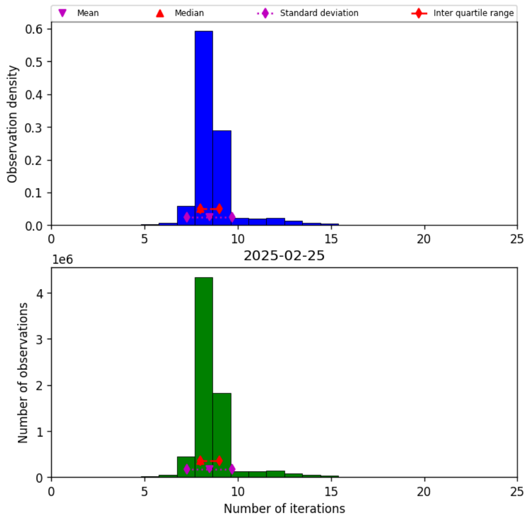
Figure 19: Histogram of “Number of iterations” for 2025-02-25 to 2025-02-26
