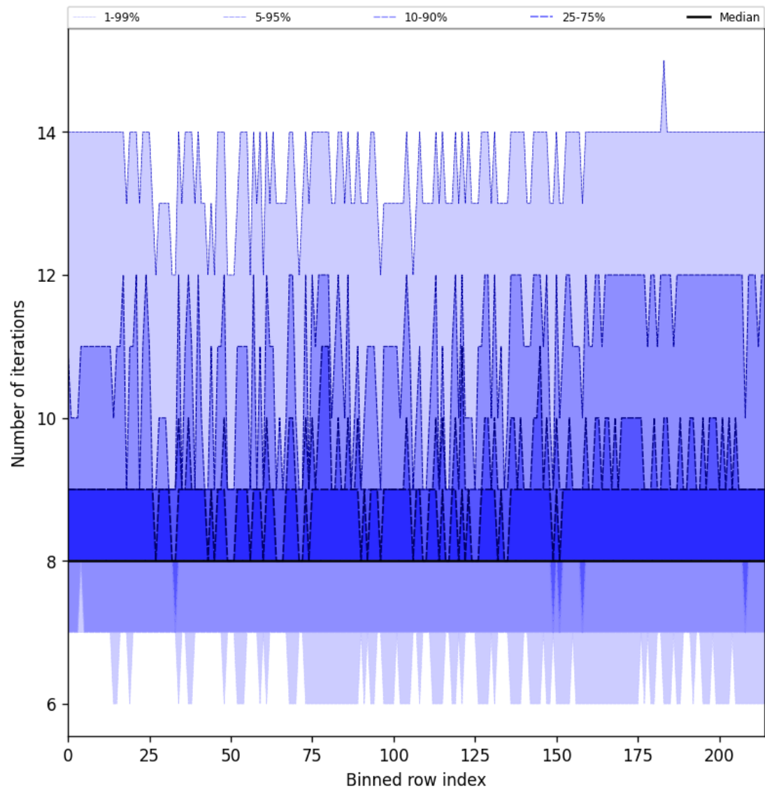
Figure 26: Along track statistics of “Number of iterations” for 2025-02-25 to 2025-02-26
