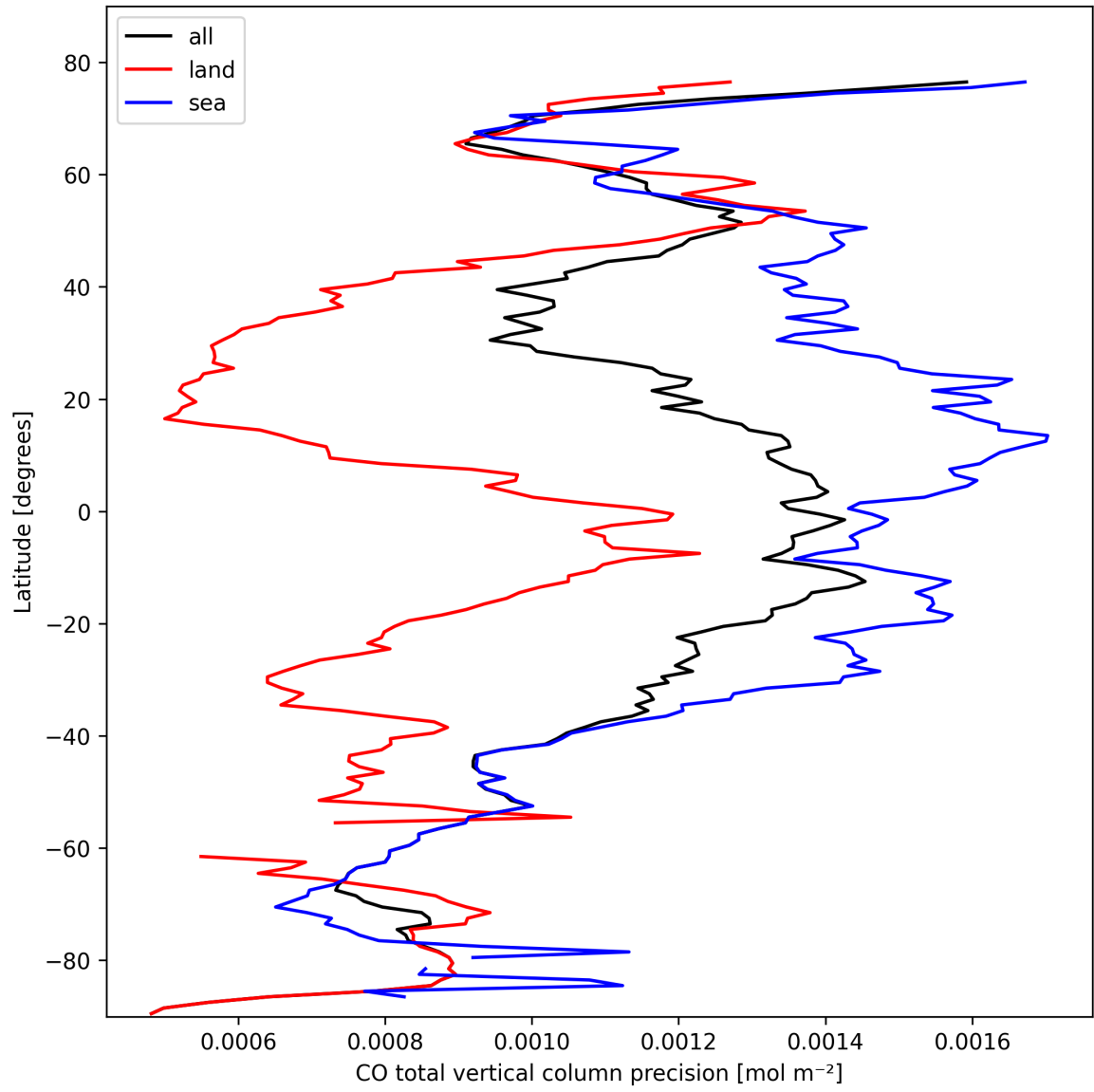
Figure 8: Zonal average of “CO total vertical column precision” for 2025-02-25 to 2025-02-26.
