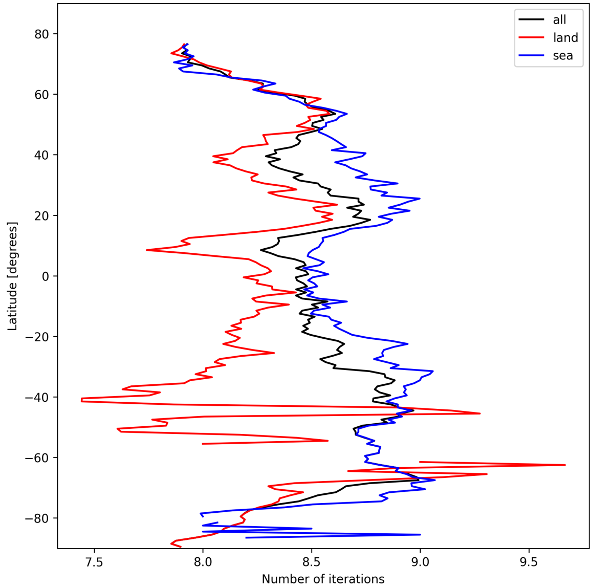
Figure 12: Zonal average of “Number of iterations” for 2025-02-25 to 2025-02-26.
