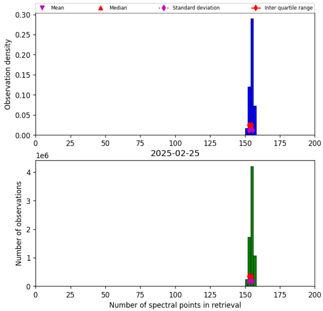
Figure 16: Histogram of “Number of spectral points in retrieval” for 2025-02-25 to 2025-02-26
