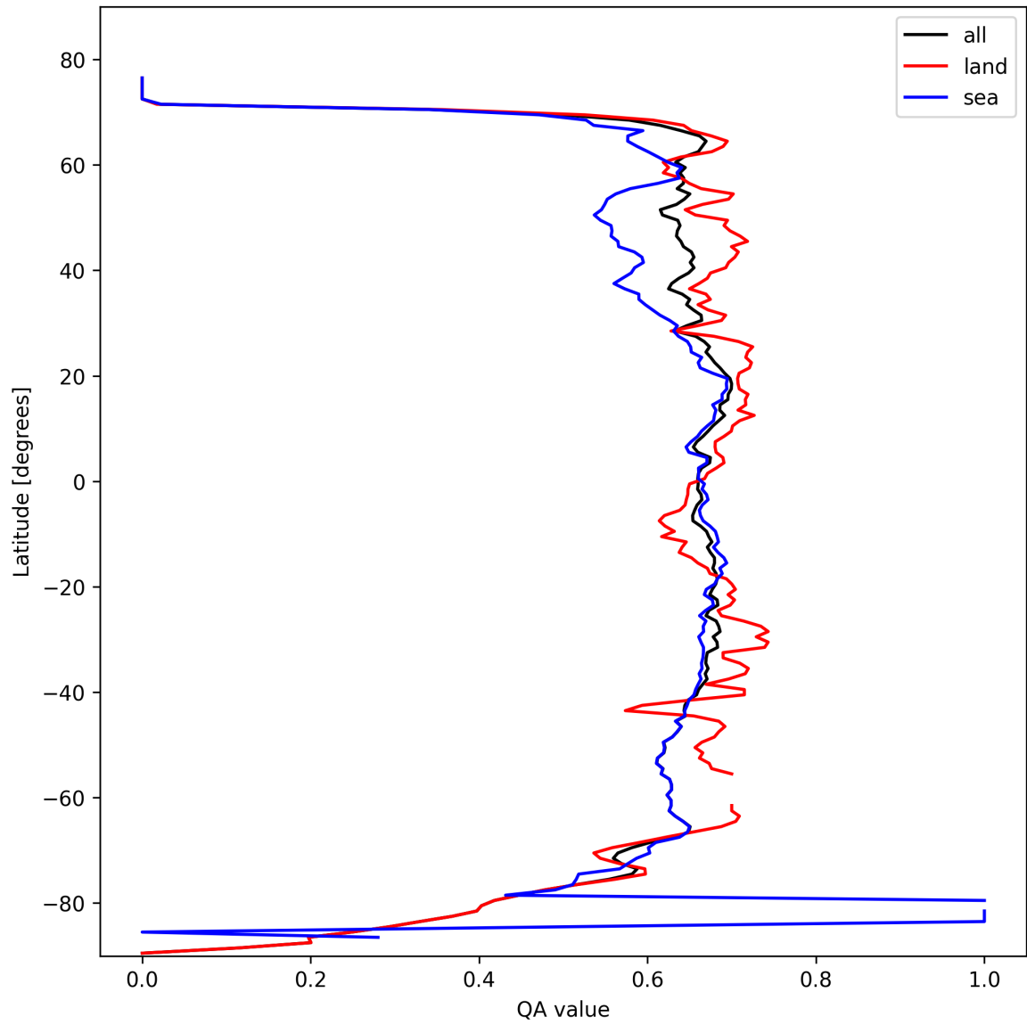
Figure 6: Zonal average of “QA value” for 2025-02-25 to 2025-02-26.
