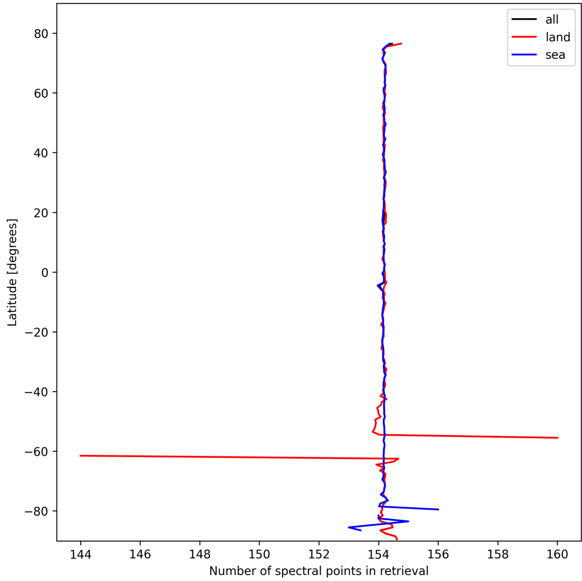
Figure 9: Zonal average of “Number of spectral points in retrieval” for 2025-02-25 to 2025-02-26.
