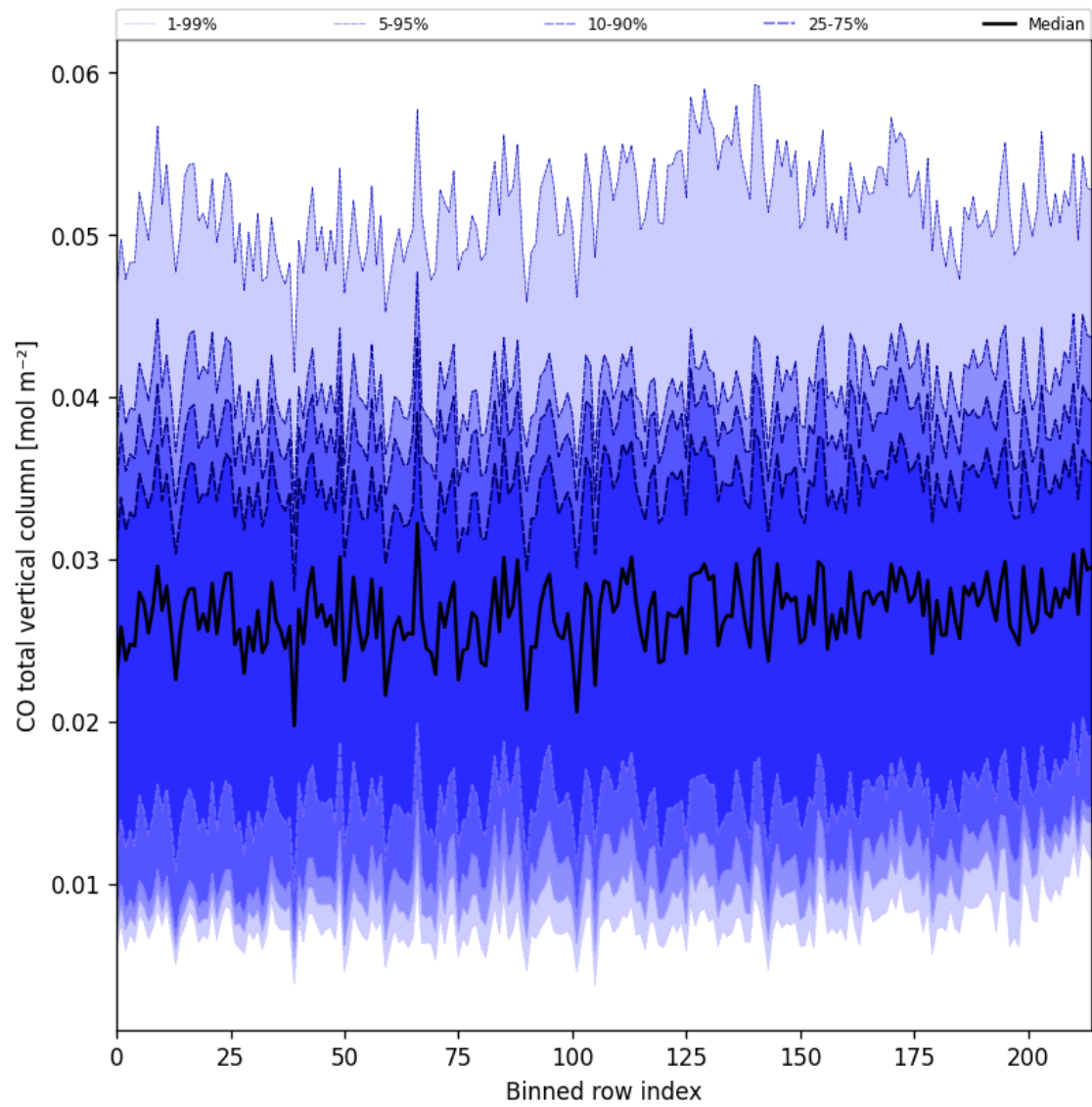
Figure 21: Along track statistics of “CO total vertical column” for 2025-02-25 to 2025-02-26
