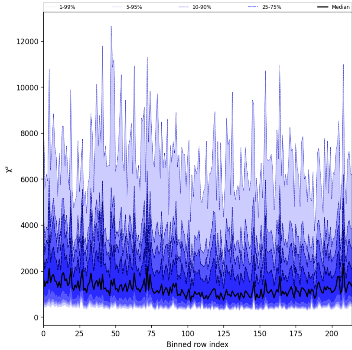
Figure 24: Along track statistics of “ \chi^2 ” for 2025-02-25 to 2025-02-26
