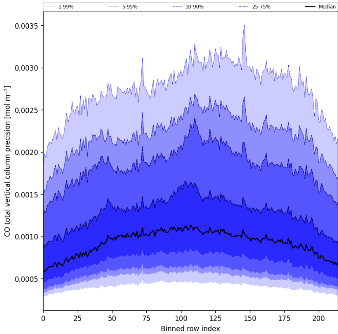
Figure 22: Along track statistics of “CO total vertical column precision” for 2025-02-25 to 2025-02-26
