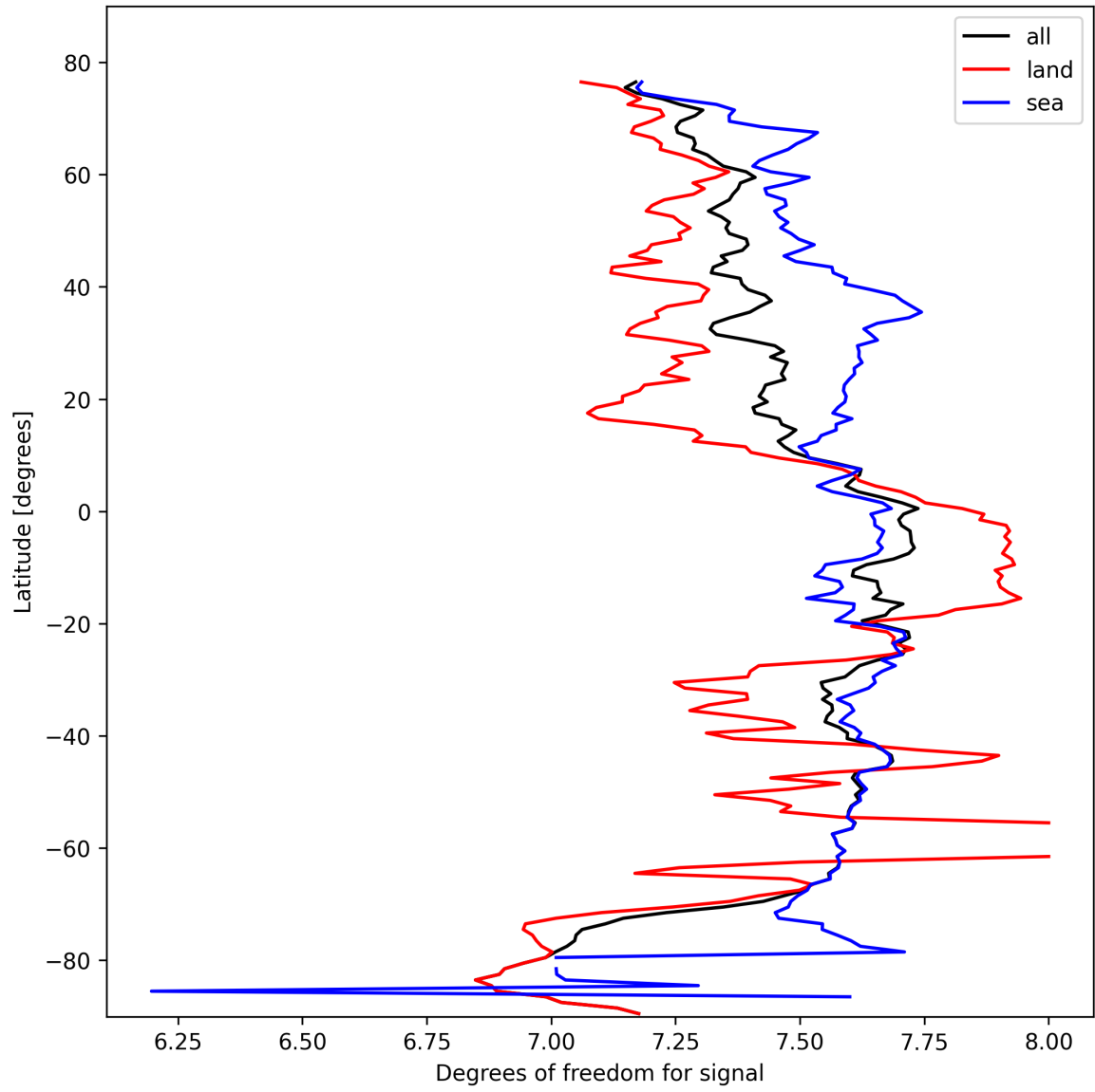
Figure 11: Zonal average of “Degrees of freedom for signal” for 2025-02-25 to 2025-02-26.
