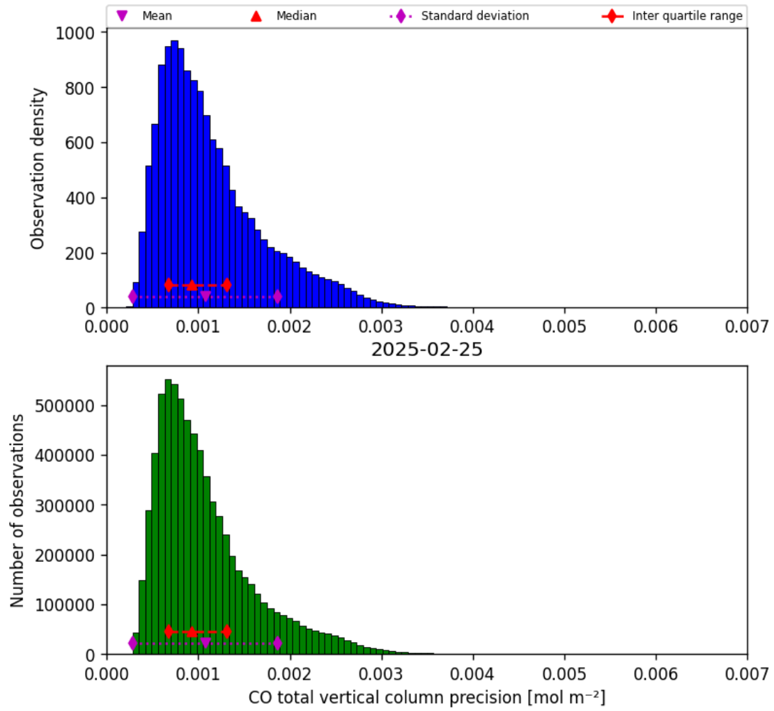
Figure 15: Histogram of “CO total vertical column precision” for 2025-02-25 to 2025-02-26
