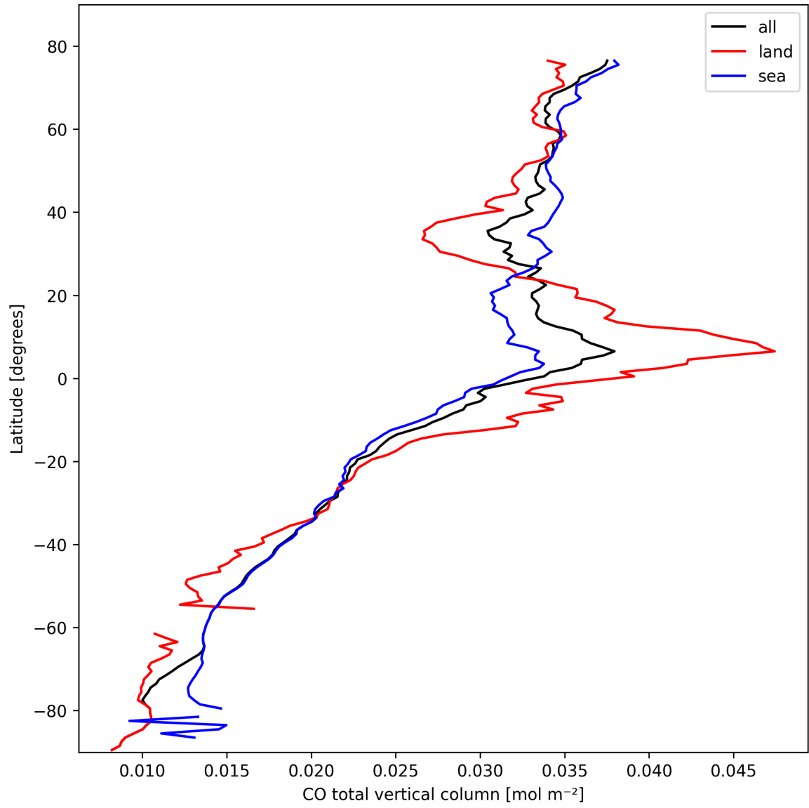
Figure 7: Zonal average of “CO total vertical column” for 2025-02-25 to 2025-02-26.
