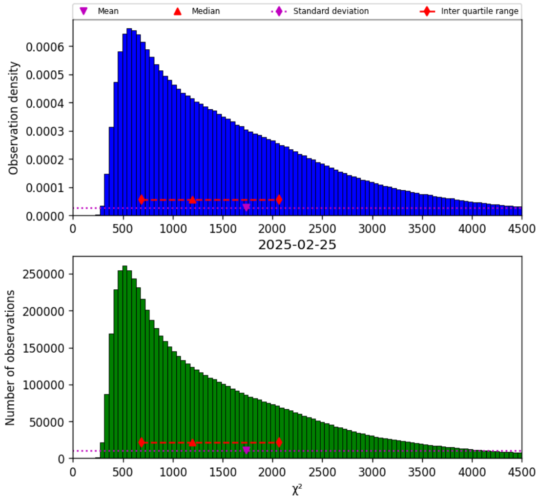
Figure 17: Histogram of “ \chi^2 ” for 2025-02-25 to 2025-02-26
