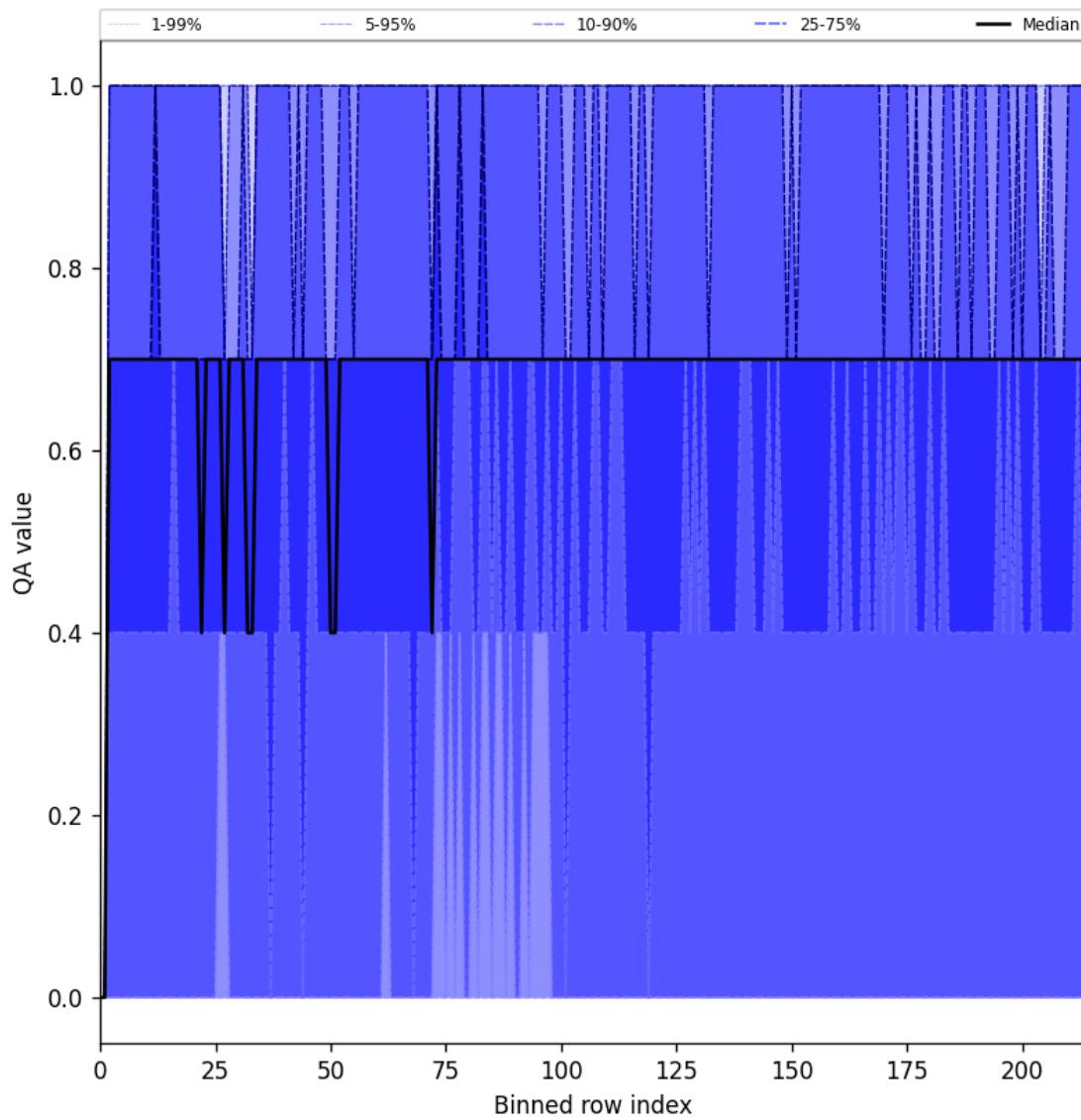
Figure 20: Along track statistics of “QA value” for 2025-02-25 to 2025-02-26
