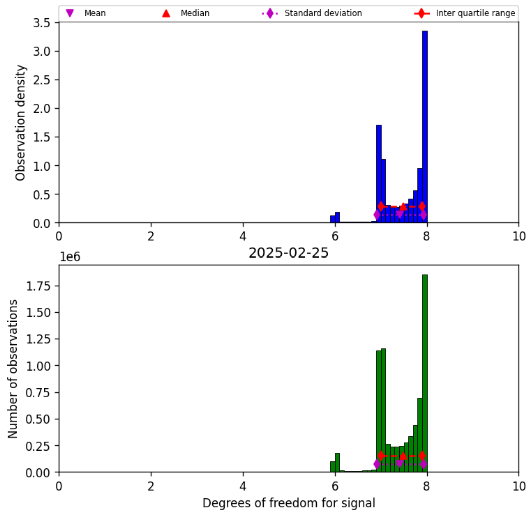
Figure 18: Histogram of “Degrees of freedom for signal” for 2025-02-25 to 2025-02-26
