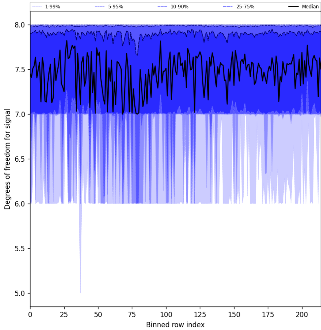
Figure 25: Along track statistics of “Degrees of freedom for signal” for 2025-02-25 to 2025-02-26
