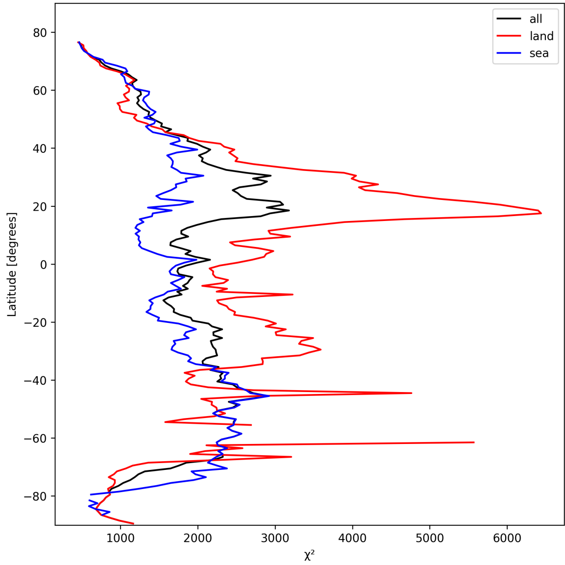
Figure 10: Zonal average of “ \chi^2 ” for 2025-02-25 to 2025-02-26.
