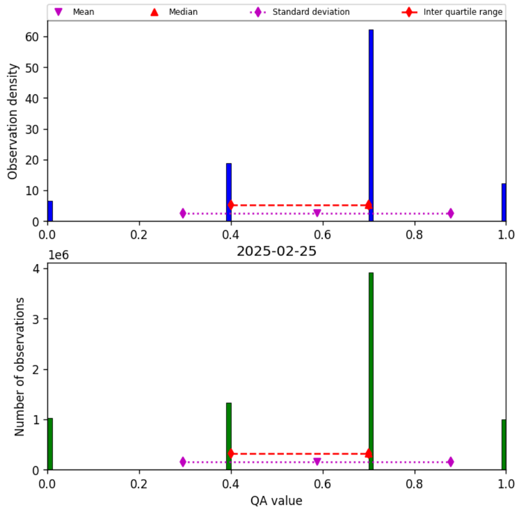
Figure 13: Histogram of “QA value” for 2025-02-25 to 2025-02-26
