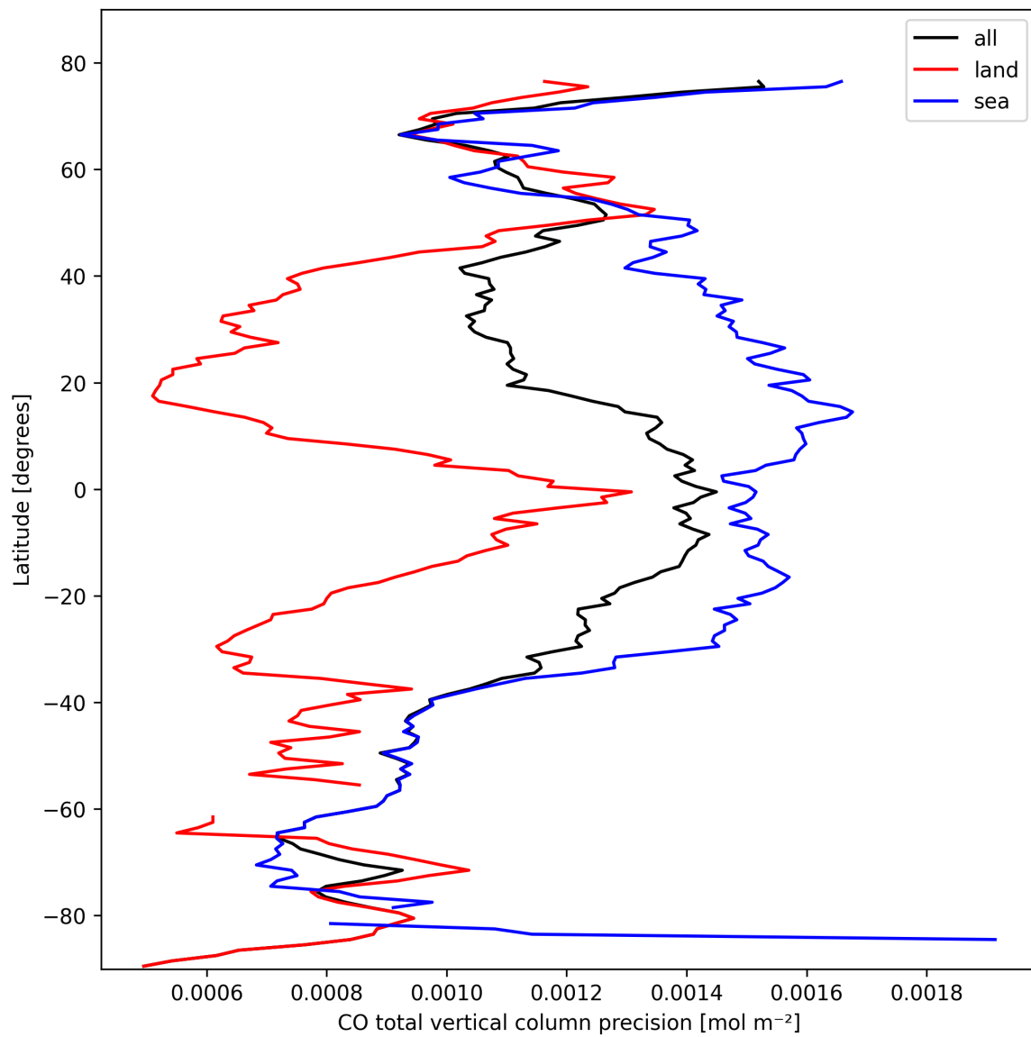
Figure 8: Zonal average of “CO total vertical column precision” for 2025-02-26 to 2025-02-27.
