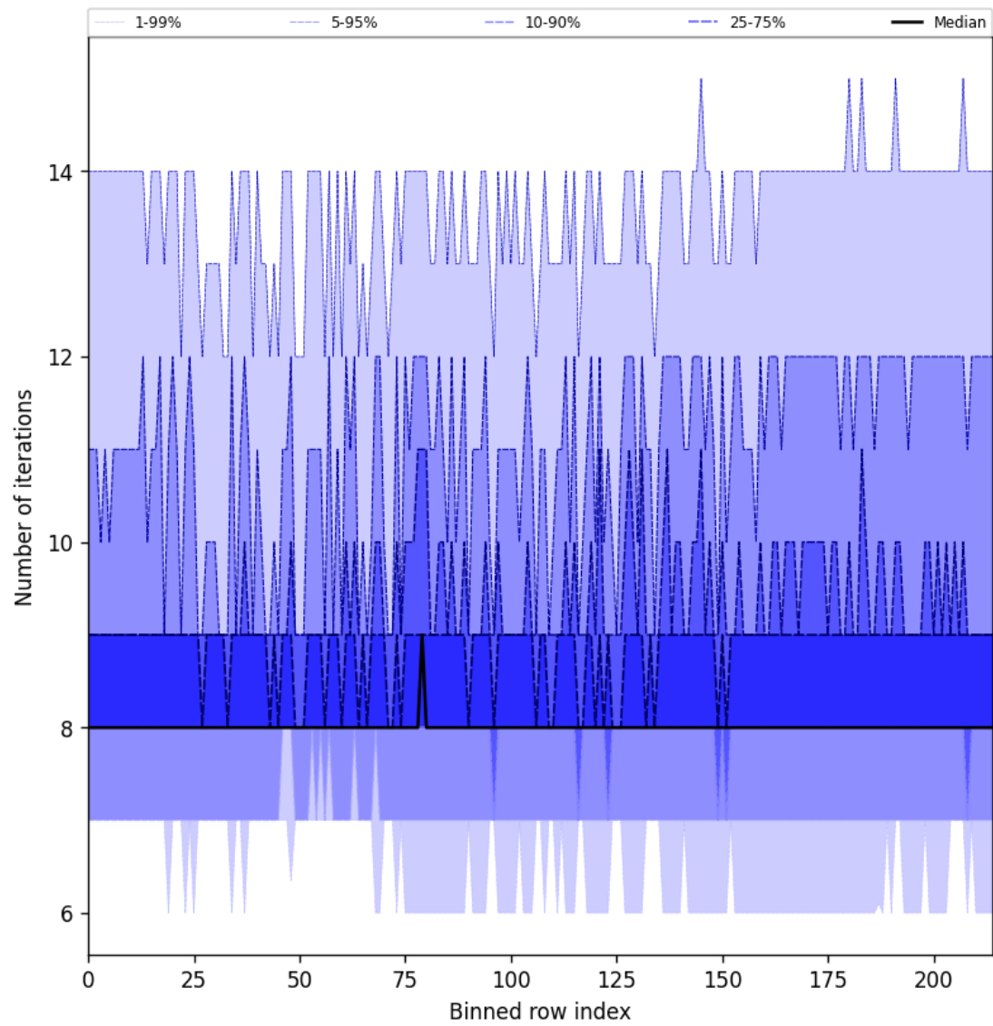
Figure 26: Along track statistics of “Number of iterations” for 2025-02-26 to 2025-02-27
