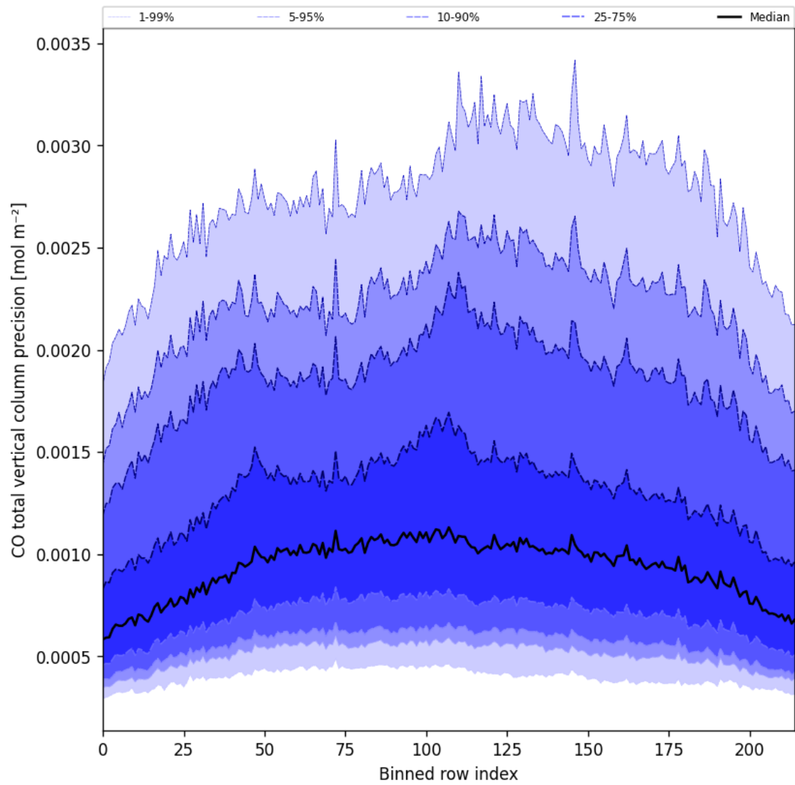
Figure 22: Along track statistics of “CO total vertical column precision” for 2025-02-26 to 2025-02-27
