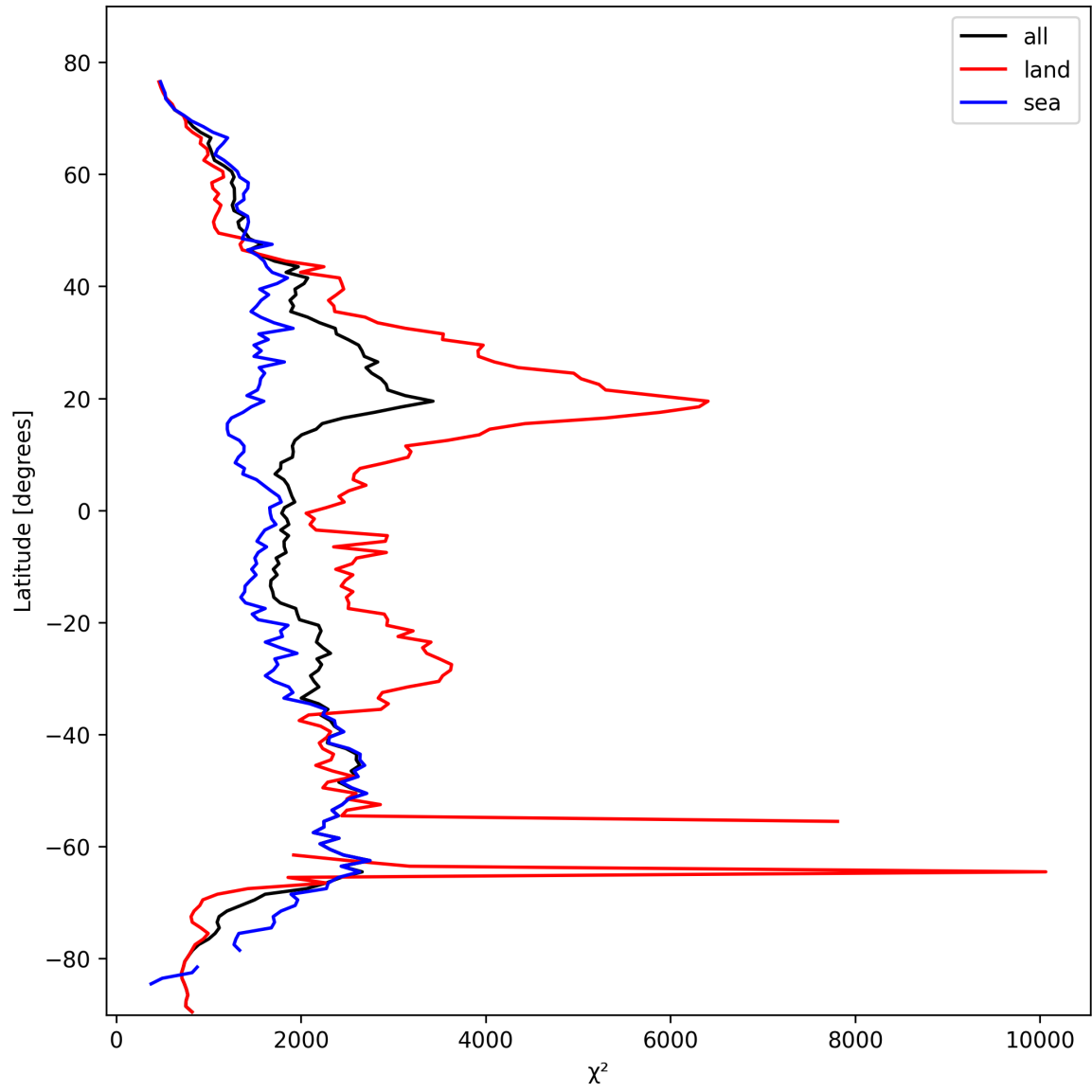
Figure 10: Zonal average of “ \chi^2 ” for 2025-02-26 to 2025-02-27.
