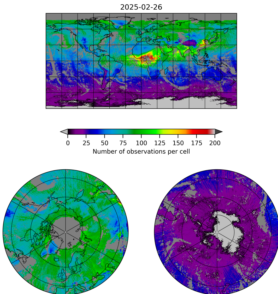
Figure 5: Map of the number of observations for 2025-02-26 to 2025-02-27
