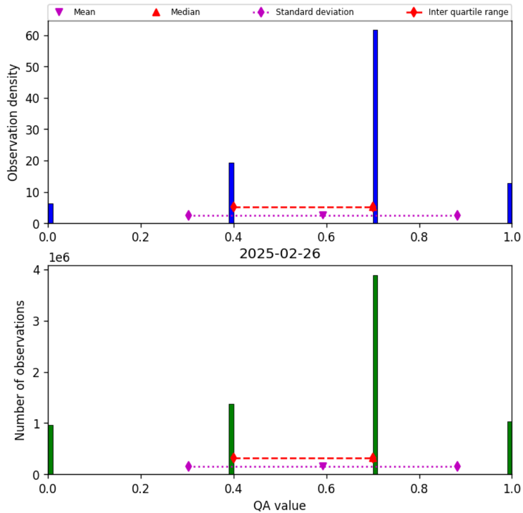
Figure 13: Histogram of “QA value” for 2025-02-26 to 2025-02-27
