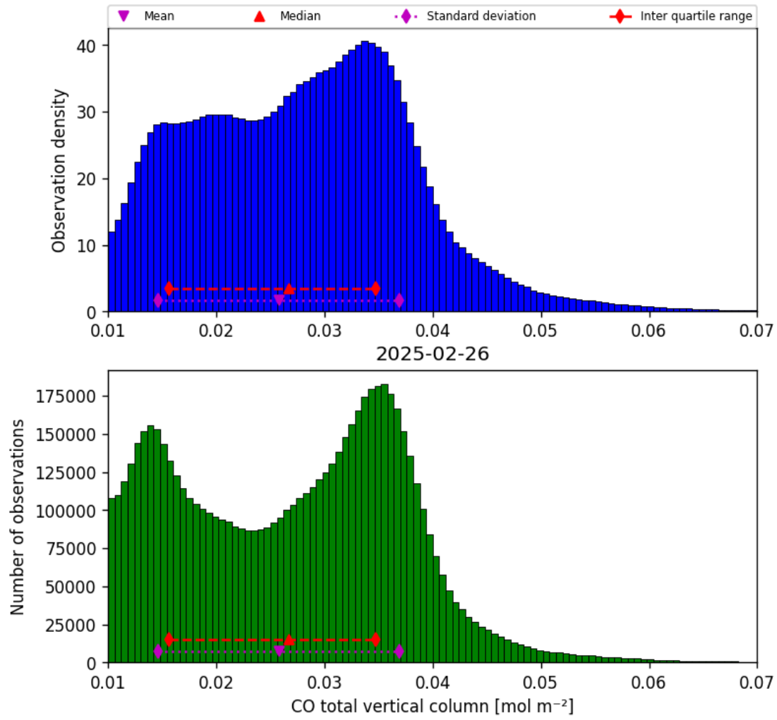
Figure 14: Histogram of “CO total vertical column” for 2025-02-26 to 2025-02-27
