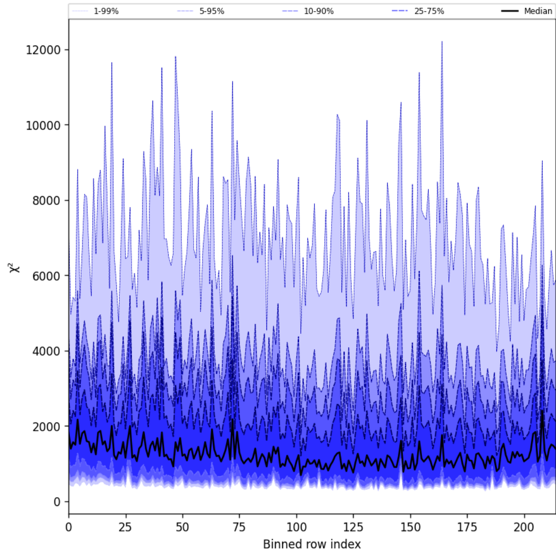
Figure 24: Along track statistics of “ \chi^2 ” for 2025-02-26 to 2025-02-27
