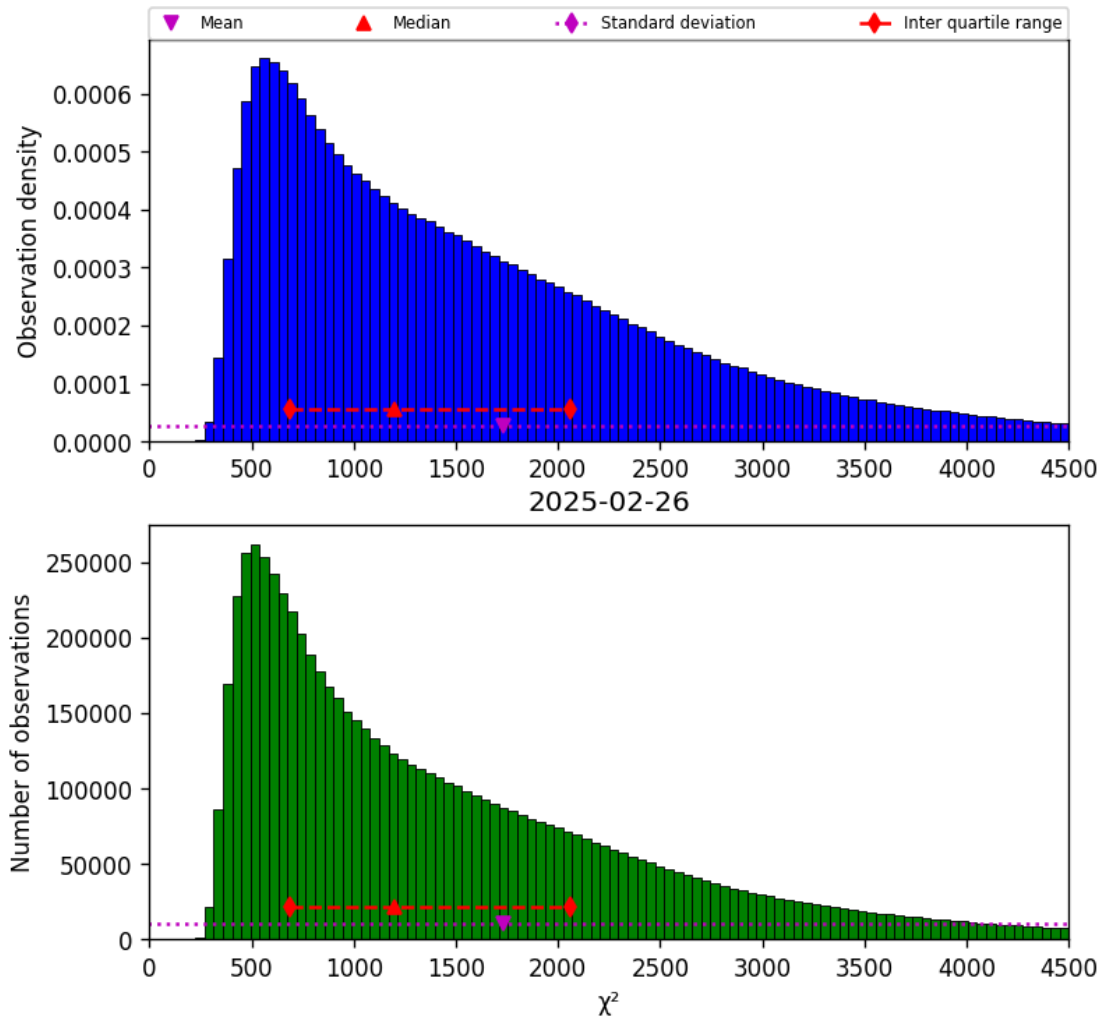
Figure 17: Histogram of “ \chi^2 ” for 2025-02-26 to 2025-02-27
