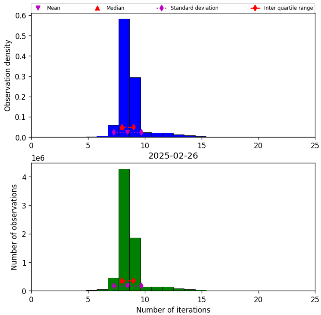
Figure 19: Histogram of “Number of iterations” for 2025-02-26 to 2025-02-27
