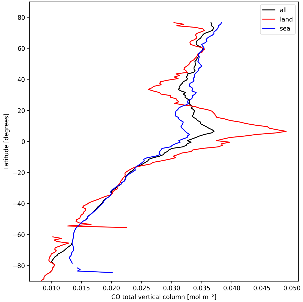
Figure 7: Zonal average of “CO total vertical column” for 2025-02-26 to 2025-02-27.
