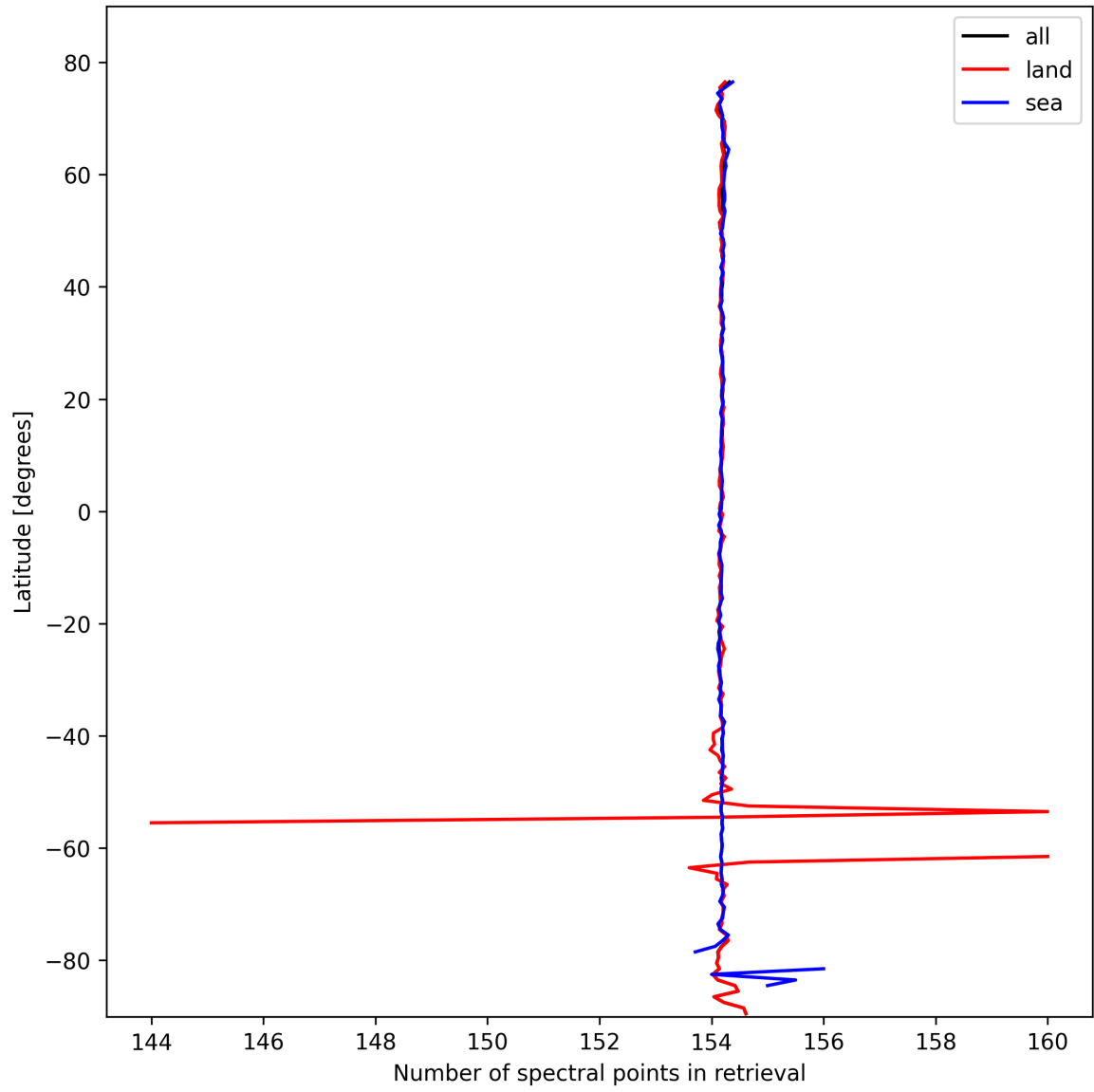
Figure 9: Zonal average of “Number of spectral points in retrieval” for 2025-02-26 to 2025-02-27.
