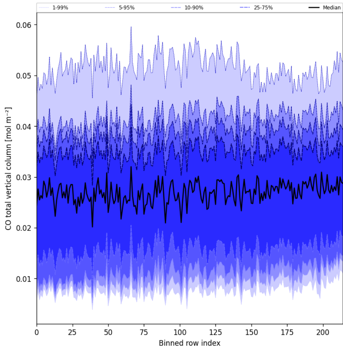
Figure 21: Along track statistics of “CO total vertical column” for 2025-02-26 to 2025-02-27
