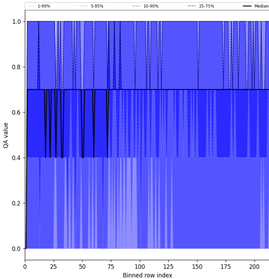
Figure 20: Along track statistics of “QA value” for 2025-02-26 to 2025-02-27
