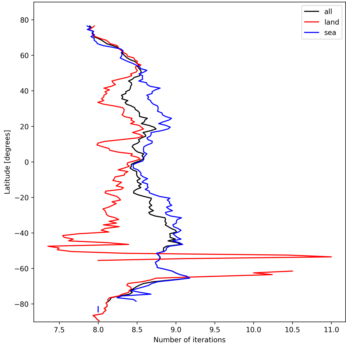
Figure 12: Zonal average of “Number of iterations” for 2025-02-26 to 2025-02-27.
