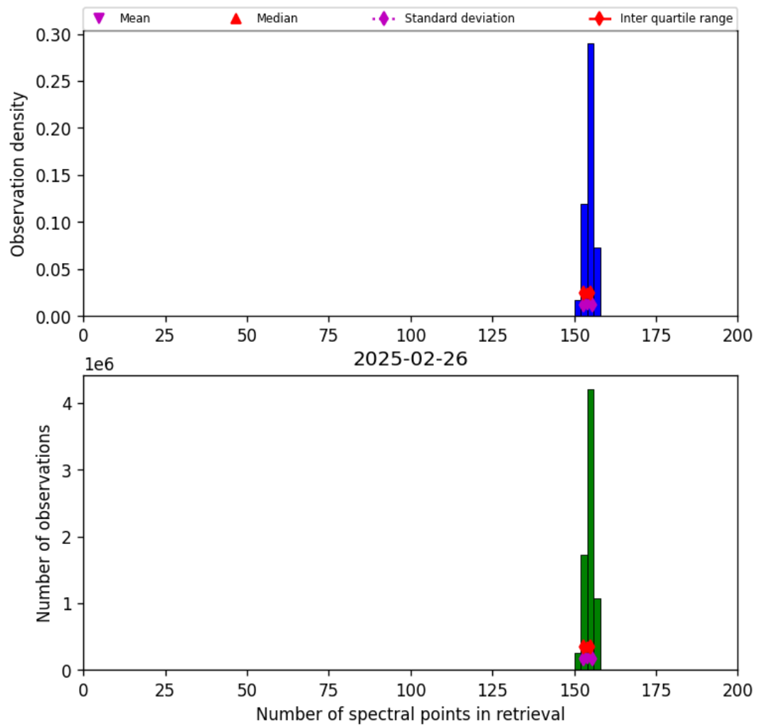
Figure 16: Histogram of “Number of spectral points in retrieval” for 2025-02-26 to 2025-02-27
