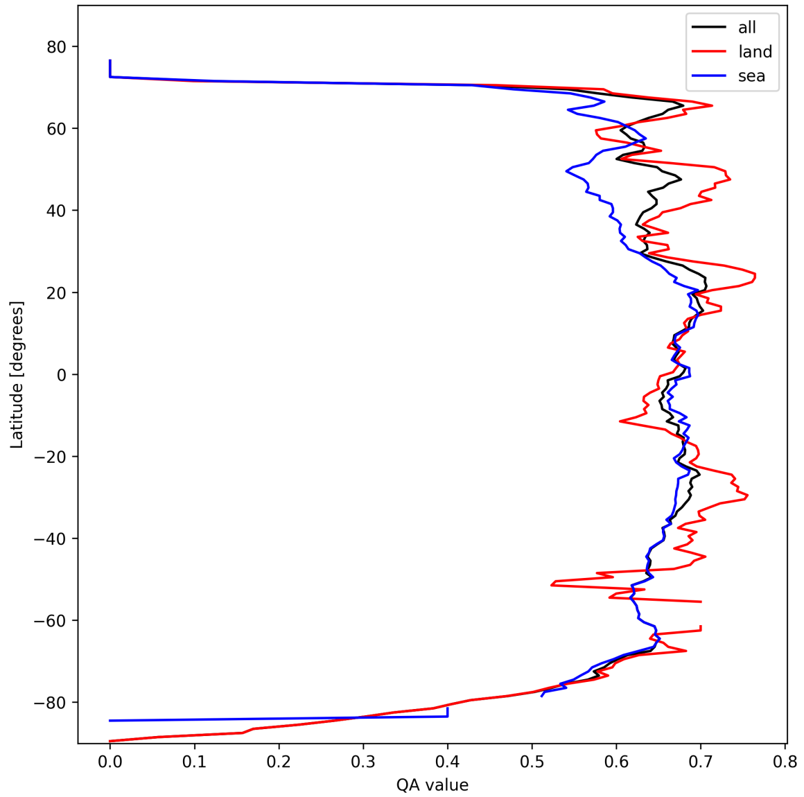
Figure 6: Zonal average of “QA value” for 2025-02-26 to 2025-02-27.
