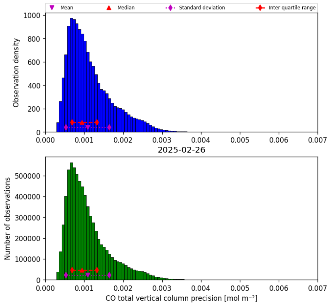
Figure 15: Histogram of “CO total vertical column precision” for 2025-02-26 to 2025-02-27
