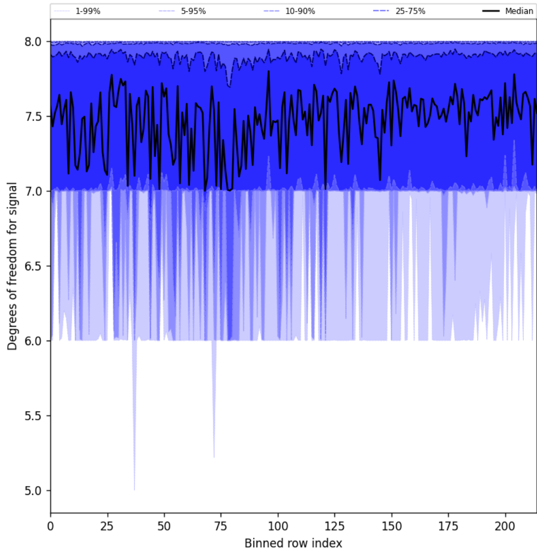
Figure 25: Along track statistics of “Degrees of freedom for signal” for 2025-02-26 to 2025-02-27
