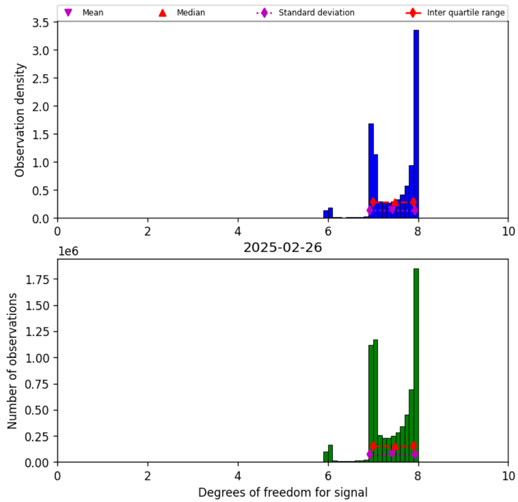
Figure 18: Histogram of “Degrees of freedom for signal” for 2025-02-26 to 2025-02-27
