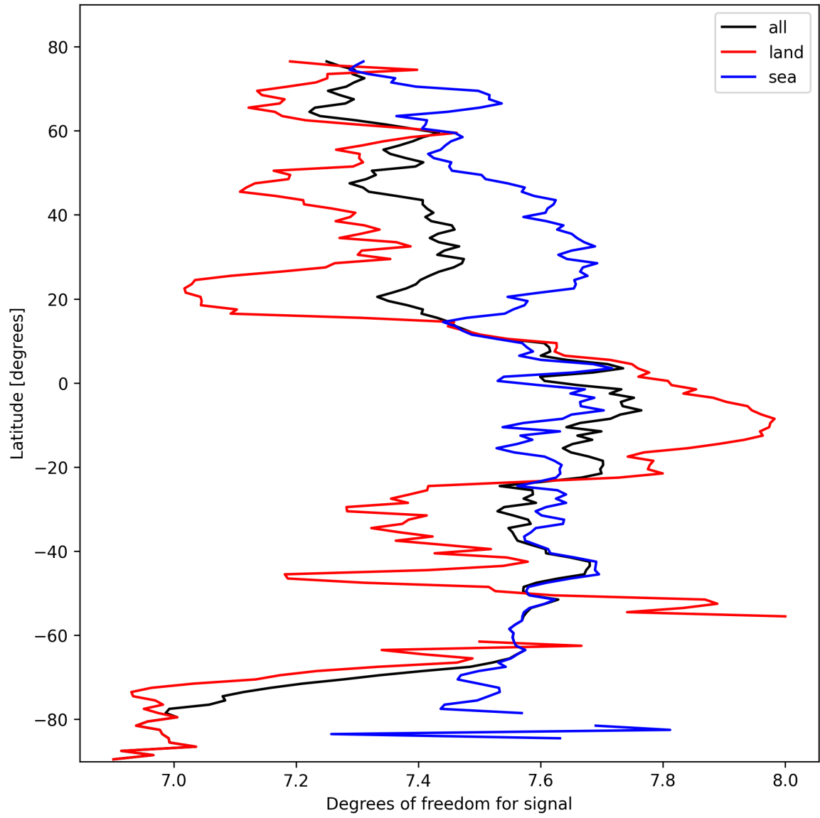
Figure 11: Zonal average of “Degrees of freedom for signal” for 2025-02-26 to 2025-02-27.
