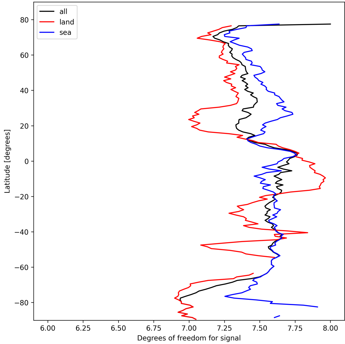
Figure 11: Zonal average of “Degrees of freedom for signal” for 2025-02-27 to 2025-02-27.
