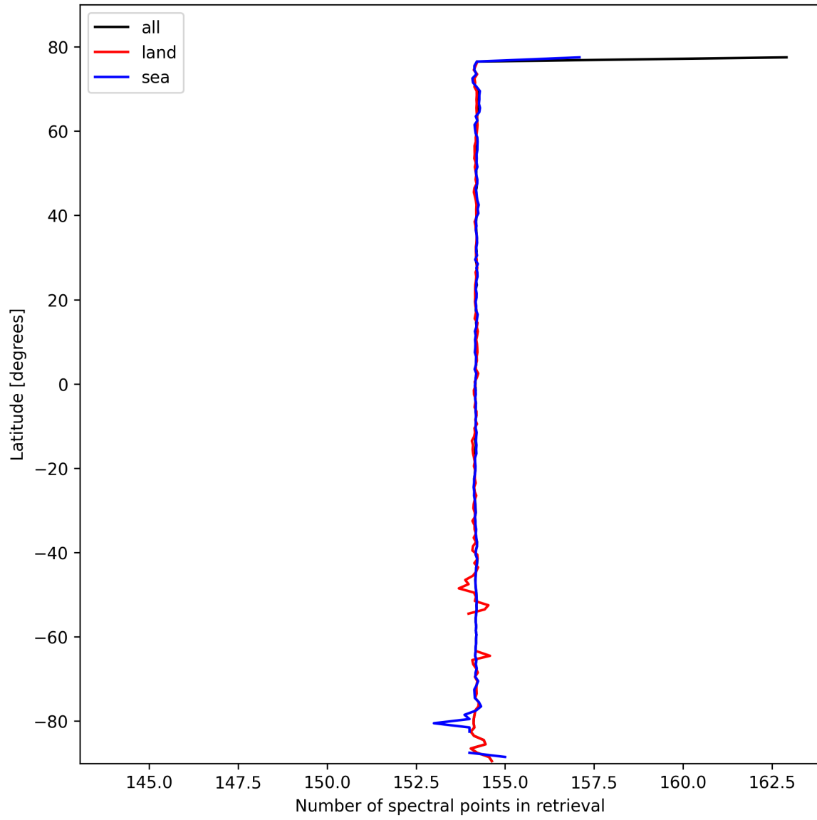
Figure 9: Zonal average of “Number of spectral points in retrieval” for 2025-02-27 to 2025-02-27.
