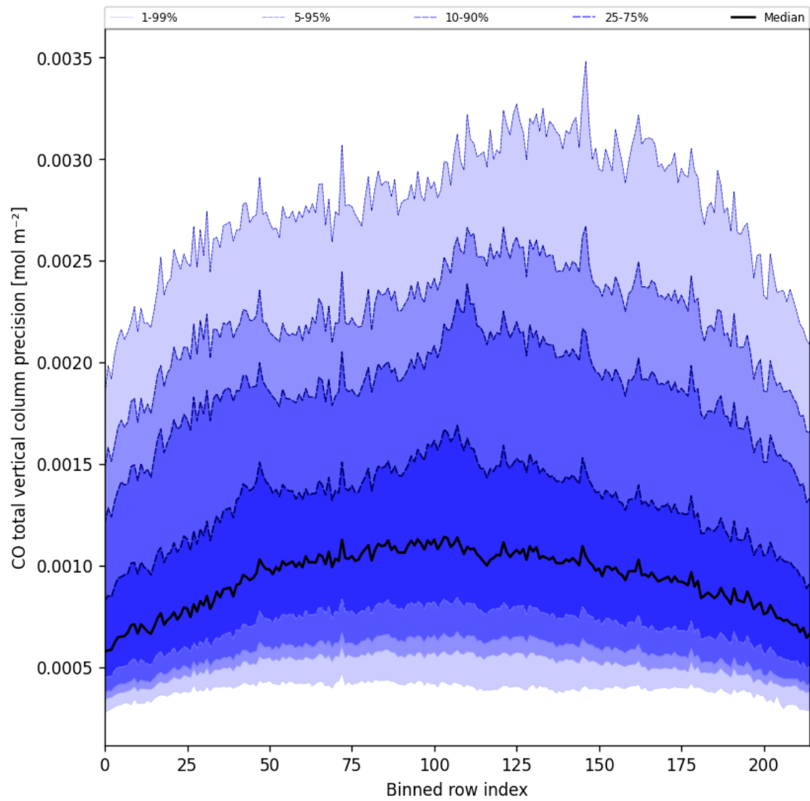
Figure 22: Along track statistics of “CO total vertical column precision” for 2025-02-27 to 2025-02-27
