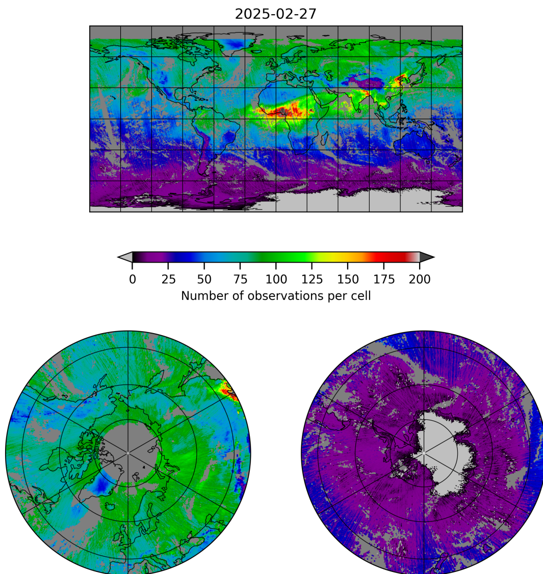
Figure 5: Map of the number of observations for 2025-02-27 to 2025-02-27
