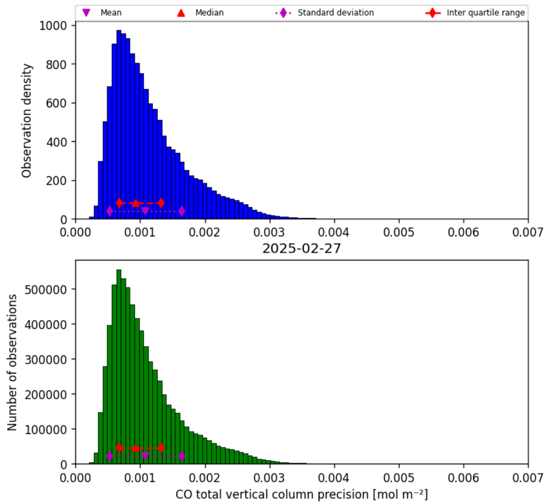
Figure 15: Histogram of “CO total vertical column precision” for 2025-02-27 to 2025-02-27
