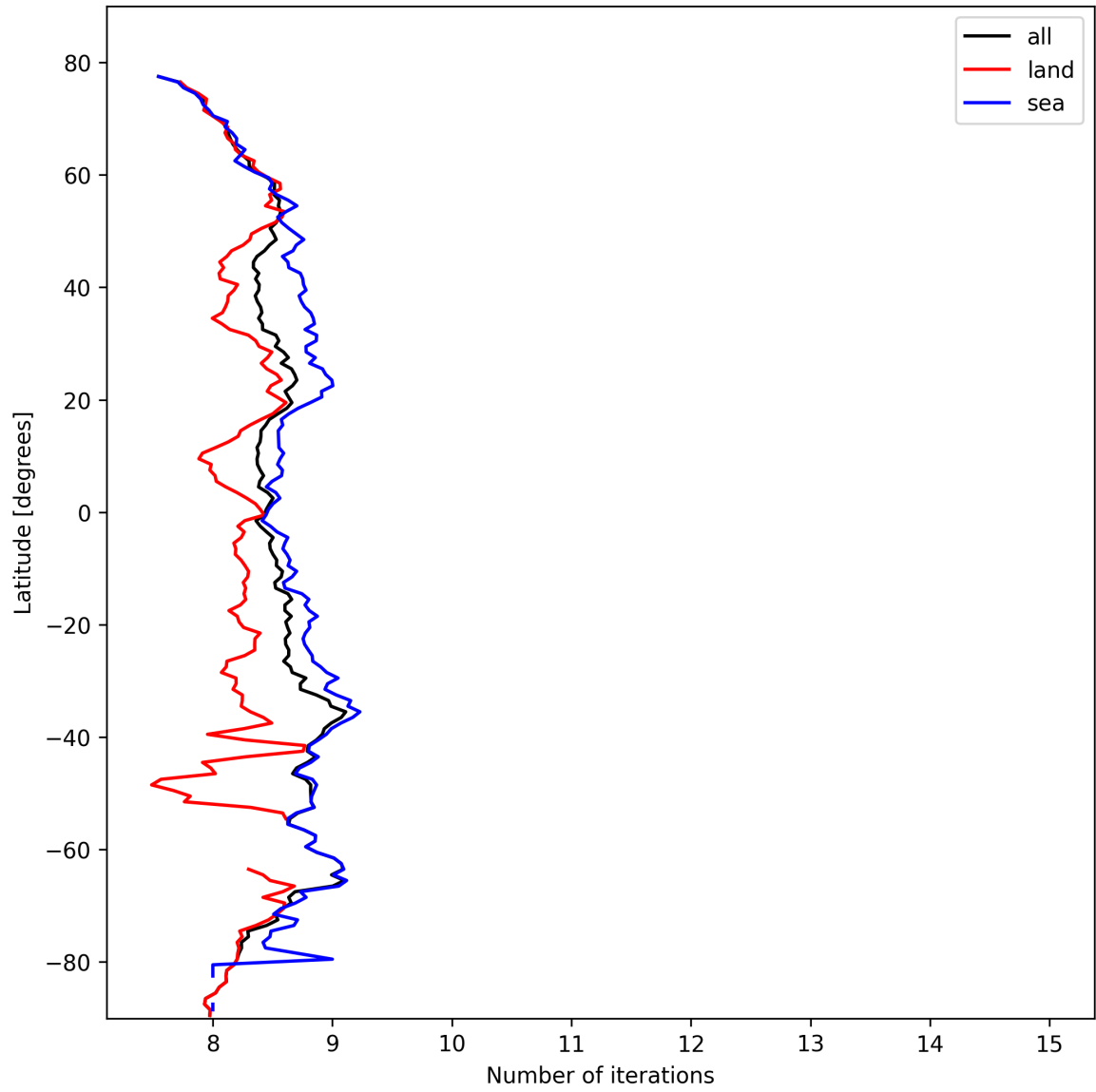
Figure 12: Zonal average of “Number of iterations” for 2025-02-27 to 2025-02-27.
