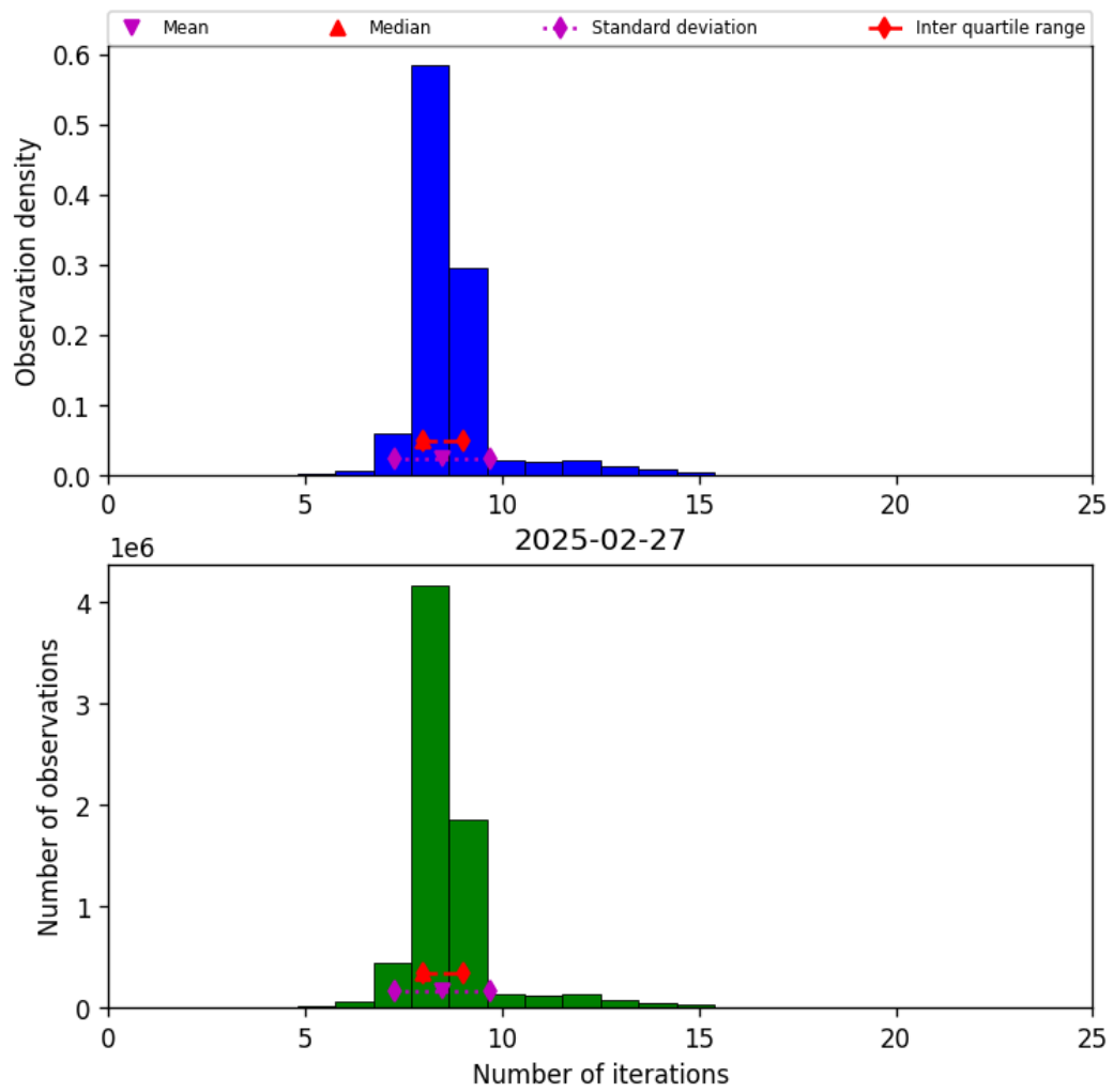
Figure 19: Histogram of “Number of iterations” for 2025-02-27 to 2025-02-27
