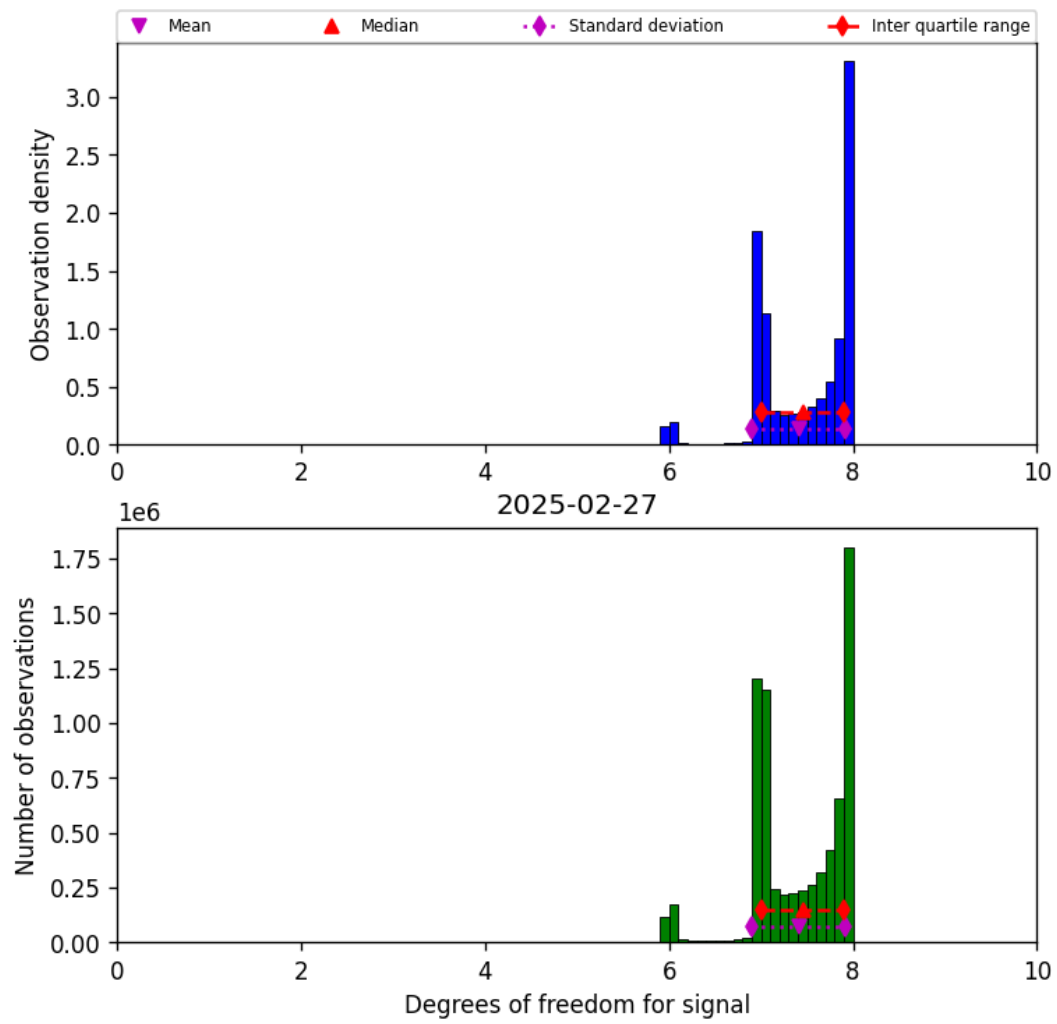
Figure 18: Histogram of “Degrees of freedom for signal” for 2025-02-27 to 2025-02-27
