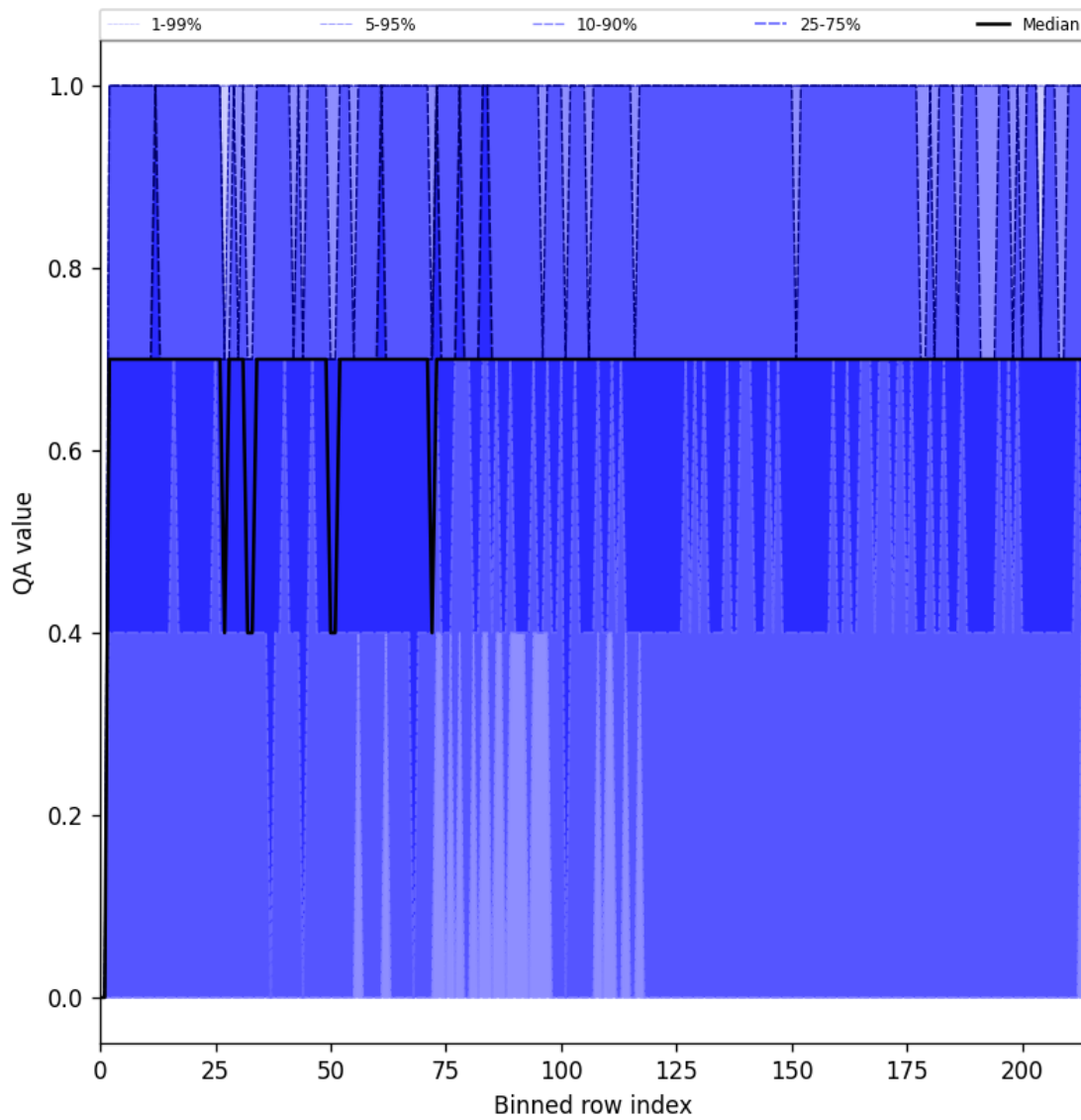
Figure 20: Along track statistics of “QA value” for 2025-02-27 to 2025-02-27
