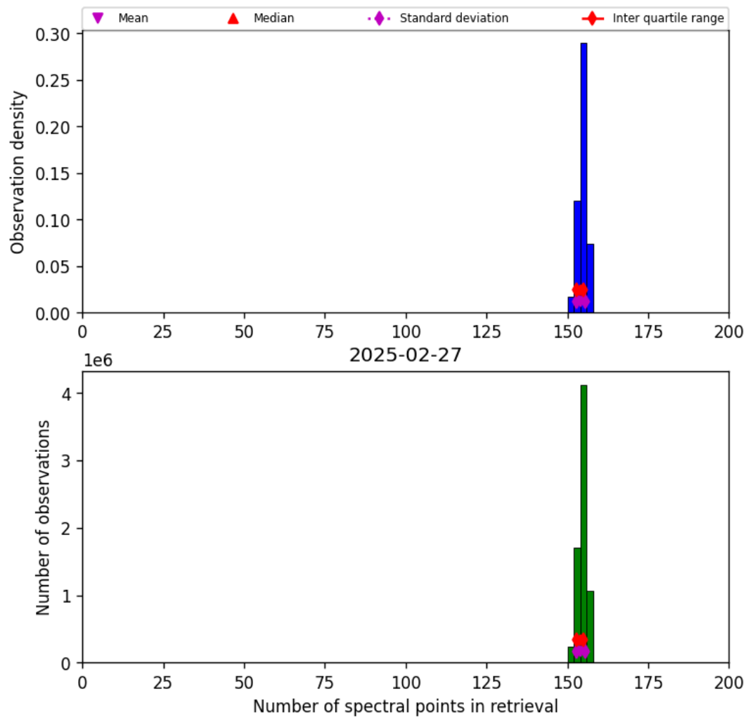
Figure 16: Histogram of “Number of spectral points in retrieval” for 2025-02-27 to 2025-02-27
