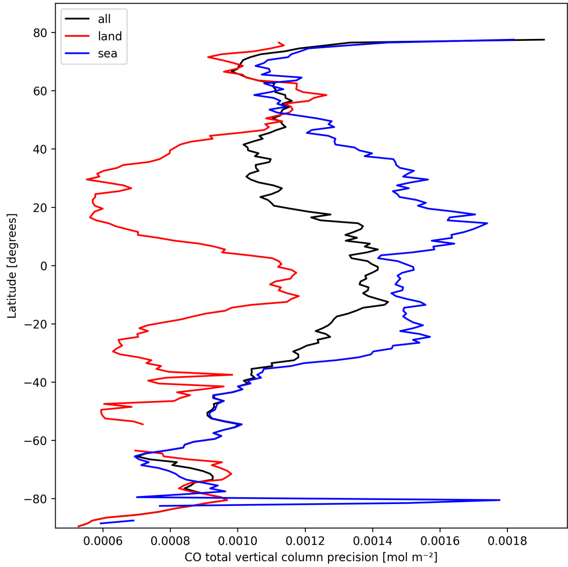
Figure 8: Zonal average of “CO total vertical column precision” for 2025-02-27 to 2025-02-27.
