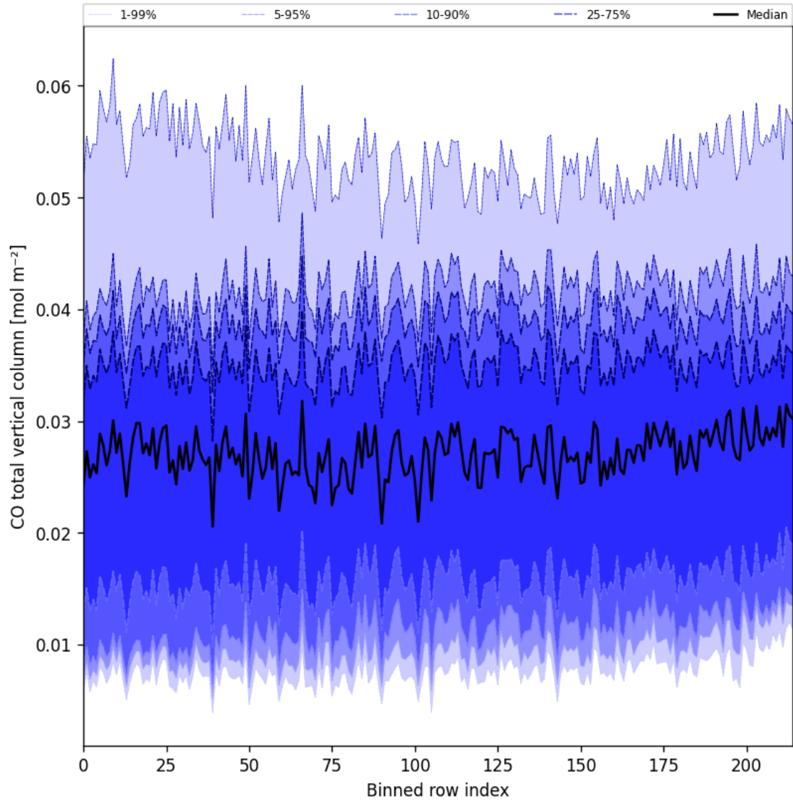
Figure 21: Along track statistics of “CO total vertical column” for 2025-02-27 to 2025-02-27
