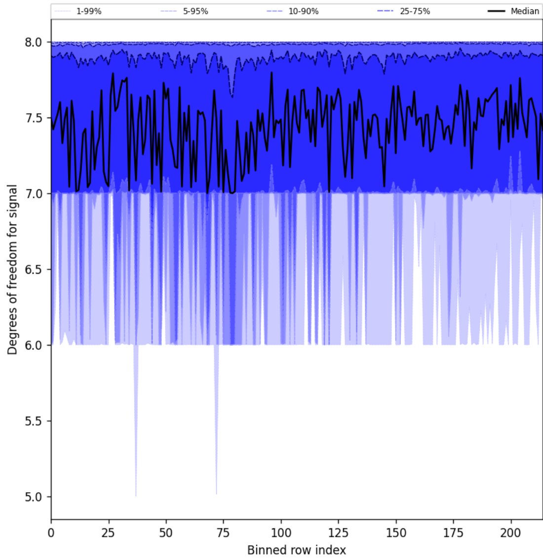
Figure 25: Along track statistics of “Degrees of freedom for signal” for 2025-02-27 to 2025-02-27
