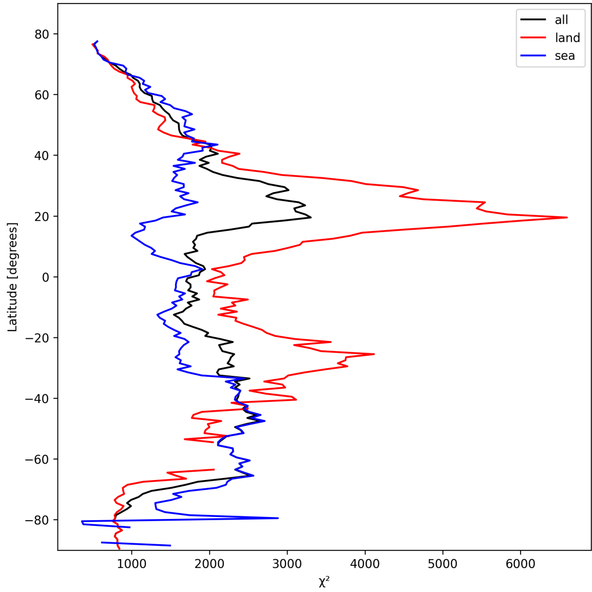
Figure 10: Zonal average of “ \chi^2 ” for 2025-02-27 to 2025-02-27.
