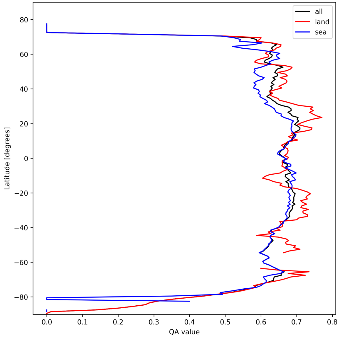
Figure 6: Zonal average of “QA value” for 2025-02-27 to 2025-02-27.
