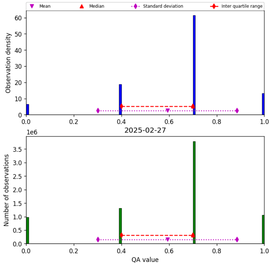
Figure 13: Histogram of “QA value” for 2025-02-27 to 2025-02-27
