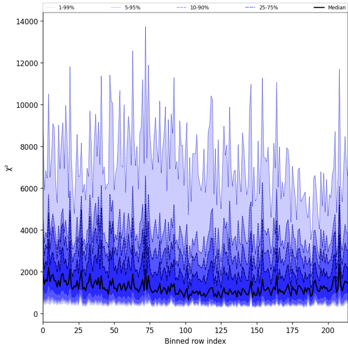
Figure 24: Along track statistics of “ \chi^2 ” for 2025-02-27 to 2025-02-27
