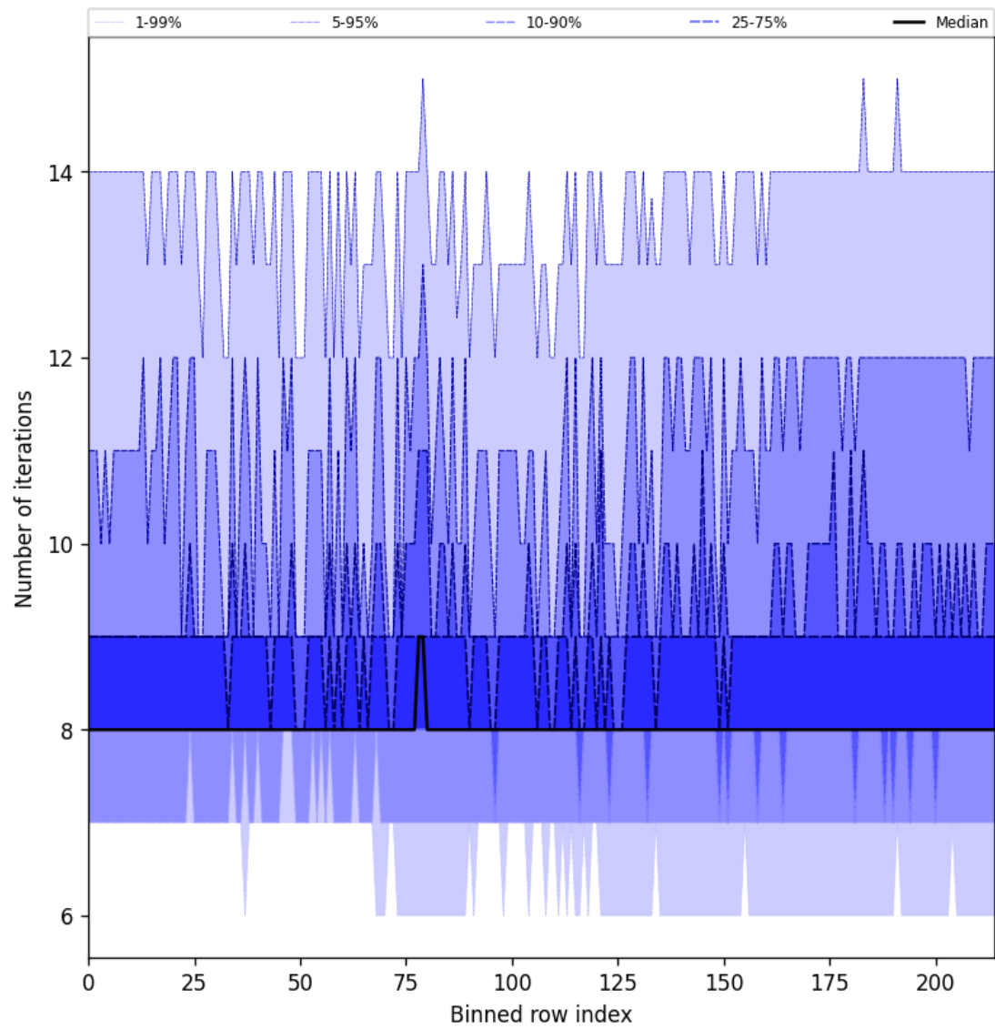
Figure 26: Along track statistics of “Number of iterations” for 2025-02-27 to 2025-02-27
