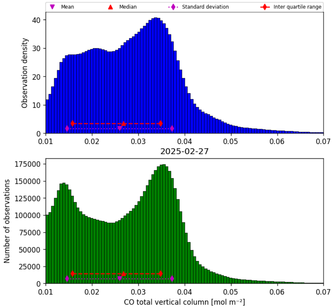
Figure 14: Histogram of “CO total vertical column” for 2025-02-27 to 2025-02-27
