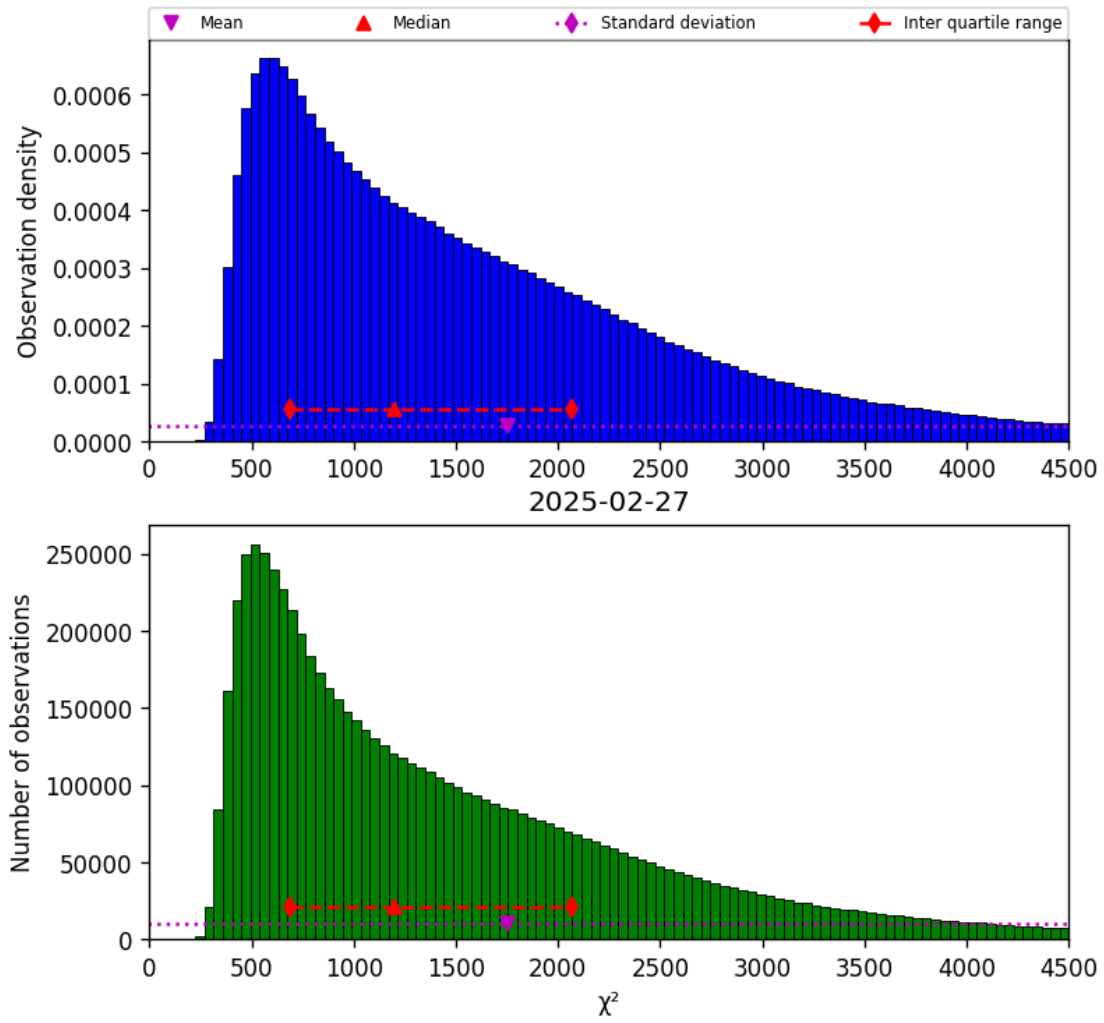
Figure 17: Histogram of " \chi^2 " for 2025-02-27 to 2025-02-27
