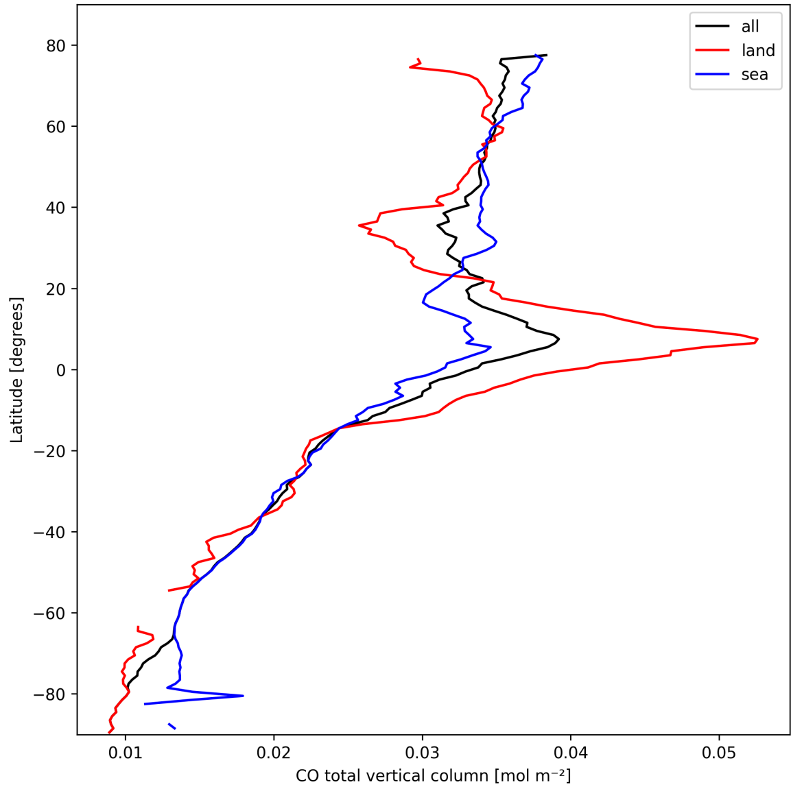
Figure 7: Zonal average of “CO total vertical column” for 2025-02-27 to 2025-02-27.
