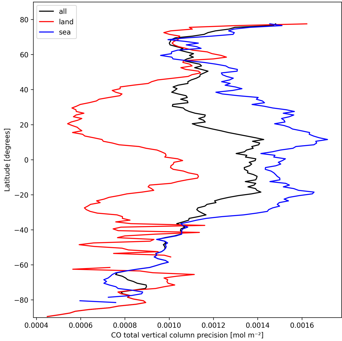
Figure 8: Zonal average of “CO total vertical column precision” for 2025-02-28 to 2025-03-01.
