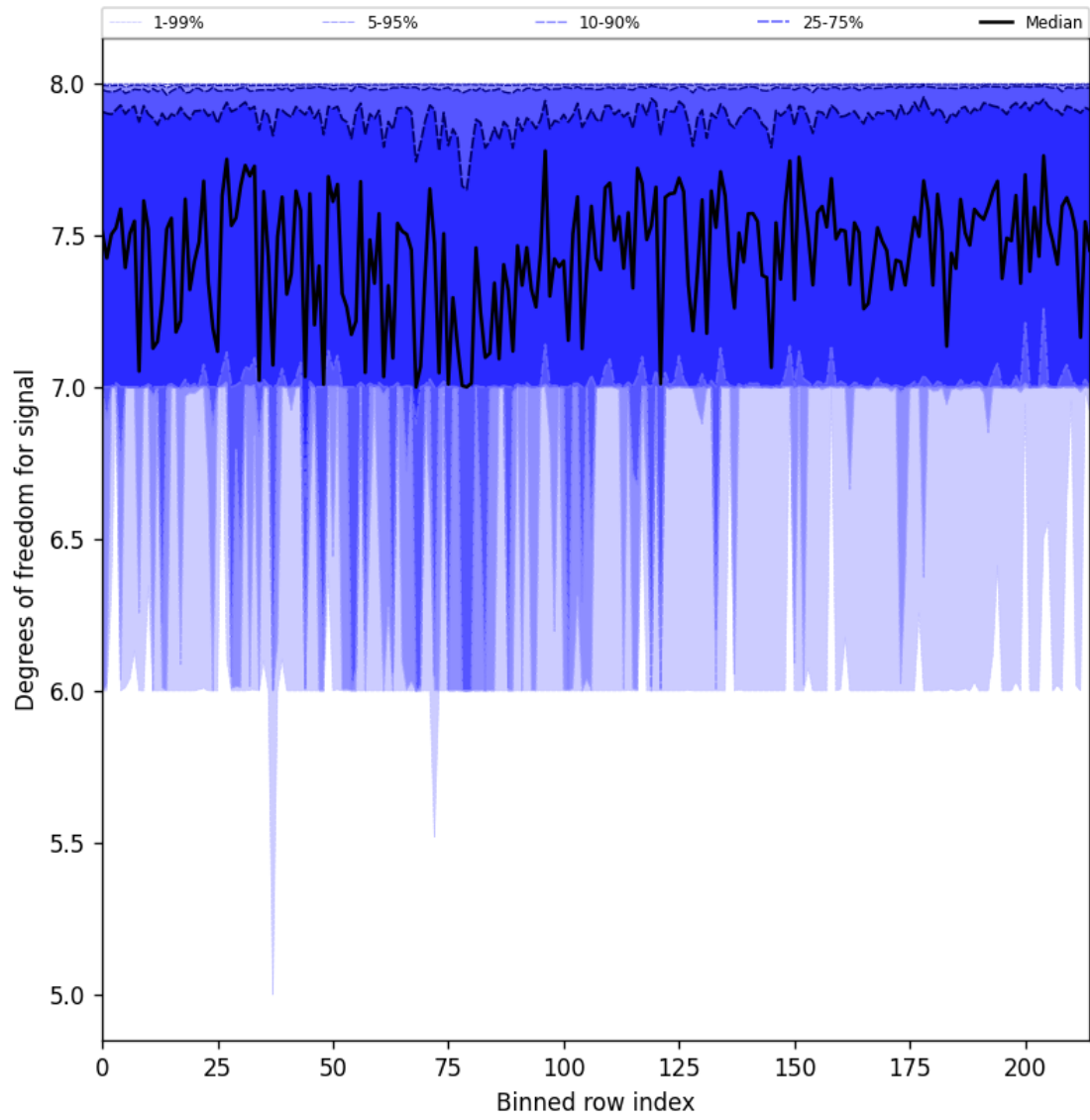
Figure 25: Along track statistics of “Degrees of freedom for signal” for 2025-02-28 to 2025-03-01
