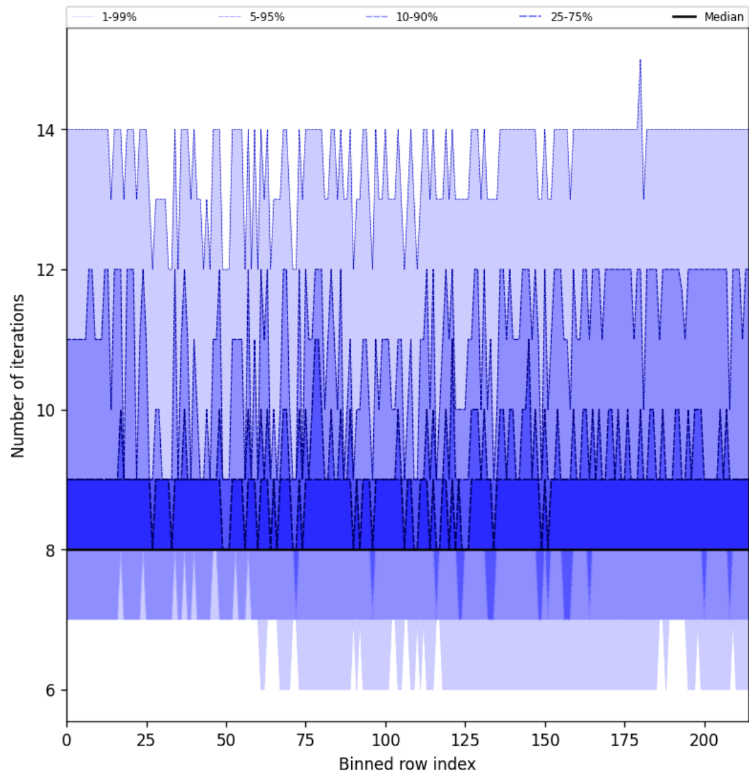
Figure 26: Along track statistics of “Number of iterations” for 2025-02-28 to 2025-03-01
