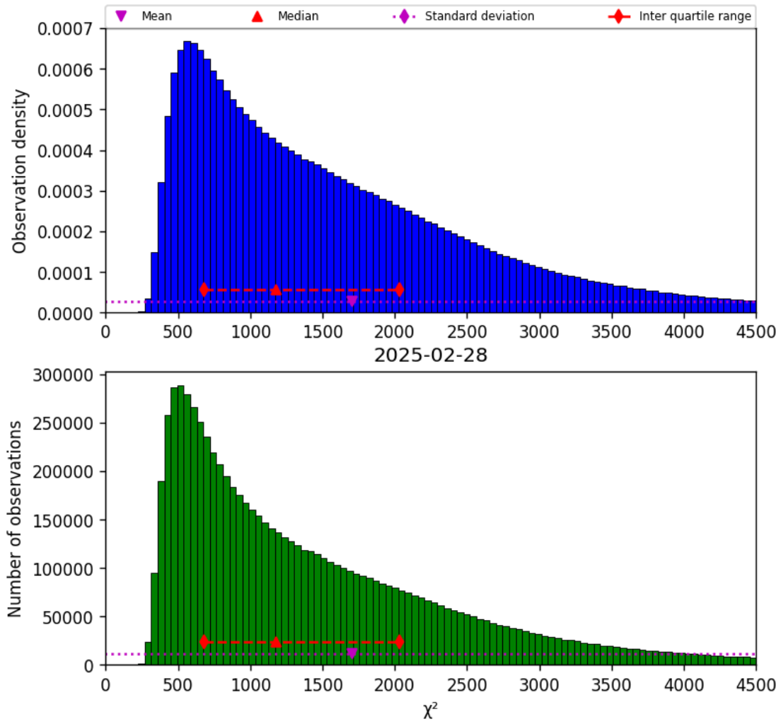
Figure 17: Histogram of " \chi^2 " for 2025-02-28 to 2025-03-01
