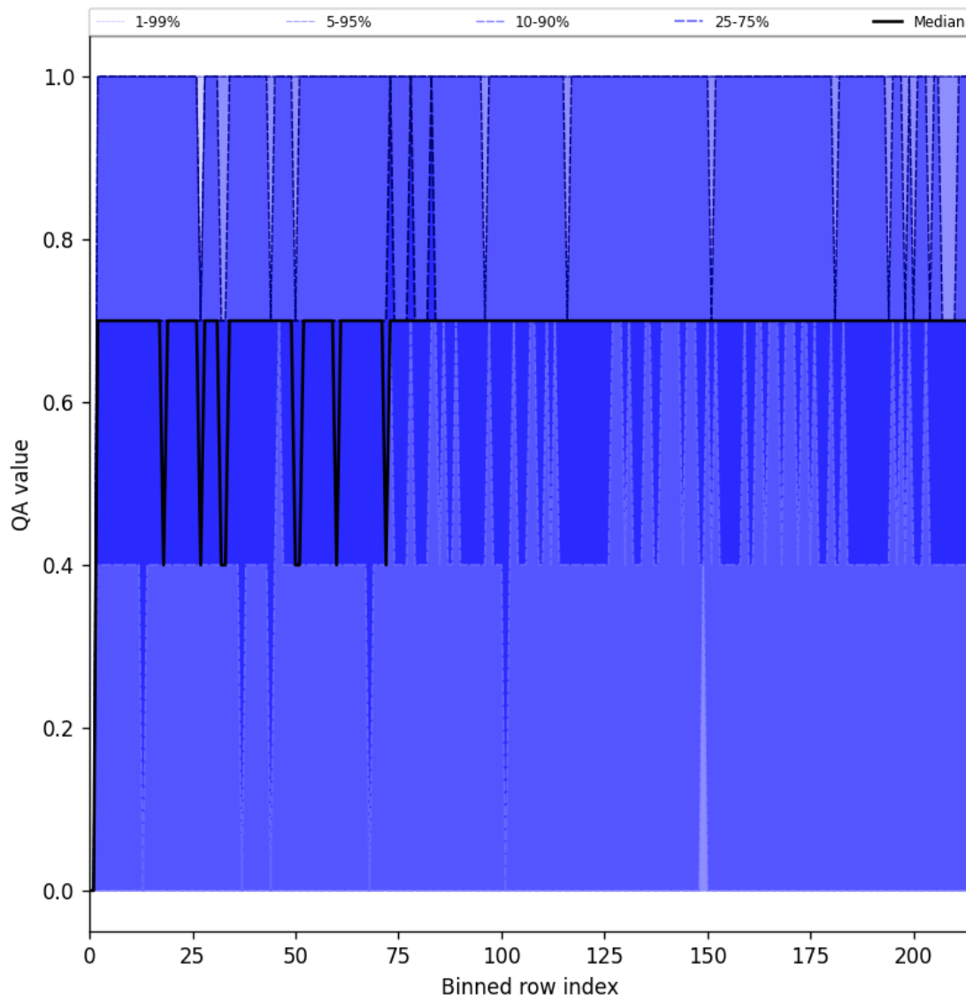
Figure 20: Along track statistics of “QA value” for 2025-02-28 to 2025-03-01
