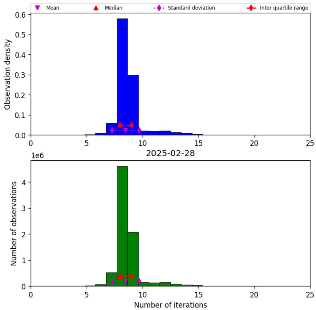
Figure 19: Histogram of “Number of iterations” for 2025-02-28 to 2025-03-01
