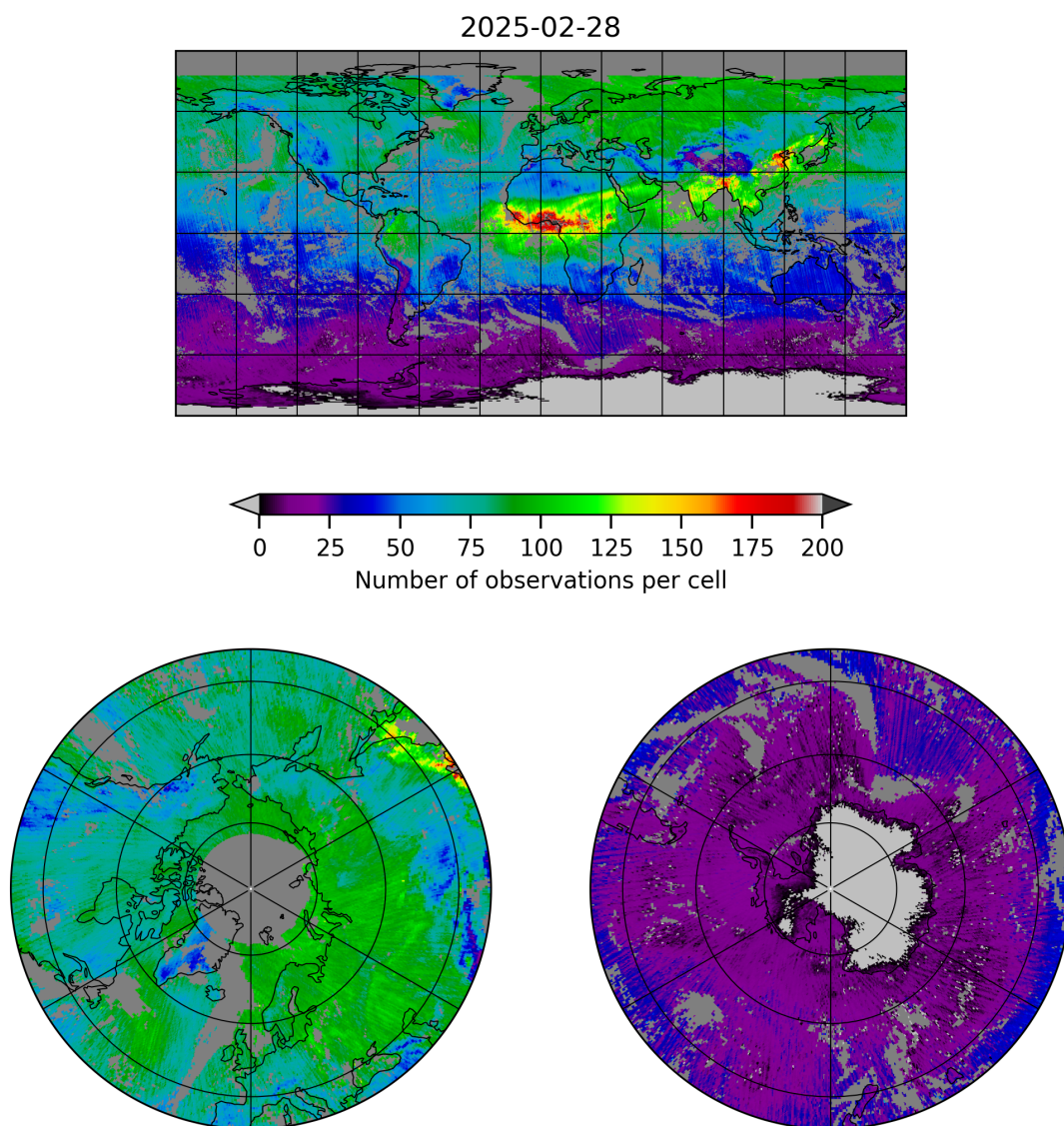
Figure 5: Map of the number of observations for 2025-02-28 to 2025-03-01
