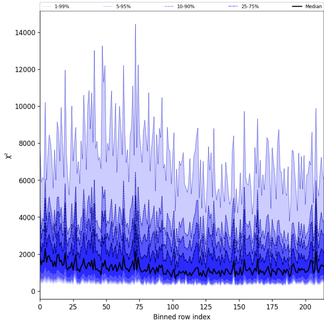
Figure 24: Along track statistics of “ \chi^2 ” for 2025-02-28 to 2025-03-01
