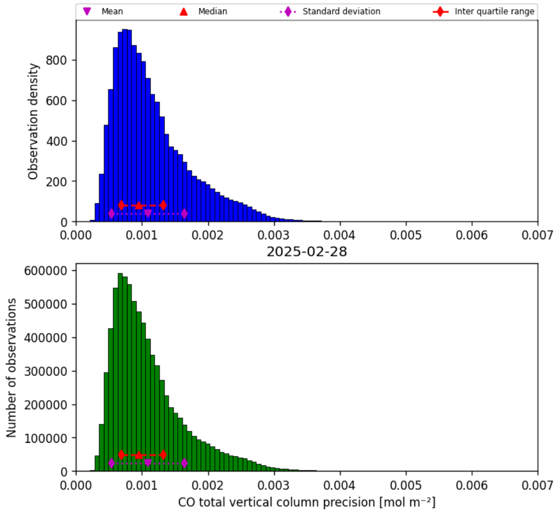
Figure 15: Histogram of “CO total vertical column precision” for 2025-02-28 to 2025-03-01
