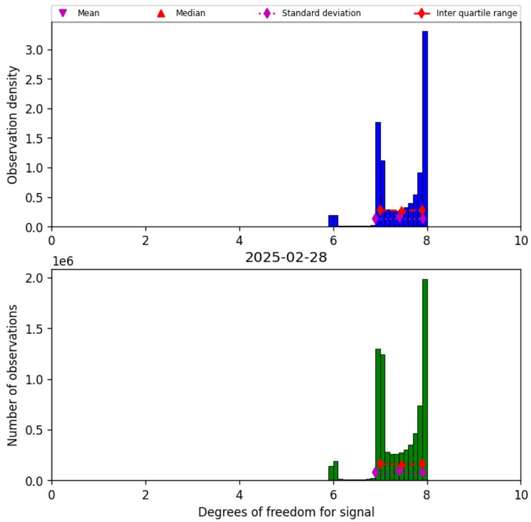
Figure 18: Histogram of “Degrees of freedom for signal” for 2025-02-28 to 2025-03-01
