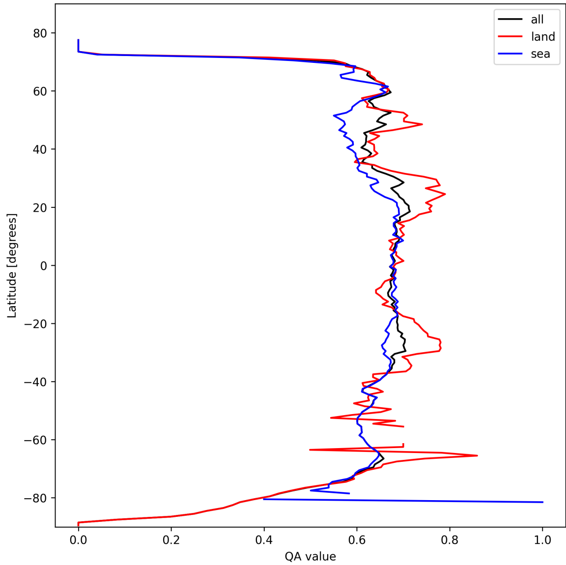
Figure 6: Zonal average of “QA value” for 2025-02-28 to 2025-03-01.
