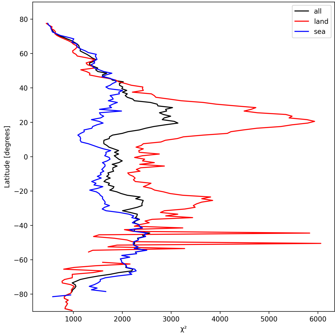
Figure 10: Zonal average of “ \chi^2 ” for 2025-02-28 to 2025-03-01.
