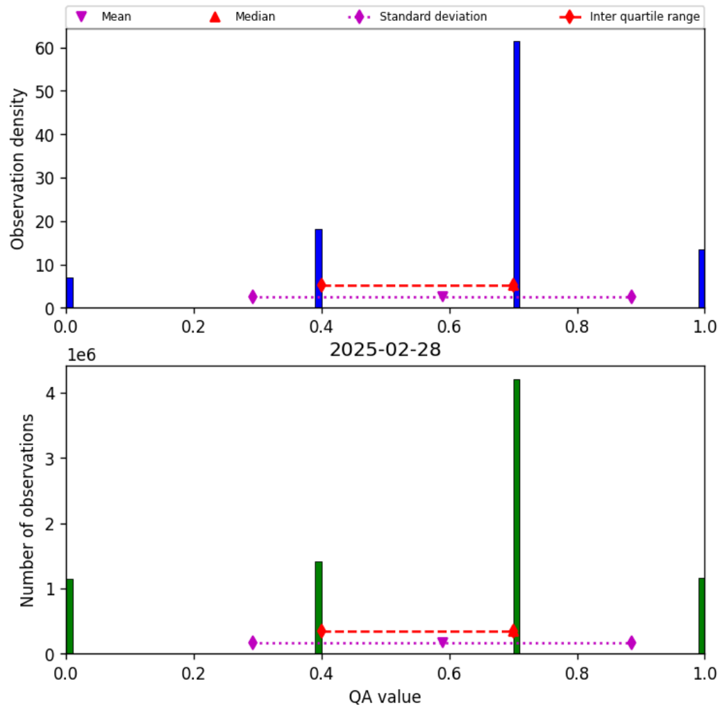
Figure 13: Histogram of “QA value” for 2025-02-28 to 2025-03-01
