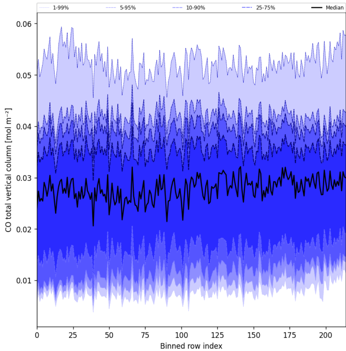
Figure 21: Along track statistics of “CO total vertical column” for 2025-02-28 to 2025-03-01
