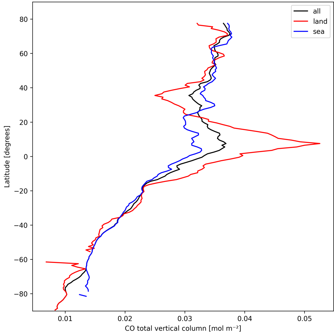
Figure 7: Zonal average of “CO total vertical column” for 2025-02-28 to 2025-03-01.
