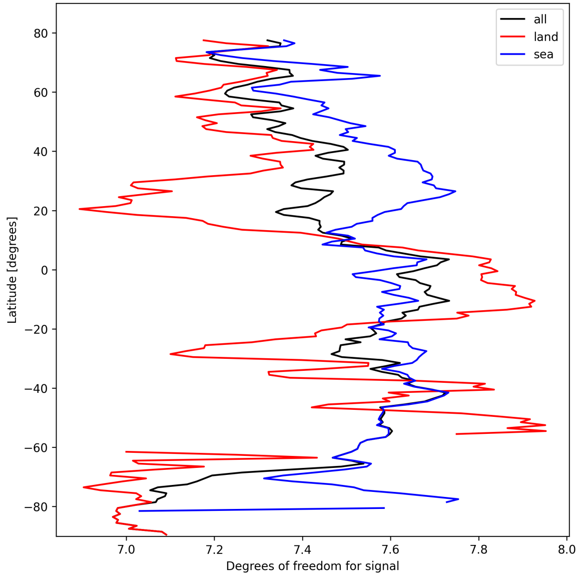
Figure 11: Zonal average of “Degrees of freedom for signal” for 2025-02-28 to 2025-03-01.
