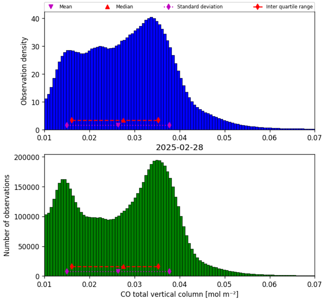
Figure 14: Histogram of “CO total vertical column” for 2025-02-28 to 2025-03-01
