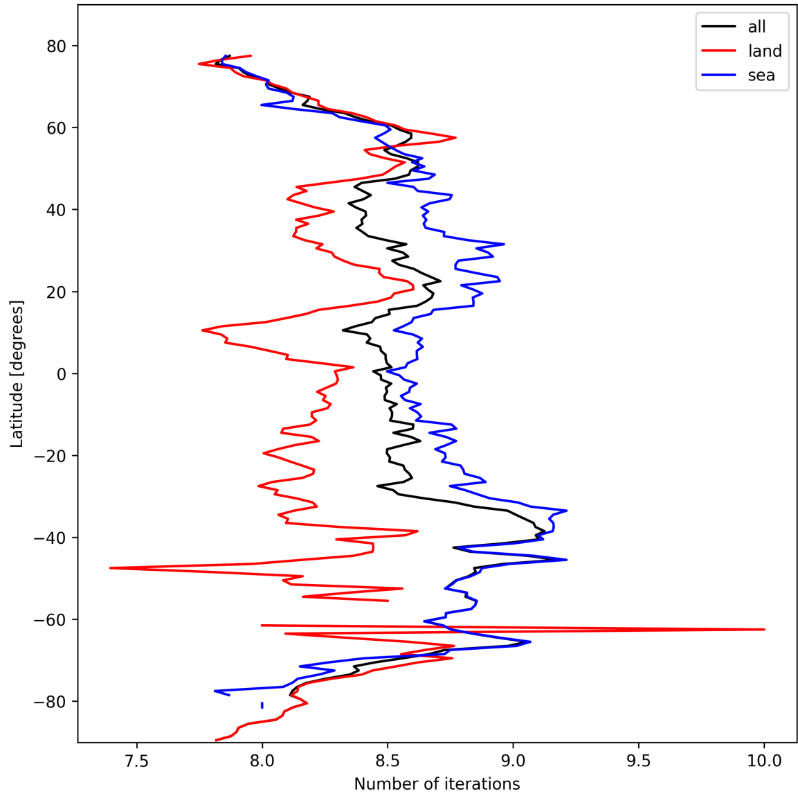
Figure 12: Zonal average of “Number of iterations” for 2025-02-28 to 2025-03-01.
