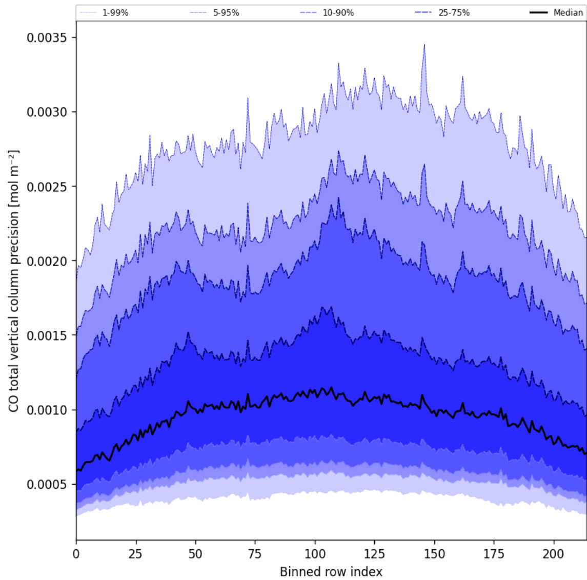
Figure 22: Along track statistics of “CO total vertical column precision” for 2025-02-28 to 2025-03-01
