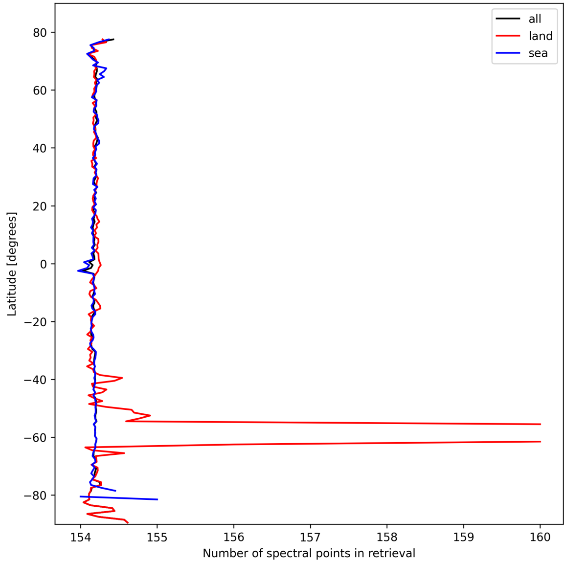
Figure 9: Zonal average of “Number of spectral points in retrieval” for 2025-02-28 to 2025-03-01.
