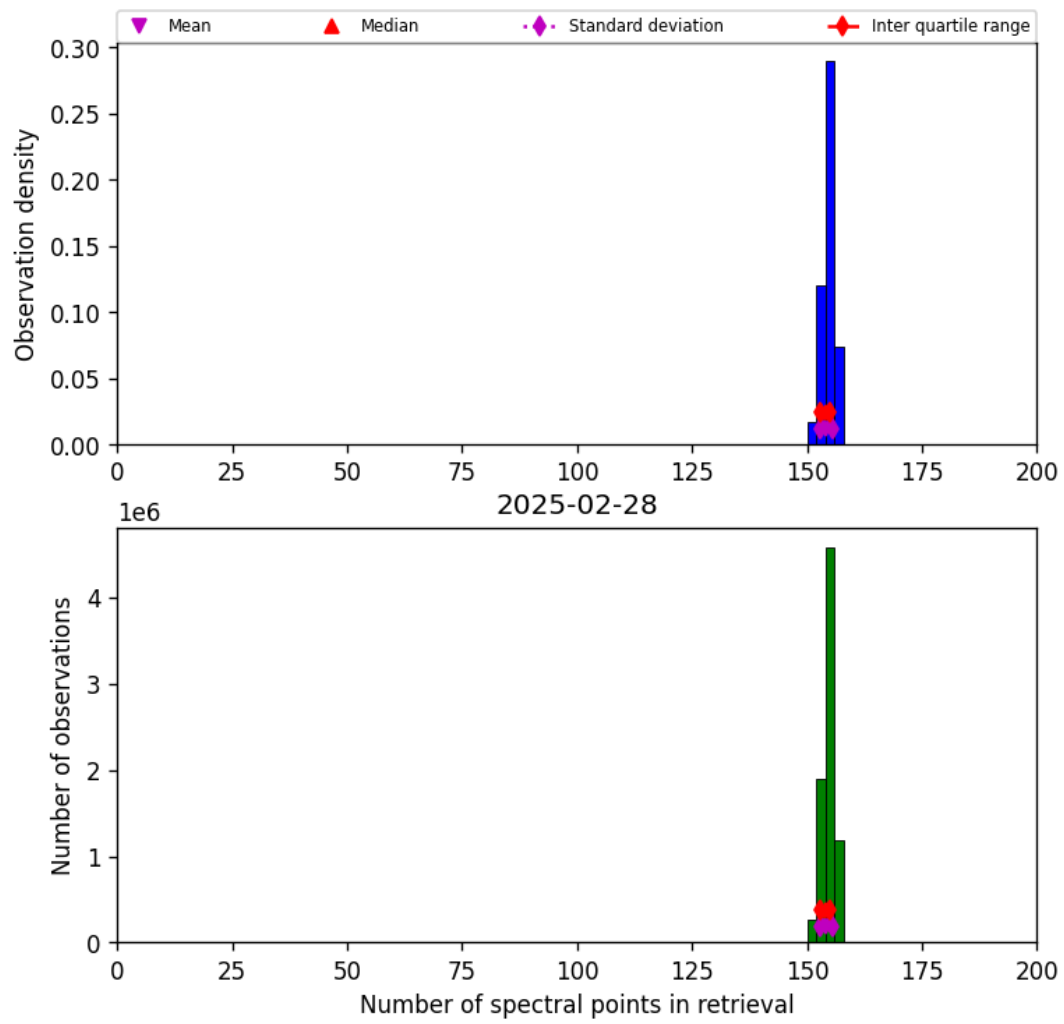
Figure 16: Histogram of “Number of spectral points in retrieval” for 2025-02-28 to 2025-03-01
