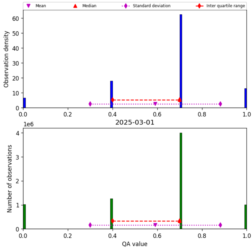
Figure 13: Histogram of “QA value” for 2025-03-01 to 2025-03-02
