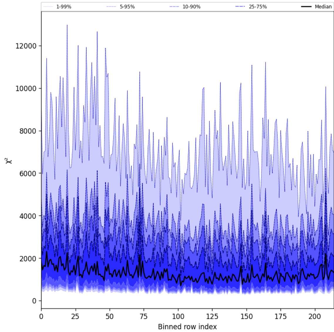
Figure 24: Along track statistics of “ \chi^2 ” for 2025-03-01 to 2025-03-02
