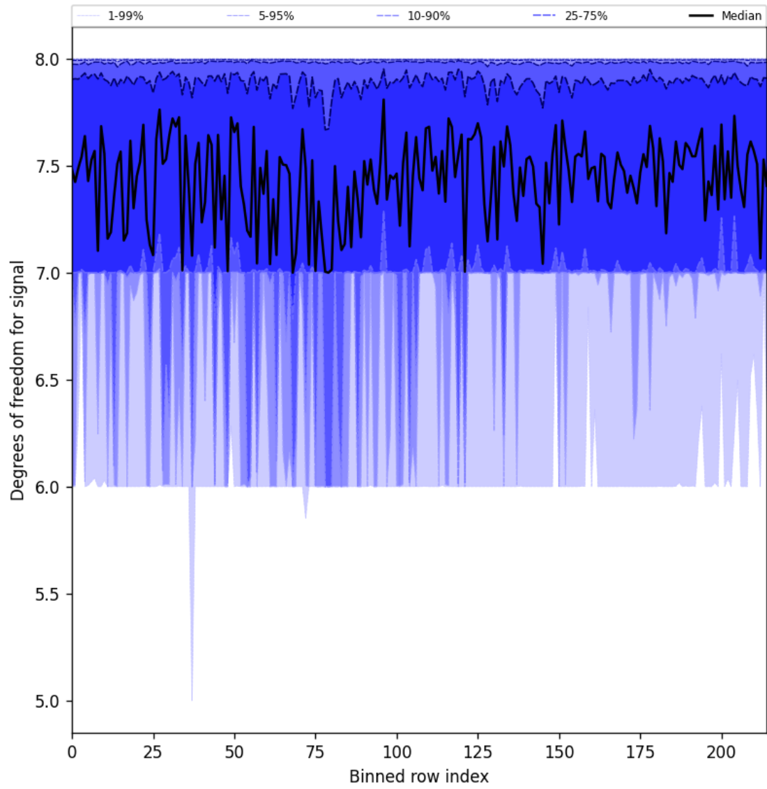
Figure 25: Along track statistics of “Degrees of freedom for signal” for 2025-03-01 to 2025-03-02
