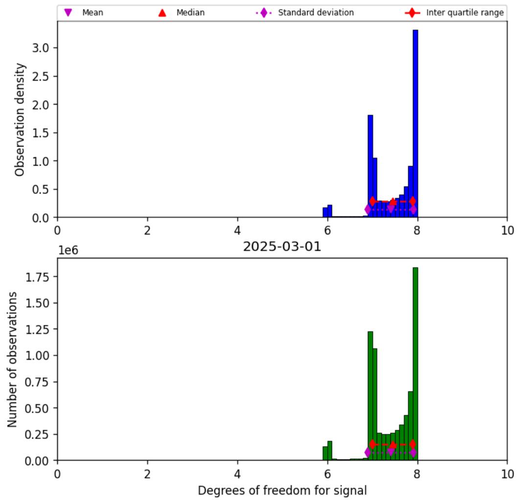
Figure 18: Histogram of “Degrees of freedom for signal” for 2025-03-01 to 2025-03-02
