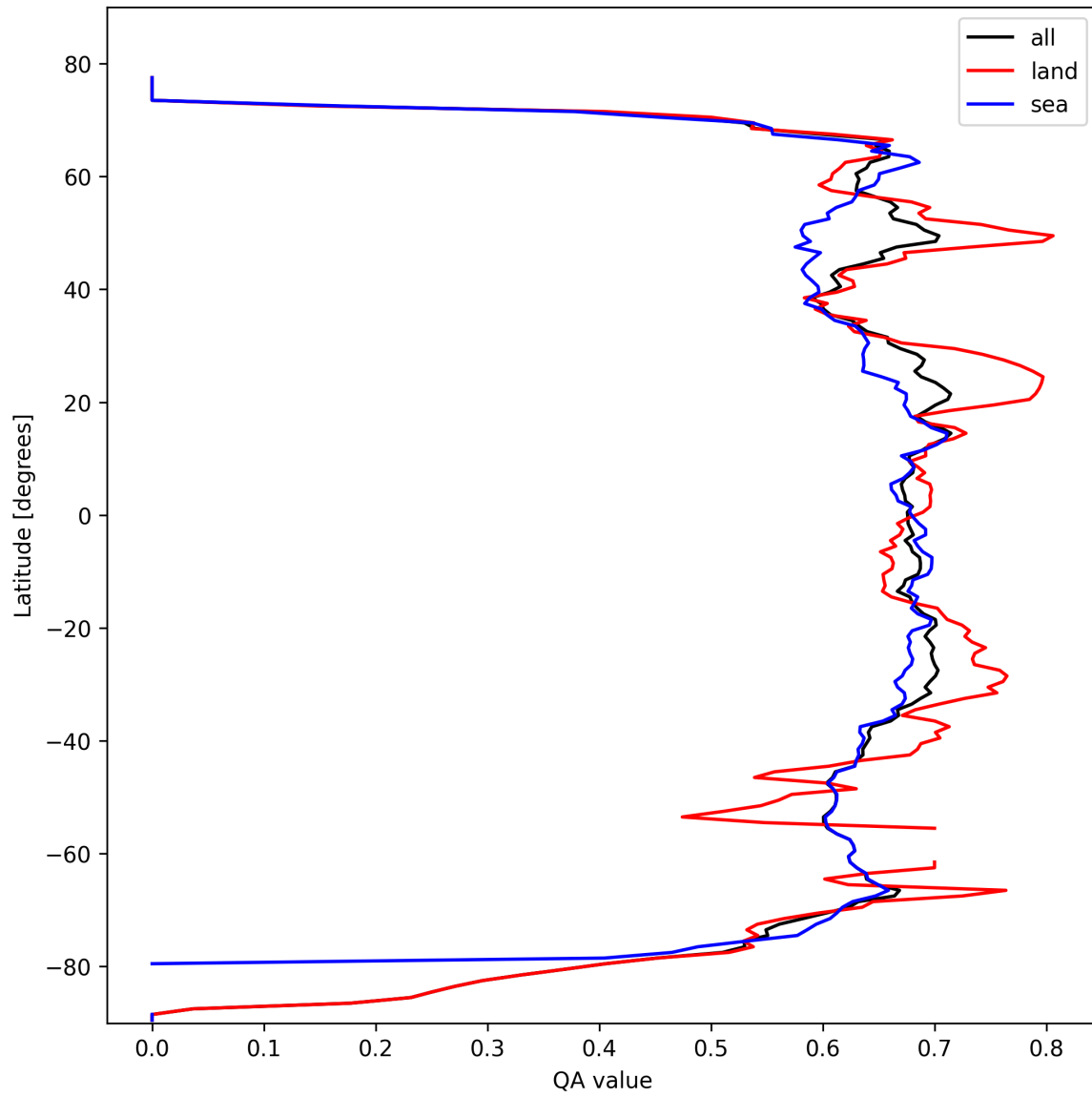
Figure 6: Zonal average of “QA value” for 2025-03-01 to 2025-03-02.
