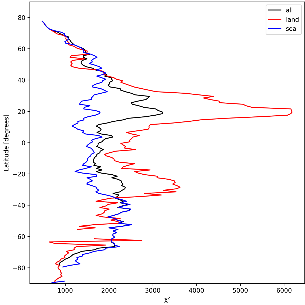
Figure 10: Zonal average of “ \chi^2 ” for 2025-03-01 to 2025-03-02.
