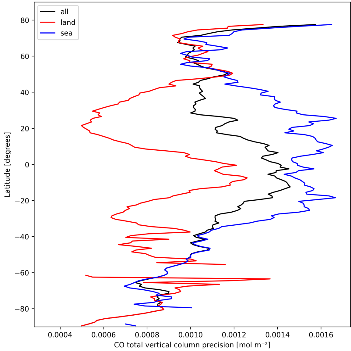
Figure 8: Zonal average of “CO total vertical column precision” for 2025-03-01 to 2025-03-02.
