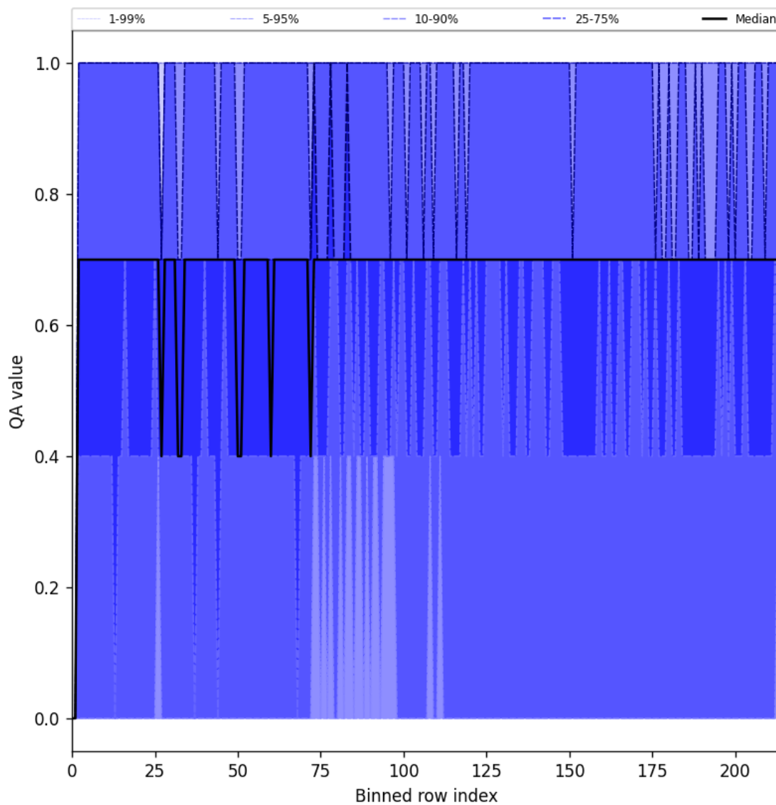
Figure 20: Along track statistics of “QA value” for 2025-03-01 to 2025-03-02
