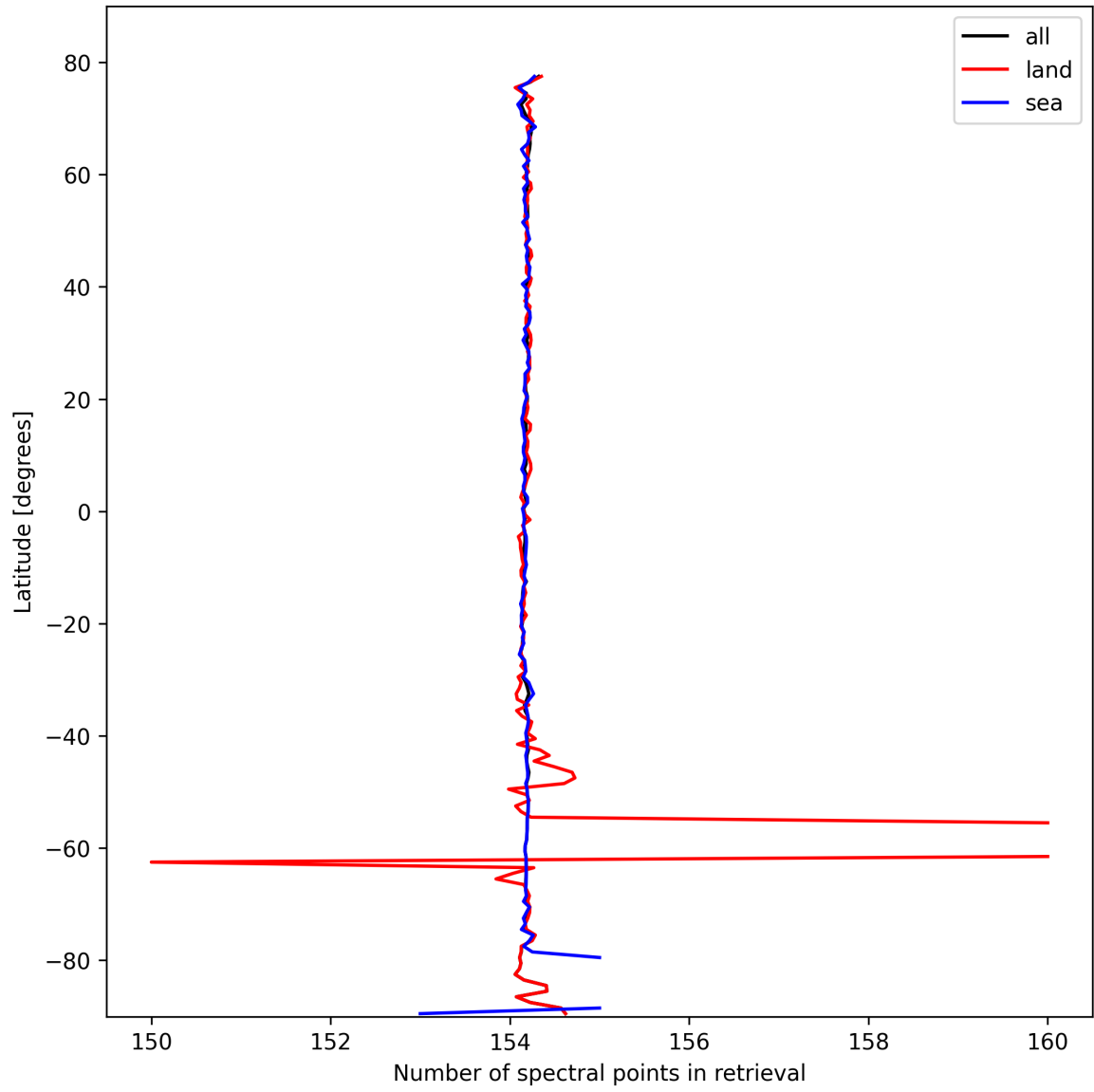
Figure 9: Zonal average of “Number of spectral points in retrieval” for 2025-03-01 to 2025-03-02.
