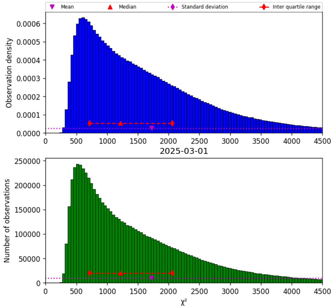
Figure 17: Histogram of “ \chi^2 ” for 2025-03-01 to 2025-03-02
