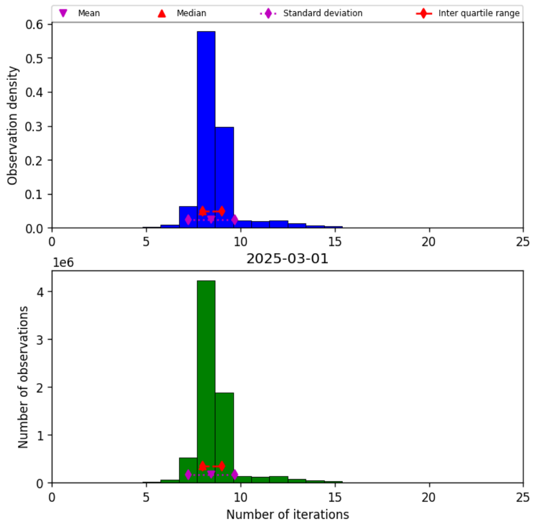
Figure 19: Histogram of “Number of iterations” for 2025-03-01 to 2025-03-02
