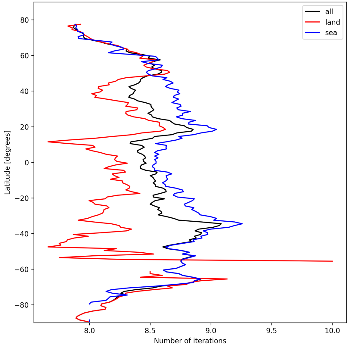
Figure 12: Zonal average of “Number of iterations” for 2025-03-01 to 2025-03-02.
