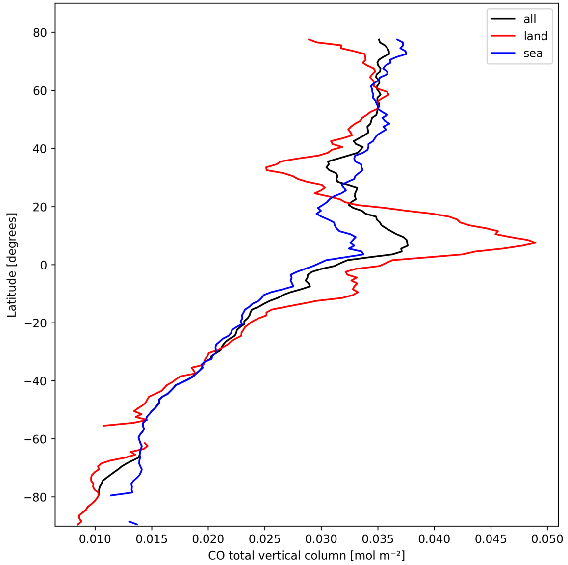
Figure 7: Zonal average of “CO total vertical column” for 2025-03-01 to 2025-03-02.
