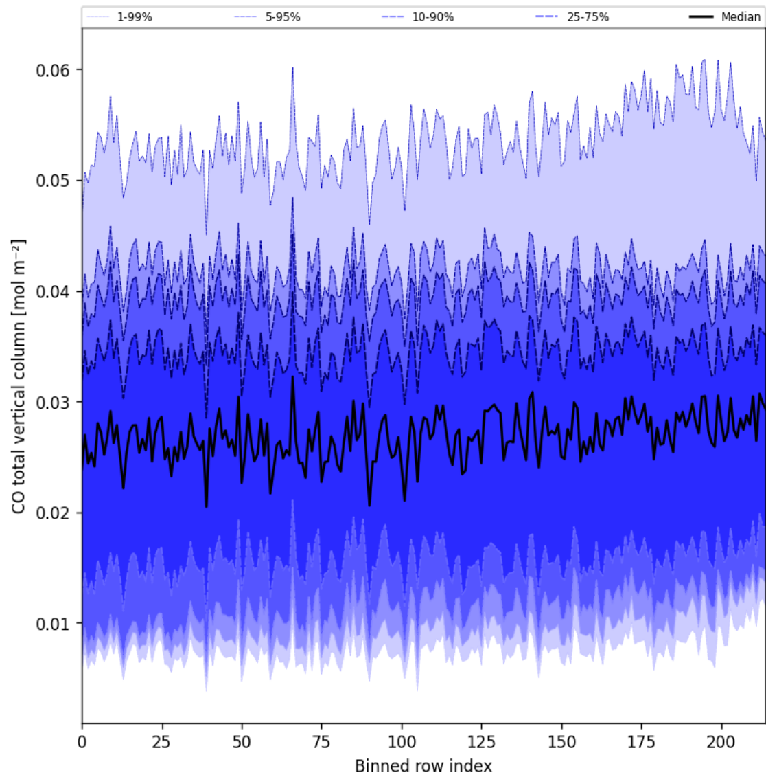
Figure 21: Along track statistics of “CO total vertical column” for 2025-03-01 to 2025-03-02
