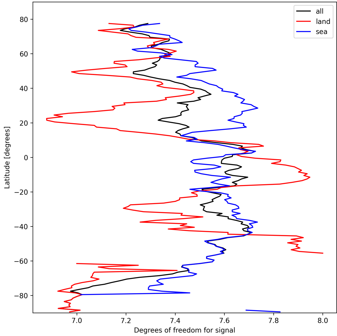
Figure 11: Zonal average of “Degrees of freedom for signal” for 2025-03-01 to 2025-03-02.
