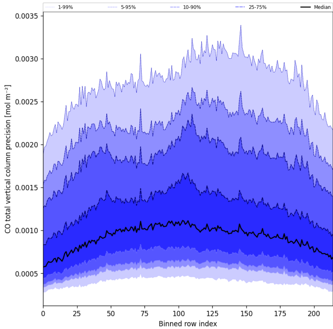
Figure 22: Along track statistics of “CO total vertical column precision” for 2025-03-01 to 2025-03-02
