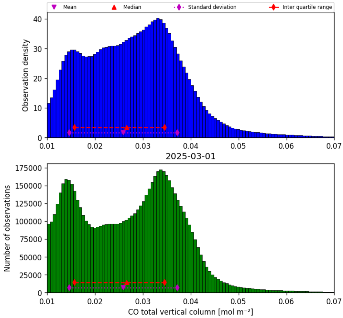
Figure 14: Histogram of “CO total vertical column” for 2025-03-01 to 2025-03-02
