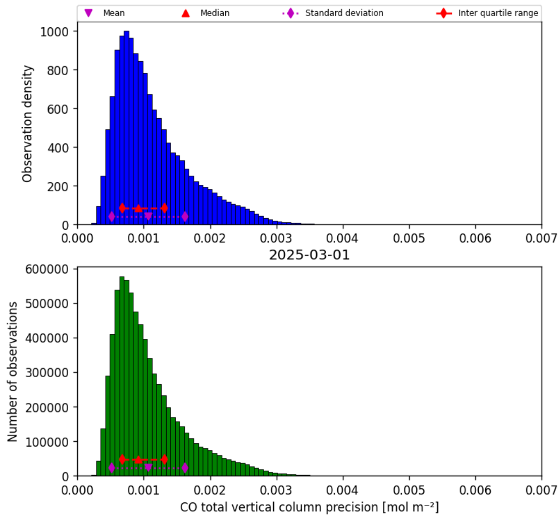
Figure 15: Histogram of “CO total vertical column precision” for 2025-03-01 to 2025-03-02
