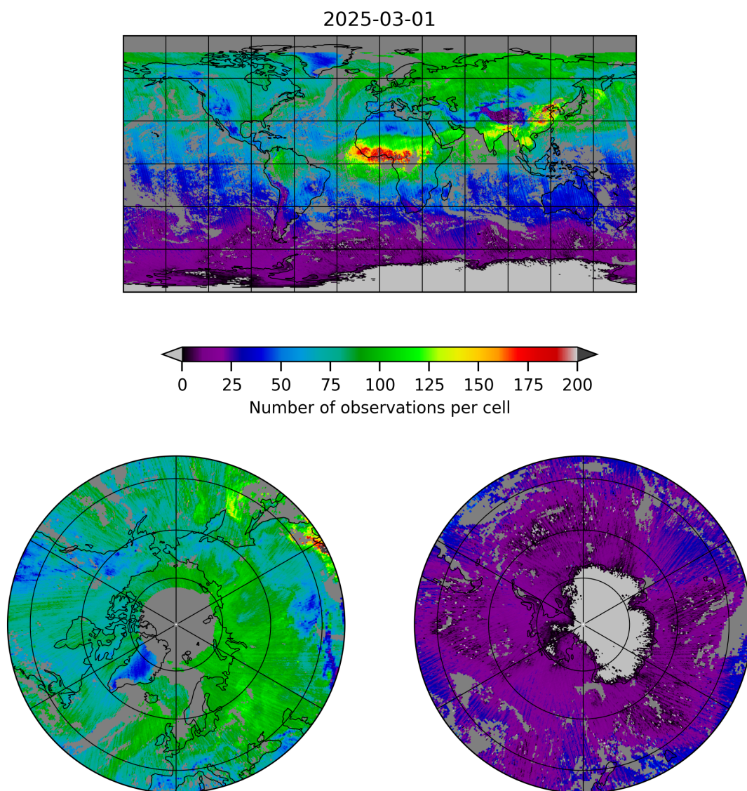
Figure 5: Map of the number of observations for 2025-03-01 to 2025-03-02
