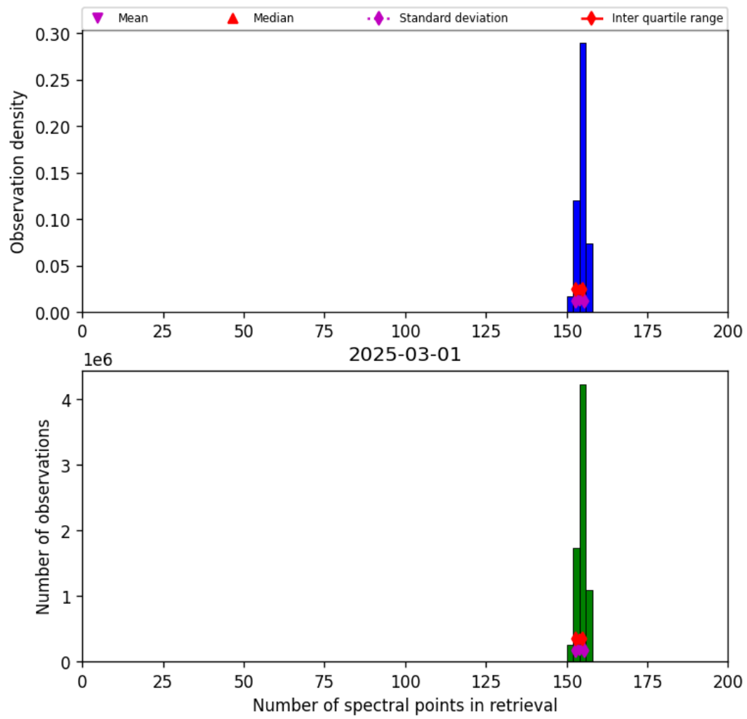
Figure 16: Histogram of “Number of spectral points in retrieval” for 2025-03-01 to 2025-03-02
