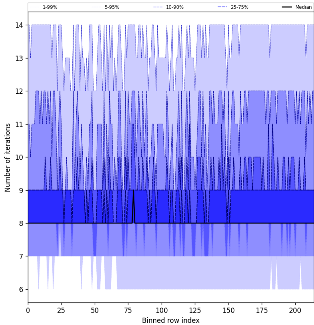
Figure 26: Along track statistics of “Number of iterations” for 2025-03-01 to 2025-03-02
