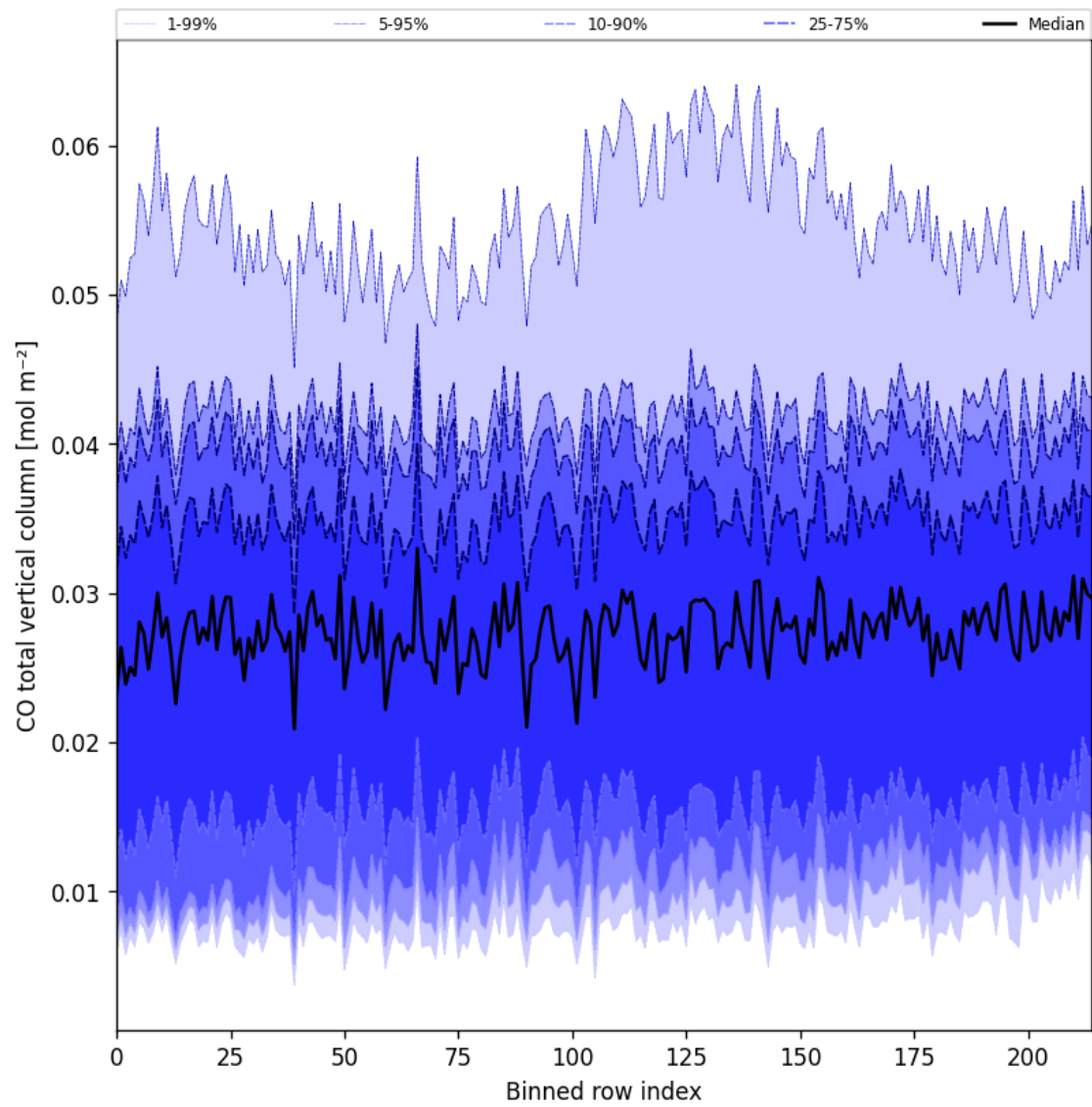
Figure 21: Along track statistics of “CO total vertical column” for 2025-03-02 to 2025-03-03
