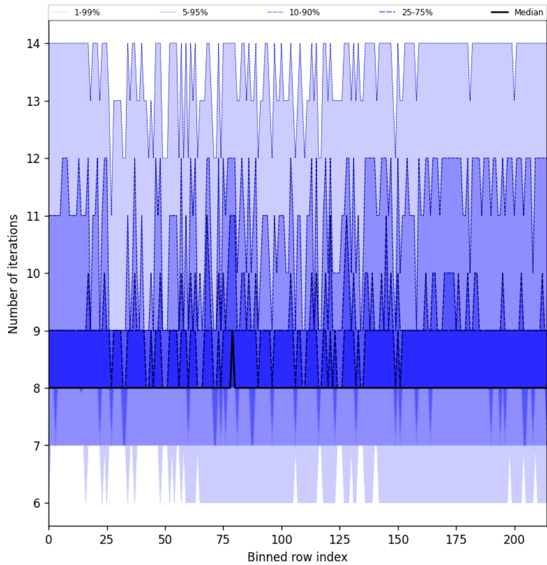
Figure 26: Along track statistics of “Number of iterations” for 2025-03-02 to 2025-03-03
