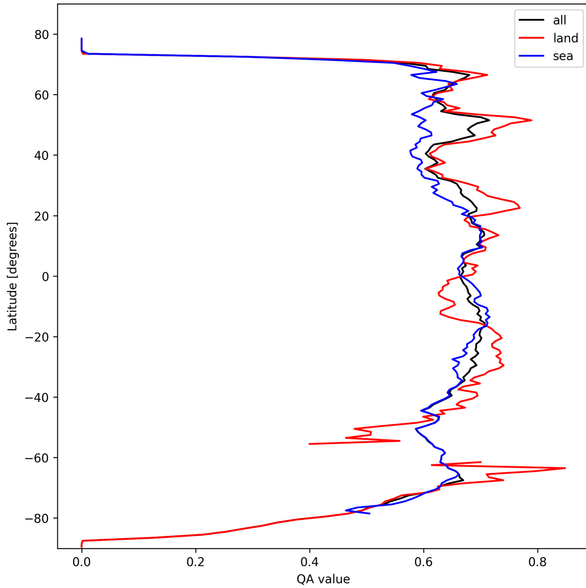
Figure 6: Zonal average of “QA value” for 2025-03-02 to 2025-03-03.
