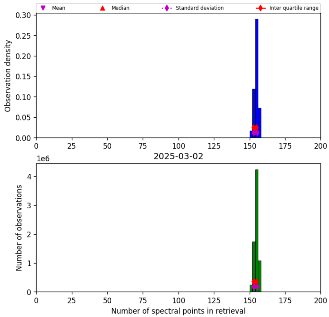
Figure 16: Histogram of “Number of spectral points in retrieval” for 2025-03-02 to 2025-03-03
