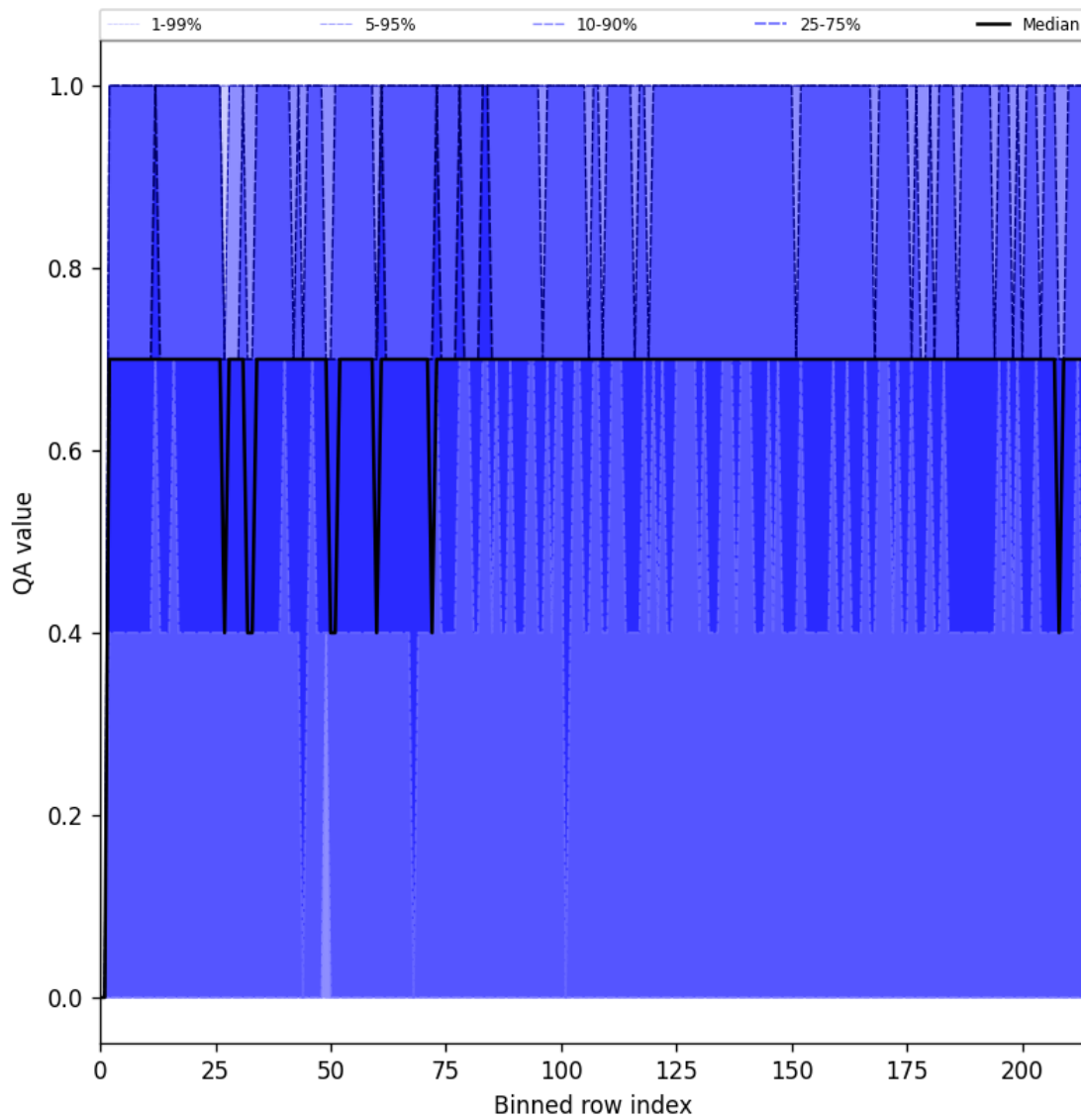
Figure 20: Along track statistics of “QA value” for 2025-03-02 to 2025-03-03
