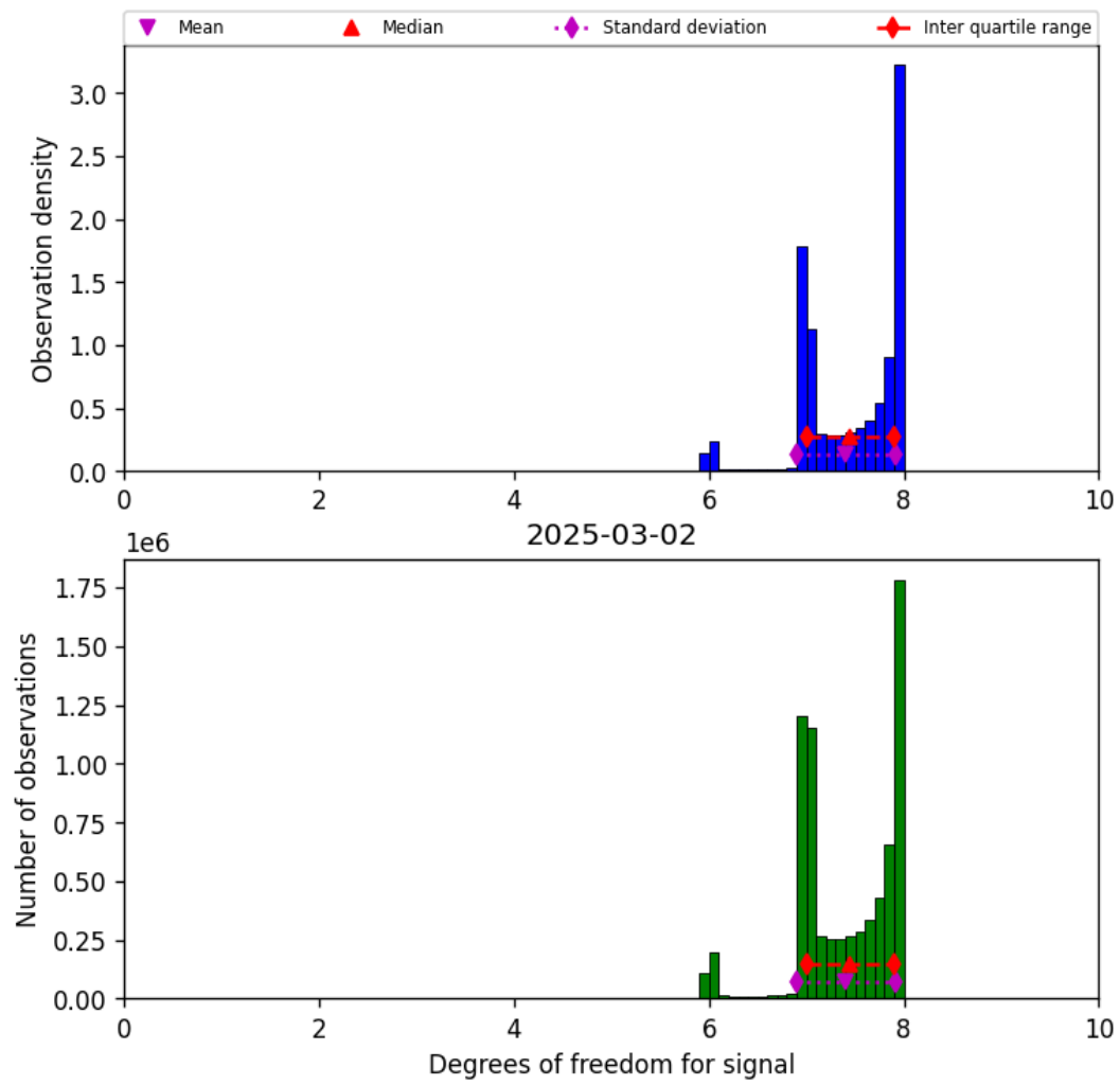
Figure 18: Histogram of “Degrees of freedom for signal” for 2025-03-02 to 2025-03-03
