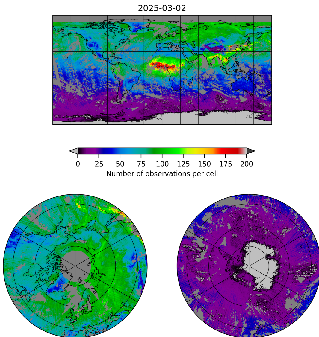
Figure 5: Map of the number of observations for 2025-03-02 to 2025-03-03
