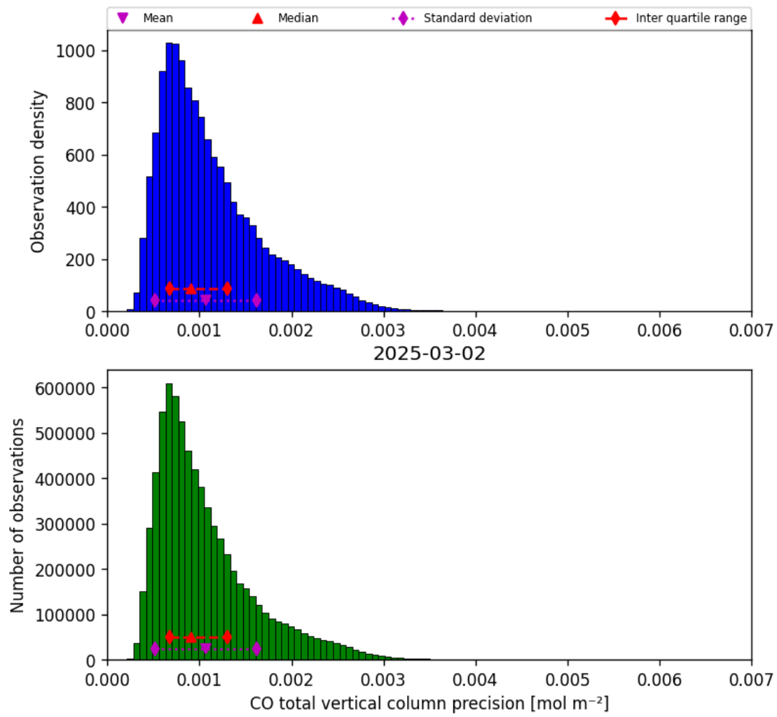
Figure 15: Histogram of “CO total vertical column precision” for 2025-03-02 to 2025-03-03
