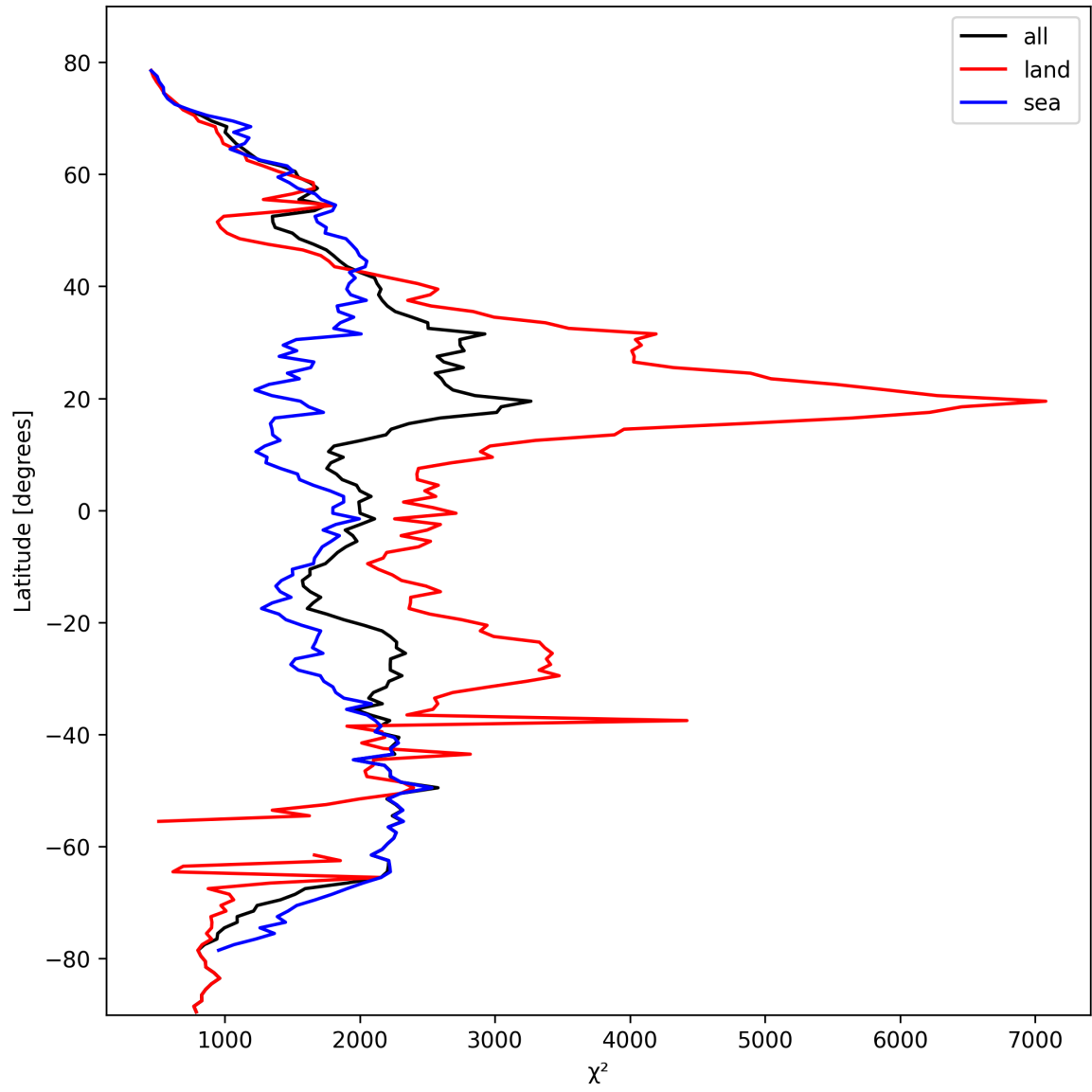
Figure 10: Zonal average of “ \chi^2 ” for 2025-03-02 to 2025-03-03.
