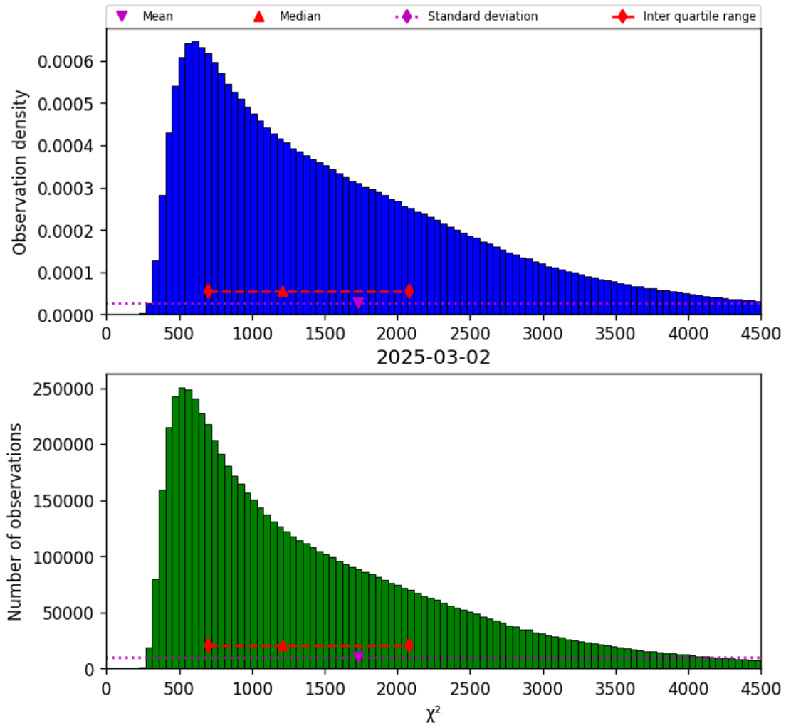
Figure 17: Histogram of " \chi^2 " for 2025-03-02 to 2025-03-03
