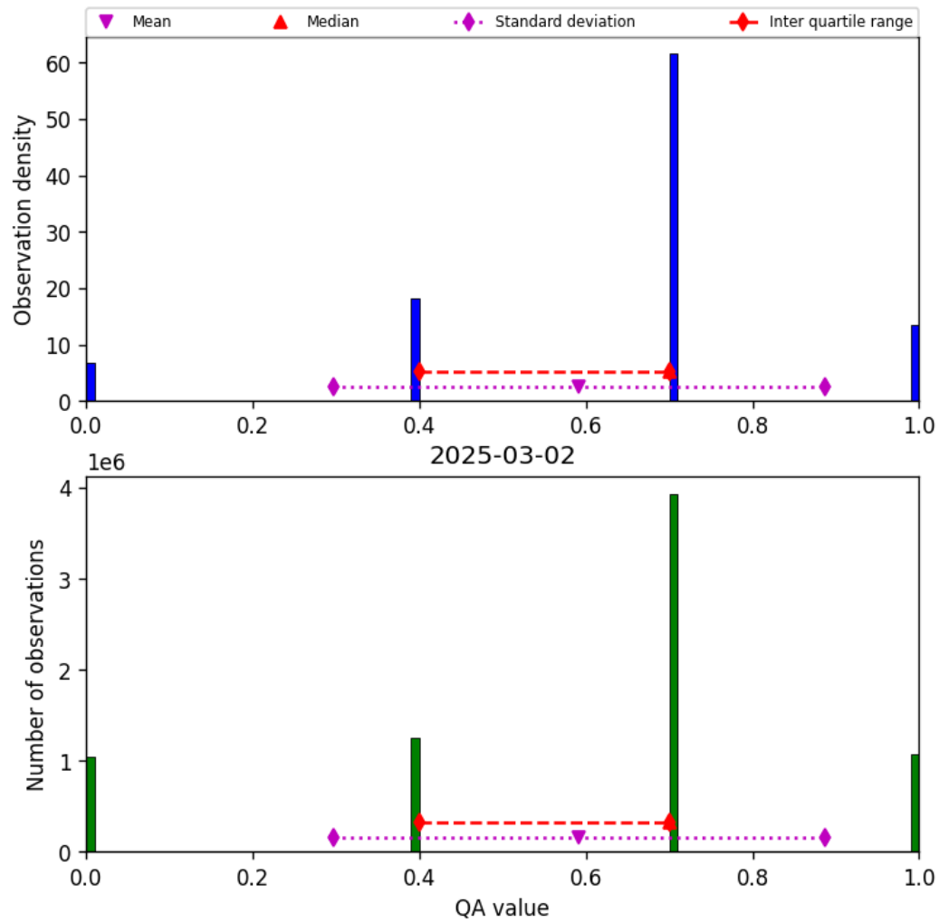
Figure 13: Histogram of “QA value” for 2025-03-02 to 2025-03-03
