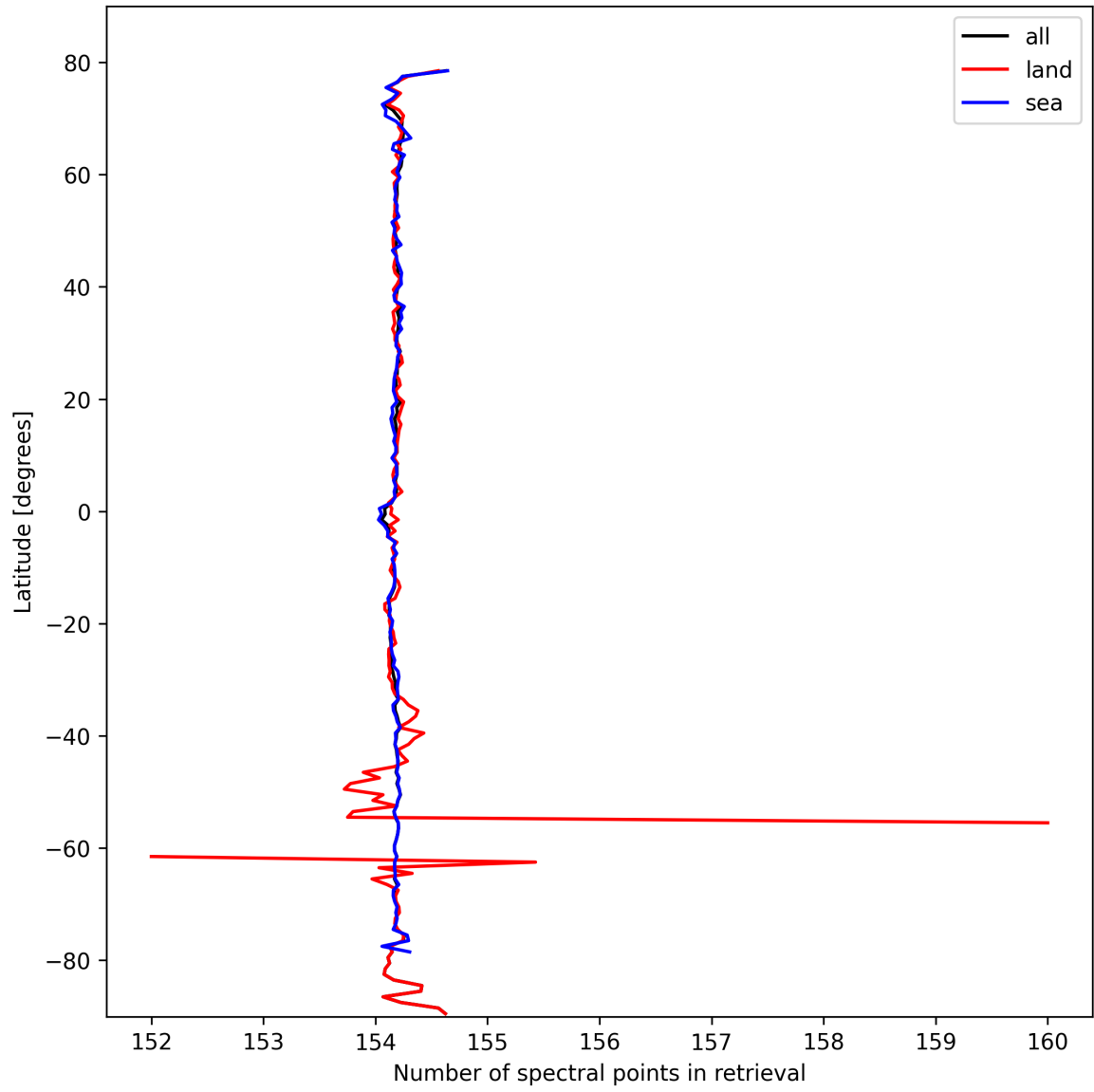
Figure 9: Zonal average of “Number of spectral points in retrieval” for 2025-03-02 to 2025-03-03.
