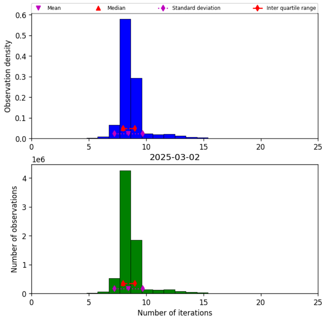
Figure 19: Histogram of “Number of iterations” for 2025-03-02 to 2025-03-03
