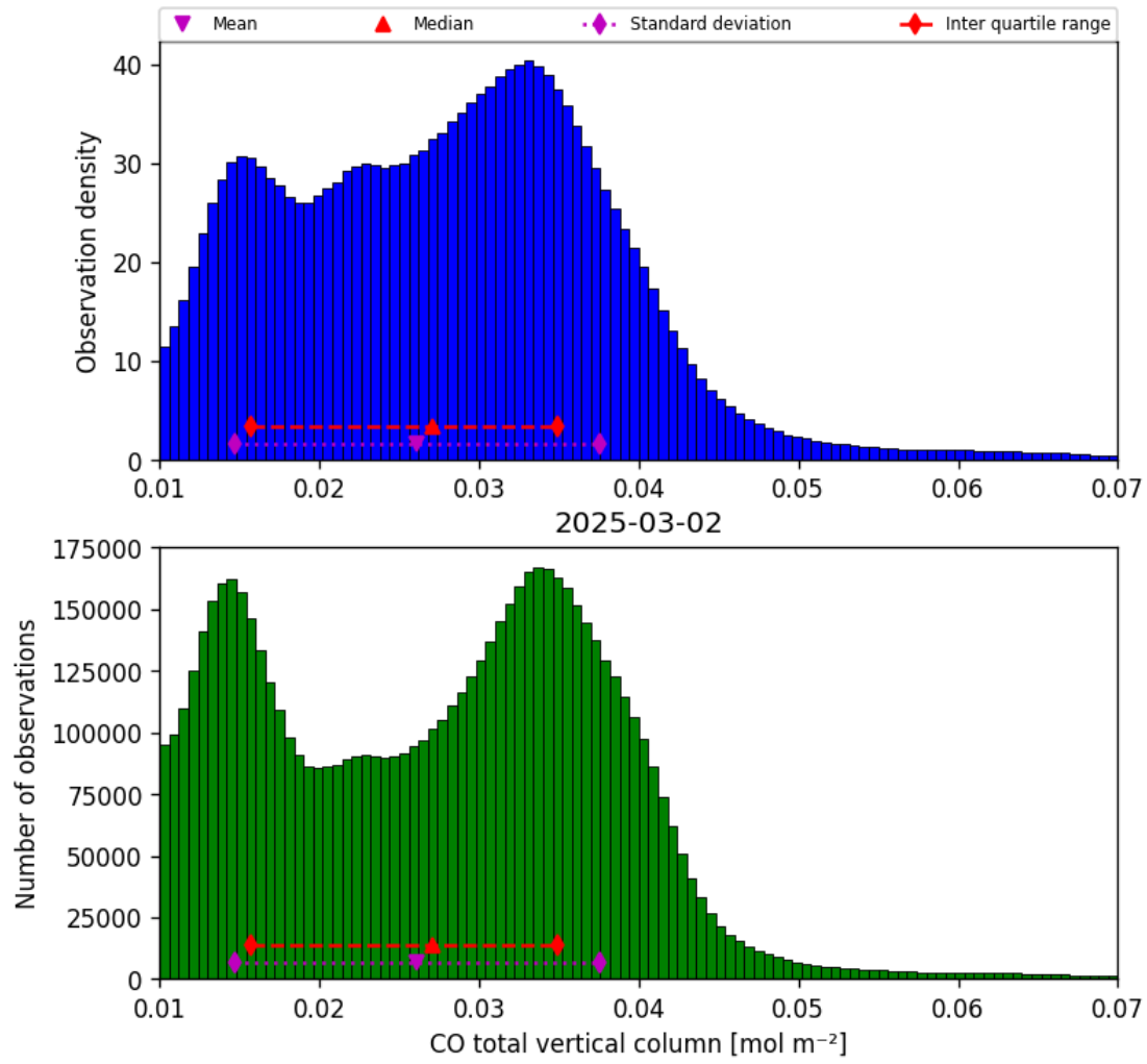
Figure 14: Histogram of “CO total vertical column” for 2025-03-02 to 2025-03-03
