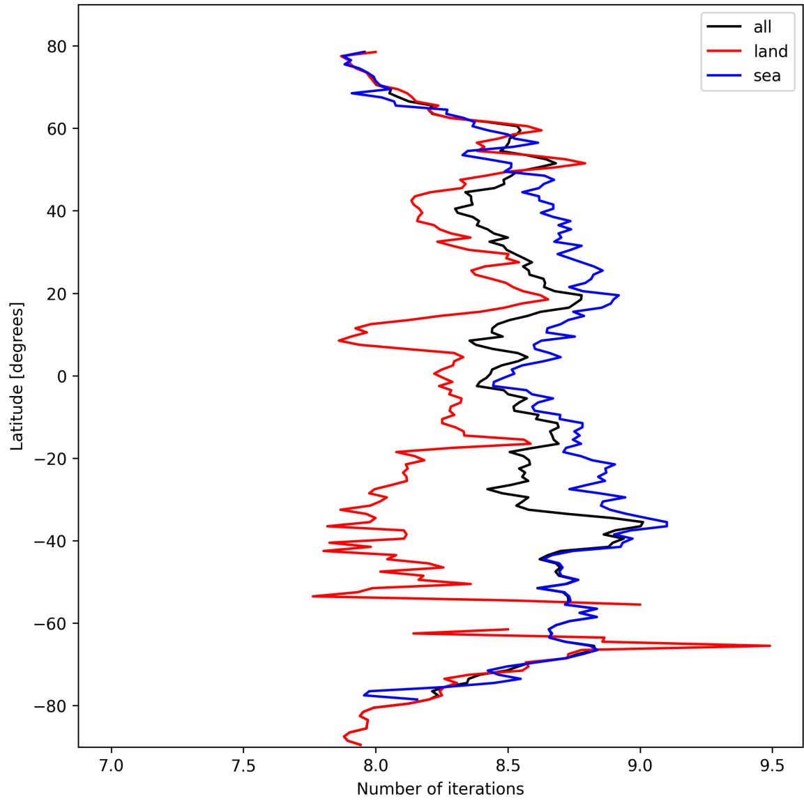
Figure 12: Zonal average of “Number of iterations” for 2025-03-02 to 2025-03-03.
