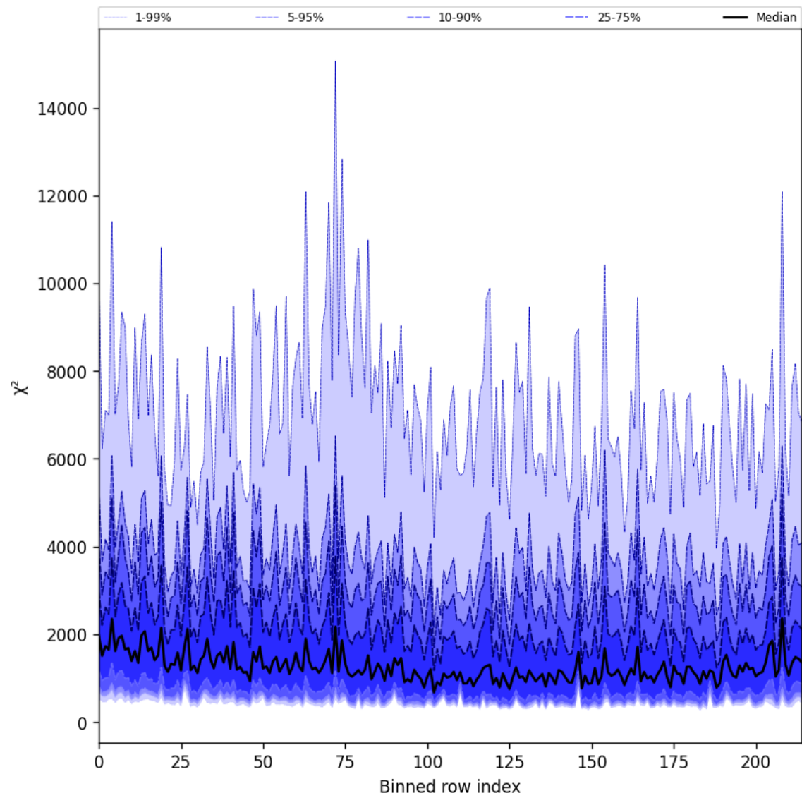
Figure 24: Along track statistics of “ \chi^2 ” for 2025-03-02 to 2025-03-03
