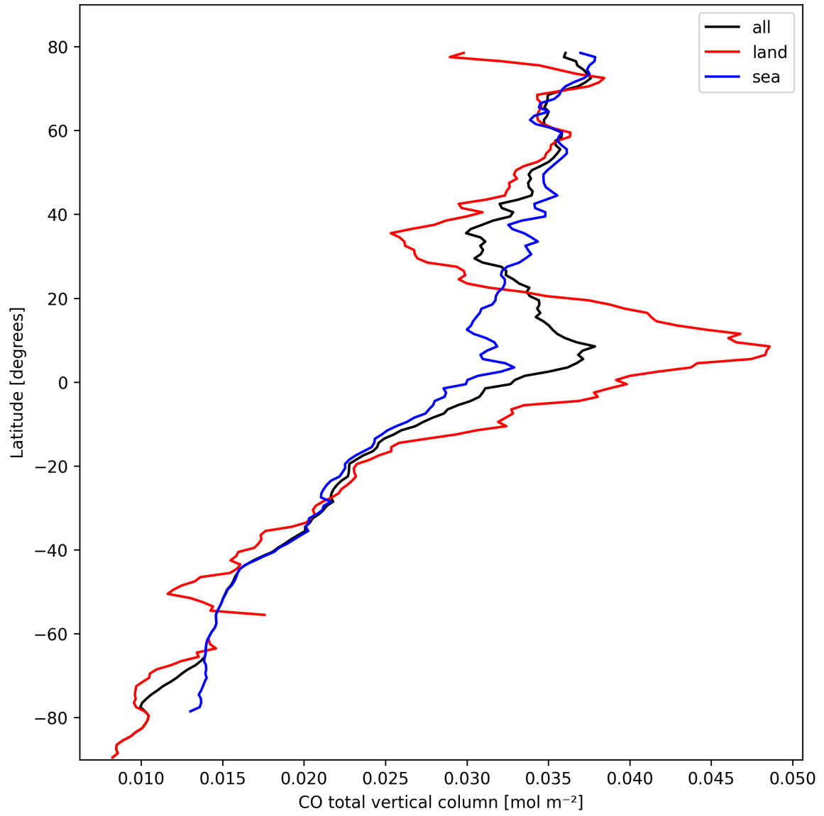
Figure 7: Zonal average of “CO total vertical column” for 2025-03-02 to 2025-03-03.
