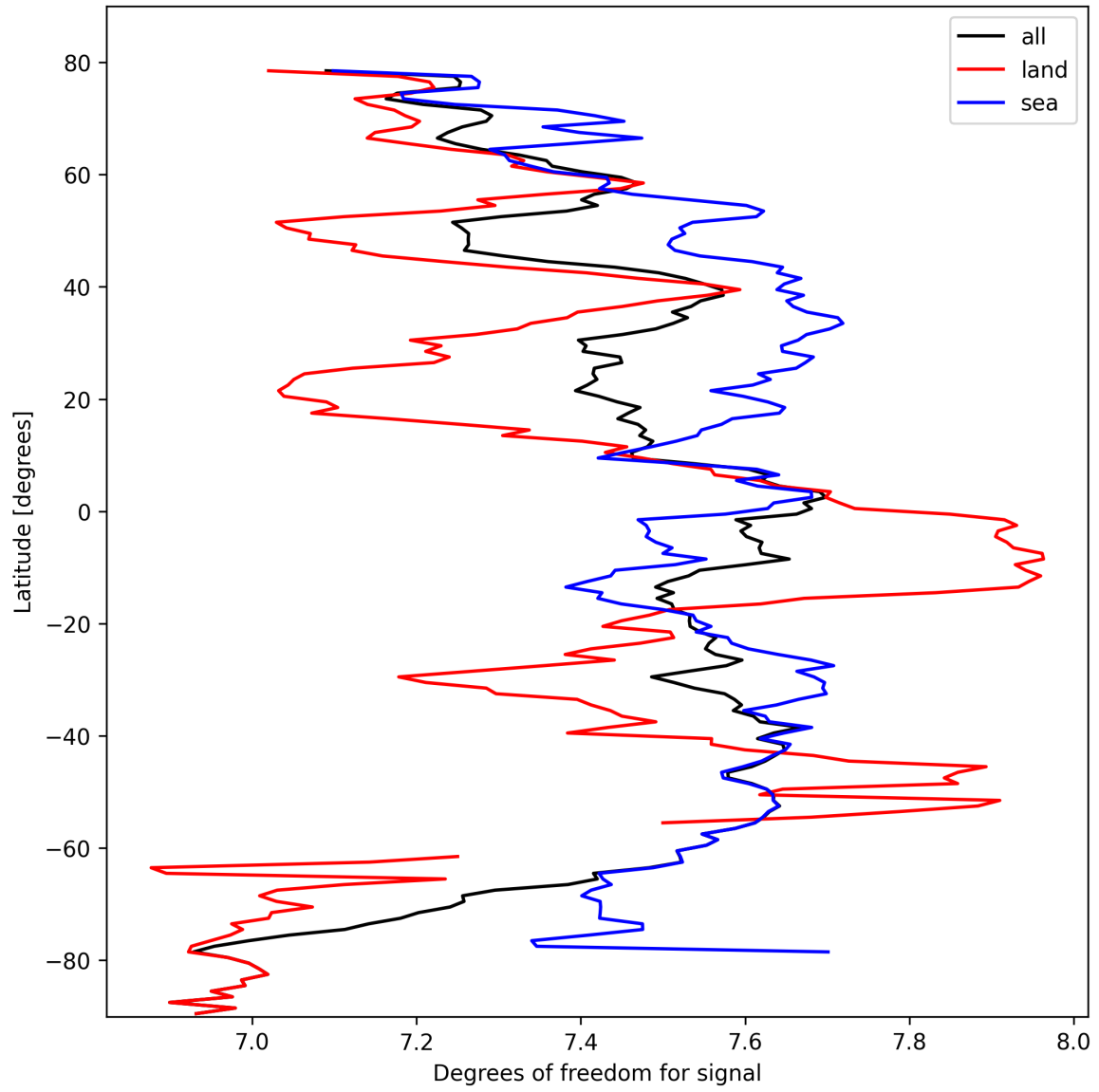
Figure 11: Zonal average of “Degrees of freedom for signal” for 2025-03-02 to 2025-03-03.
