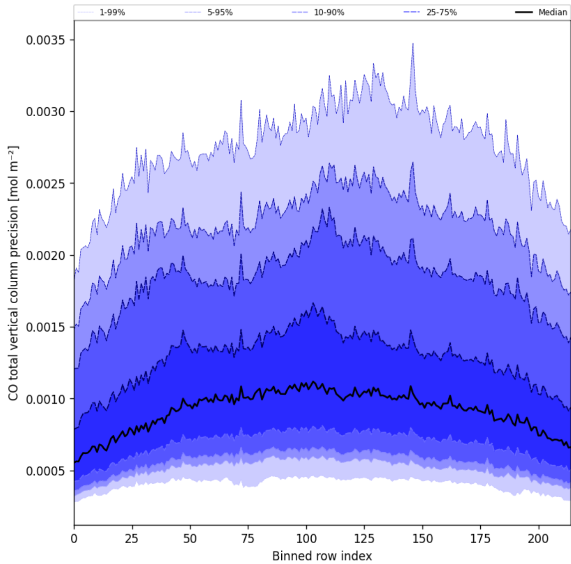
Figure 22: Along track statistics of “CO total vertical column precision” for 2025-03-02 to 2025-03-03
