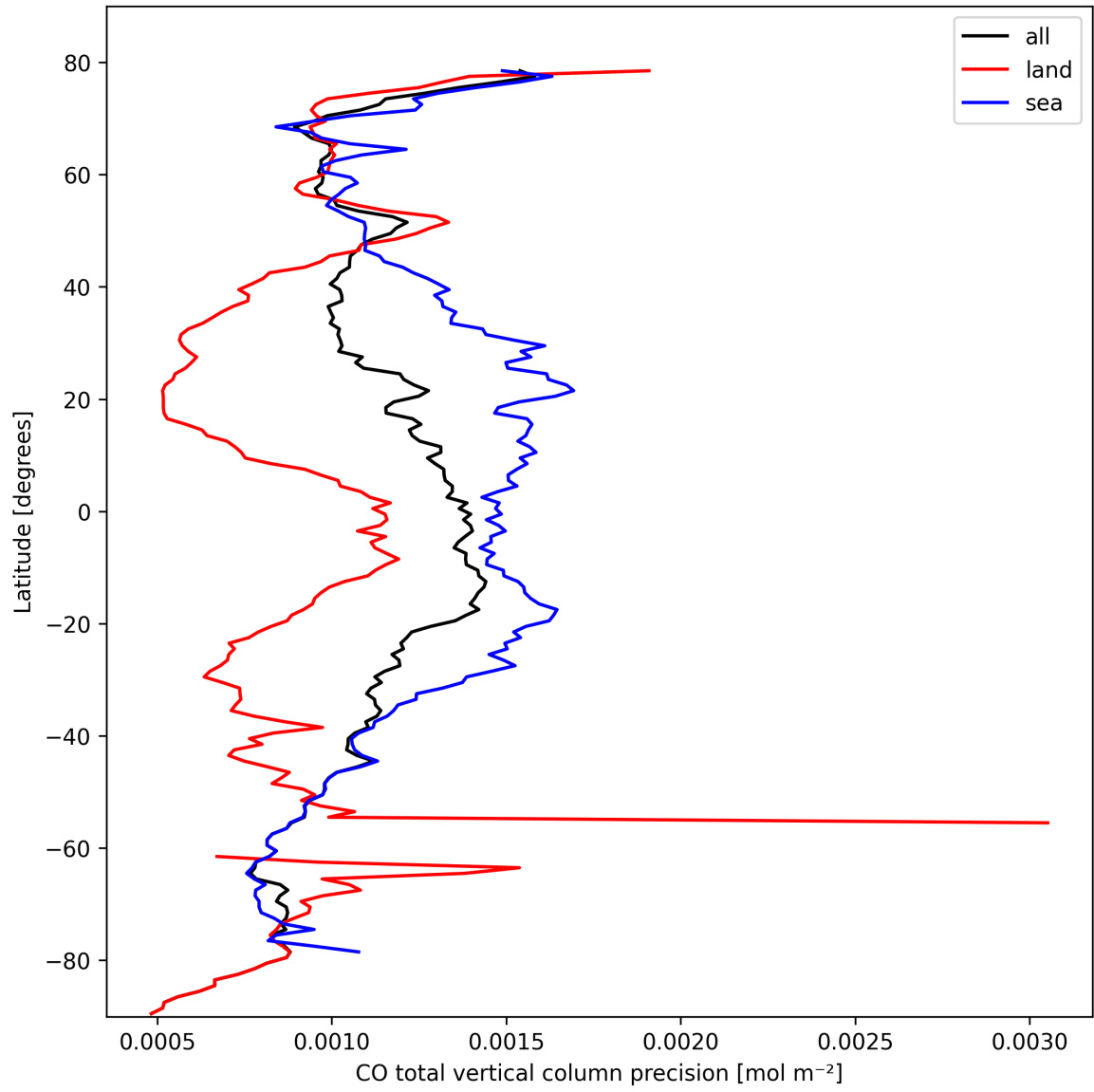
Figure 8: Zonal average of “CO total vertical column precision” for 2025-03-02 to 2025-03-03.
