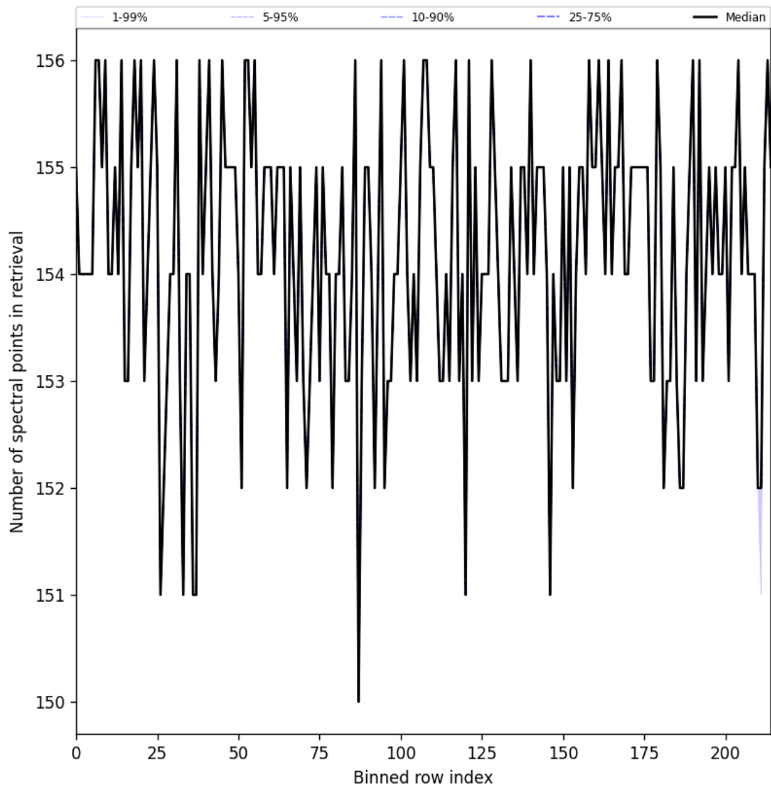
Figure 23: Along track statistics of “Number of spectral points in retrieval” for 2025-03-02 to 2025-03-03
