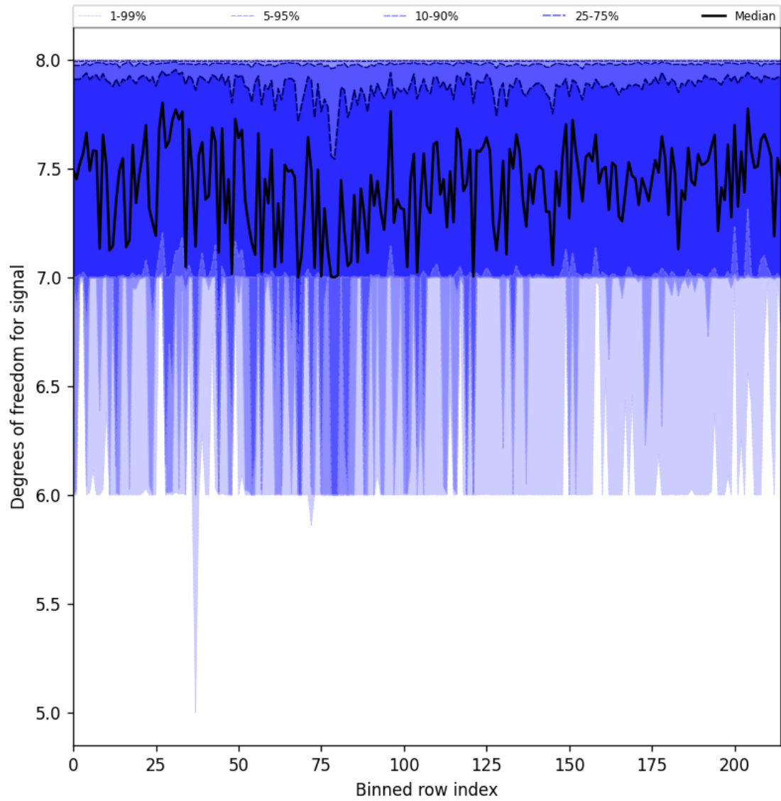
Figure 25: Along track statistics of “Degrees of freedom for signal” for 2025-03-02 to 2025-03-03
