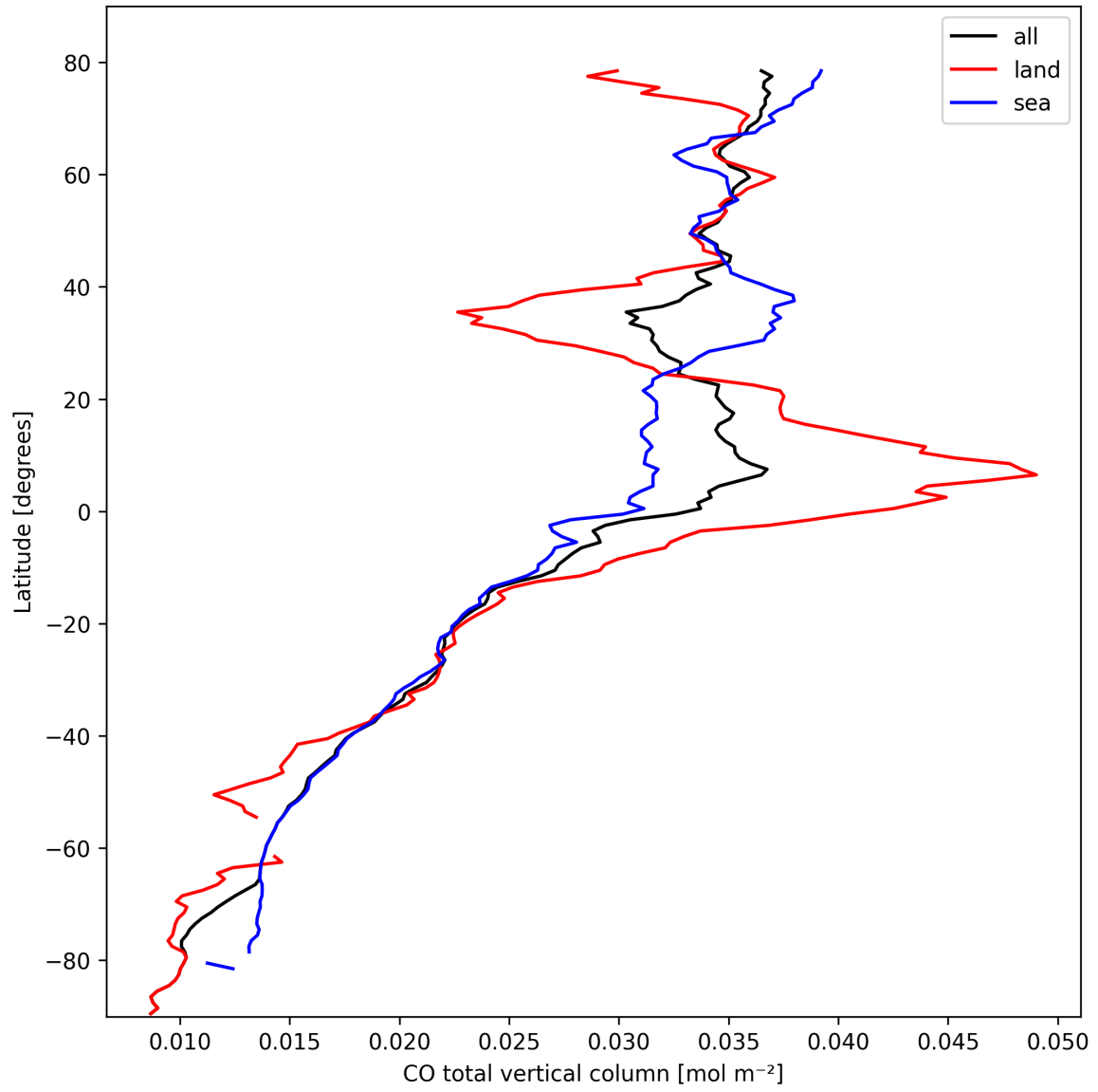
Figure 7: Zonal average of “CO total vertical column” for 2025-03-04 to 2025-03-04.
