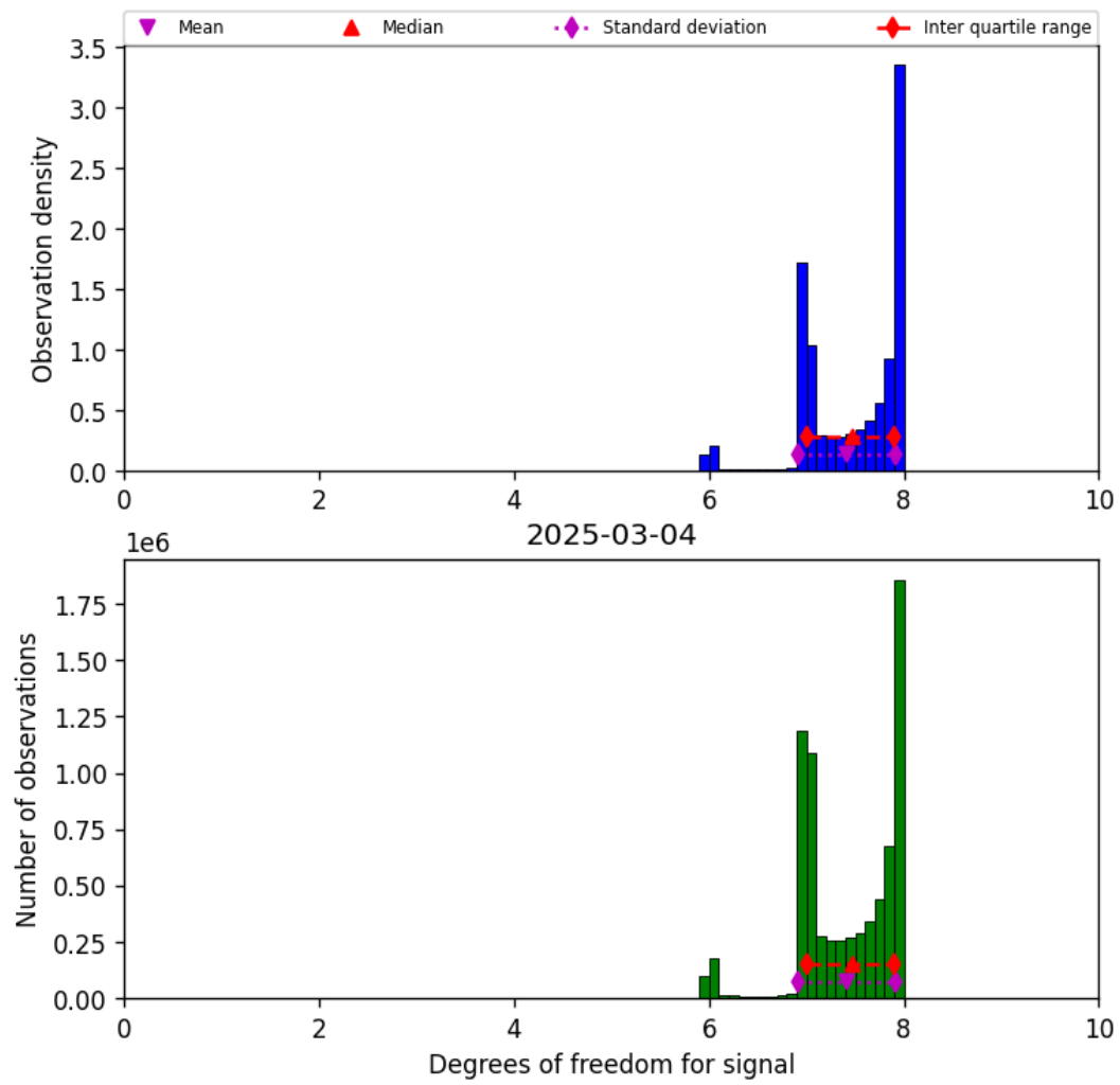
Figure 18: Histogram of “Degrees of freedom for signal” for 2025-03-04 to 2025-03-04
