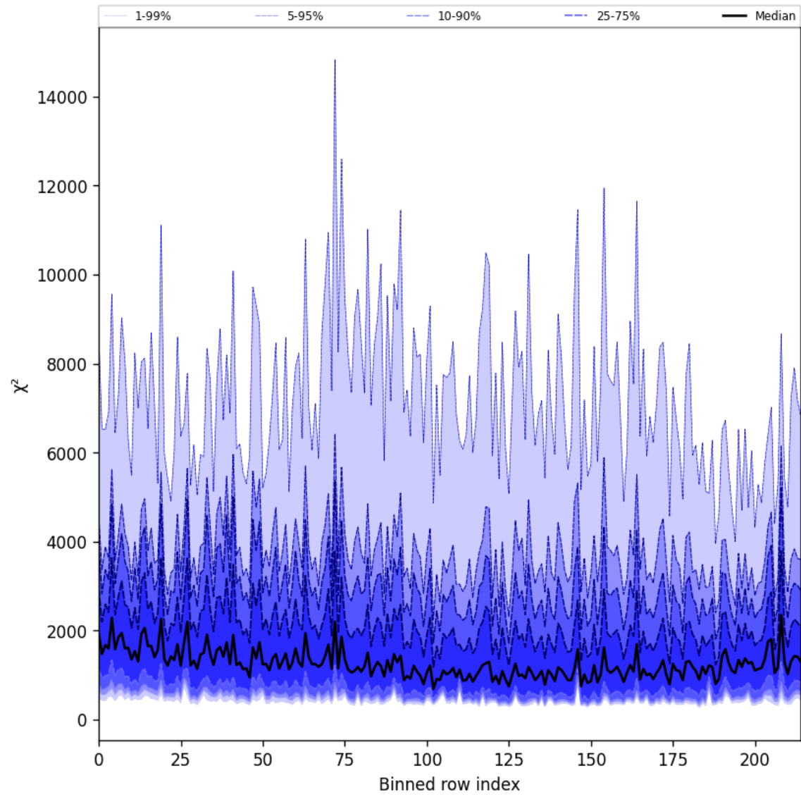
Figure 24: Along track statistics of “ \chi^2 ” for 2025-03-04 to 2025-03-04
