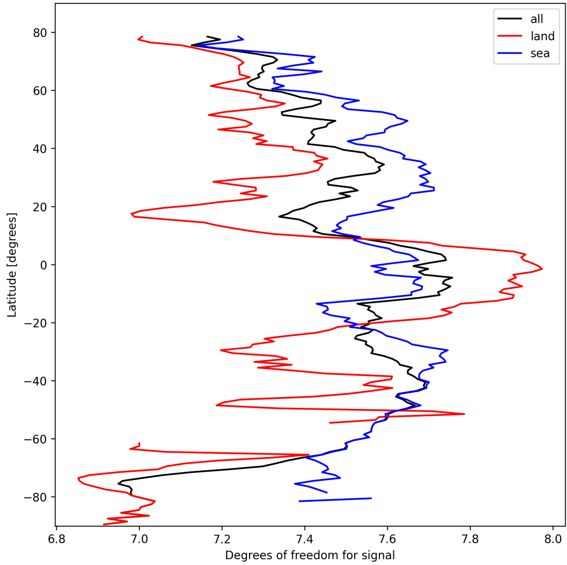
Figure 11: Zonal average of “Degrees of freedom for signal” for 2025-03-04 to 2025-03-04.
