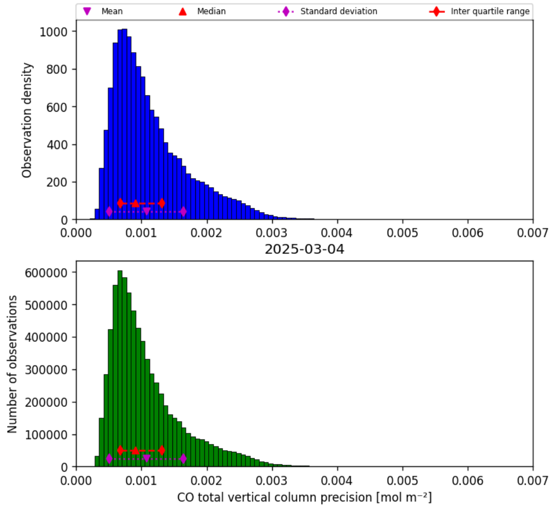
Figure 15: Histogram of “CO total vertical column precision” for 2025-03-04 to 2025-03-04
