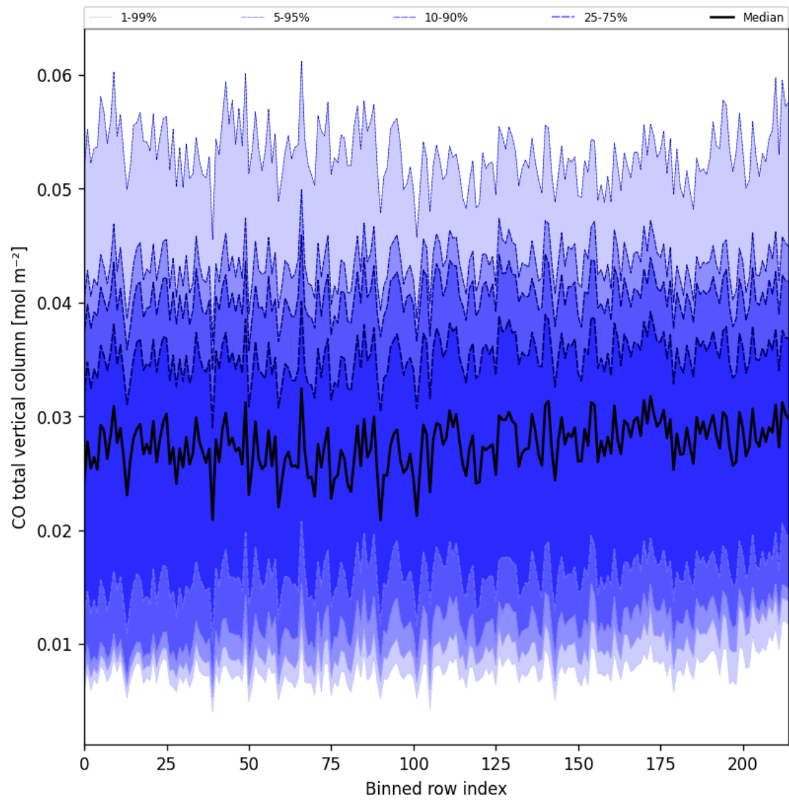
Figure 21: Along track statistics of “CO total vertical column” for 2025-03-04 to 2025-03-04
