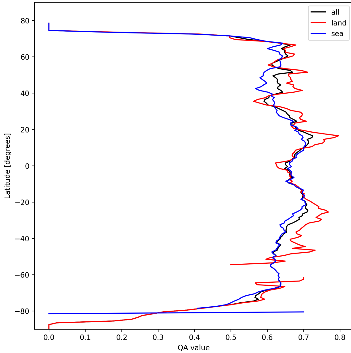
Figure 6: Zonal average of “QA value” for 2025-03-04 to 2025-03-04.
