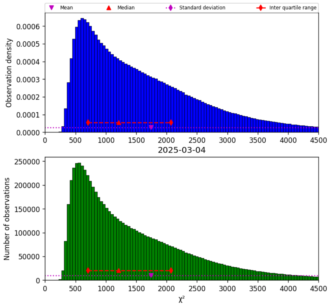
Figure 17: Histogram of “ \chi^2 ” for 2025-03-04 to 2025-03-04
