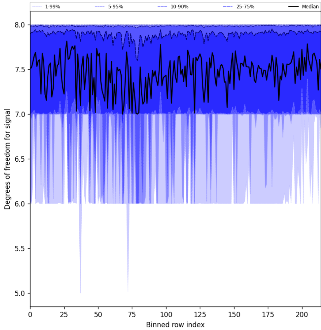
Figure 25: Along track statistics of “Degrees of freedom for signal” for 2025-03-04 to 2025-03-04
