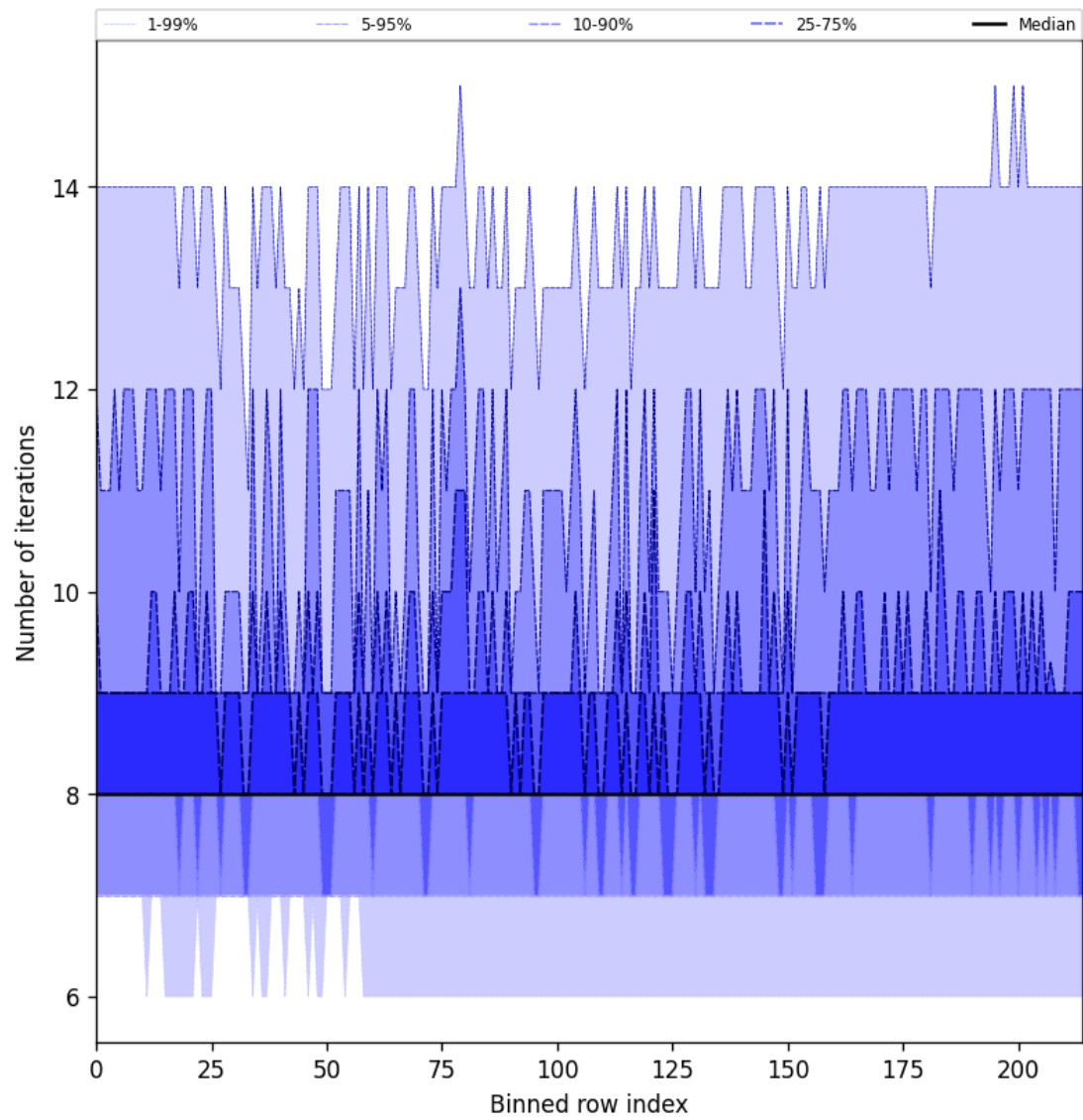
Figure 26: Along track statistics of “Number of iterations” for 2025-03-04 to 2025-03-04
