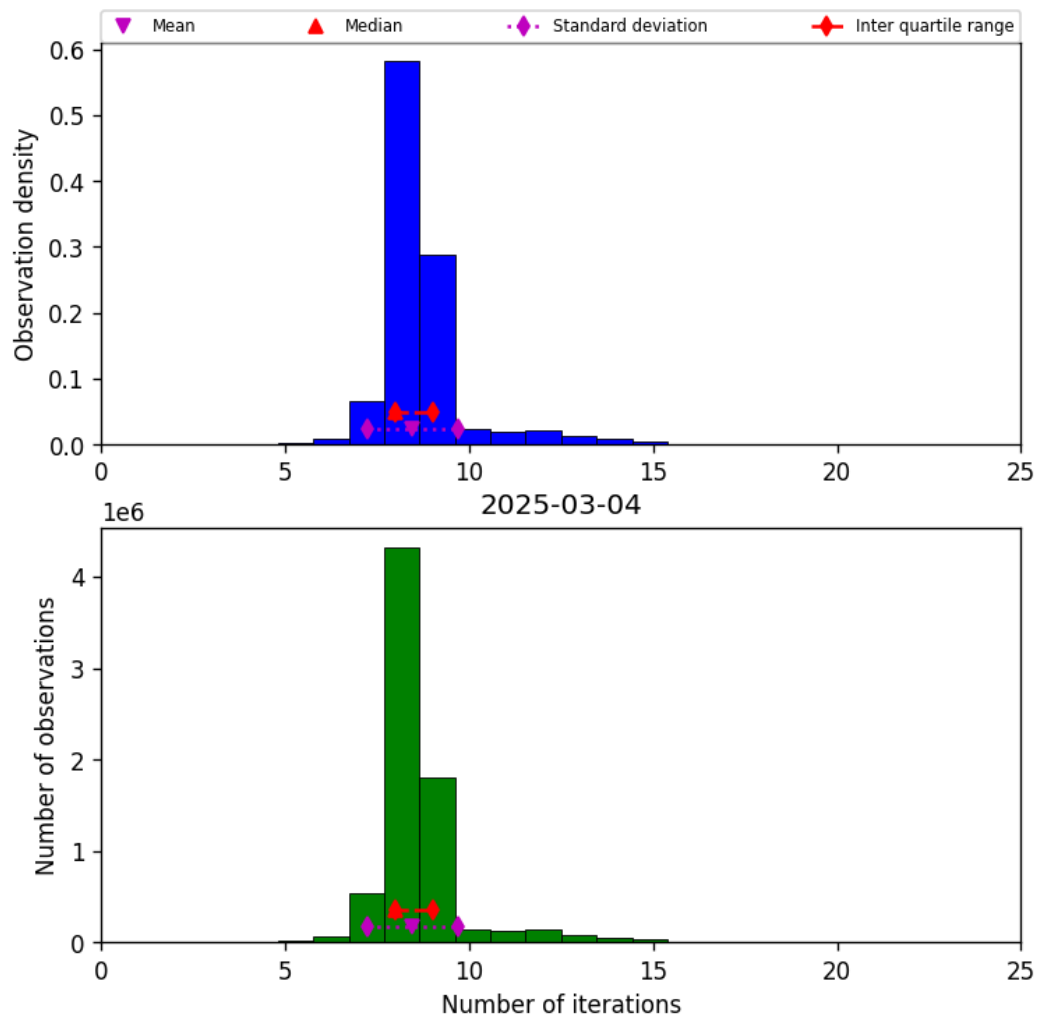
Figure 19: Histogram of “Number of iterations” for 2025-03-04 to 2025-03-04
