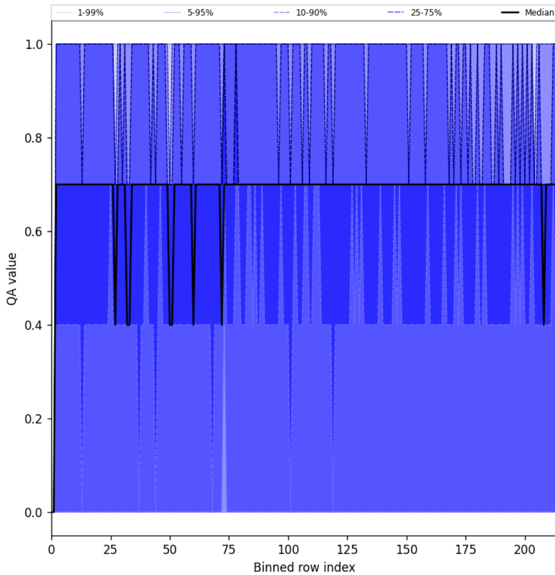
Figure 20: Along track statistics of “QA value” for 2025-03-04 to 2025-03-04
