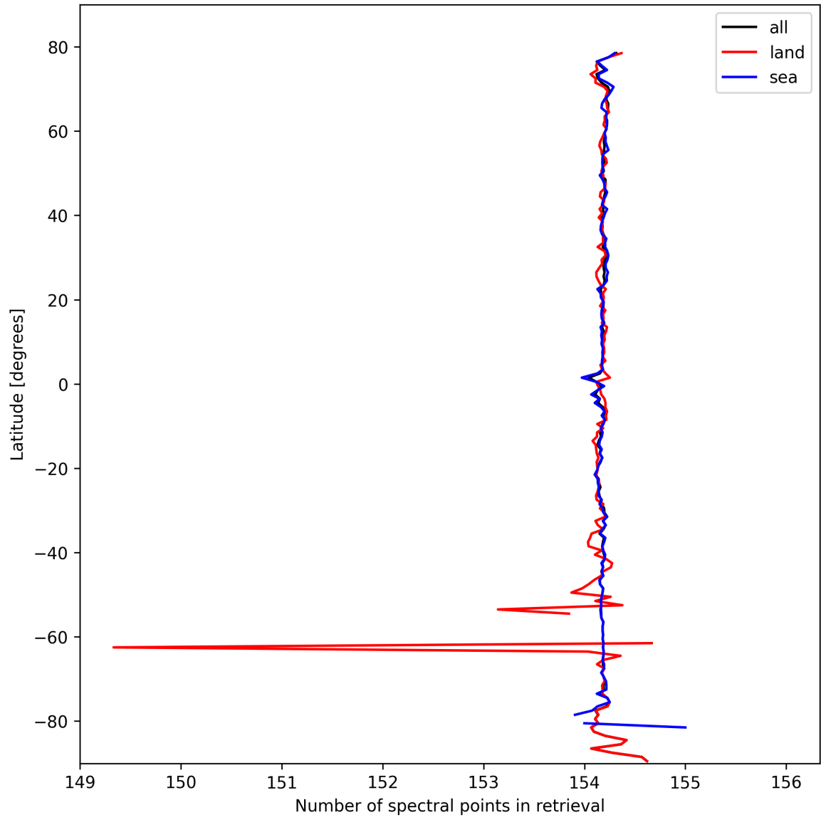
Figure 9: Zonal average of “Number of spectral points in retrieval” for 2025-03-04 to 2025-03-04.
