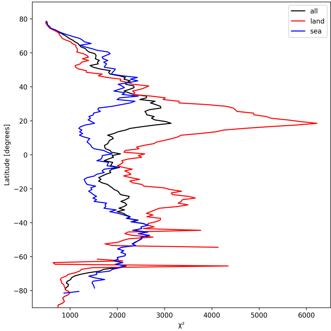
Figure 10: Zonal average of “ \chi^2 ” for 2025-03-04 to 2025-03-04.
