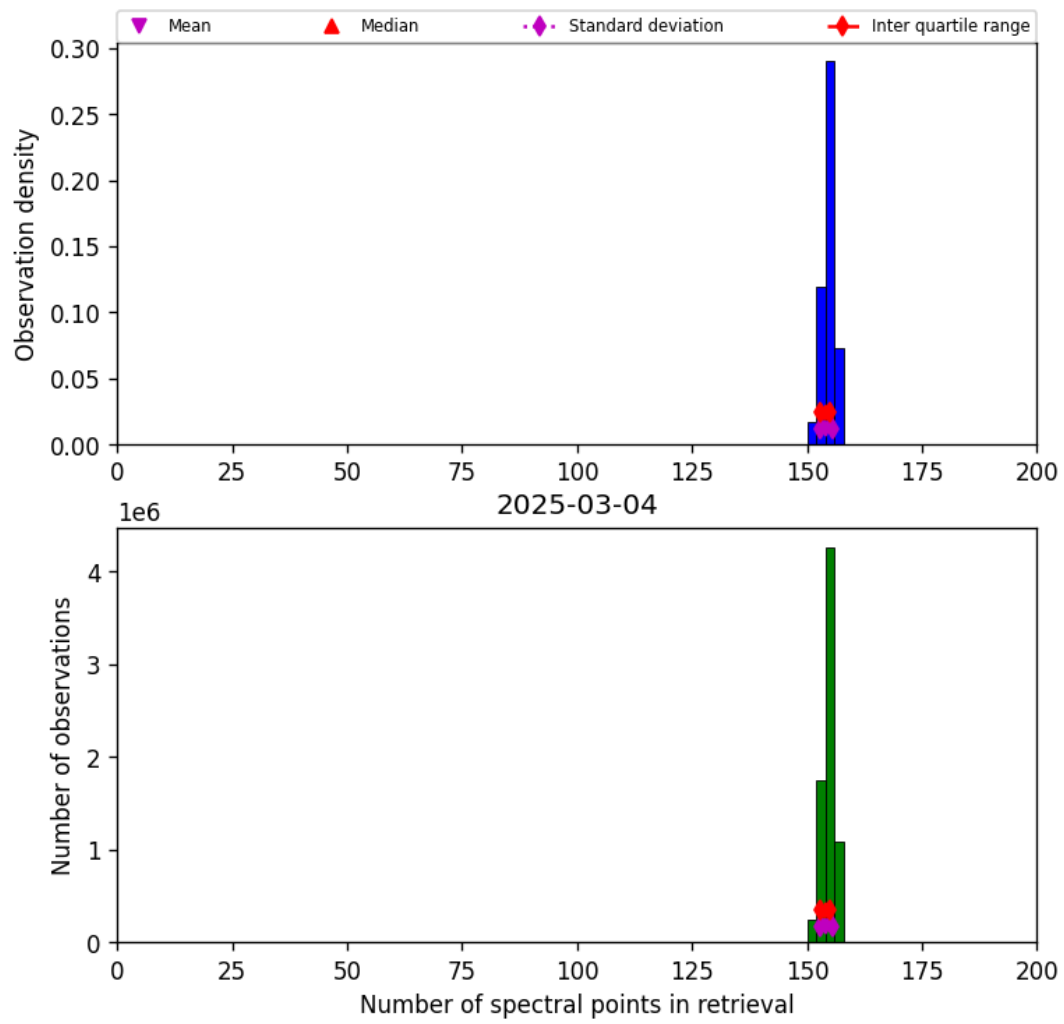
Figure 16: Histogram of “Number of spectral points in retrieval” for 2025-03-04 to 2025-03-04
