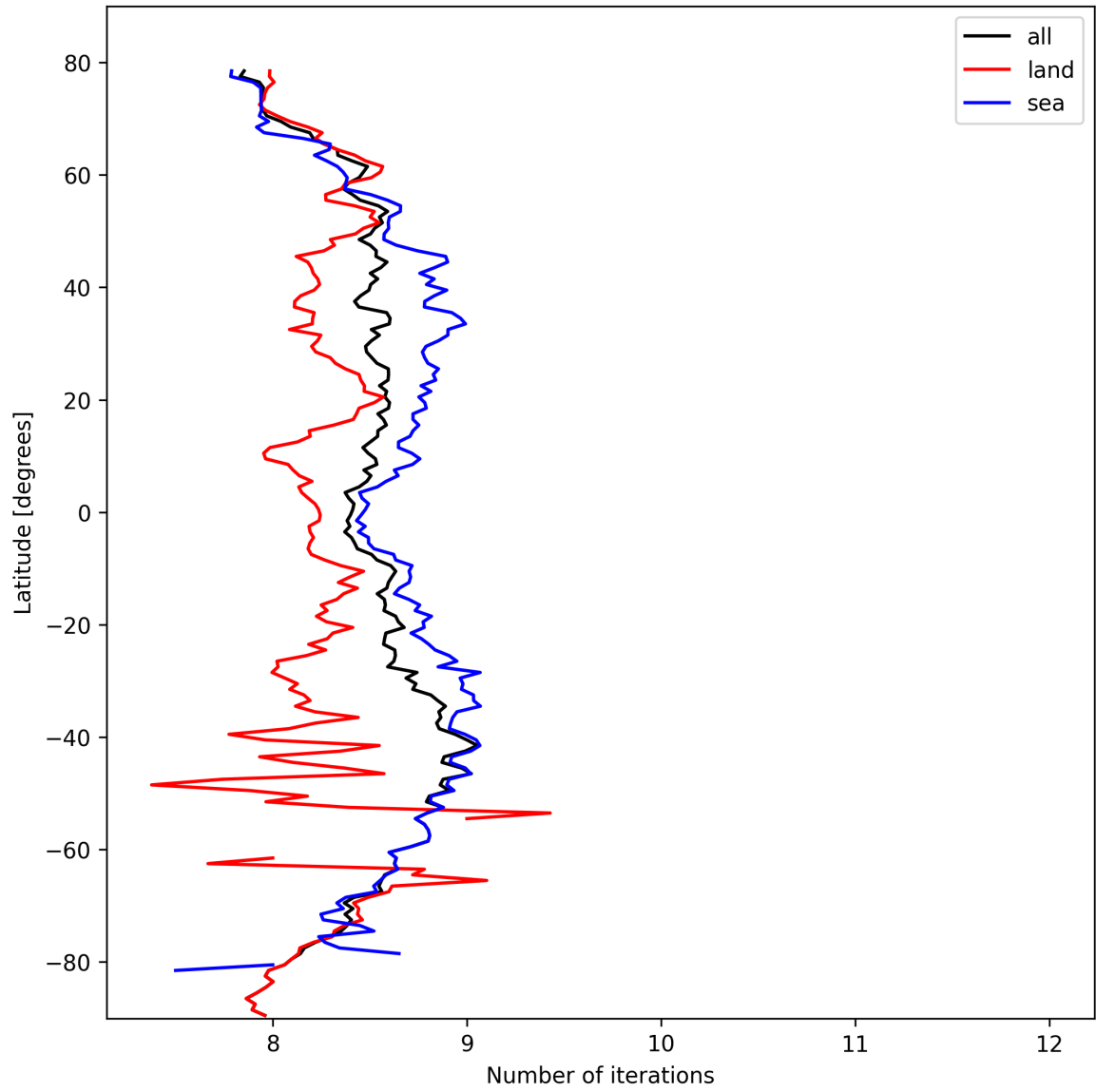
Figure 12: Zonal average of “Number of iterations” for 2025-03-04 to 2025-03-04.
