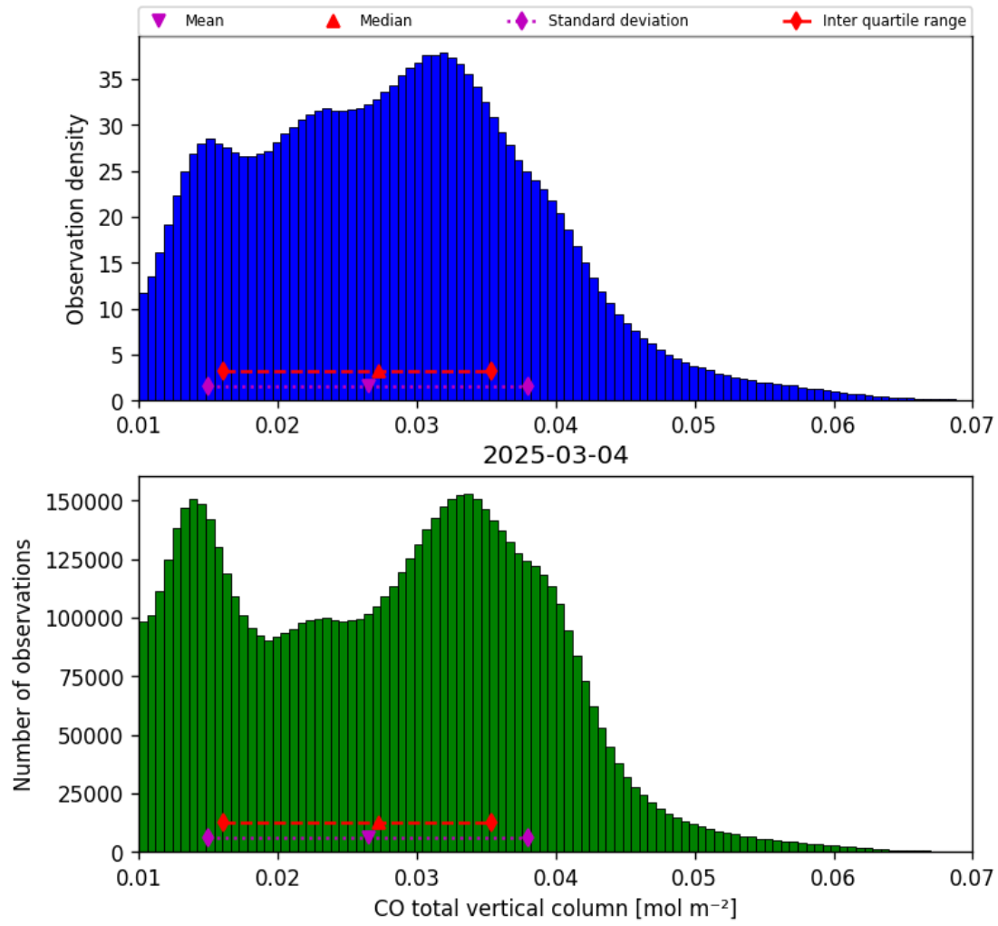
Figure 14: Histogram of “CO total vertical column” for 2025-03-04 to 2025-03-04
