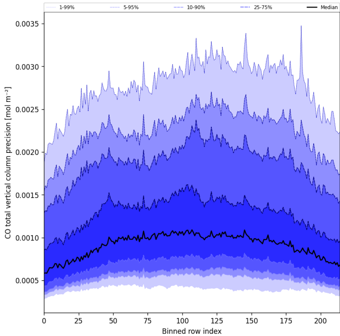
Figure 22: Along track statistics of “CO total vertical column precision” for 2025-03-04 to 2025-03-04
