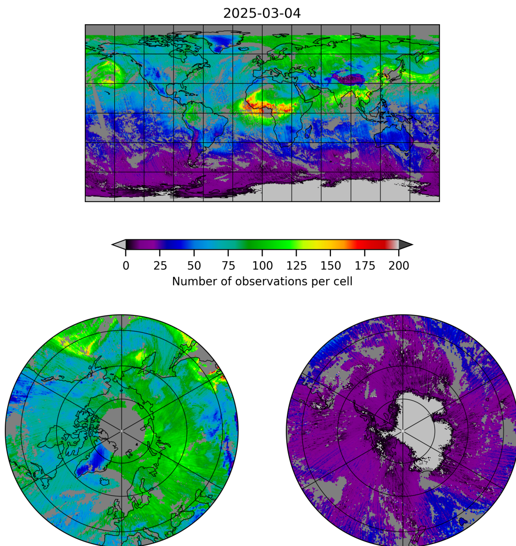
Figure 5: Map of the number of observations for 2025-03-04 to 2025-03-04
