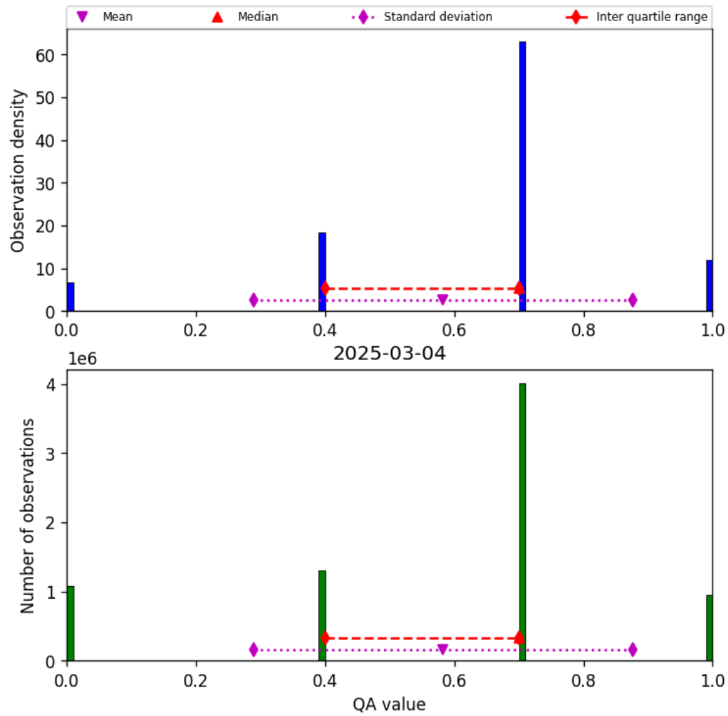
Figure 13: Histogram of “QA value” for 2025-03-04 to 2025-03-04
