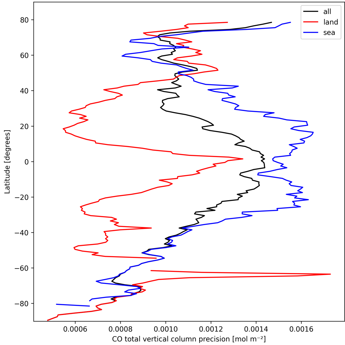
Figure 8: Zonal average of “CO total vertical column precision” for 2025-03-04 to 2025-03-04.
