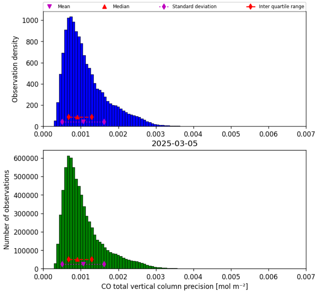
Figure 15: Histogram of “CO total vertical column precision” for 2025-03-05 to 2025-03-05
