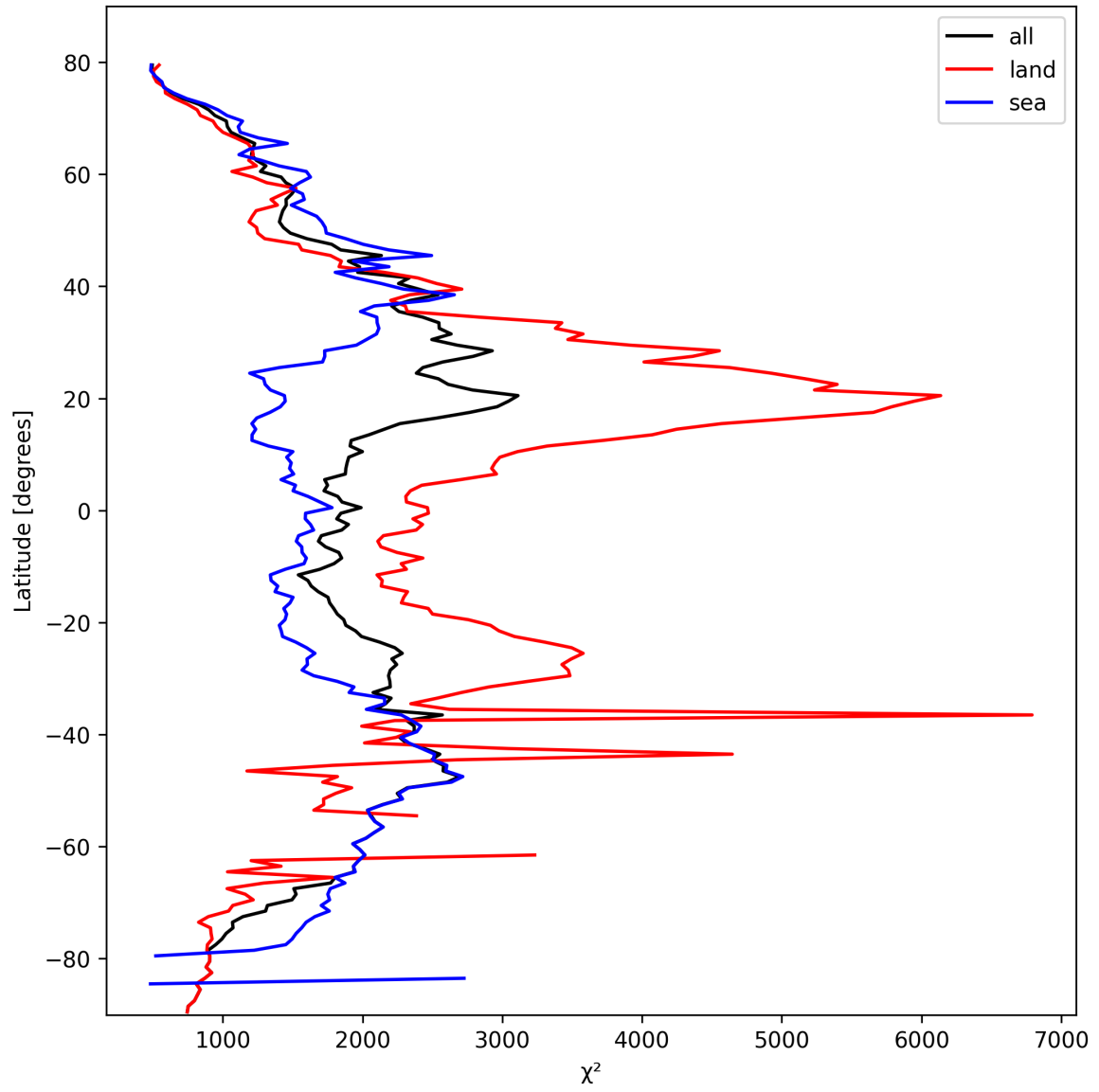
Figure 10: Zonal average of “ \chi^2 ” for 2025-03-05 to 2025-03-05.
