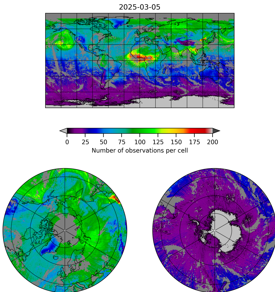
Figure 5: Map of the number of observations for 2025-03-05 to 2025-03-05
