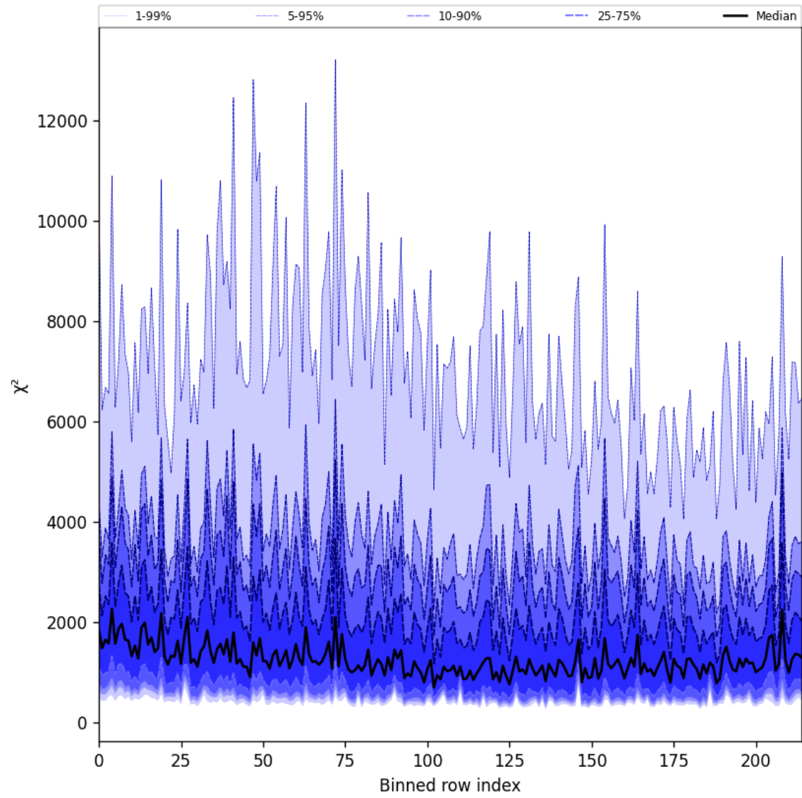
Figure 24: Along track statistics of “ \chi^2 ” for 2025-03-05 to 2025-03-05
