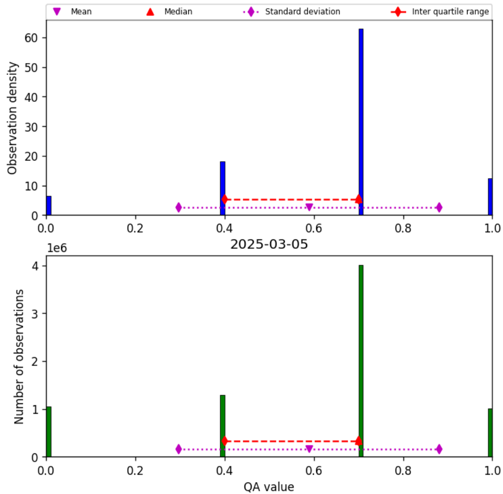
Figure 13: Histogram of “QA value” for 2025-03-05 to 2025-03-05
