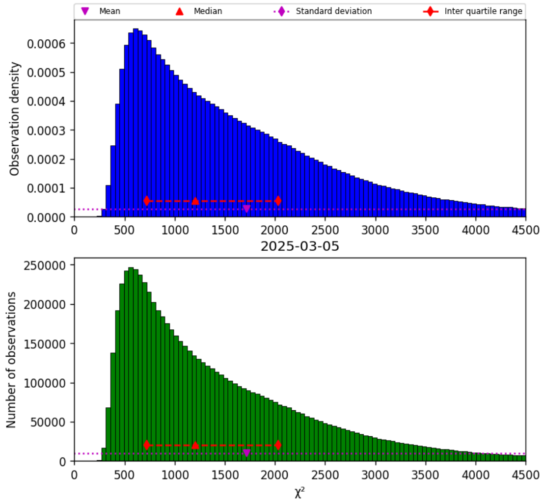
Figure 17: Histogram of " \chi^2 " for 2025-03-05 to 2025-03-05
