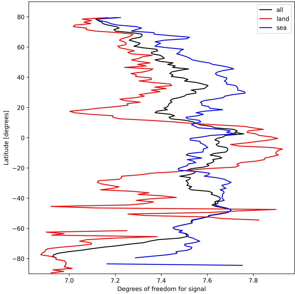
Figure 11: Zonal average of “Degrees of freedom for signal” for 2025-03-05 to 2025-03-05.
