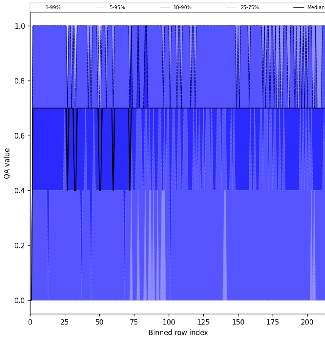
Figure 20: Along track statistics of “QA value” for 2025-03-05 to 2025-03-05
