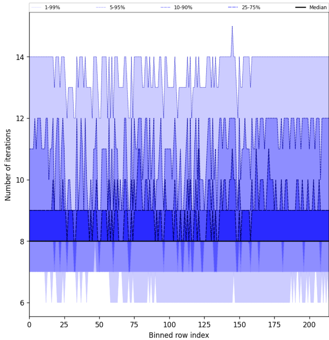
Figure 26: Along track statistics of “Number of iterations” for 2025-03-05 to 2025-03-05
