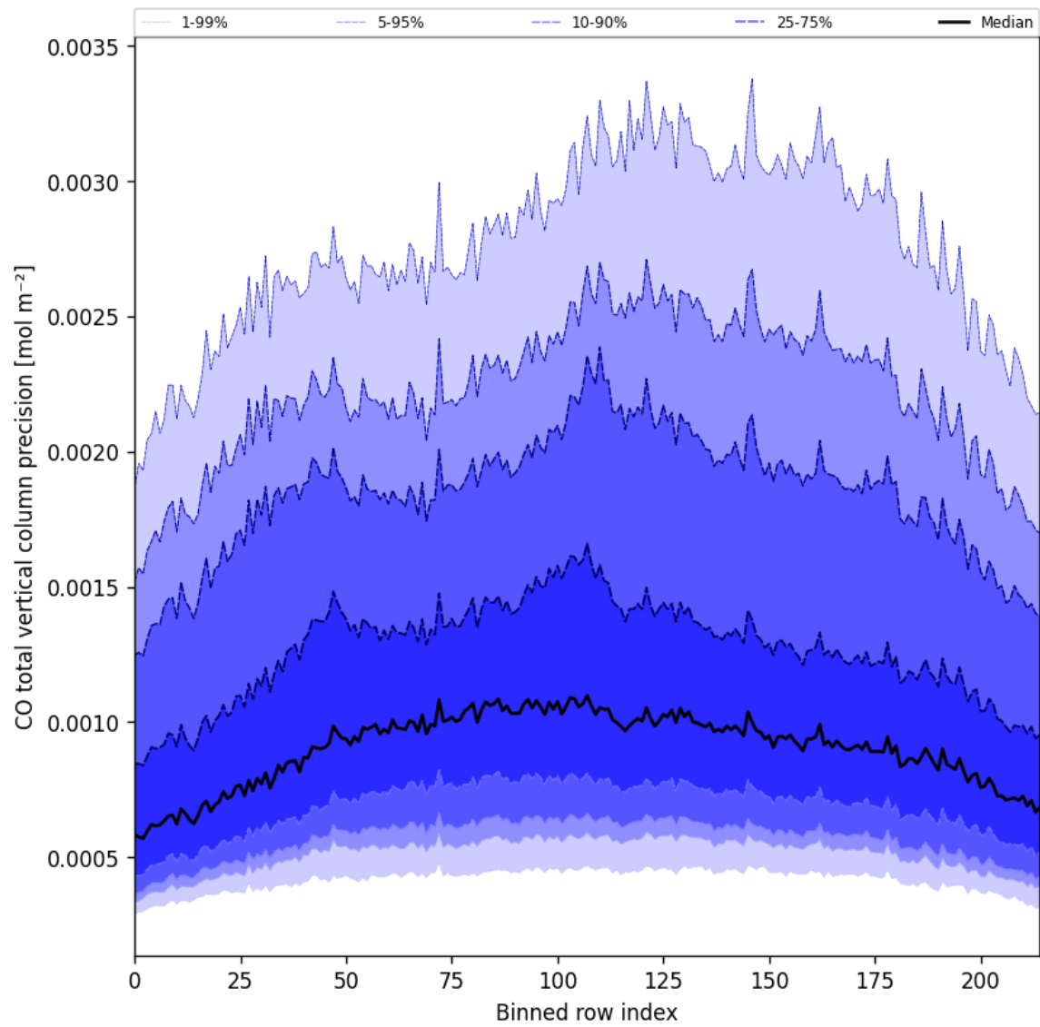
Figure 22: Along track statistics of “CO total vertical column precision” for 2025-03-05 to 2025-03-05
