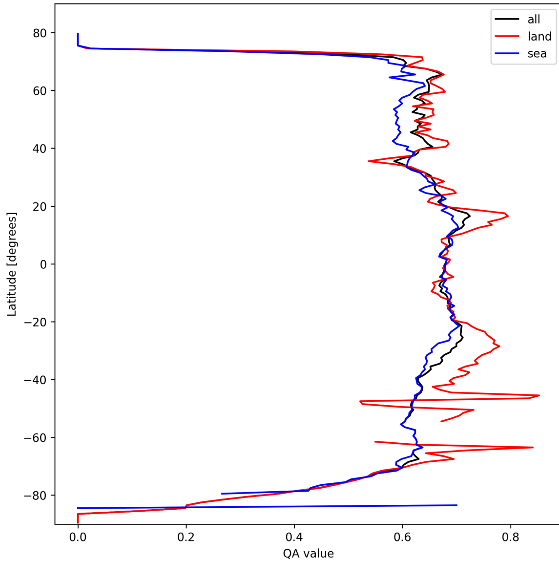
Figure 6: Zonal average of “QA value” for 2025-03-05 to 2025-03-05.
