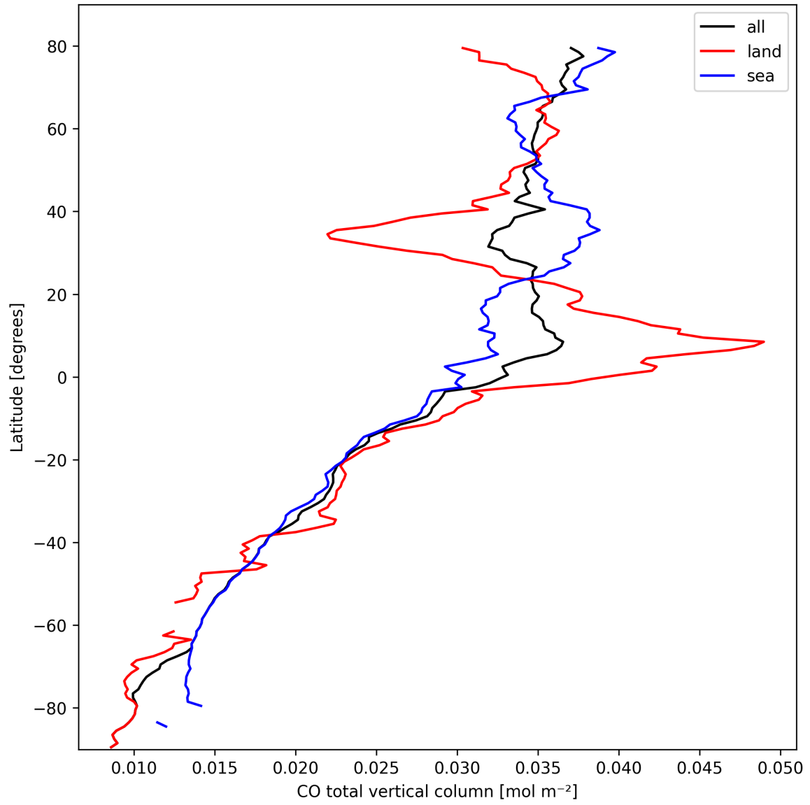
Figure 7: Zonal average of “CO total vertical column” for 2025-03-05 to 2025-03-05.
