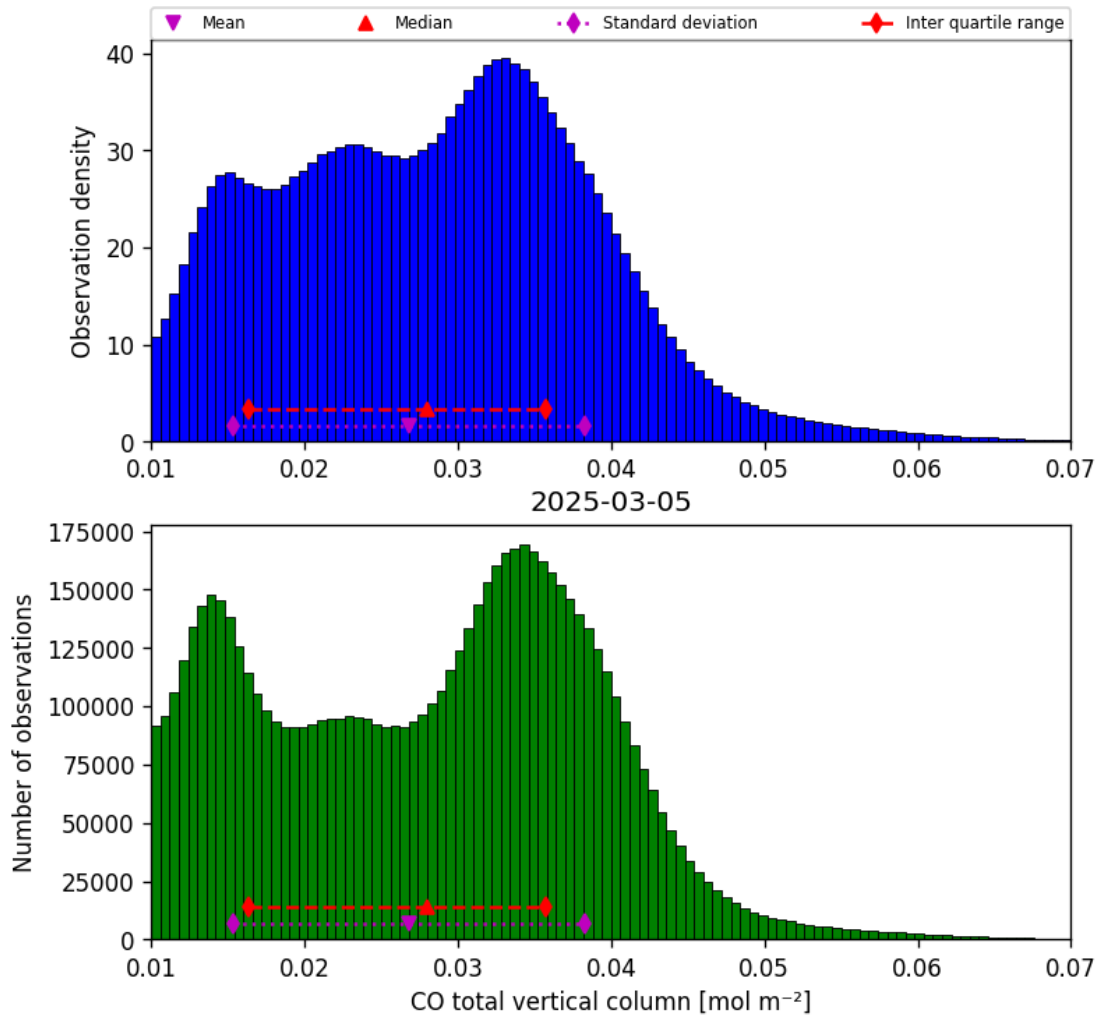
Figure 14: Histogram of “CO total vertical column” for 2025-03-05 to 2025-03-05
