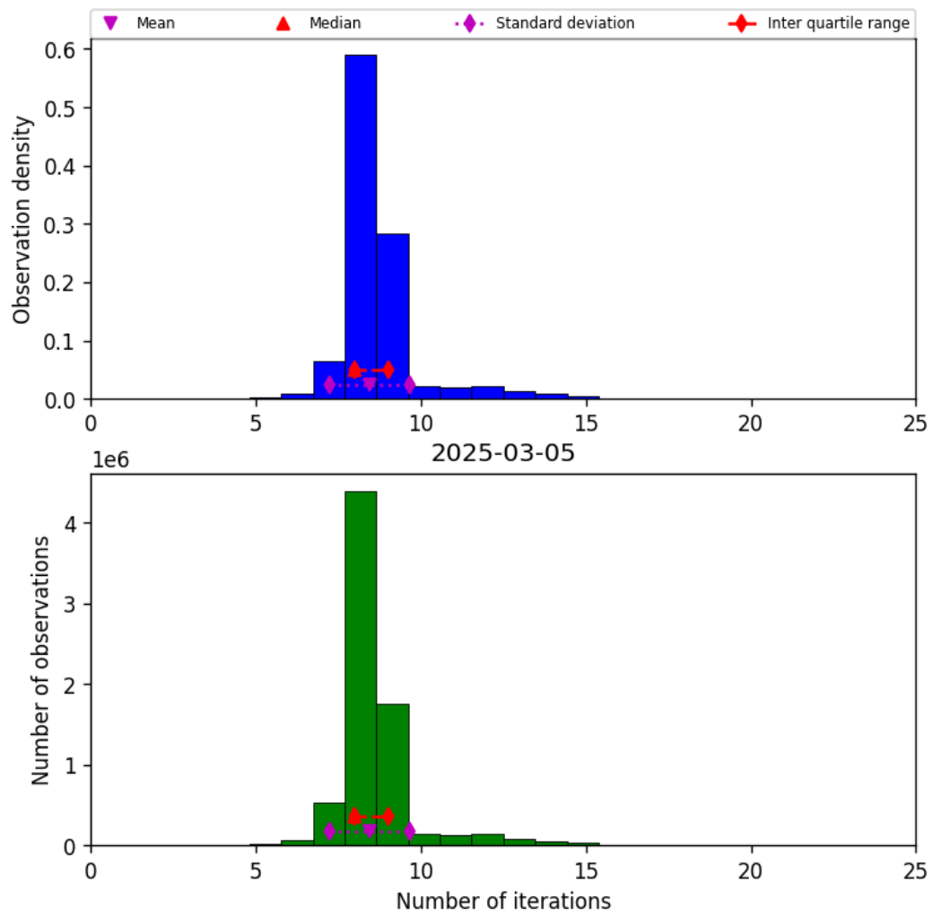
Figure 19: Histogram of “Number of iterations” for 2025-03-05 to 2025-03-05
