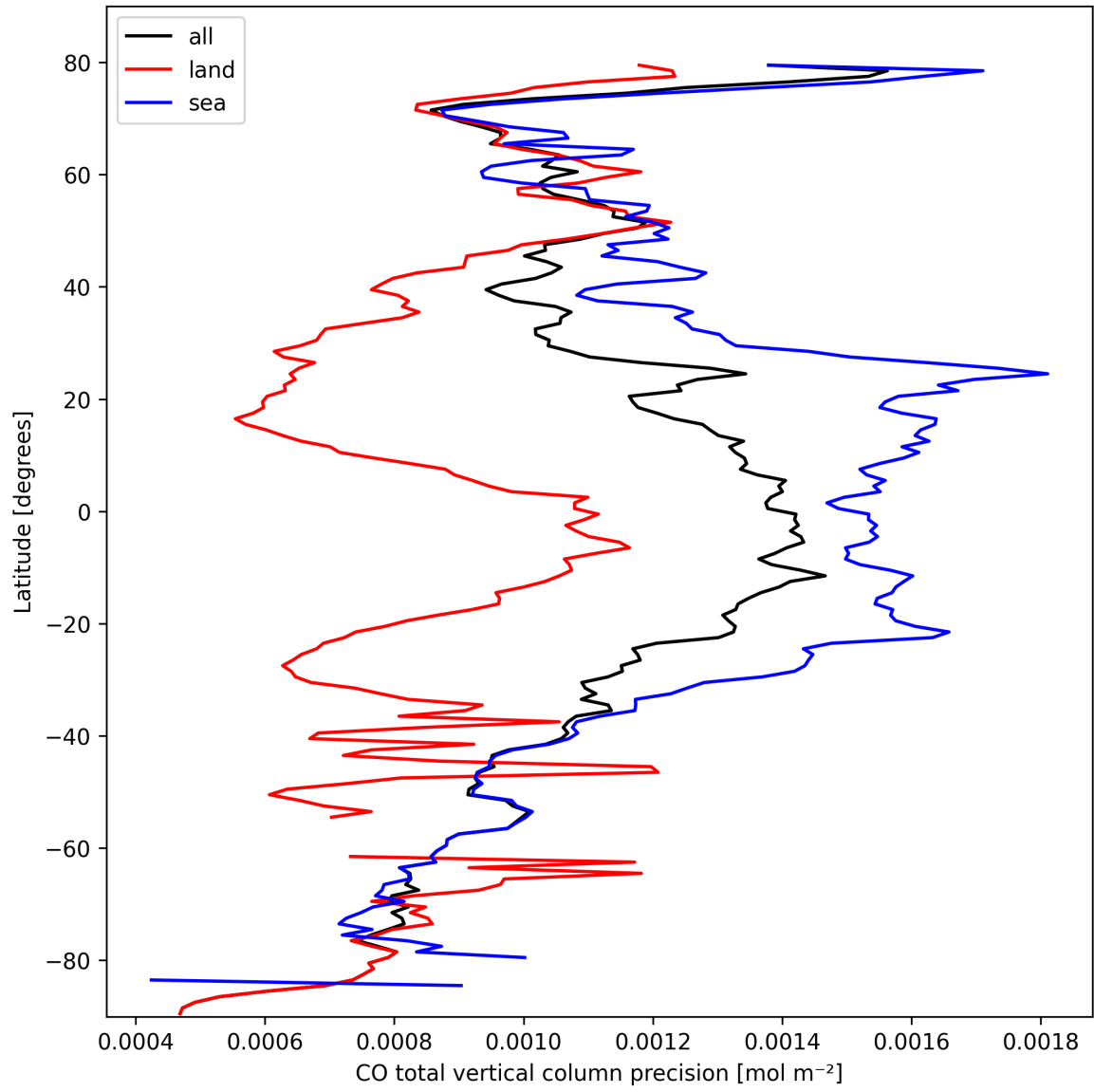
Figure 8: Zonal average of "CO total vertical column precision" for 2025-03-05 to 2025-03-05.
