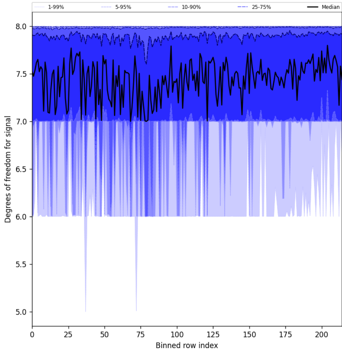
Figure 25: Along track statistics of “Degrees of freedom for signal” for 2025-03-05 to 2025-03-05
