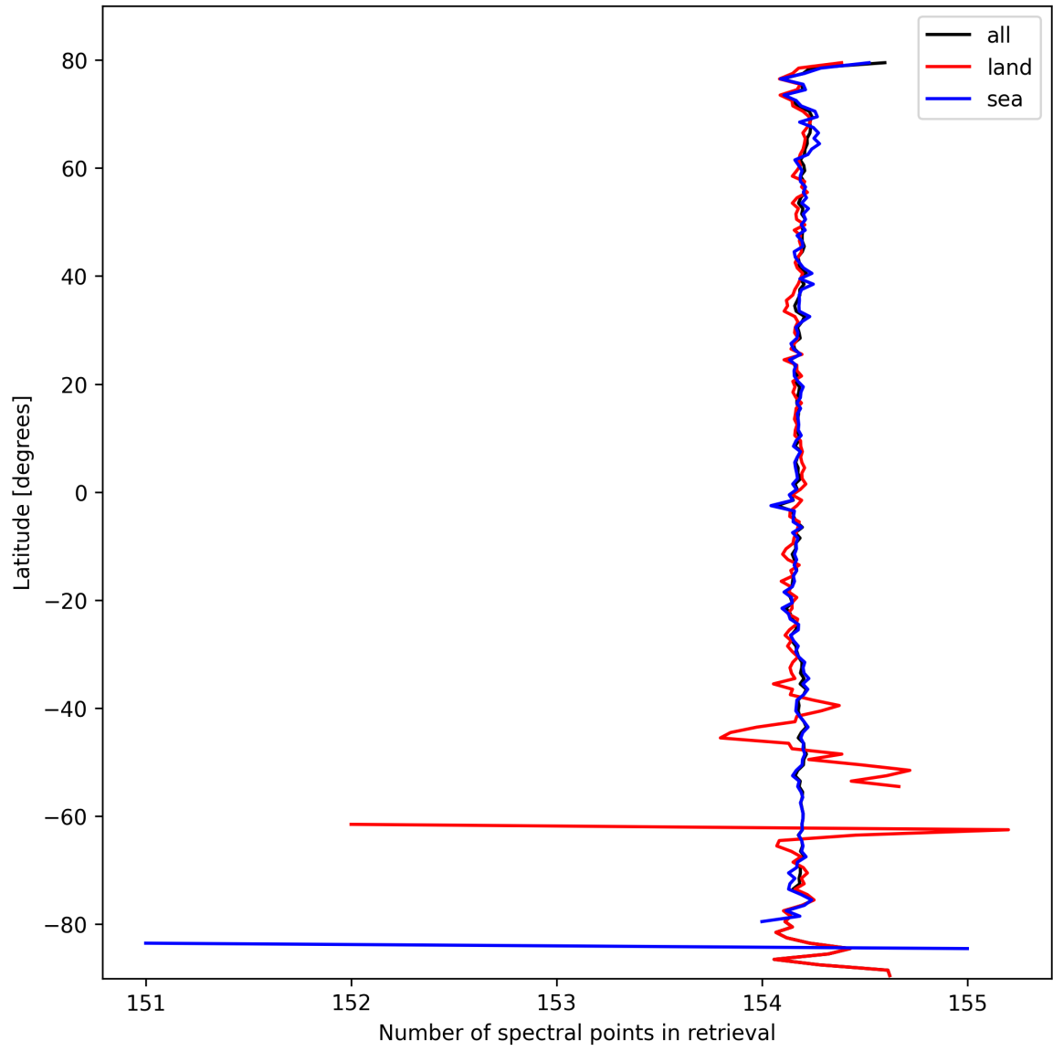
Figure 9: Zonal average of “Number of spectral points in retrieval” for 2025-03-05 to 2025-03-05.
