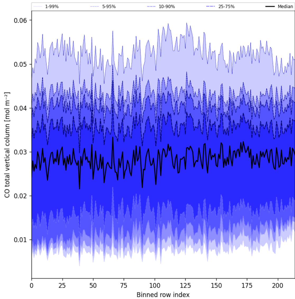
Figure 21: Along track statistics of “CO total vertical column” for 2025-03-05 to 2025-03-05
