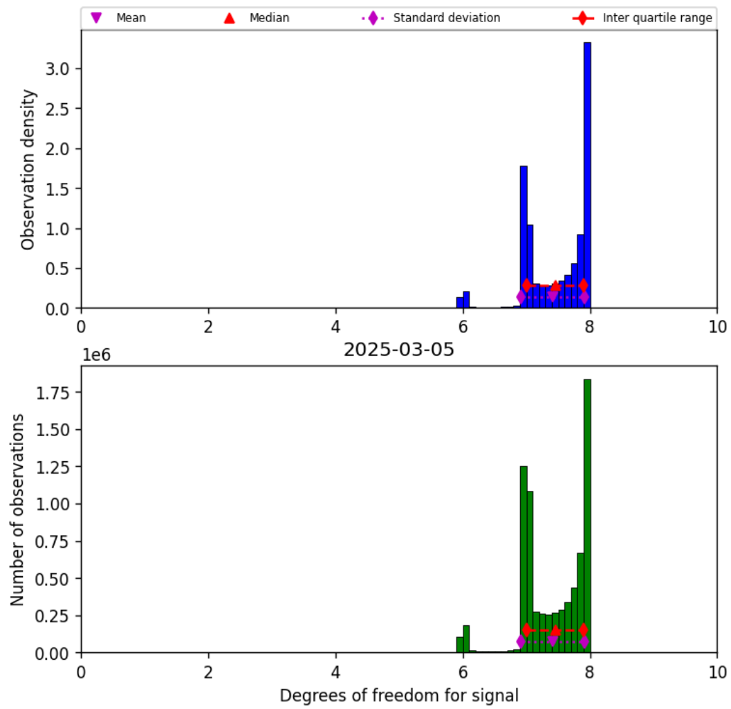
Figure 18: Histogram of “Degrees of freedom for signal” for 2025-03-05 to 2025-03-05
