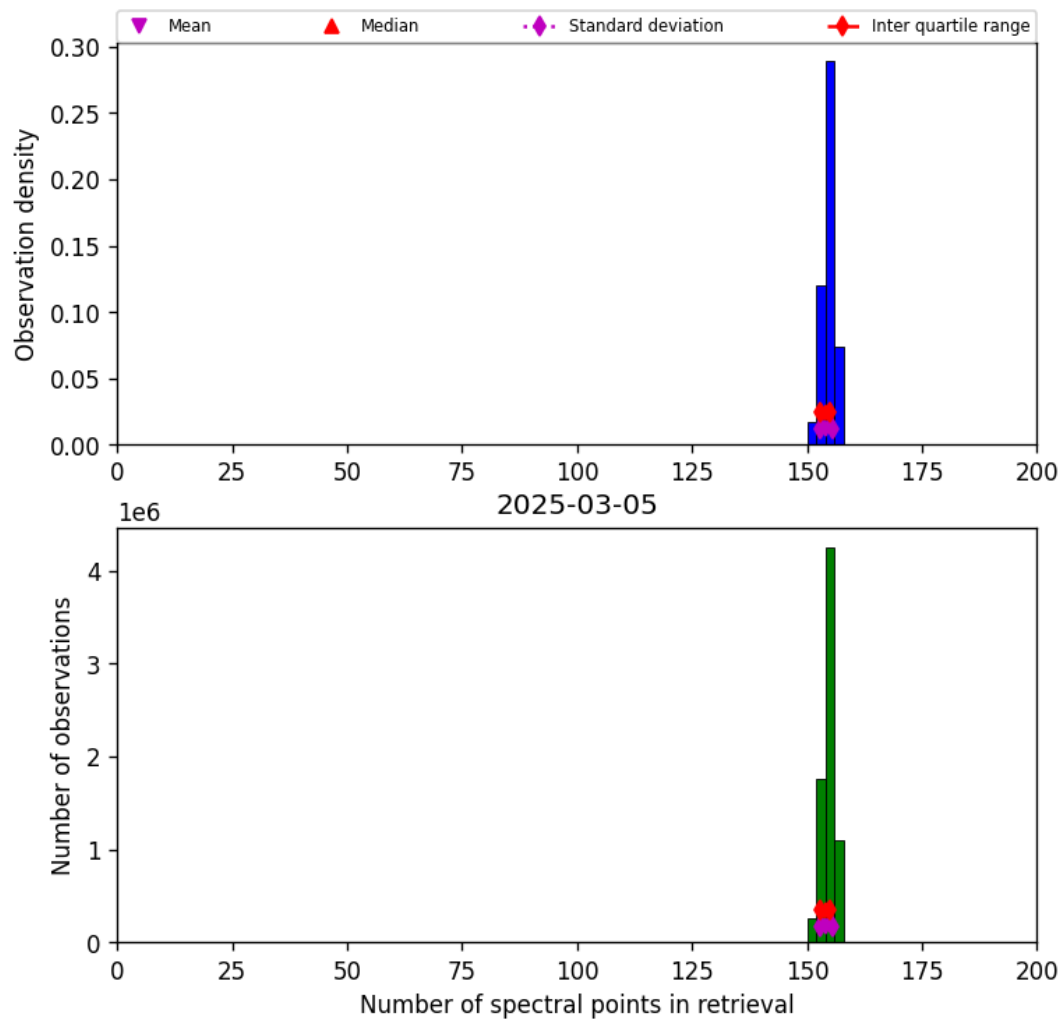
Figure 16: Histogram of “Number of spectral points in retrieval” for 2025-03-05 to 2025-03-05
