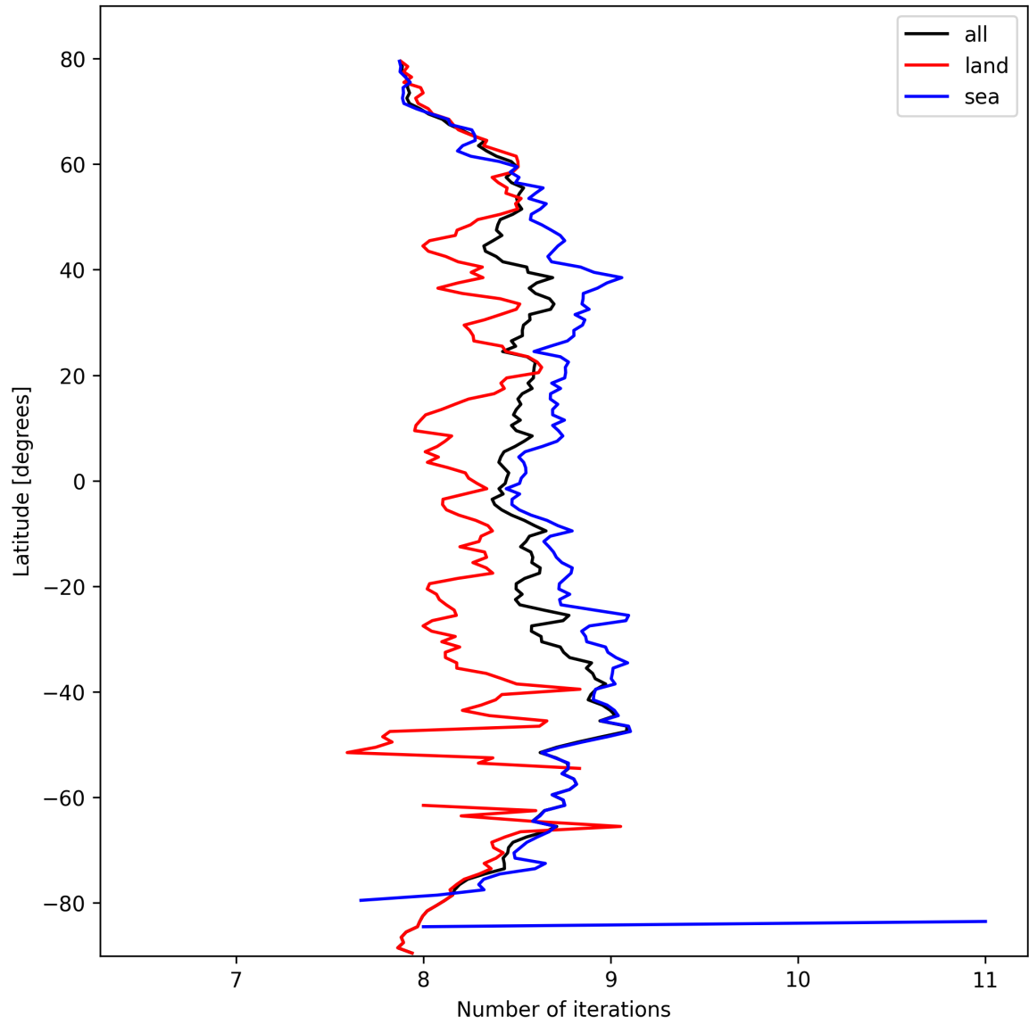
Figure 12: Zonal average of “Number of iterations” for 2025-03-05 to 2025-03-05.
