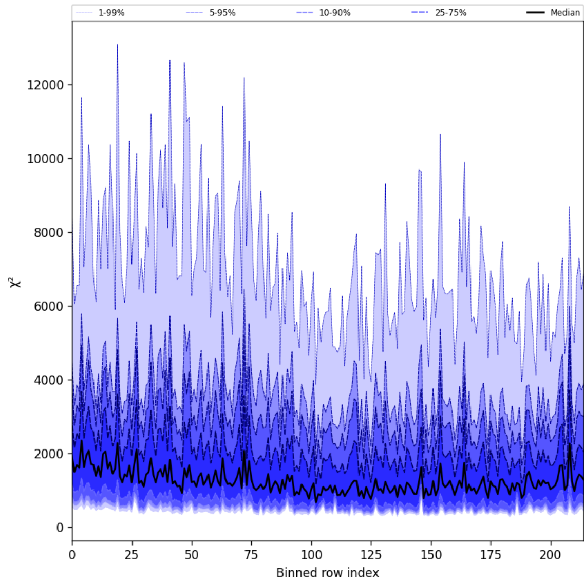
Figure 24: Along track statistics of “ \chi^2 ” for 2025-03-06 to 2025-03-07
