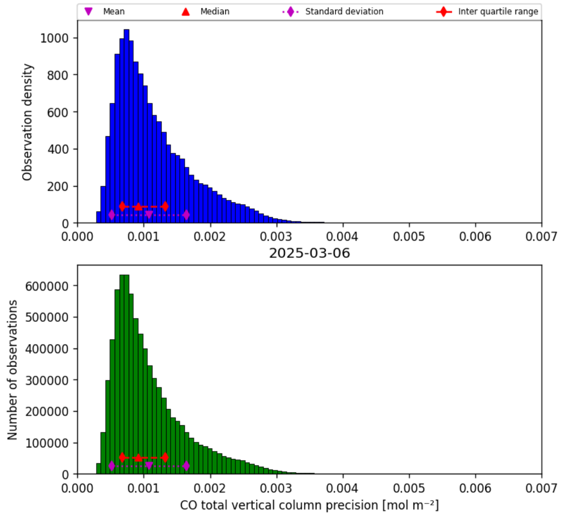
Figure 15: Histogram of “CO total vertical column precision” for 2025-03-06 to 2025-03-07
