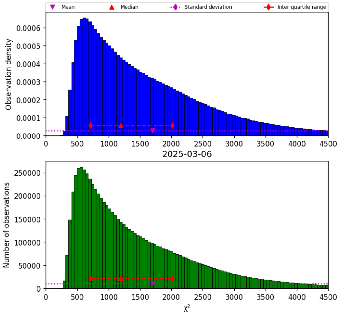
Figure 17: Histogram of “ \chi^2 ” for 2025-03-06 to 2025-03-07
