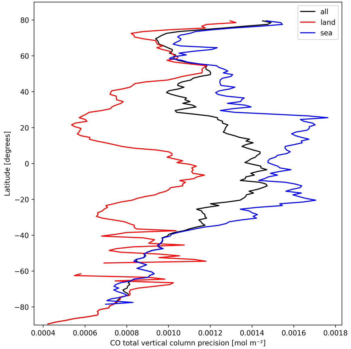
Figure 8: Zonal average of “CO total vertical column precision” for 2025-03-06 to 2025-03-07.
