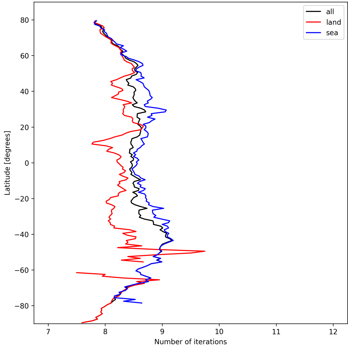
Figure 12: Zonal average of “Number of iterations” for 2025-03-06 to 2025-03-07.
