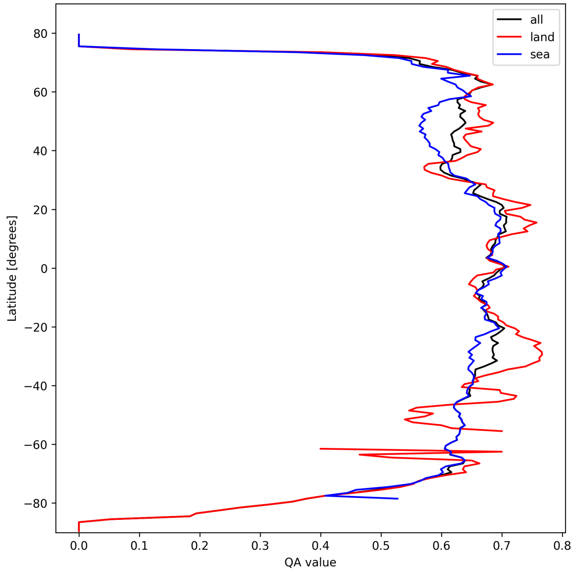
Figure 6: Zonal average of “QA value” for 2025-03-06 to 2025-03-07.
