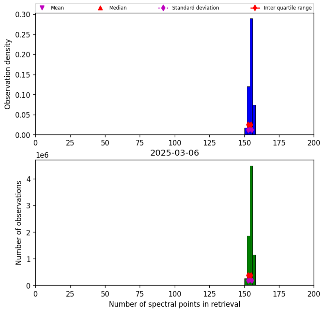
Figure 16: Histogram of “Number of spectral points in retrieval” for 2025-03-06 to 2025-03-07
