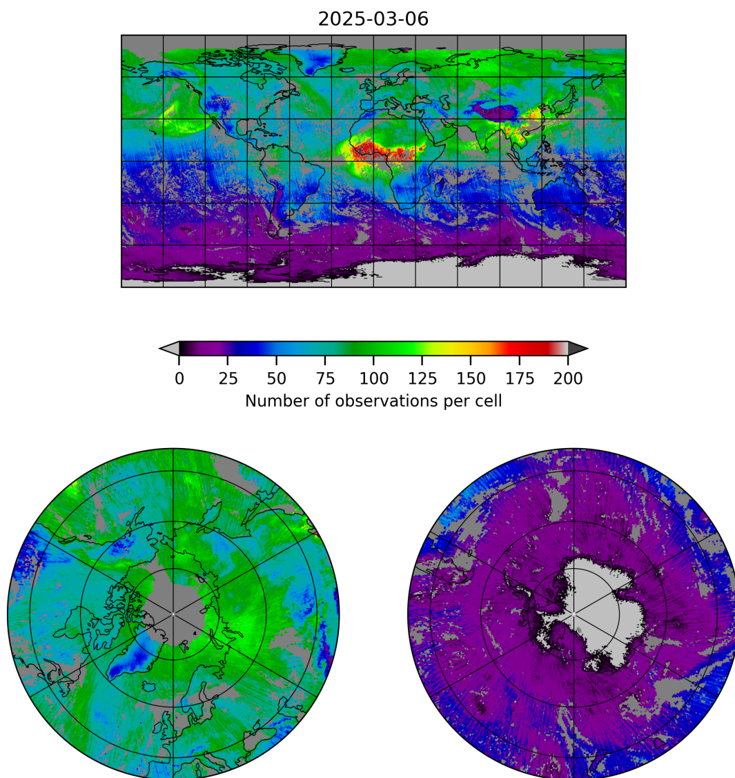
Figure 5: Map of the number of observations for 2025-03-06 to 2025-03-07
