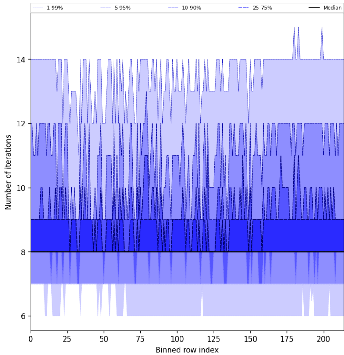
Figure 26: Along track statistics of “Number of iterations” for 2025-03-06 to 2025-03-07
