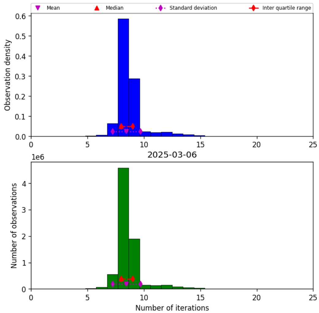
Figure 19: Histogram of “Number of iterations” for 2025-03-06 to 2025-03-07
