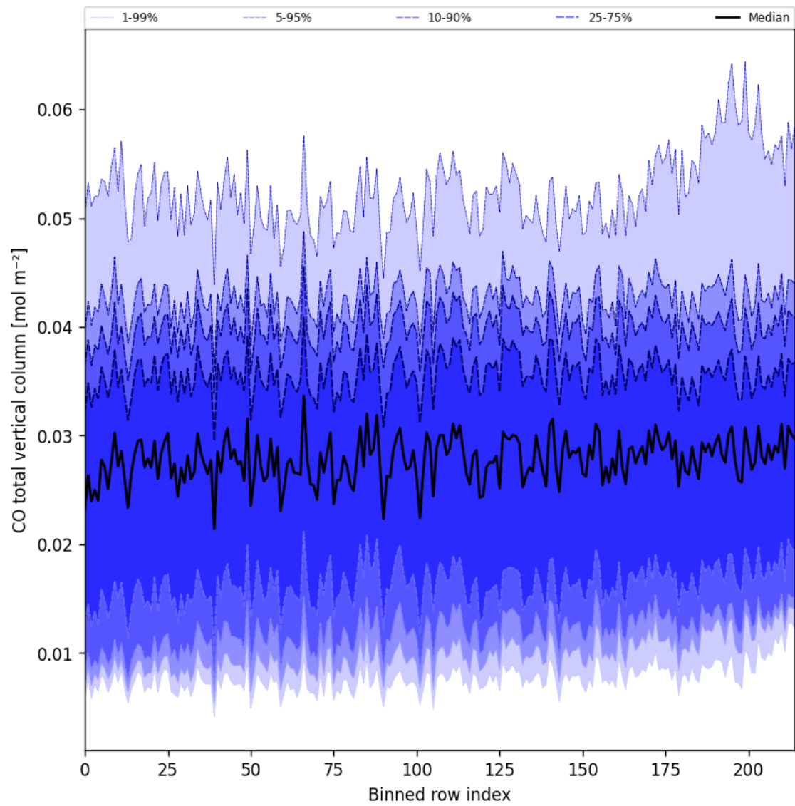
Figure 21: Along track statistics of “CO total vertical column” for 2025-03-06 to 2025-03-07
