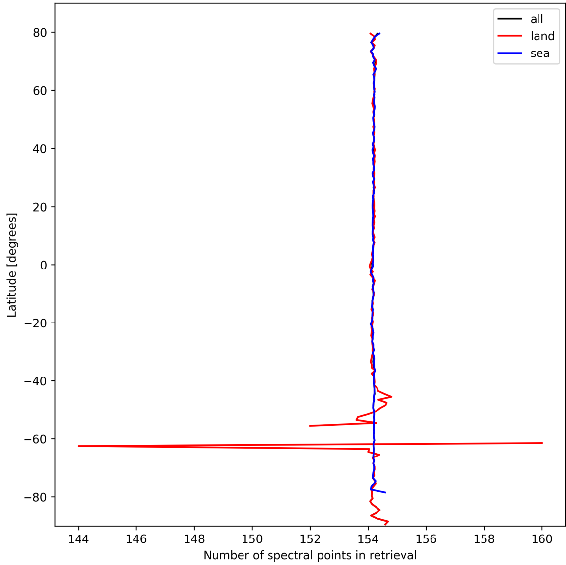
Figure 9: Zonal average of “Number of spectral points in retrieval” for 2025-03-06 to 2025-03-07.
