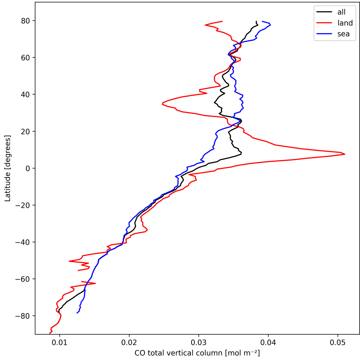
Figure 7: Zonal average of “CO total vertical column” for 2025-03-06 to 2025-03-07.
