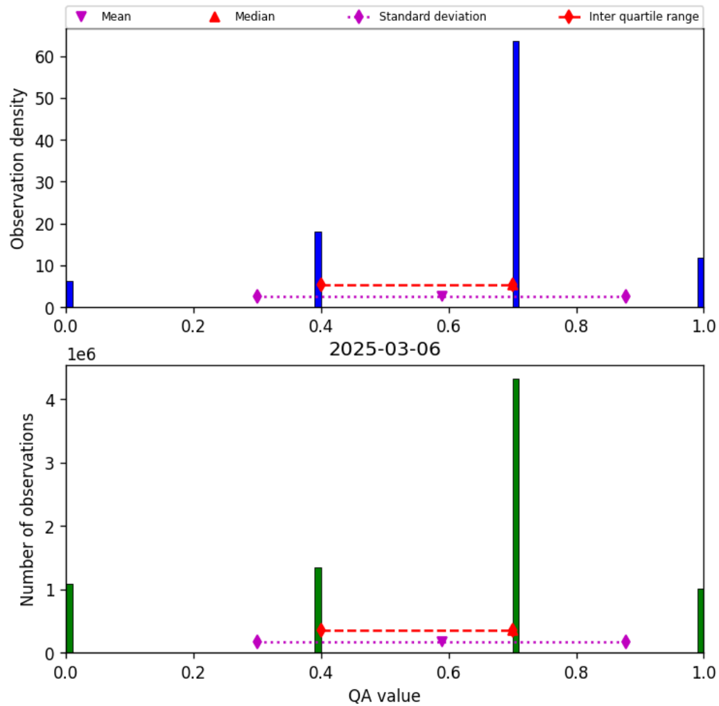
Figure 13: Histogram of “QA value” for 2025-03-06 to 2025-03-07
