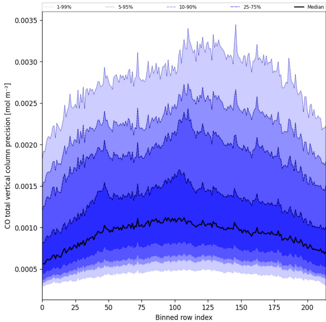
Figure 22: Along track statistics of “CO total vertical column precision” for 2025-03-06 to 2025-03-07
