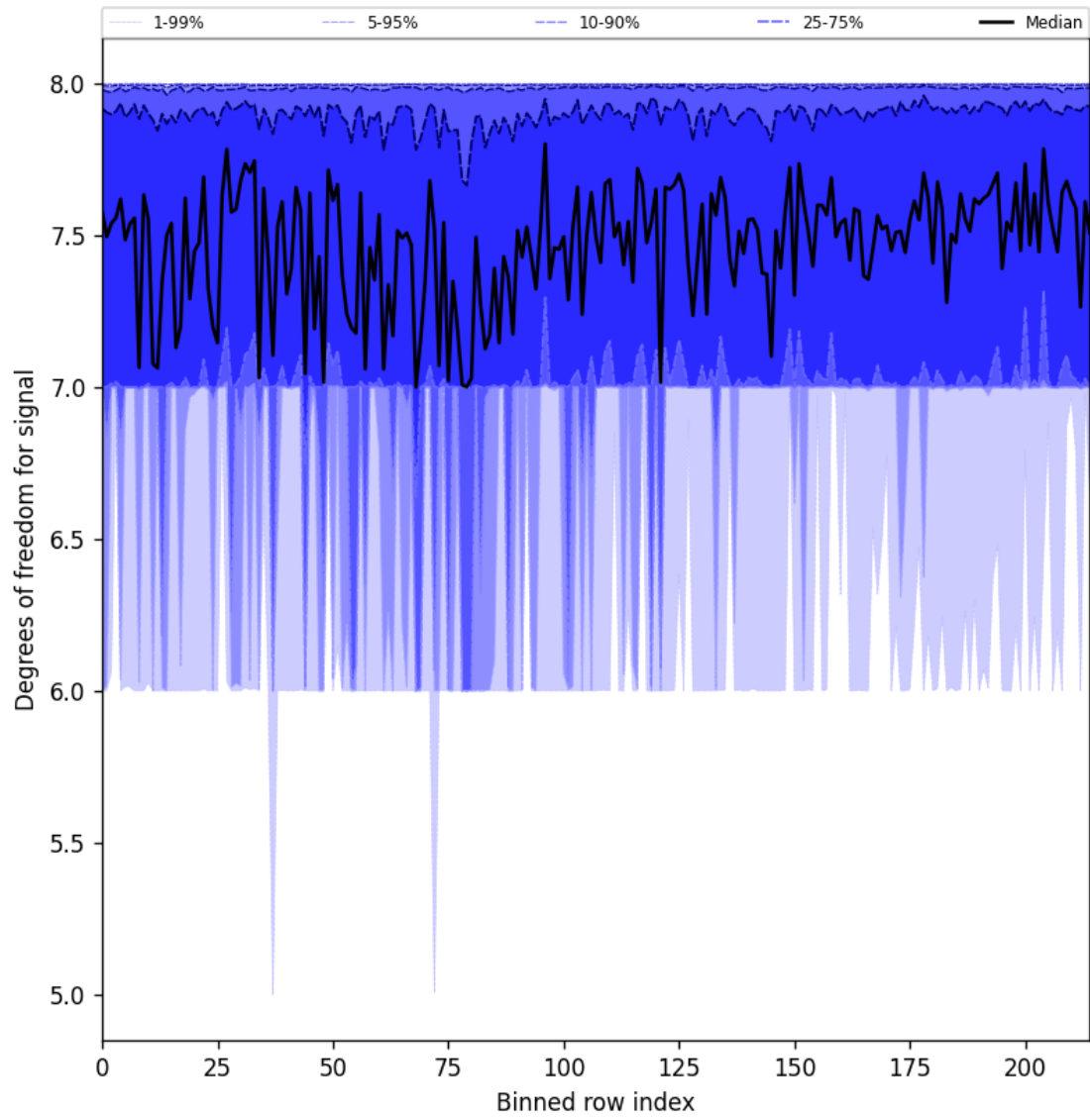
Figure 25: Along track statistics of “Degrees of freedom for signal” for 2025-03-06 to 2025-03-07
