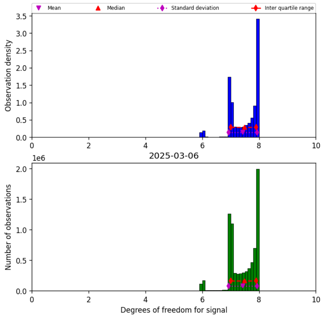
Figure 18: Histogram of “Degrees of freedom for signal” for 2025-03-06 to 2025-03-07
