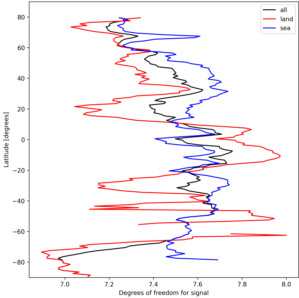
Figure 11: Zonal average of “Degrees of freedom for signal” for 2025-03-06 to 2025-03-07.
