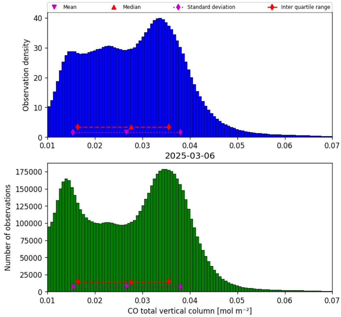
Figure 14: Histogram of “CO total vertical column” for 2025-03-06 to 2025-03-07
