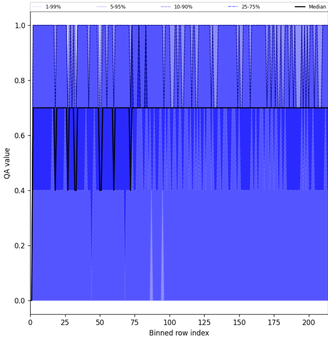
Figure 20: Along track statistics of “QA value” for 2025-03-06 to 2025-03-07
