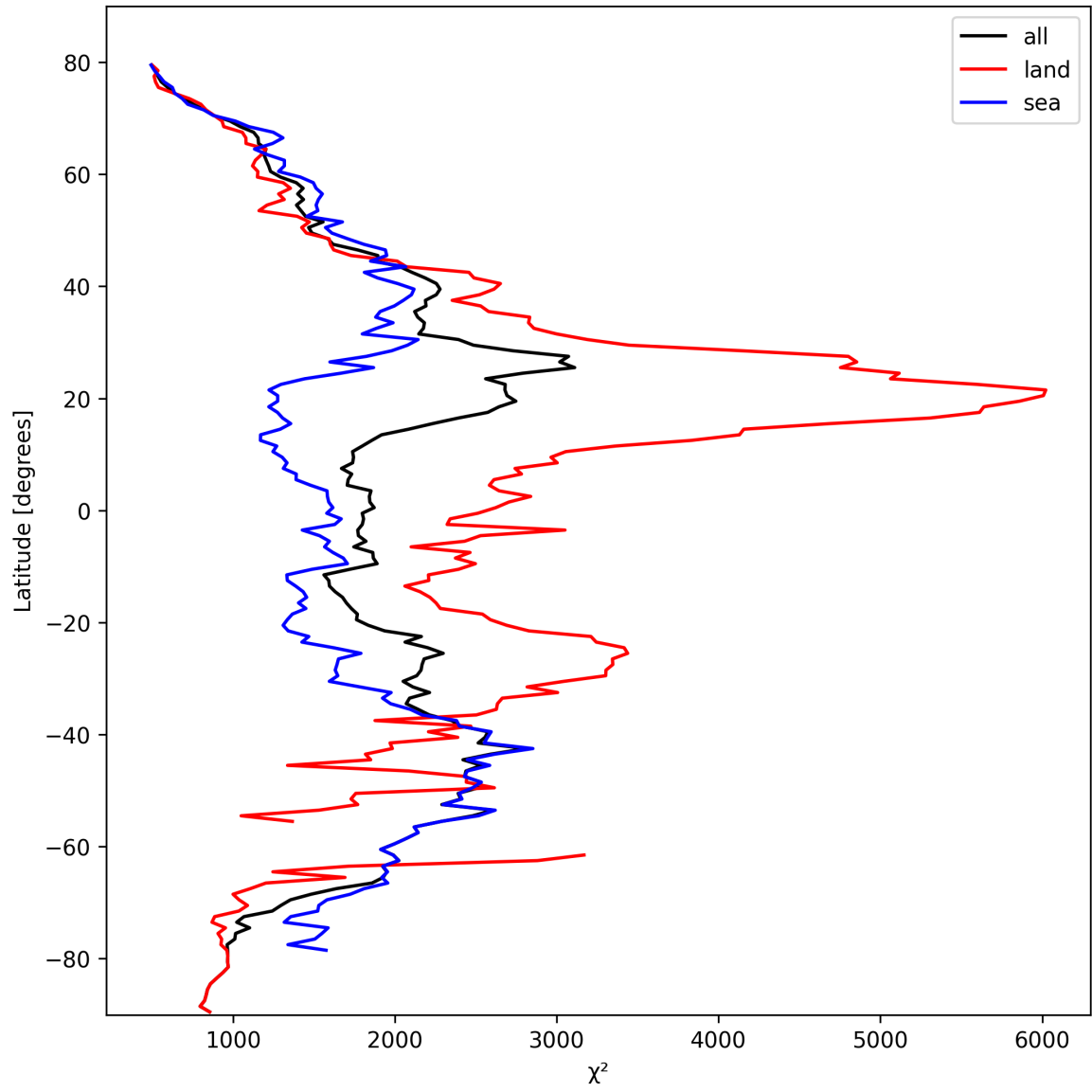
Figure 10: Zonal average of “ \chi^2 ” for 2025-03-06 to 2025-03-07.
