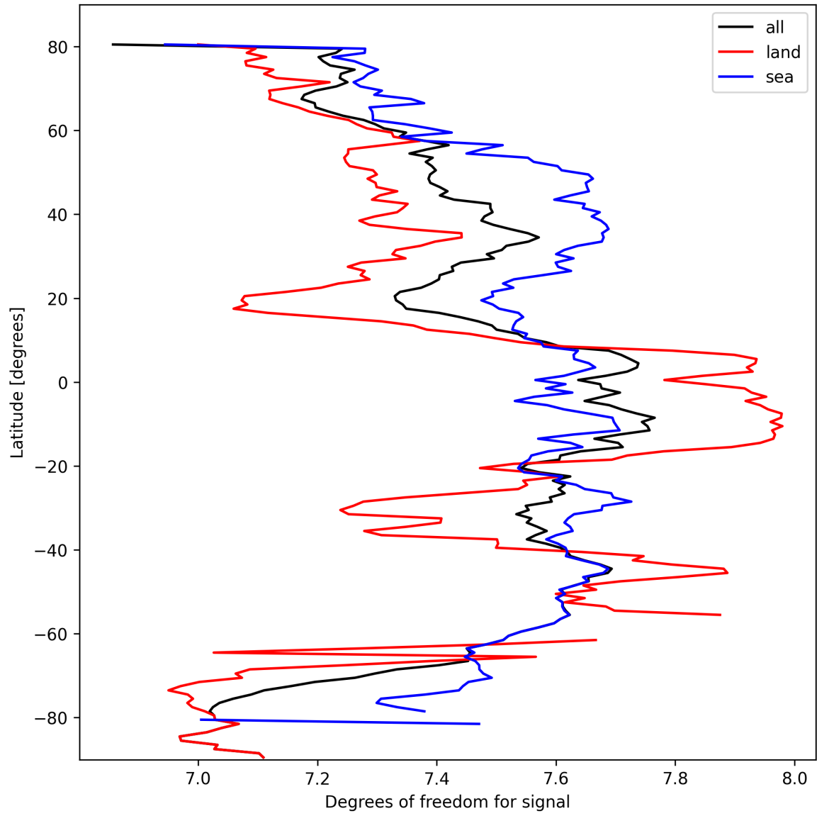
Figure 11: Zonal average of “Degrees of freedom for signal” for 2025-03-07 to 2025-03-08.
