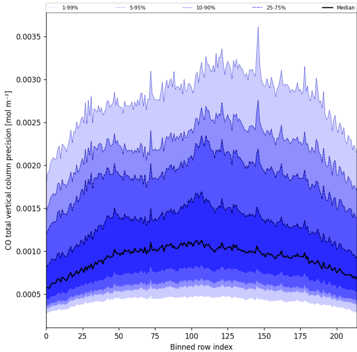
Figure 22: Along track statistics of “CO total vertical column precision” for 2025-03-07 to 2025-03-08
