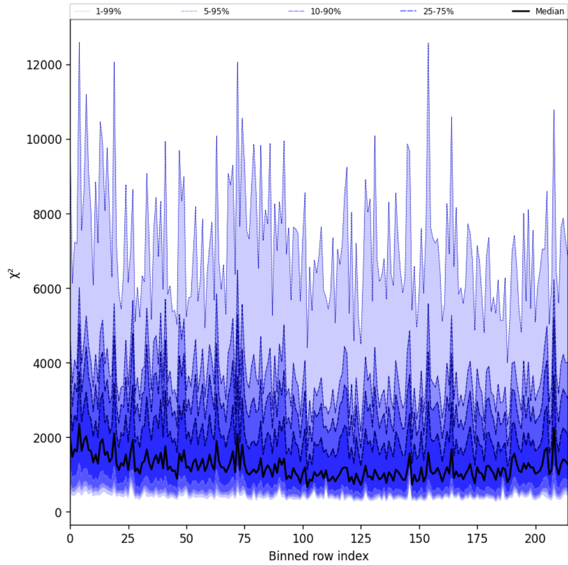
Figure 24: Along track statistics of “ \chi^2 ” for 2025-03-07 to 2025-03-08
