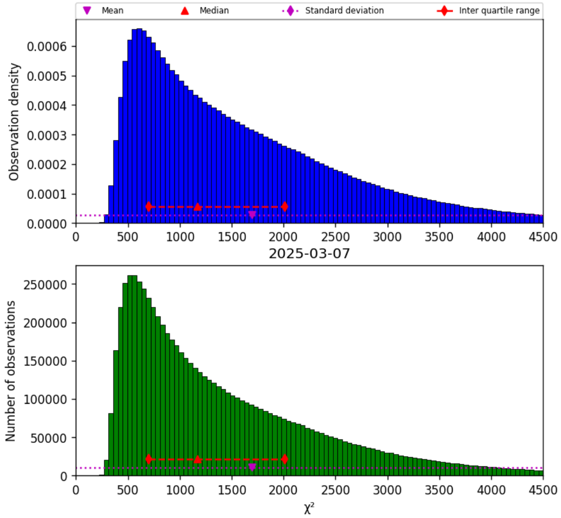
Figure 17: Histogram of " \chi^2 " for 2025-03-07 to 2025-03-08
