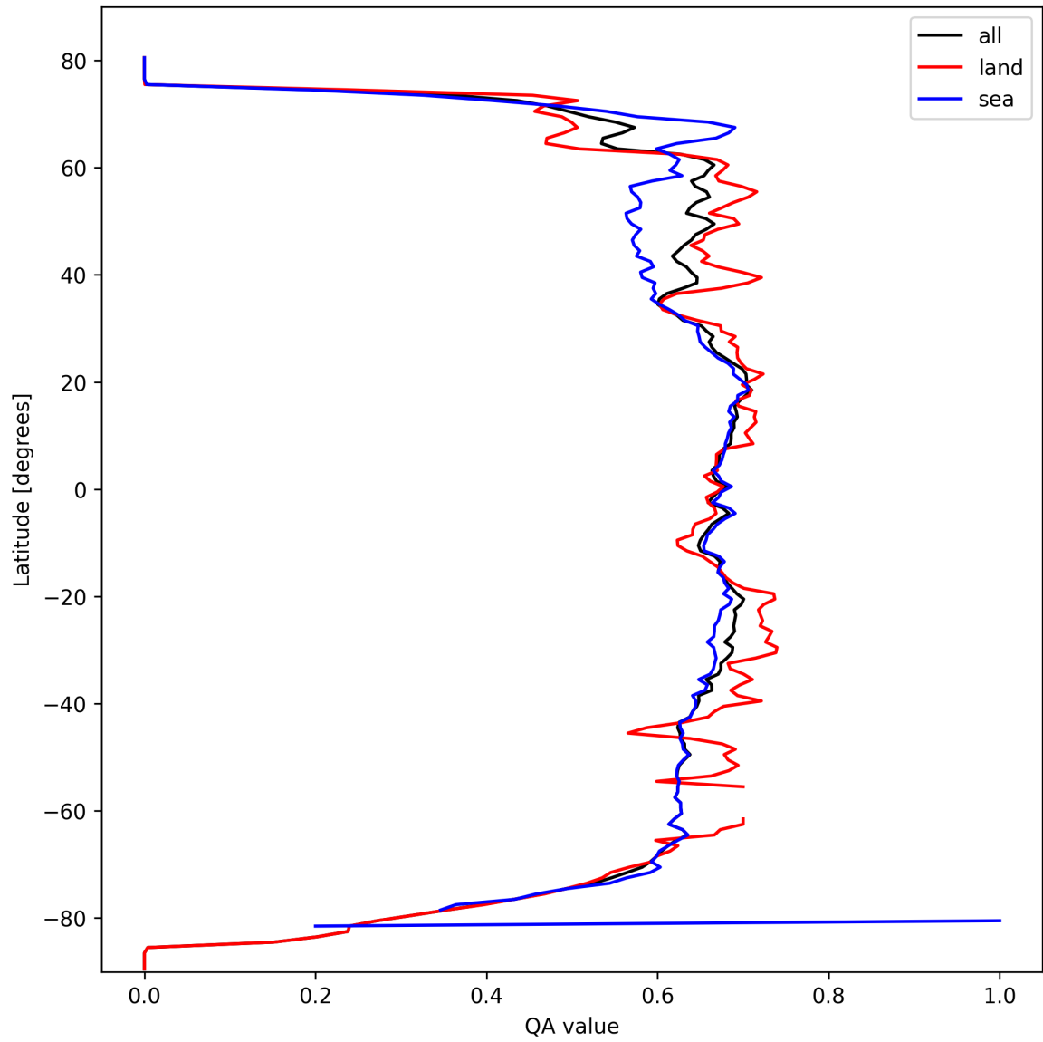
Figure 6: Zonal average of “QA value” for 2025-03-07 to 2025-03-08.
