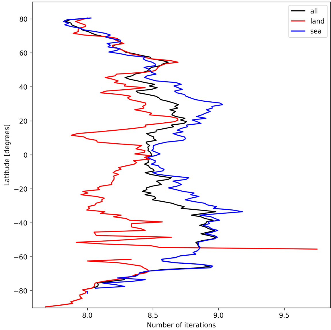
Figure 12: Zonal average of “Number of iterations” for 2025-03-07 to 2025-03-08.
