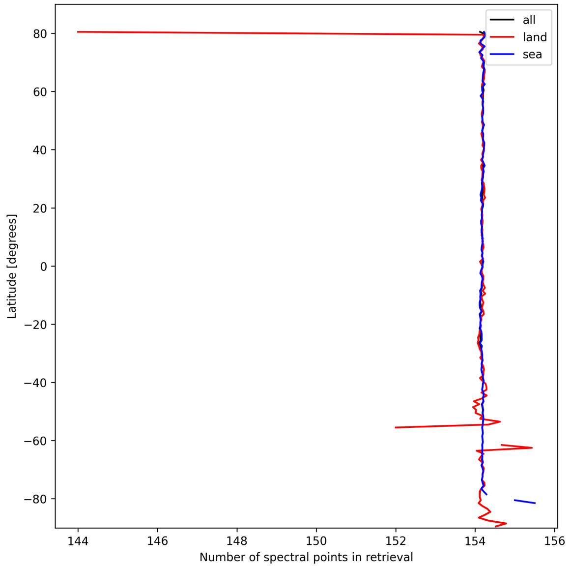
Figure 9: Zonal average of “Number of spectral points in retrieval” for 2025-03-07 to 2025-03-08.
