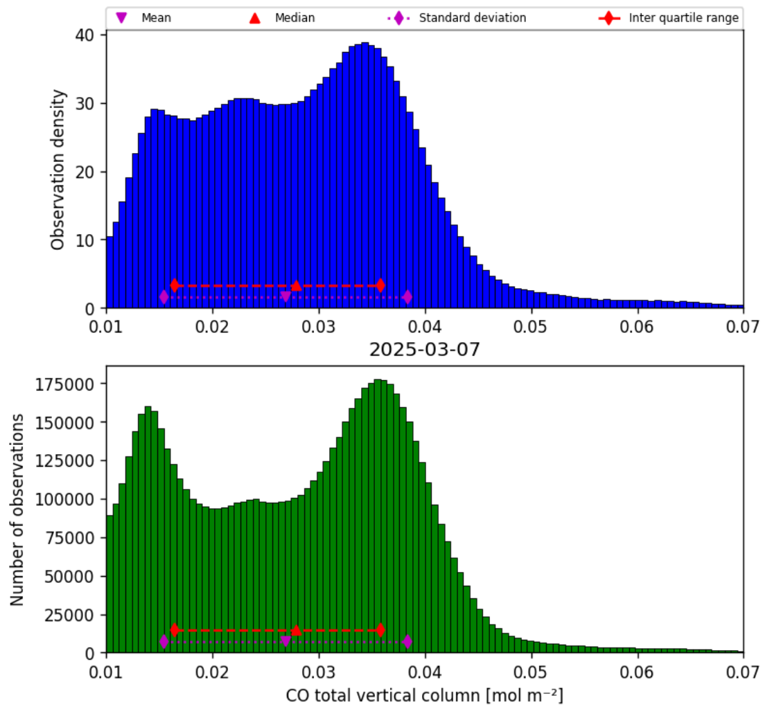
Figure 14: Histogram of “CO total vertical column” for 2025-03-07 to 2025-03-08
