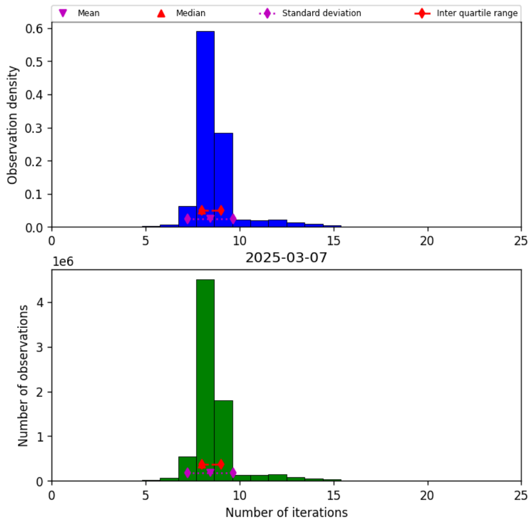
Figure 19: Histogram of “Number of iterations” for 2025-03-07 to 2025-03-08
