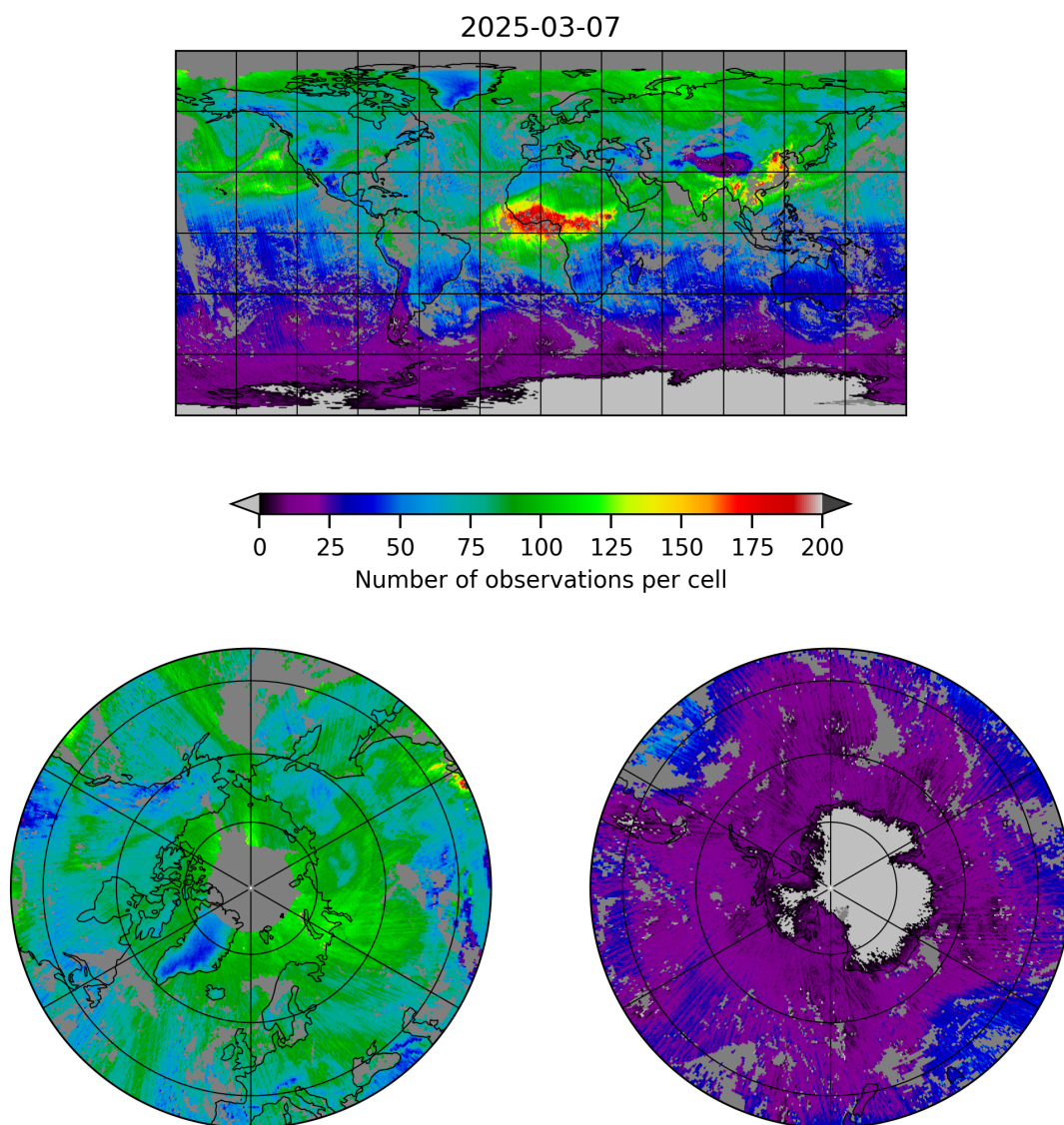
Figure 5: Map of the number of observations for 2025-03-07 to 2025-03-08
