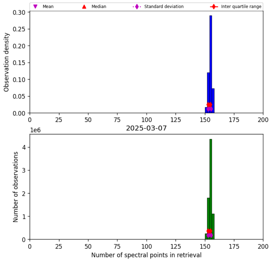
Figure 16: Histogram of “Number of spectral points in retrieval” for 2025-03-07 to 2025-03-08
