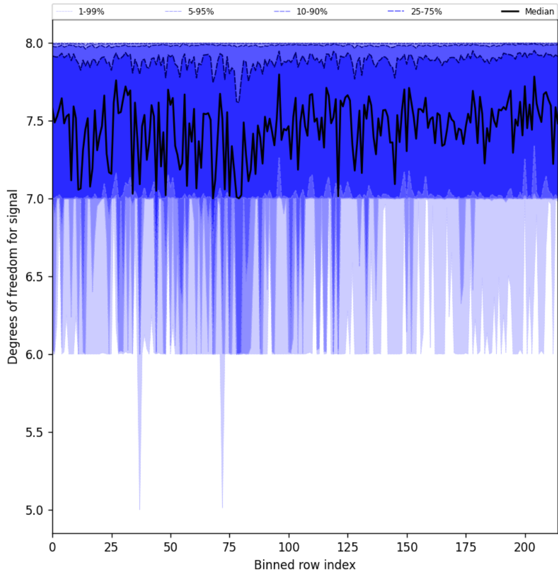
Figure 25: Along track statistics of “Degrees of freedom for signal” for 2025-03-07 to 2025-03-08
