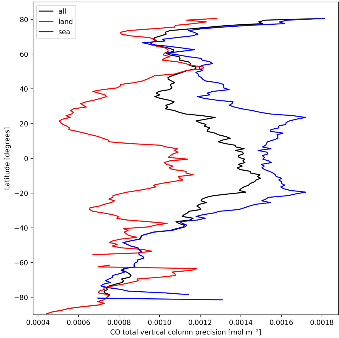
Figure 8: Zonal average of "CO total vertical column precision" for 2025-03-07 to 2025-03-08.
