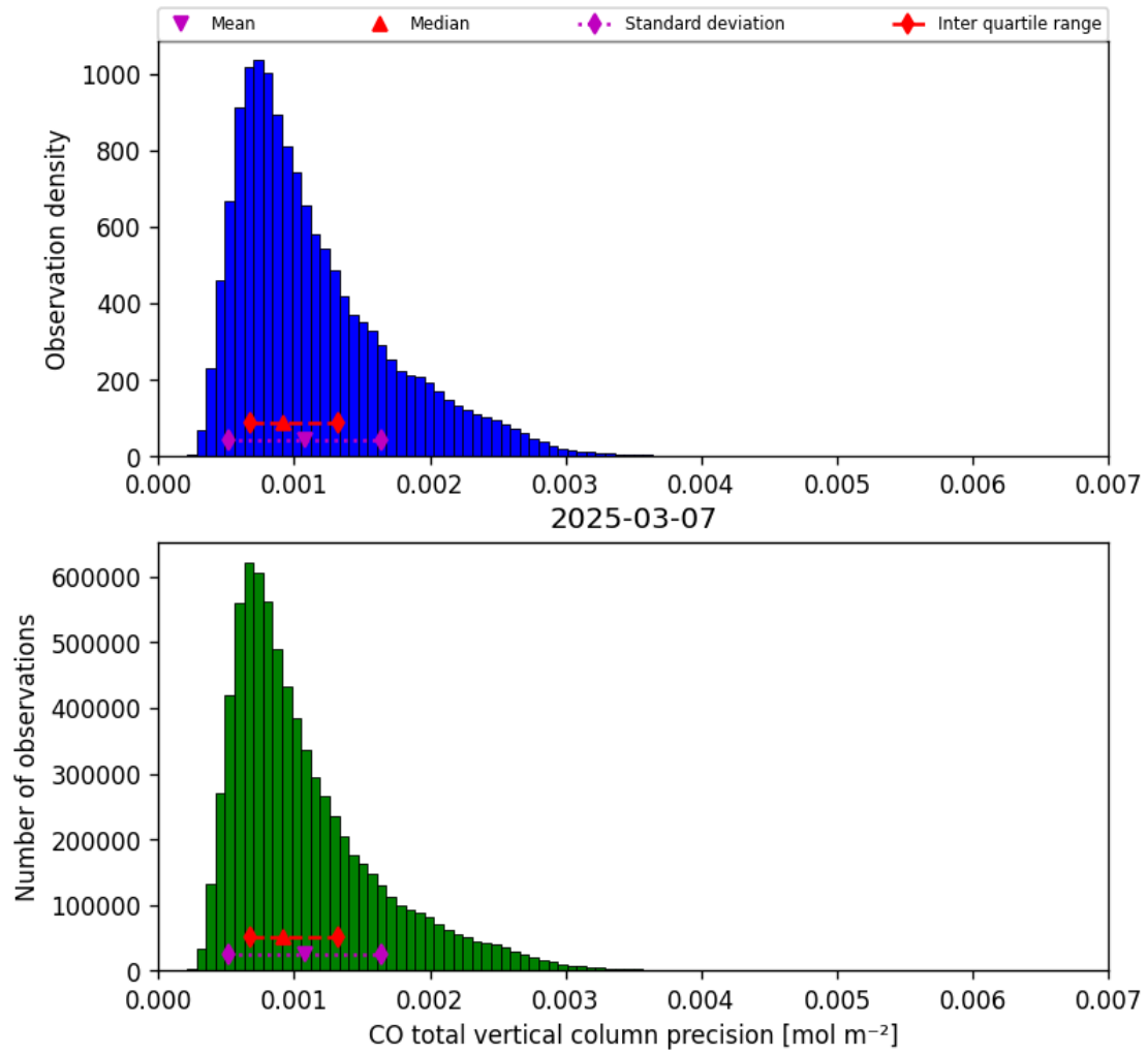
Figure 15: Histogram of “CO total vertical column precision” for 2025-03-07 to 2025-03-08
