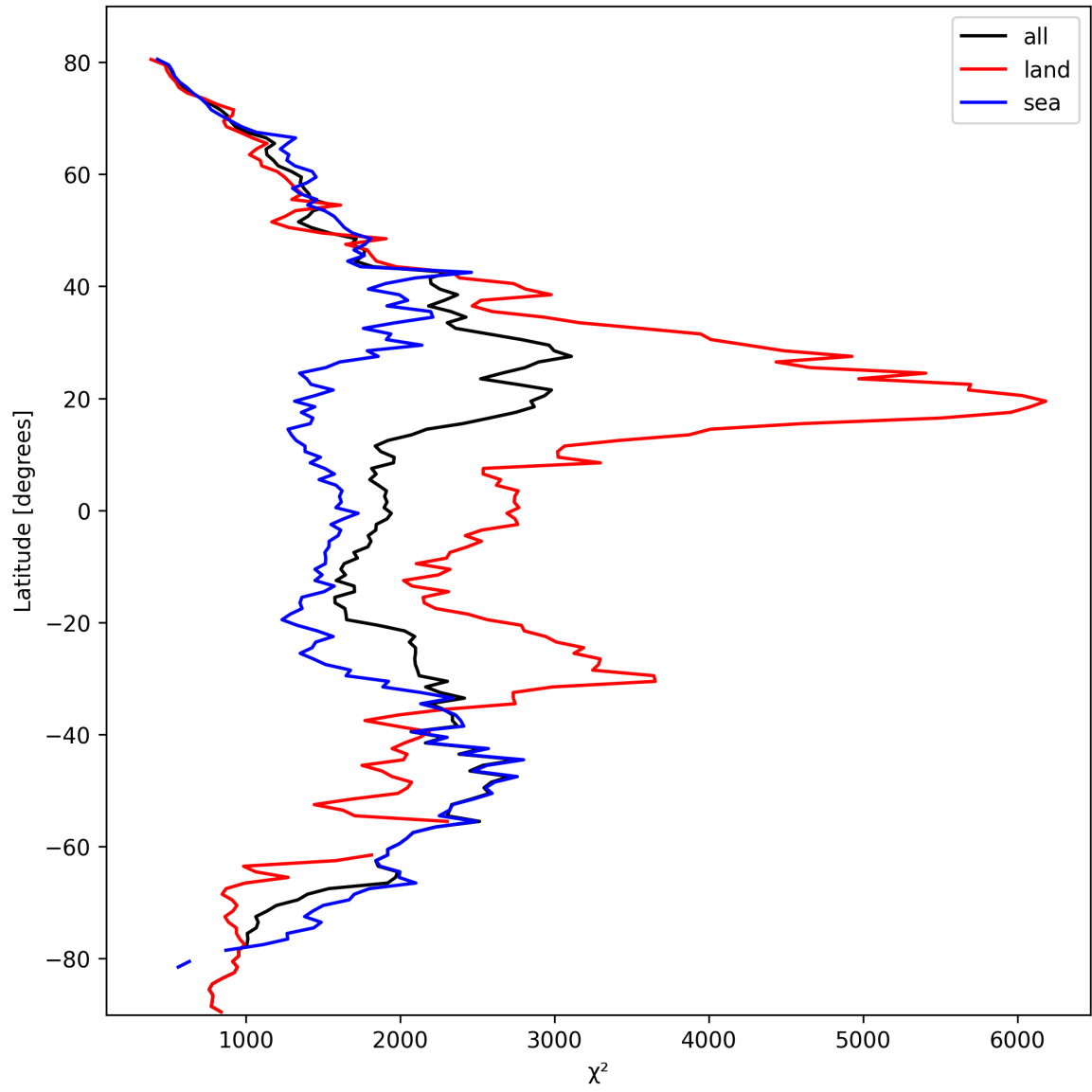
Figure 10: Zonal average of “ \chi^2 ” for 2025-03-07 to 2025-03-08.
