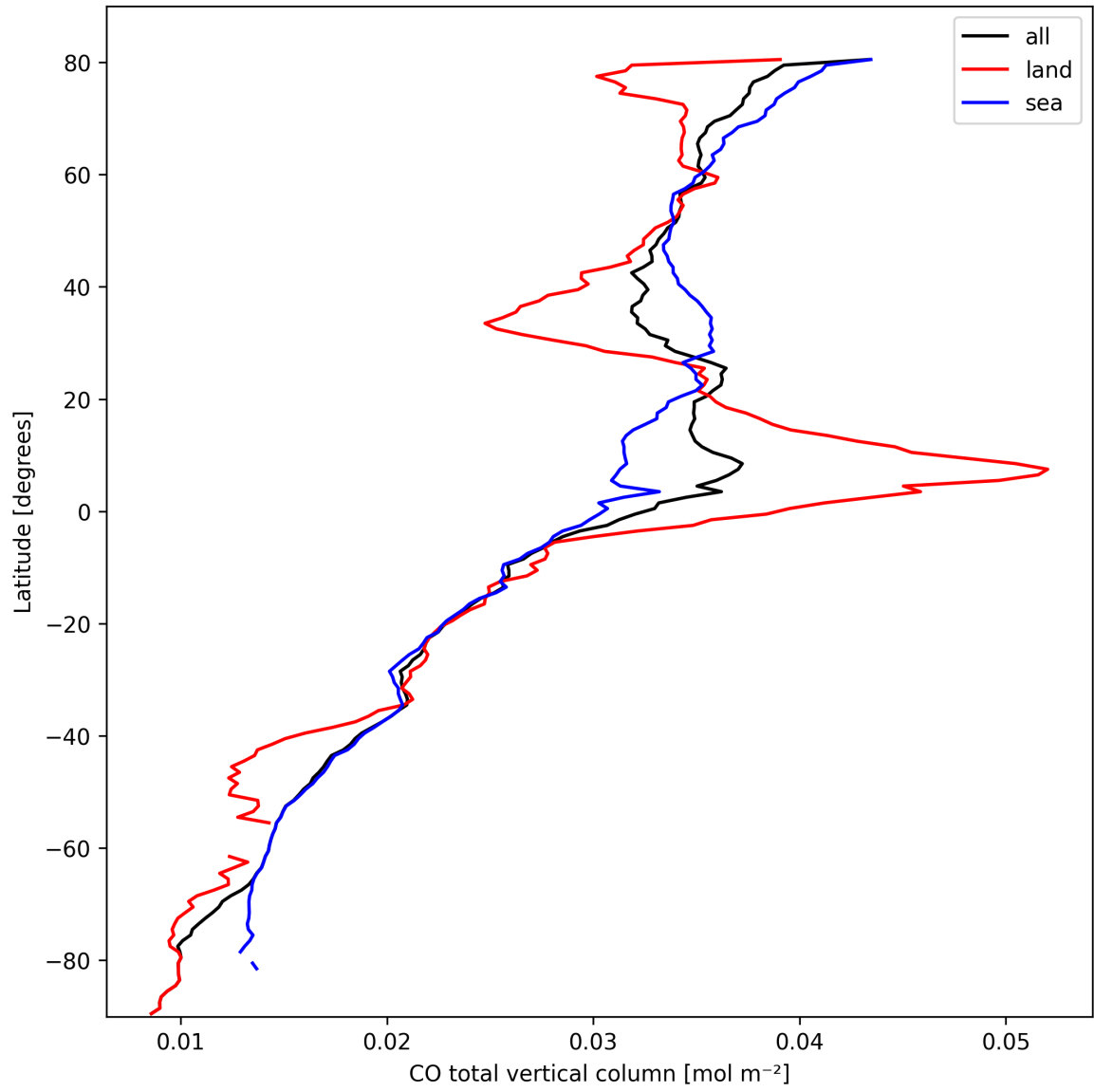
Figure 7: Zonal average of “CO total vertical column” for 2025-03-07 to 2025-03-08.
