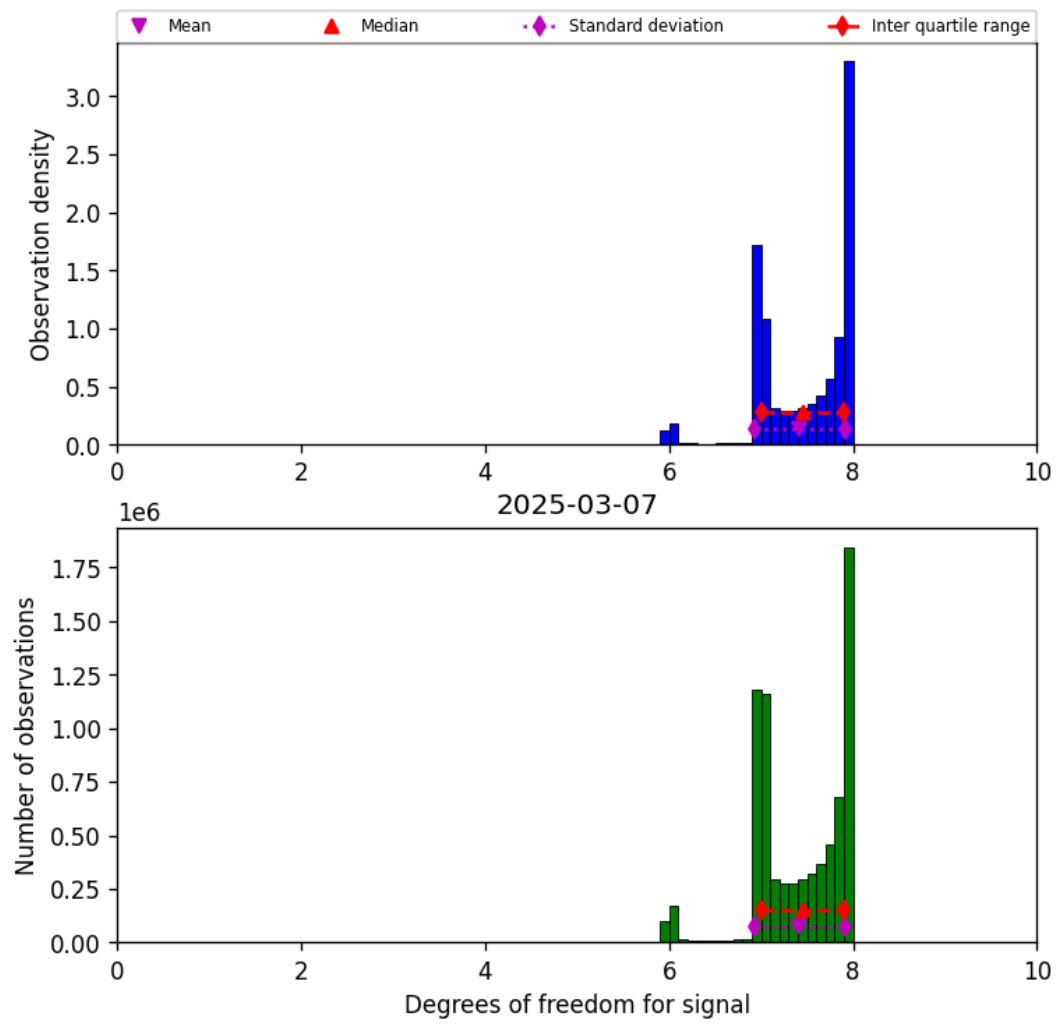
Figure 18: Histogram of “Degrees of freedom for signal” for 2025-03-07 to 2025-03-08
