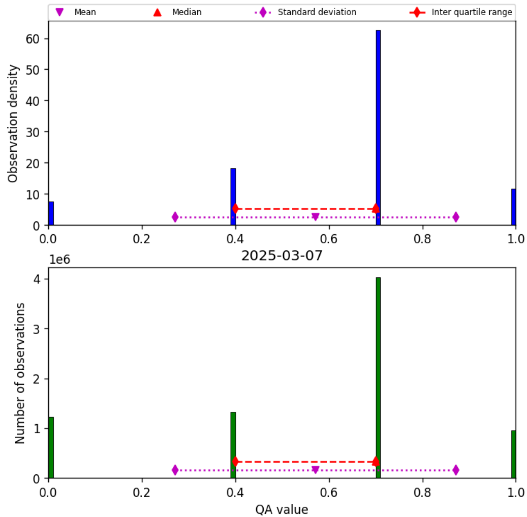
Figure 13: Histogram of “QA value” for 2025-03-07 to 2025-03-08
