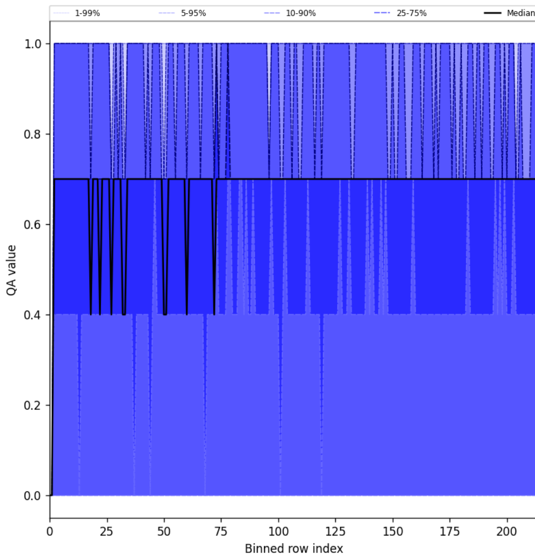
Figure 20: Along track statistics of “QA value” for 2025-03-07 to 2025-03-08
