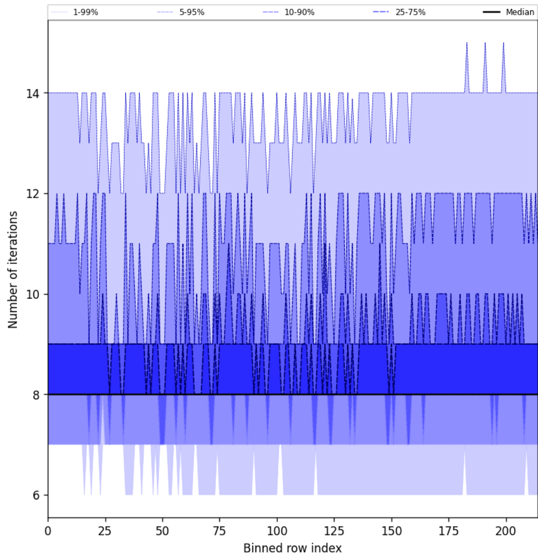
Figure 26: Along track statistics of “Number of iterations” for 2025-03-07 to 2025-03-08
