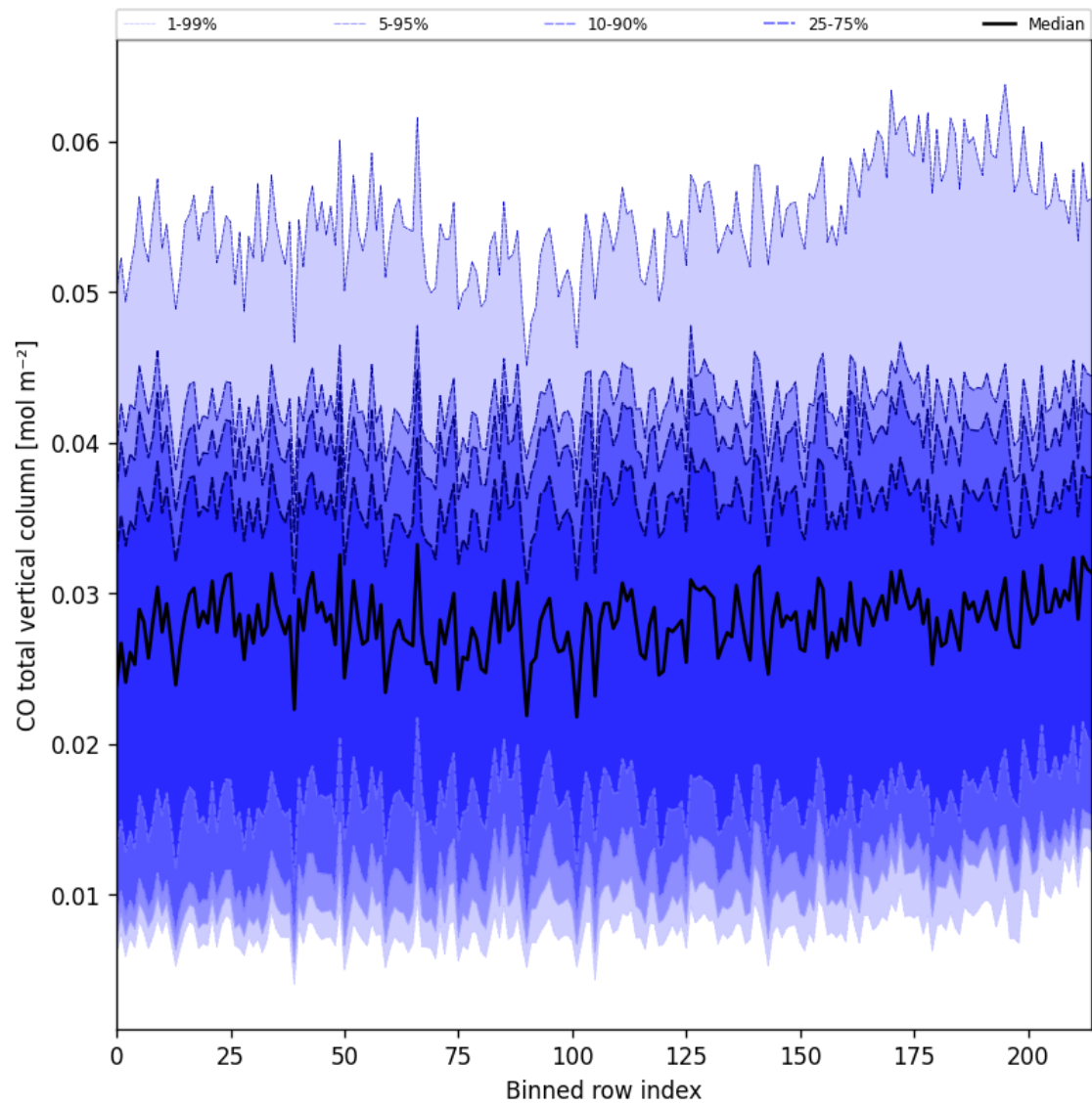
Figure 21: Along track statistics of “CO total vertical column” for 2025-03-07 to 2025-03-08
